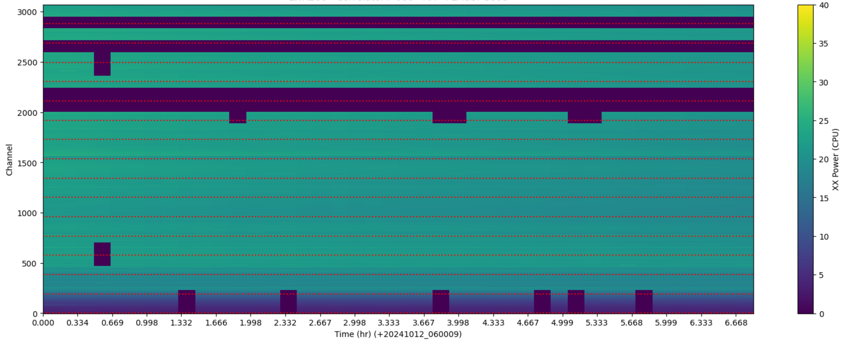
LWA266 - Correlator# 000 - XX - FLAGS: Good
