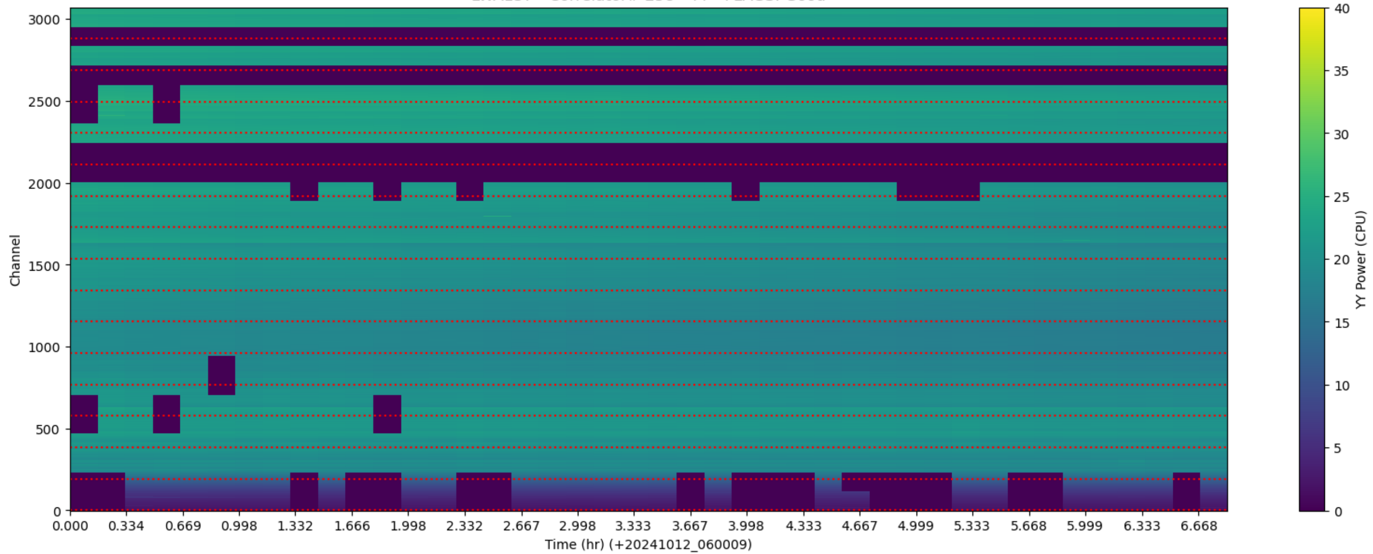
LWA137 - Correlator# 258 - YY - FLAGS: Good
