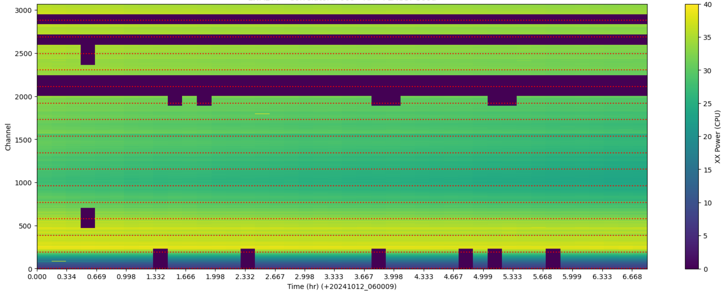
LWA277 - Correlator# 009 - XX - FLAGS: Good
