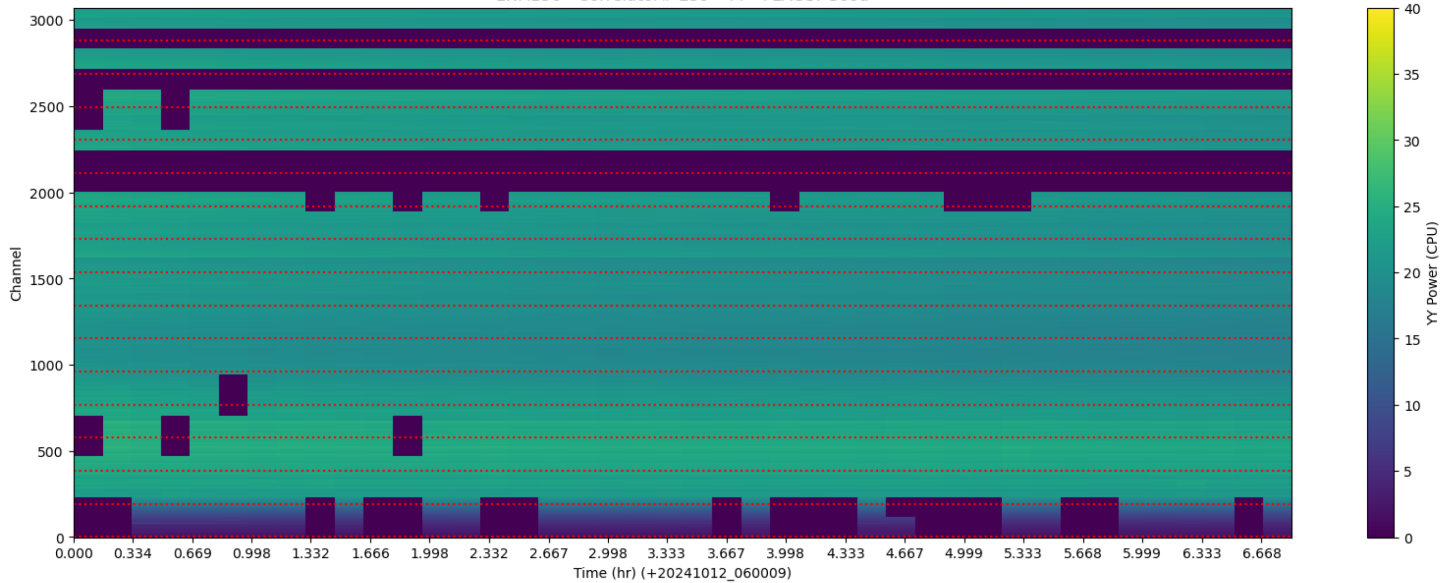
LWA136 - Correlator# 259 - YY - FLAGS: Good
