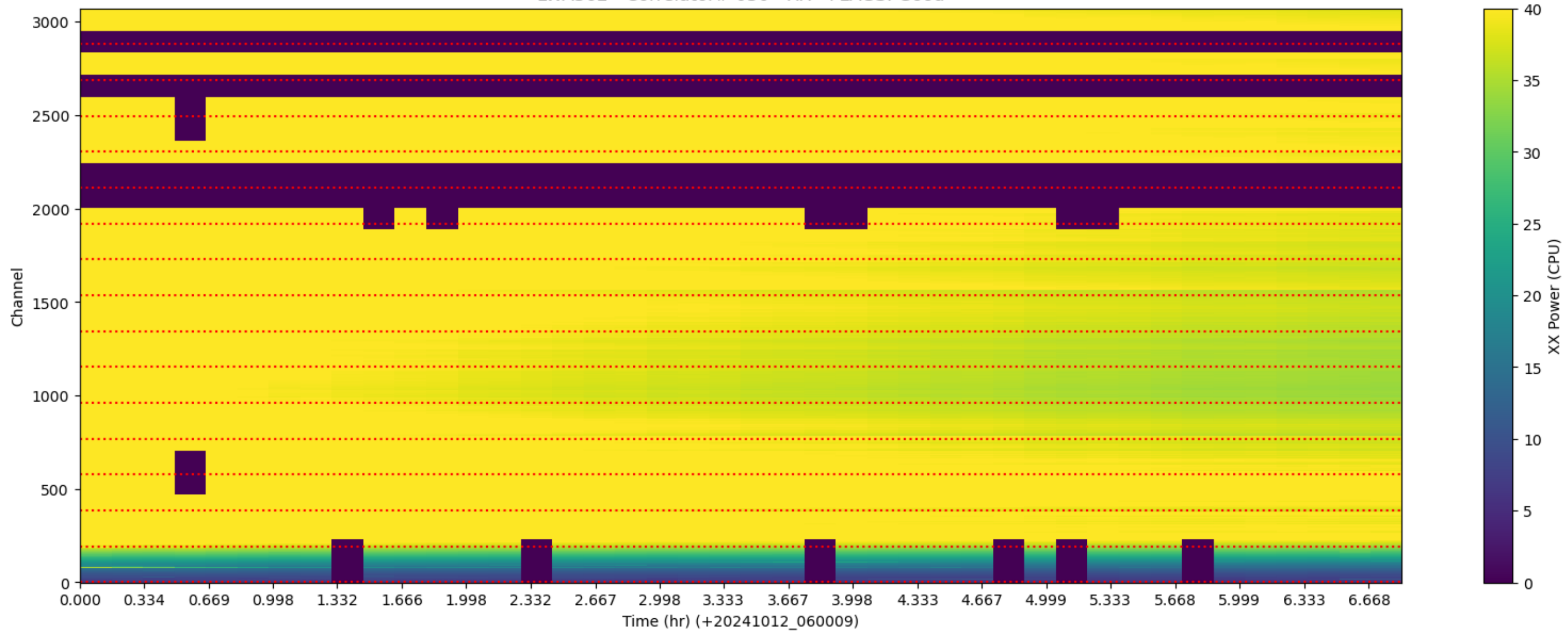
LWA362 - Correlator# 030 - XX - FLAGS: Good
