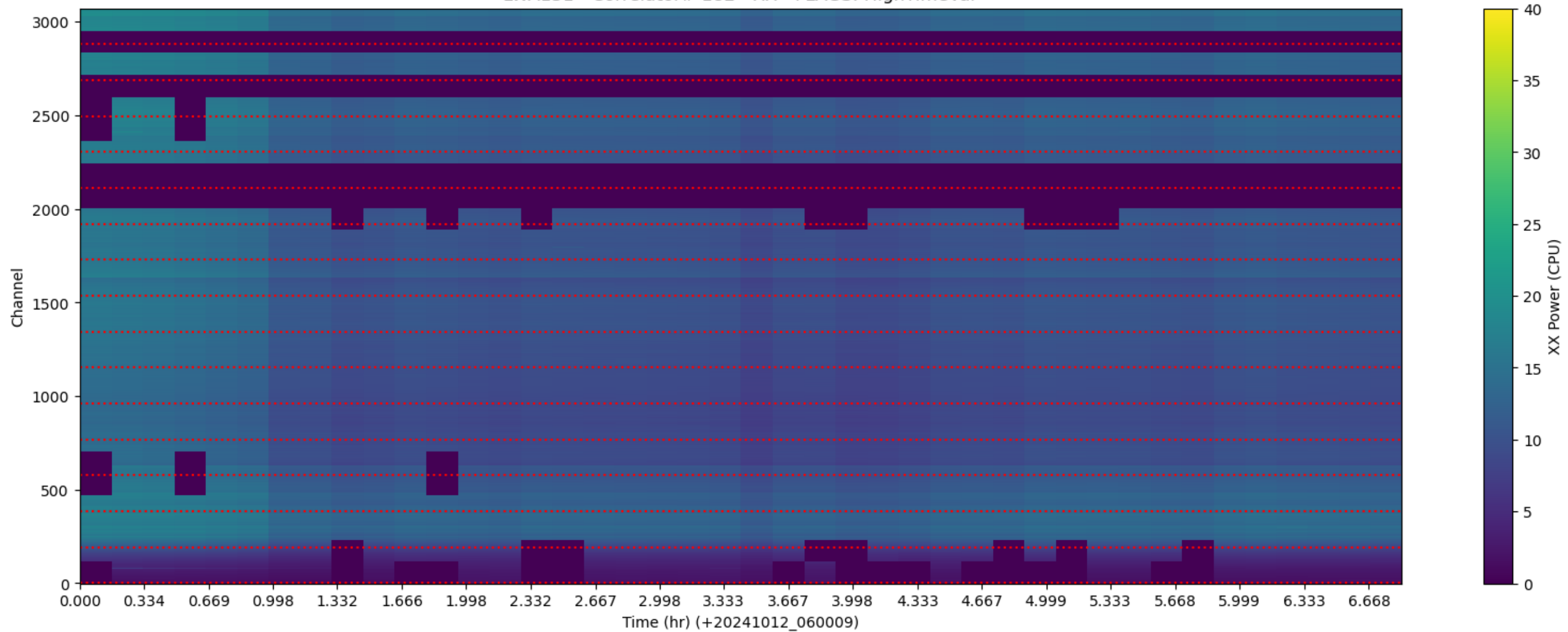
LWA131 - Correlator# 182 - XX - FLAGS: HighTimeVar
