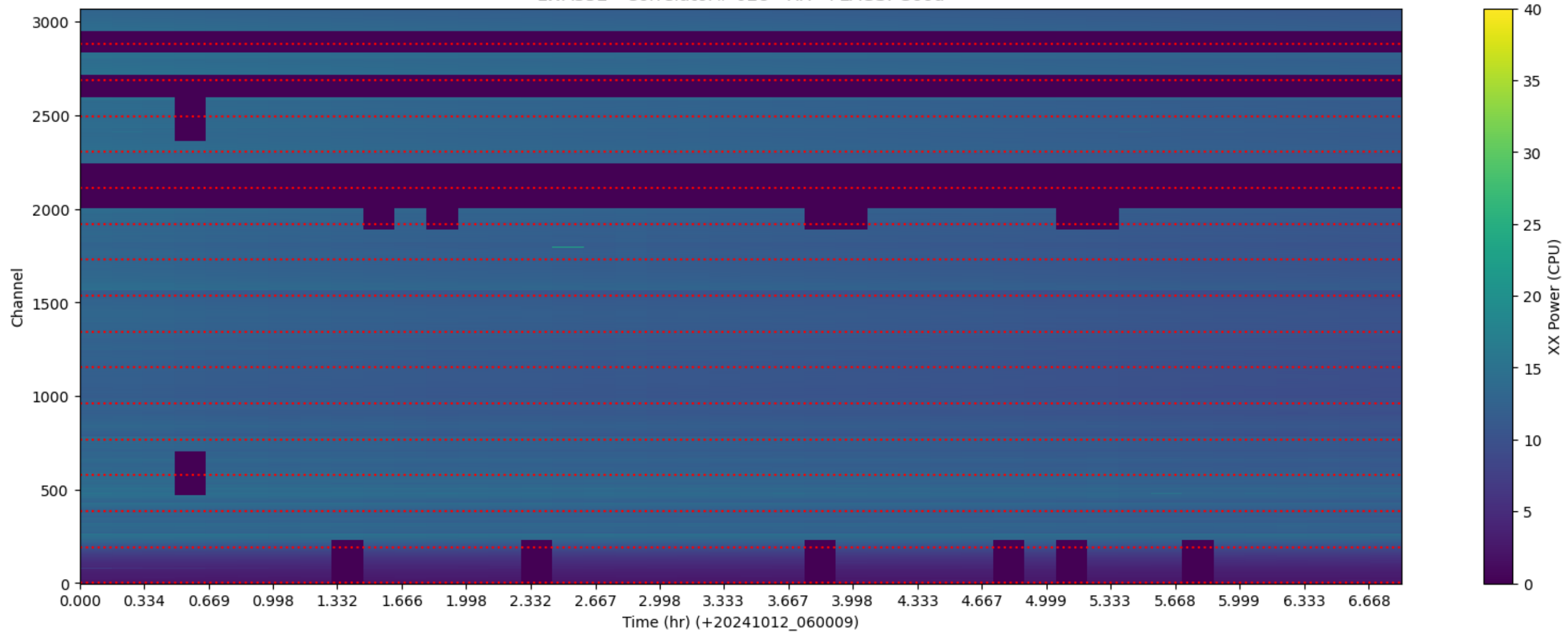
LWA352 - Correlator# 028 - XX - FLAGS: Good
