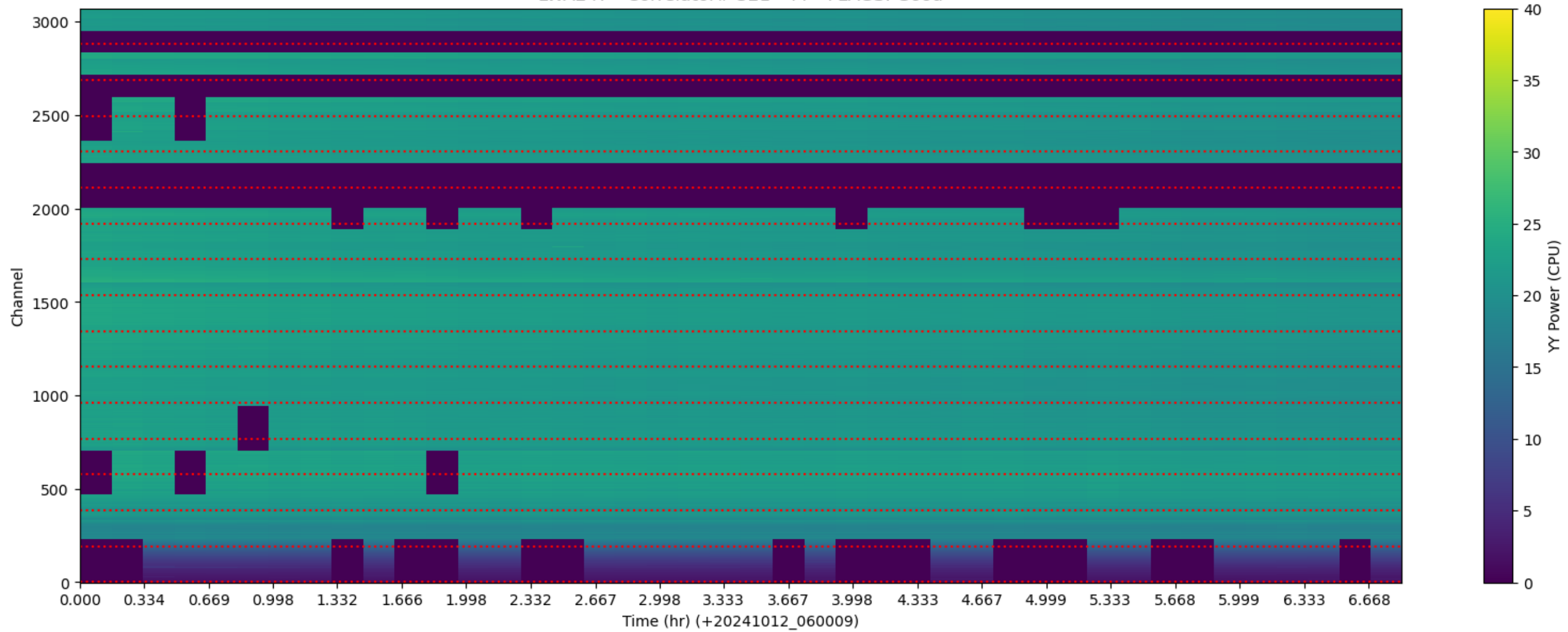
LWA247 - Correlator# 321 - YY - FLAGS: Good
