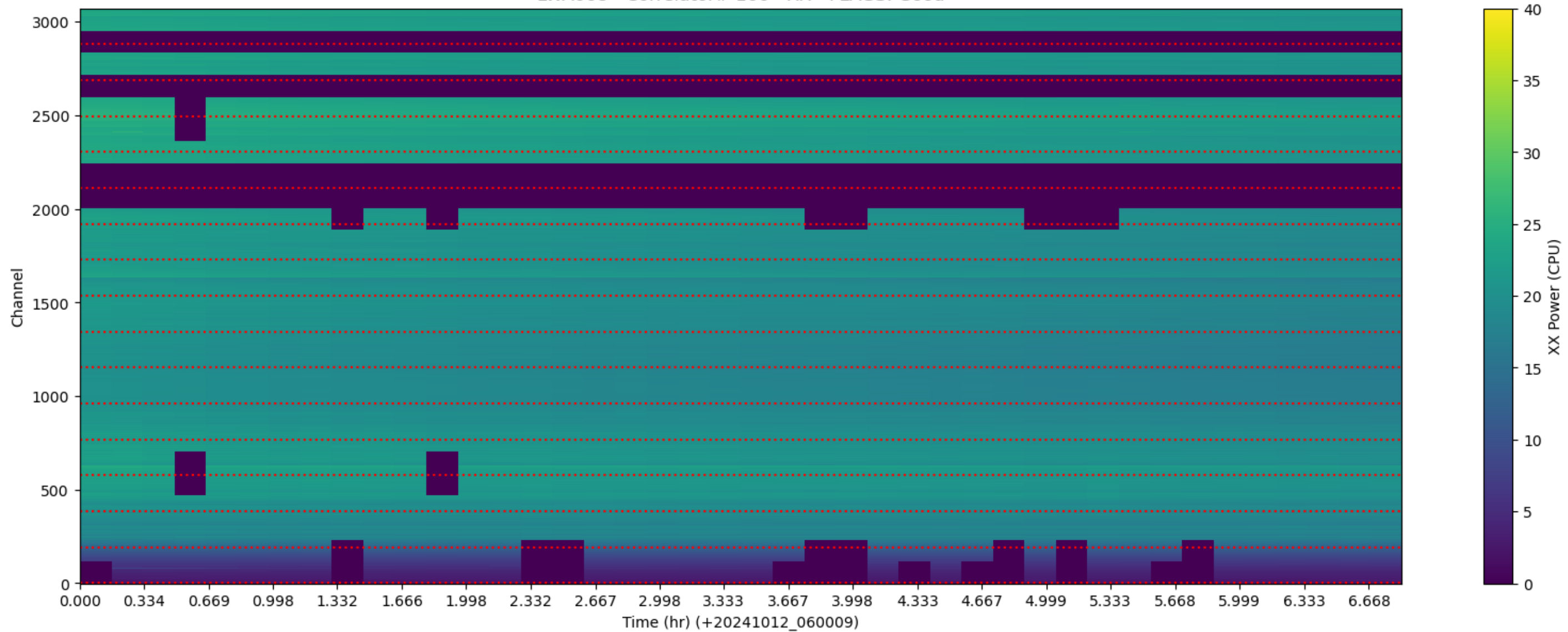
LWA068 - Correlator# 166 - XX - FLAGS: Good
