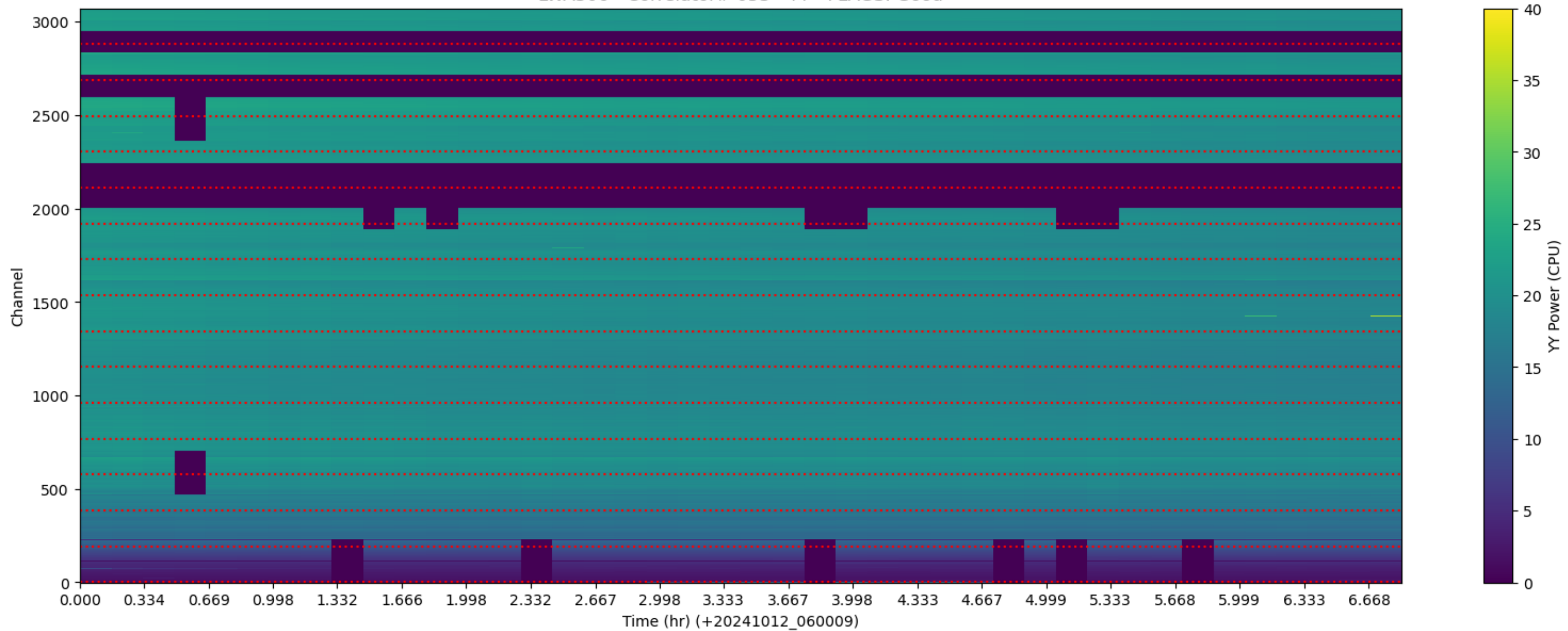
LWA306 - Correlator# 053 - YY - FLAGS: Good
