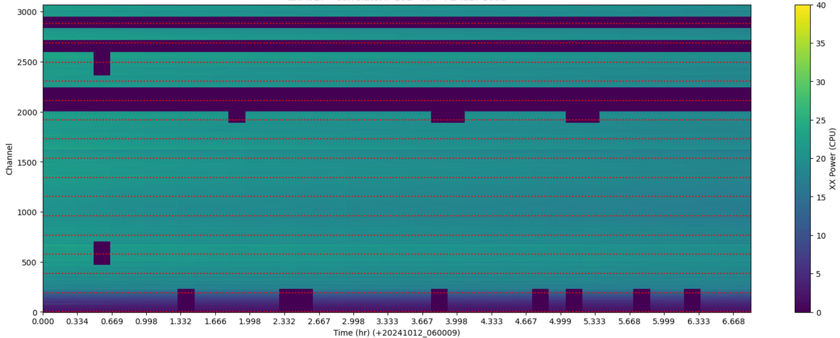
LWA017 - Correlator# 101 - XX - FLAGS: Good
