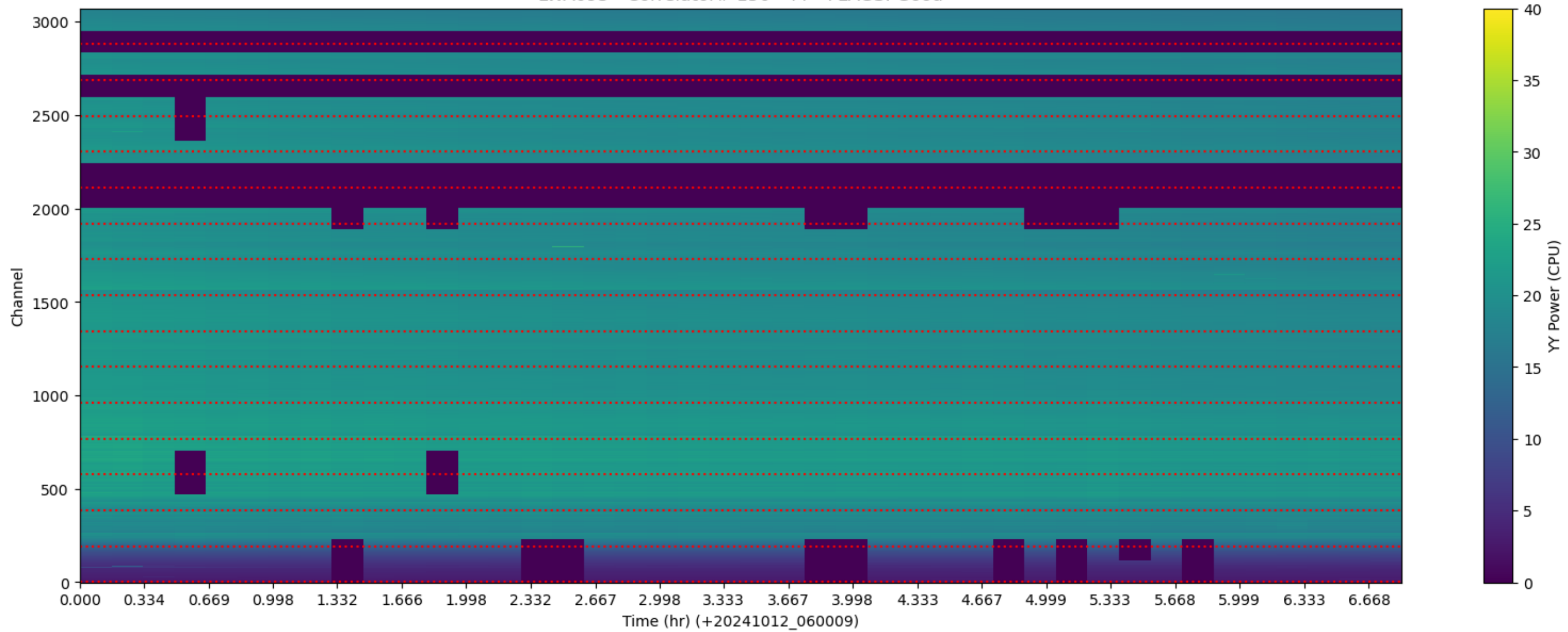
LWA095 - Correlator# 150 - YY - FLAGS: Good
