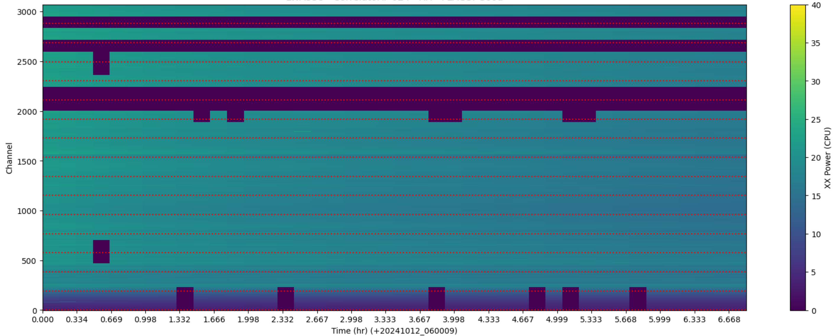
LWA338 - Correlator# 024 - XX - FLAGS: Good
