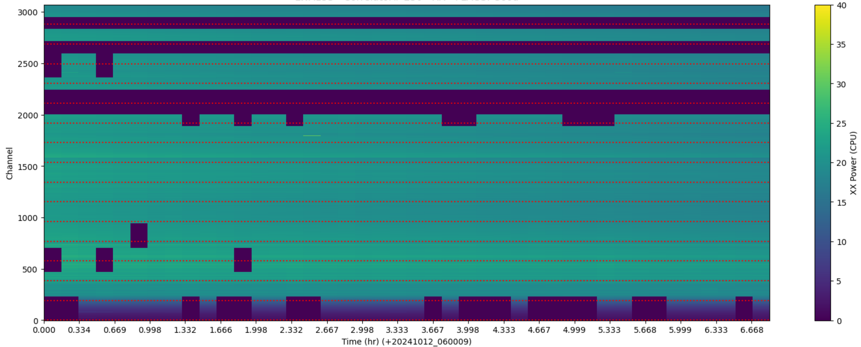
LWA153 - Correlator# 230 - XX - FLAGS: Good
