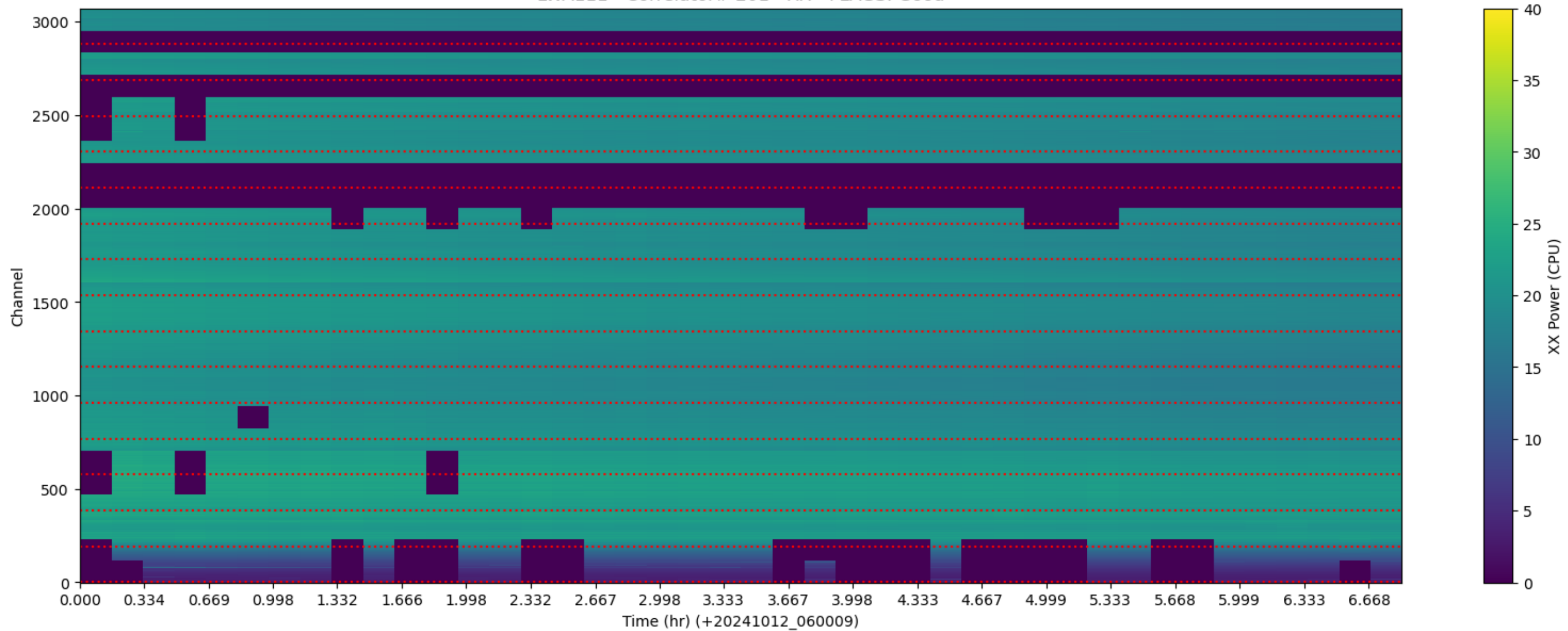
LWA111 - Correlator# 201 - XX - FLAGS: Good
