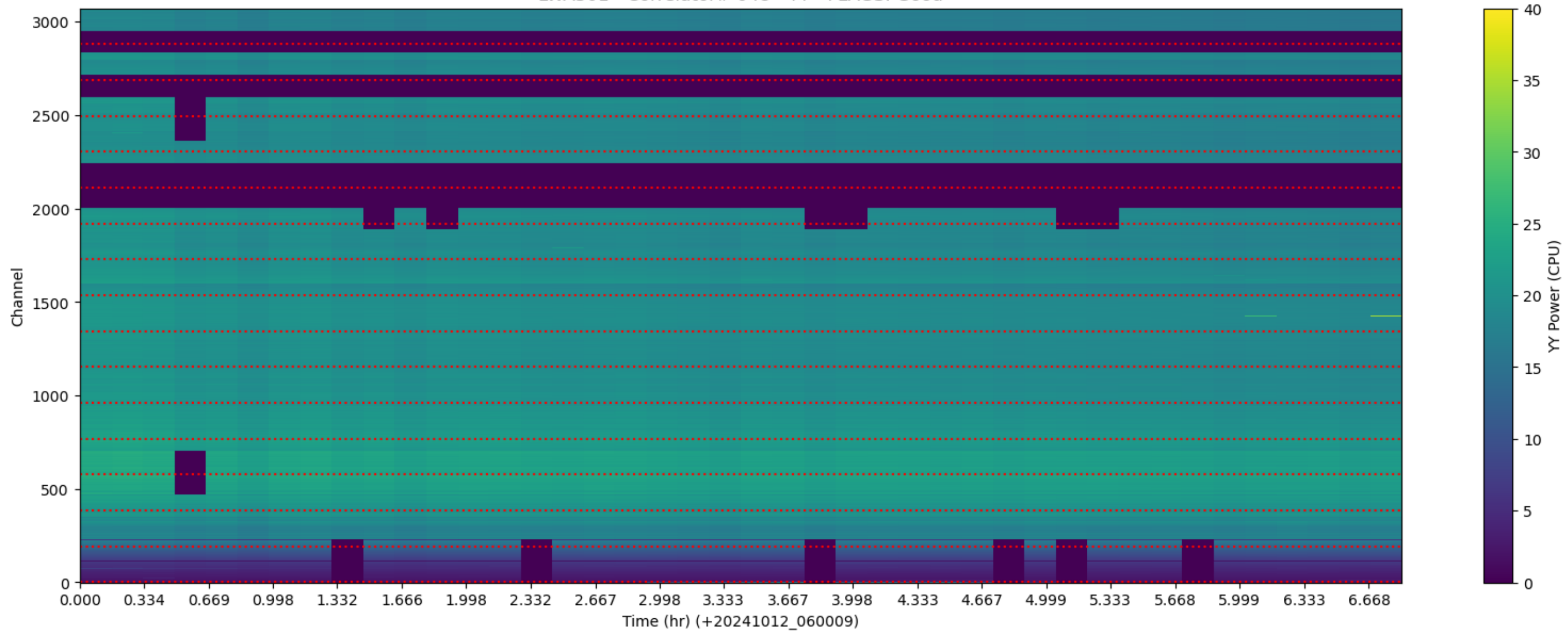
LWA301 - Correlator# 048 - YY - FLAGS: Good
