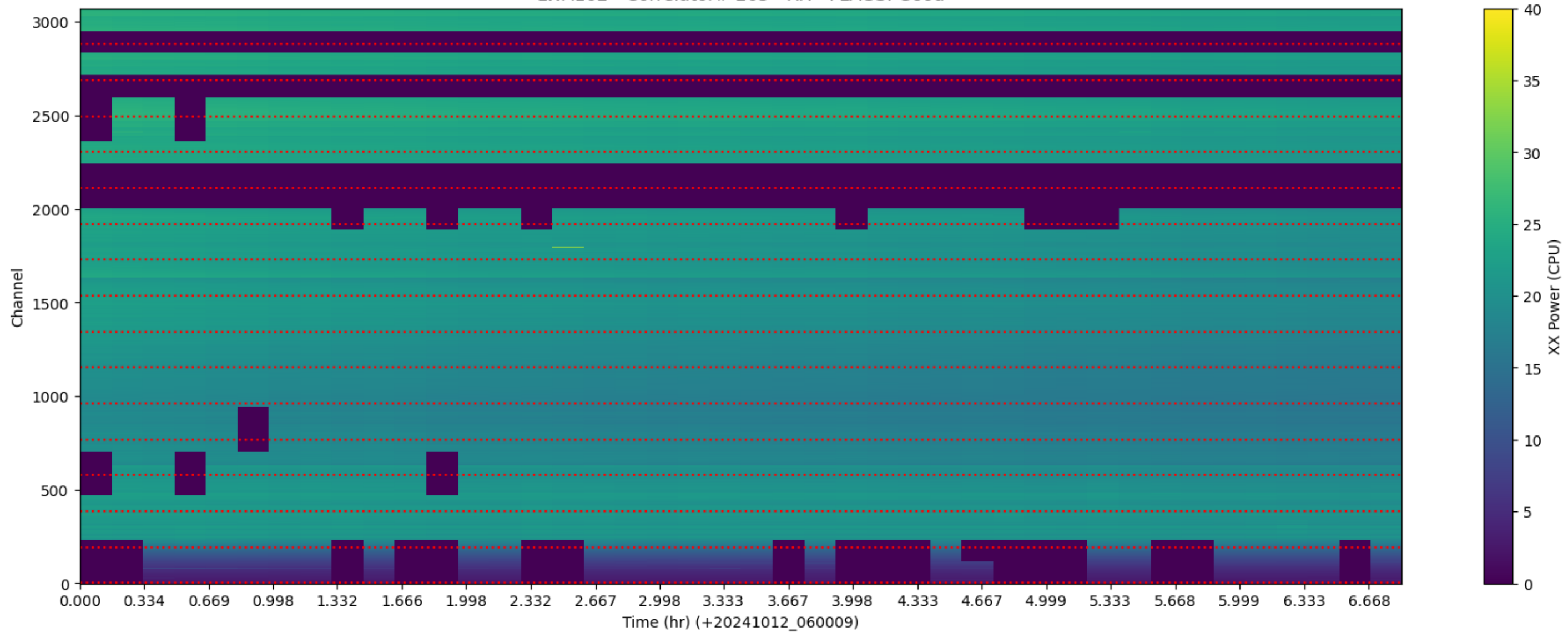
LWA162 - Correlator# 265 - XX - FLAGS: Good
