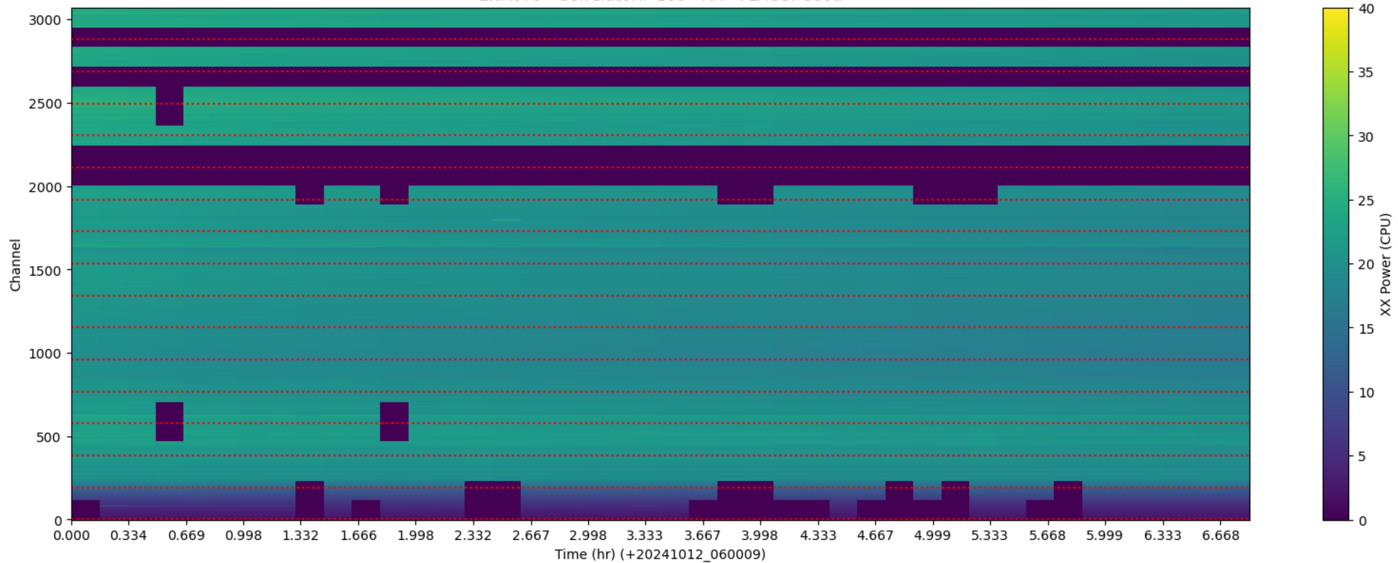
LWA070 - Correlator# 168 - XX - FLAGS: Good
