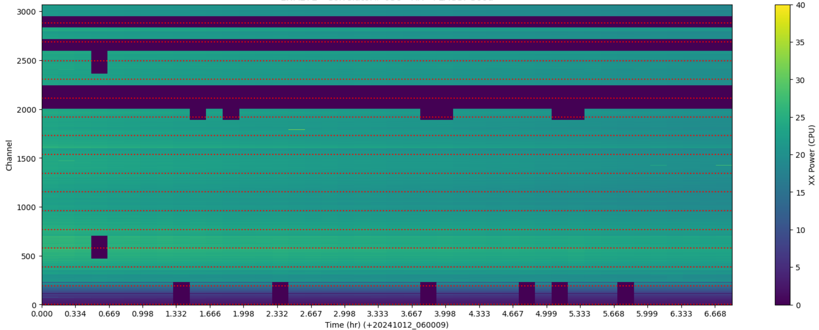
LWA272 - Correlator# 038 - XX - FLAGS: Good
