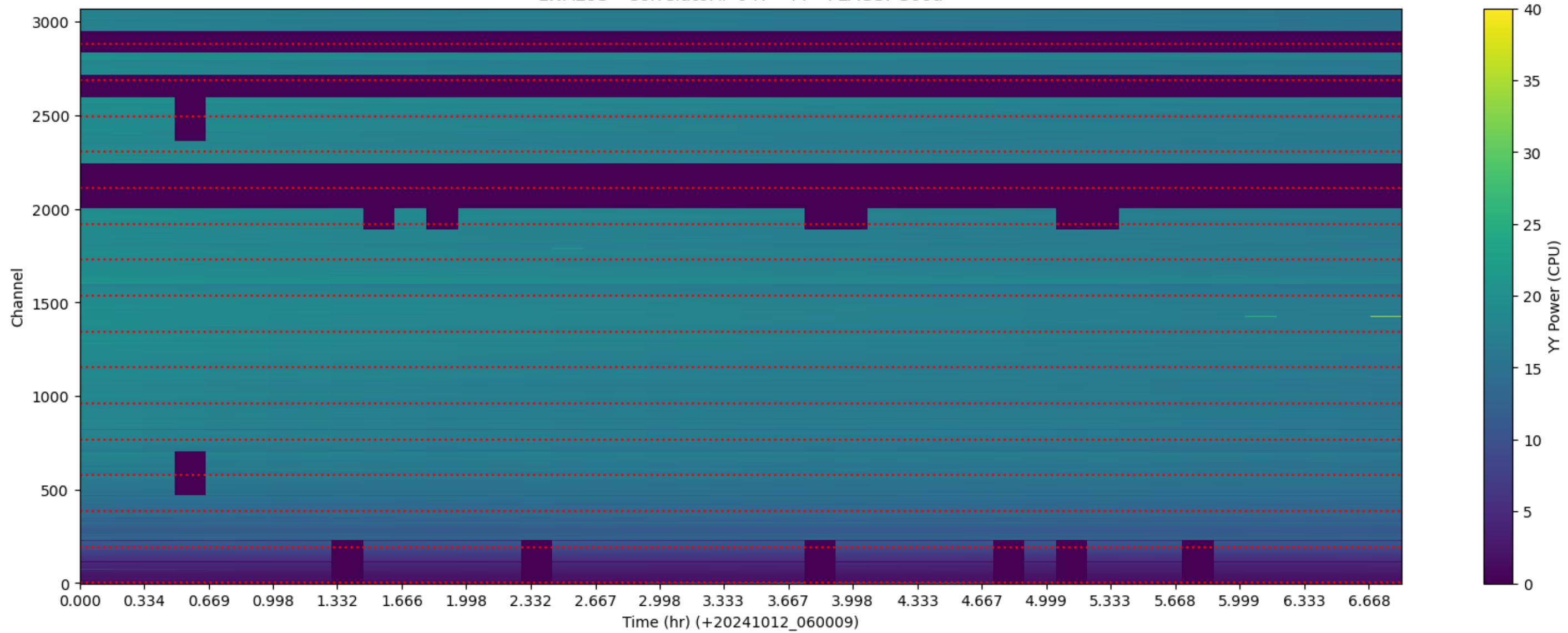
LWA295 - Correlator# 047 - YY - FLAGS: Good
