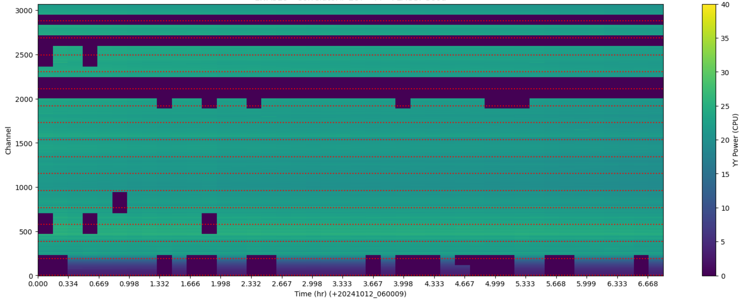
LWA329 - Correlator# 287 - YY - FLAGS: Good
