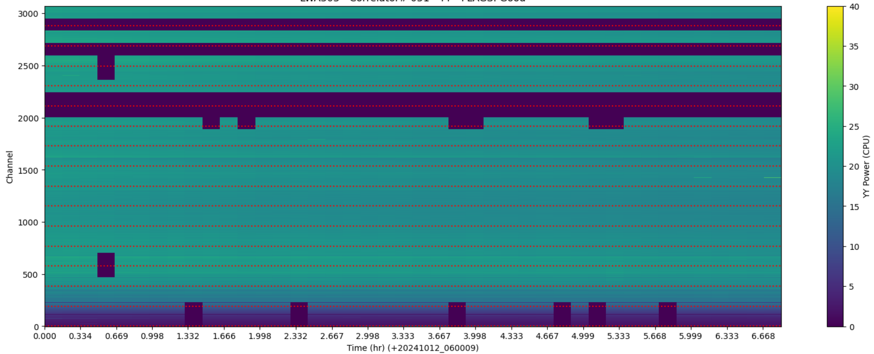
LWA303 - Correlator# 051 - YY - FLAGS: Good
