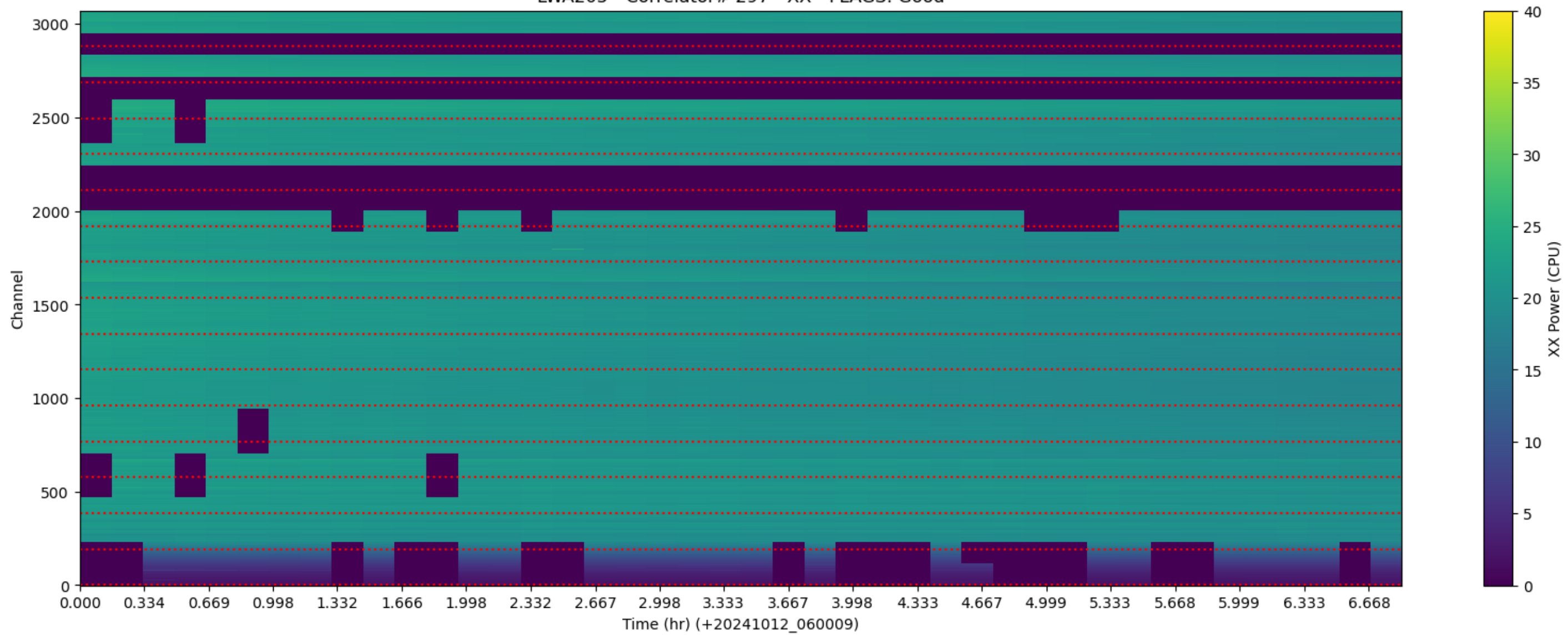
LWA205 - Correlator# 297 - XX - FLAGS: Good
