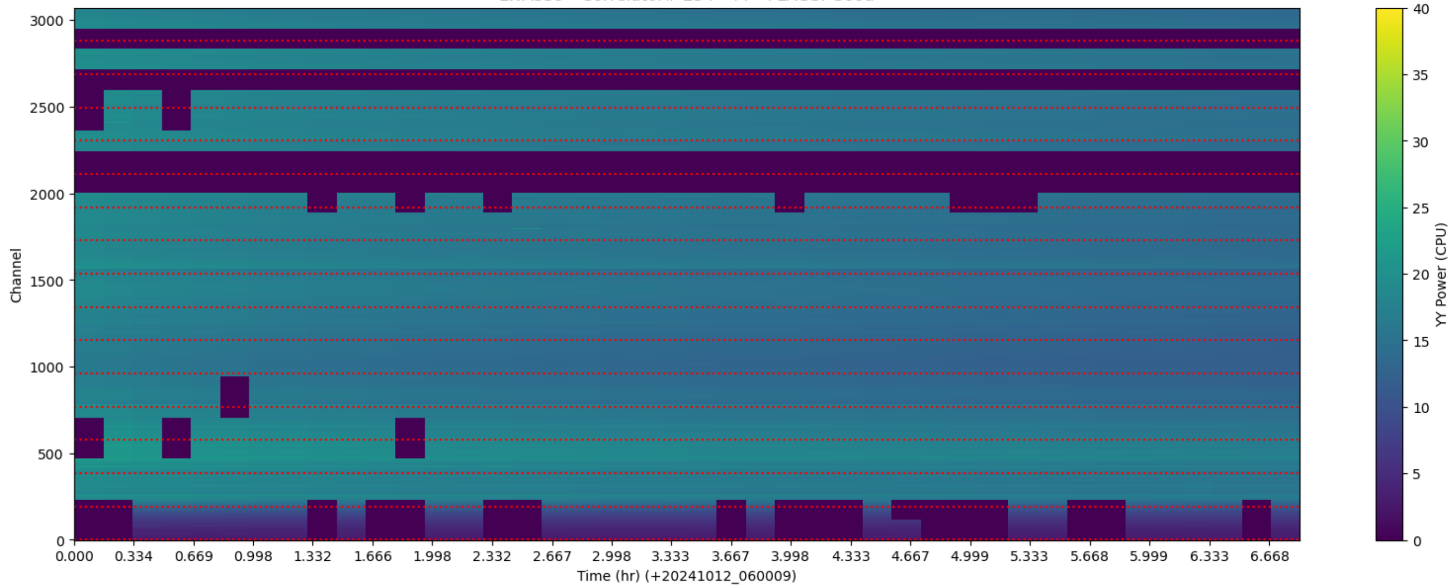
LWA359 - Correlator# 254 - YY - FLAGS: Good
