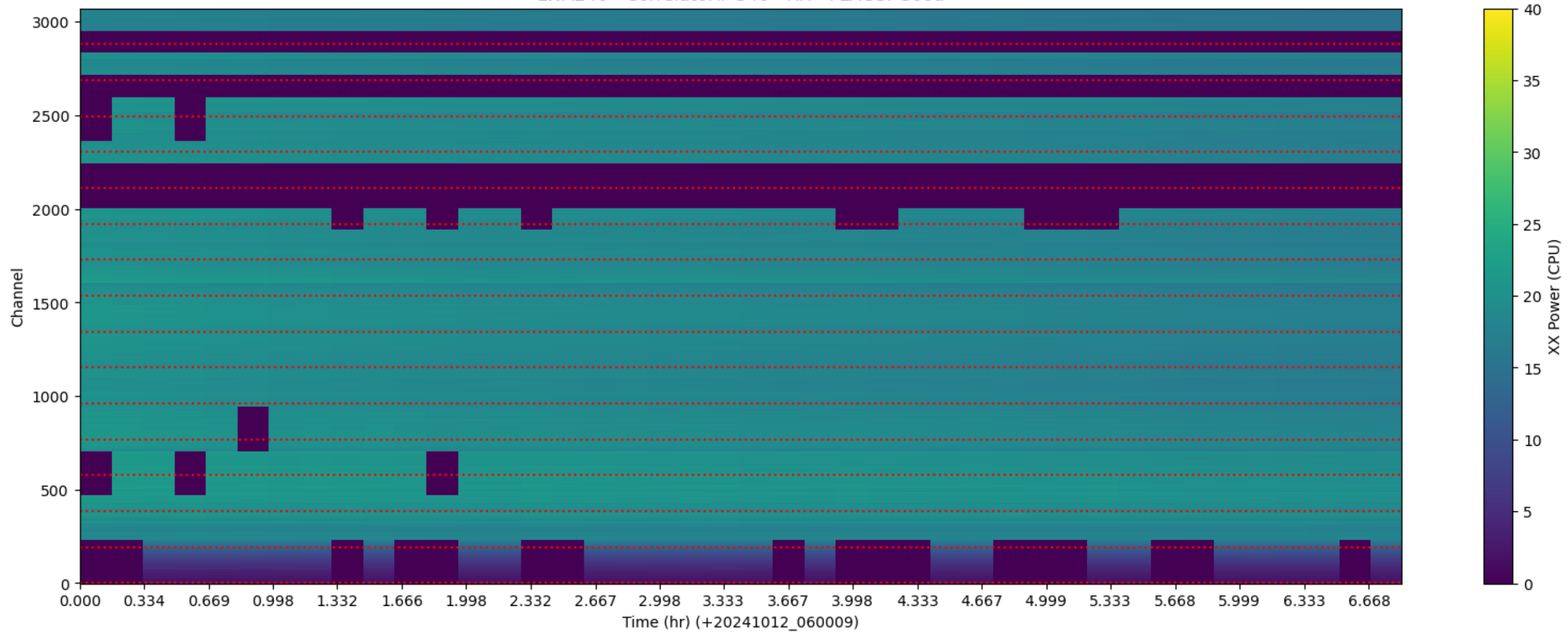
LWA246 - Correlator# 340 - XX - FLAGS: Good
