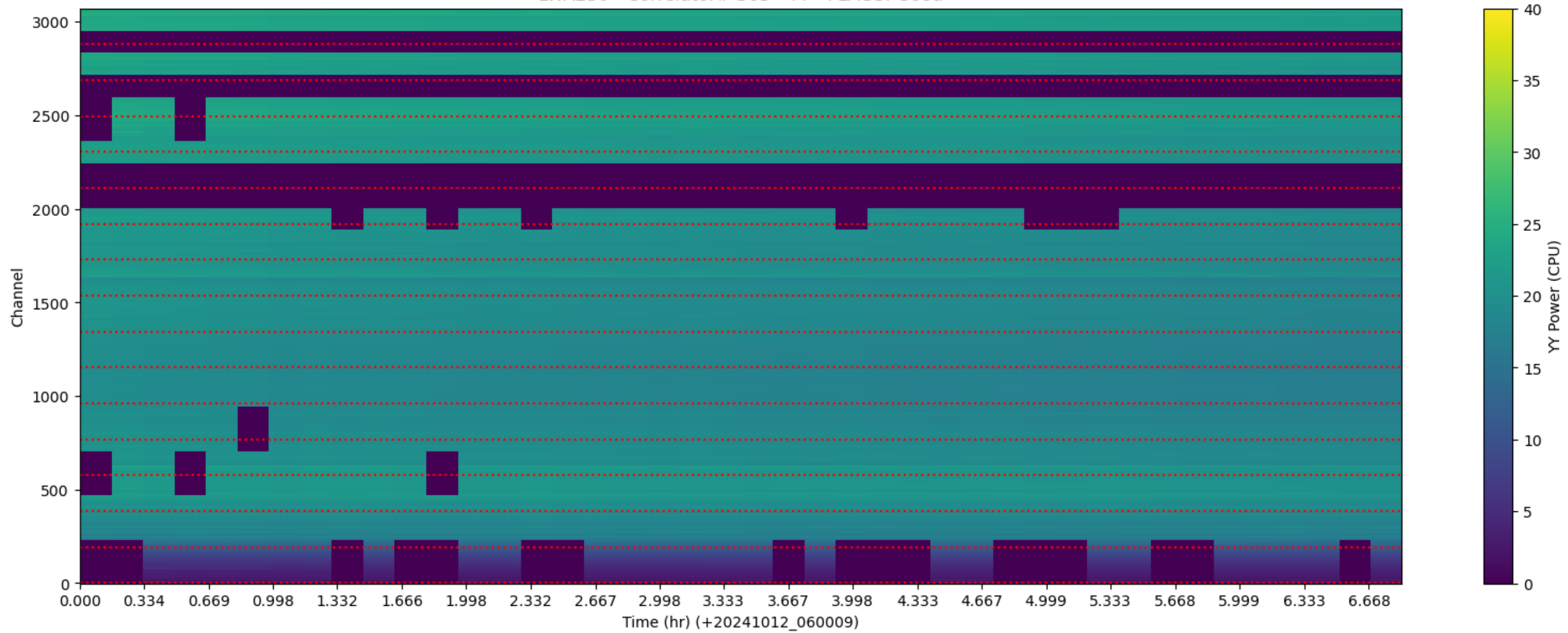
LWA230 - Correlator# 303 - YY - FLAGS: Good
