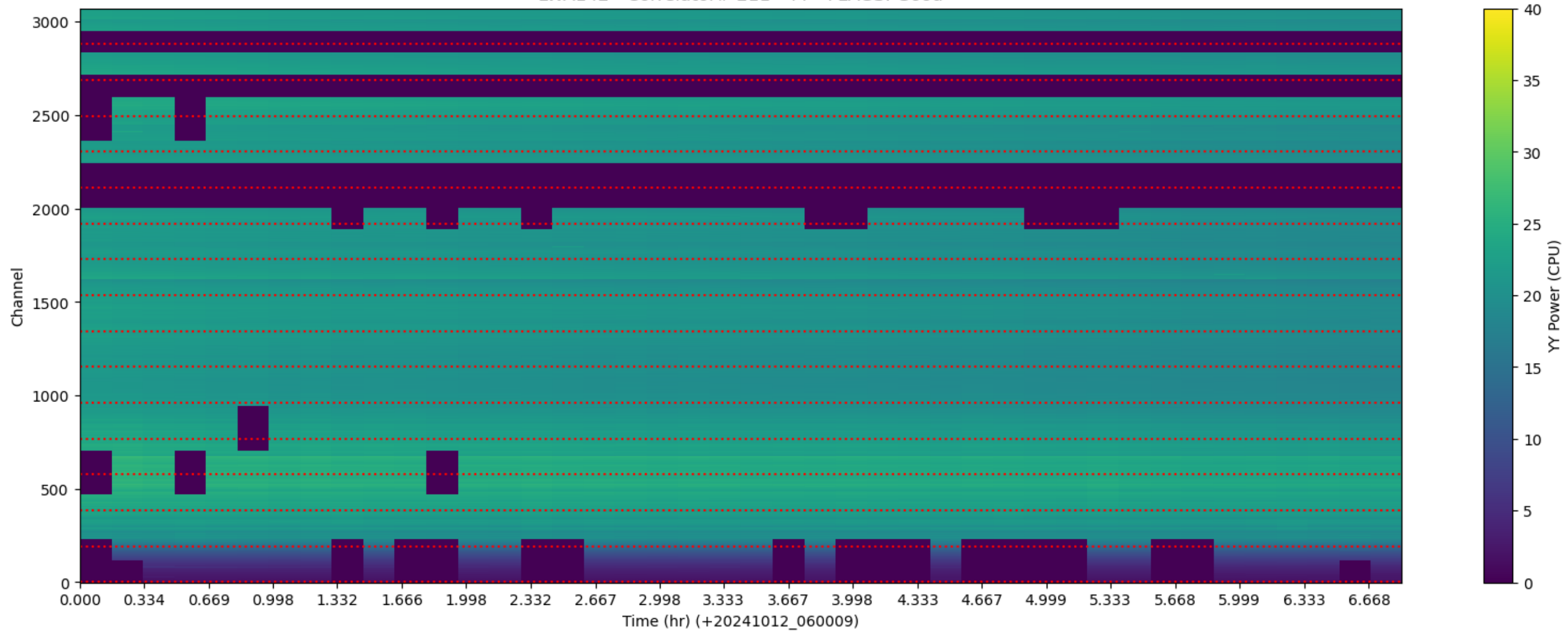
LWA142 - Correlator# 211 - YY - FLAGS: Good
