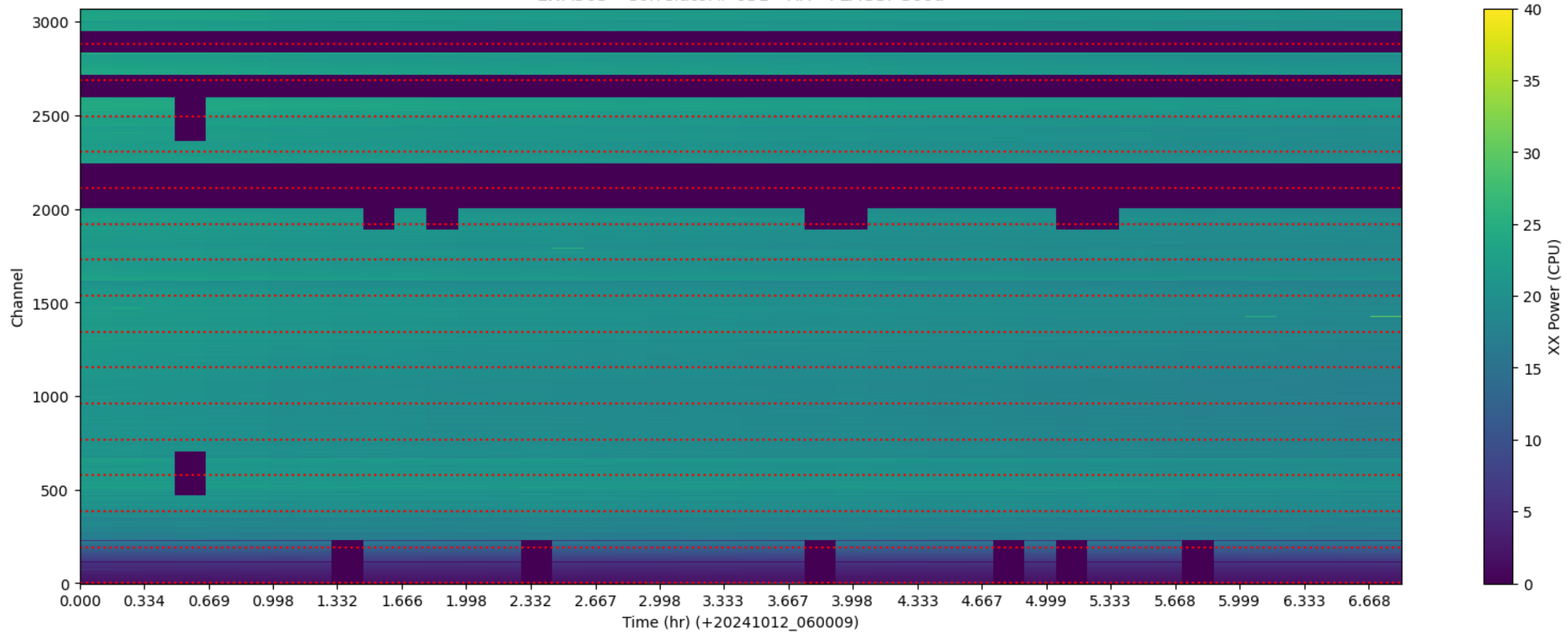
LWA303 - Correlator# 051 - XX - FLAGS: Good
