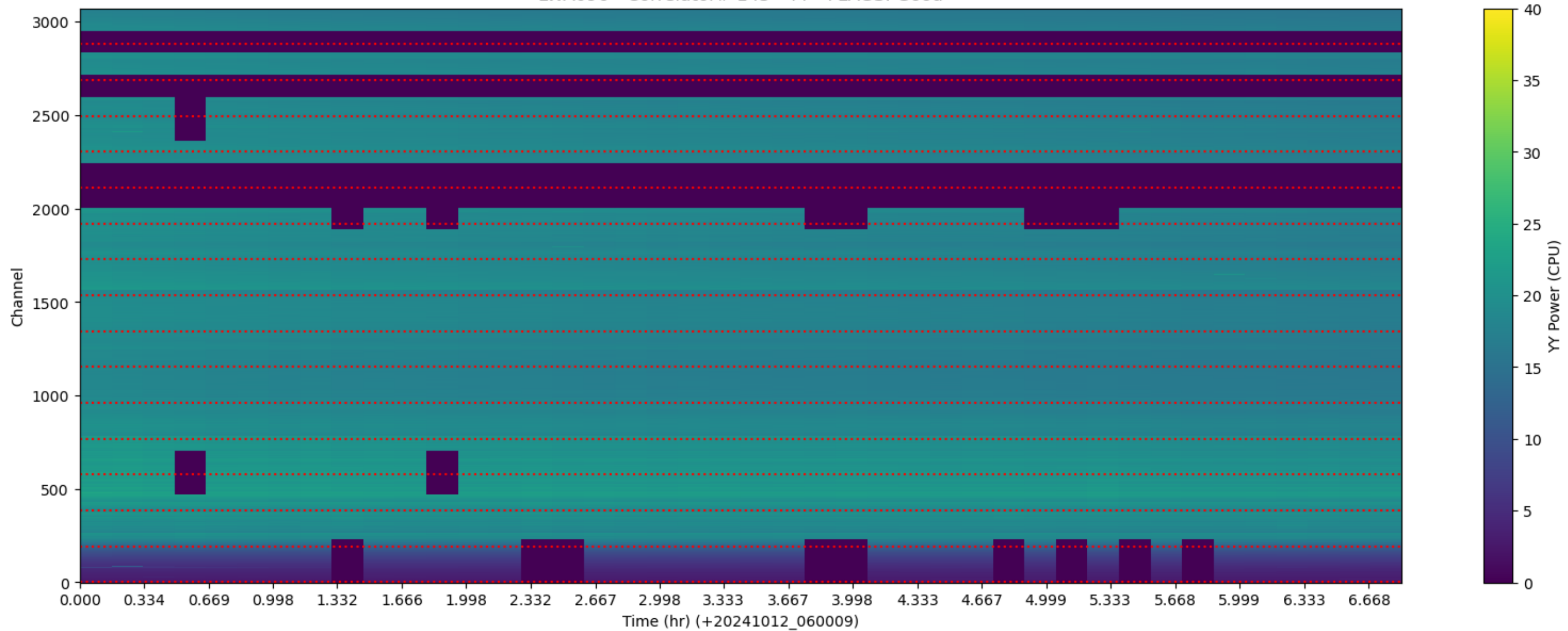
LWA096 - Correlator# 145 - YY - FLAGS: Good
