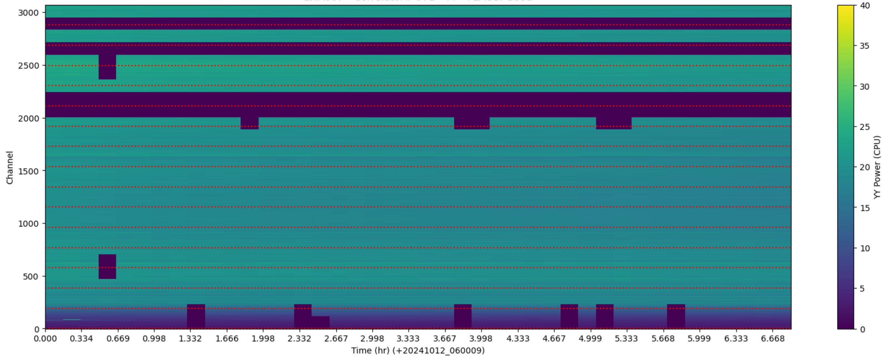
LWA007 - Correlator# 071 - YY - FLAGS: Good
