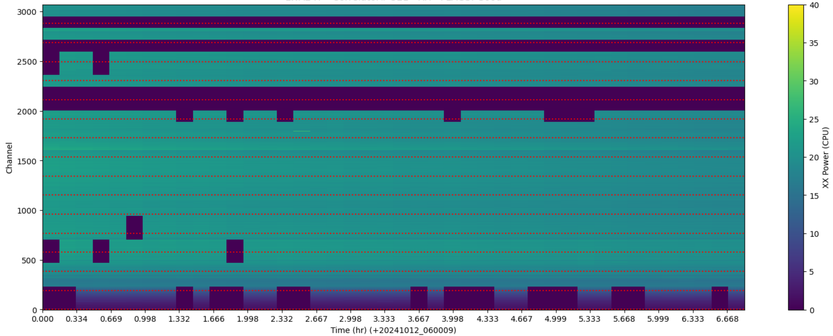
LWA247 - Correlator# 321 - XX - FLAGS: Good
