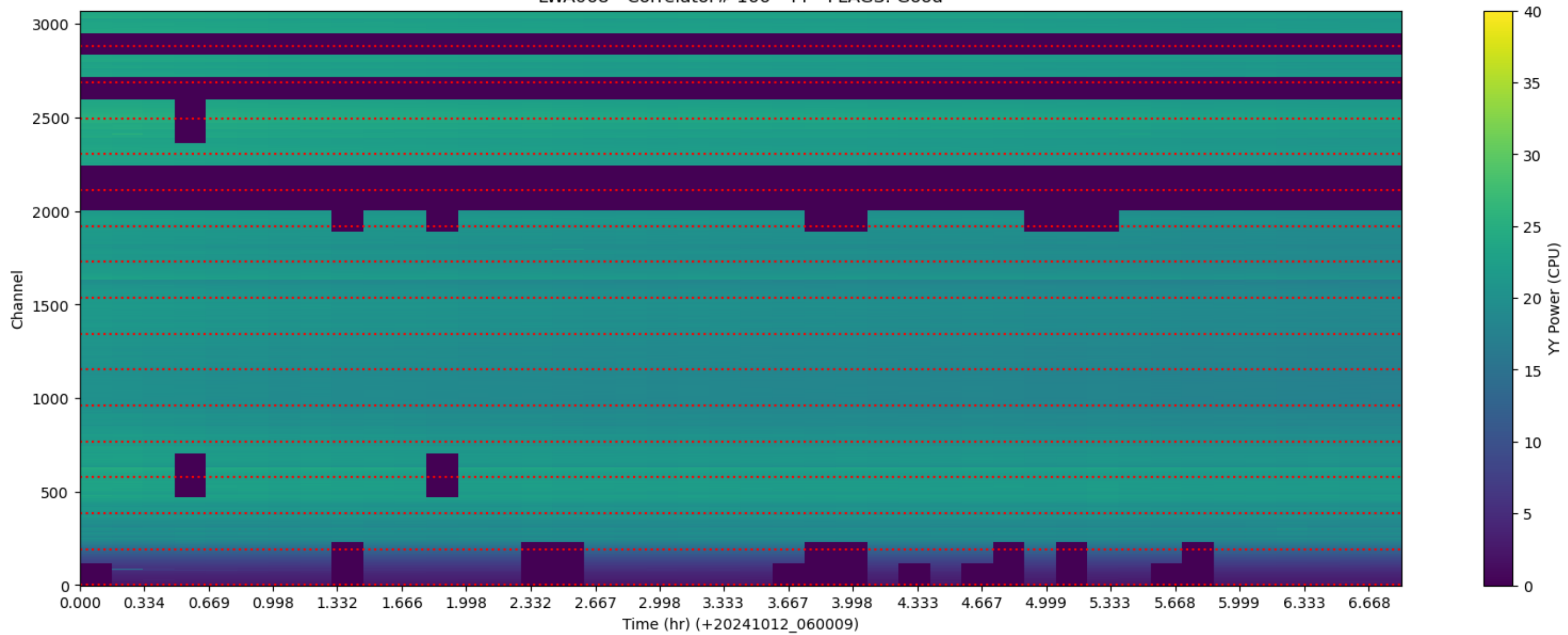
LWA068 - Correlator# 166 - YY - FLAGS: Good
