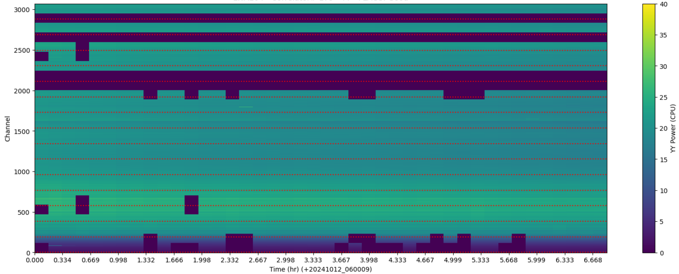
LWA104 - Correlator# 179 - YY - FLAGS: Good
