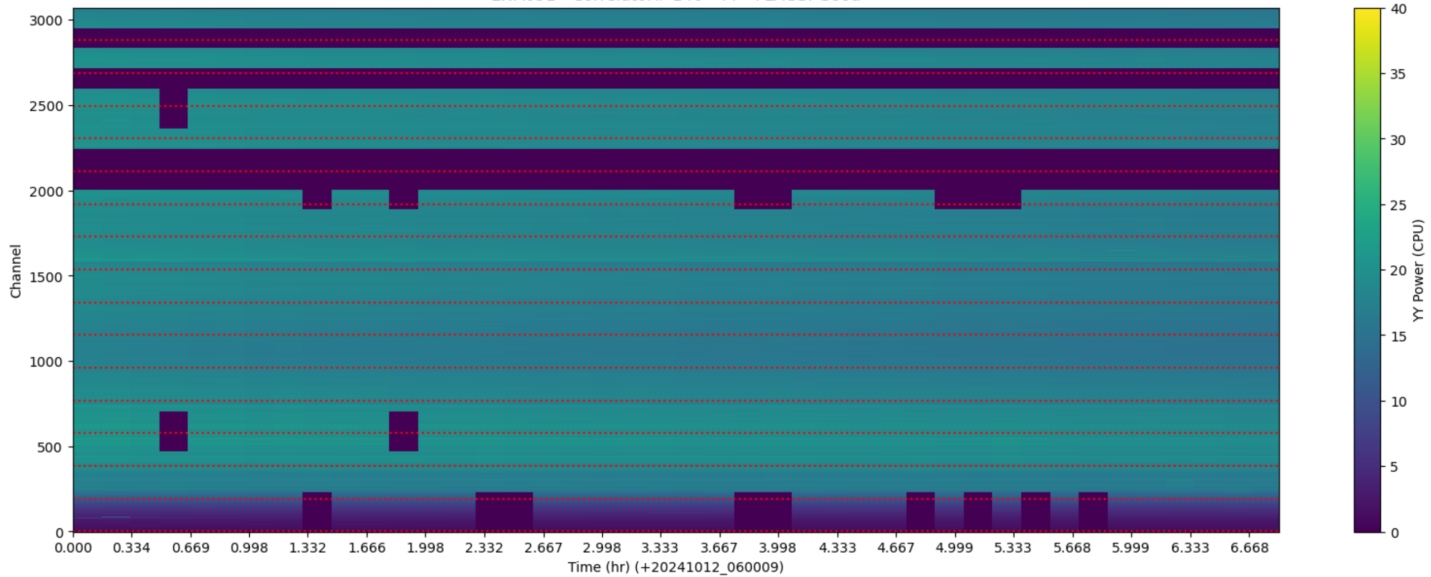
LWA091 - Correlator# 146 - YY - FLAGS: Good
