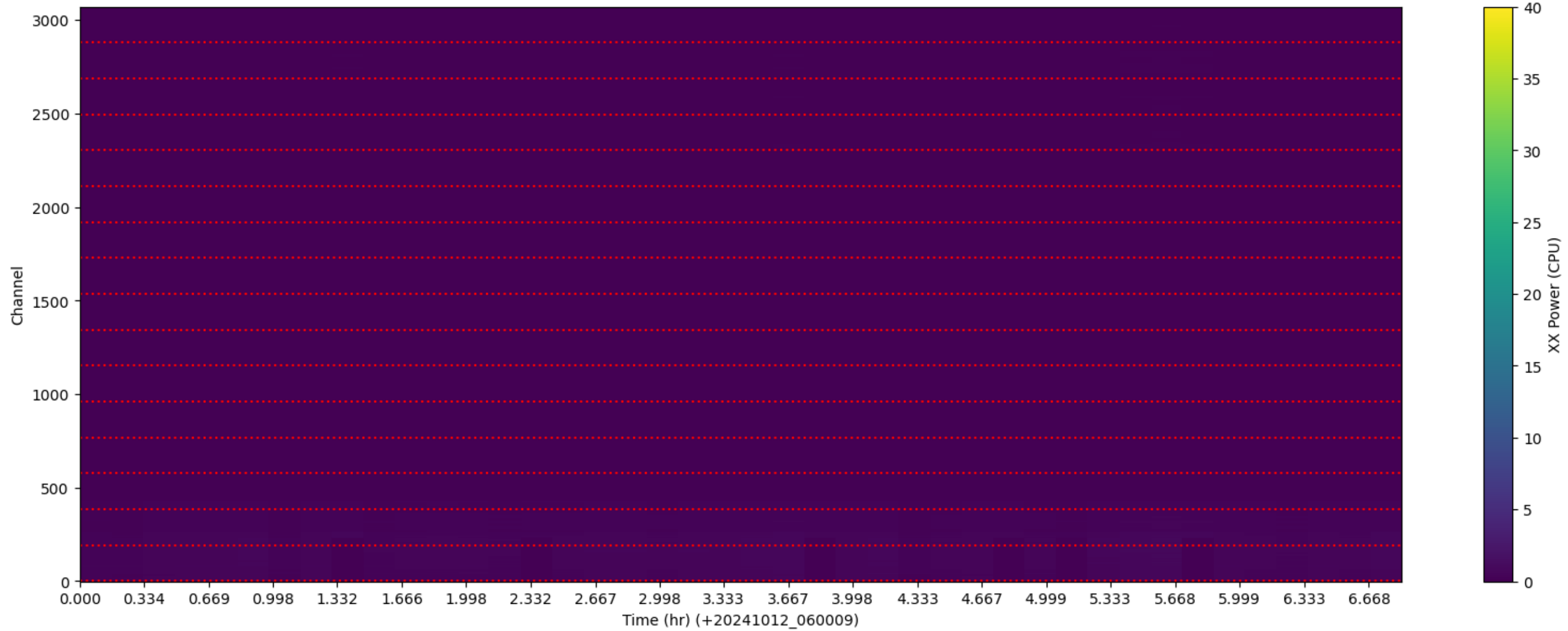
LWA339 - Correlator# 027 - XX - FLAGS: LowPower
