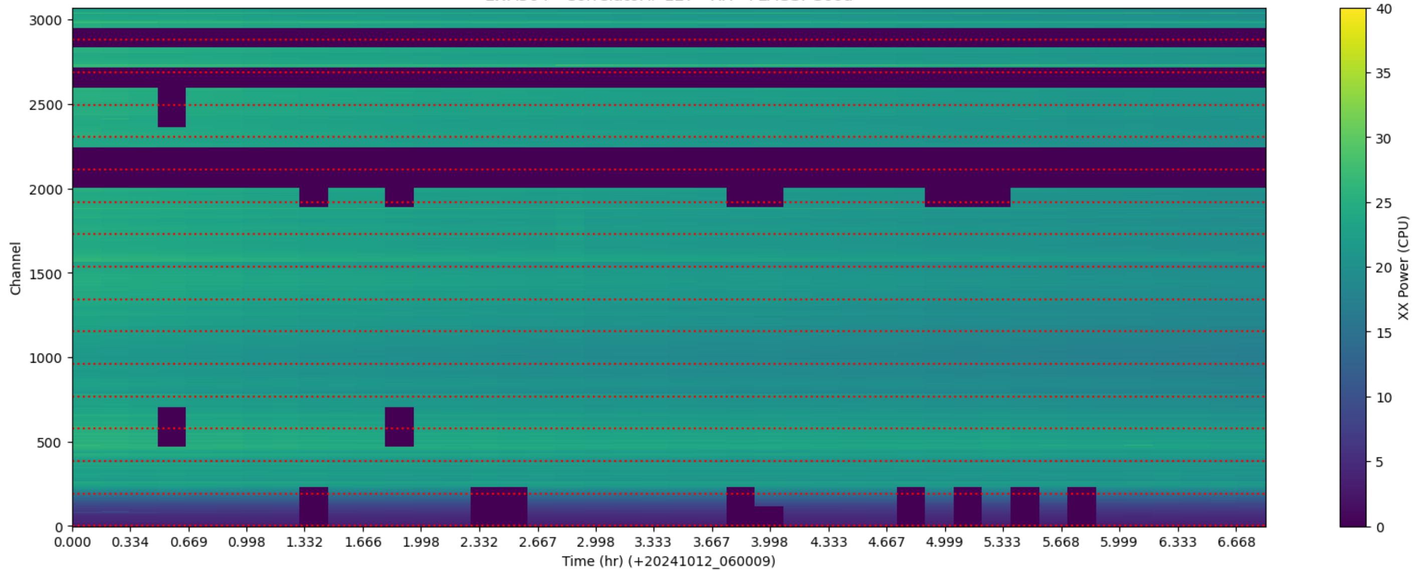
LWA364 - Correlator# 127 - XX - FLAGS: Good
