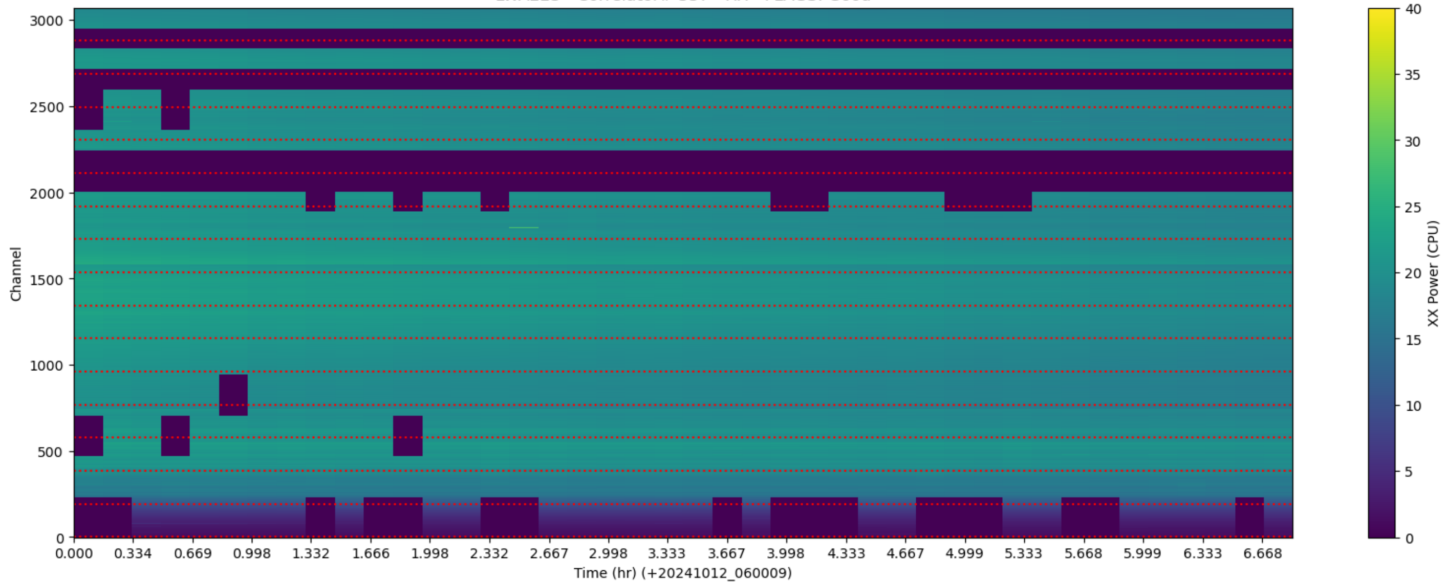
LWA223 - Correlator# 337 - XX - FLAGS: Good
