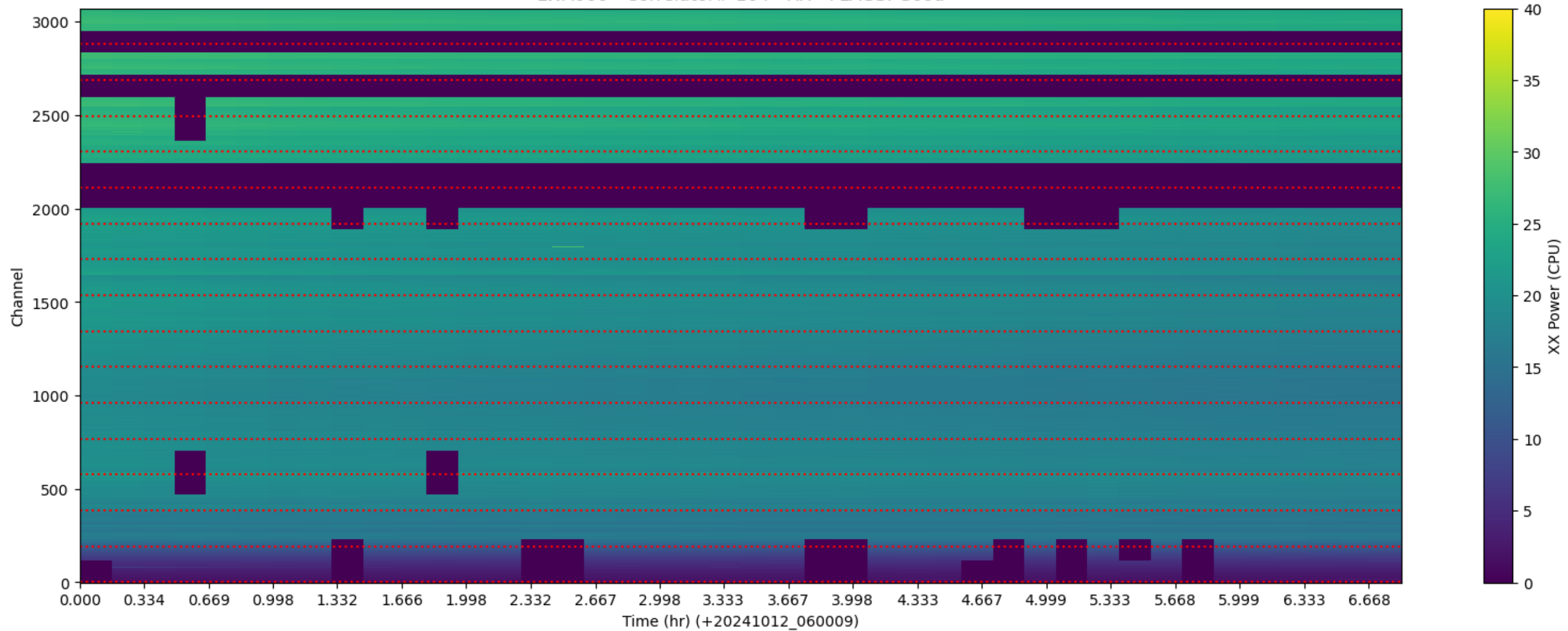
LWA066 - Correlator# 164 - XX - FLAGS: Good
