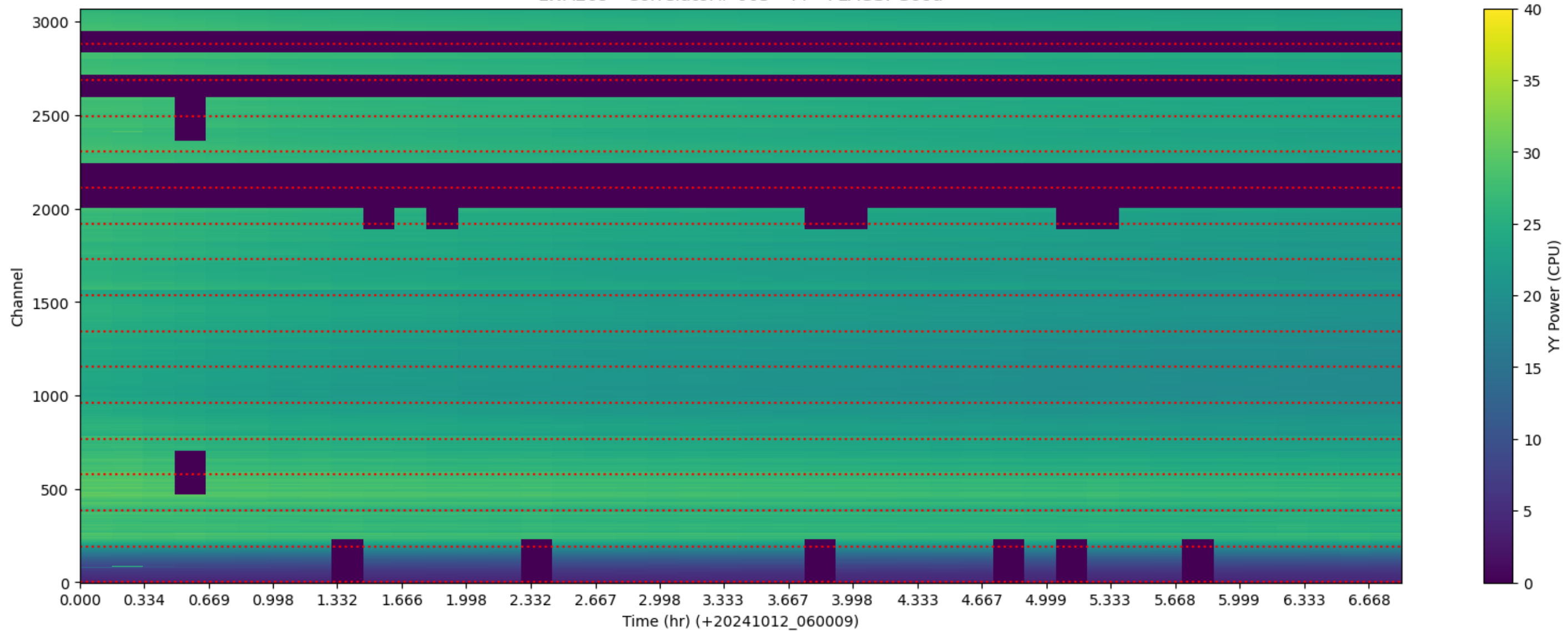
LWA269 - Correlator# 005 - YY - FLAGS: Good
