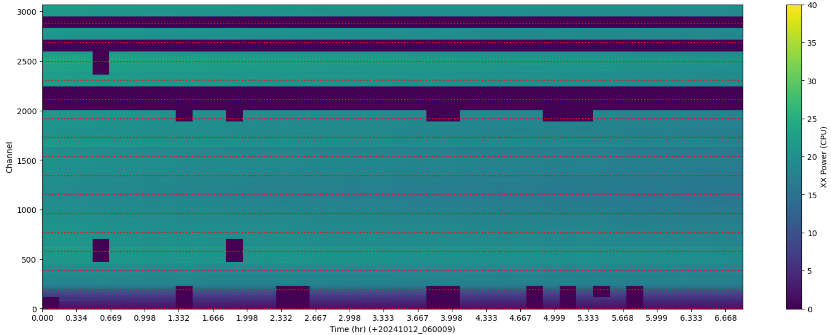
LWA036 - Correlator# 163 - XX - FLAGS: Good
