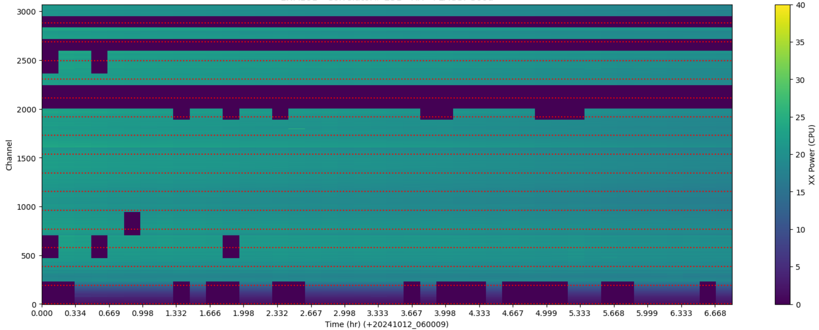
LWA181 - Correlator# 231 - XX - FLAGS: Good
