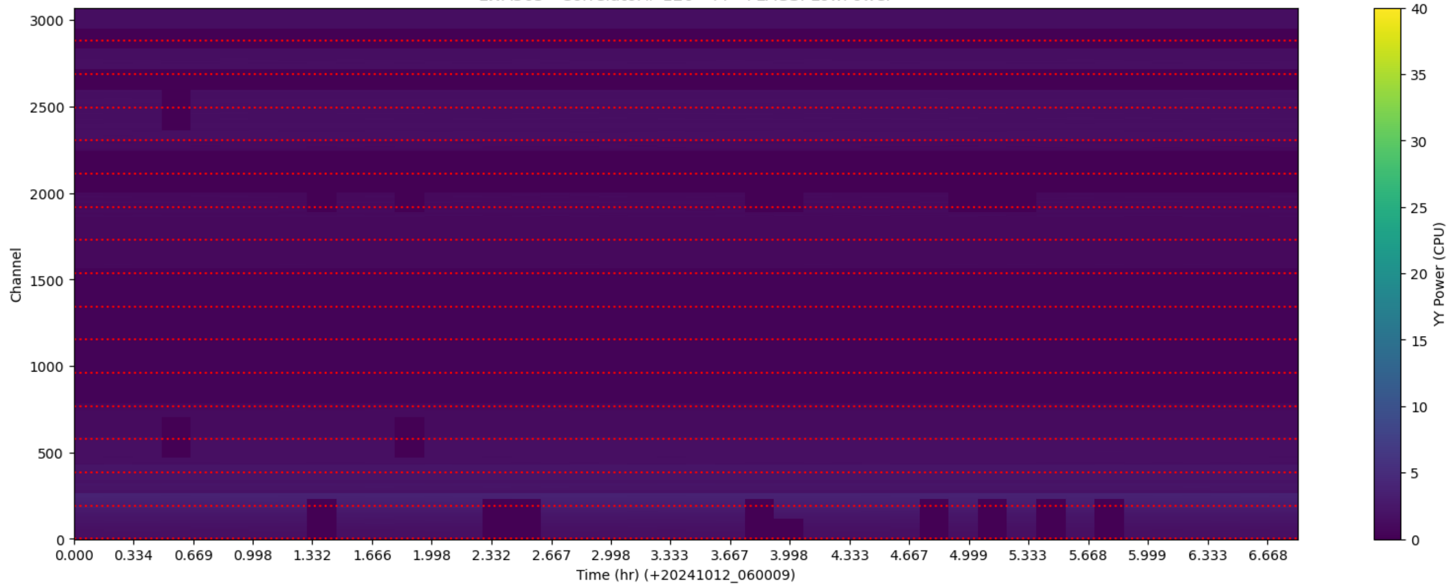
LWA365 - Correlator# 126 - YY - FLAGS: LowPower
