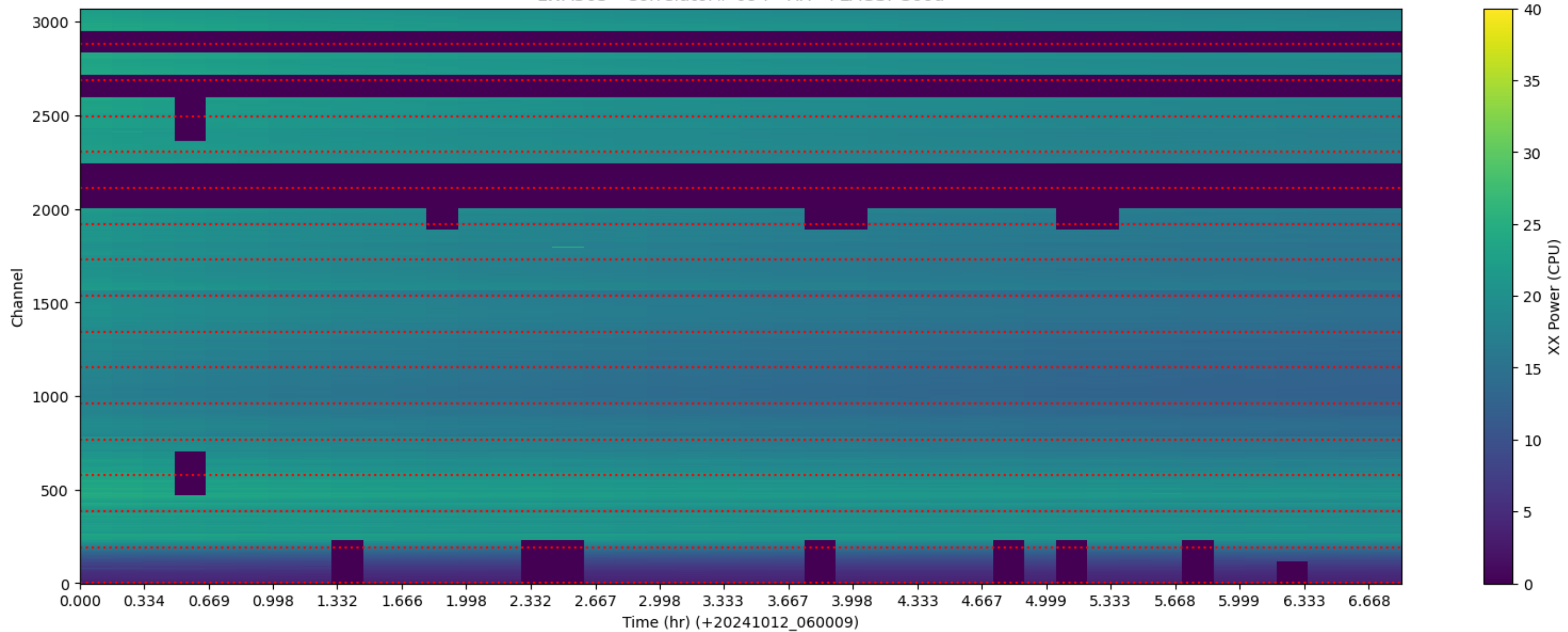
LWA363 - Correlator# 094 - XX - FLAGS: Good
