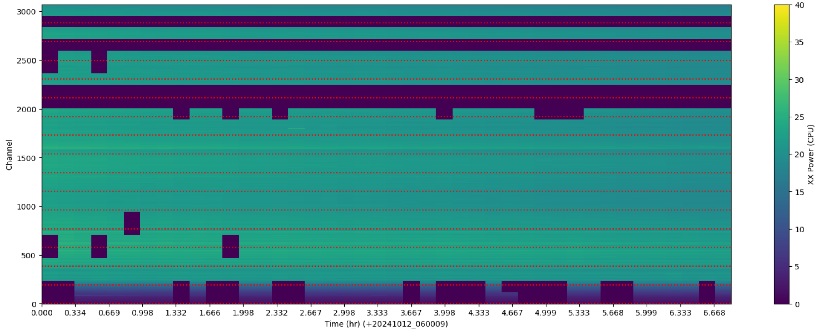
LWA184 - Correlator# 241 - XX - FLAGS: Good
