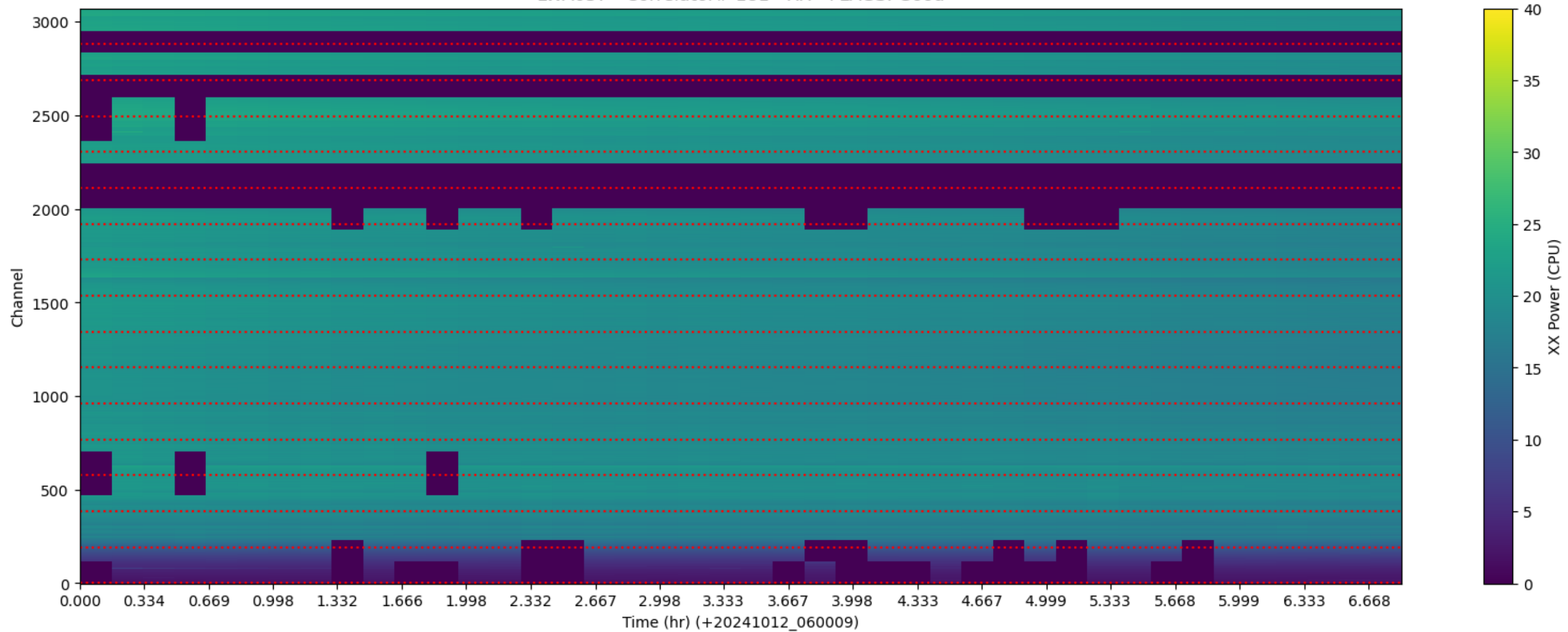
LWA037 - Correlator# 181 - XX - FLAGS: Good
