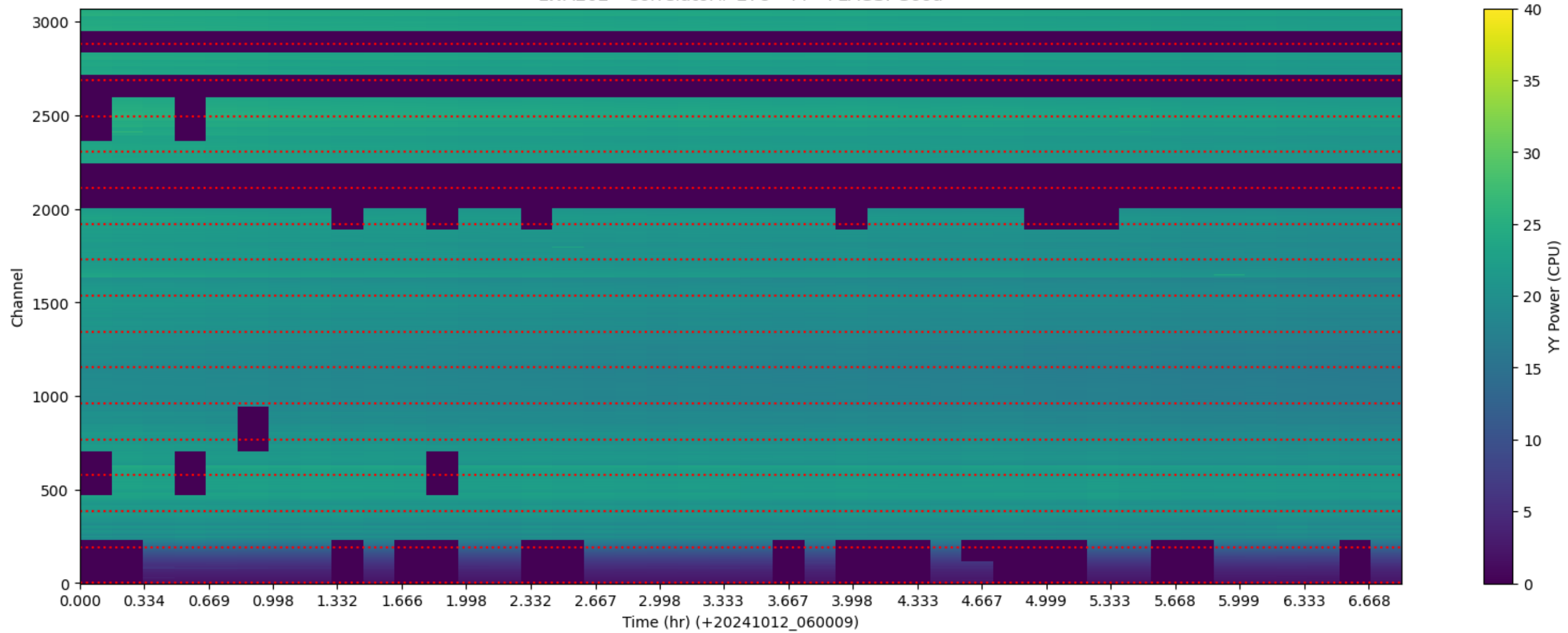
LWA202 - Correlator# 278 - YY - FLAGS: Good
