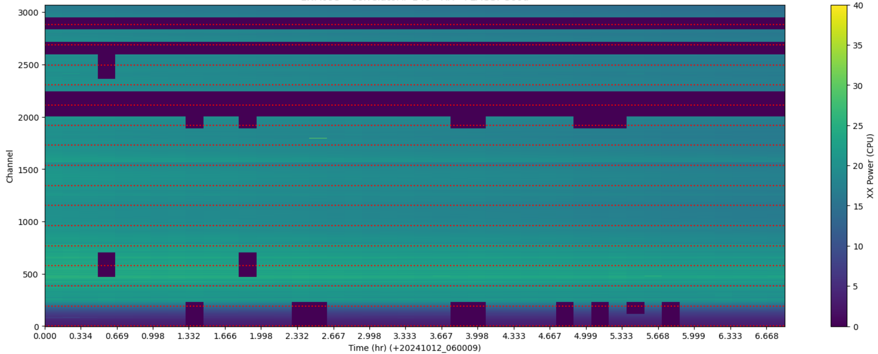
LWA093 - Correlator# 148 - XX - FLAGS: Good
