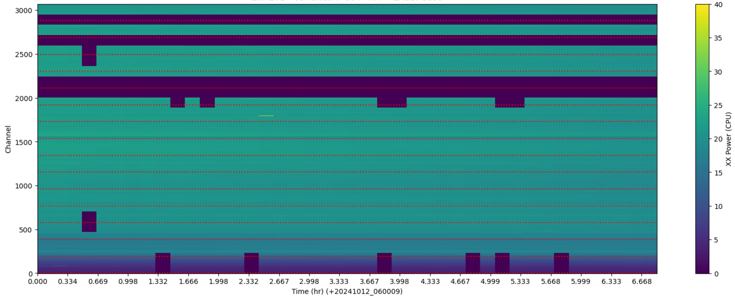
LWA271 - Correlator# 004 - XX - FLAGS: Good
