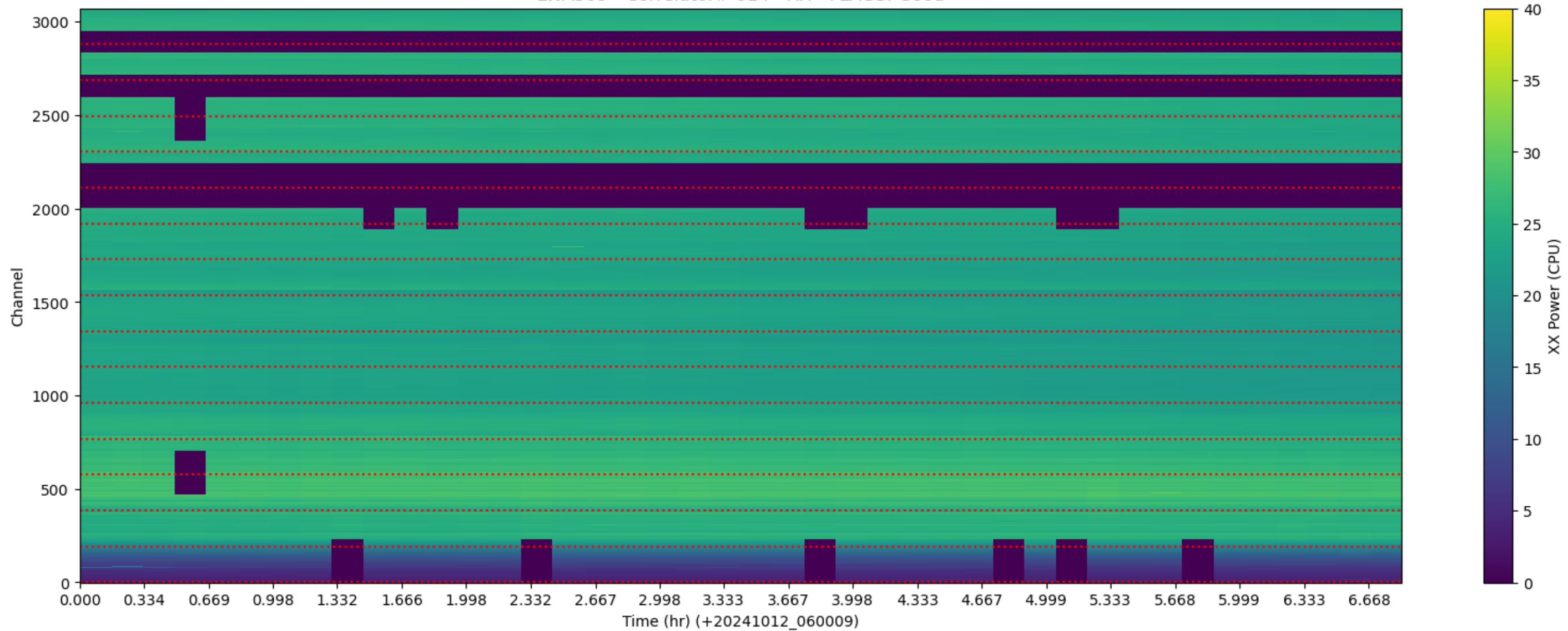
LWA309 - Correlator# 014 - XX - FLAGS: Good
