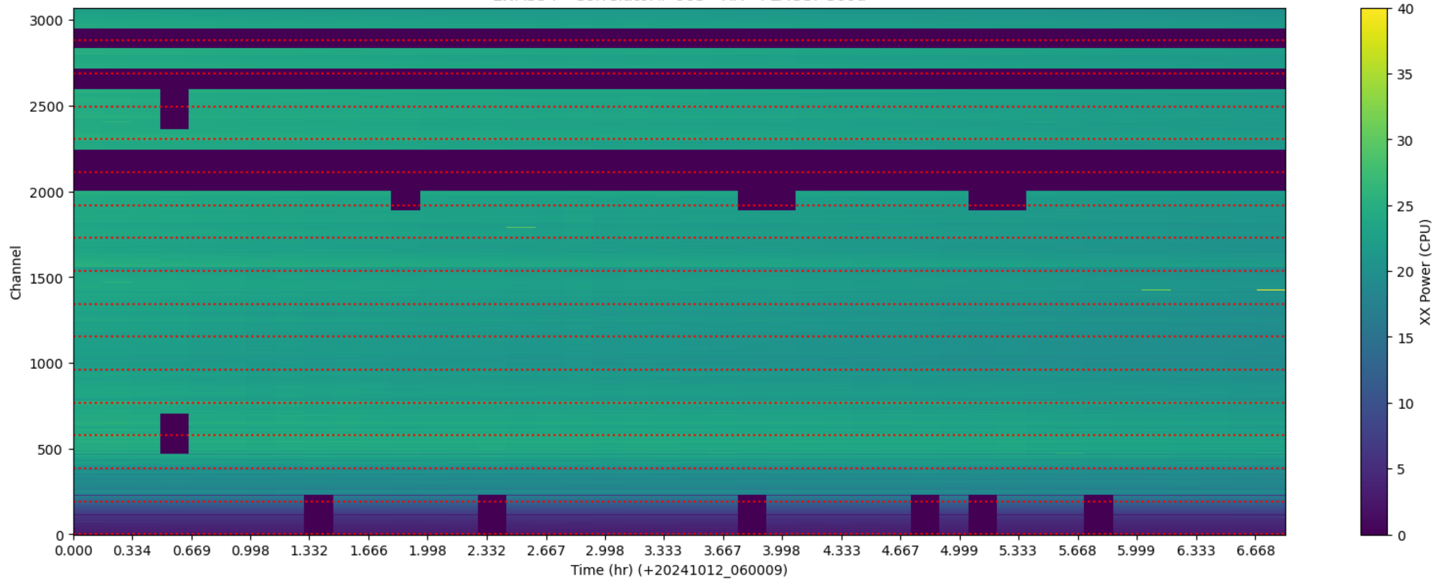
LWA354 - Correlator# 063 - XX - FLAGS: Good
