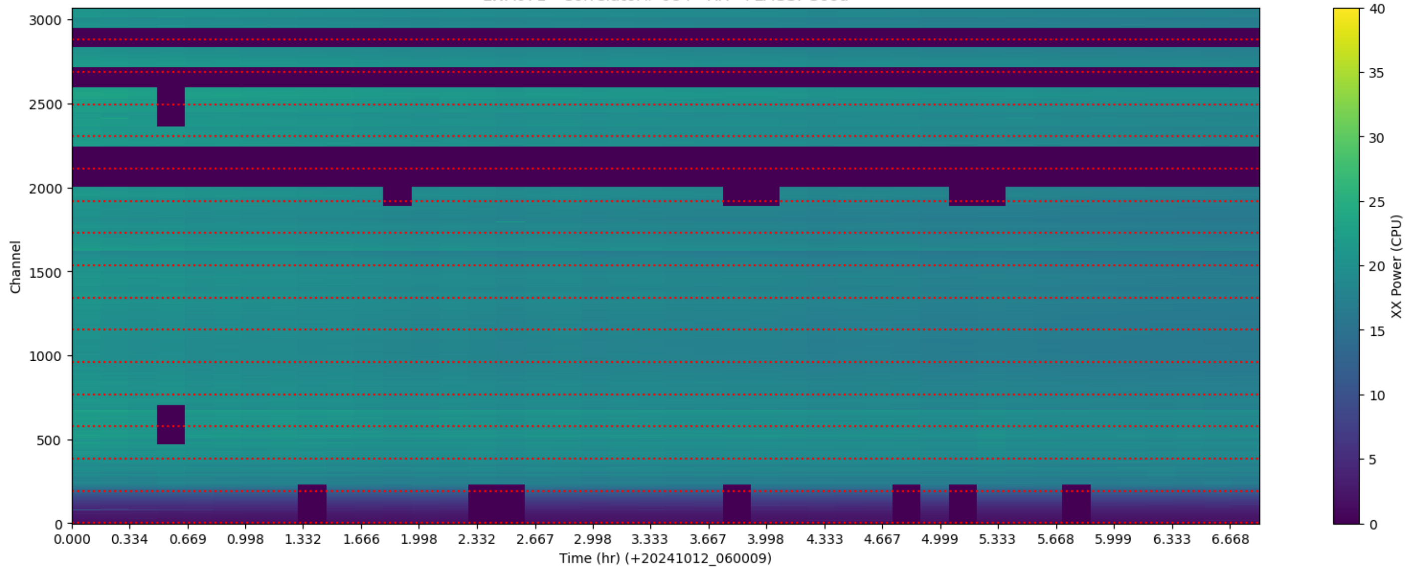
LWA071 - Correlator# 084 - XX - FLAGS: Good
