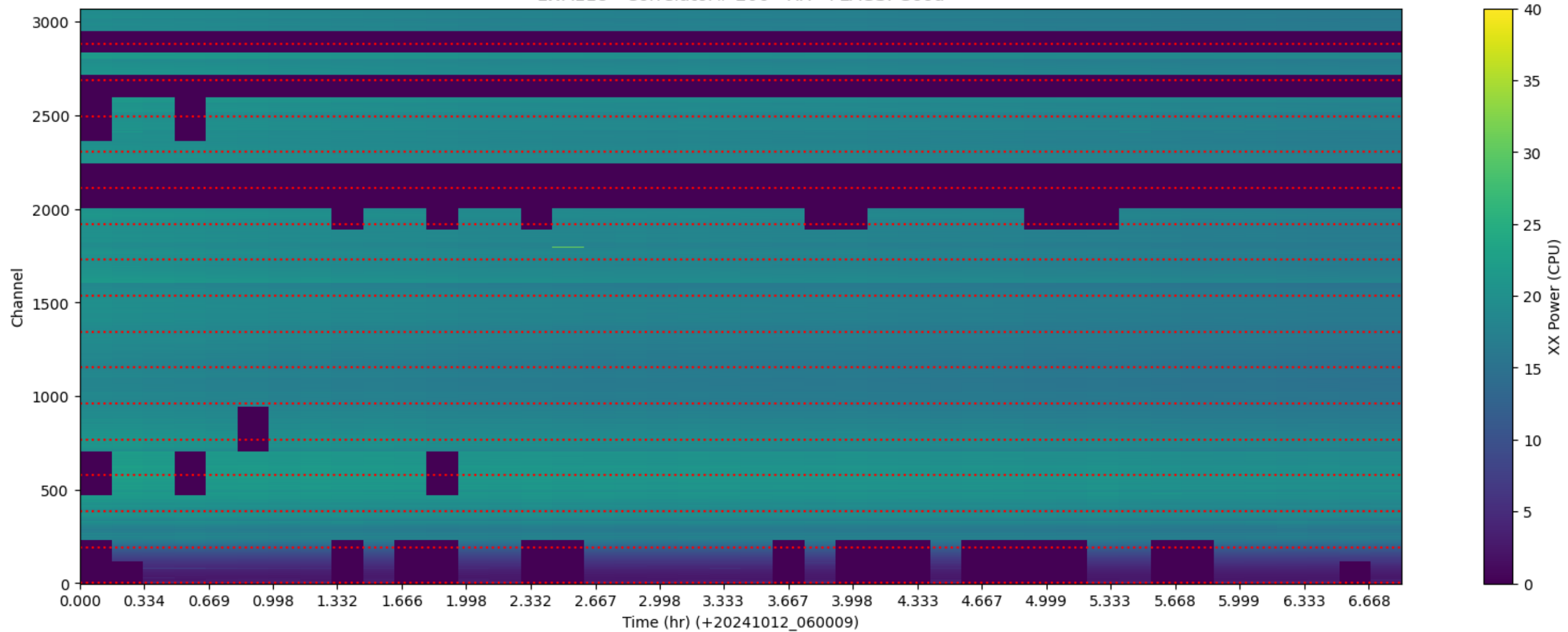
LWA118 - Correlator# 206 - XX - FLAGS: Good
