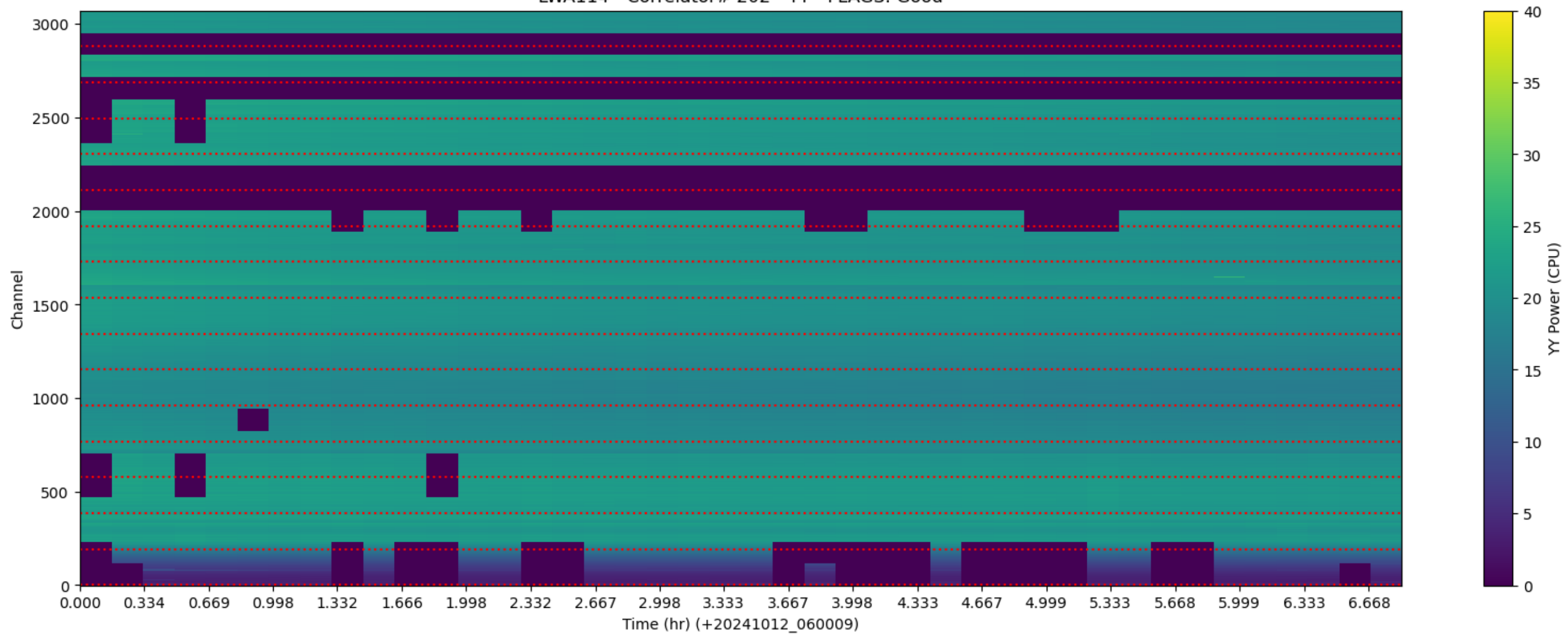
LWA114 - Correlator# 202 - YY - FLAGS: Good
