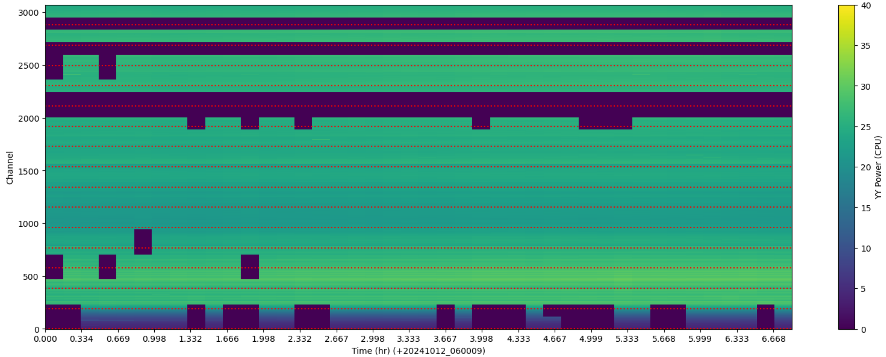
LWA333 - Correlator# 253 - YY - FLAGS: Good
