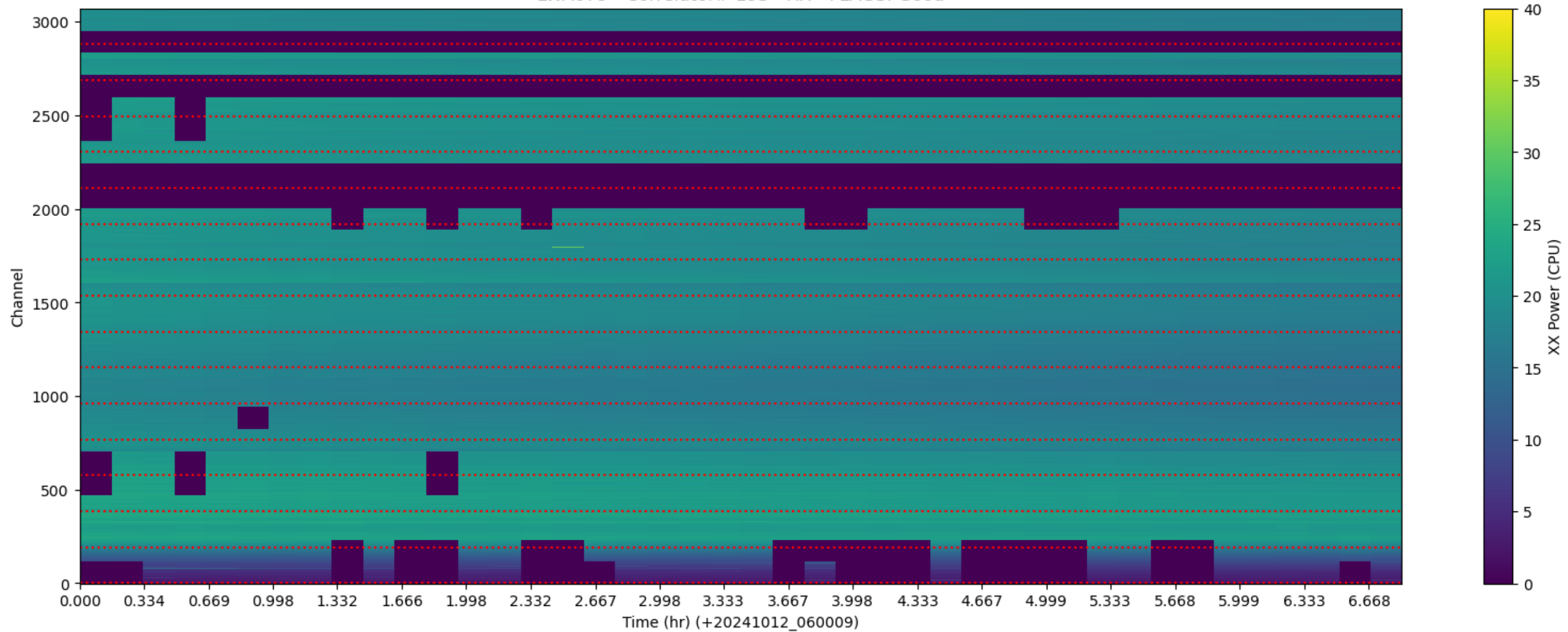
LWA079 - Correlator# 195 - XX - FLAGS: Good
