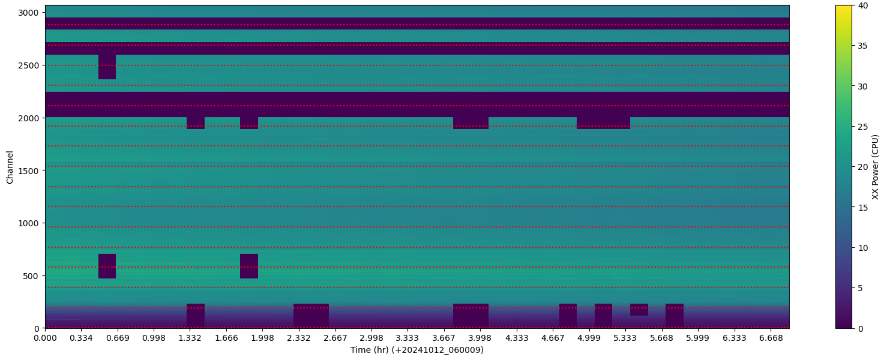
LWA122 - Correlator# 152 - XX - FLAGS: Good
