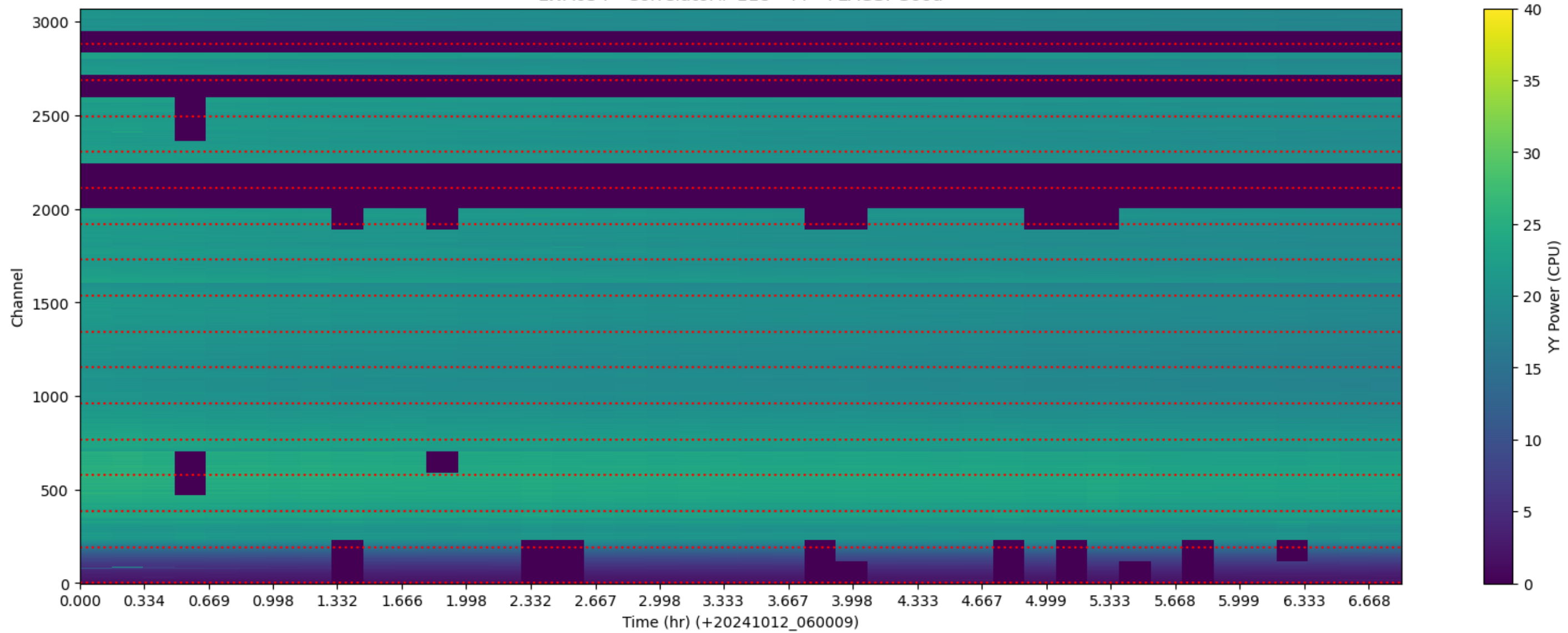
LWA054 - Correlator# 118 - YY - FLAGS: Good
