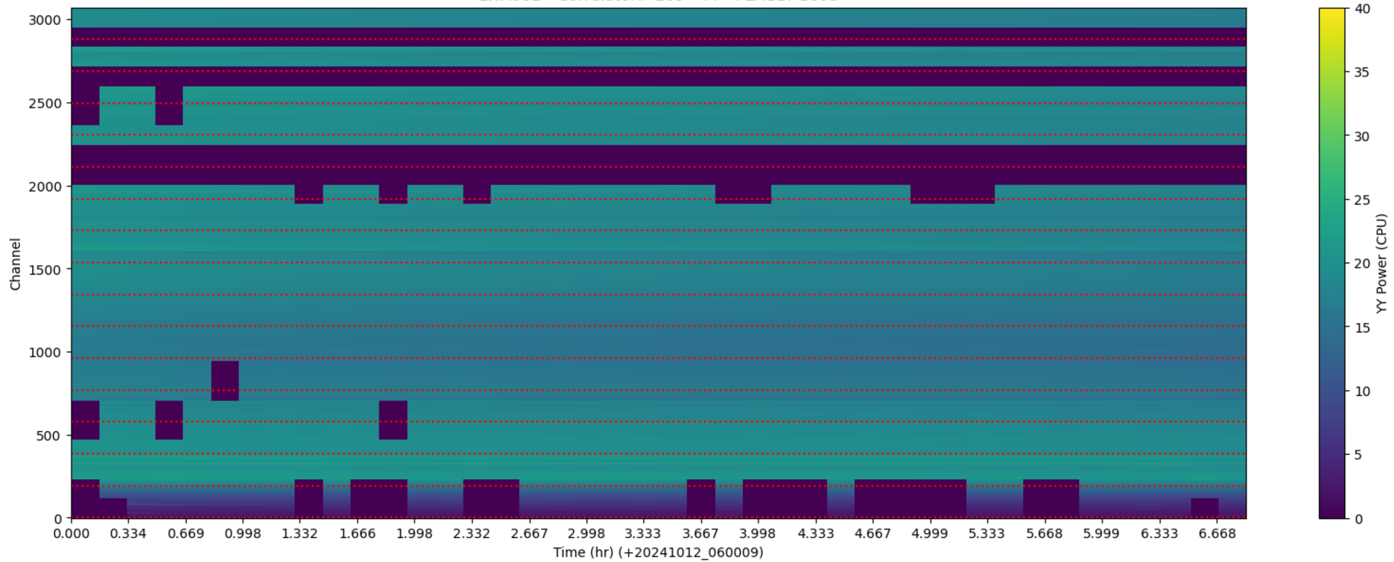
LWA082 - Correlator# 209 - YY - FLAGS: Good
