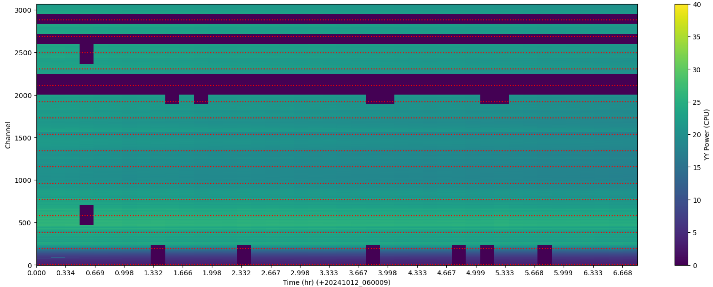
LWA312 - Correlator# 019 - YY - FLAGS: Good
