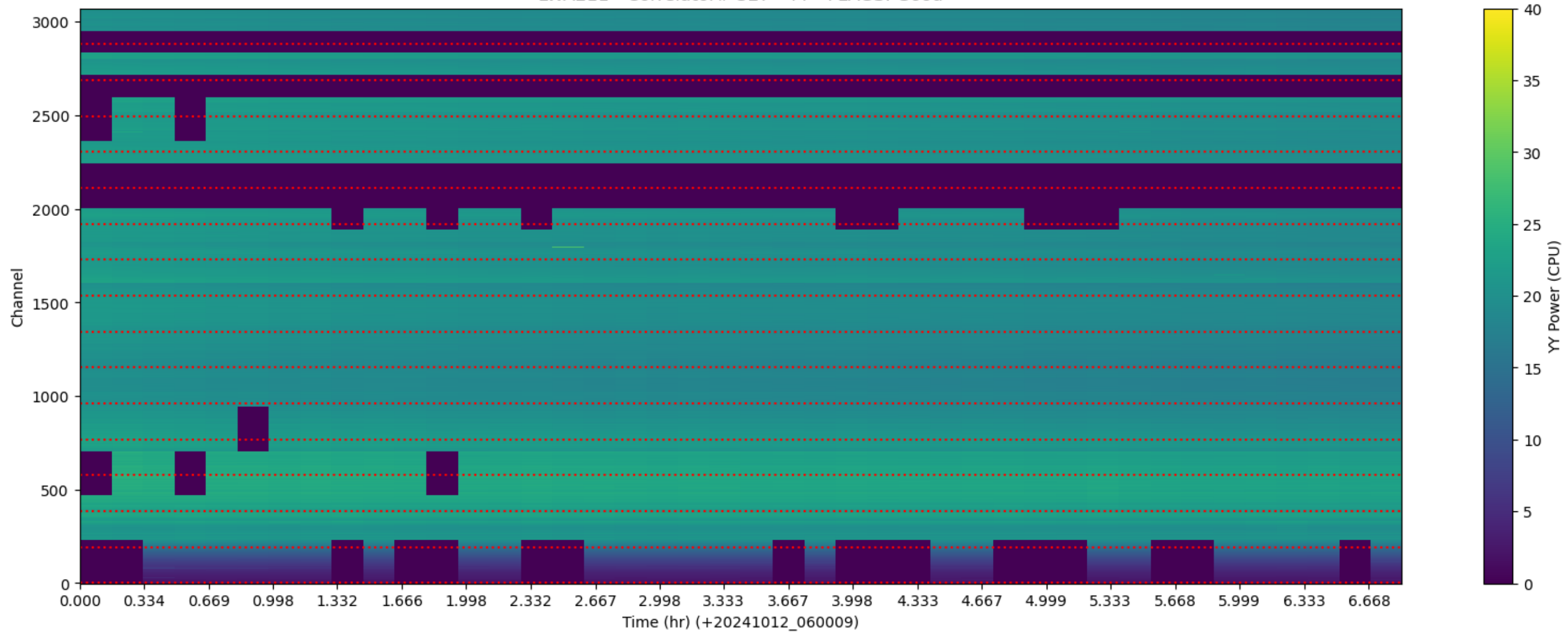
LWA211 - Correlator# 327 - YY - FLAGS: Good
