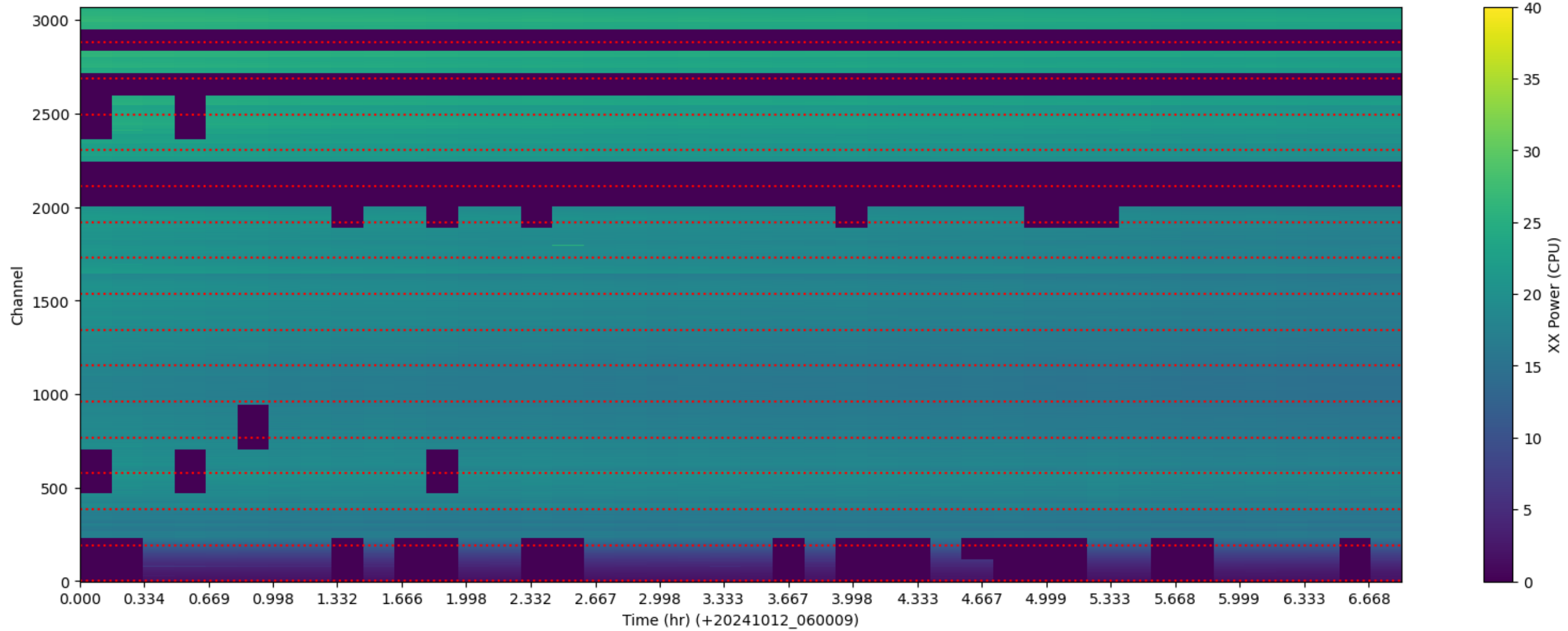
LWA194 - Correlator# 273 - XX - FLAGS: Good
