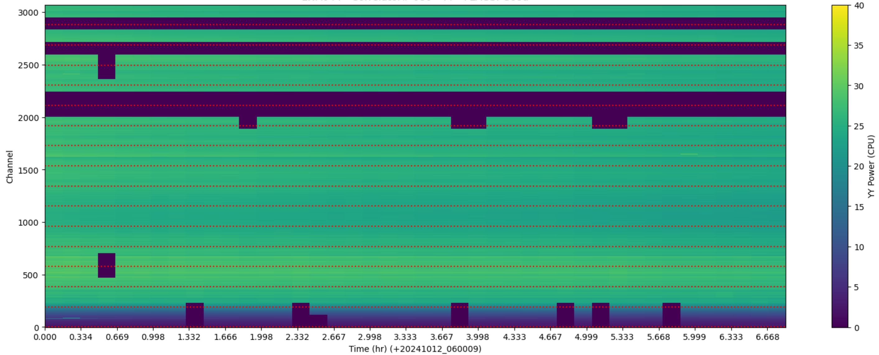
LWA044 - Correlator# 080 - YY - FLAGS: Good
