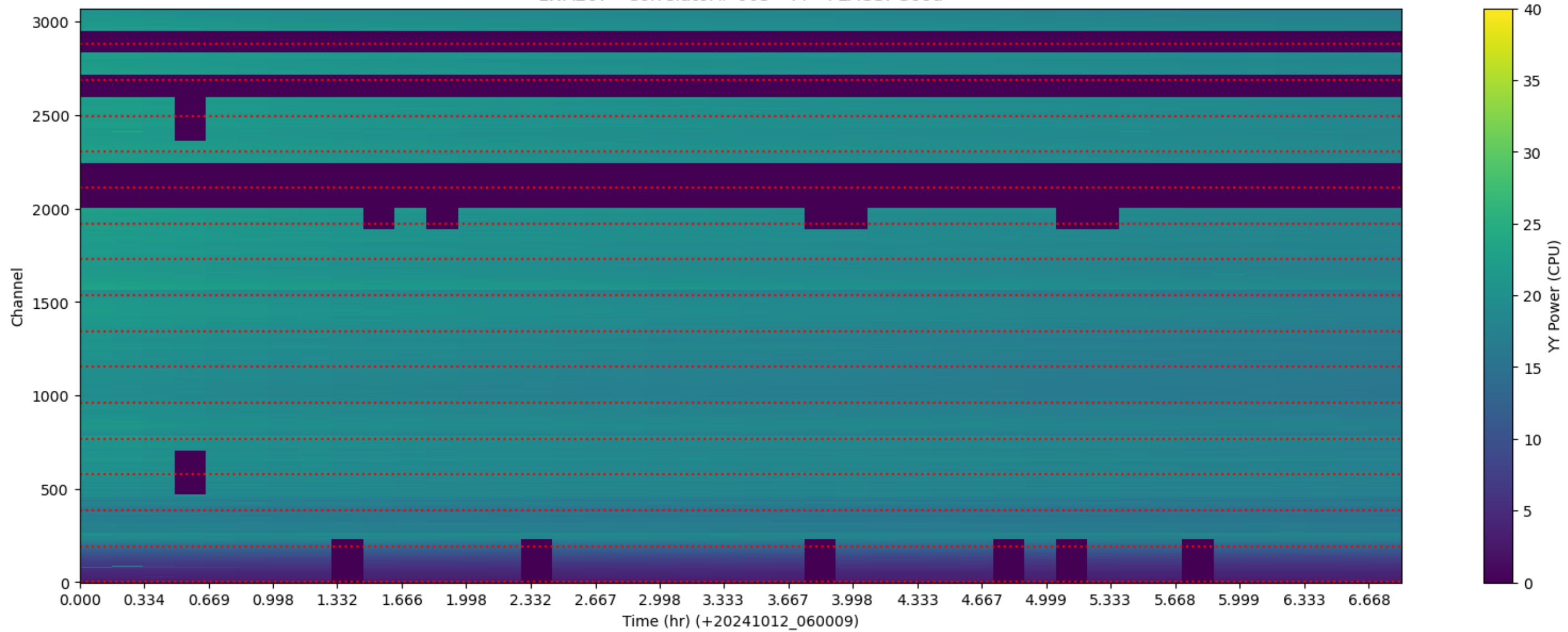
LWA267 - Correlator# 003 - YY - FLAGS: Good
