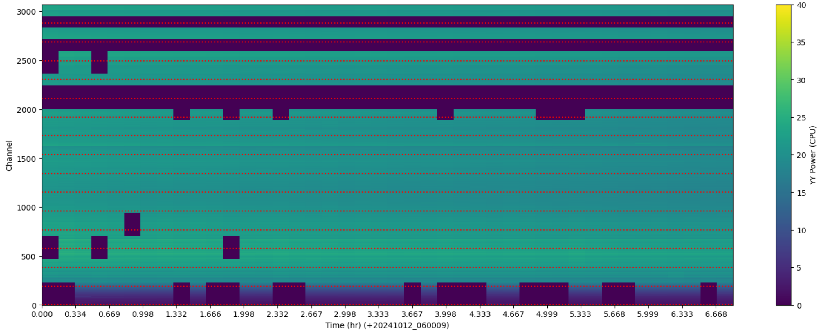
LWA236 - Correlator# 308 - YY - FLAGS: Good
