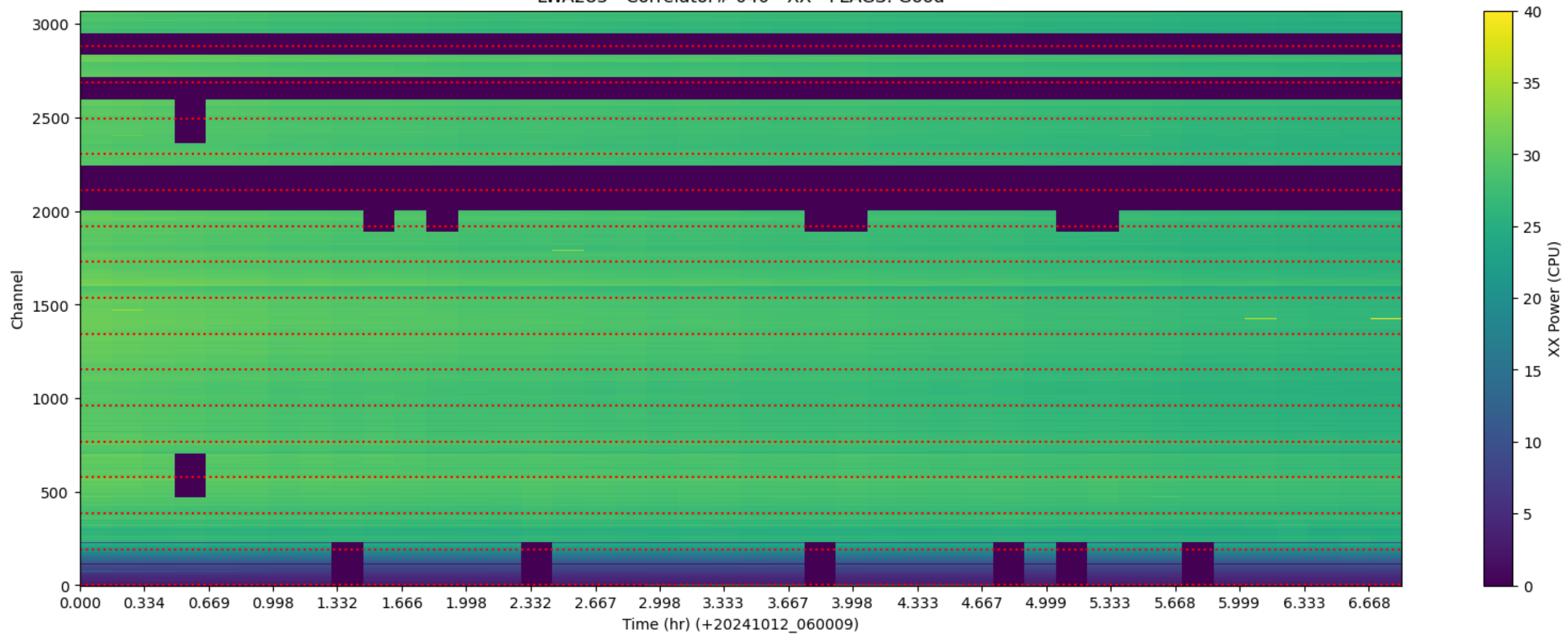
LWA283 - Correlator# 040 - XX - FLAGS: Good
