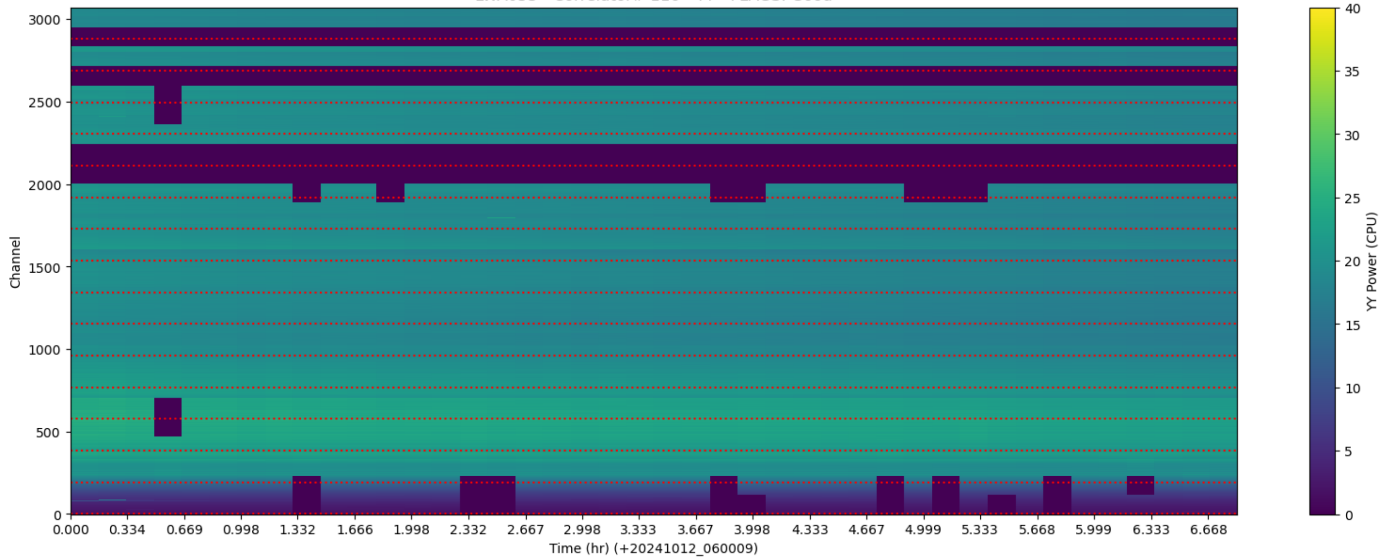
LWA053 - Correlator# 116 - YY - FLAGS: Good
