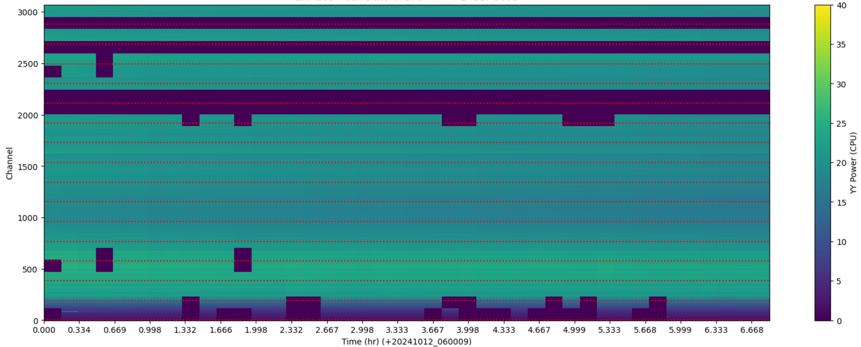
LWA103 - Correlator# 176 - YY - FLAGS: Good
