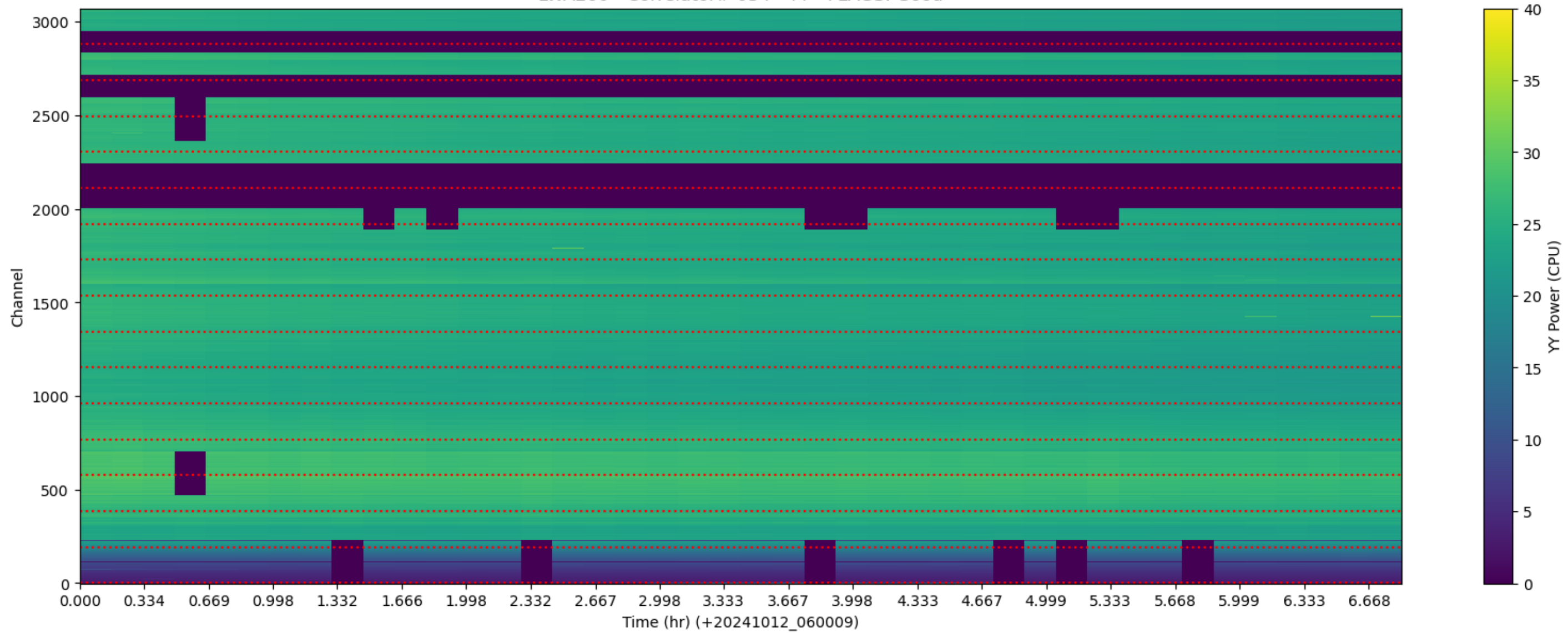
LWA260 - Correlator# 034 - YY - FLAGS: Good
