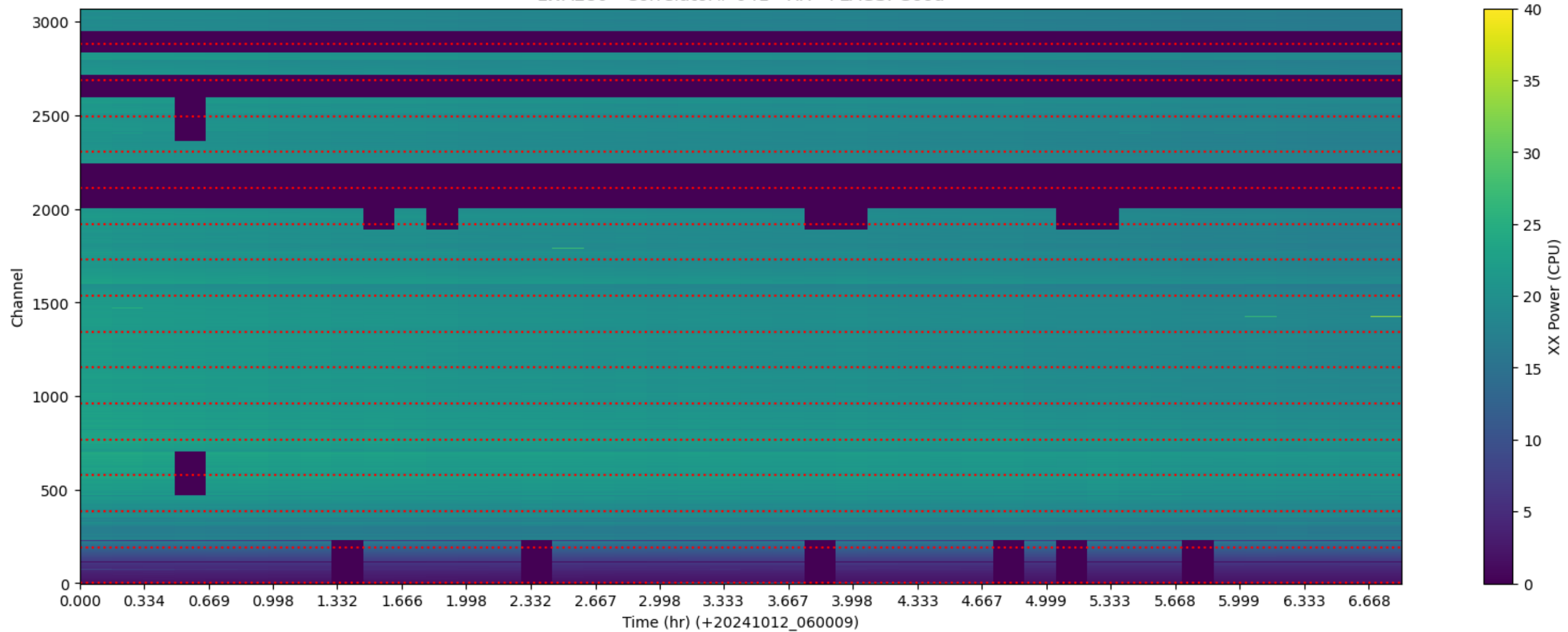
LWA280 - Correlator# 041 - XX - FLAGS: Good
