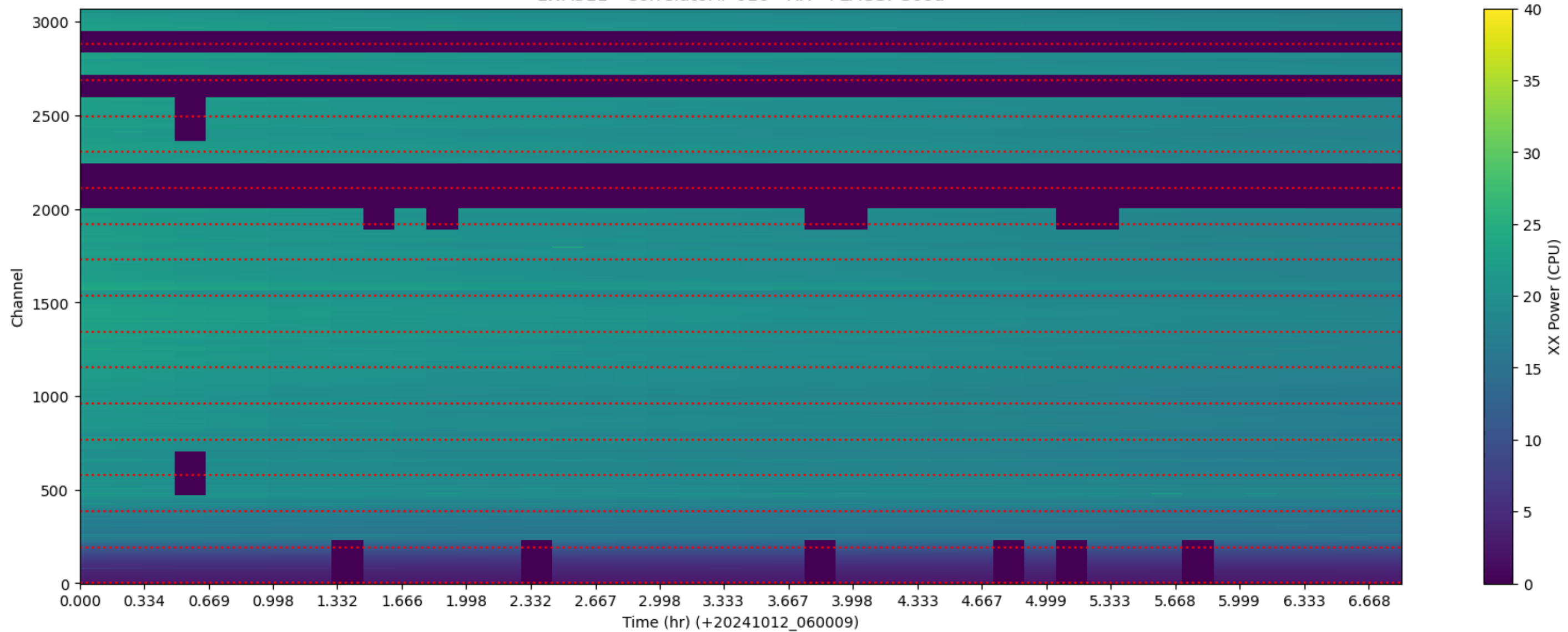
LWA311 - Correlator# 016 - XX - FLAGS: Good
