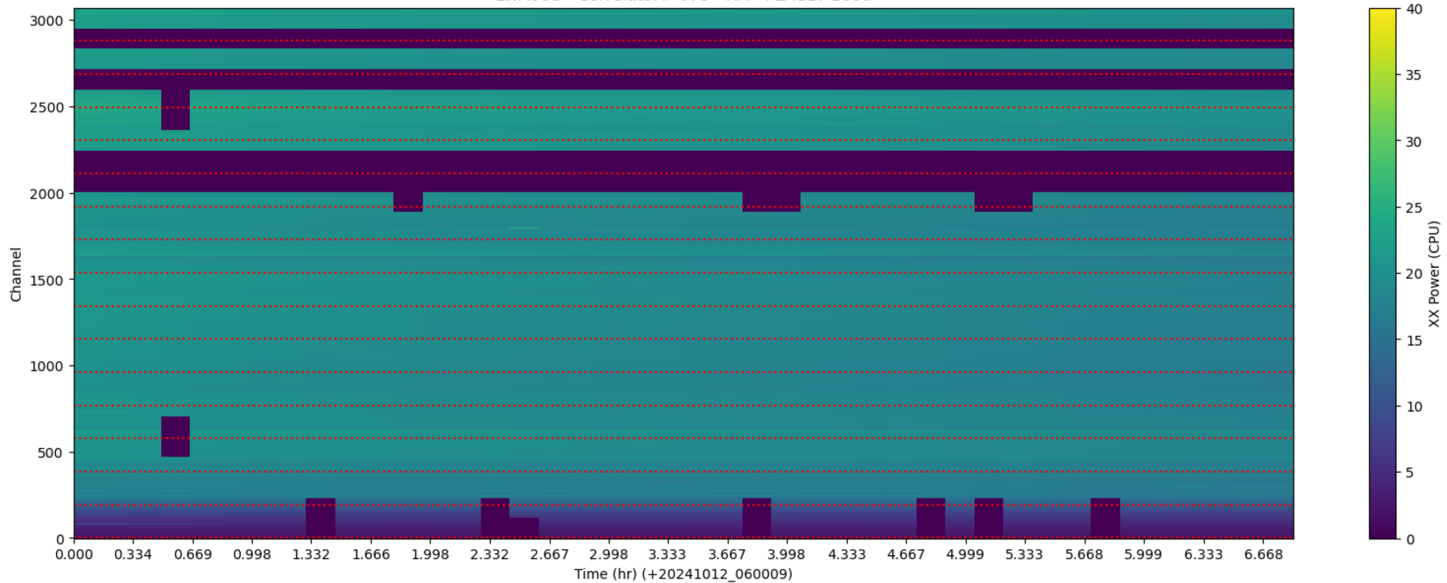
LWA008 - Correlator# 075 - XX - FLAGS: Good
