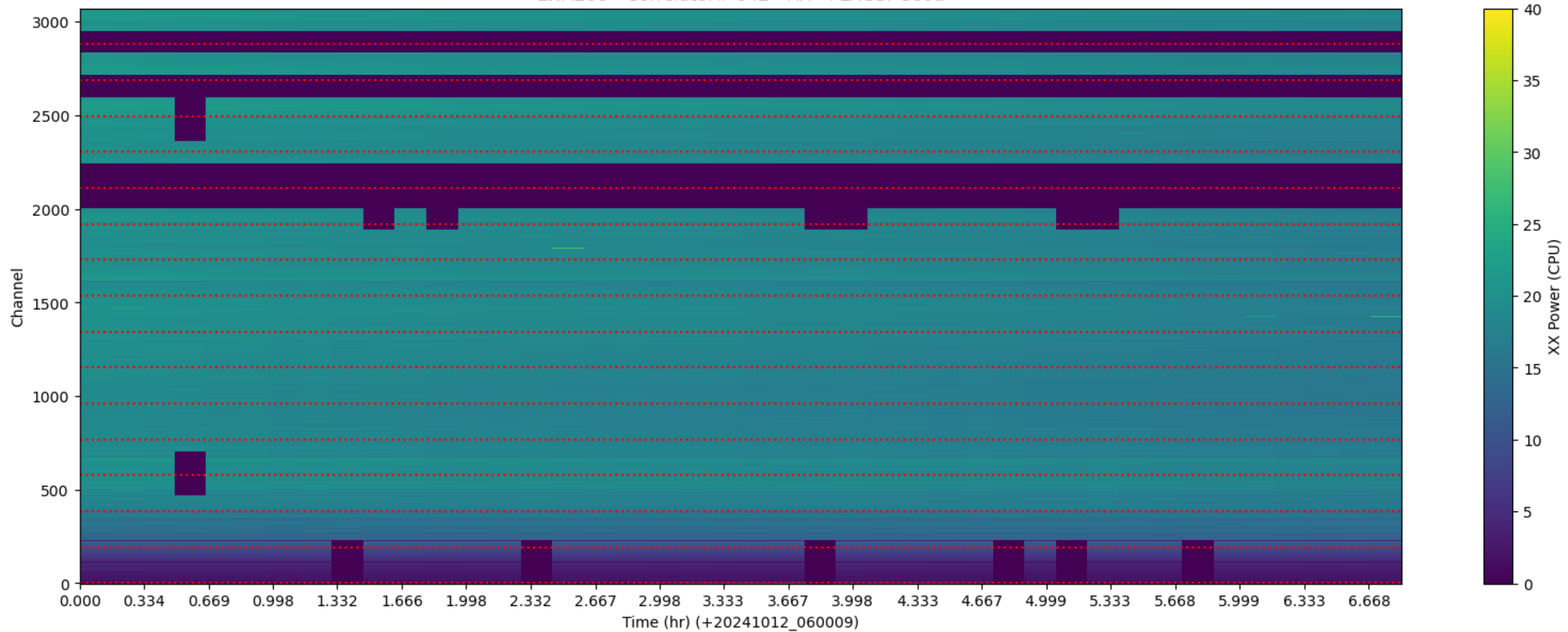
LWA288 - Correlator# 042 - XX - FLAGS: Good
