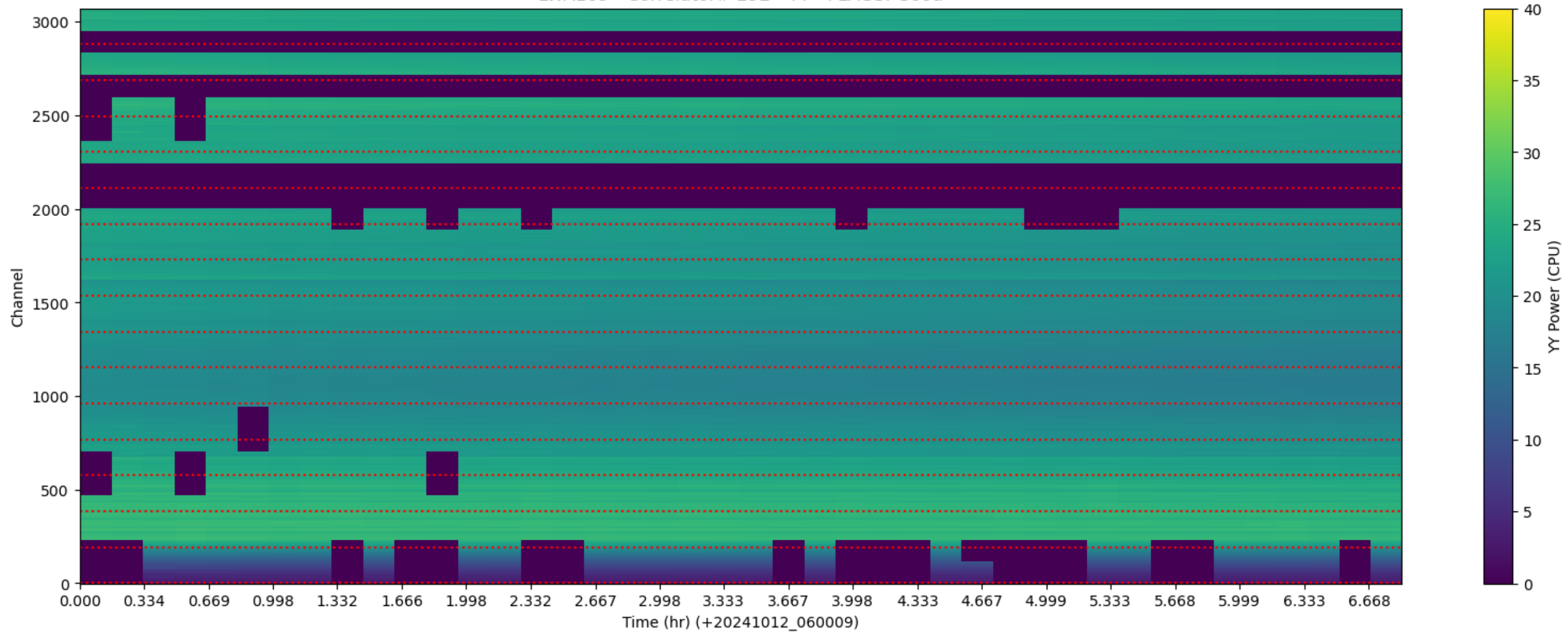
LWA169 - Correlator# 292 - YY - FLAGS: Good
