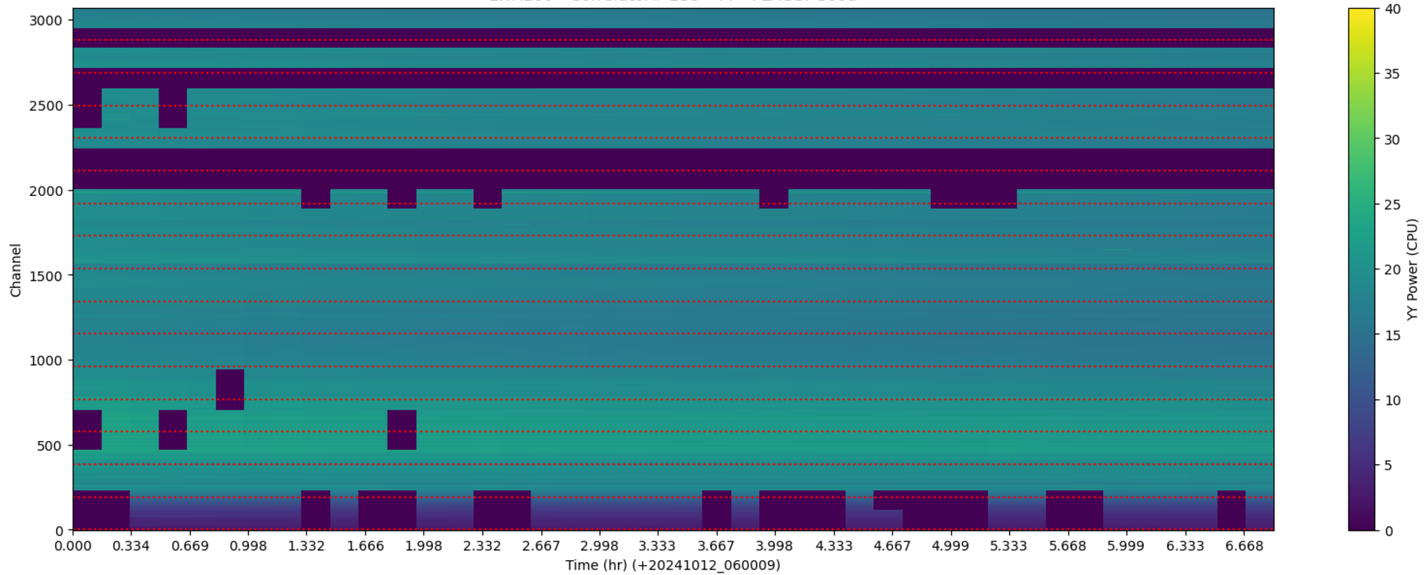
LWA160 - Correlator# 239 - YY - FLAGS: Good
