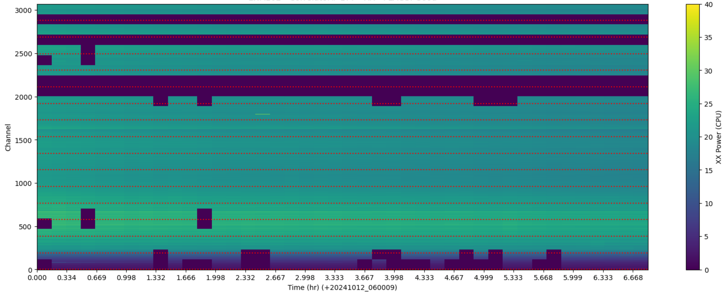
LWA102 - Correlator# 177 - XX - FLAGS: Good
