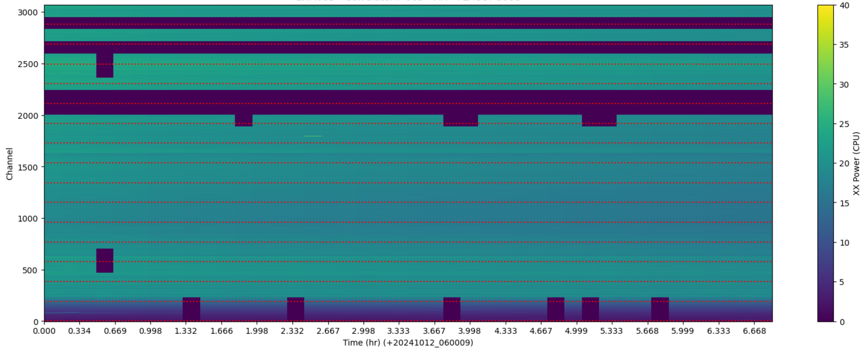
LWA005 - Correlator# 069 - XX - FLAGS: Good
