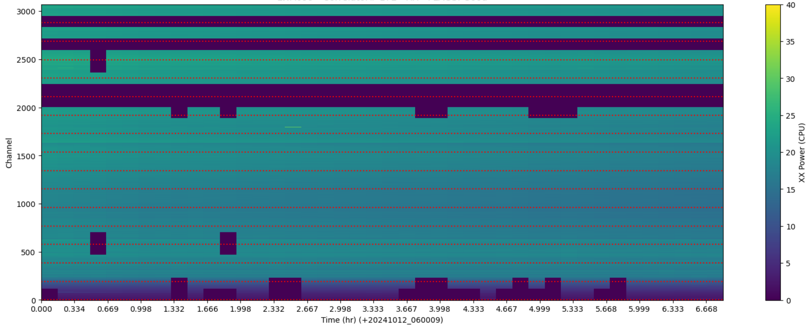
LWA099 - Correlator# 172 - XX - FLAGS: Good
