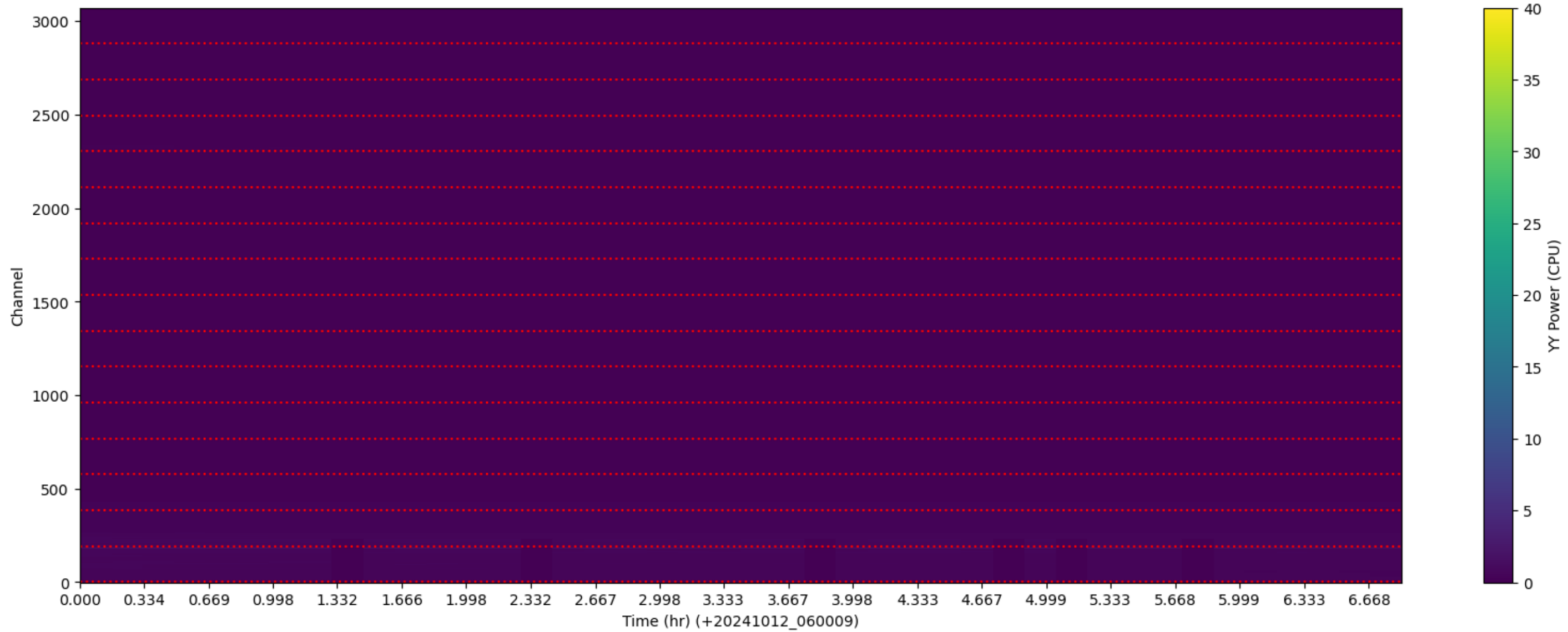
LWA266 - Correlator# 000 - YY - FLAGS: LowPower
