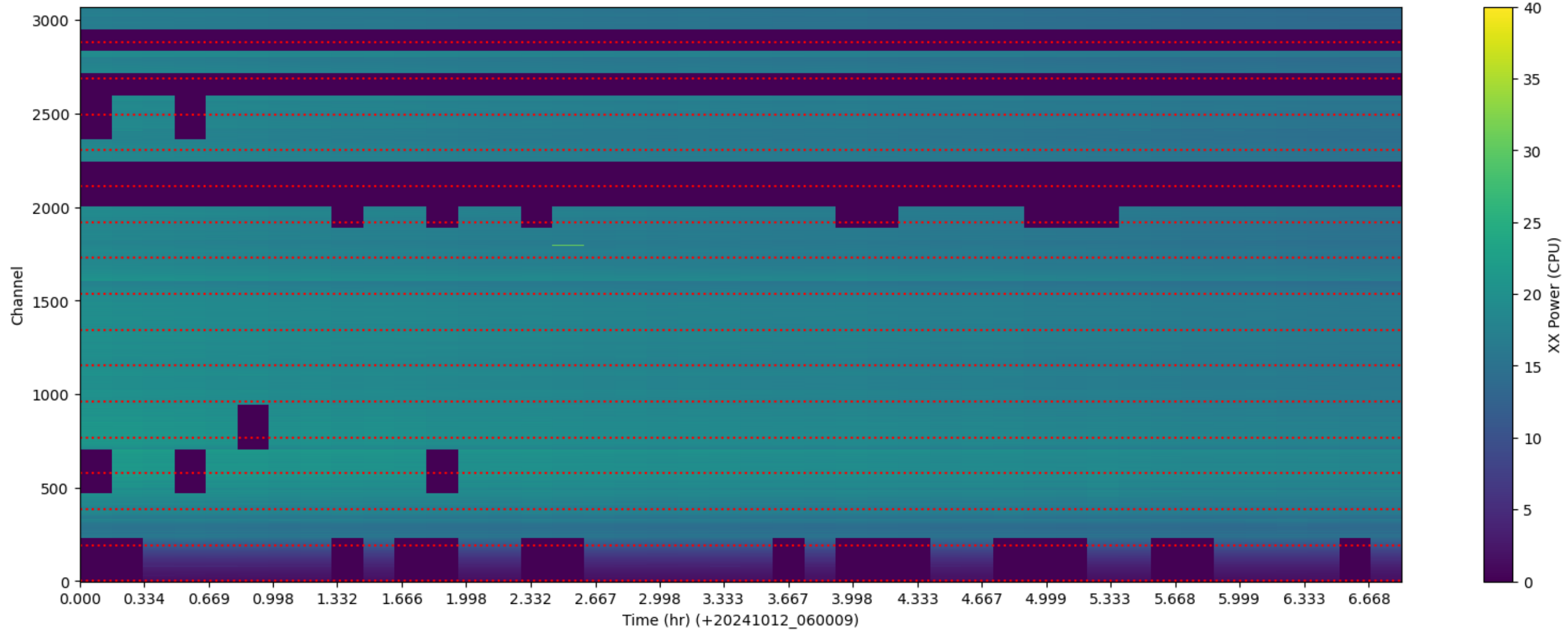
LWA215 - Correlator# 331 - XX - FLAGS: Good
