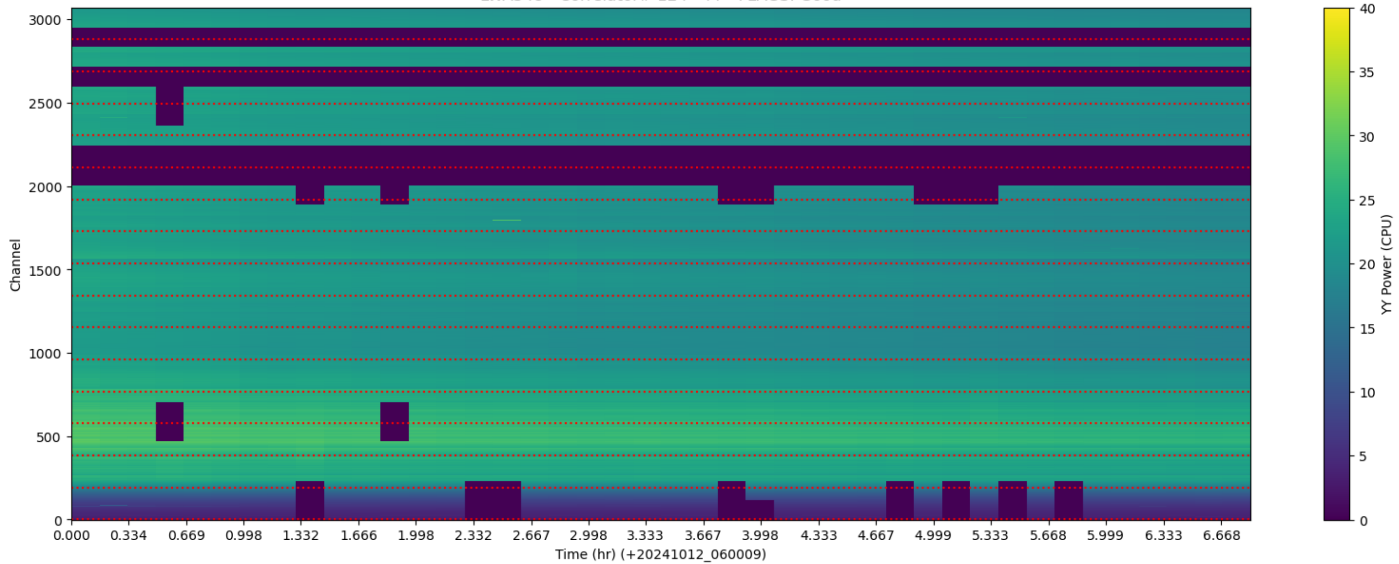
LWA348 - Correlator# 124 - YY - FLAGS: Good
