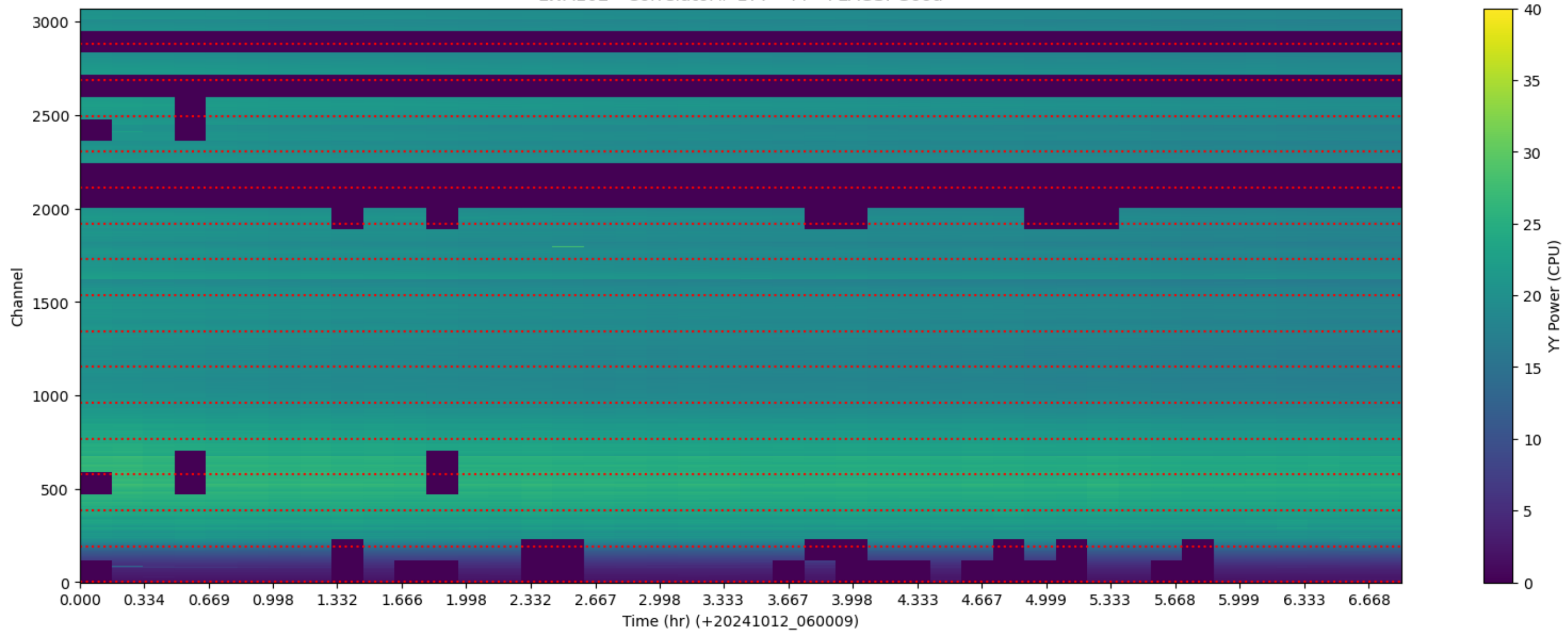
LWA102 - Correlator# 177 - YY - FLAGS: Good
