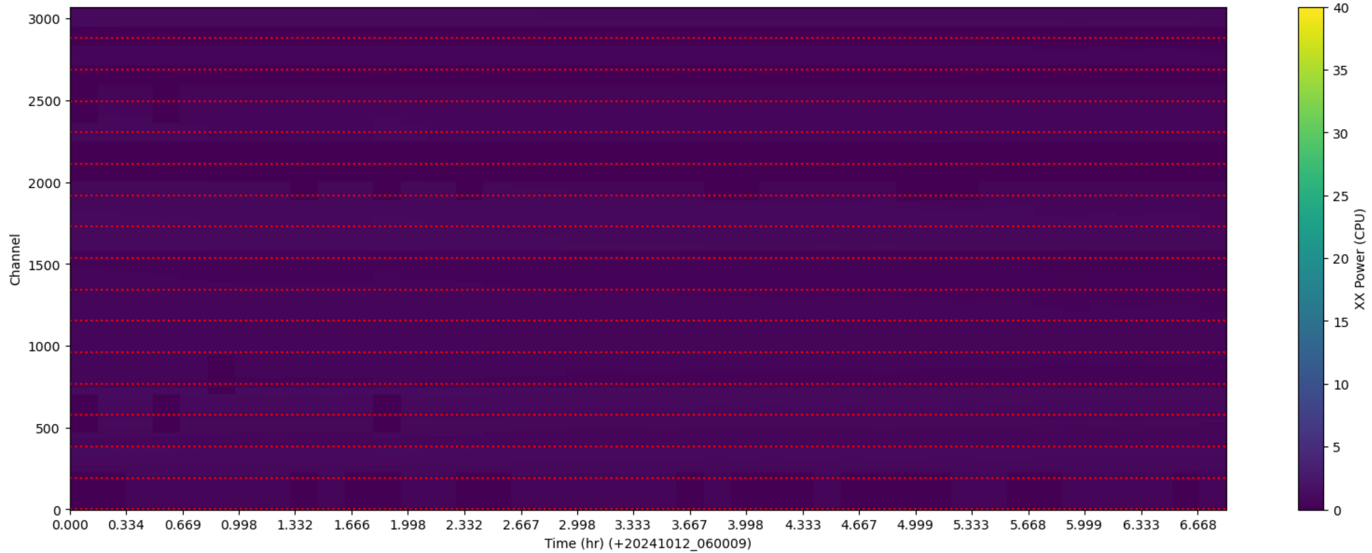
LWA150 - Correlator# 215 - XX - FLAGS: LowPower
