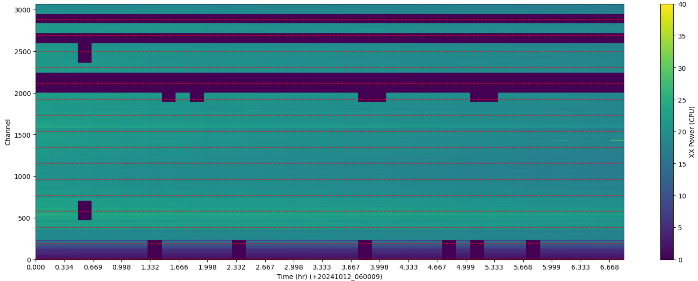
LWA336 - Correlator# 056 - XX - FLAGS: Good
