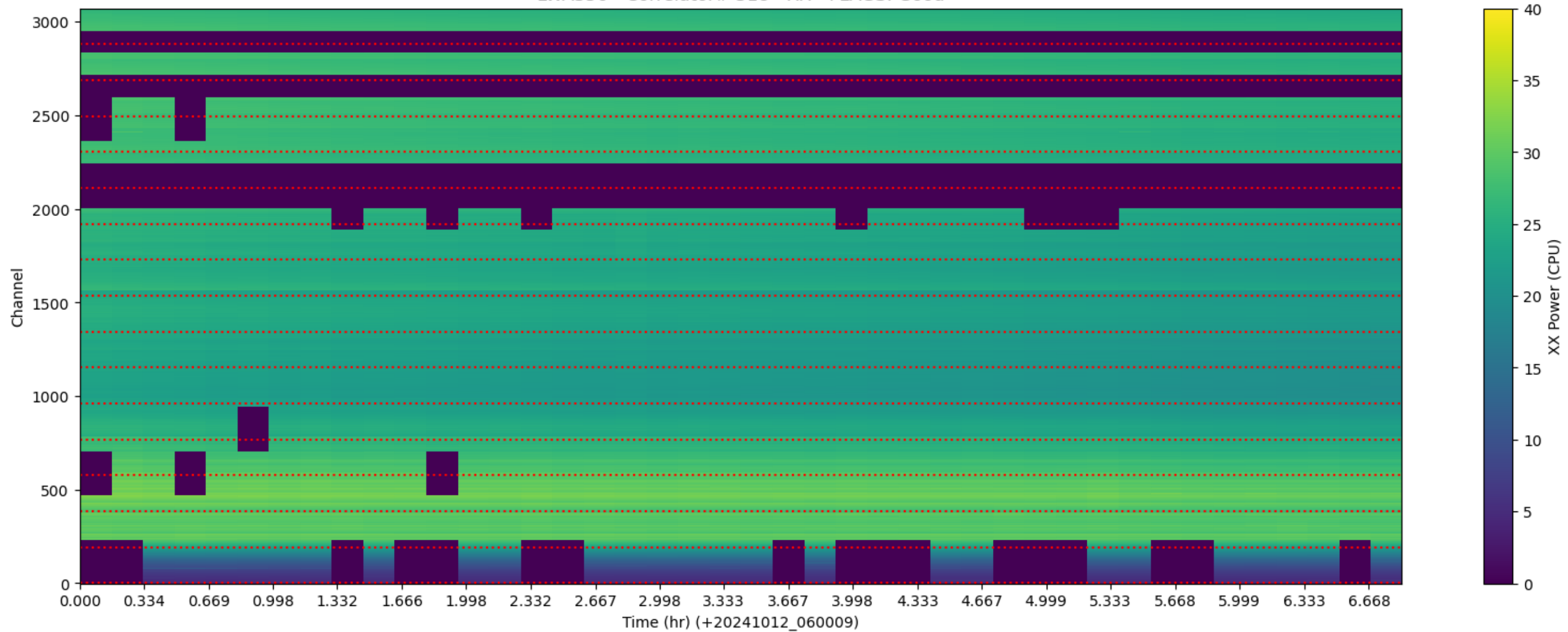
LWA356 - Correlator# 318 - XX - FLAGS: Good
