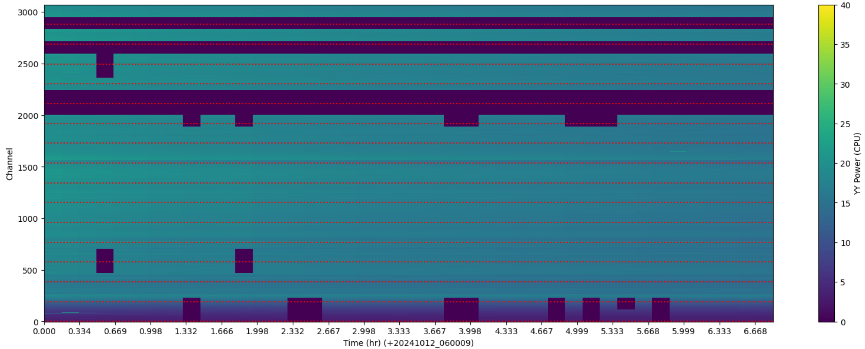
LWA334 - Correlator# 156 - YY - FLAGS: Good
