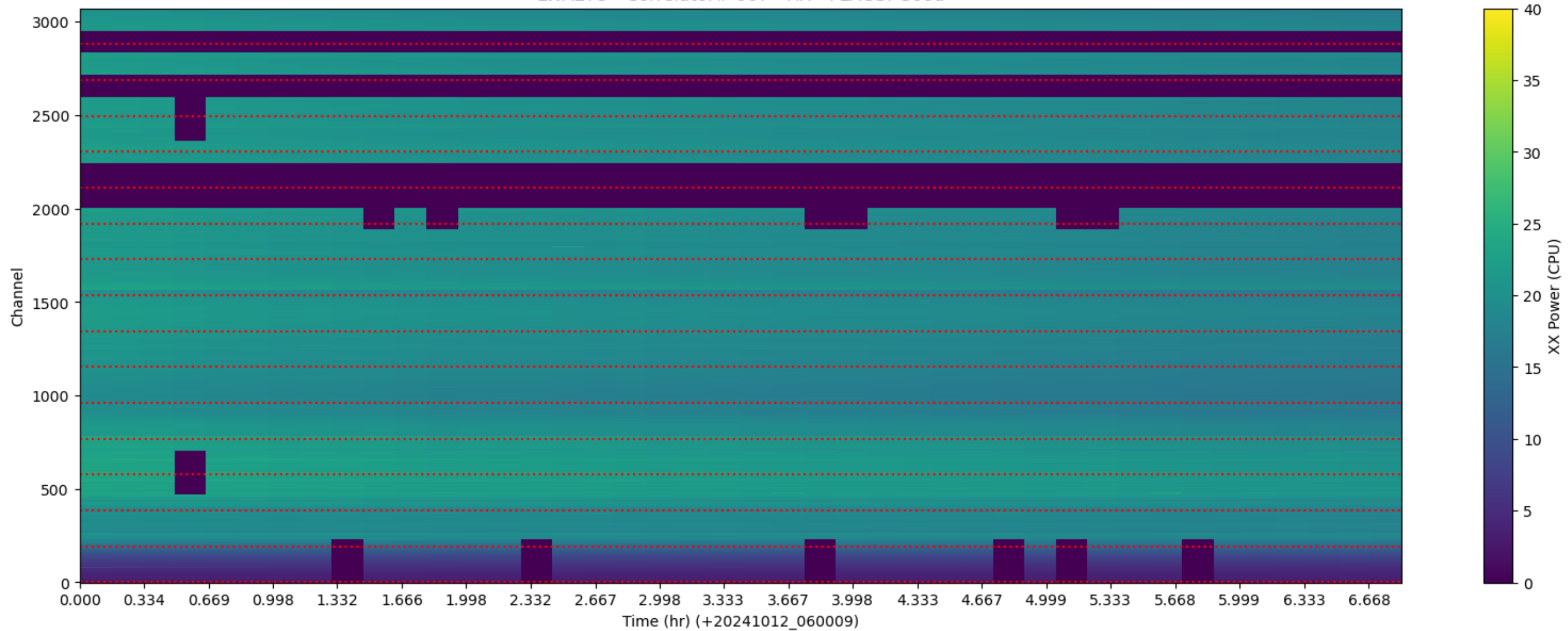
LWA273 - Correlator# 007 - XX - FLAGS: Good
