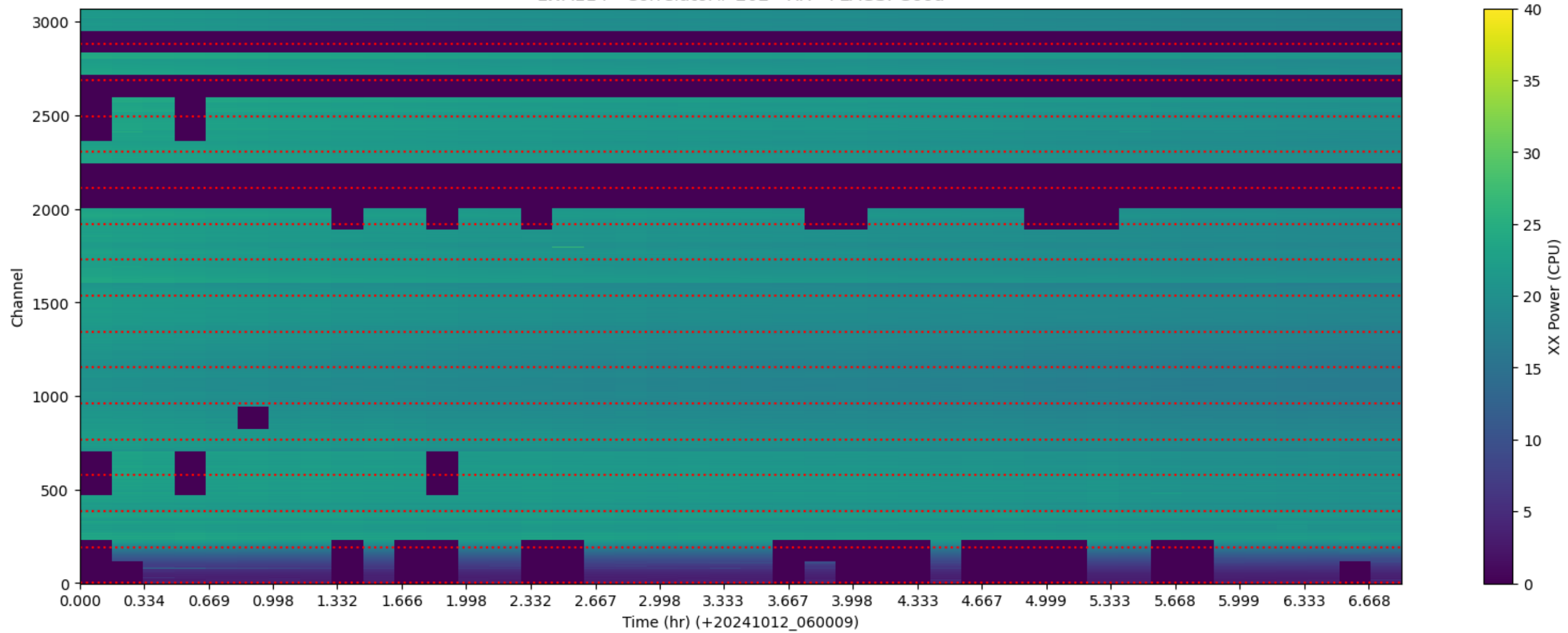
LWA114 - Correlator# 202 - XX - FLAGS: Good
