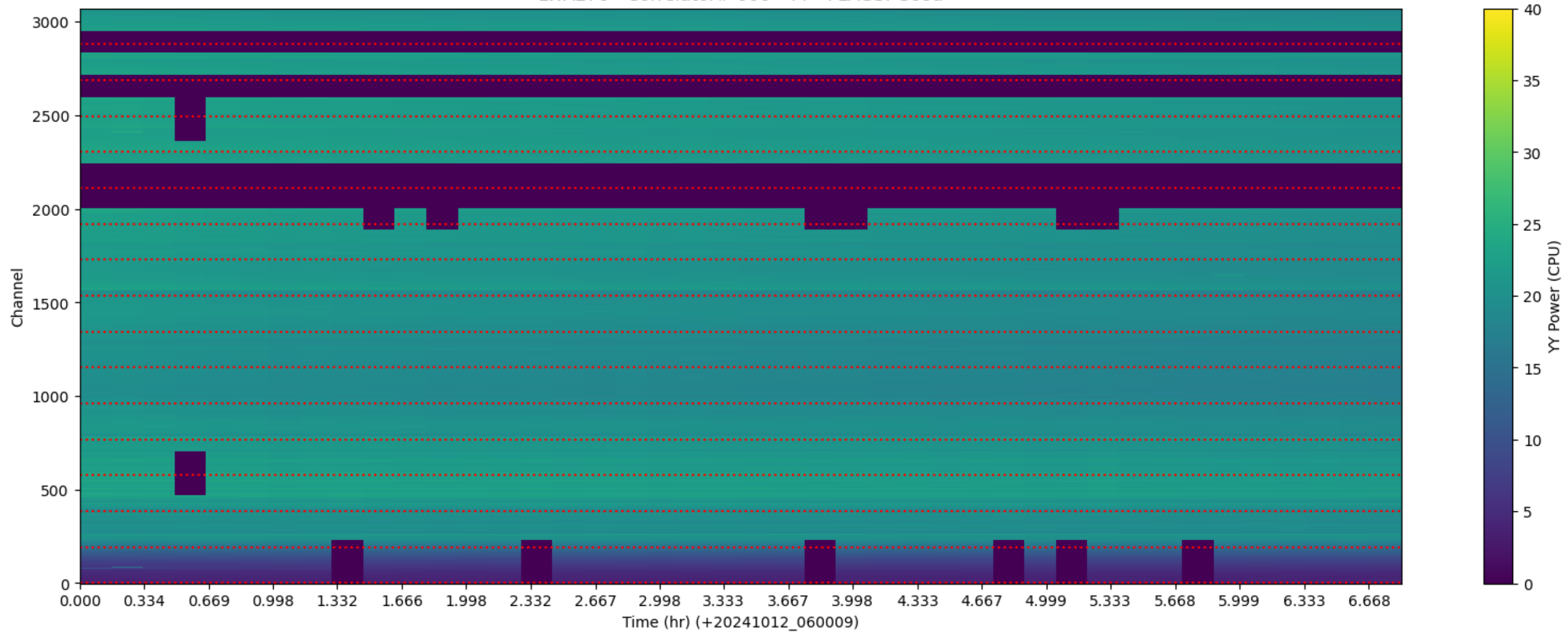
LWA276 - Correlator# 006 - YY - FLAGS: Good
