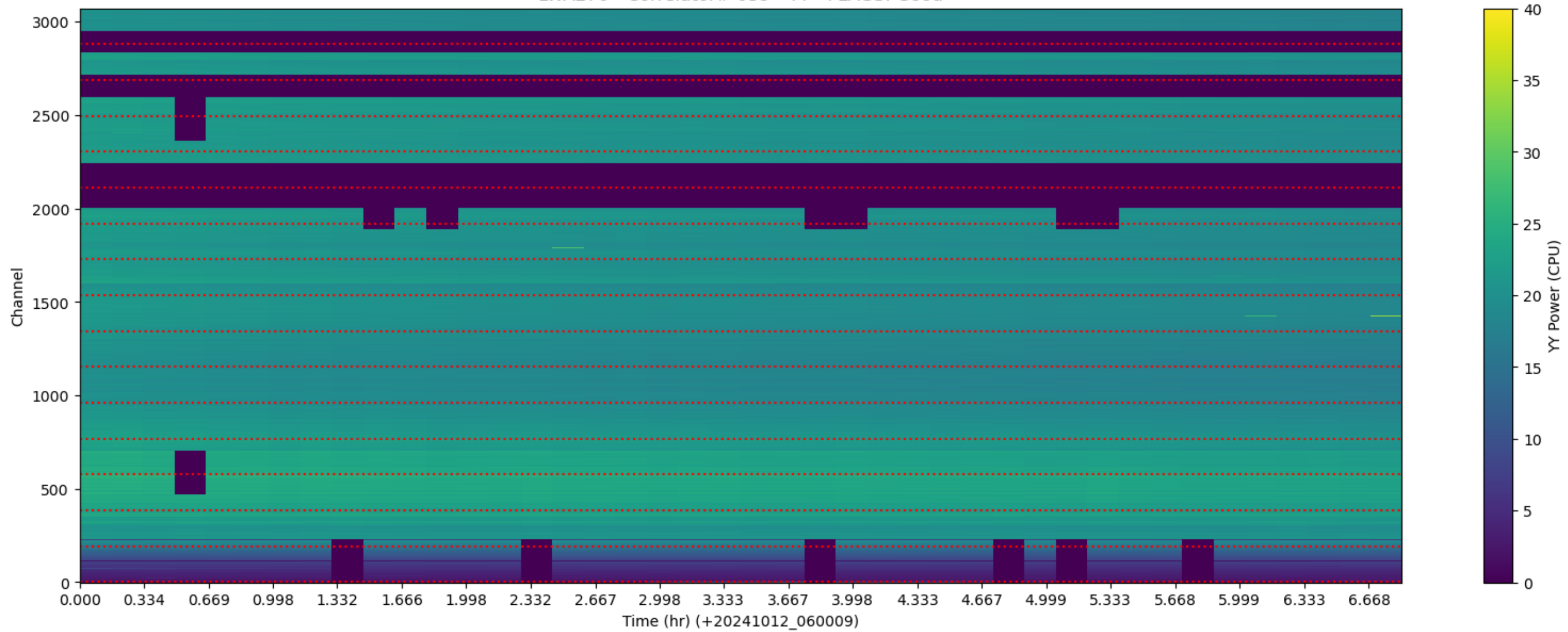
LWA270 - Correlator# 039 - YY - FLAGS: Good
