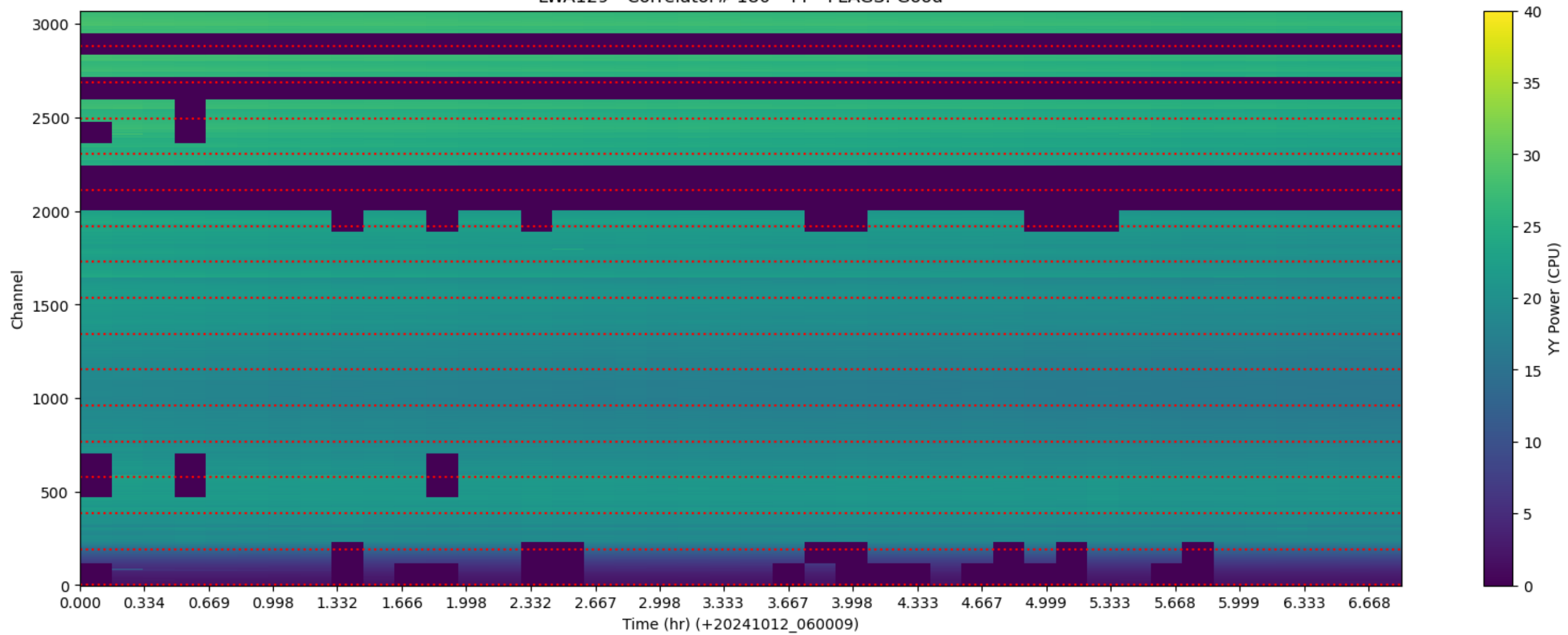
LWA129 - Correlator# 180 - YY - FLAGS: Good
