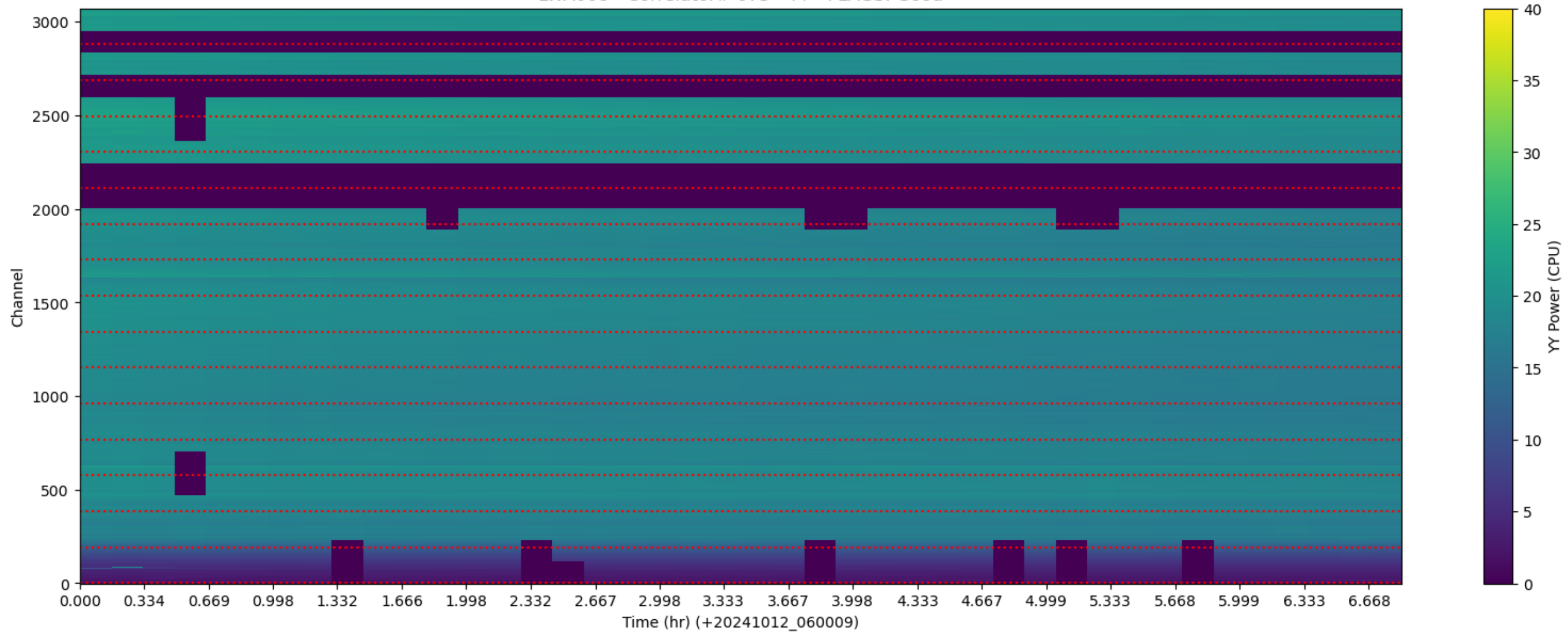
LWA008 - Correlator# 075 - YY - FLAGS: Good
