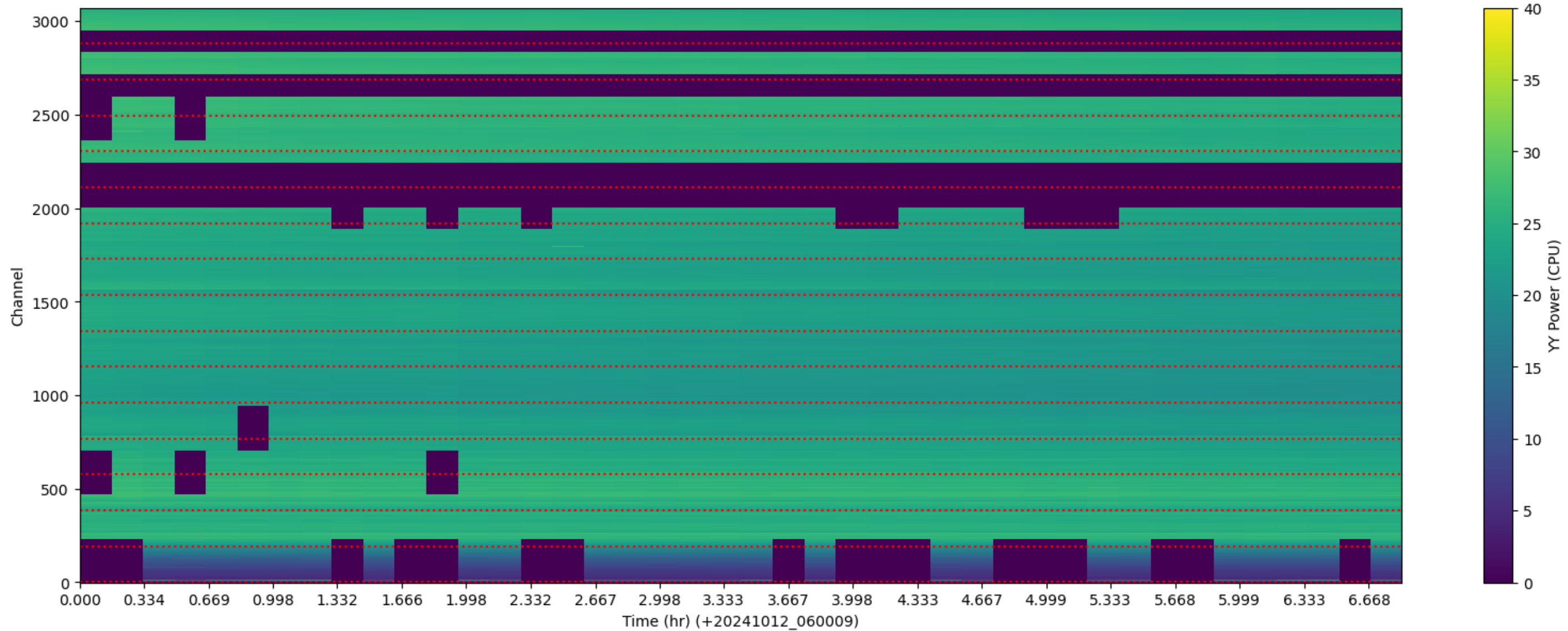
LWA300 - Correlator# 348 - YY - FLAGS: Good
