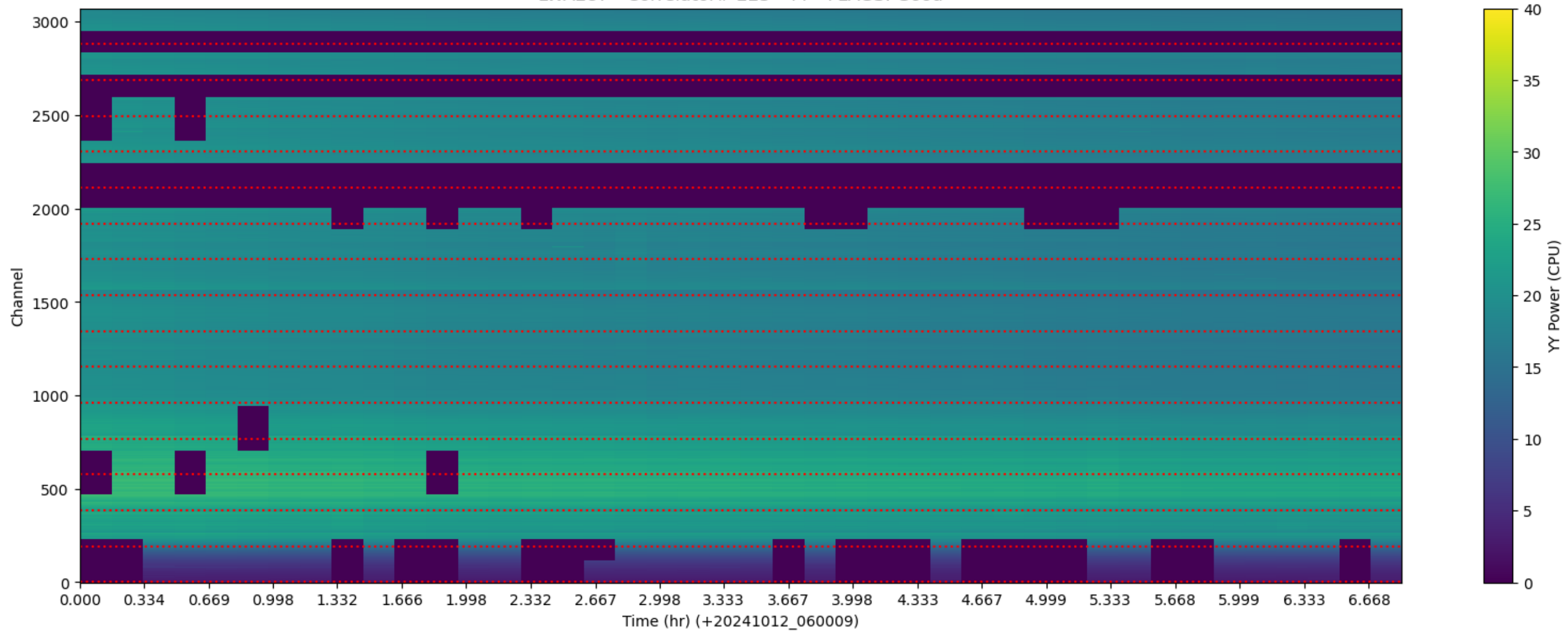
LWA287 - Correlator# 223 - YY - FLAGS: Good
