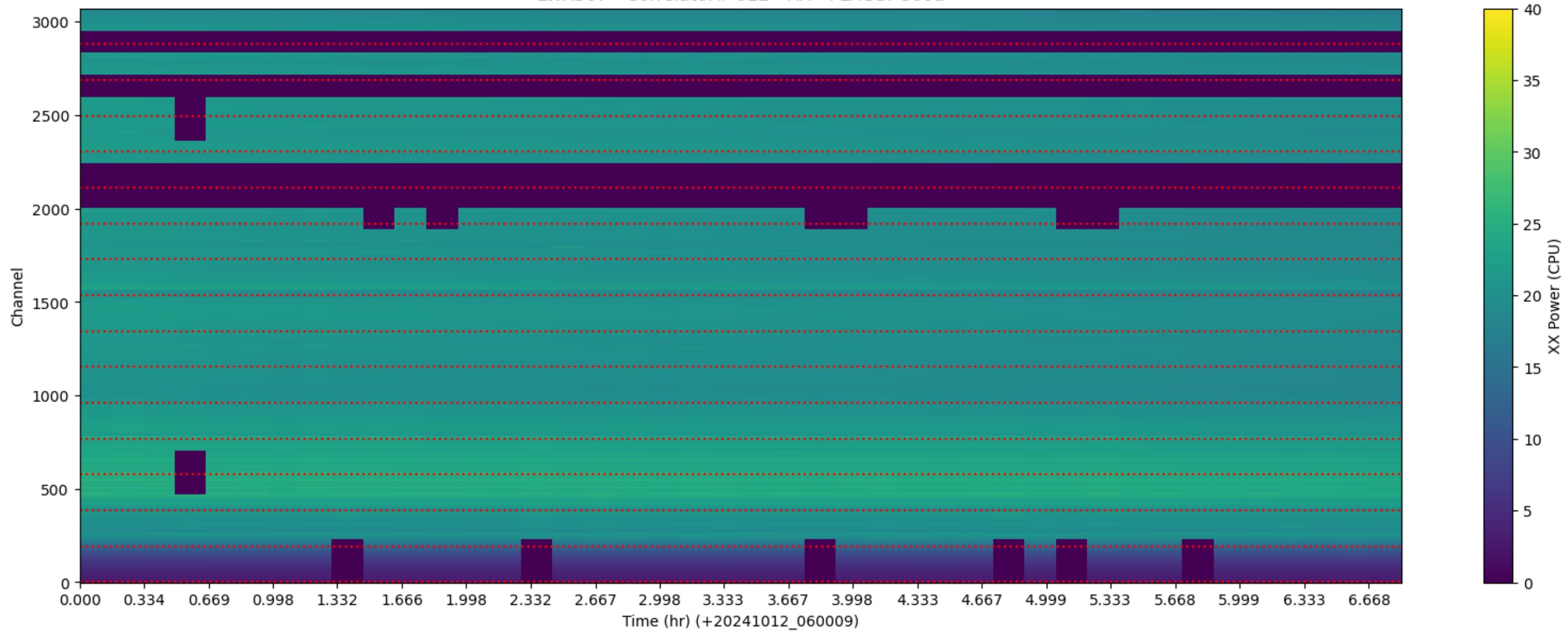
LWA307 - Correlator# 012 - XX - FLAGS: Good
