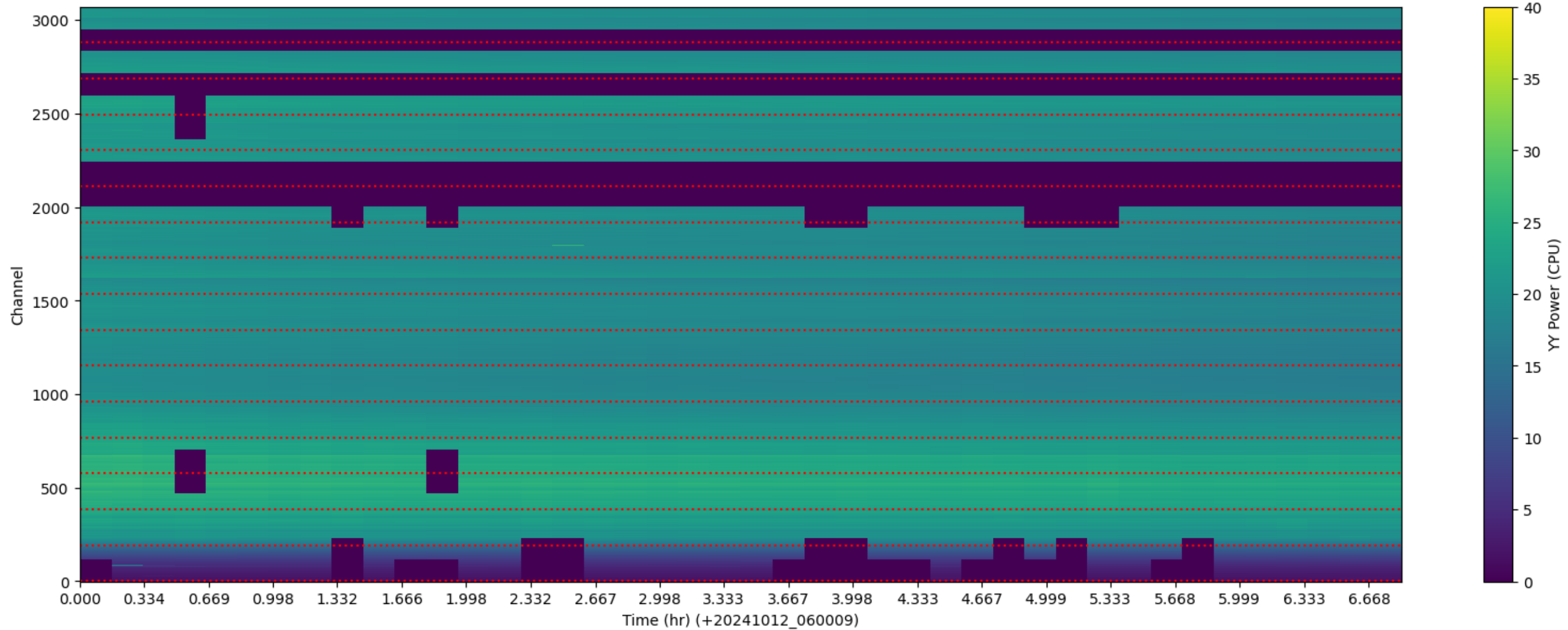
LWA072 - Correlator# 171 - YY - FLAGS: Good
