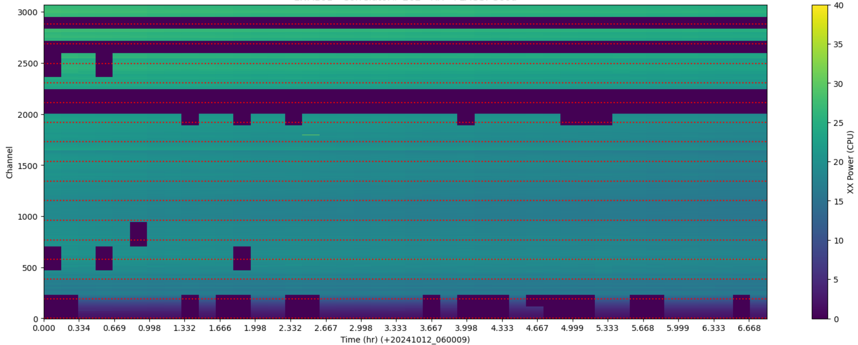
LWA161 - Correlator# 262 - XX - FLAGS: Good
