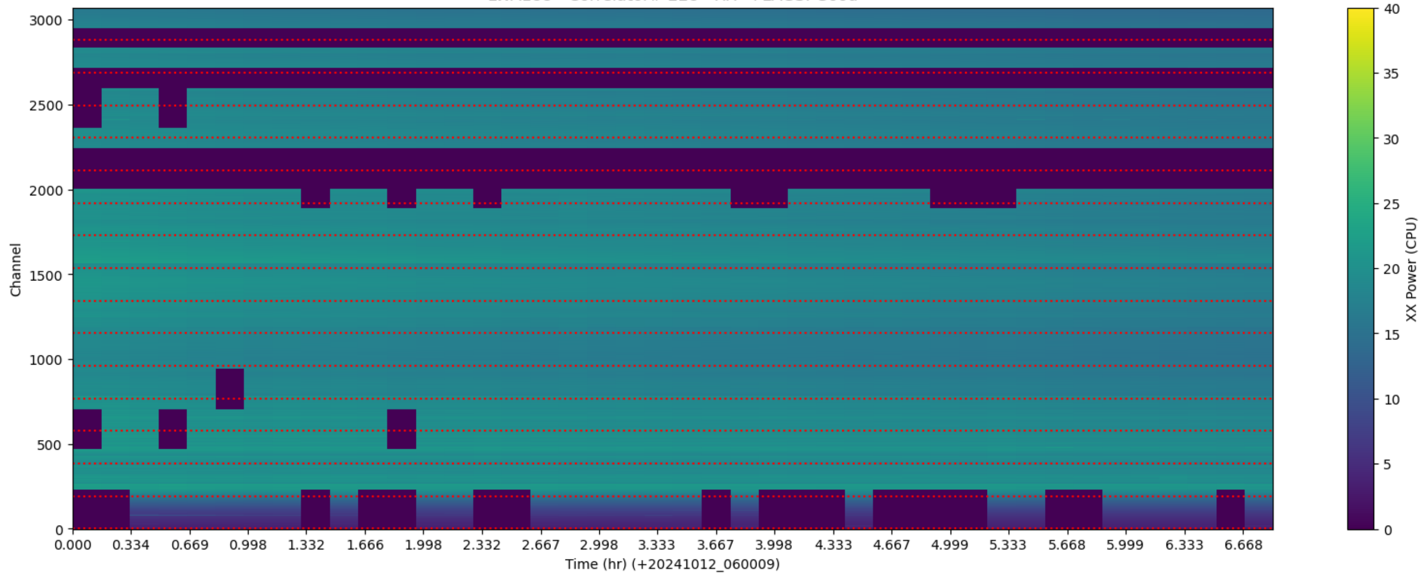
LWA188 - Correlator# 228 - XX - FLAGS: Good
