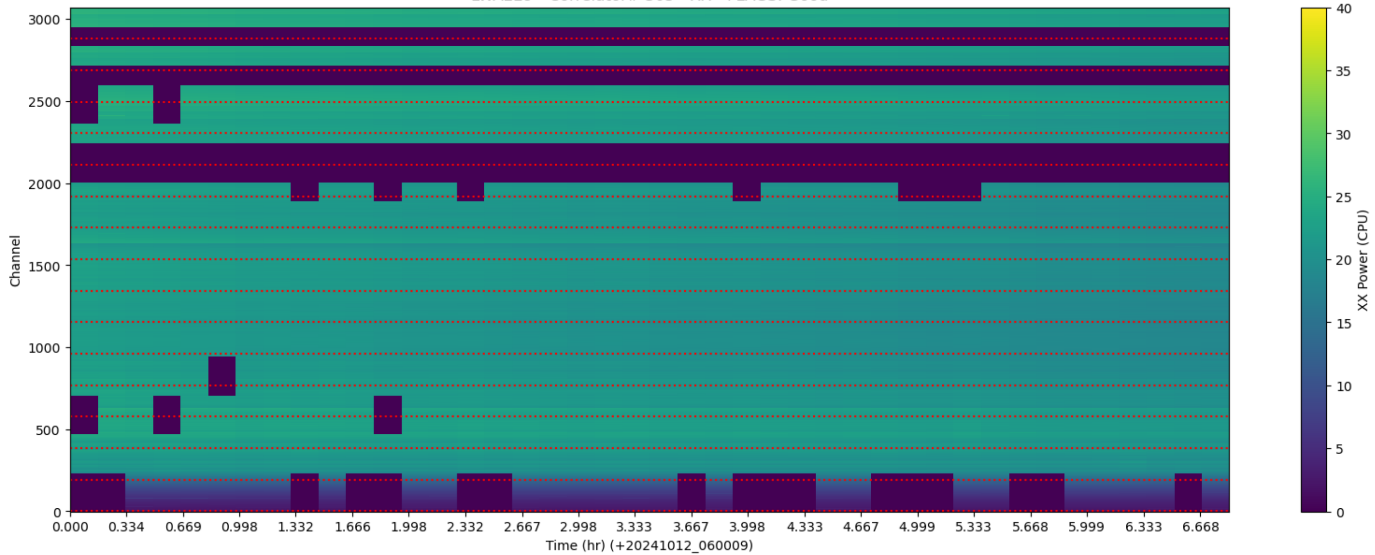
LWA229 - Correlator# 305 - XX - FLAGS: Good
