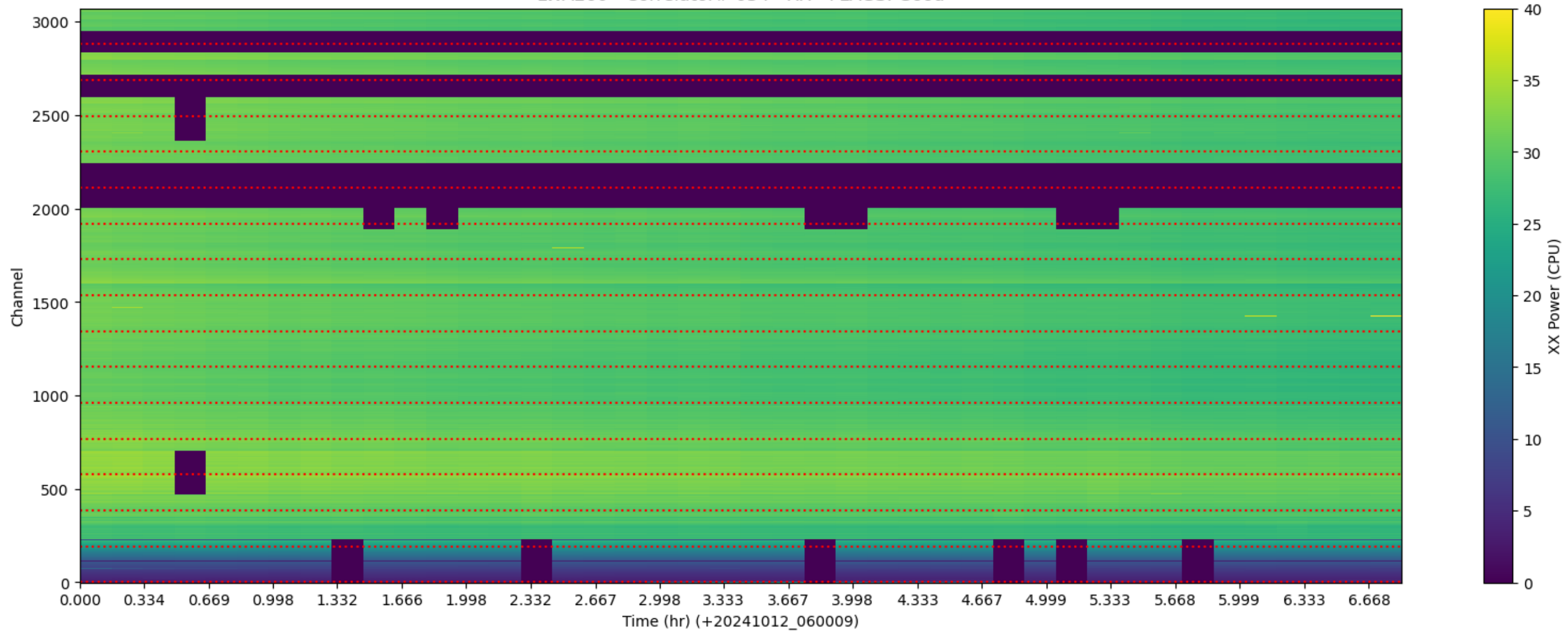
LWA260 - Correlator# 034 - XX - FLAGS: Good
