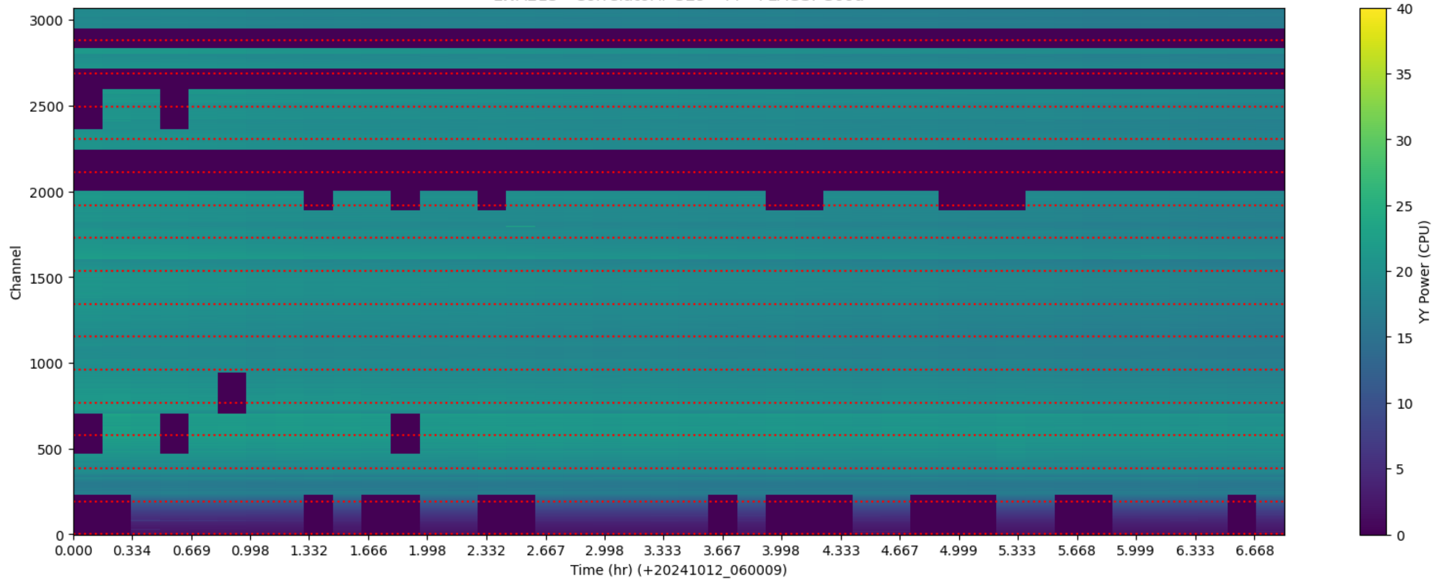
LWA213 - Correlator# 329 - YY - FLAGS: Good
