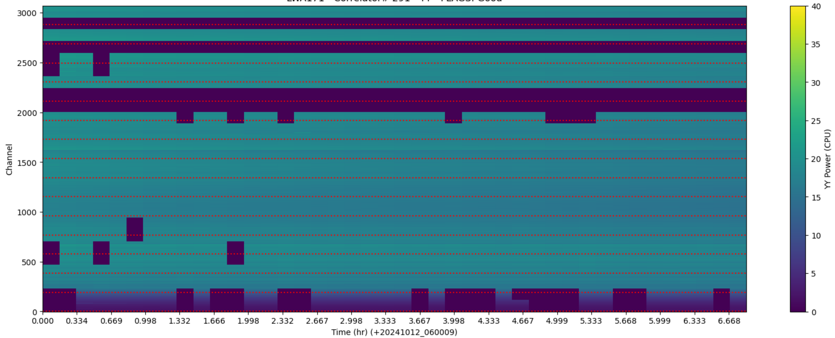
LWA171 - Correlator# 291 - YY - FLAGS: Good
