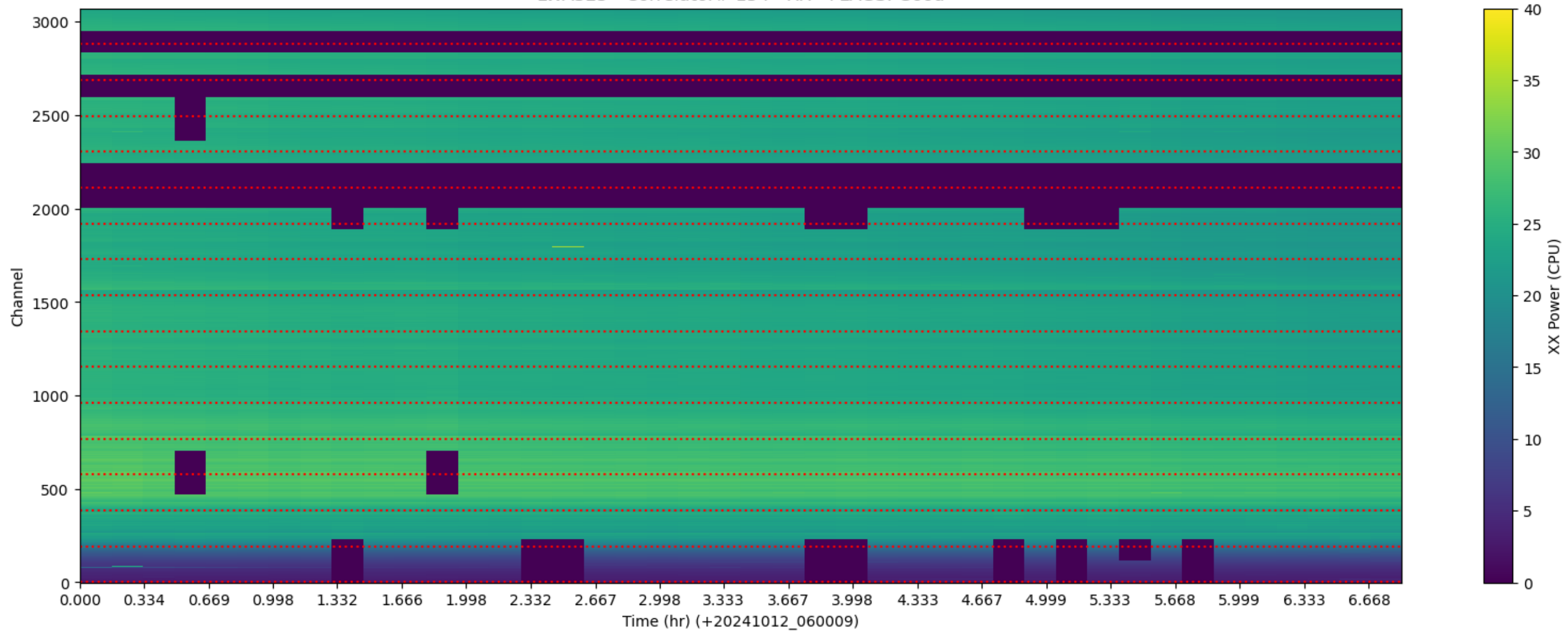
LWA325 - Correlator# 154 - XX - FLAGS: Good
