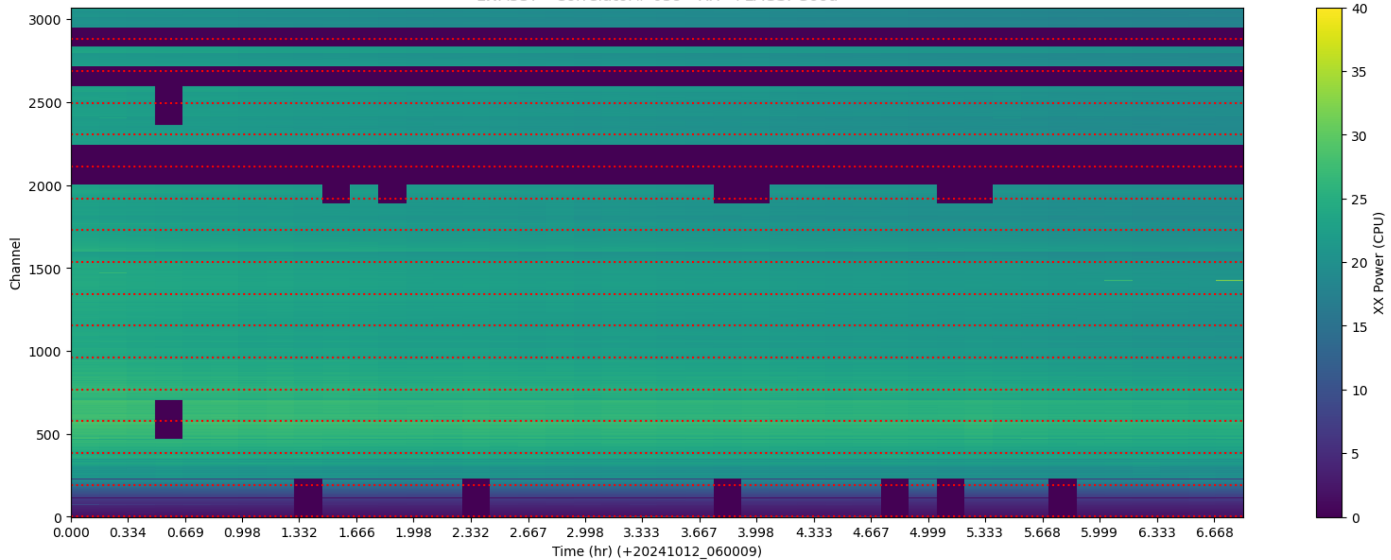
LWA337 - Correlator# 059 - XX - FLAGS: Good
