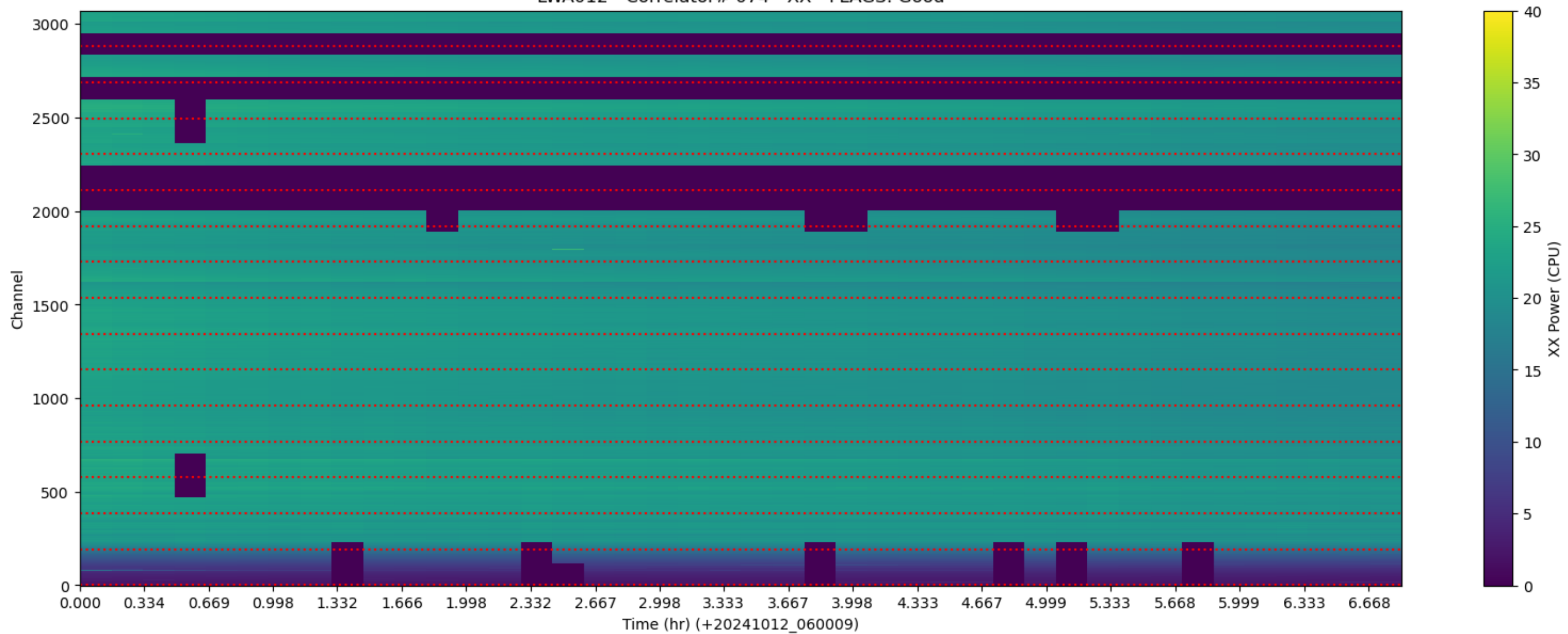
LWA012 - Correlator# 074 - XX - FLAGS: Good
