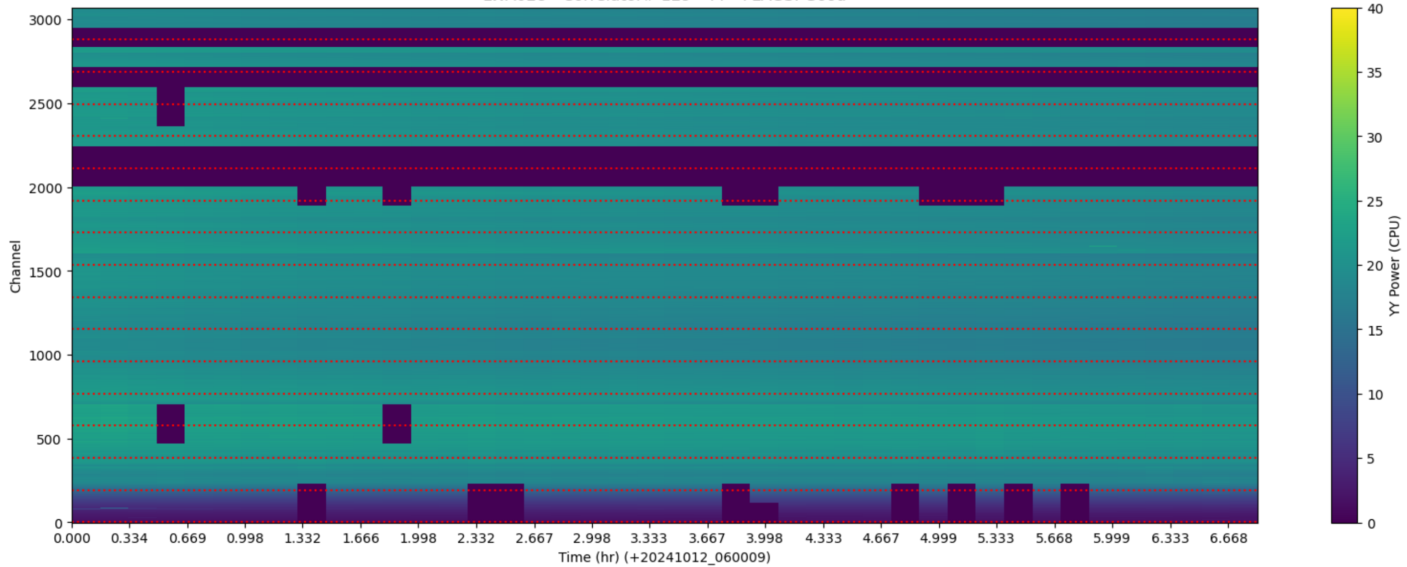
LWA028 - Correlator# 129 - YY - FLAGS: Good
