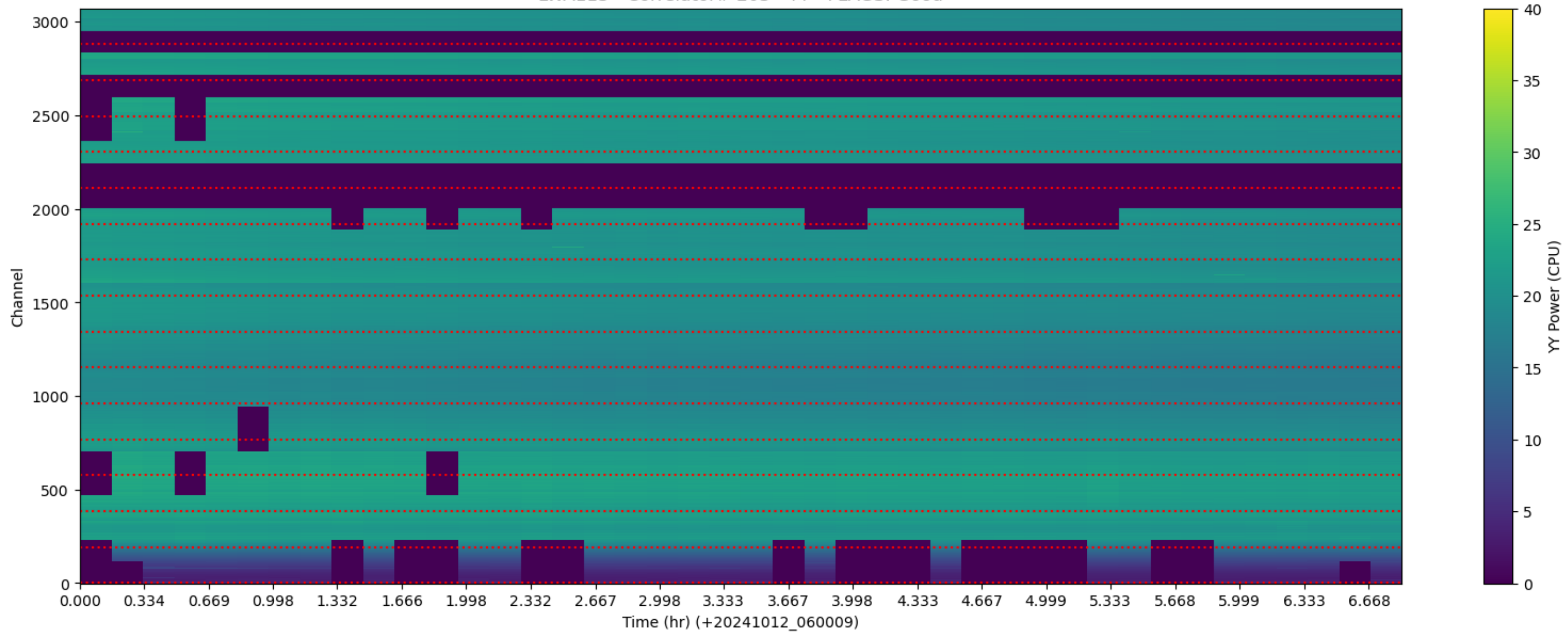
LWA113 - Correlator# 203 - YY - FLAGS: Good
