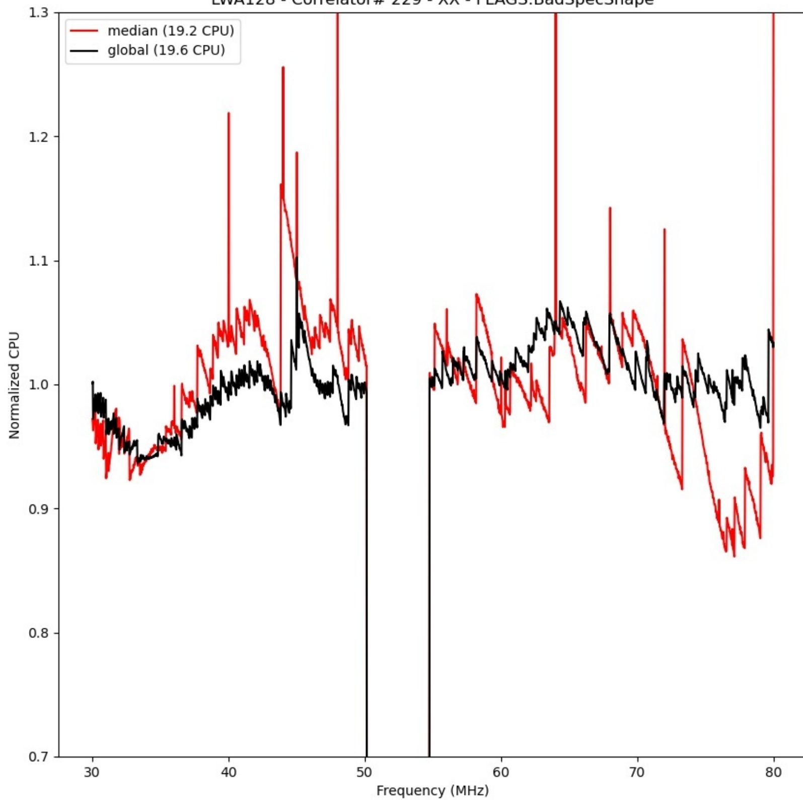
LWA128 - Correlator# 229 - XX - FLAGS:BadSpecShape
