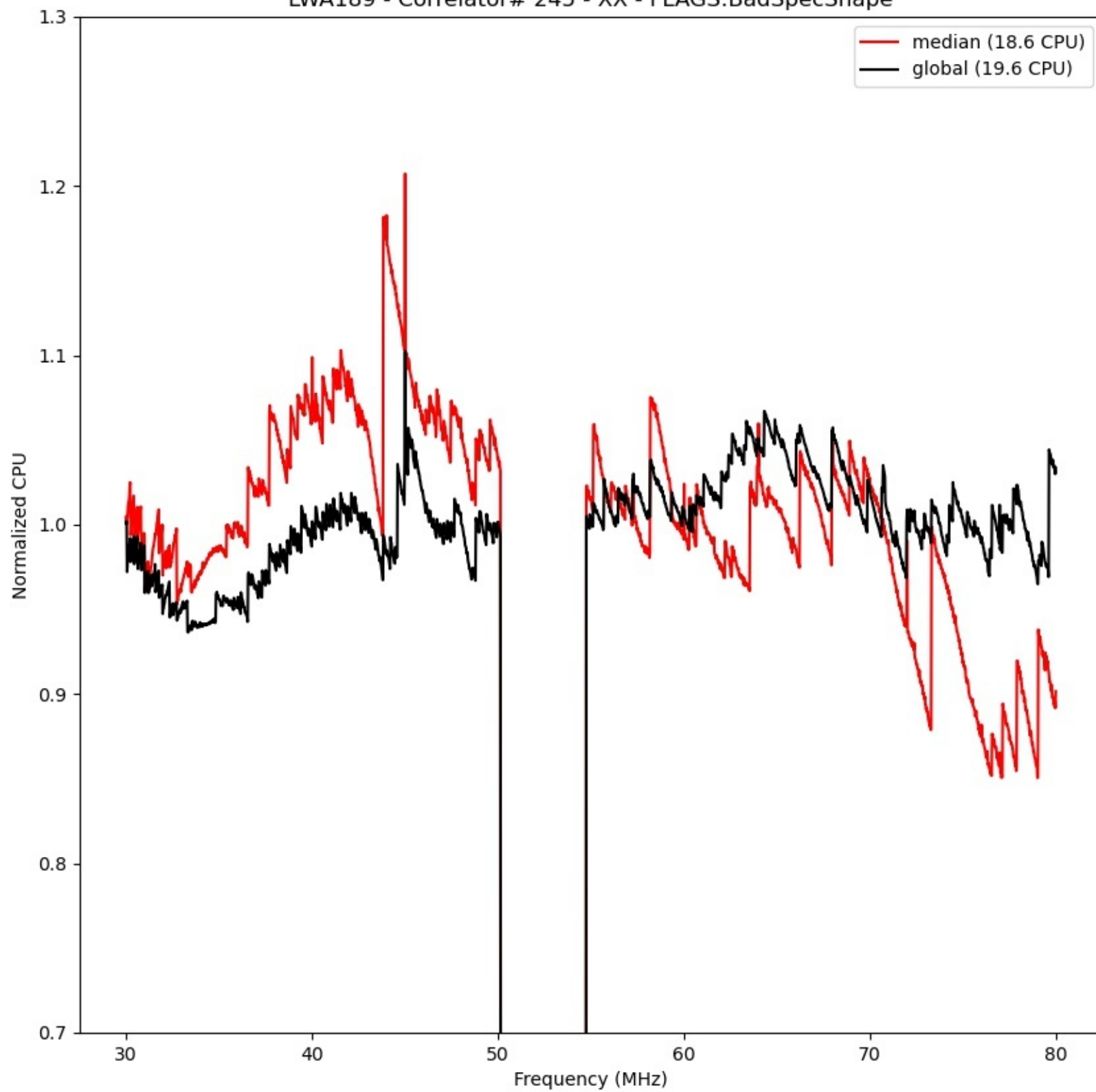
LWA189 - Correlator# 245 - XX - FLAGS:BadSpecShape
