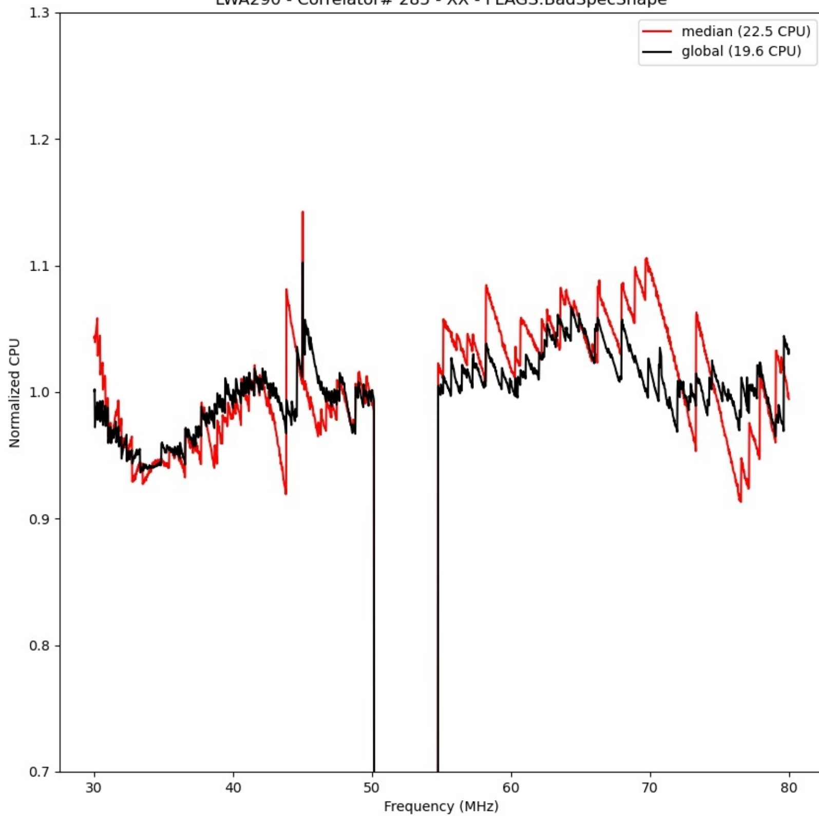
LWA290 - Correlator# 285 - XX - FLAGS:BadSpecShape
