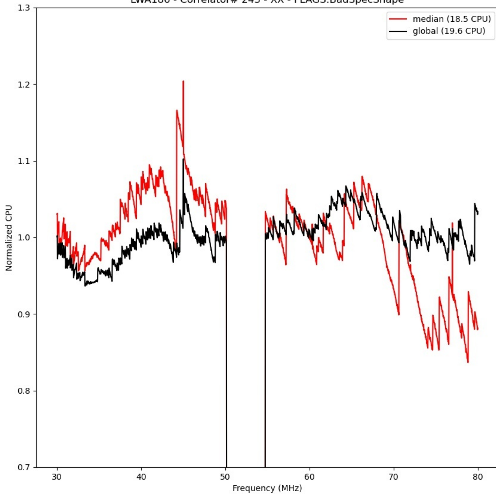
LWA186 - Correlator# 243 - XX - FLAGS:BadSpecShape
