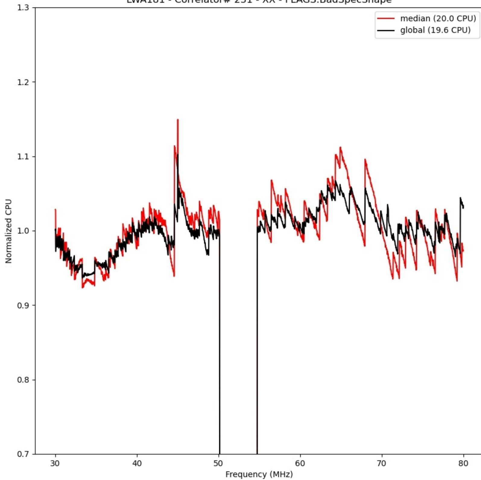
LWA181 - Correlator# 231 - XX - FLAGS:BadSpecShape
