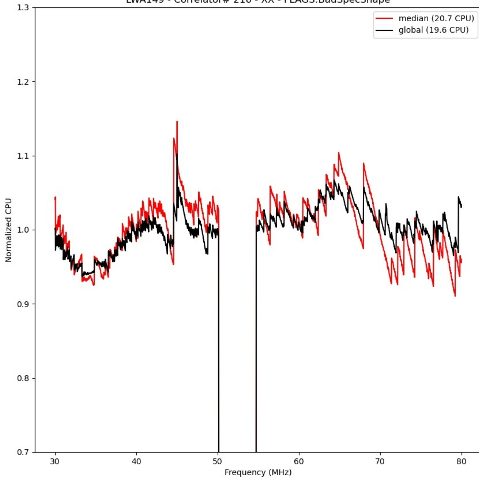
LWA149 - Correlator# 216 - XX - FLAGS:BadSpecShape
