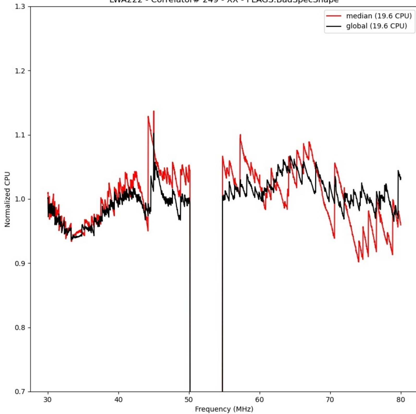
LWA222 - Correlator# 249 - XX - FLAGS:BadSpecShape
