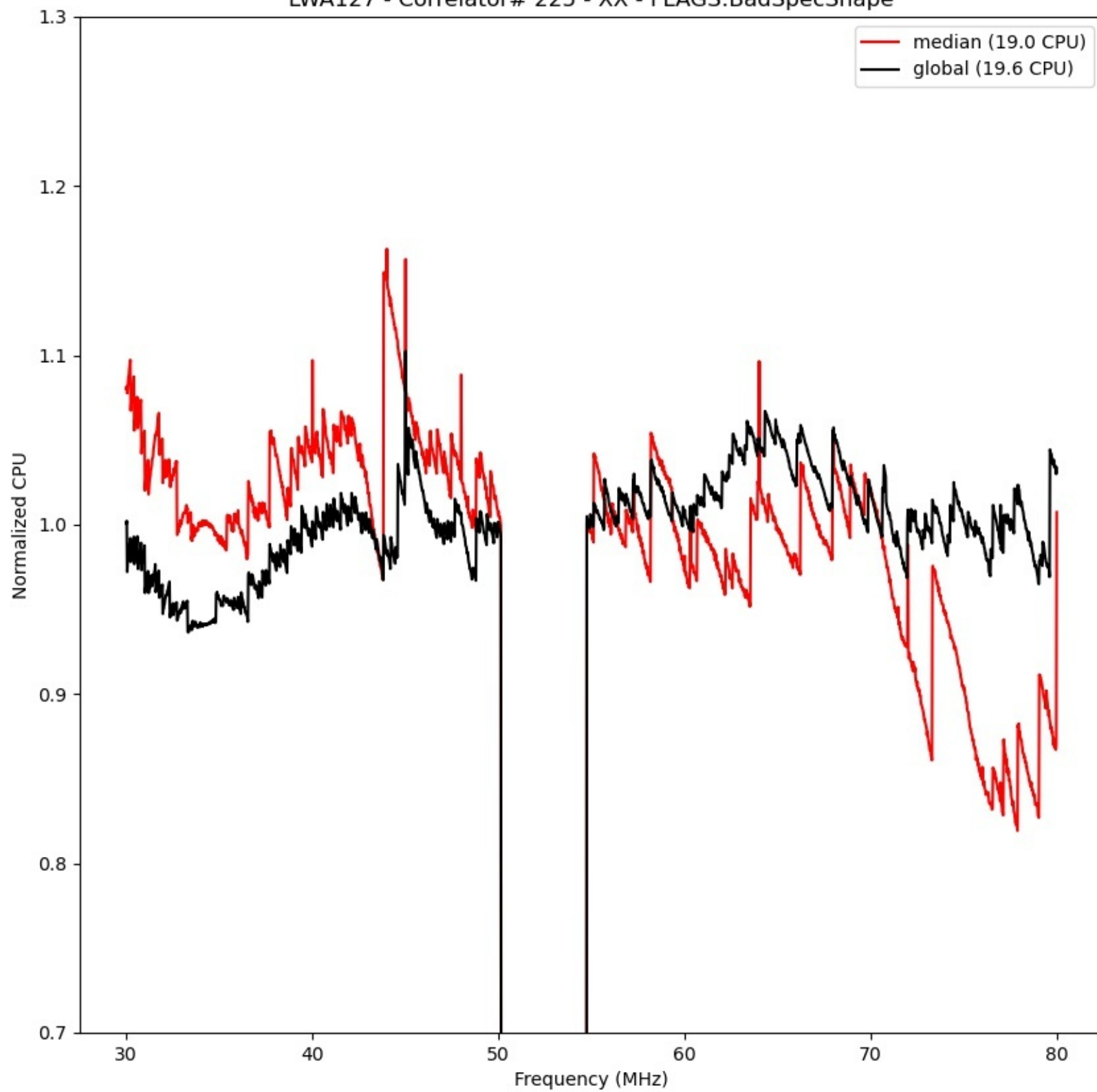
LWA127 - Correlator# 225 - XX - FLAGS:BadSpecShape
