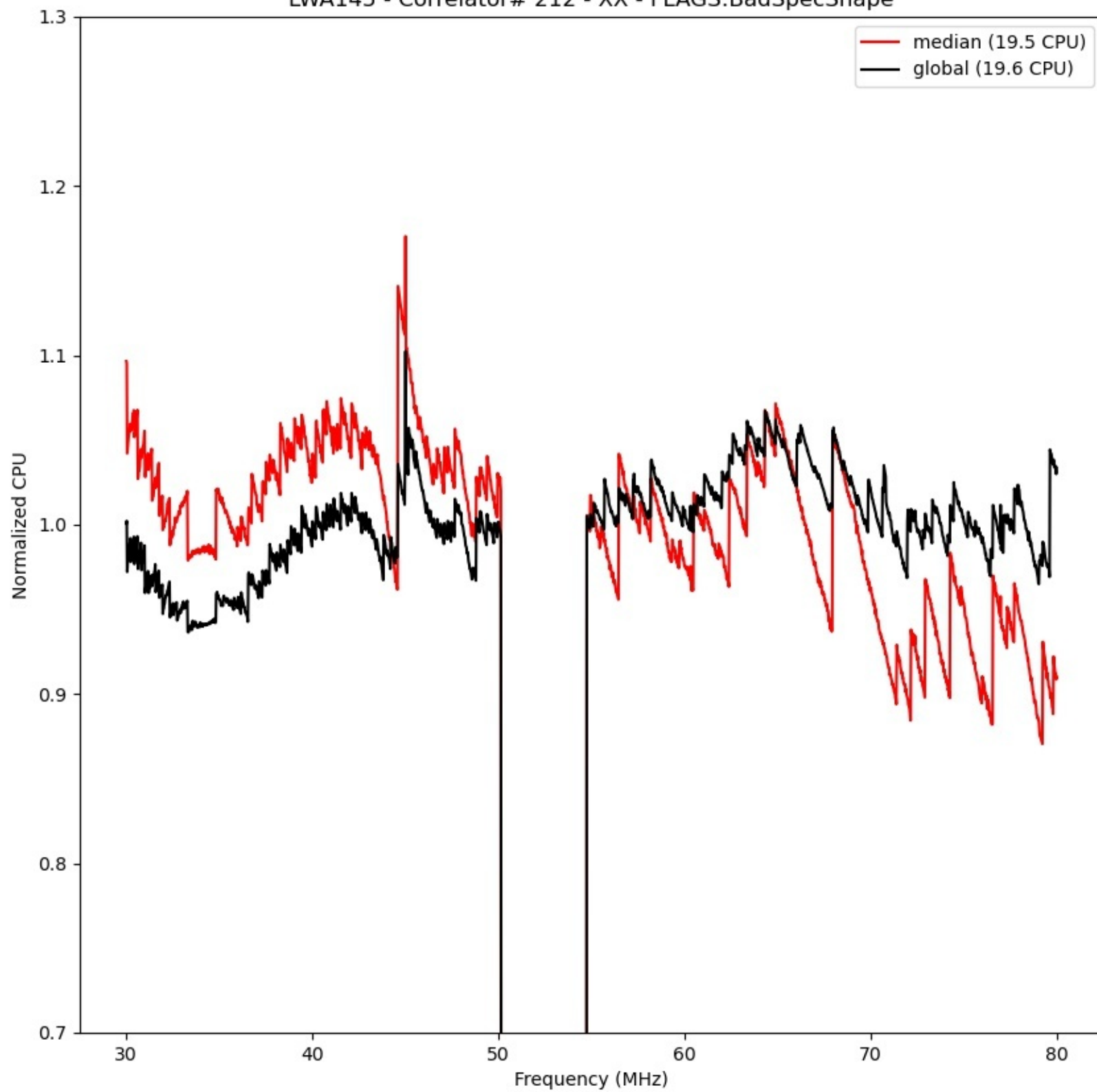
LWA145 - Correlator# 212 - XX - FLAGS:BadSpecShape
