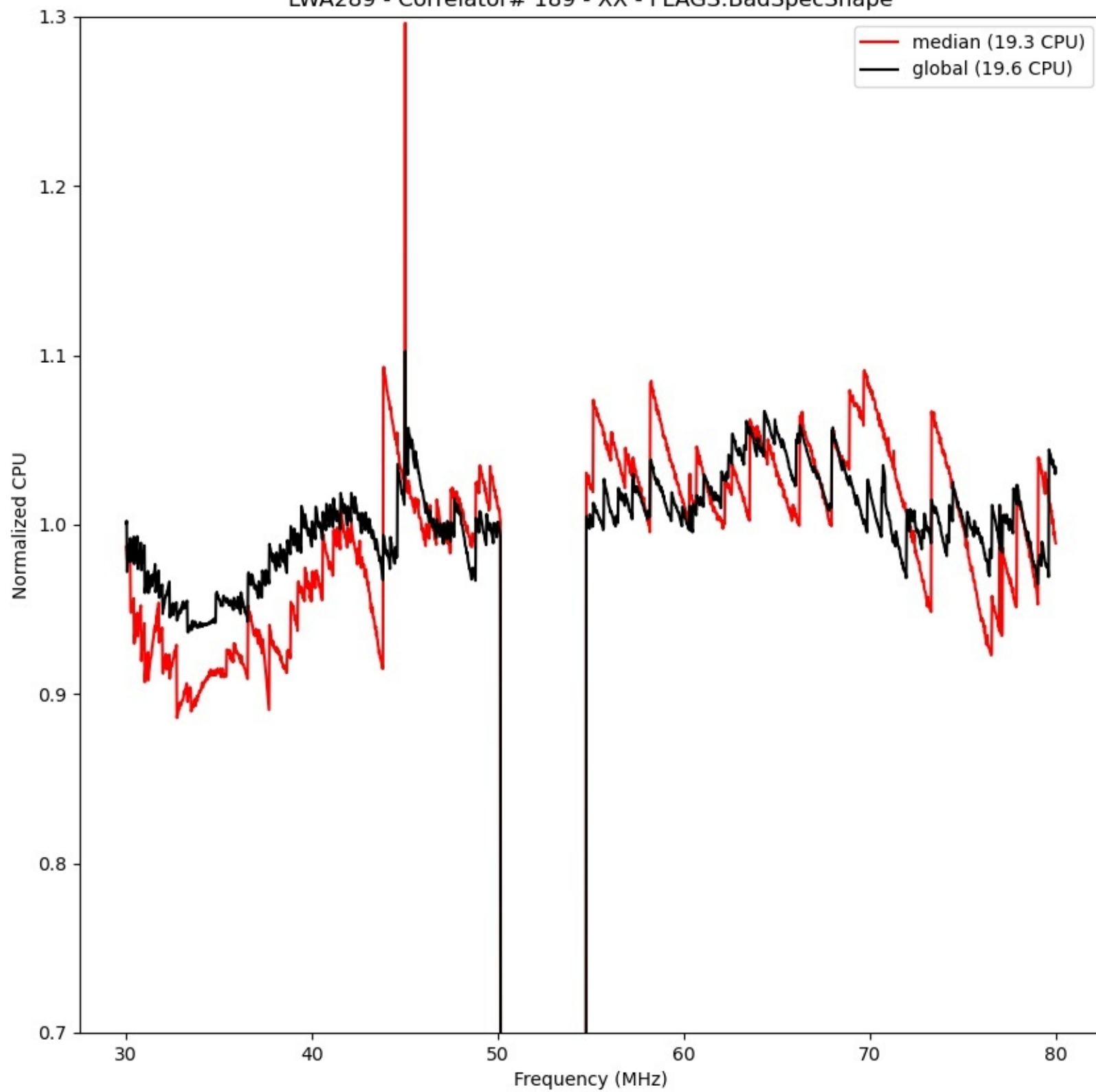
LWA289 - Correlator# 189 - XX - FLAGS:BadSpecShape
