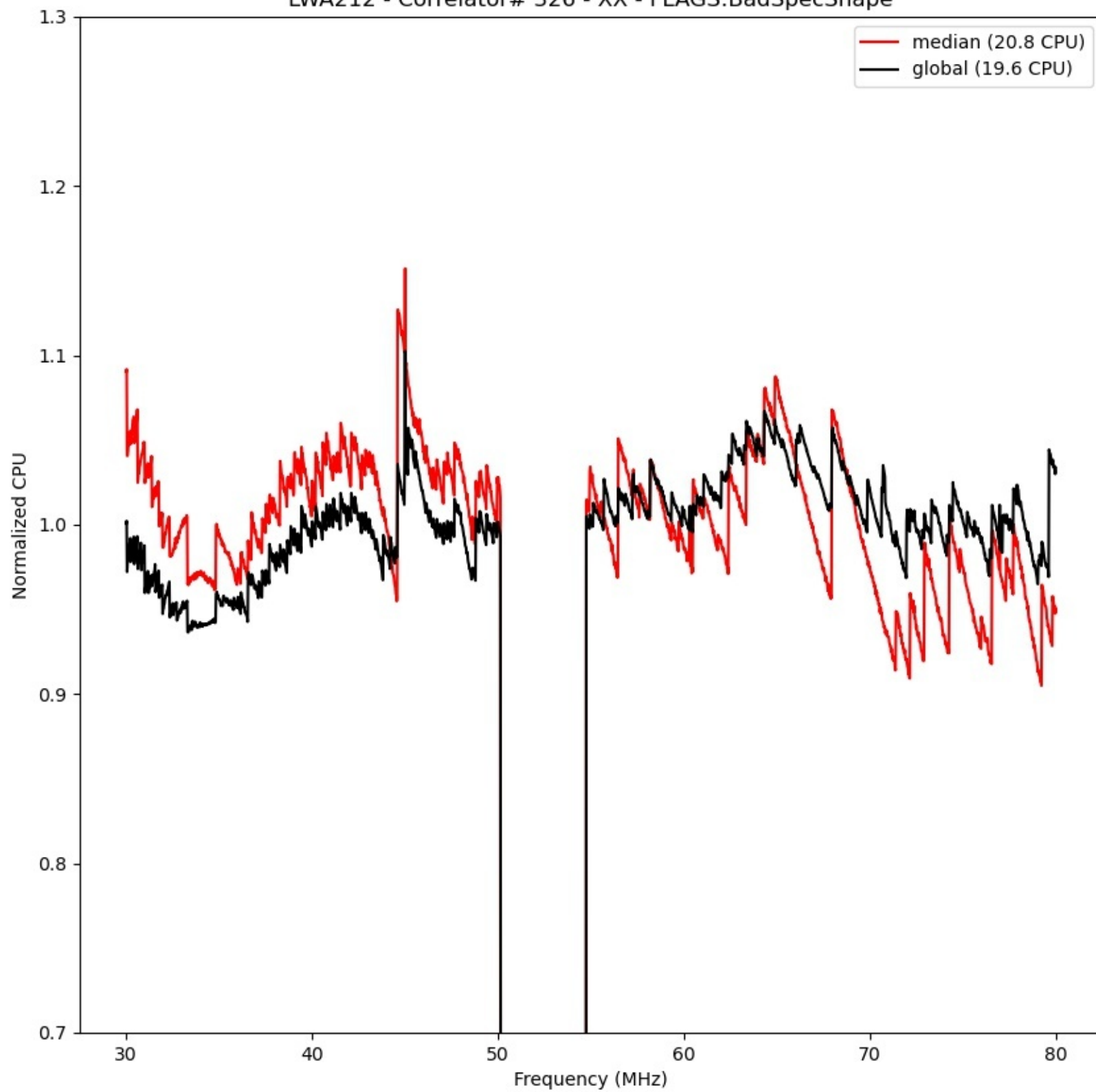
LWA212 - Correlator# 326 - XX - FLAGS:BadSpecShape
