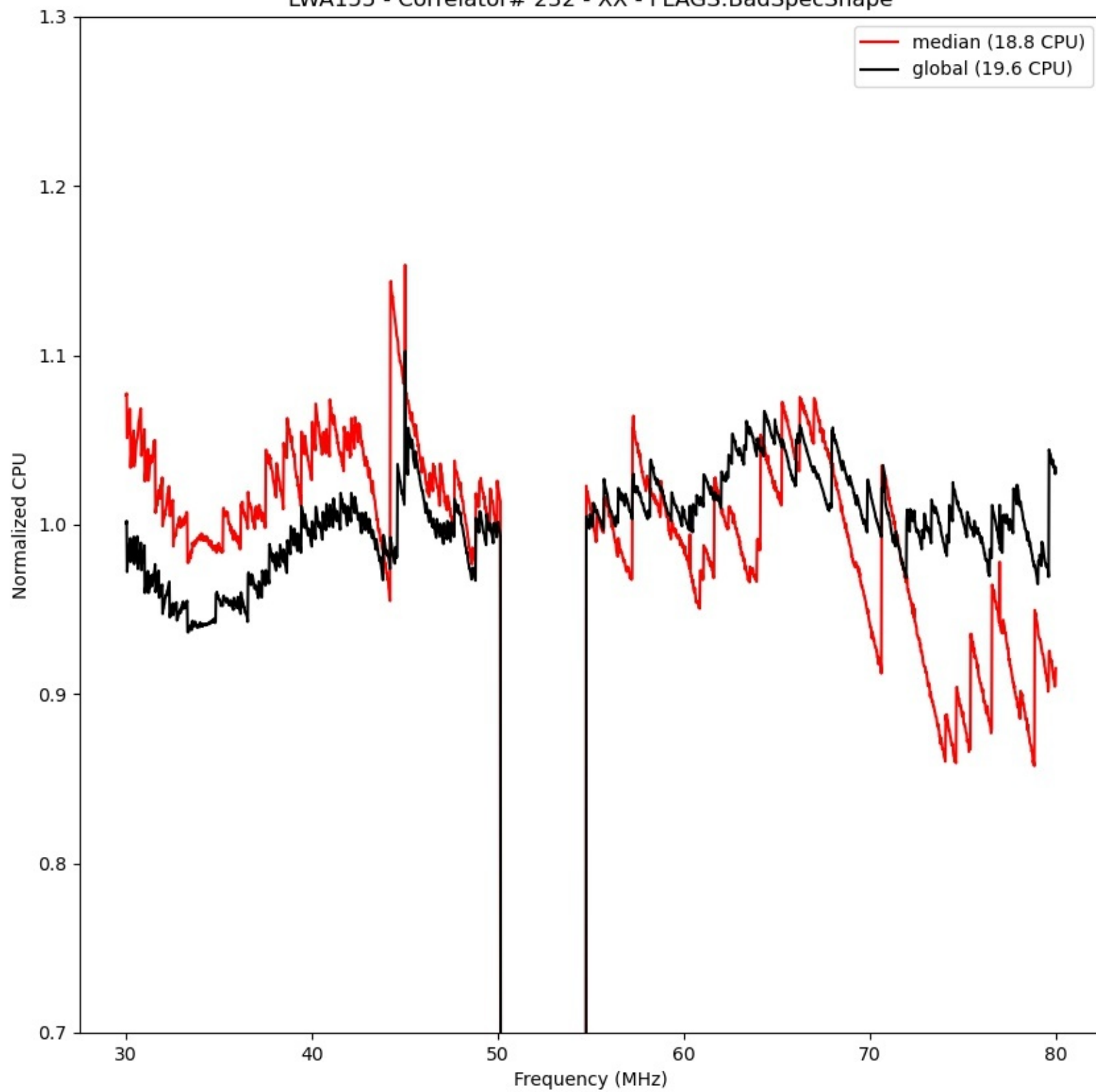
LWA155 - Correlator# 232 - XX - FLAGS:BadSpecShape
