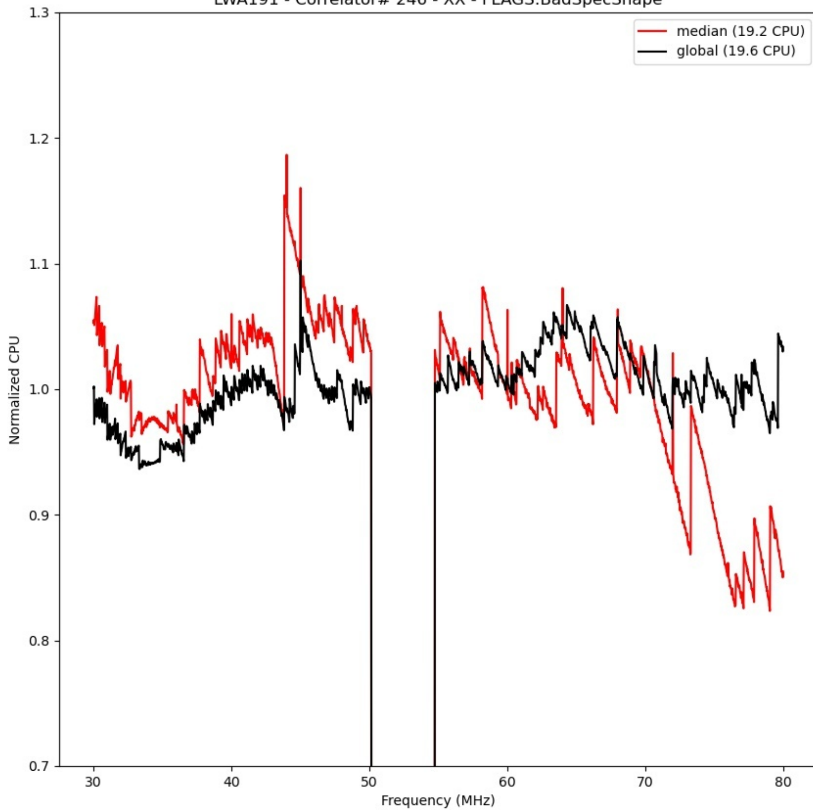
LWA191 - Correlator# 246 - XX - FLAGS:BadSpecShape
