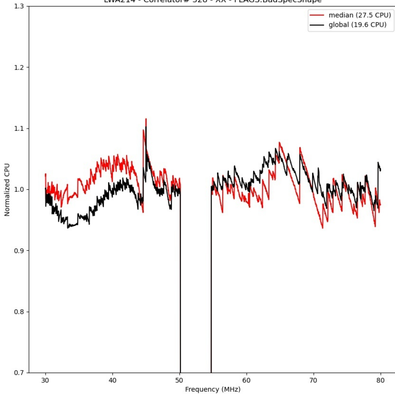
LWA214 - Correlator# 328 - XX - FLAGS:BadSpecShape
