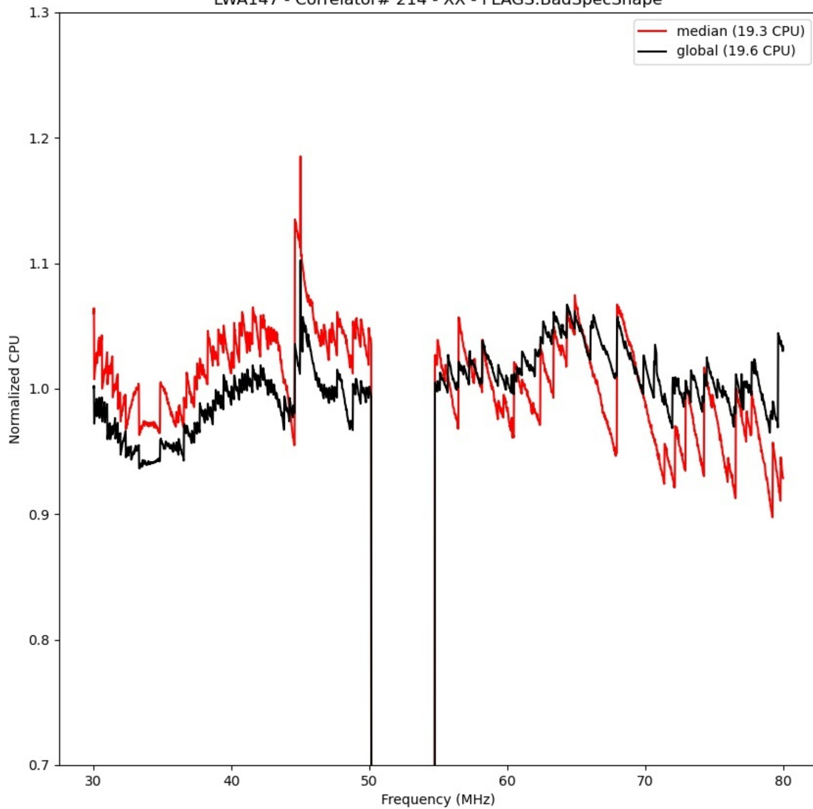
LWA147 - Correlator# 214 - XX - FLAGS:BadSpecShape
