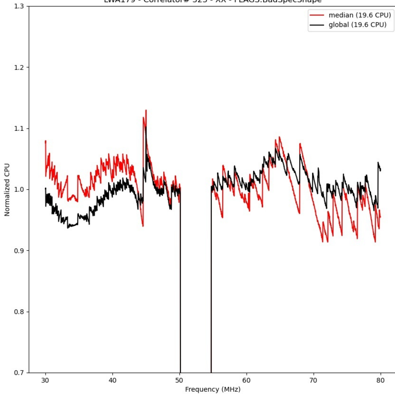
LWA179 - Correlator# 323 - XX - FLAGS:BadSpecShape
