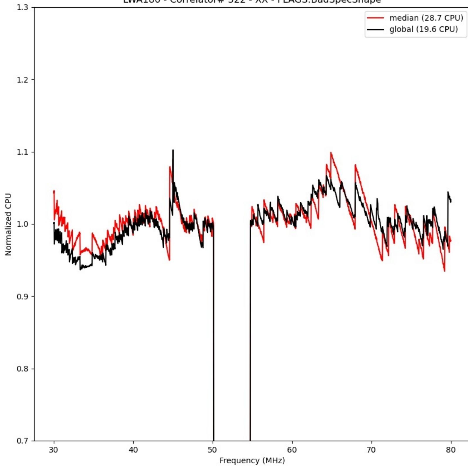
LWA180 - Correlator# 322 - XX - FLAGS:BadSpecShape
