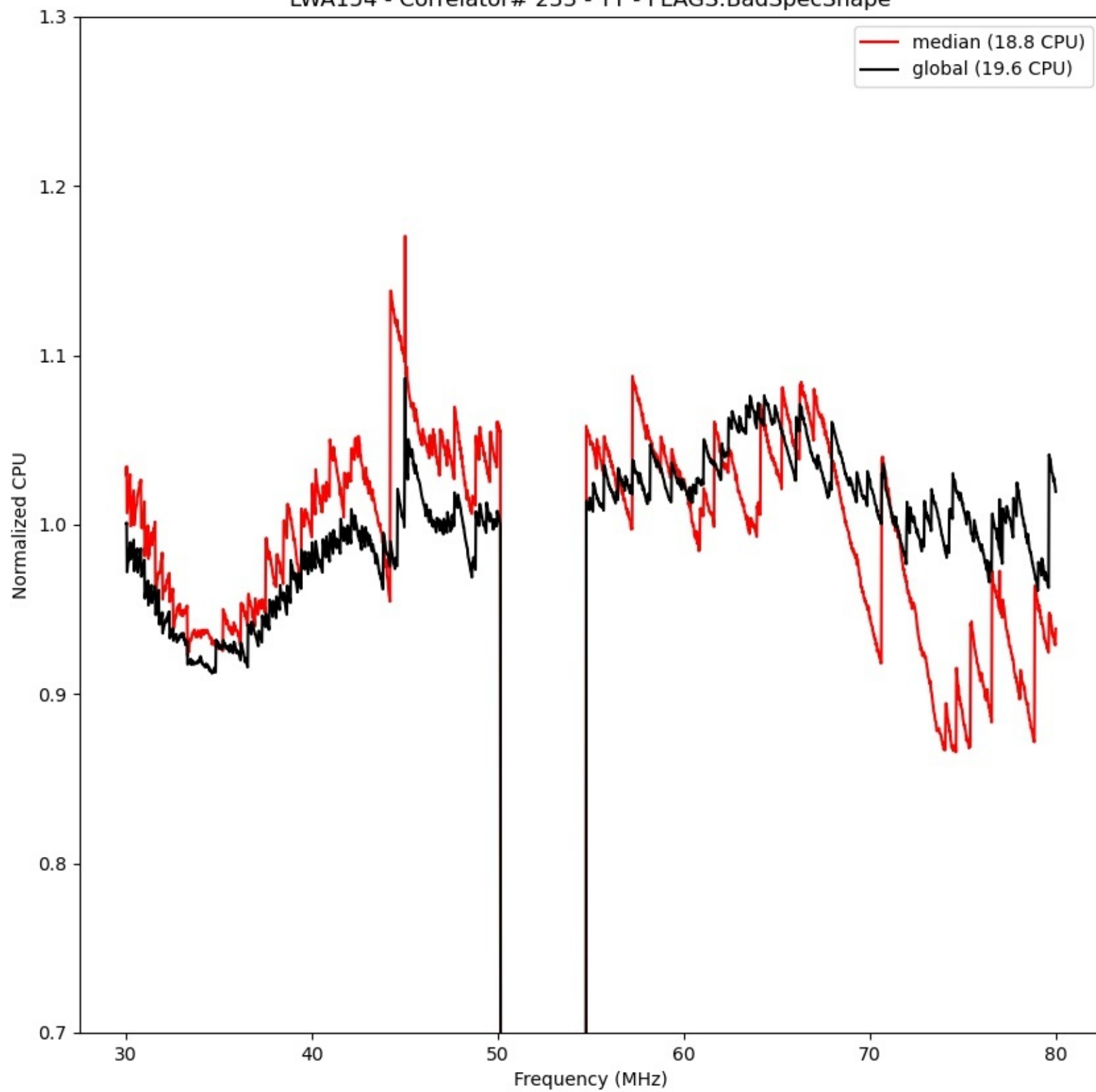
LWA154 - Correlator# 233 - YY - FLAGS:BadSpecShape
