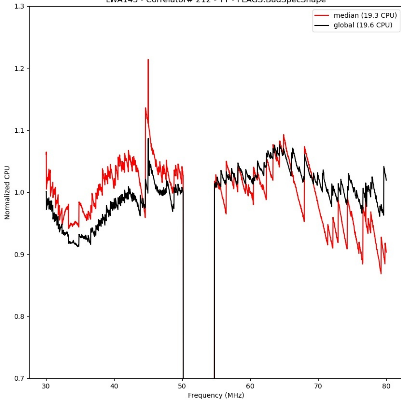
LWA145 - Correlator# 212 - YY - FLAGS:BadSpecShape
