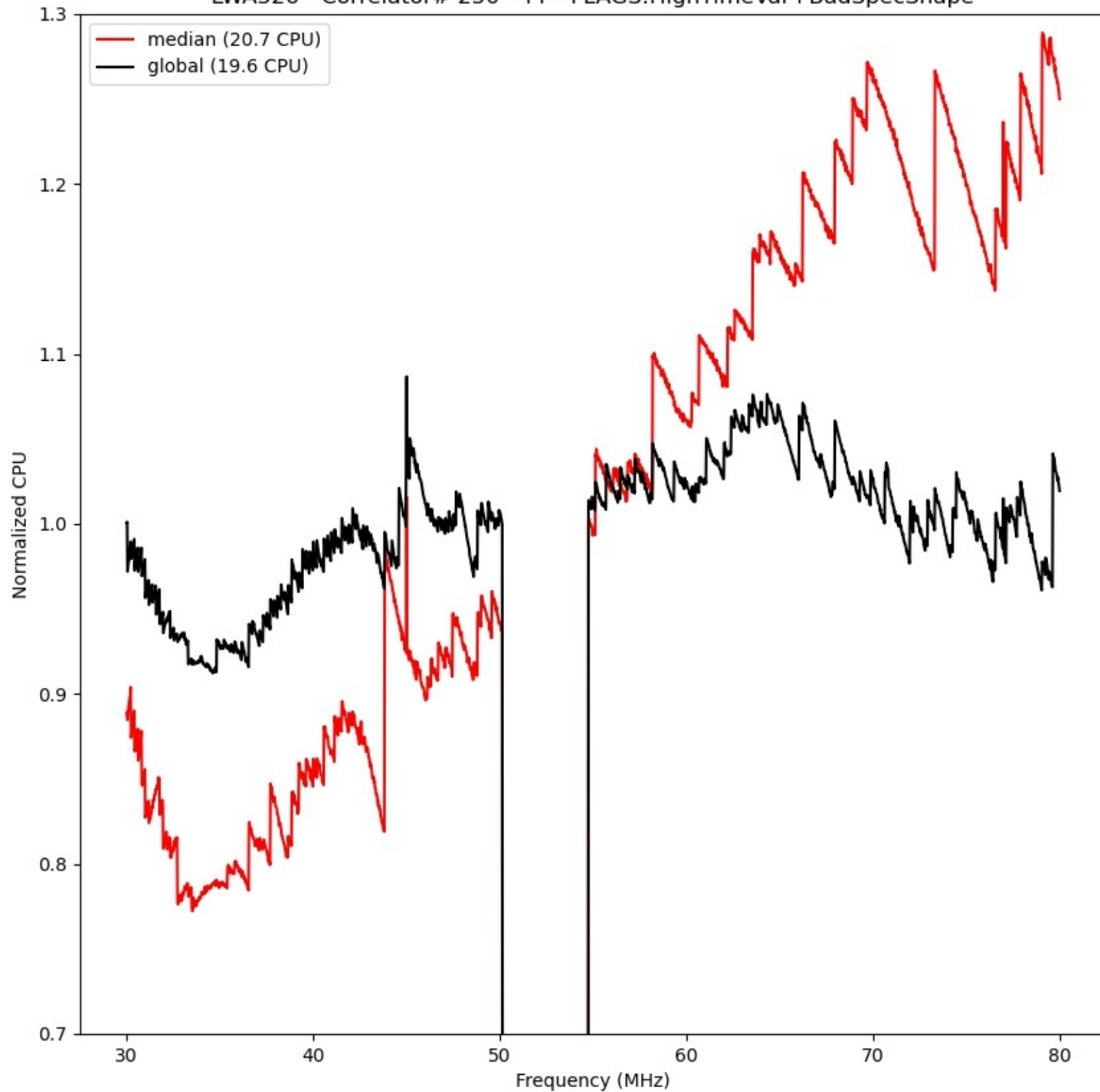
LWA326 - Correlator# 250 - YY - FLAGS:HighTimeVar+BadSpecShape
