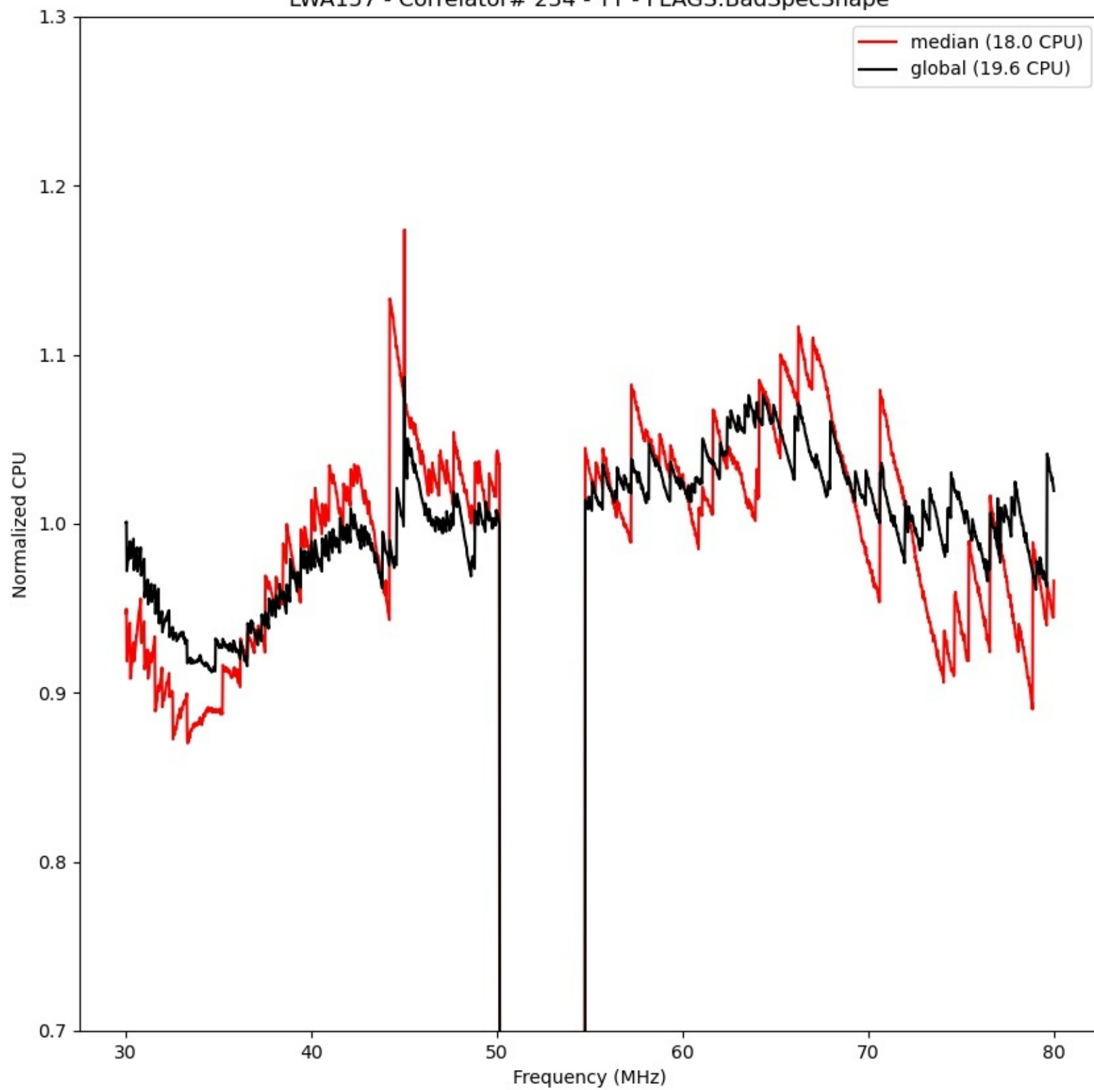
LWA157 - Correlator# 234 - YY - FLAGS:BadSpecShape
