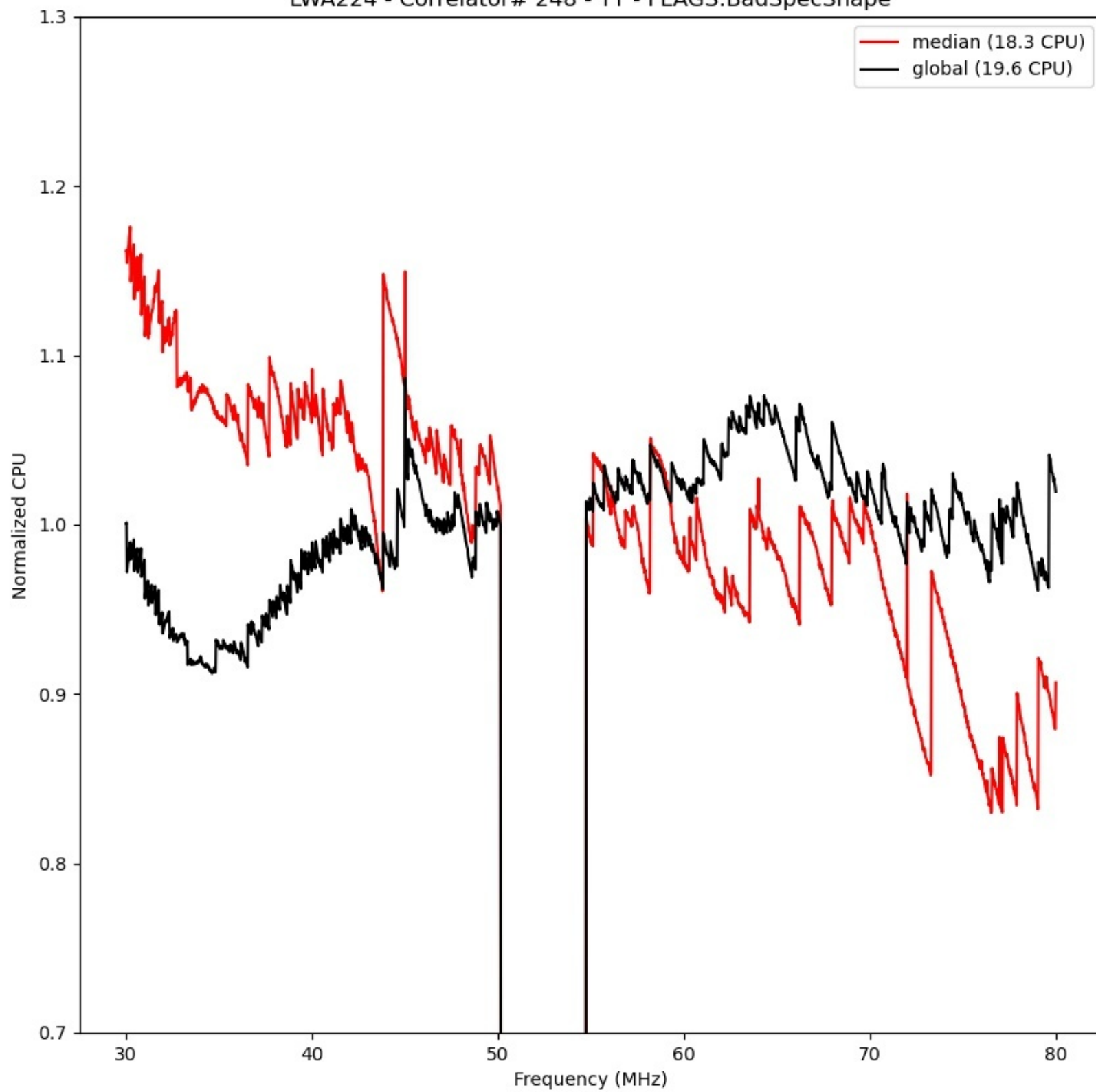
LWA224 - Correlator# 248 - YY - FLAGS:BadSpecShape
