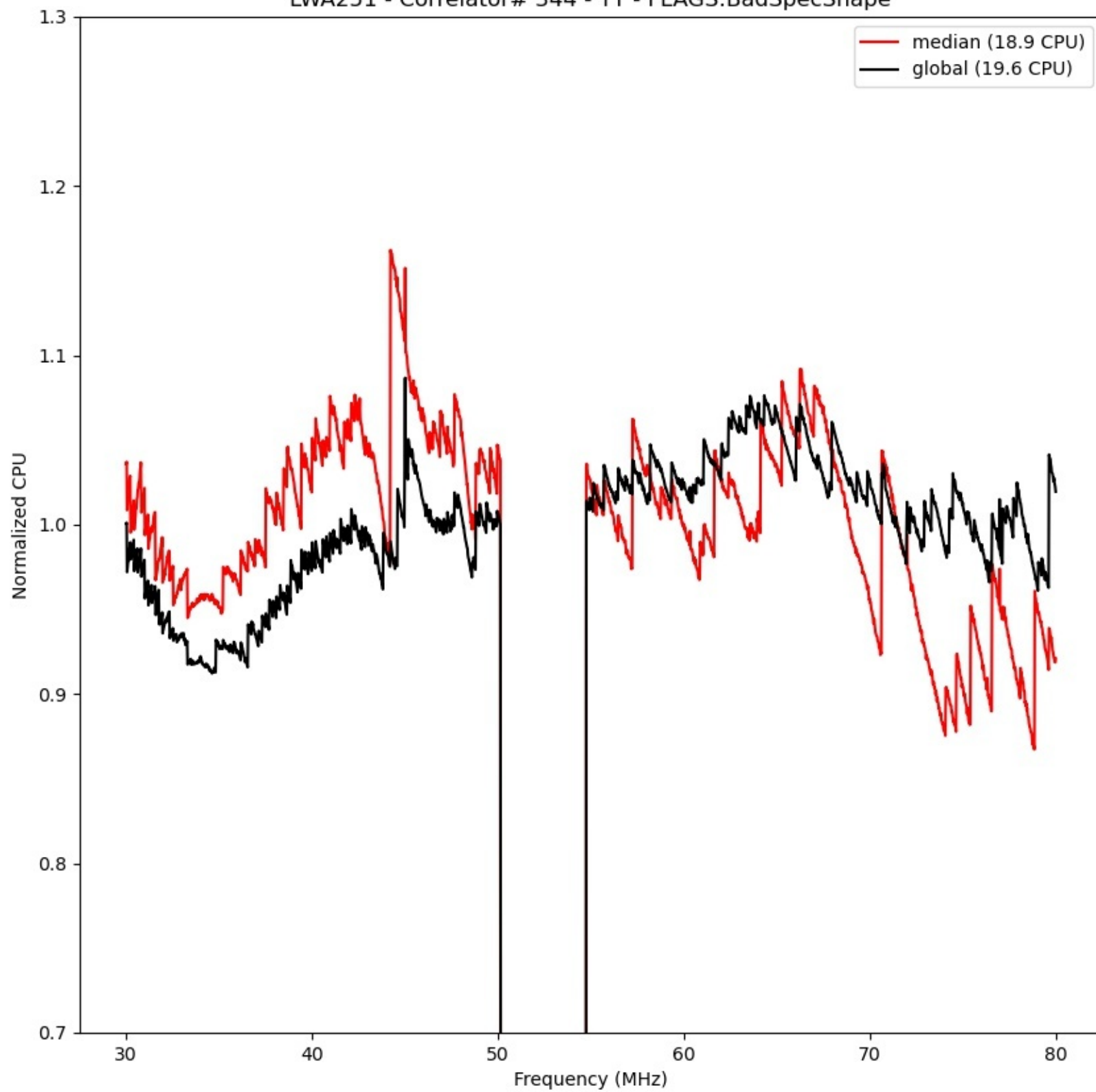
LWA251 - Correlator# 344 - YY - FLAGS:BadSpecShape
