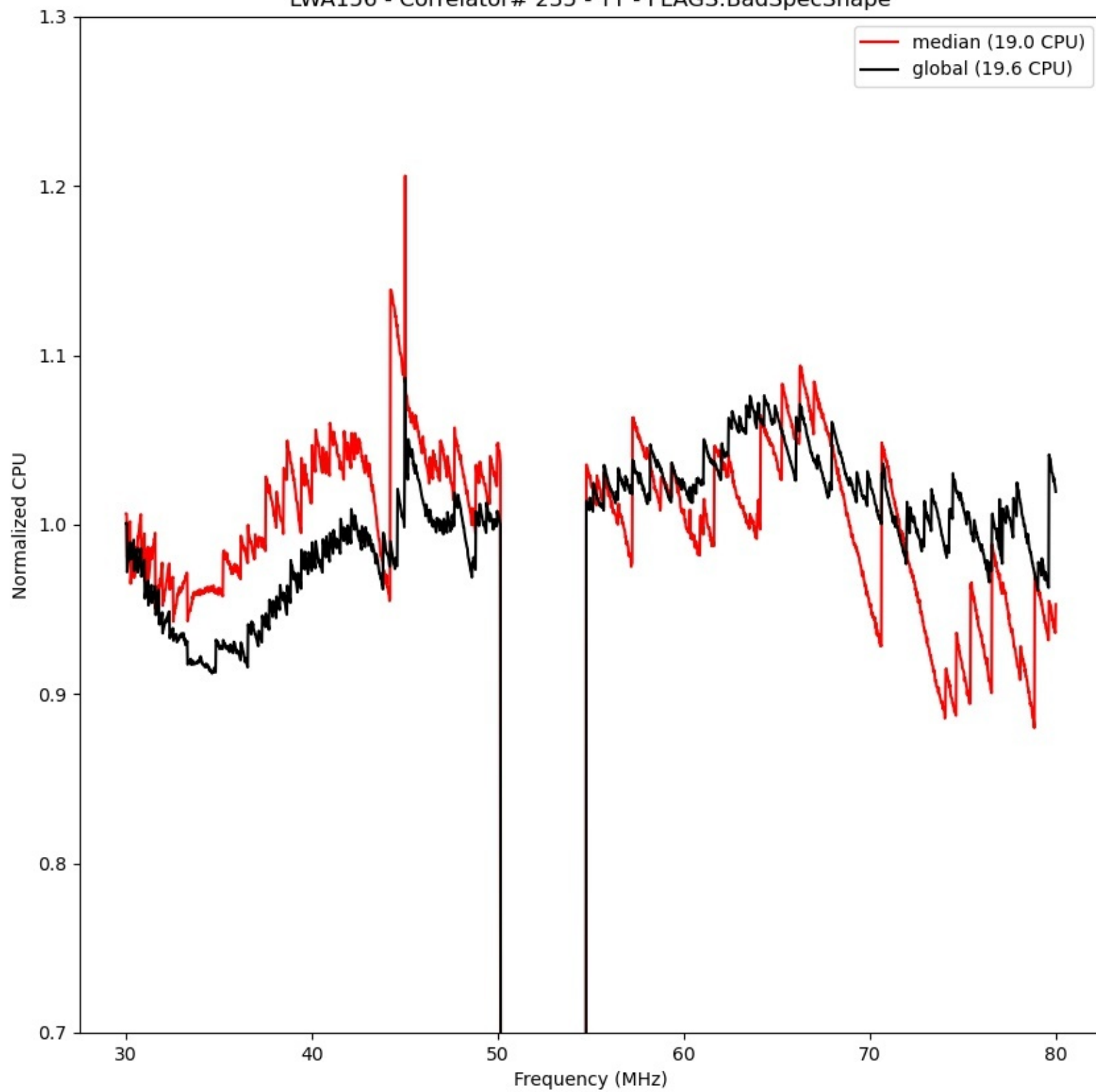
LWA156 - Correlator# 235 - YY - FLAGS:BadSpecShape
