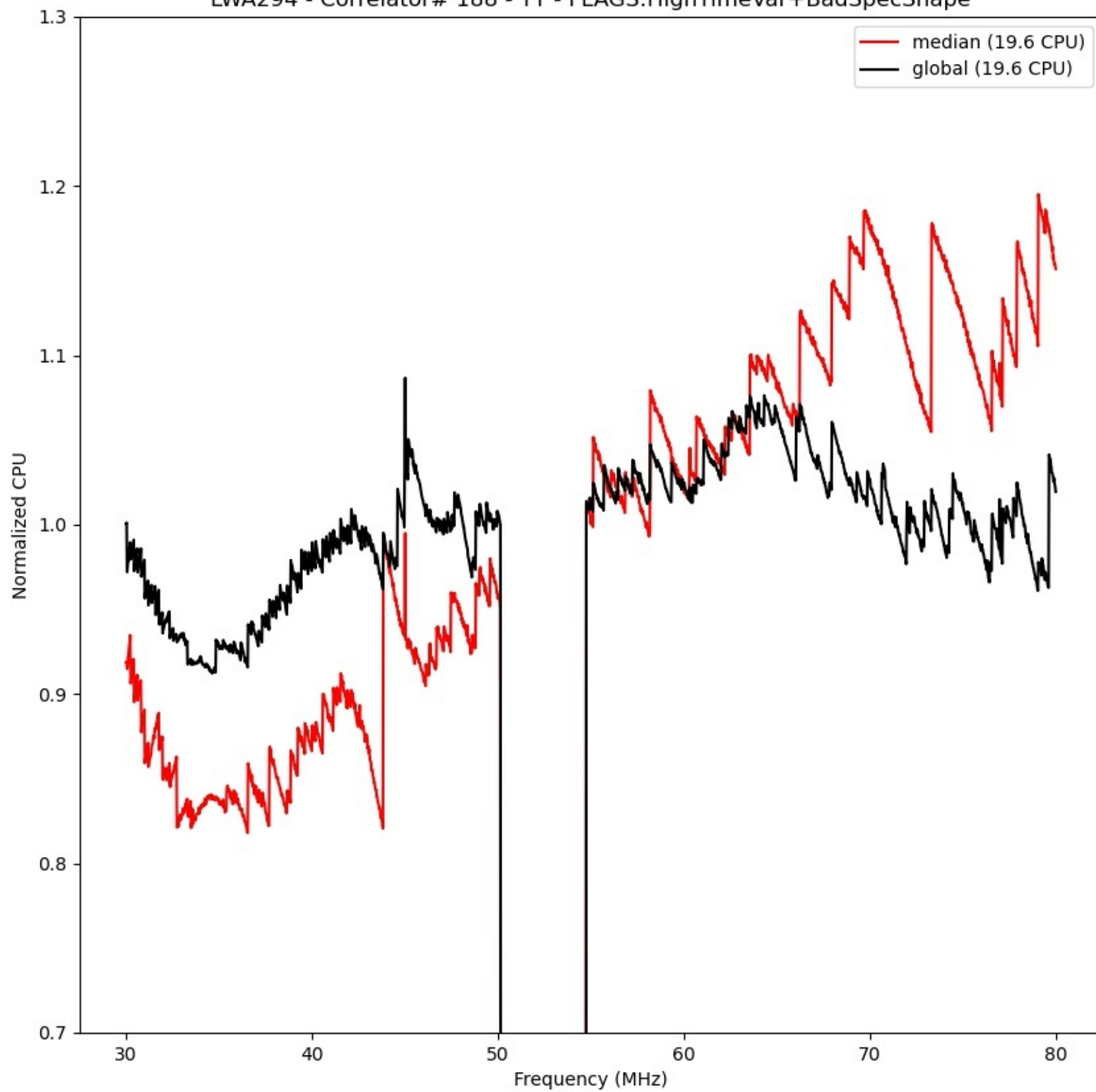
LWA294 - Correlator# 188 - YY - FLAGS:HighTimeVar+BadSpecShape
