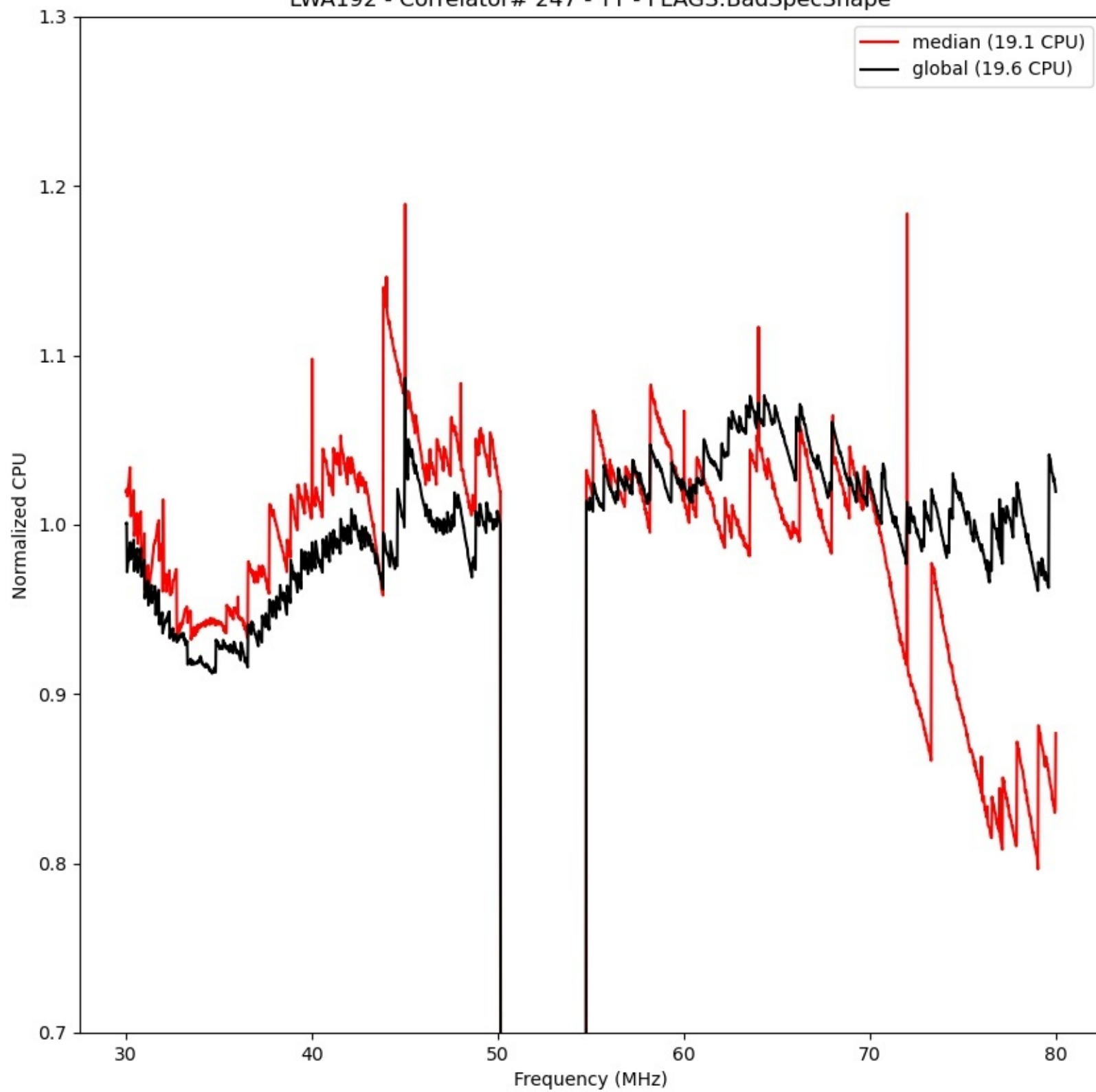
LWA192 - Correlator# 247 - YY - FLAGS:BadSpecShape
