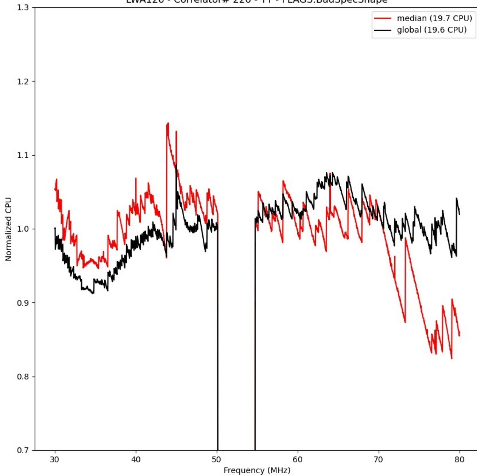
LWA126 - Correlator# 226 - YY - FLAGS:BadSpecShape
