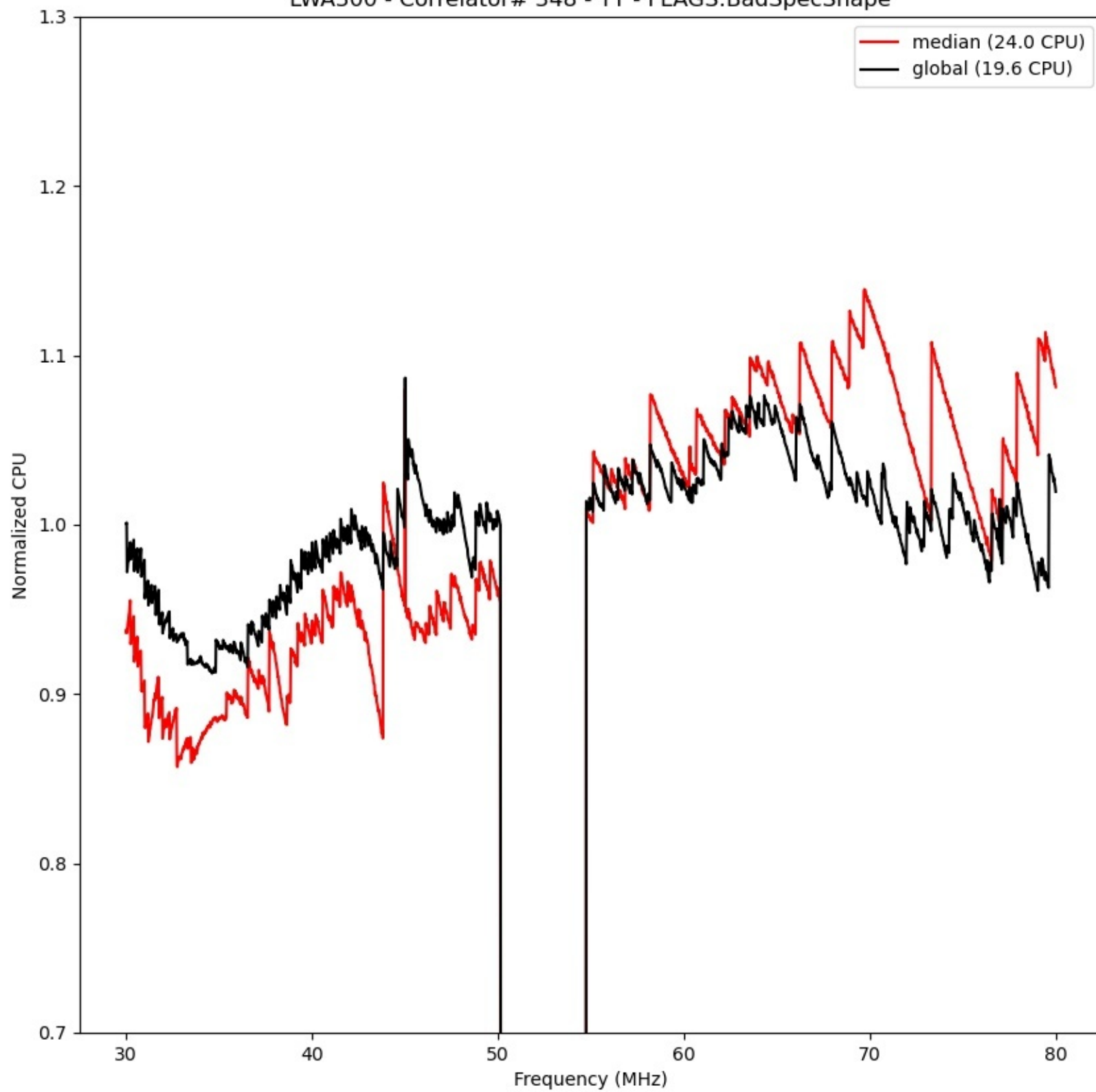
LWA300 - Correlator# 348 - YY - FLAGS:BadSpecShape
