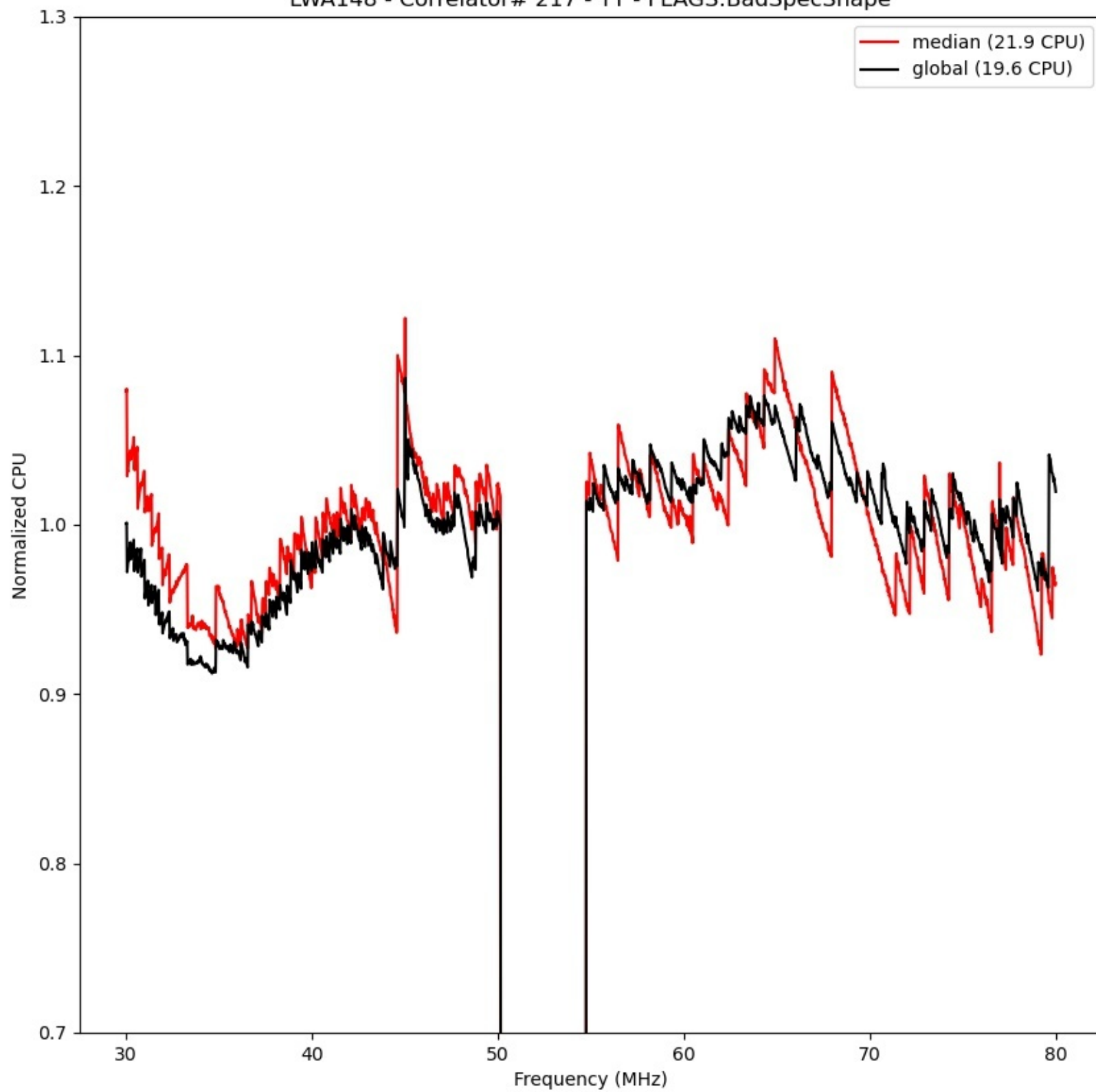
LWA148 - Correlator# 217 - YY - FLAGS:BadSpecShape
