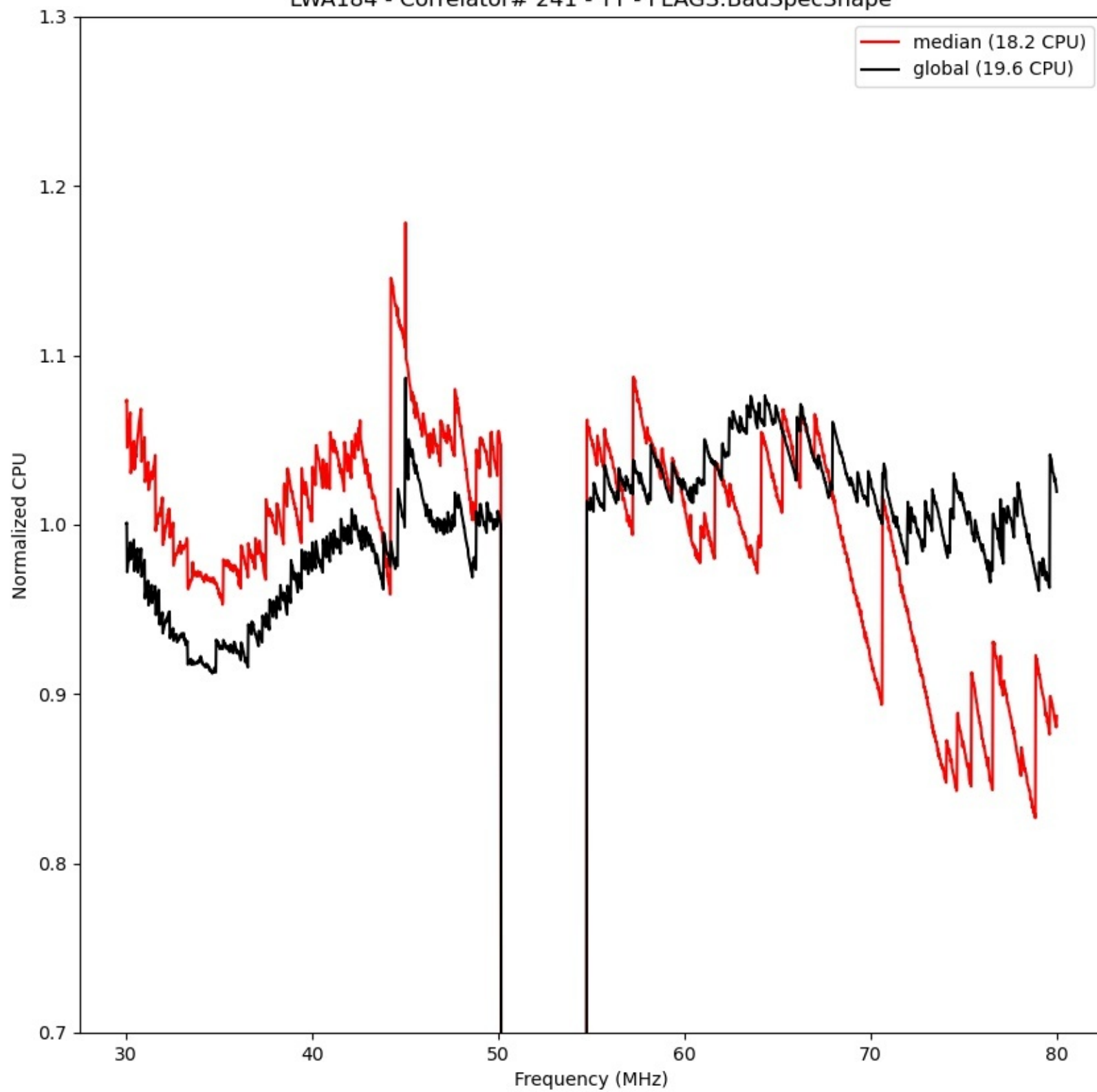
LWA184 - Correlator# 241 - YY - FLAGS:BadSpecShape
