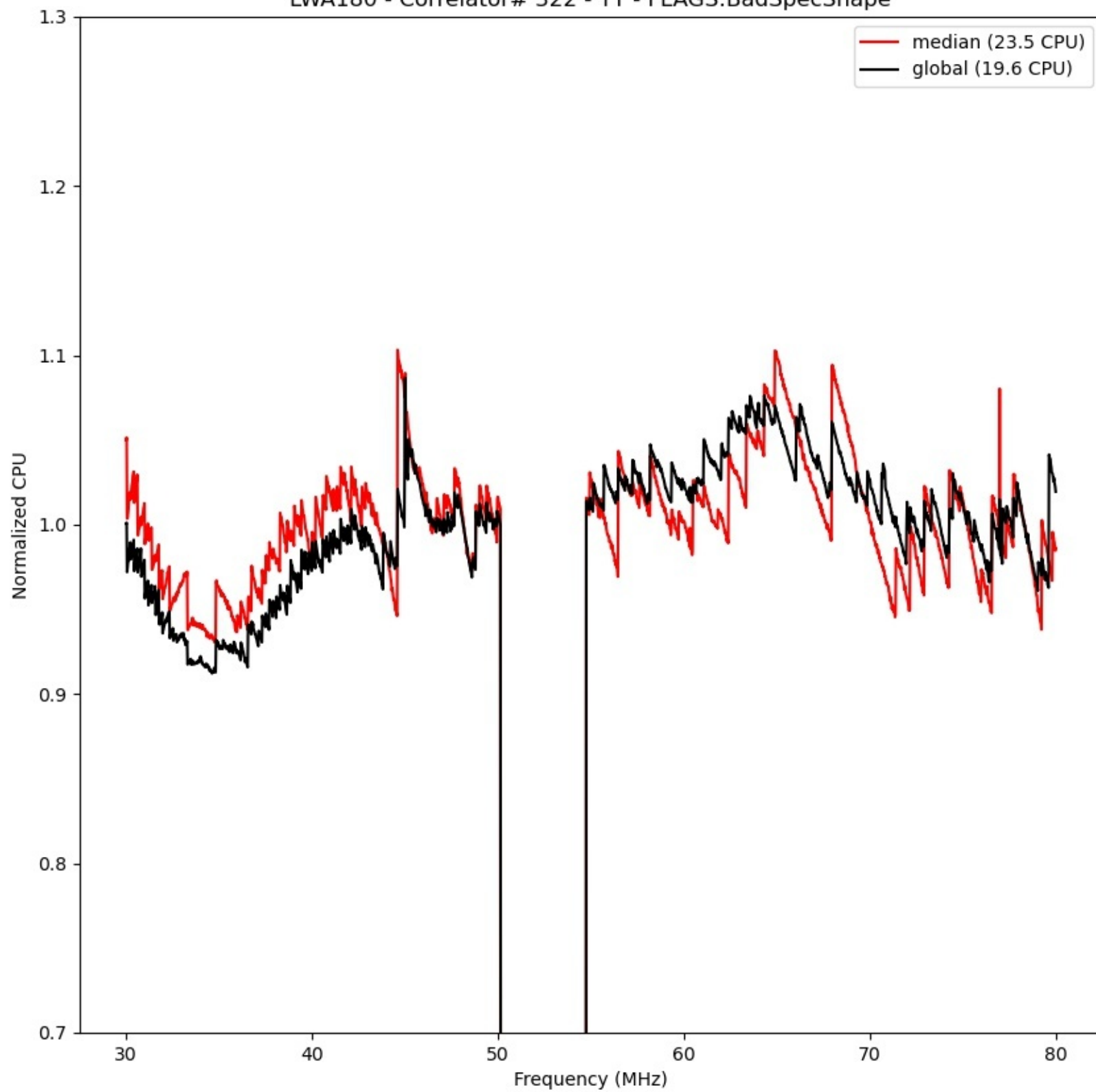
LWA180 - Correlator# 322 - YY - FLAGS:BadSpecShape
