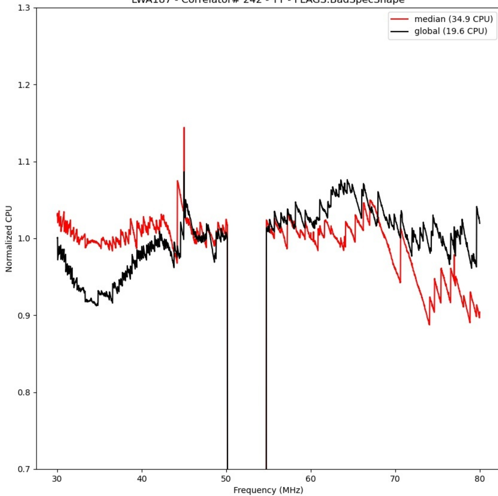
LWA187 - Correlator# 242 - YY - FLAGS:BadSpecShape
