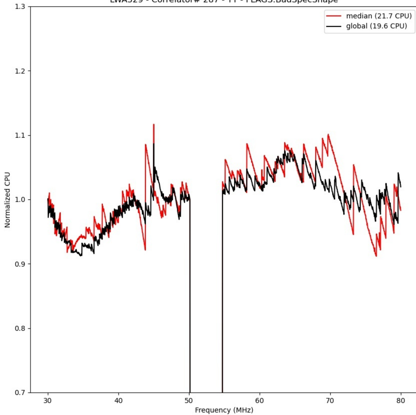
LWA329 - Correlator# 287 - YY - FLAGS:BadSpecShape
