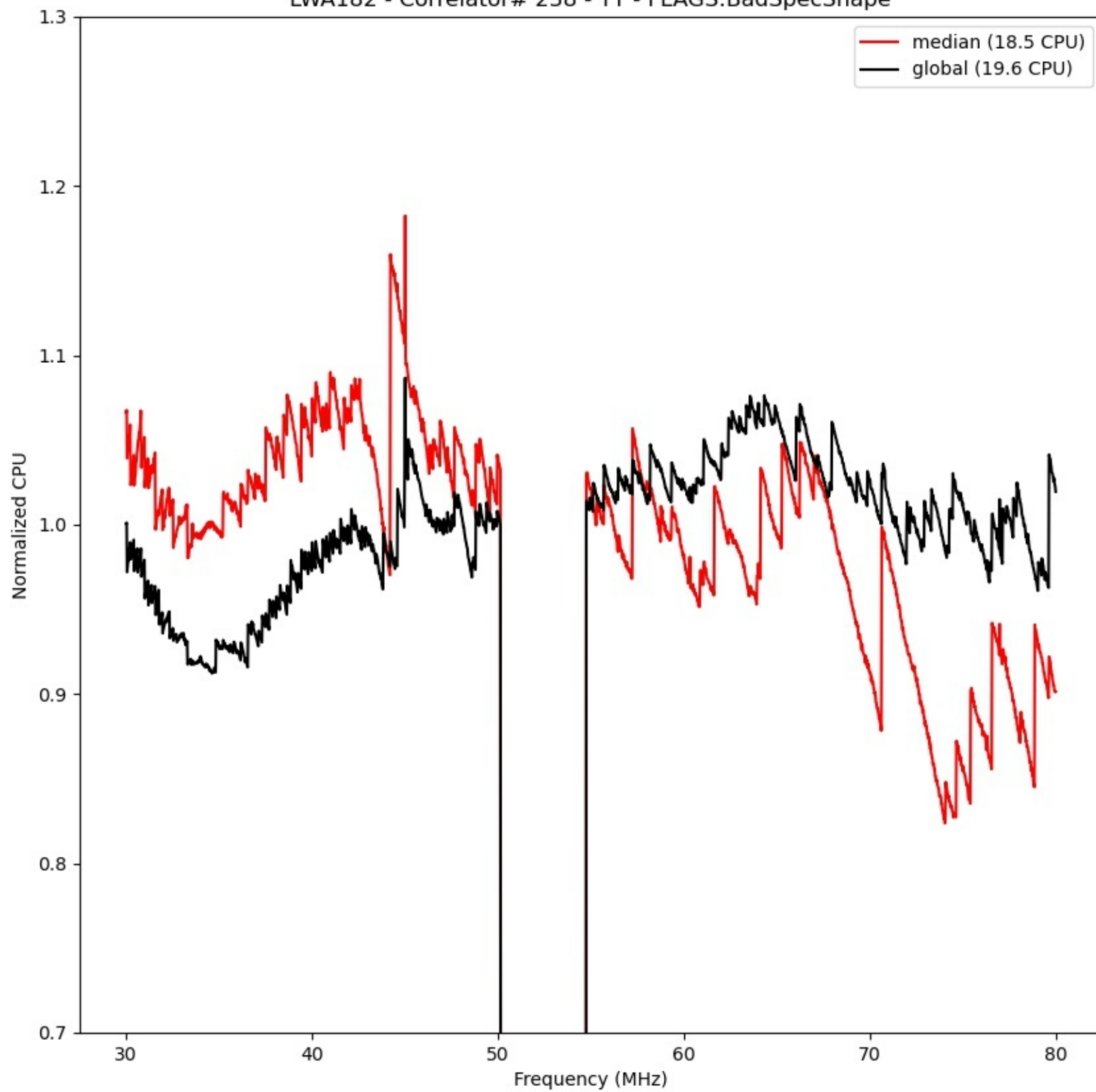
LWA182 - Correlator# 238 - YY - FLAGS:BadSpecShape
