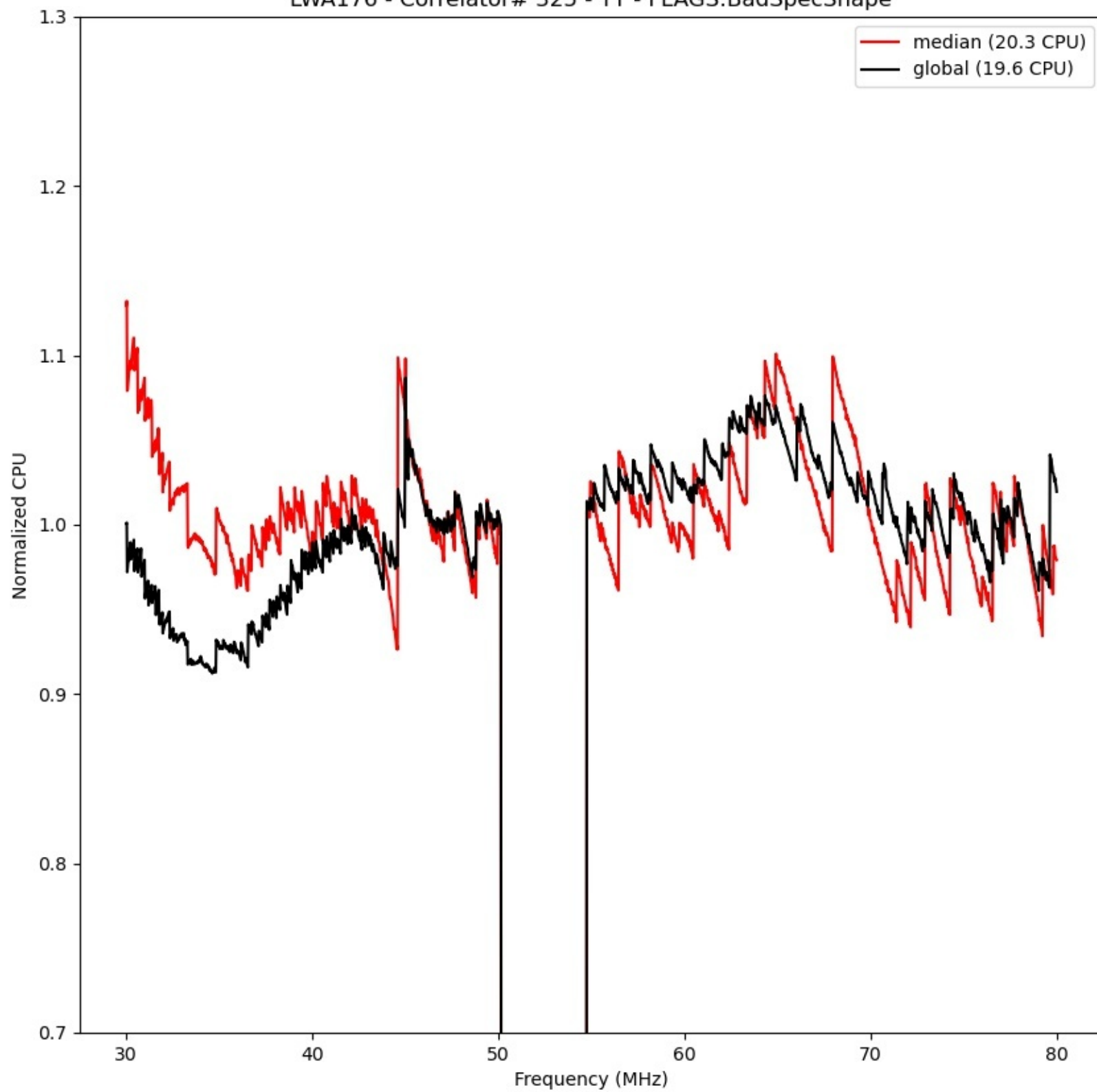
LWA176 - Correlator# 325 - YY - FLAGS:BadSpecShape
