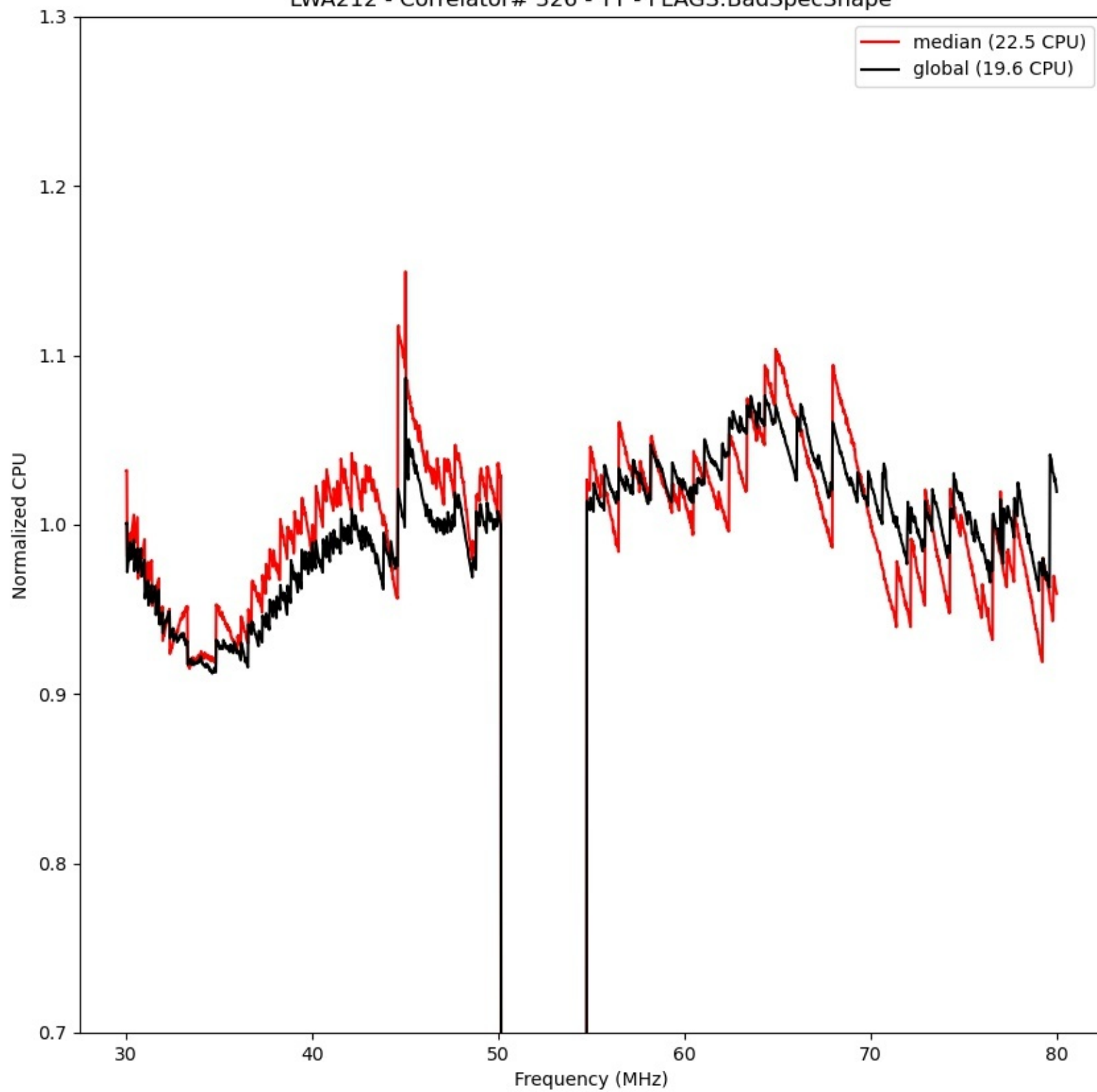
LWA212 - Correlator# 326 - YY - FLAGS:BadSpecShape
