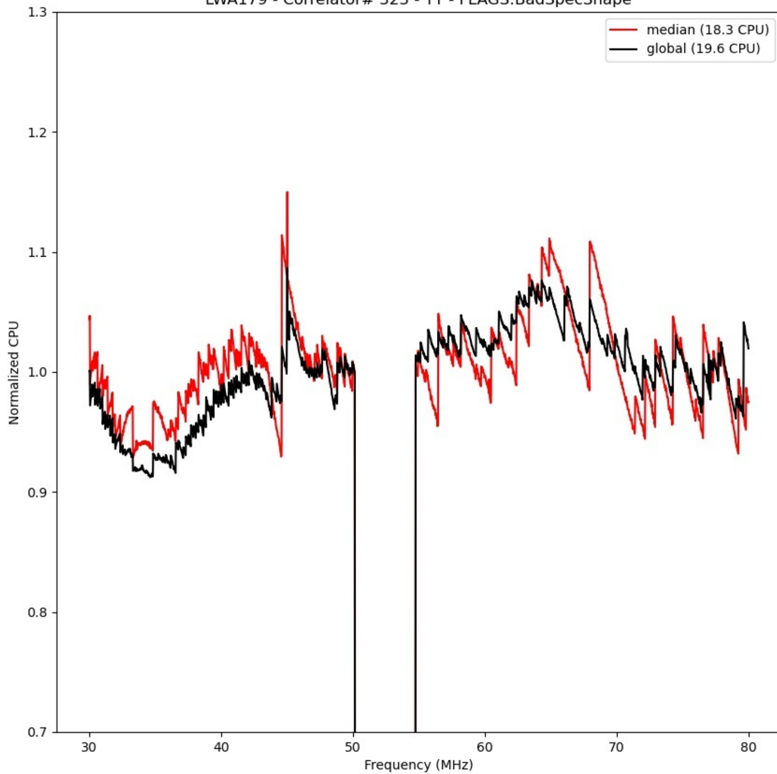
LWA179 - Correlator# 323 - YY - FLAGS:BadSpecShape
