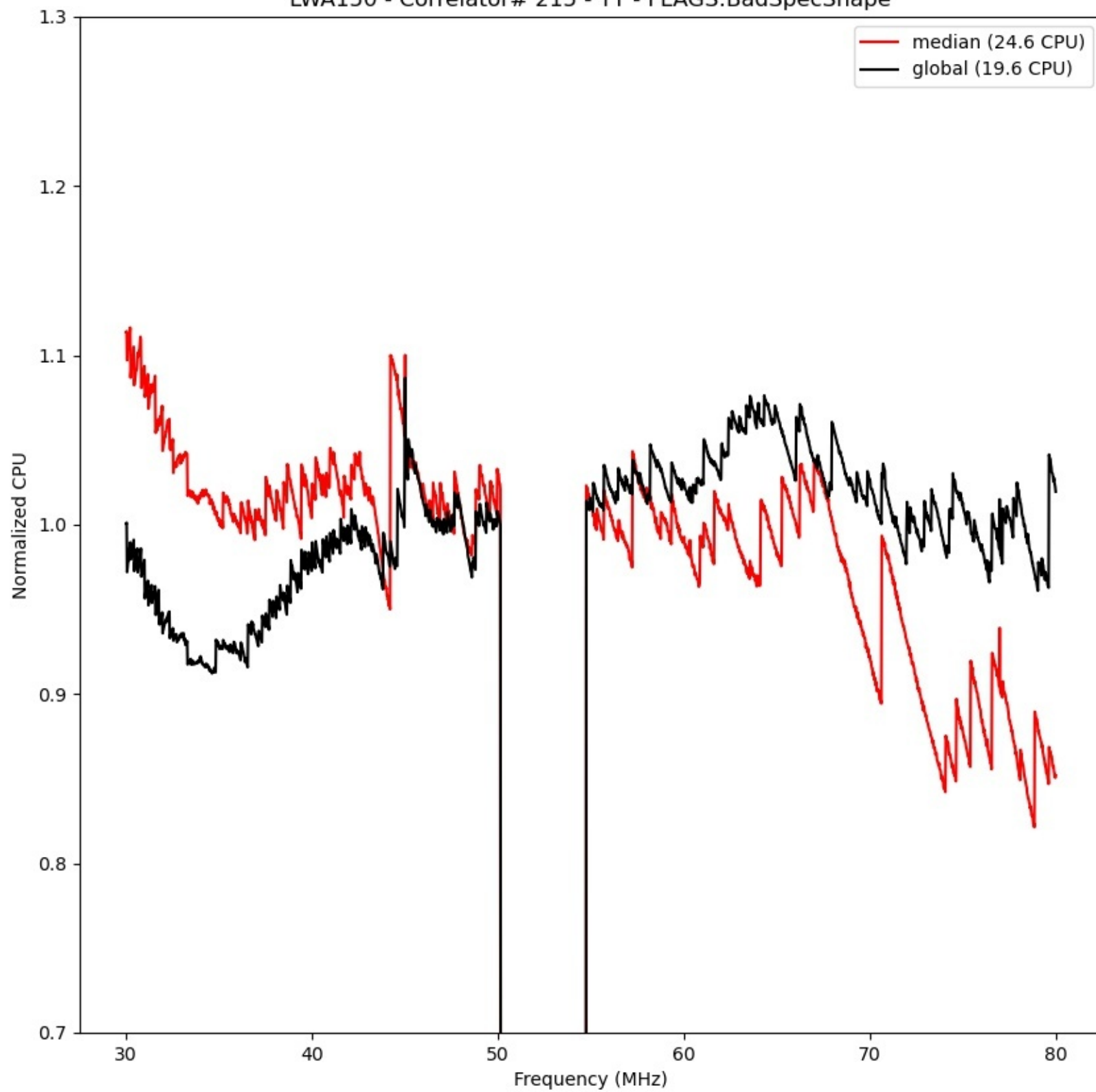
LWA150 - Correlator# 215 - YY - FLAGS:BadSpecShape
