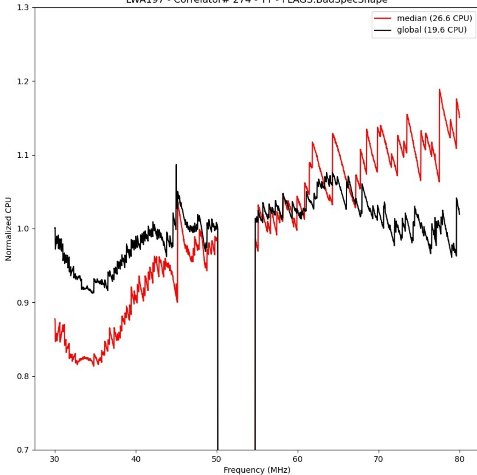
LWA197 - Correlator# 274 - YY - FLAGS:BadSpecShape
