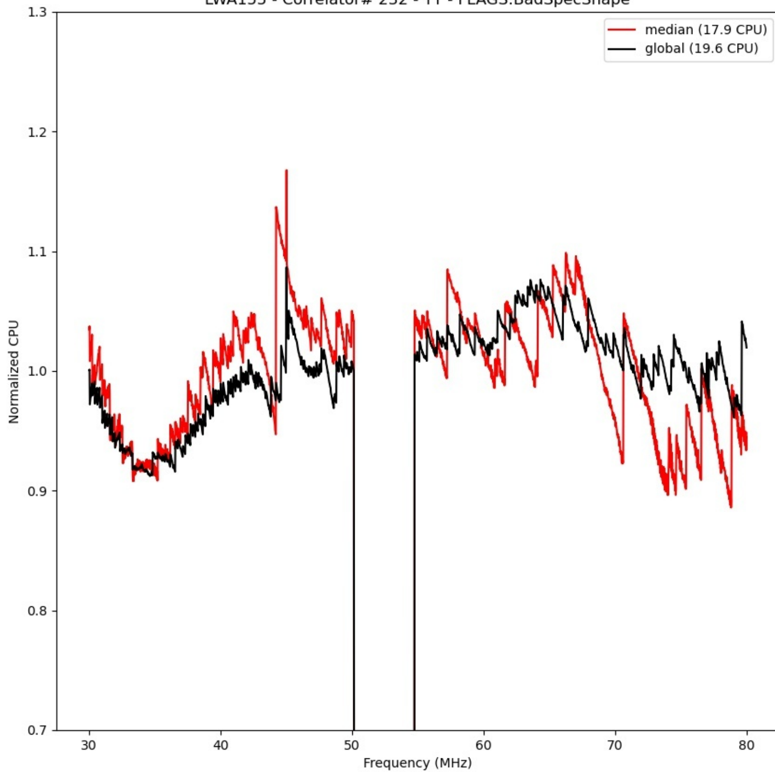
LWA155 - Correlator# 232 - YY - FLAGS:BadSpecShape
