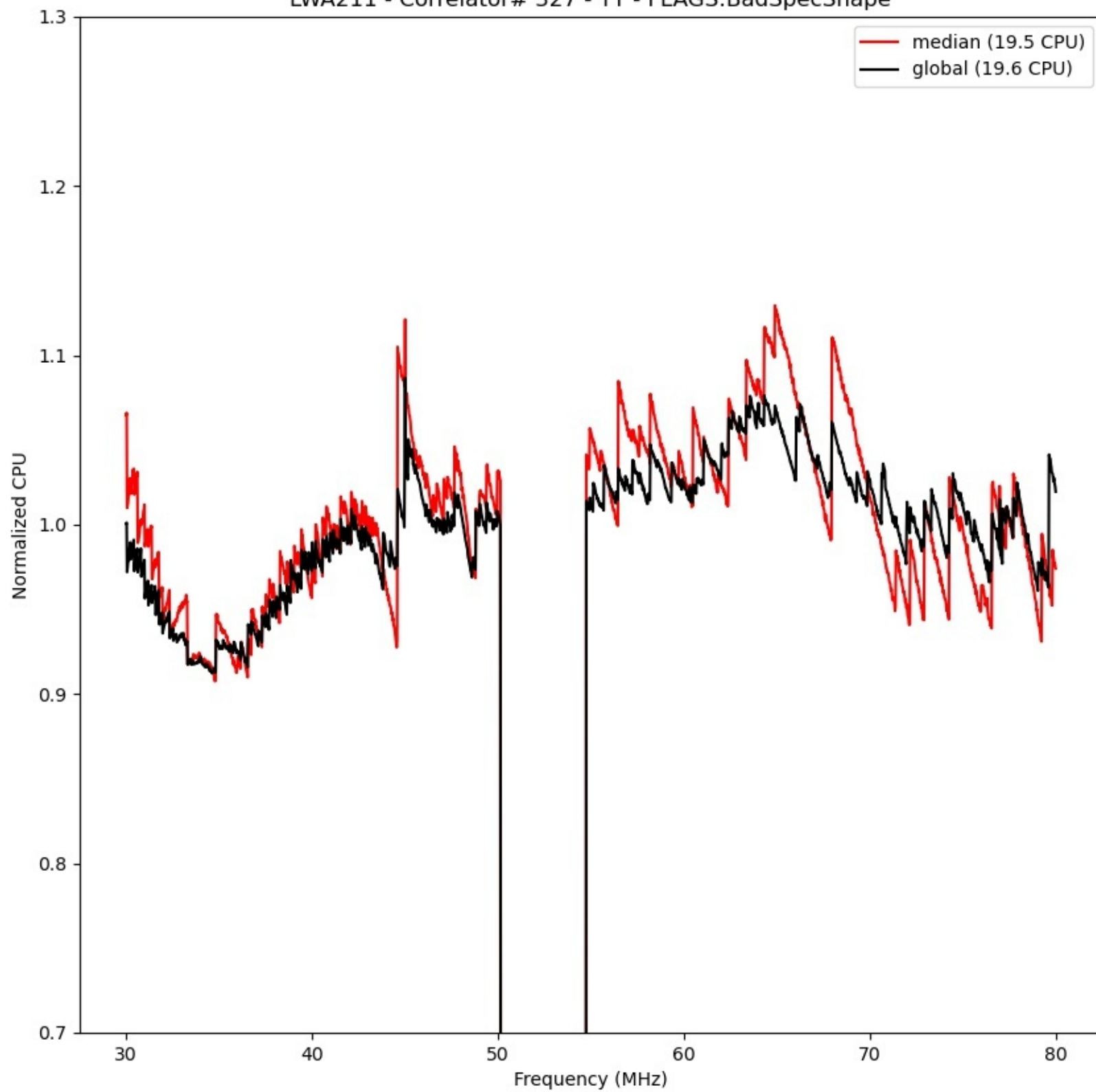
LWA211 - Correlator# 327 - YY - FLAGS:BadSpecShape
