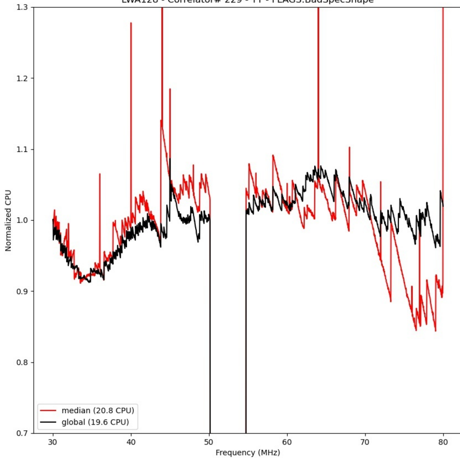
LWA128 - Correlator# 229 - YY - FLAGS:BadSpecShape
