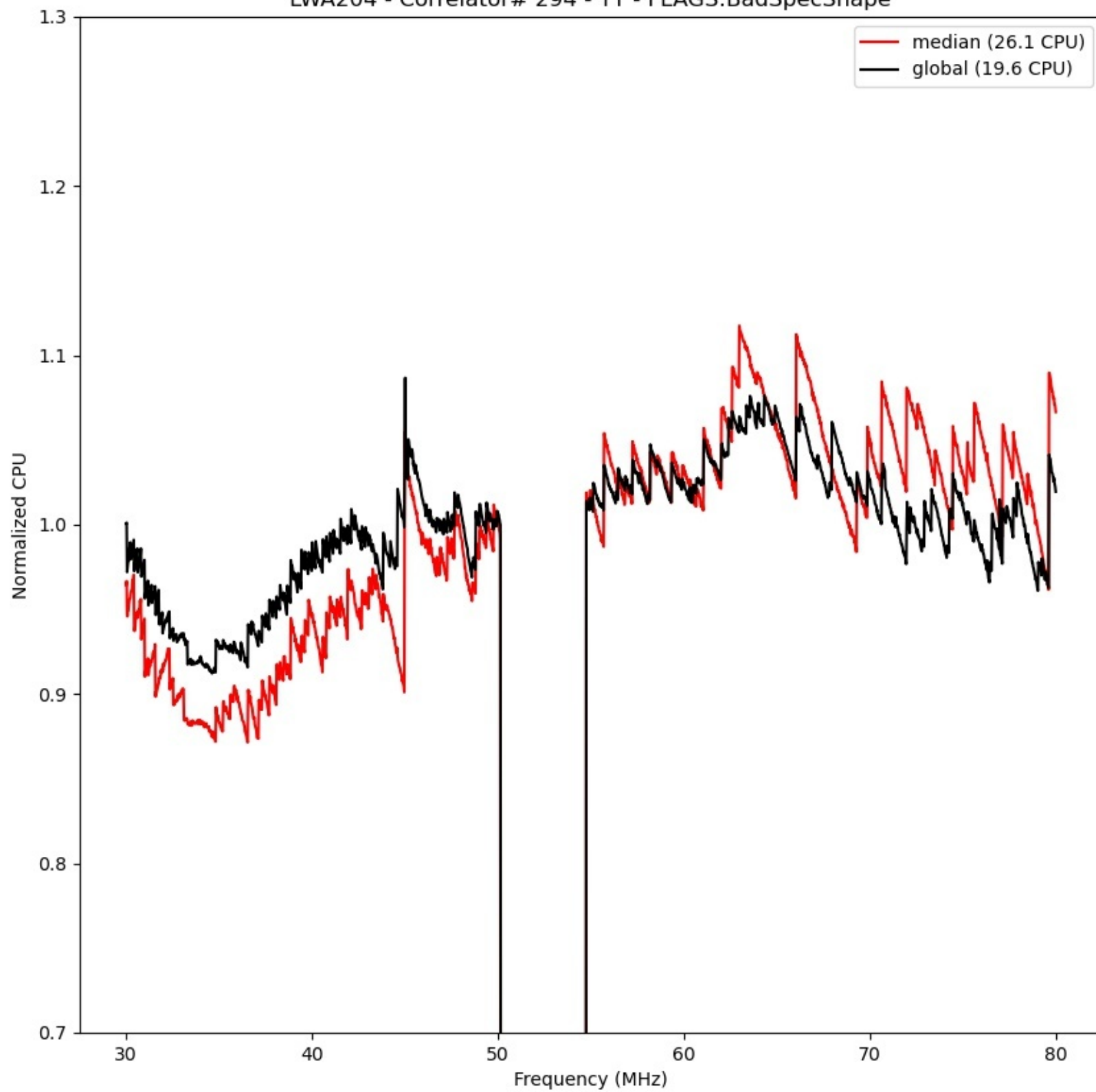
LWA204 - Correlator# 294 - YY - FLAGS:BadSpecShape
