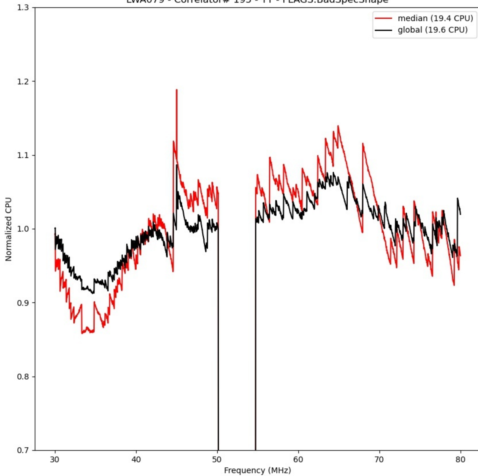
LWA079 - Correlator# 195 - YY - FLAGS:BadSpecShape
