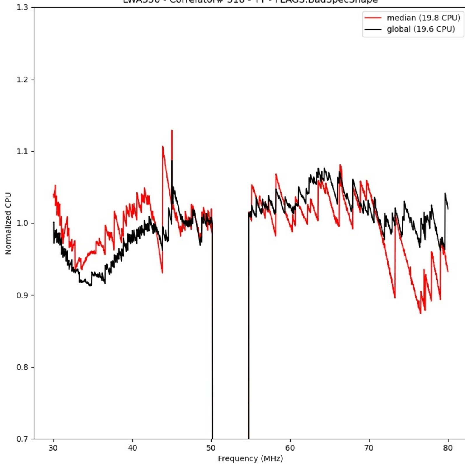
LWA356 - Correlator# 318 - YY - FLAGS:BadSpecShape
