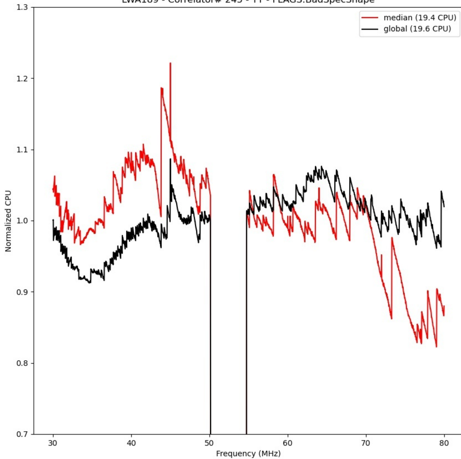
LWA189 - Correlator# 245 - YY - FLAGS:BadSpecShape
