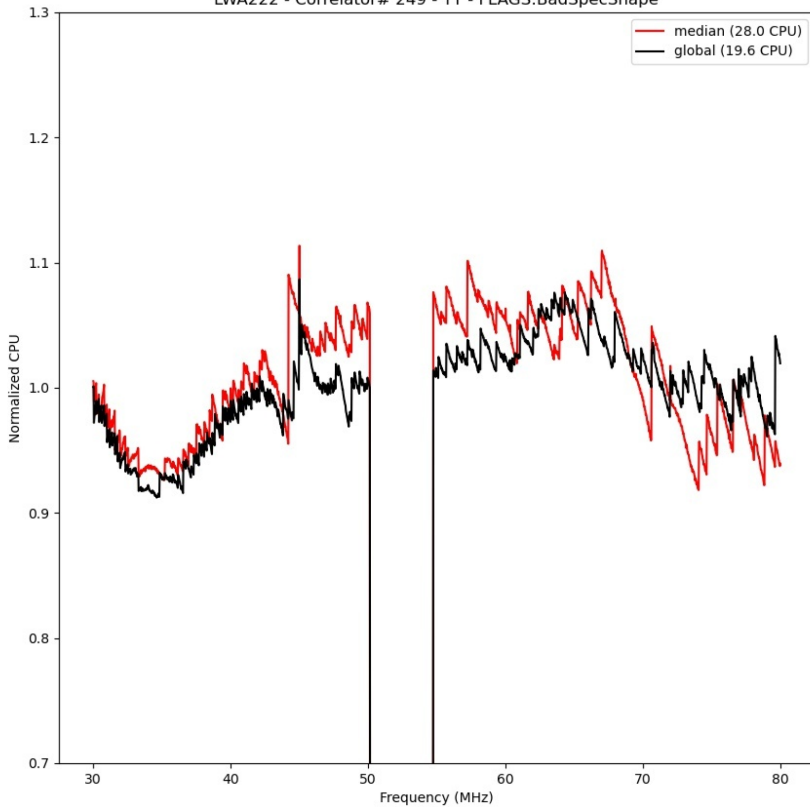
LWA222 - Correlator# 249 - YY - FLAGS:BadSpecShape
