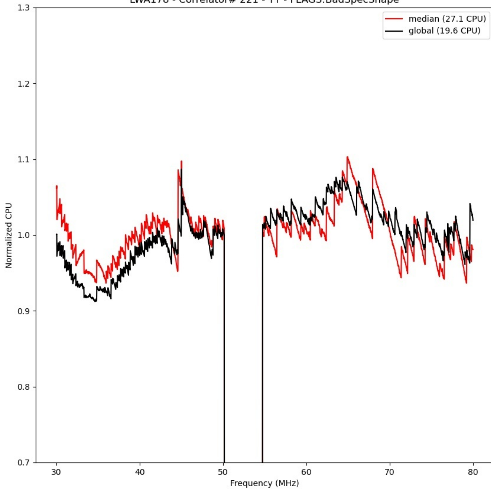
LWA178 - Correlator# 221 - YY - FLAGS:BadSpecShape
