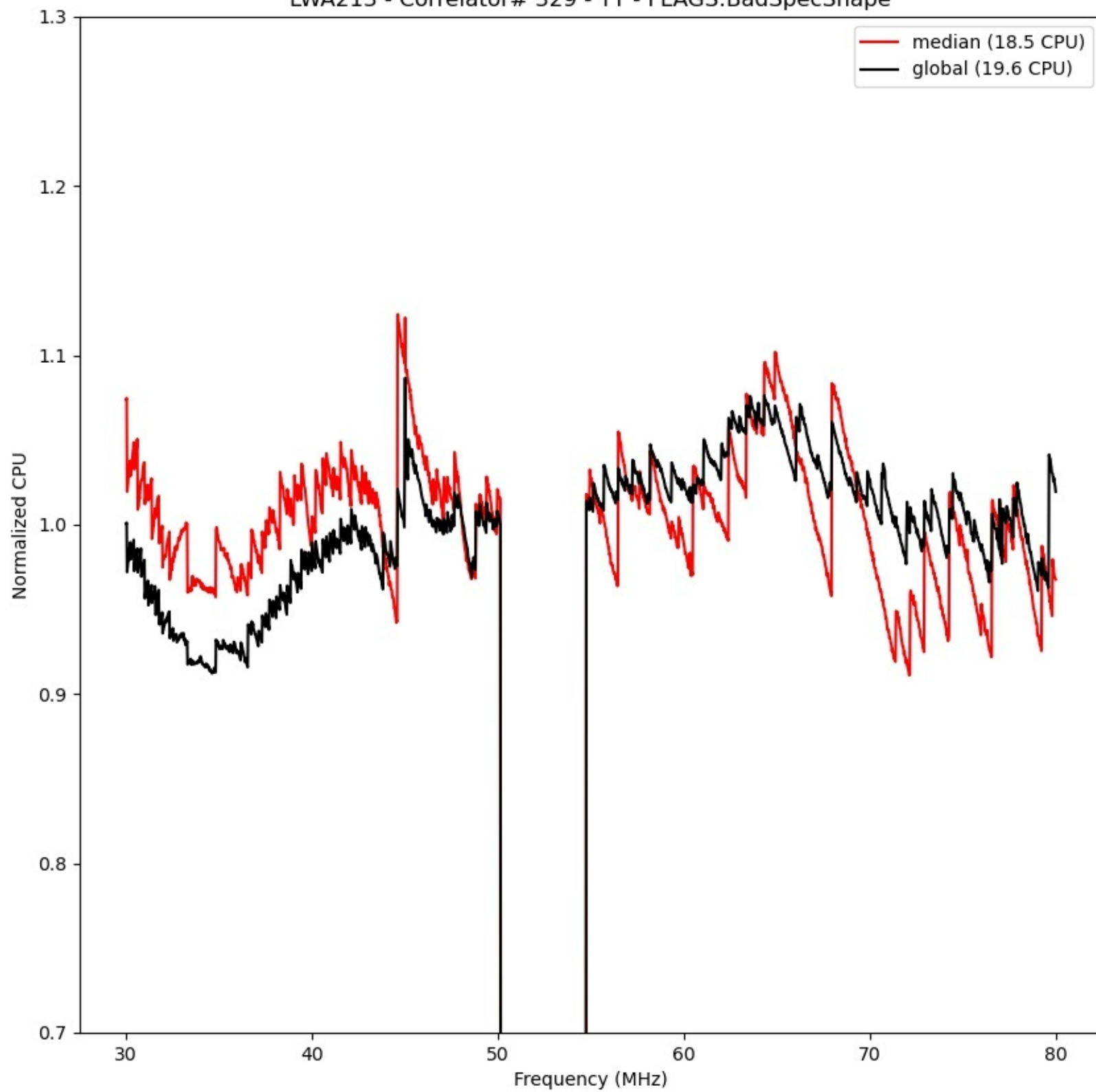
LWA213 - Correlator# 329 - YY - FLAGS:BadSpecShape
