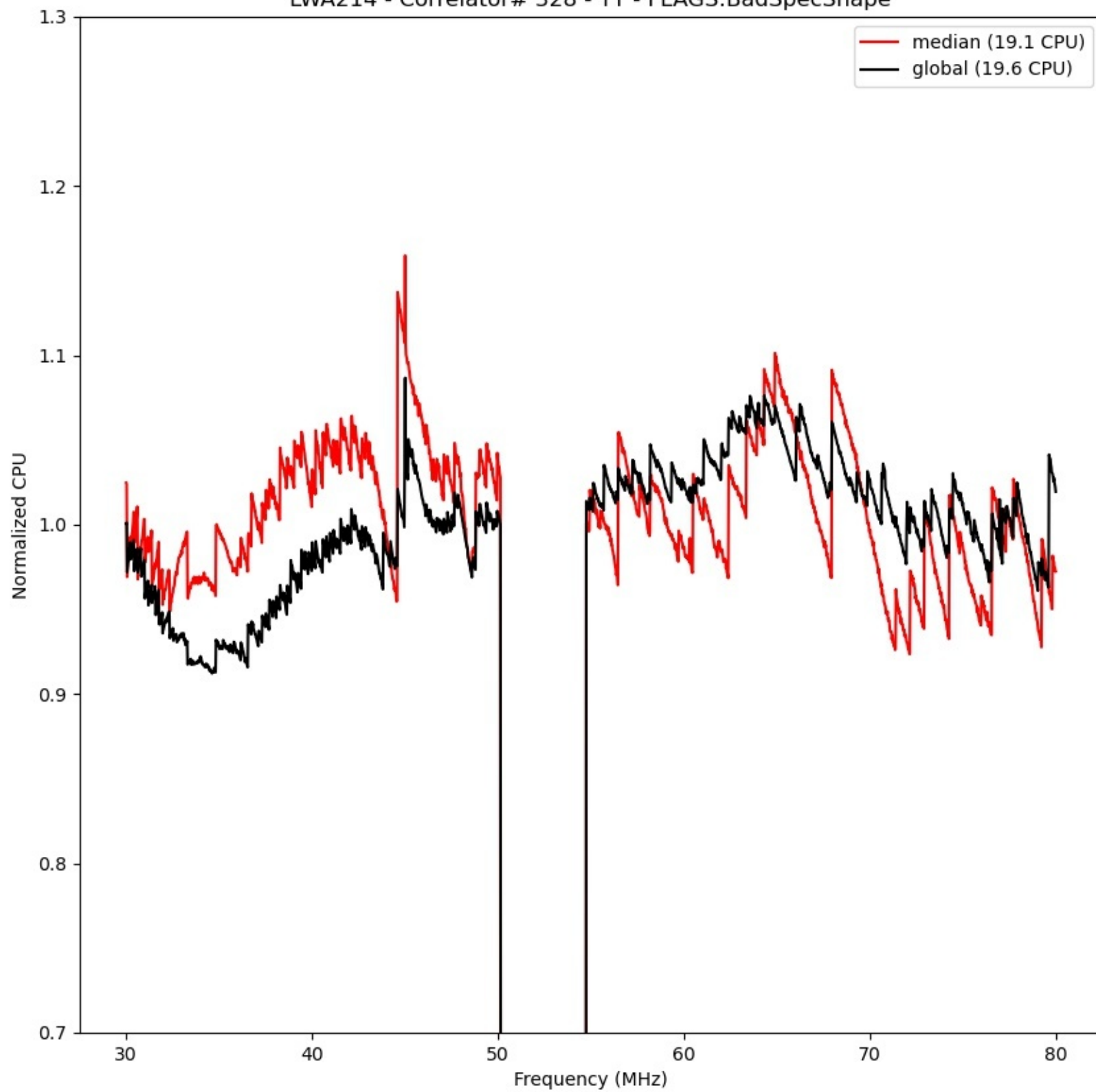
LWA214 - Correlator# 328 - YY - FLAGS:BadSpecShape
