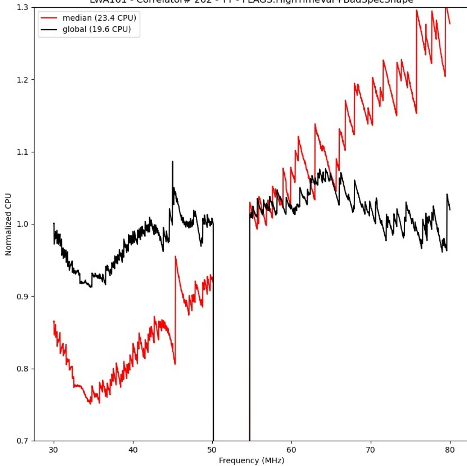
LWA161 - Correlator# 262 - YY - FLAGS:HighTimeVar+BadSpecShape
