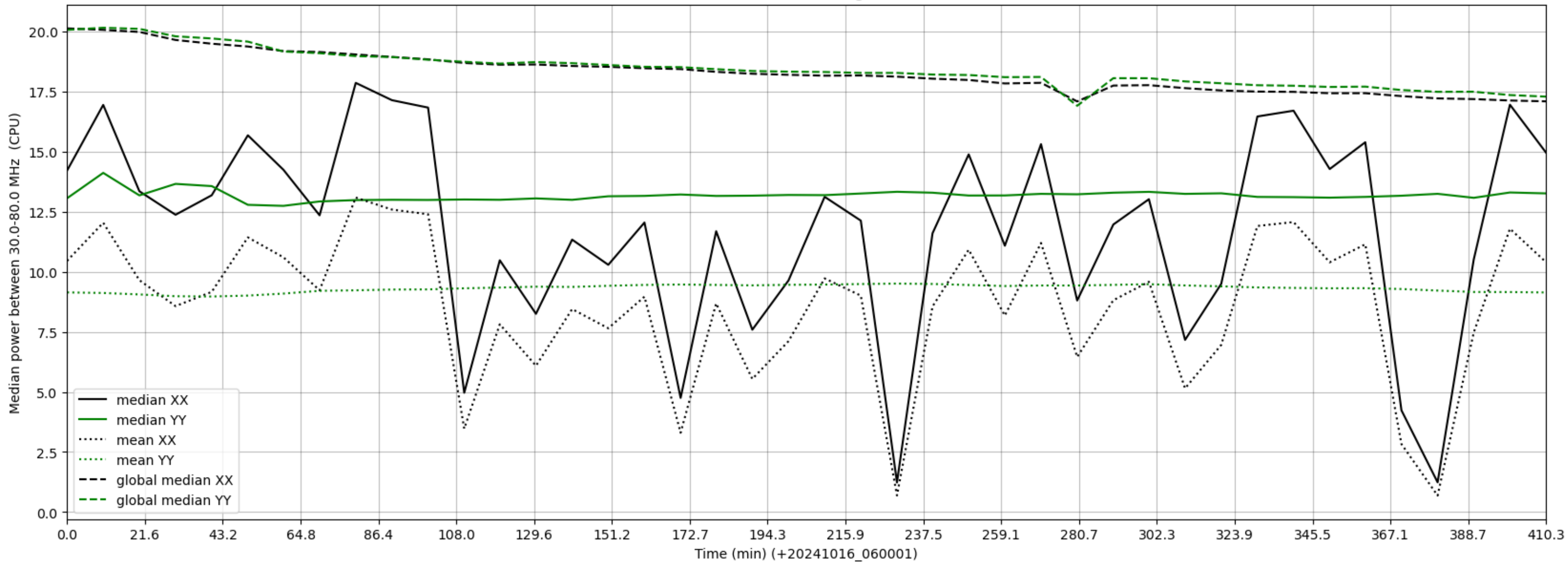
LWA043 - Correlator# 081 - XX FLAGS:HighTimeVar - YY FLAGS:Good
