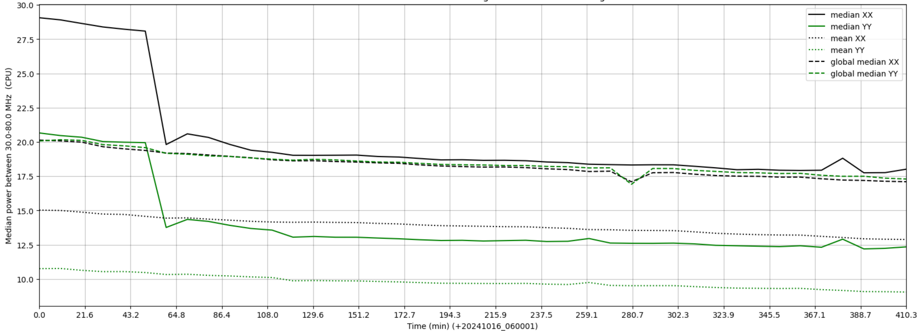
LWA283 - Correlator# 040 - XX FLAGS:HighTimeVar - YY FLAGS:HighTimeVar
