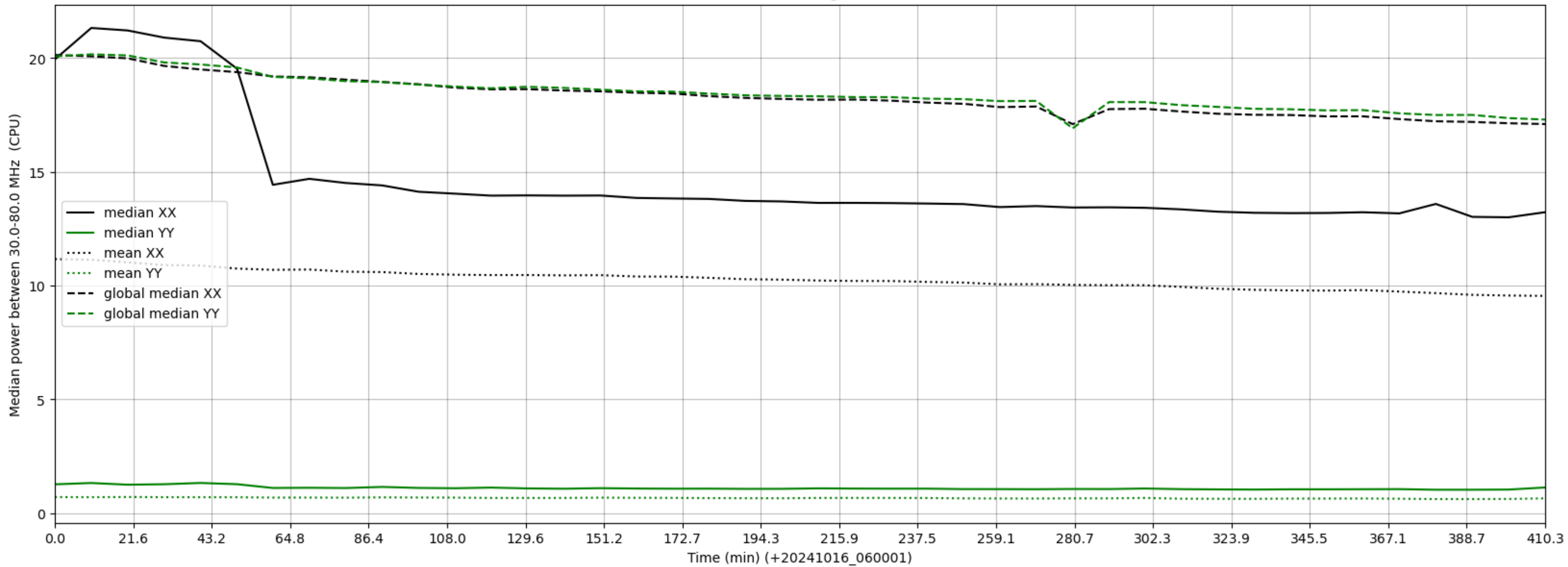
LWA305 - Correlator# 050 - XX FLAGS:HighTimeVar - YY FLAGS:LowPower
