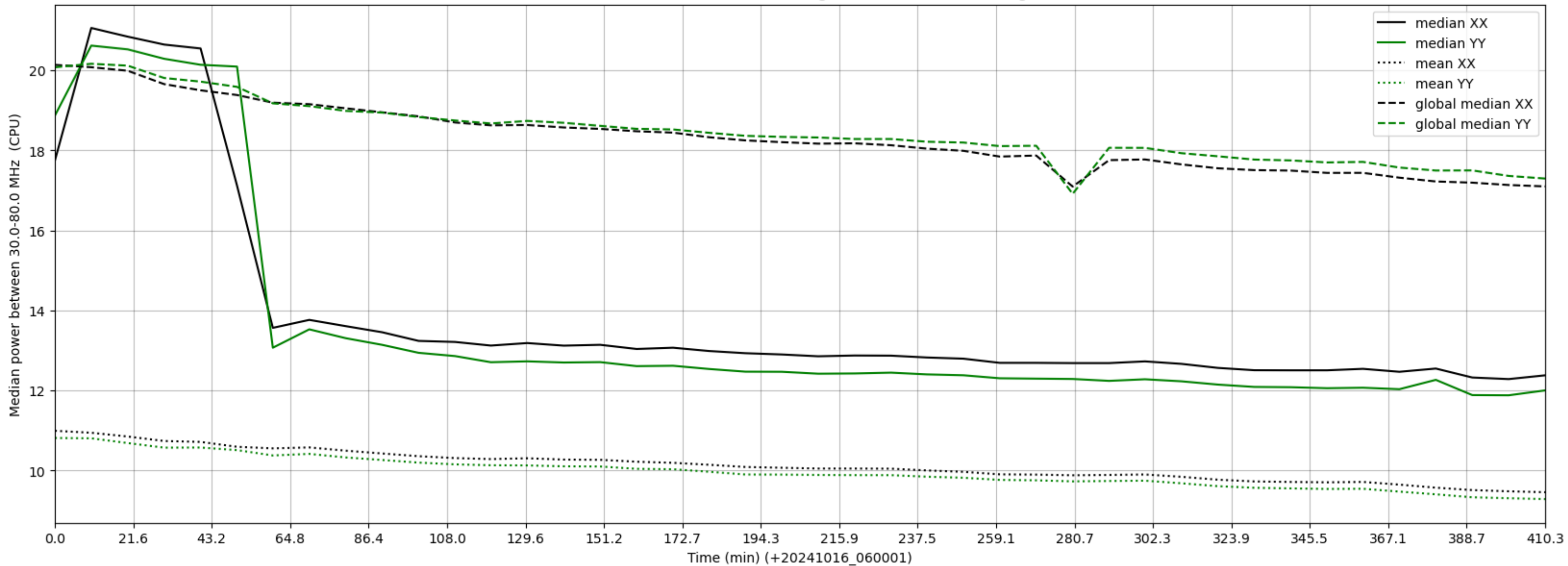
LWA303 - Correlator# 051 - XX FLAGS:HighTimeVar - YY FLAGS:HighTimeVar
