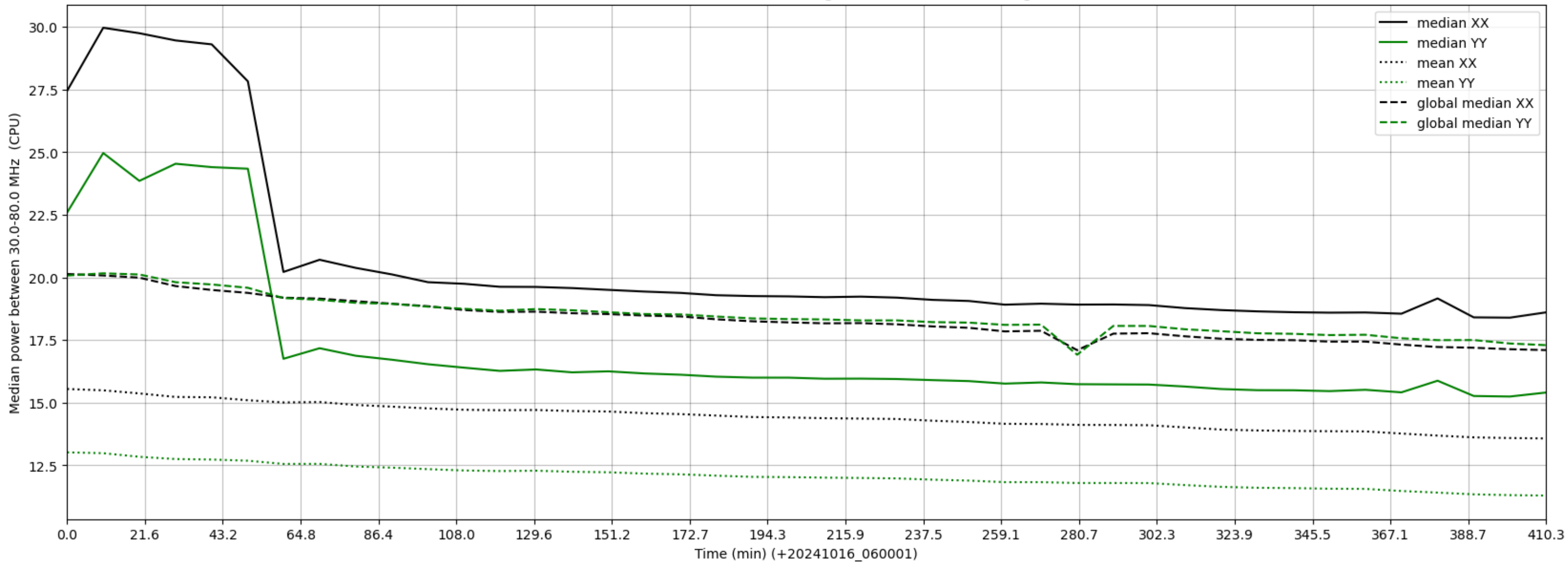
LWA260 - Correlator# 034 - XX FLAGS:HighTimeVar - YY FLAGS:HighTimeVar
