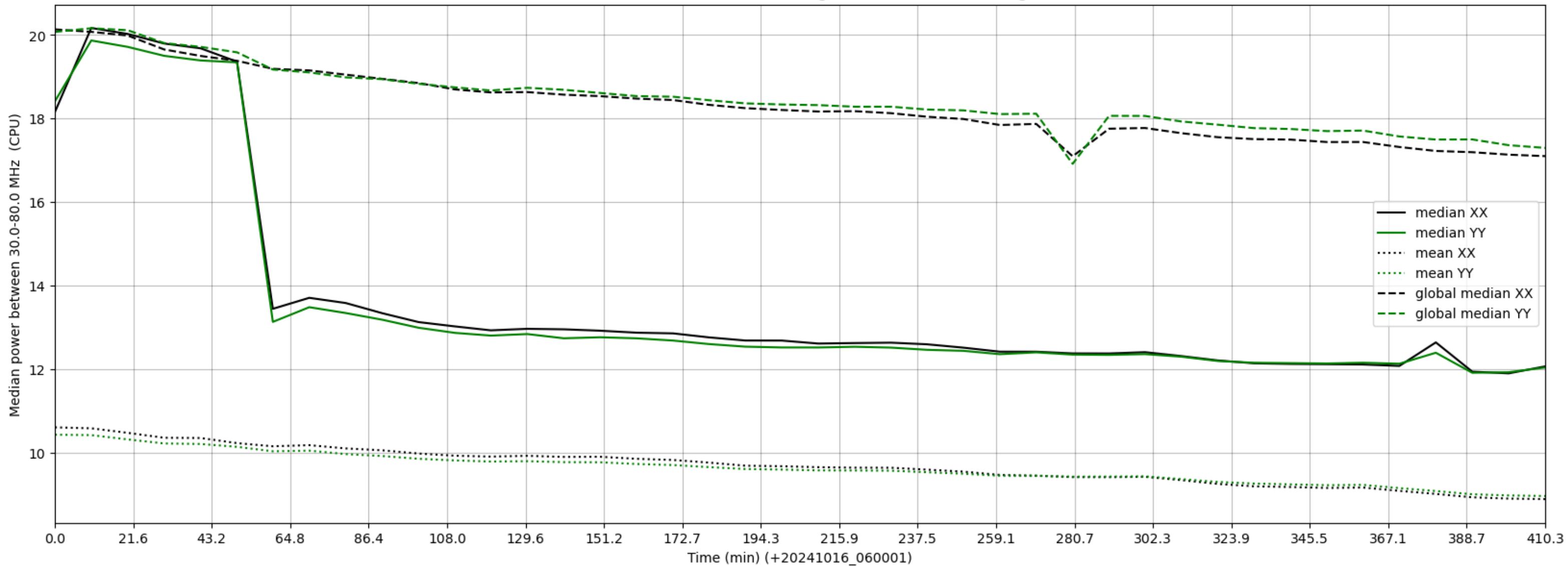
LWA280 - Correlator# 041 - XX FLAGS:HighTimeVar - YY FLAGS:HighTimeVar
