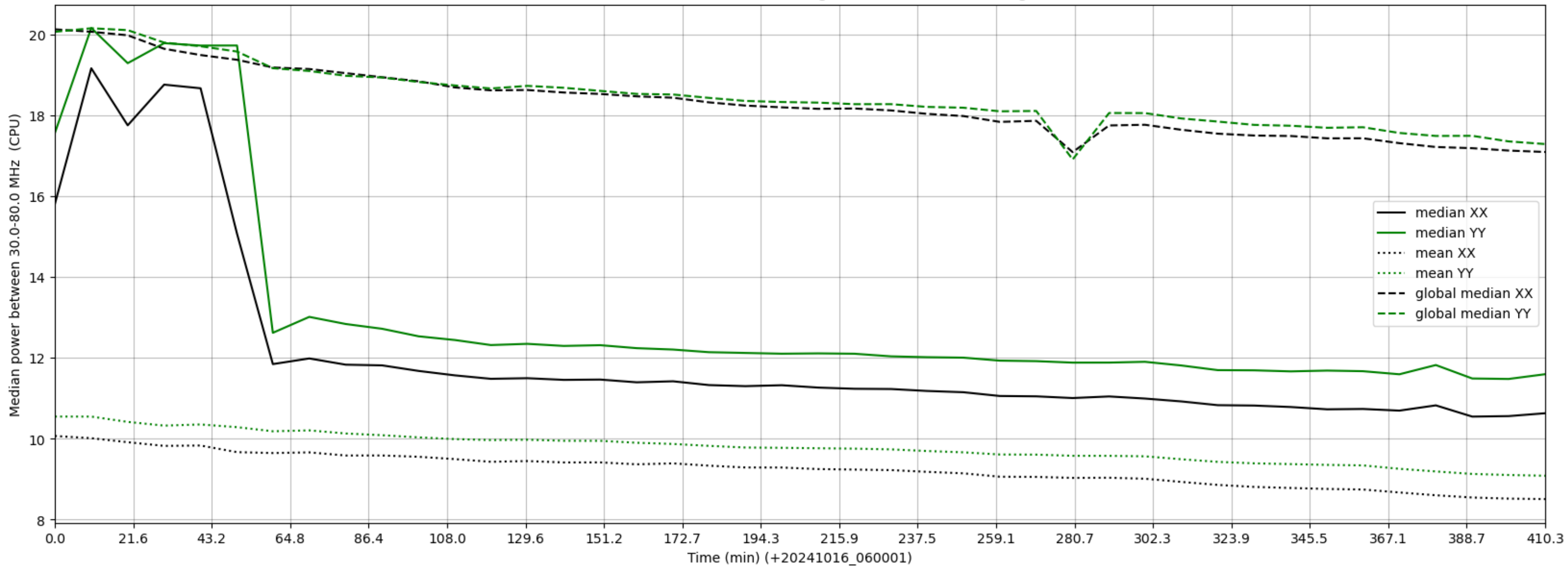
LWA288 - Correlator# 042 - XX FLAGS:HighTimeVar - YY FLAGS:HighTimeVar
