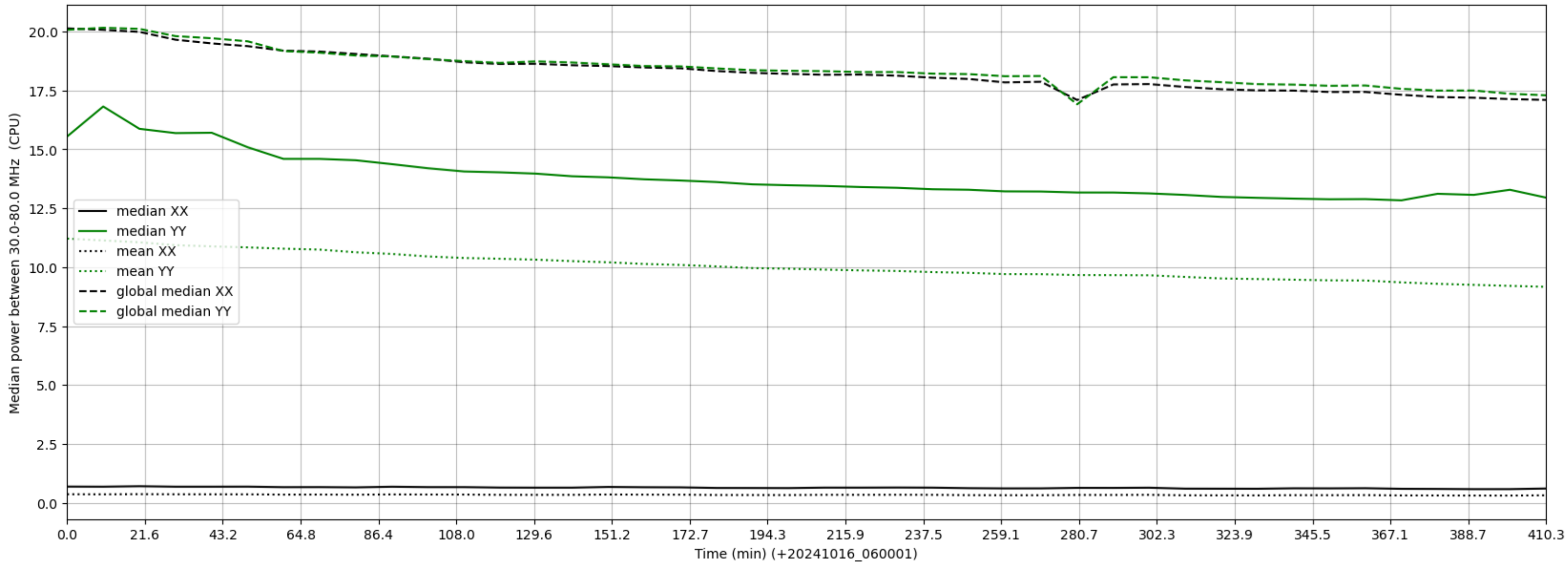
LWA003 - Correlator# 067 - XX FLAGS:LowPower - YY FLAGS:Good
