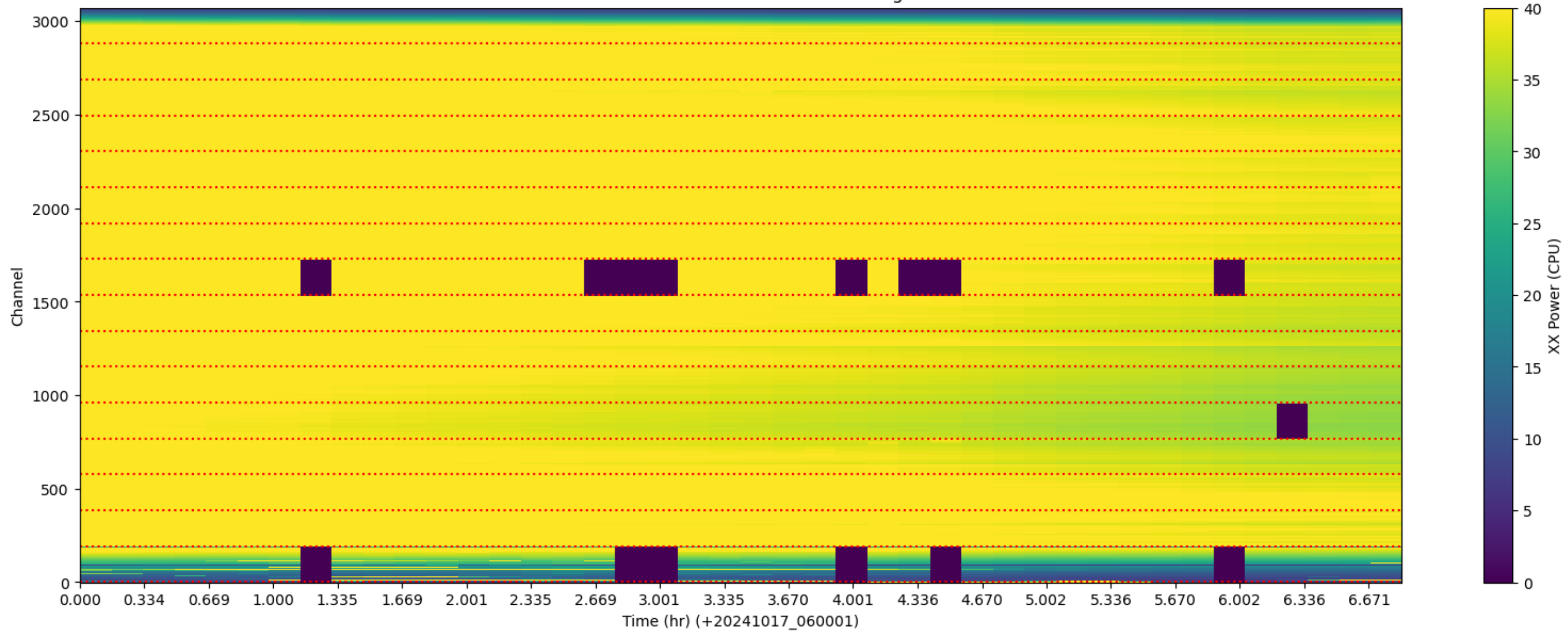
LWA363 - Correlator# 094 - XX - FLAGS: HighPower
