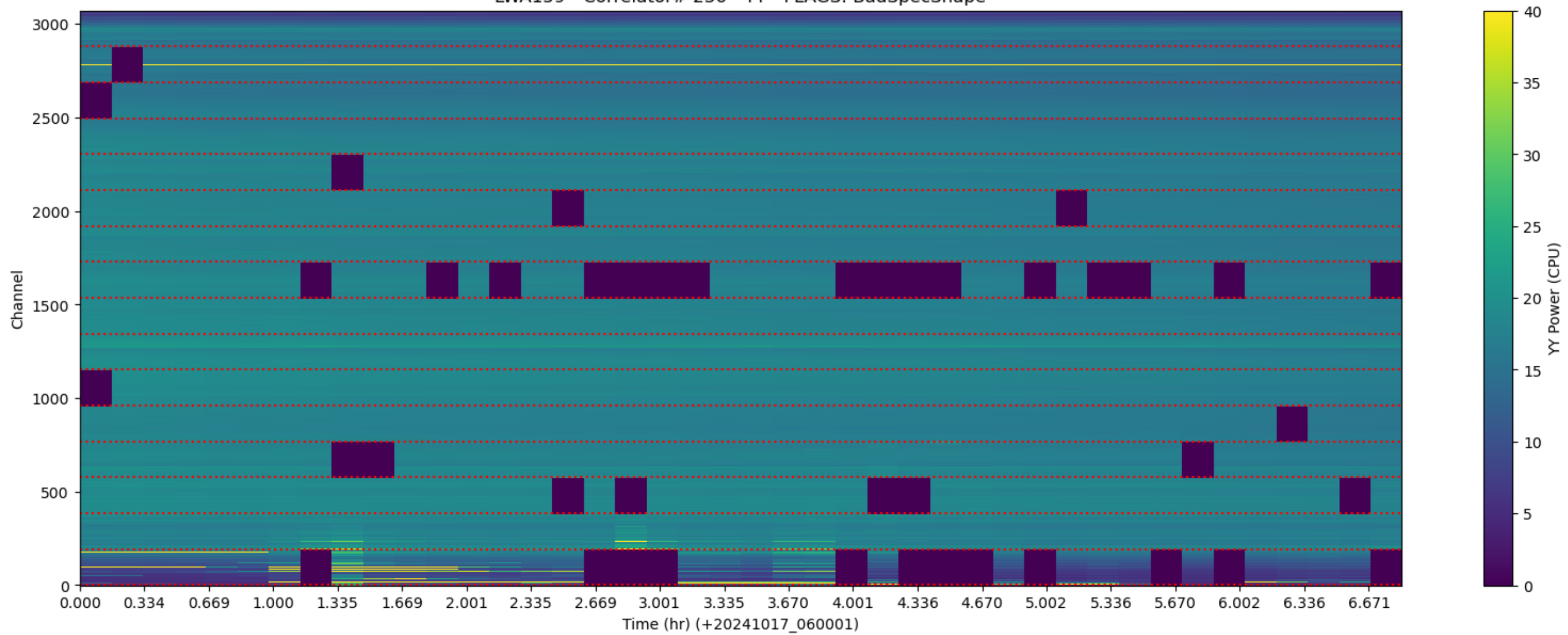
LWA159 - Correlator# 236 - YY - FLAGS: BadSpecShape
