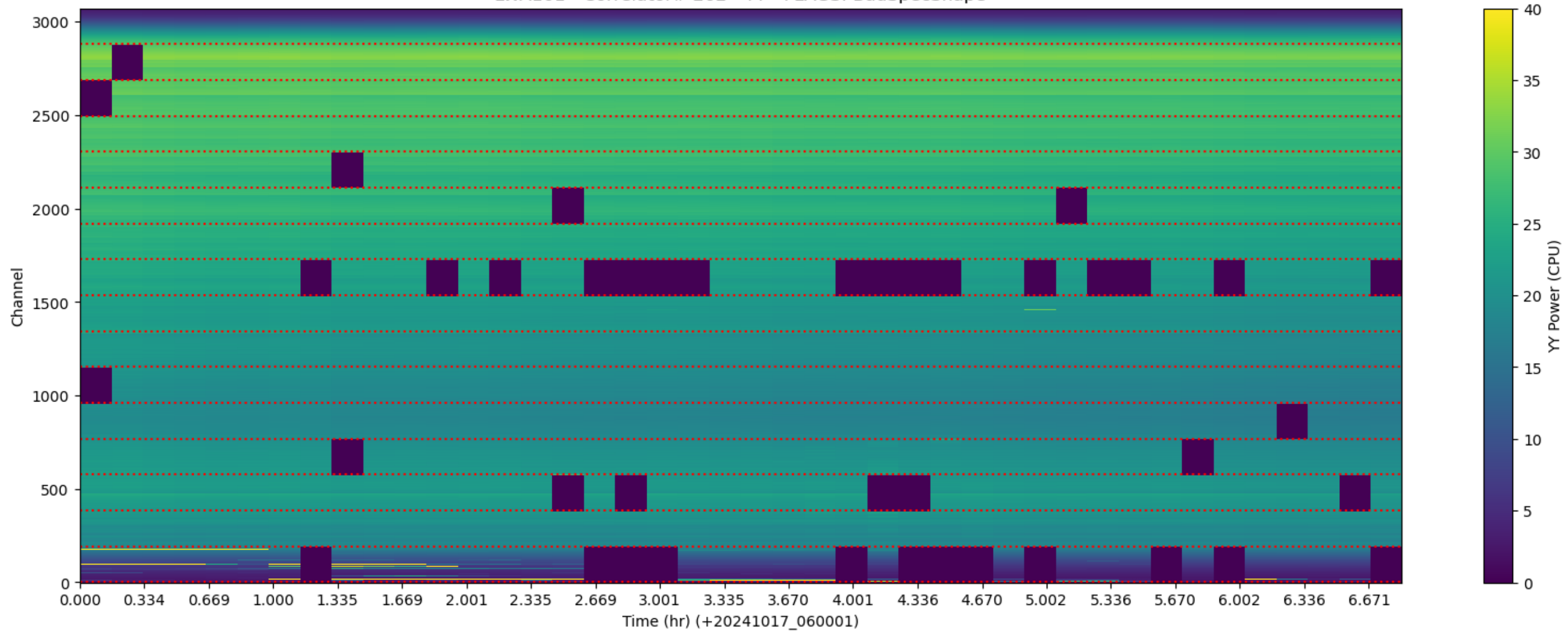
LWA161 - Correlator# 262 - YY - FLAGS: BadSpecShape
