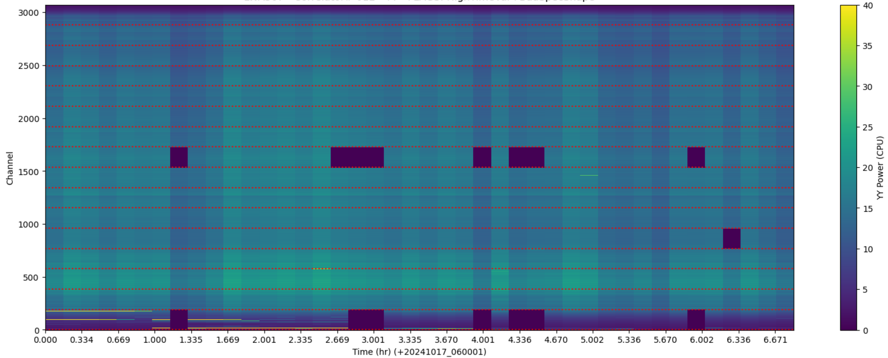
LWA307 - Correlator# 012 - YY - FLAGS: HighTimeVar+BadSpecShape
