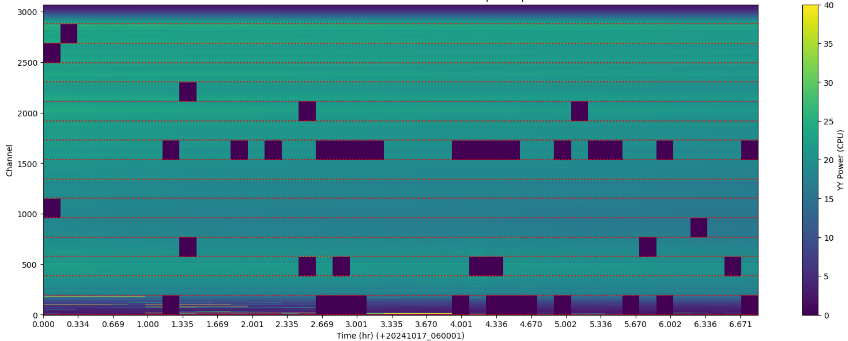
LWA135 - Correlator# 256 - YY - FLAGS: BadSpecShape
