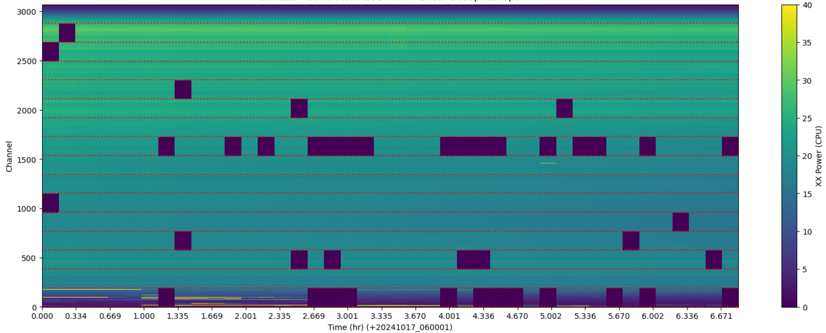
LWA225 - Correlator# 281 - XX - FLAGS: BadSpecShape
