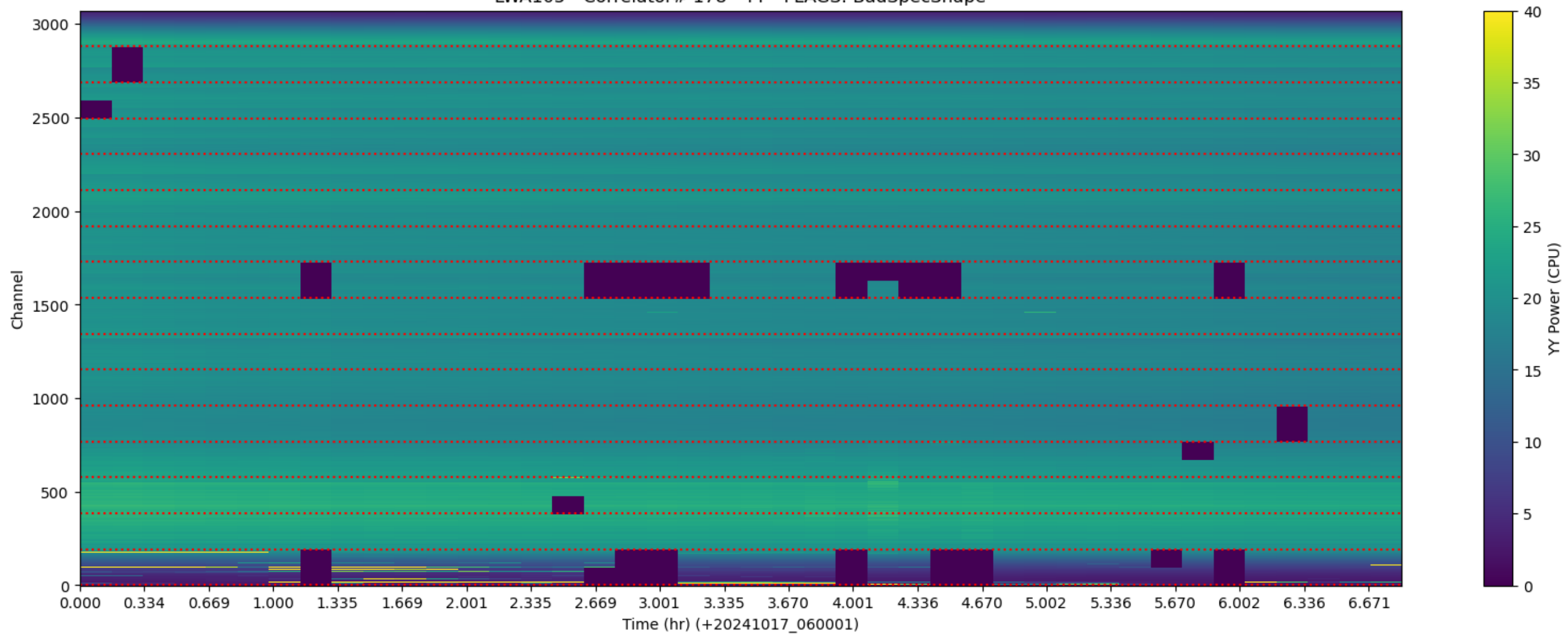
LWA105 - Correlator# 178 - YY - FLAGS: BadSpecShape
