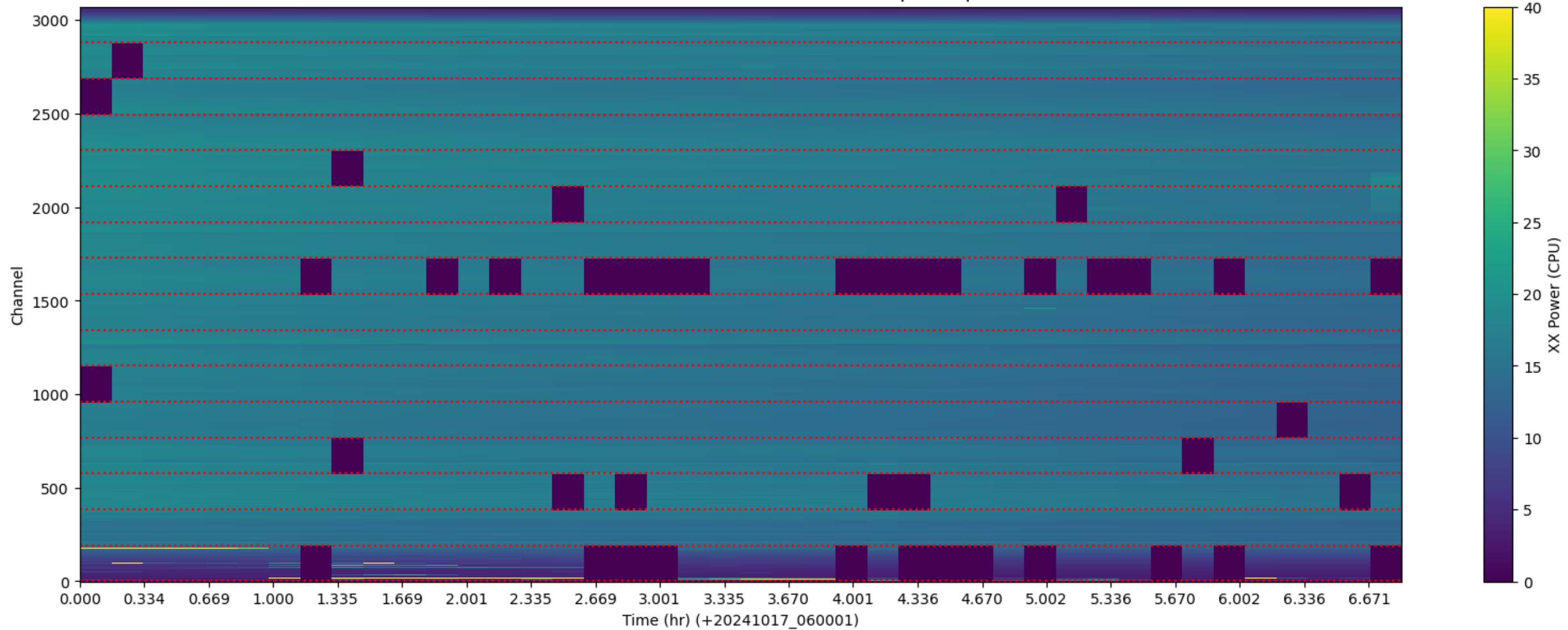
LWA297 - Correlator# 314 - XX - FLAGS: BadSpecShape
