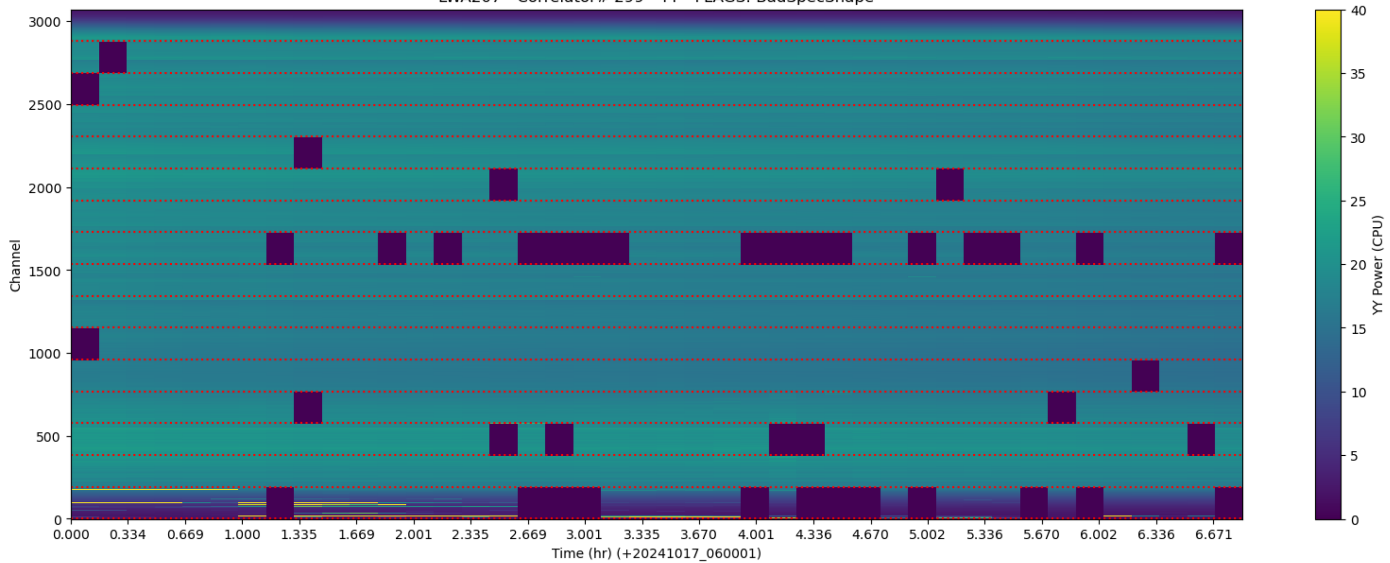
LWA207 - Correlator# 299 - YY - FLAGS: BadSpecShape
