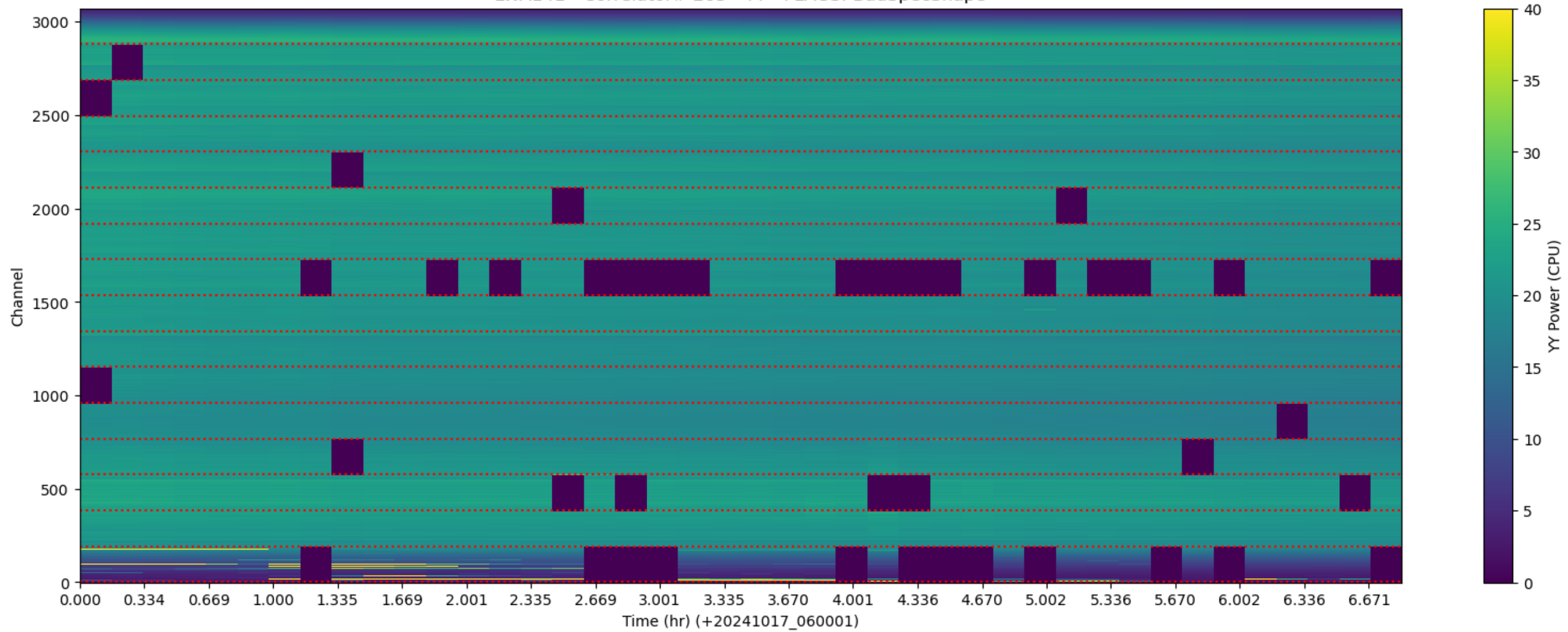
LWA141 - Correlator# 263 - YY - FLAGS: BadSpecShape
