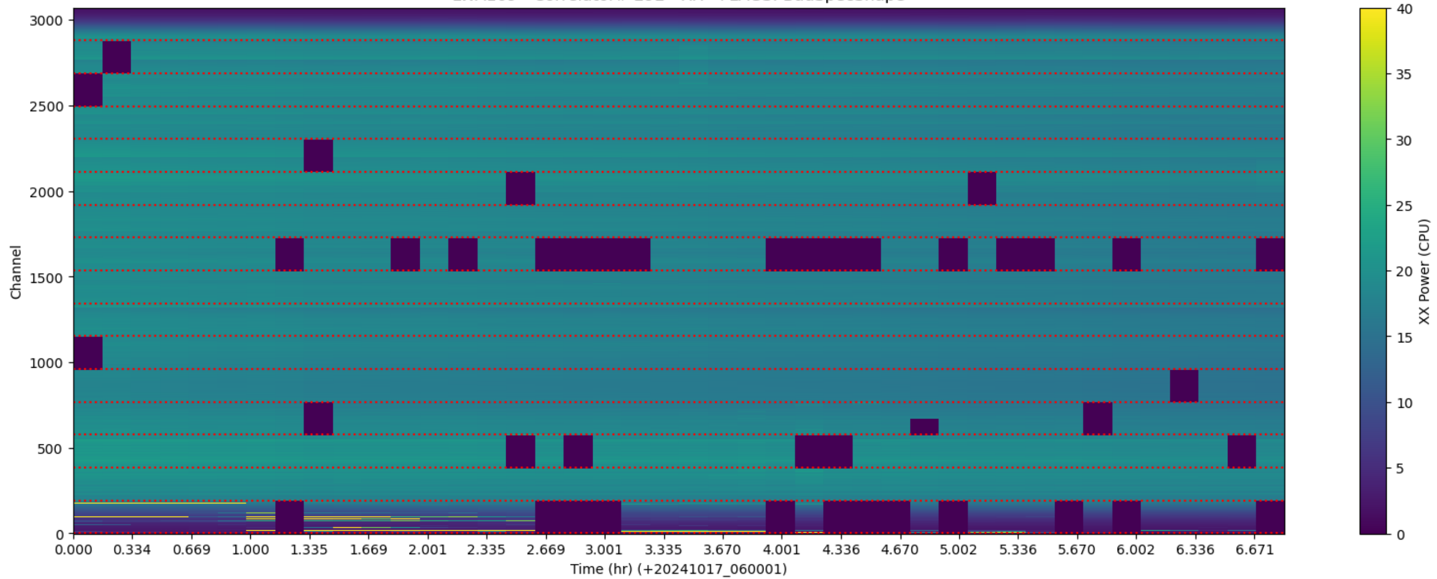
LWA169 - Correlator# 292 - XX - FLAGS: BadSpecShape
