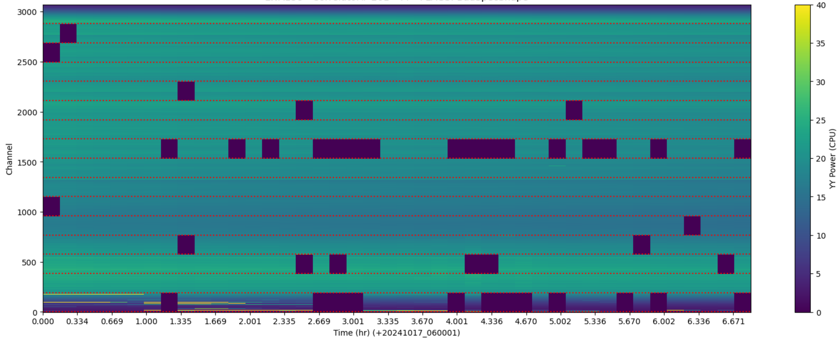
LWA138 - Correlator# 261 - YY - FLAGS: BadSpecShape
