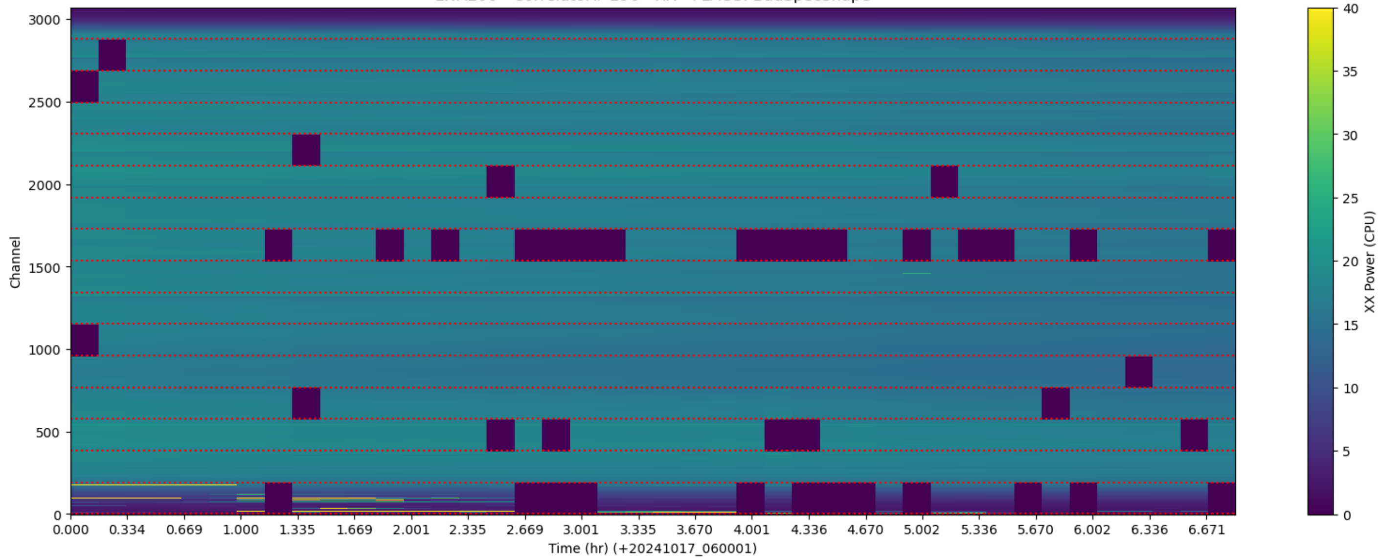
LWA206 - Correlator# 296 - XX - FLAGS: BadSpecShape
