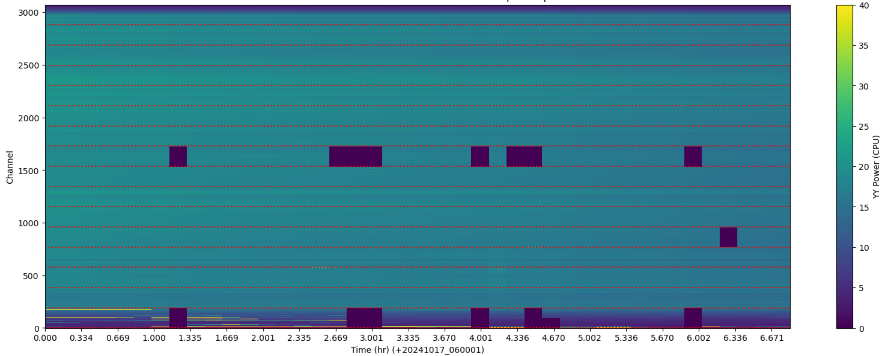
LWA334 - Correlator# 156 - YY - FLAGS: BadSpecShape
