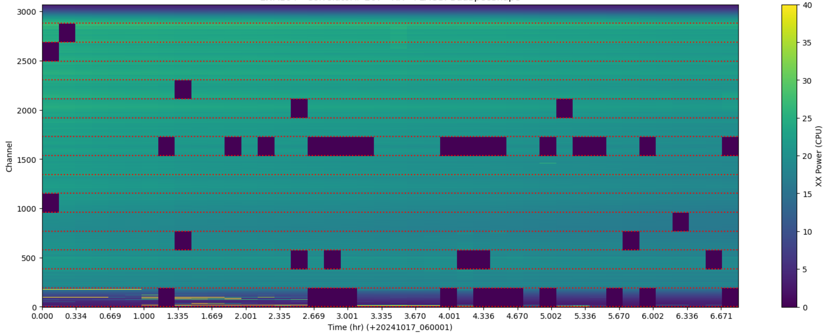
LWA164 - Correlator# 267 - XX - FLAGS: BadSpecShape
