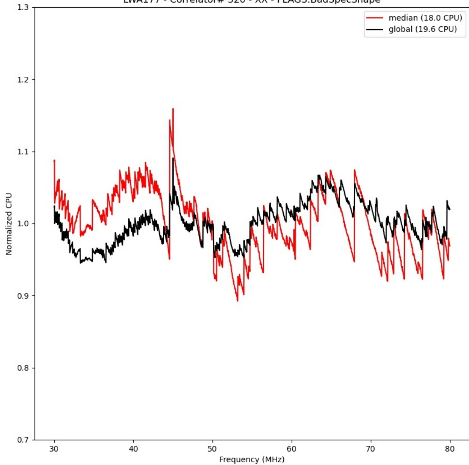
LWA177 - Correlator# 320 - XX - FLAGS:BadSpecShape
