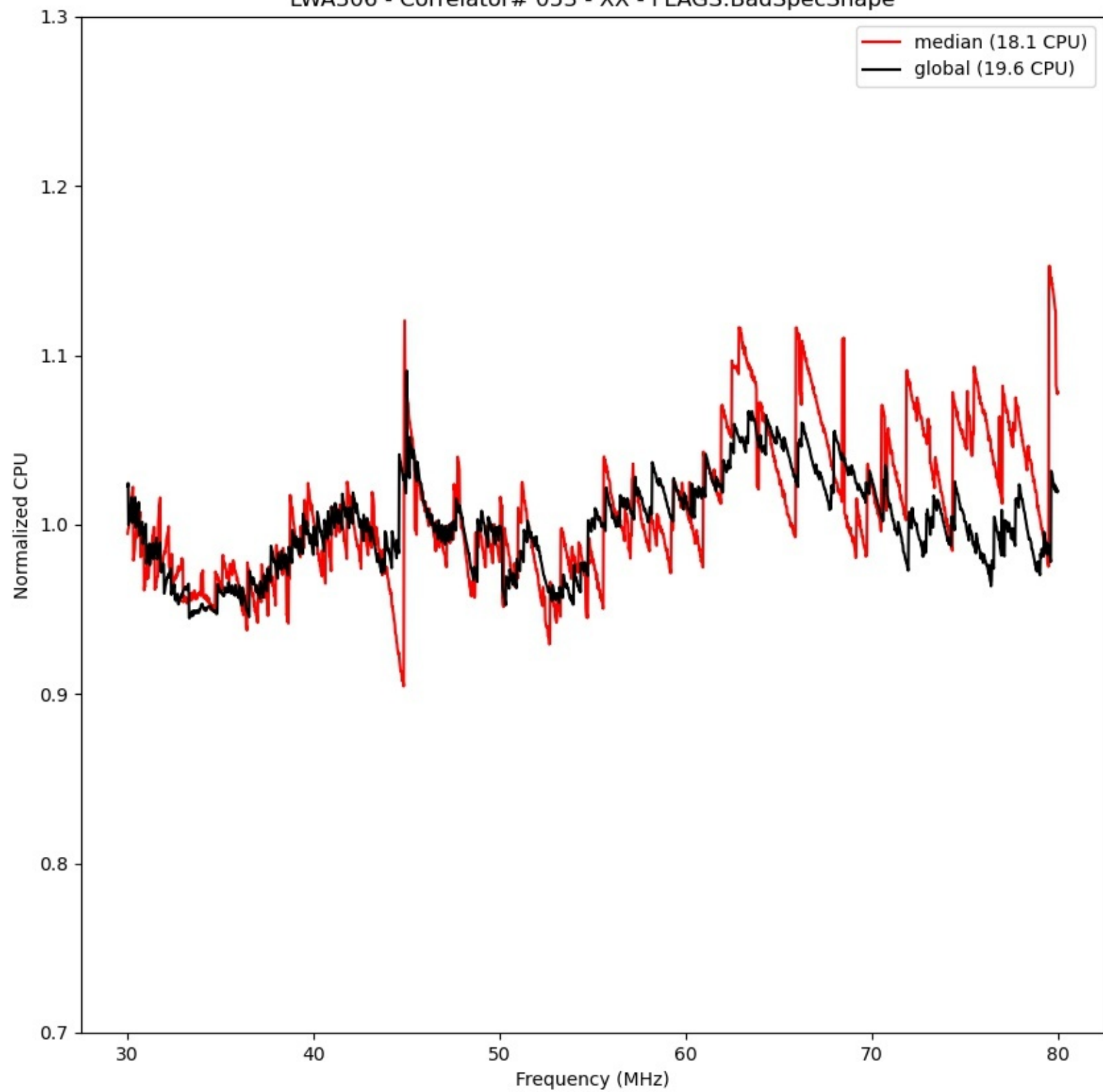
LWA306 - Correlator# 053 - XX - FLAGS:BadSpecShape
