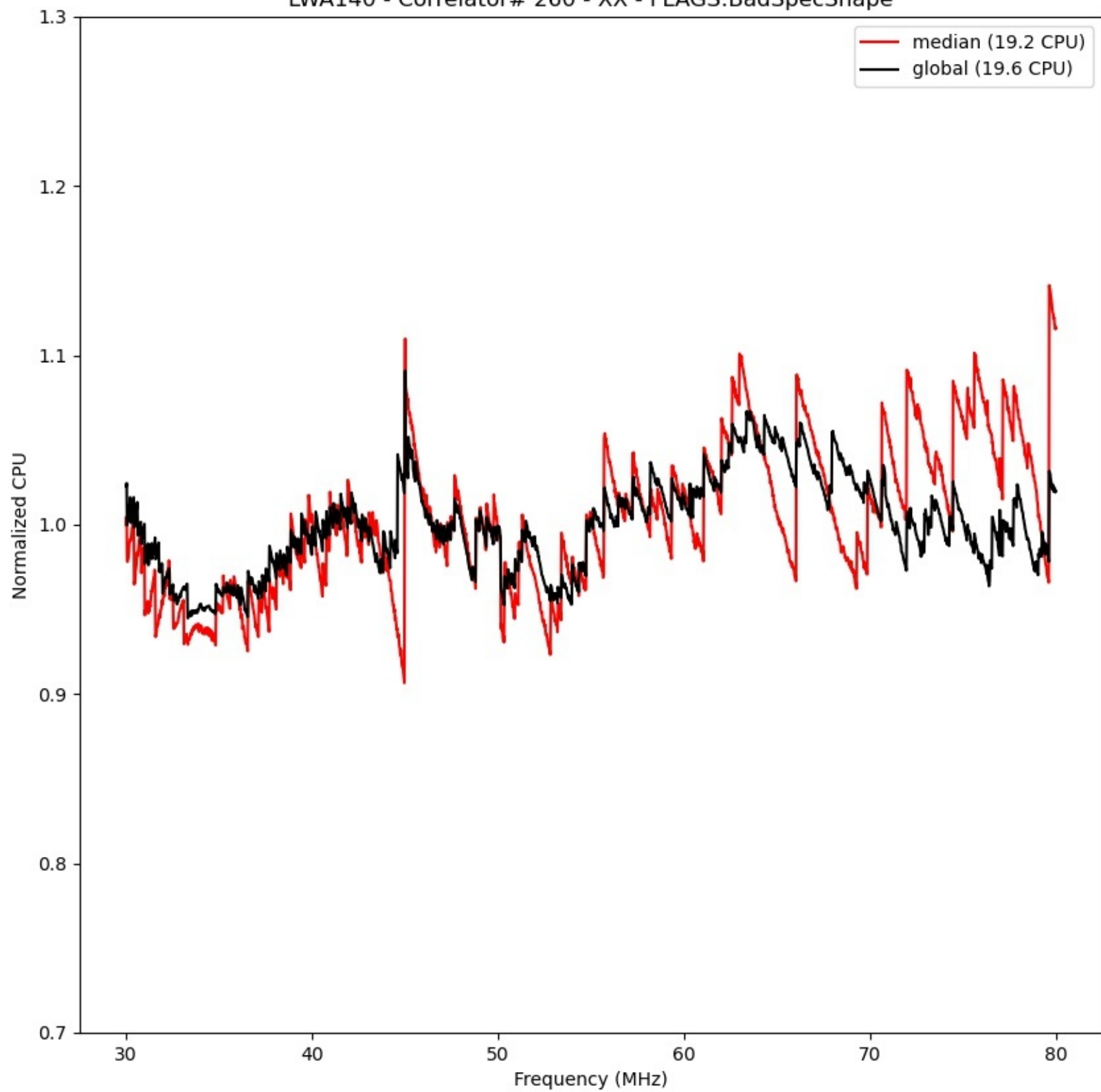
LWA140 - Correlator# 260 - XX - FLAGS:BadSpecShape
