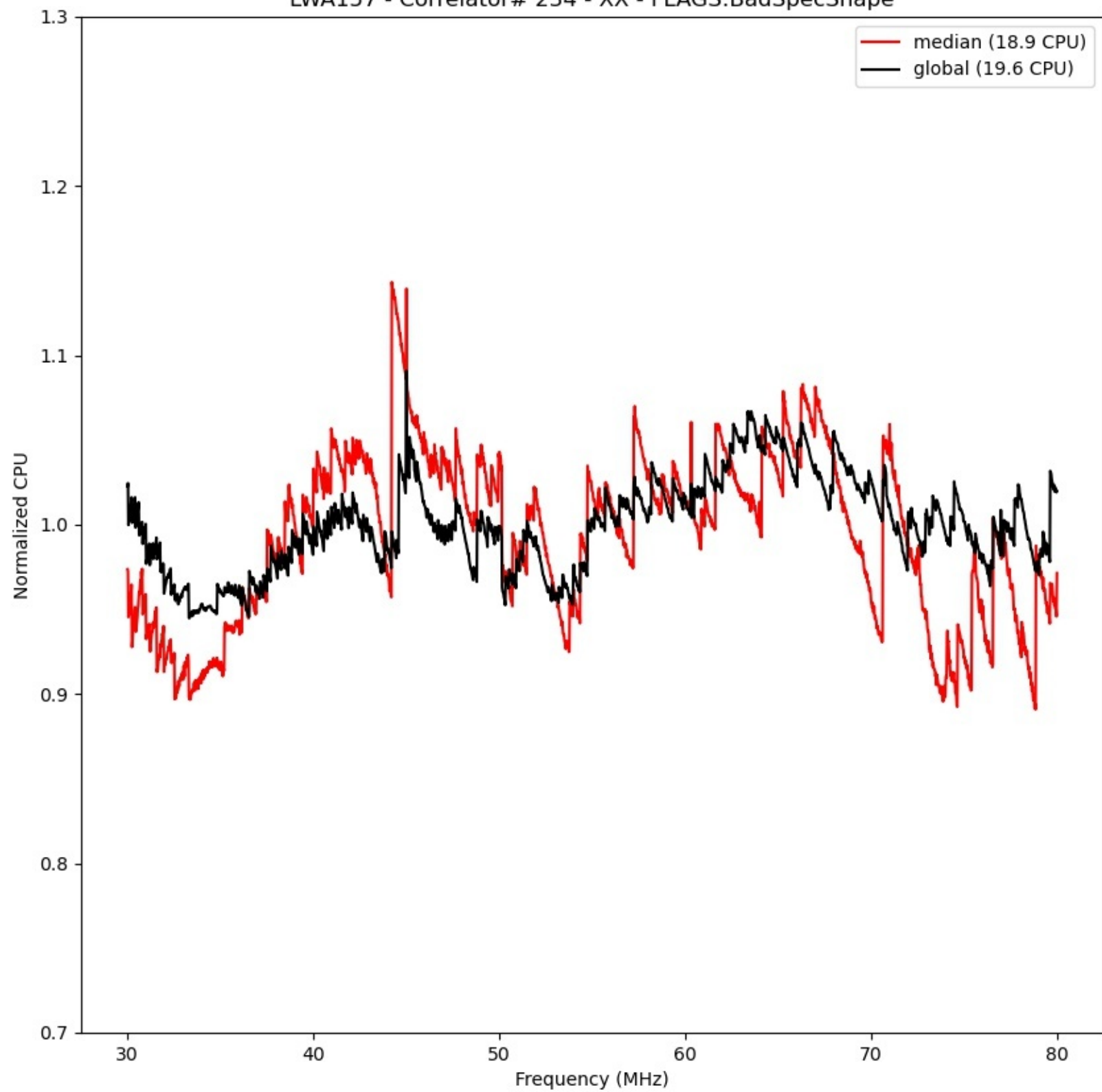
LWA157 - Correlator# 234 - XX - FLAGS:BadSpecShape
