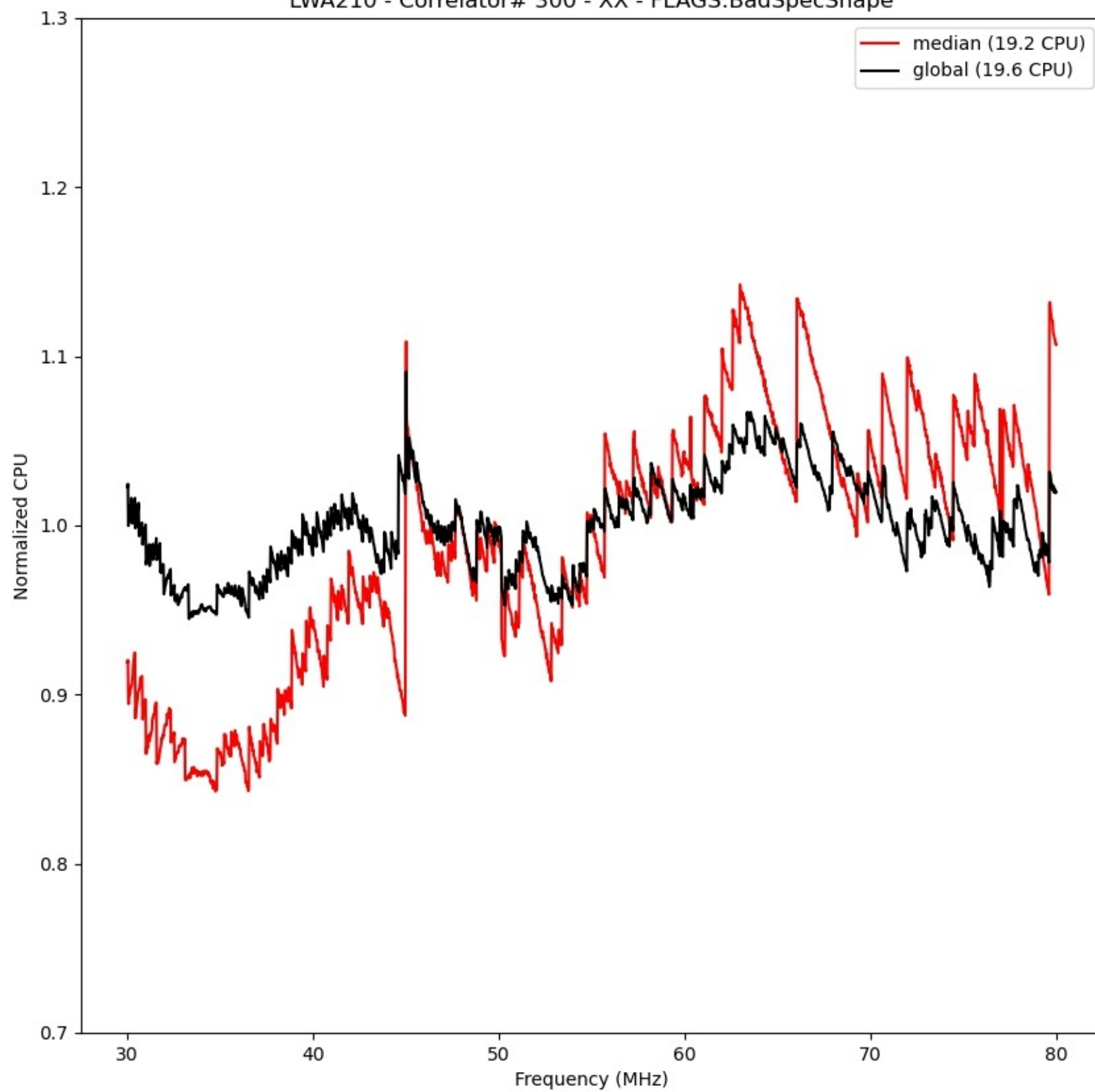
LWA210 - Correlator# 300 - XX - FLAGS:BadSpecShape
