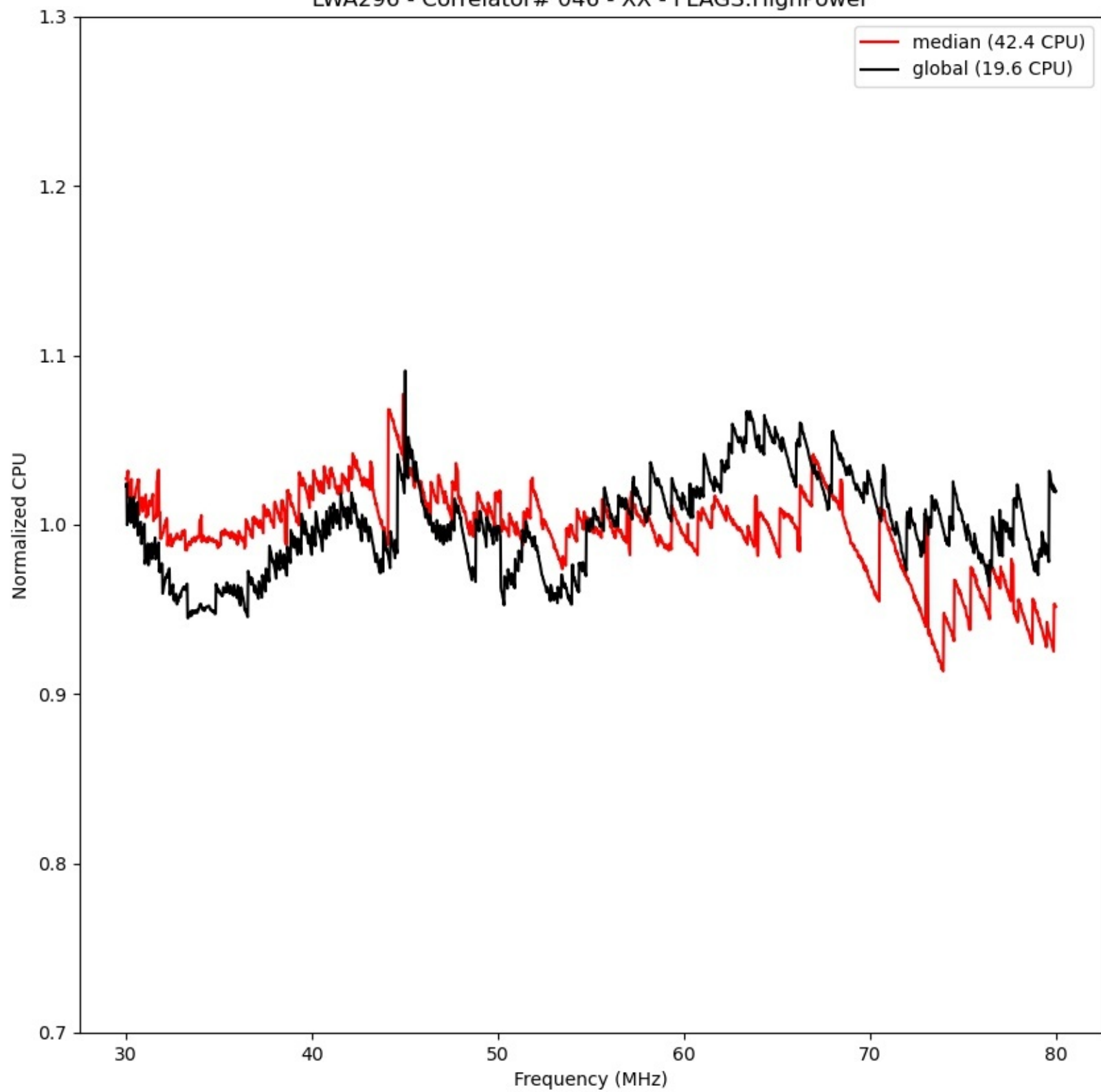
LWA296 - Correlator# 046 - XX - FLAGS:HighPower
