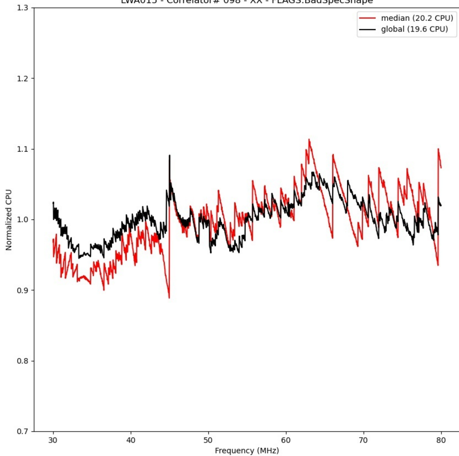
LWA015 - Correlator# 098 - XX - FLAGS:BadSpecShape
