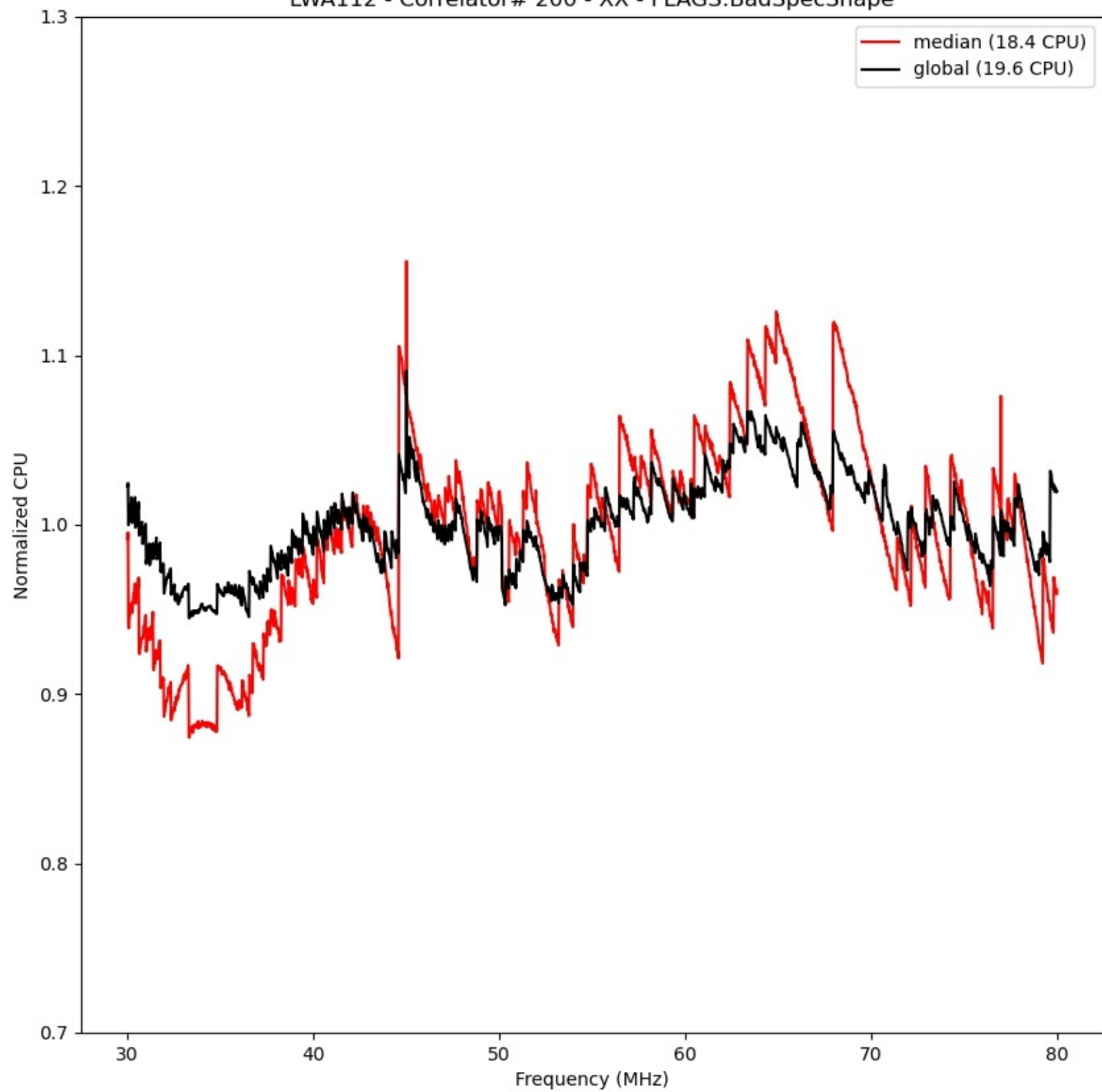
LWA112 - Correlator# 200 - XX - FLAGS:BadSpecShape
