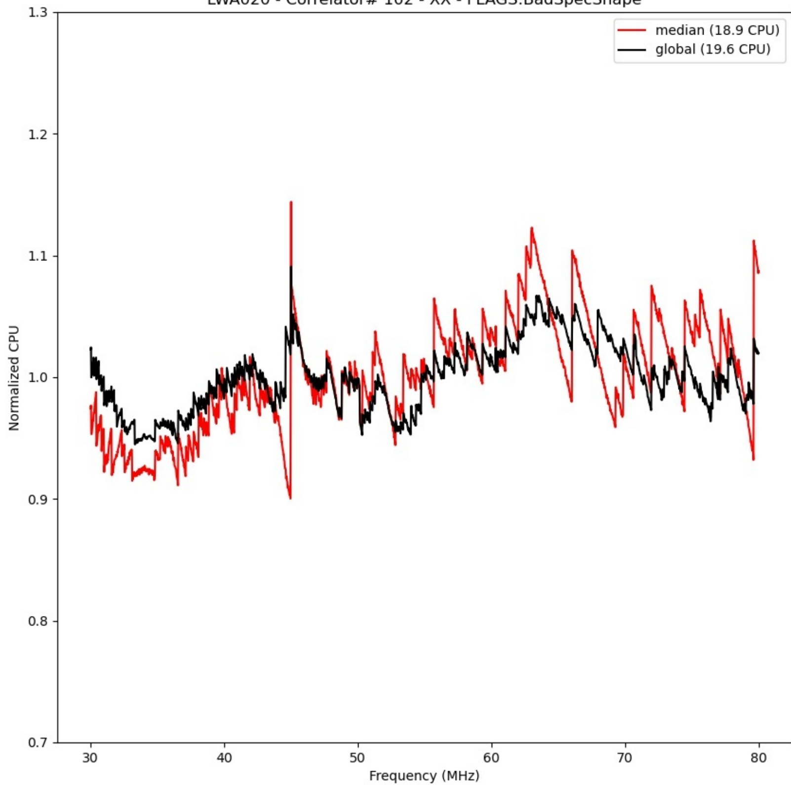
LWA020 - Correlator# 102 - XX - FLAGS:BadSpecShape
