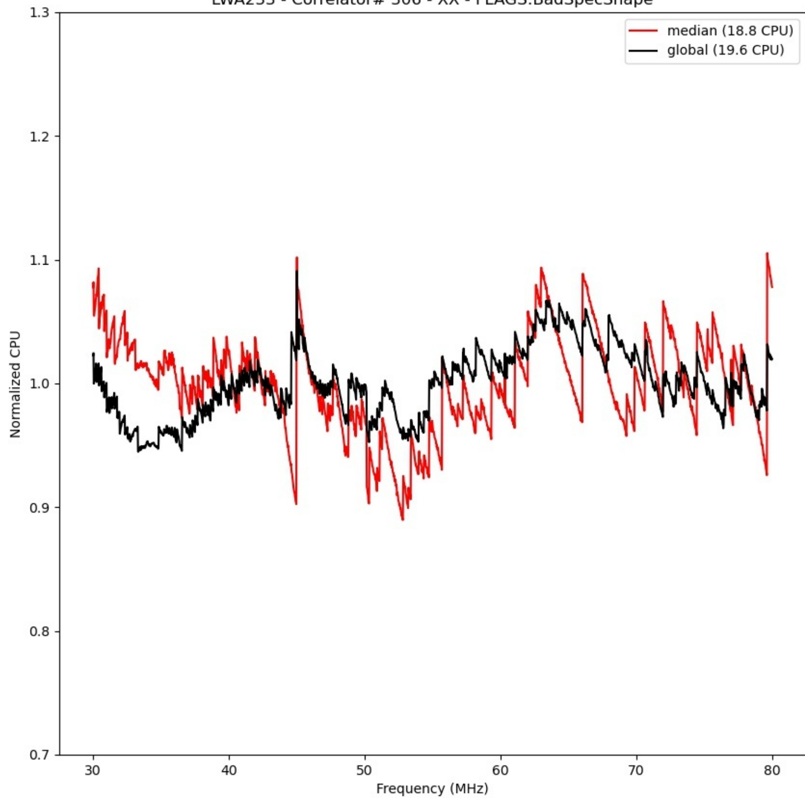
LWA233 - Correlator# 306 - XX - FLAGS:BadSpecShape
