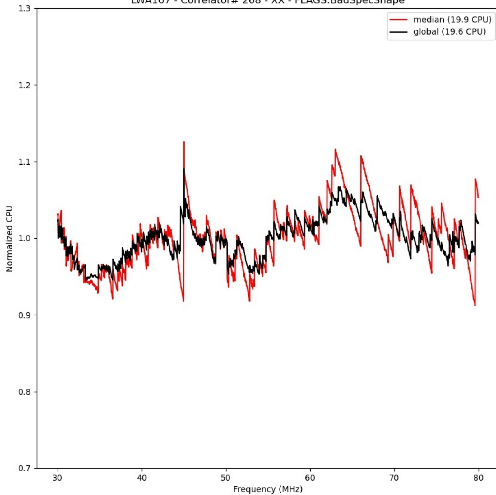
LWA167 - Correlator# 268 - XX - FLAGS:BadSpecShape
