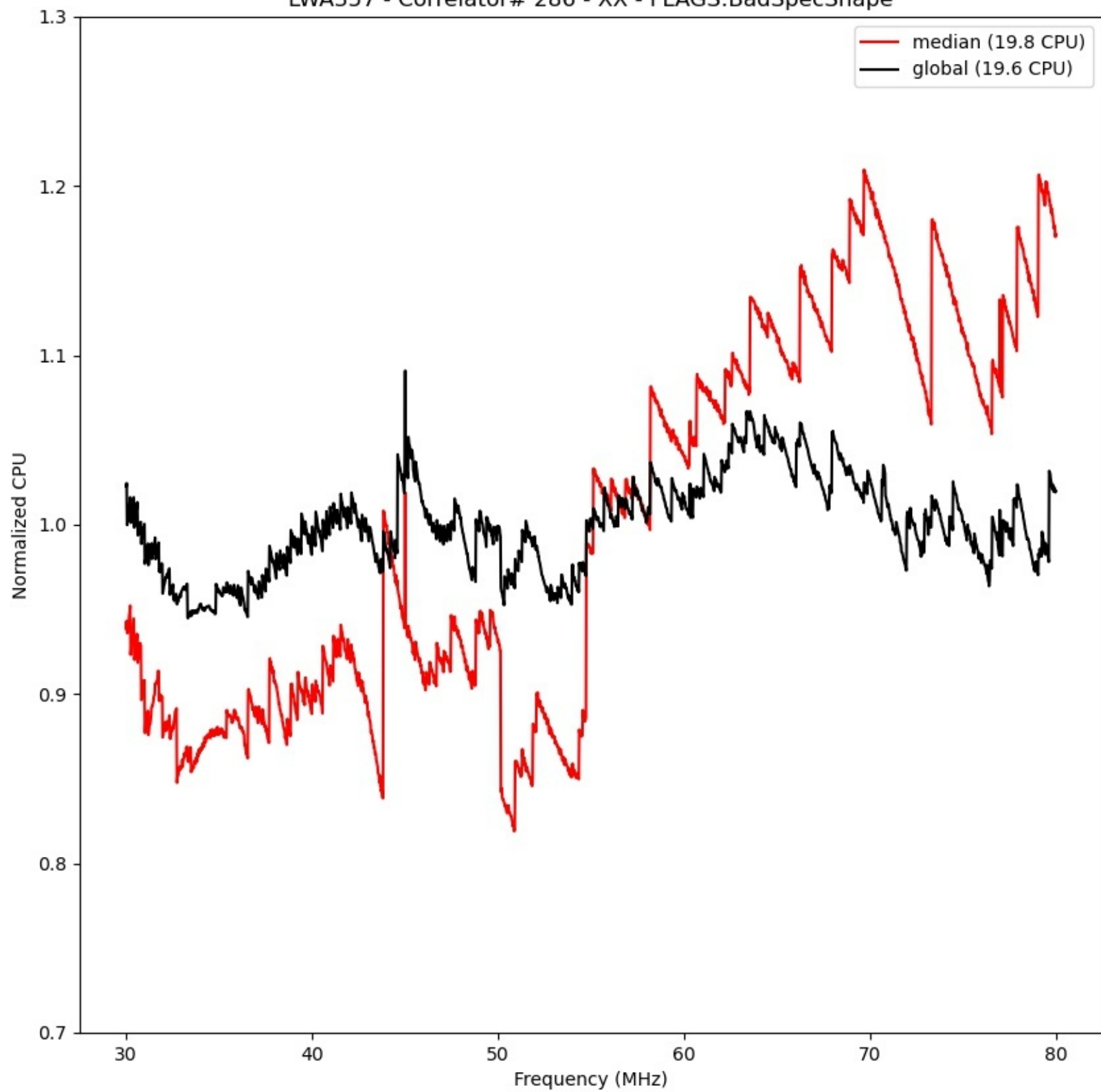
LWA357 - Correlator# 286 - XX - FLAGS:BadSpecShape
