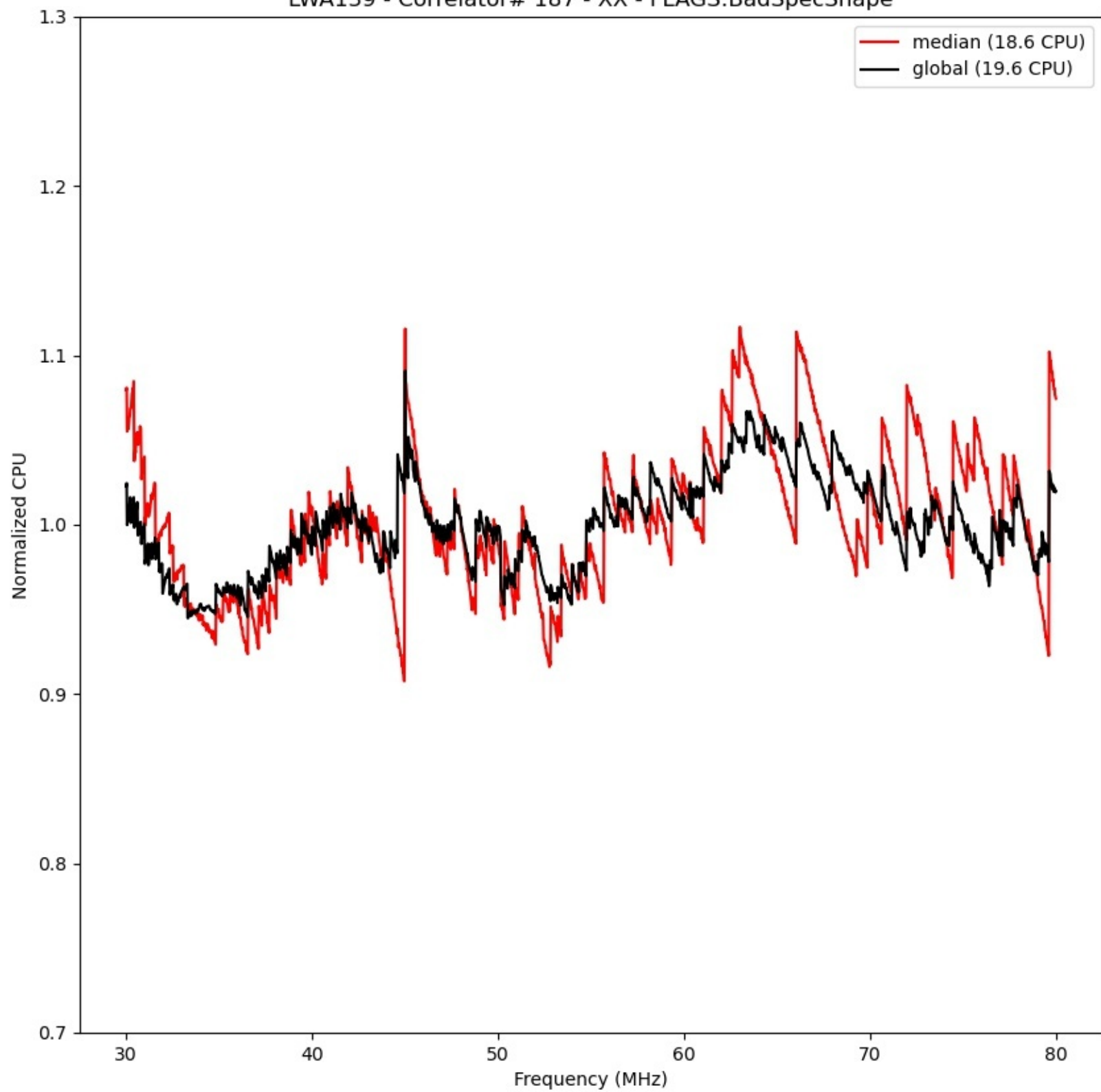
LWA139 - Correlator# 187 - XX - FLAGS:BadSpecShape
