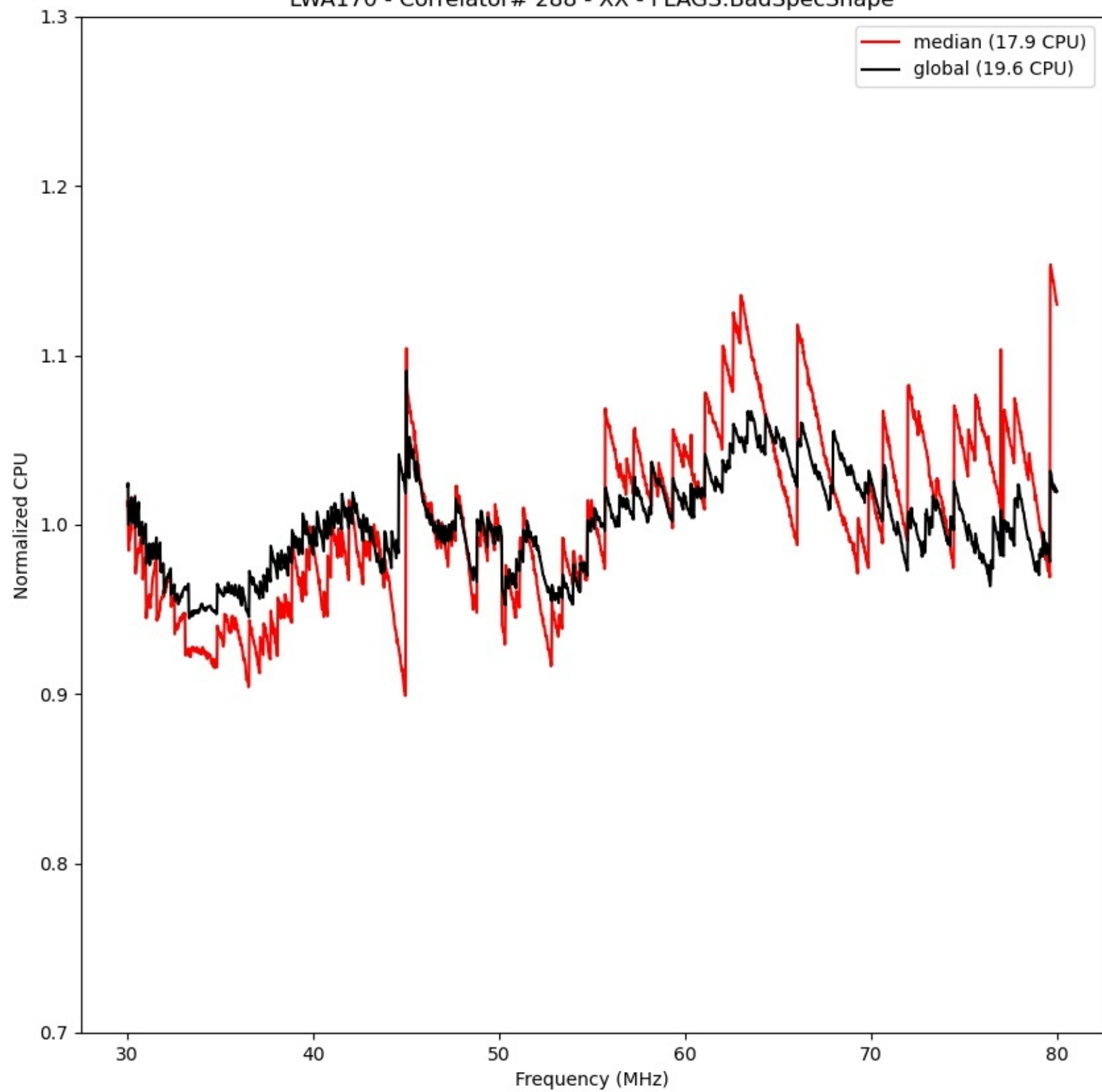
LWA170 - Correlator# 288 - XX - FLAGS:BadSpecShape
