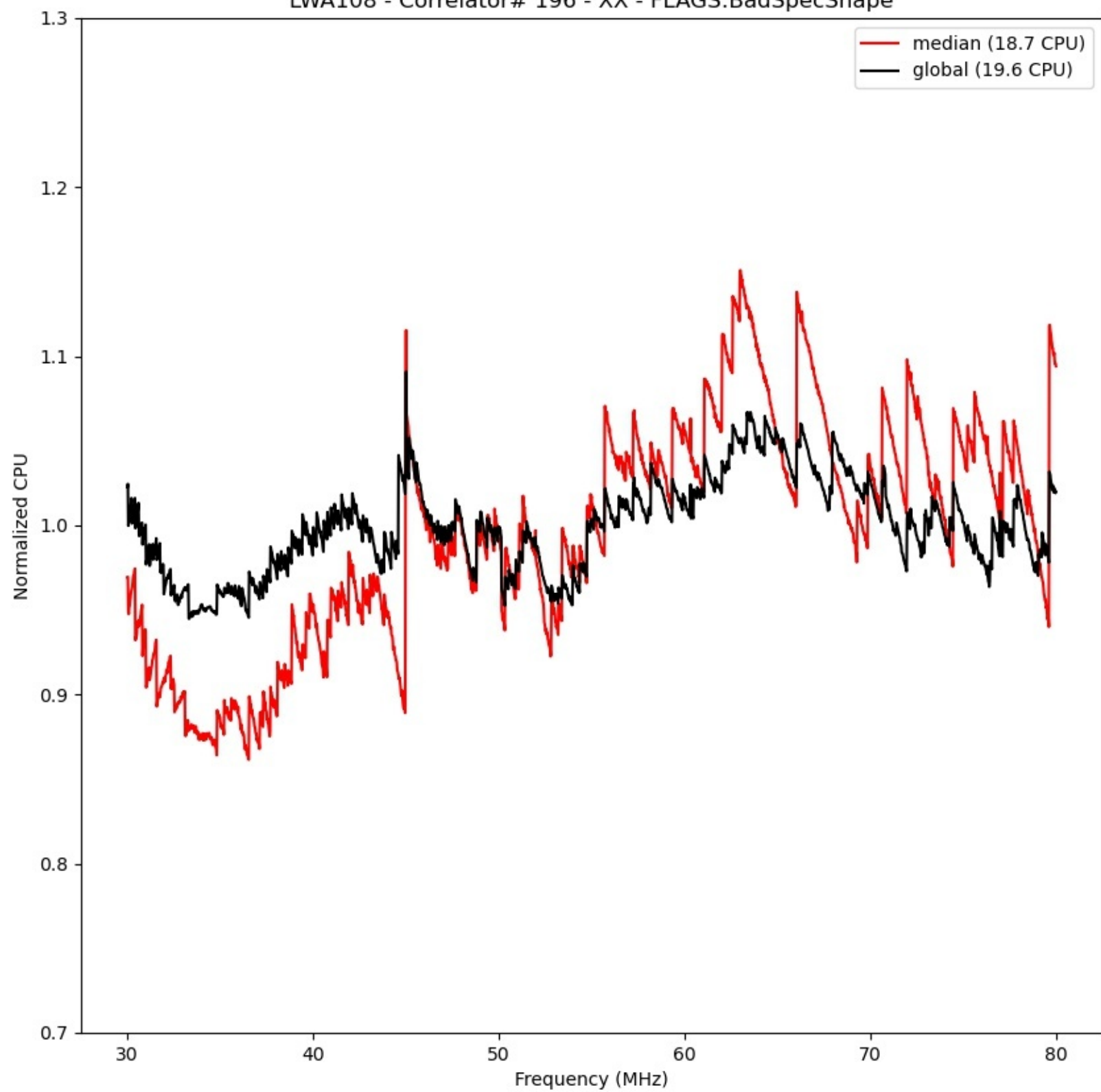
LWA108 - Correlator# 196 - XX - FLAGS:BadSpecShape
