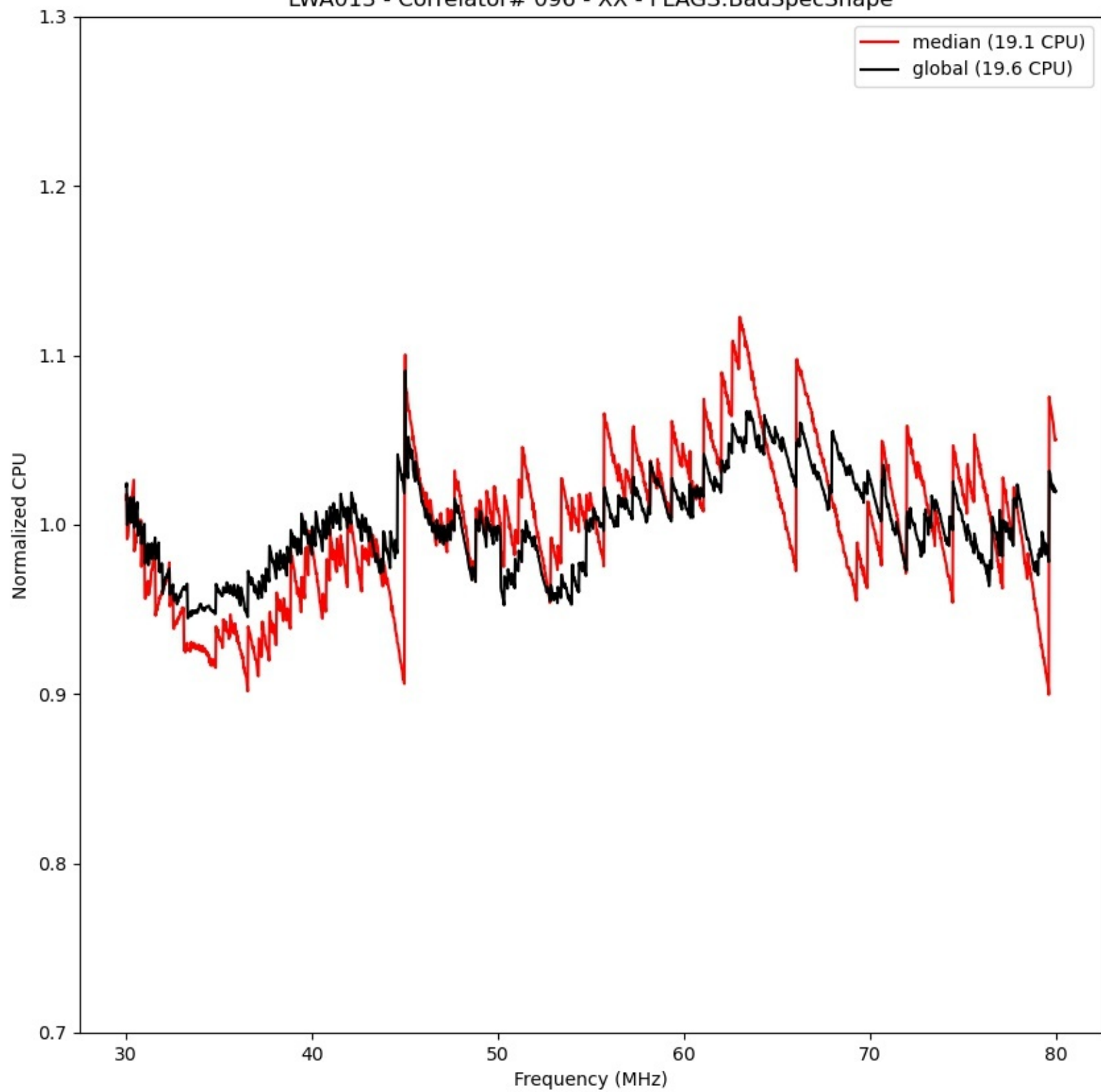
LWA013 - Correlator# 096 - XX - FLAGS:BadSpecShape
