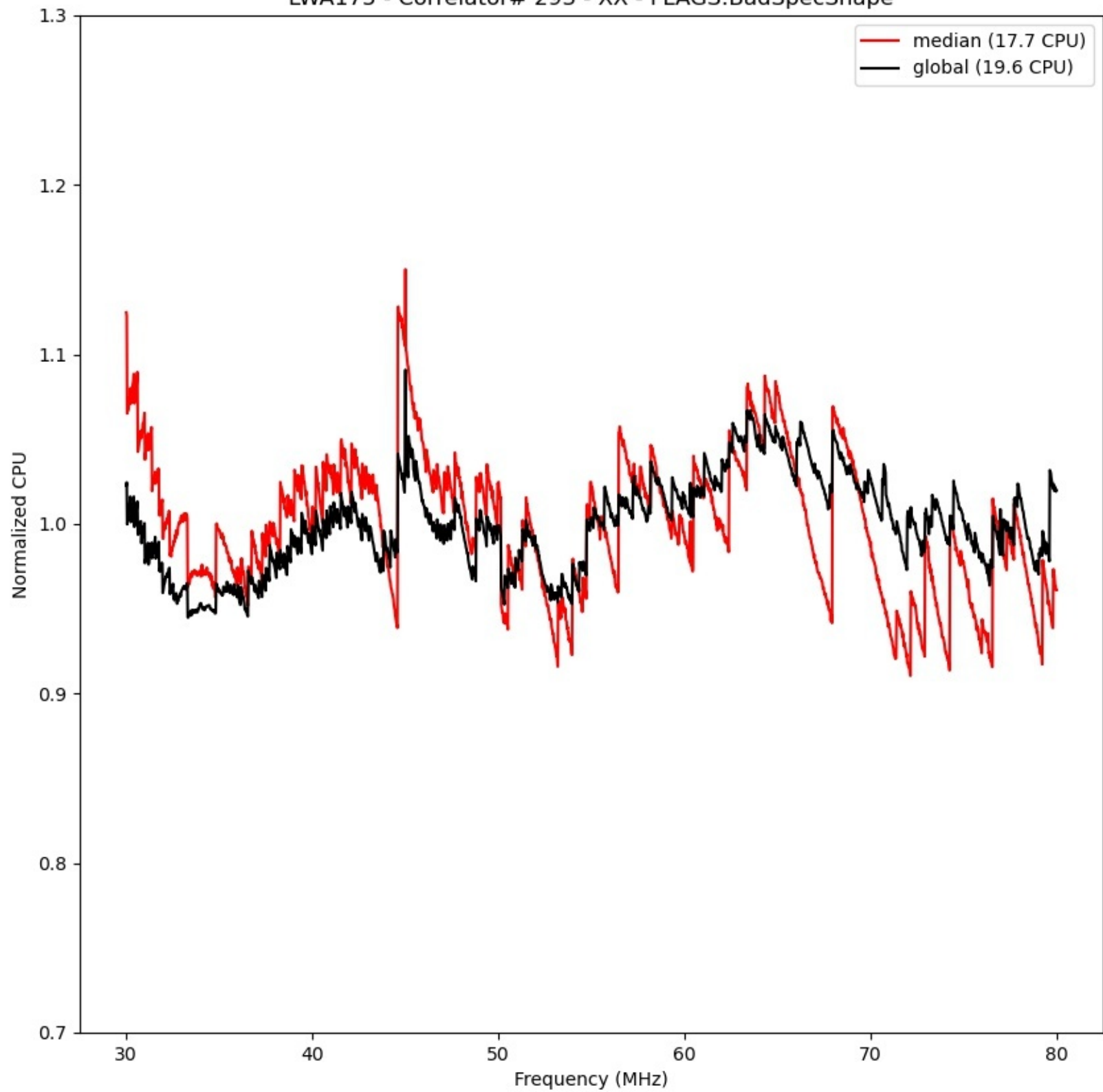
LWA175 - Correlator# 293 - XX - FLAGS:BadSpecShape
