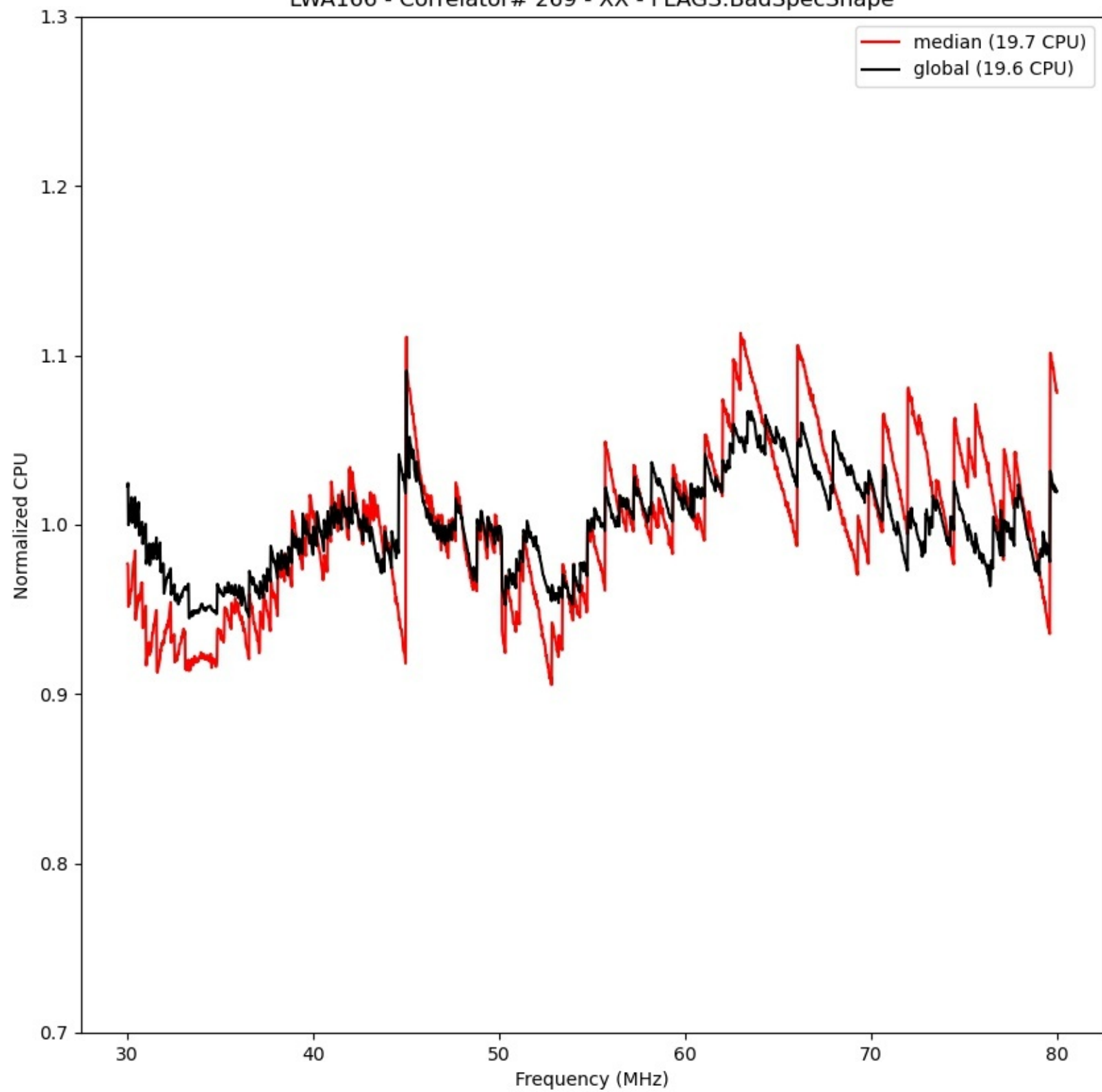
LWA166 - Correlator# 269 - XX - FLAGS:BadSpecShape
