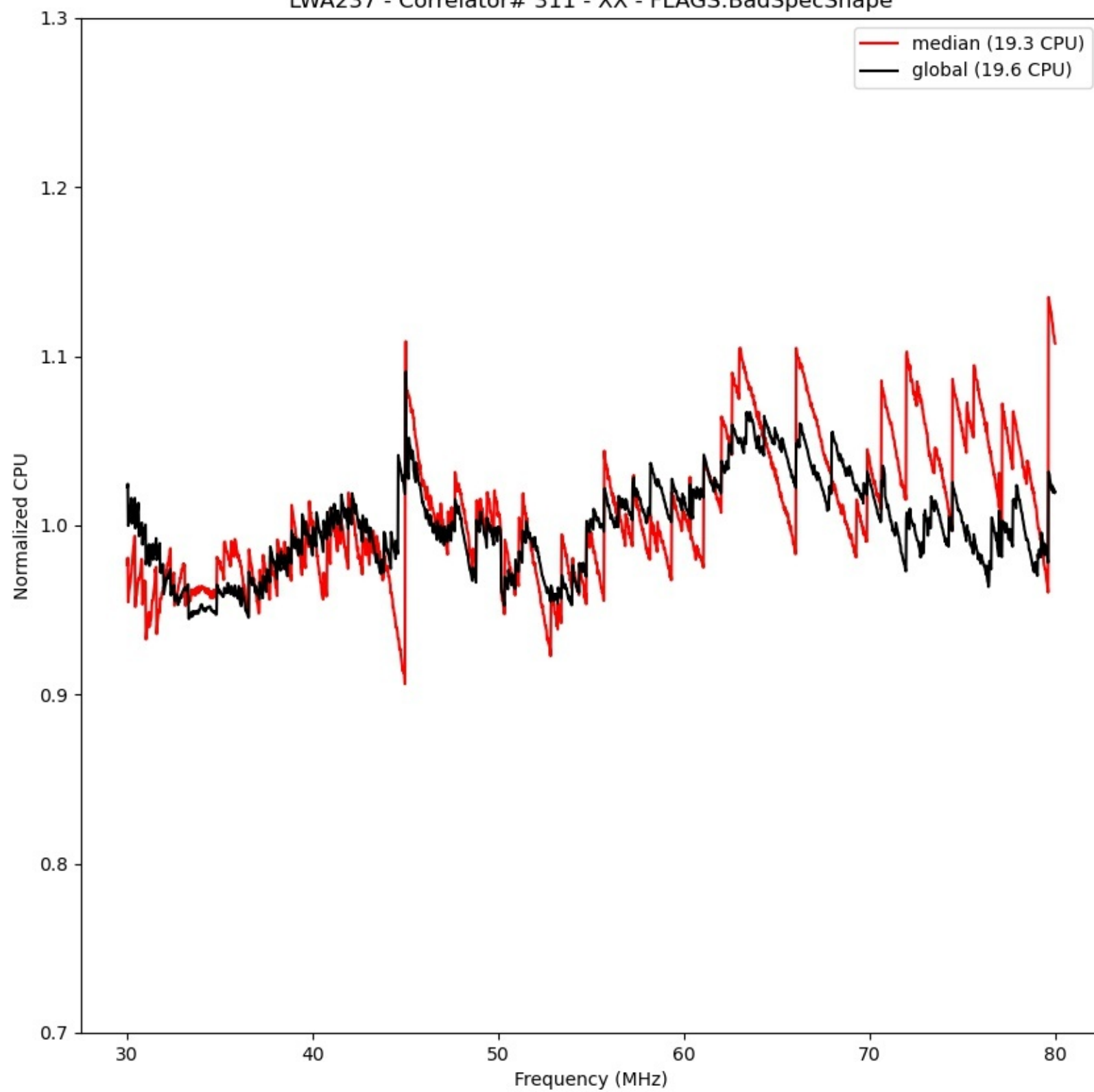
LWA237 - Correlator# 311 - XX - FLAGS:BadSpecShape
