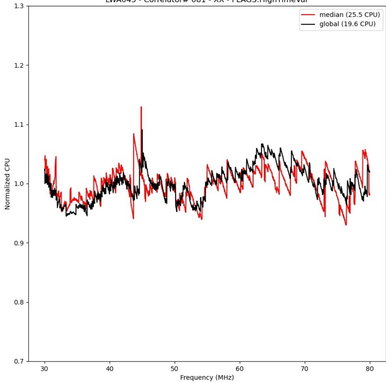
LWA043 - Correlator# 081 - XX - FLAGS:HighTimeVar
