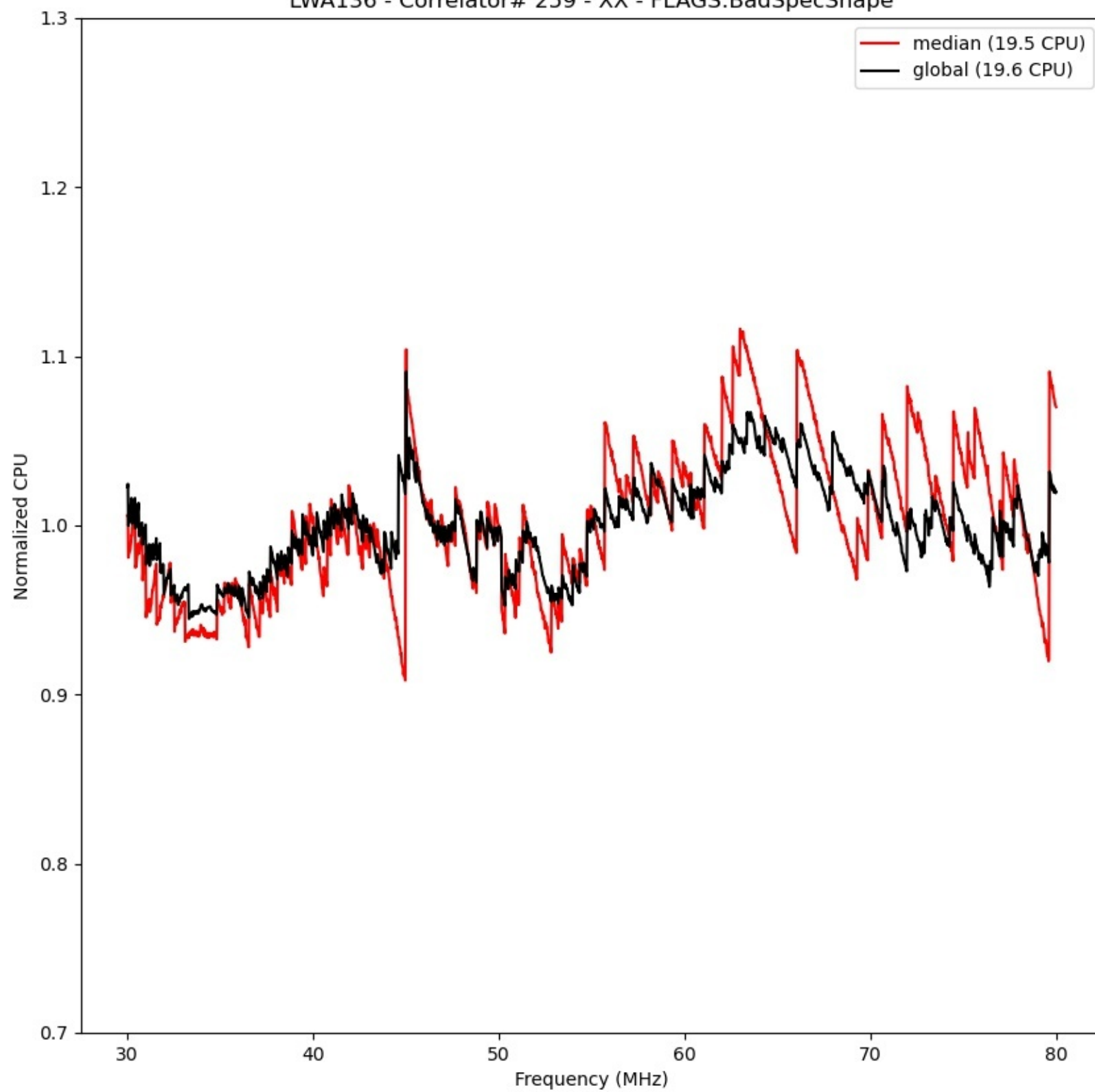
LWA136 - Correlator# 259 - XX - FLAGS:BadSpecShape
