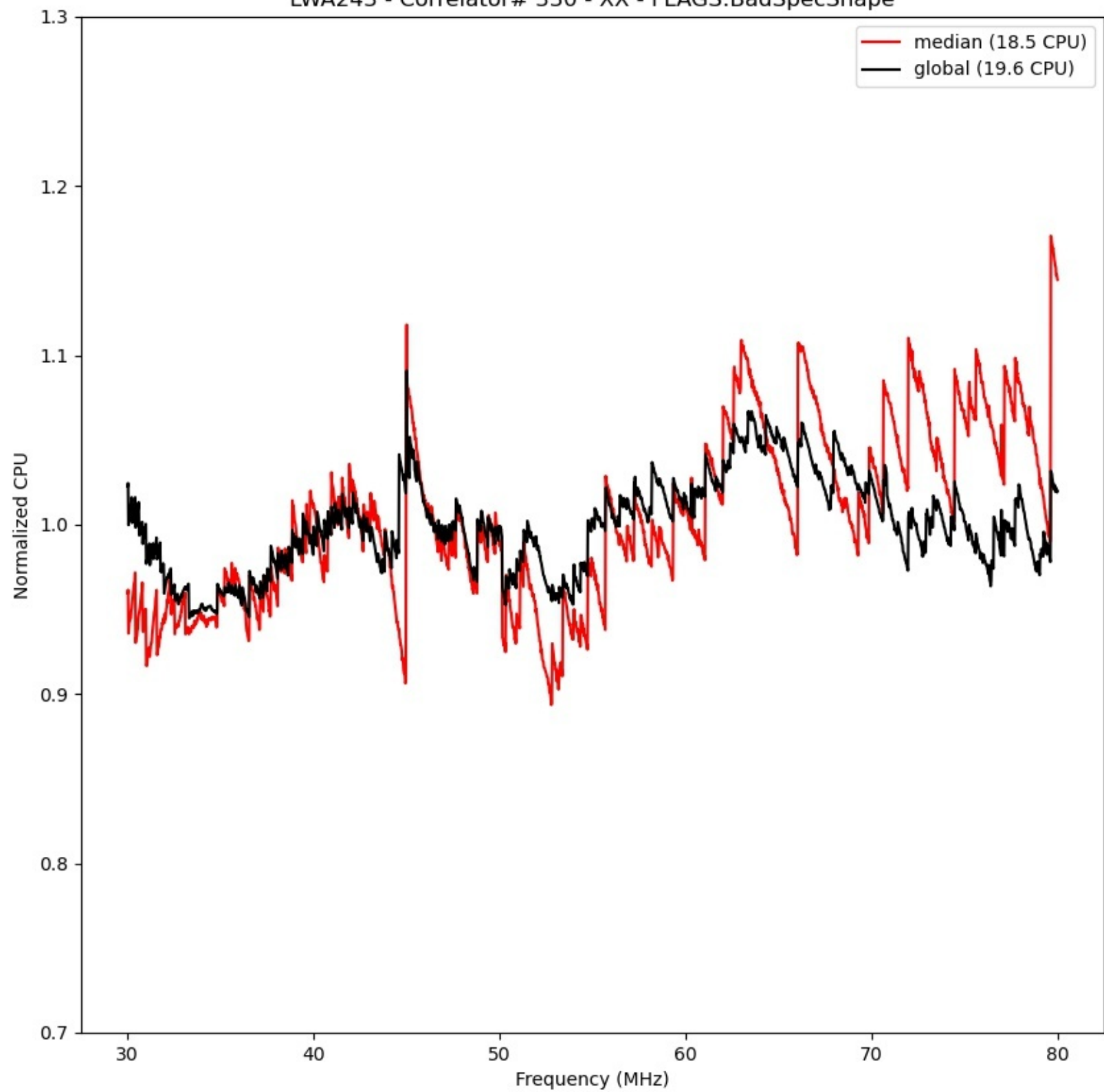
LWA243 - Correlator# 330 - XX - FLAGS:BadSpecShape
