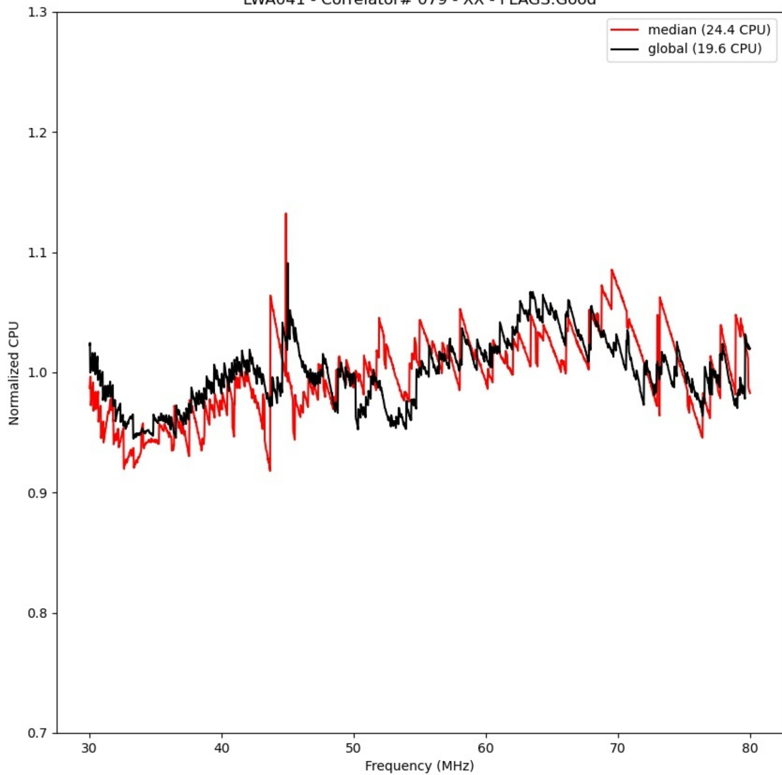
LWA041 - Correlator# 079 - XX - FLAGS:Good
