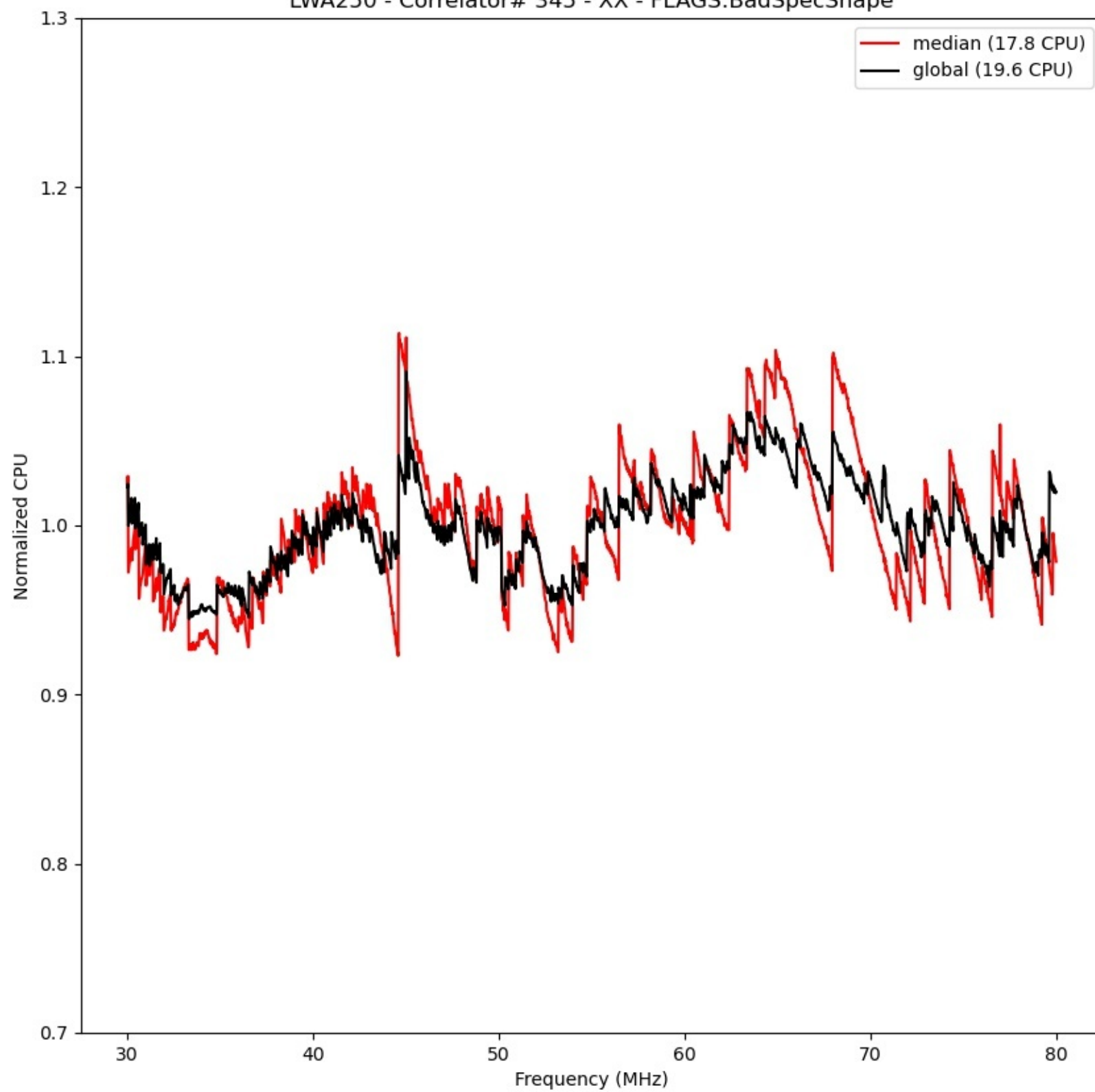
LWA250 - Correlator# 345 - XX - FLAGS:BadSpecShape
