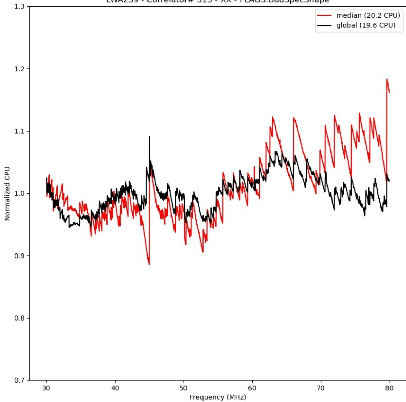
LWA239 - Correlator# 313 - XX - FLAGS:BadSpecShape
