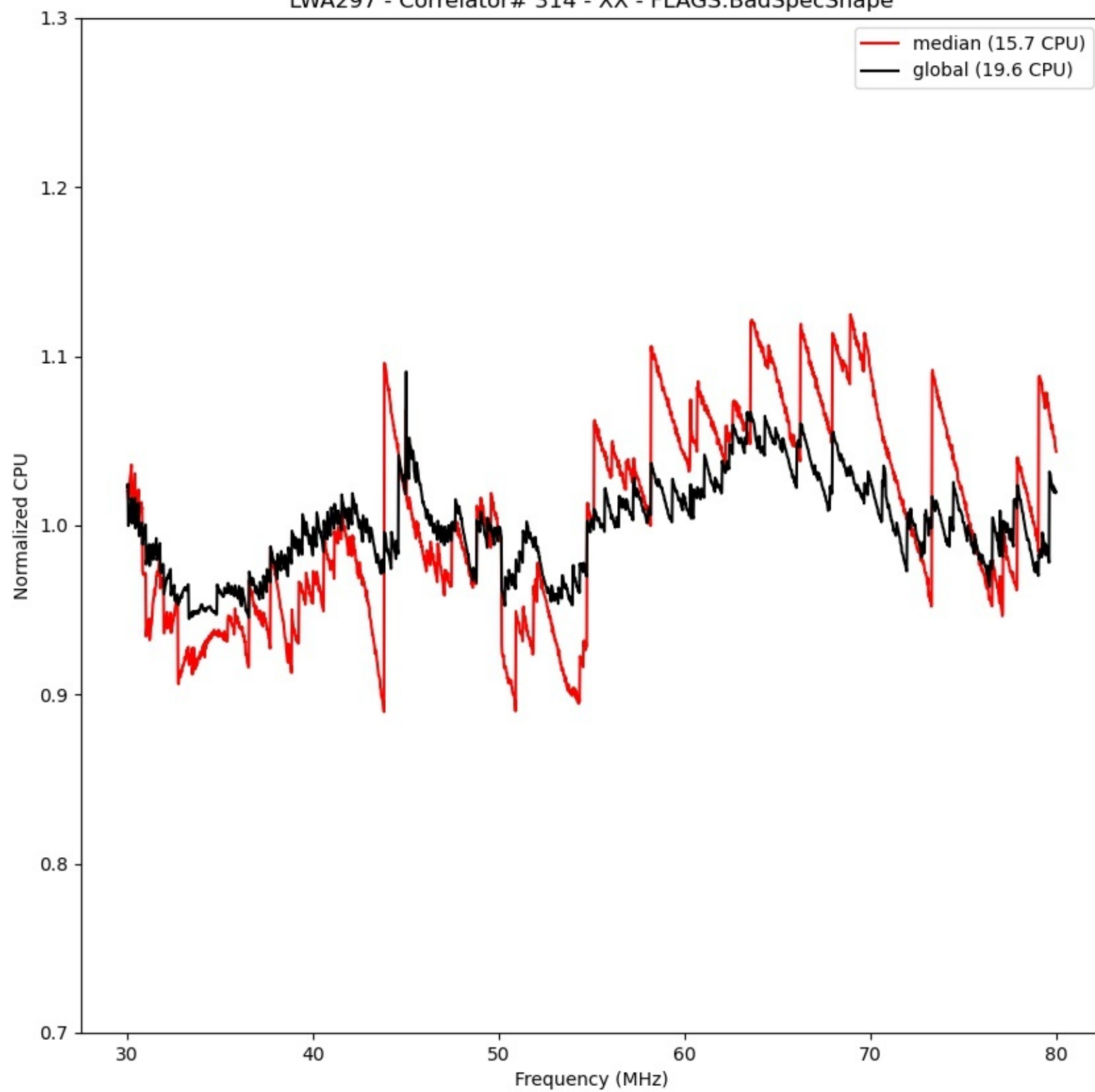
LWA297 - Correlator# 314 - XX - FLAGS:BadSpecShape
