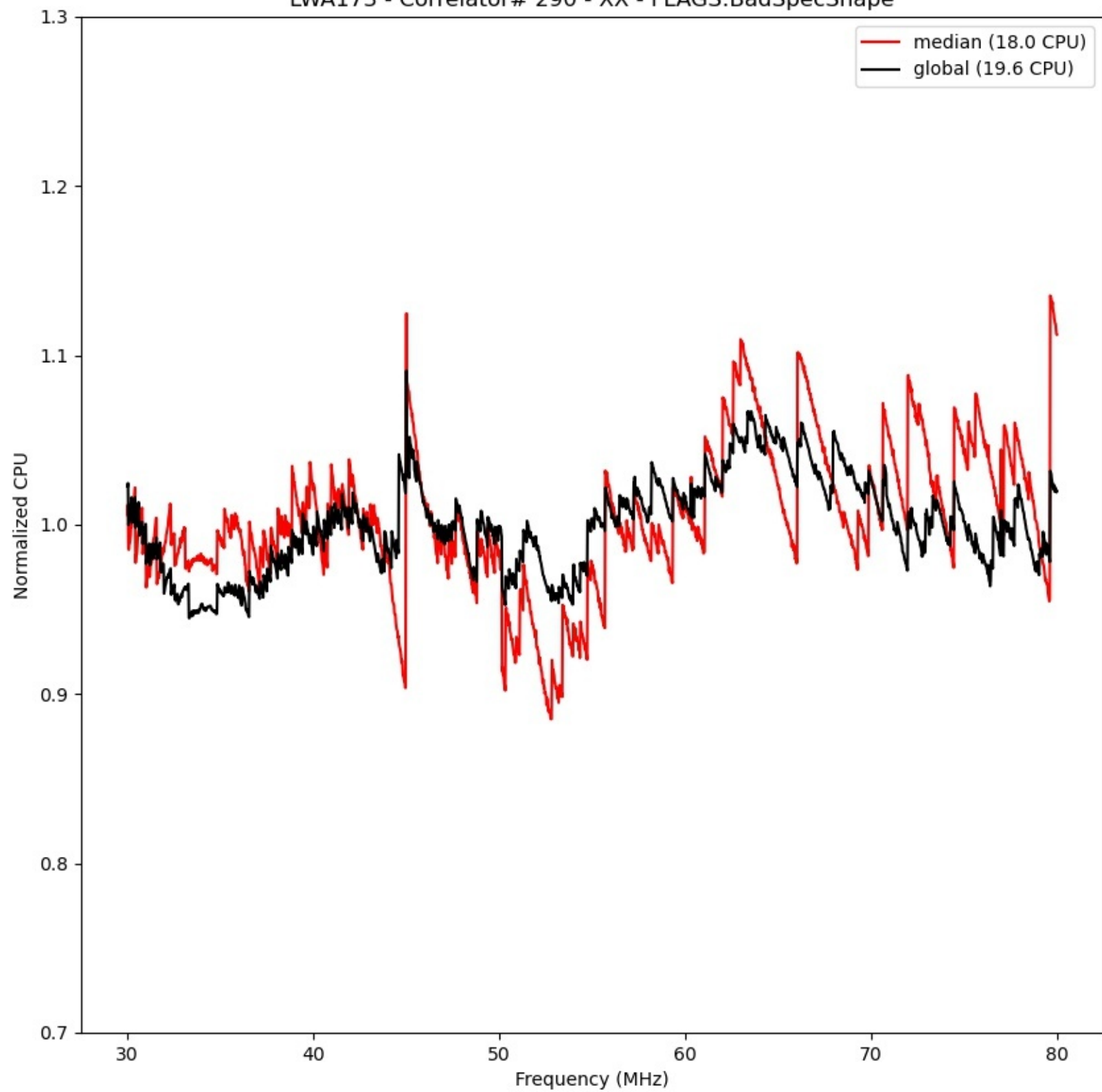
LWA173 - Correlator# 290 - XX - FLAGS:BadSpecShape
