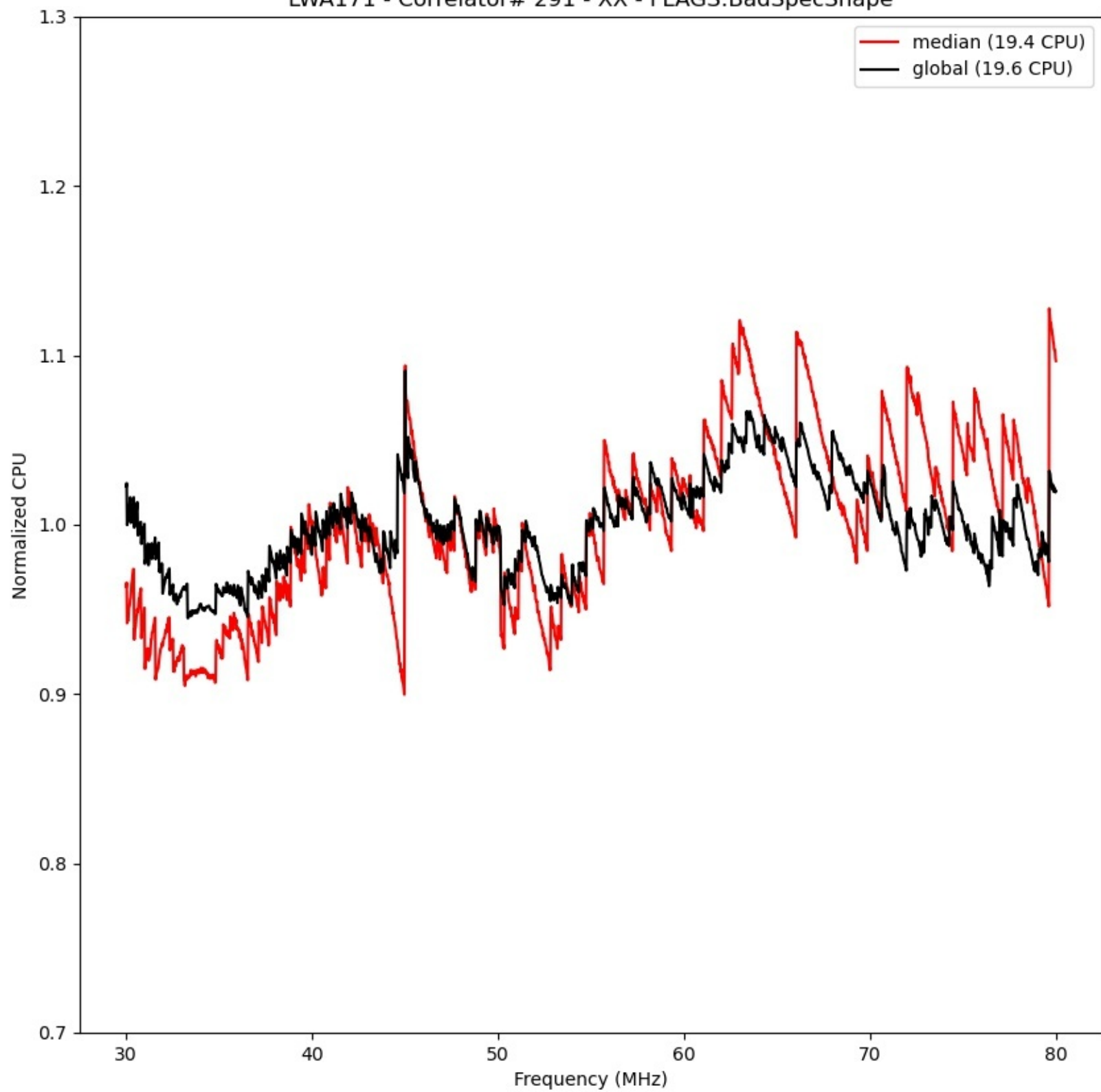
LWA171 - Correlator# 291 - XX - FLAGS:BadSpecShape
