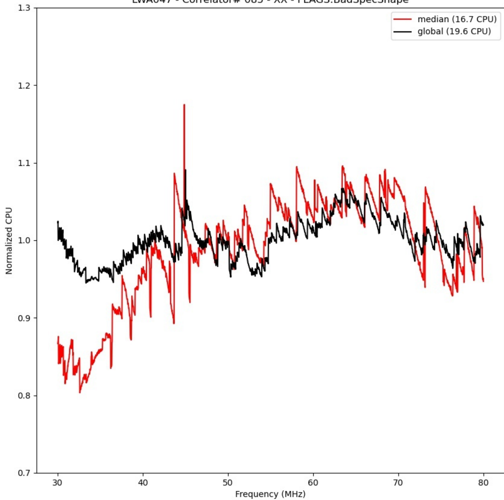
LWA047 - Correlator# 085 - XX - FLAGS:BadSpecShape
