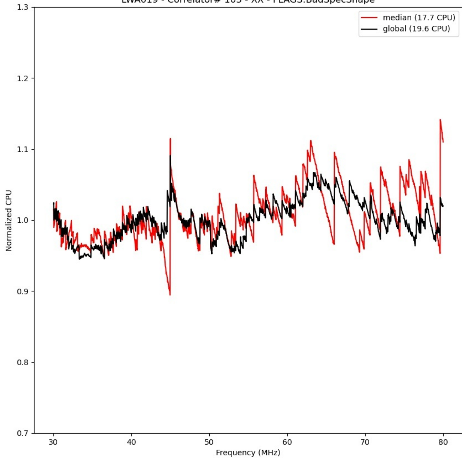
LWA019 - Correlator# 103 - XX - FLAGS:BadSpecShape
