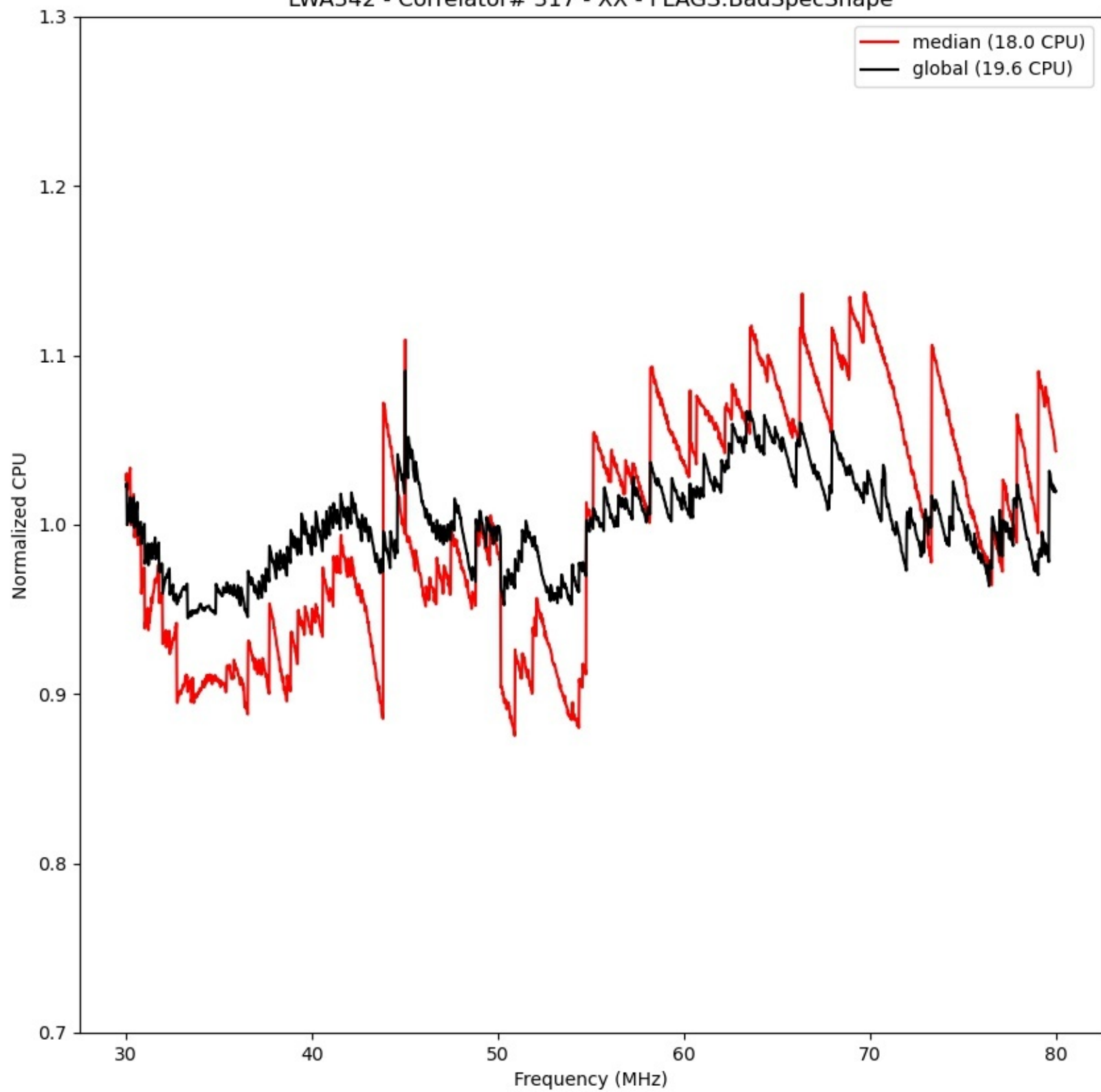
LWA342 - Correlator# 317 - XX - FLAGS:BadSpecShape
