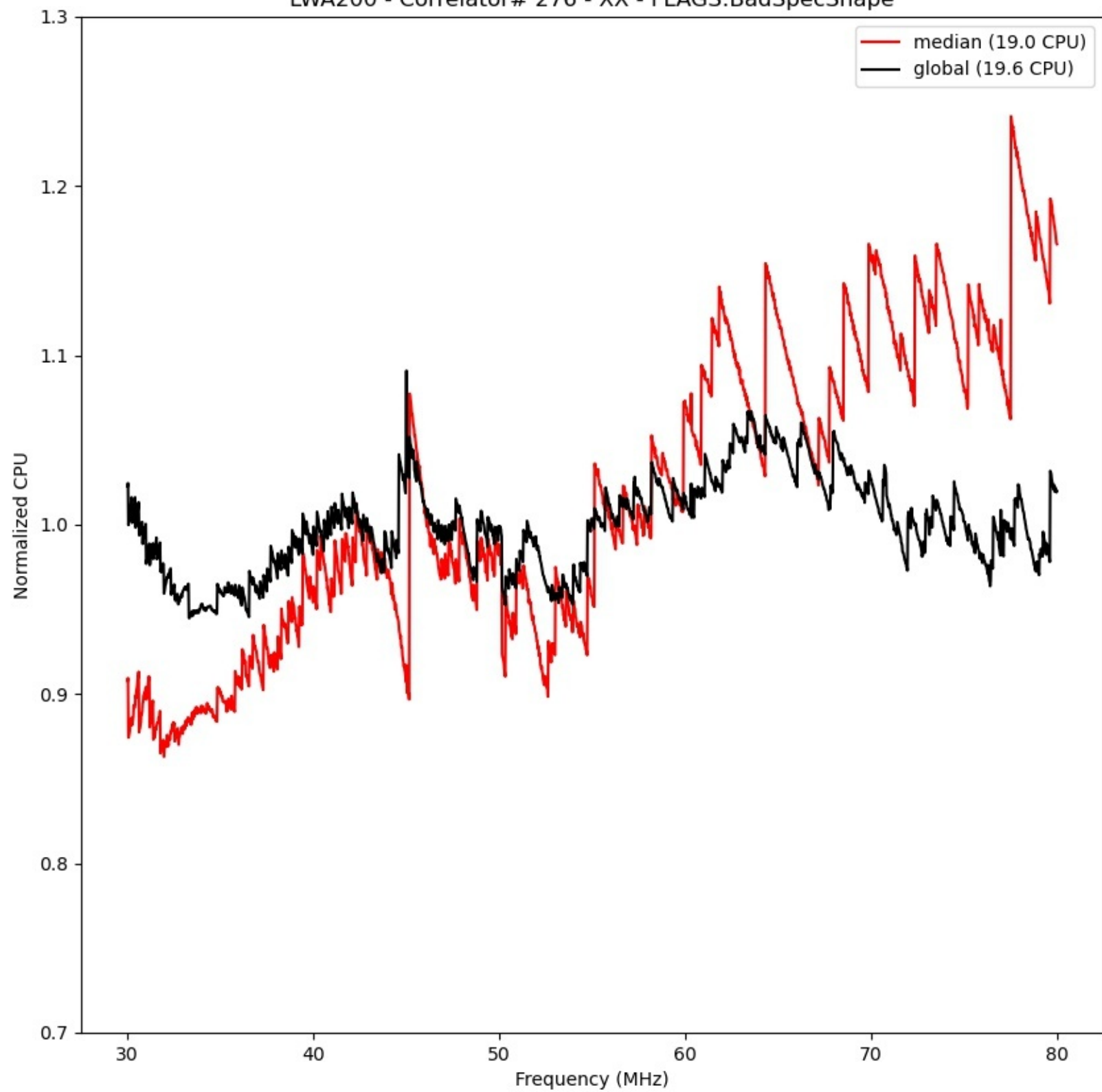
LWA200 - Correlator# 276 - XX - FLAGS:BadSpecShape
