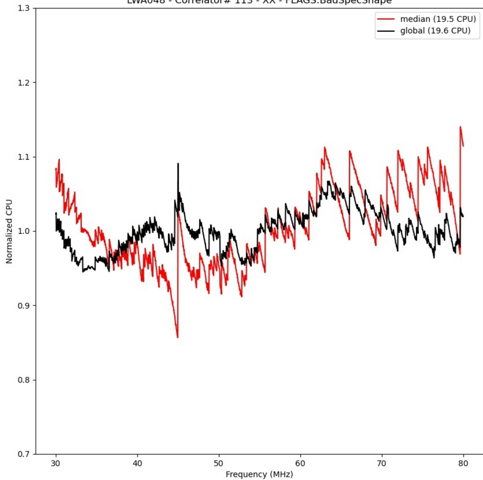
LWA048 - Correlator# 113 - XX - FLAGS:BadSpecShape
