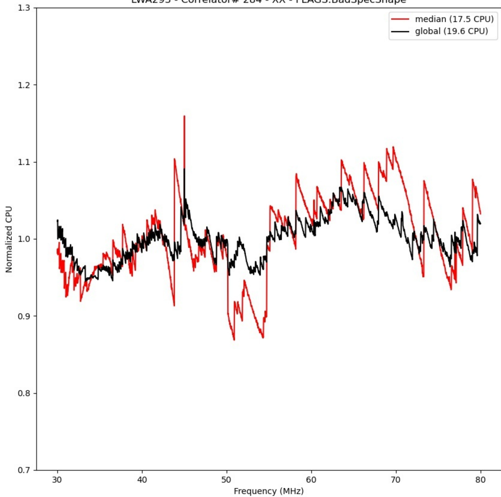
LWA293 - Correlator# 284 - XX - FLAGS:BadSpecShape
