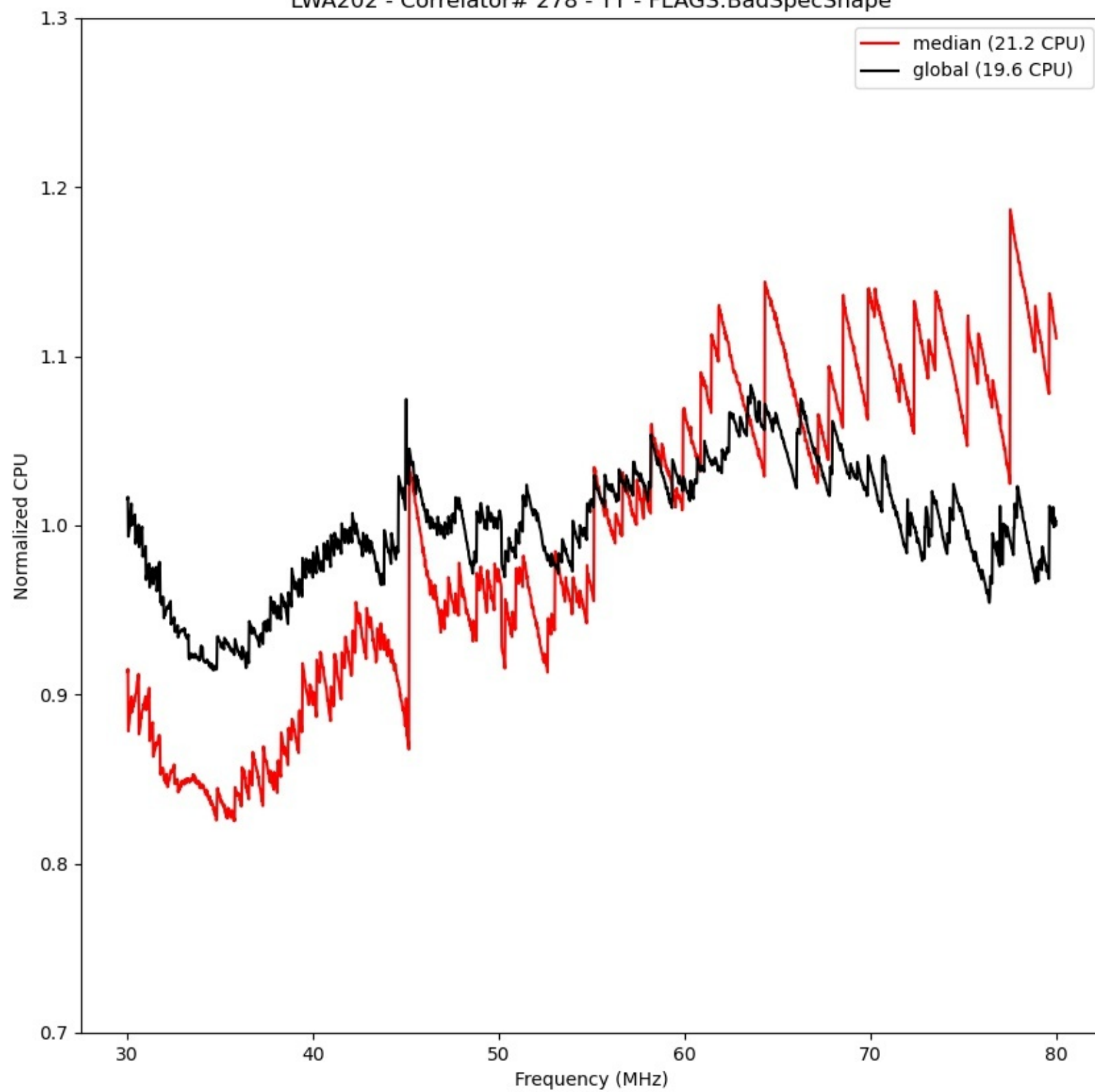
LWA202 - Correlator# 278 - YY - FLAGS:BadSpecShape
