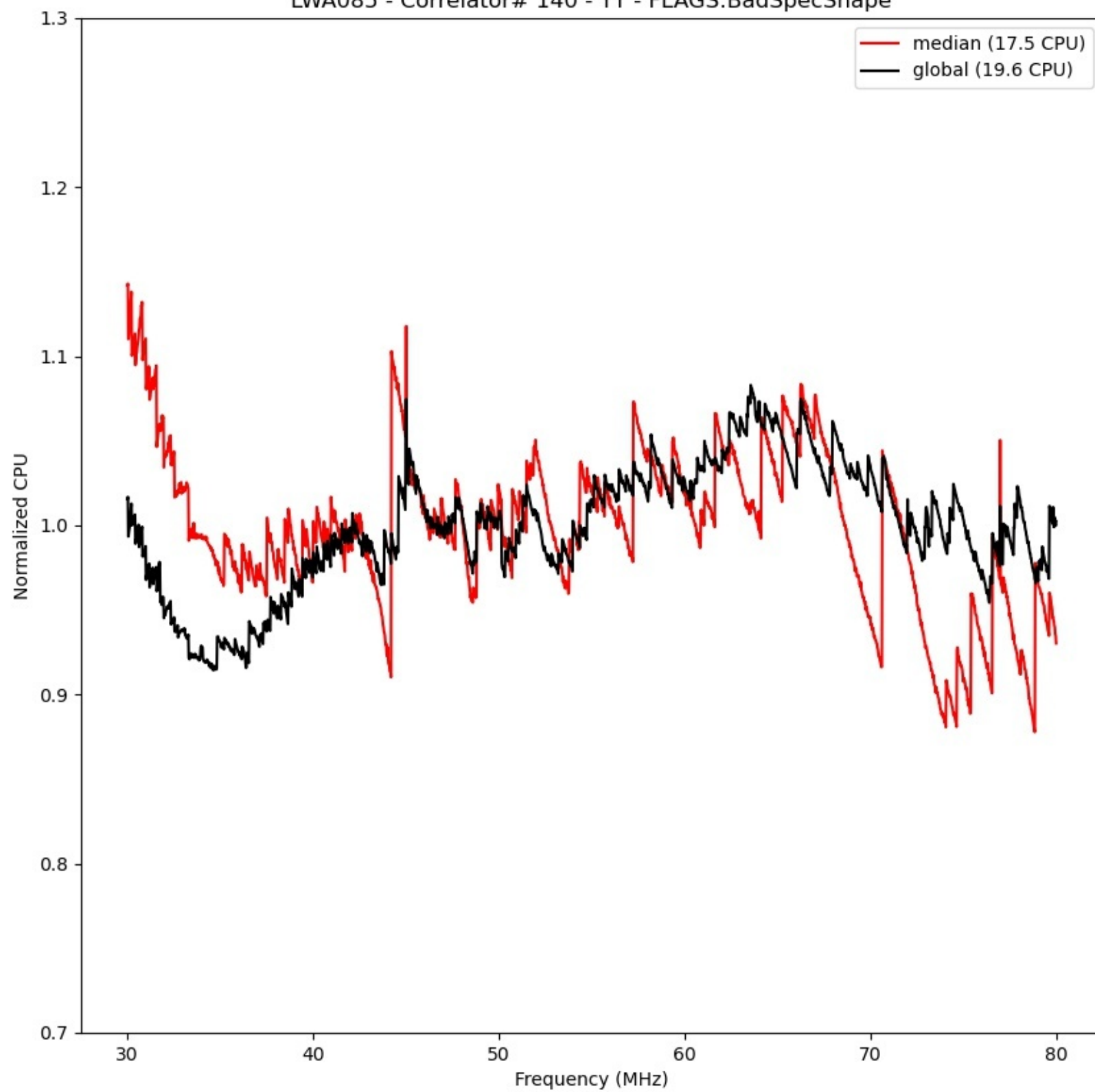
LWA085 - Correlator# 140 - YY - FLAGS:BadSpecShape
