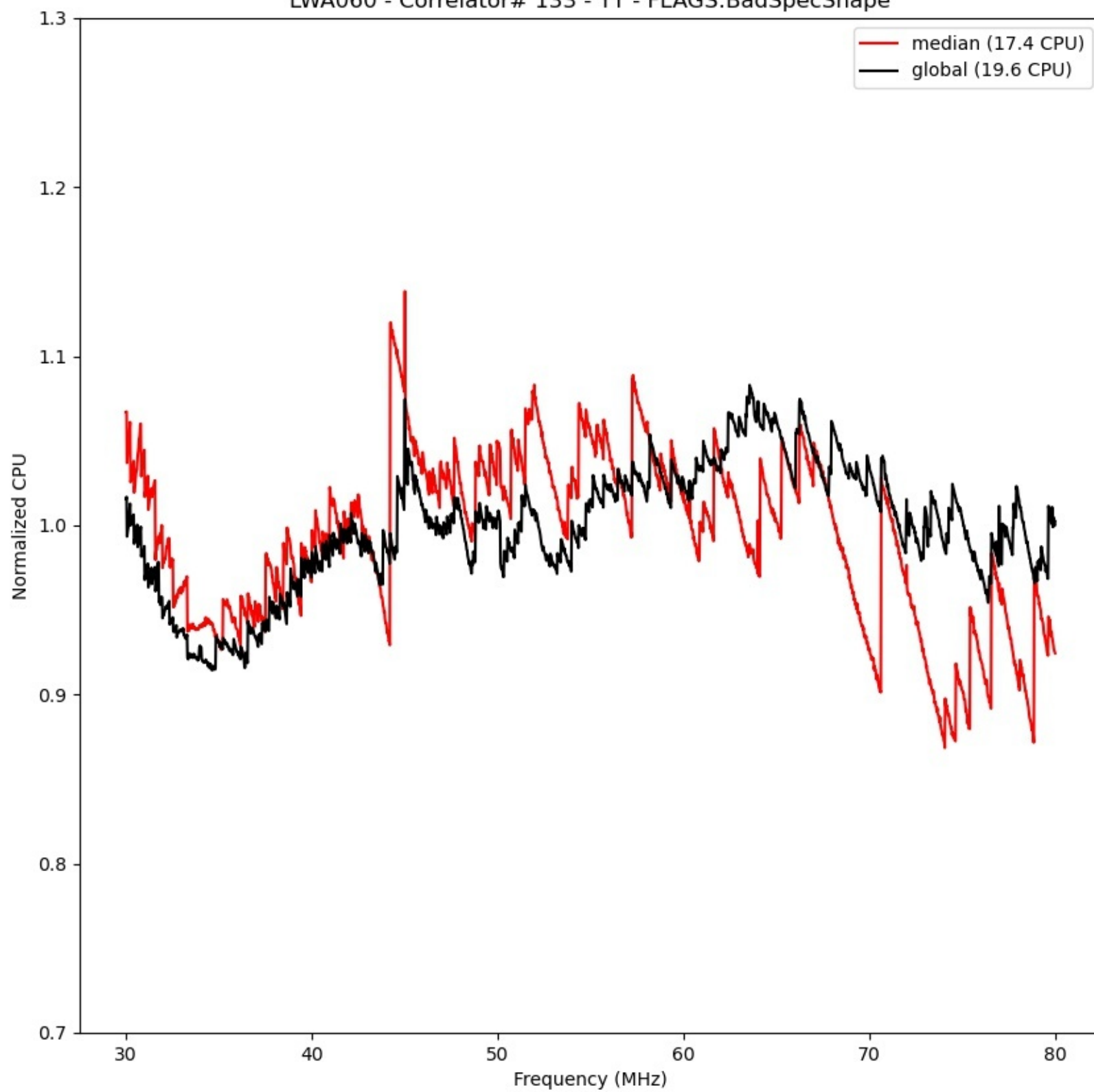
LWA060 - Correlator# 133 - YY - FLAGS:BadSpecShape
