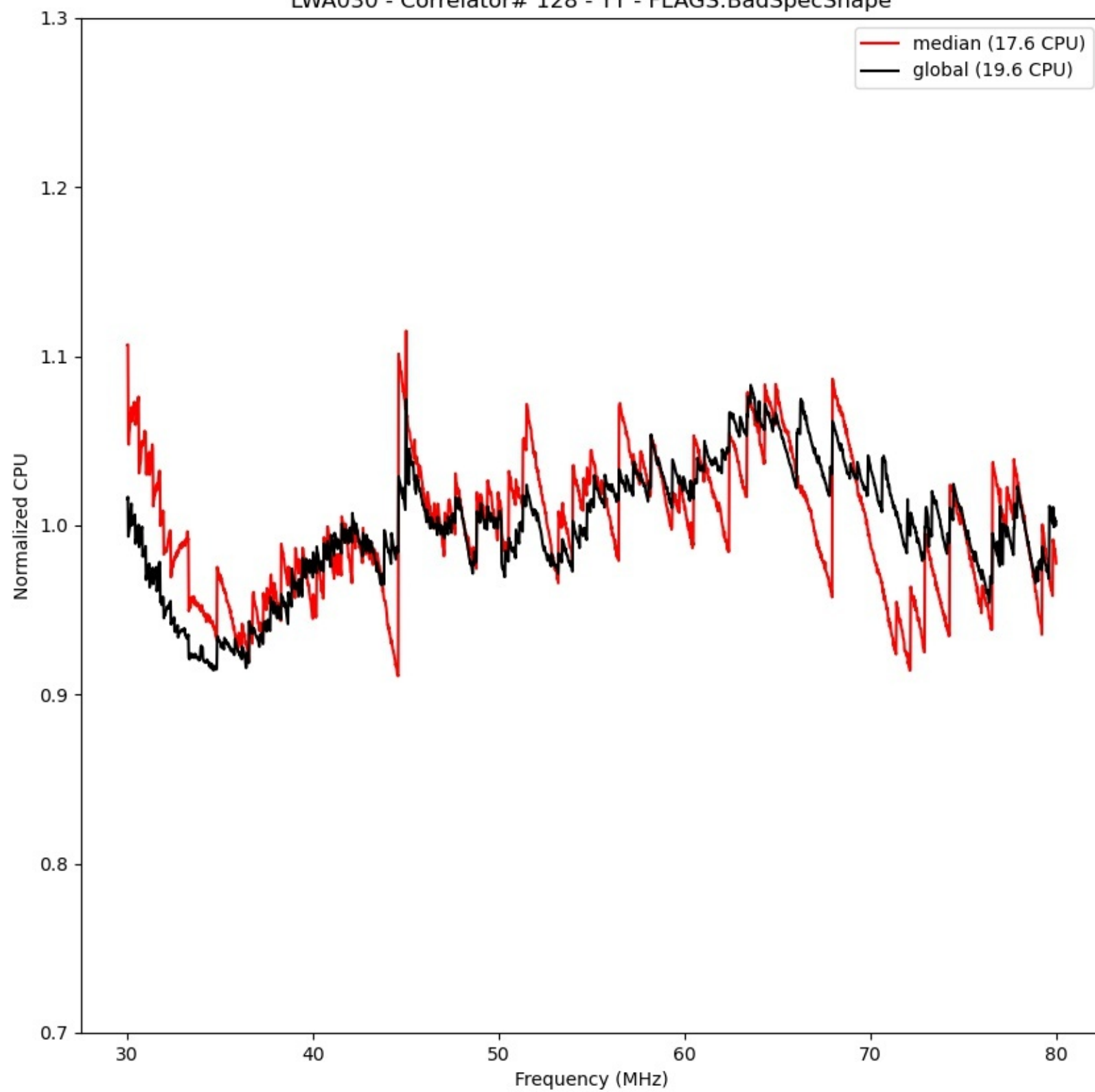
LWA030 - Correlator# 128 - YY - FLAGS:BadSpecShape
