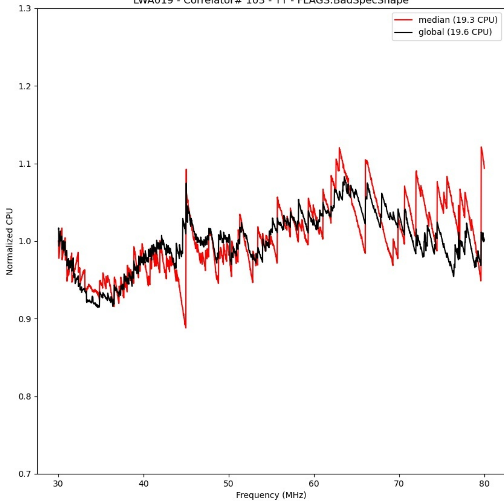
LWA019 - Correlator# 103 - YY - FLAGS:BadSpecShape
