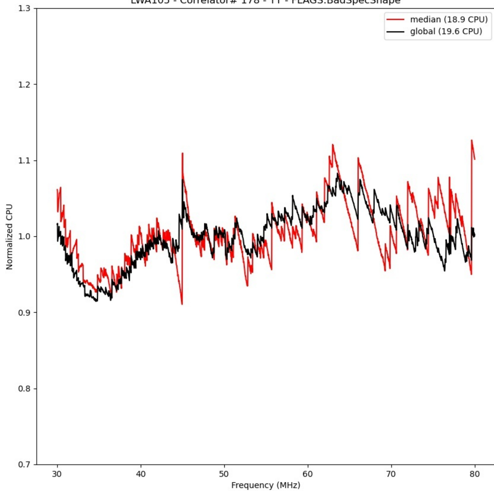
LWA105 - Correlator# 178 - YY - FLAGS:BadSpecShape
