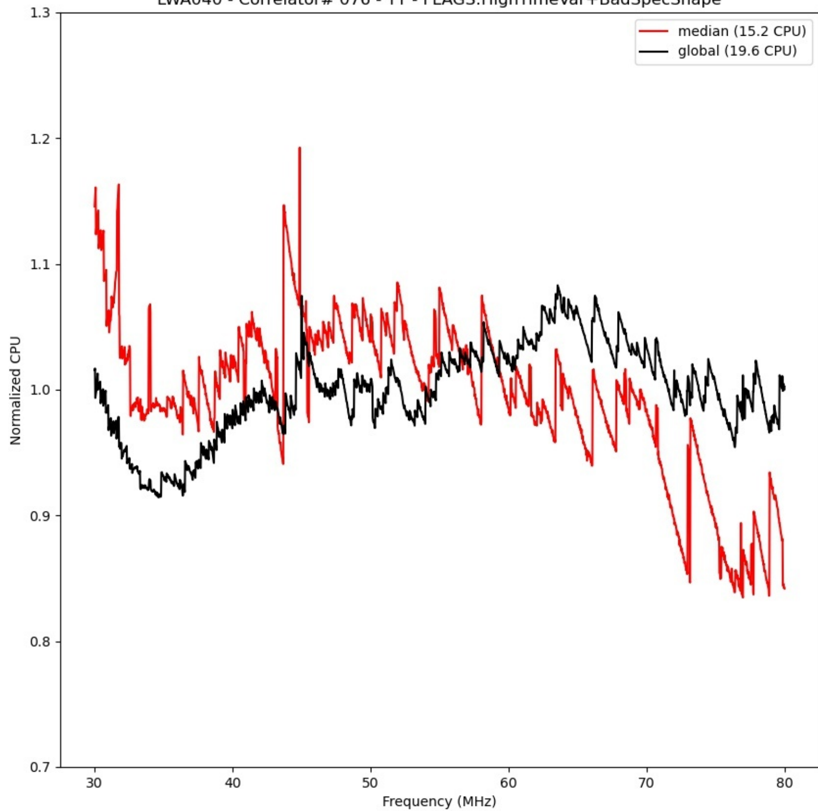
LWA040 - Correlator# 076 - YY - FLAGS:HighTimeVar+BadSpecShape
