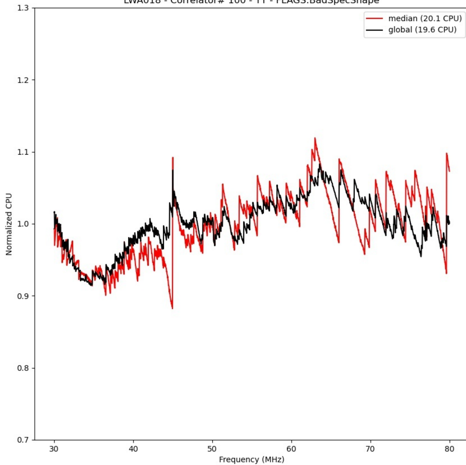
LWA018 - Correlator# 100 - YY - FLAGS:BadSpecShape
