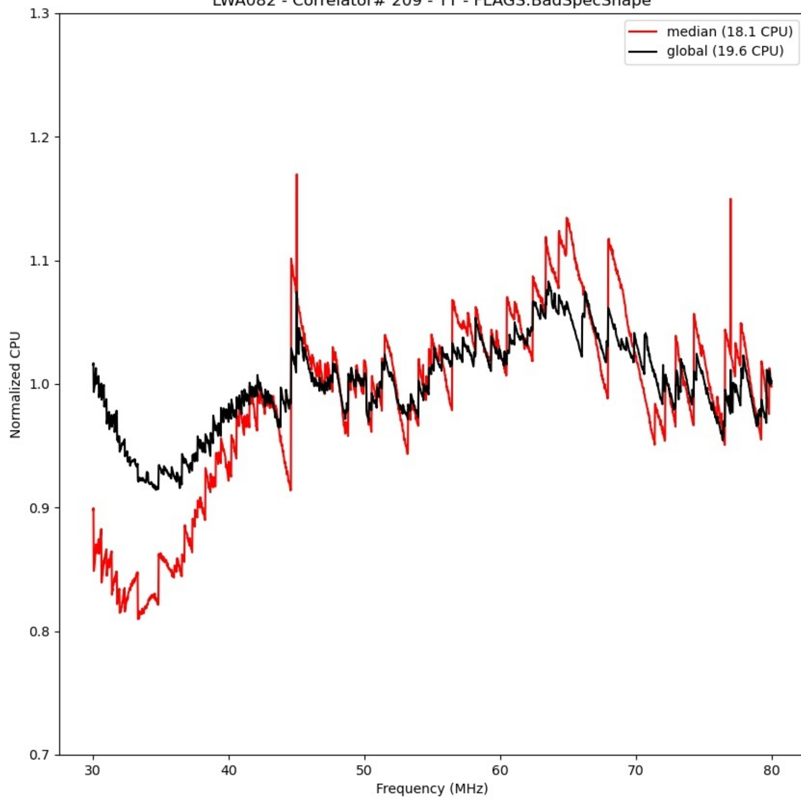
LWA082 - Correlator# 209 - YY - FLAGS:BadSpecShape
