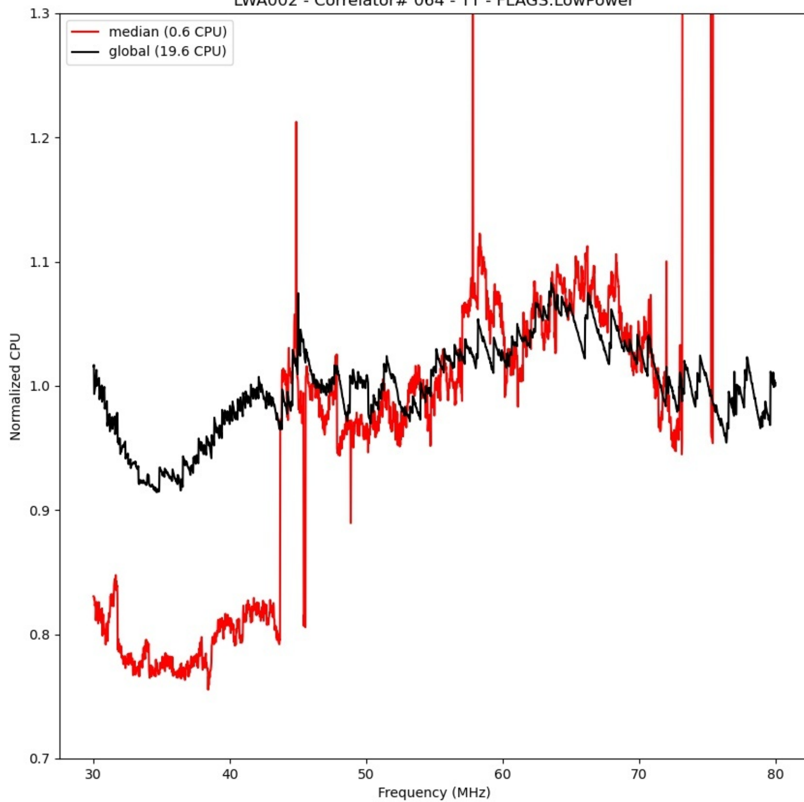
LWA002 - Correlator# 064 - YY - FLAGS:LowPower
