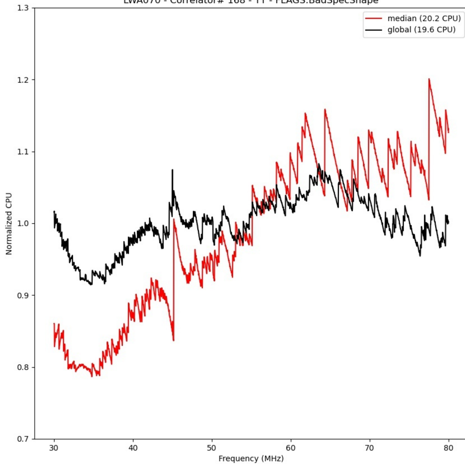
LWA070 - Correlator# 168 - YY - FLAGS:BadSpecShape
