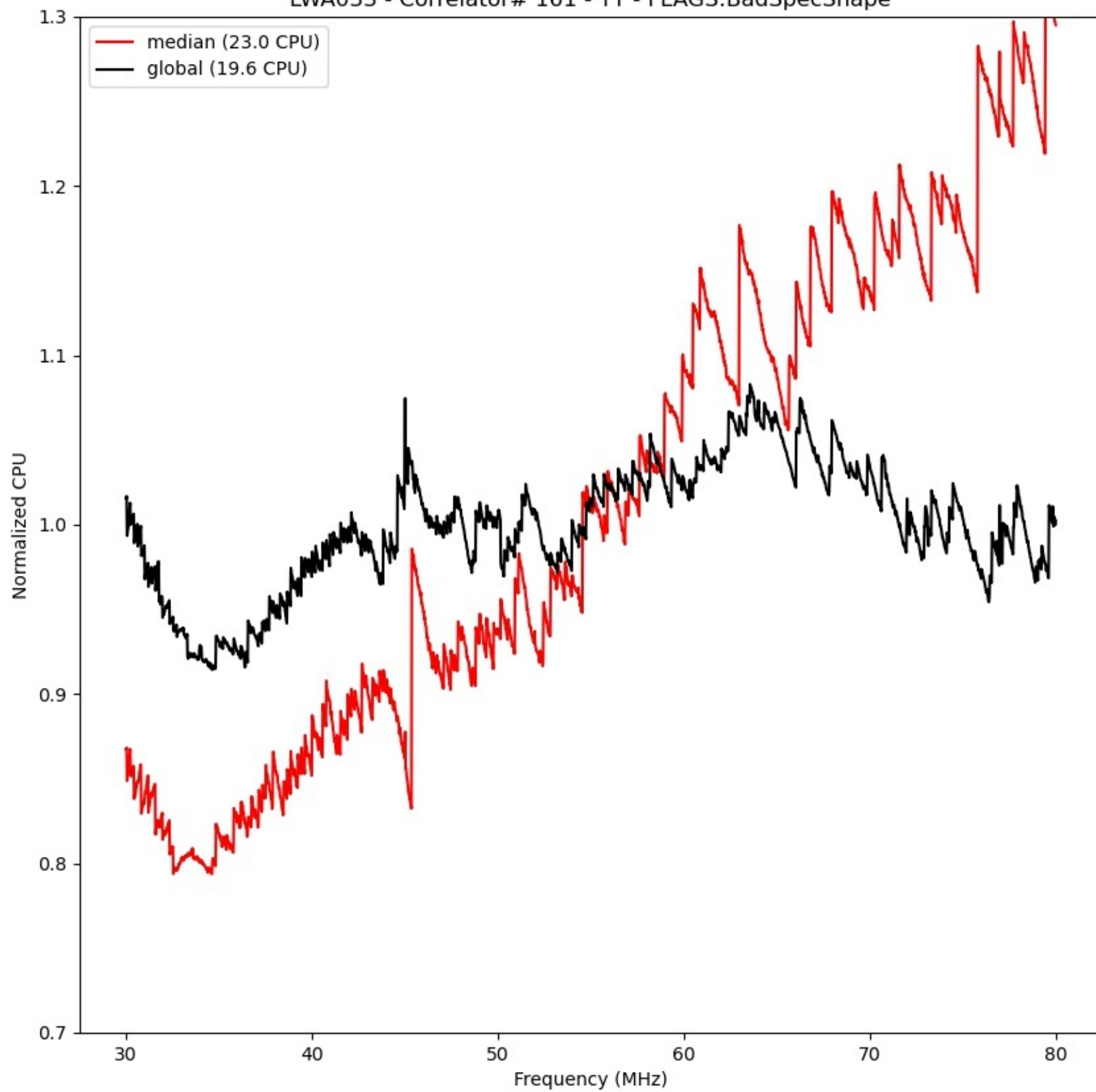
LWA033 - Correlator# 161 - YY - FLAGS:BadSpecShape
