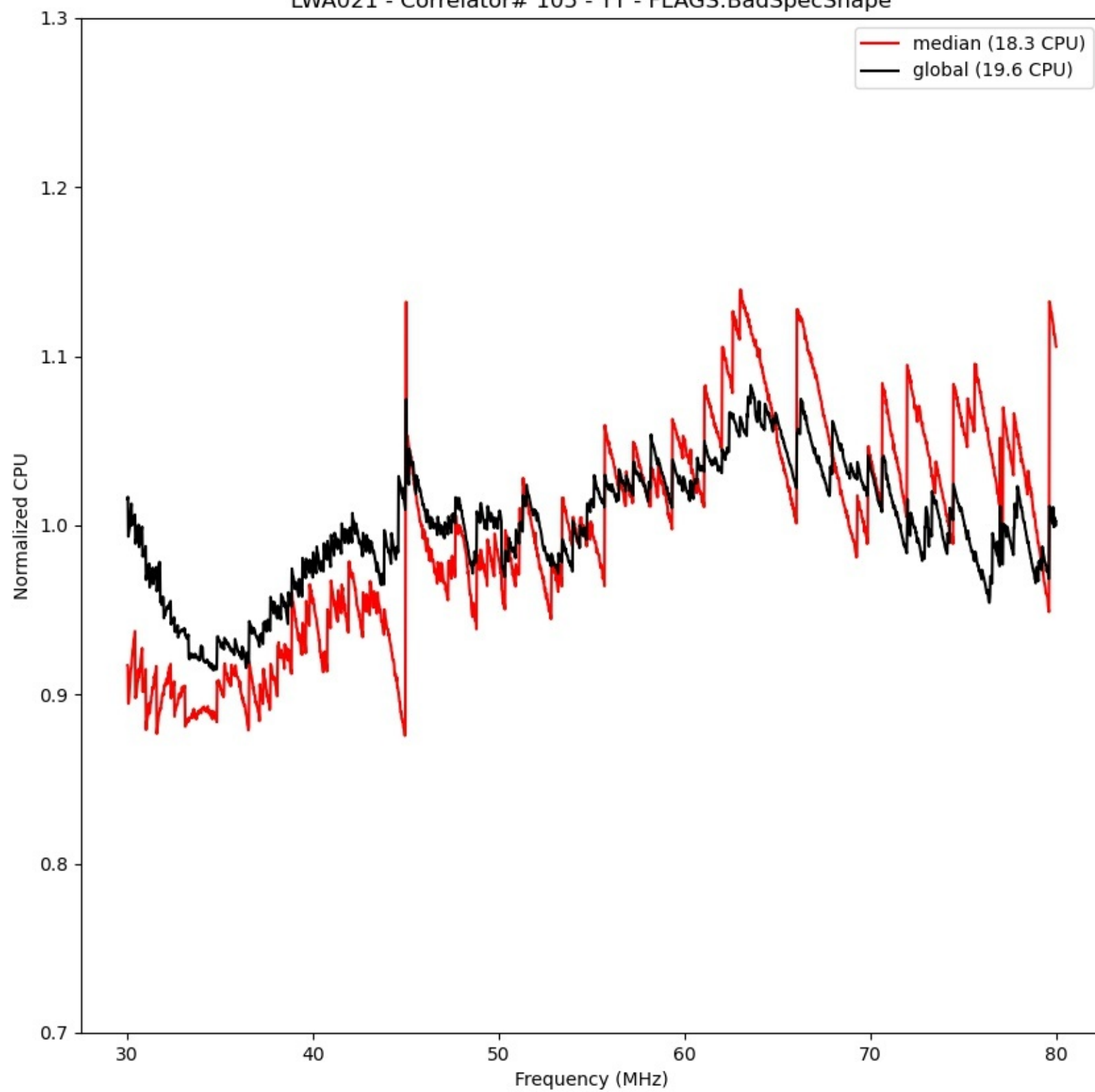
LWA021 - Correlator# 105 - YY - FLAGS:BadSpecShape
