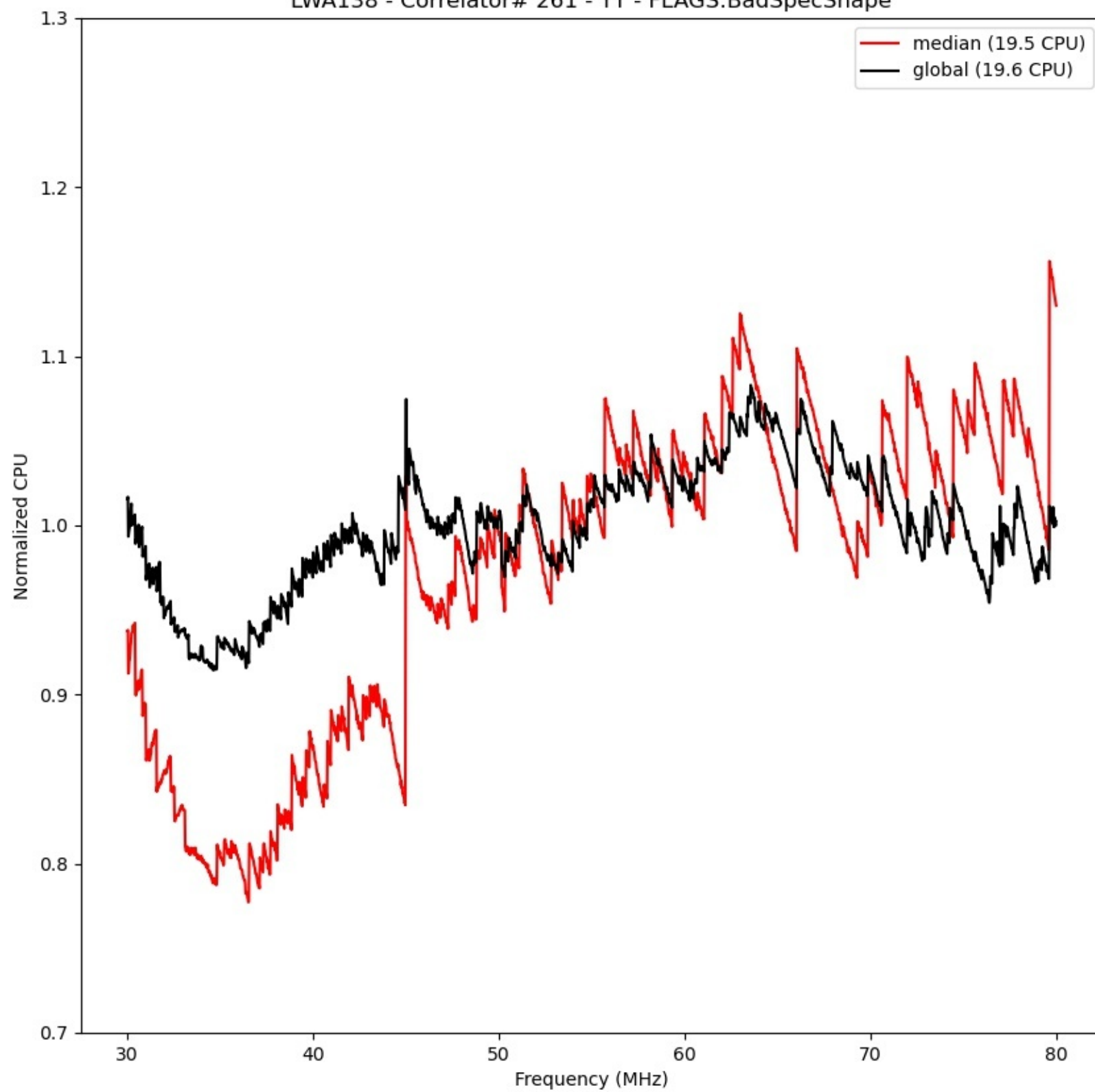
LWA138 - Correlator# 261 - YY - FLAGS:BadSpecShape
