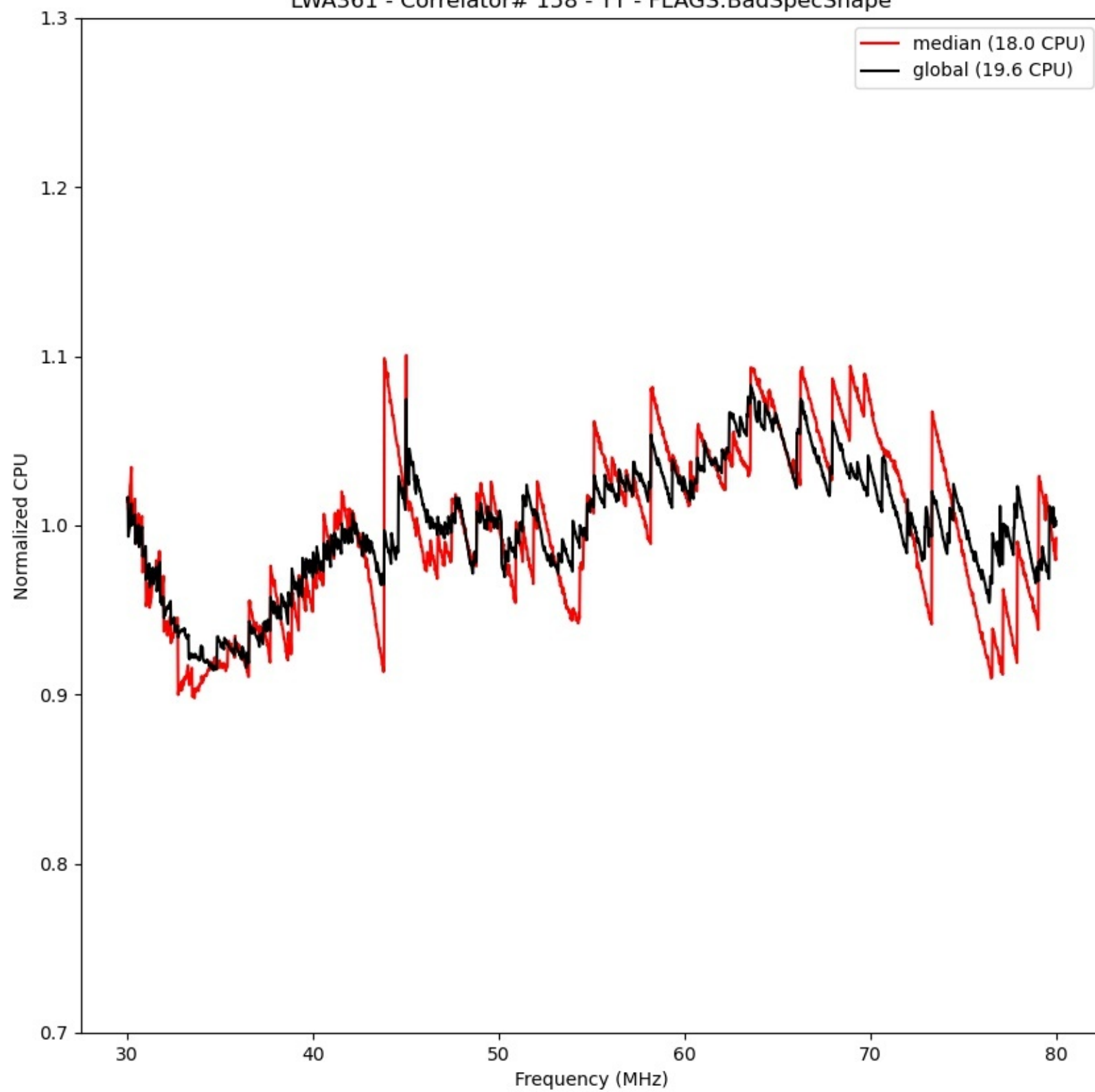
LWA361 - Correlator# 158 - YY - FLAGS:BadSpecShape
