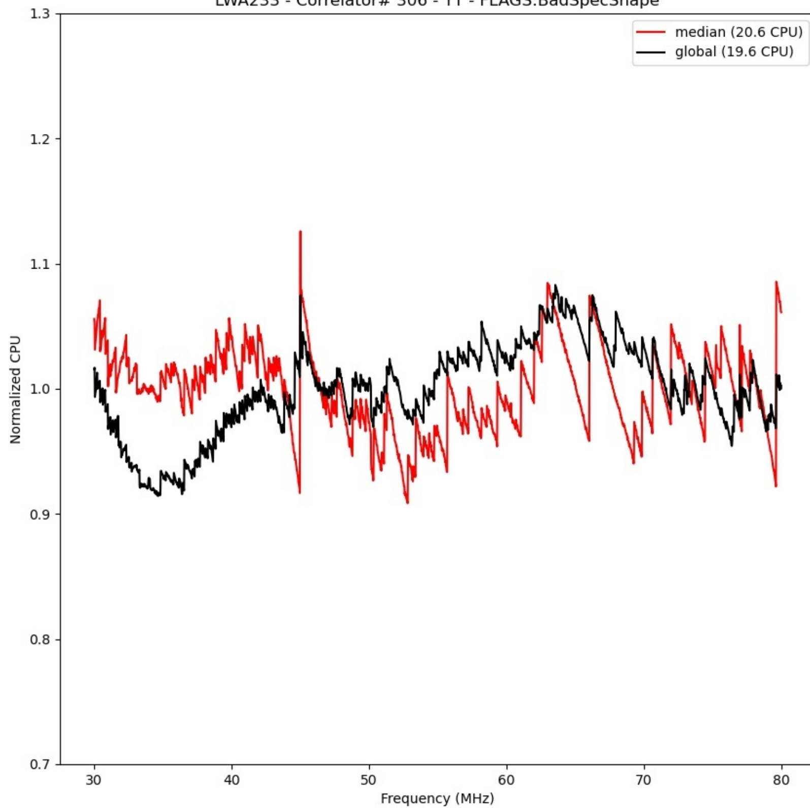
LWA233 - Correlator# 306 - YY - FLAGS:BadSpecShape
