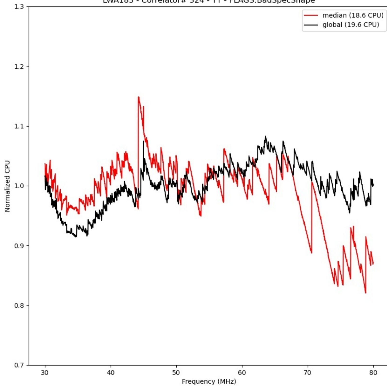
LWA183 - Correlator# 324 - YY - FLAGS:BadSpecShape
