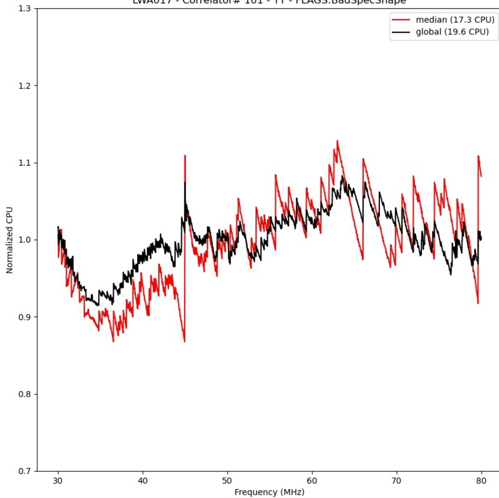
LWA017 - Correlator# 101 - YY - FLAGS:BadSpecShape
