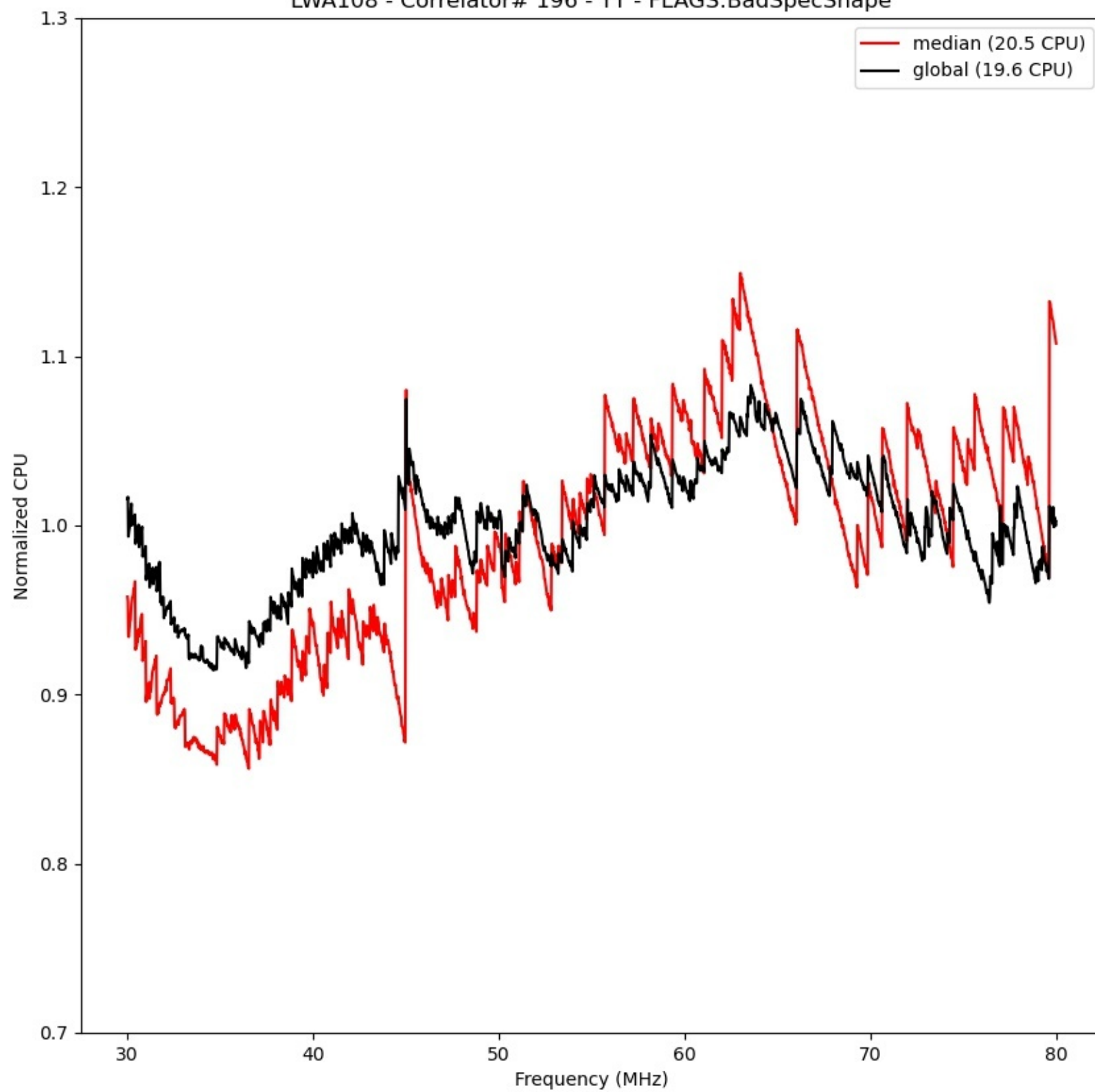
LWA108 - Correlator# 196 - YY - FLAGS:BadSpecShape
