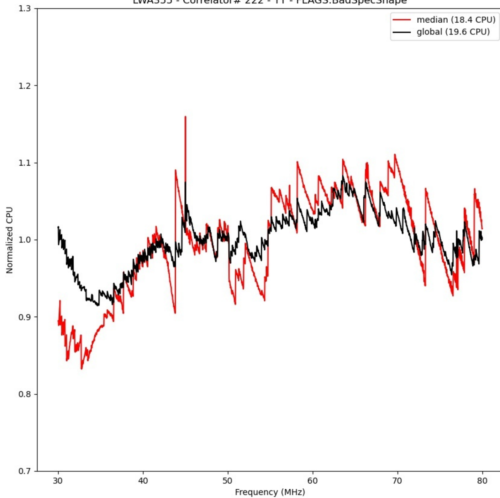
LWA355 - Correlator# 222 - YY - FLAGS:BadSpecShape
