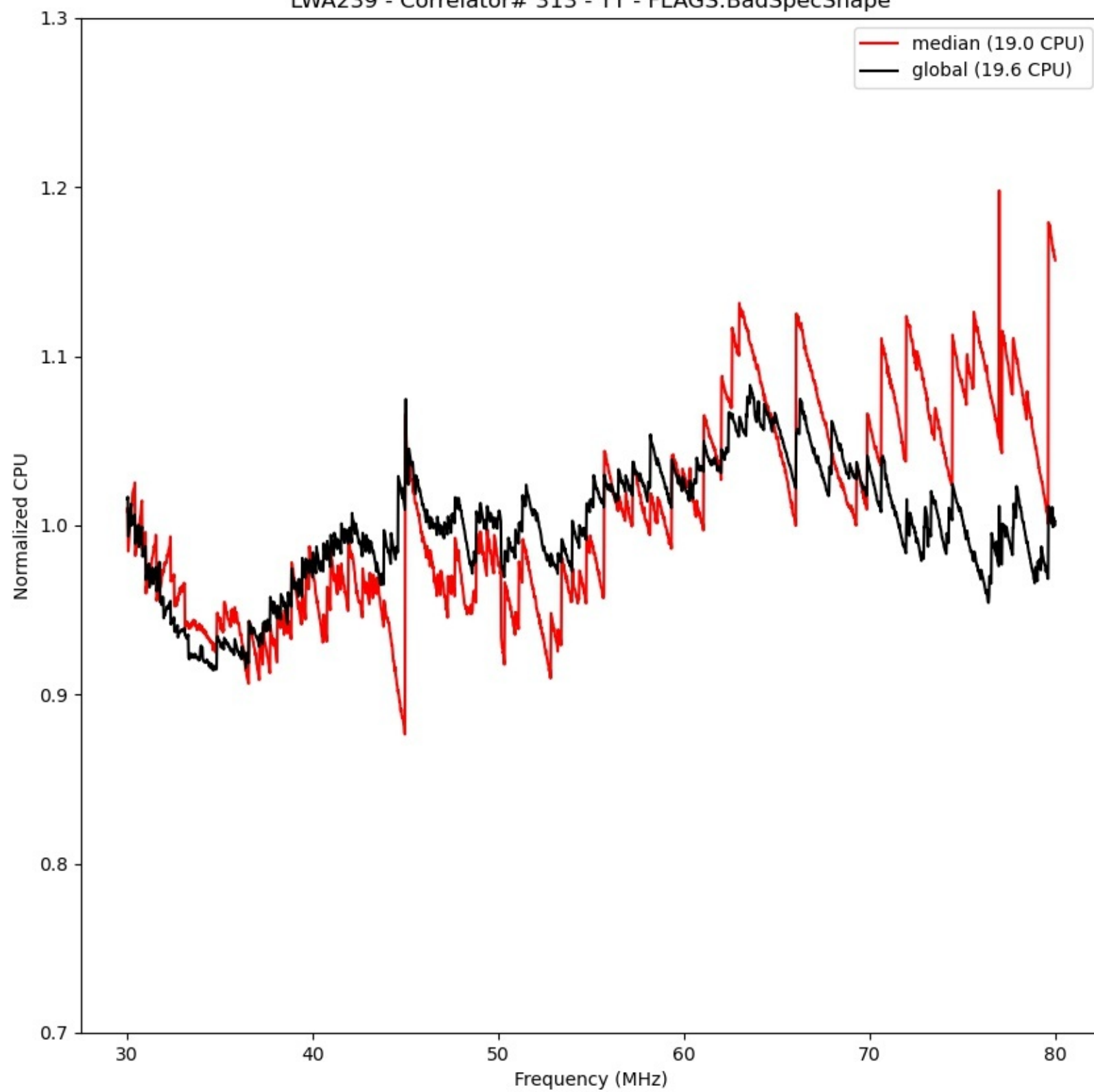
LWA239 - Correlator# 313 - YY - FLAGS:BadSpecShape
