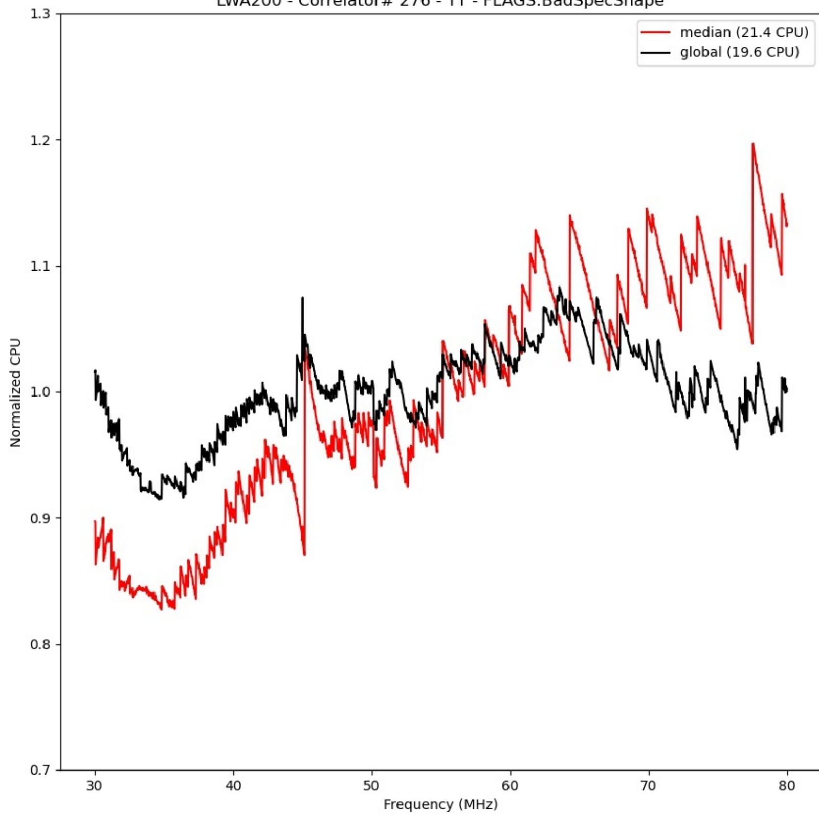
LWA200 - Correlator# 276 - YY - FLAGS:BadSpecShape
