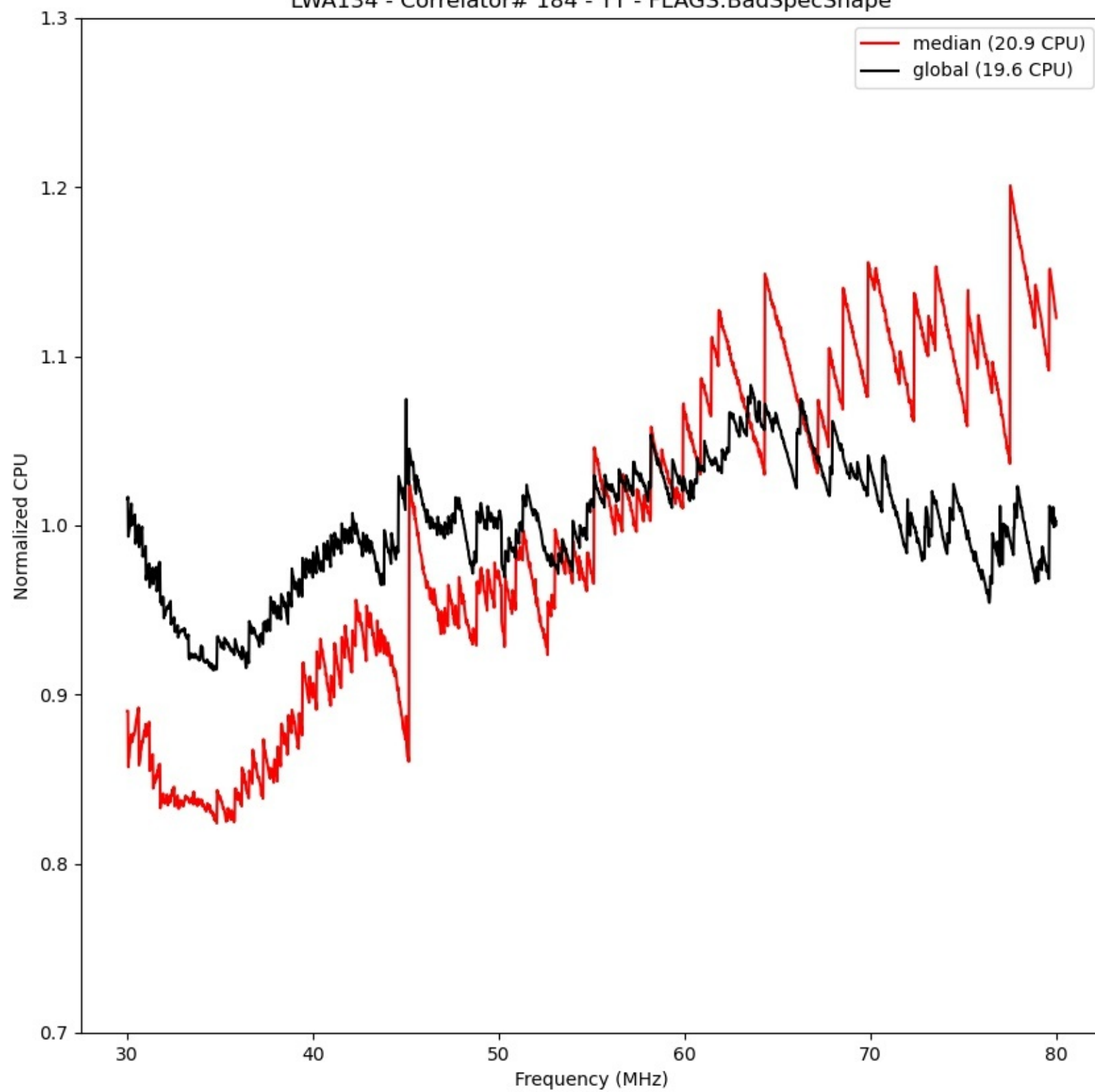
LWA134 - Correlator# 184 - YY - FLAGS:BadSpecShape
