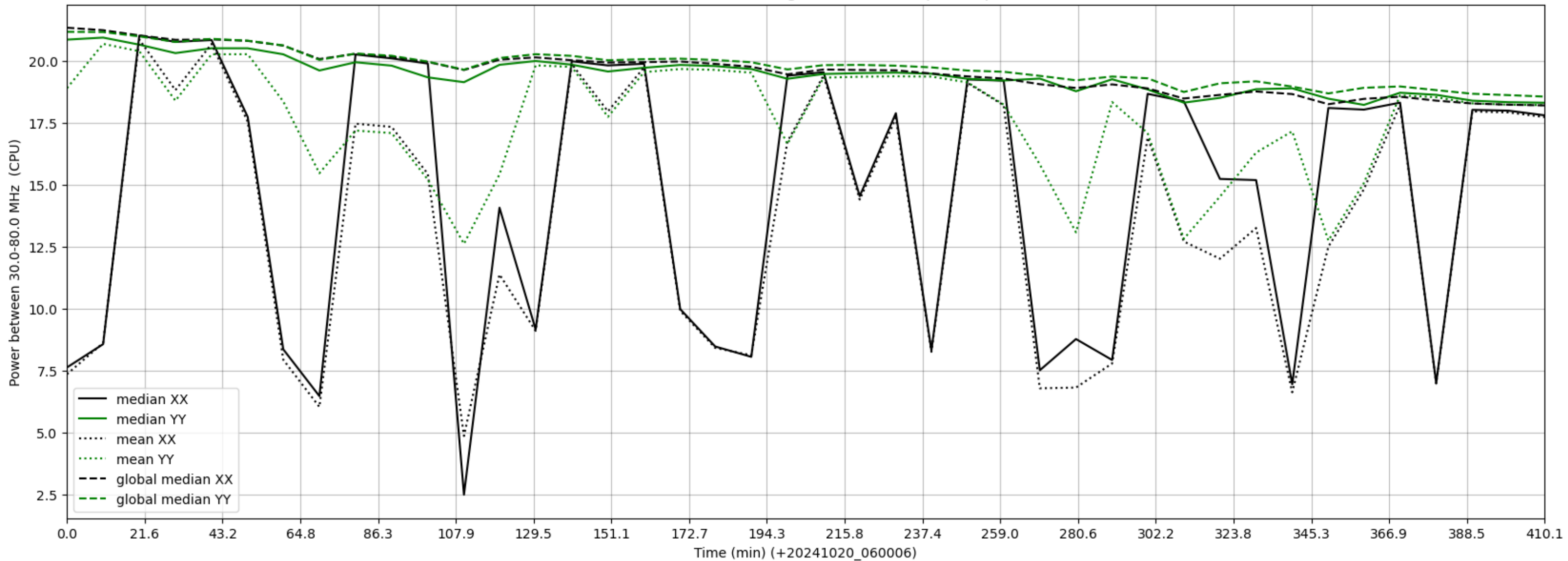
LWA145 - Correlator# 212 - XX FLAGS:HighTimeVar+BadSpecShape - YY FLAGS:Good
