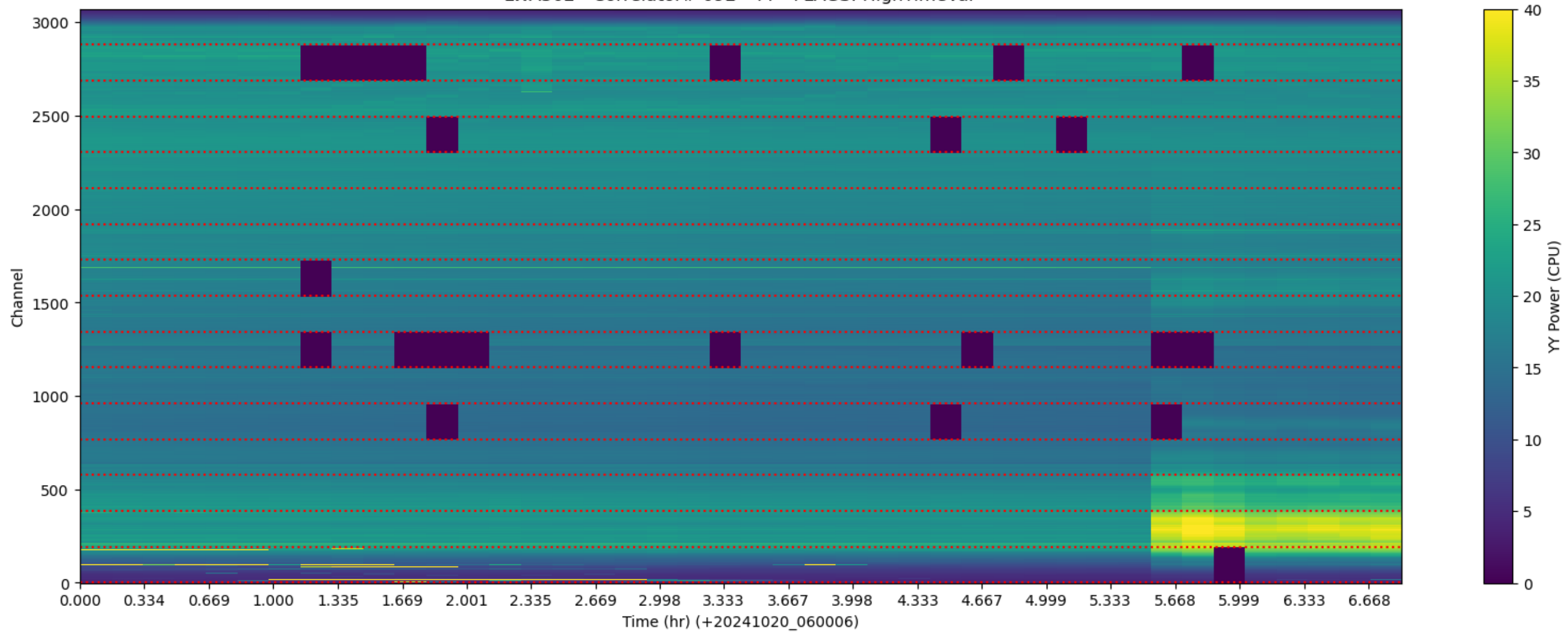
LWA302 - Correlator# 092 - YY - FLAGS: HighTimeVar
