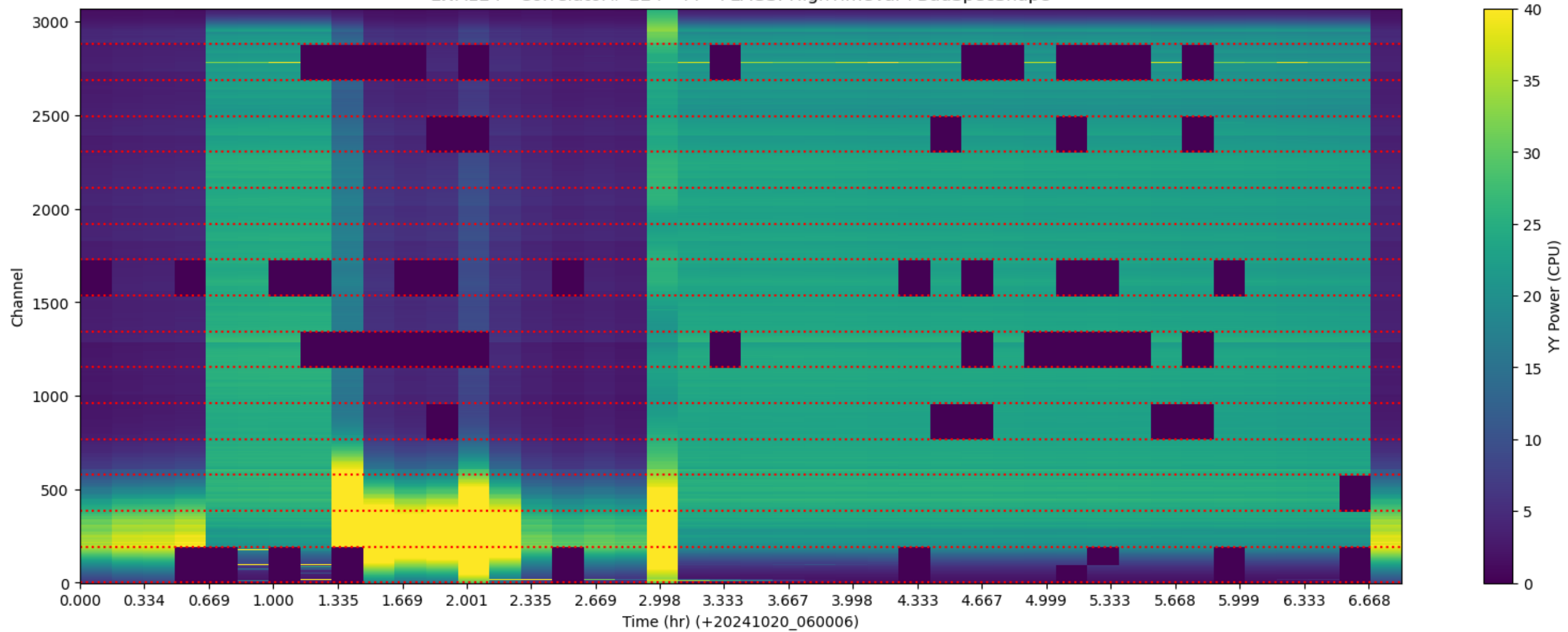
LWA124 - Correlator# 224 - YY - FLAGS: HighTimeVar+BadSpecShape
