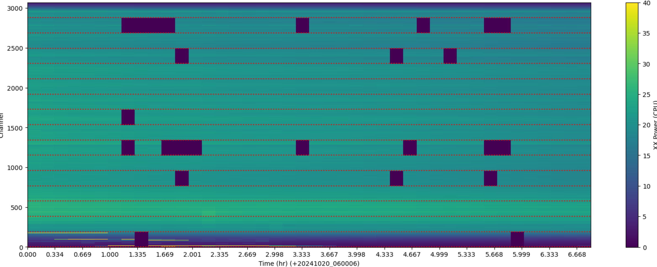
LWA059 - Correlator# 136 - XX - FLAGS: Good
