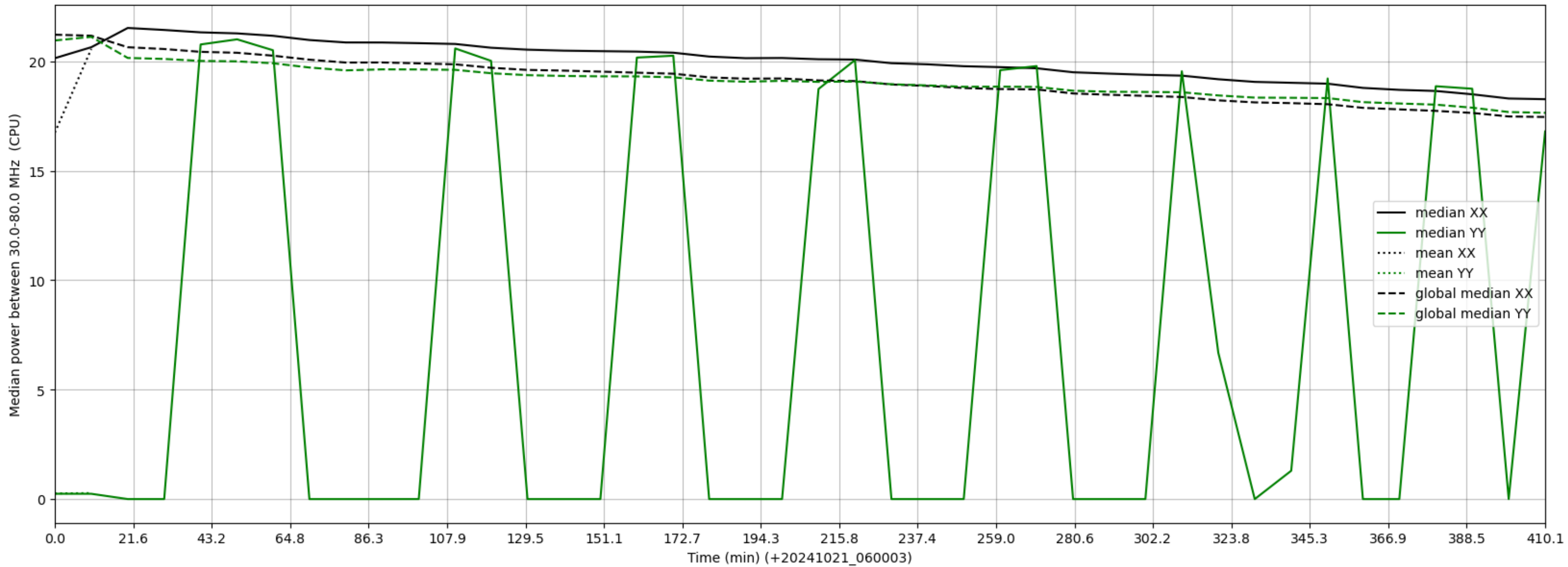
LWA058 - Correlator# 137 - XX FLAGS:Good - YY FLAGS:LowPower
