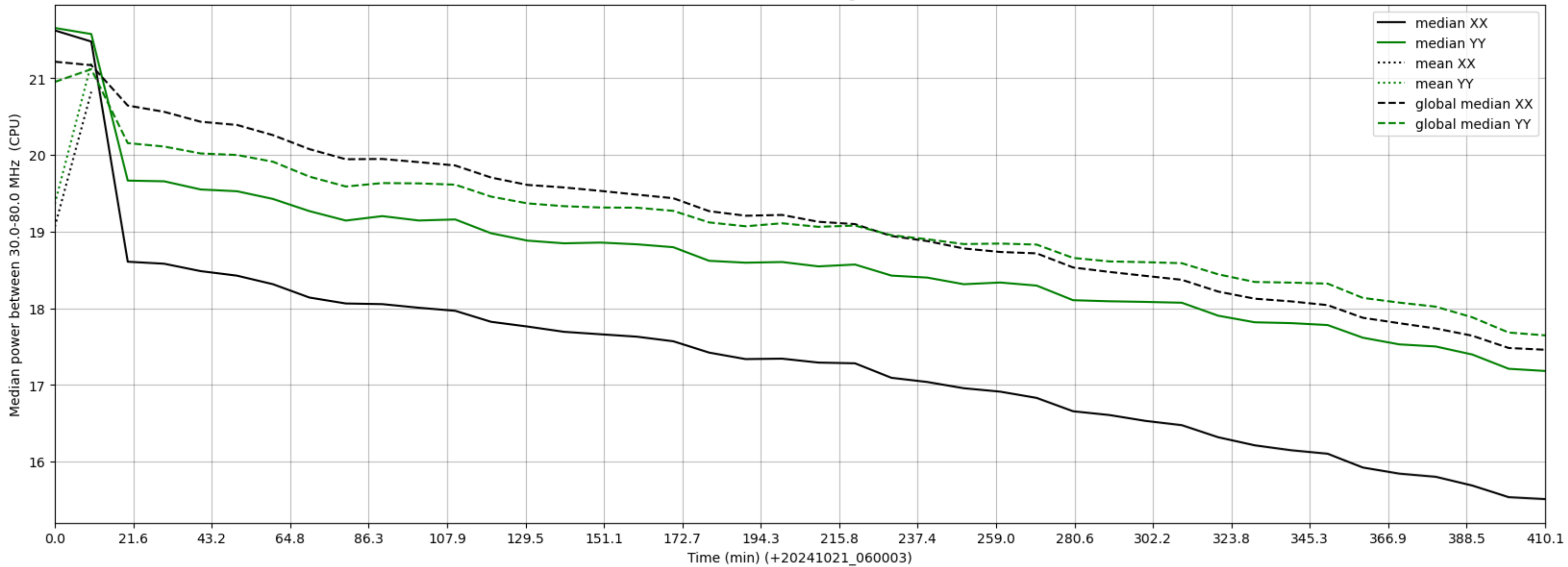
LWA107 - Correlator# 197 - XX FLAGS:HighTimeVar - YY FLAGS:Good
