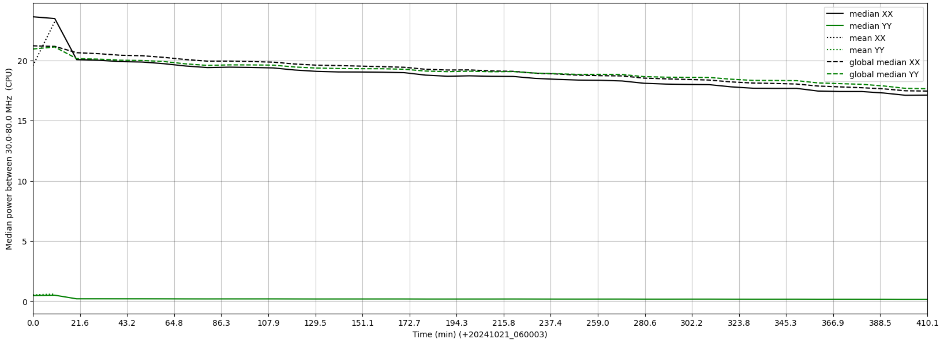
LWA066 - Correlator# 164 - XX FLAGS:HighTimeVar - YY FLAGS:LowPower
