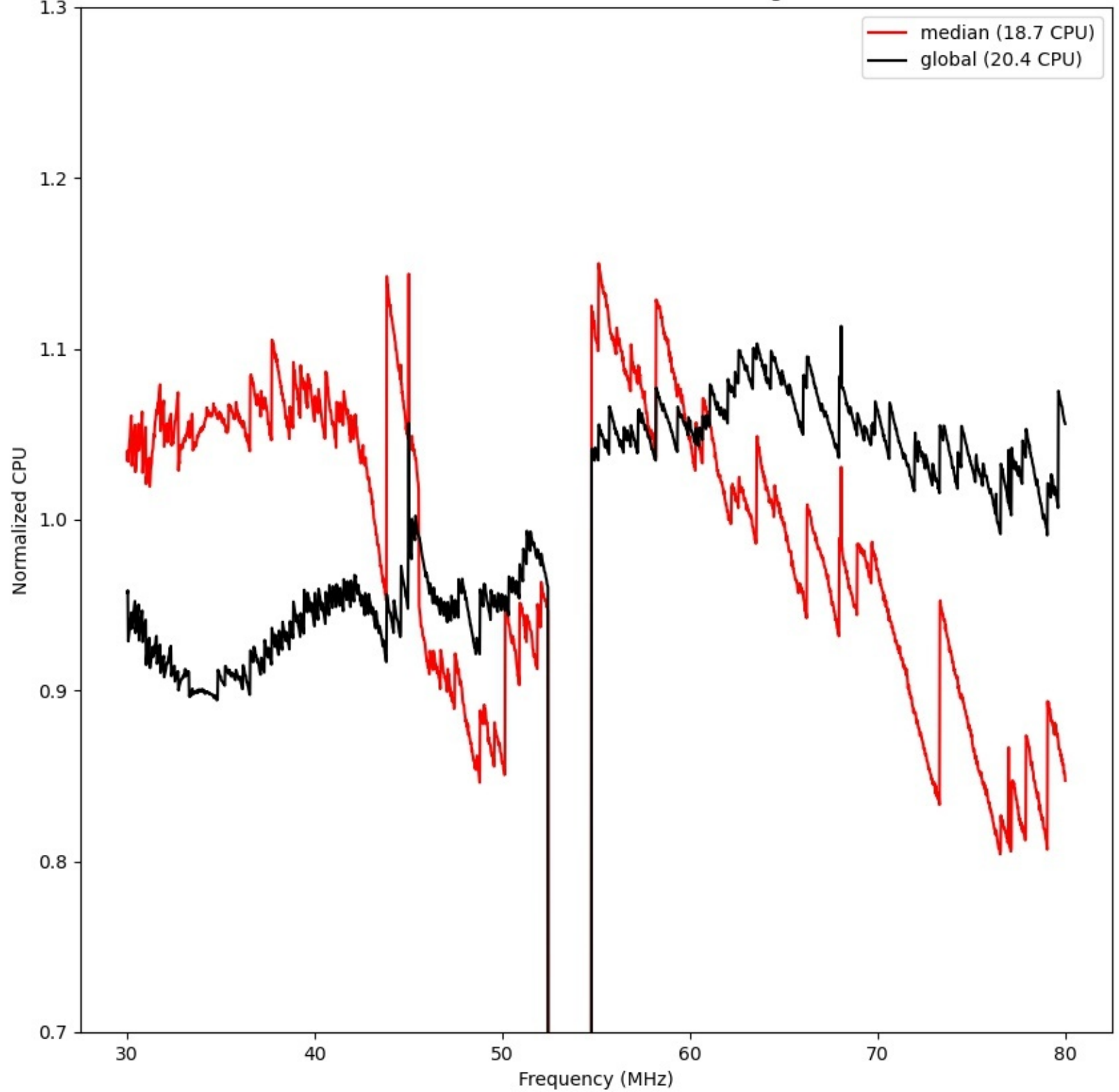
LWA255 - Correlator# 033 - XX - FLAGS:HighTimeVar
