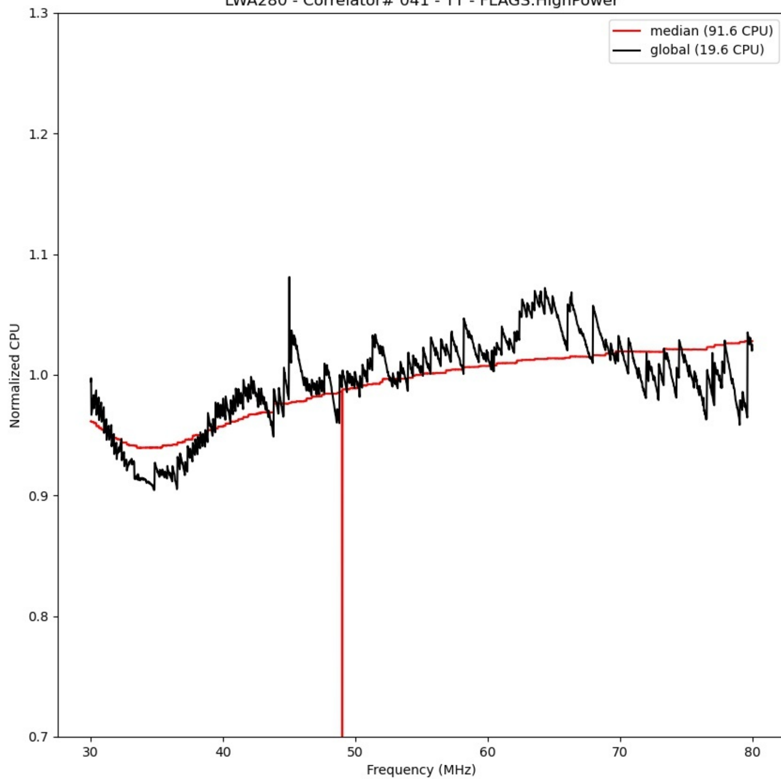
LWA280 - Correlator# 041 - YY - FLAGS:HighPower
