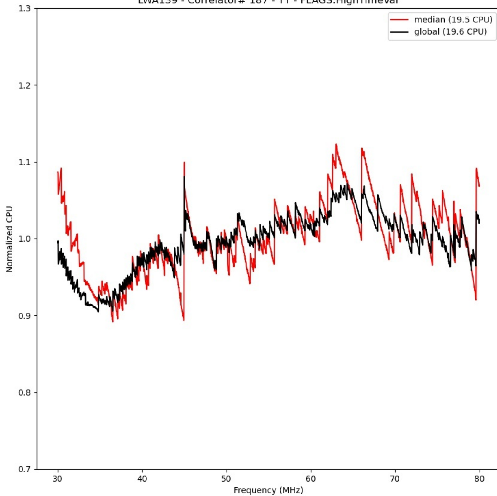
LWA139 - Correlator# 187 - YY - FLAGS:HighTimeVar
