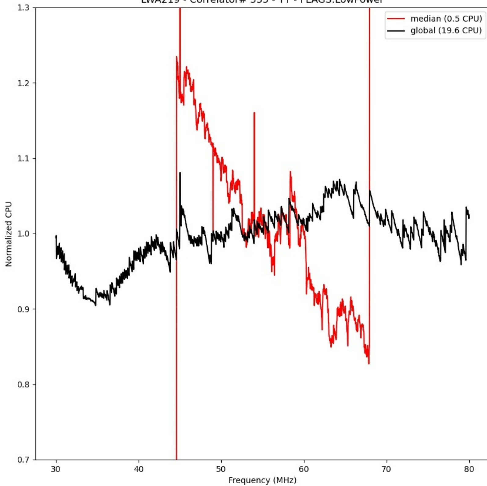
LWA219 - Correlator# 335 - YY - FLAGS:LowPower
