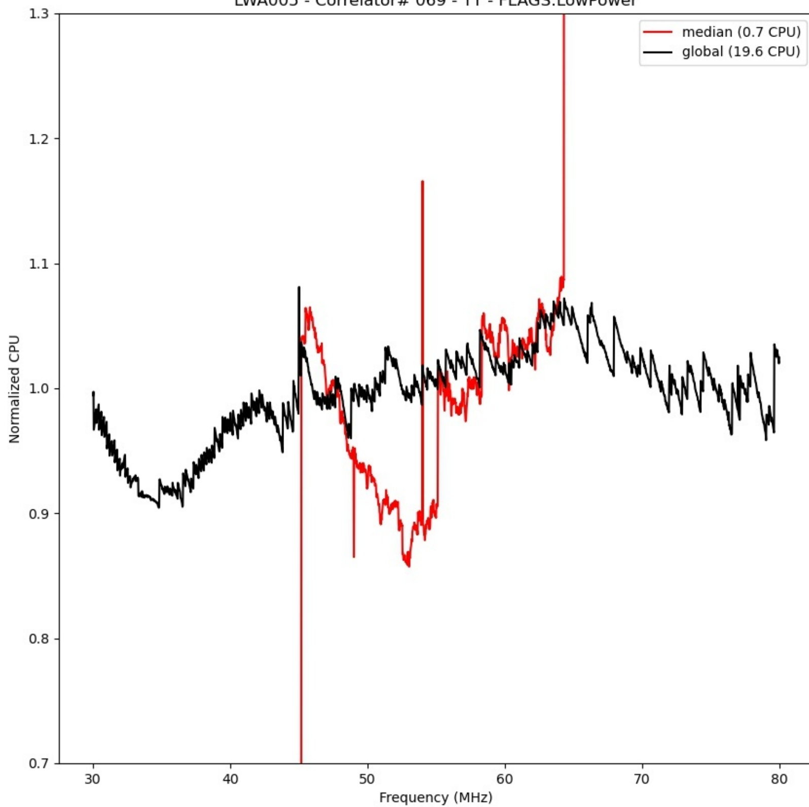
LWA005 - Correlator# 069 - YY - FLAGS:LowPower
