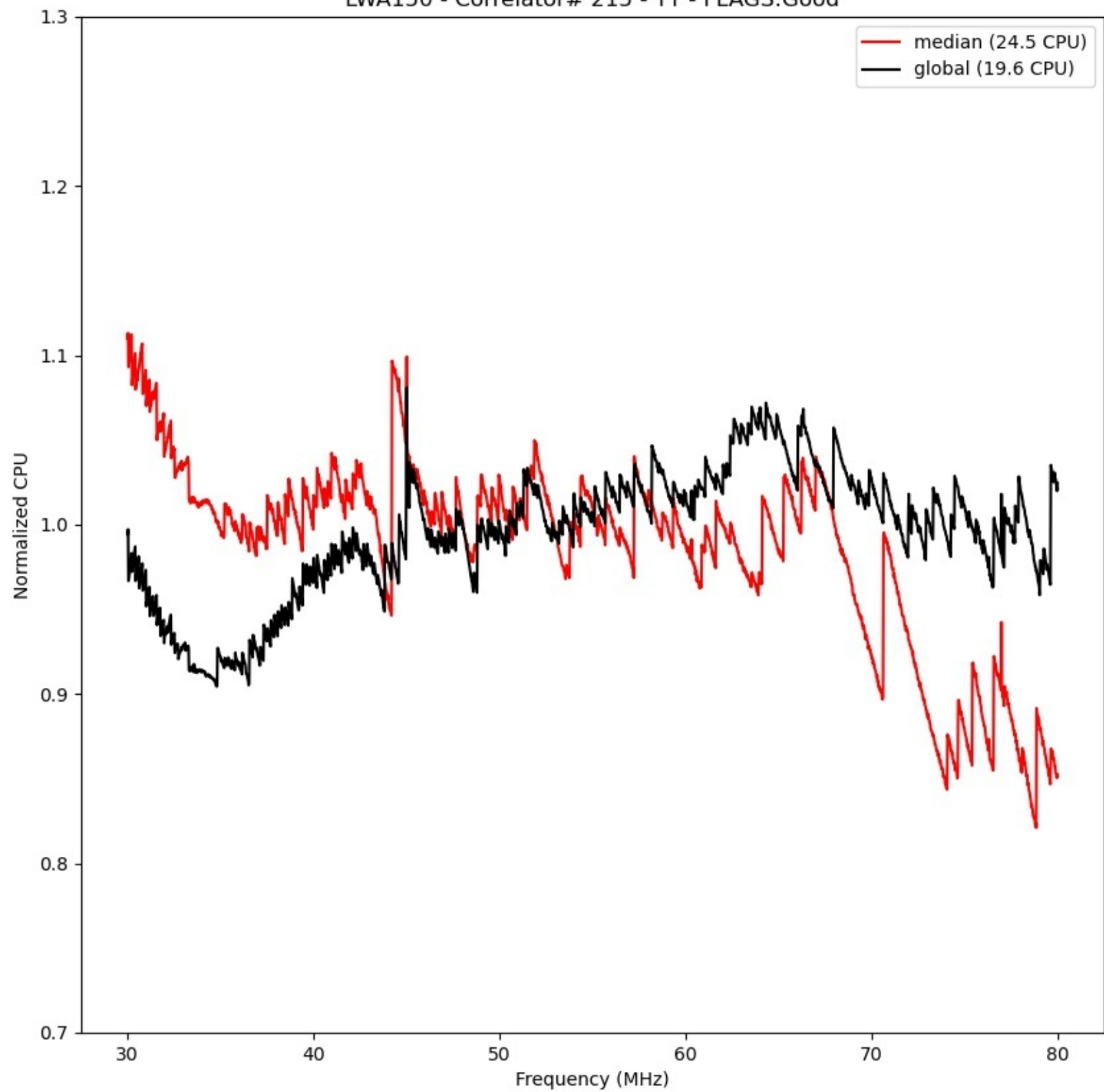
LWA150 - Correlator# 215 - YY - FLAGS:Good
