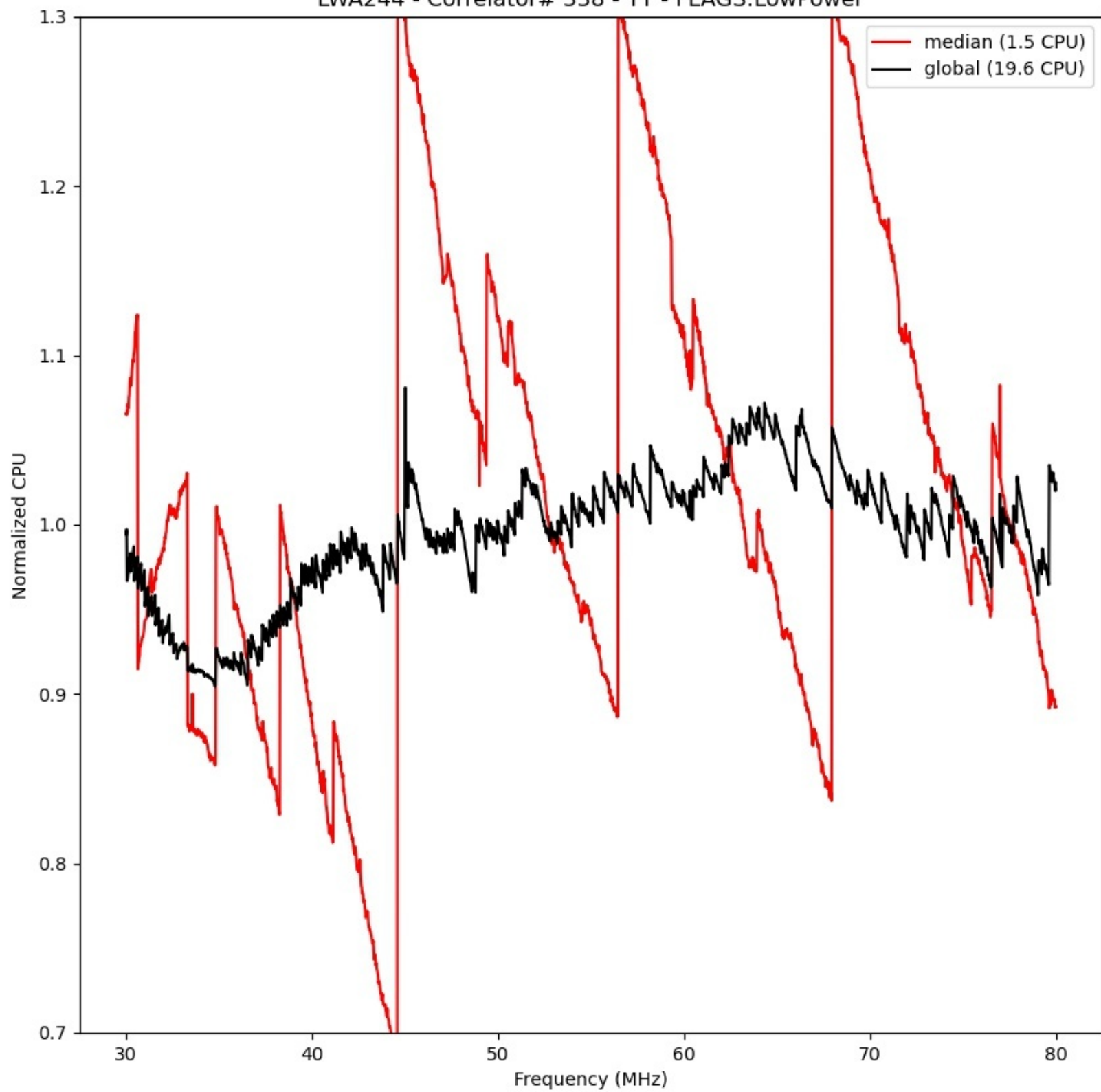
LWA244 - Correlator# 338 - YY - FLAGS:LowPower
