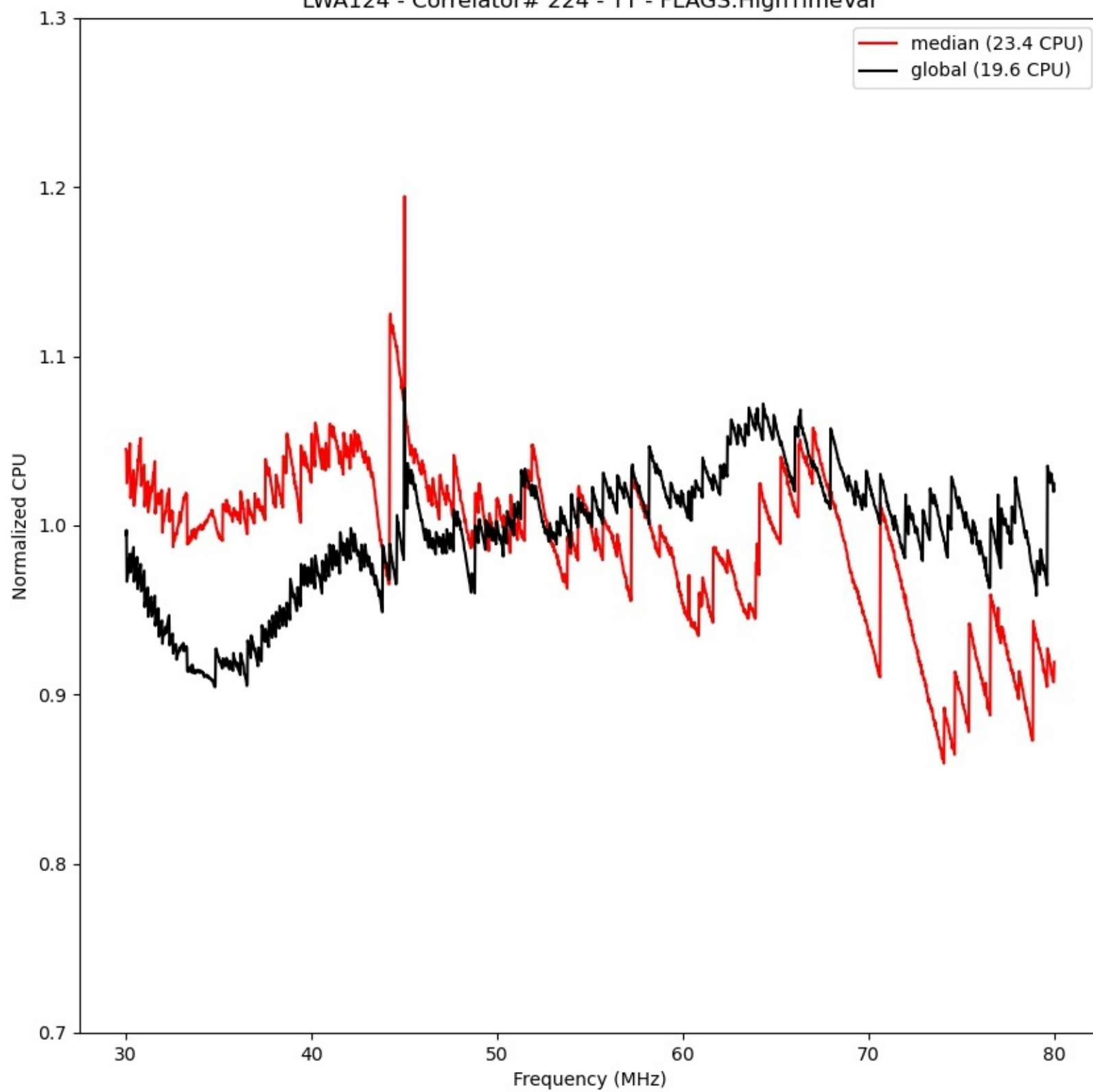
LWA124 - Correlator# 224 - YY - FLAGS:HighTimeVar
