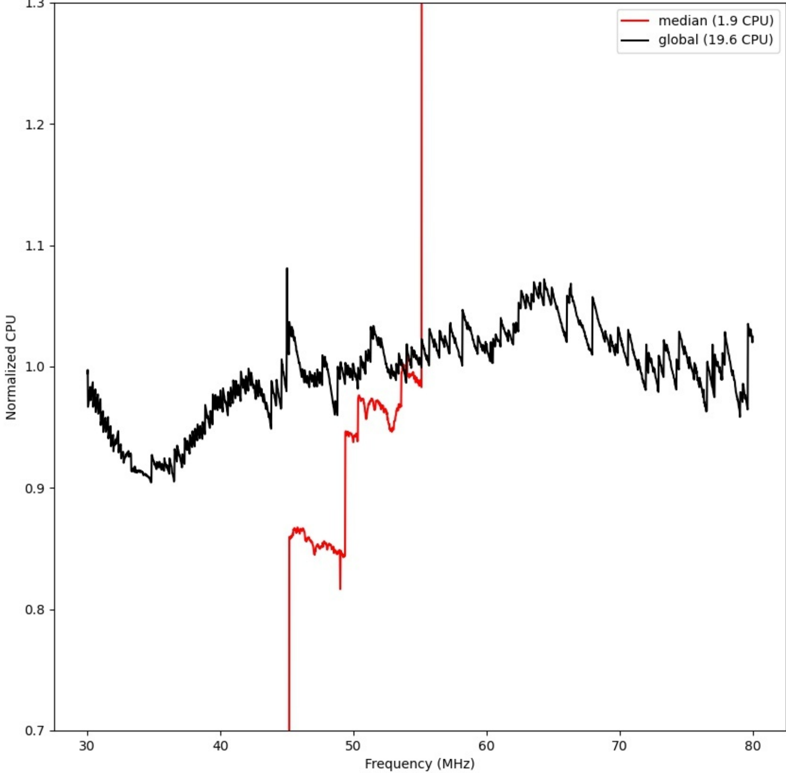
LWA232 - Correlator# 307 - YY - FLAGS:LowPower
