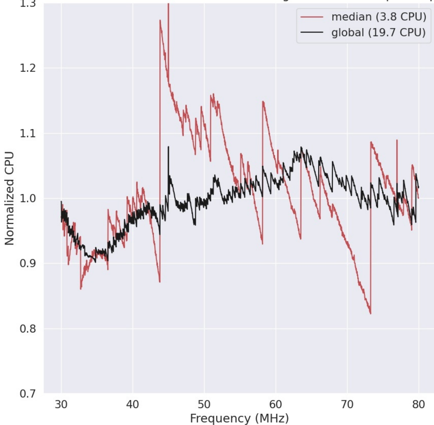
LWA307 - Correlator# 012 - YY - FLAGS:HighTimeVar+BadSpecShape
