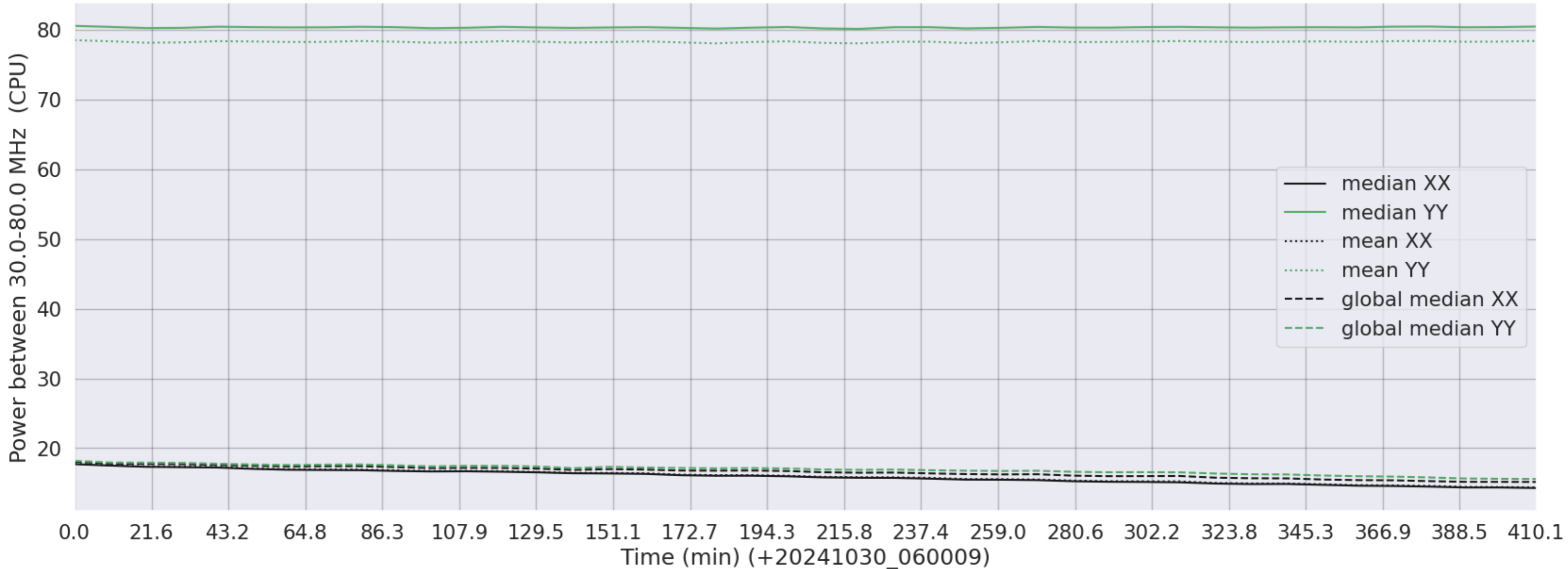
LWA280 - Correlator# 041 - XX FLAGS:BadSpecShape - YY FLAGS:HighPower
