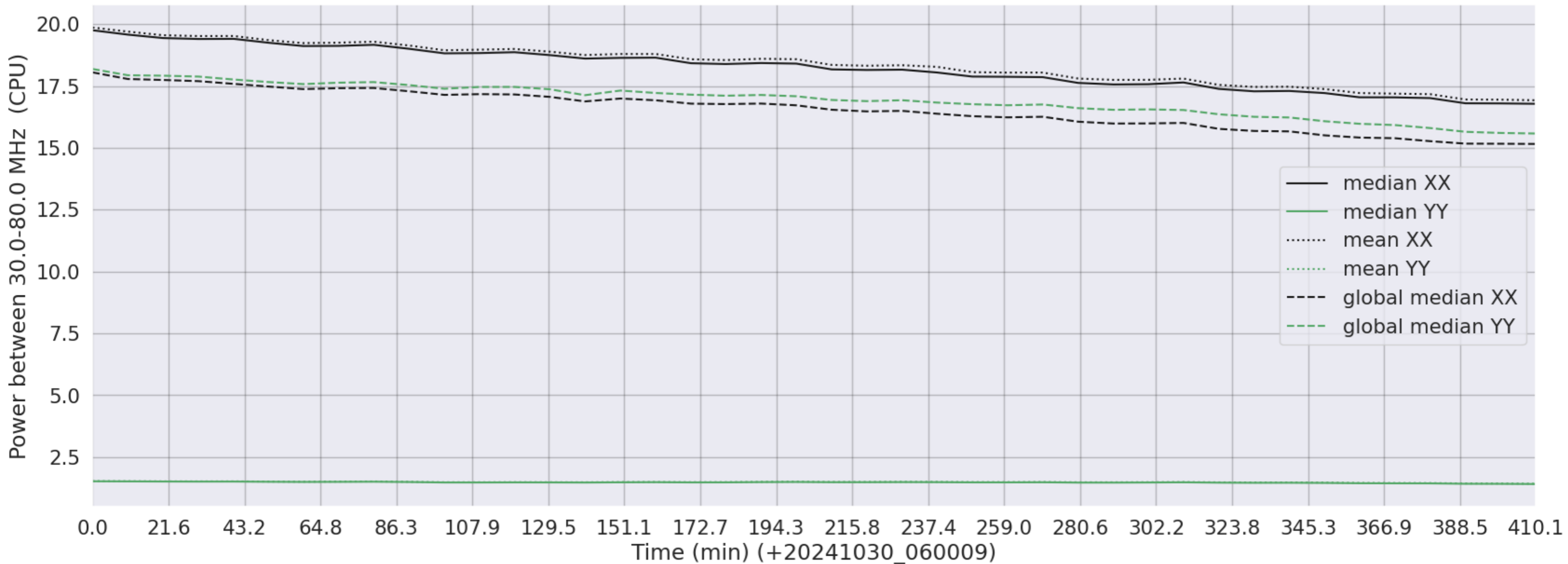
LWA325 - Correlator# 154 - XX FLAGS:Good - YY FLAGS:LowPower
