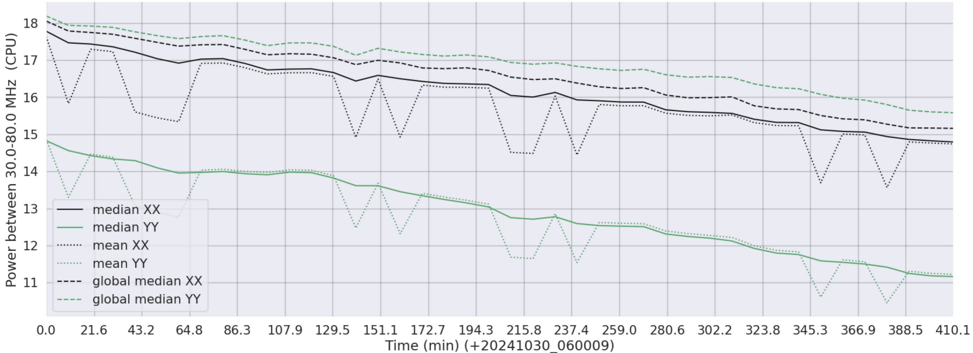
LWA326 - Correlator# 250 - XX FLAGS:Good - YY FLAGS:BadSpecShape
