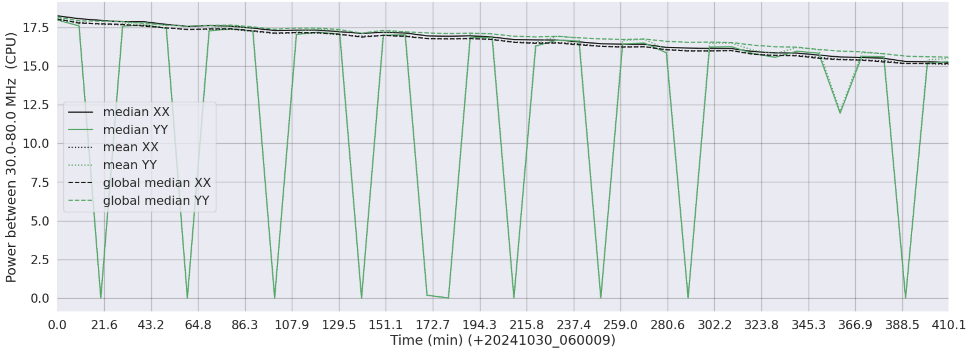
LWA058 - Correlator# 137 - XX FLAGS:Good - YY FLAGS:HighTimeVar
