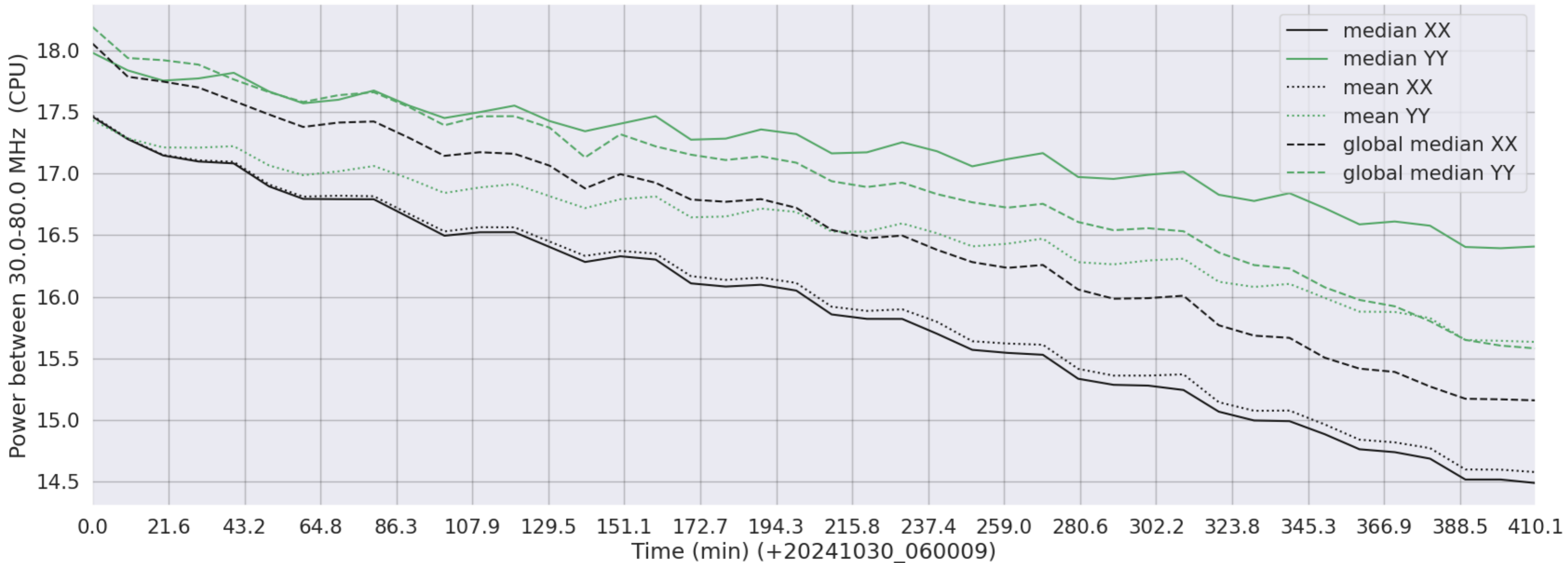
LWA069 - Correlator# 169 - XX FLAGS:Good - YY FLAGS:Good
