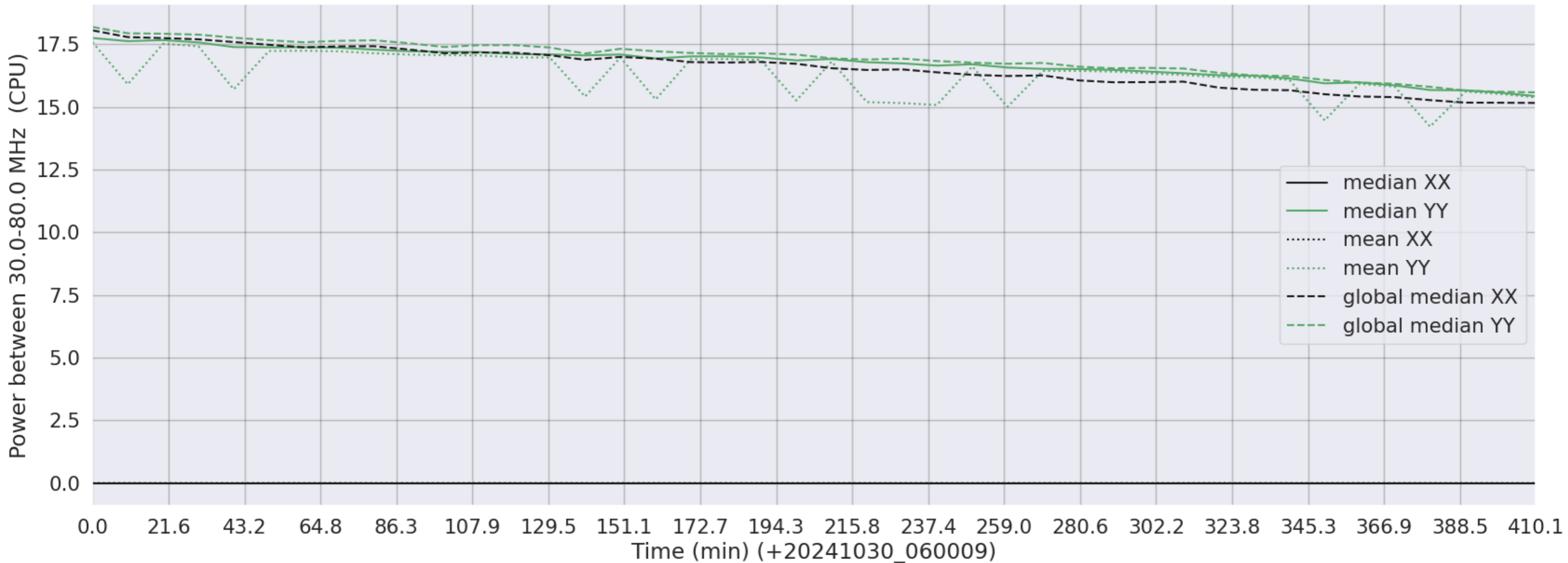
LWA315 - Correlator# 350 - XX FLAGS:LowPower - YY FLAGS:Good
