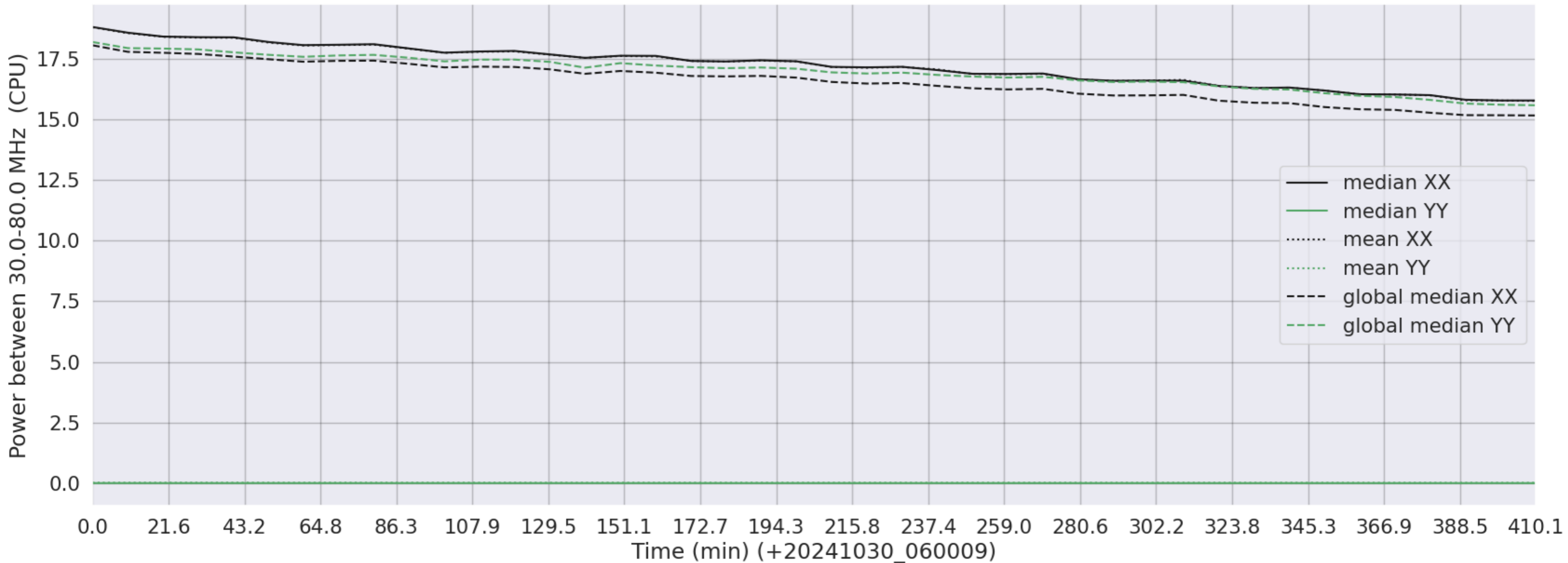
LWA011 - Correlator# 072 - XX FLAGS:Good - YY FLAGS:LowPower
