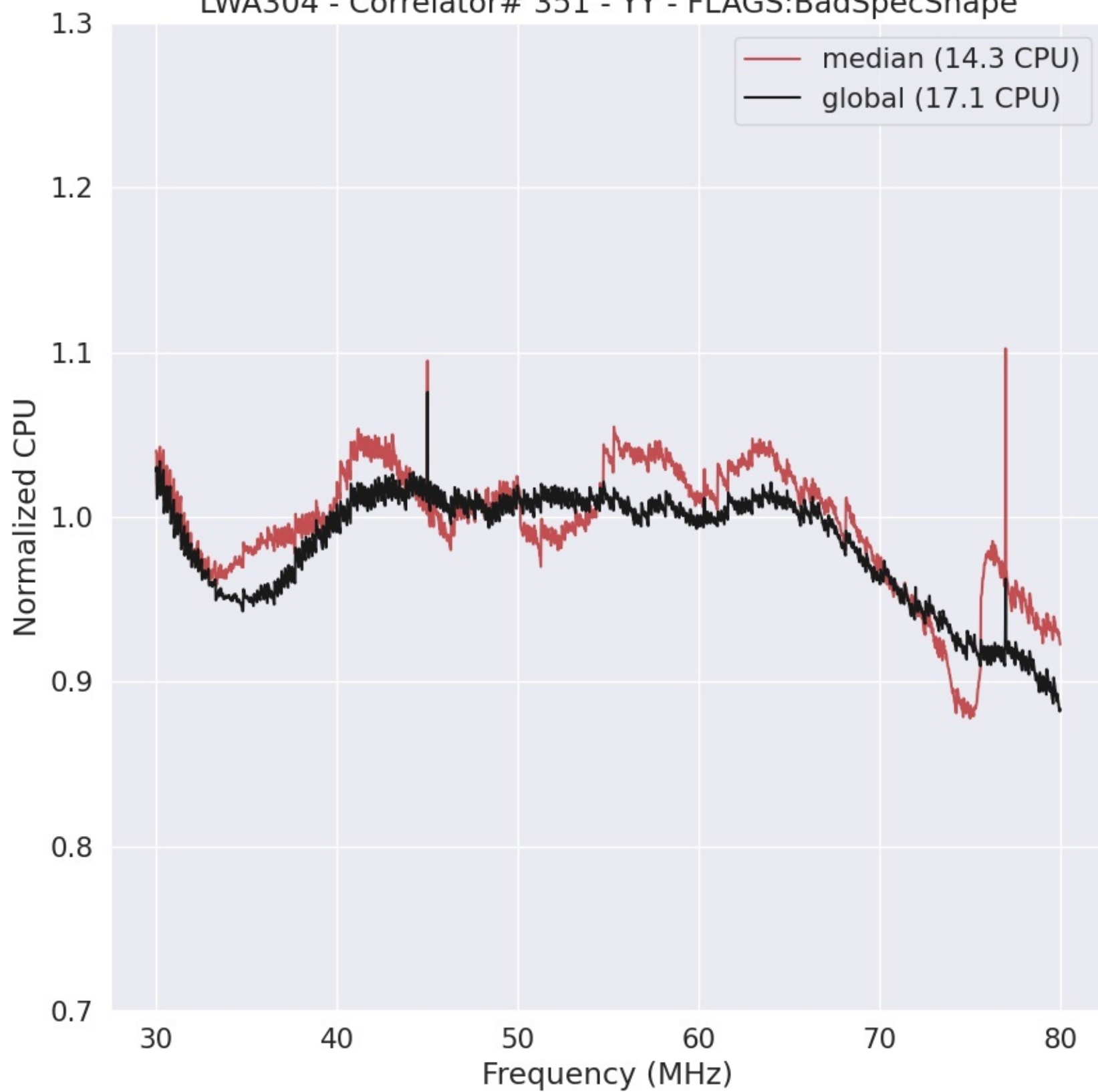
LWA304 - Correlator# 351 - YY - FLAGS:BadSpecShape
