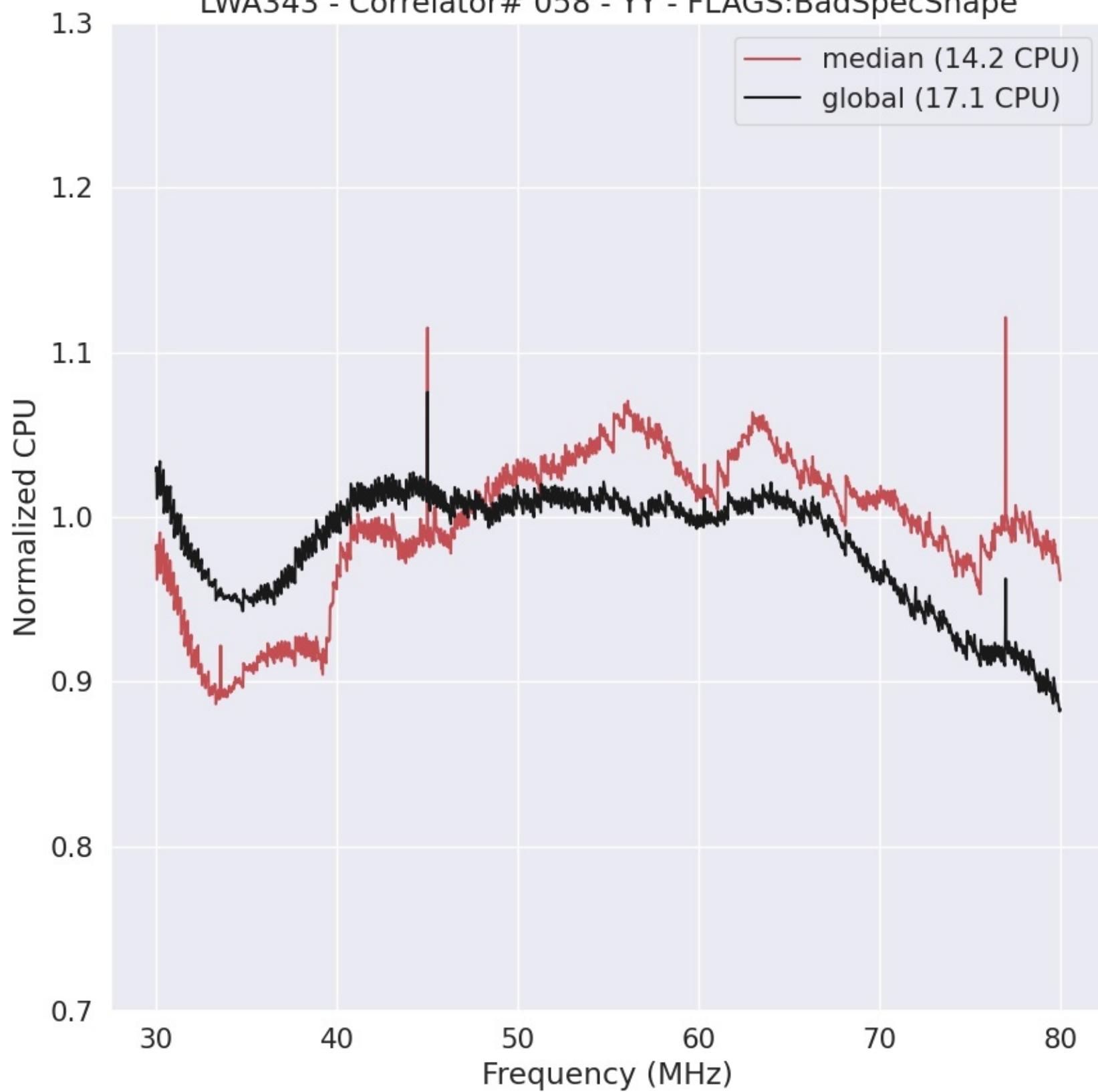
LWA343 - Correlator# 058 - YY - FLAGS:BadSpecShape
