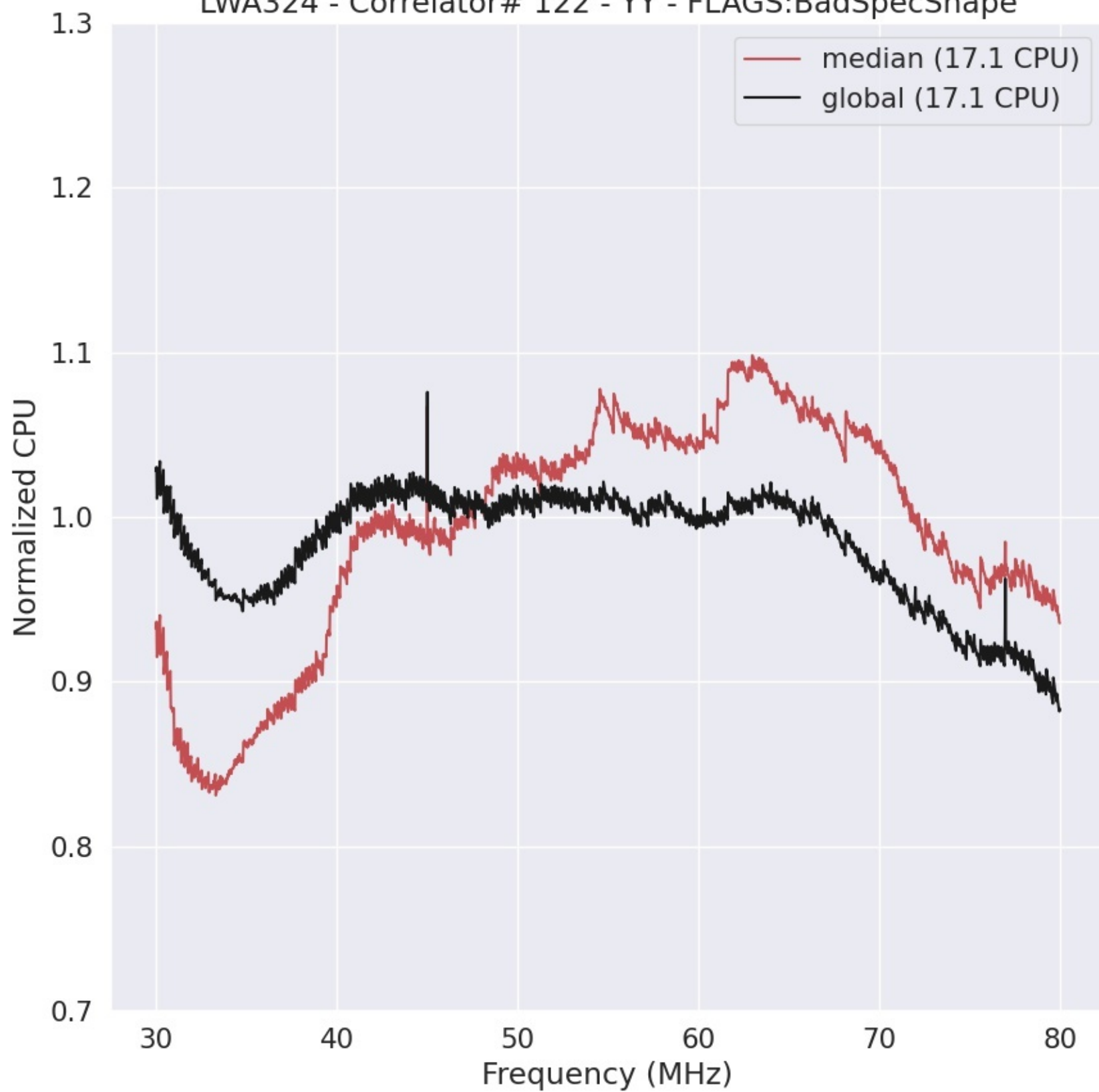
LWA324 - Correlator# 122 - YY - FLAGS:BadSpecShape
