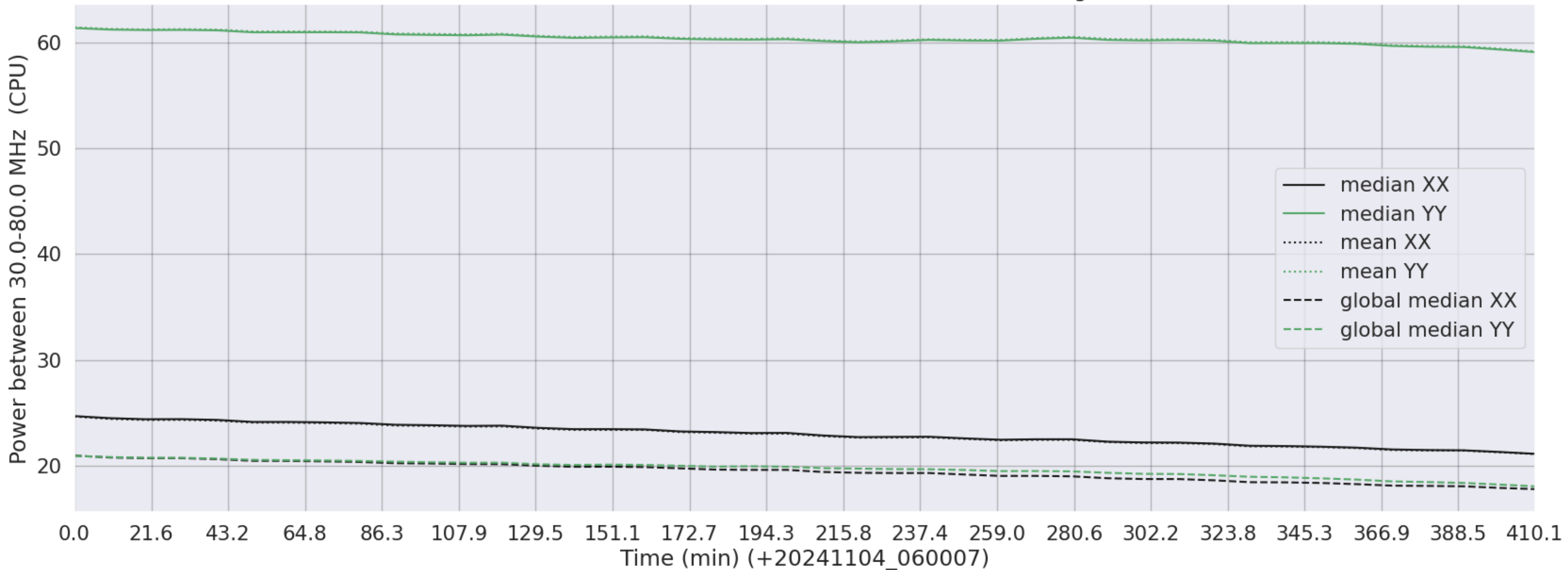
LWA325 - Correlator# 154 - XX FLAGS:Good - YY FLAGS:HighPower
