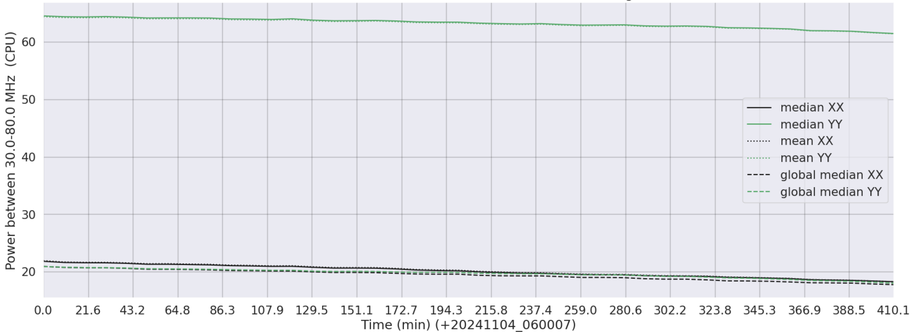
LWA292 - Correlator# 044 - XX FLAGS:Good - YY FLAGS:HighPower
