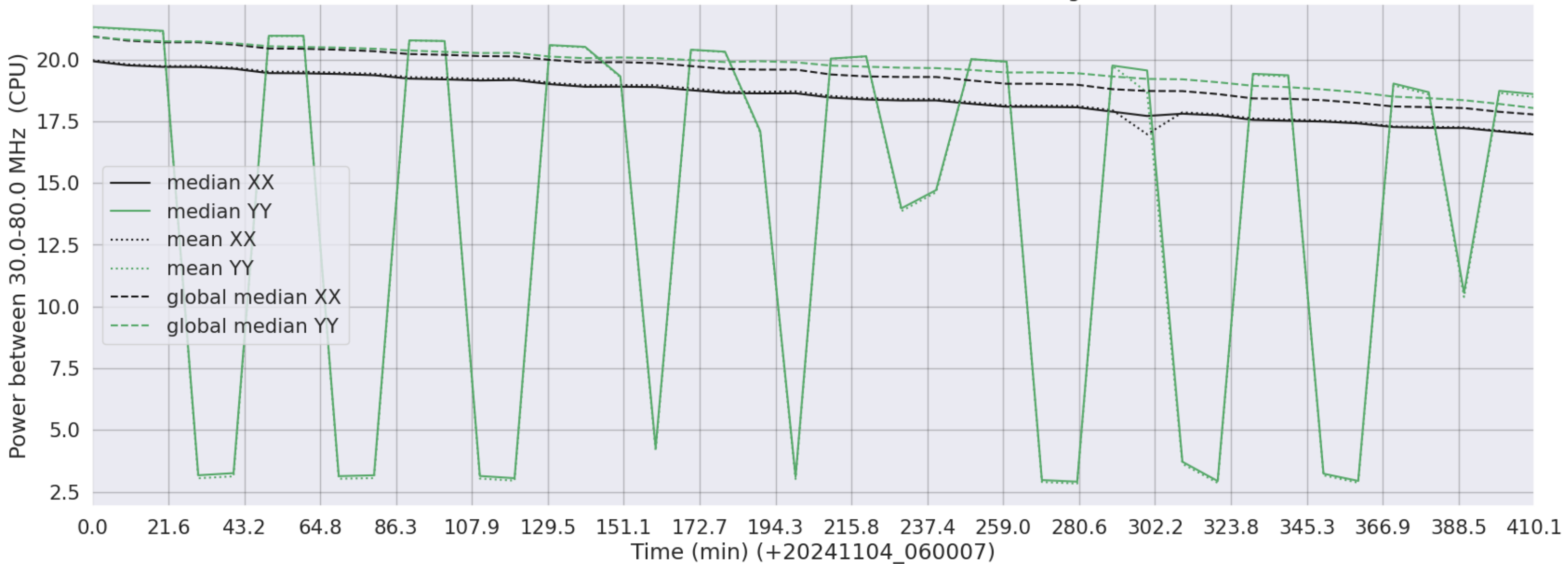
LWA139 - Correlator# 187 - XX FLAGS:Good - YY FLAGS:HighTimeVar
