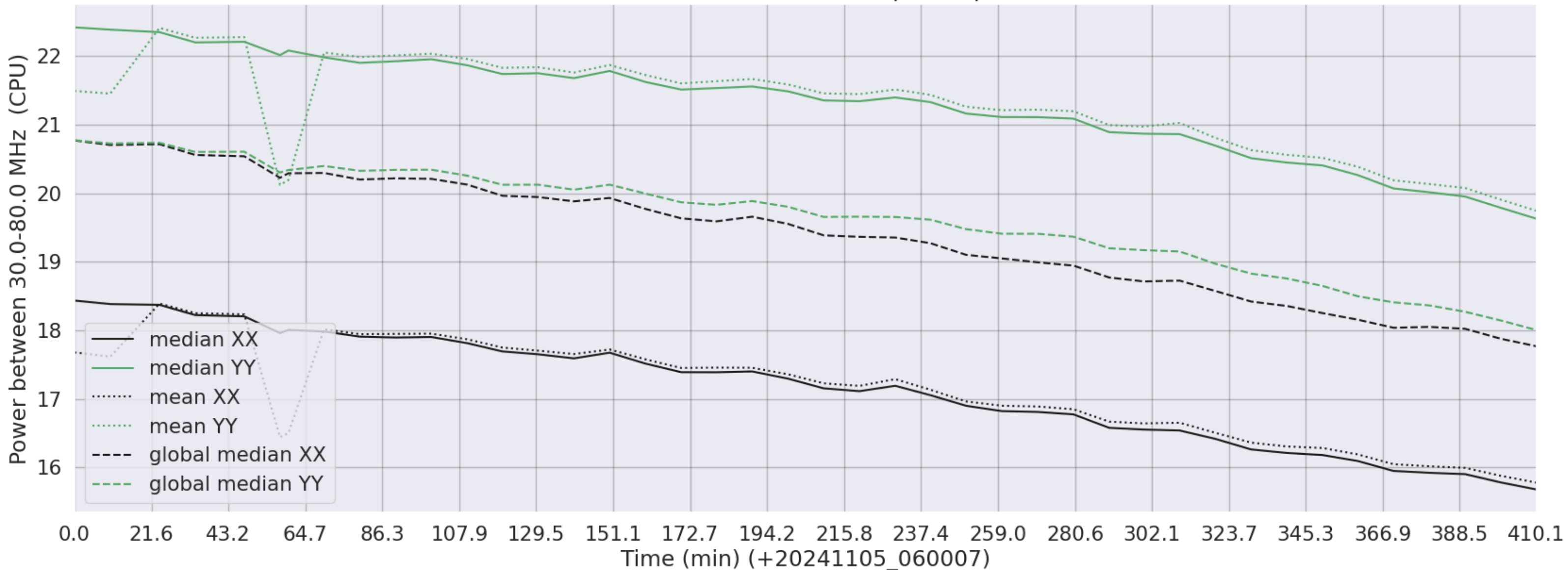
LWA045 - Correlator# 083 - XX FLAGS:BadSpecShape - YY FLAGS:Good
