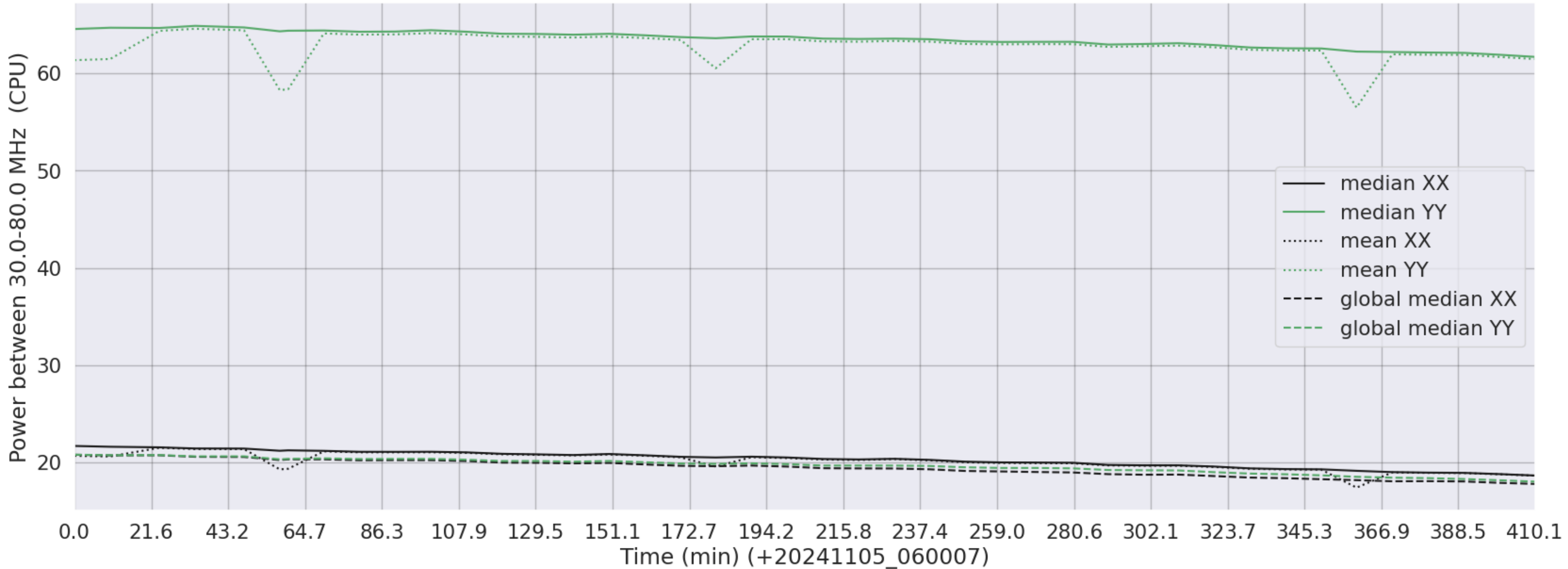
LWA244 - Correlator# 338 - XX FLAGS:Good - YY FLAGS:HighPower
