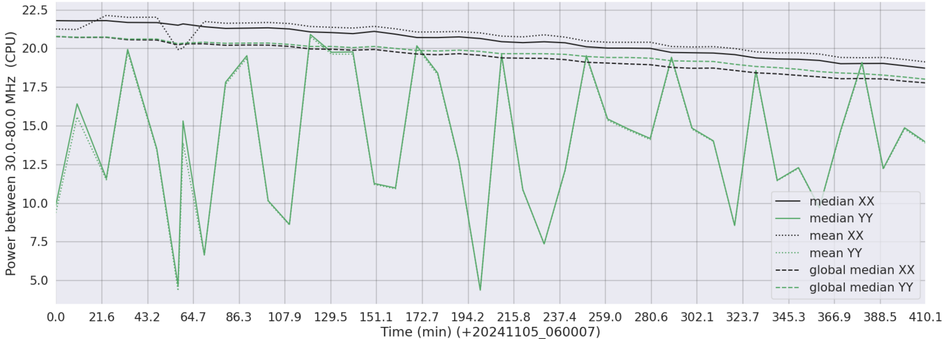
LWA009 - Correlator# 070 - XX FLAGS:Good - YY FLAGS:HighTimeVar+BadSpecShape
