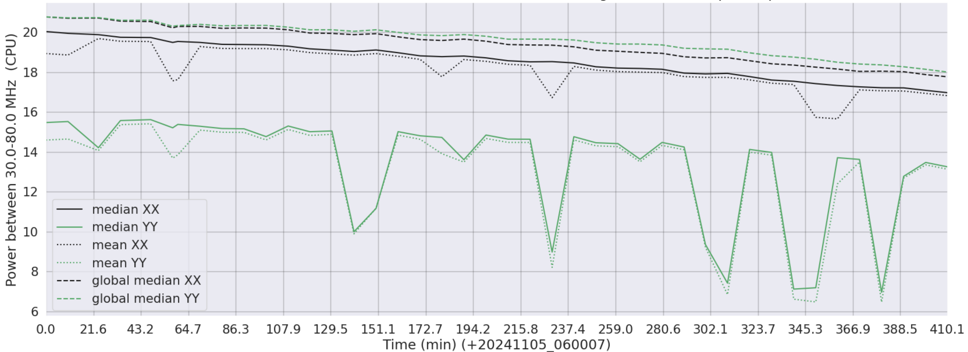
LWA127 - Correlator# 225 - XX FLAGS:Good - YY FLAGS:HighTimeVar+BadSpecShape
