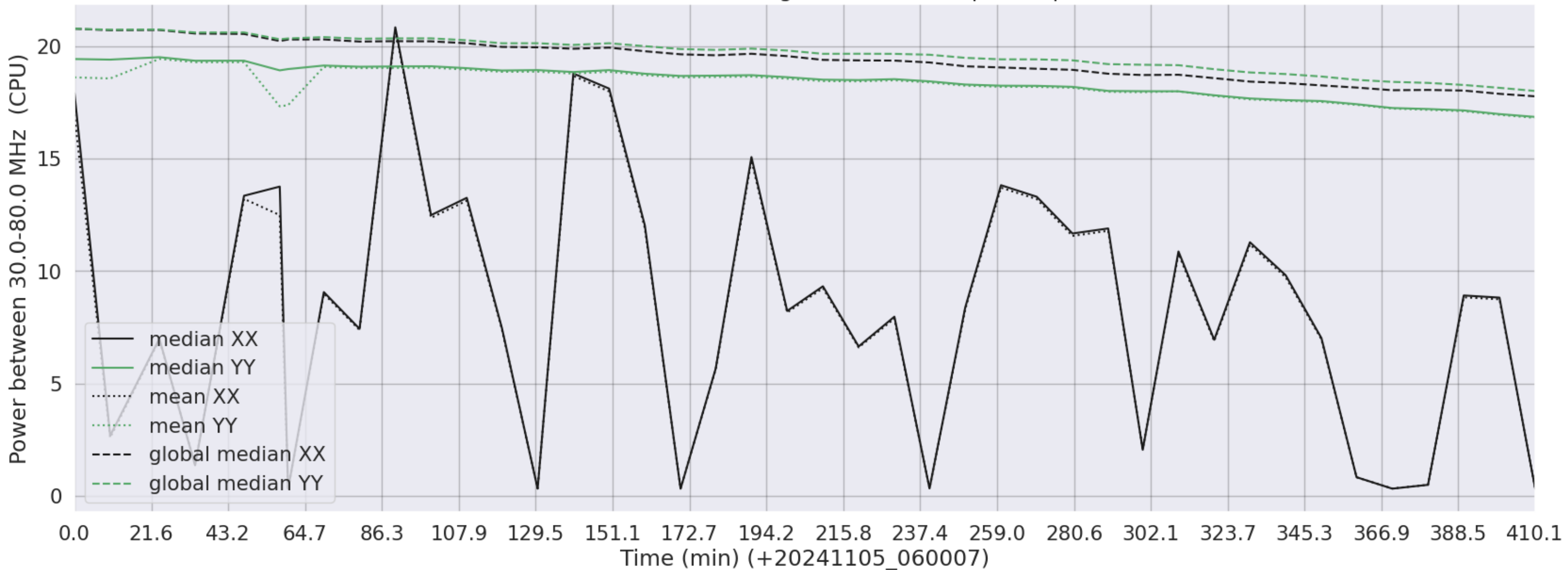
LWA052 - Correlator# 117 - XX FLAGS:HighTimeVar+BadSpecShape - YY FLAGS:Good
