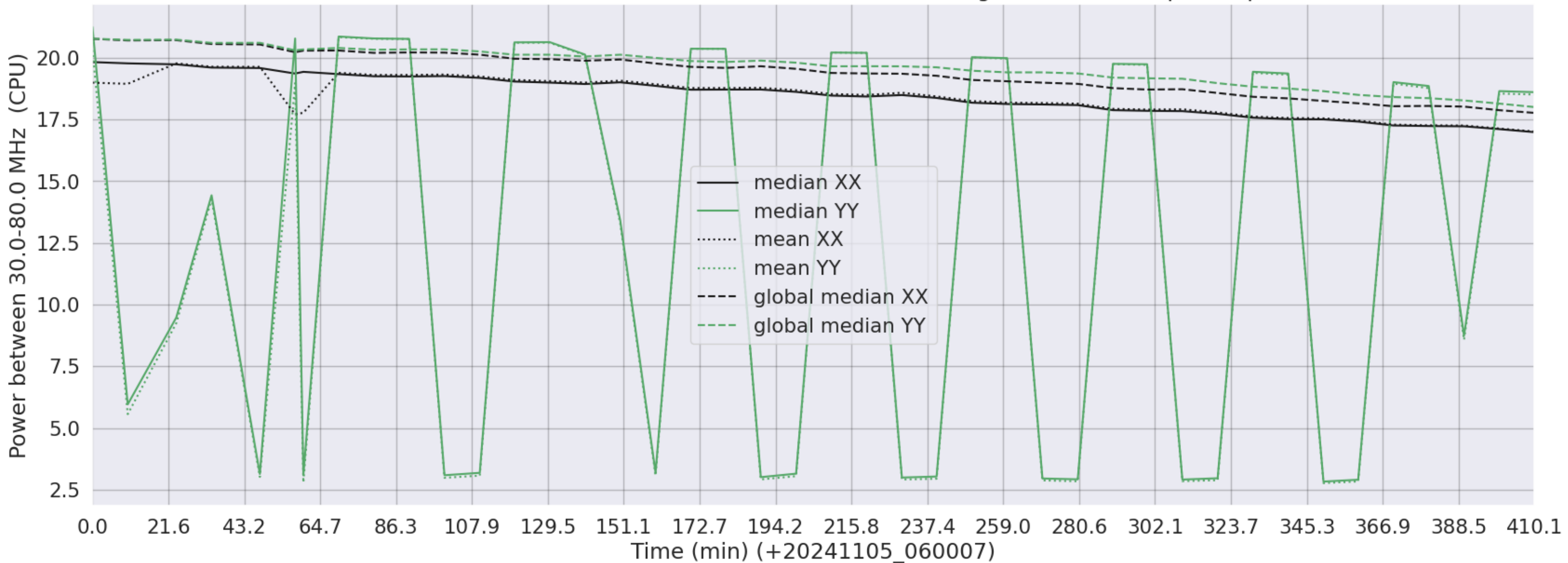
LWA139 - Correlator# 187 - XX FLAGS:Good - YY FLAGS:HighTimeVar+BadSpecShape
