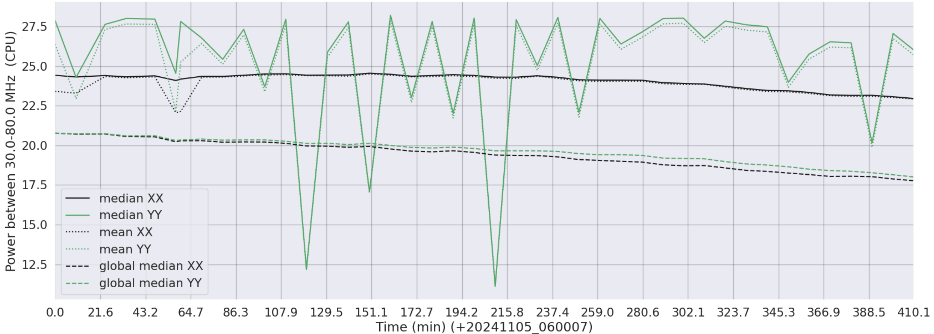
LWA309 - Correlator# 014 - XX FLAGS:Good - YY FLAGS:HighTimeVar
