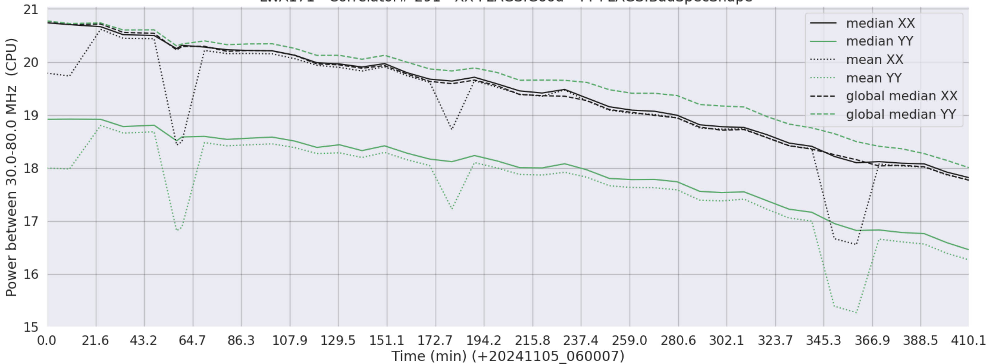
LWA171 - Correlator# 291 - XX FLAGS:Good - YY FLAGS:BadSpecShape
