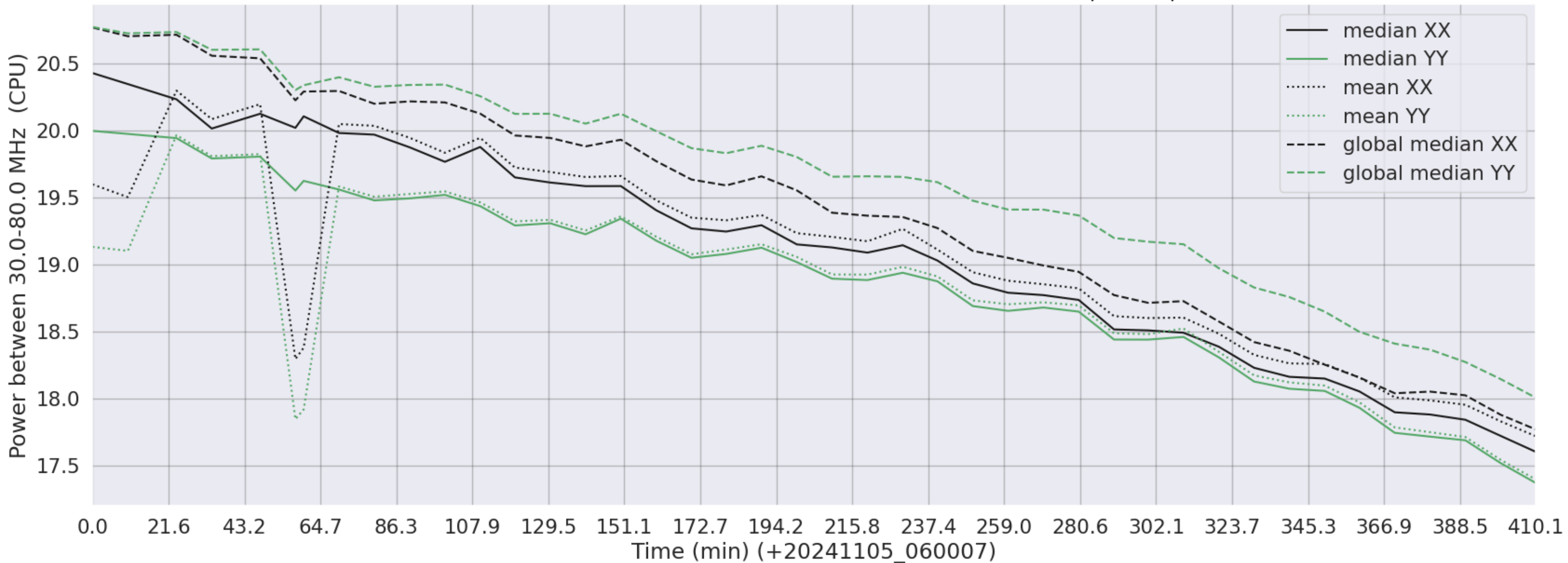
LWA102 - Correlator# 177 - XX FLAGS:Good - YY FLAGS:BadSpecShape
