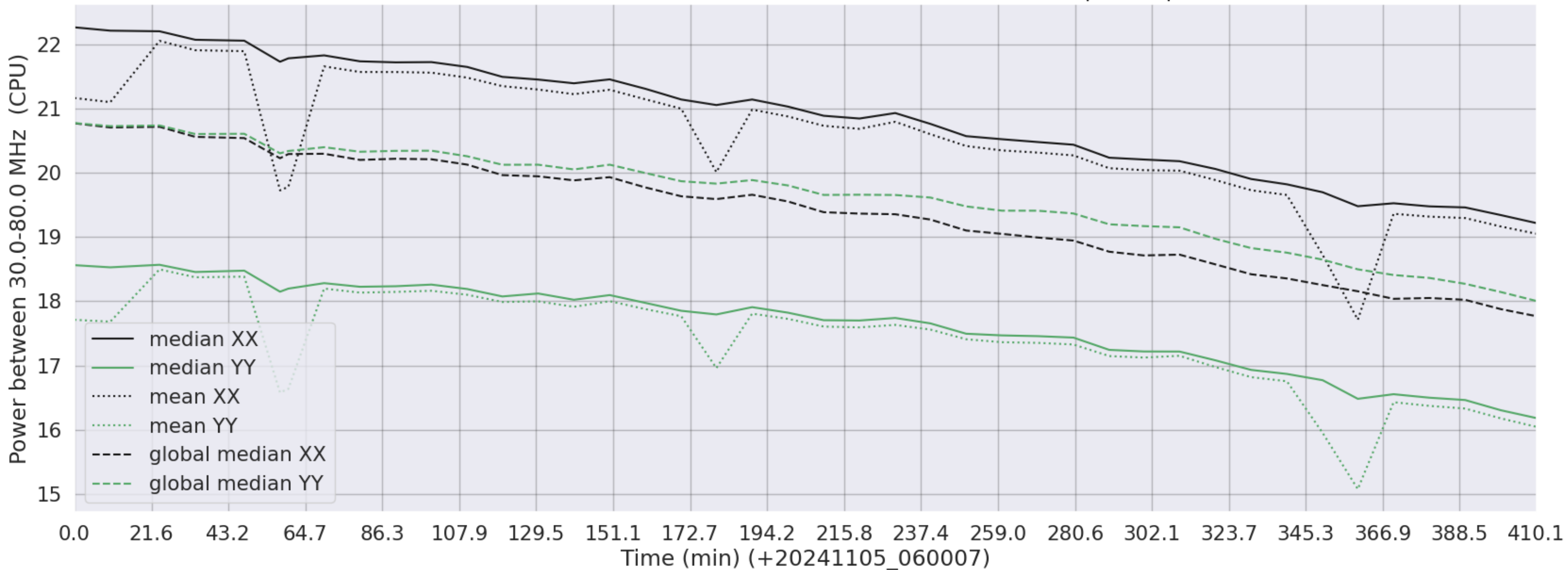
LWA207 - Correlator# 299 - XX FLAGS:Good - YY FLAGS:BadSpecShape
