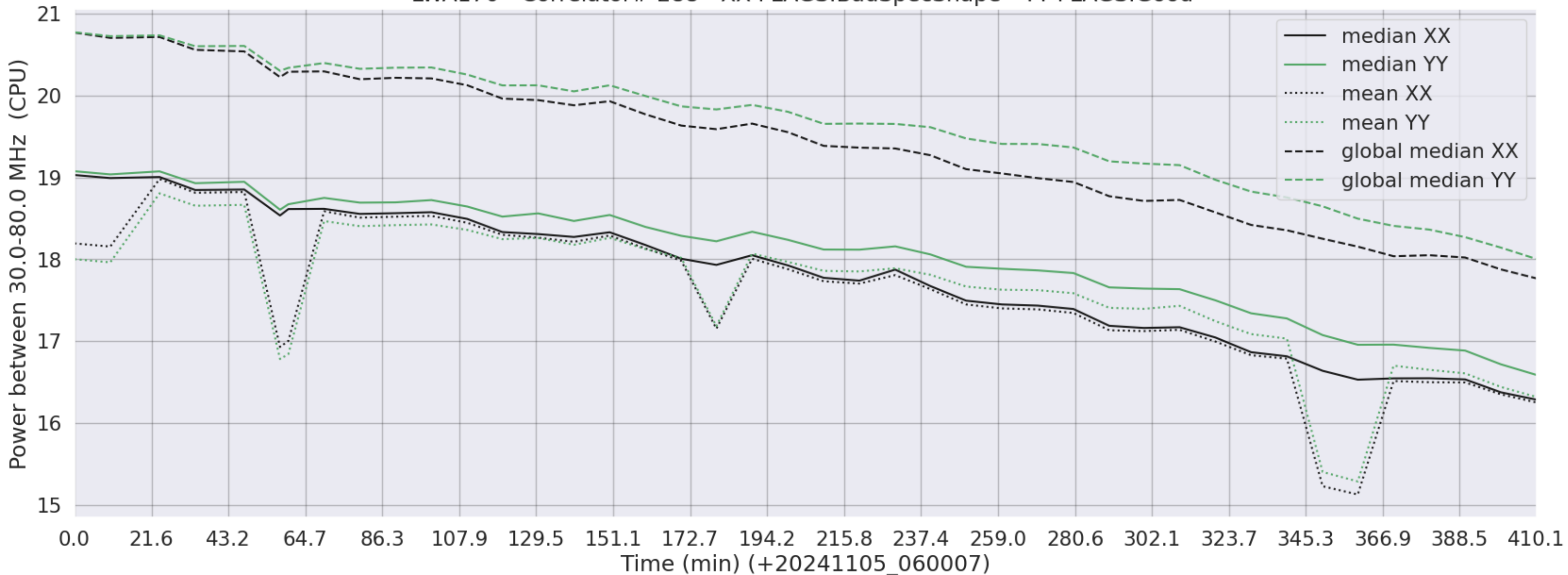
LWA170 - Correlator# 288 - XX FLAGS:BadSpecShape - YY FLAGS:Good
