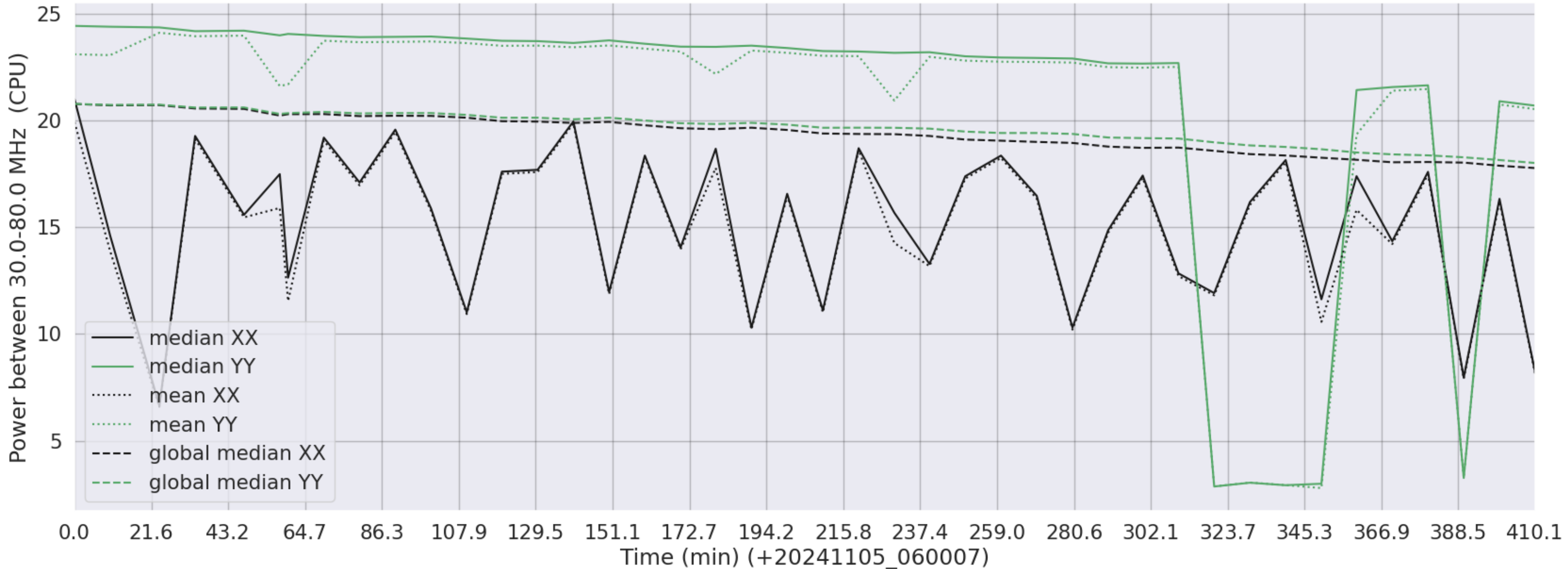
LWA124 - Correlator# 224 - XX FLAGS:HighTimeVar - YY FLAGS:HighTimeVar
