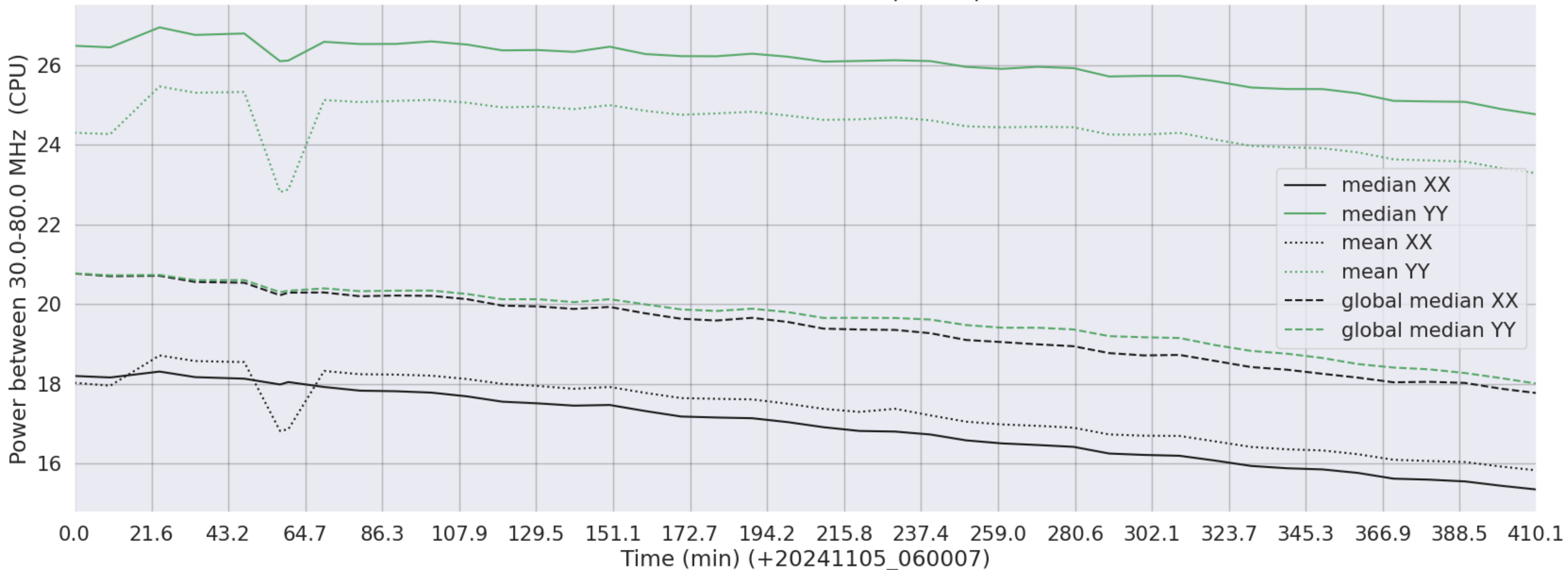
LWA069 - Correlator# 169 - XX FLAGS:BadSpecShape - YY FLAGS:Good
