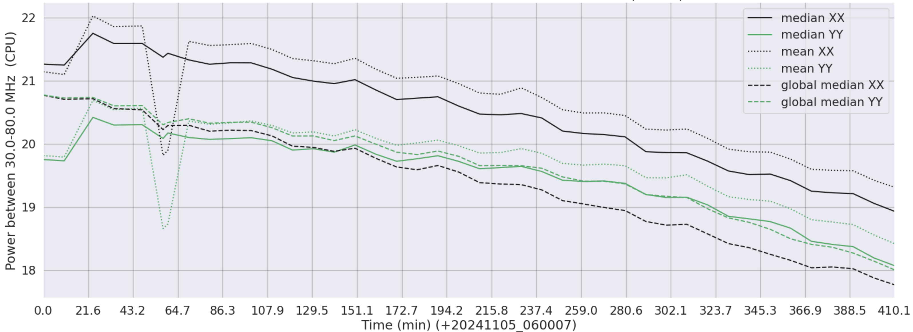
LWA034 - Correlator# 162 - XX FLAGS:Good - YY FLAGS:BadSpecShape
