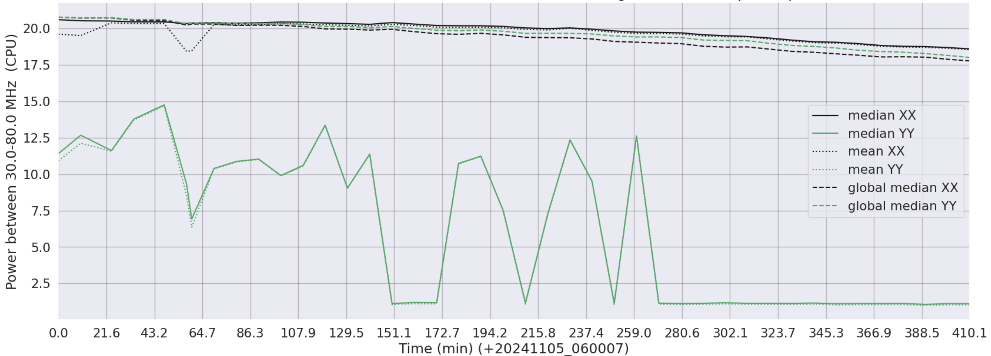
LWA307 - Correlator# 012 - XX FLAGS:Good - YY FLAGS:HighTimeVar+BadSpecShape
