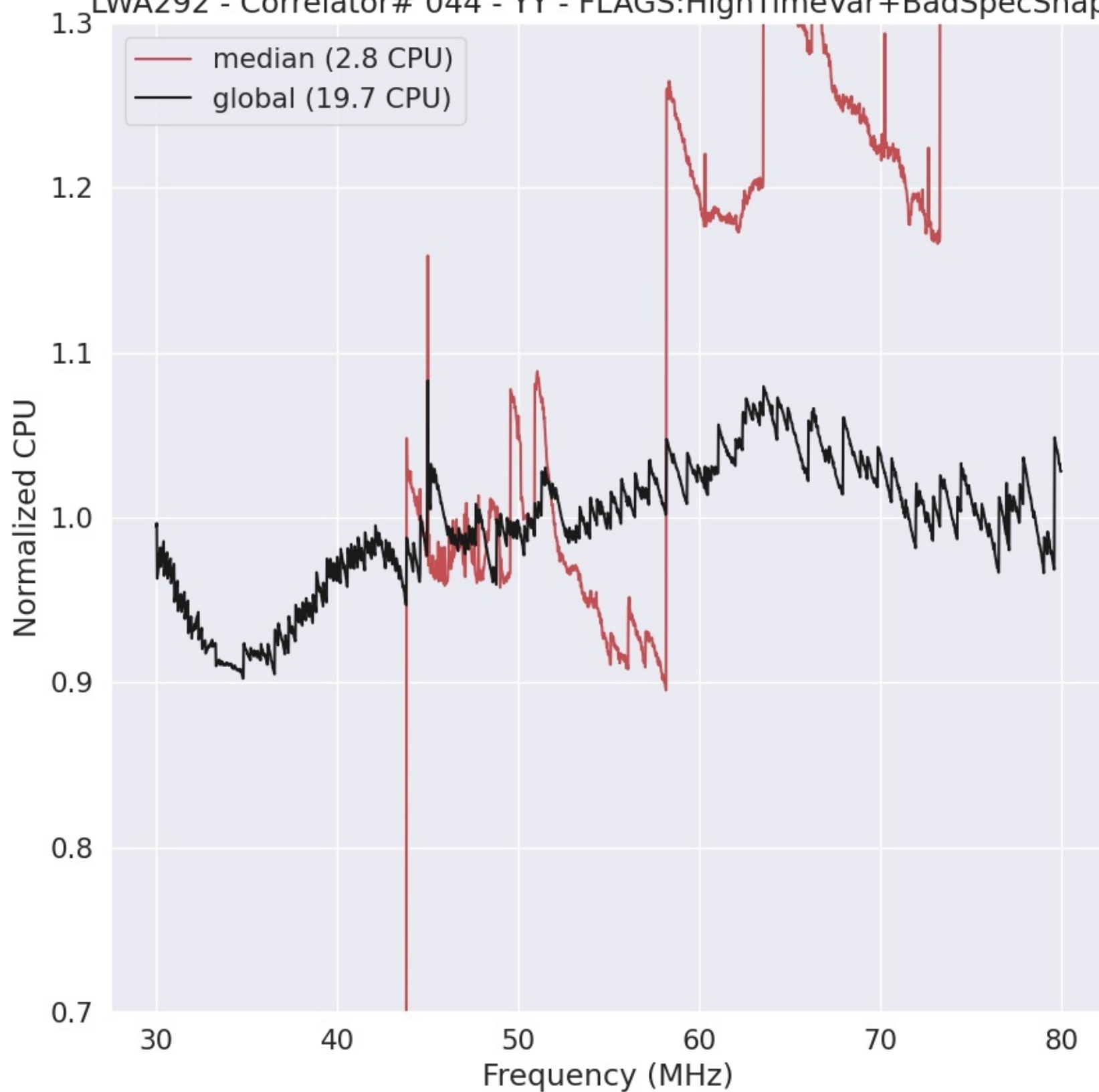
LWA292 - Correlator# 044 - YY - FLAGS:HighTimeVar+BadSpecShape
