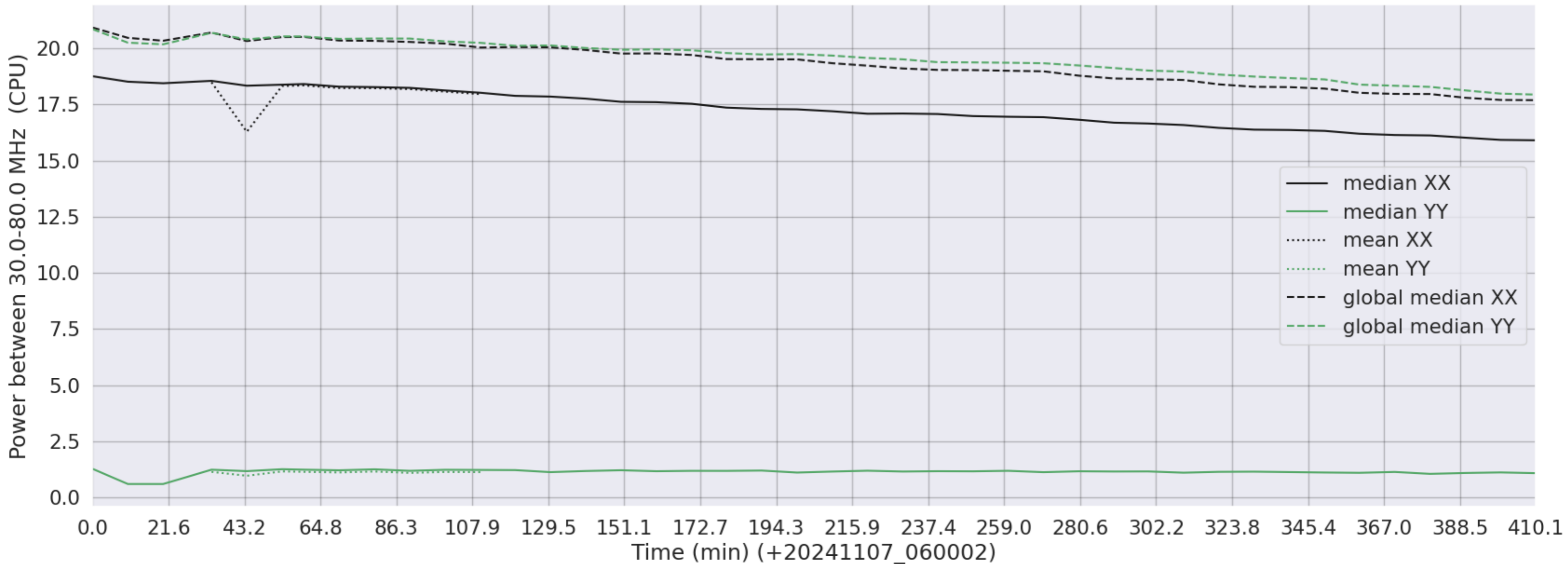
LWA307 - Correlator# 012 - XX FLAGS:Good - YY FLAGS:LowPower
