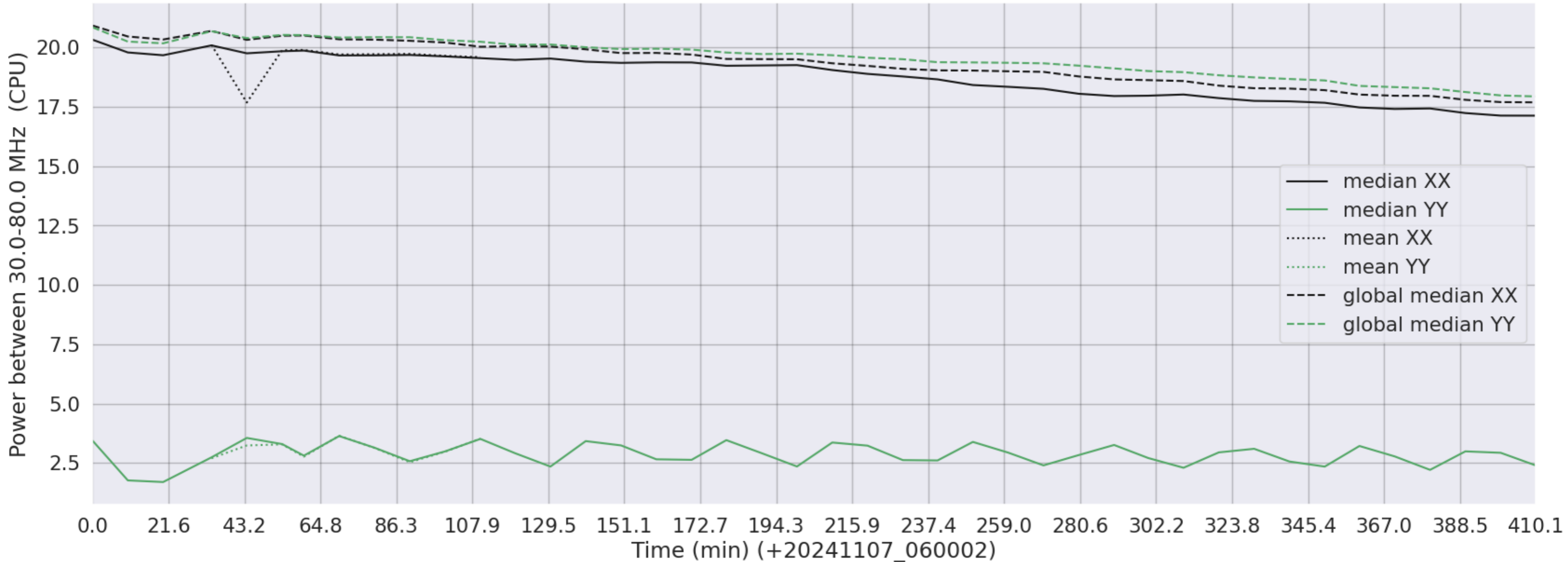
LWA292 - Correlator# 044 - XX FLAGS:Good - YY FLAGS:HighTimeVar+BadSpecShape
