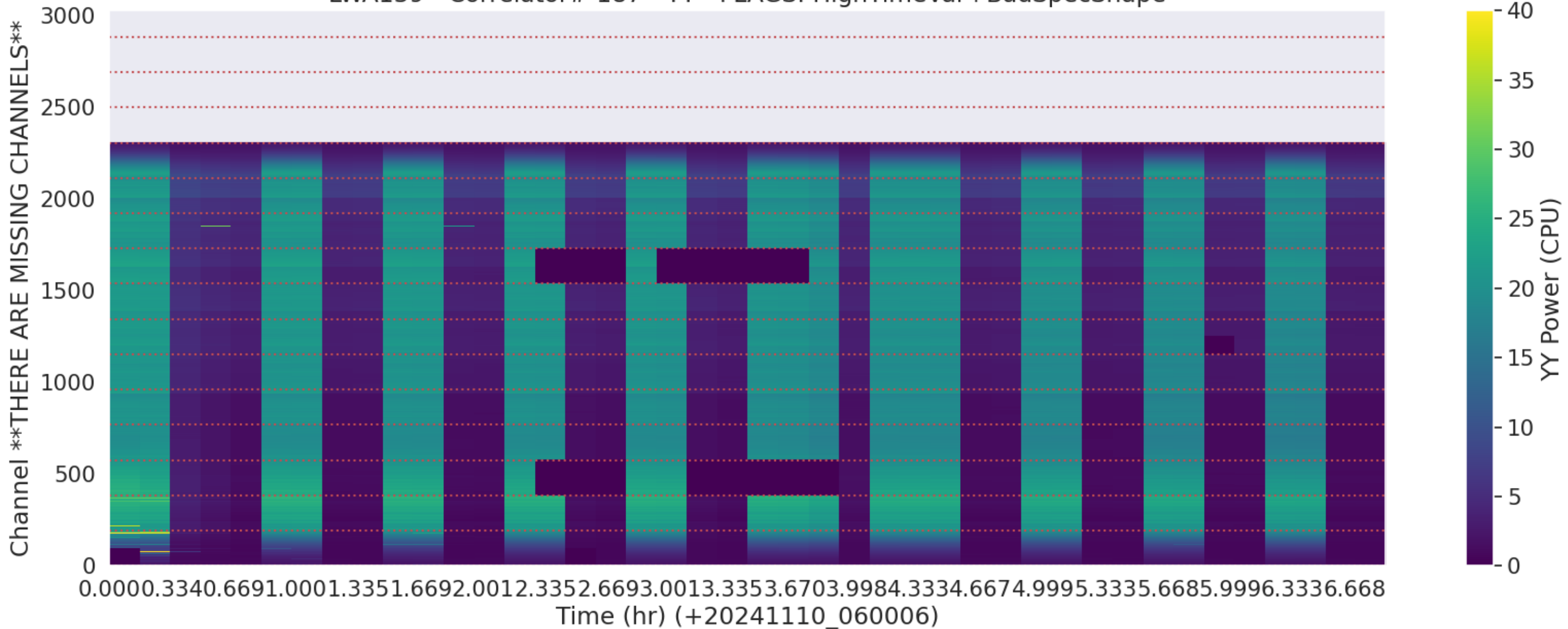
LWA139 - Correlator# 187 - YY - FLAGS: HighTimeVar+BadSpecShape
