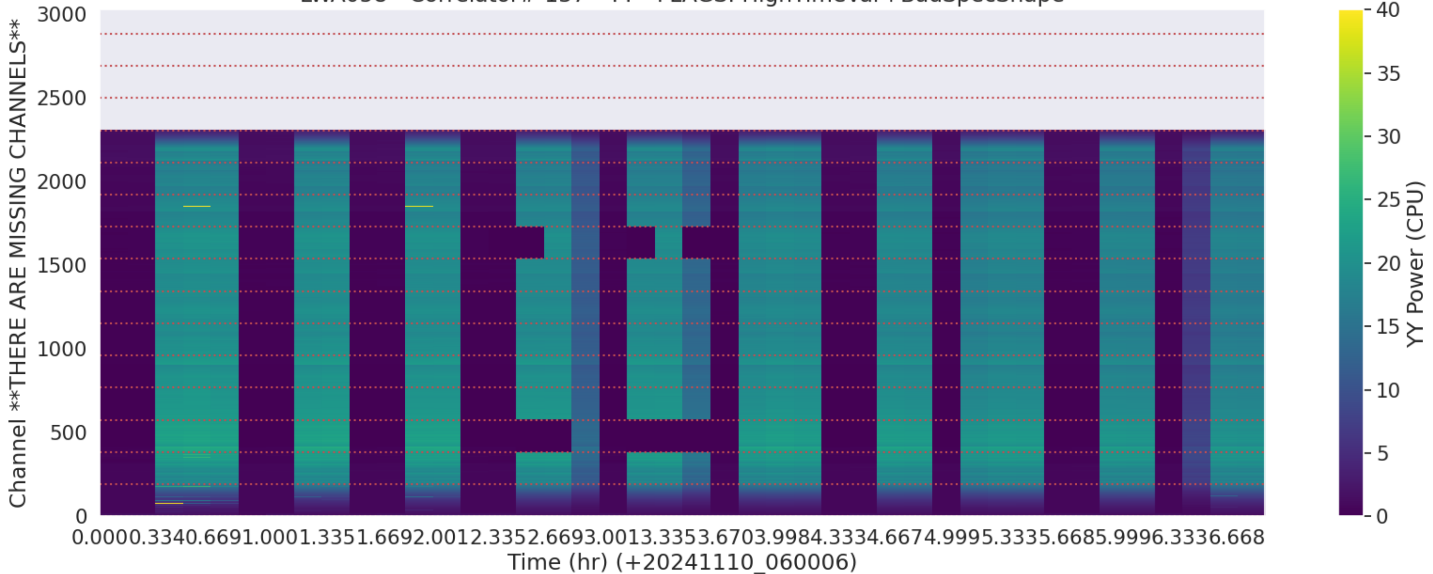
LWA058 - Correlator# 137 - YY - FLAGS: HighTimeVar+BadSpecShape
