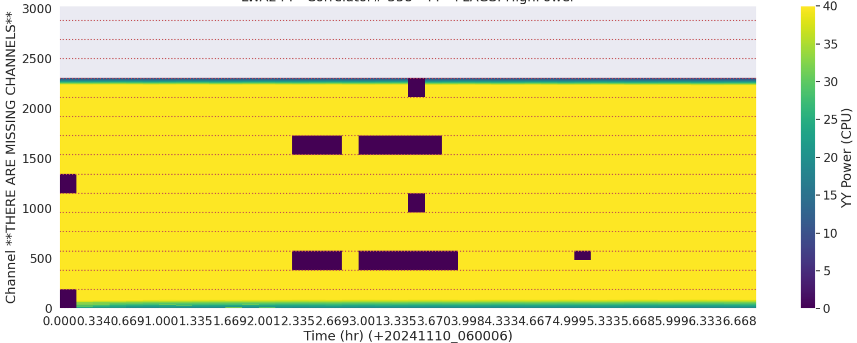
LWA244 - Correlator# 338 - YY - FLAGS: HighPower
