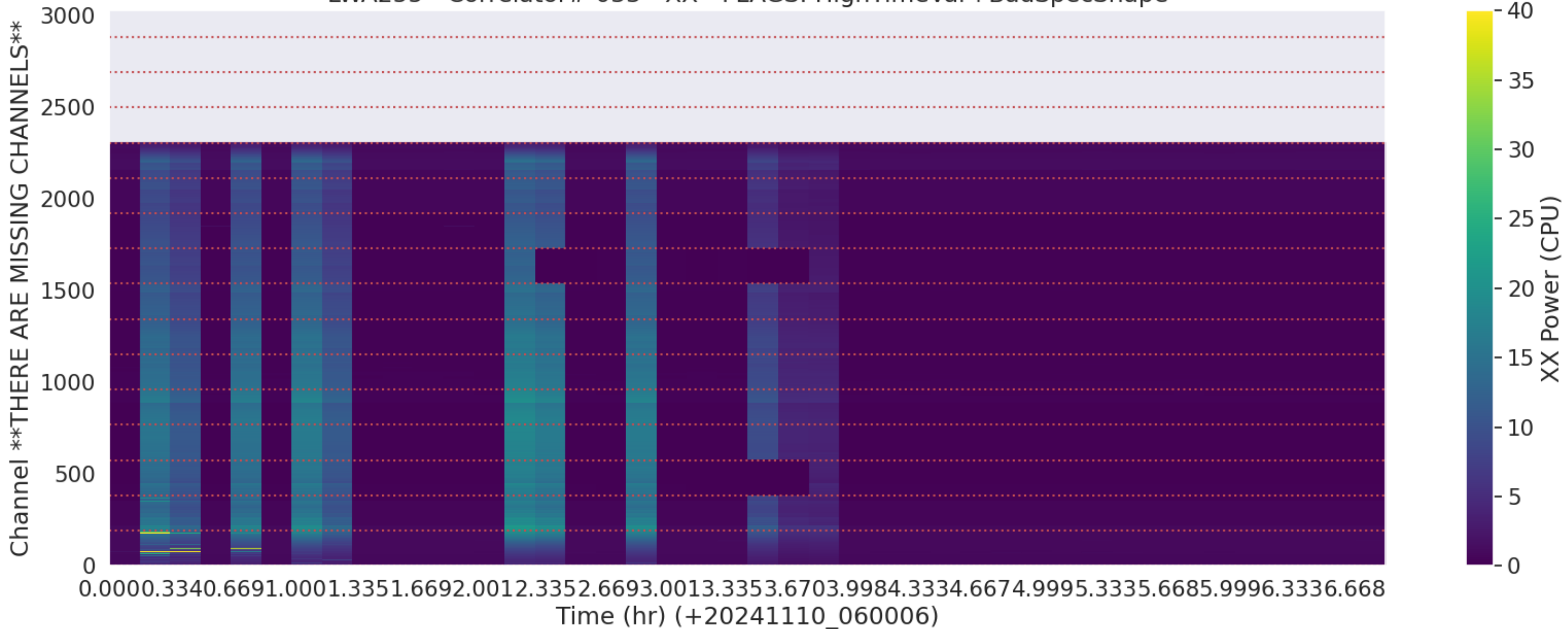
LWA255 - Correlator# 033 - XX - FLAGS: HighTimeVar+BadSpecShape
