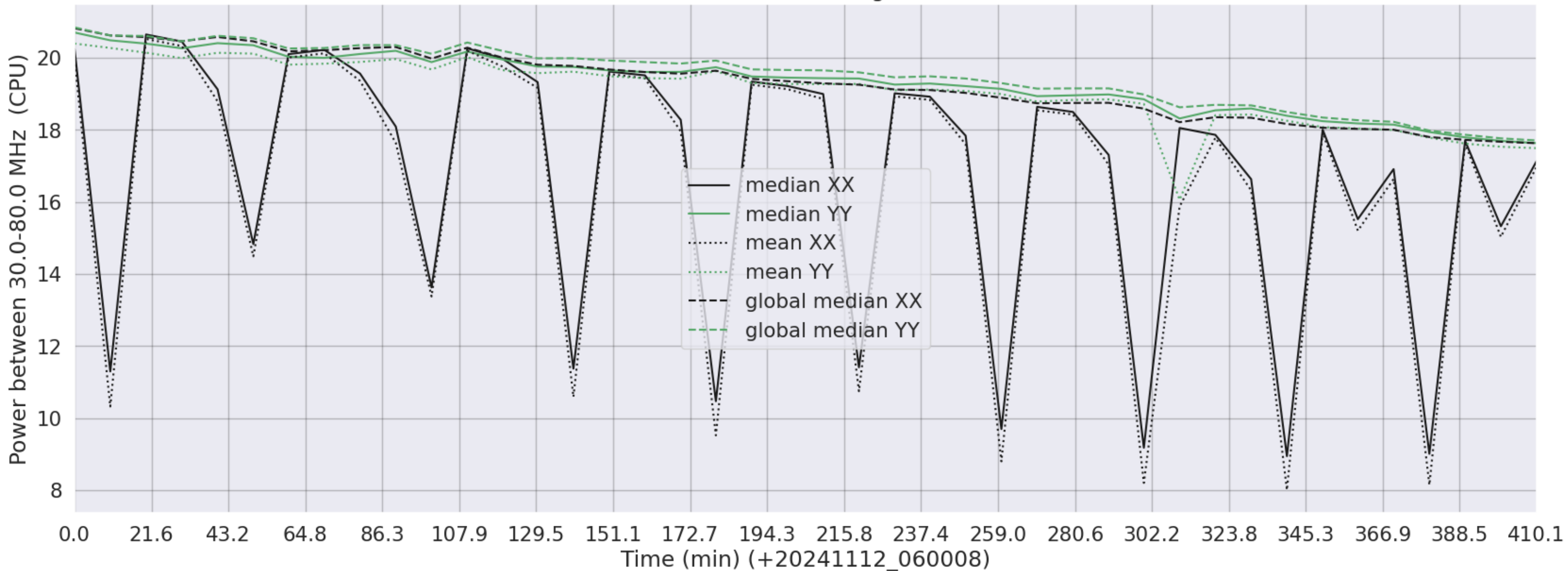
LWA145 - Correlator# 212 - XX FLAGS:HighTimeVar - YY FLAGS:Good
