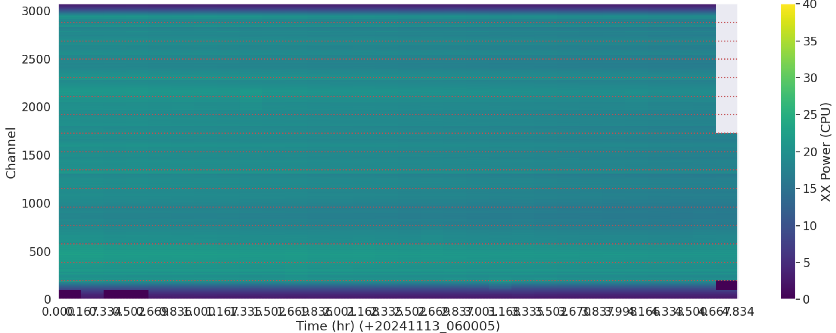
LWA110 - Correlator# 198 - XX - FLAGS: Good
