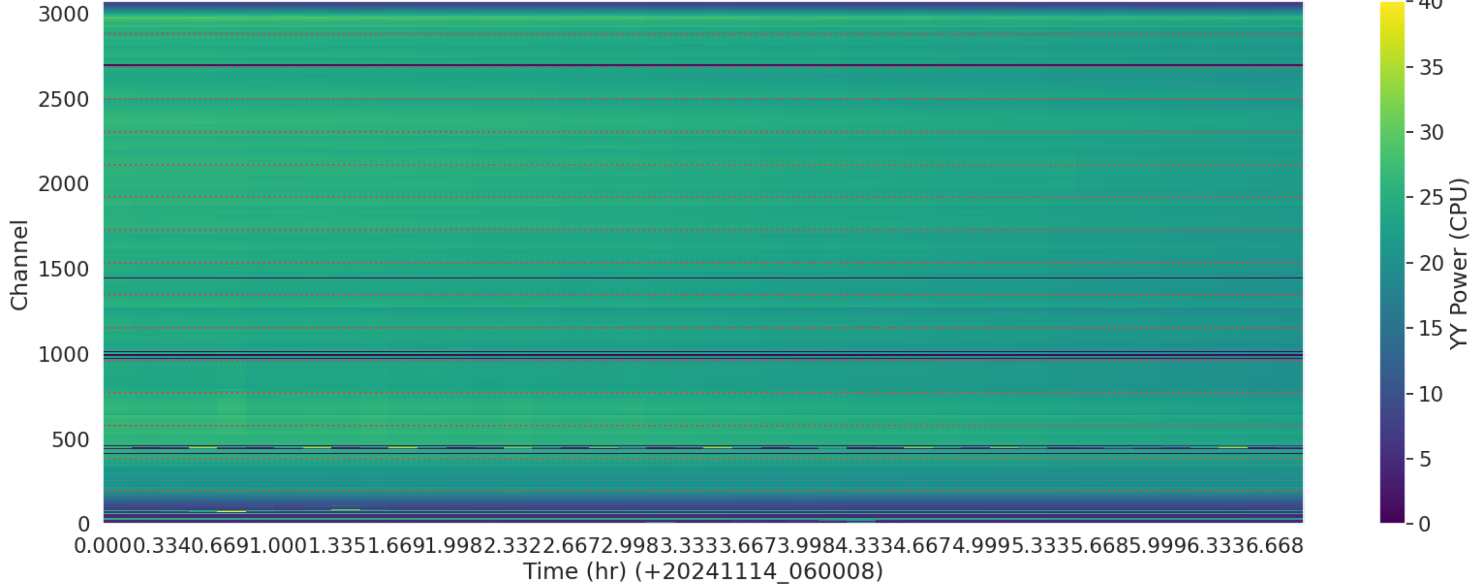
LWA353 - Correlator# 031 - YY - FLAGS: BadSpecShape
