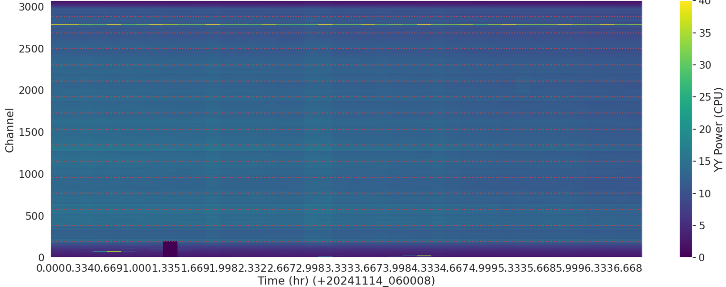
LWA190 - Correlator# 244 - YY - FLAGS: BadSpecShape
