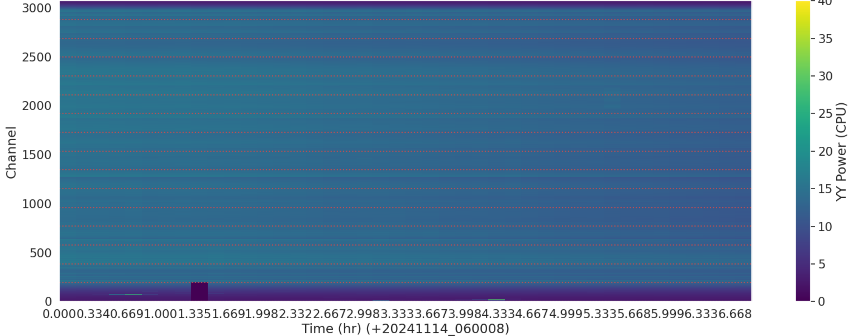
LWA293 - Correlator# 284 - YY - FLAGS: BadSpecShape
