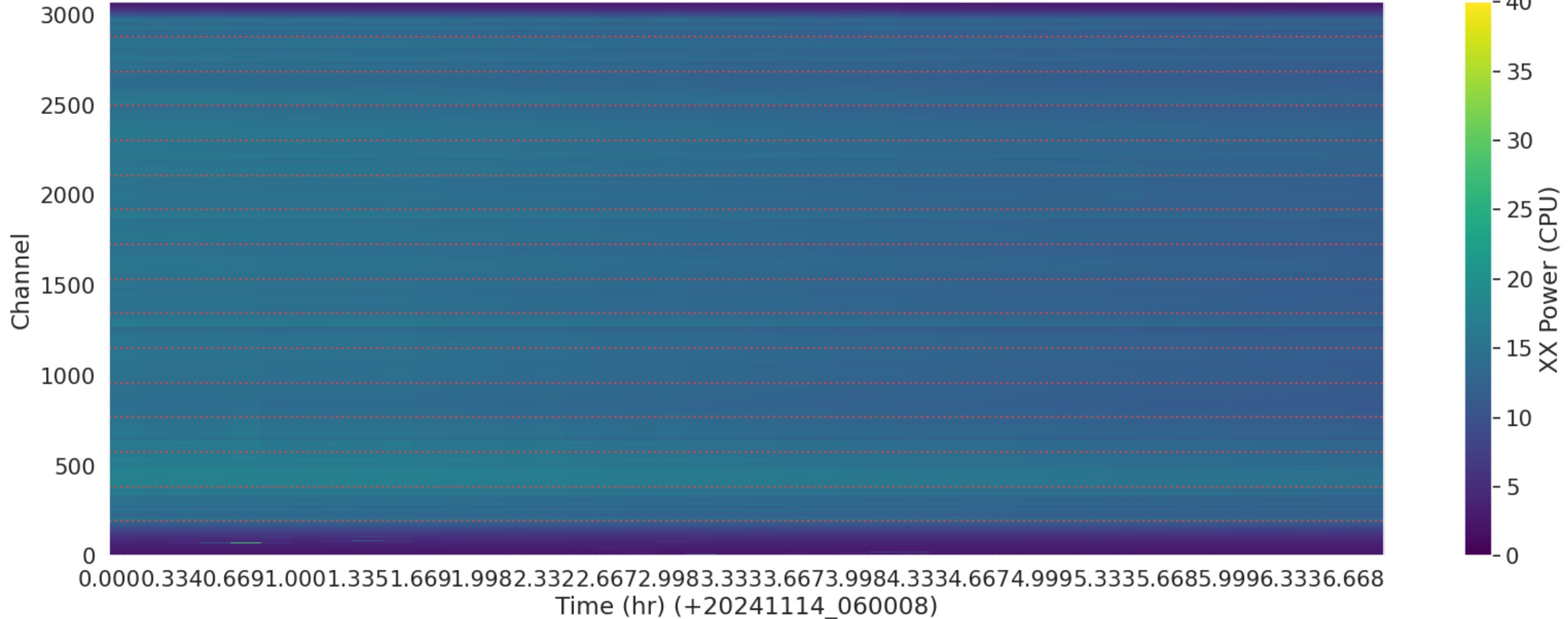
LWA258 - Correlator# 035 - XX - FLAGS: BadSpecShape
