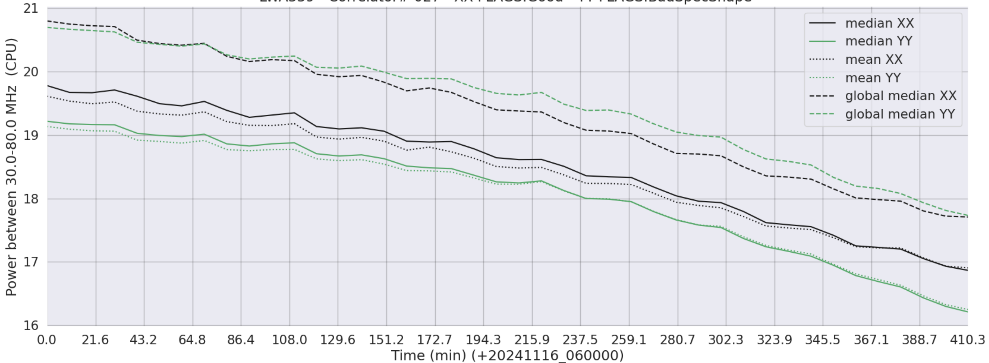
LWA339 - Correlator# 027 - XX FLAGS:Good - YY FLAGS:BadSpecShape
