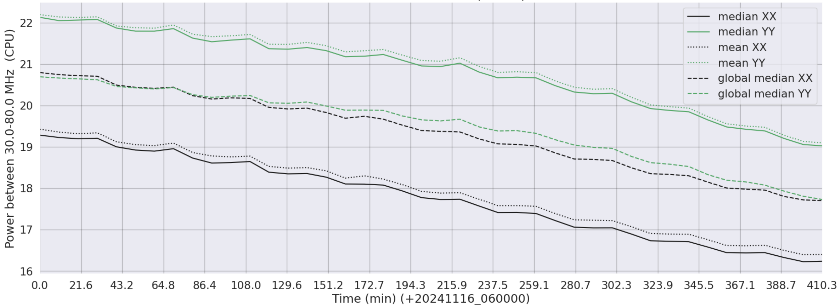
LWA173 - Correlator# 290 - XX FLAGS:BadSpecShape - YY FLAGS:Good
