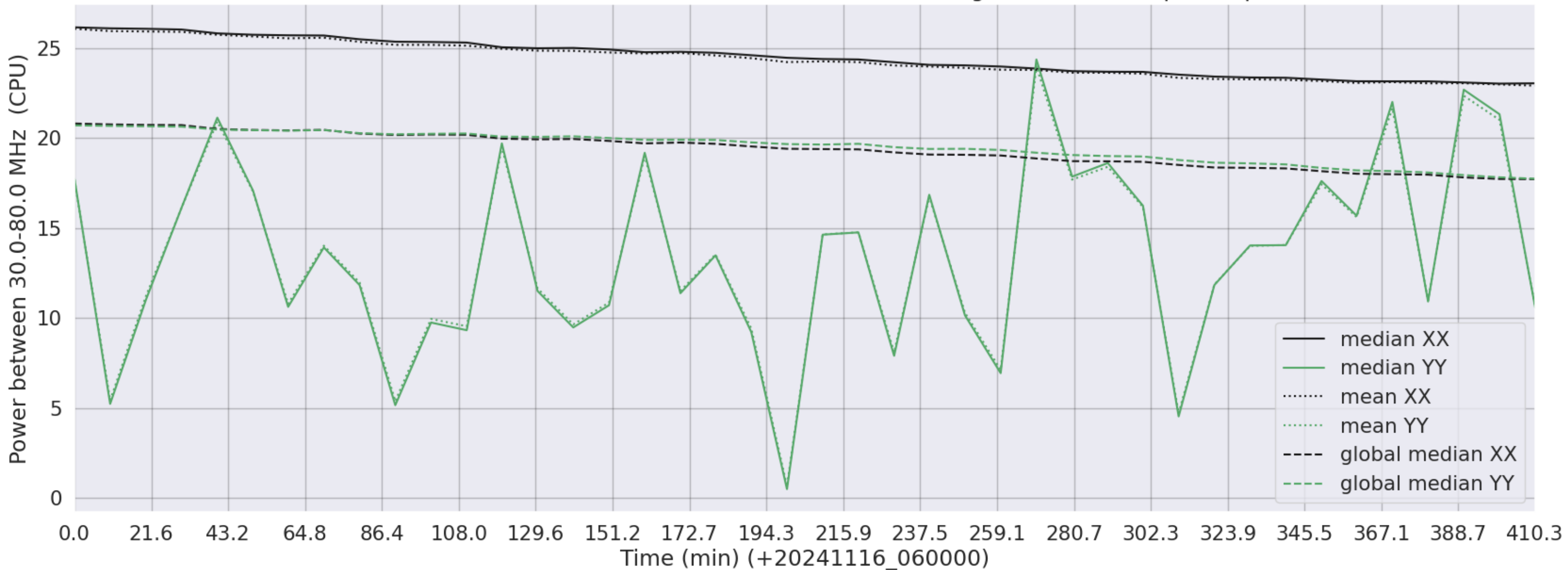
LWA309 - Correlator# 014 - XX FLAGS:Good - YY FLAGS:HighTimeVar+BadSpecShape
