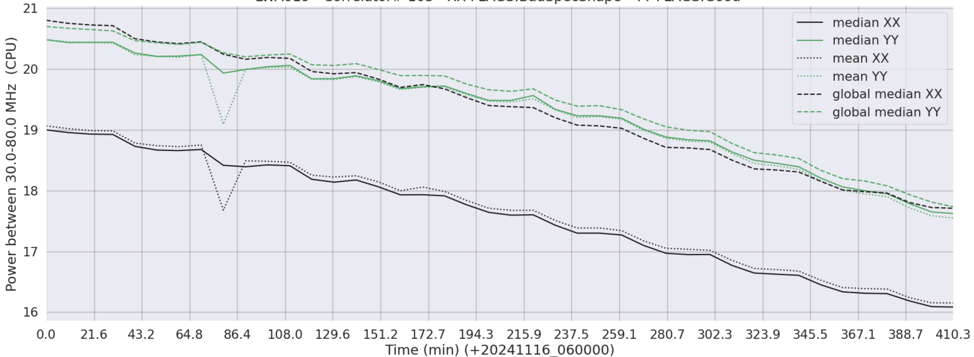
LWA019 - Correlator# 103 - XX FLAGS:BadSpecShape - YY FLAGS:Good
