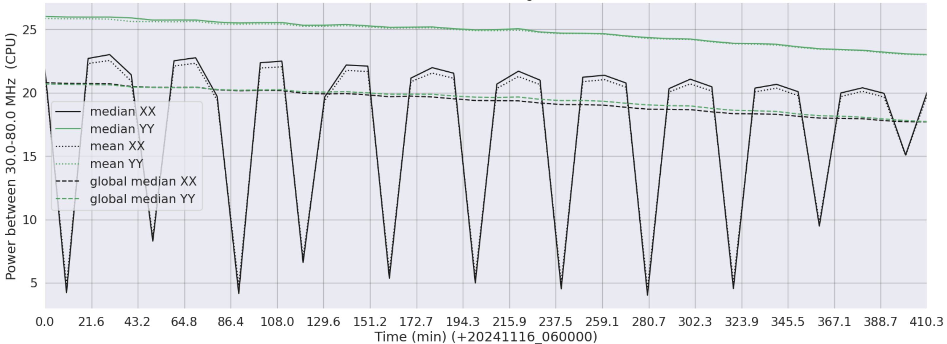
LWA065 - Correlator# 165 - XX FLAGS:HighTimeVar - YY FLAGS:Good
