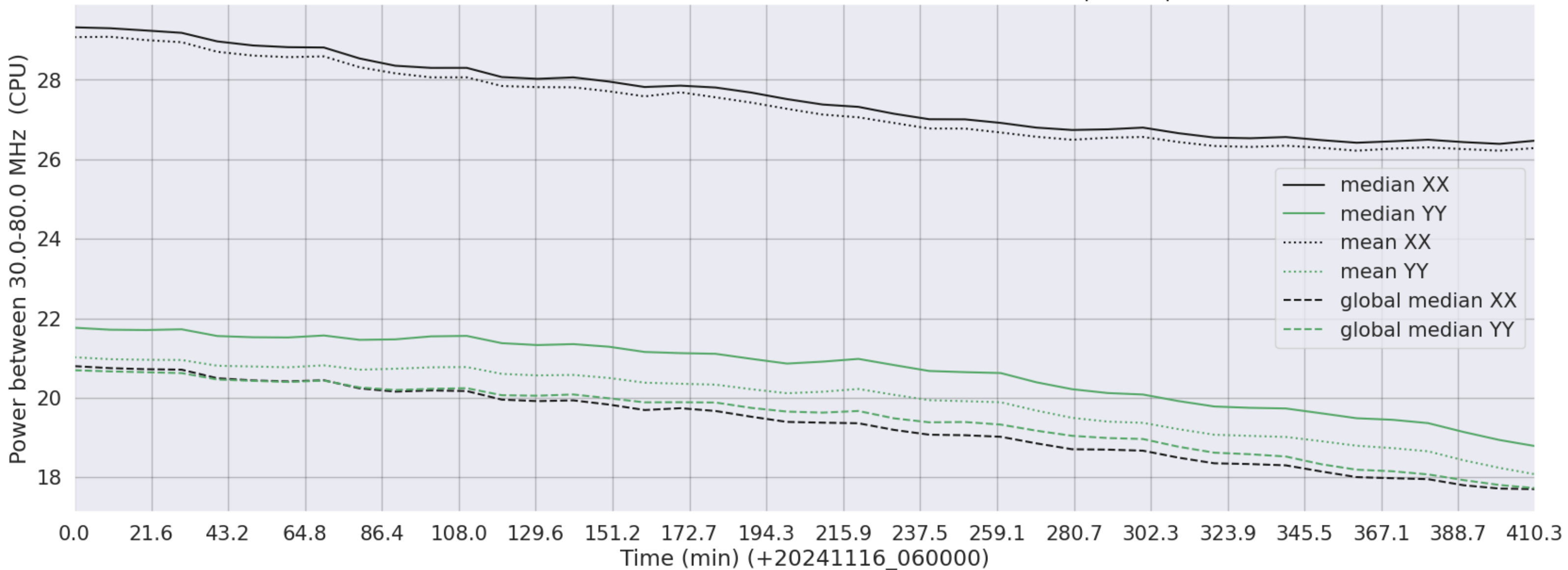
LWA308 - Correlator# 015 - XX FLAGS:Good - YY FLAGS:BadSpecShape
