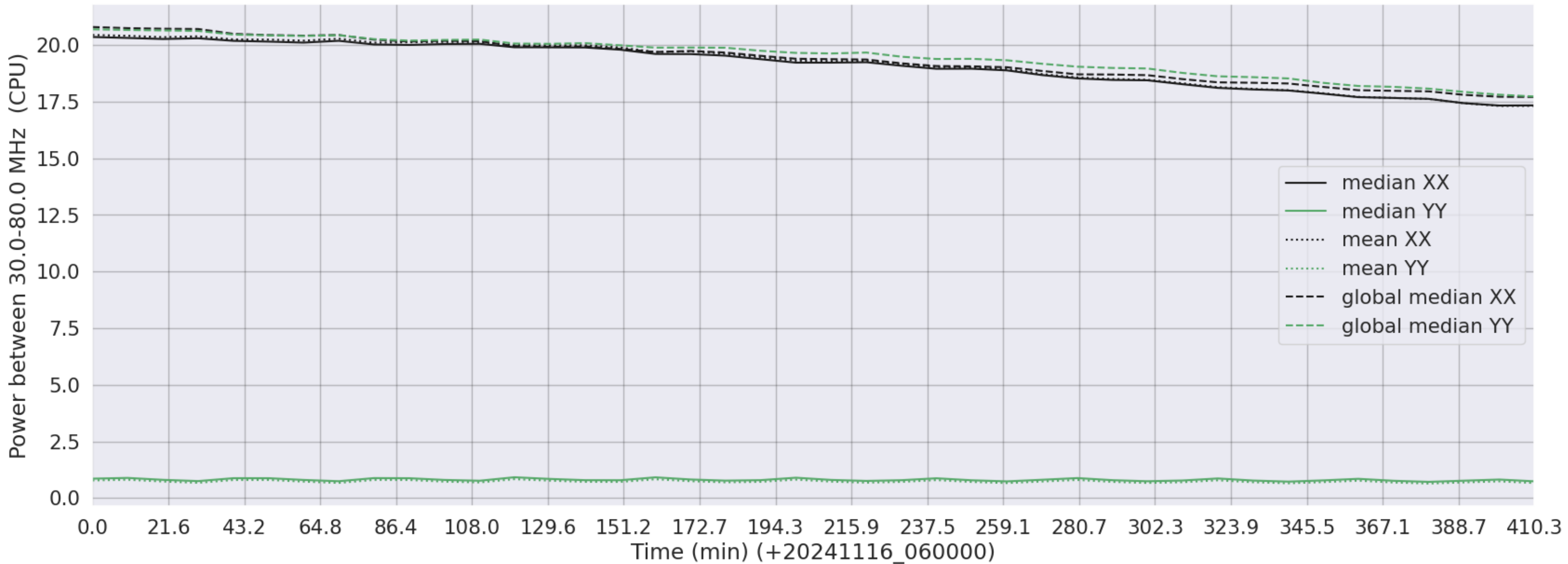
LWA292 - Correlator# 044 - XX FLAGS:Good - YY FLAGS:LowPower
