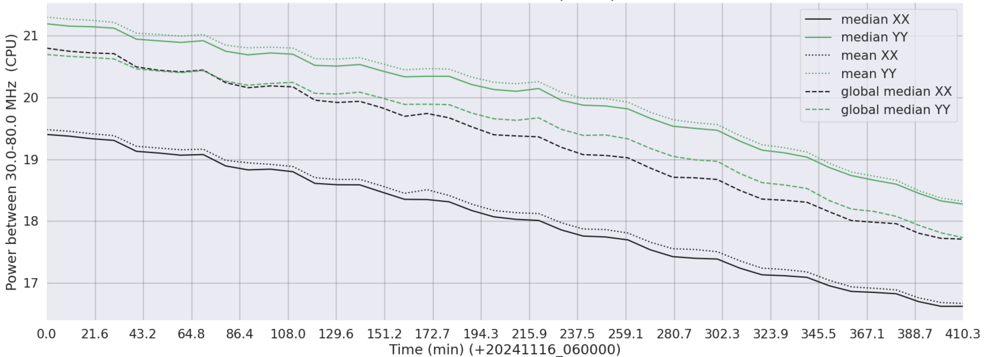
LWA101 - Correlator# 174 - XX FLAGS:BadSpecShape - YY FLAGS:Good
