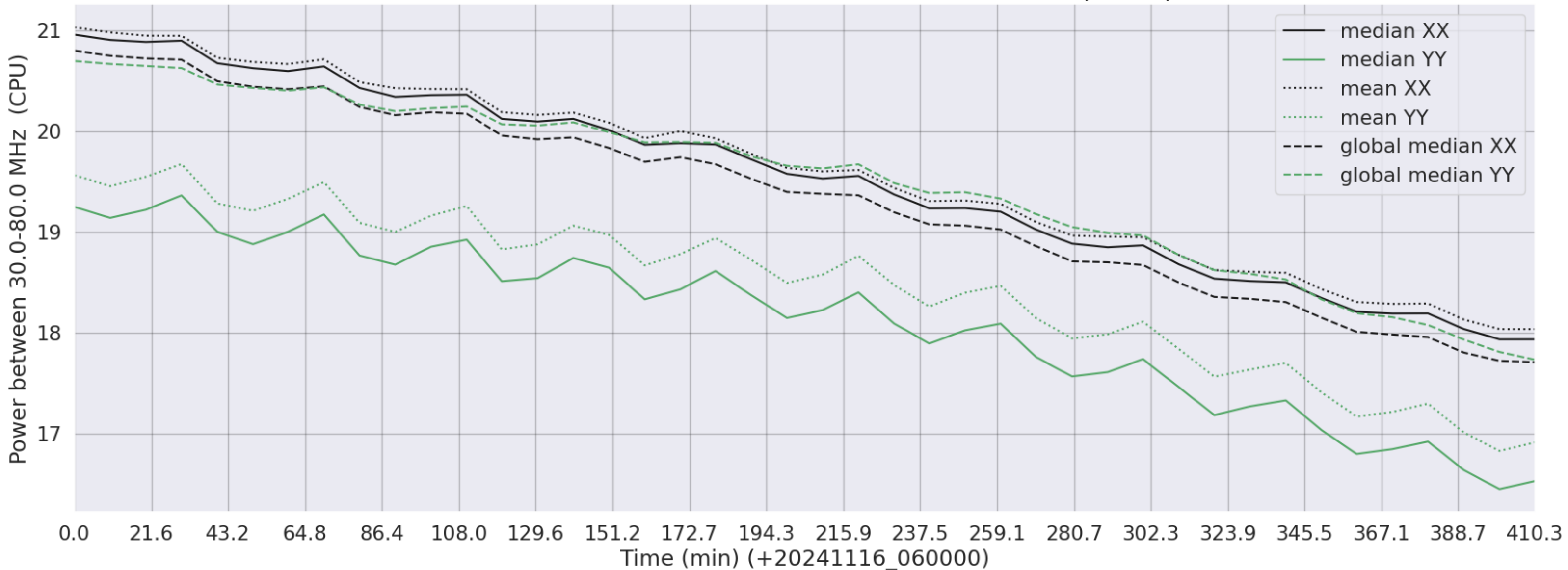
LWA235 - Correlator# 309 - XX FLAGS:Good - YY FLAGS:BadSpecShape
