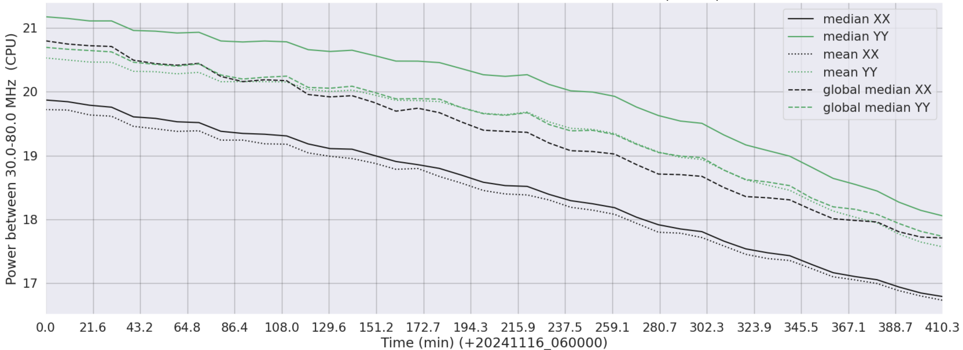
LWA273 - Correlator# 007 - XX FLAGS:Good - YY FLAGS:BadSpecShape
