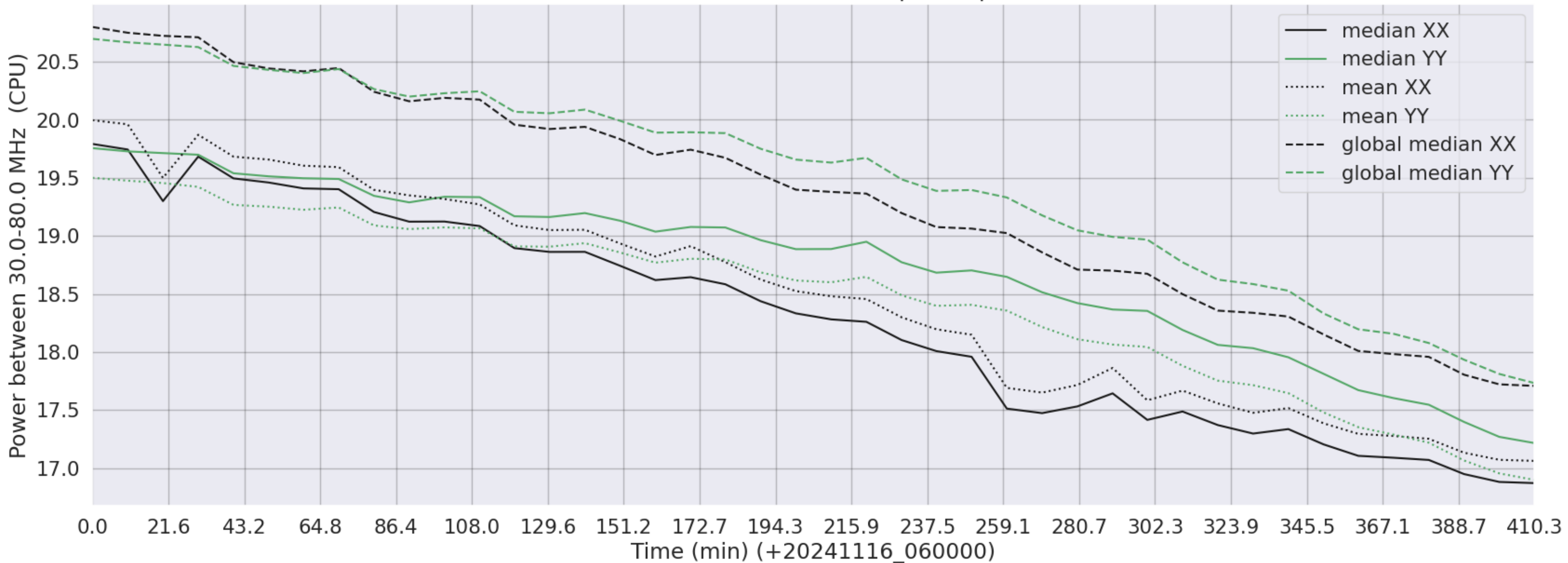
LWA071 - Correlator# 084 - XX FLAGS:BadSpecShape - YY FLAGS:Good
