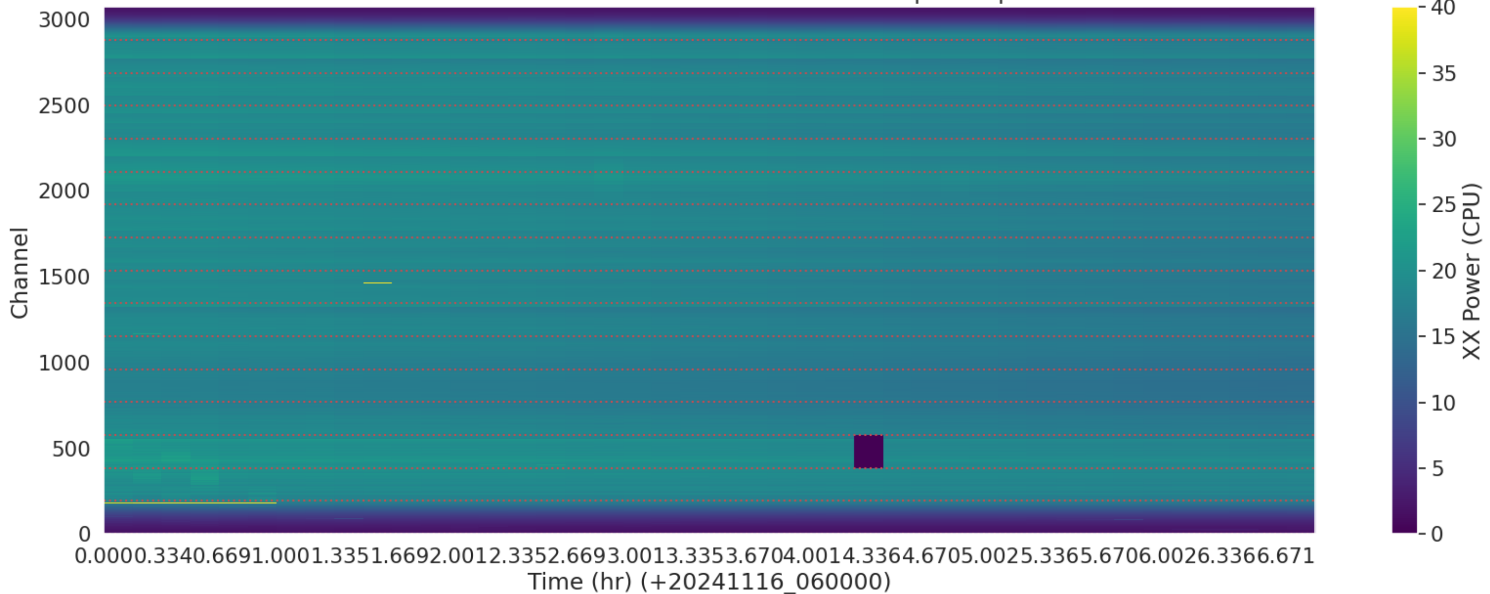
LWA169 - Correlator# 292 - XX - FLAGS: BadSpecShape
