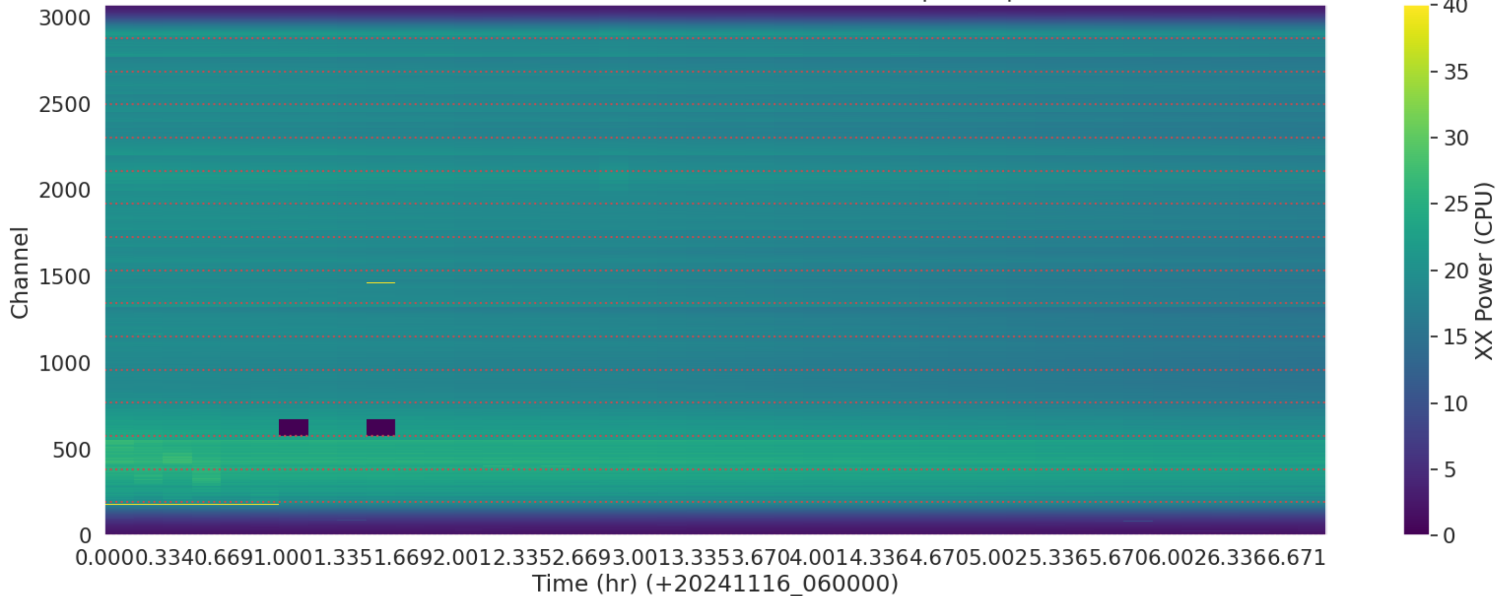
LWA101 - Correlator# 174 - XX - FLAGS: BadSpecShape
