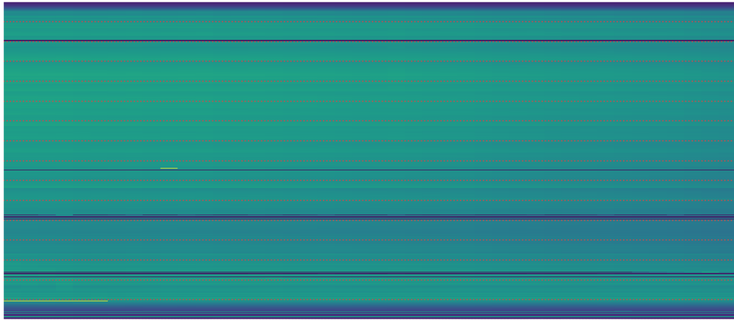
LWA308 - Correlator# 015 - YY - FLAGS: BadSpecShape
