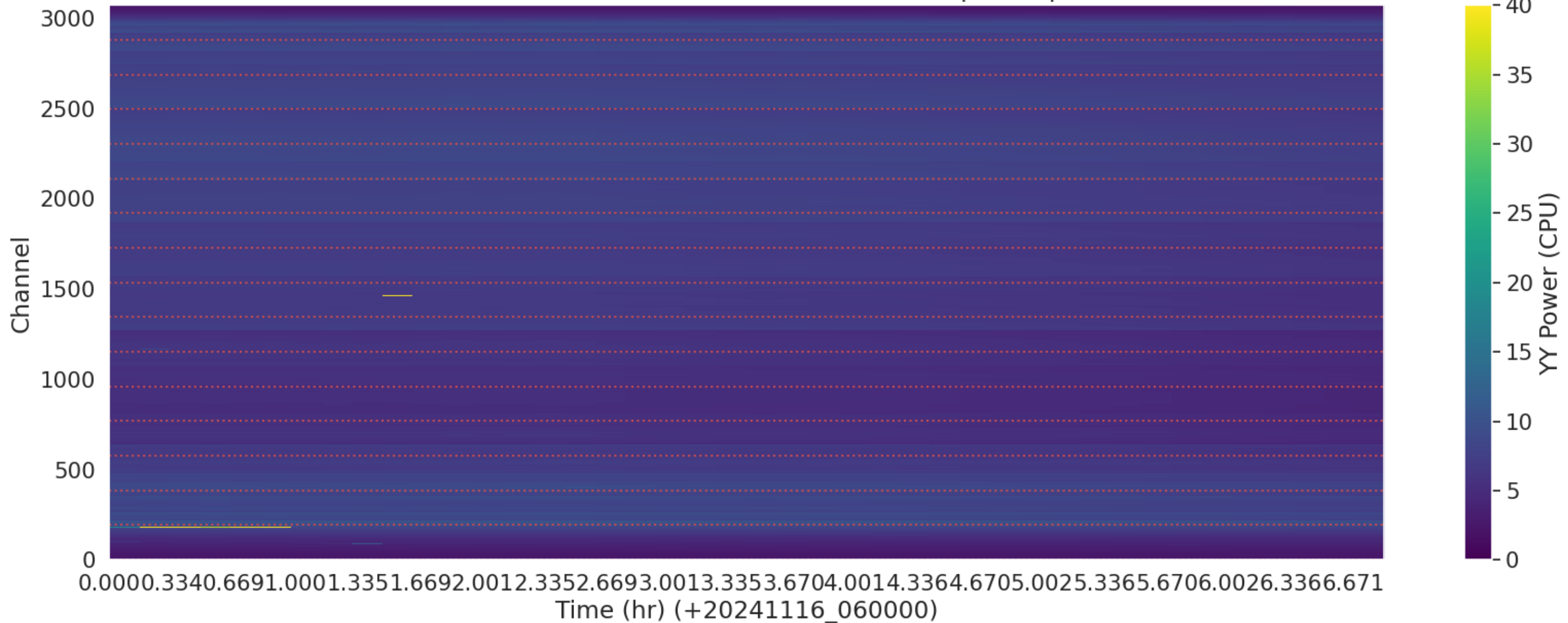
LWA303 - Correlator# 051 - YY - FLAGS: BadSpecShape
