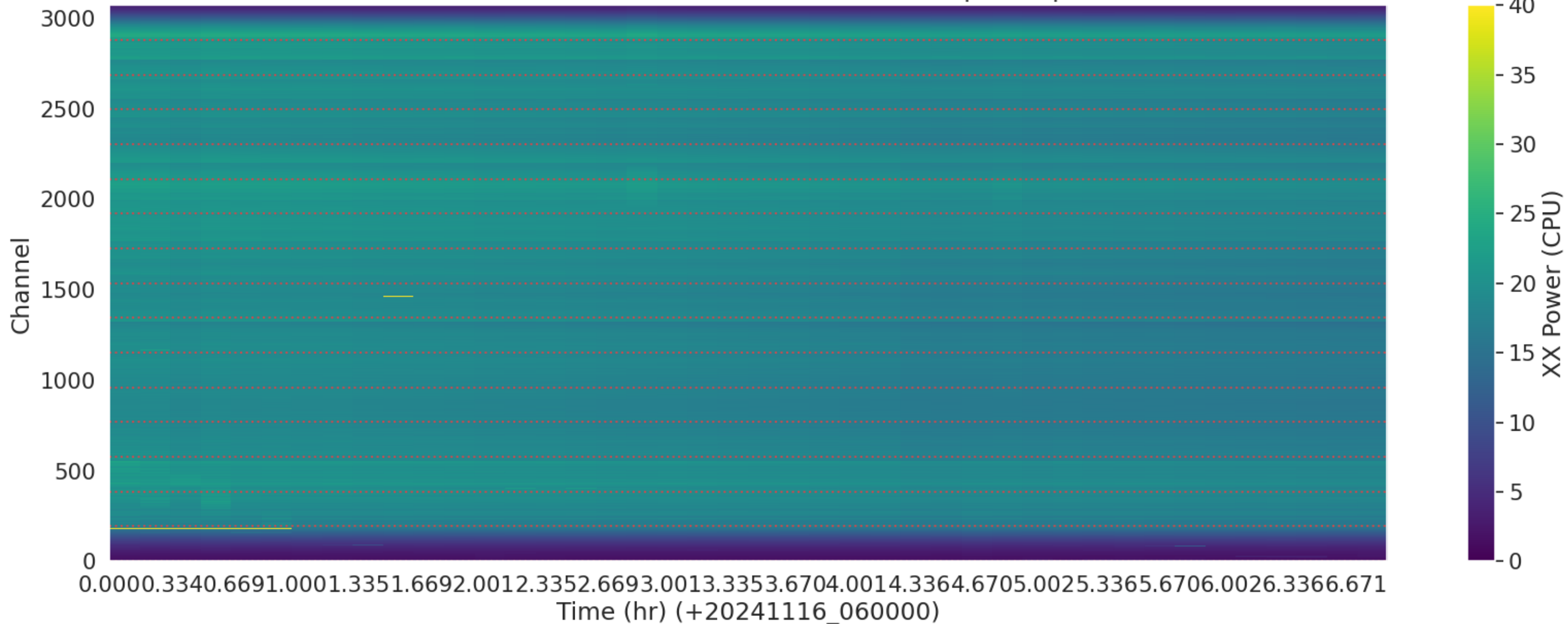
LWA071 - Correlator# 084 - XX - FLAGS: BadSpecShape
