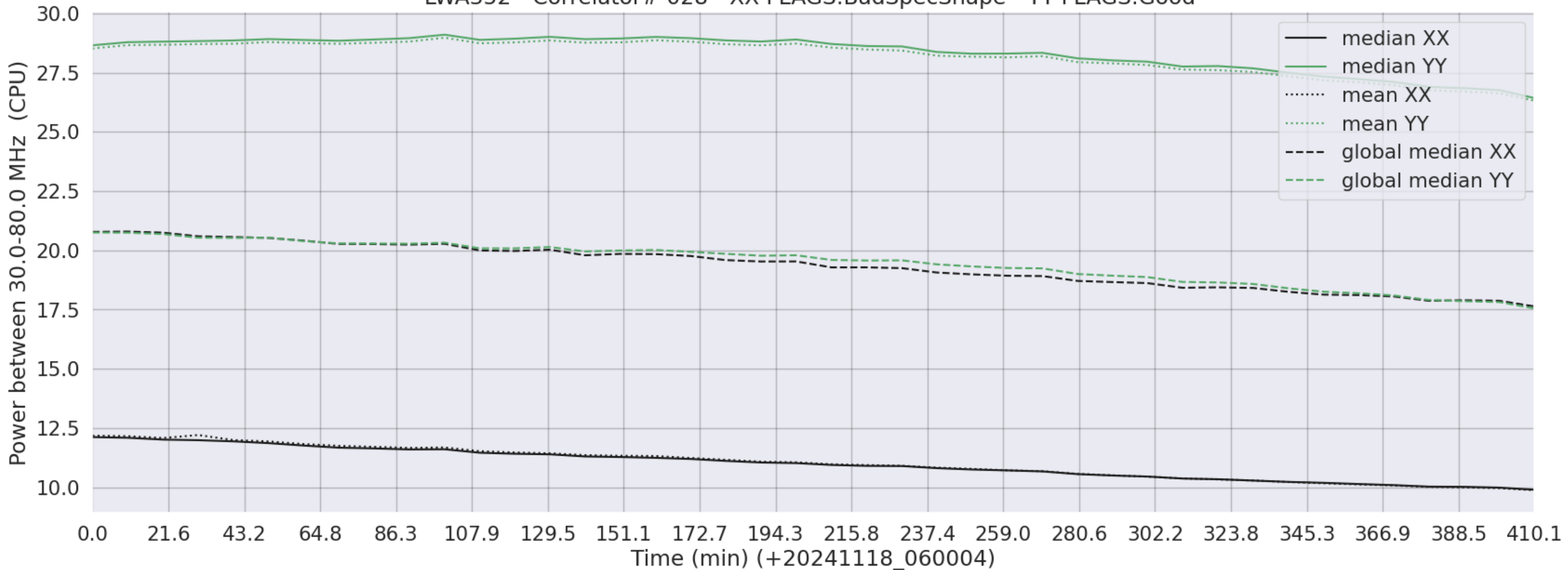
LWA352 - Correlator# 028 - XX FLAGS:BadSpecShape - YY FLAGS:Good
