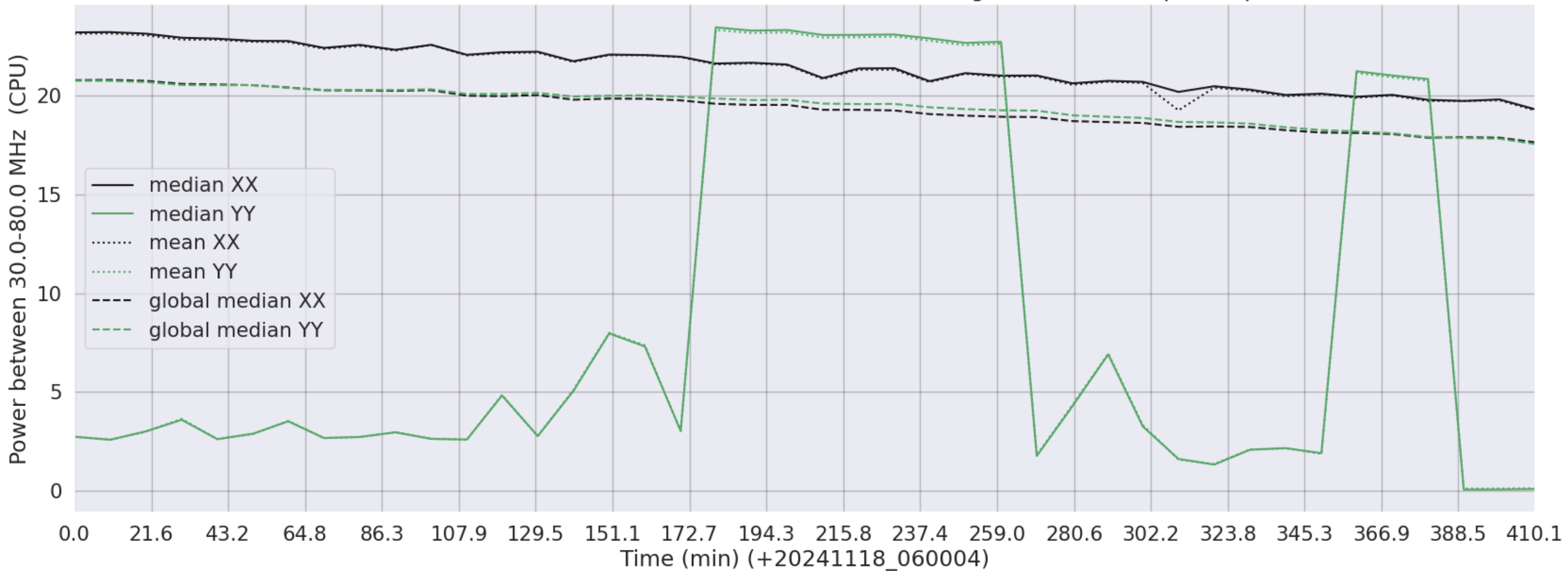
LWA124 - Correlator# 224 - XX FLAGS:Good - YY FLAGS:HighTimeVar+BadSpecShape
