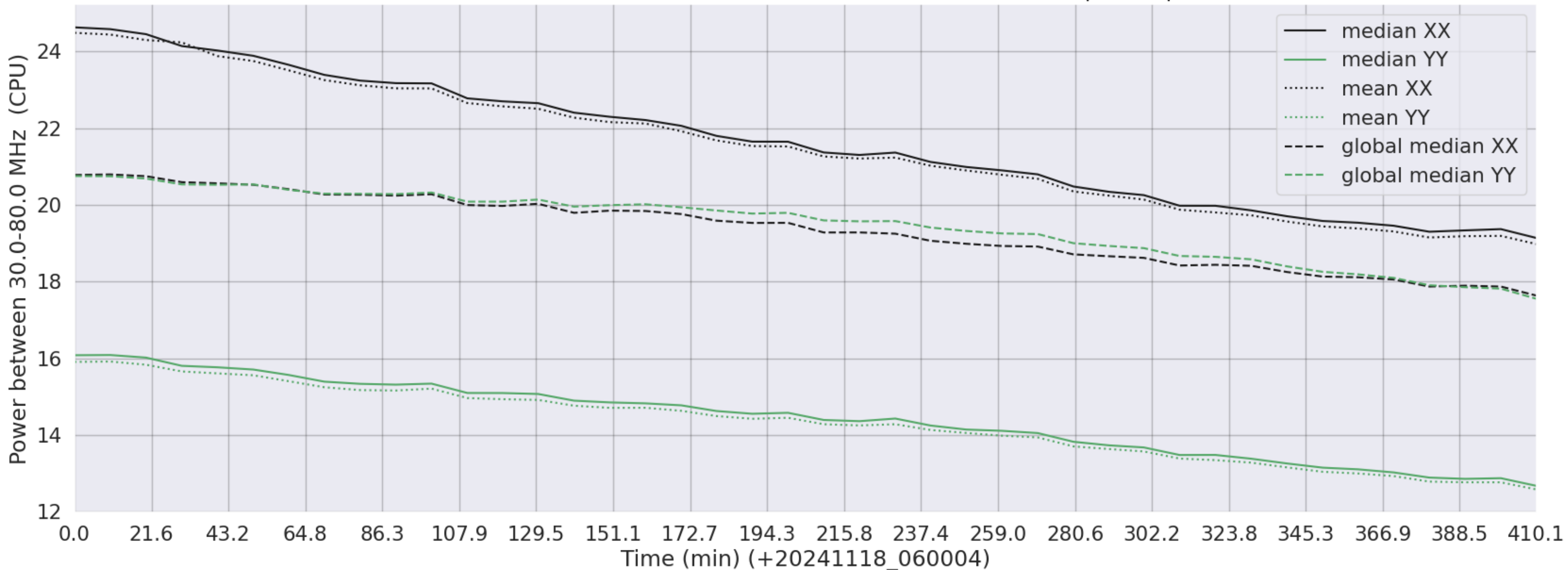
LWA295 - Correlator# 047 - XX FLAGS:Good - YY FLAGS:BadSpecShape
