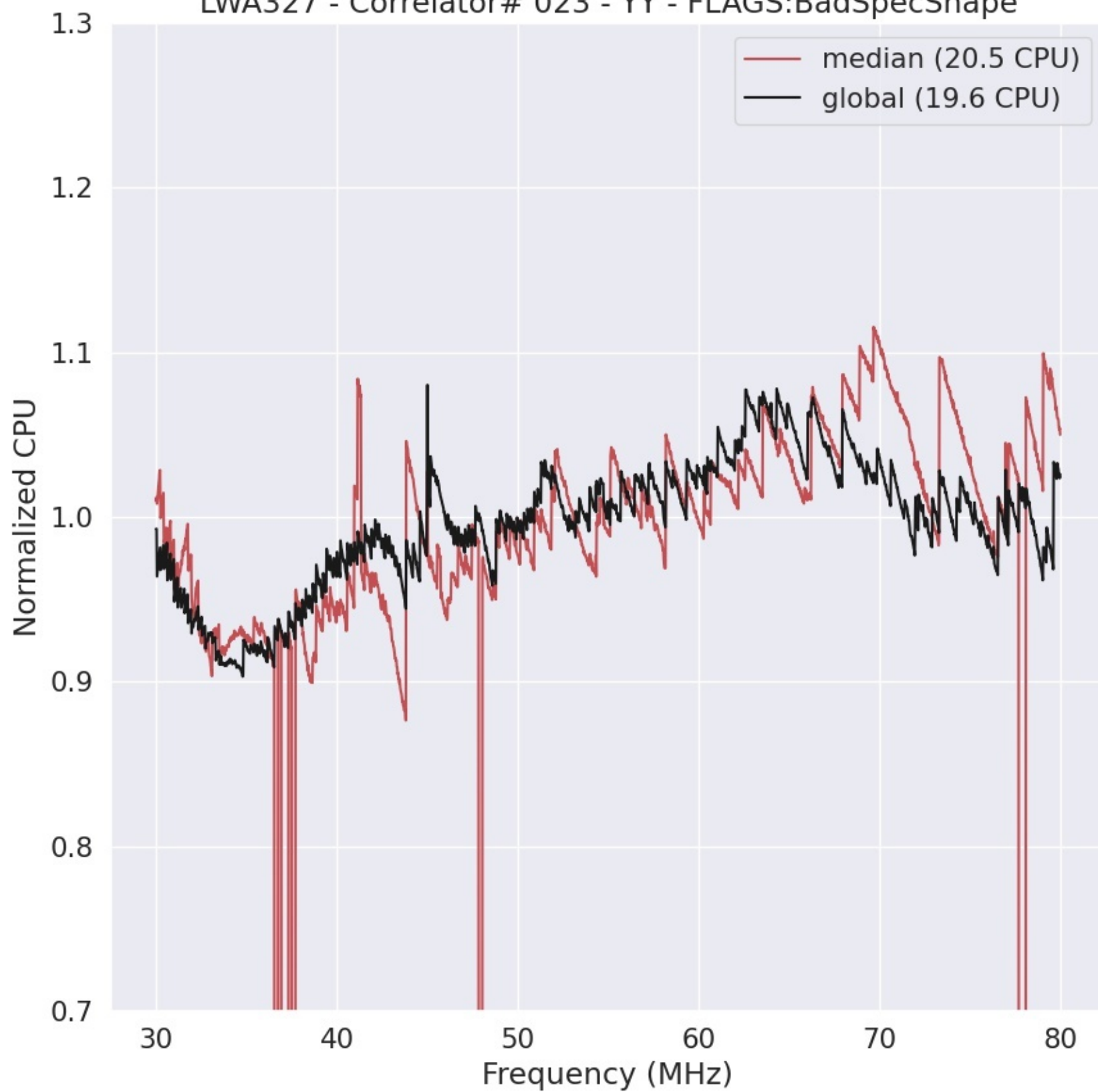
LWA327 - Correlator# 023 - YY - FLAGS:BadSpecShape
