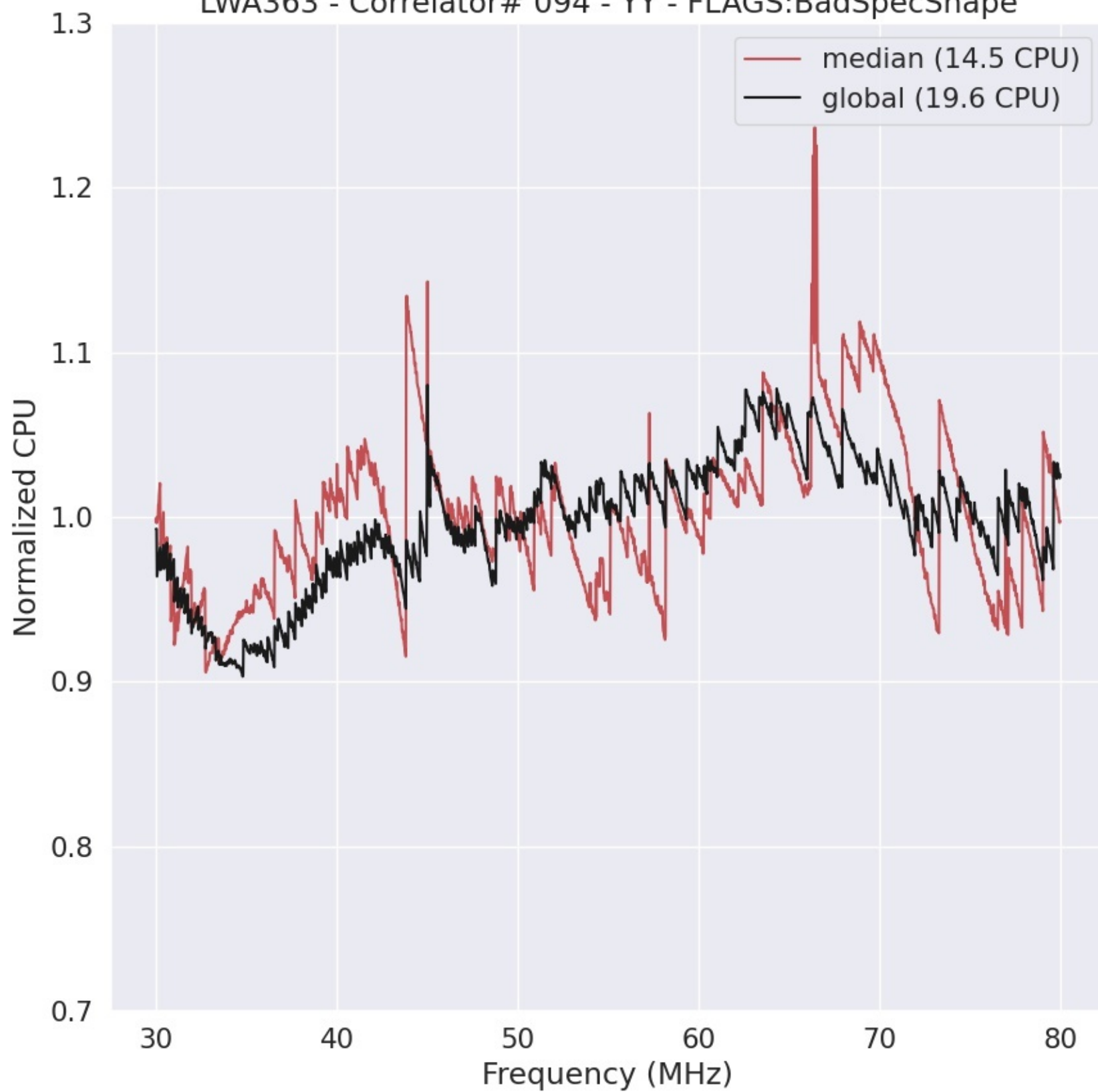
LWA363 - Correlator# 094 - YY - FLAGS:BadSpecShape
