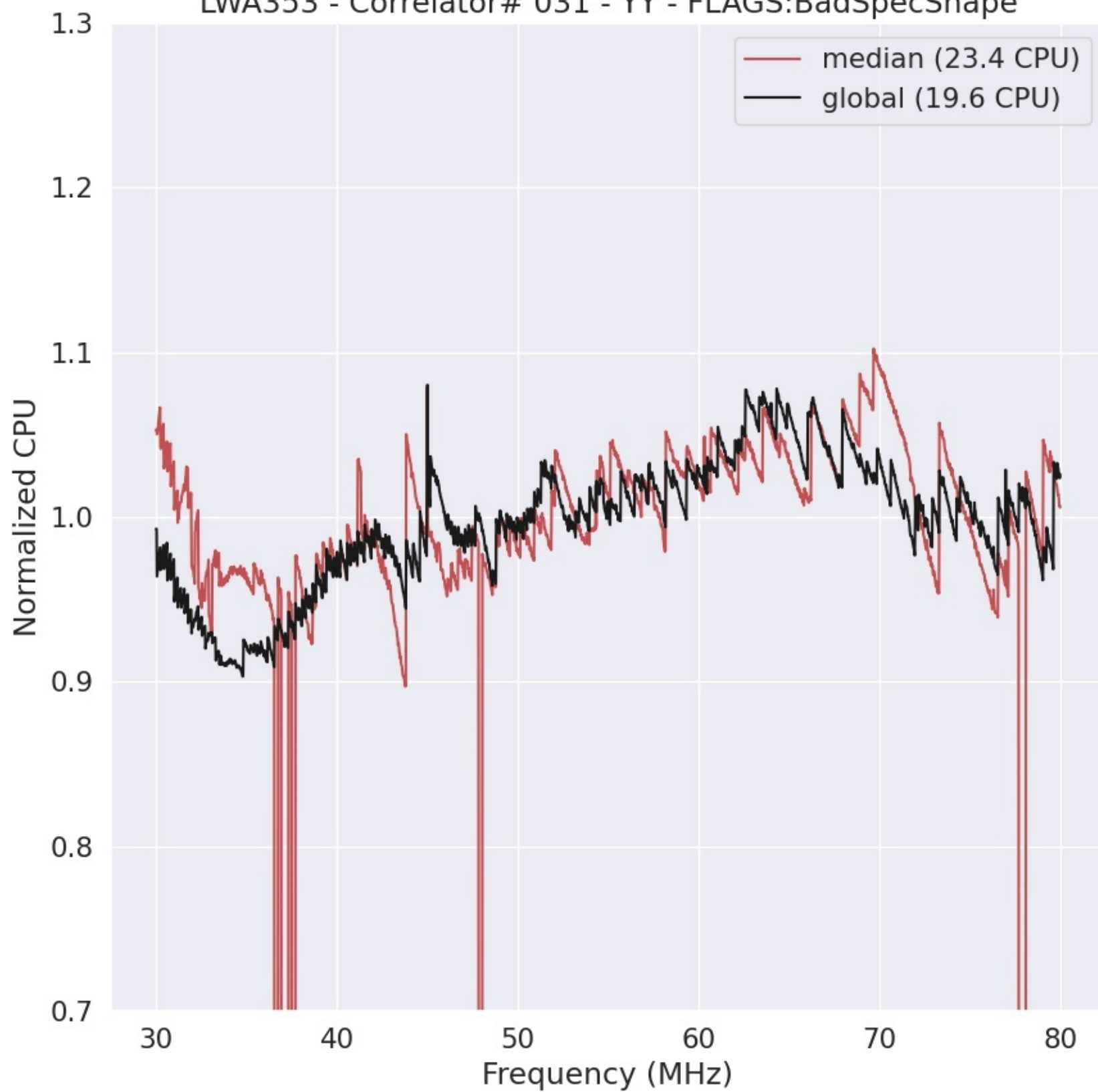
LWA353 - Correlator# 031 - YY - FLAGS:BadSpecShape
