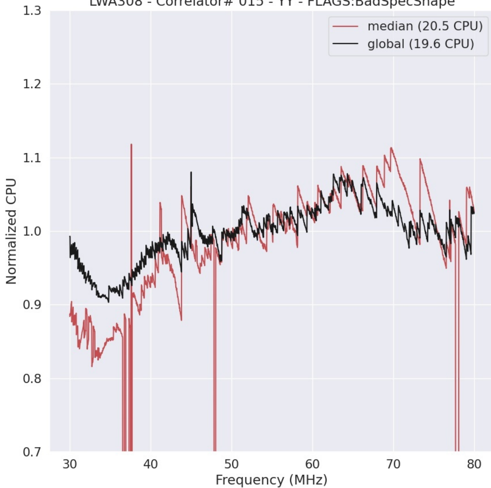
LWA308 - Correlator# 015 - YY - FLAGS:BadSpecShape
