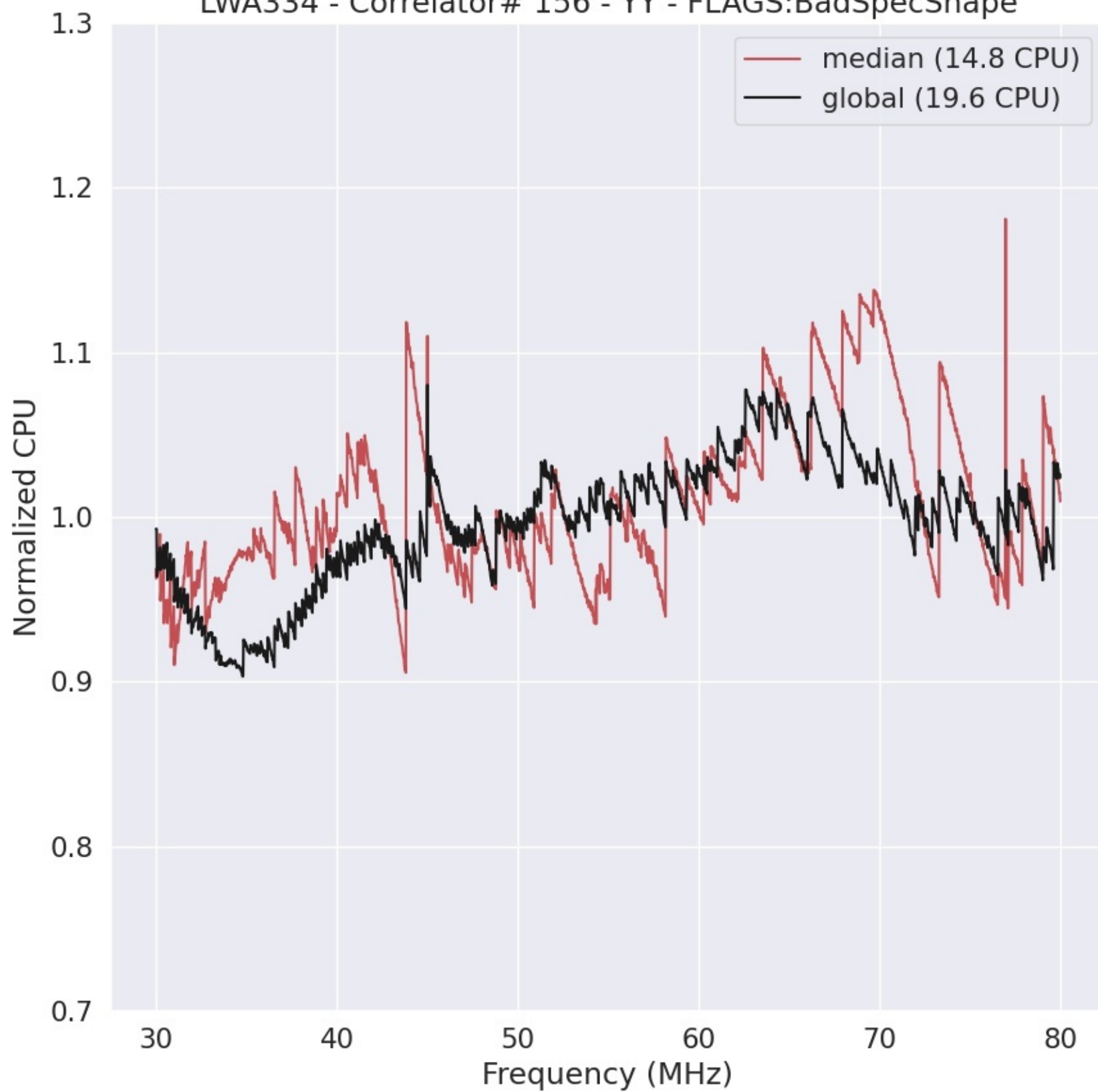
LWA334 - Correlator# 156 - YY - FLAGS:BadSpecShape
