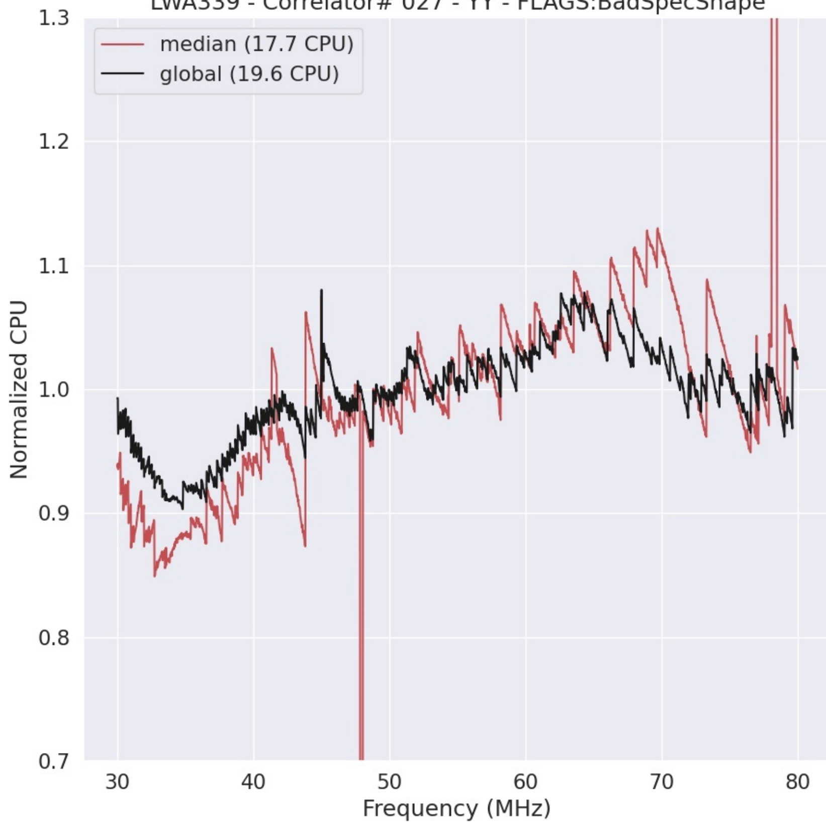
LWA339 - Correlator# 027 - YY - FLAGS:BadSpecShape
