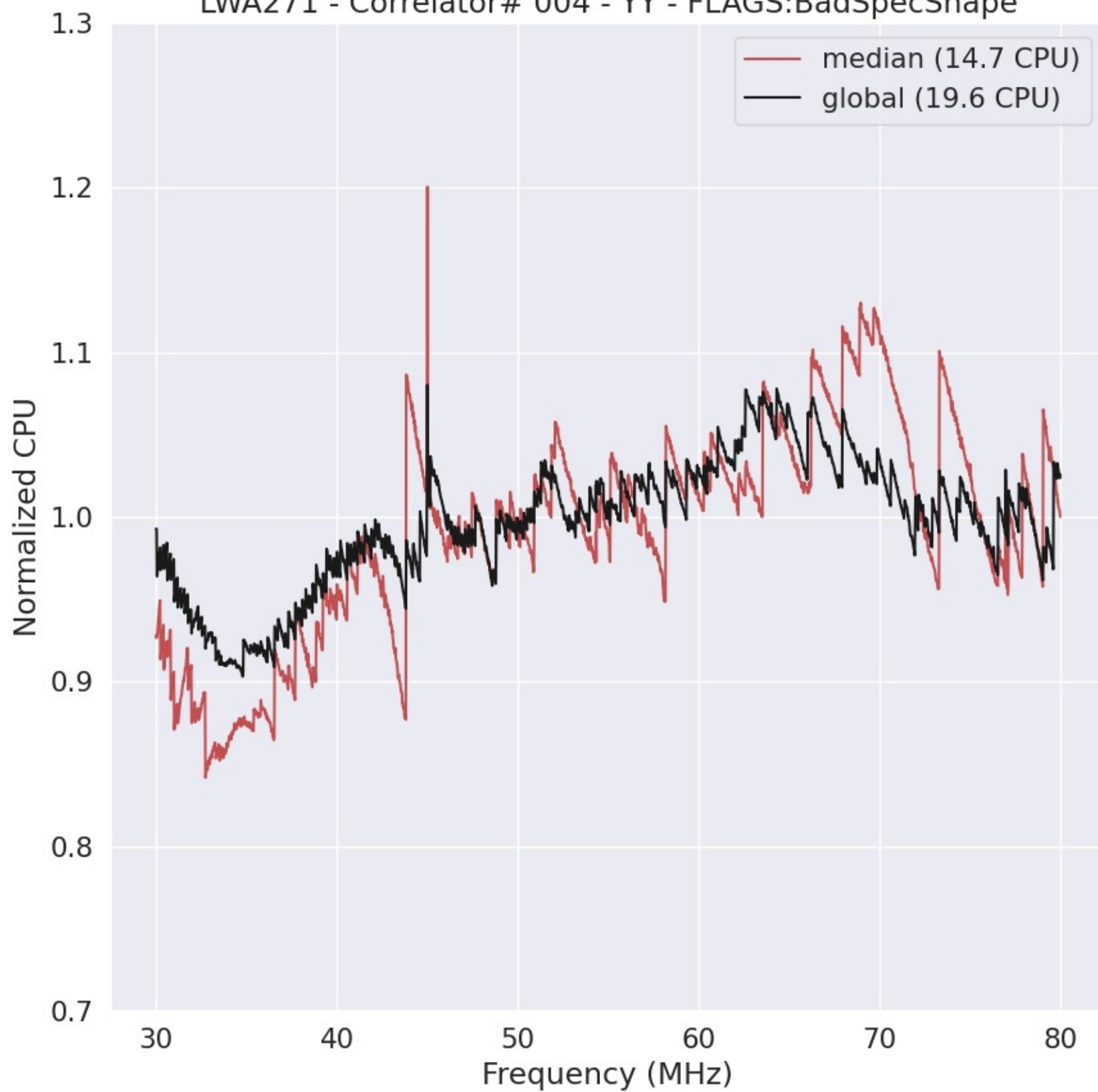
LWA271 - Correlator# 004 - YY - FLAGS:BadSpecShape
