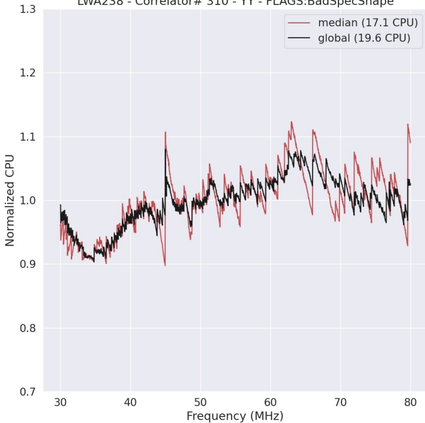
LWA238 - Correlator# 310 - YY - FLAGS:BadSpecShape
