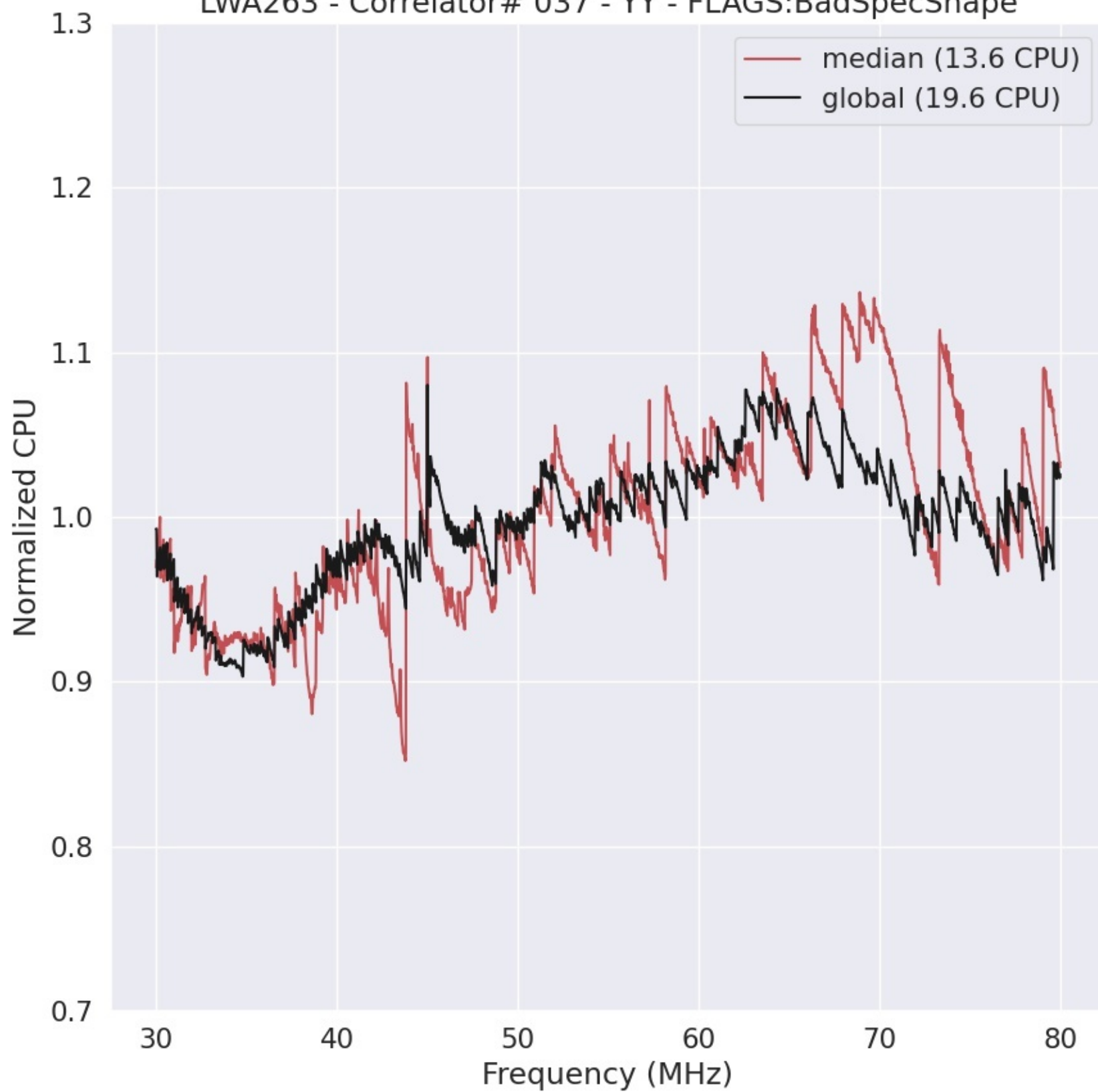
LWA263 - Correlator# 037 - YY - FLAGS:BadSpecShape
