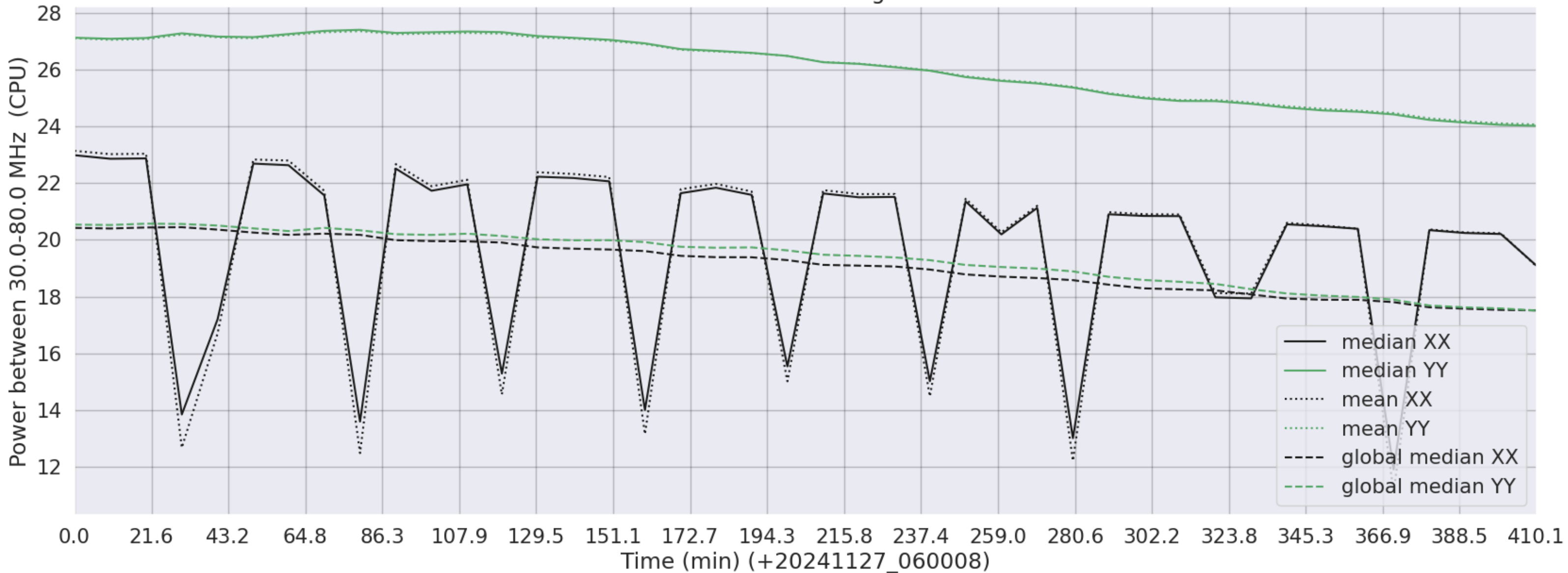
LWA316 - Correlator# 155 - XX FLAGS:HighTimeVar - YY FLAGS:Good
