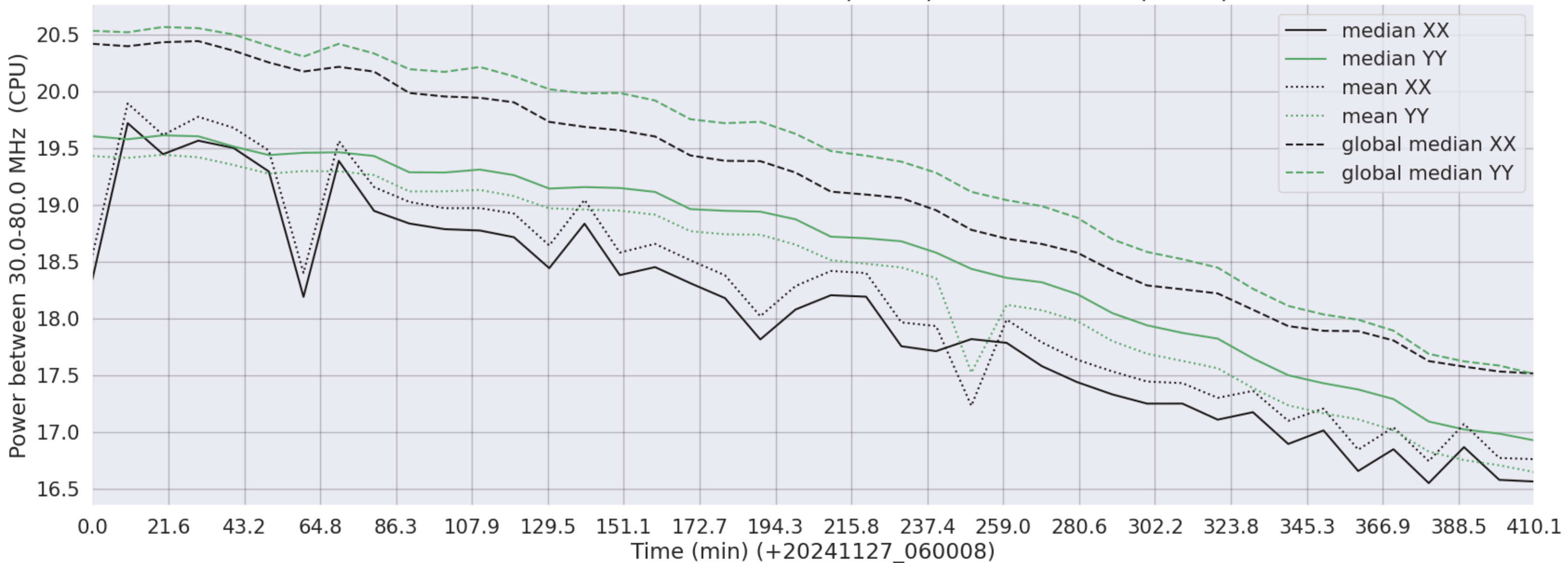
LWA071 - Correlator# 084 - XX FLAGS:BadSpecShape - YY FLAGS:BadSpecShape
