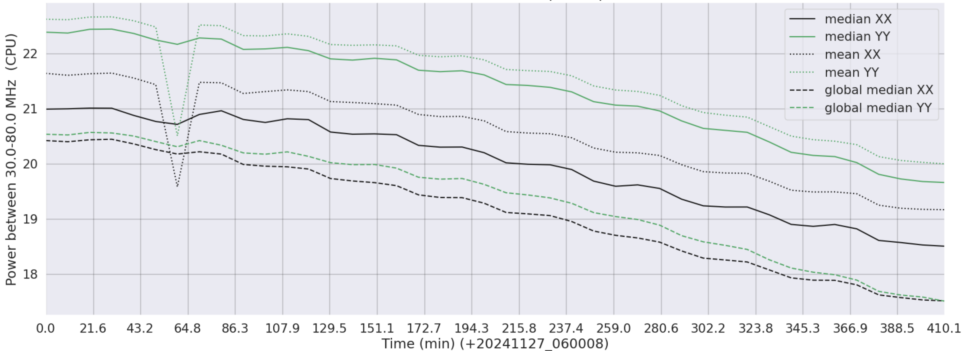
LWA194 - Correlator# 273 - XX FLAGS:BadSpecShape - YY FLAGS:Good
