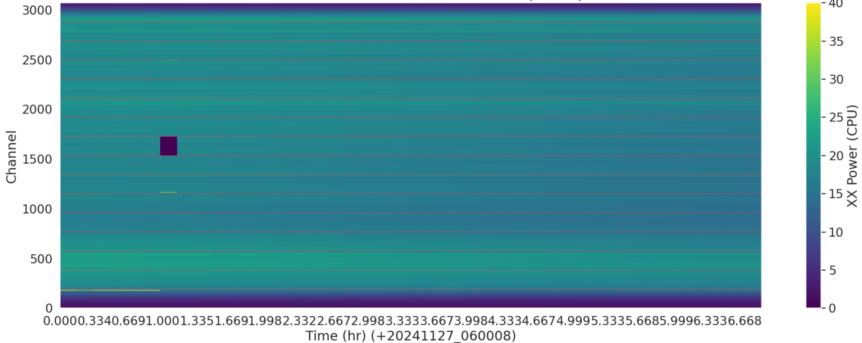
LWA170 - Correlator# 288 - XX - FLAGS: BadSpecShape
