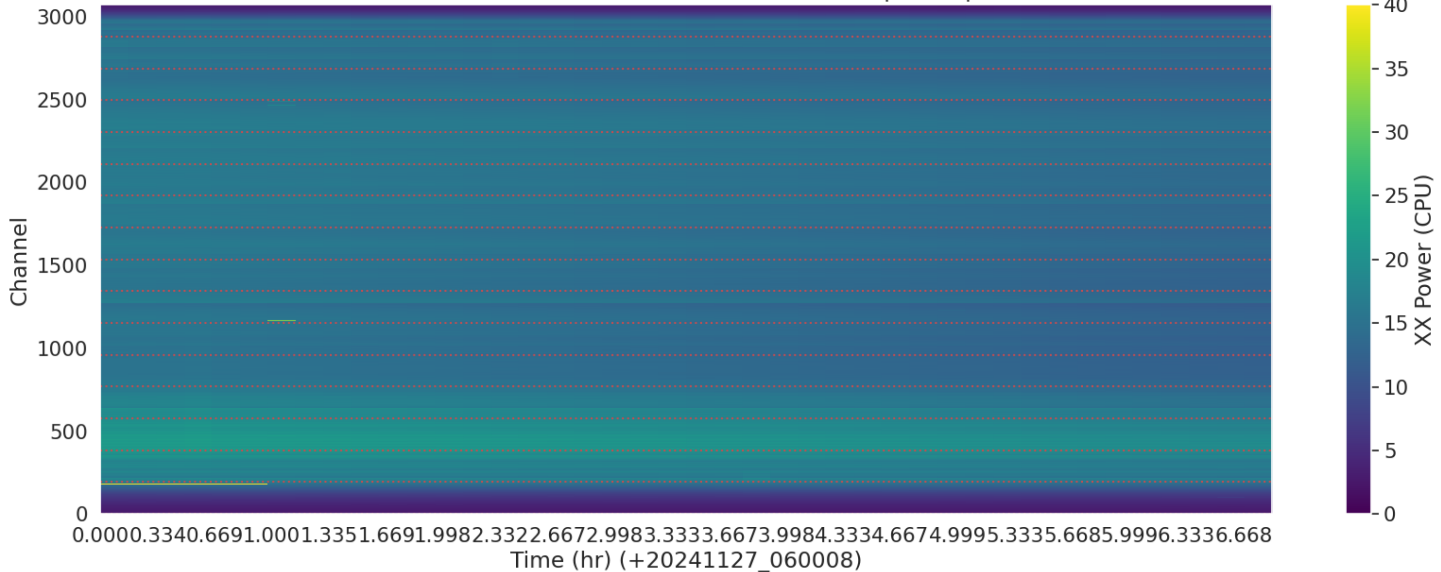
LWA291 - Correlator# 045 - XX - FLAGS: BadSpecShape
