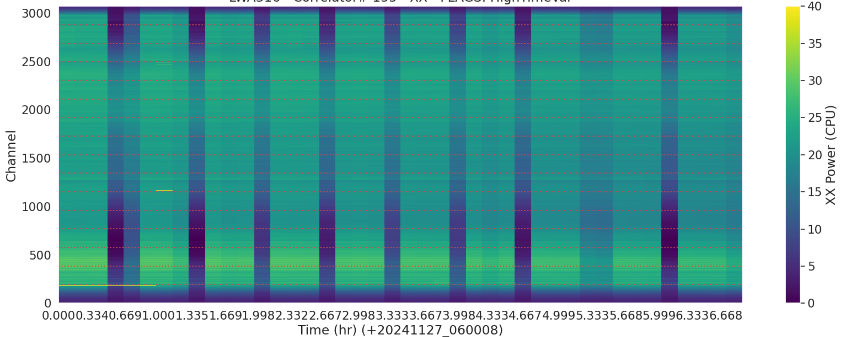
LWA316 - Correlator# 155 - XX - FLAGS: HighTimeVar
