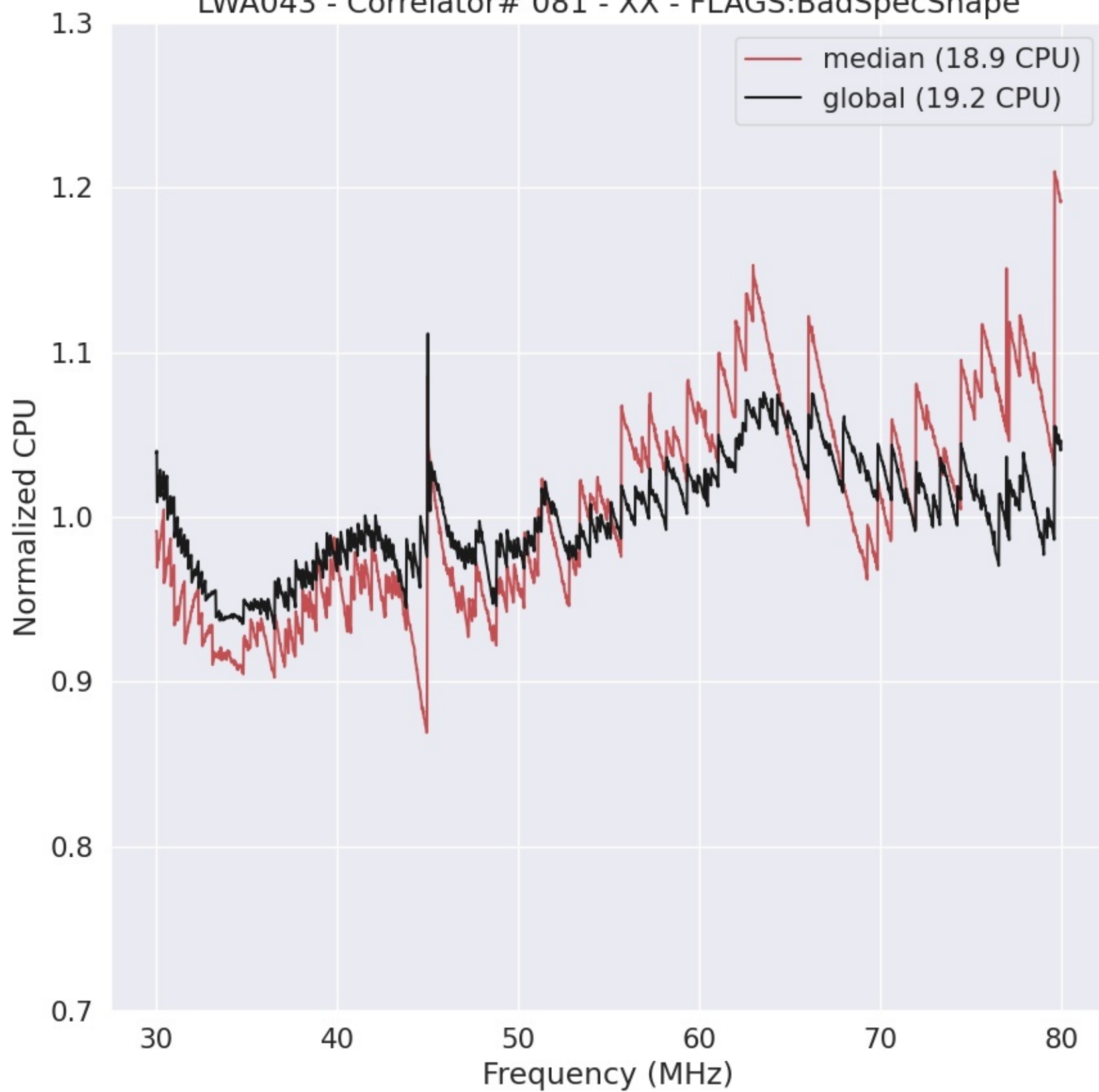
LWA043 - Correlator# 081 - XX - FLAGS:BadSpecShape
