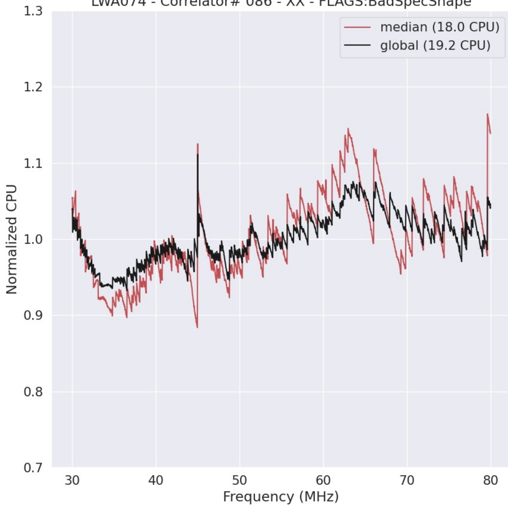
LWA074 - Correlator# 086 - XX - FLAGS:BadSpecShape
