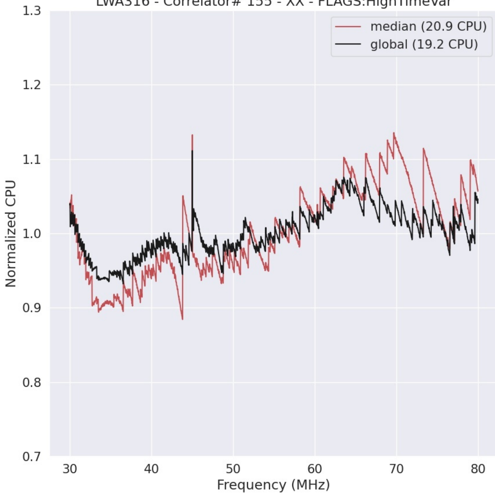
LWA316 - Correlator# 155 - XX - FLAGS:HighTimeVar
