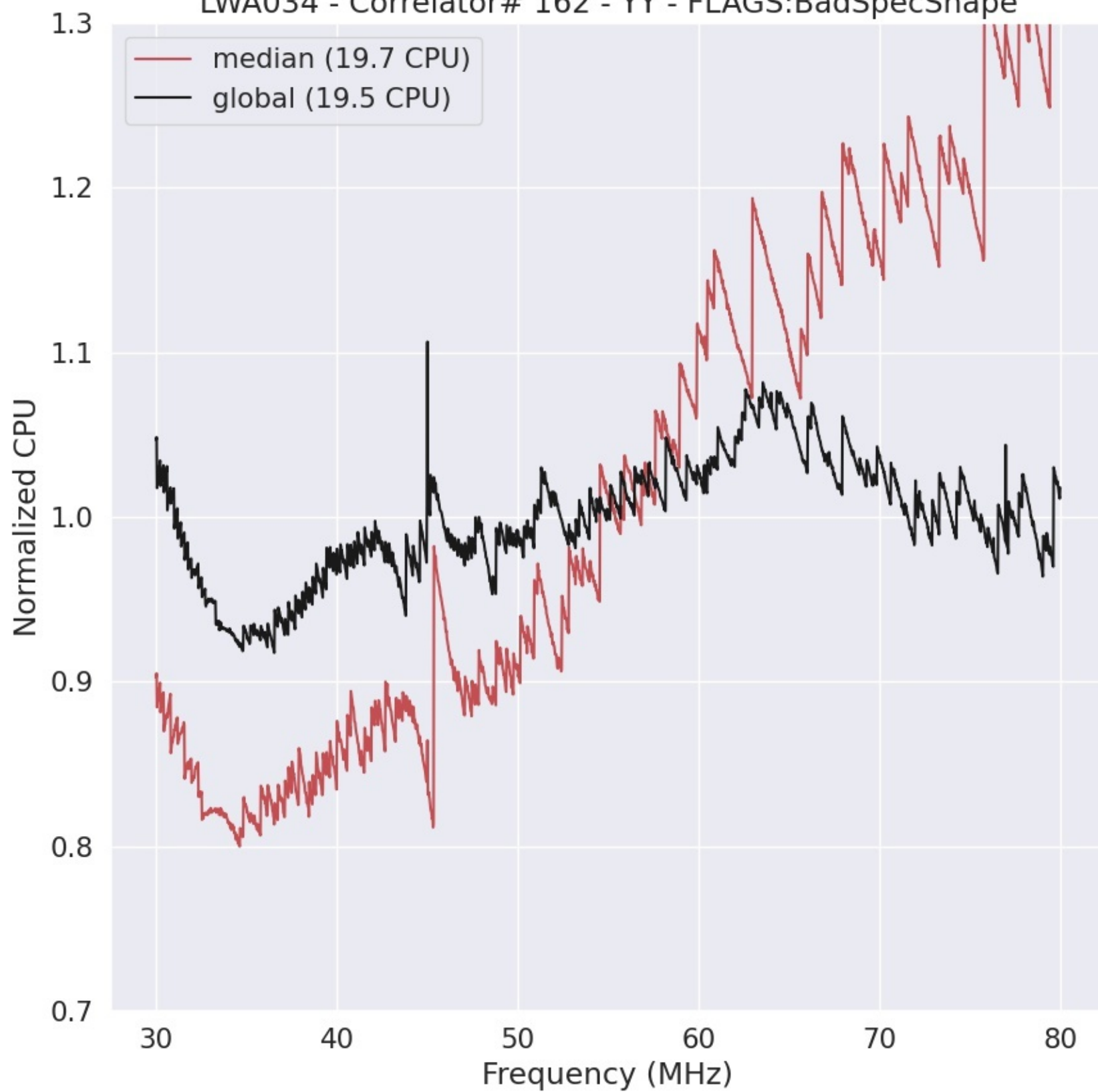
LWA034 - Correlator# 162 - YY - FLAGS:BadSpecShape
