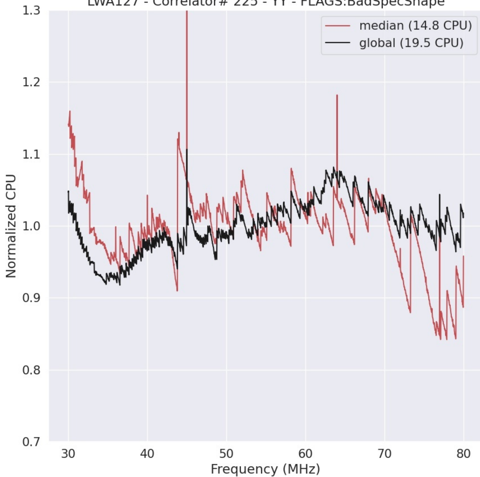
LWA127 - Correlator# 225 - YY - FLAGS:BadSpecShape
