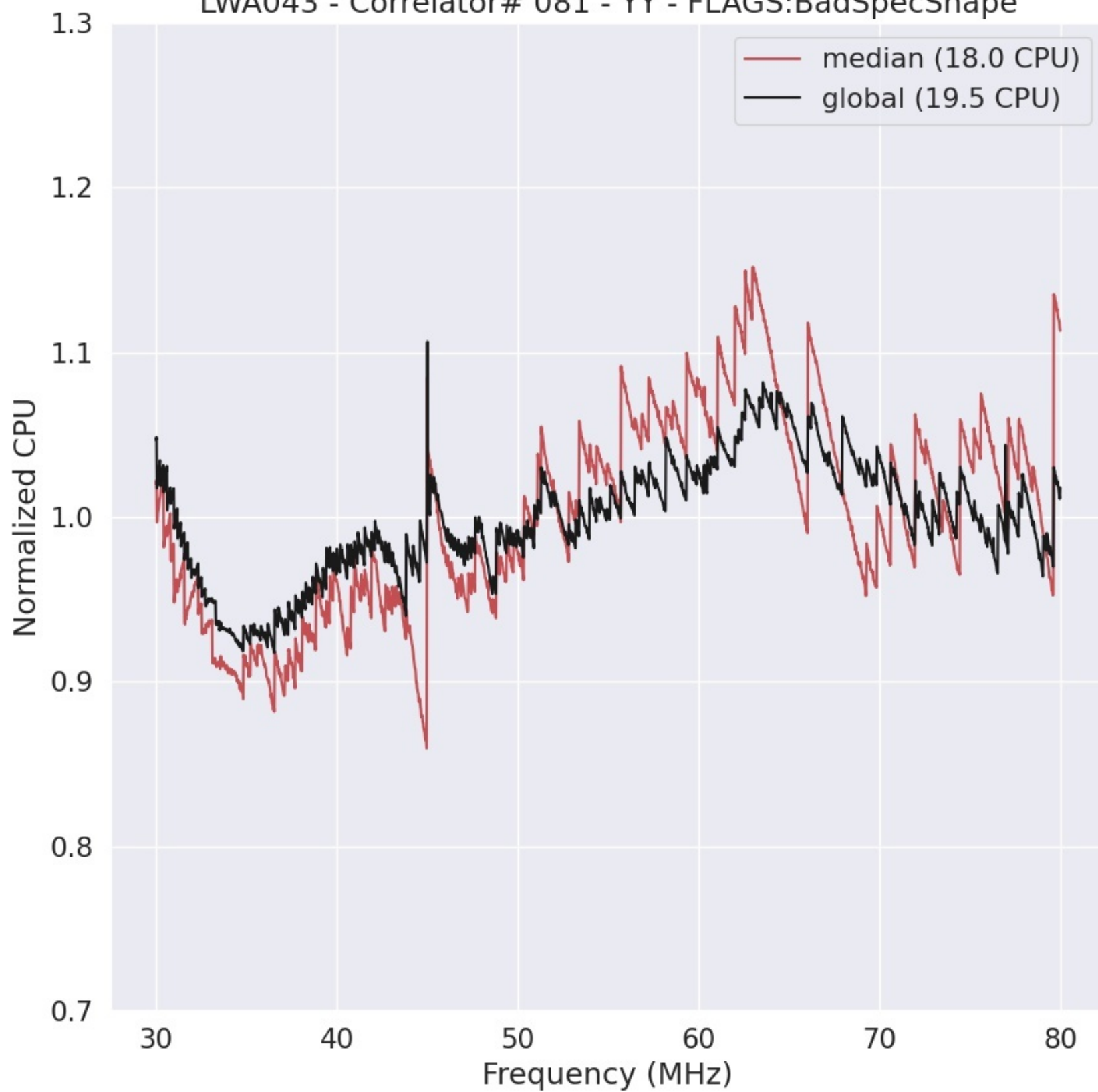
LWA043 - Correlator# 081 - YY - FLAGS:BadSpecShape
