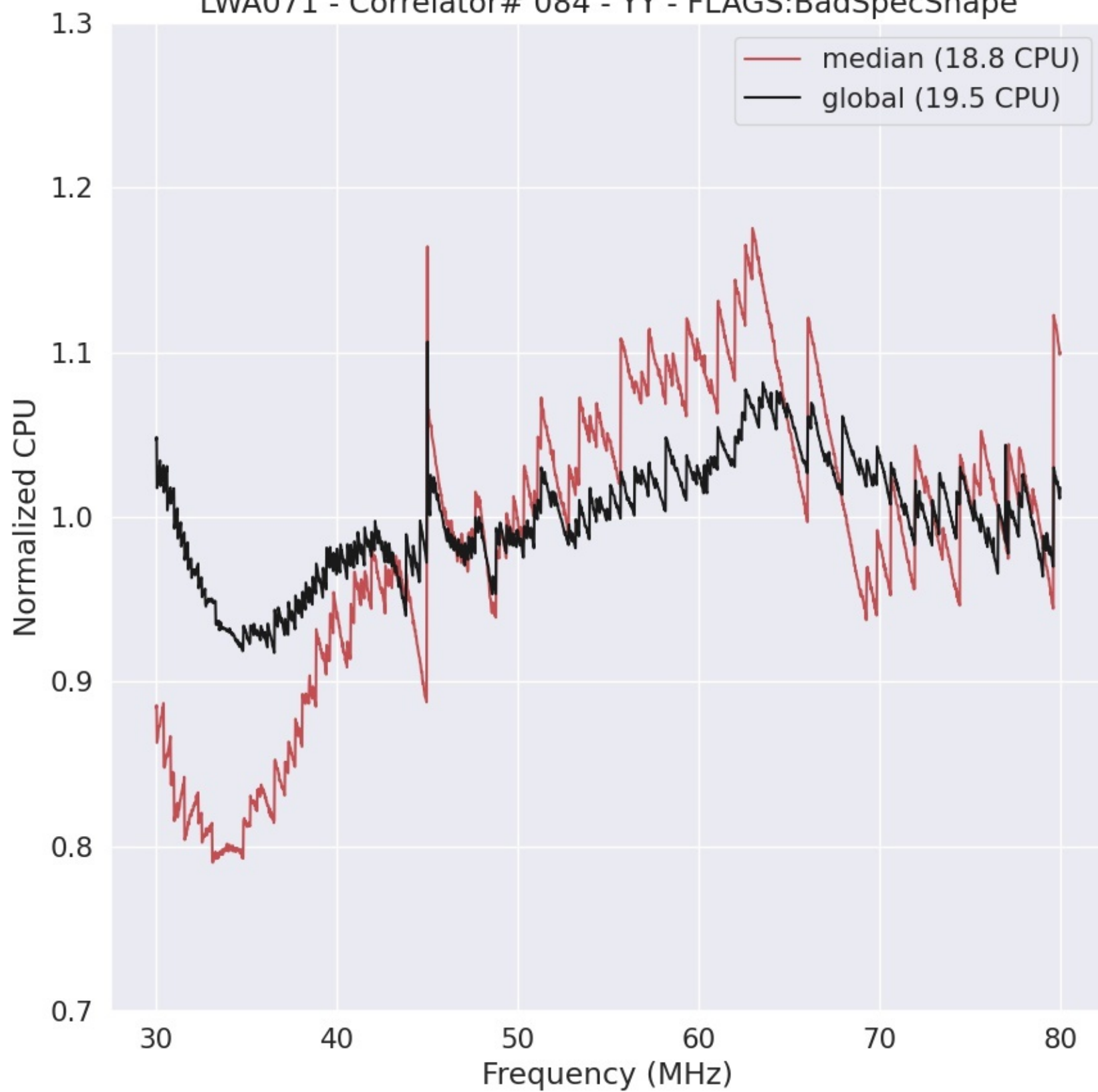
LWA071 - Correlator# 084 - YY - FLAGS:BadSpecShape
