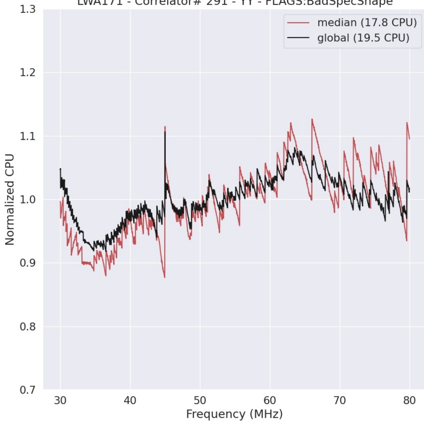
LWA171 - Correlator# 291 - YY - FLAGS:BadSpecShape
