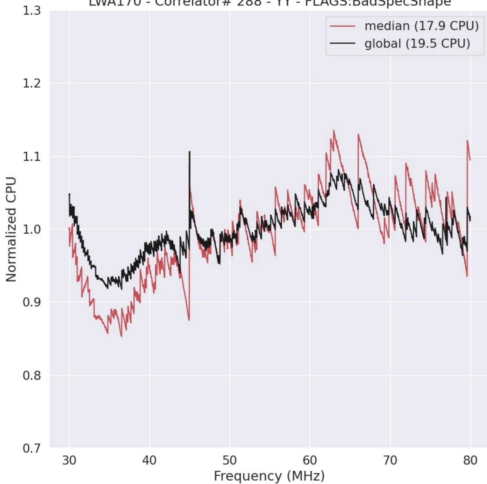
LWA170 - Correlator# 288 - YY - FLAGS:BadSpecShape
