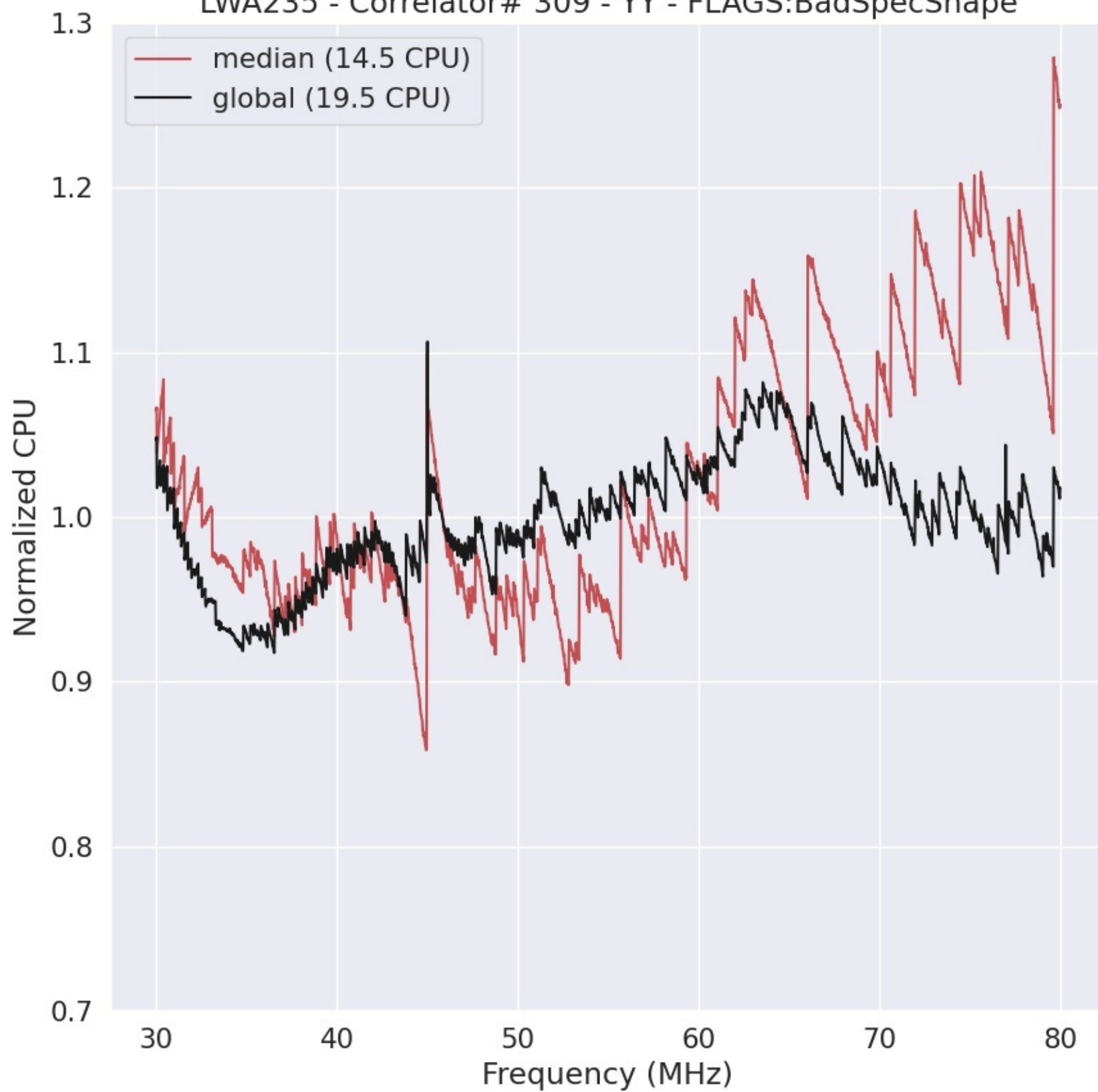
LWA235 - Correlator# 309 - YY - FLAGS:BadSpecShape
