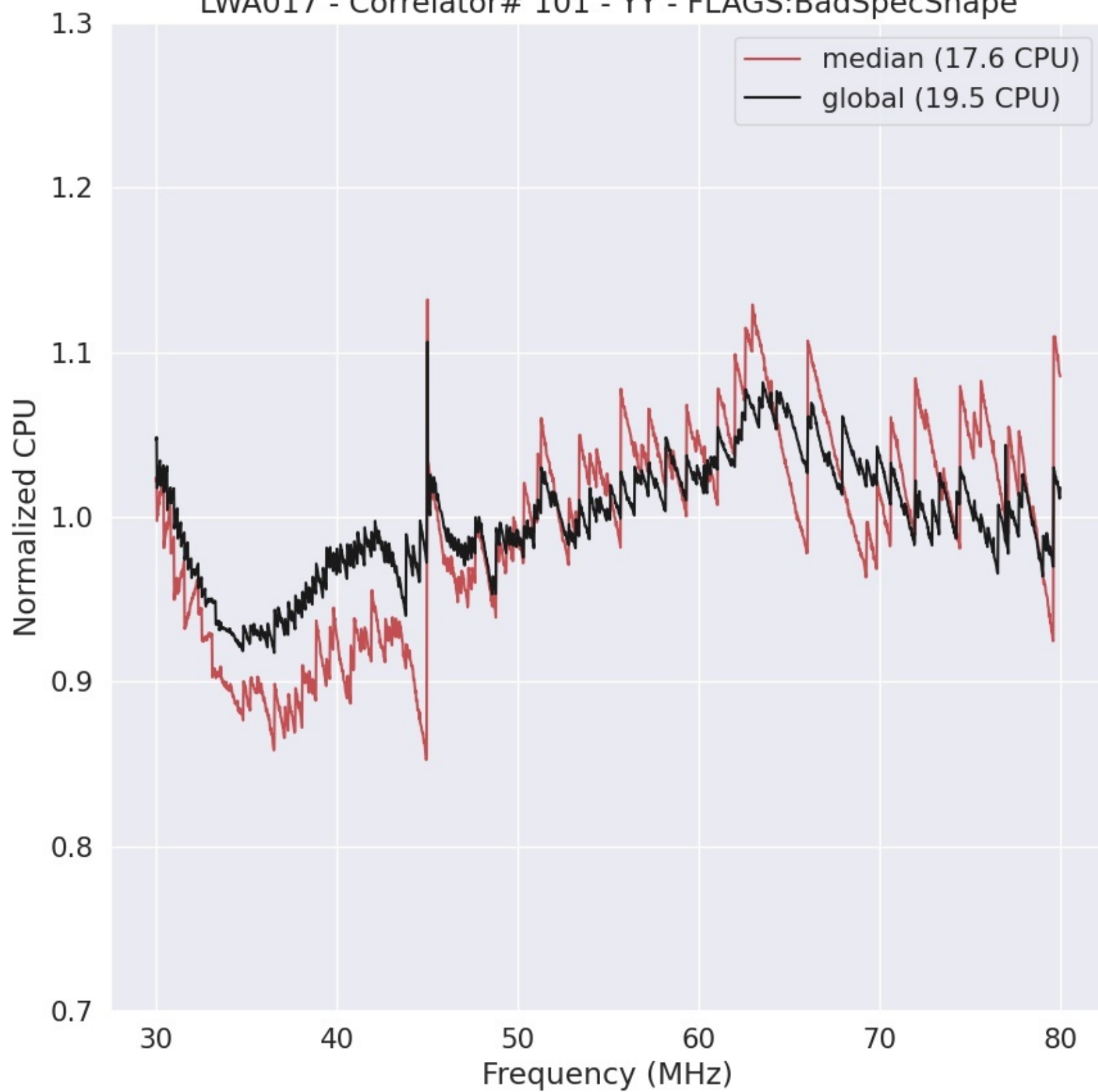
LWA017 - Correlator# 101 - YY - FLAGS:BadSpecShape
