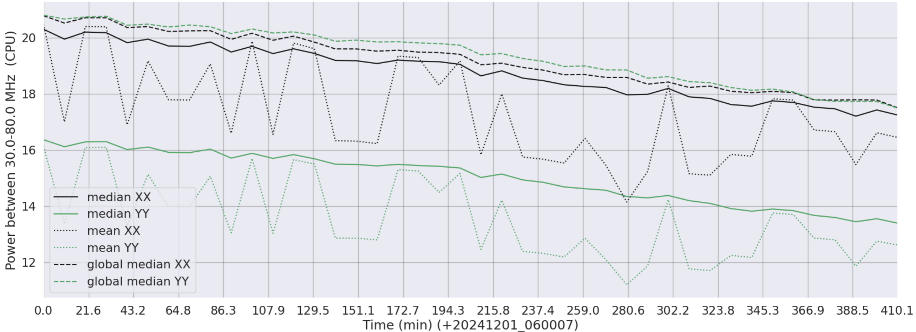
LWA158 - Correlator# 237 - XX FLAGS:BadSpecShape - YY FLAGS:BadSpecShape
