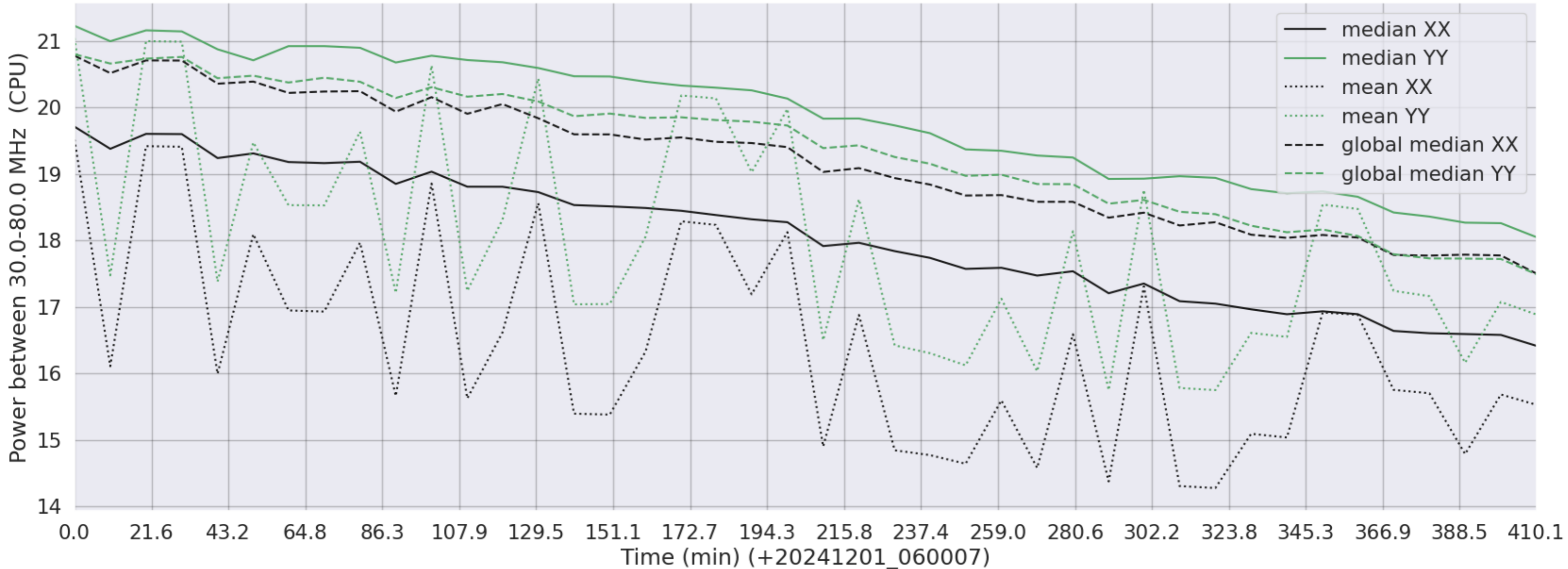
LWA113 - Correlator# 203 - XX FLAGS:BadSpecShape - YY FLAGS:BadSpecShape
