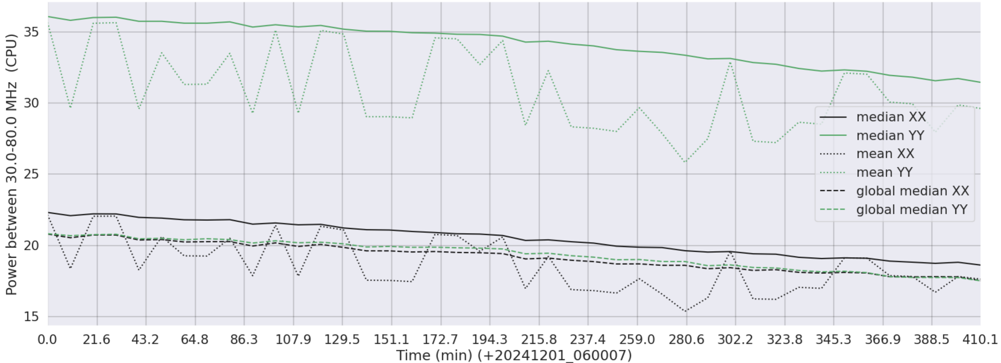
LWA187 - Correlator# 242 - XX FLAGS:BadSpecShape - YY FLAGS:BadSpecShape
