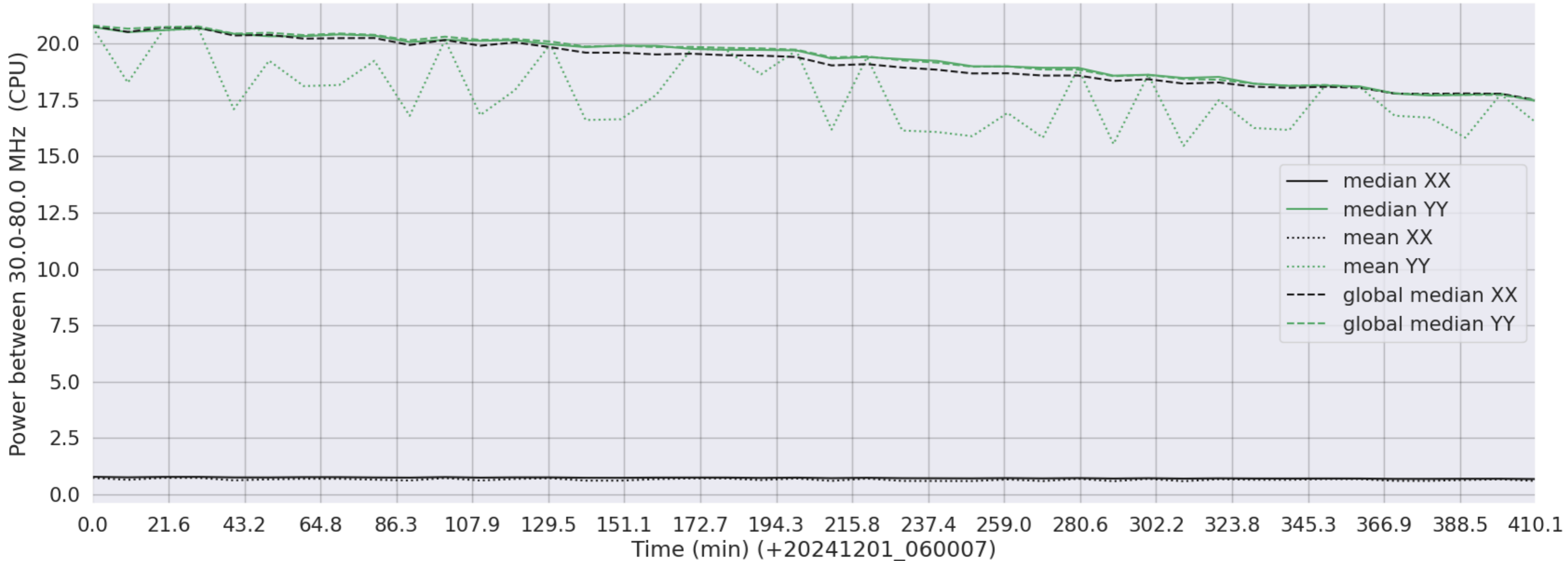
LWA105 - Correlator# 178 - XX FLAGS:LowPower - YY FLAGS:BadSpecShape
