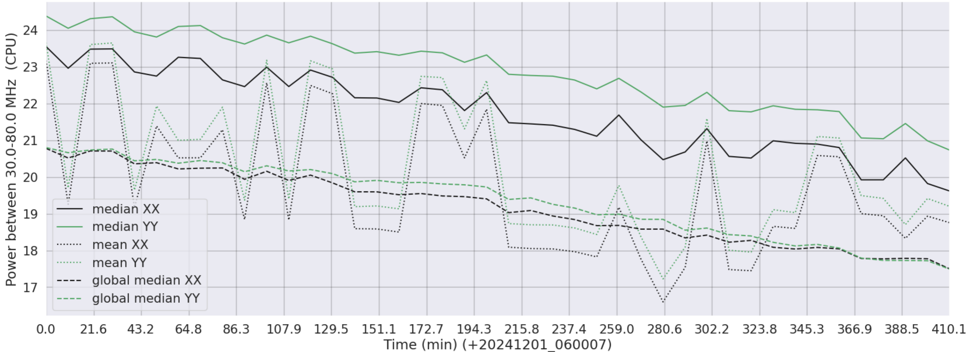
LWA163 - Correlator# 264 - XX FLAGS:BadSpecShape - YY FLAGS:BadSpecShape
