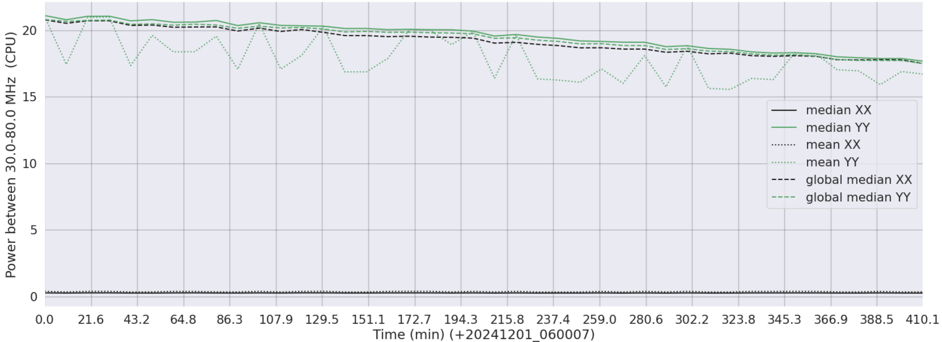
LWA110 - Correlator# 198 - XX FLAGS:LowPower - YY FLAGS:BadSpecShape
