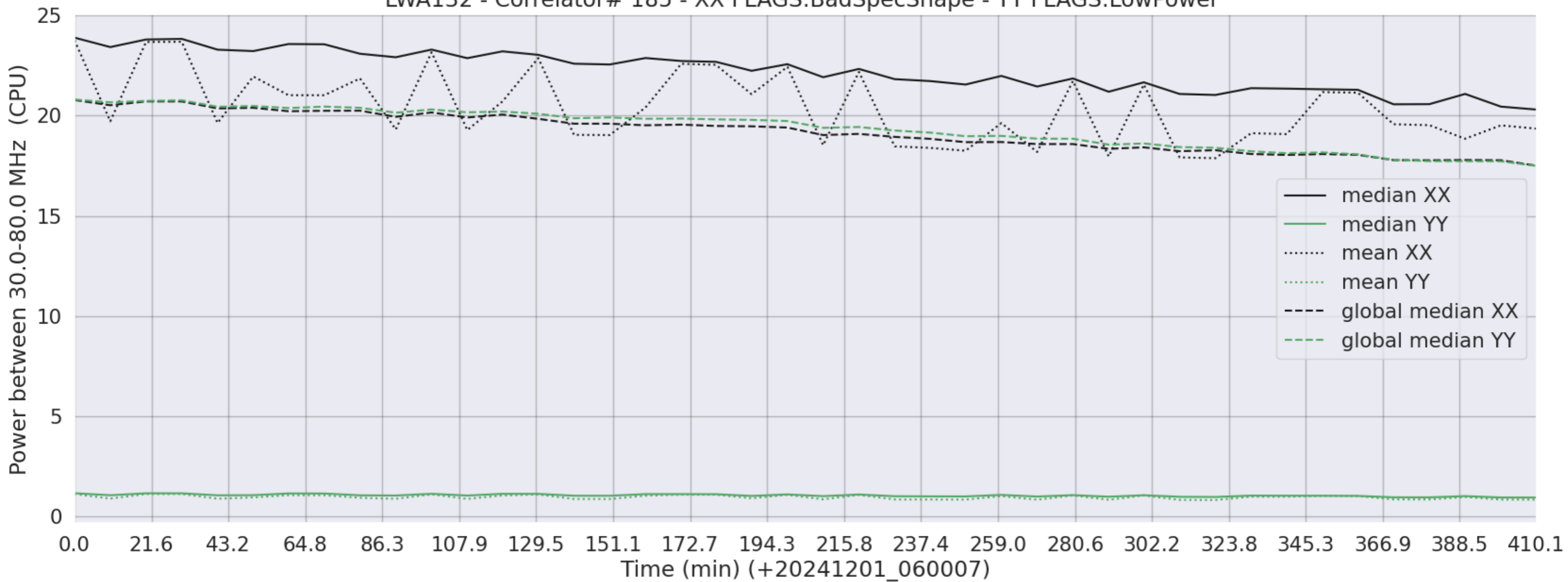
LWA132 - Correlator# 185 - XX FLAGS:BadSpecShape - YY FLAGS:LowPower
