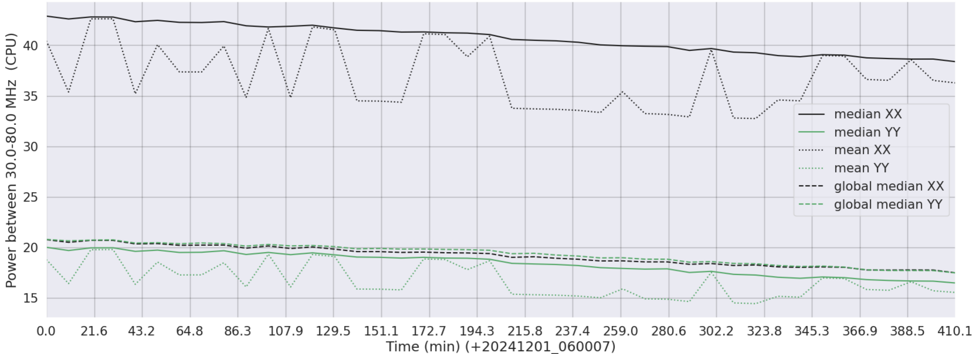
LWA221 - Correlator# 334 - XX FLAGS:BadSpecShape - YY FLAGS:BadSpecShape
