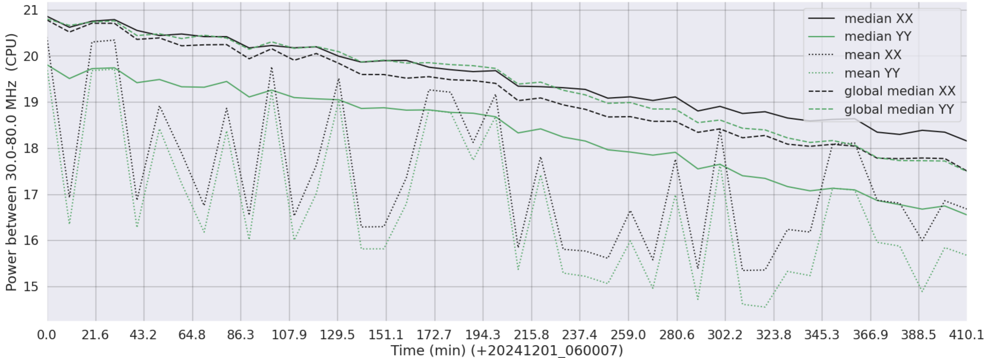
LWA117 - Correlator# 207 - XX FLAGS:BadSpecShape - YY FLAGS:BadSpecShape
