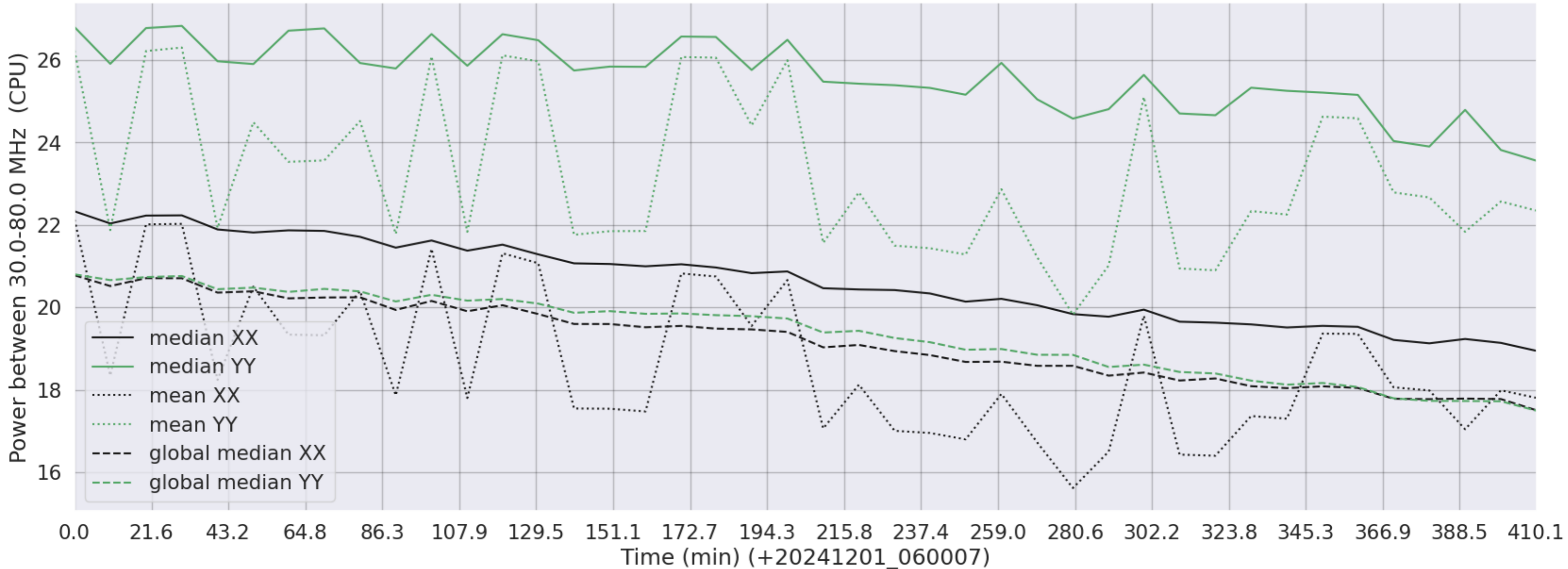
LWA326 - Correlator# 250 - XX FLAGS:BadSpecShape - YY FLAGS:BadSpecShape
