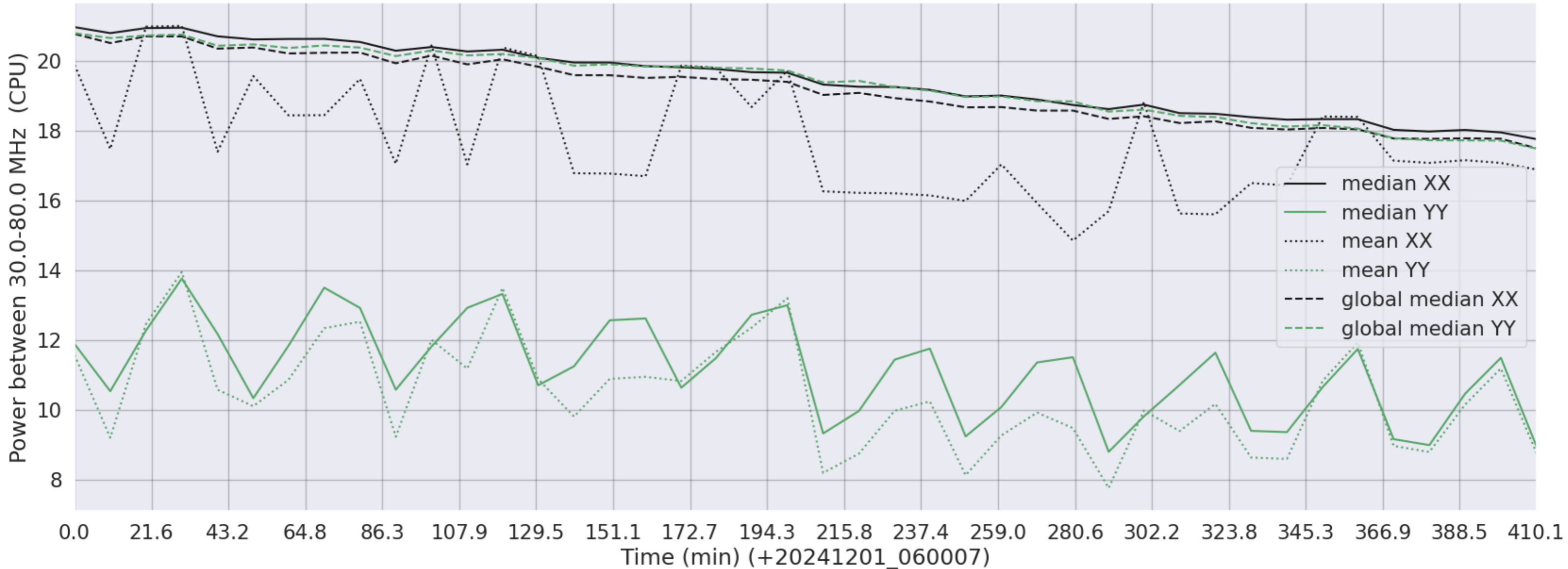
LWA235 - Correlator# 309 - XX FLAGS:BadSpecShape - YY FLAGS:HighTimeVar+BadSpecShape
