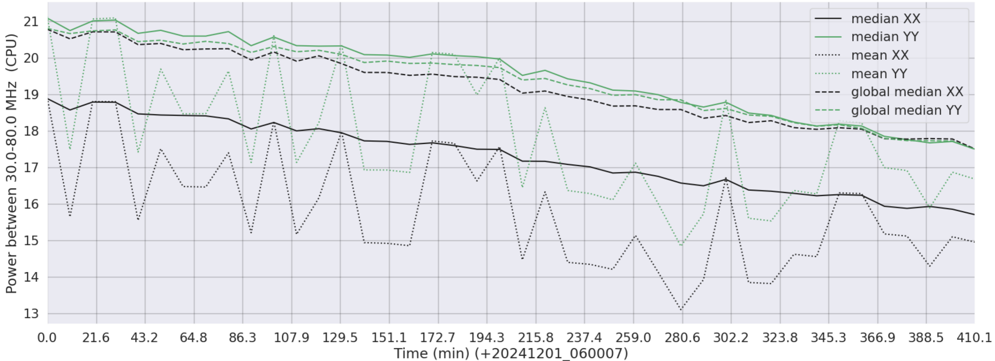
LWA151 - Correlator# 218 - XX FLAGS:BadSpecShape - YY FLAGS:BadSpecShape
