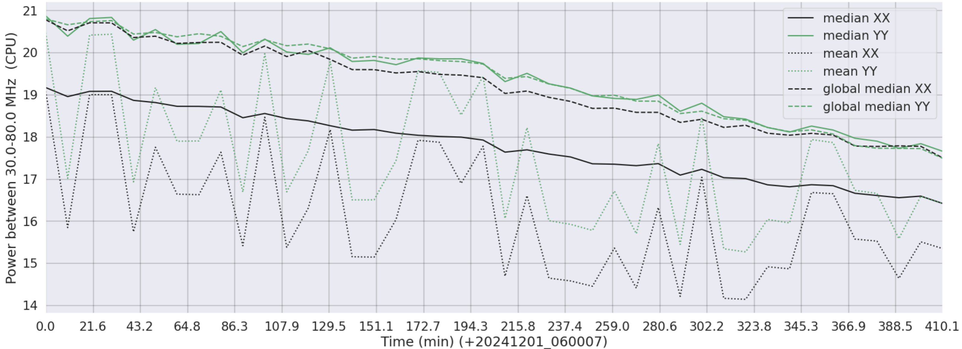
LWA115 - Correlator# 205 - XX FLAGS:BadSpecShape - YY FLAGS:BadSpecShape
