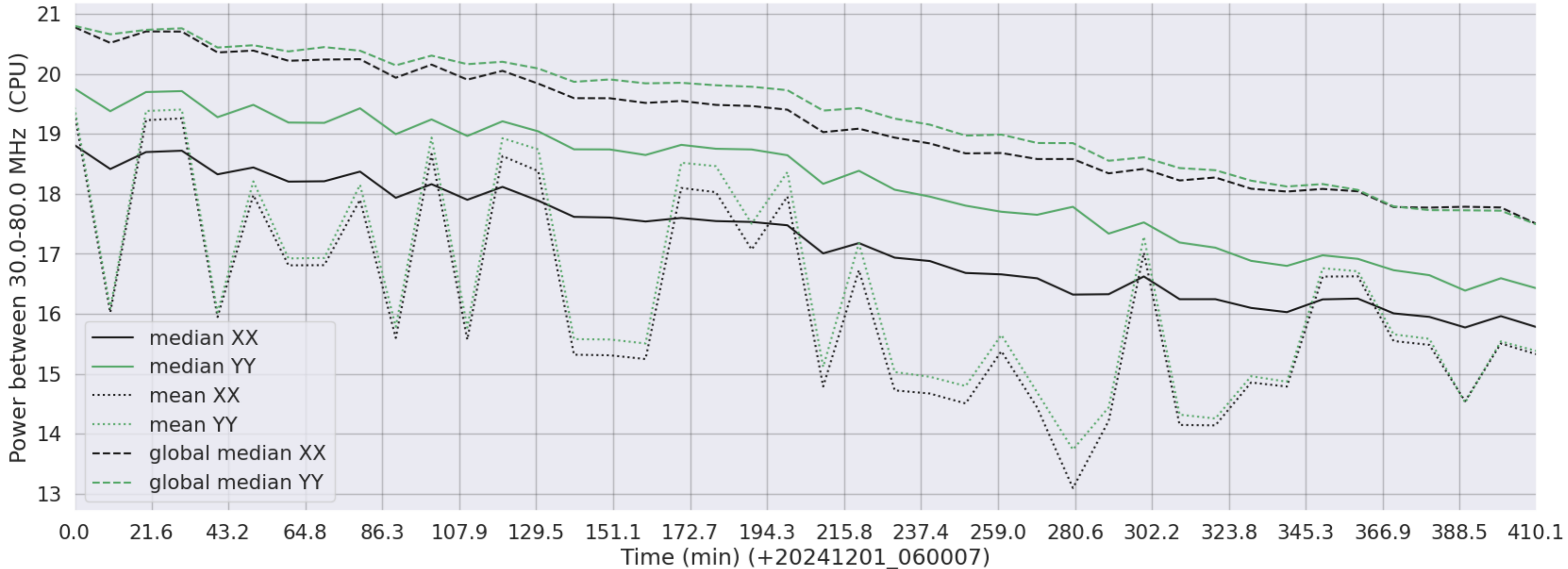
LWA154 - Correlator# 233 - XX FLAGS:BadSpecShape - YY FLAGS:BadSpecShape
