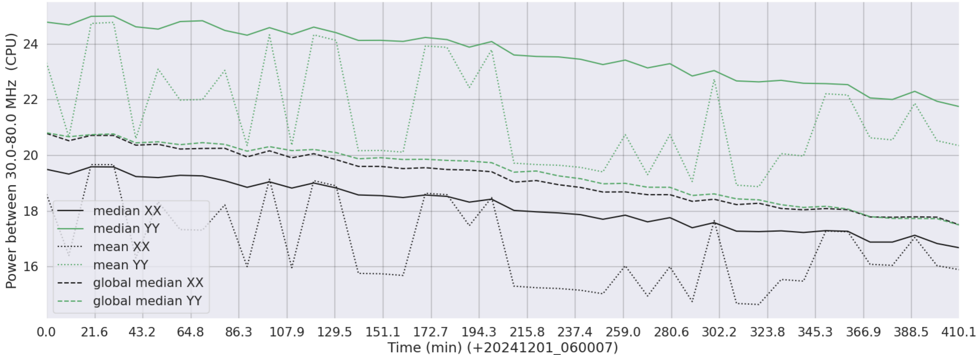
LWA300 - Correlator# 348 - XX FLAGS:BadSpecShape - YY FLAGS:BadSpecShape
