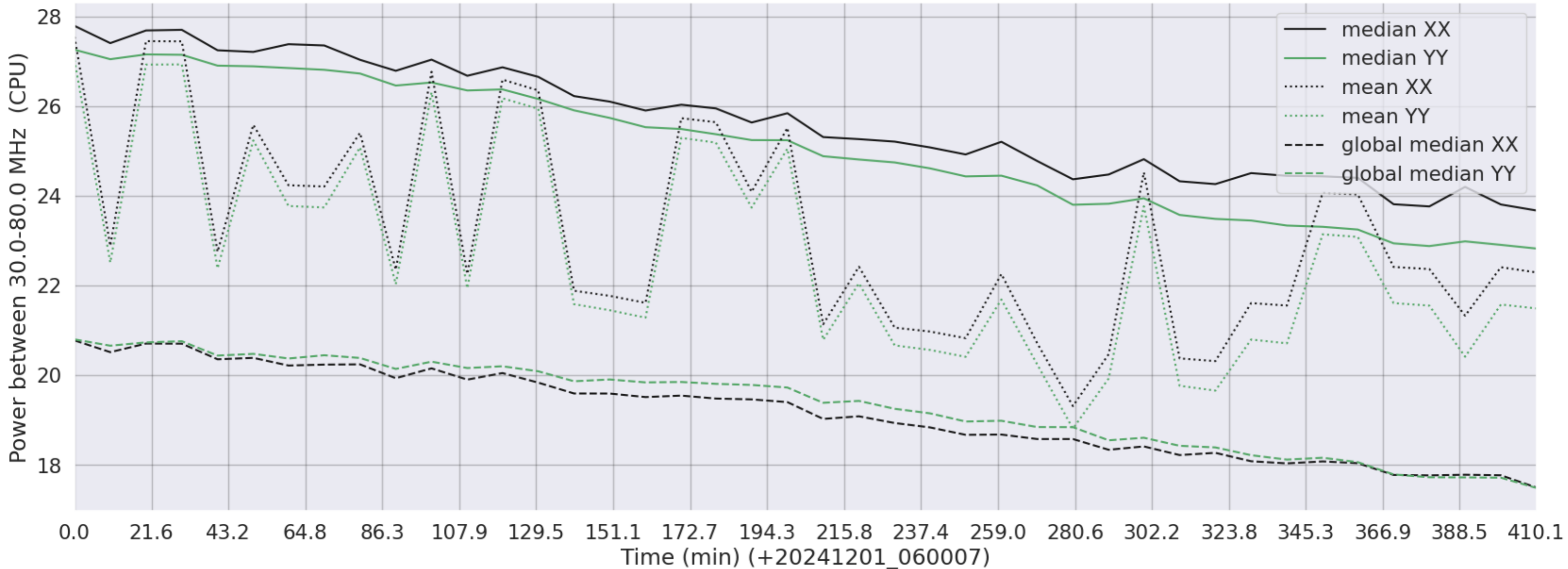
LWA333 - Correlator# 253 - XX FLAGS:BadSpecShape - YY FLAGS:BadSpecShape
