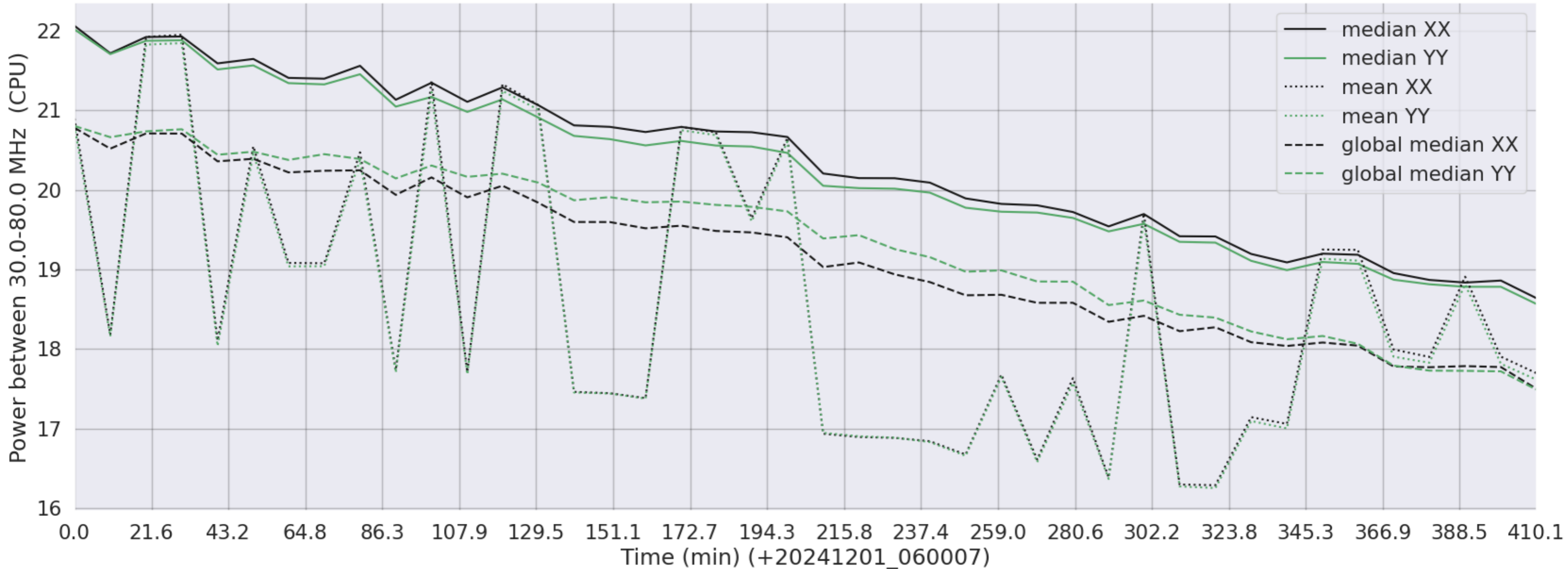
LWA256 - Correlator# 347 - XX FLAGS:BadSpecShape - YY FLAGS:BadSpecShape
