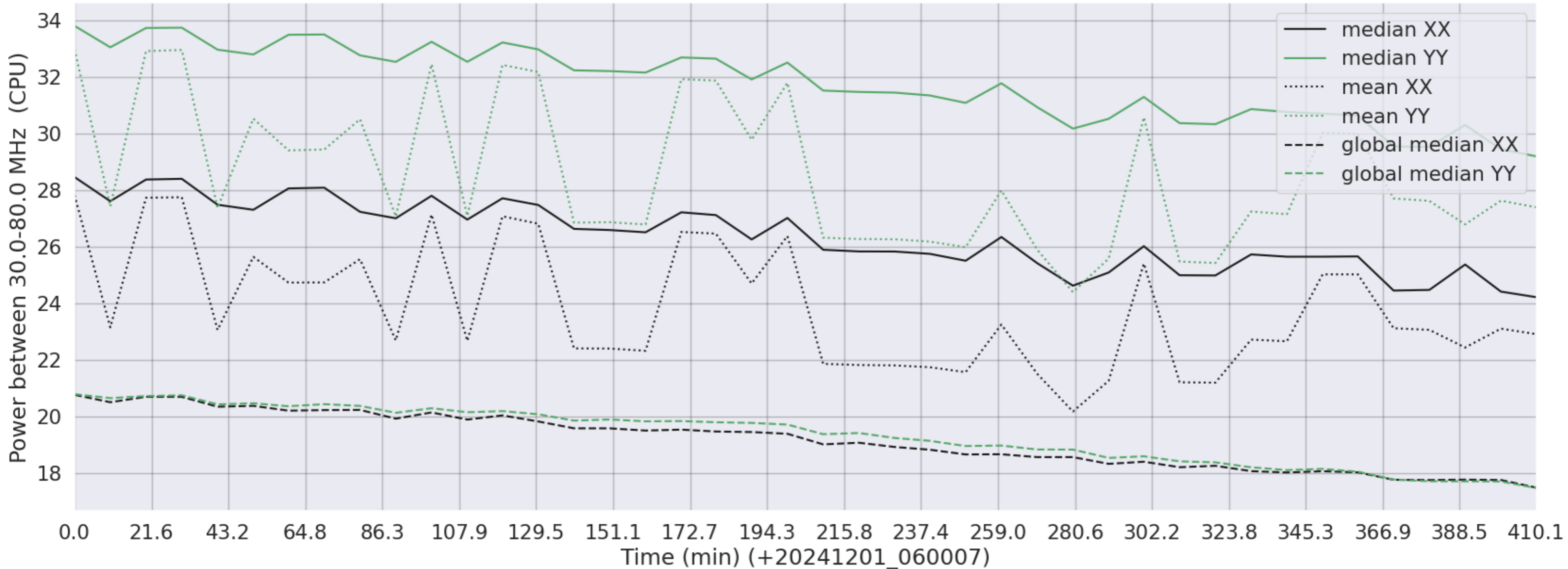
LWA195 - Correlator# 272 - XX FLAGS:BadSpecShape - YY FLAGS:BadSpecShape
