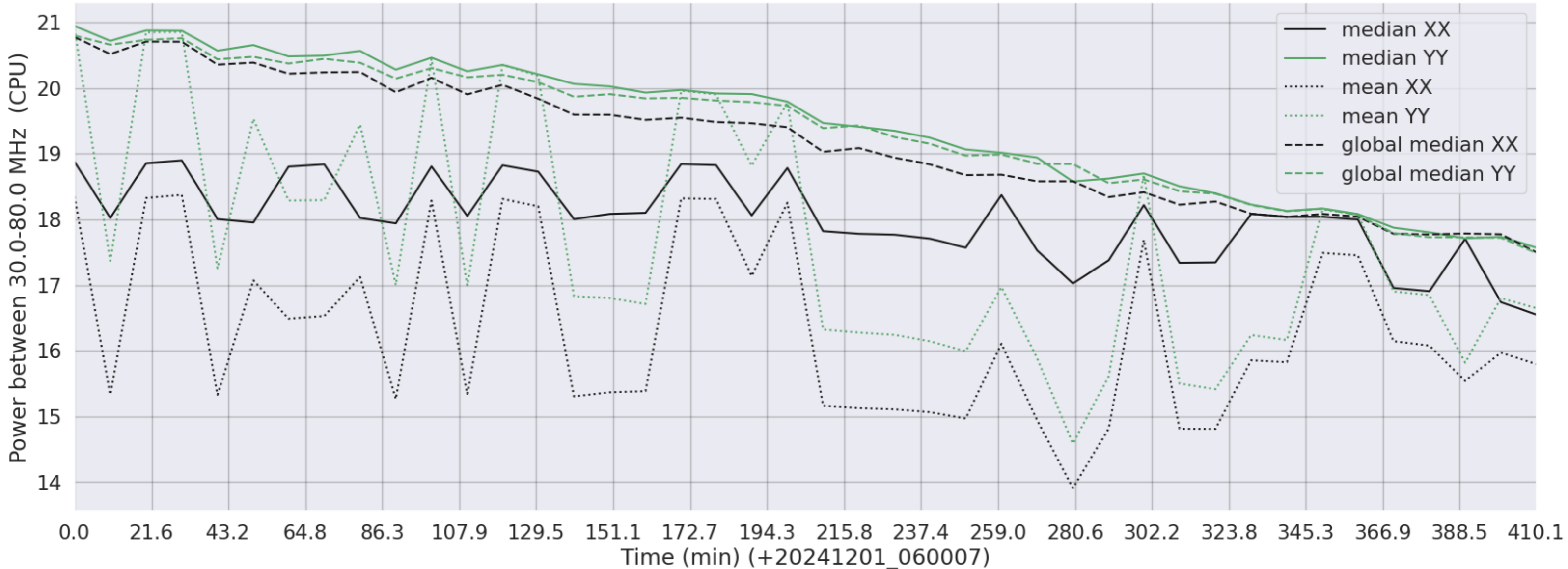
LWA357 - Correlator# 286 - XX FLAGS:BadSpecShape - YY FLAGS:BadSpecShape
