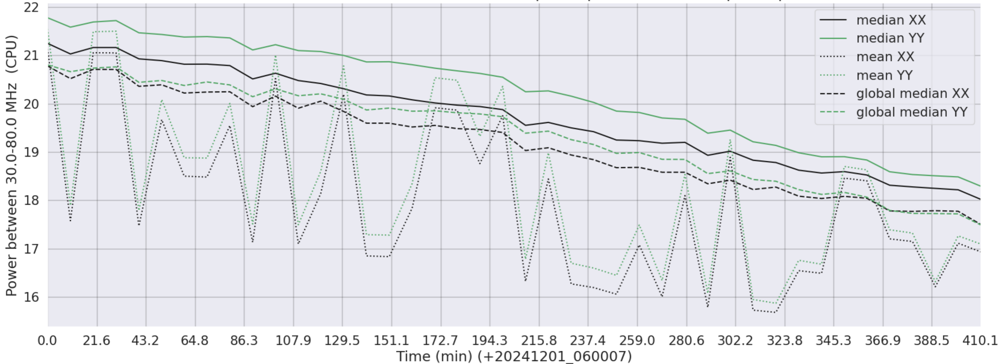
LWA114 - Correlator# 202 - XX FLAGS:BadSpecShape - YY FLAGS:BadSpecShape
