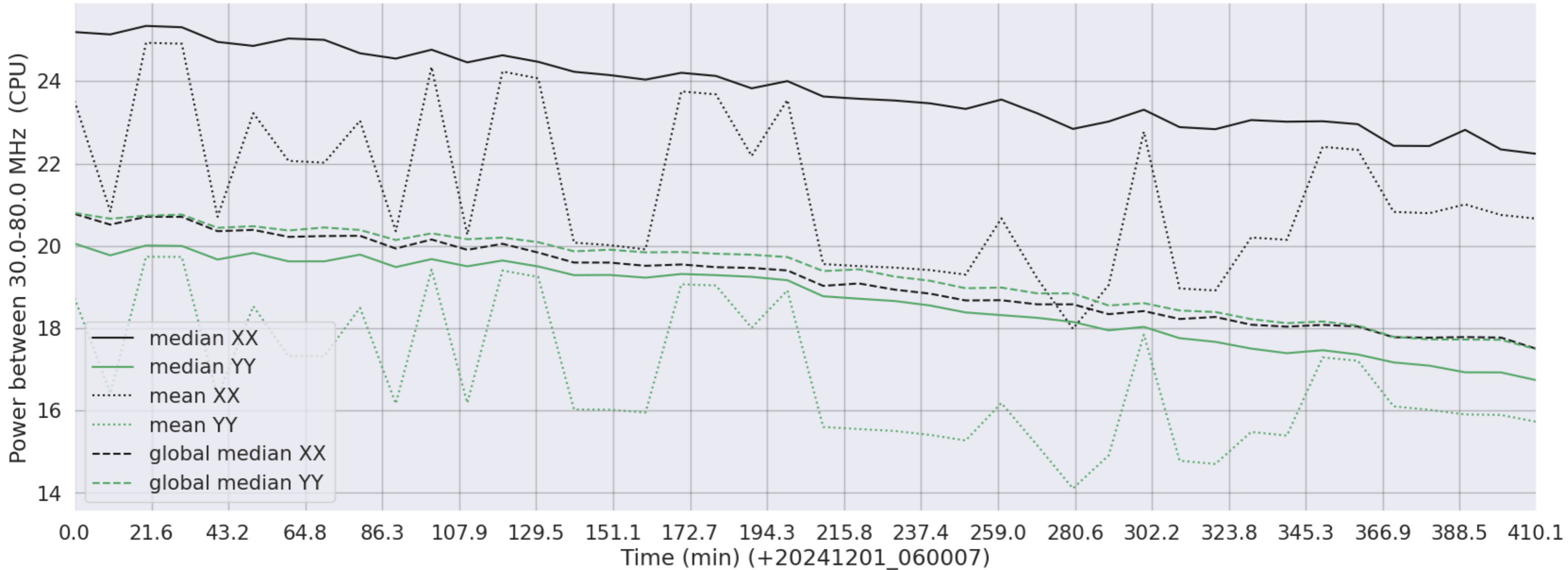
LWA356 - Correlator# 318 - XX FLAGS:BadSpecShape - YY FLAGS:BadSpecShape
