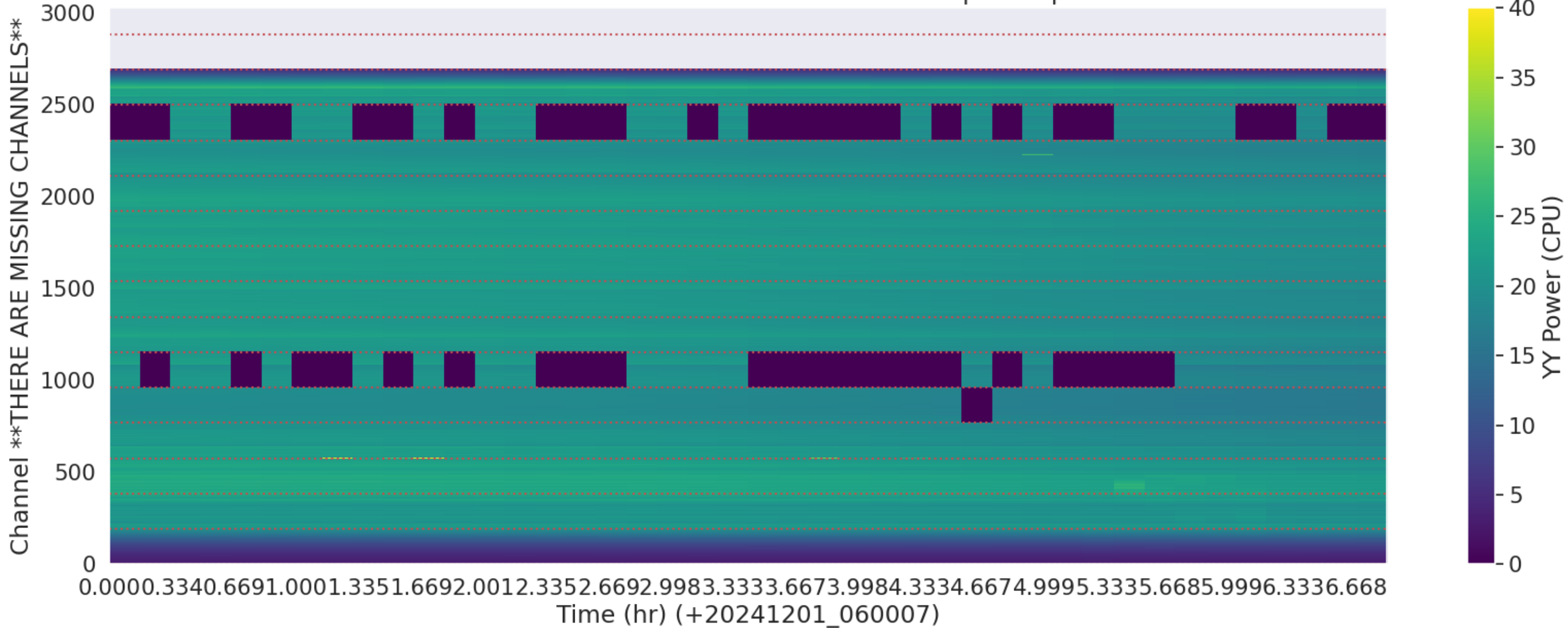
LWA261 - Correlator# 346 - YY - FLAGS: BadSpecShape
