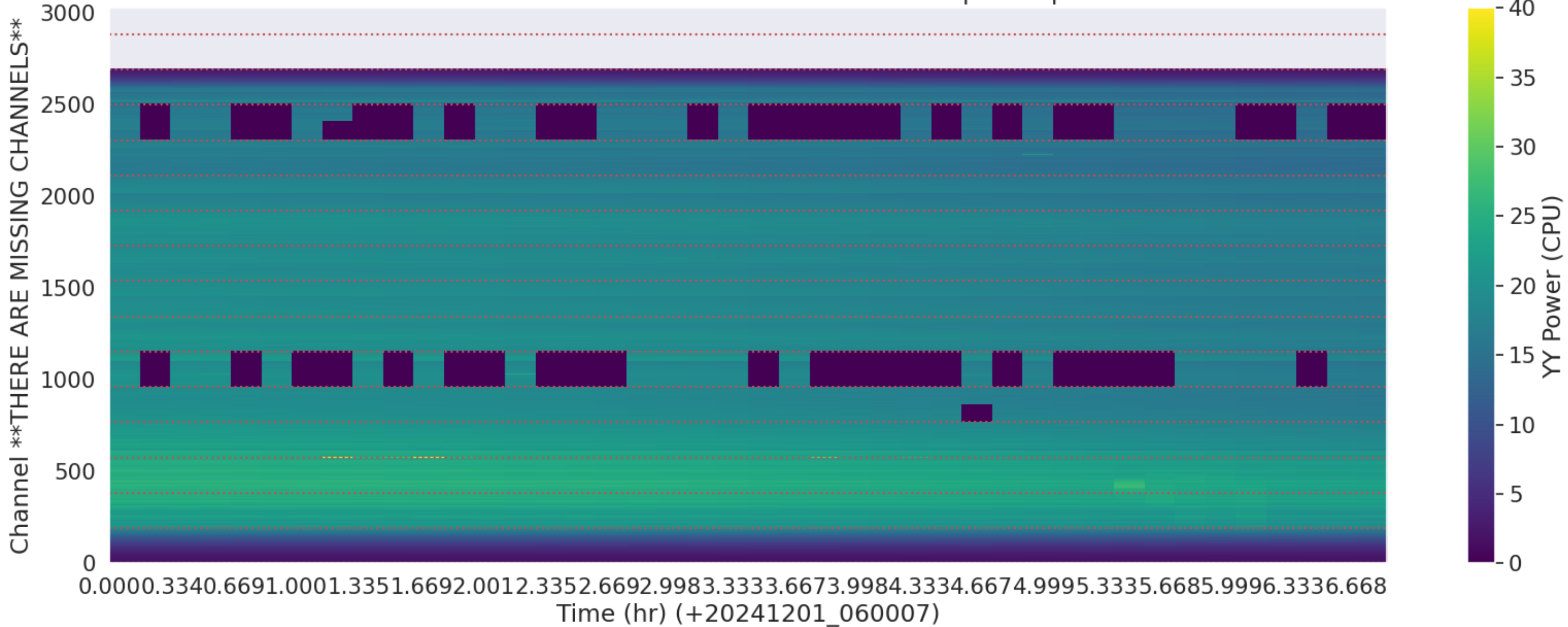
LWA120 - Correlator# 208 - YY - FLAGS: BadSpecShape
