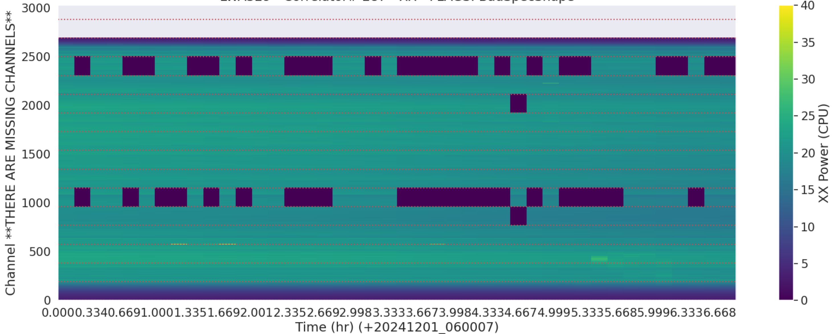
LWA329 - Correlator# 287 - XX - FLAGS: BadSpecShape
