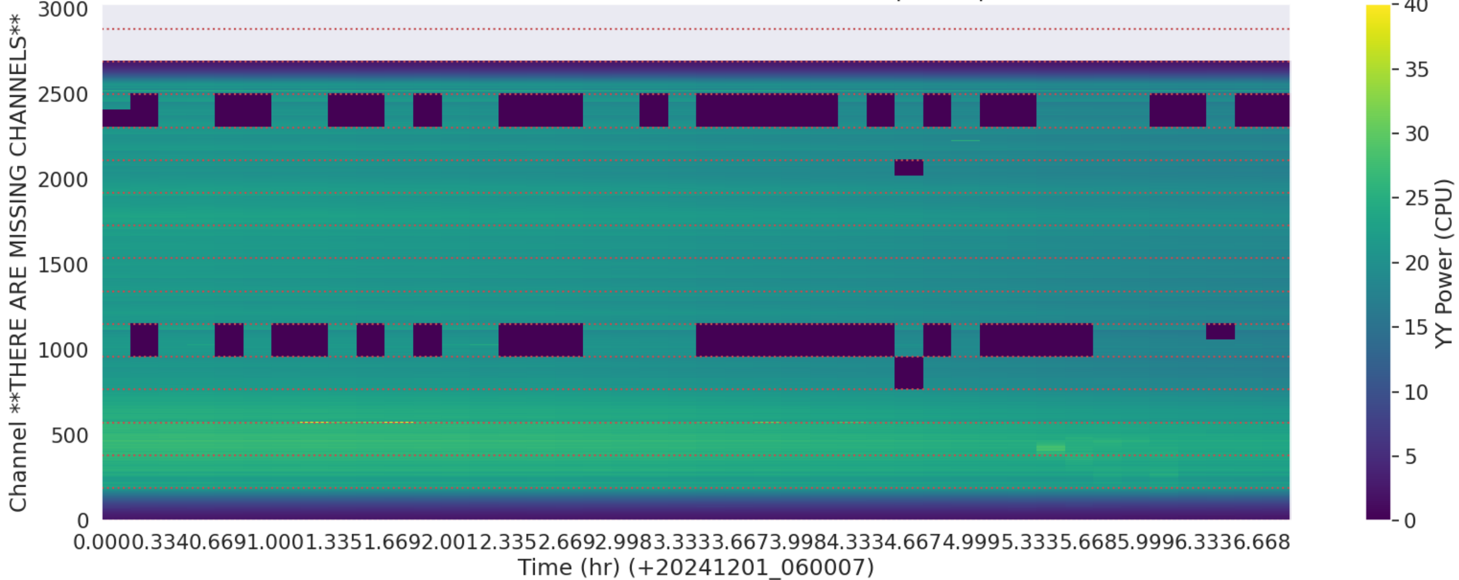
LWA176 - Correlator# 325 - YY - FLAGS: BadSpecShape
