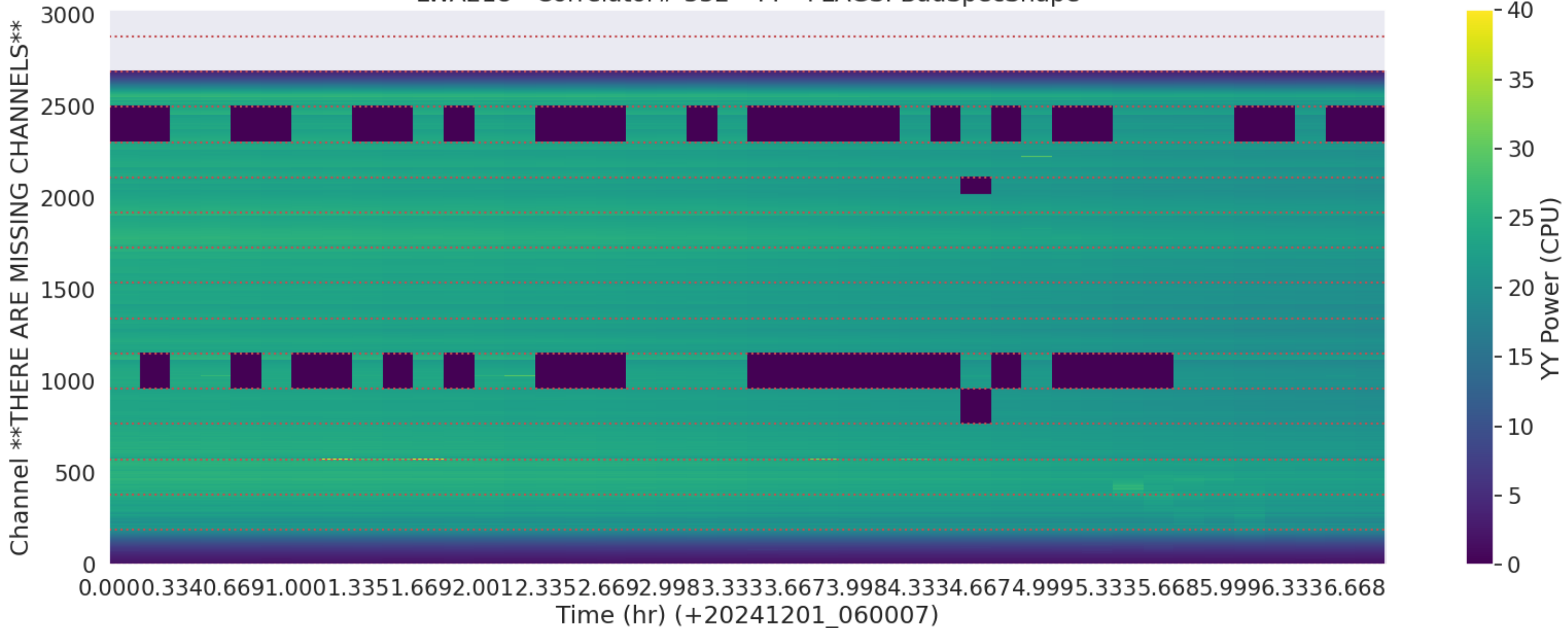
LWA218 - Correlator# 332 - YY - FLAGS: BadSpecShape
