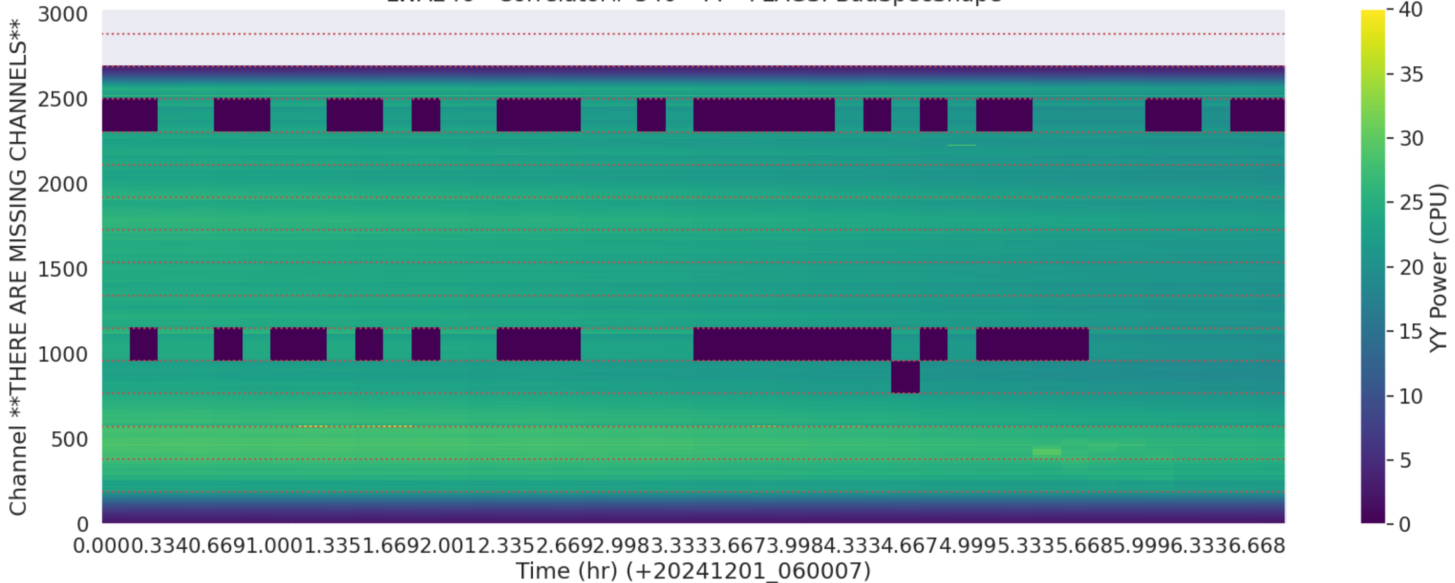
LWA246 - Correlator# 340 - YY - FLAGS: BadSpecShape
