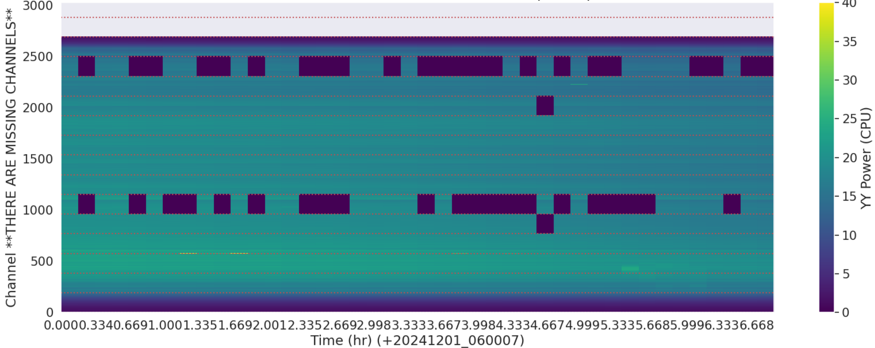
LWA185 - Correlator# 240 - YY - FLAGS: BadSpecShape
