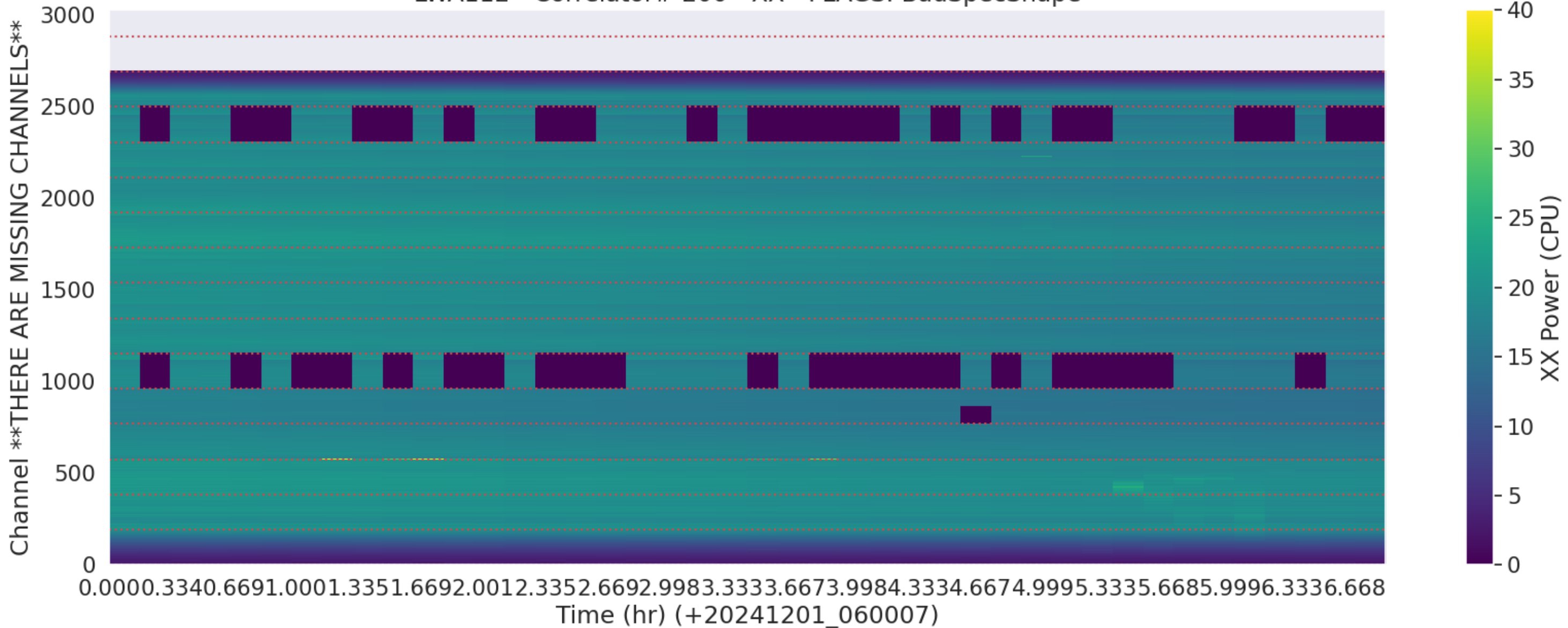
LWA112 - Correlator# 200 - XX - FLAGS: BadSpecShape
