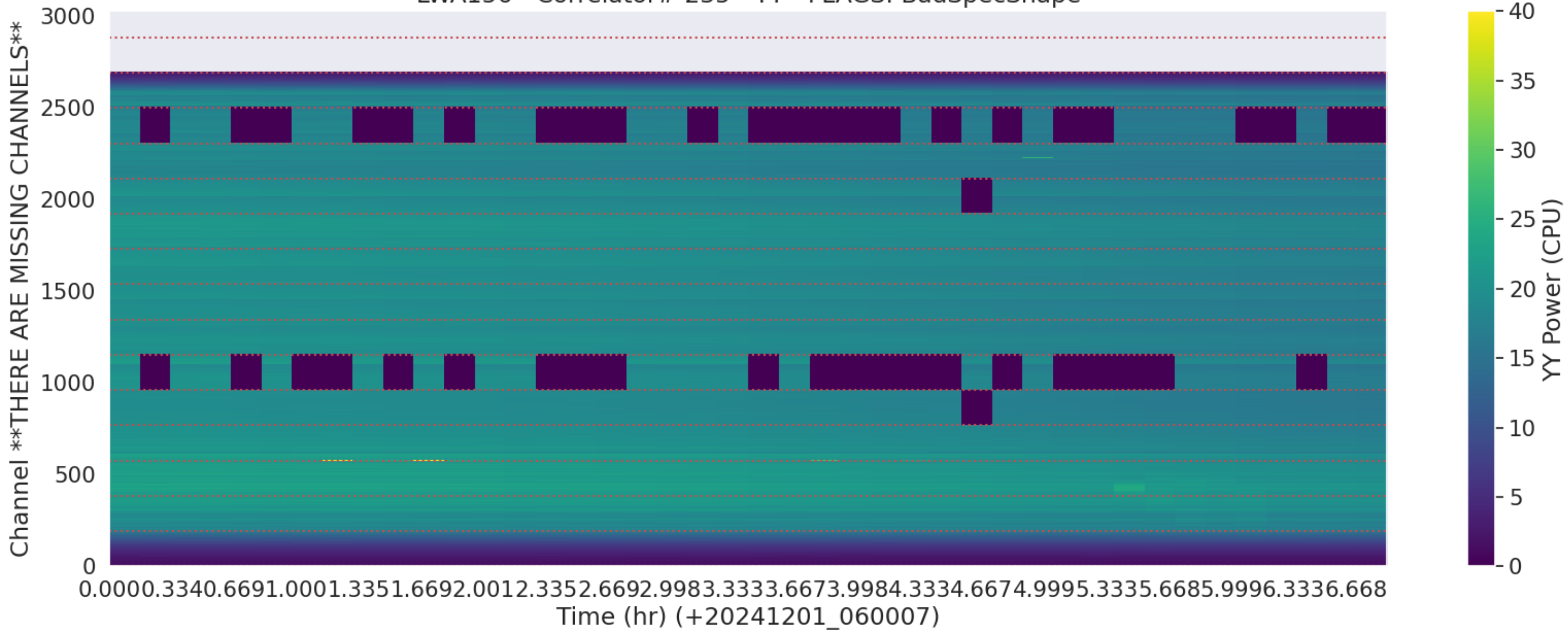
LWA156 - Correlator# 235 - YY - FLAGS: BadSpecShape
