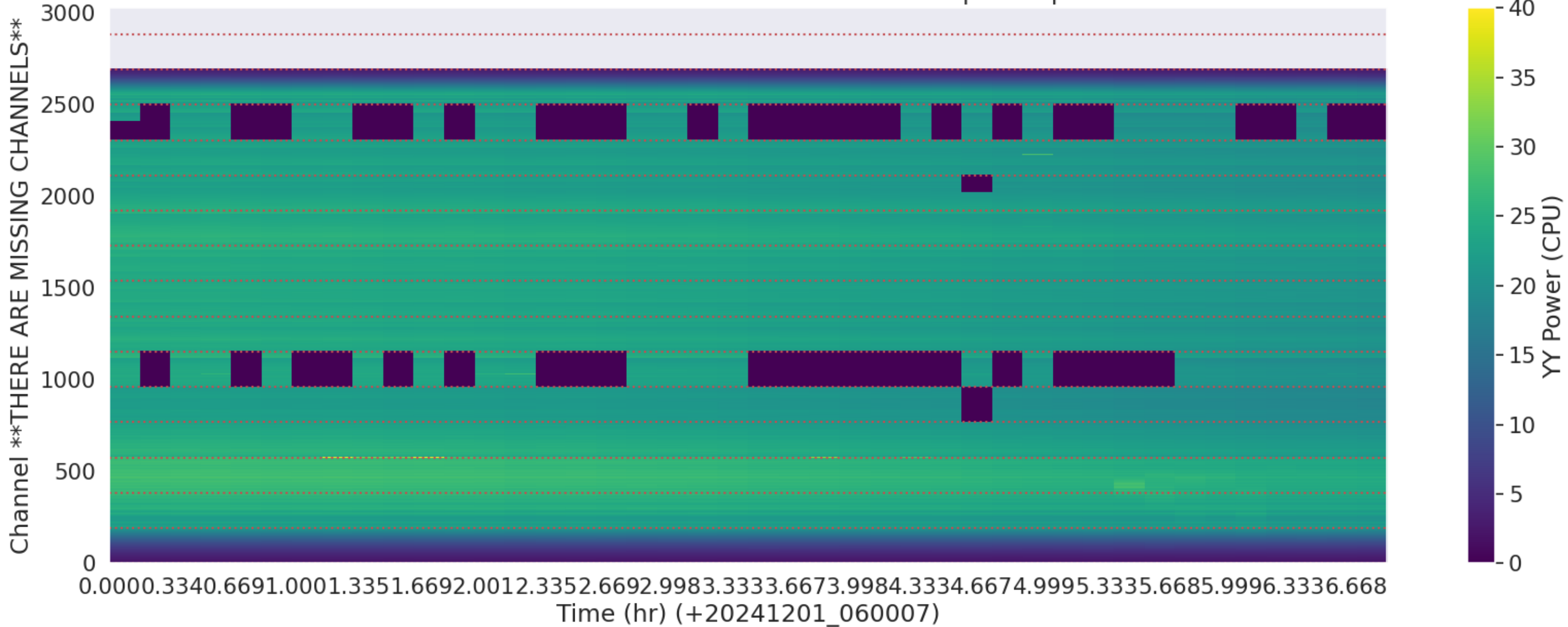
LWA212 - Correlator# 326 - YY - FLAGS: BadSpecShape
