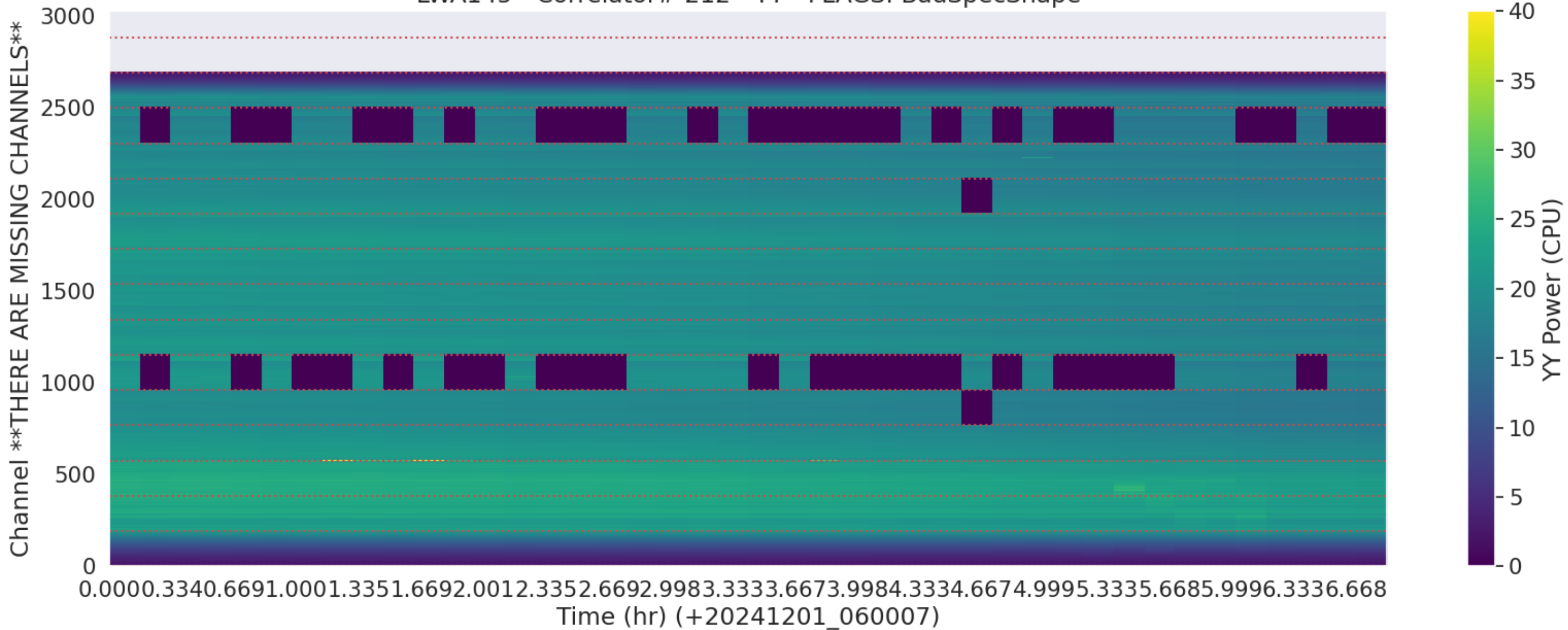
LWA145 - Correlator# 212 - YY - FLAGS: BadSpecShape
