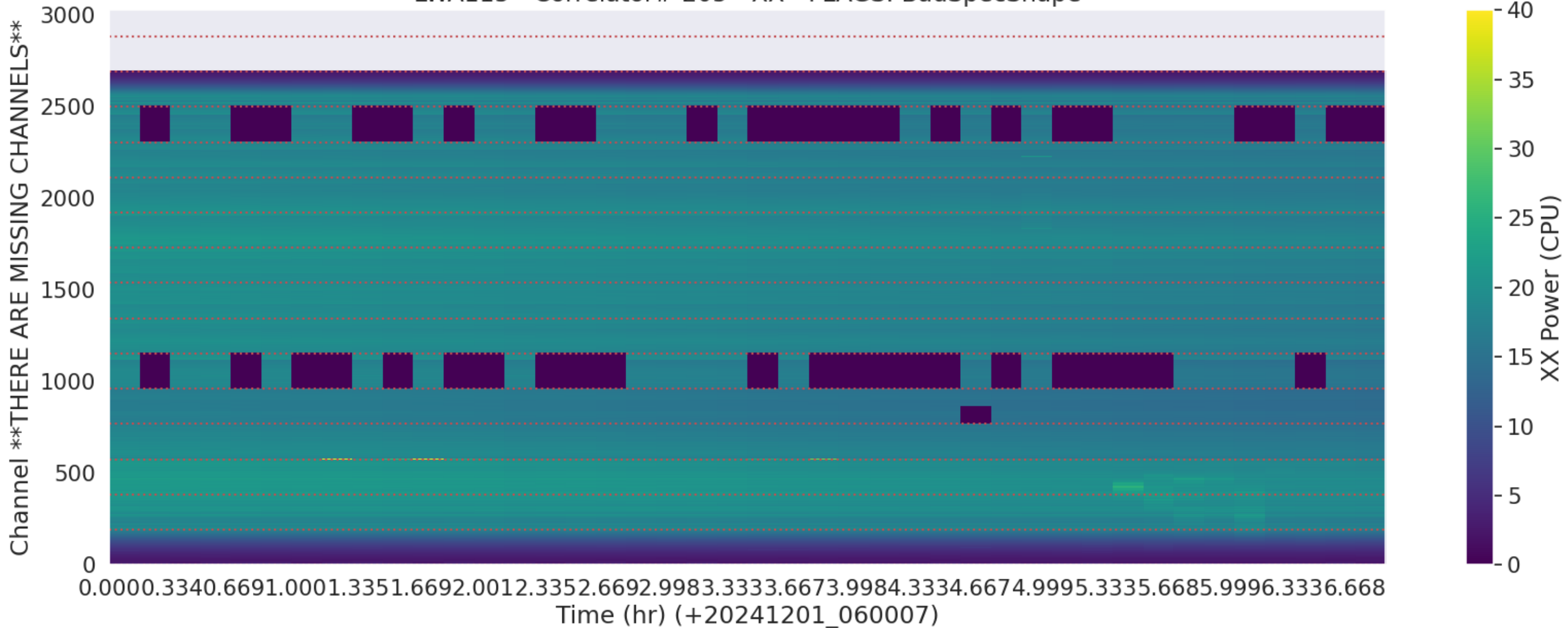
LWA115 - Correlator# 205 - XX - FLAGS: BadSpecShape
