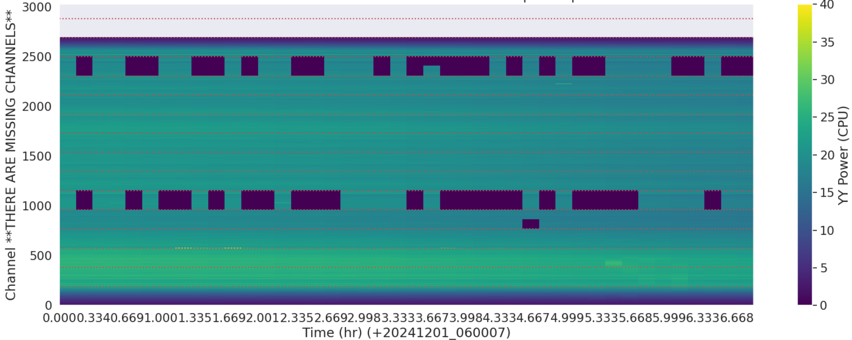
LWA078 - Correlator# 192 - YY - FLAGS: BadSpecShape
