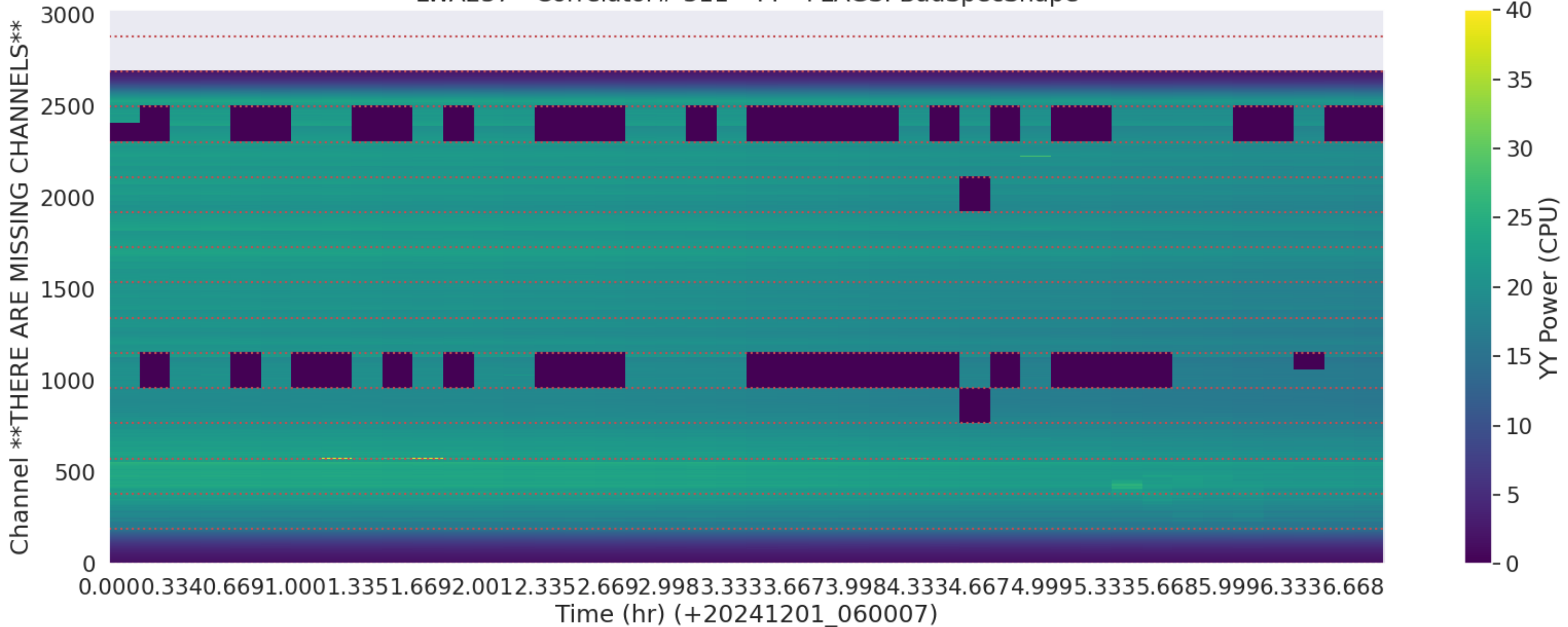
LWA237 - Correlator# 311 - YY - FLAGS: BadSpecShape
