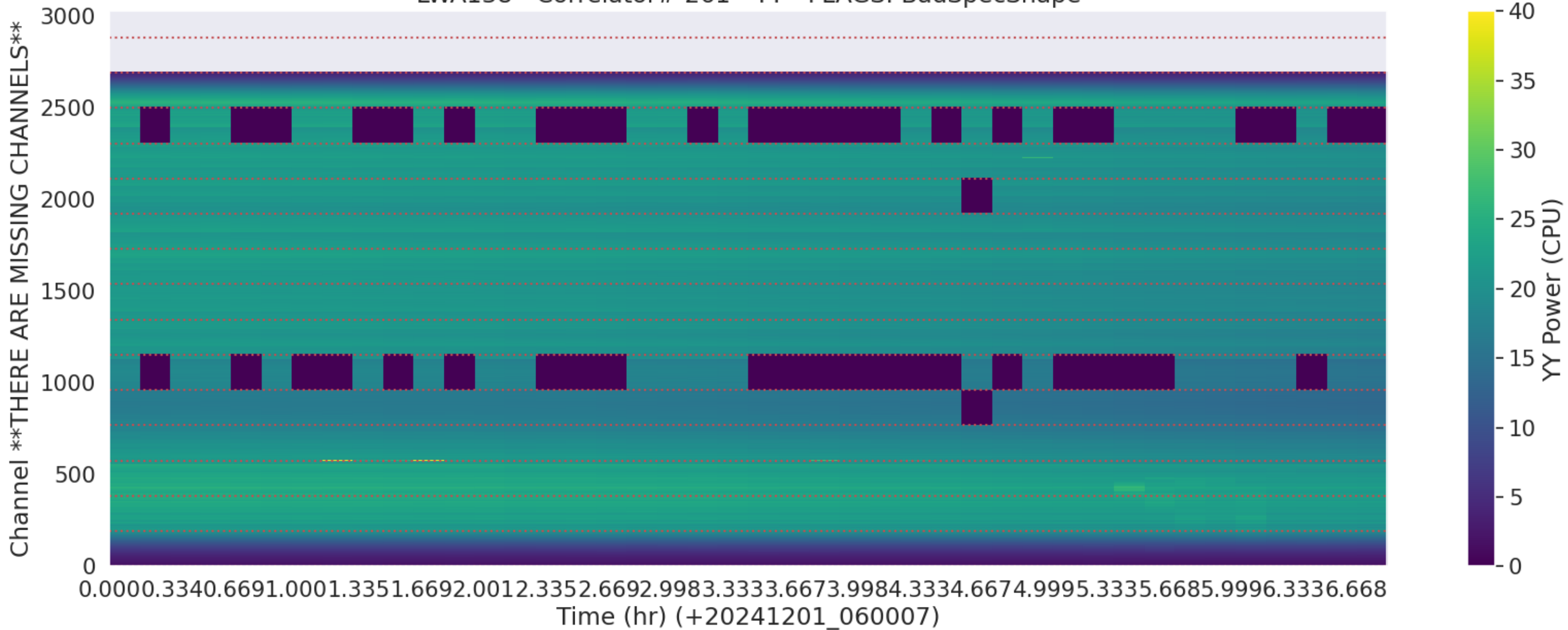
LWA138 - Correlator# 261 - YY - FLAGS: BadSpecShape
