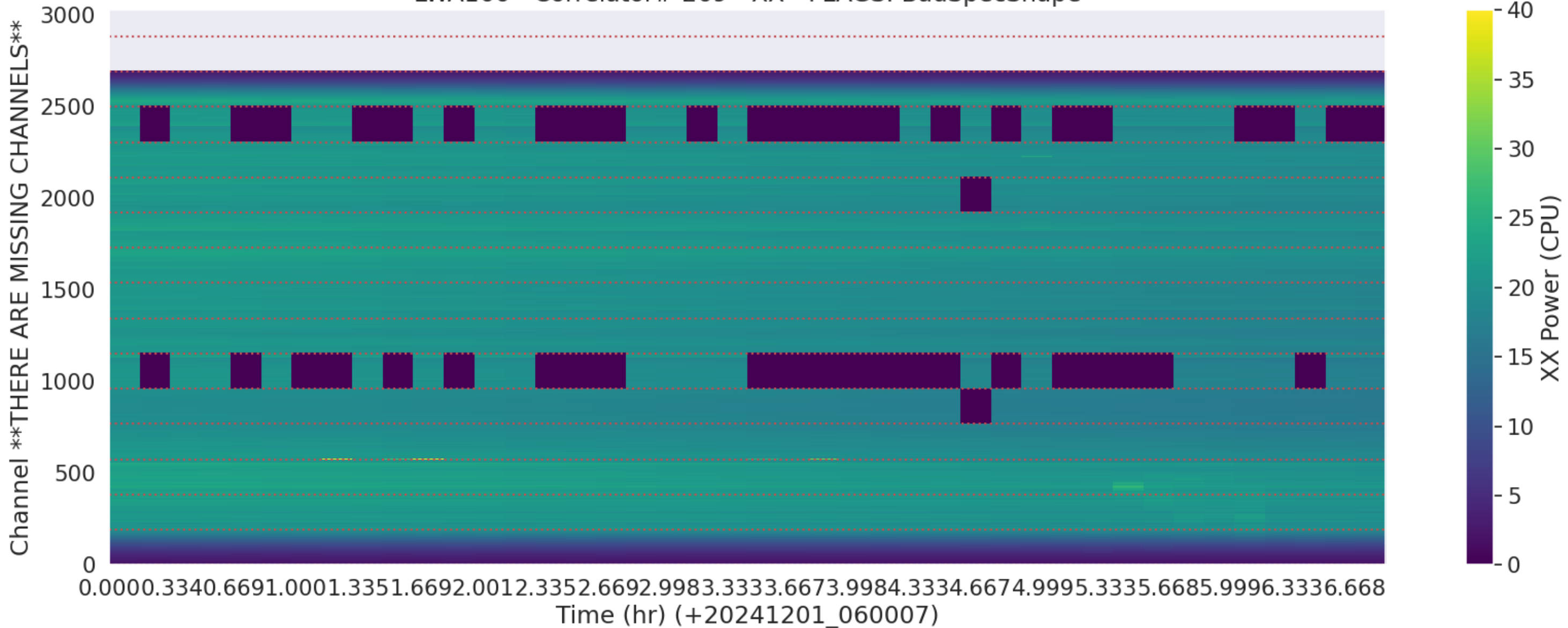
LWA166 - Correlator# 269 - XX - FLAGS: BadSpecShape
