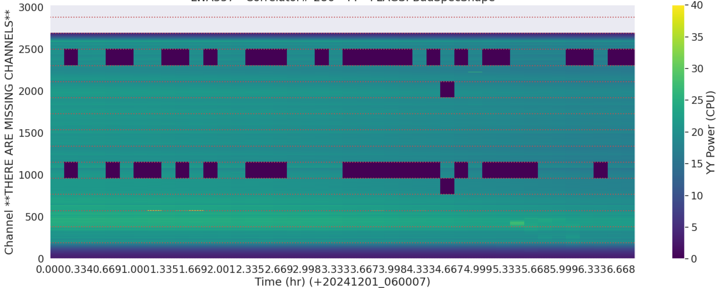
LWA357 - Correlator# 286 - YY - FLAGS: BadSpecShape
