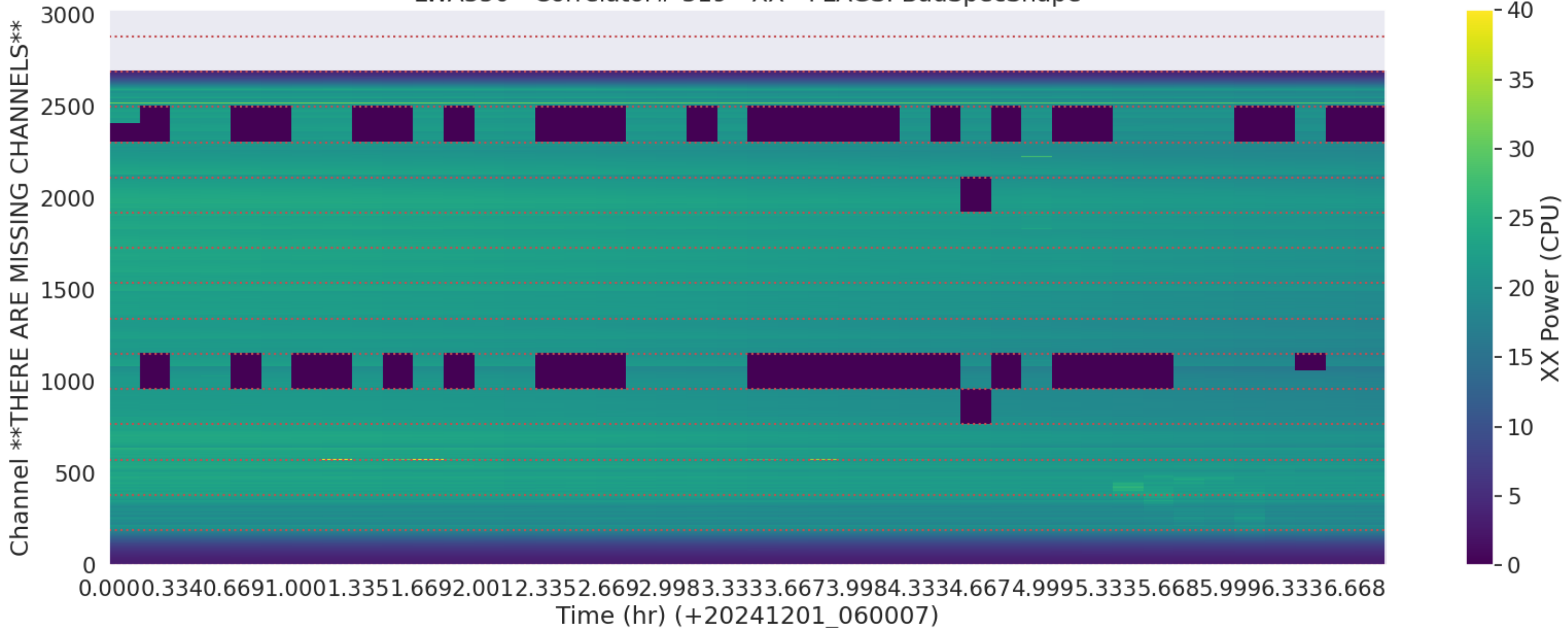
LWA350 - Correlator# 319 - XX - FLAGS: BadSpecShape
