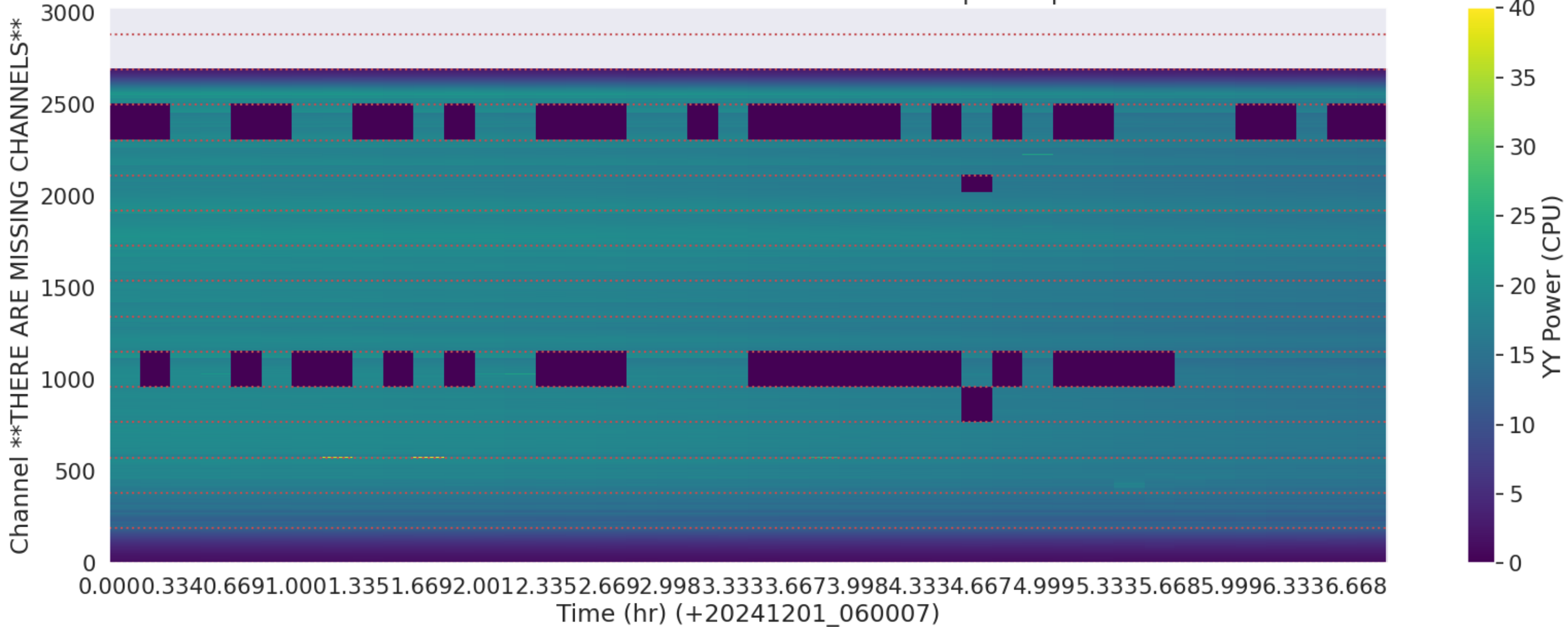
LWA219 - Correlator# 335 - YY - FLAGS: BadSpecShape
