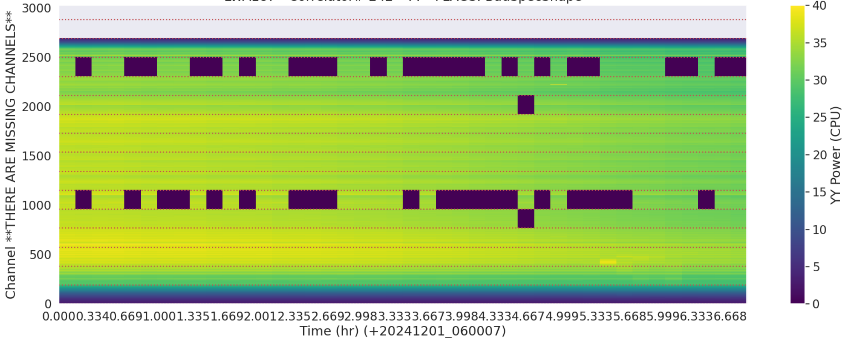
LWA187 - Correlator# 242 - YY - FLAGS: BadSpecShape
