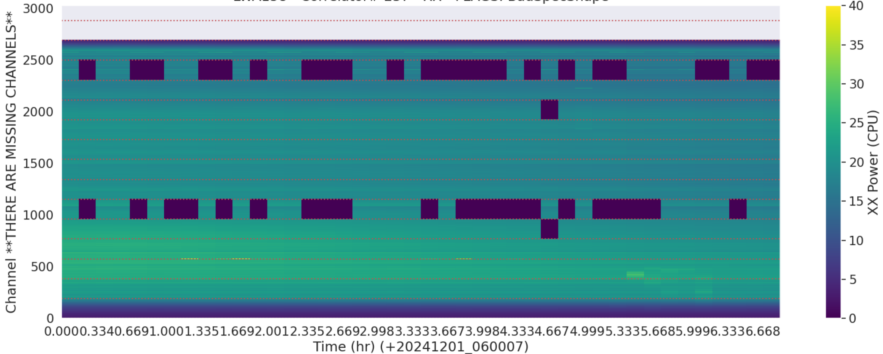
LWA158 - Correlator# 237 - XX - FLAGS: BadSpecShape
