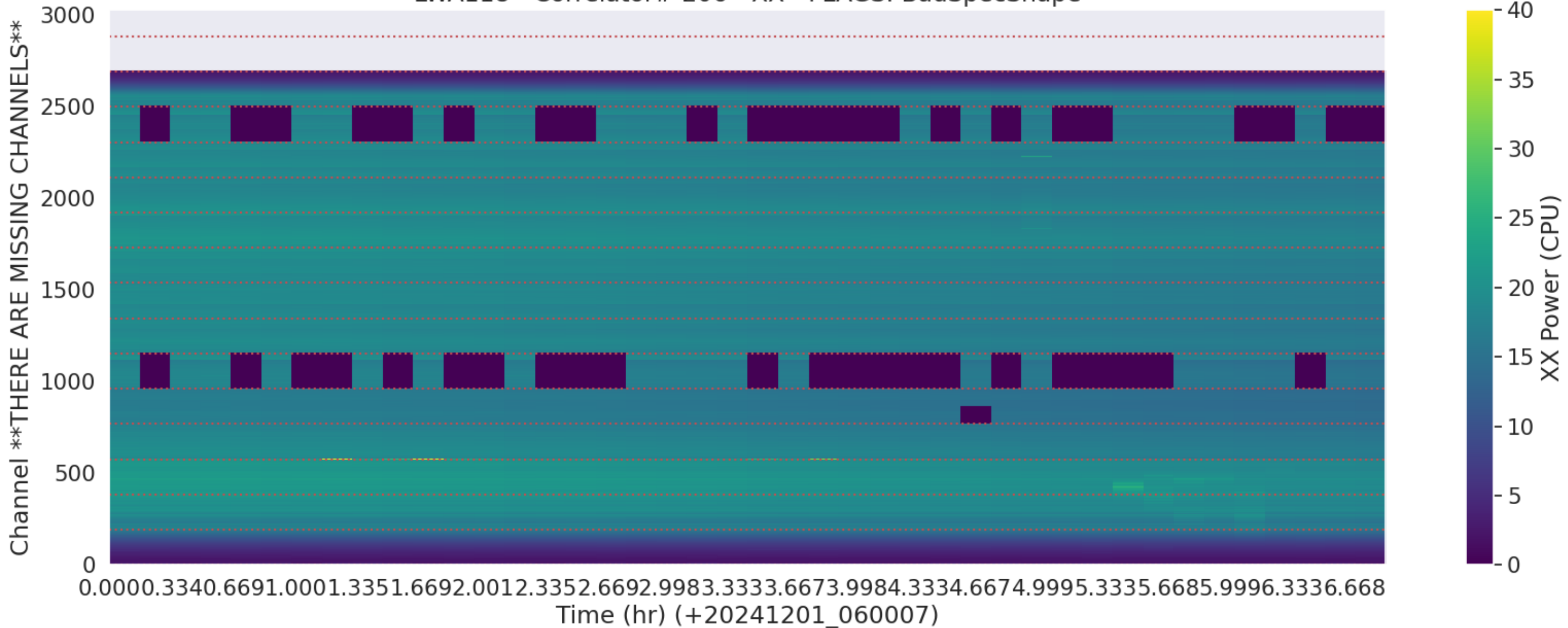
LWA118 - Correlator# 206 - XX - FLAGS: BadSpecShape
