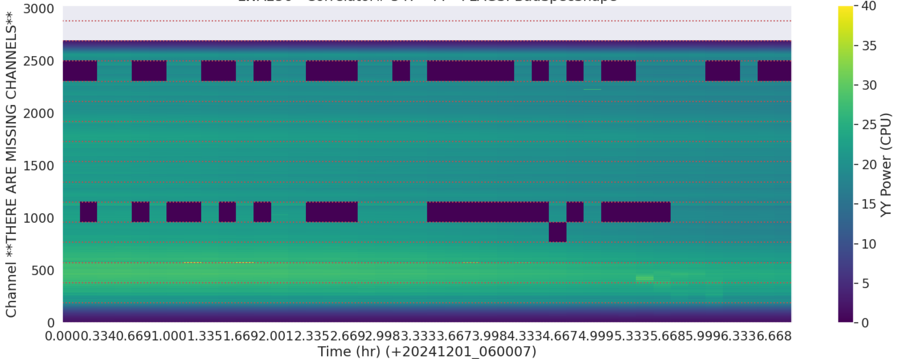
LWA256 - Correlator# 347 - YY - FLAGS: BadSpecShape
