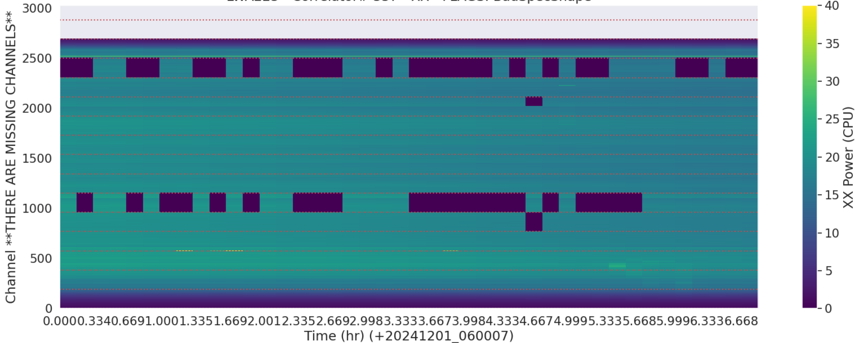
LWA223 - Correlator# 337 - XX - FLAGS: BadSpecShape
