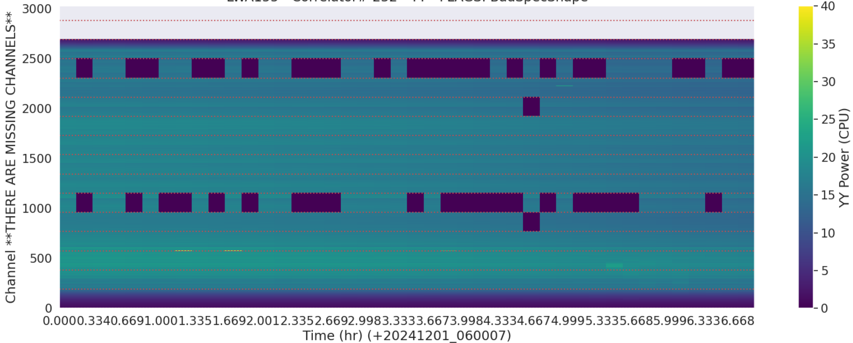
LWA155 - Correlator# 232 - YY - FLAGS: BadSpecShape
