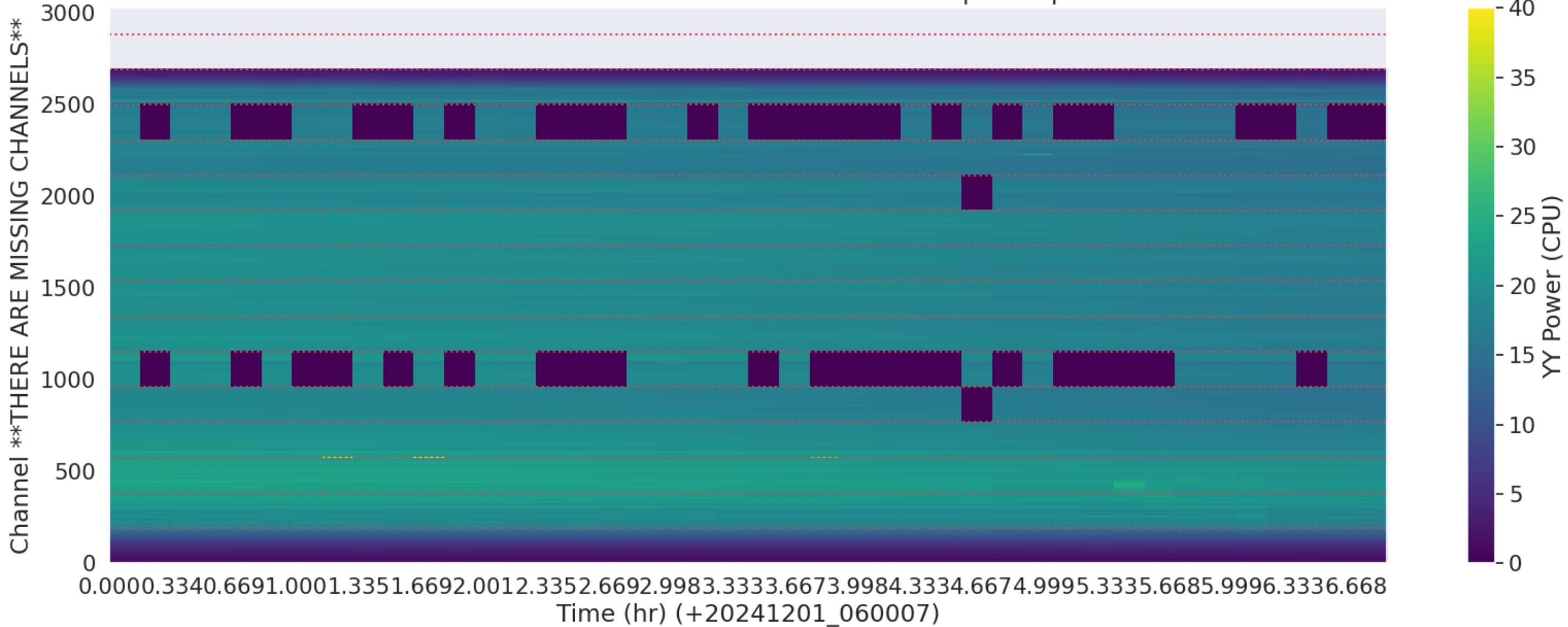
LWA154 - Correlator# 233 - YY - FLAGS: BadSpecShape
