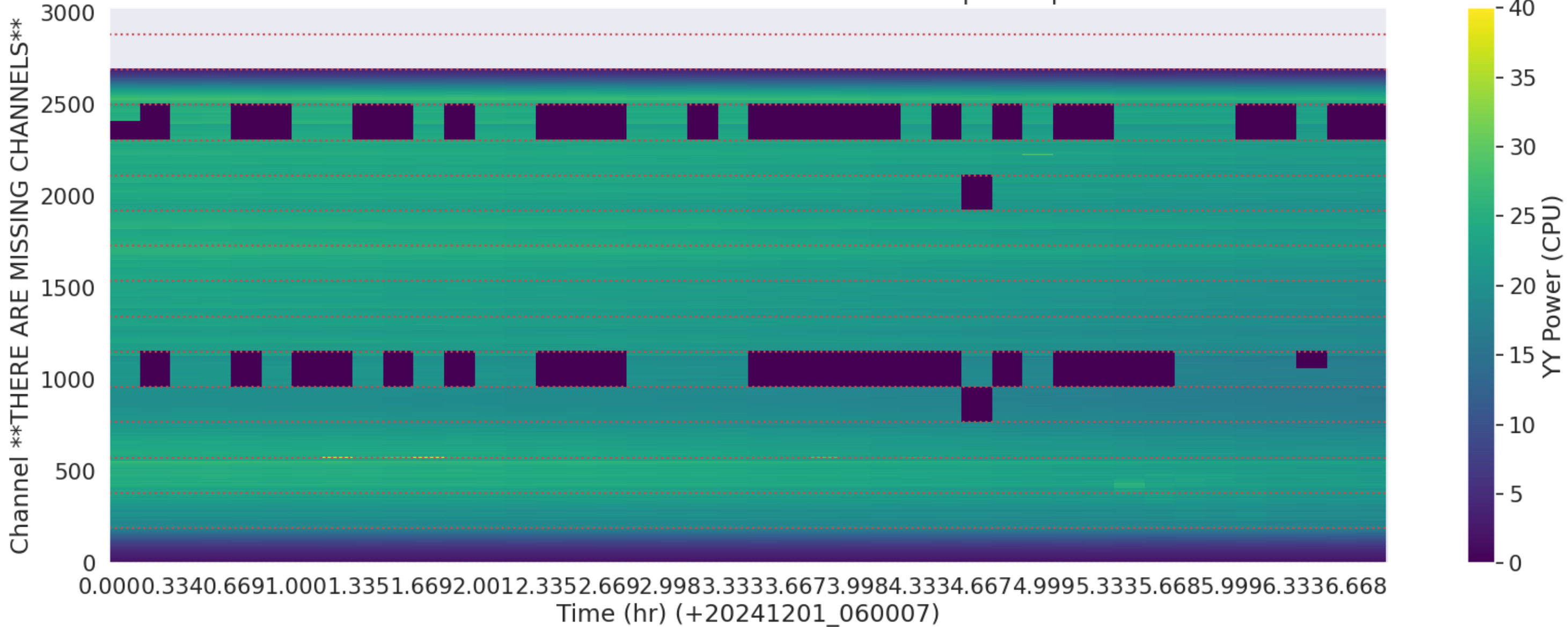
LWA254 - Correlator# 315 - YY - FLAGS: BadSpecShape
