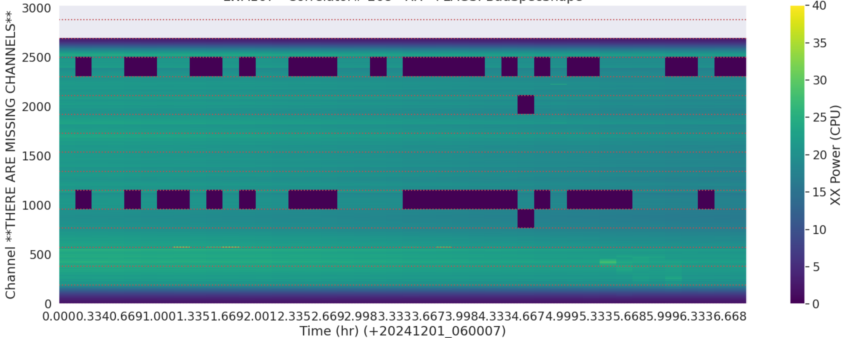
LWA167 - Correlator# 268 - XX - FLAGS: BadSpecShape
