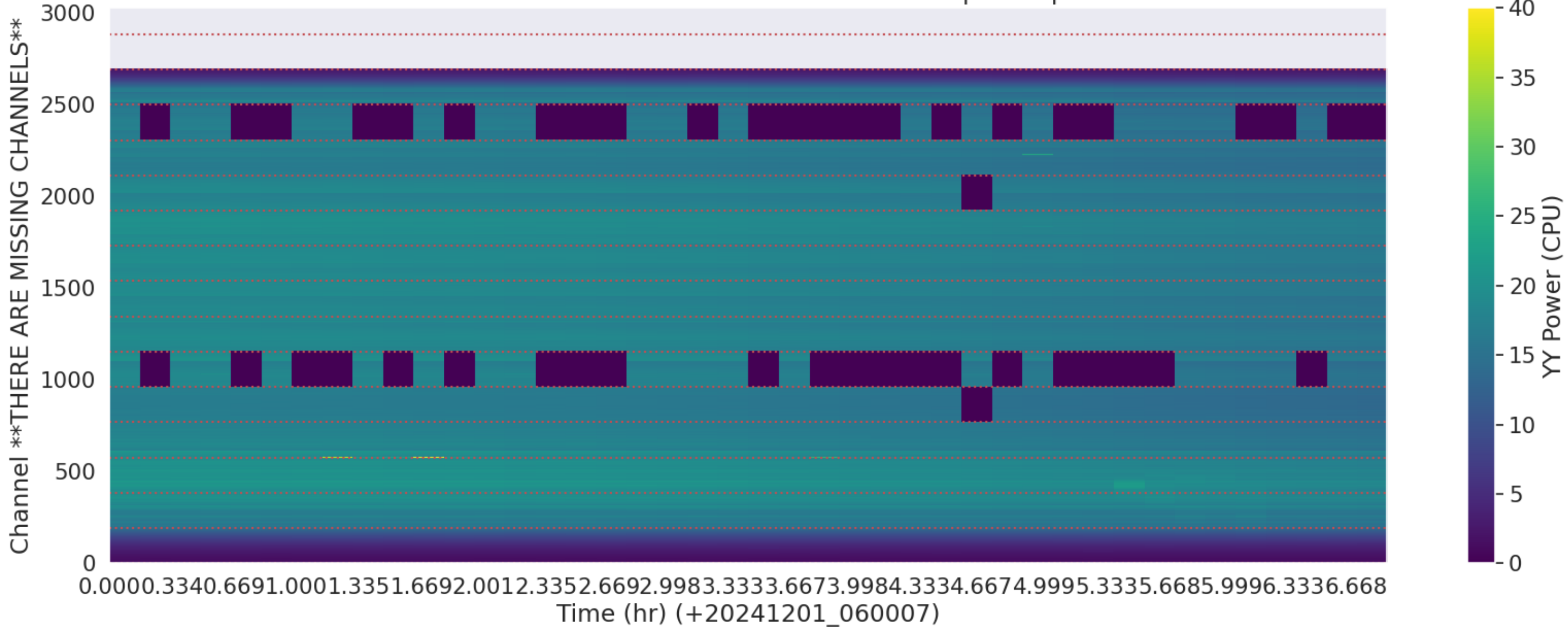
LWA157 - Correlator# 234 - YY - FLAGS: BadSpecShape
