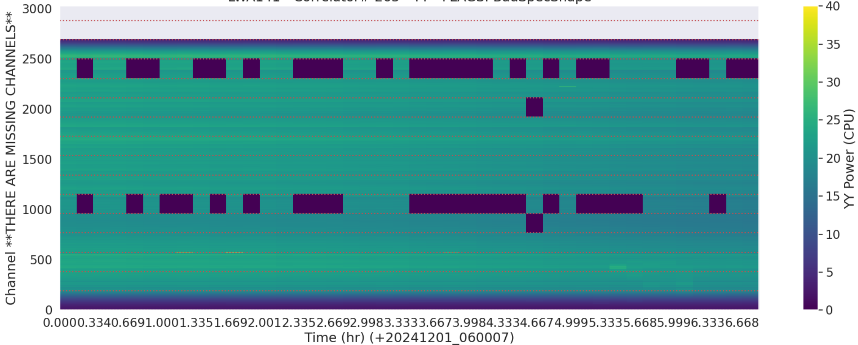
LWA141 - Correlator# 263 - YY - FLAGS: BadSpecShape
