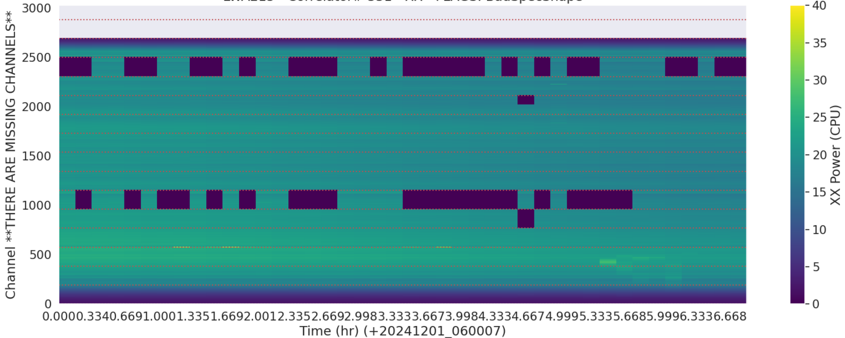
LWA215 - Correlator# 331 - XX - FLAGS: BadSpecShape
