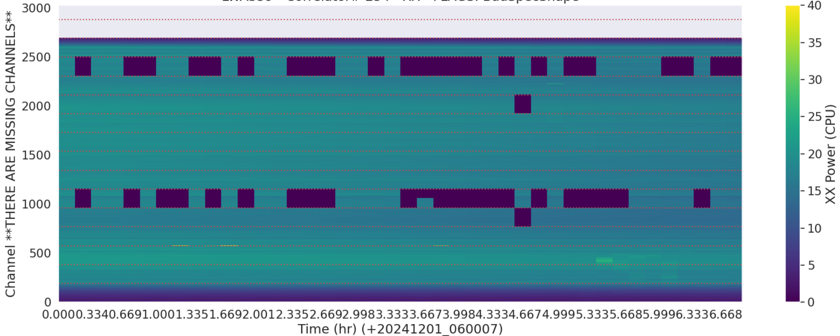
LWA359 - Correlator# 254 - XX - FLAGS: BadSpecShape
