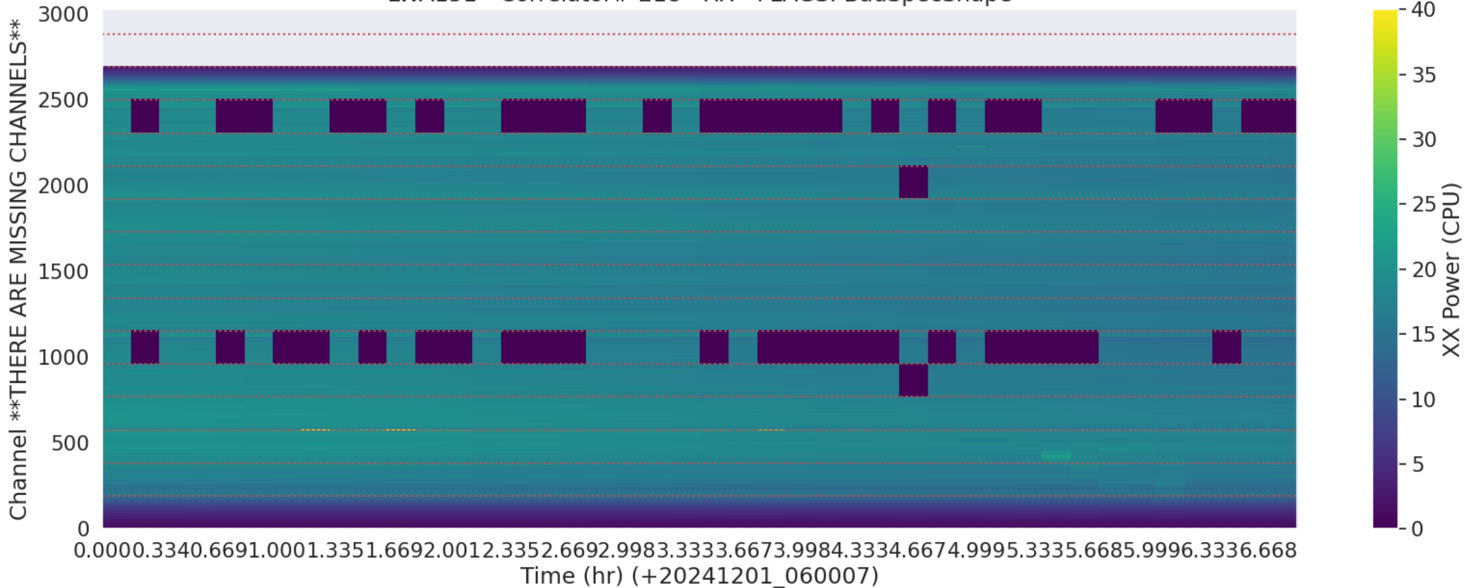
LWA151 - Correlator# 218 - XX - FLAGS: BadSpecShape
