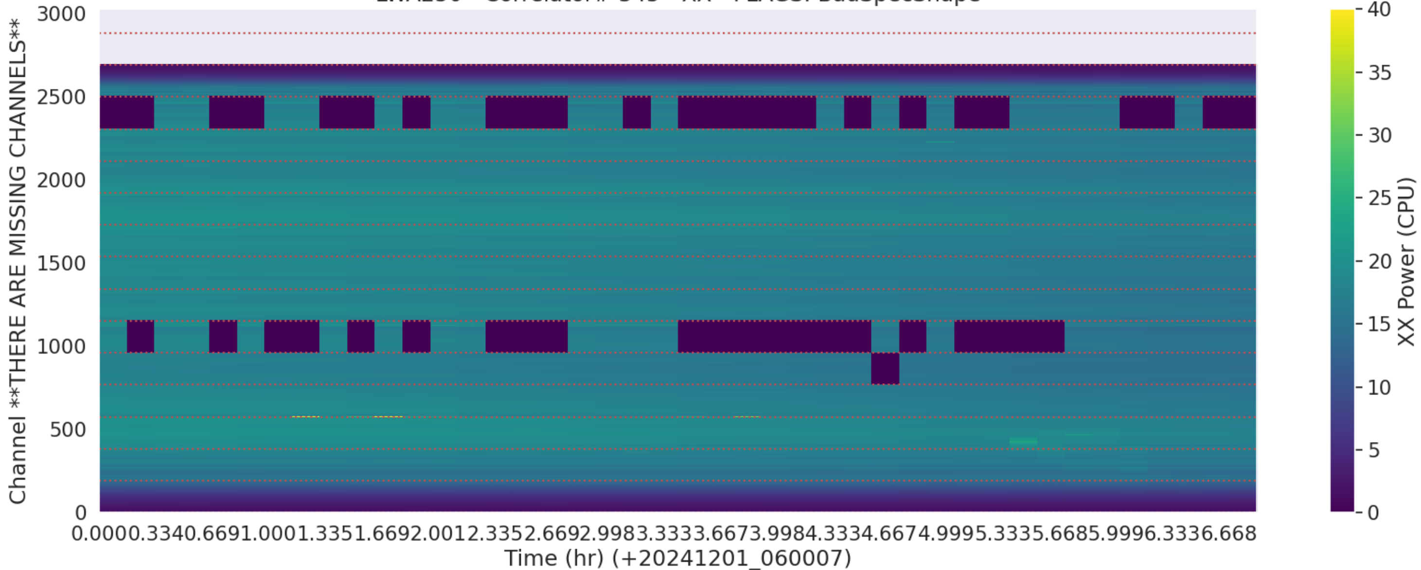
LWA250 - Correlator# 345 - XX - FLAGS: BadSpecShape
