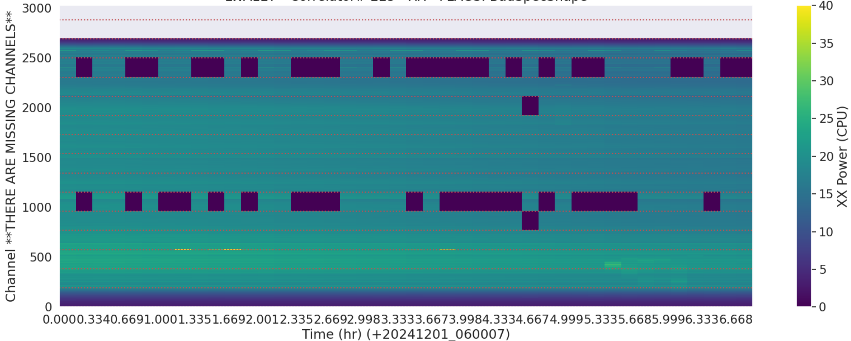
LWA127 - Correlator# 225 - XX - FLAGS: BadSpecShape
