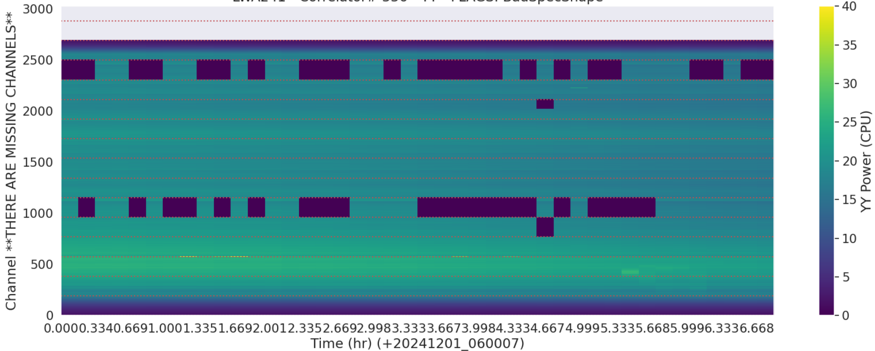
LWA241 - Correlator# 336 - YY - FLAGS: BadSpecShape
