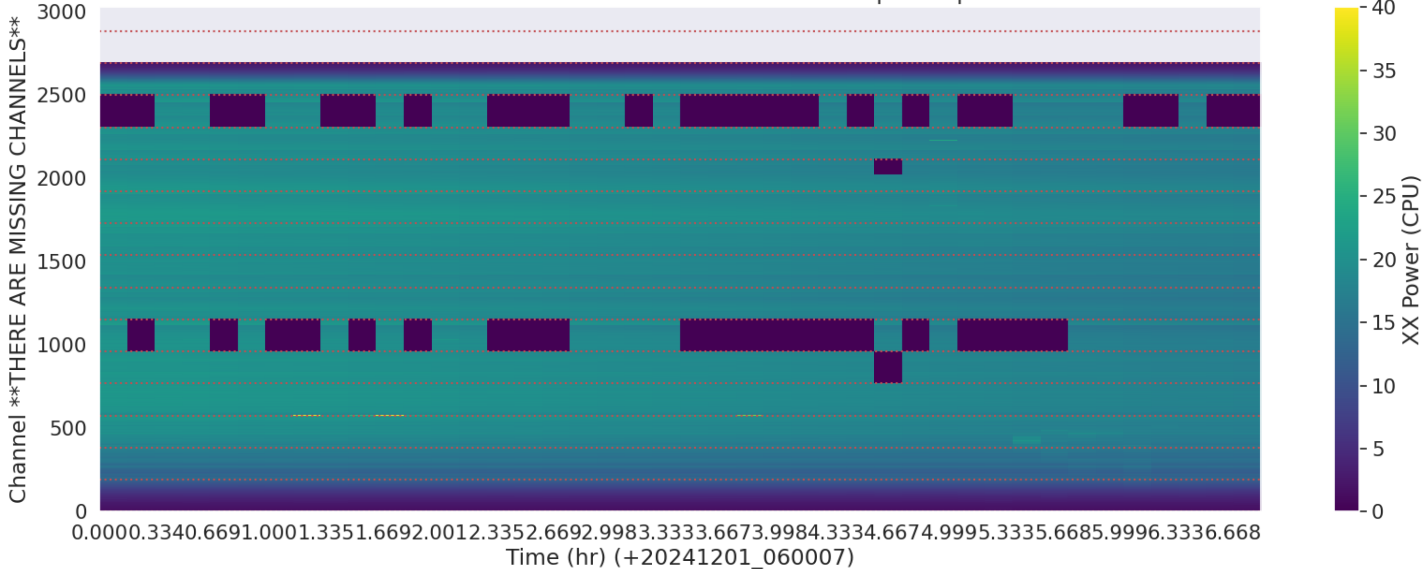
LWA219 - Correlator# 335 - XX - FLAGS: BadSpecShape
