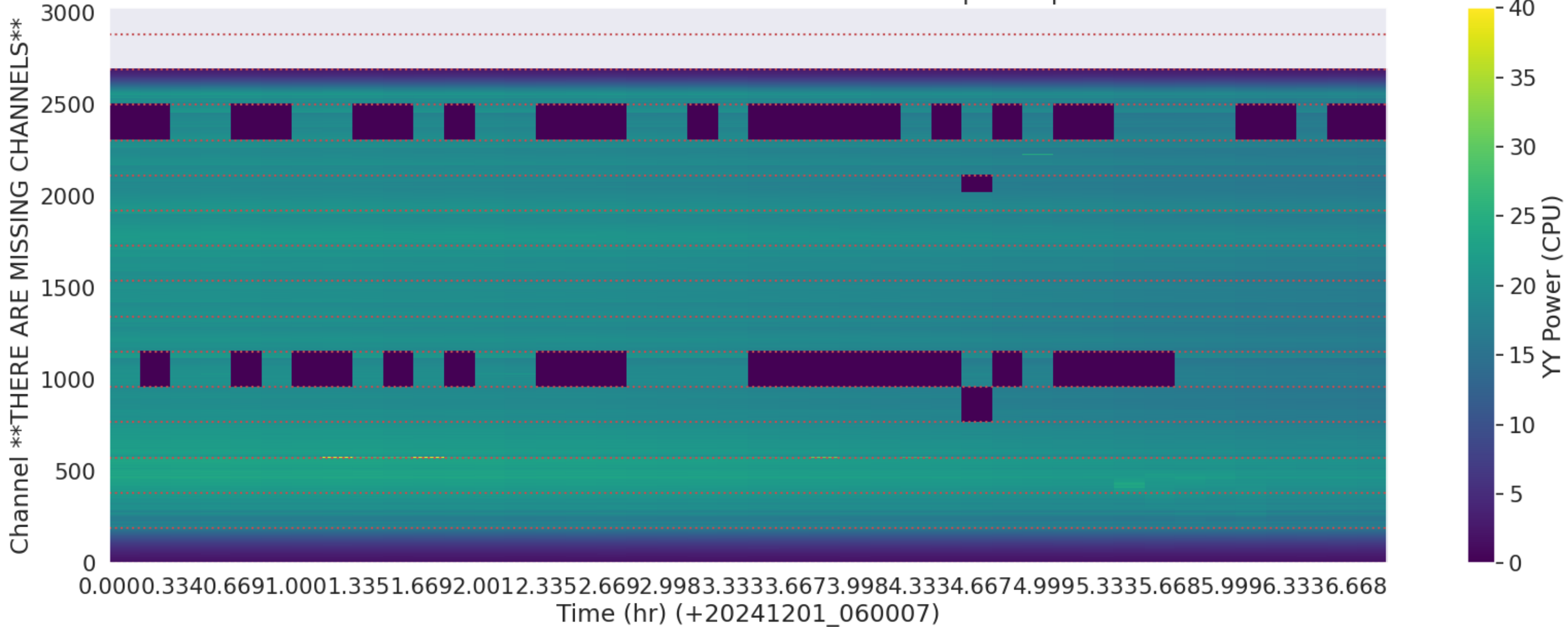
LWA213 - Correlator# 329 - YY - FLAGS: BadSpecShape
