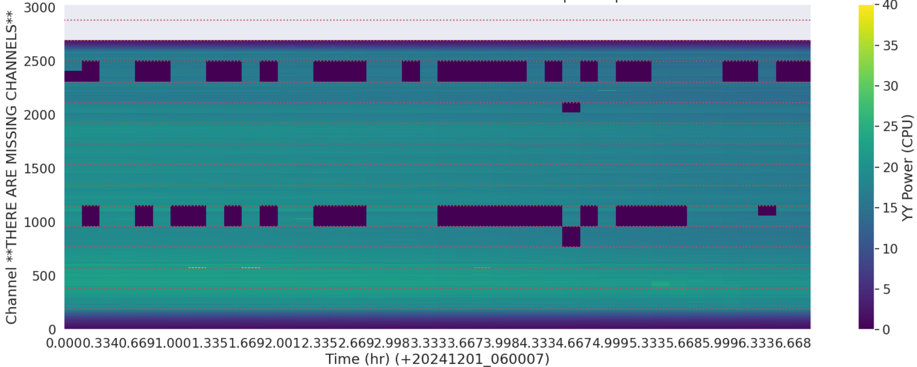
LWA183 - Correlator# 324 - YY - FLAGS: BadSpecShape
