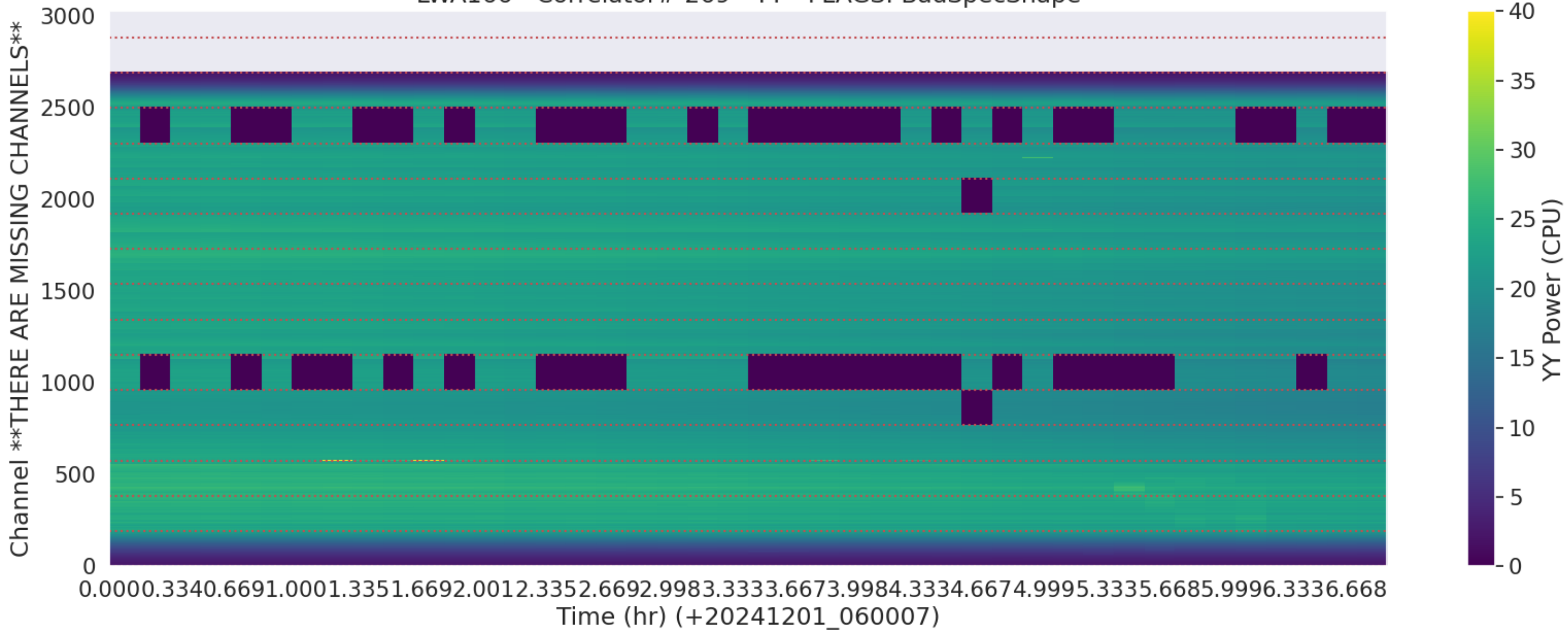
LWA166 - Correlator# 269 - YY - FLAGS: BadSpecShape
