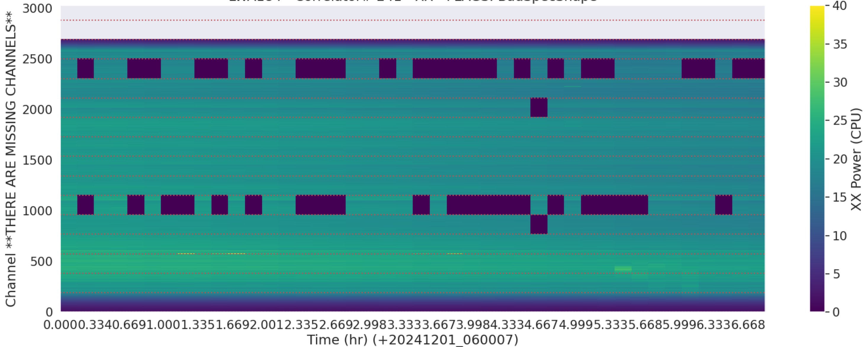
LWA184 - Correlator# 241 - XX - FLAGS: BadSpecShape
