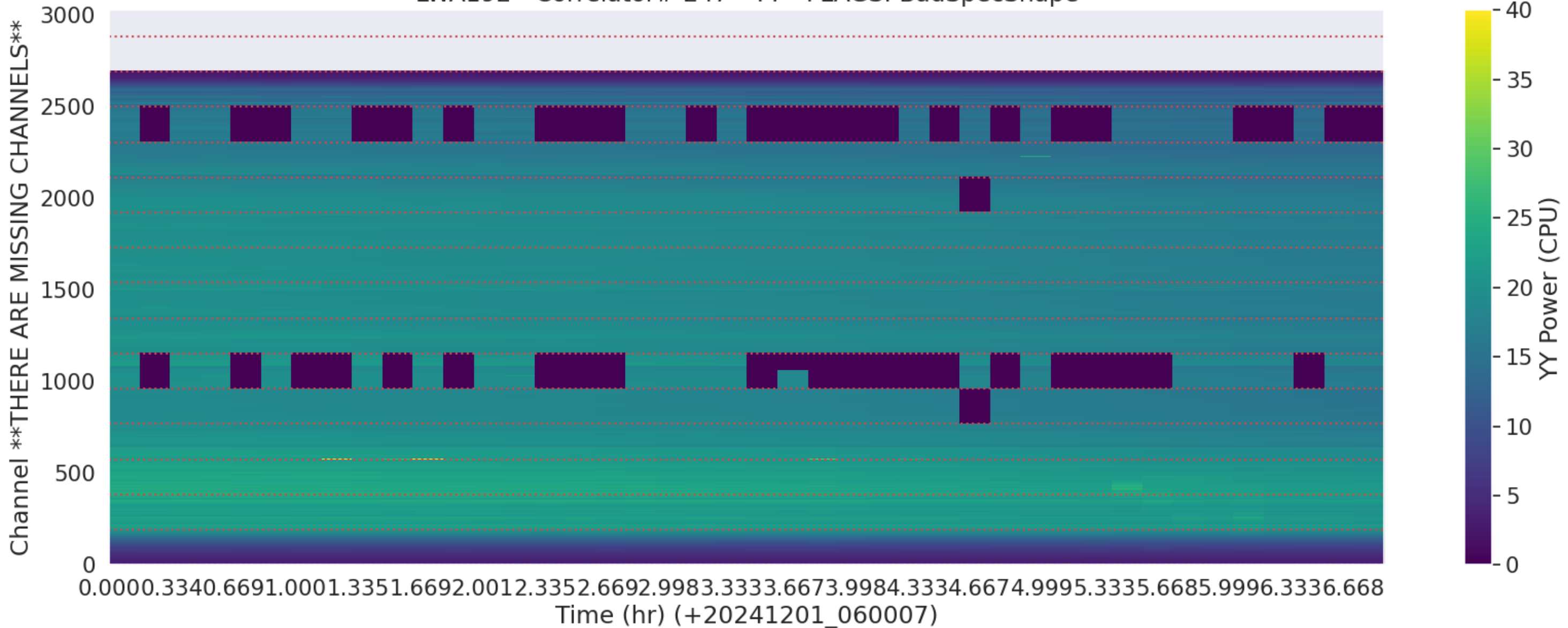
LWA192 - Correlator# 247 - YY - FLAGS: BadSpecShape
