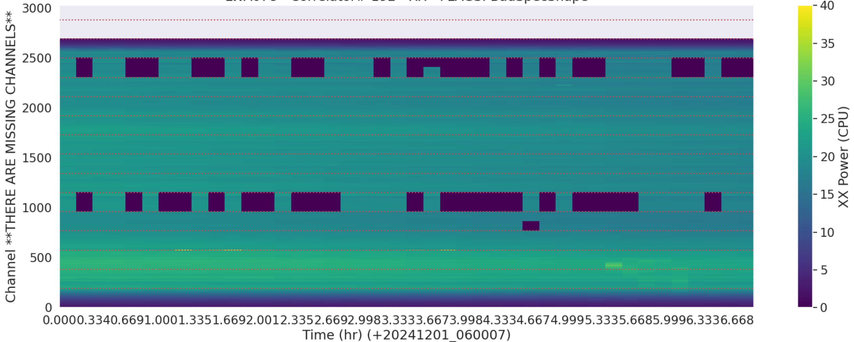
LWA078 - Correlator# 192 - XX - FLAGS: BadSpecShape
