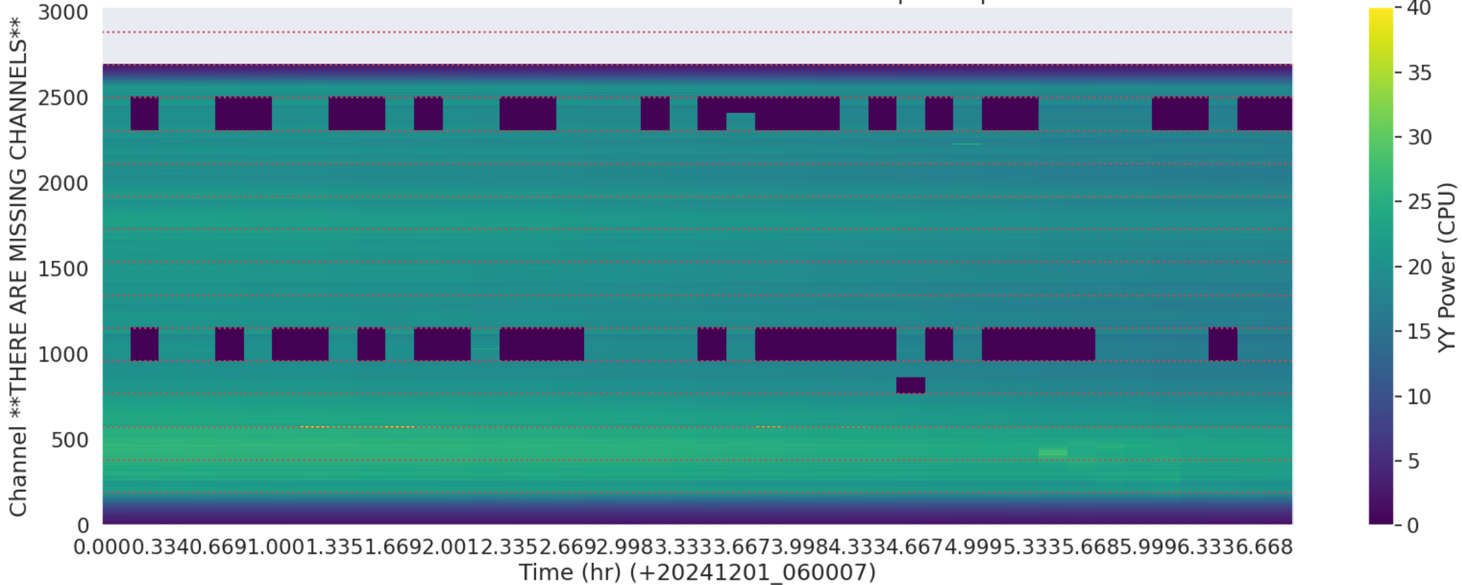
LWA076 - Correlator# 193 - YY - FLAGS: BadSpecShape
