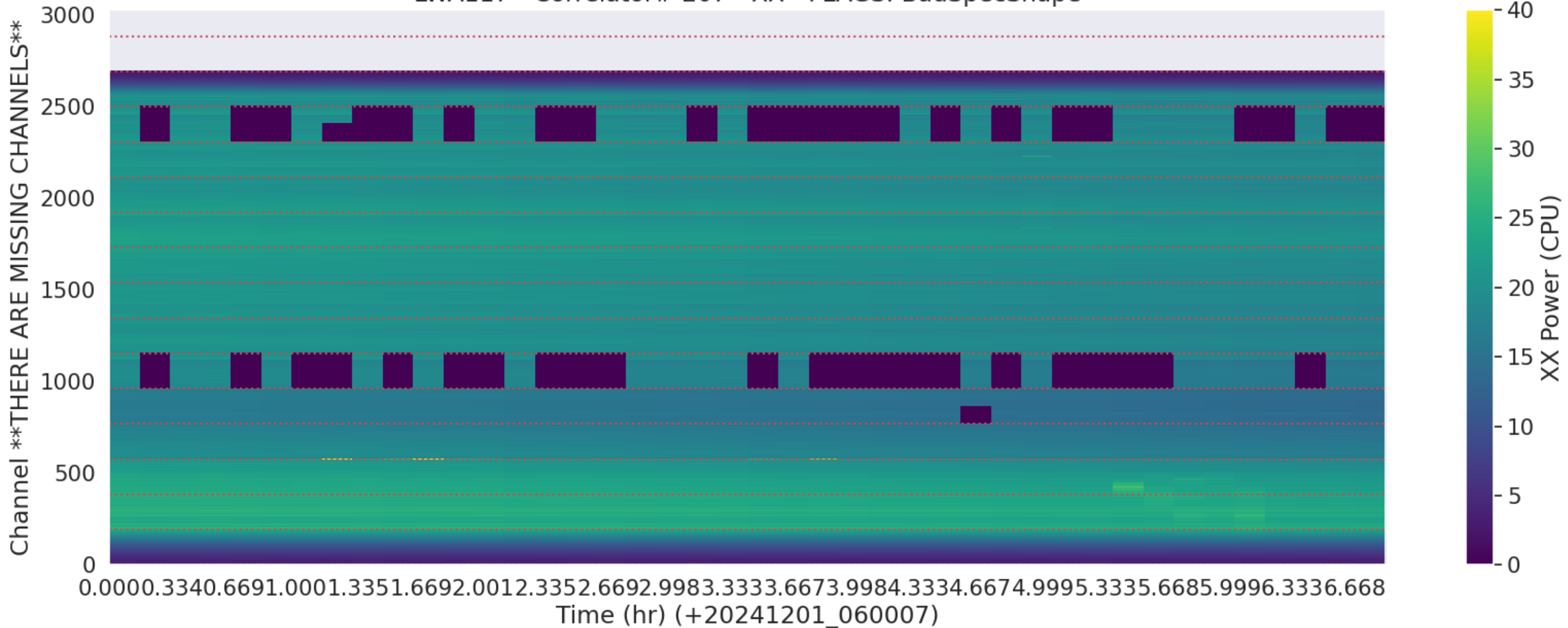
LWA117 - Correlator# 207 - XX - FLAGS: BadSpecShape
