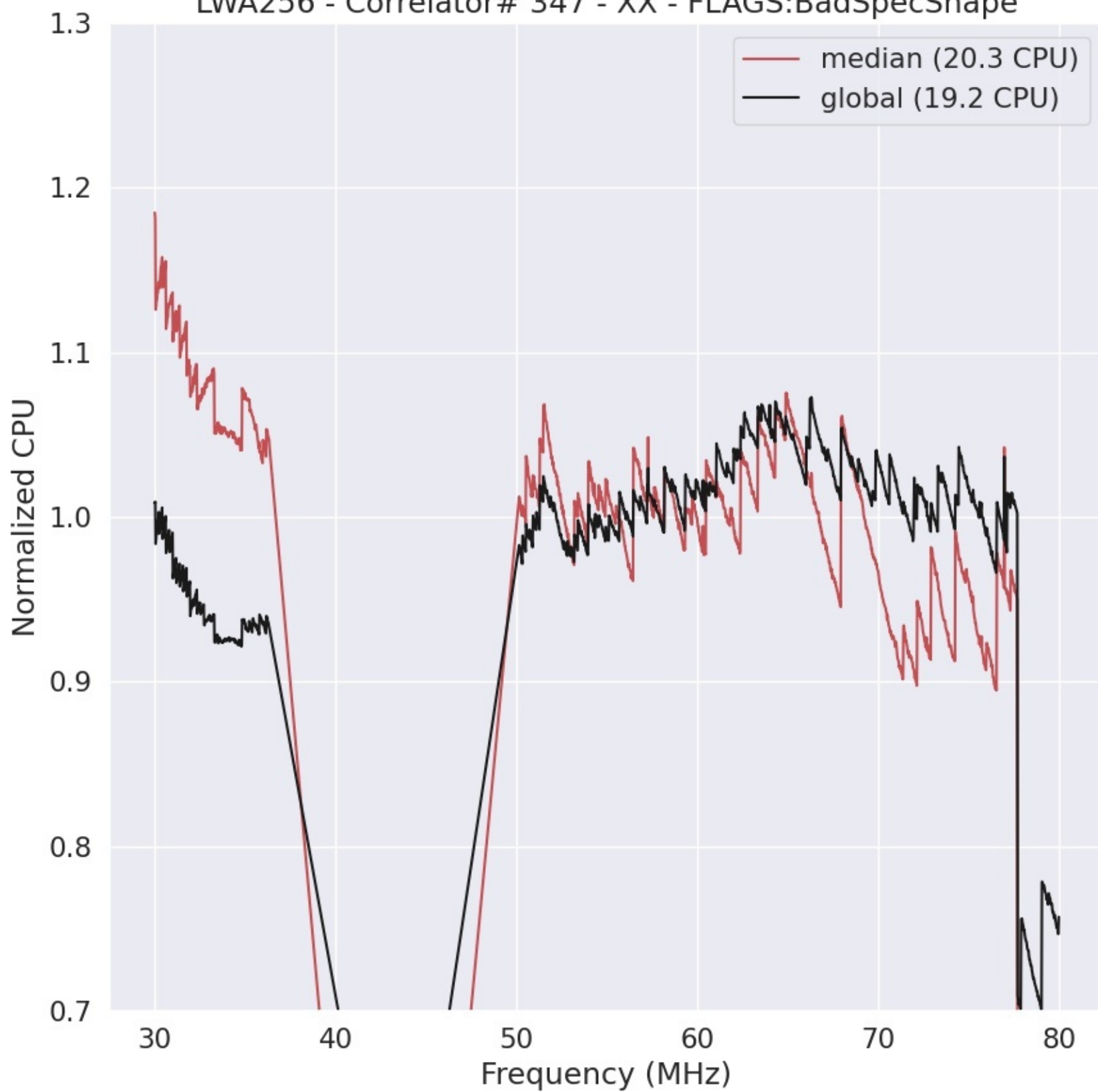
LWA256 - Correlator# 347 - XX - FLAGS:BadSpecShape
