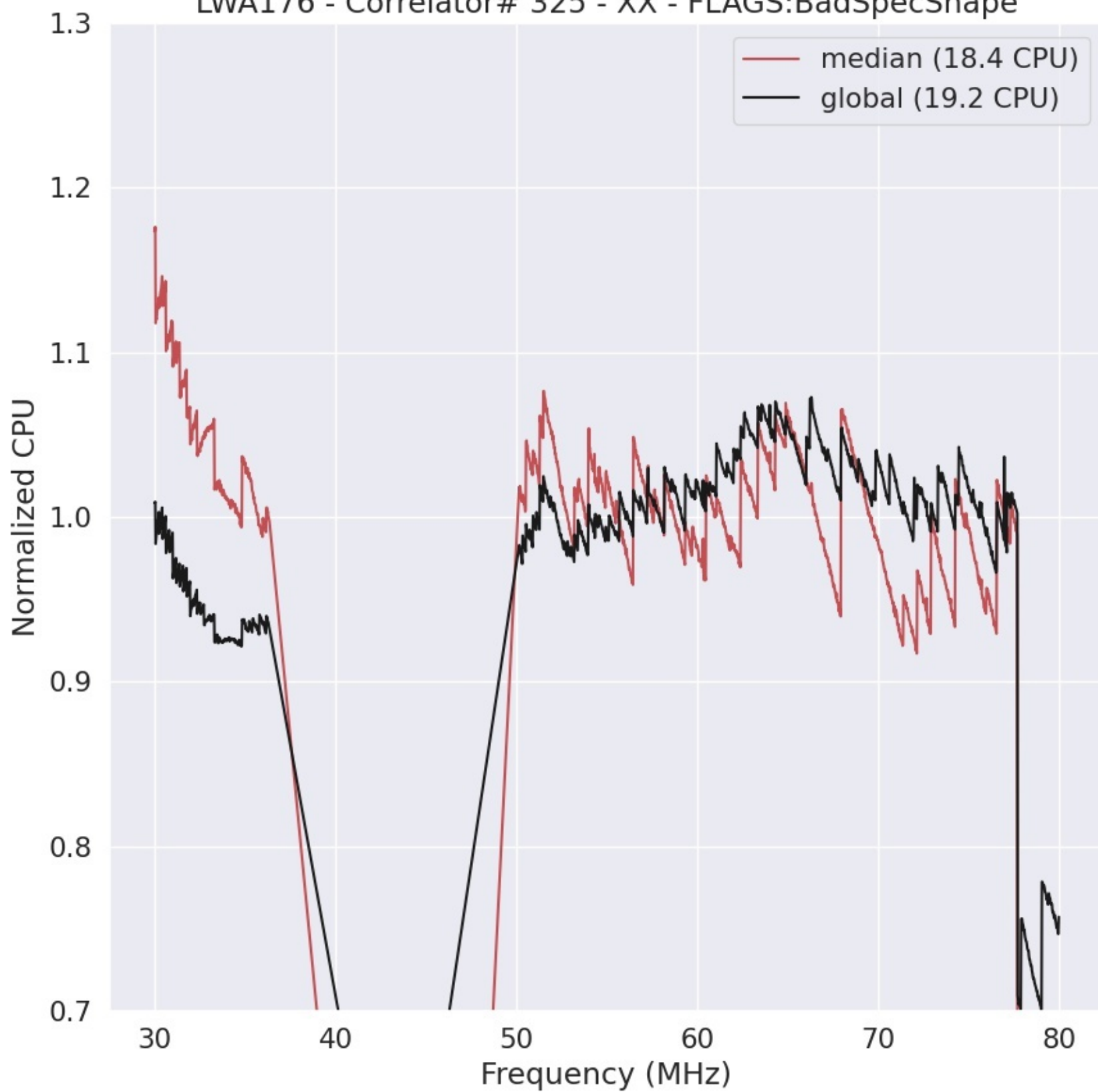
LWA176 - Correlator# 325 - XX - FLAGS:BadSpecShape
