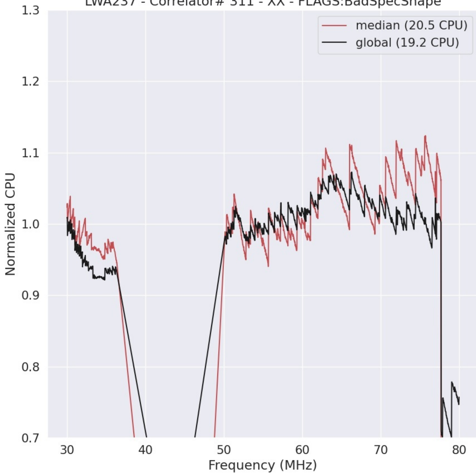
LWA237 - Correlator# 311 - XX - FLAGS:BadSpecShape
