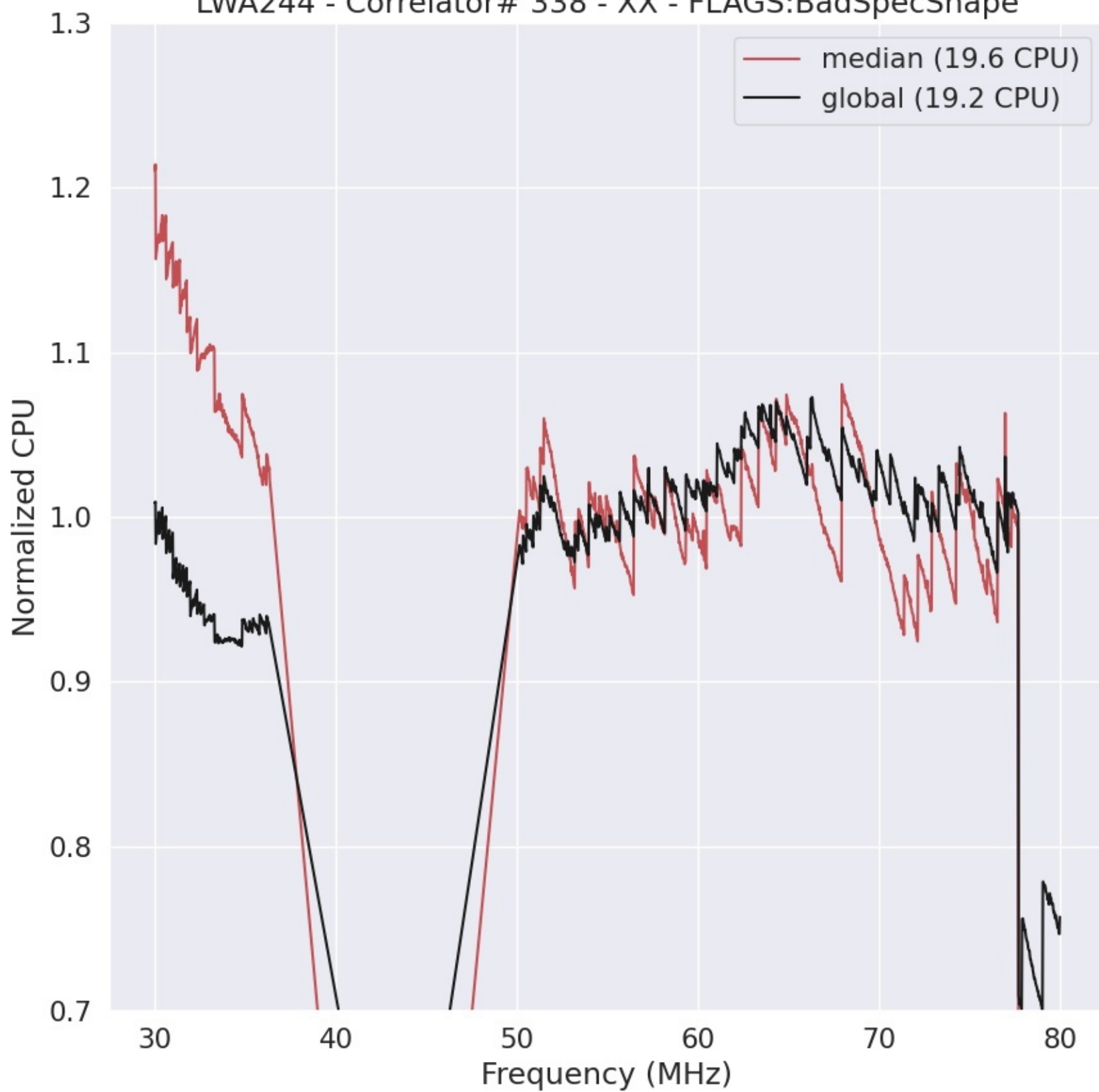
LWA244 - Correlator# 338 - XX - FLAGS:BadSpecShape
