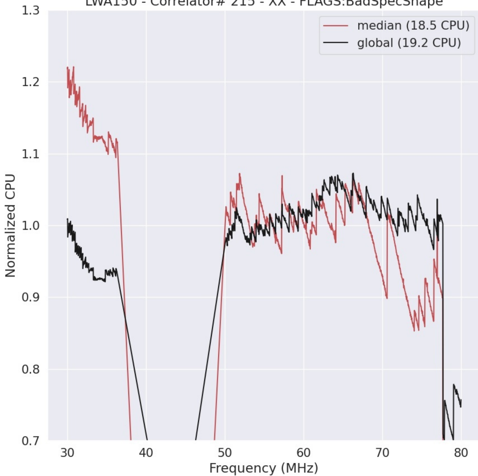
LWA150 - Correlator# 215 - XX - FLAGS:BadSpecShape
