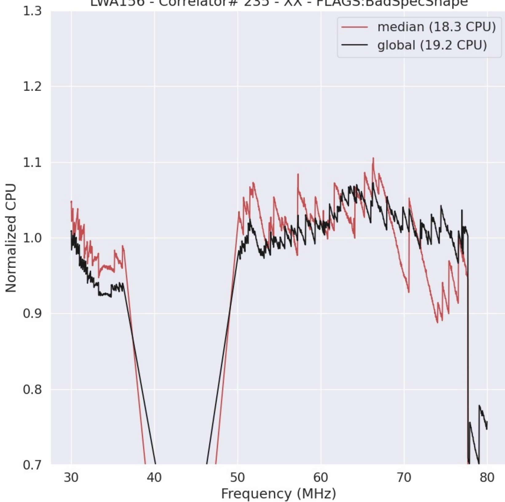
LWA156 - Correlator# 235 - XX - FLAGS:BadSpecShape
