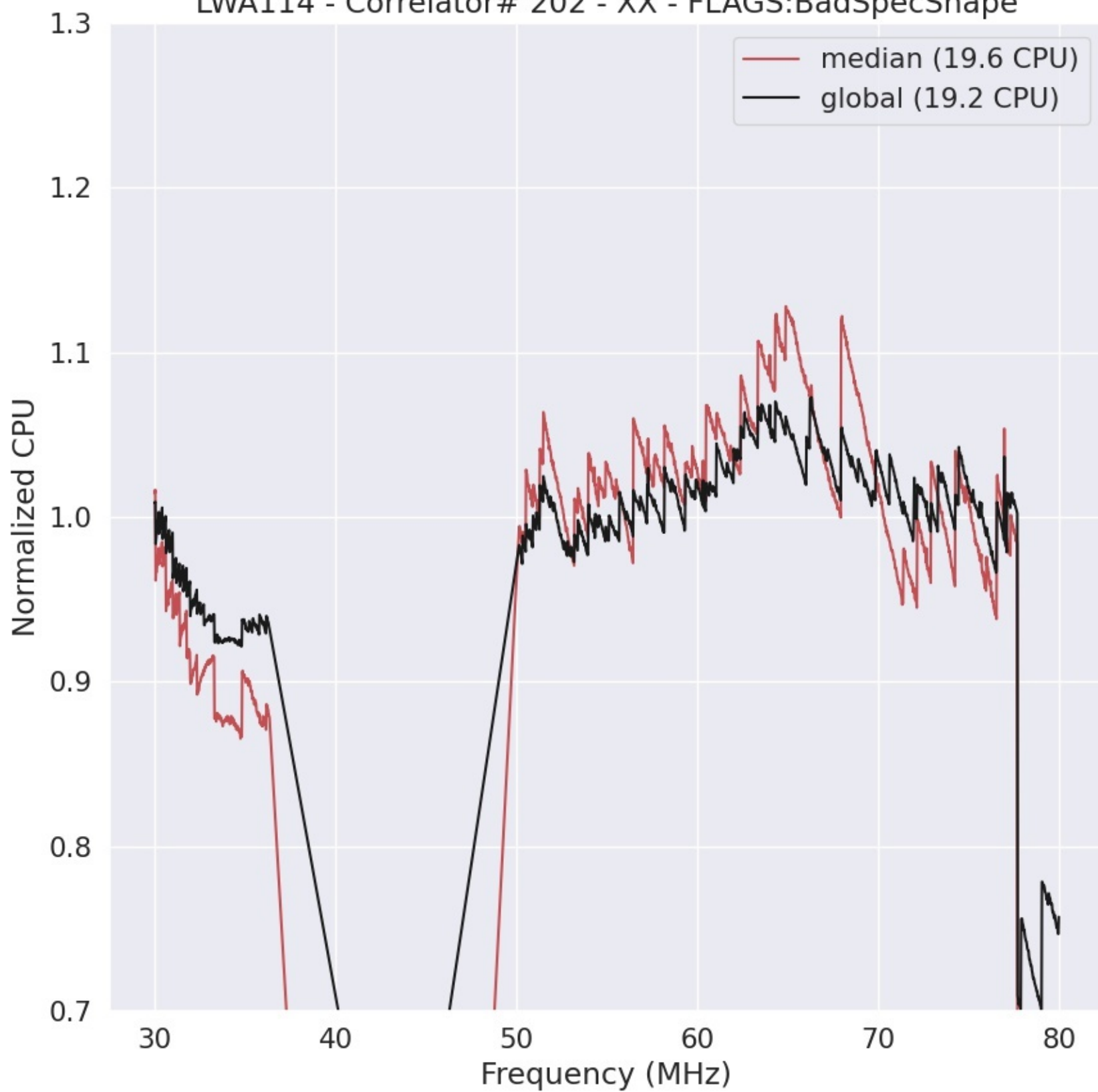
LWA114 - Correlator# 202 - XX - FLAGS:BadSpecShape
