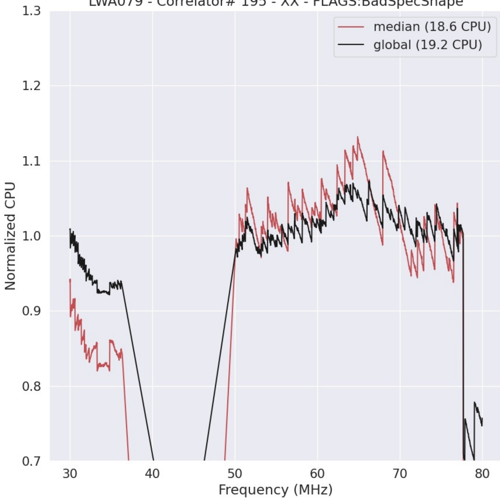
LWA079 - Correlator# 195 - XX - FLAGS:BadSpecShape
