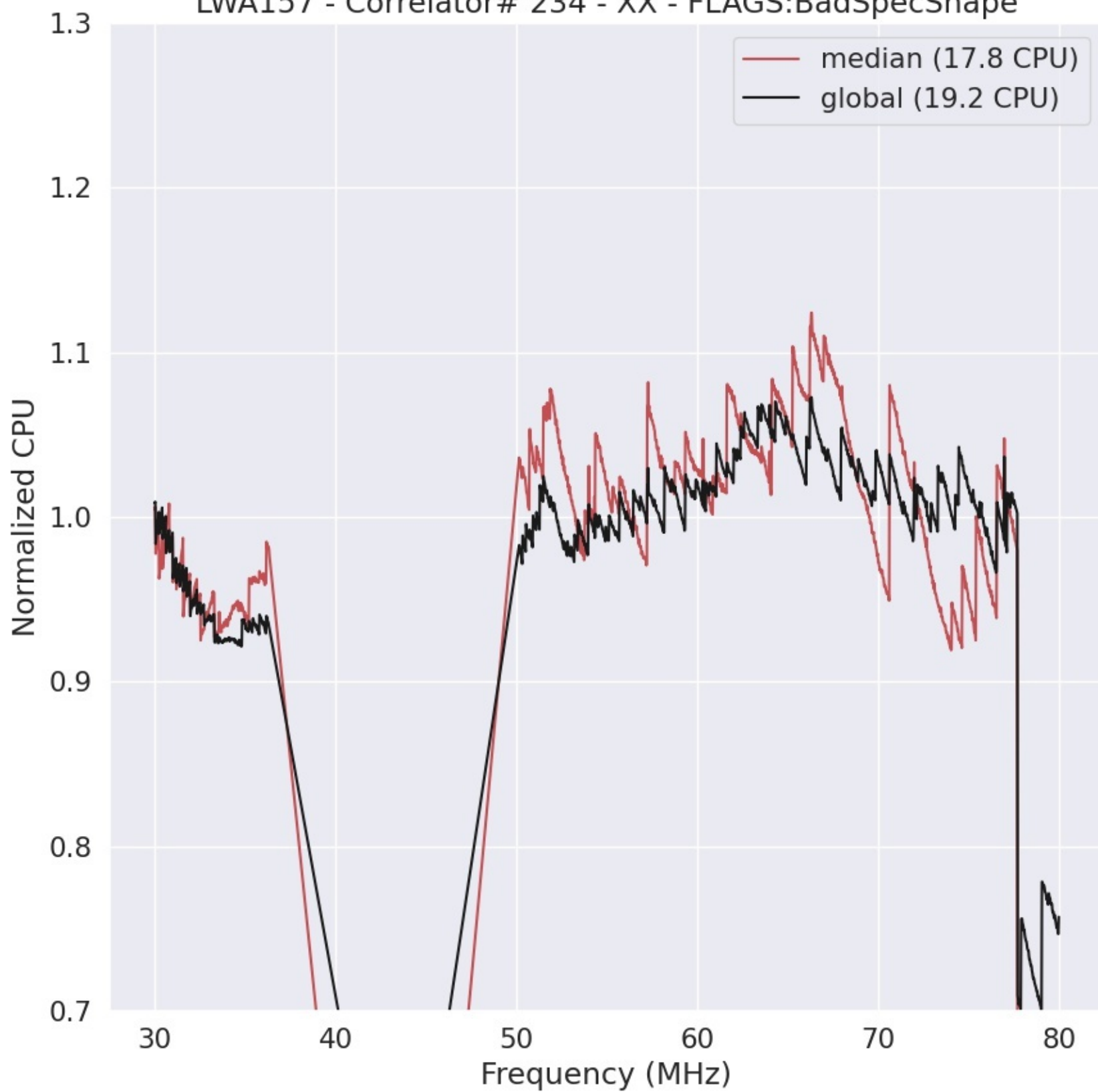
LWA157 - Correlator# 234 - XX - FLAGS:BadSpecShape
