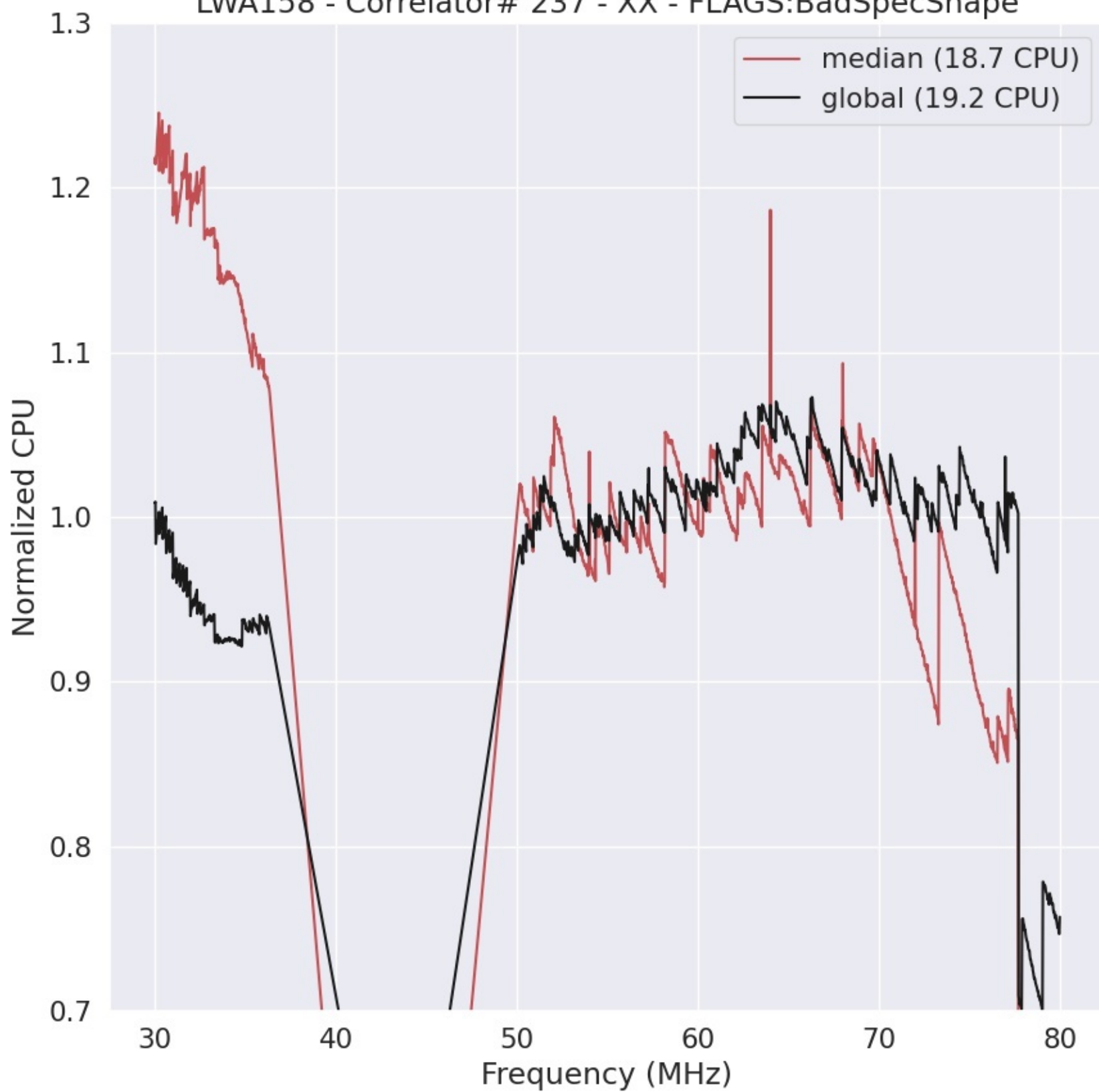
LWA158 - Correlator# 237 - XX - FLAGS:BadSpecShape
