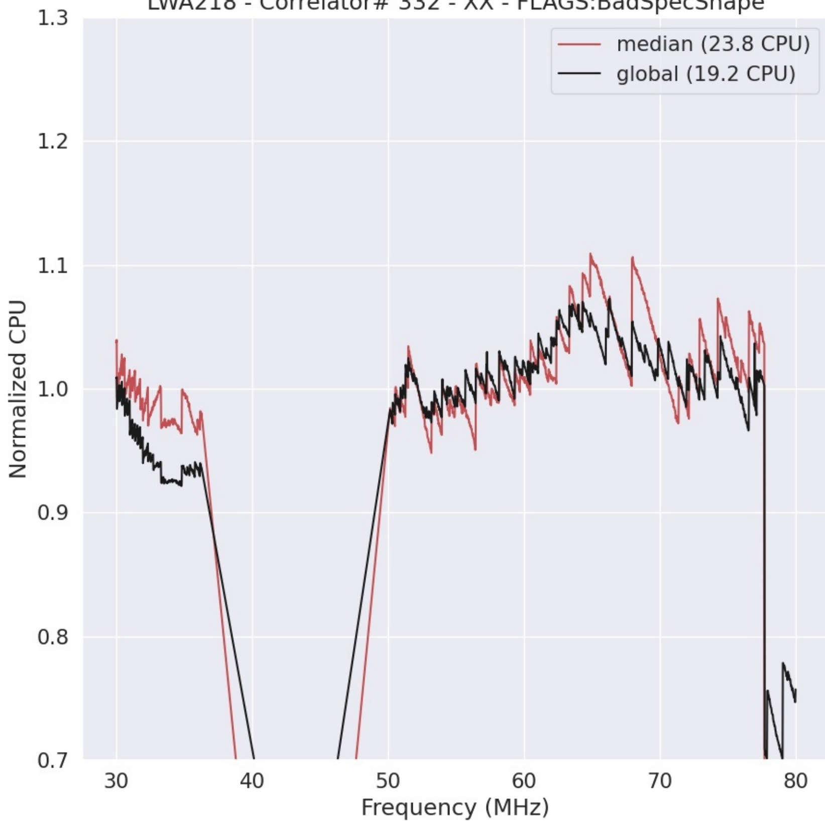
LWA218 - Correlator# 332 - XX - FLAGS:BadSpecShape
