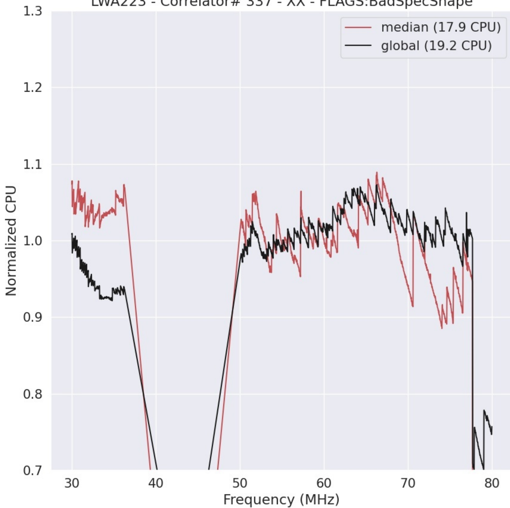
LWA223 - Correlator# 337 - XX - FLAGS:BadSpecShape
