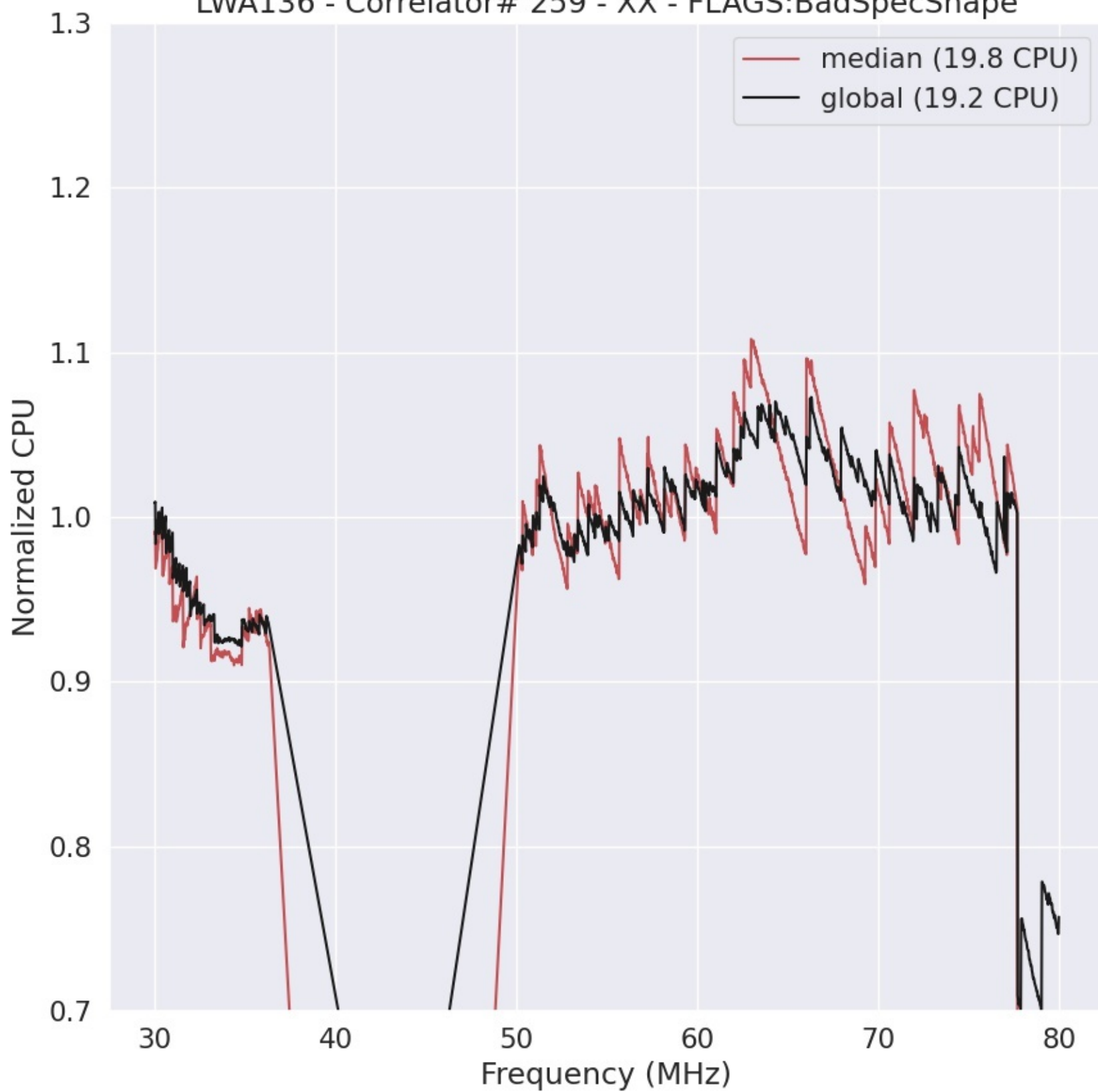
LWA136 - Correlator# 259 - XX - FLAGS:BadSpecShape
