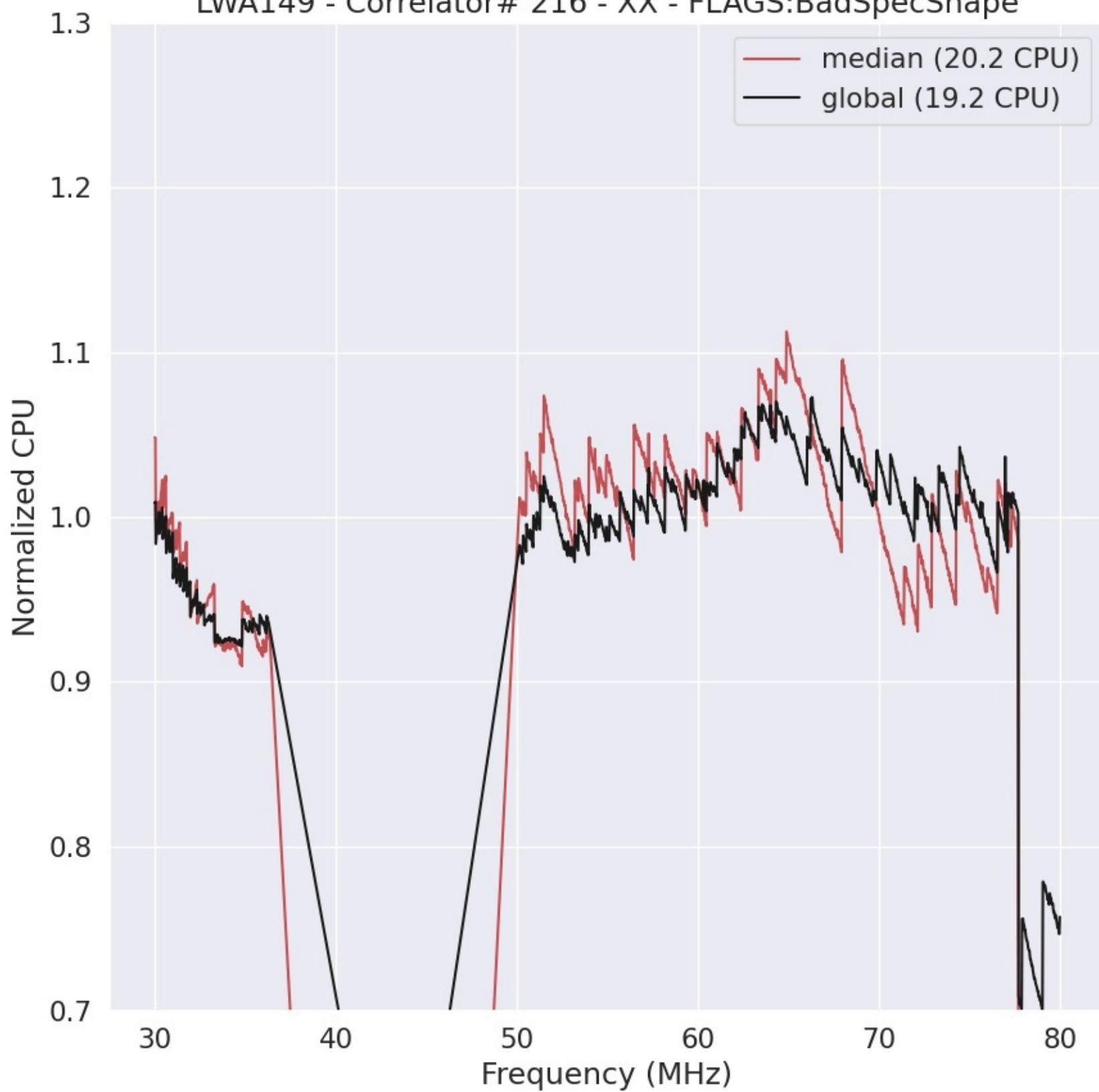
LWA149 - Correlator# 216 - XX - FLAGS:BadSpecShape
