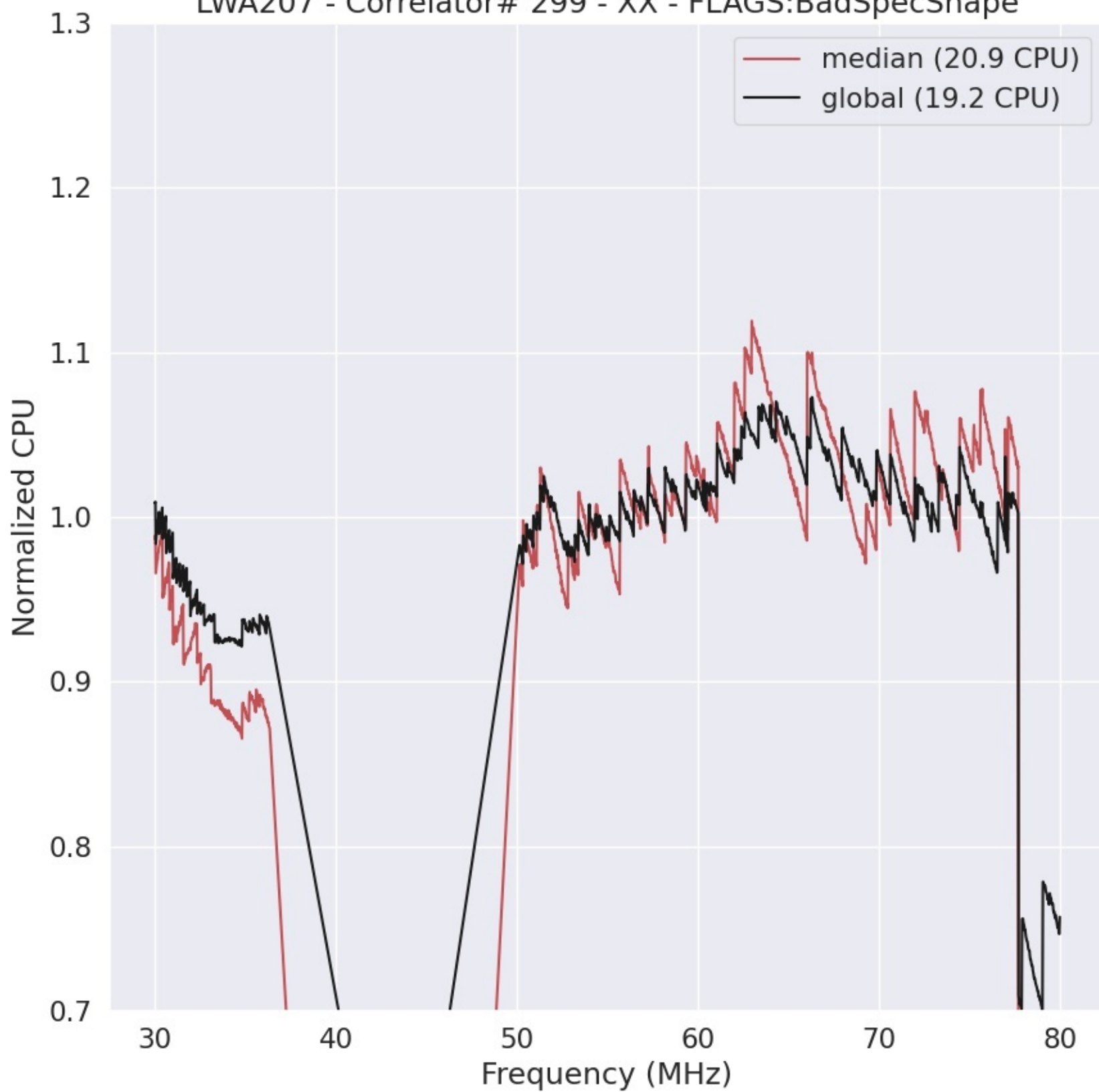
LWA207 - Correlator# 299 - XX - FLAGS:BadSpecShape
