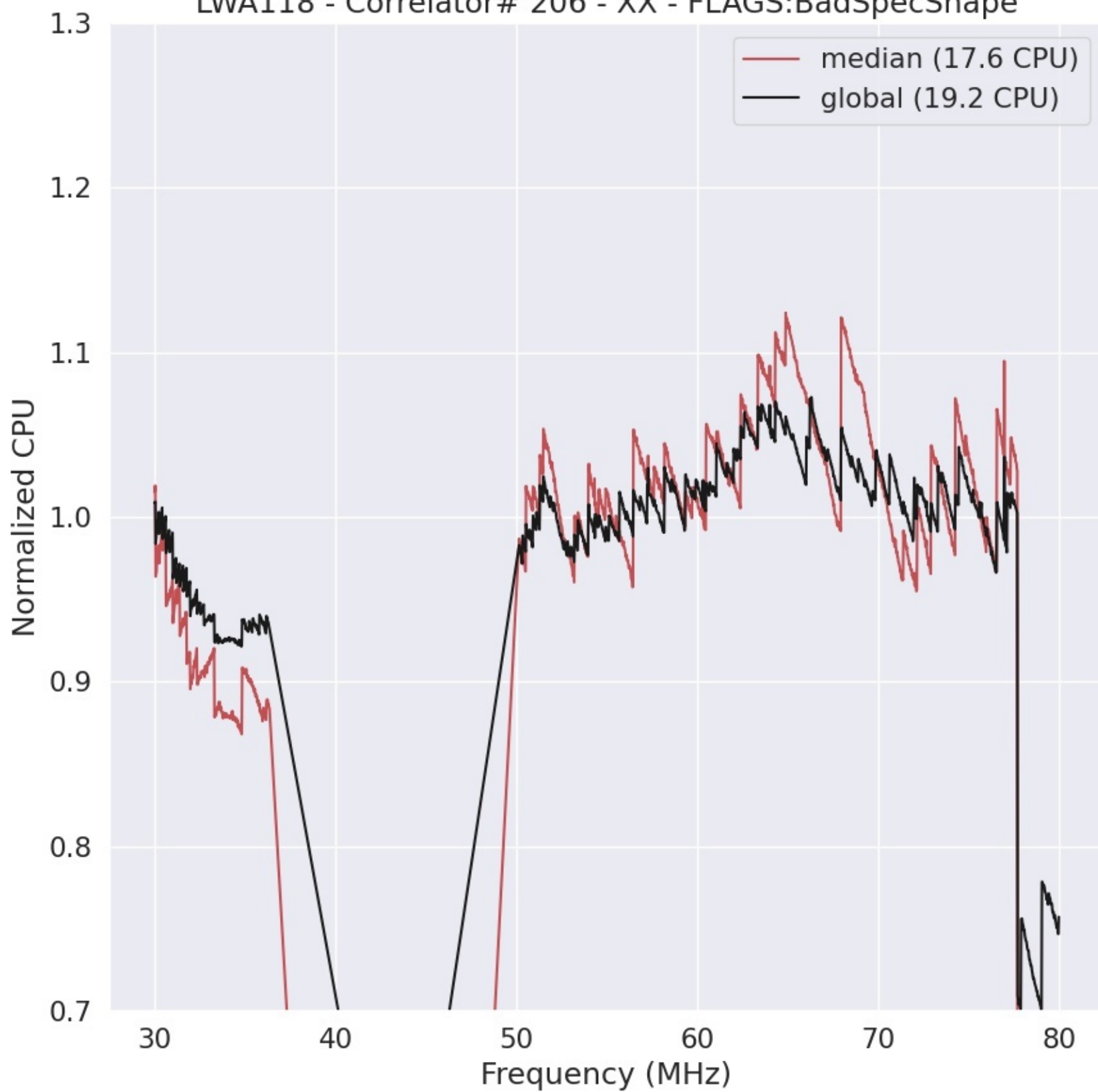
LWA118 - Correlator# 206 - XX - FLAGS:BadSpecShape
