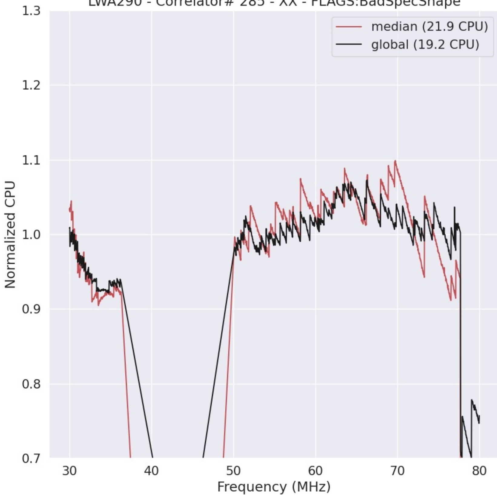
LWA290 - Correlator# 285 - XX - FLAGS:BadSpecShape
