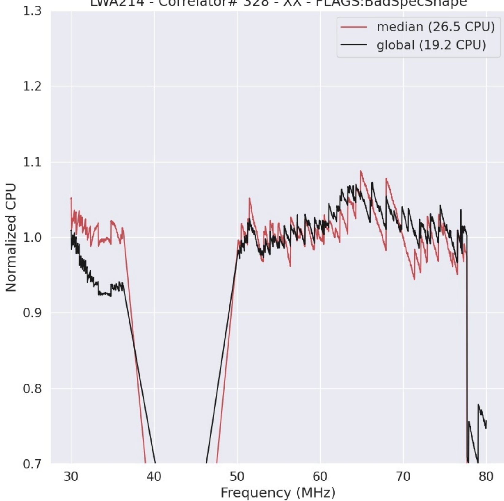
LWA214 - Correlator# 328 - XX - FLAGS:BadSpecShape
