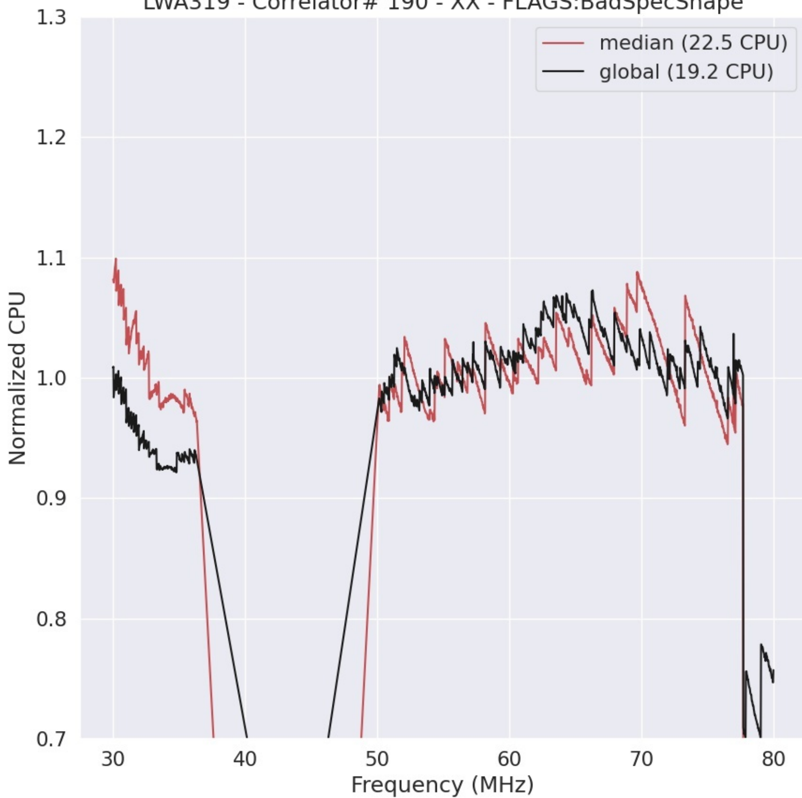
LWA319 - Correlator# 190 - XX - FLAGS:BadSpecShape
