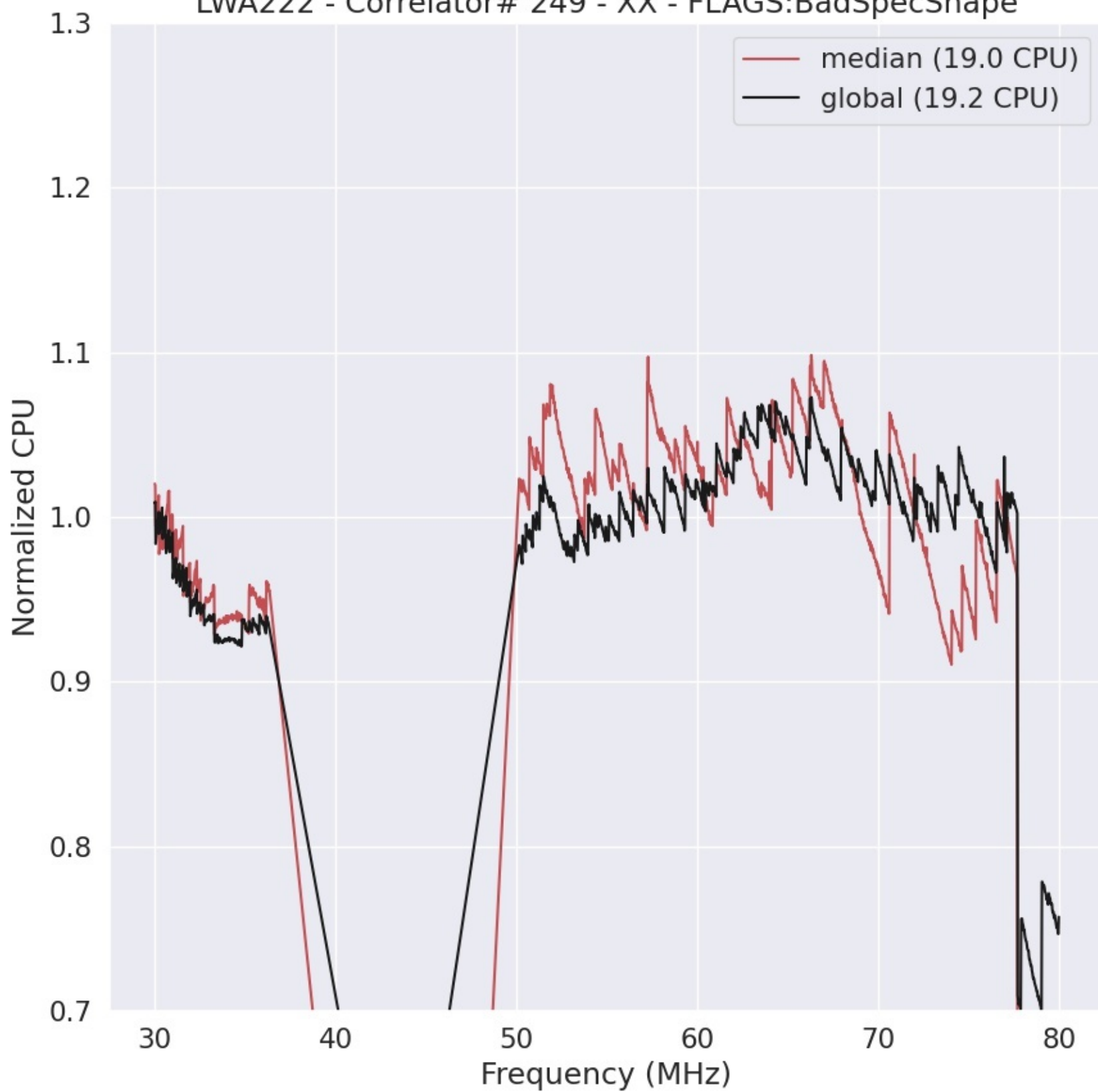
LWA222 - Correlator# 249 - XX - FLAGS:BadSpecShape
