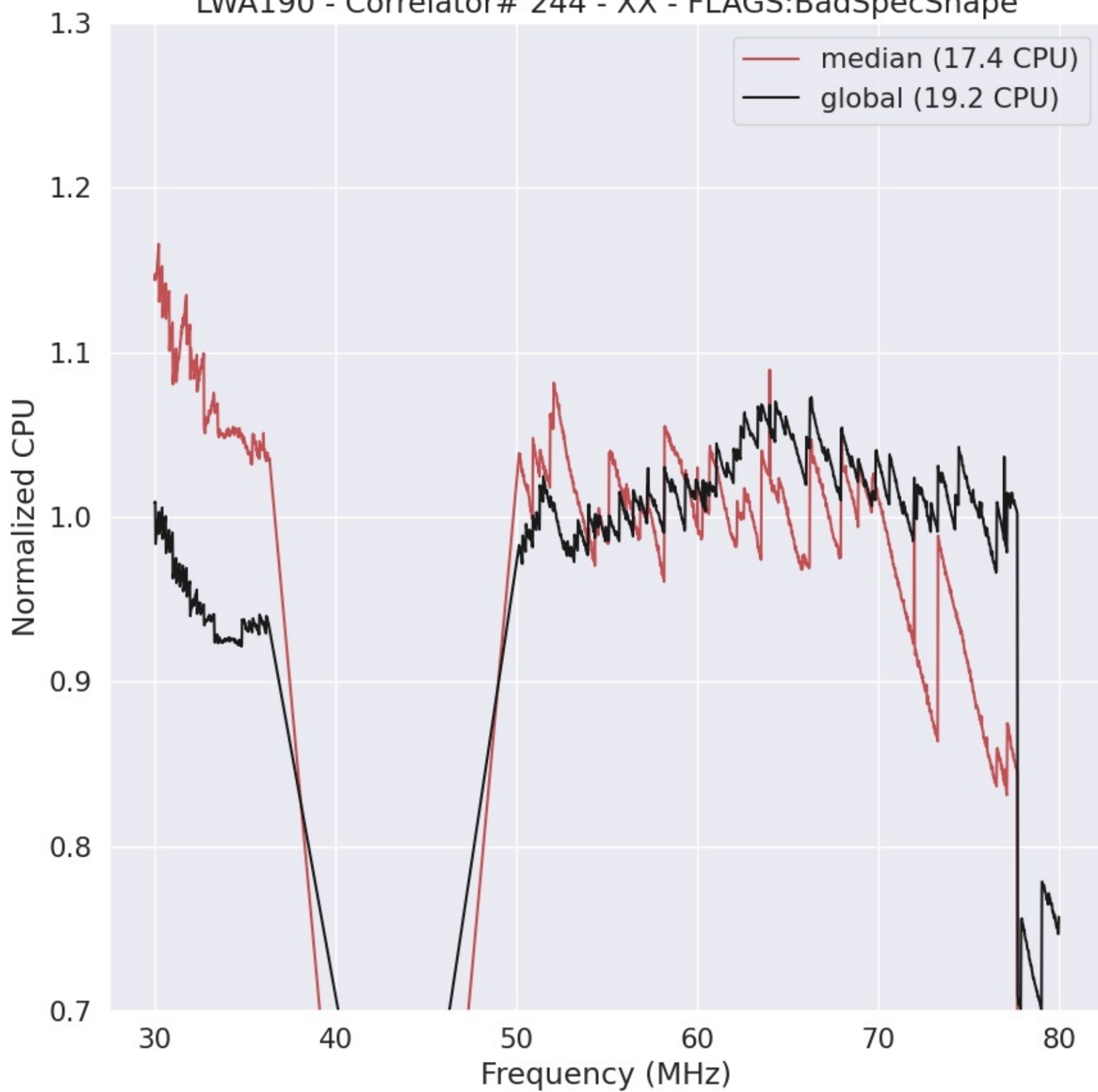
LWA190 - Correlator# 244 - XX - FLAGS:BadSpecShape
