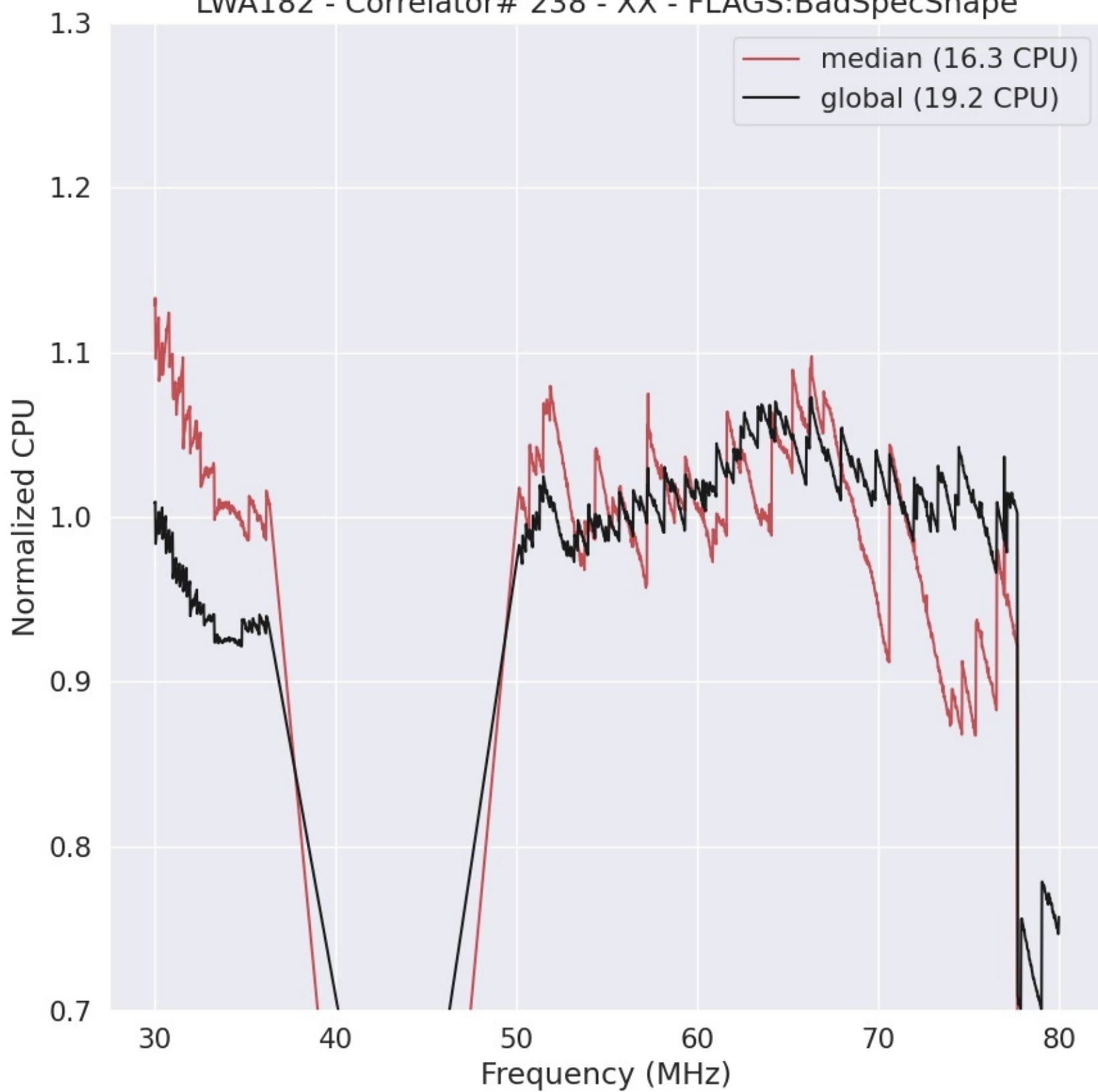
LWA182 - Correlator# 238 - XX - FLAGS:BadSpecShape
