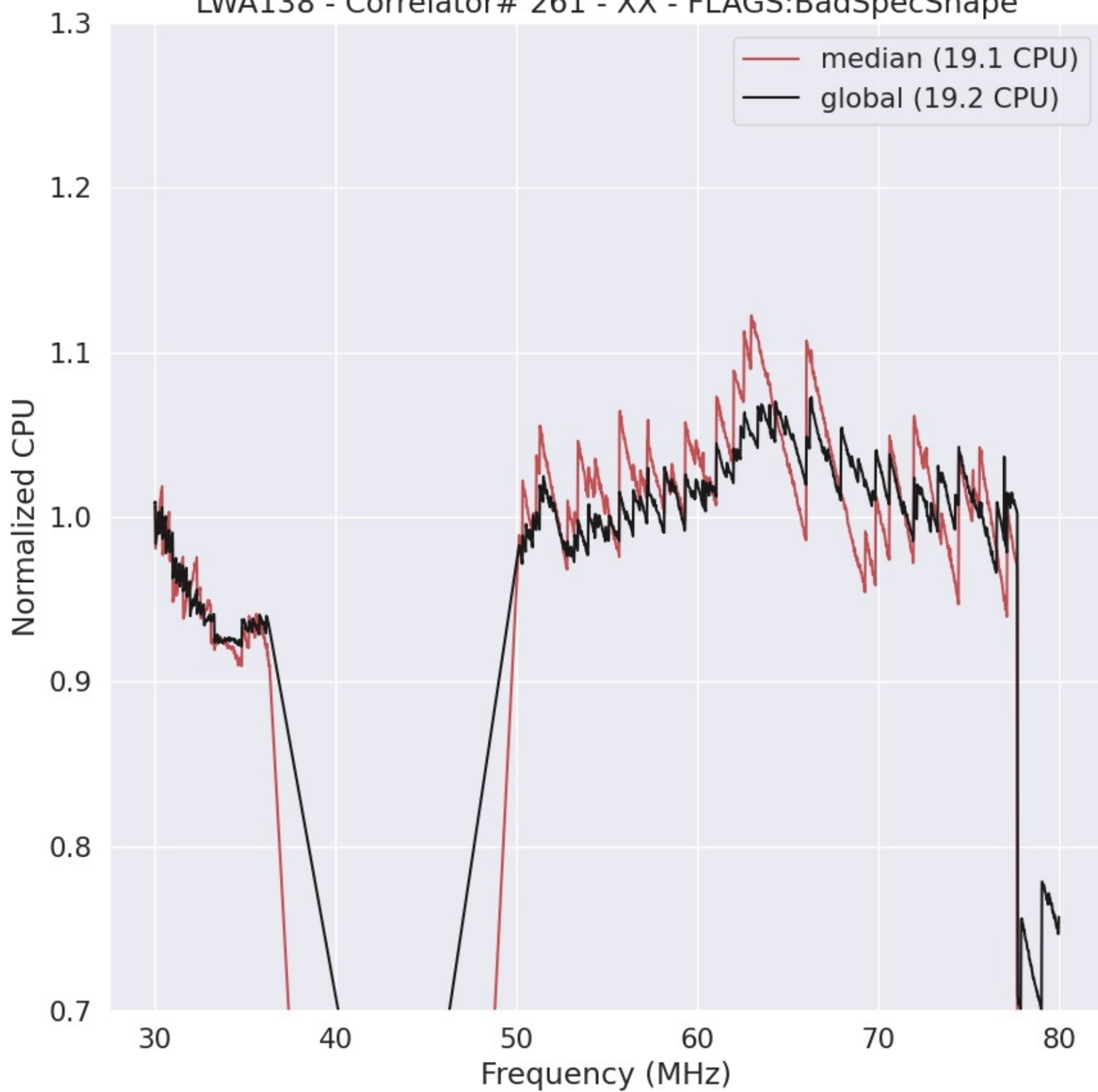
LWA138 - Correlator# 261 - XX - FLAGS:BadSpecShape
