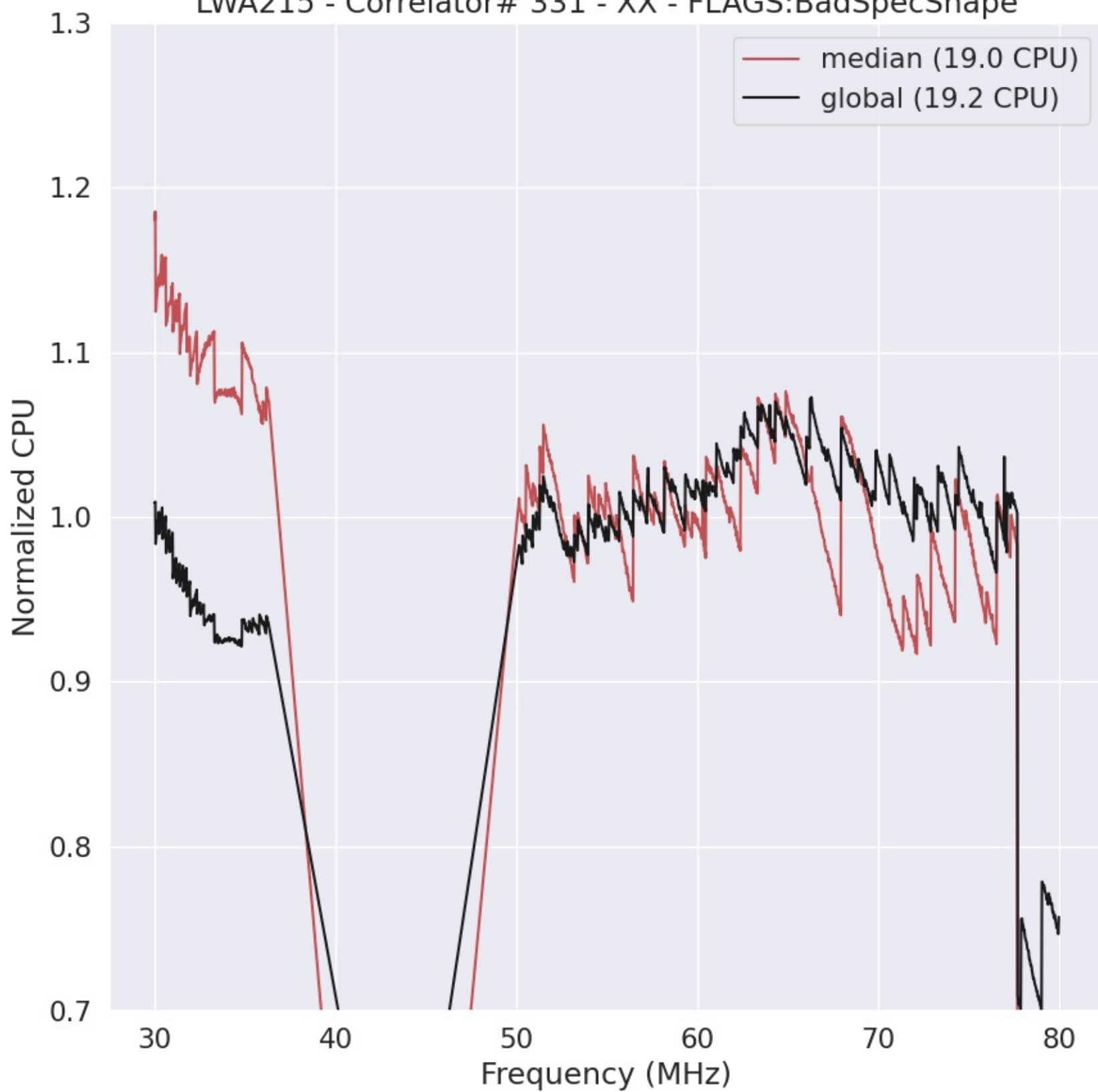
LWA215 - Correlator# 331 - XX - FLAGS:BadSpecShape
