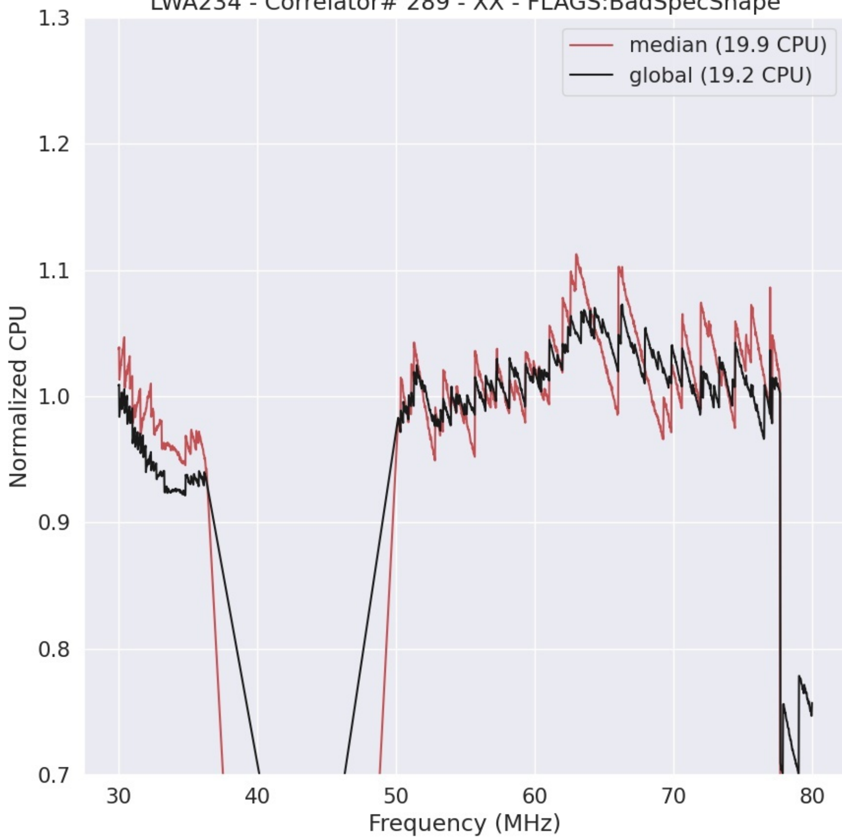
LWA234 - Correlator# 289 - XX - FLAGS:BadSpecShape
