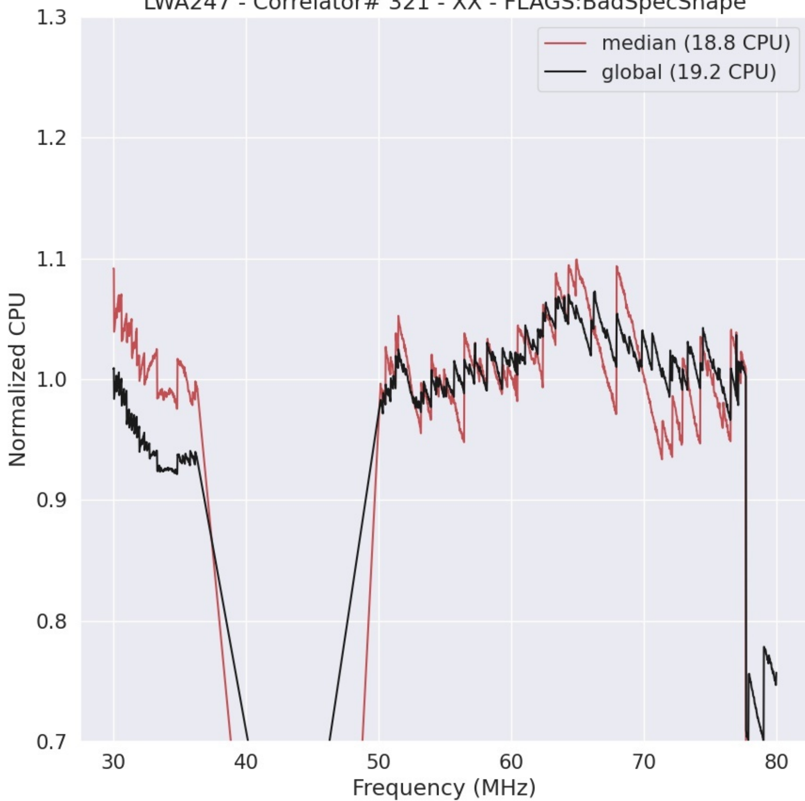
LWA247 - Correlator# 321 - XX - FLAGS:BadSpecShape
