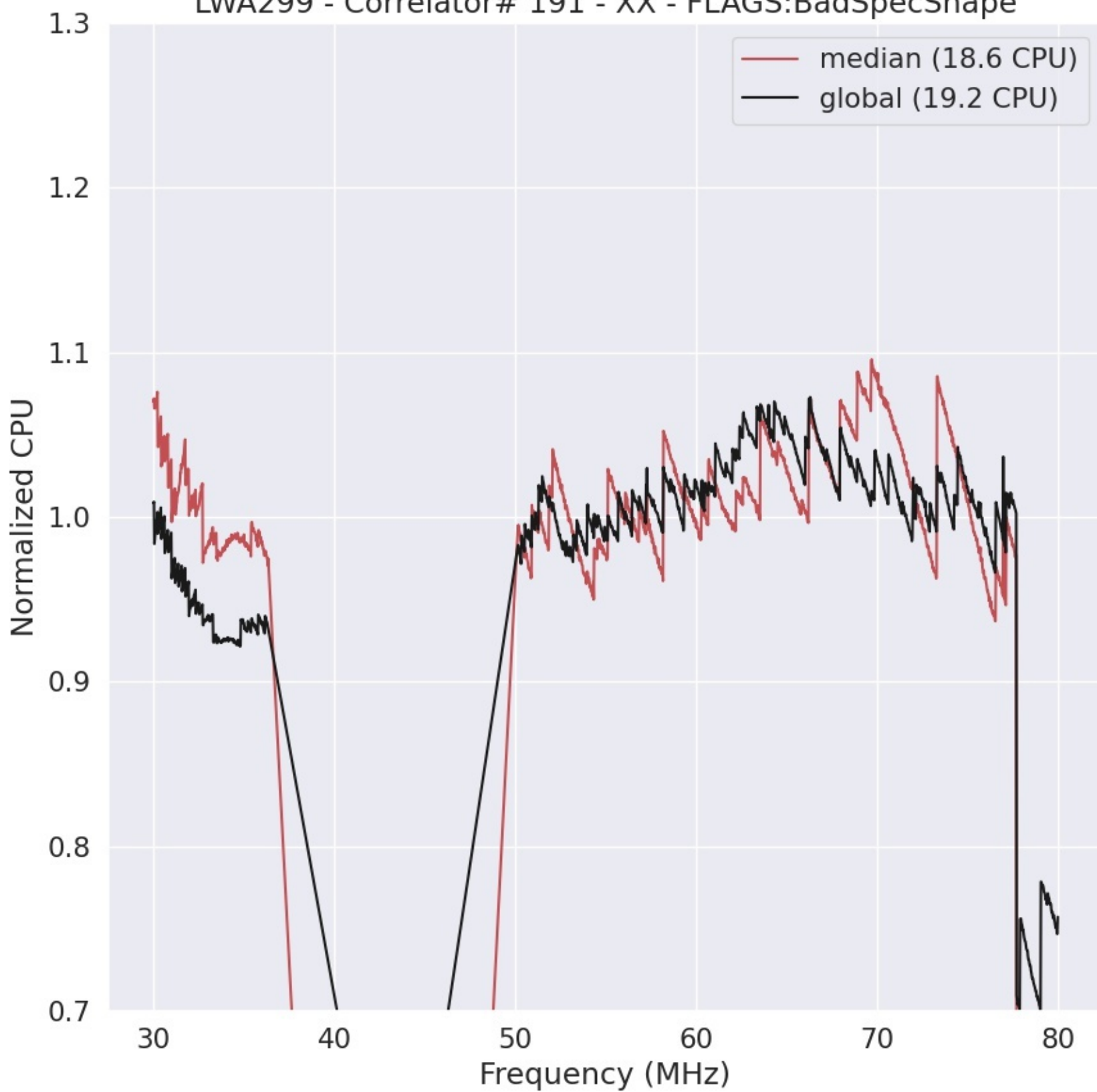
LWA299 - Correlator# 191 - XX - FLAGS:BadSpecShape
