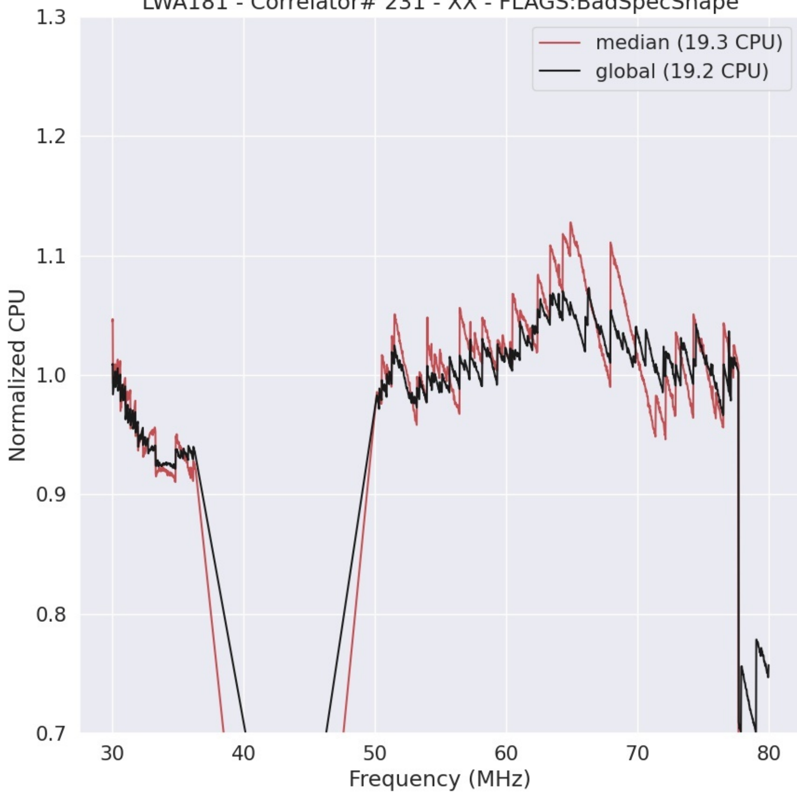
LWA181 - Correlator# 231 - XX - FLAGS:BadSpecShape
