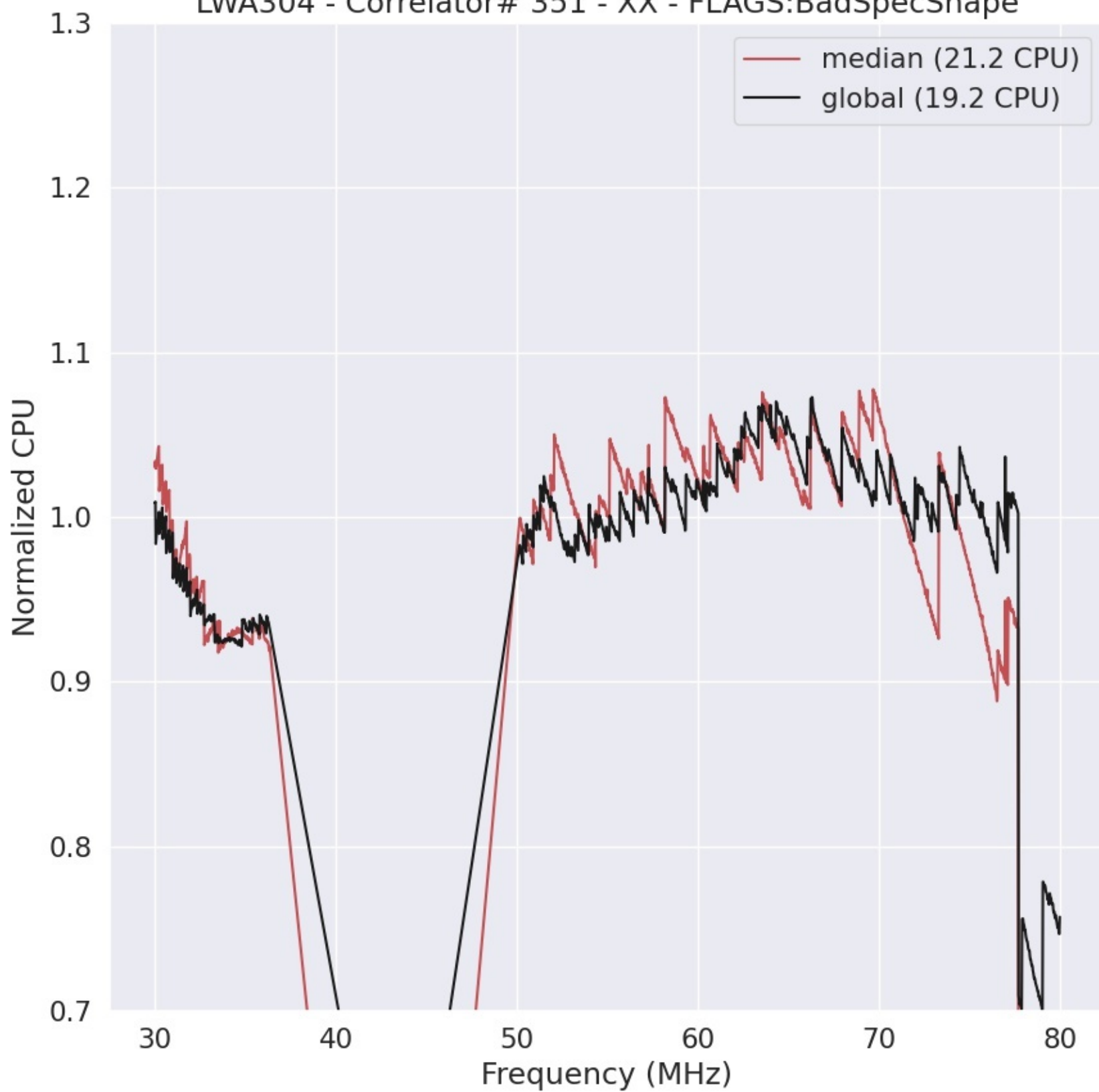
LWA304 - Correlator# 351 - XX - FLAGS:BadSpecShape
