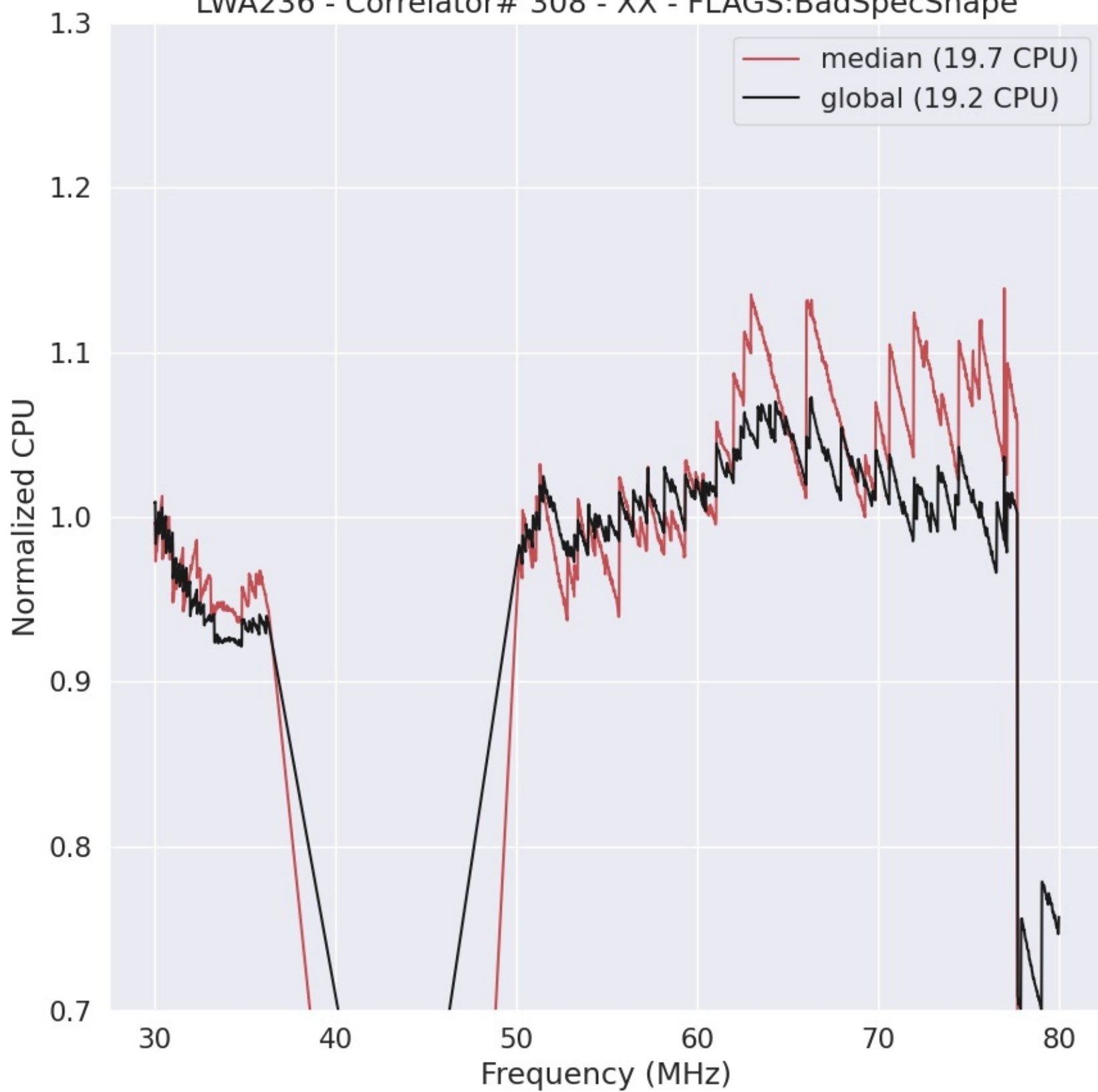
LWA236 - Correlator# 308 - XX - FLAGS:BadSpecShape
