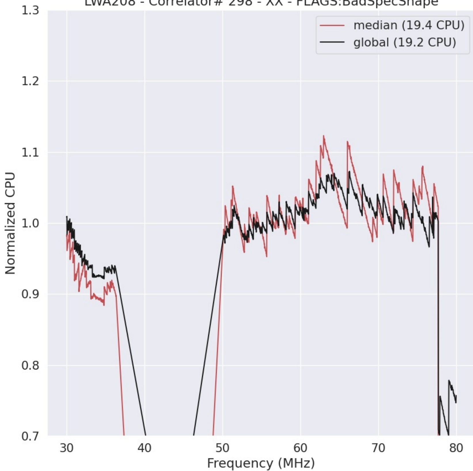
LWA208 - Correlator# 298 - XX - FLAGS:BadSpecShape
