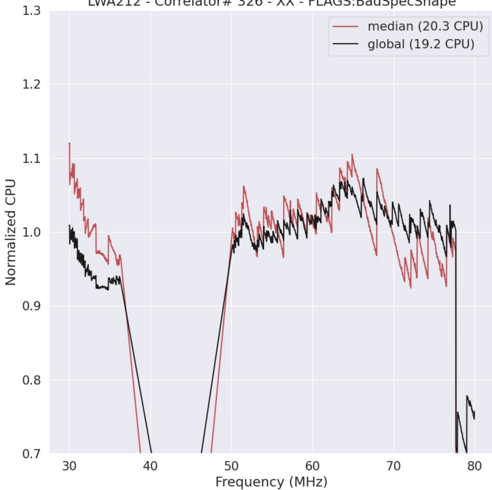
LWA212 - Correlator# 326 - XX - FLAGS:BadSpecShape
