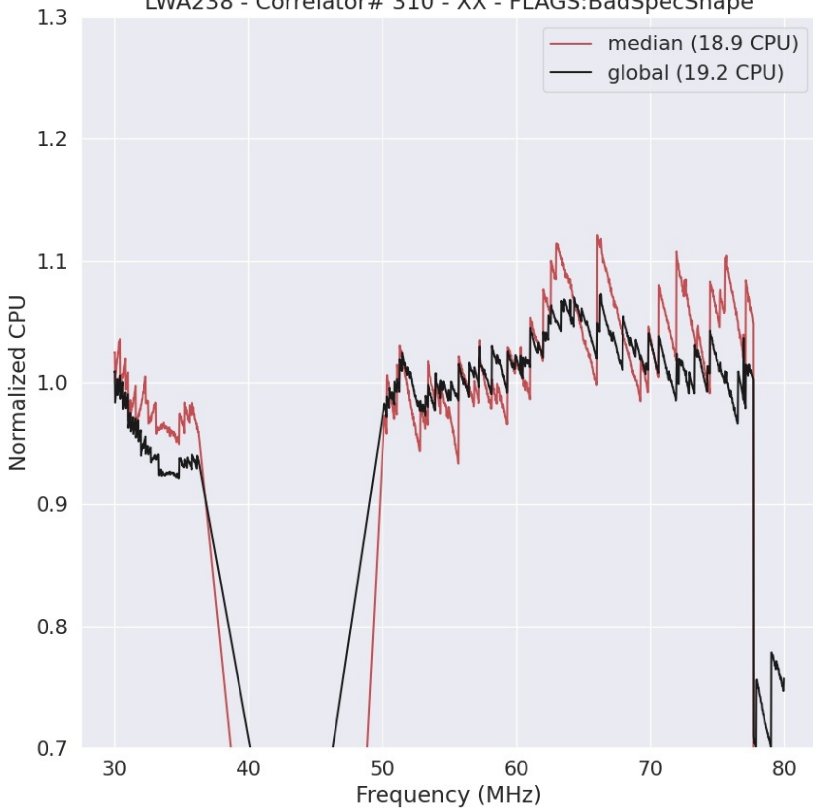
LWA238 - Correlator# 310 - XX - FLAGS:BadSpecShape
