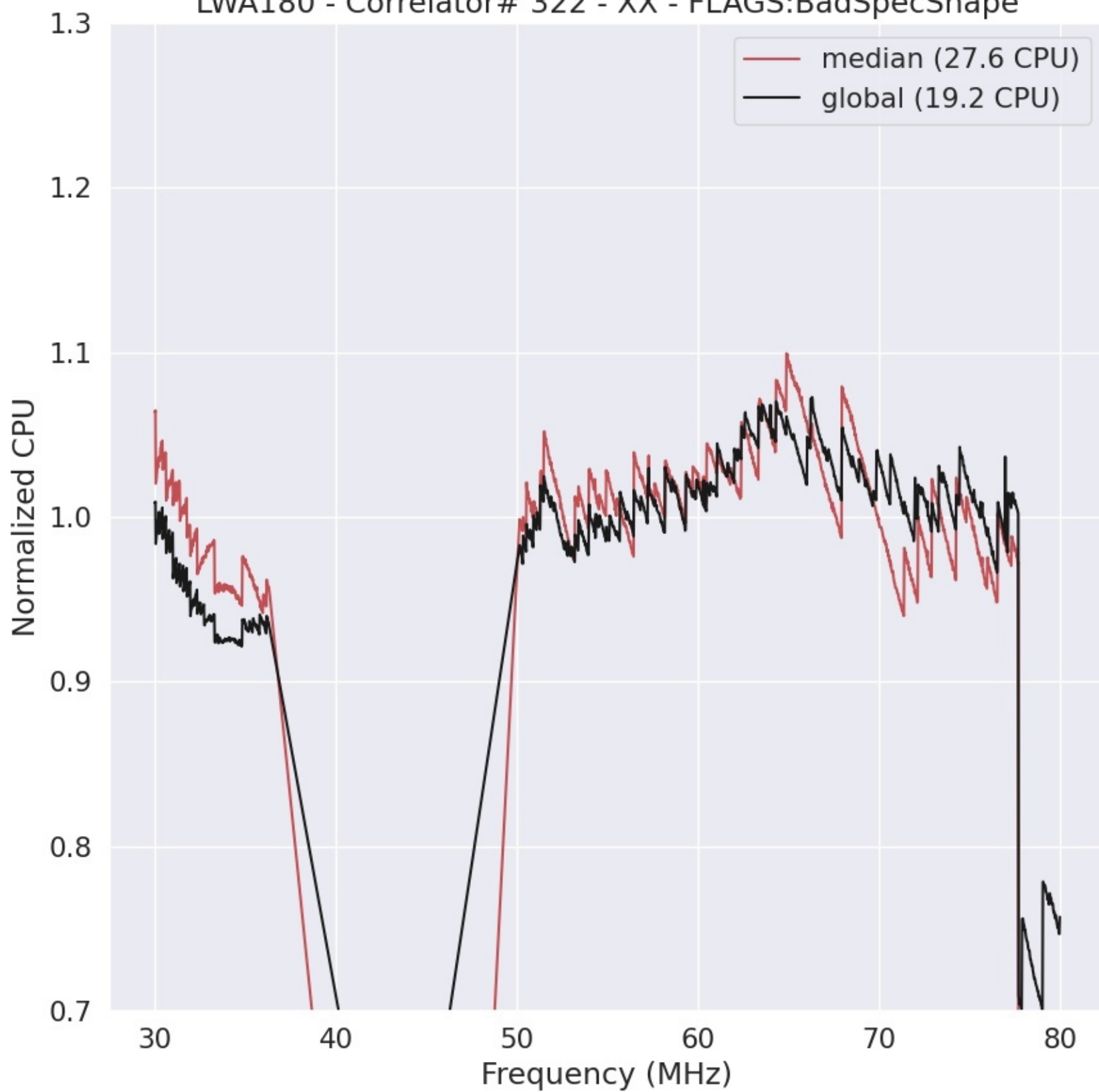
LWA180 - Correlator# 322 - XX - FLAGS:BadSpecShape
