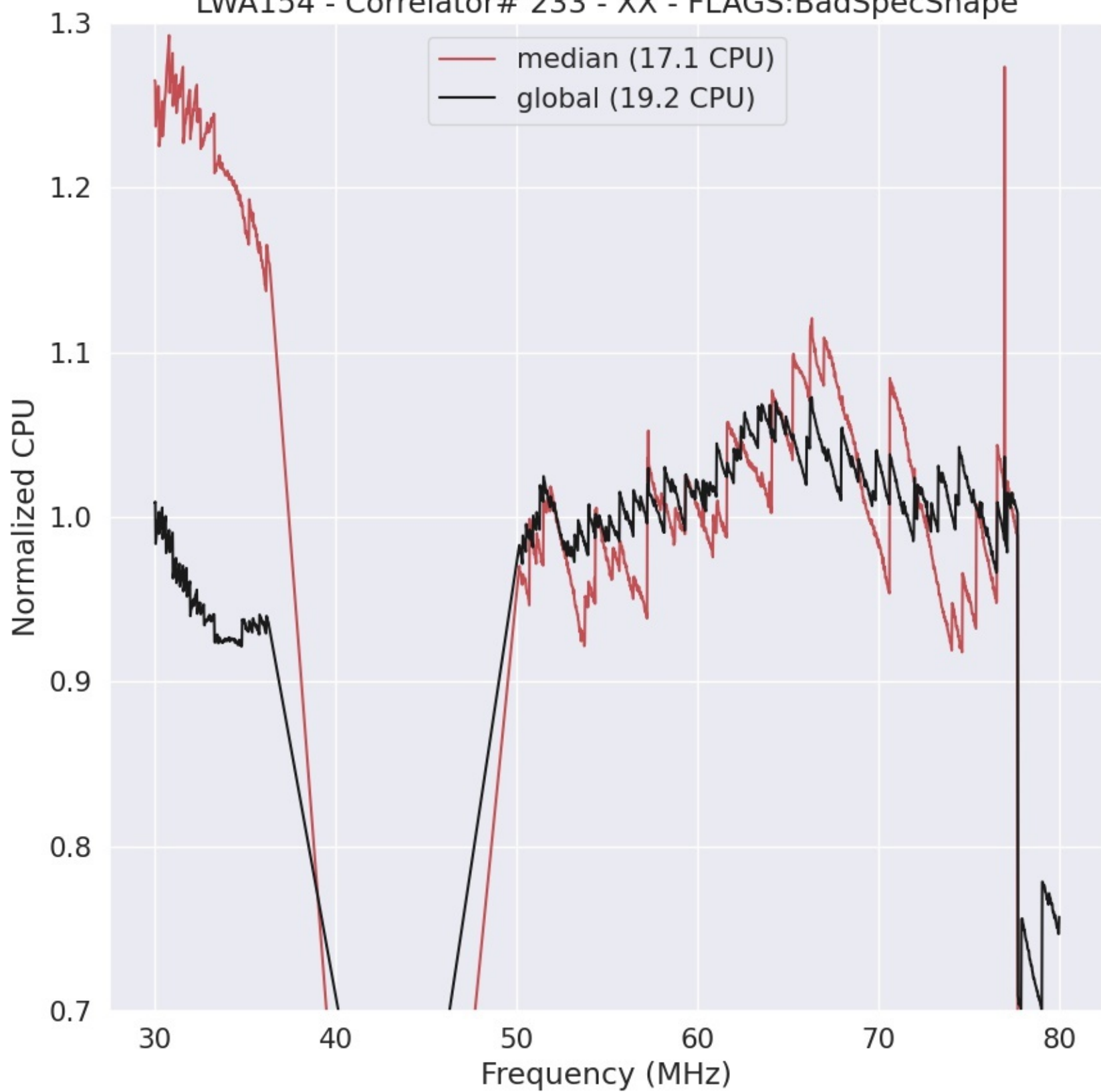
LWA154 - Correlator# 233 - XX - FLAGS:BadSpecShape
