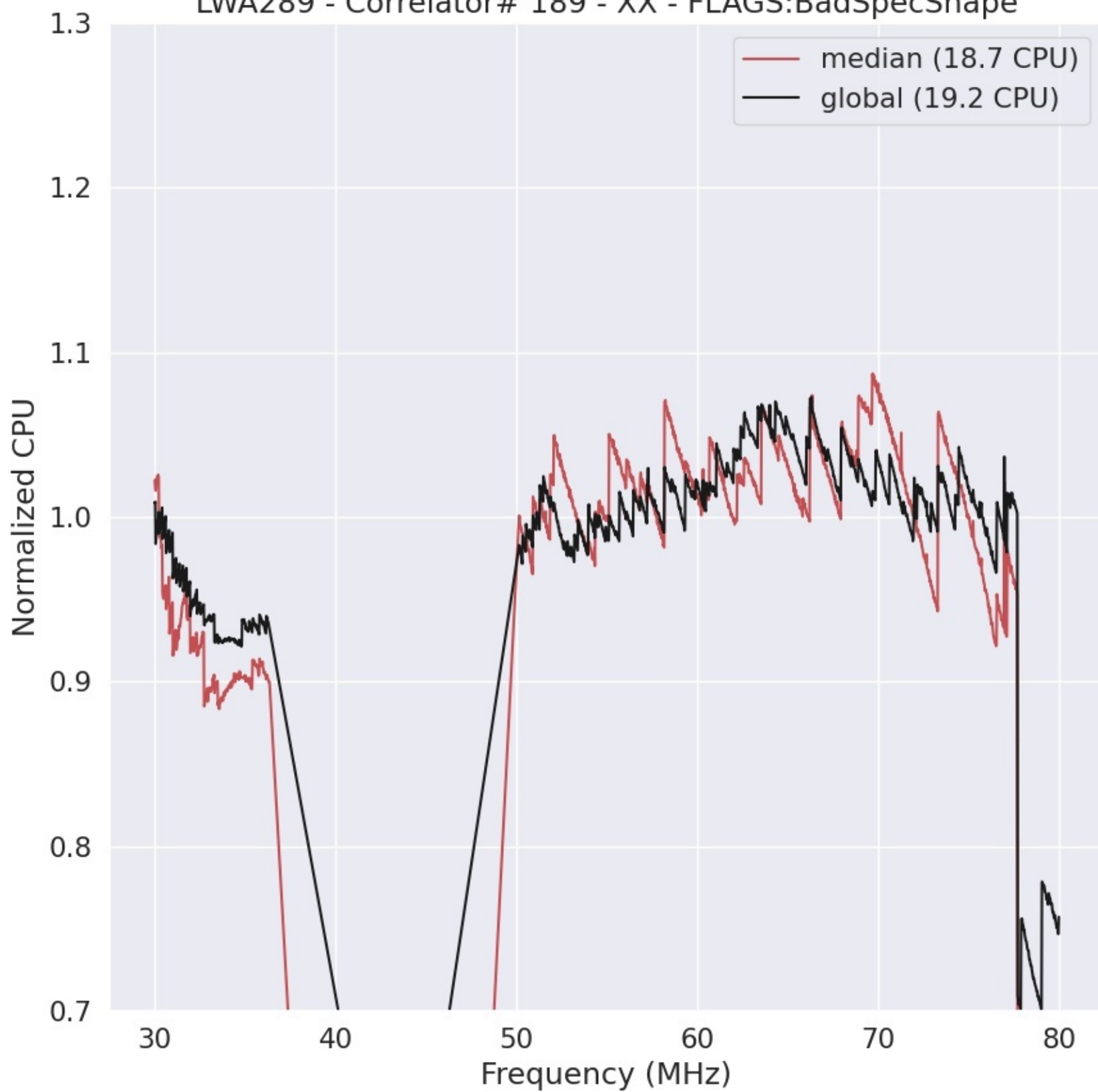
LWA289 - Correlator# 189 - XX - FLAGS:BadSpecShape
