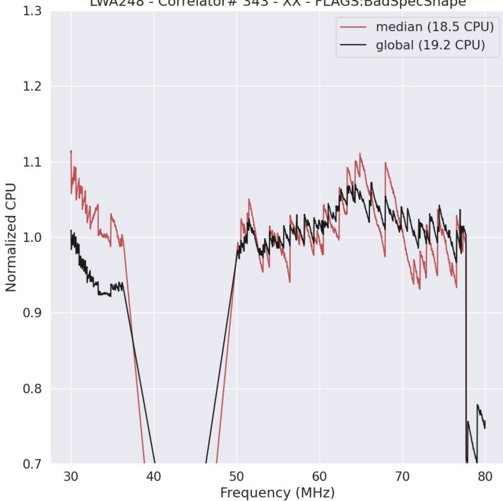
LWA248 - Correlator# 343 - XX - FLAGS:BadSpecShape
