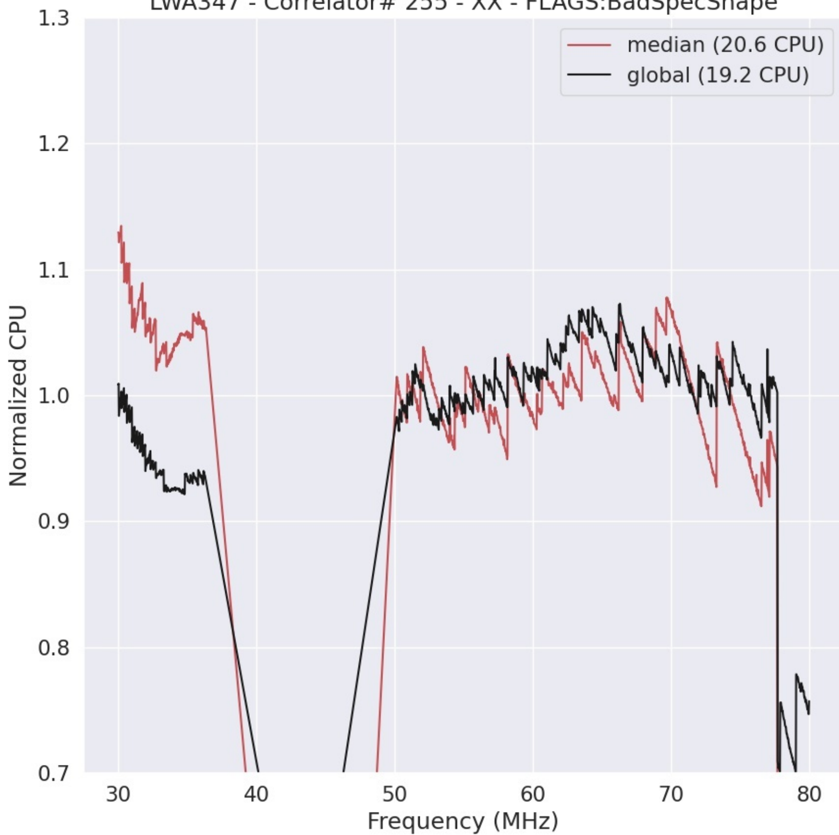
LWA347 - Correlator# 255 - XX - FLAGS:BadSpecShape
