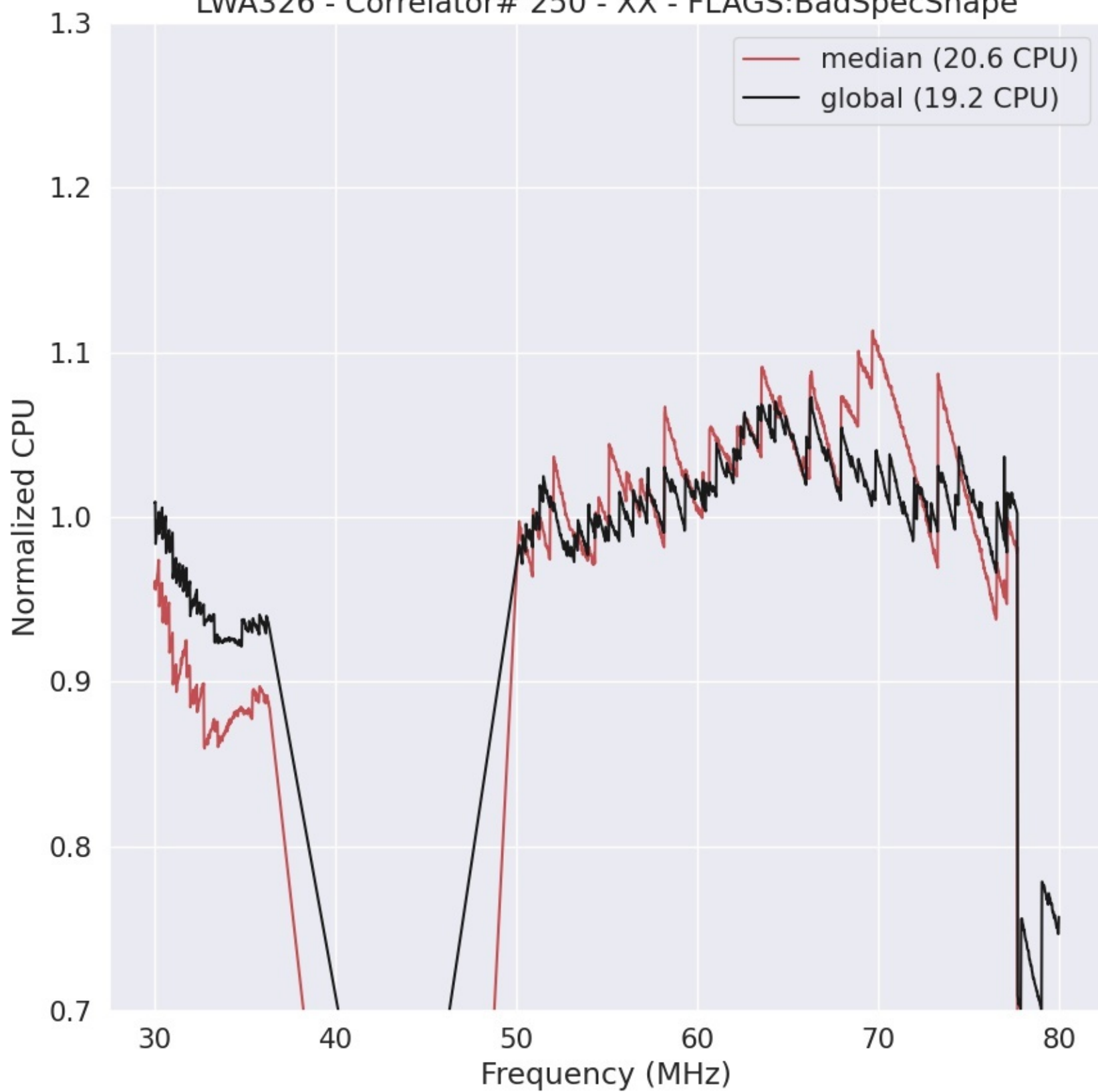
LWA326 - Correlator# 250 - XX - FLAGS:BadSpecShape
