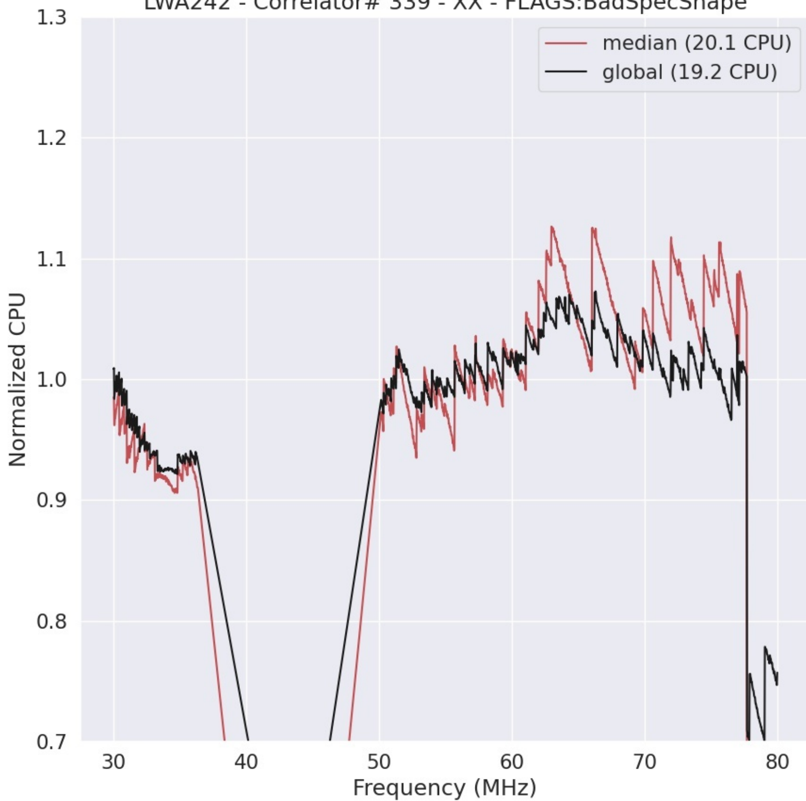
LWA242 - Correlator# 339 - XX - FLAGS:BadSpecShape
