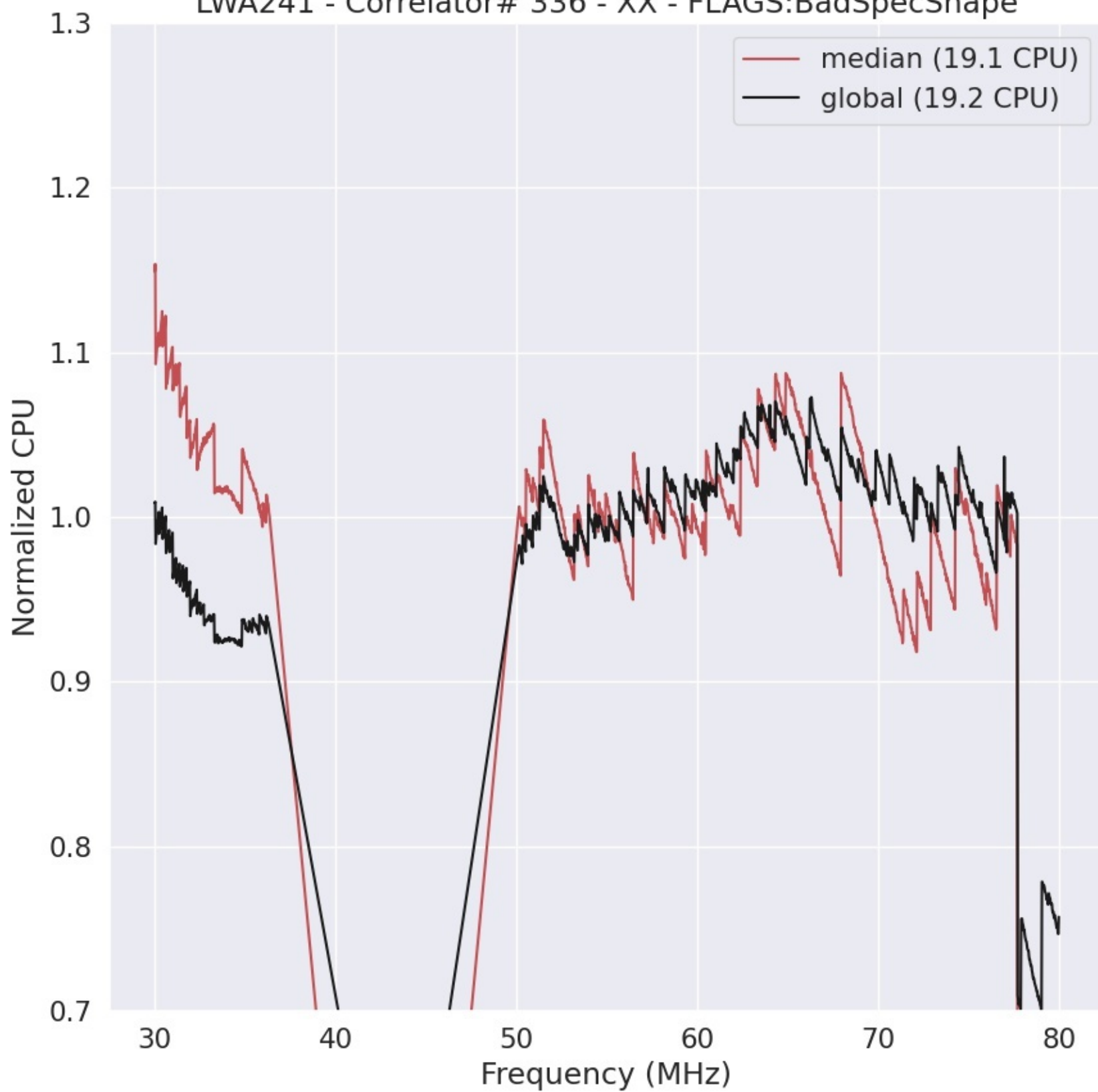
LWA241 - Correlator# 336 - XX - FLAGS:BadSpecShape
