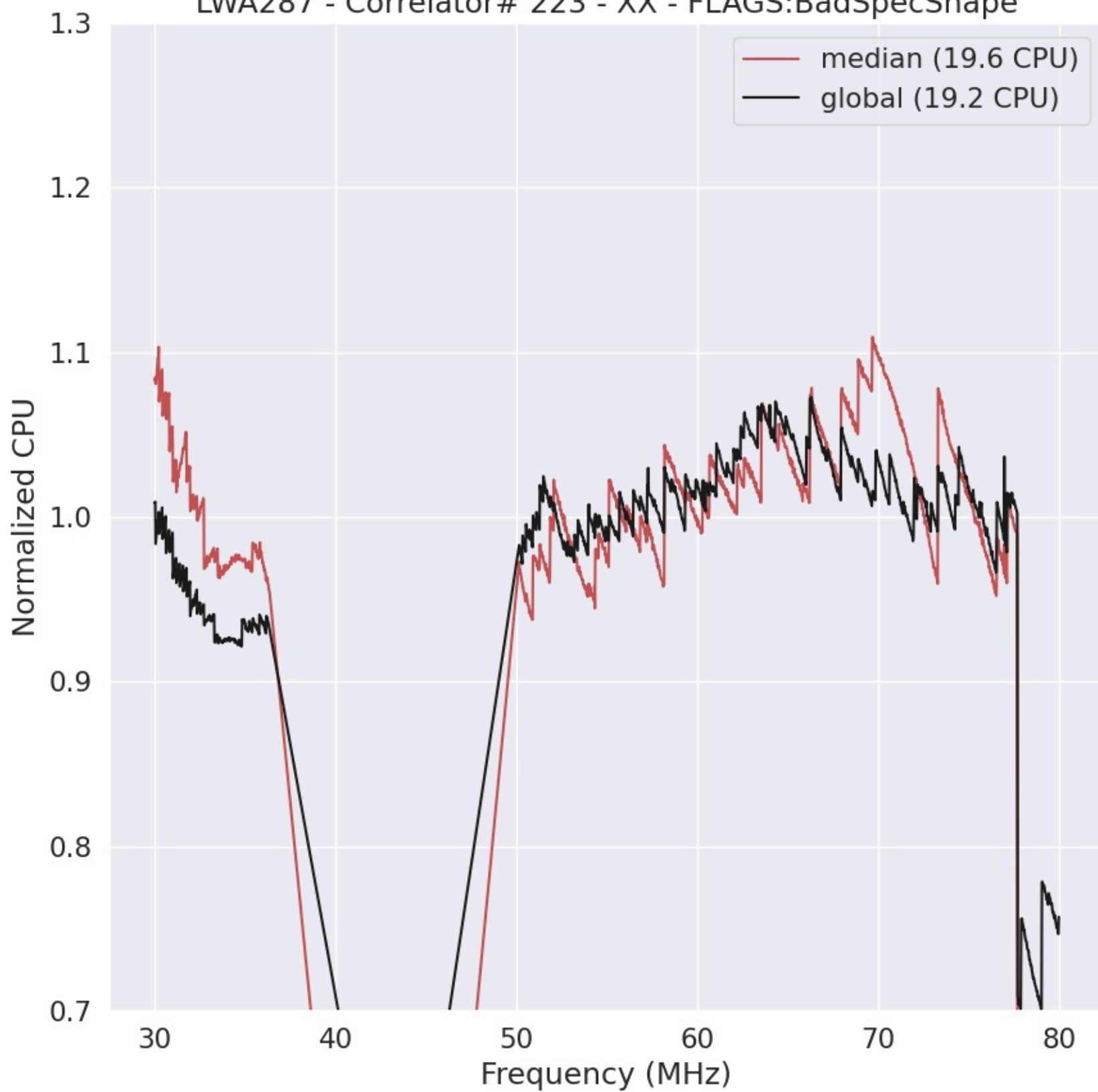
LWA287 - Correlator# 223 - XX - FLAGS:BadSpecShape
