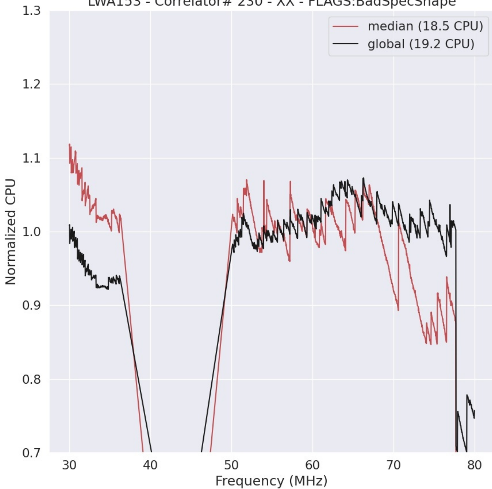
LWA153 - Correlator# 230 - XX - FLAGS:BadSpecShape
