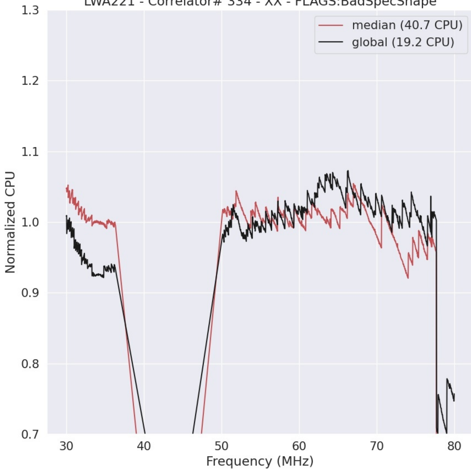
LWA221 - Correlator# 334 - XX - FLAGS:BadSpecShape
