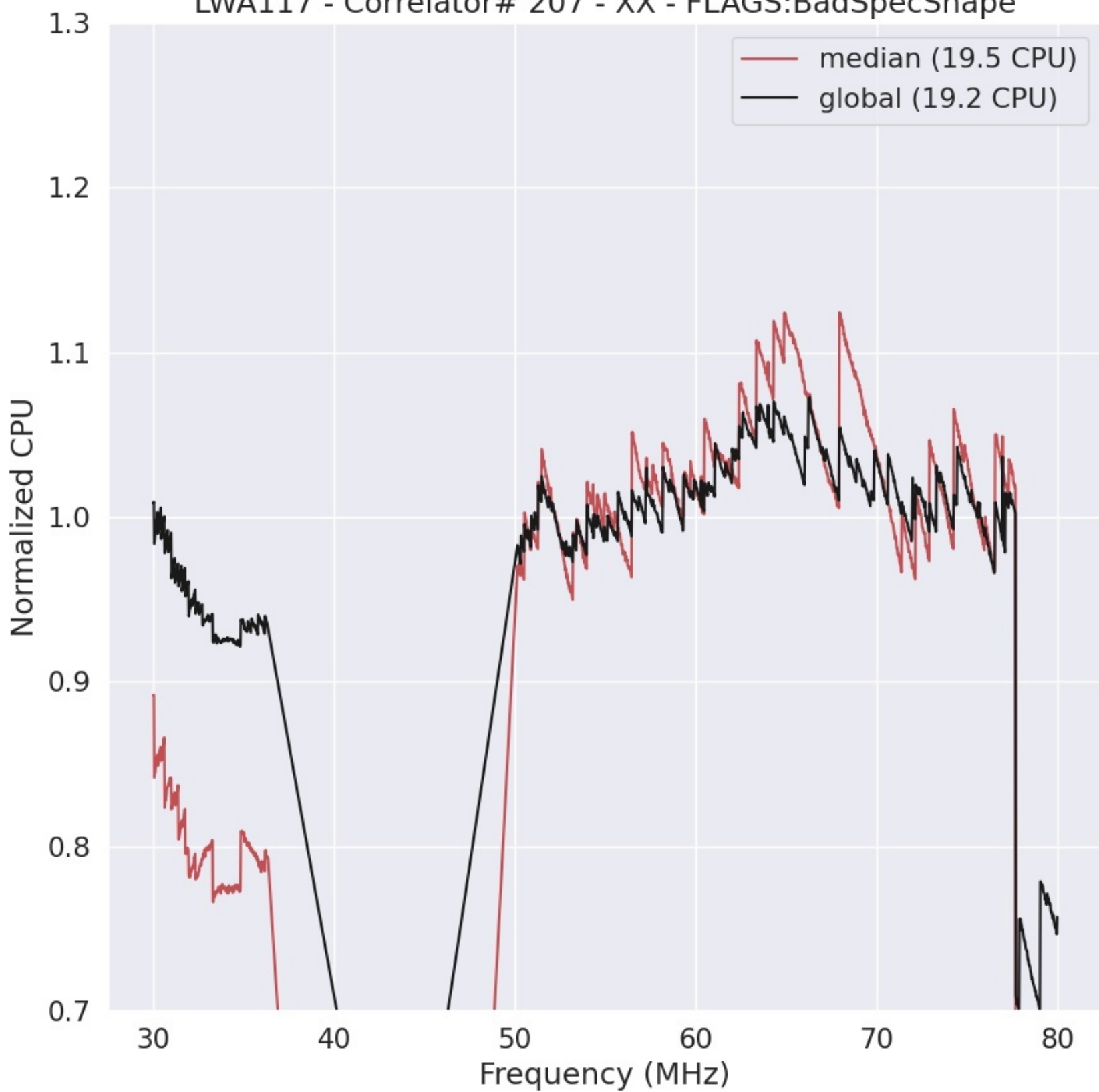
LWA117 - Correlator# 207 - XX - FLAGS:BadSpecShape
