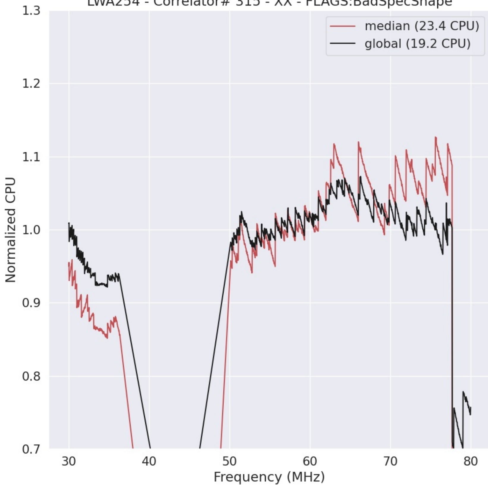
LWA254 - Correlator# 315 - XX - FLAGS:BadSpecShape
