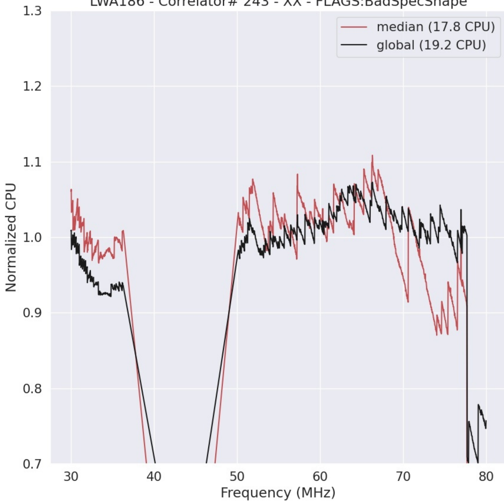
LWA186 - Correlator# 243 - XX - FLAGS:BadSpecShape
