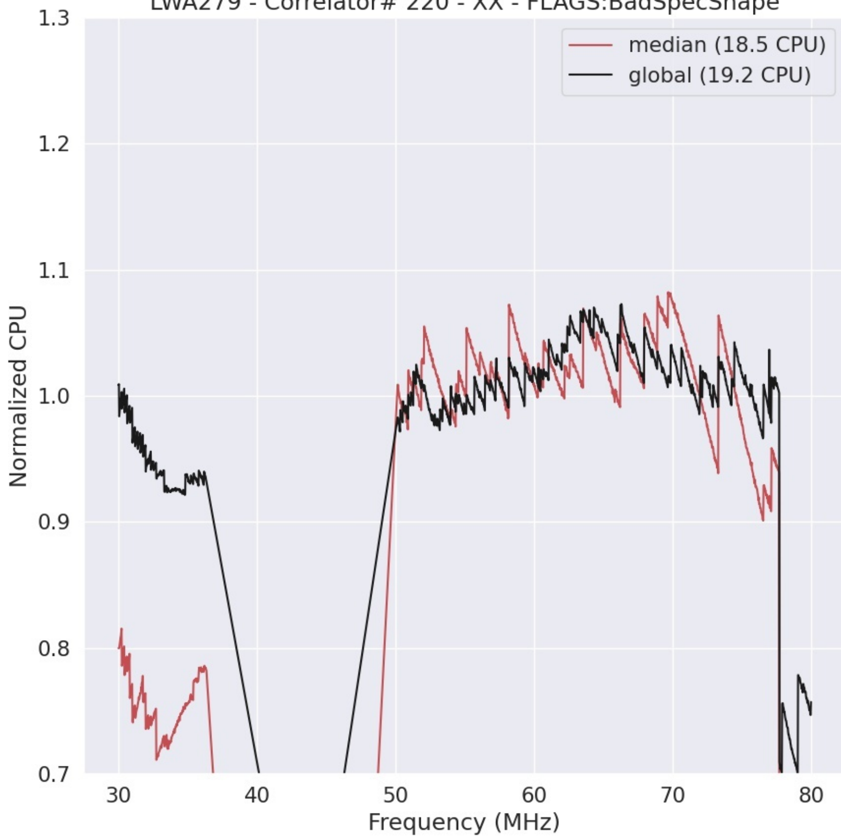
LWA279 - Correlator# 220 - XX - FLAGS:BadSpecShape
