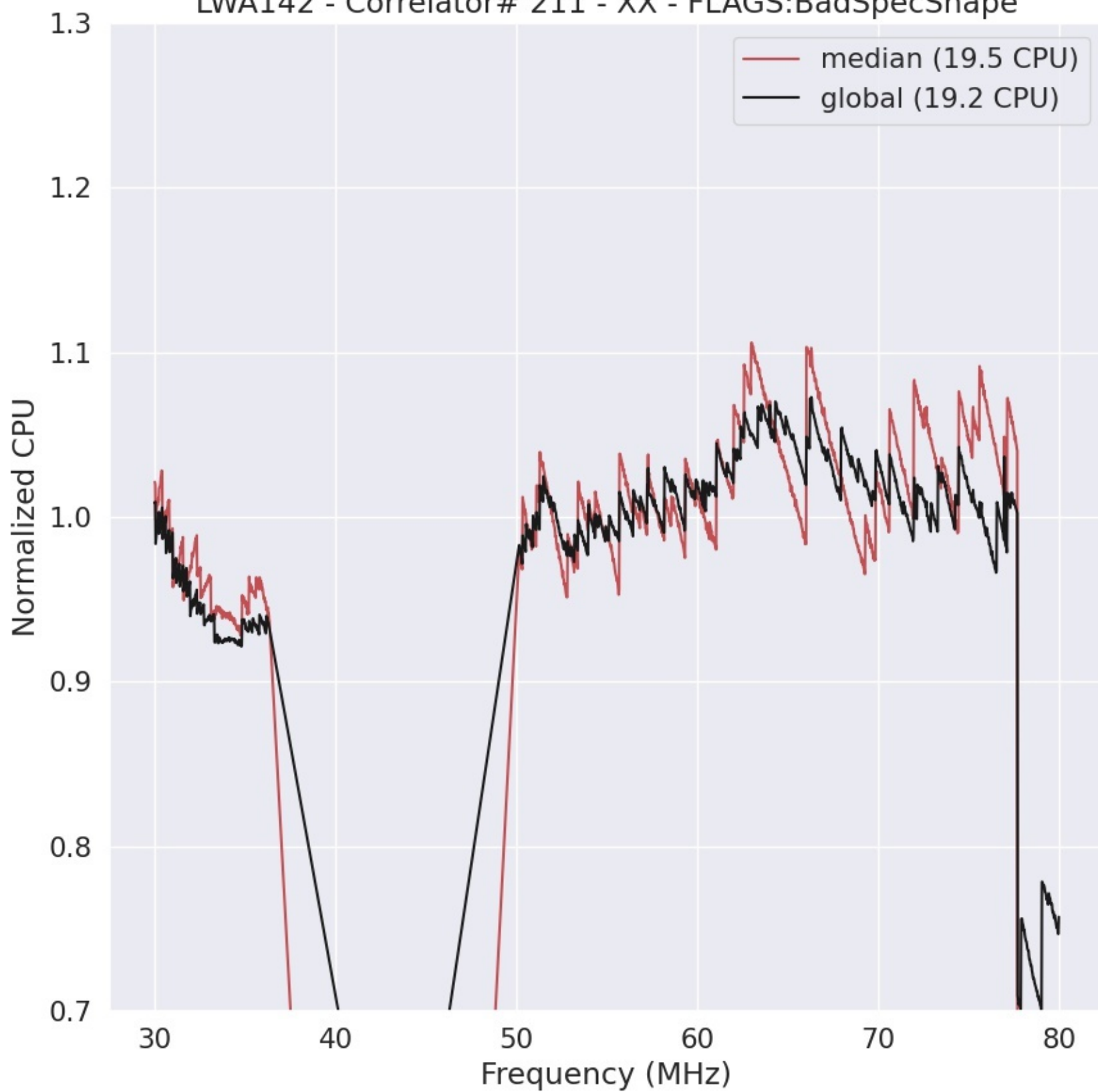
LWA142 - Correlator# 211 - XX - FLAGS:BadSpecShape
