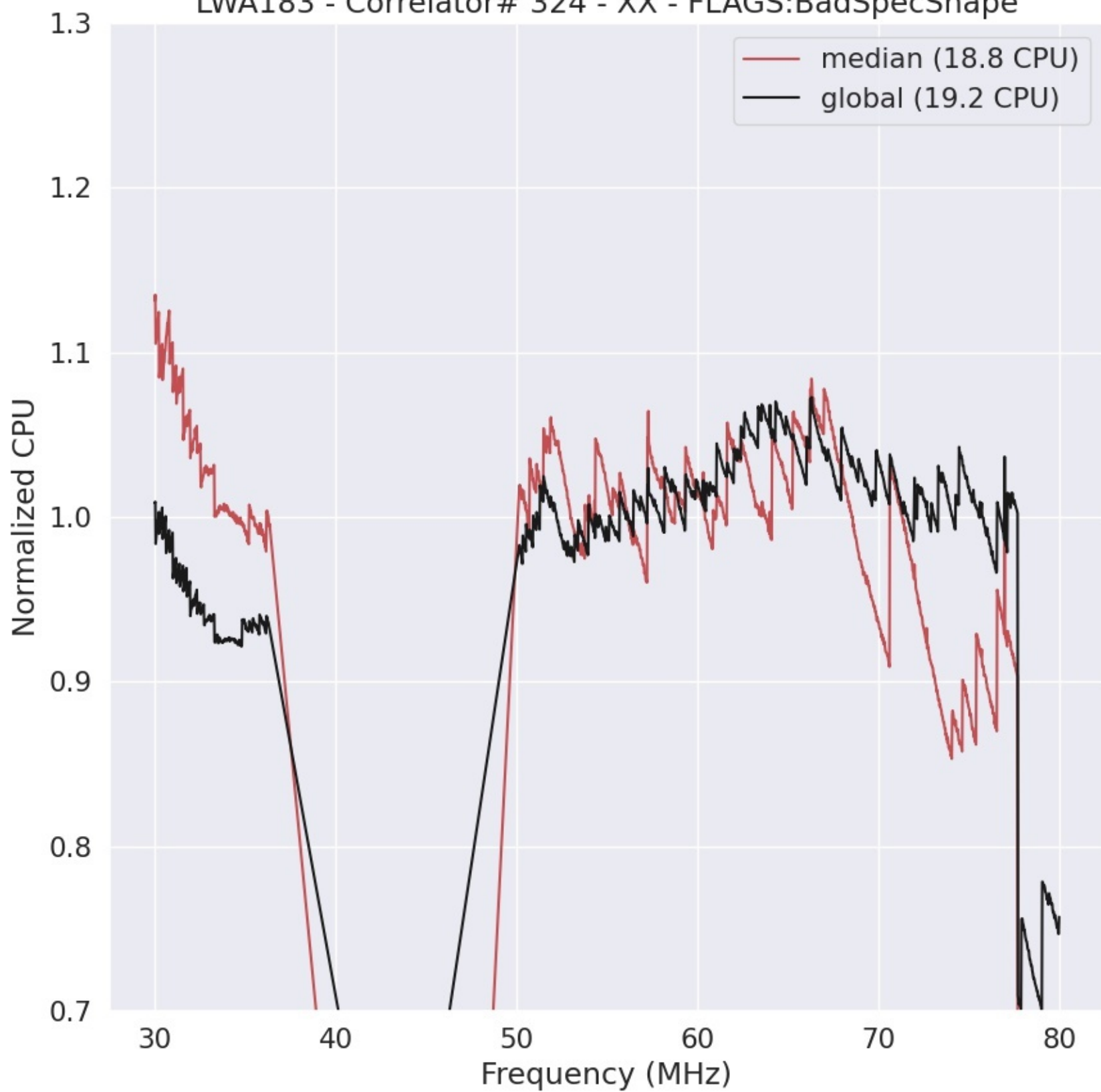
LWA183 - Correlator# 324 - XX - FLAGS:BadSpecShape
