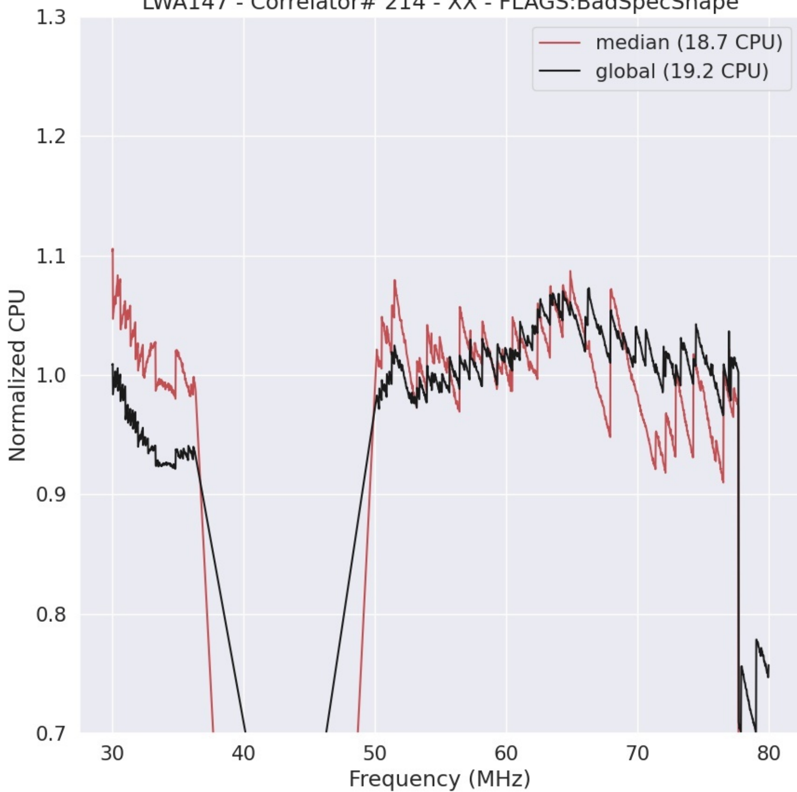
LWA147 - Correlator# 214 - XX - FLAGS:BadSpecShape
