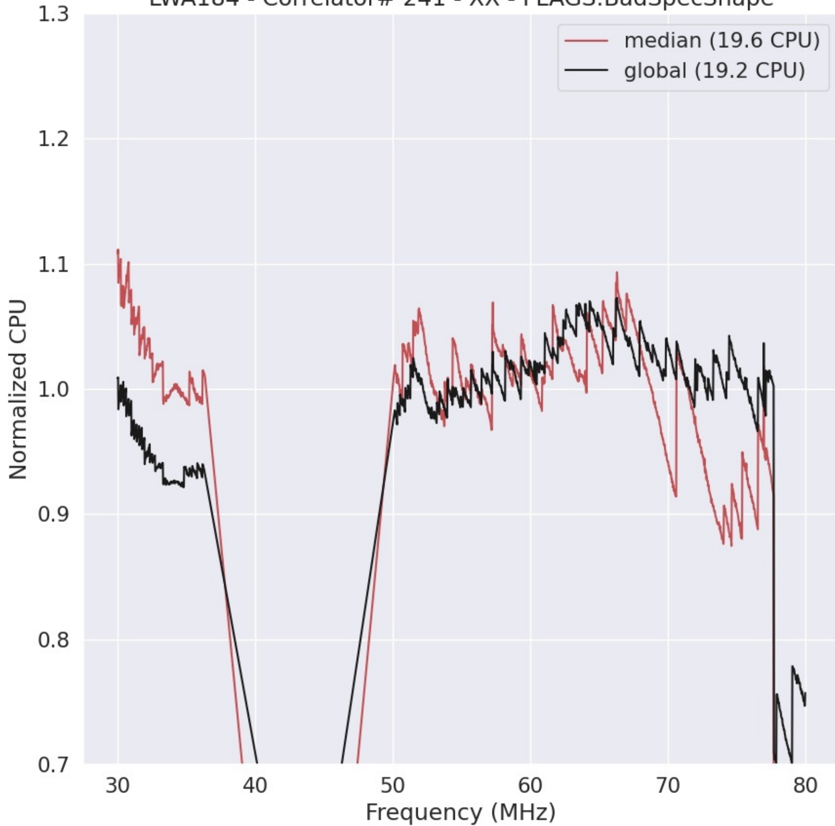
LWA184 - Correlator# 241 - XX - FLAGS:BadSpecShape
