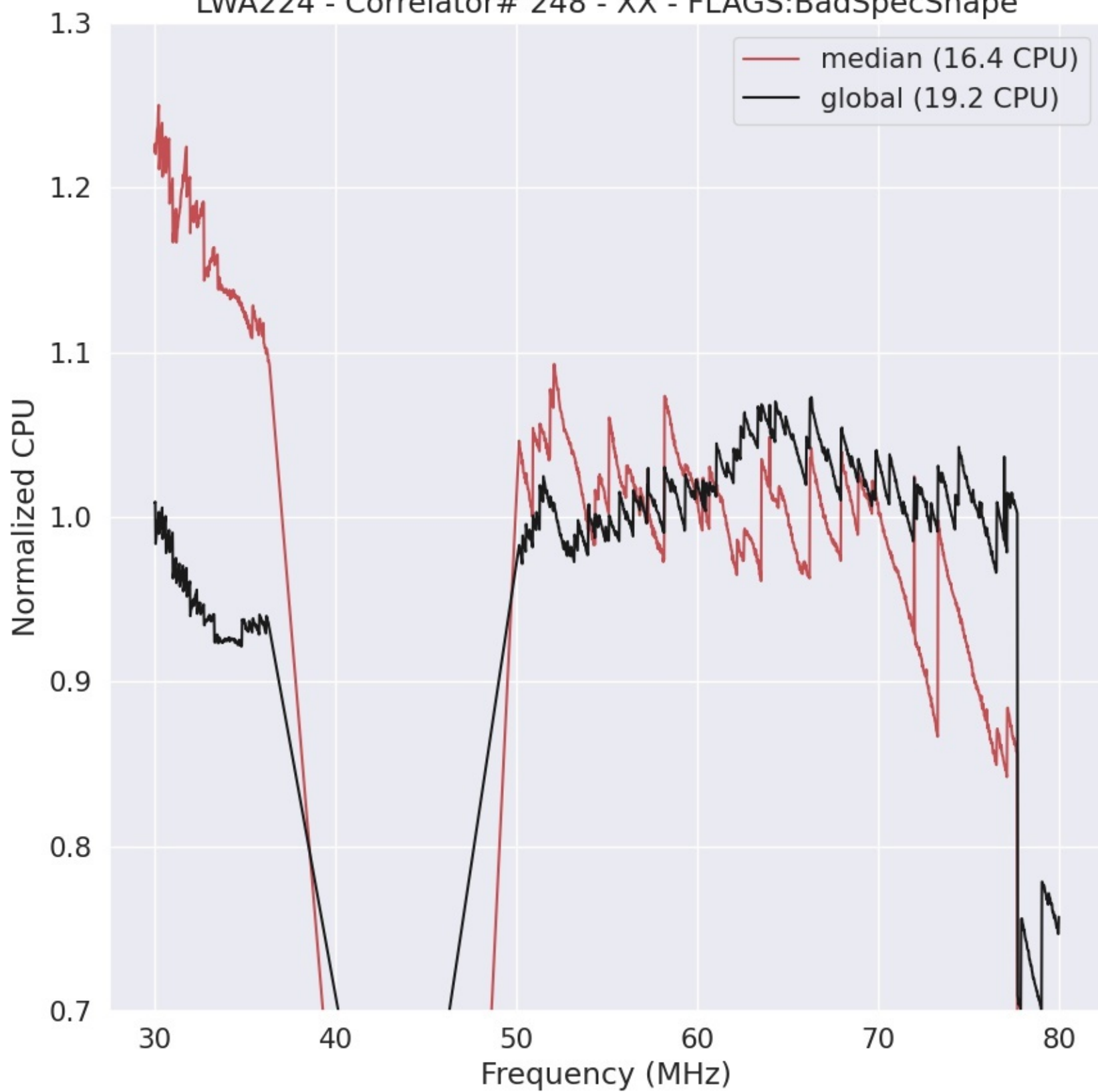
LWA224 - Correlator# 248 - XX - FLAGS:BadSpecShape
