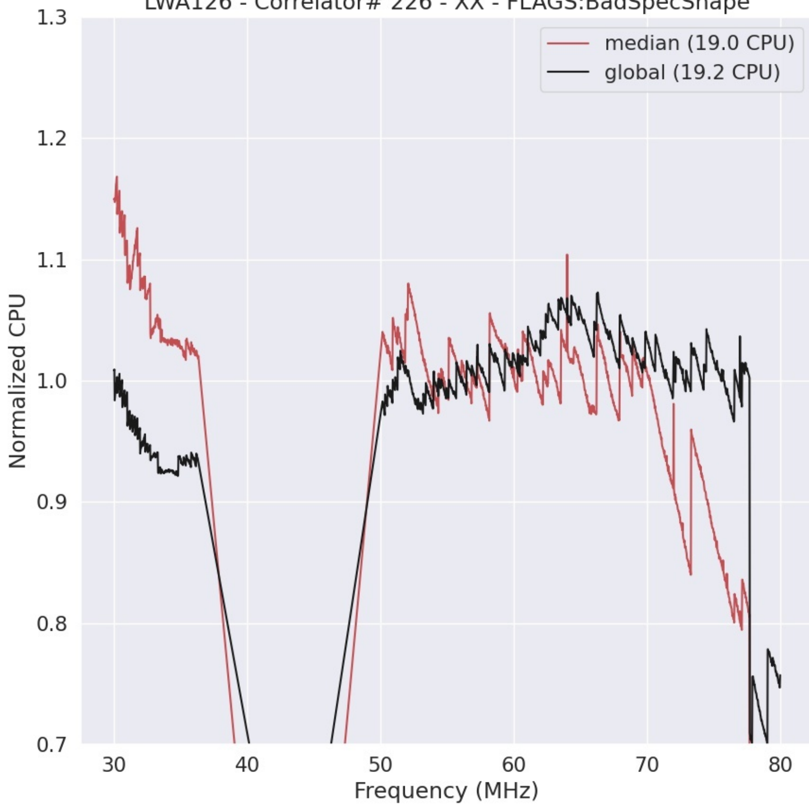
LWA126 - Correlator# 226 - XX - FLAGS:BadSpecShape
