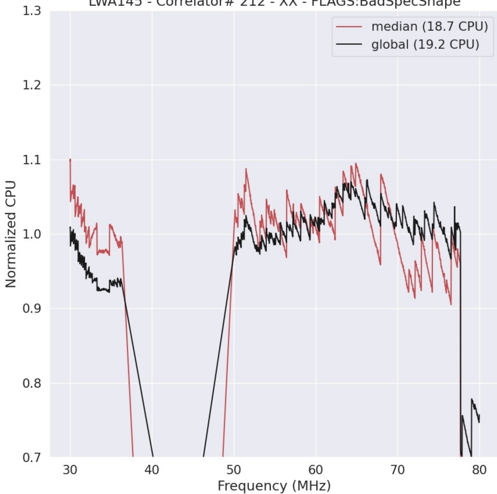
LWA145 - Correlator# 212 - XX - FLAGS:BadSpecShape
