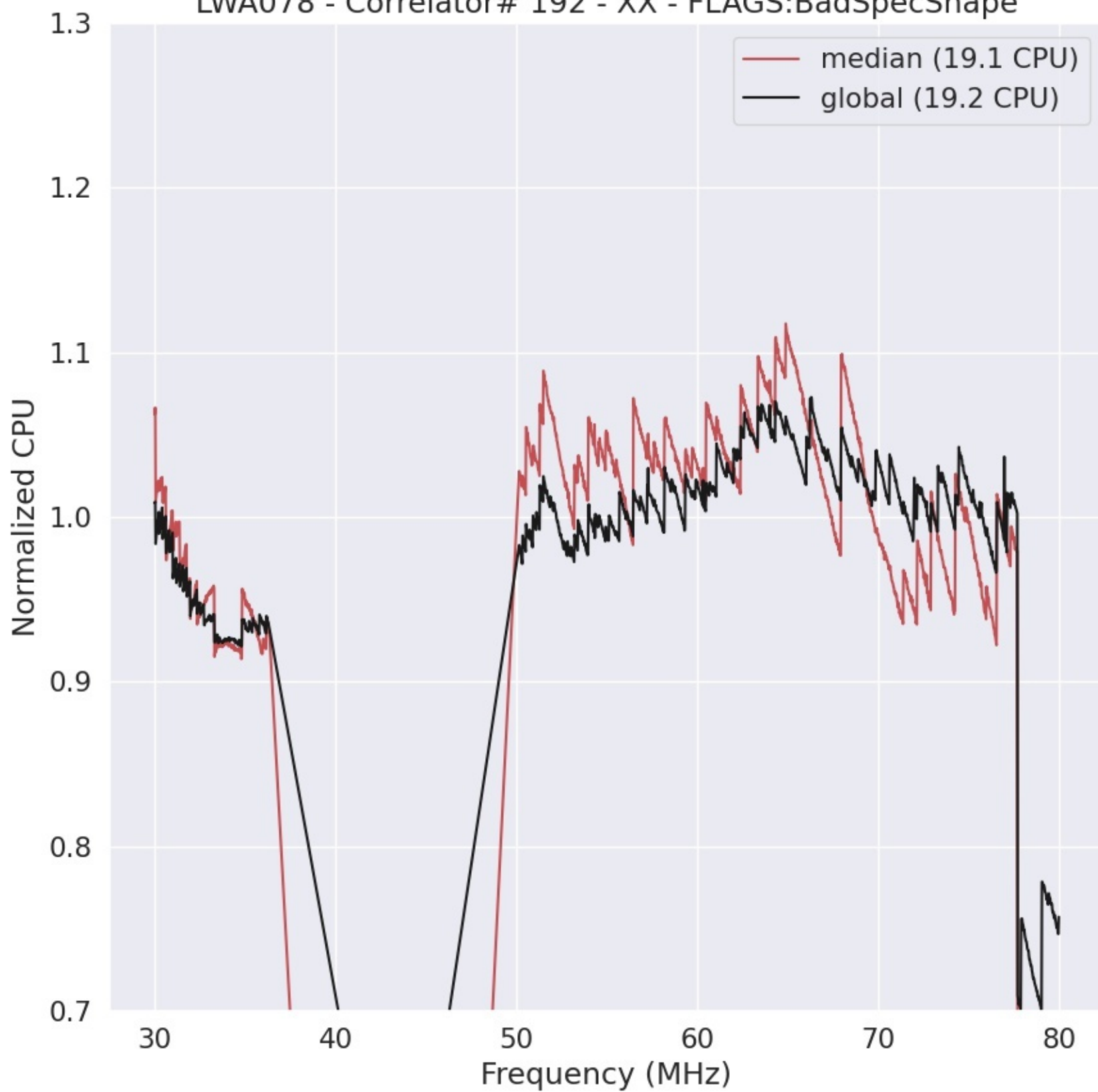
LWA078 - Correlator# 192 - XX - FLAGS:BadSpecShape
