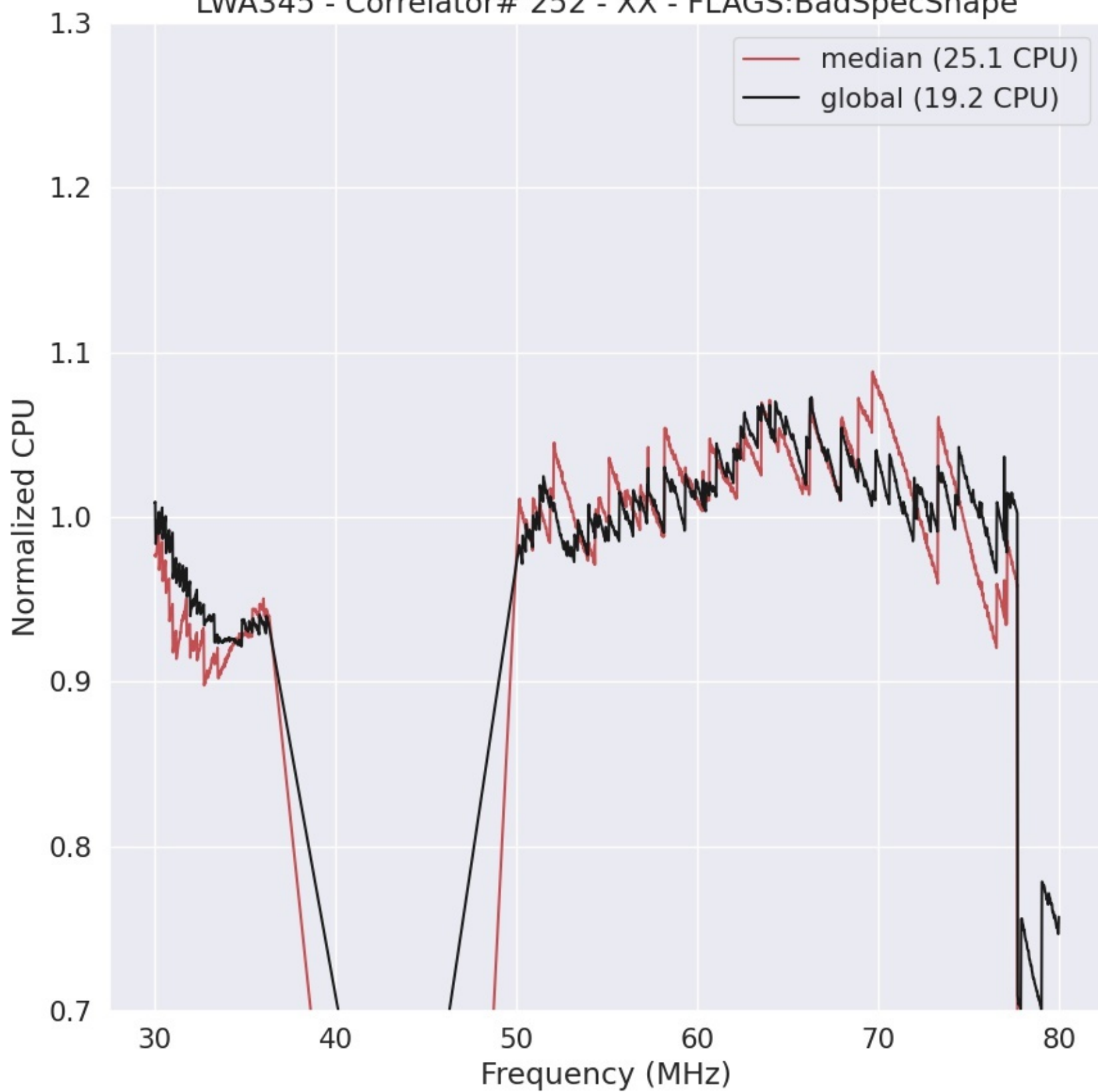
LWA345 - Correlator# 252 - XX - FLAGS:BadSpecShape
