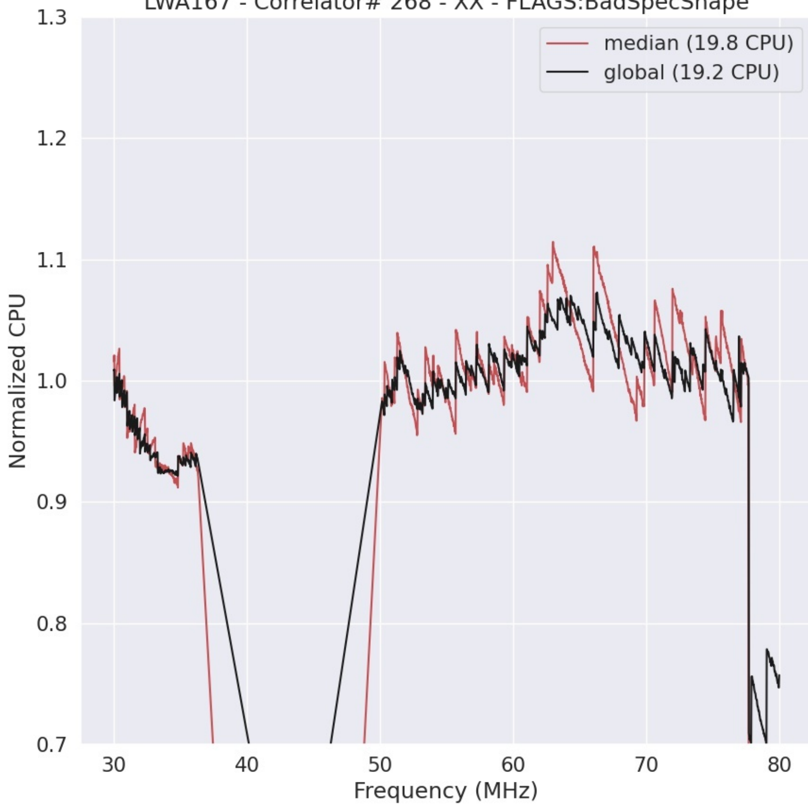
LWA167 - Correlator# 268 - XX - FLAGS:BadSpecShape
