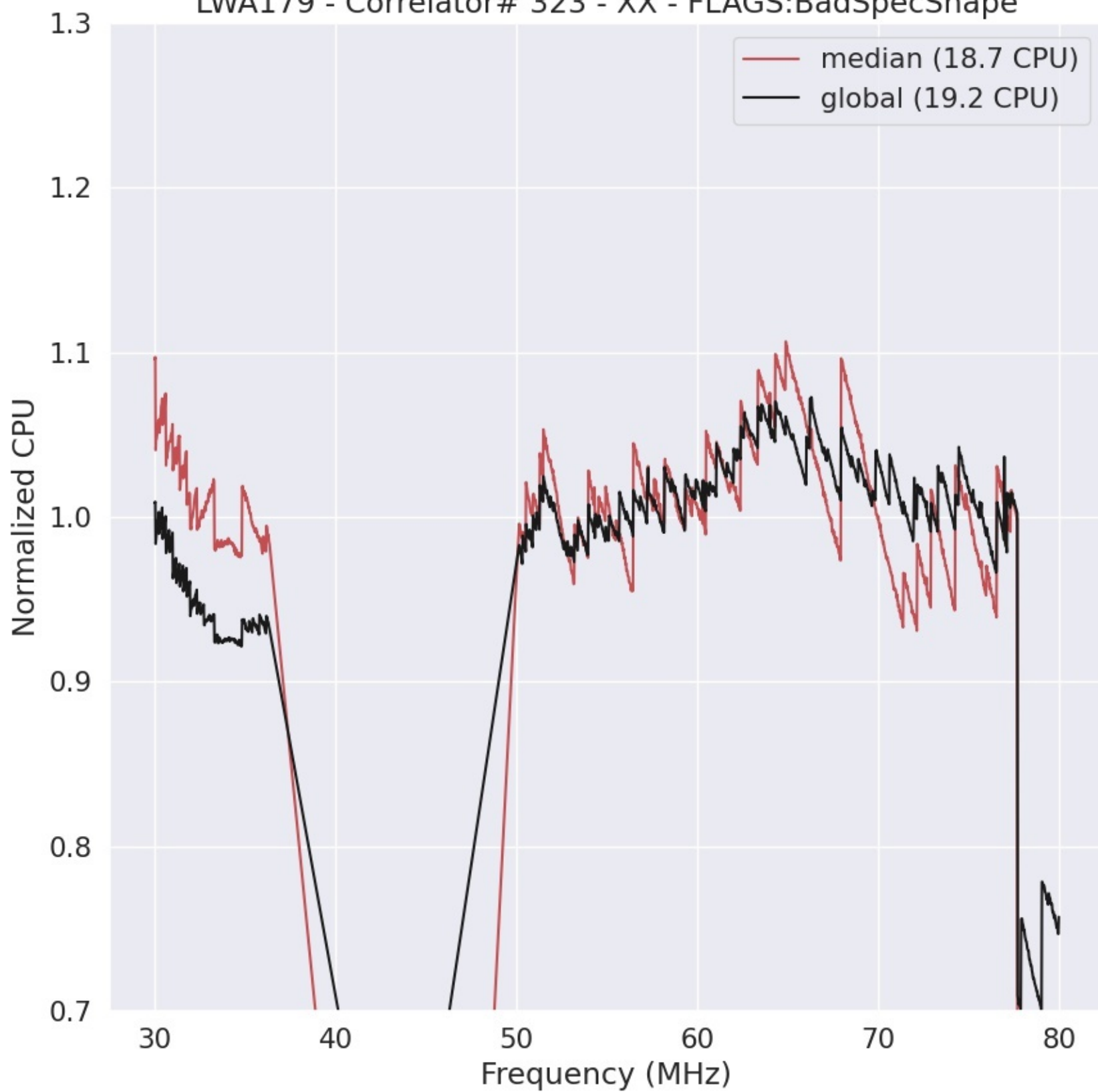
LWA179 - Correlator# 323 - XX - FLAGS:BadSpecShape
