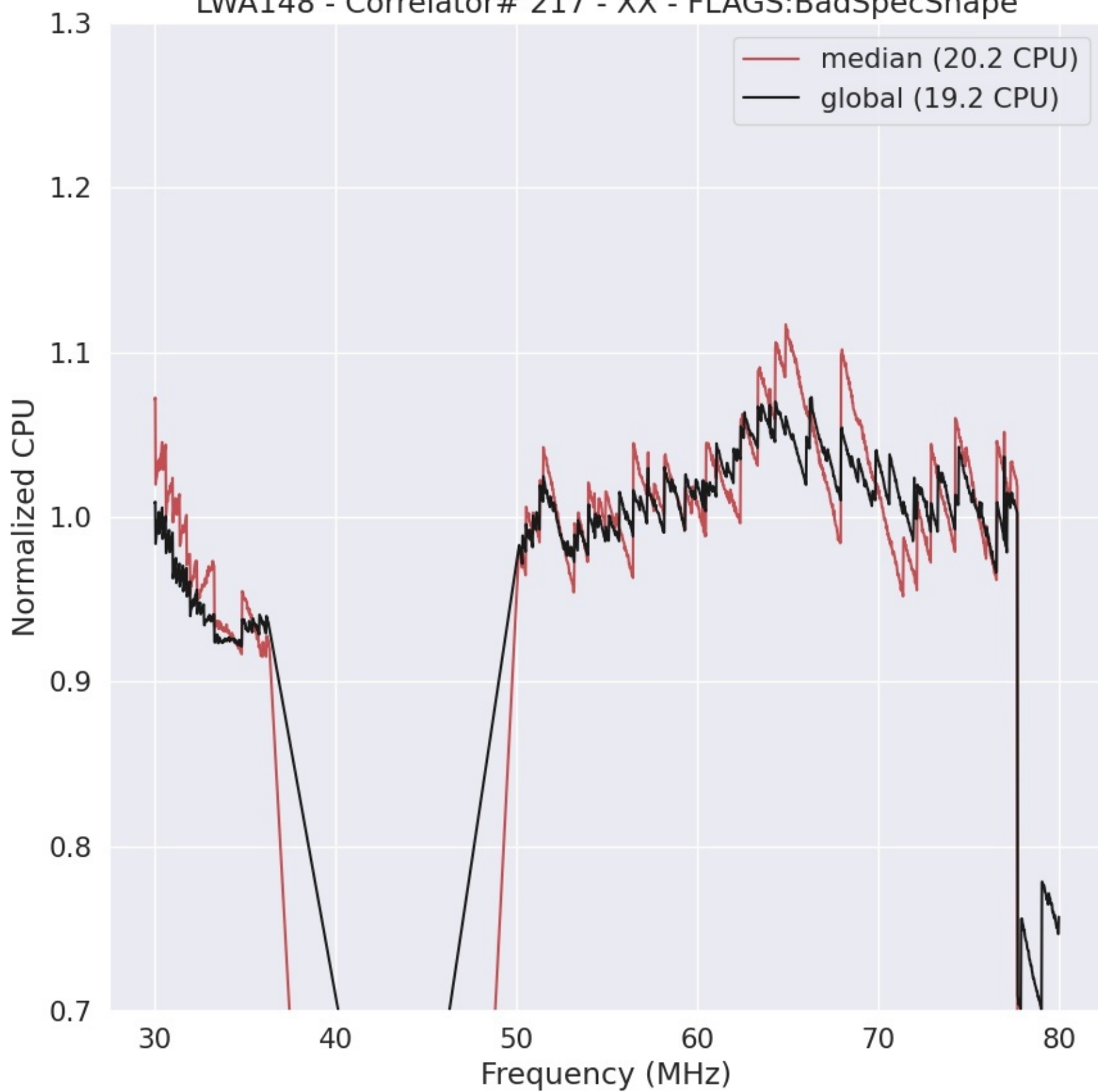
LWA148 - Correlator# 217 - XX - FLAGS:BadSpecShape
