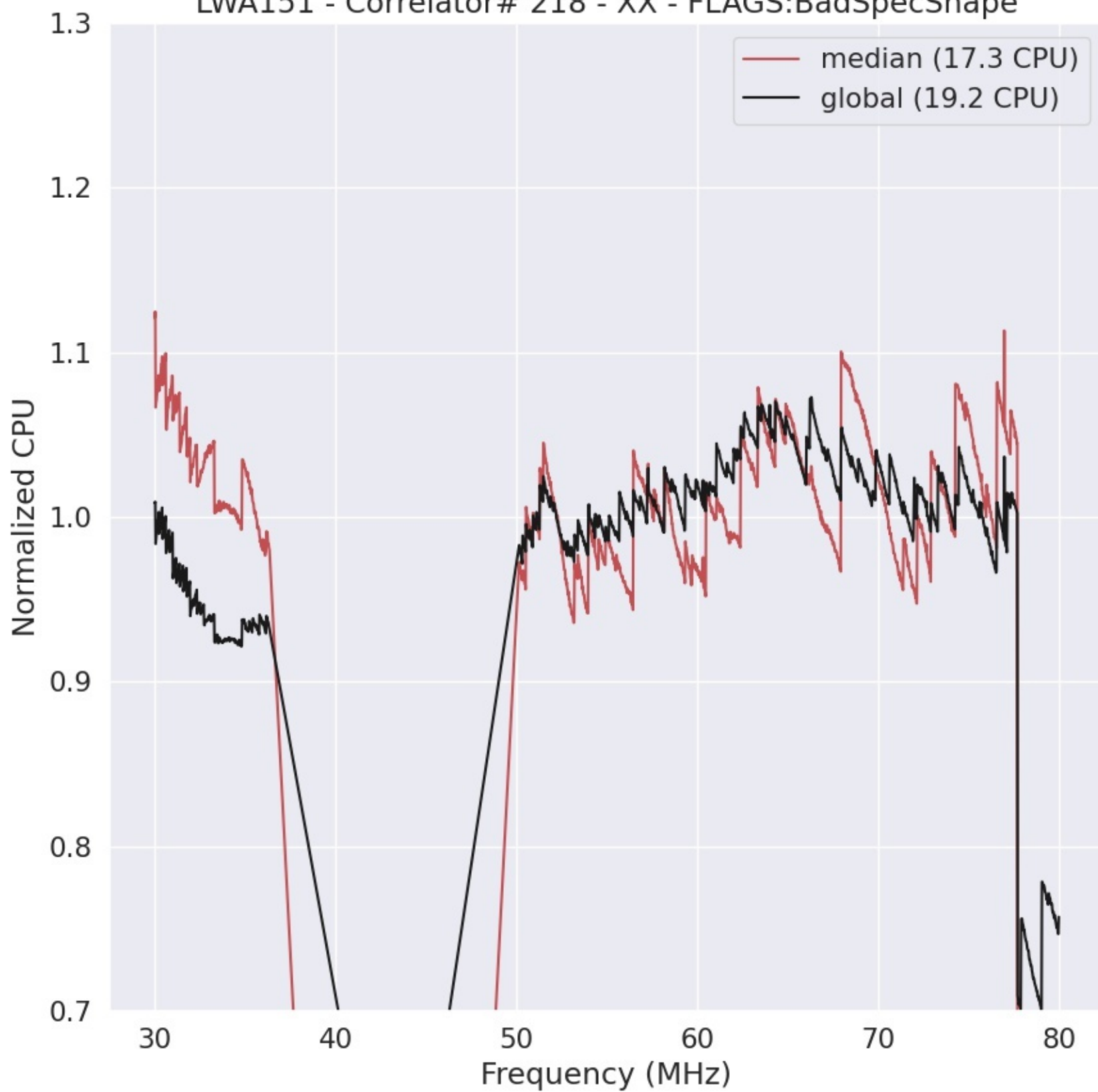
LWA151 - Correlator# 218 - XX - FLAGS:BadSpecShape
