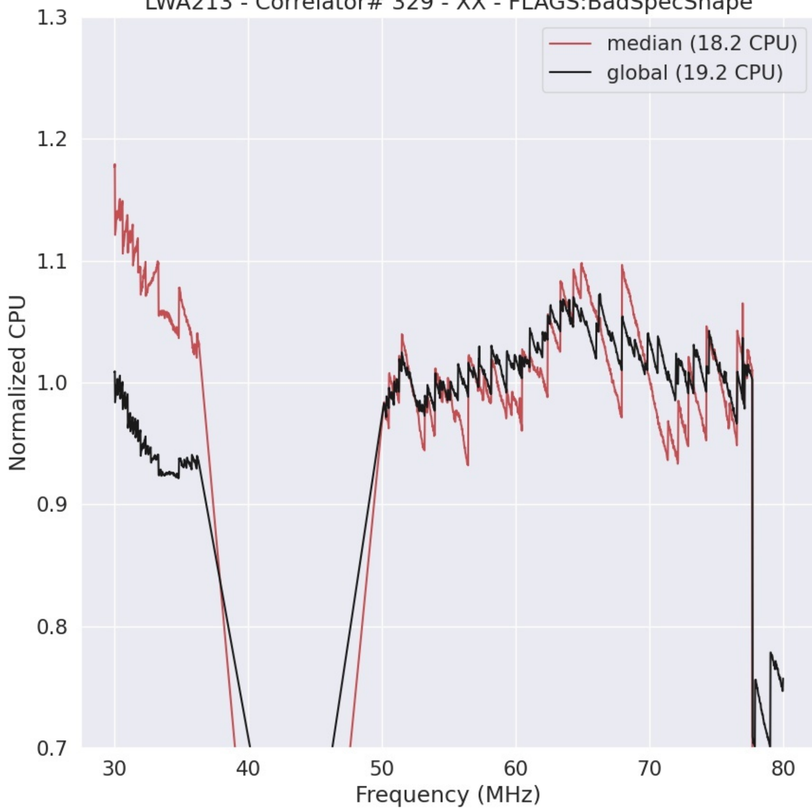
LWA213 - Correlator# 329 - XX - FLAGS:BadSpecShape
