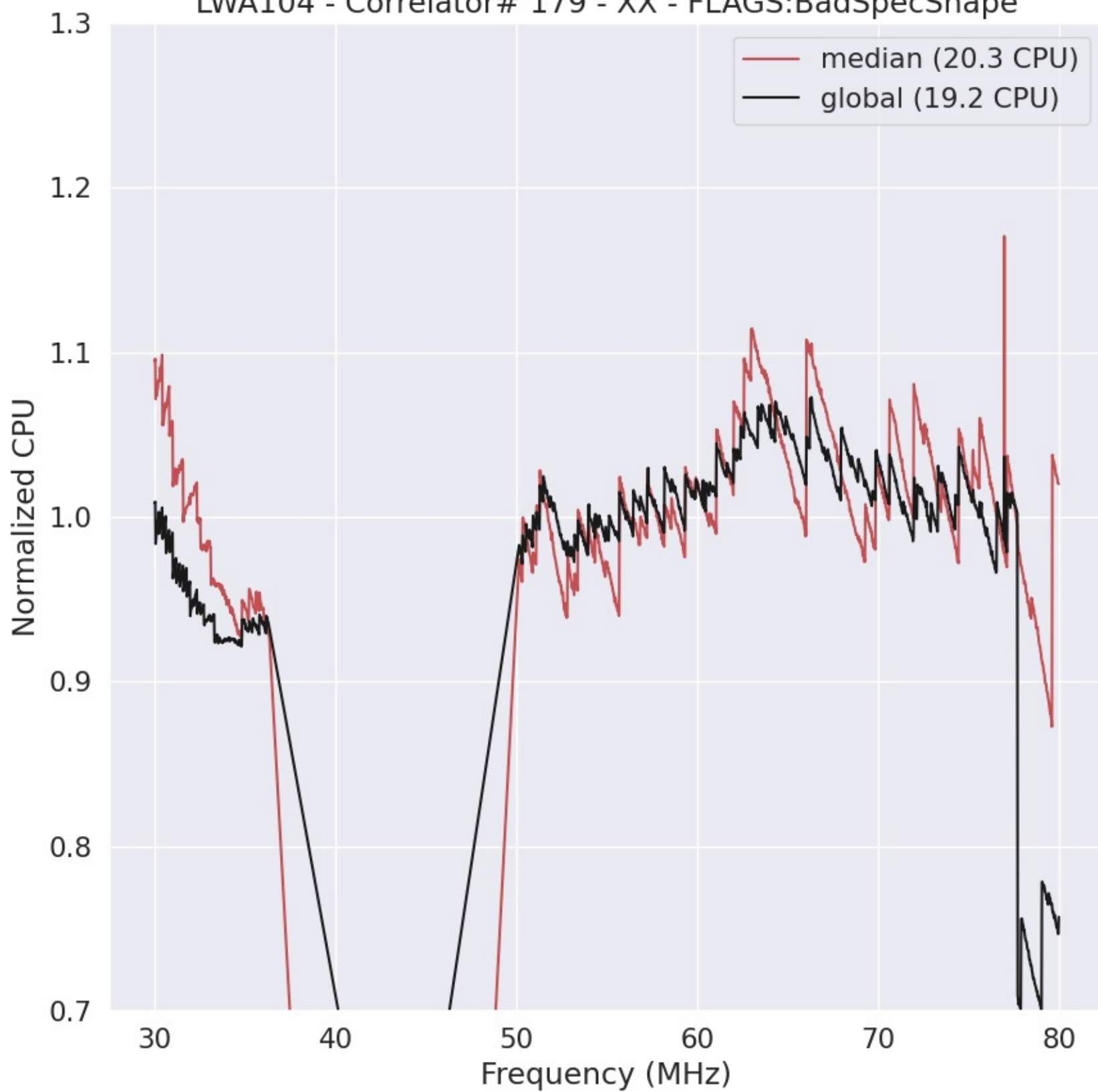
LWA104 - Correlator# 179 - XX - FLAGS:BadSpecShape
