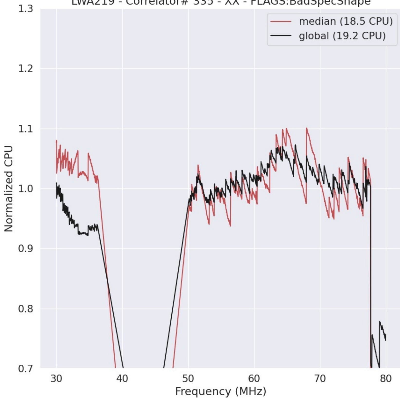
LWA219 - Correlator# 335 - XX - FLAGS:BadSpecShape
