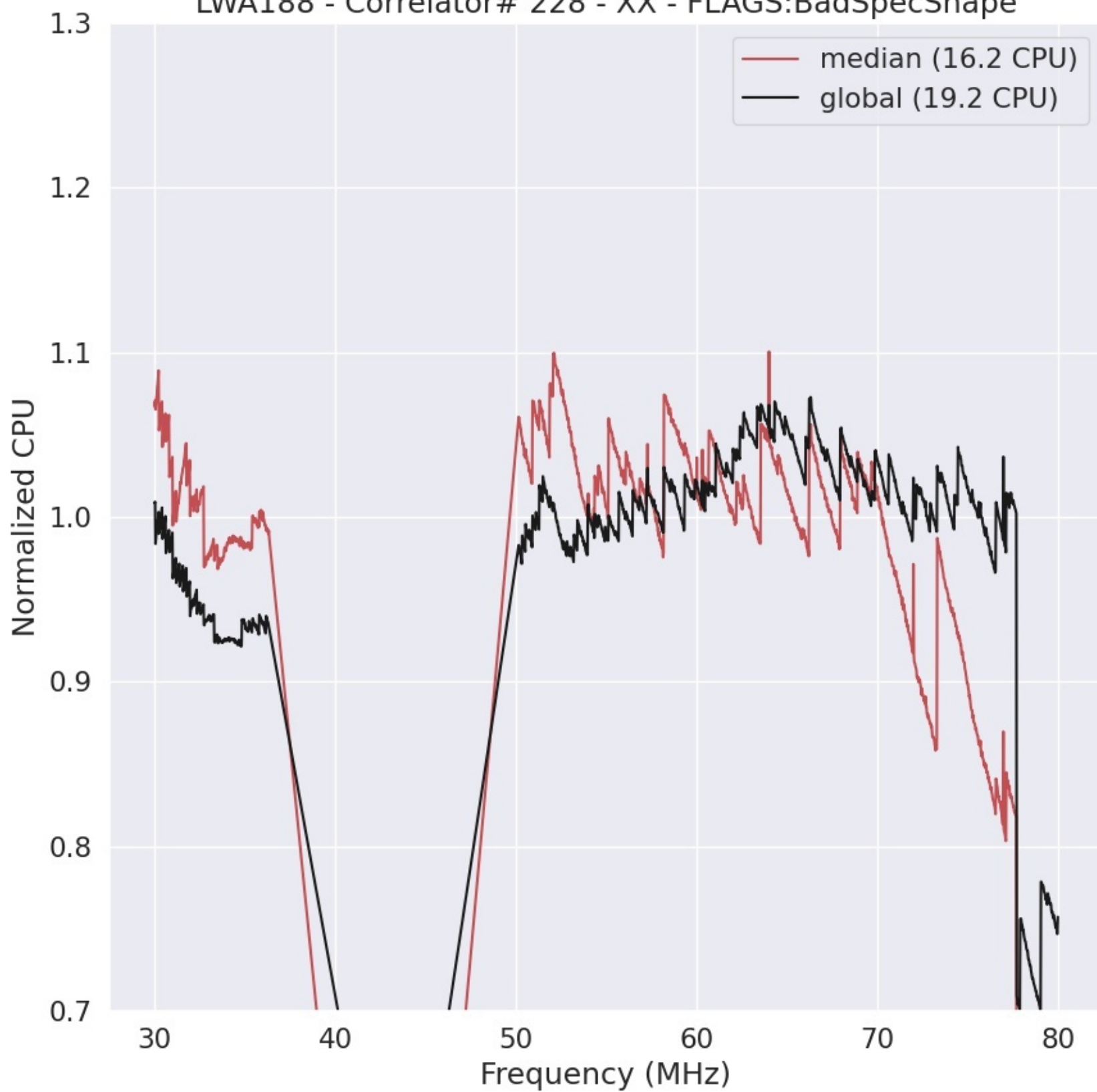
LWA188 - Correlator# 228 - XX - FLAGS:BadSpecShape
