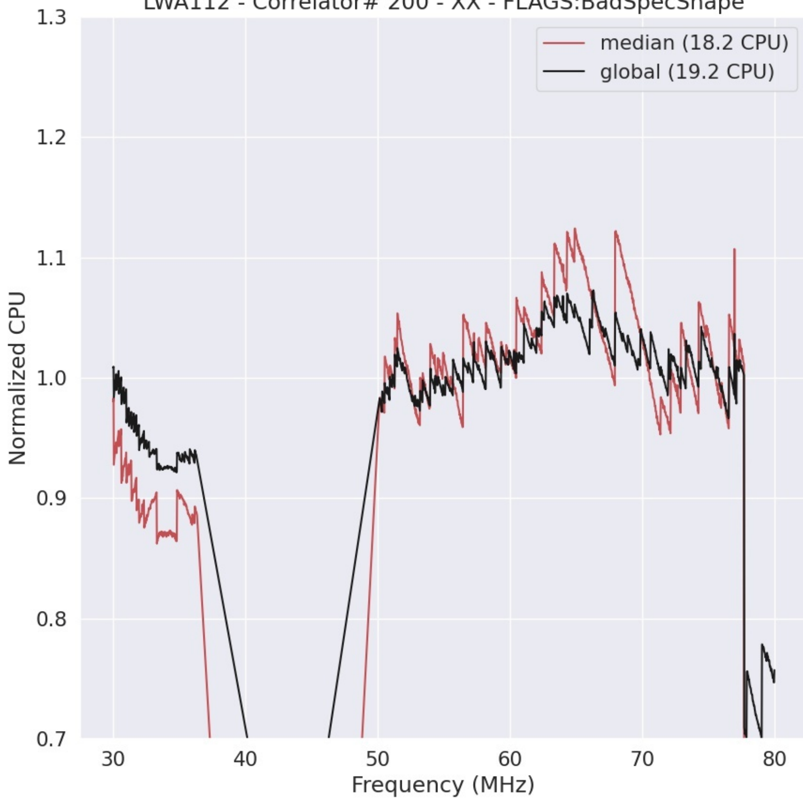
LWA112 - Correlator# 200 - XX - FLAGS:BadSpecShape
