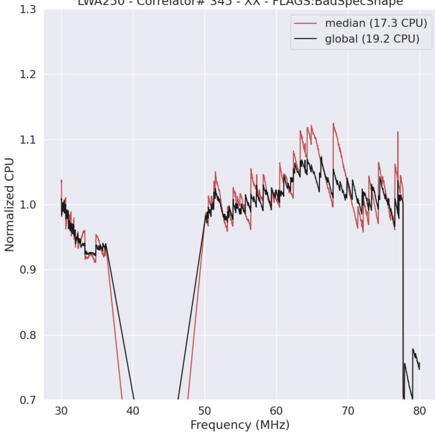
LWA250 - Correlator# 345 - XX - FLAGS:BadSpecShape
