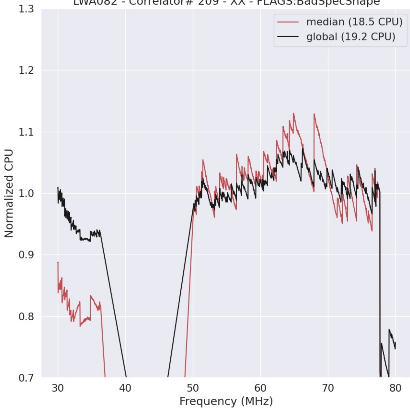
LWA082 - Correlator# 209 - XX - FLAGS:BadSpecShape
