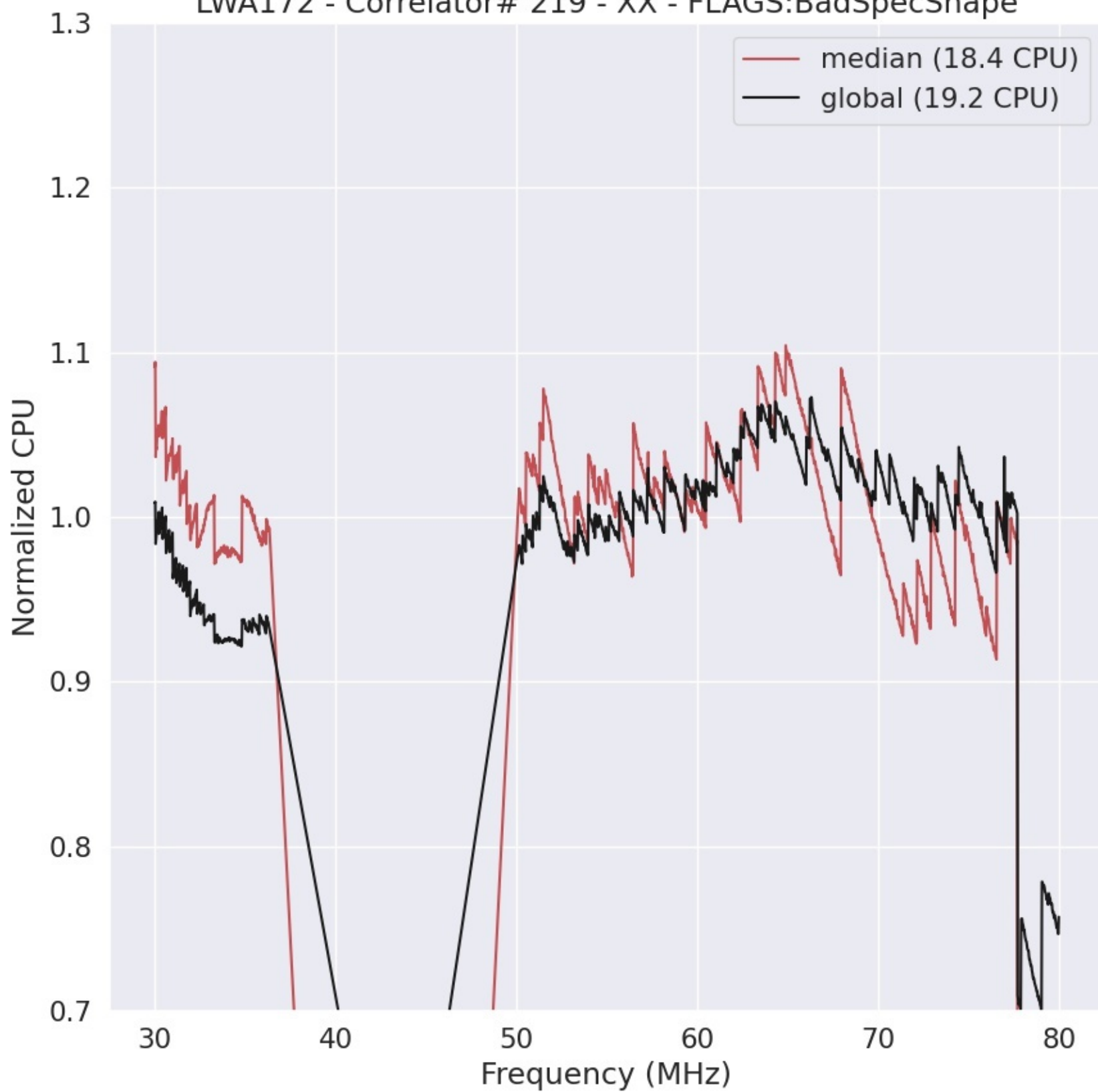
LWA172 - Correlator# 219 - XX - FLAGS:BadSpecShape
