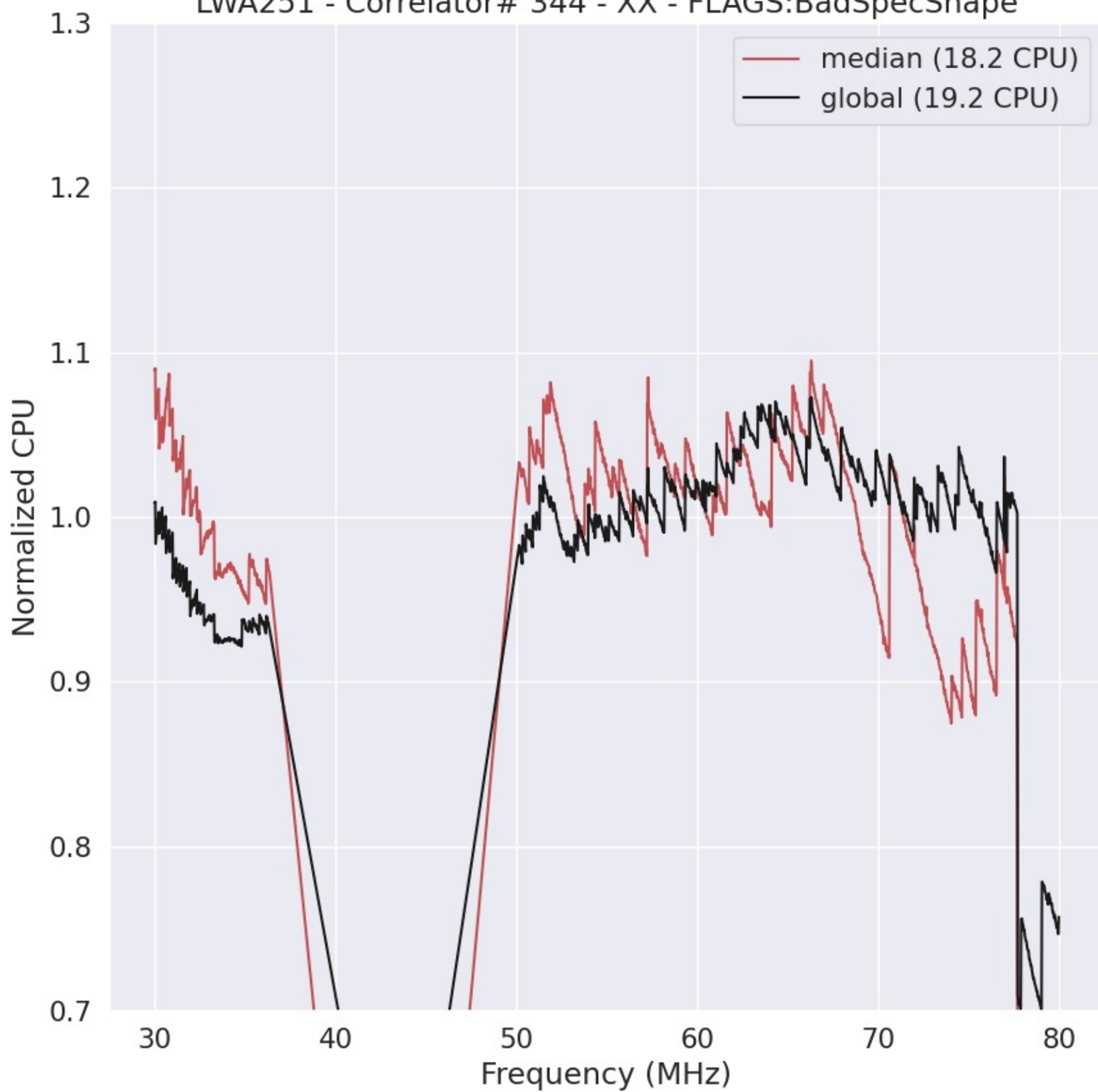
LWA251 - Correlator# 344 - XX - FLAGS:BadSpecShape
