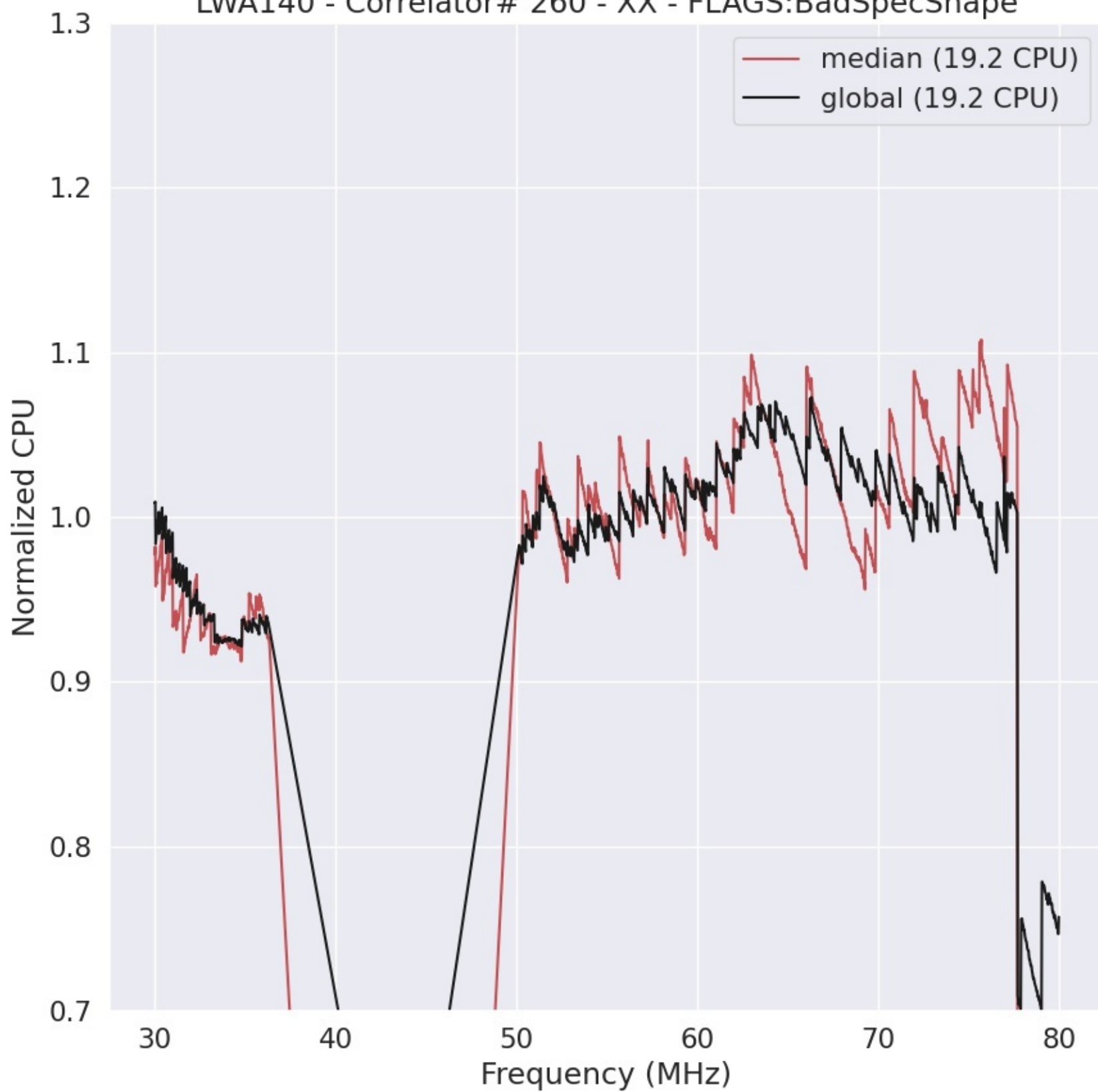
LWA140 - Correlator# 260 - XX - FLAGS:BadSpecShape
