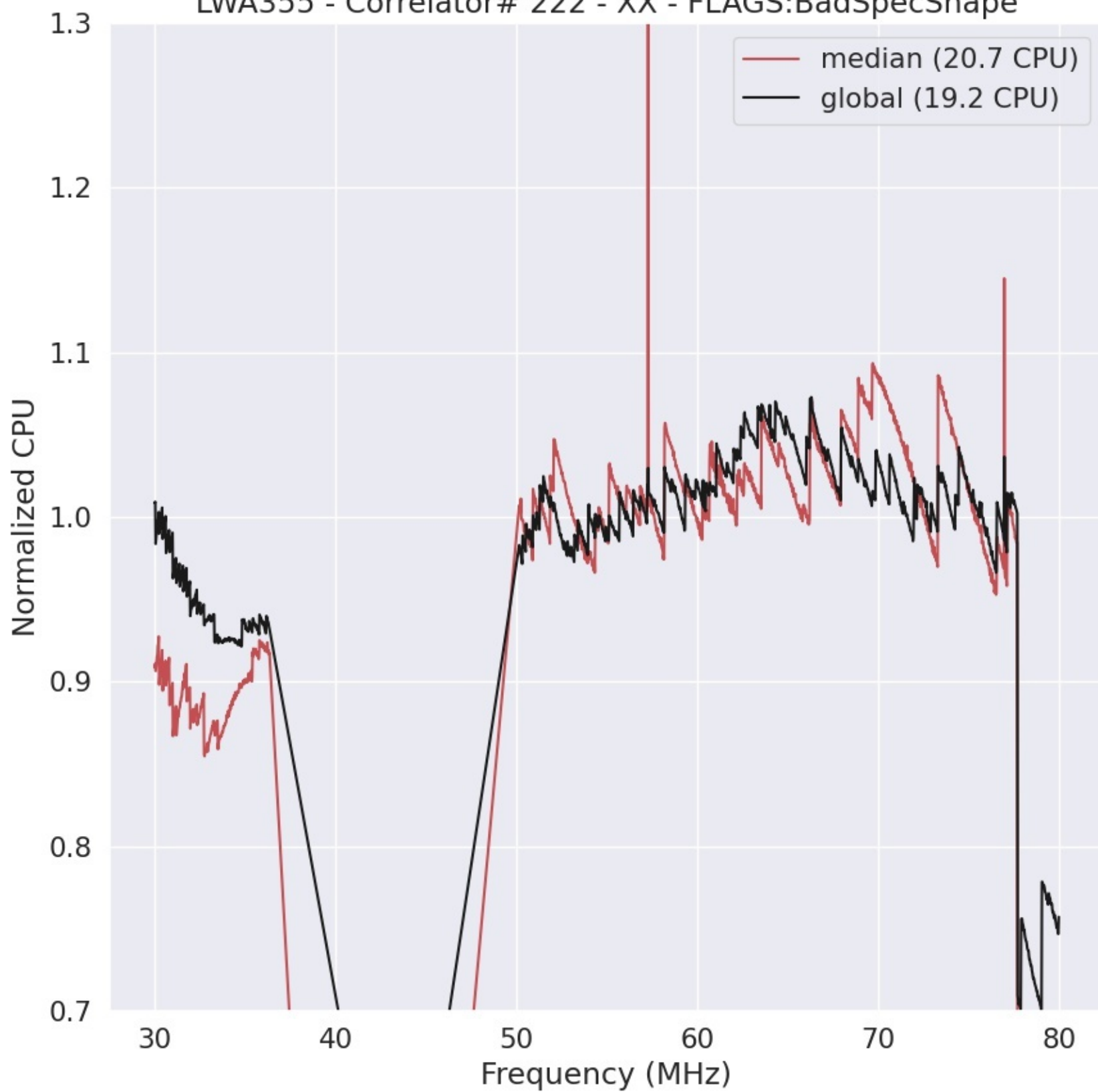
LWA355 - Correlator# 222 - XX - FLAGS:BadSpecShape
