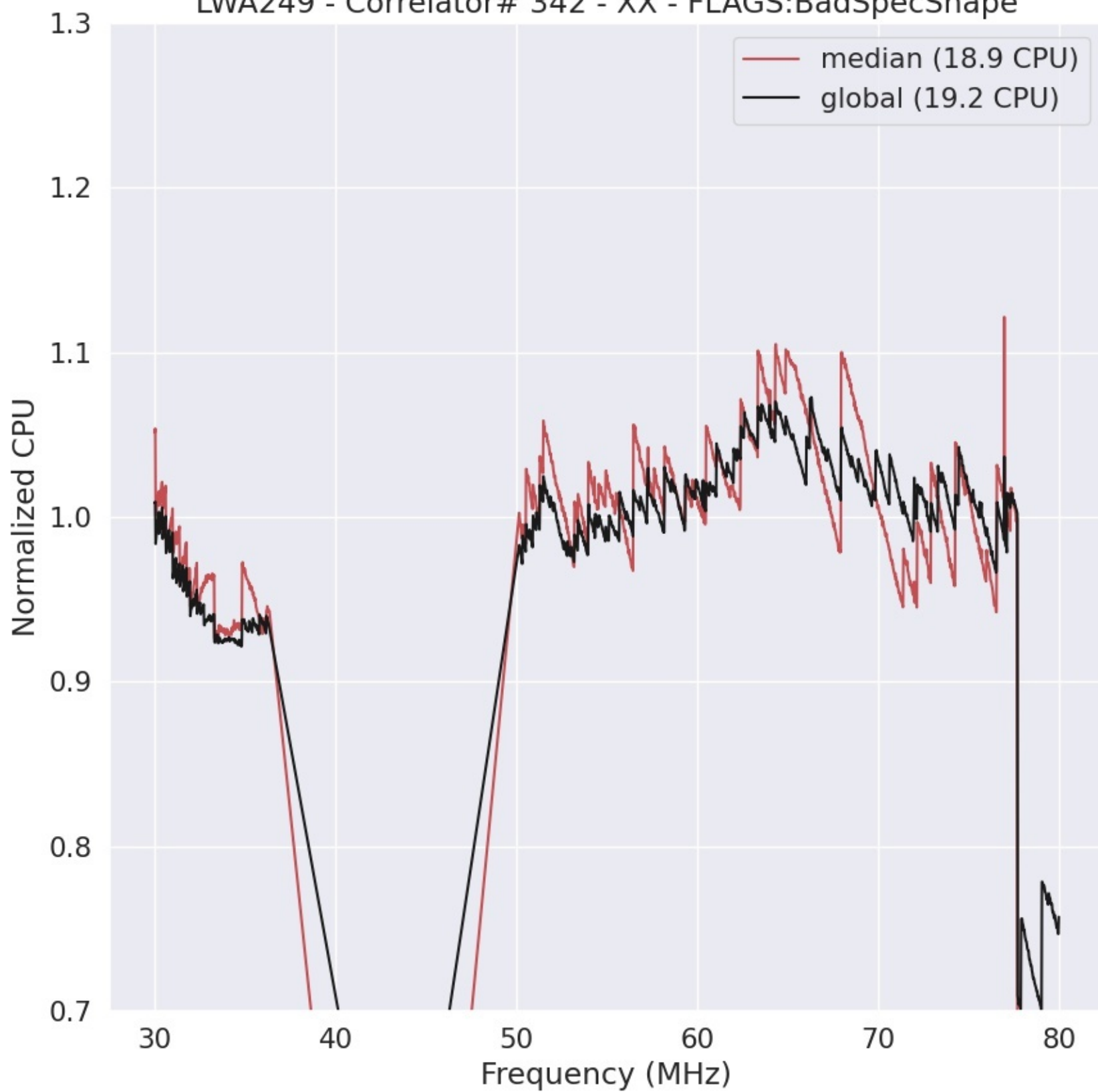
LWA249 - Correlator# 342 - XX - FLAGS:BadSpecShape
