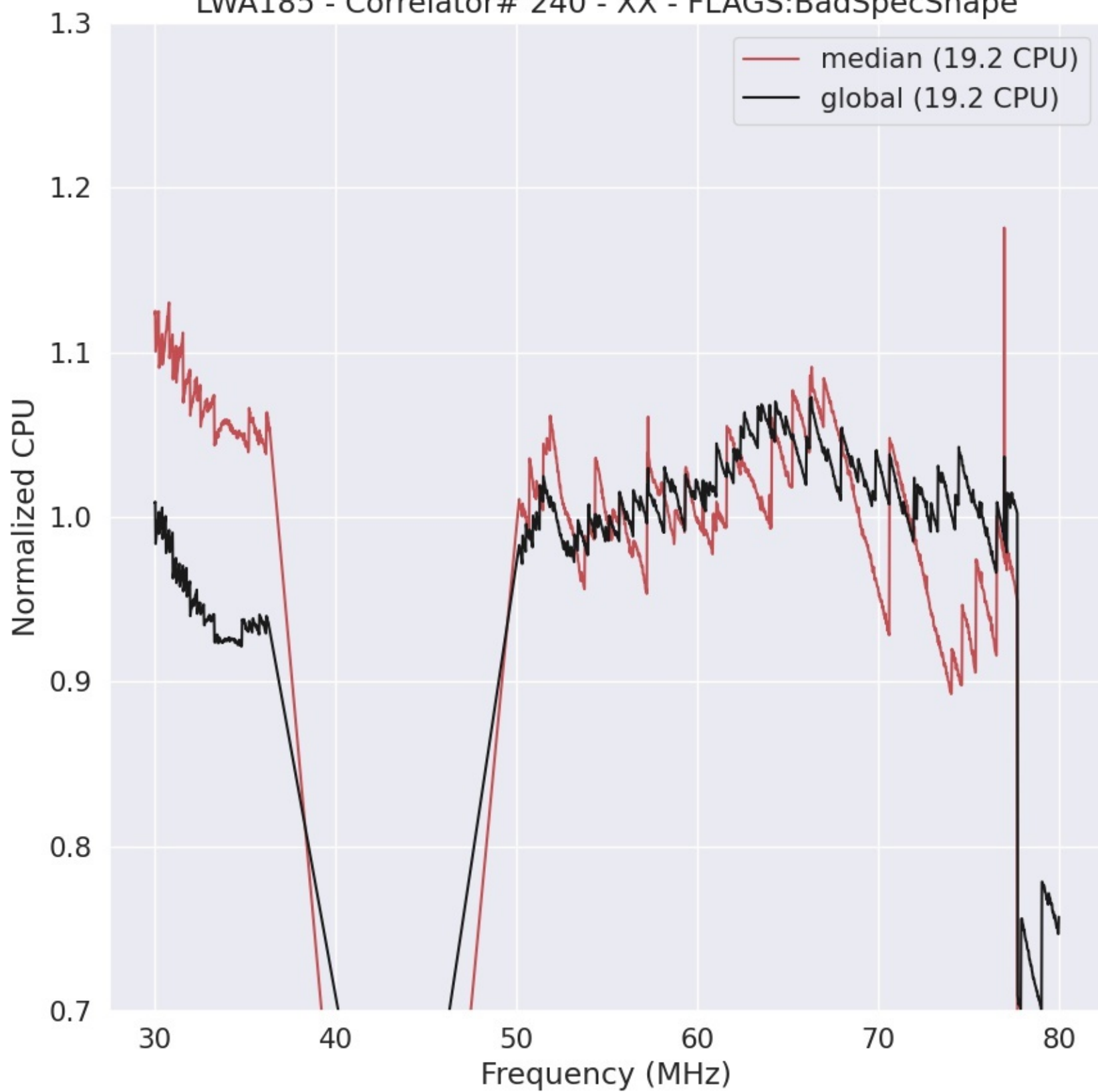
LWA185 - Correlator# 240 - XX - FLAGS:BadSpecShape
