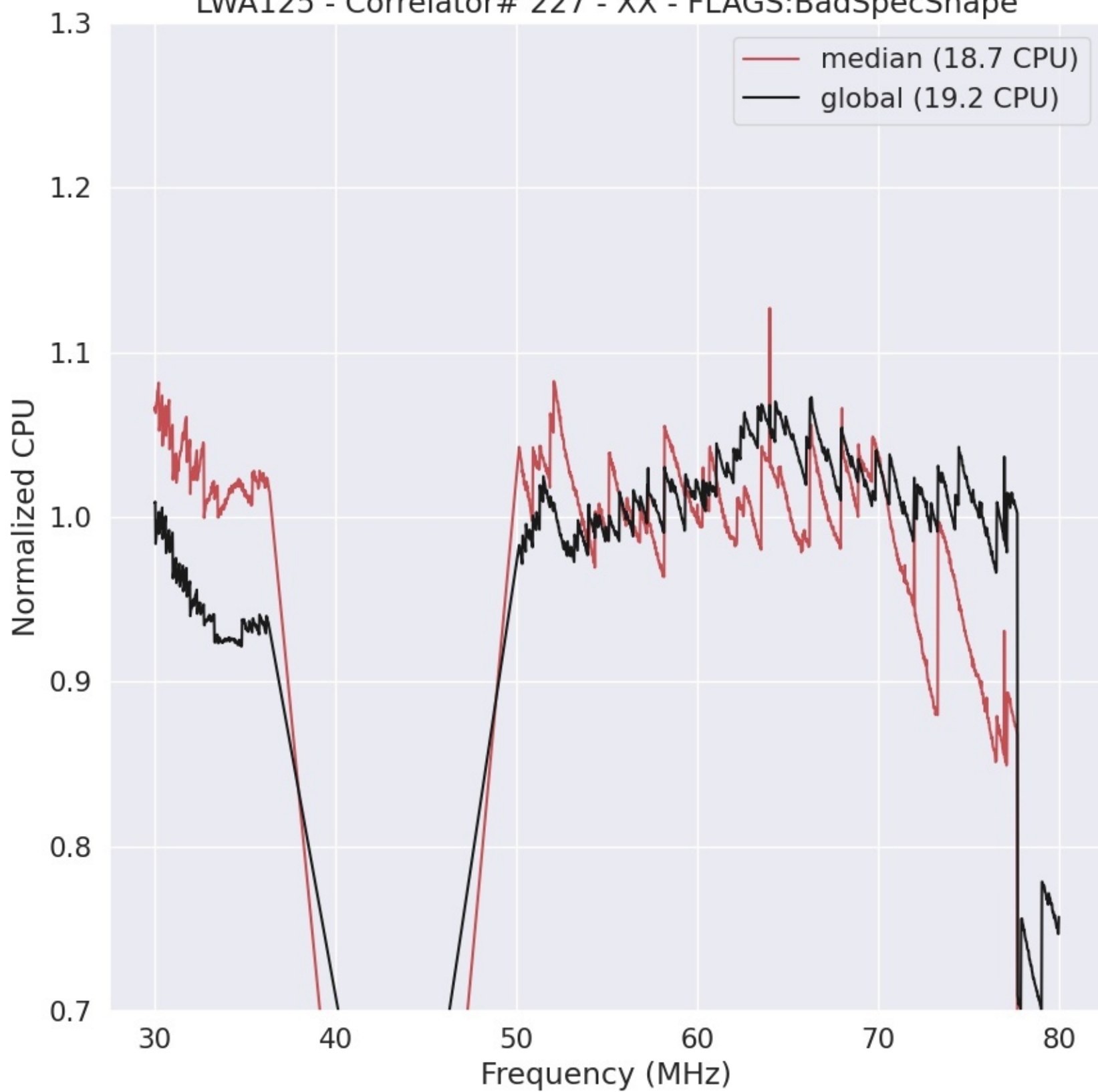
LWA125 - Correlator# 227 - XX - FLAGS:BadSpecShape
