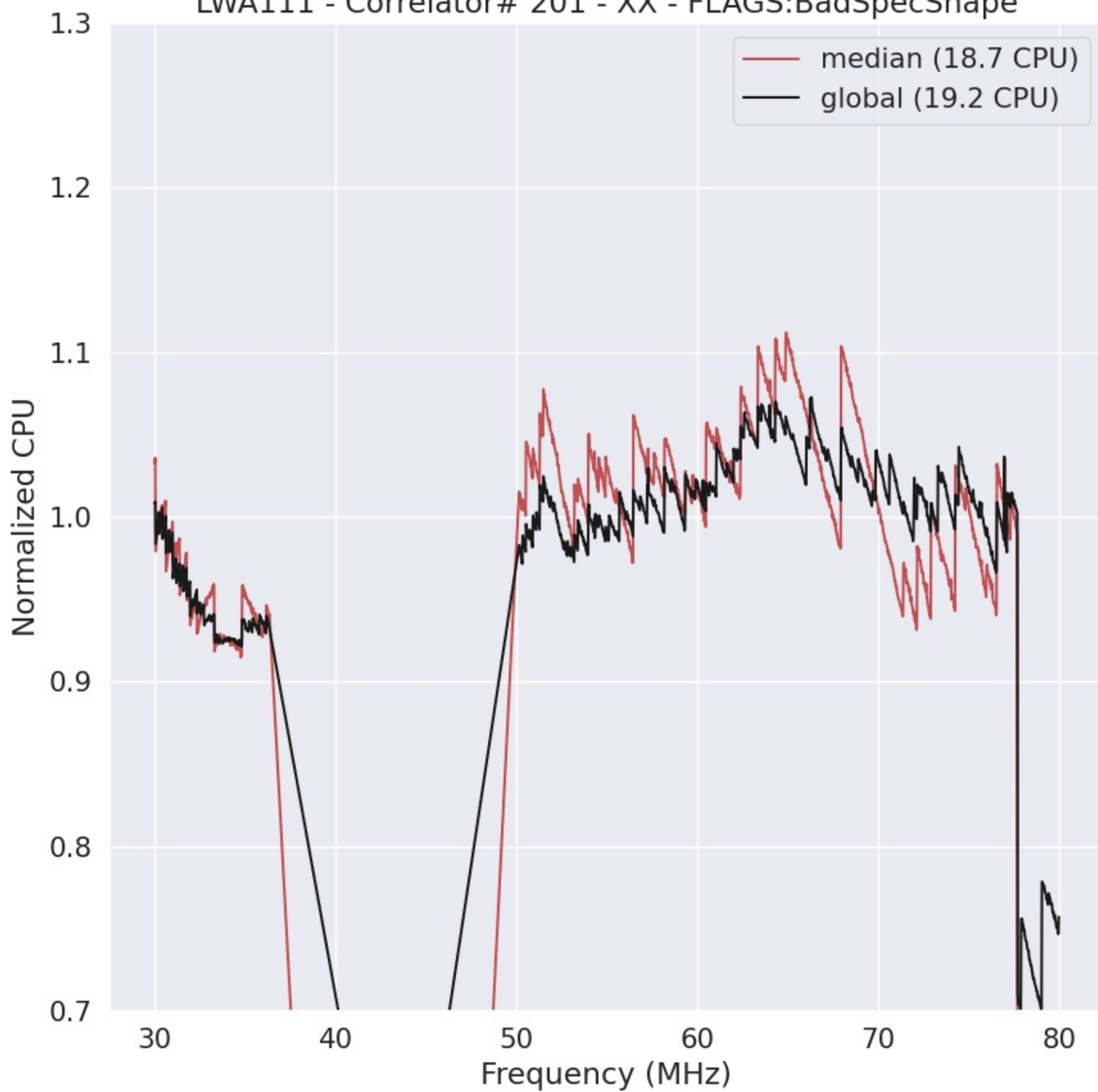
LWA111 - Correlator# 201 - XX - FLAGS:BadSpecShape
