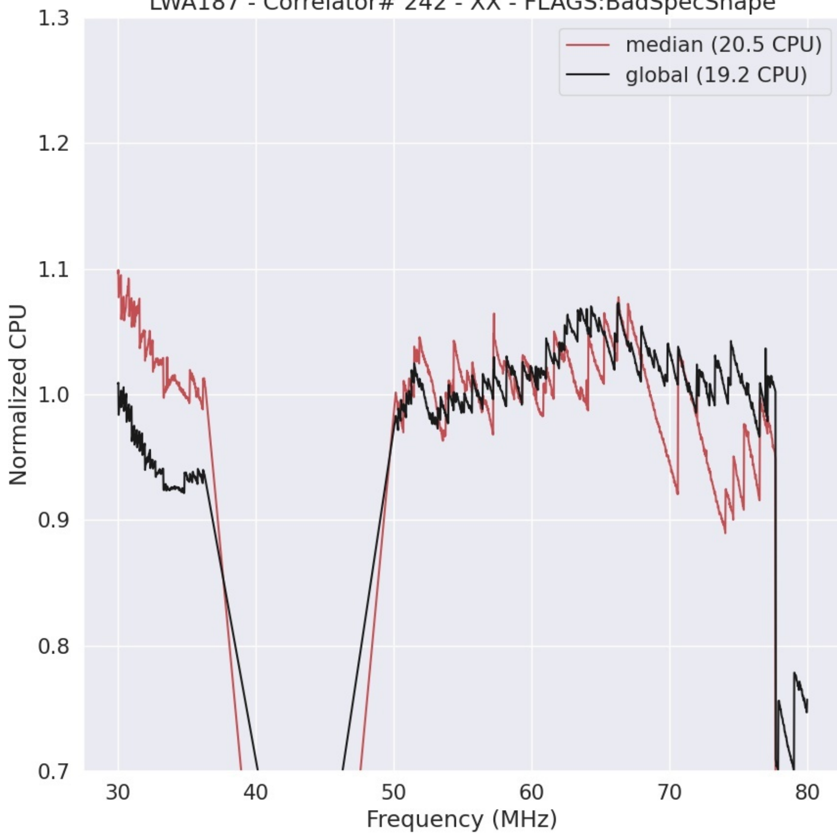
LWA187 - Correlator# 242 - XX - FLAGS:BadSpecShape
