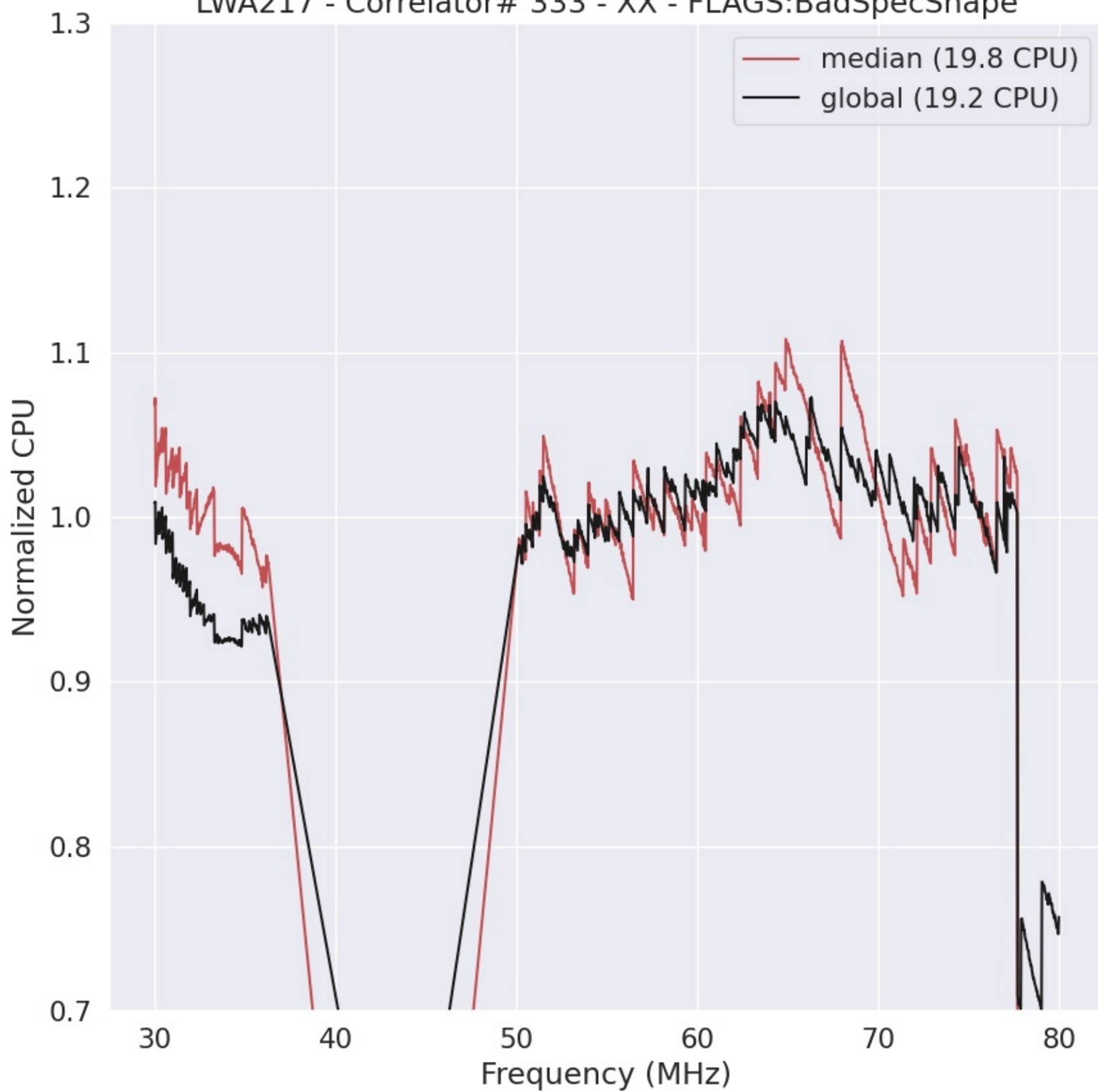
LWA217 - Correlator# 333 - XX - FLAGS:BadSpecShape
