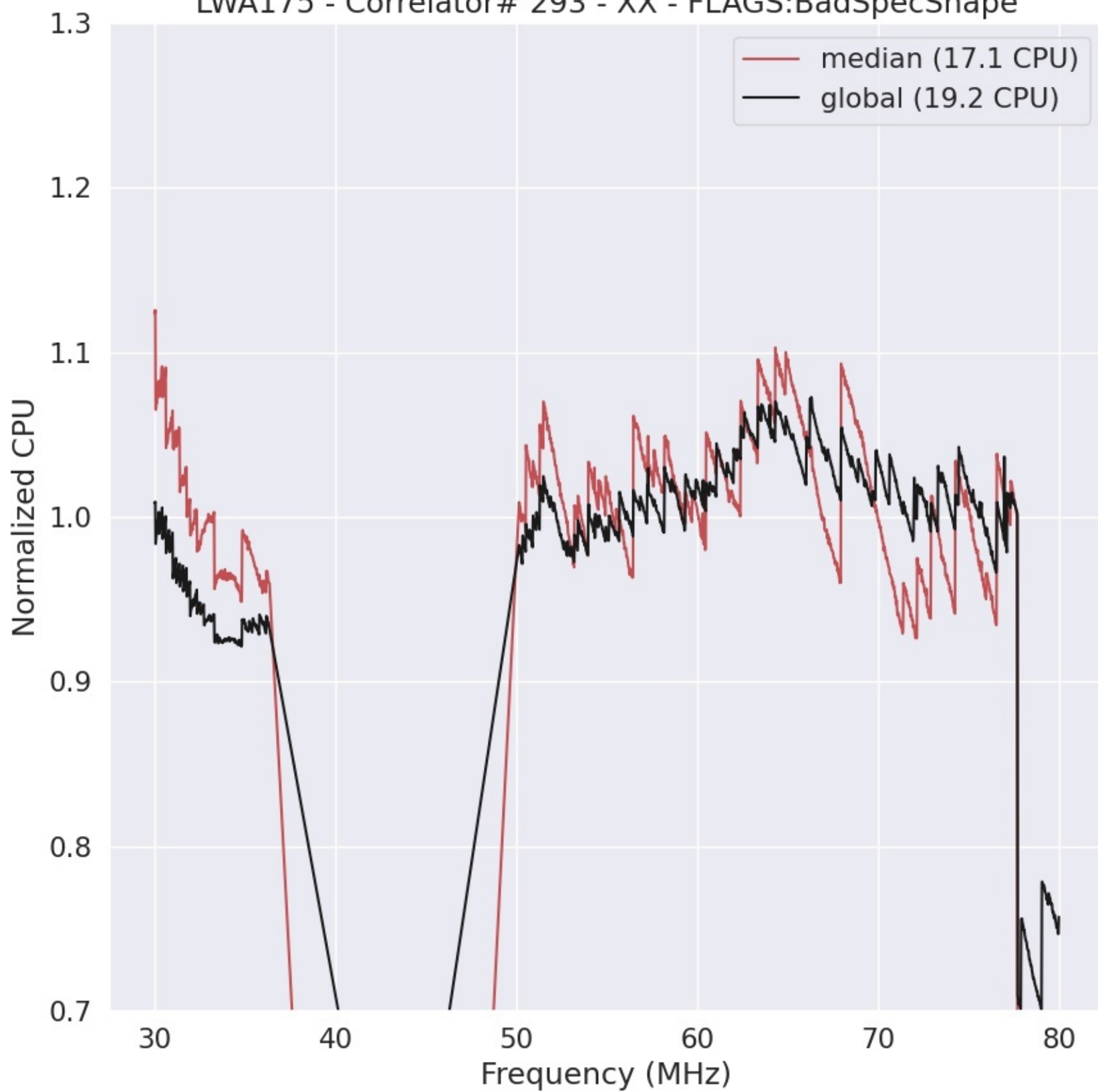
LWA175 - Correlator# 293 - XX - FLAGS:BadSpecShape
