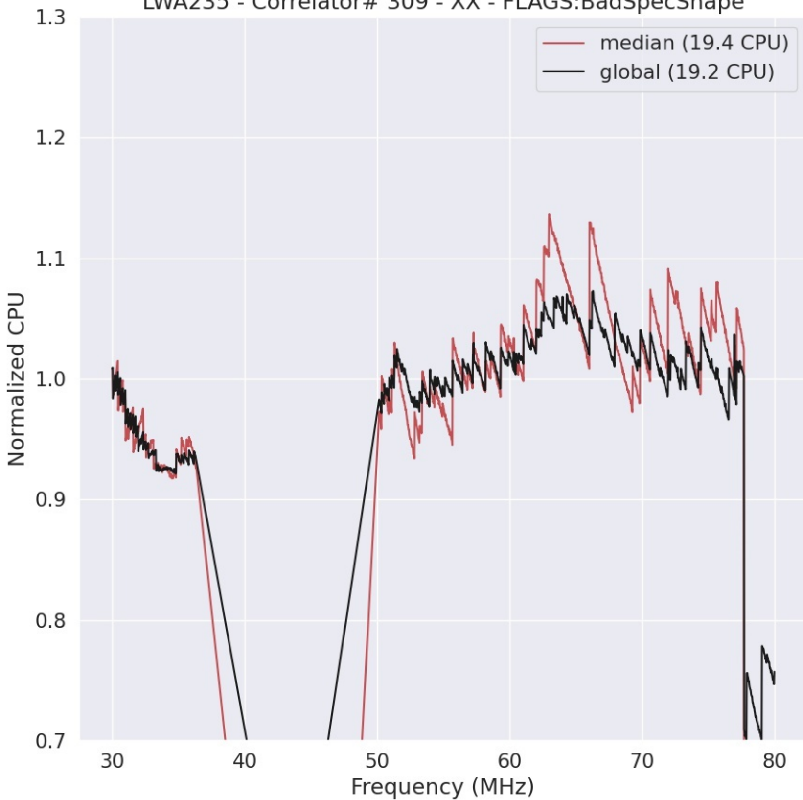
LWA235 - Correlator# 309 - XX - FLAGS:BadSpecShape
