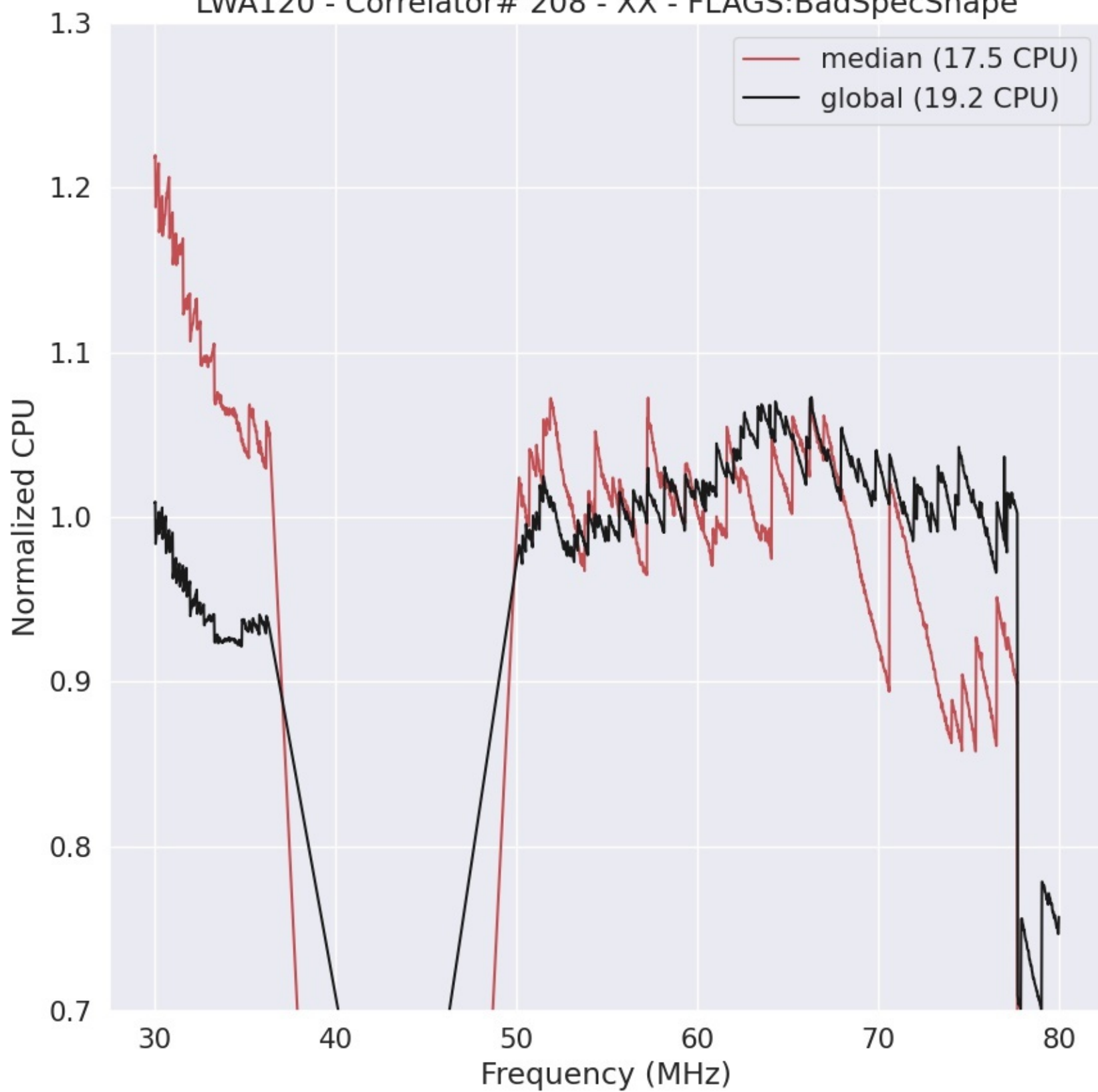
LWA120 - Correlator# 208 - XX - FLAGS:BadSpecShape
