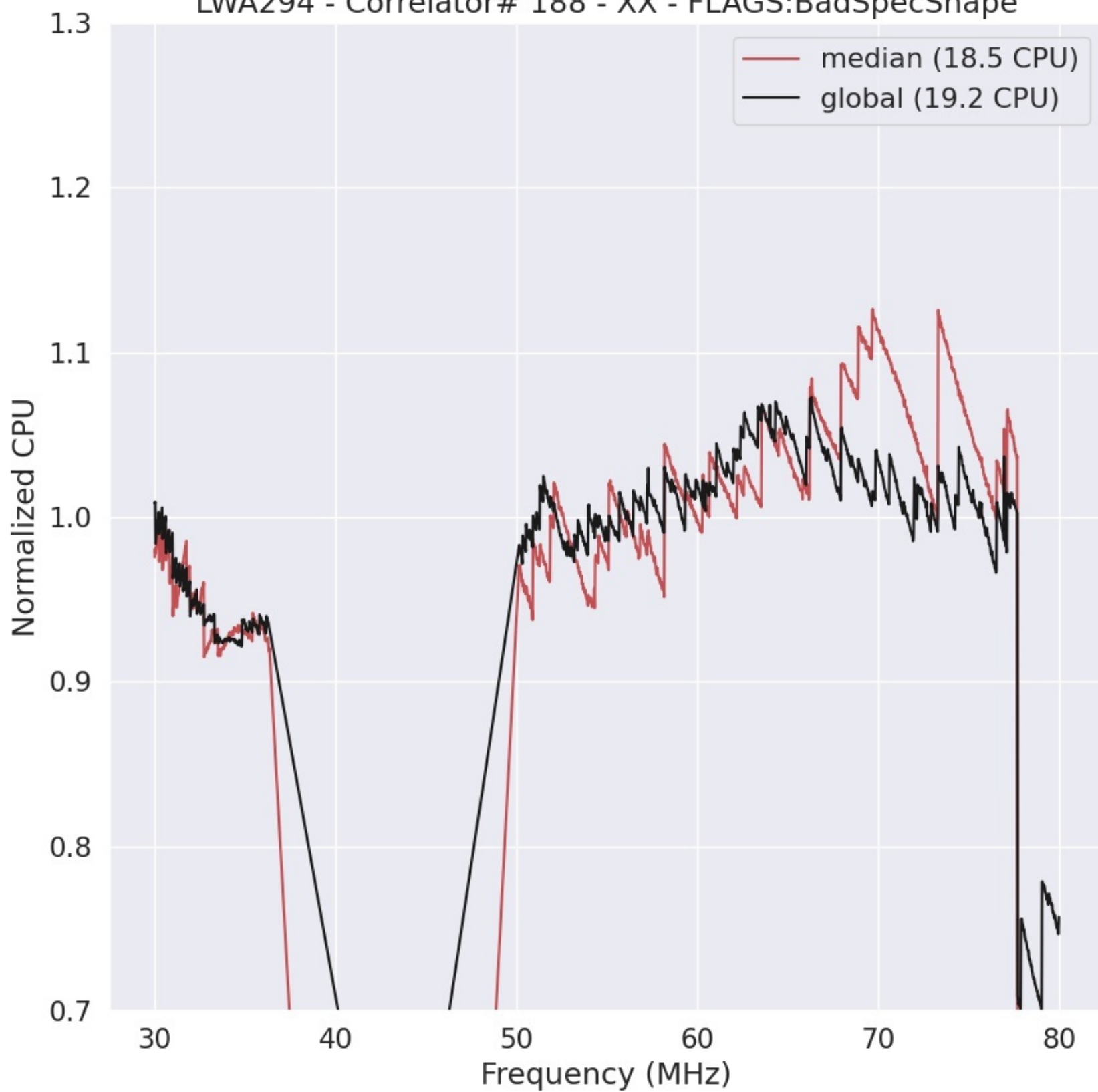
LWA294 - Correlator# 188 - XX - FLAGS:BadSpecShape
