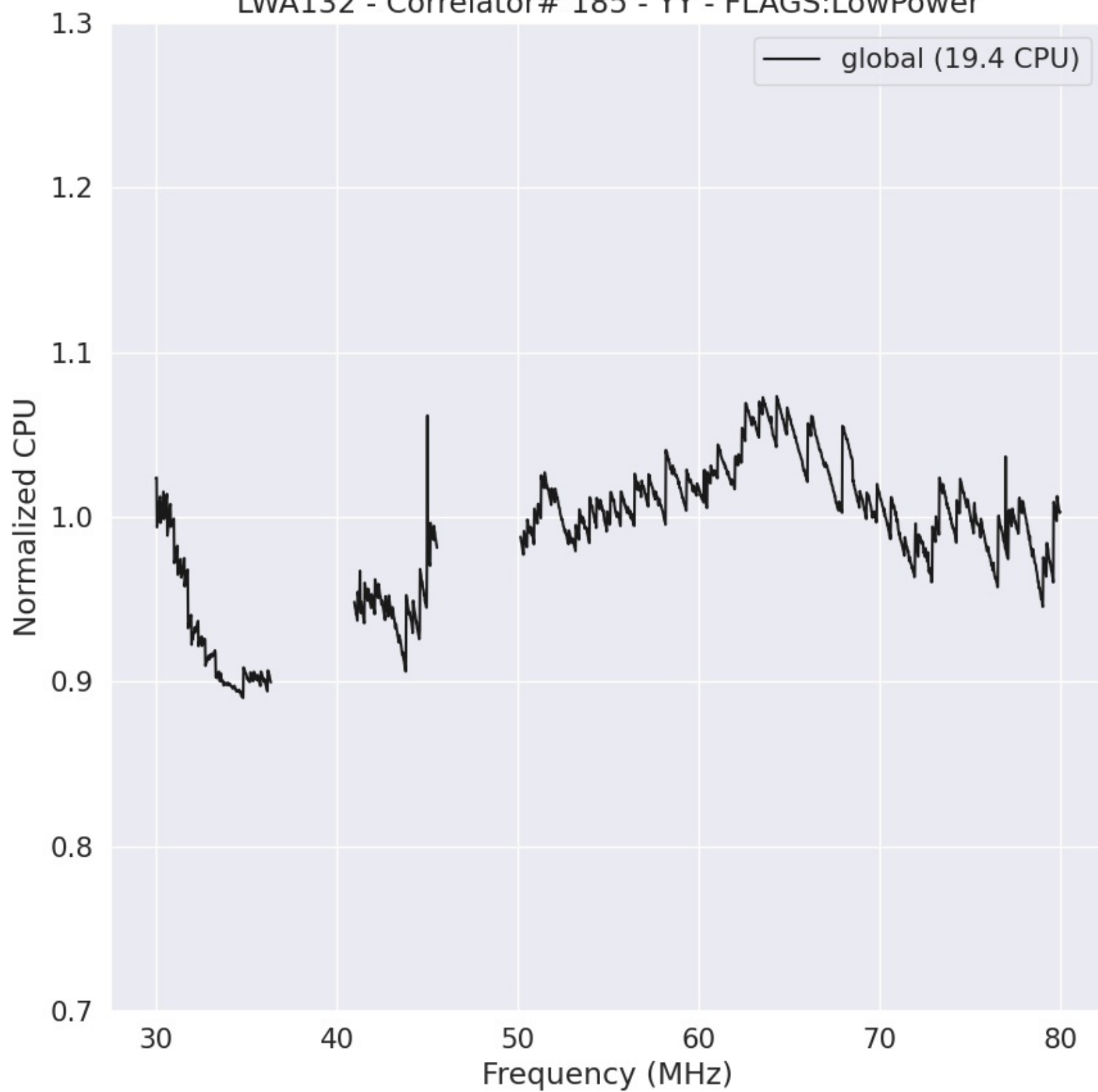
LWA132 - Correlator# 185 - YY - FLAGS:LowPower
