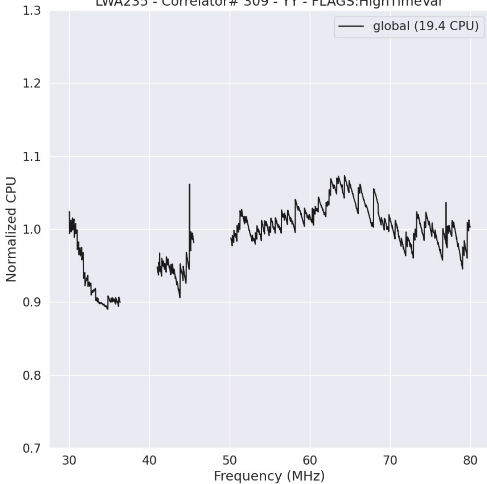
LWA235 - Correlator# 309 - YY - FLAGS:HighTimeVar
