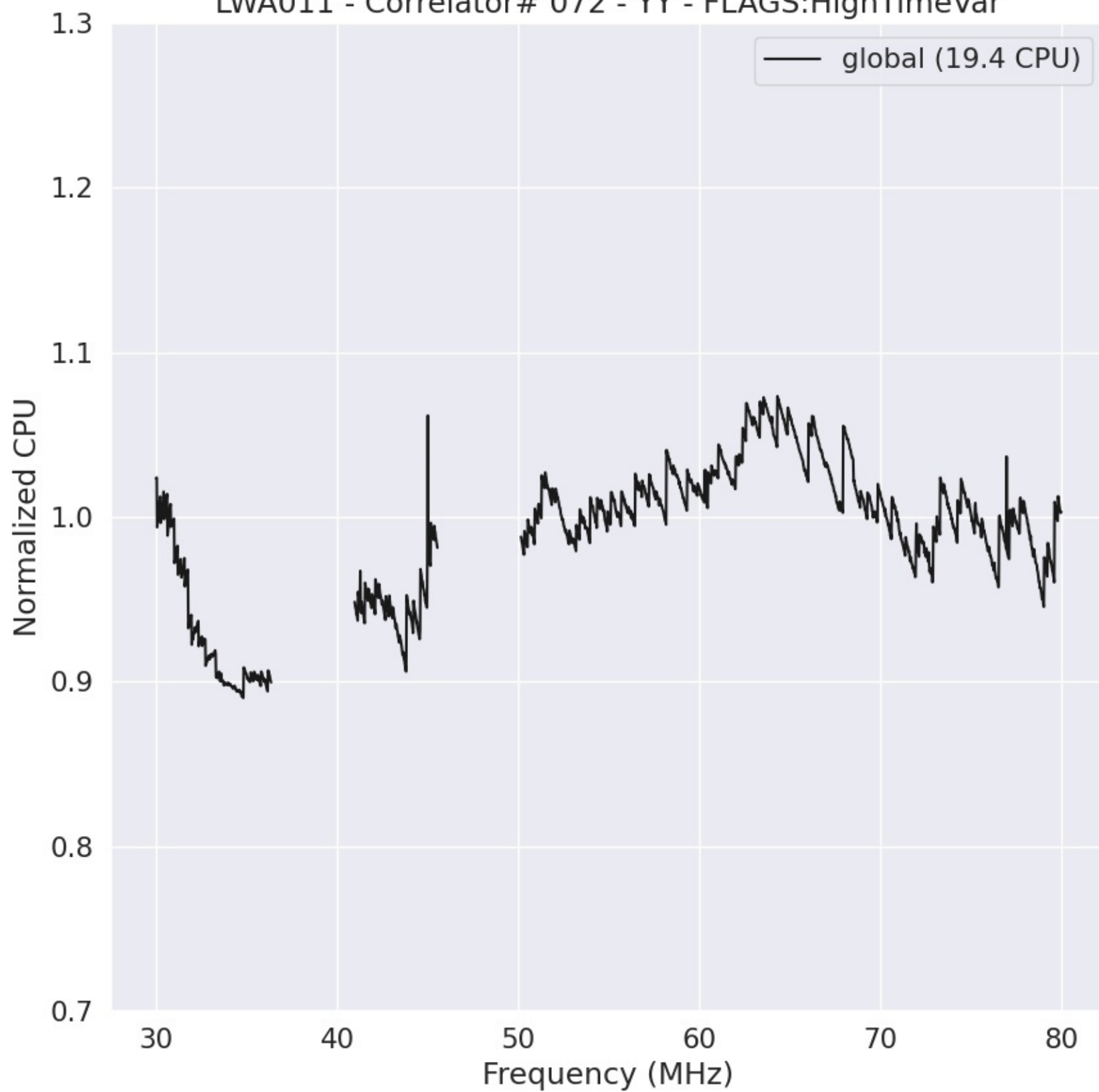
LWA011 - Correlator# 072 - YY - FLAGS:HighTimeVar
