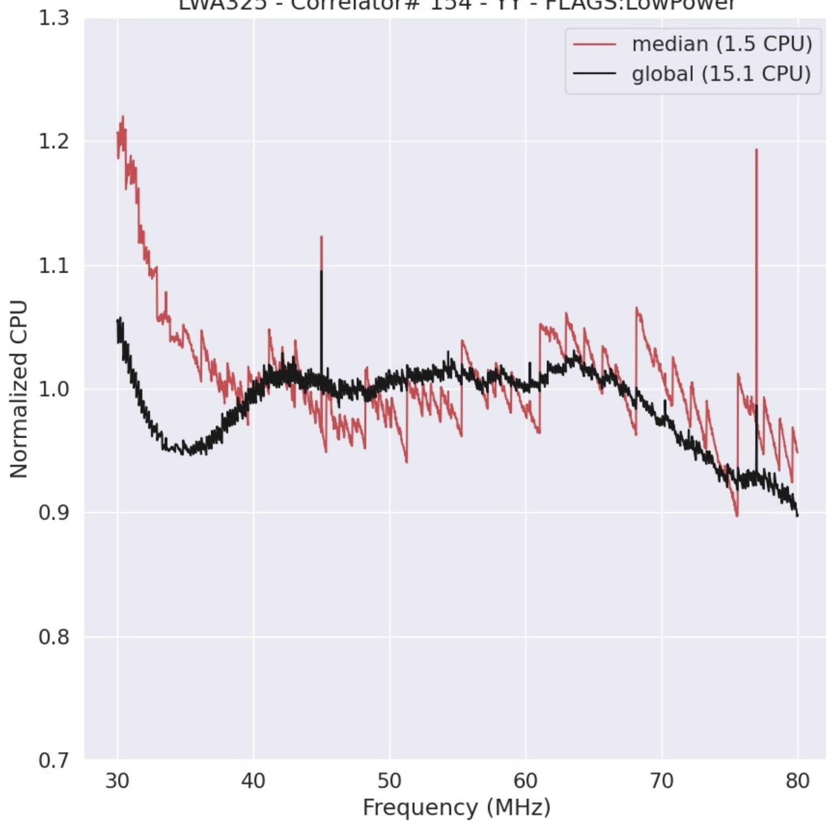
LWA325 - Correlator# 154 - YY - FLAGS:LowPower
