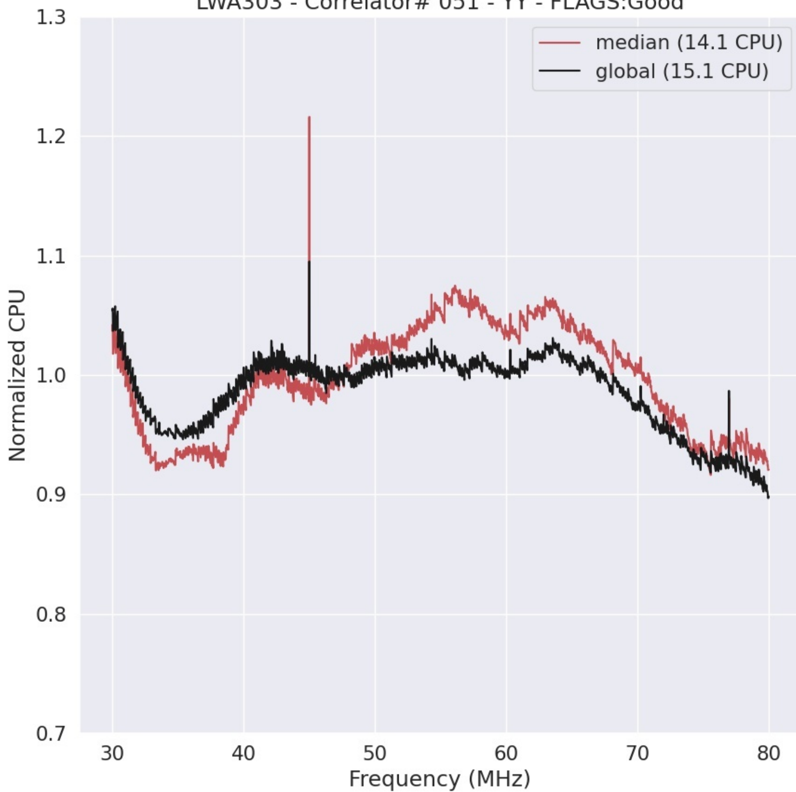
LWA303 - Correlator# 051 - YY - FLAGS:Good
