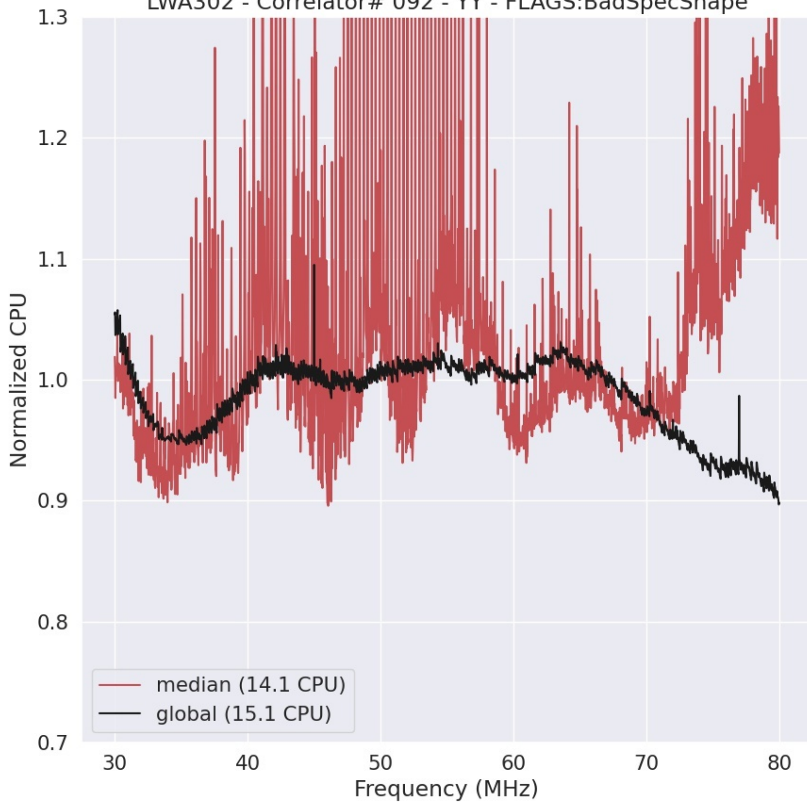
LWA302 - Correlator# 092 - YY - FLAGS:BadSpecShape
