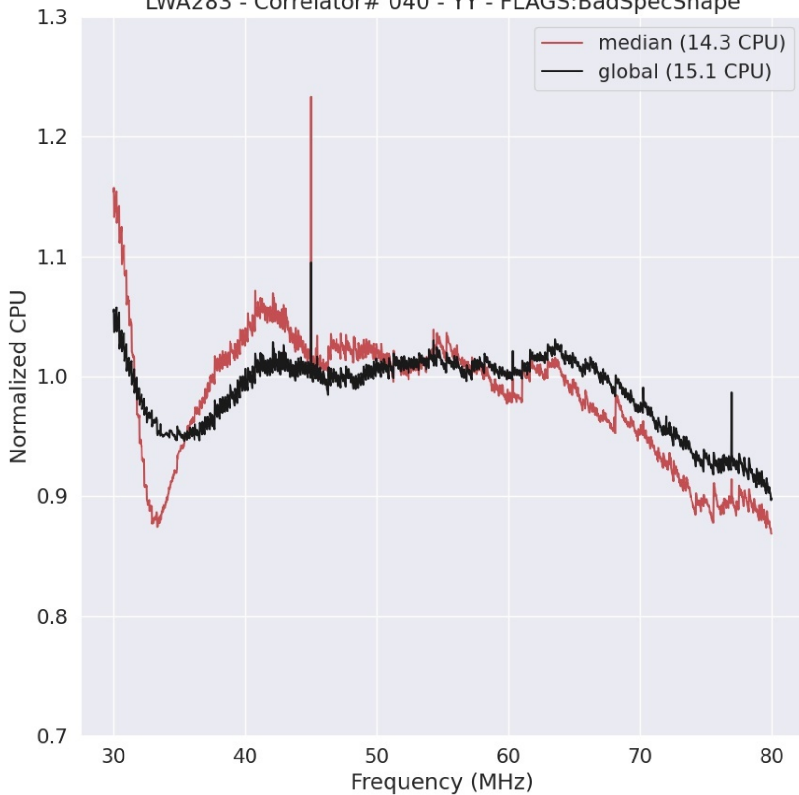
LWA283 - Correlator# 040 - YY - FLAGS:BadSpecShape
