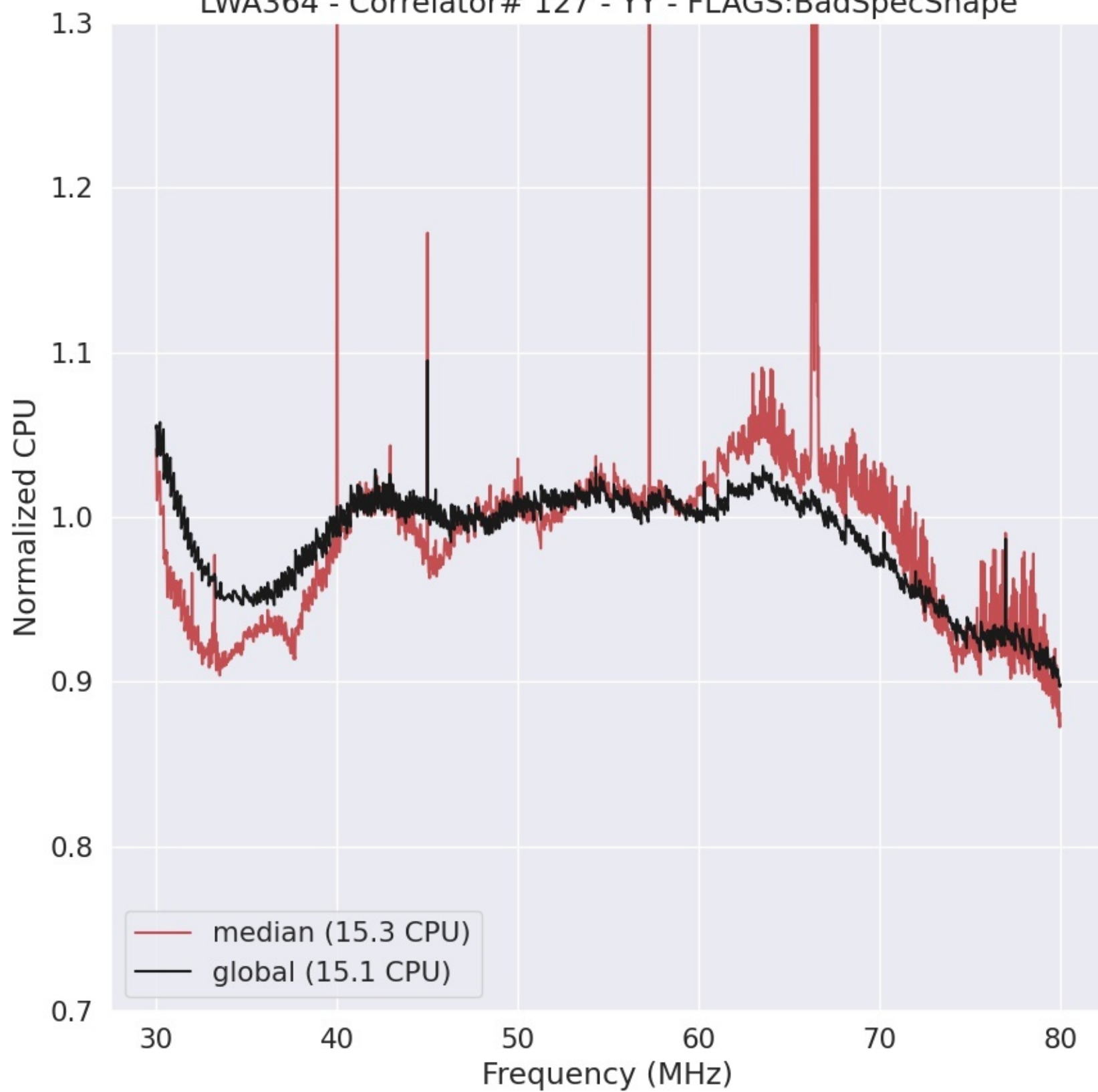
LWA364 - Correlator# 127 - YY - FLAGS:BadSpecShape
