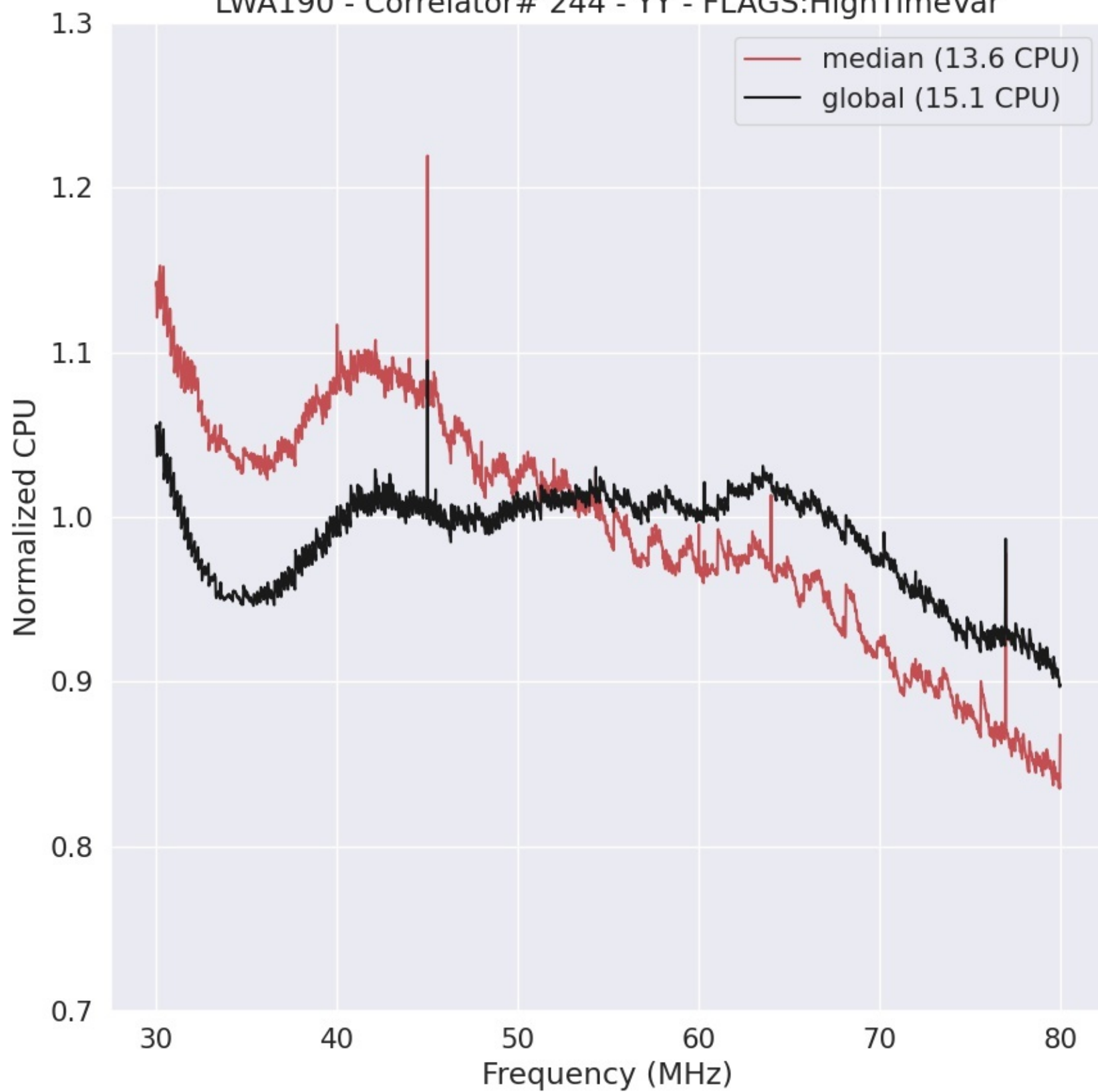
LWA190 - Correlator# 244 - YY - FLAGS:HighTimeVar
