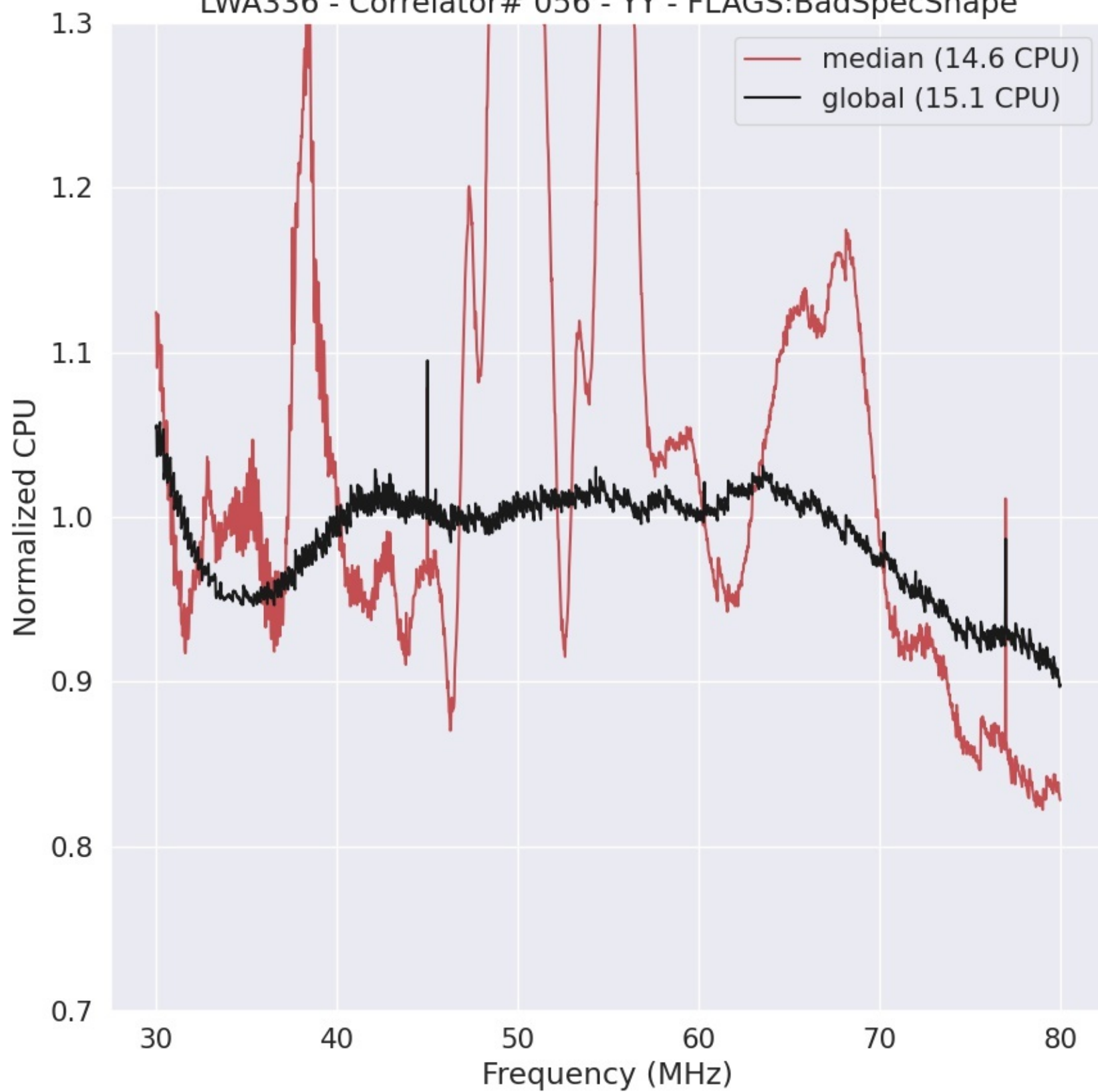
LWA336 - Correlator# 056 - YY - FLAGS:BadSpecShape
