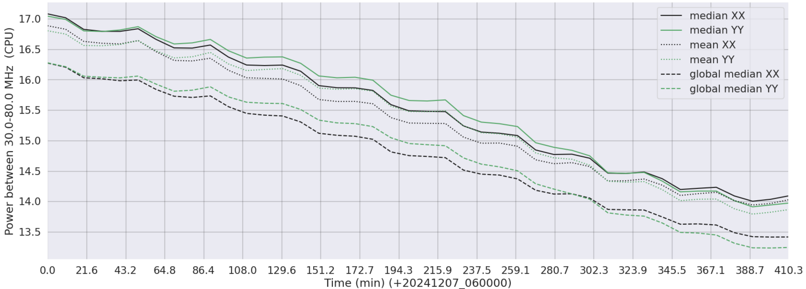
LWA197 - Correlator# 274 - XX FLAGS:Good - YY FLAGS:Good
