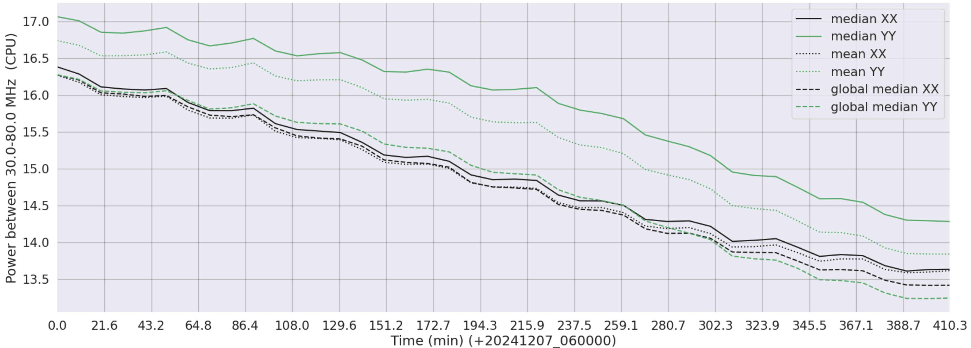
LWA003 - Correlator# 067 - XX FLAGS:Good - YY FLAGS:Good
