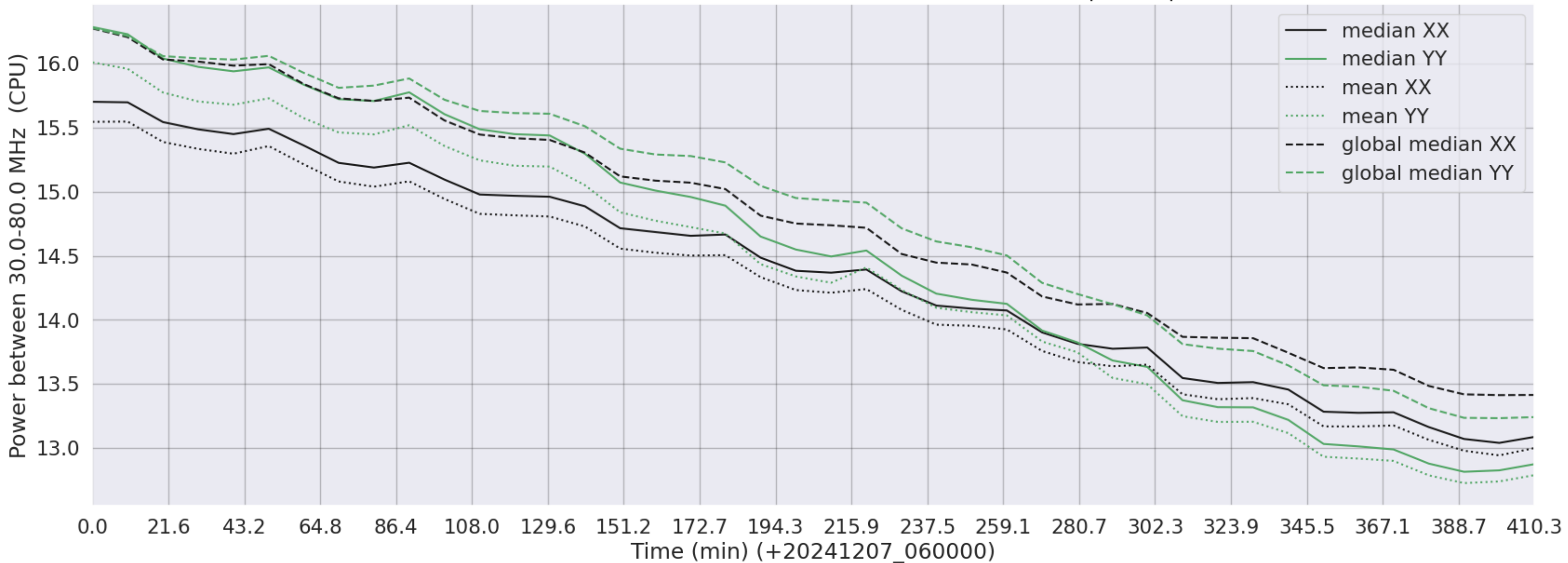
LWA348 - Correlator# 124 - XX FLAGS:Good - YY FLAGS:BadSpecShape
