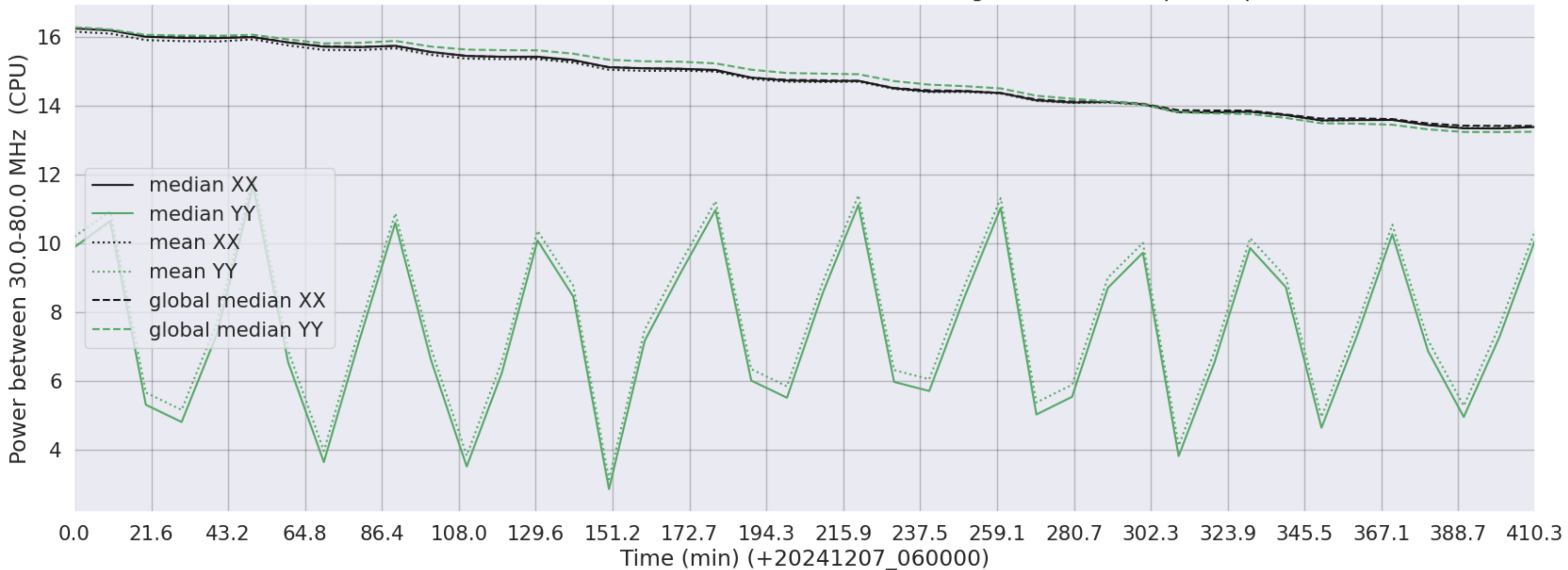
LWA235 - Correlator# 309 - XX FLAGS:Good - YY FLAGS:HighTimeVar+BadSpecShape
