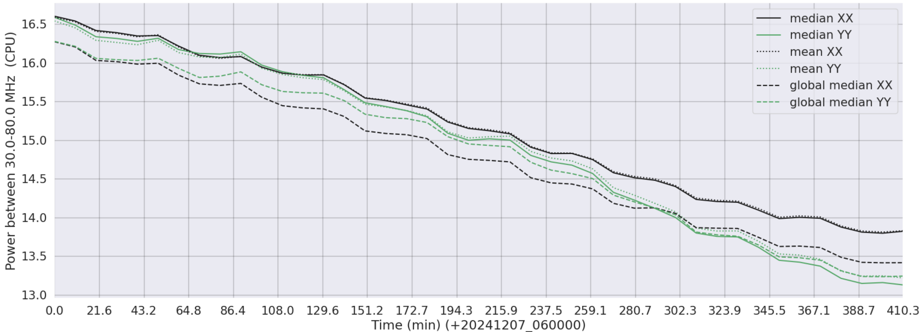
LWA354 - Correlator# 063 - XX FLAGS:Good - YY FLAGS:Good
