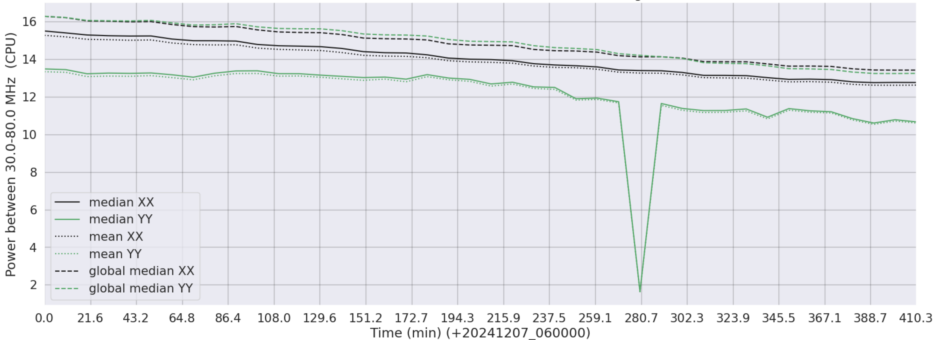
LWA190 - Correlator# 244 - XX FLAGS:Good - YY FLAGS:HighTimeVar
