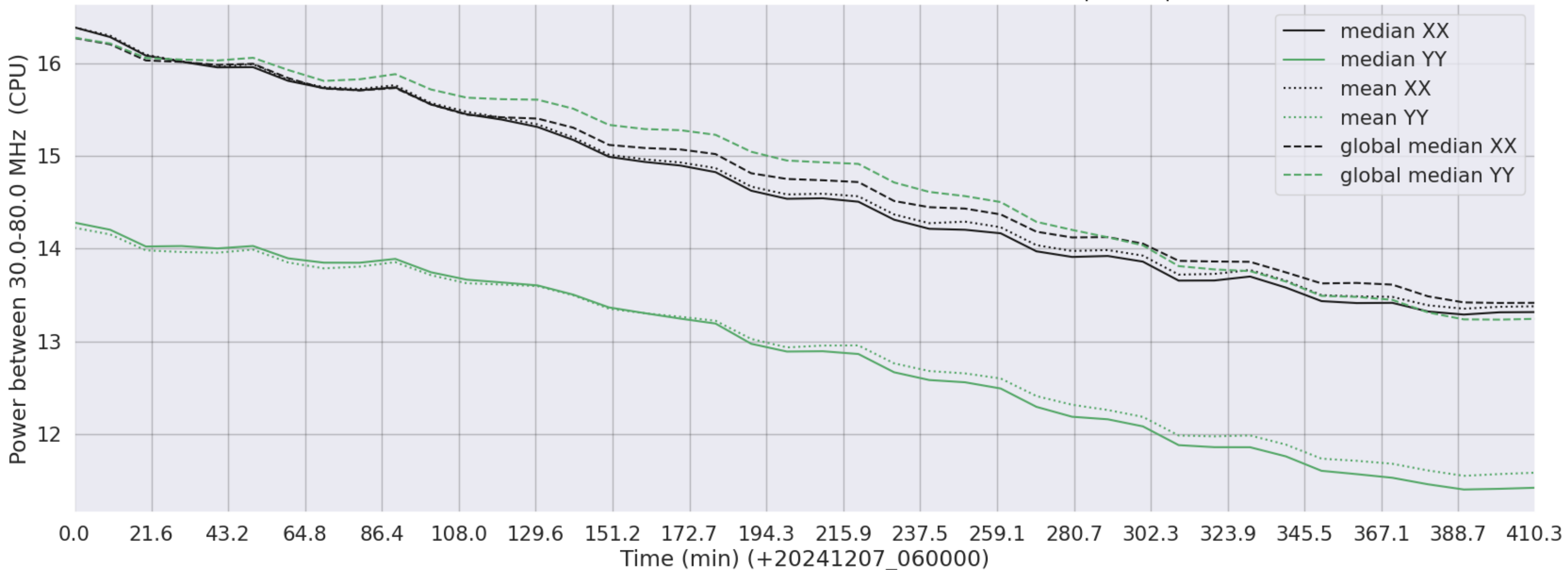
LWA292 - Correlator# 044 - XX FLAGS:Good - YY FLAGS:BadSpecShape
