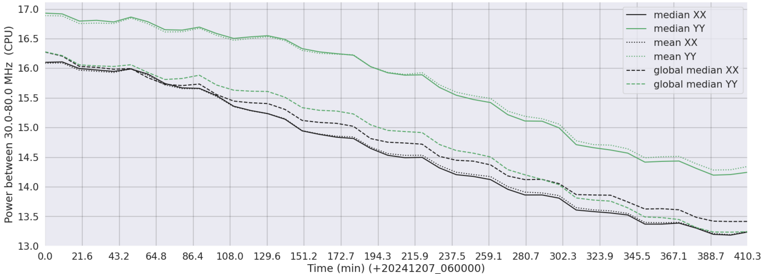
LWA332 - Correlator# 025 - XX FLAGS:Good - YY FLAGS:Good
