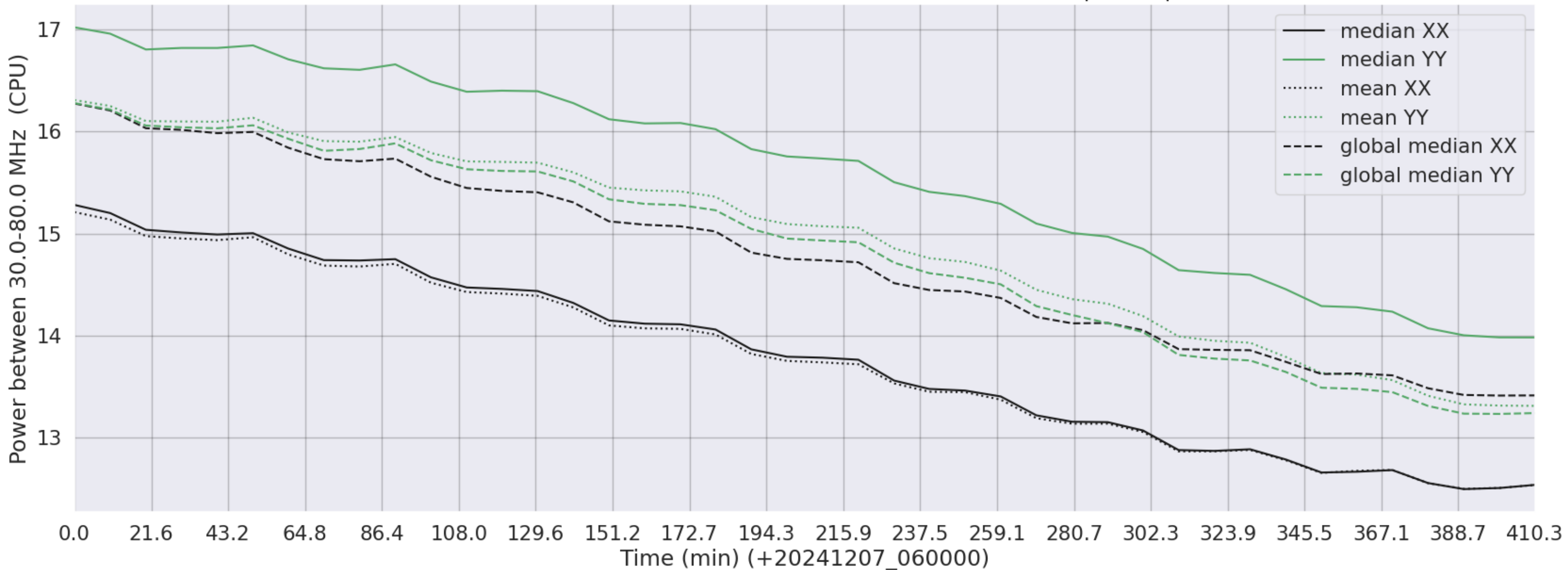
LWA205 - Correlator# 297 - XX FLAGS:Good - YY FLAGS:BadSpecShape
