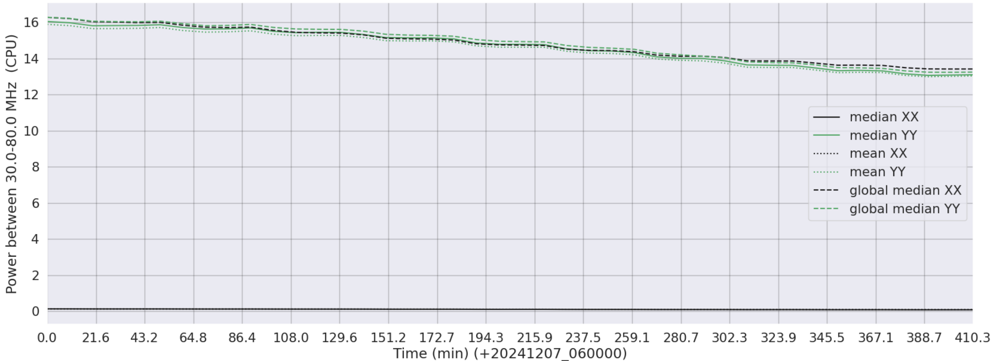
LWA226 - Correlator# 304 - XX FLAGS:LowPower - YY FLAGS:Good
