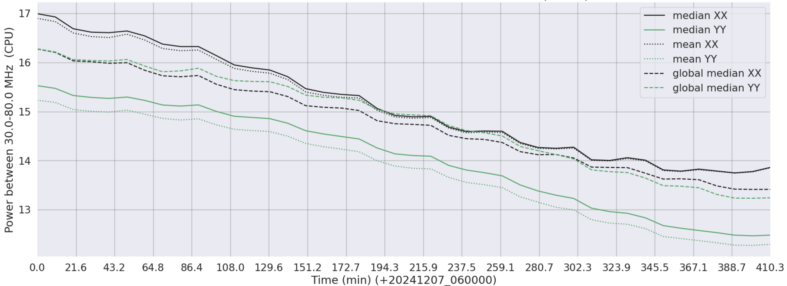
LWA283 - Correlator# 040 - XX FLAGS:Good - YY FLAGS:BadSpecShape
