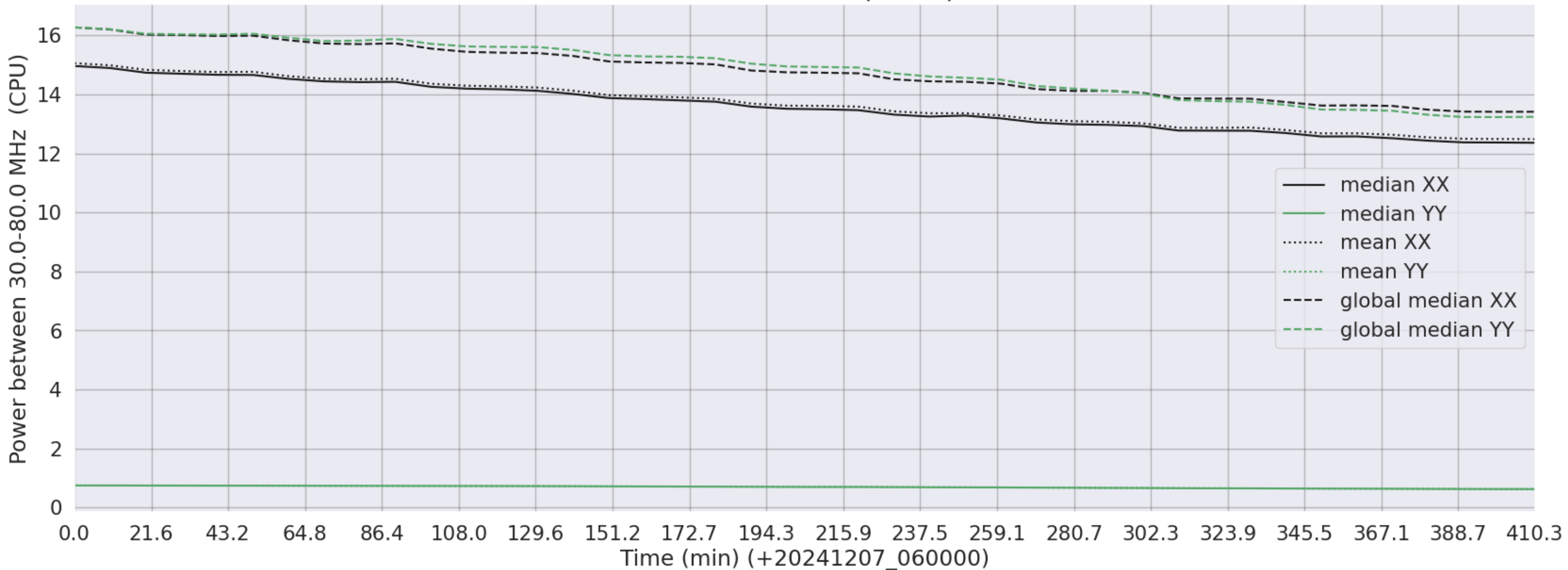
LWA280 - Correlator# 041 - XX FLAGS:BadSpecShape - YY FLAGS:LowPower
