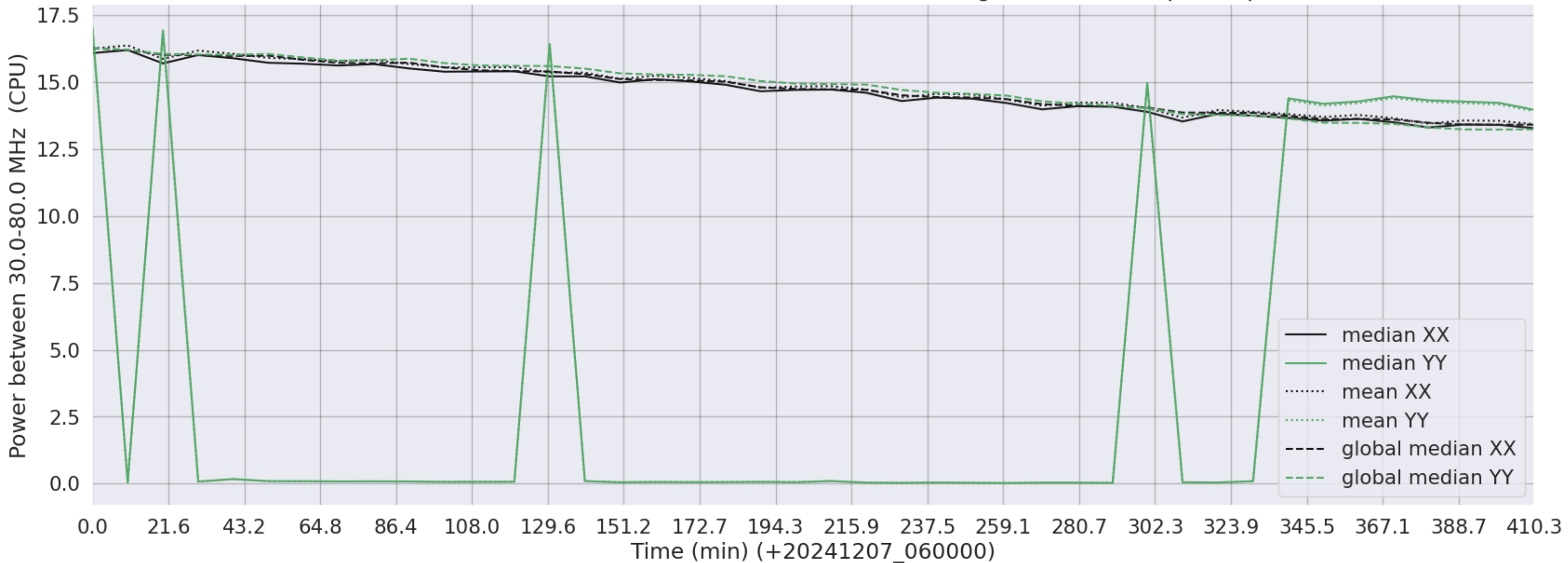
LWA124 - Correlator# 224 - XX FLAGS:Good - YY FLAGS:HighTimeVar+BadSpecShape
