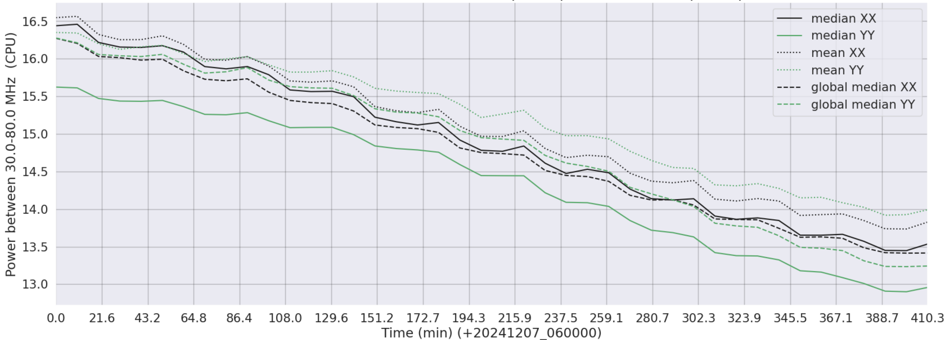
LWA336 - Correlator# 056 - XX FLAGS:BadSpecShape - YY FLAGS:BadSpecShape
