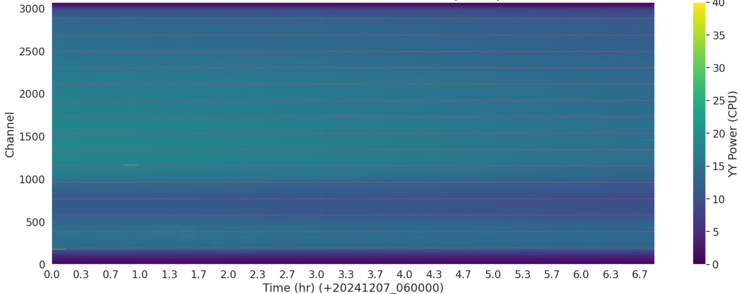
LWA205 - Correlator# 297 - YY - FLAGS: BadSpecShape
