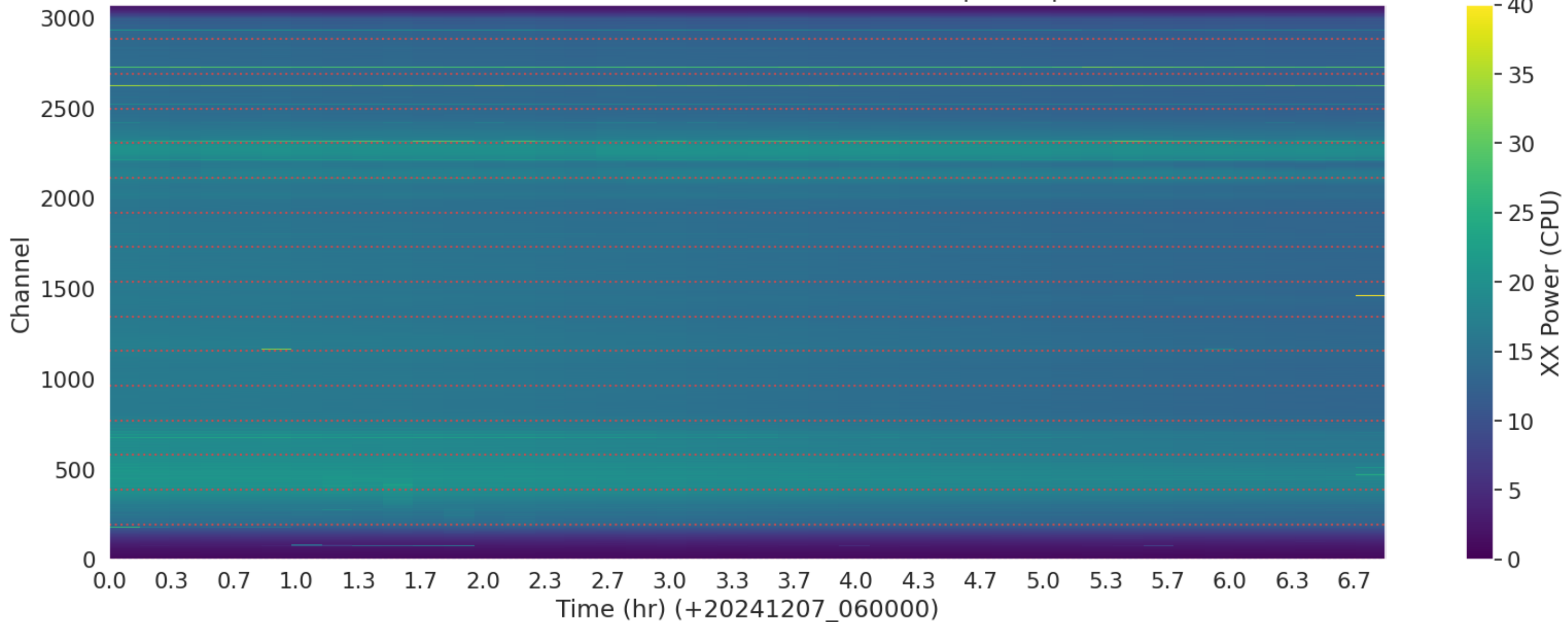
LWA341 - Correlator# 029 - XX - FLAGS: BadSpecShape
