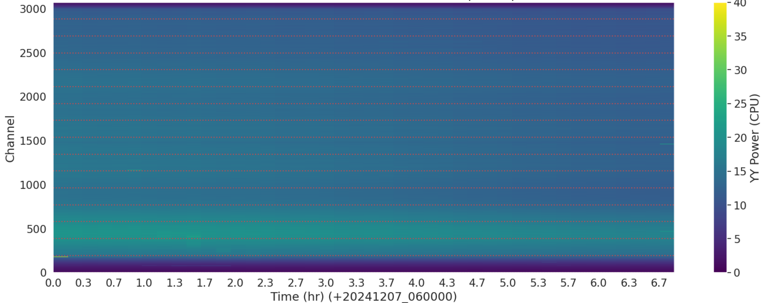
LWA102 - Correlator# 177 - YY - FLAGS: BadSpecShape
