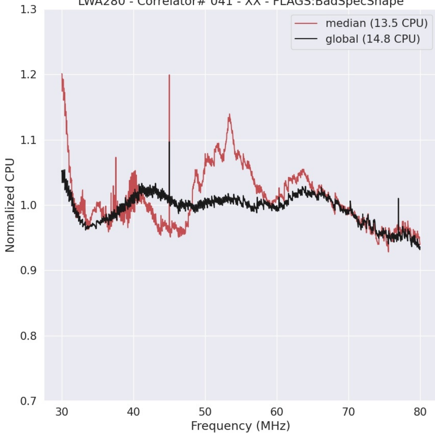
LWA280 - Correlator# 041 - XX - FLAGS:BadSpecShape
