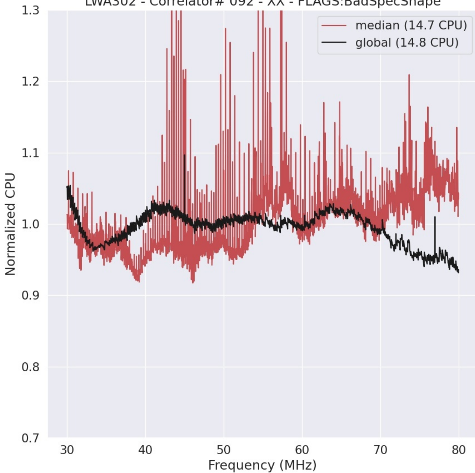
LWA302 - Correlator# 092 - XX - FLAGS:BadSpecShape
