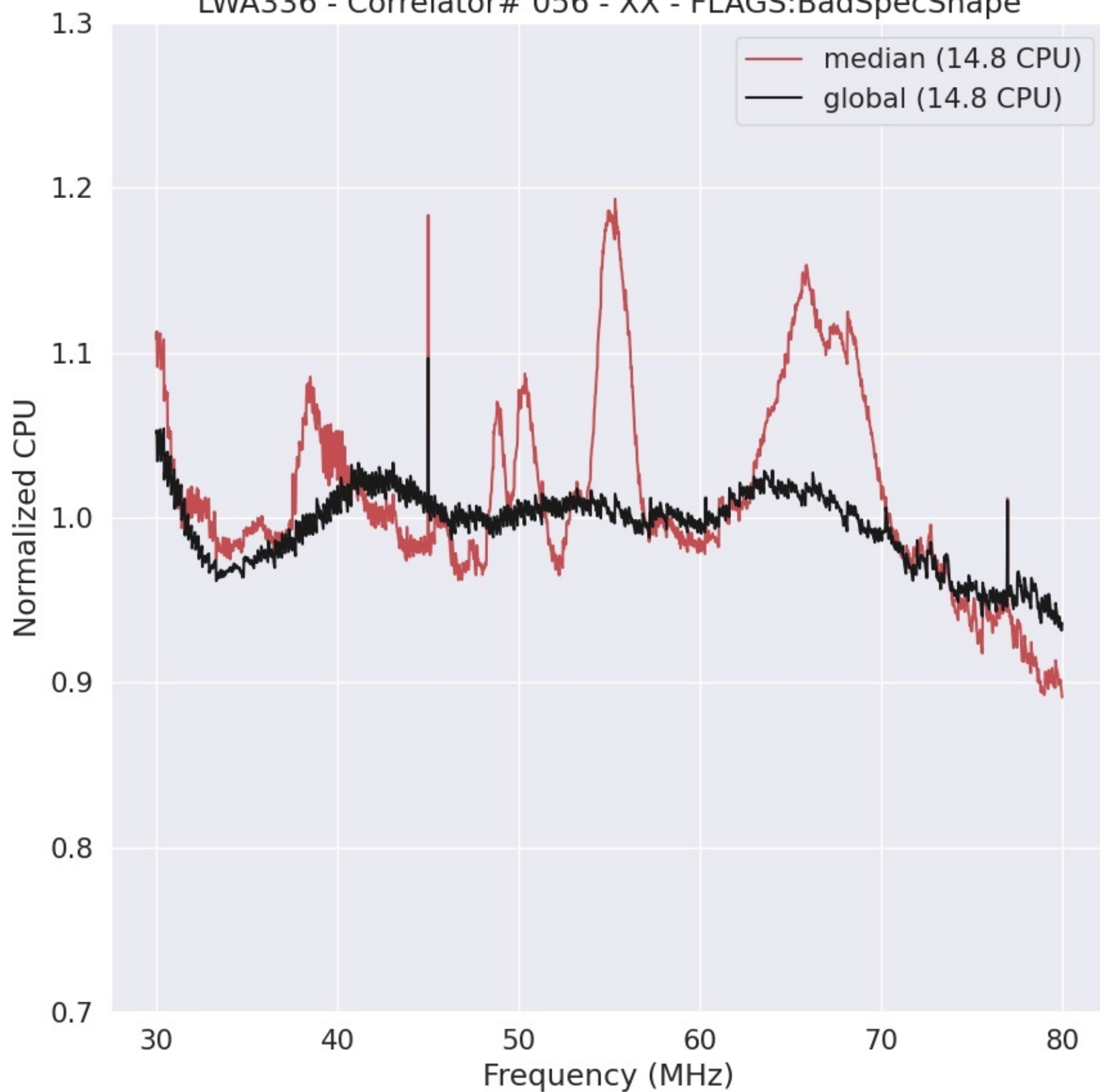
LWA336 - Correlator# 056 - XX - FLAGS:BadSpecShape
