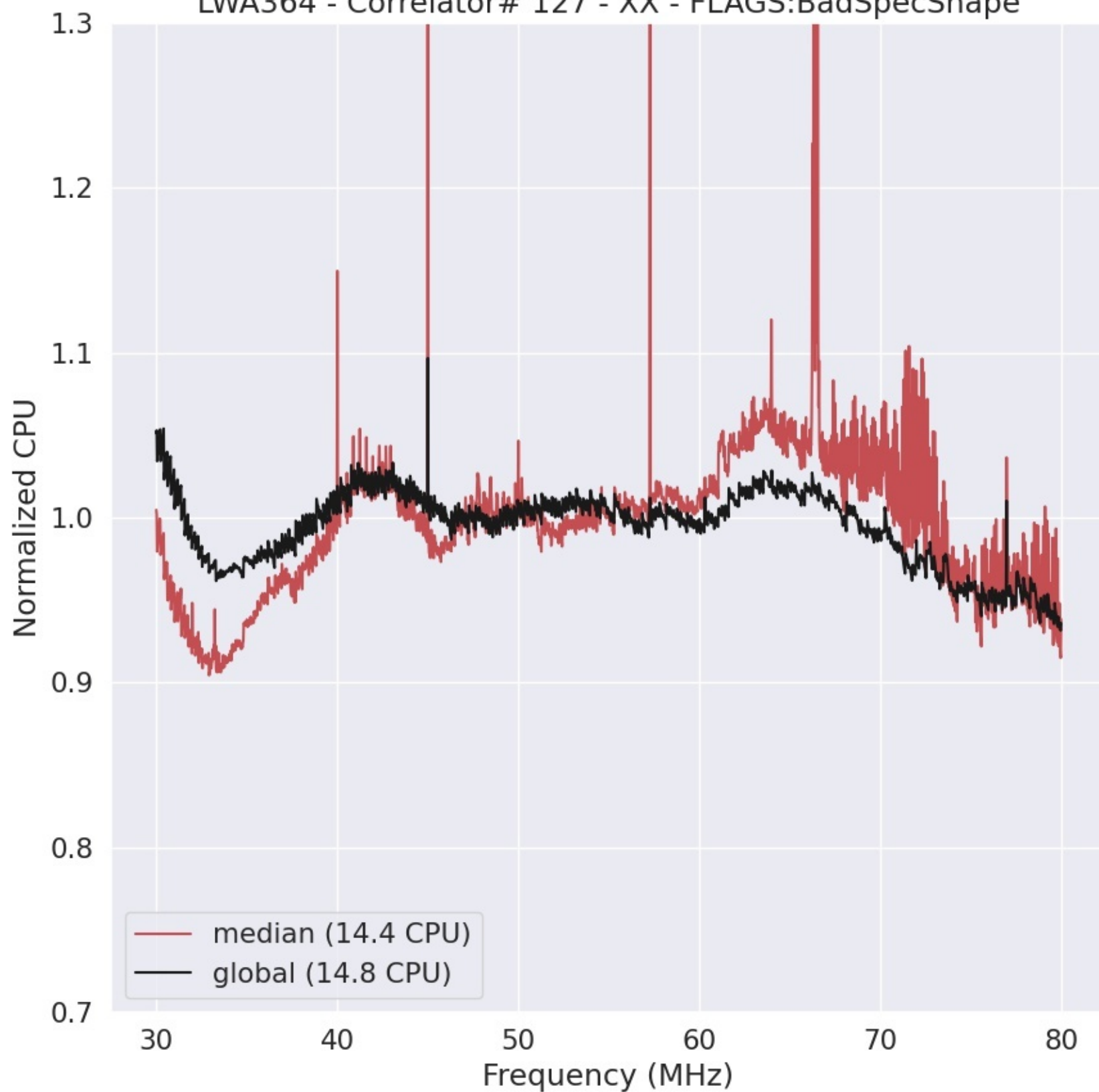
LWA364 - Correlator# 127 - XX - FLAGS:BadSpecShape
