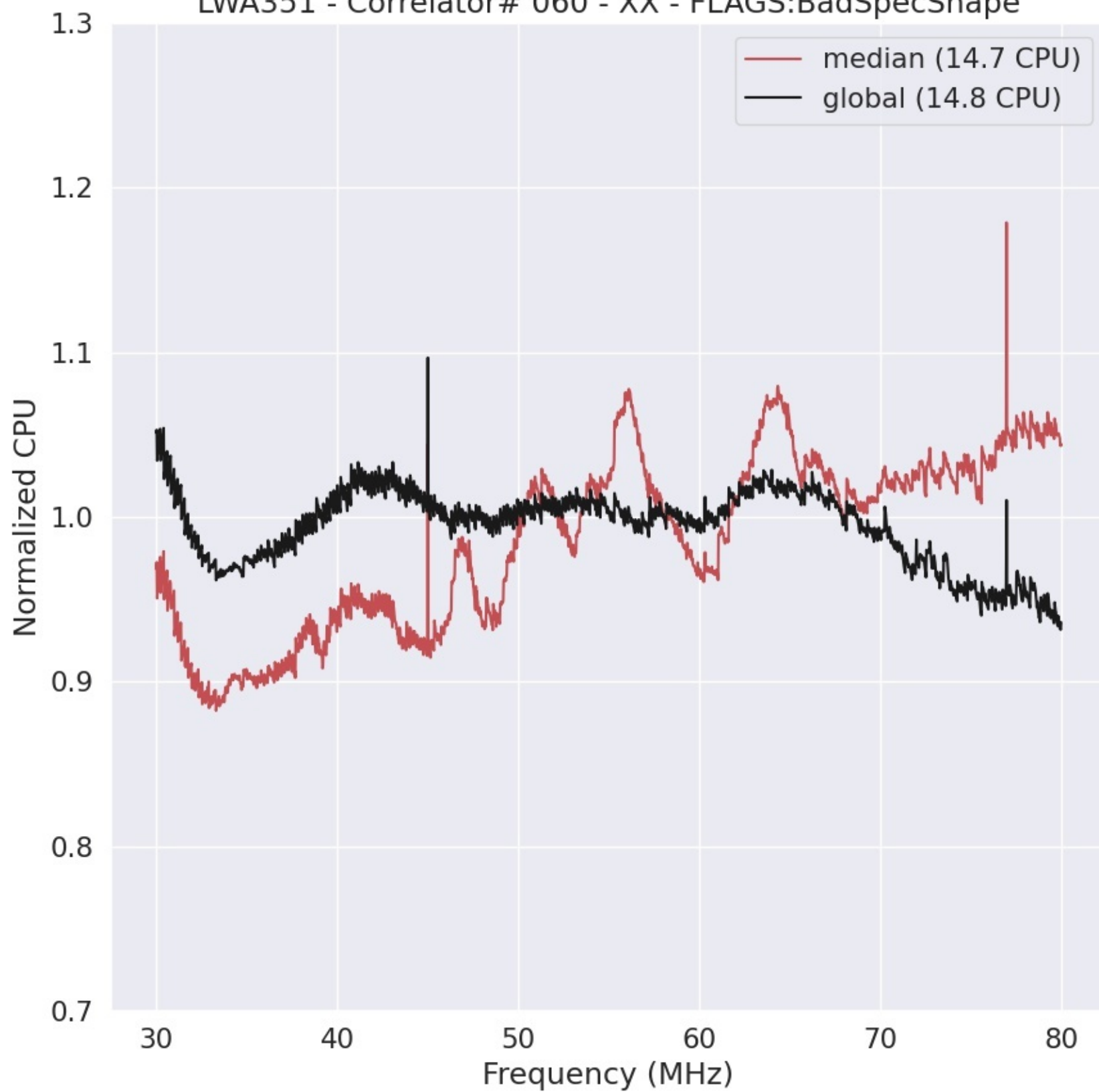
LWA351 - Correlator# 060 - XX - FLAGS:BadSpecShape
