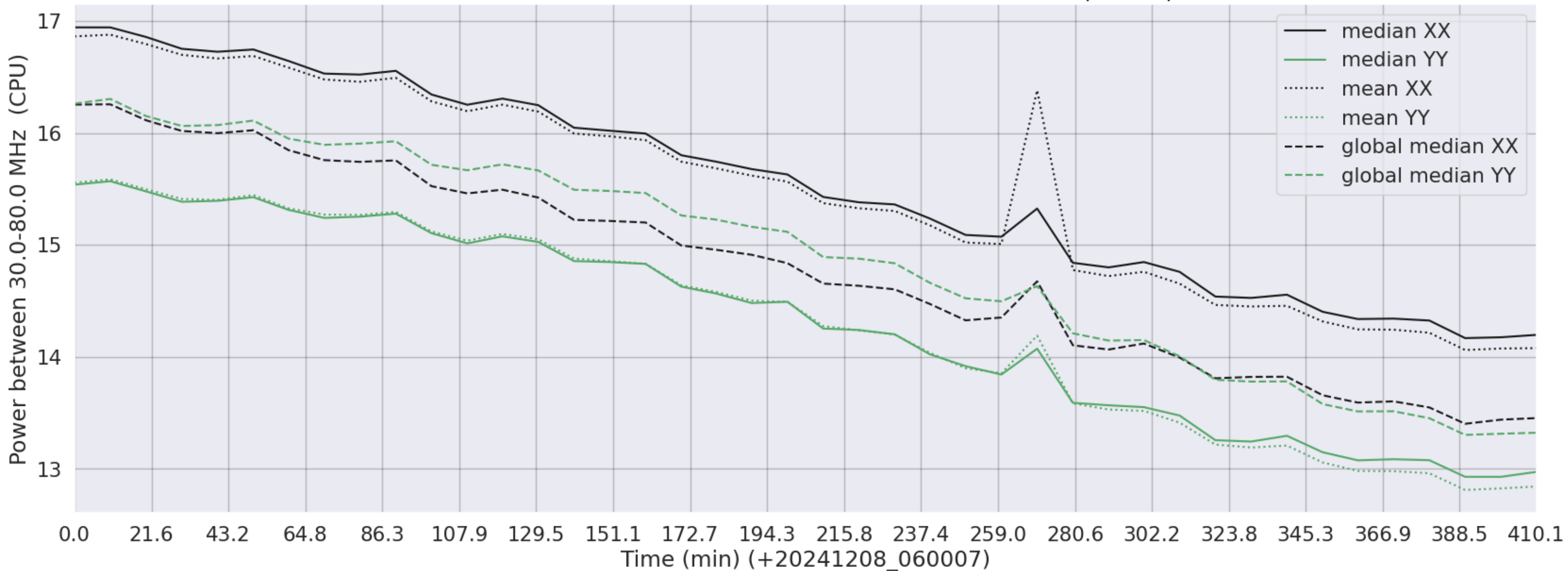
LWA289 - Correlator# 189 - XX FLAGS:Good - YY FLAGS:BadSpecShape
