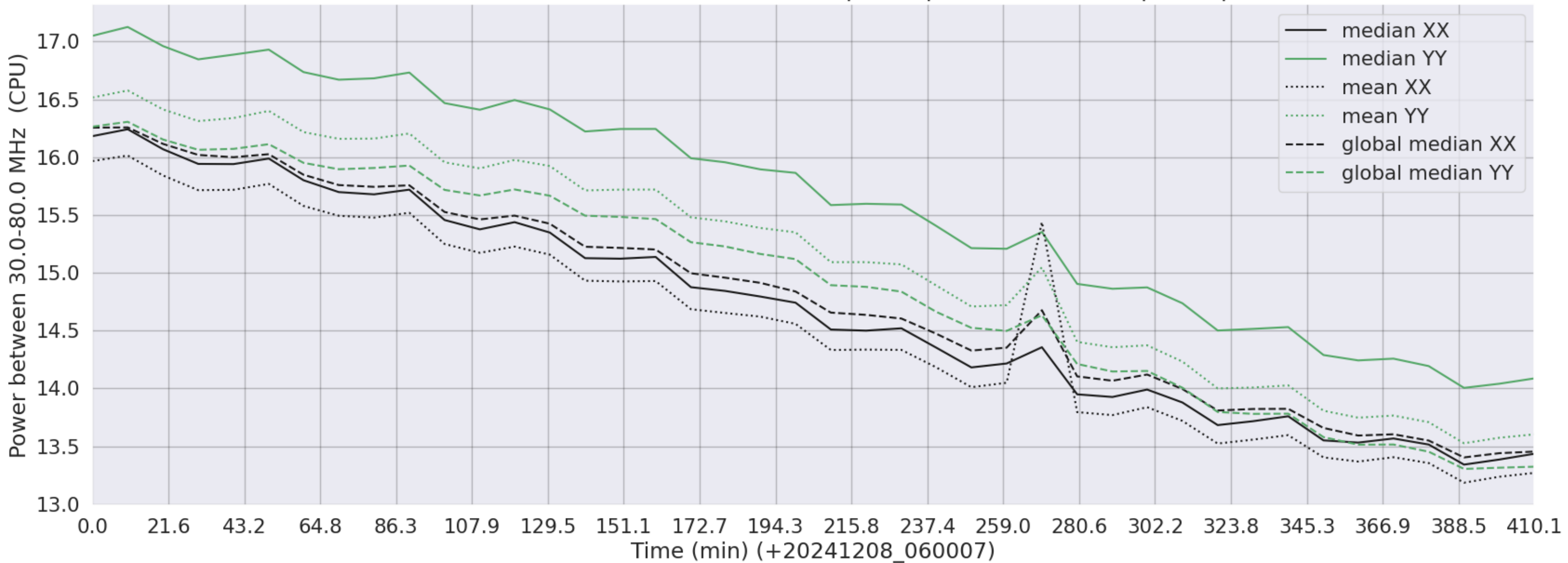
LWA195 - Correlator# 272 - XX FLAGS:BadSpecShape - YY FLAGS:BadSpecShape
