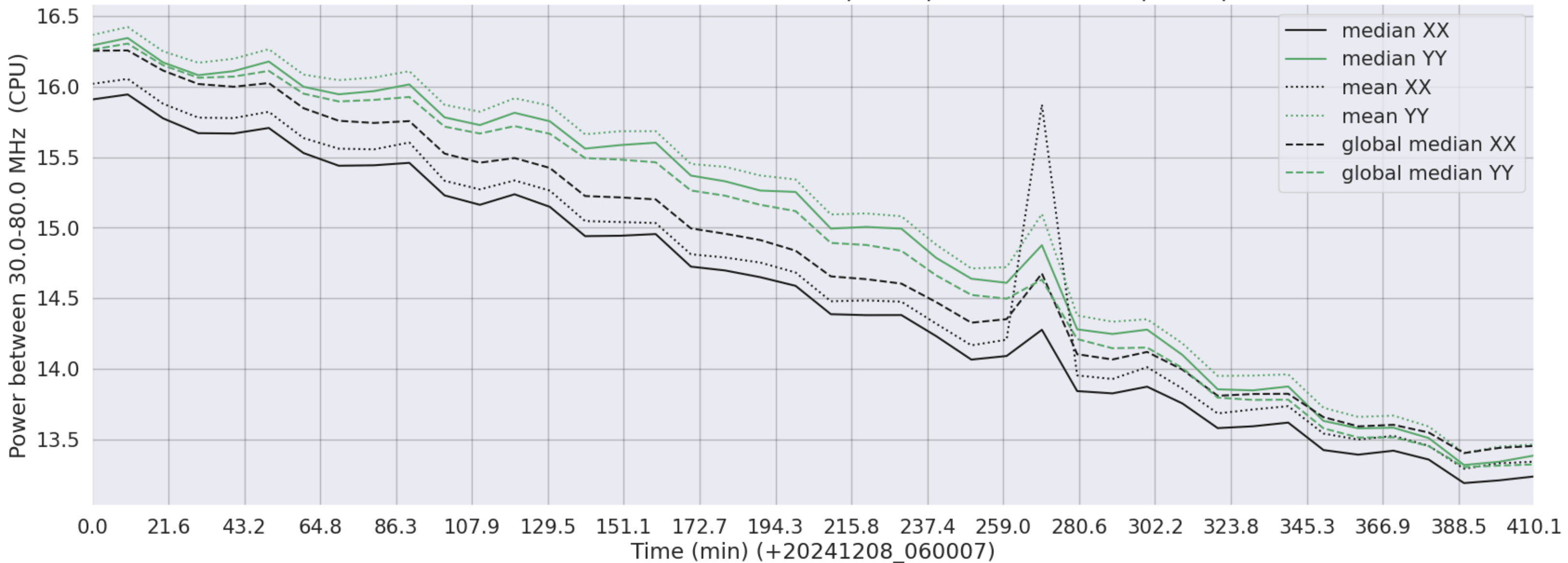
LWA002 - Correlator# 064 - XX FLAGS:BadSpecShape - YY FLAGS:BadSpecShape
