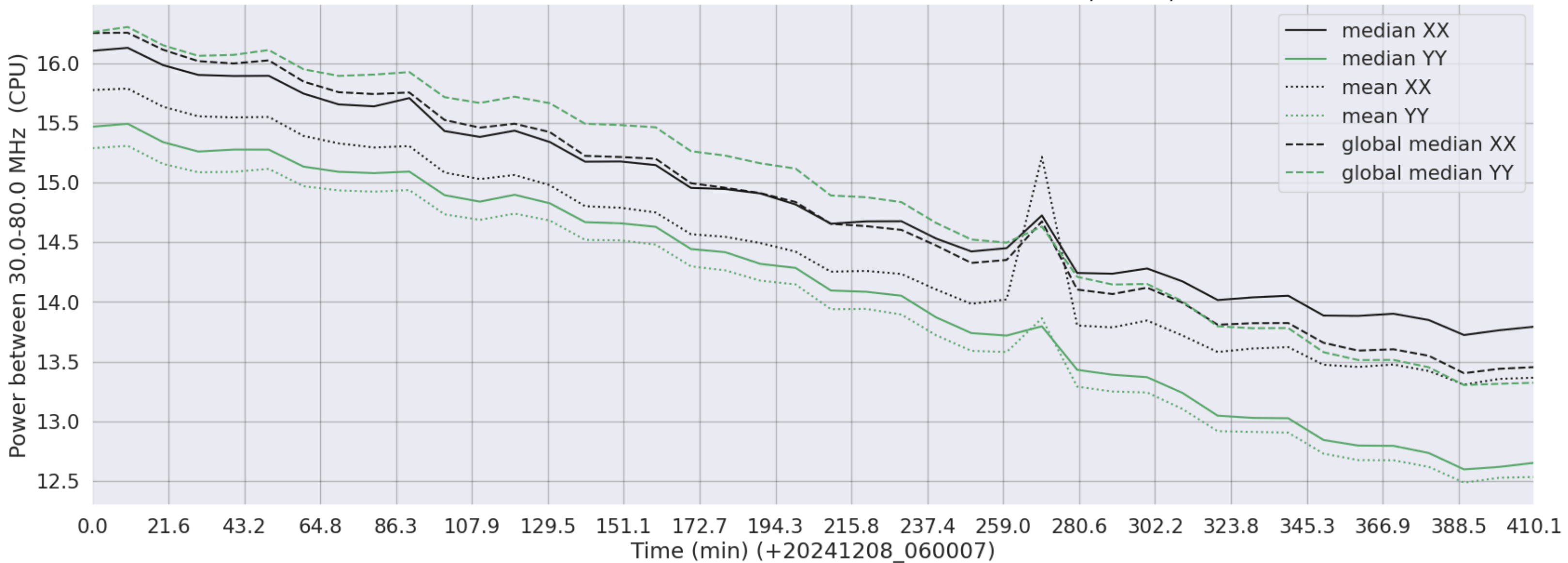
LWA107 - Correlator# 197 - XX FLAGS:Good - YY FLAGS:BadSpecShape
