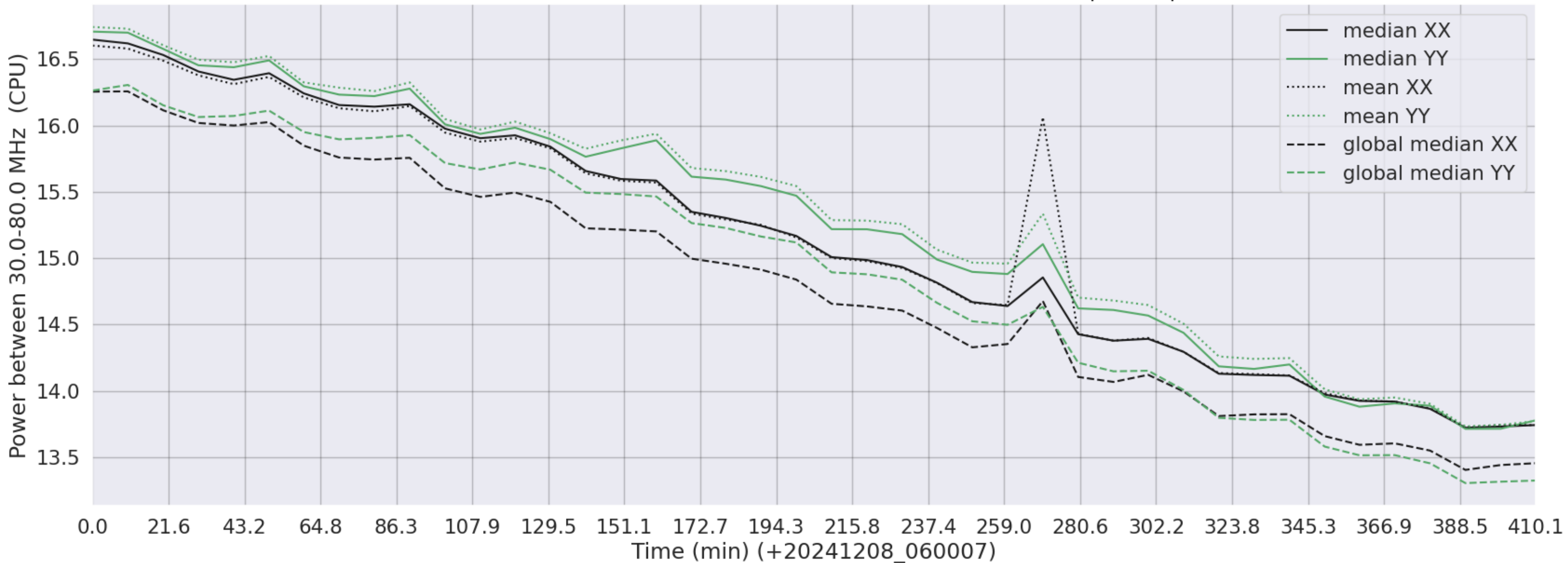
LWA354 - Correlator# 063 - XX FLAGS:Good - YY FLAGS:BadSpecShape
