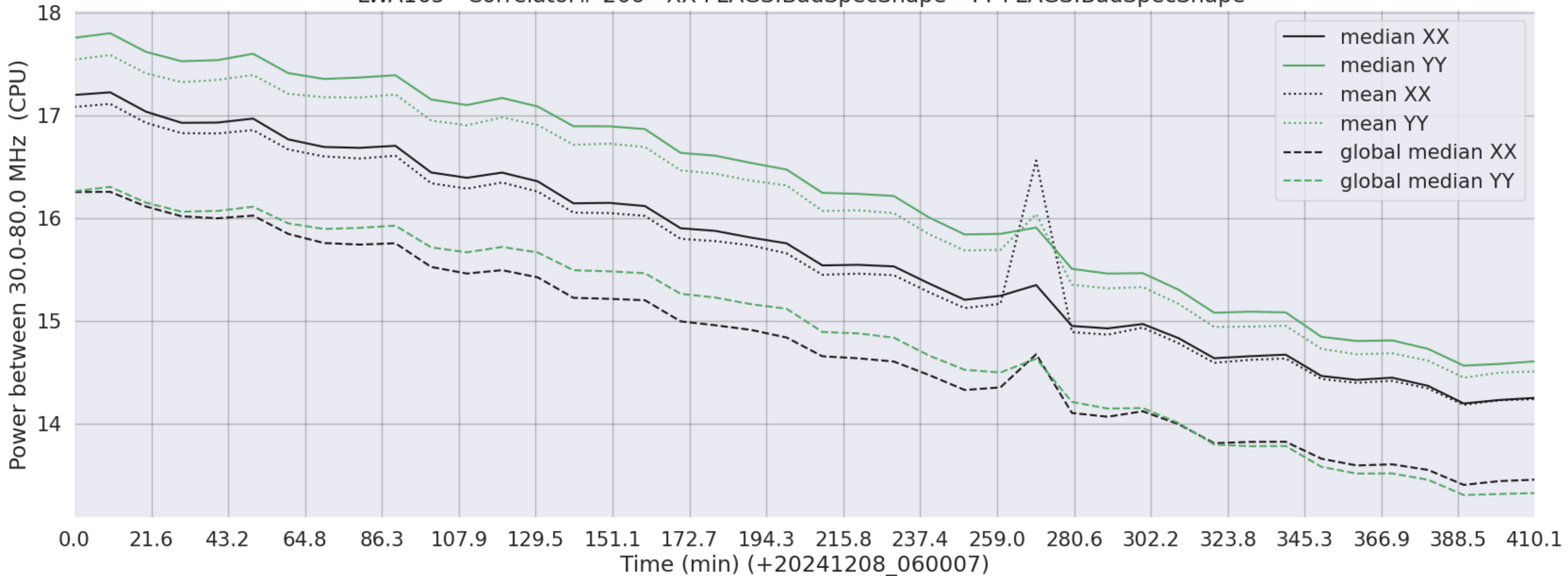
LWA165 - Correlator# 266 - XX FLAGS:BadSpecShape - YY FLAGS:BadSpecShape
