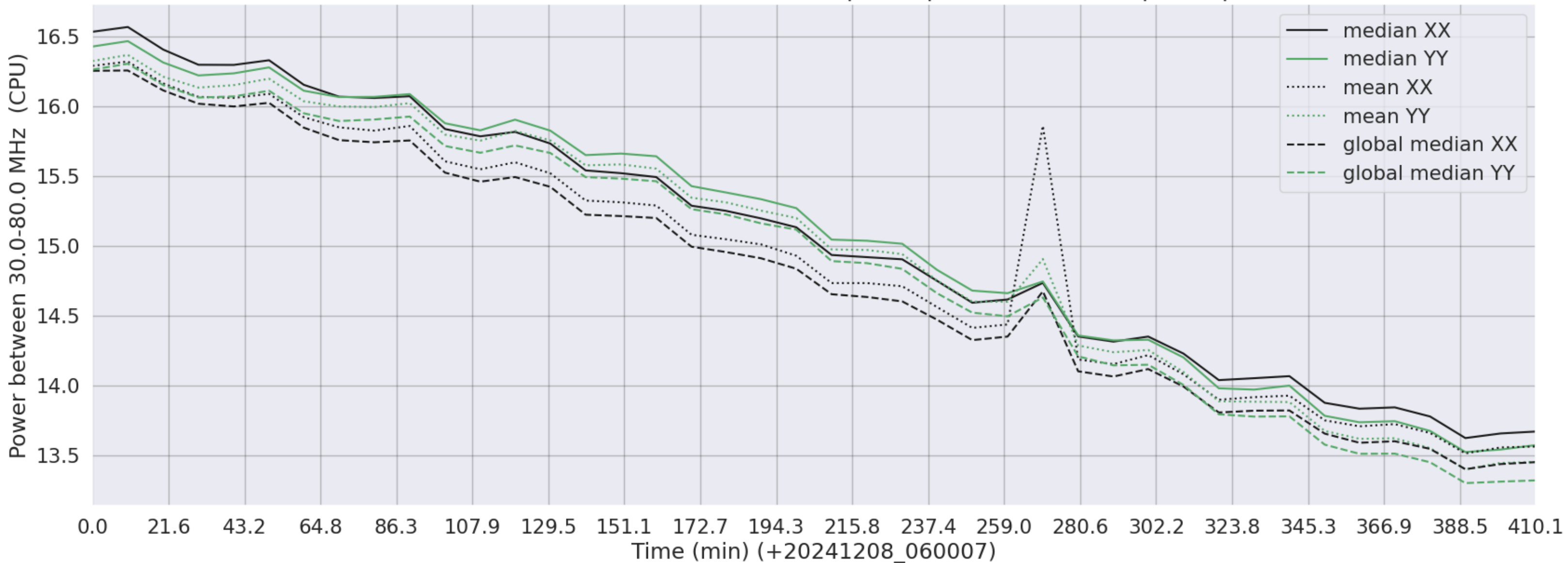
LWA164 - Correlator# 267 - XX FLAGS:BadSpecShape - YY FLAGS:BadSpecShape
