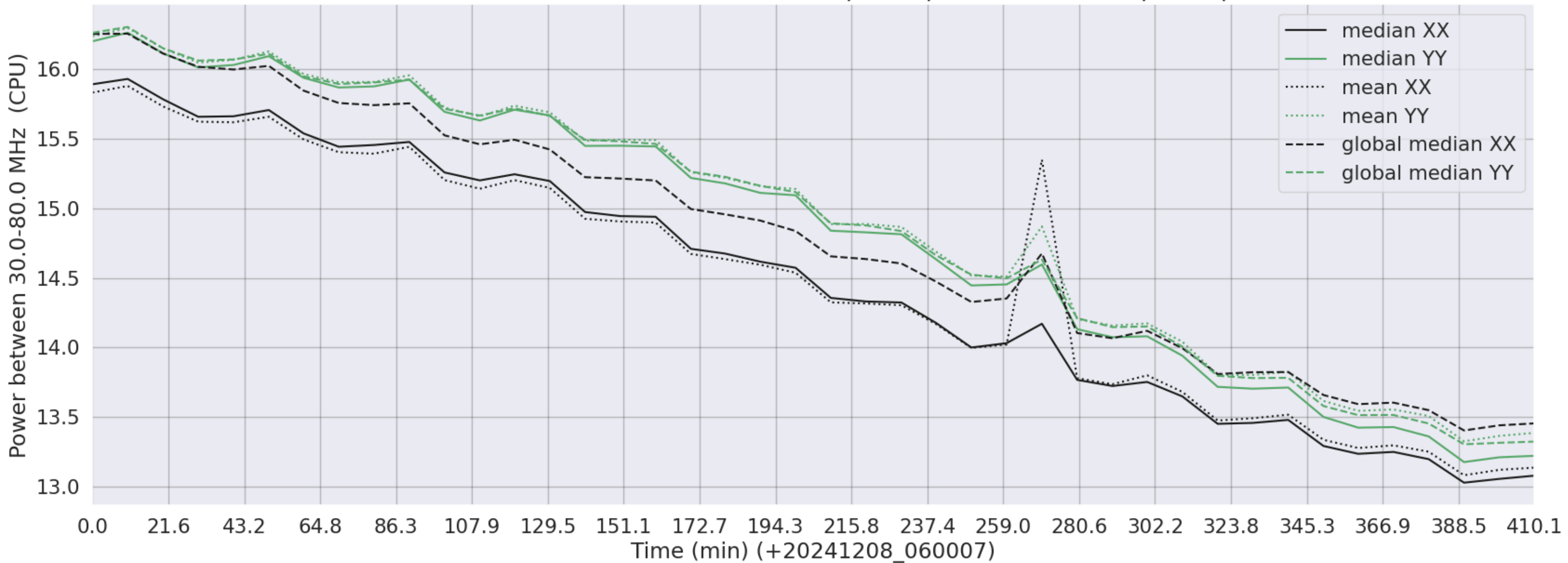
LWA230 - Correlator# 303 - XX FLAGS:BadSpecShape - YY FLAGS:BadSpecShape
