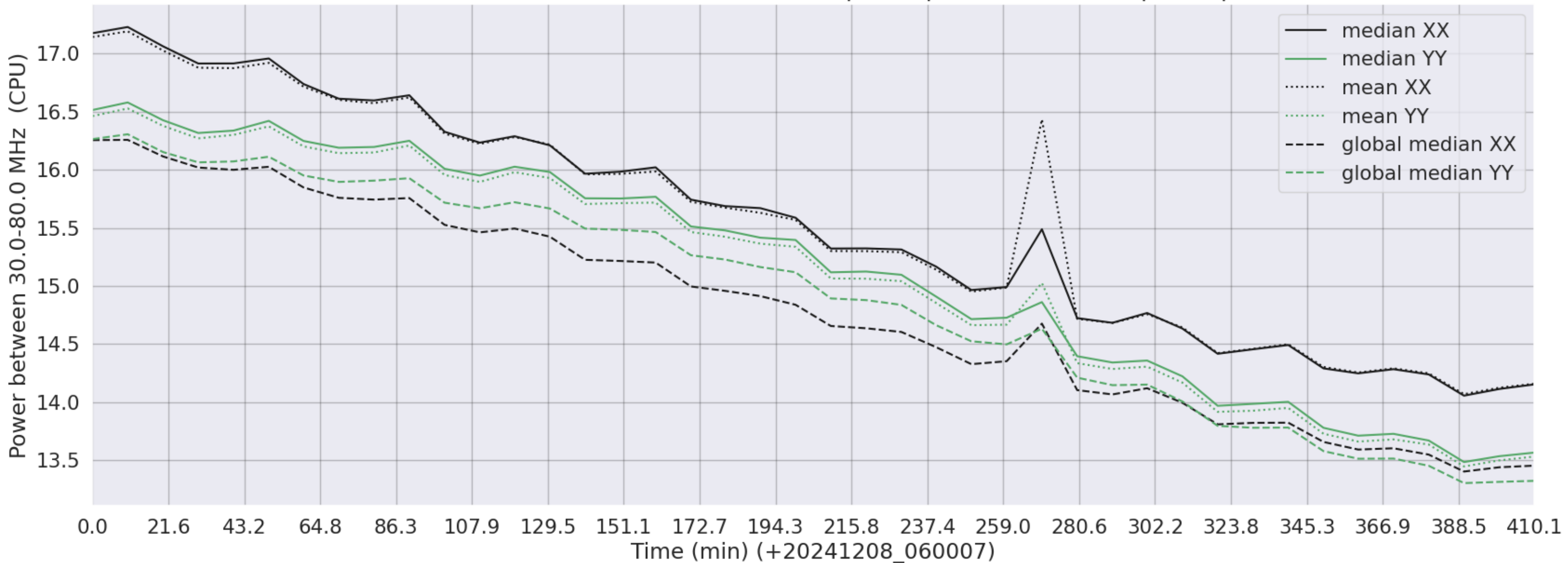
LWA227 - Correlator# 280 - XX FLAGS:BadSpecShape - YY FLAGS:BadSpecShape
