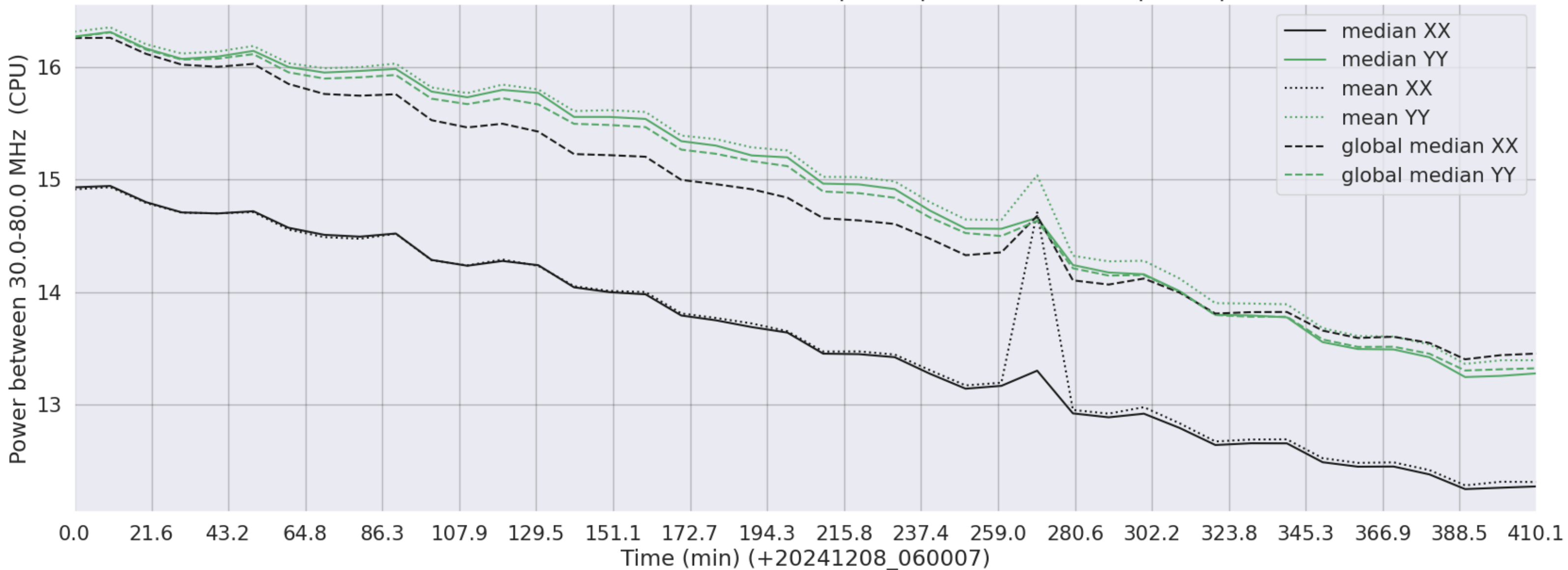
LWA007 - Correlator# 071 - XX FLAGS:BadSpecShape - YY FLAGS:BadSpecShape
