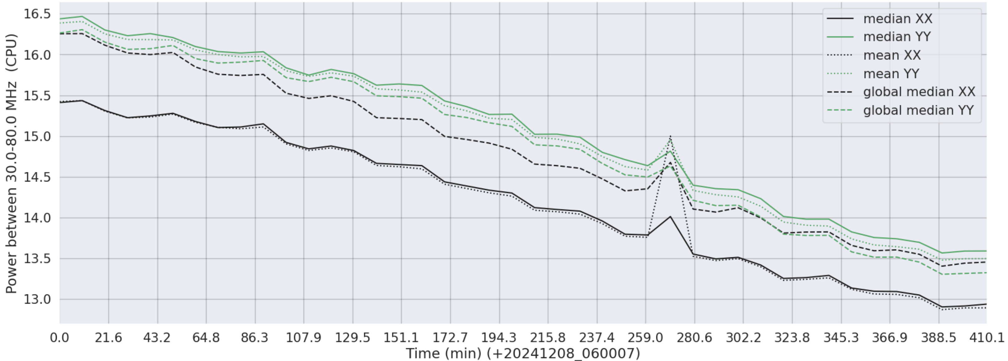
LWA305 - Correlator# 050 - XX FLAGS:Good - YY FLAGS:BadSpecShape
