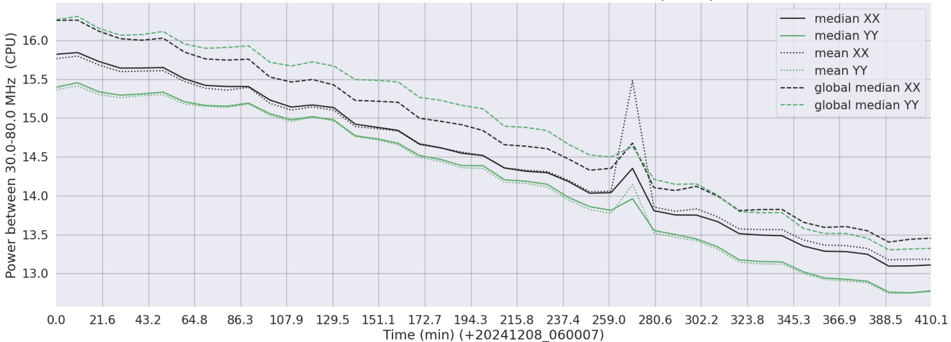
LWA316 - Correlator# 155 - XX FLAGS:Good - YY FLAGS:BadSpecShape
