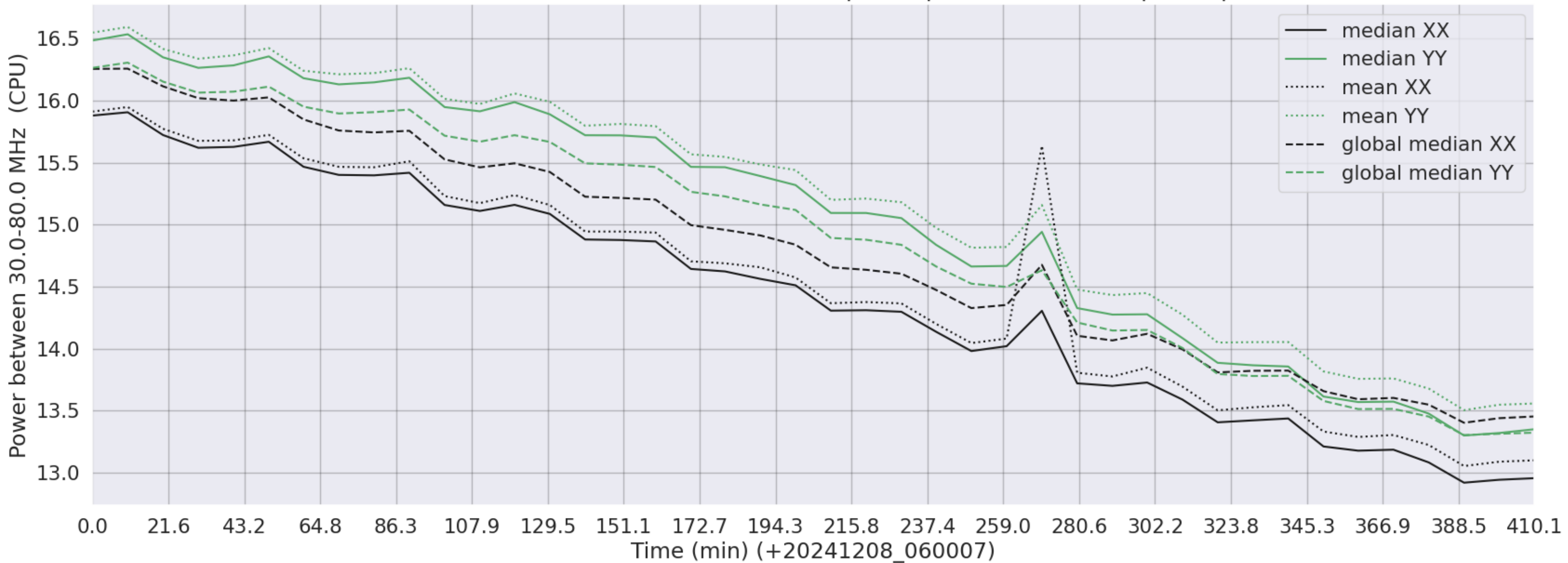
LWA034 - Correlator# 162 - XX FLAGS:BadSpecShape - YY FLAGS:BadSpecShape
