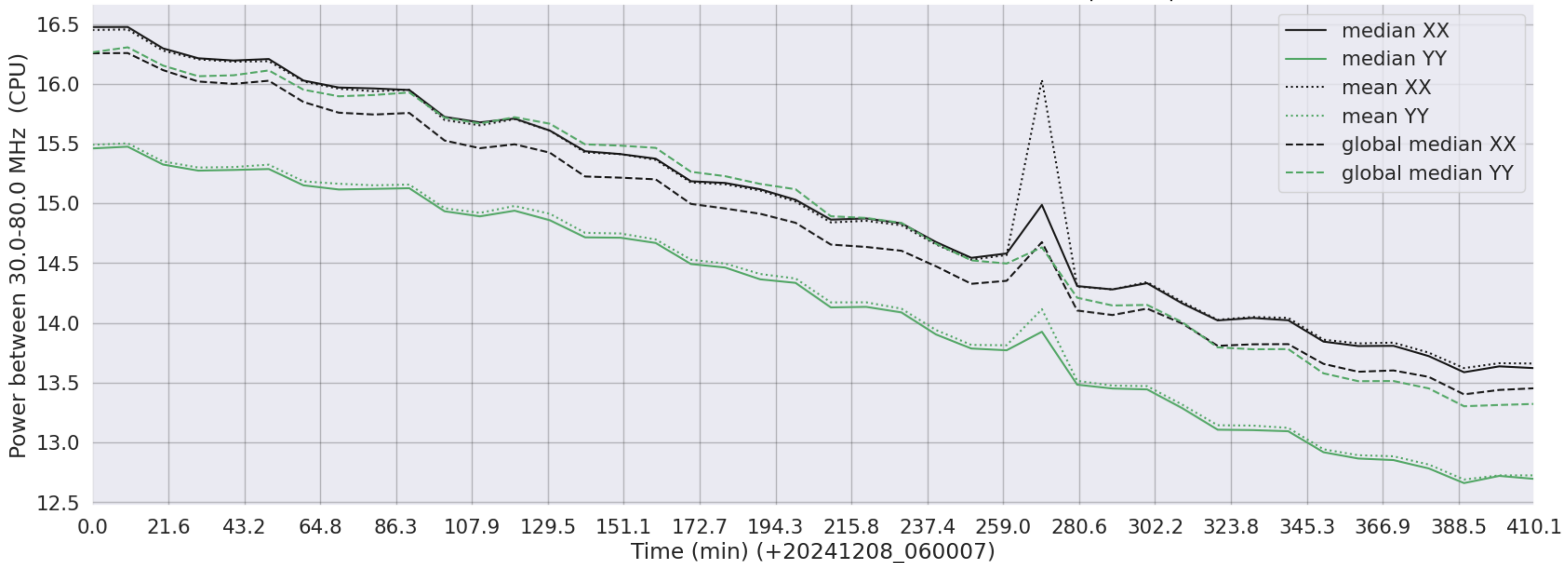
LWA014 - Correlator# 099 - XX FLAGS:Good - YY FLAGS:BadSpecShape
