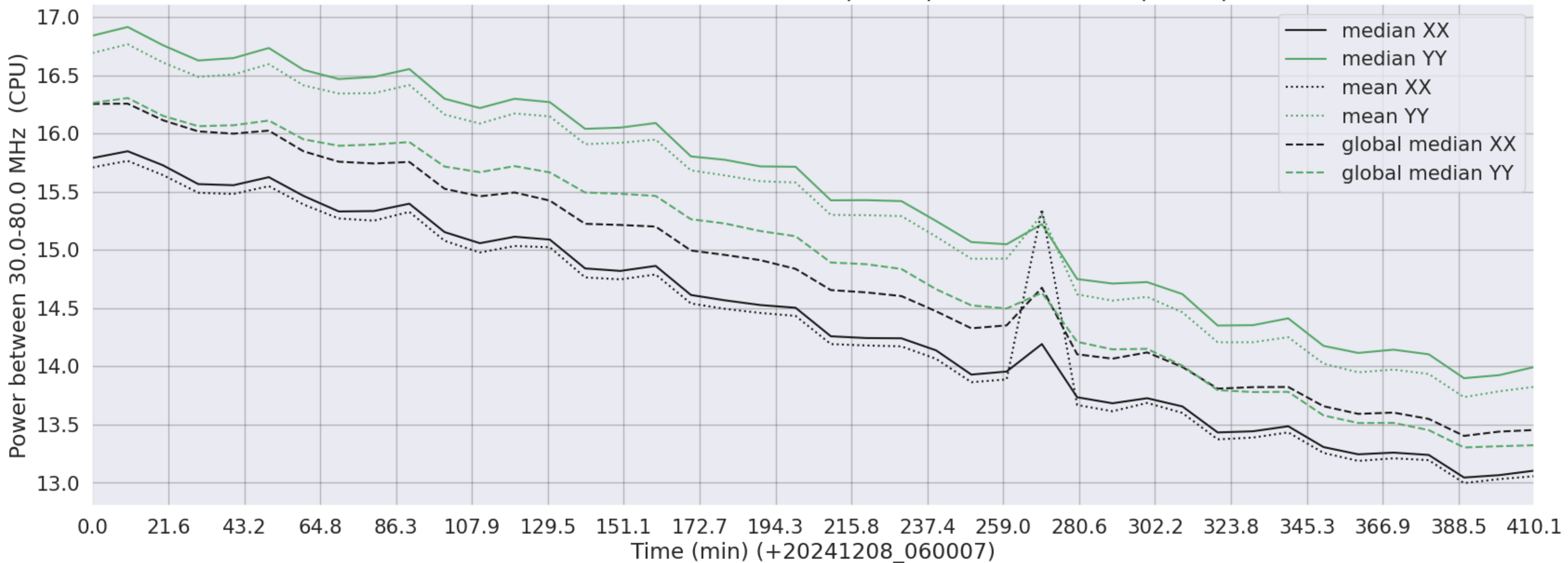
LWA134 - Correlator# 184 - XX FLAGS:BadSpecShape - YY FLAGS:BadSpecShape
