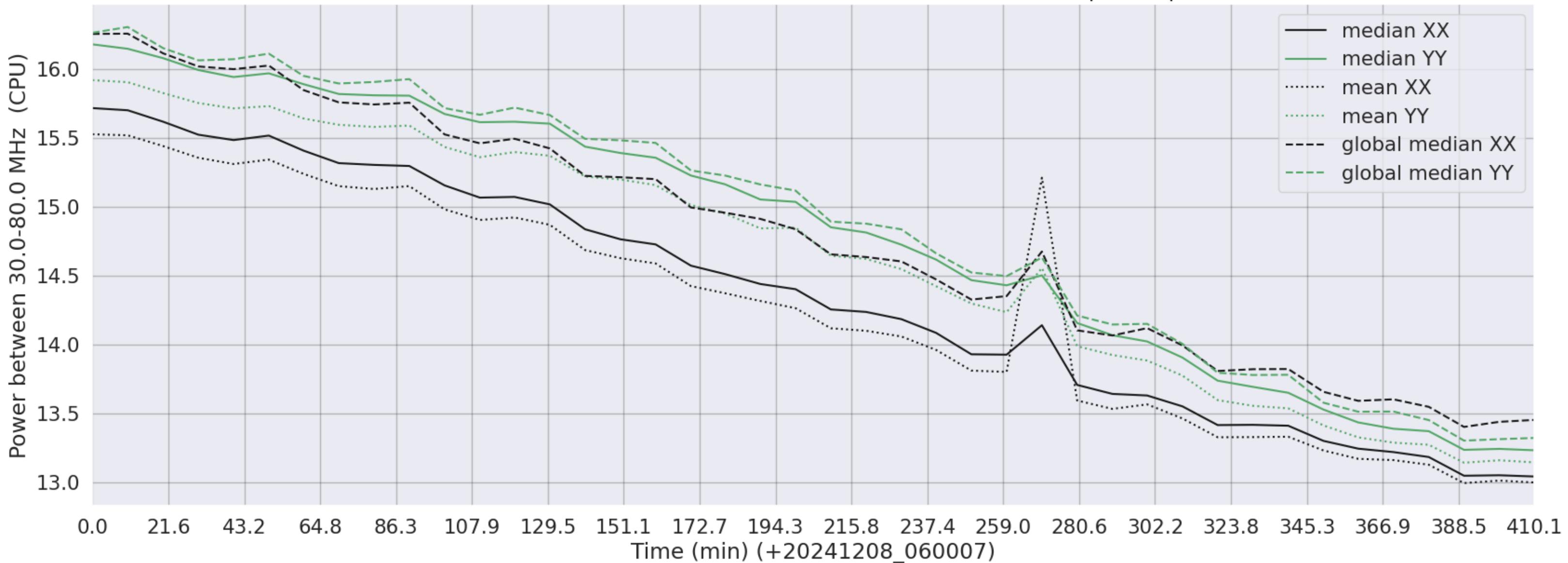
LWA307 - Correlator# 012 - XX FLAGS:Good - YY FLAGS:BadSpecShape
