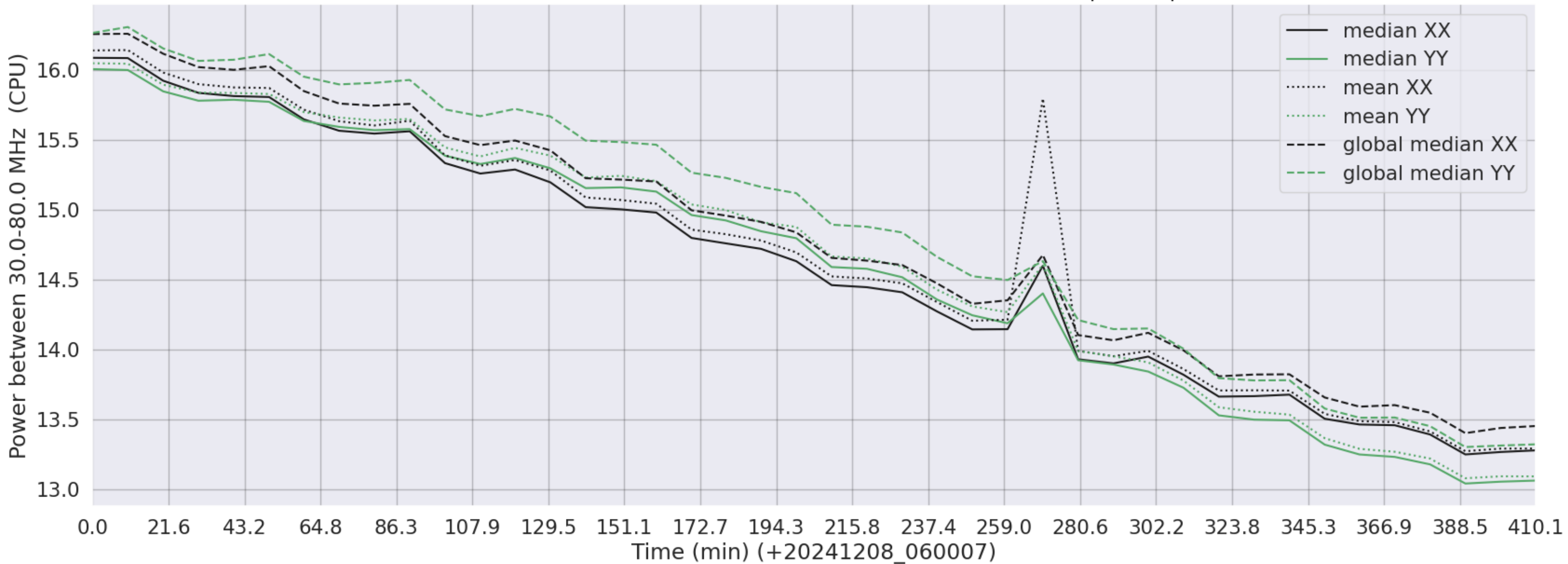
LWA260 - Correlator# 034 - XX FLAGS:Good - YY FLAGS:BadSpecShape
