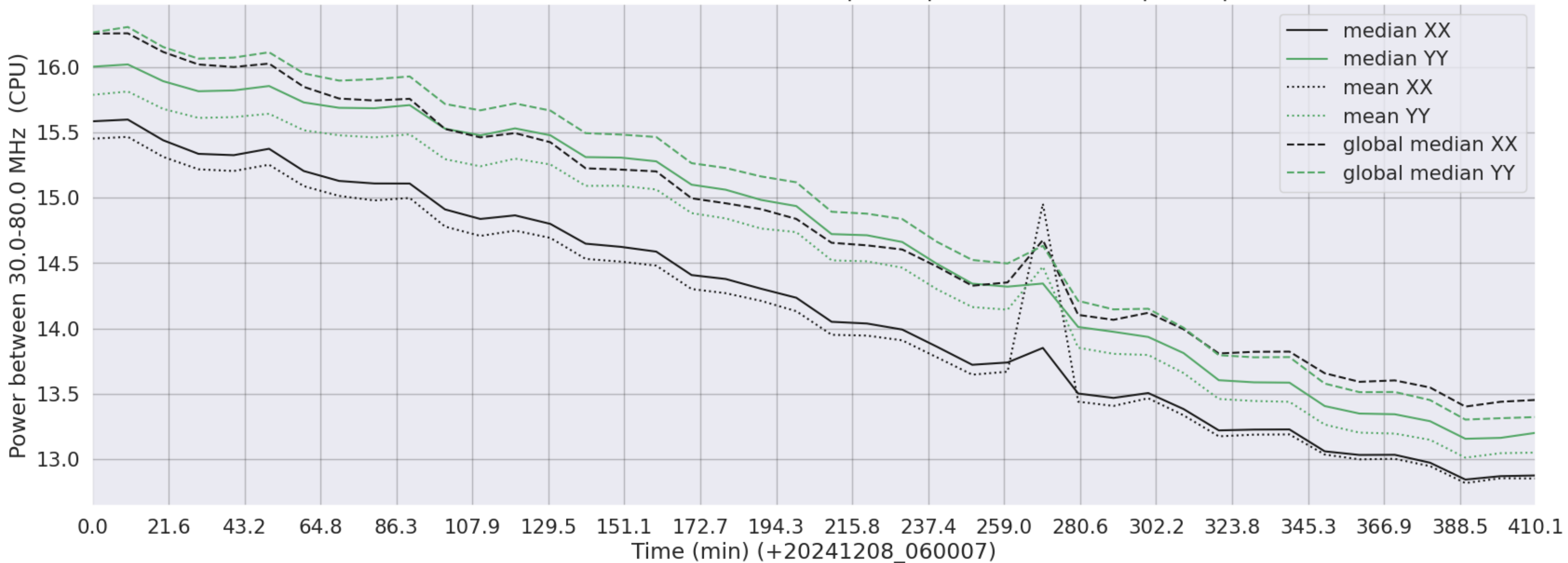
LWA132 - Correlator# 185 - XX FLAGS:BadSpecShape - YY FLAGS:BadSpecShape
