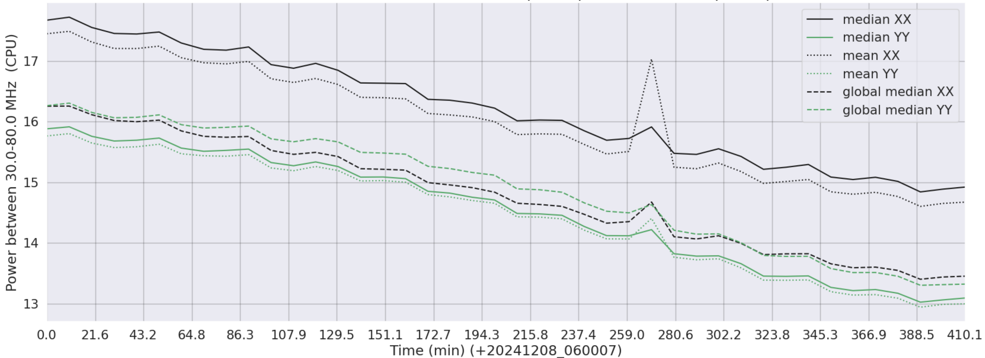
LWA133 - Correlator# 257 - XX FLAGS:BadSpecShape - YY FLAGS:BadSpecShape
