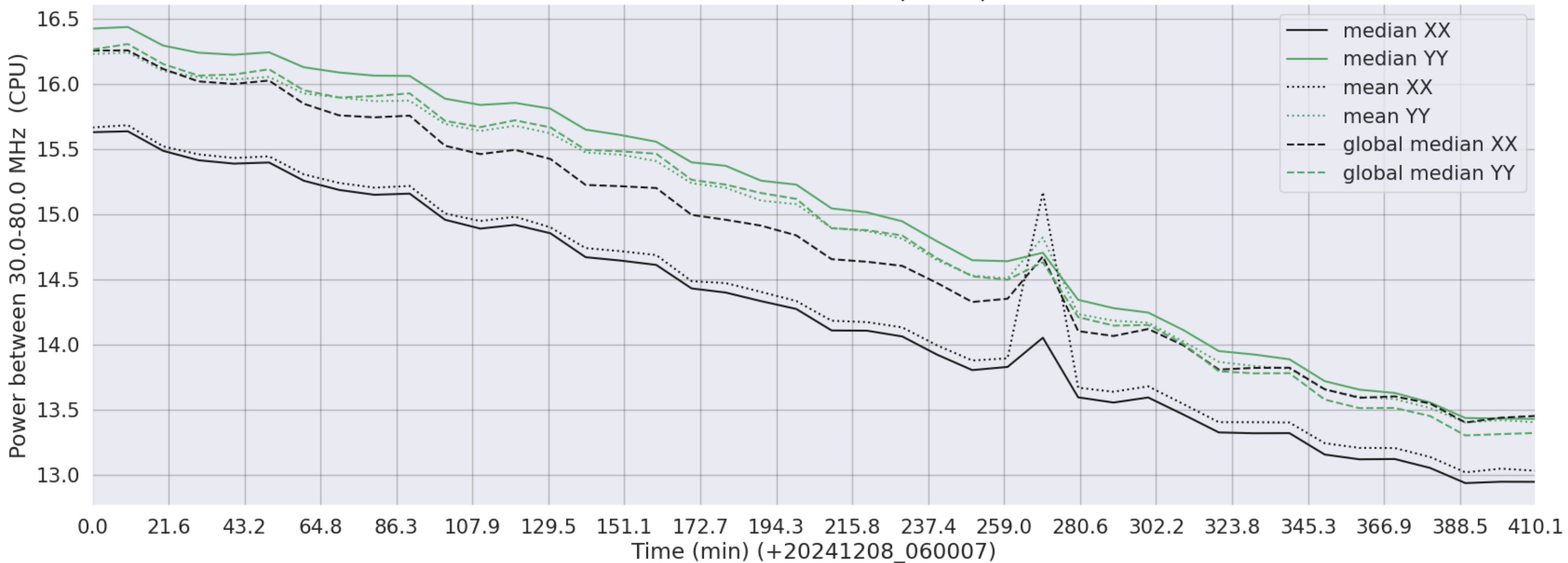
LWA160 - Correlator# 239 - XX FLAGS:BadSpecShape - YY FLAGS:Good
