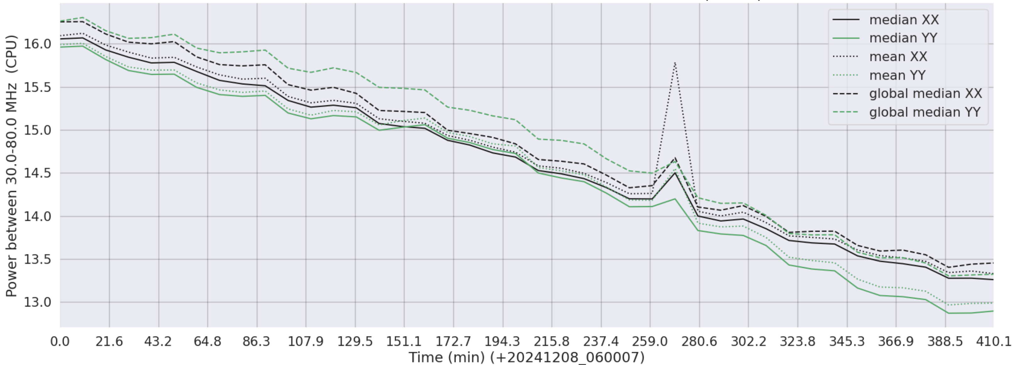
LWA262 - Correlator# 123 - XX FLAGS:Good - YY FLAGS:BadSpecShape
