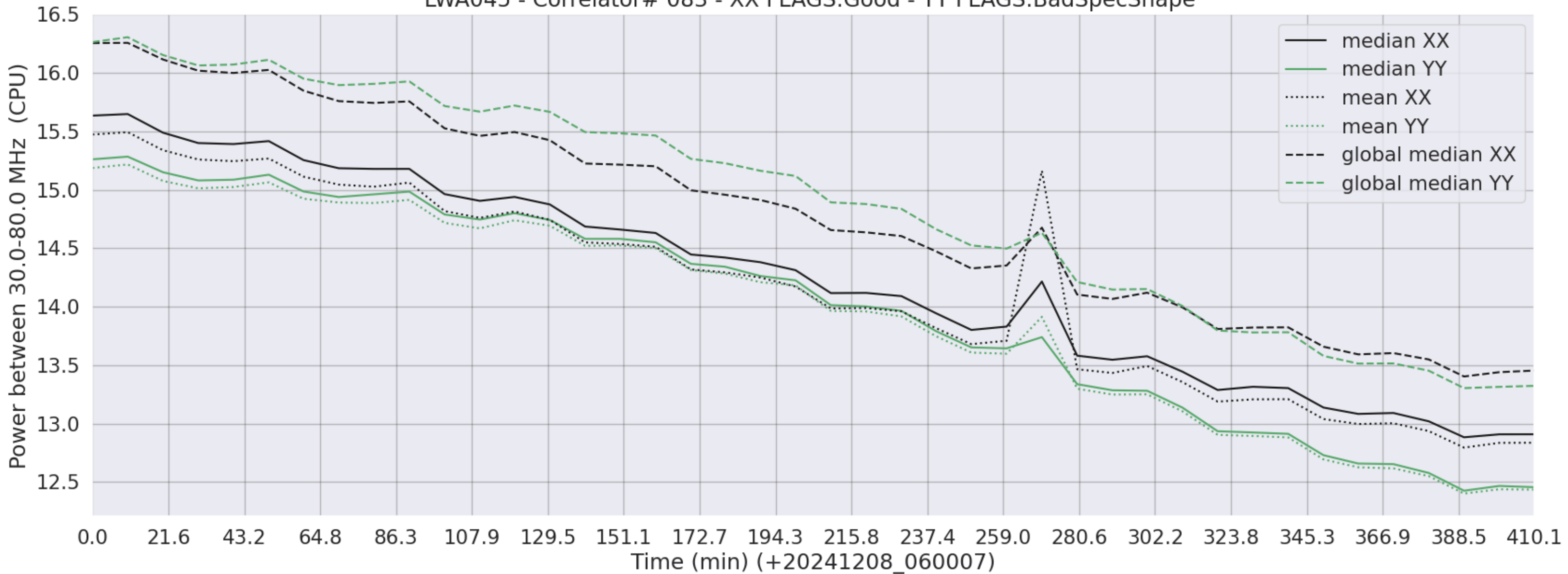
LWA045 - Correlator# 083 - XX FLAGS:Good - YY FLAGS:BadSpecShape
