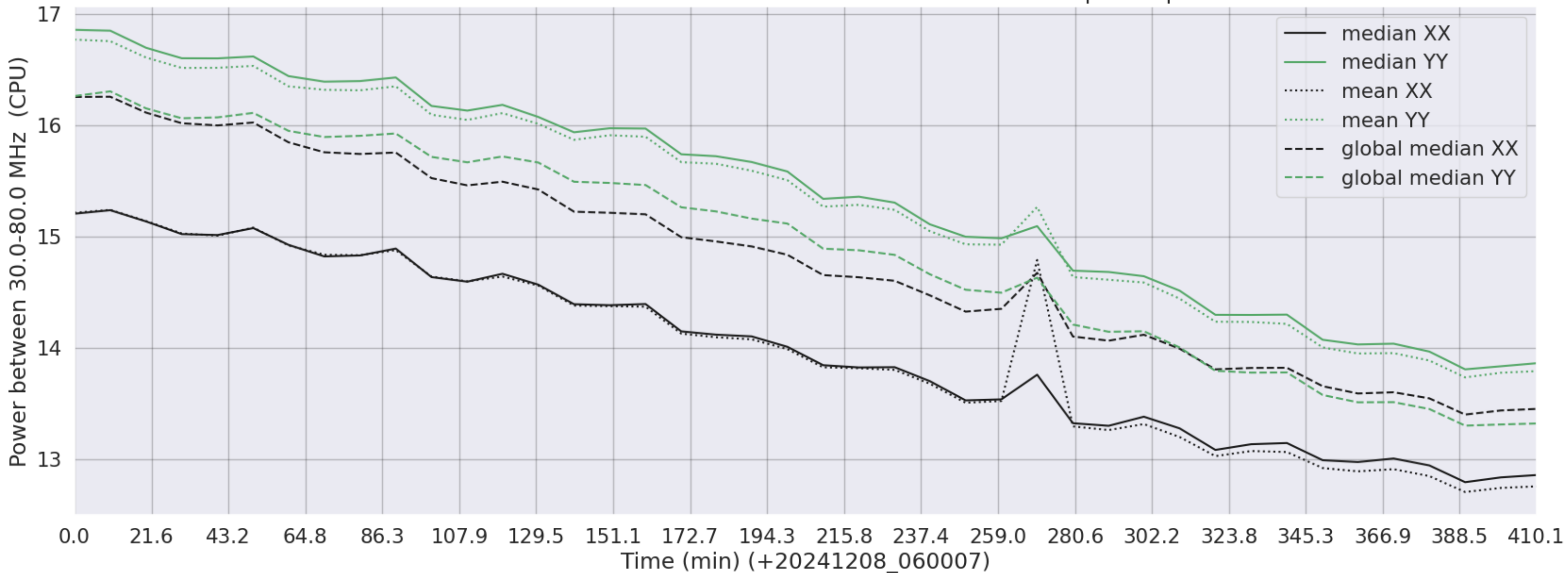
LWA321 - Correlator# 020 - XX FLAGS:Good - YY FLAGS:BadSpecShape
