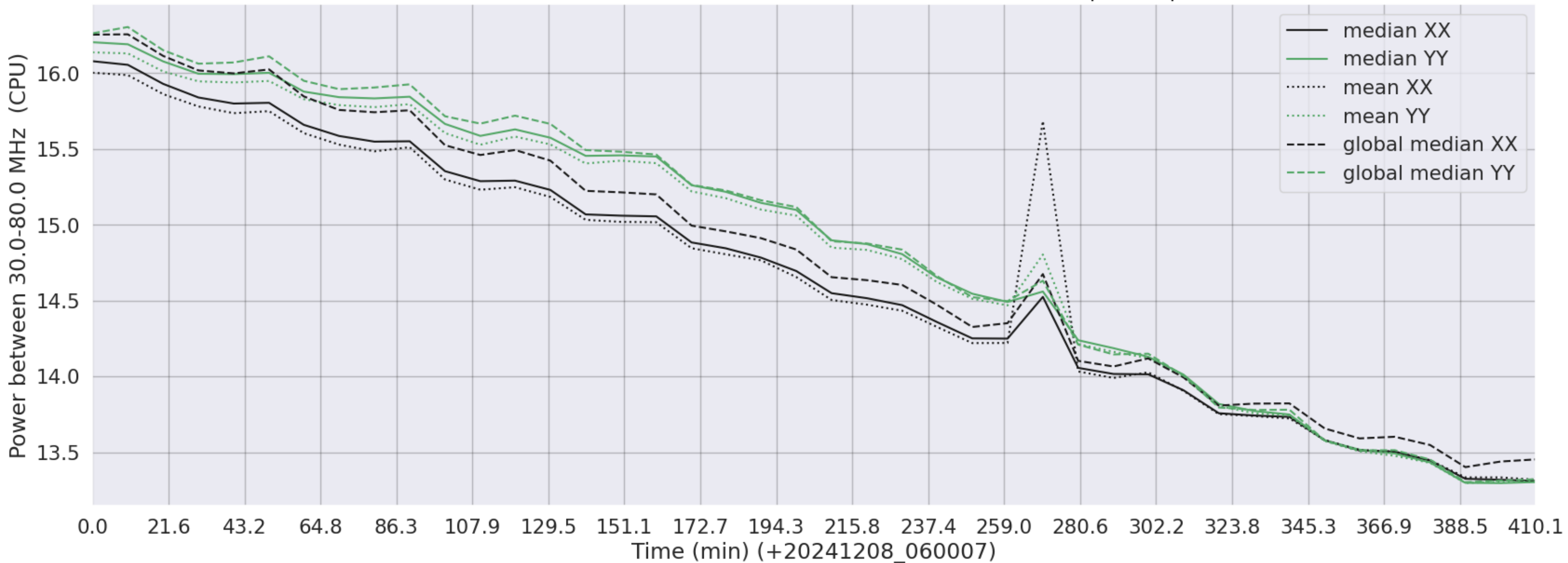
LWA273 - Correlator# 007 - XX FLAGS:Good - YY FLAGS:BadSpecShape
