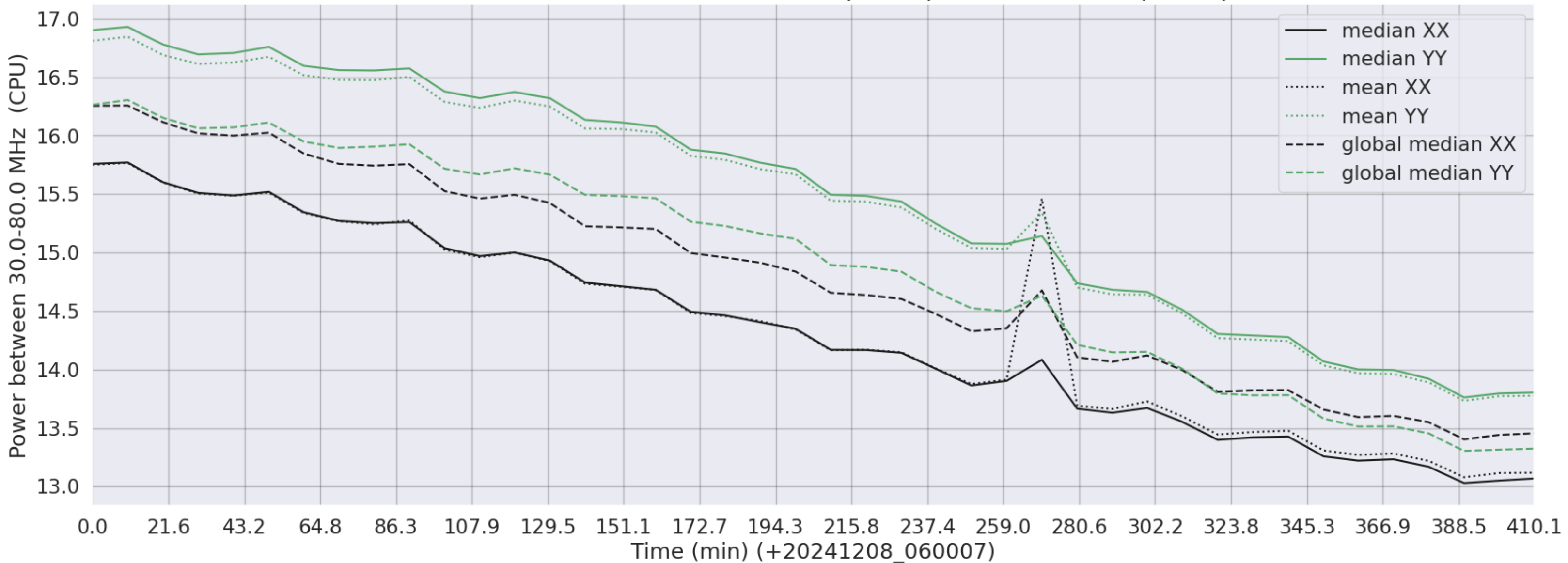
LWA037 - Correlator# 181 - XX FLAGS:BadSpecShape - YY FLAGS:BadSpecShape
