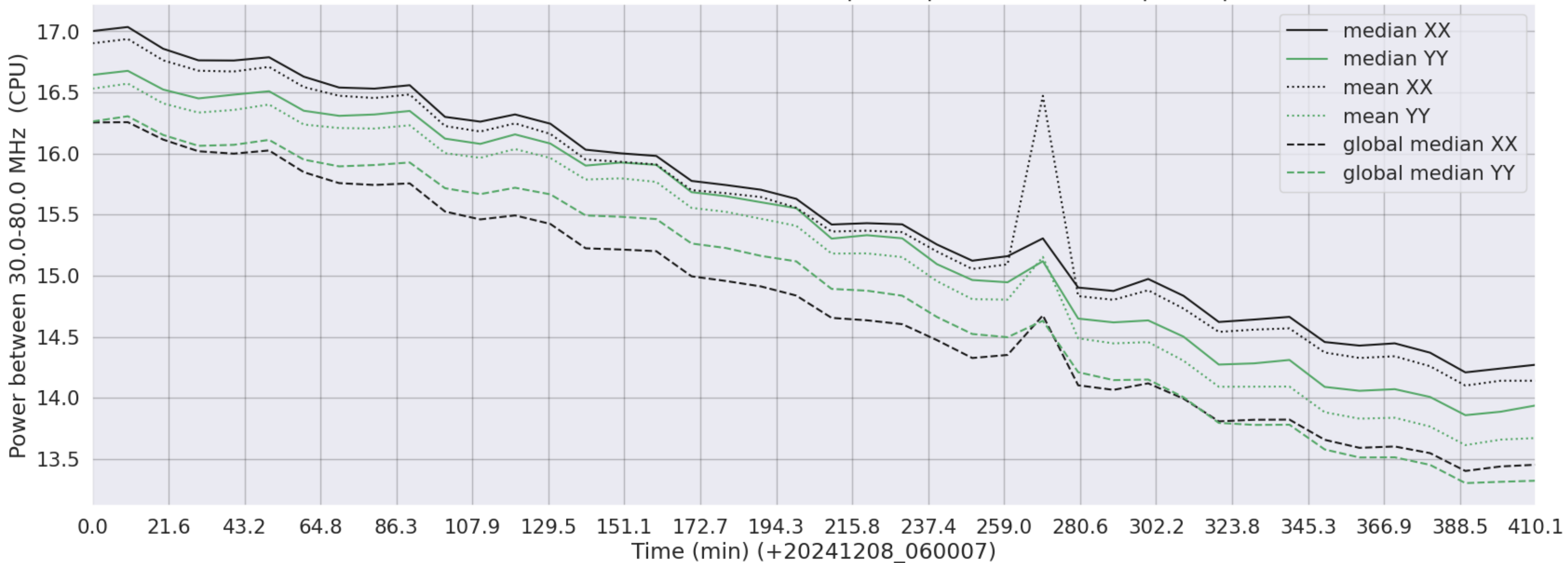
LWA135 - Correlator# 256 - XX FLAGS:BadSpecShape - YY FLAGS:BadSpecShape
