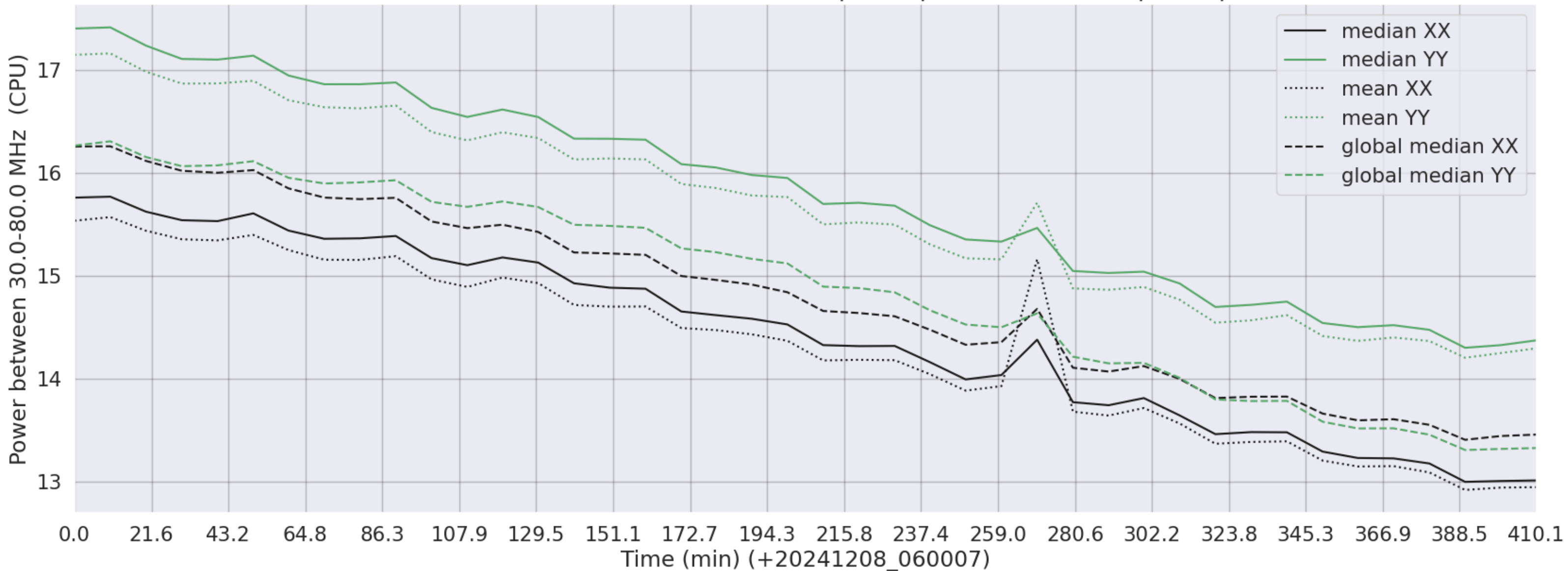
LWA252 - Correlator# 186 - XX FLAGS:BadSpecShape - YY FLAGS:BadSpecShape
