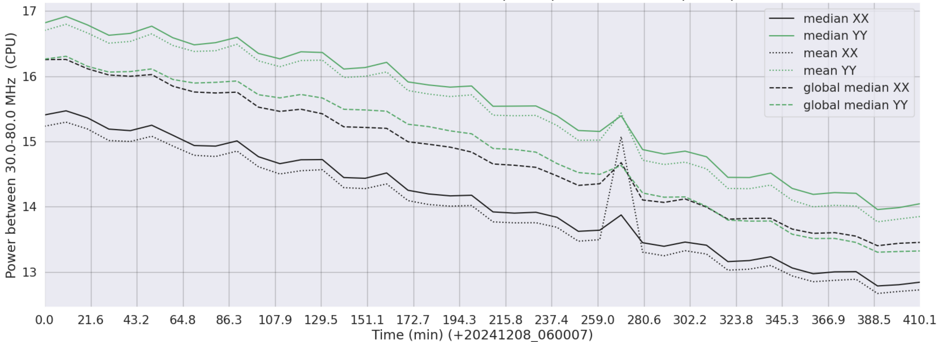
LWA198 - Correlator# 271 - XX FLAGS:BadSpecShape - YY FLAGS:BadSpecShape
