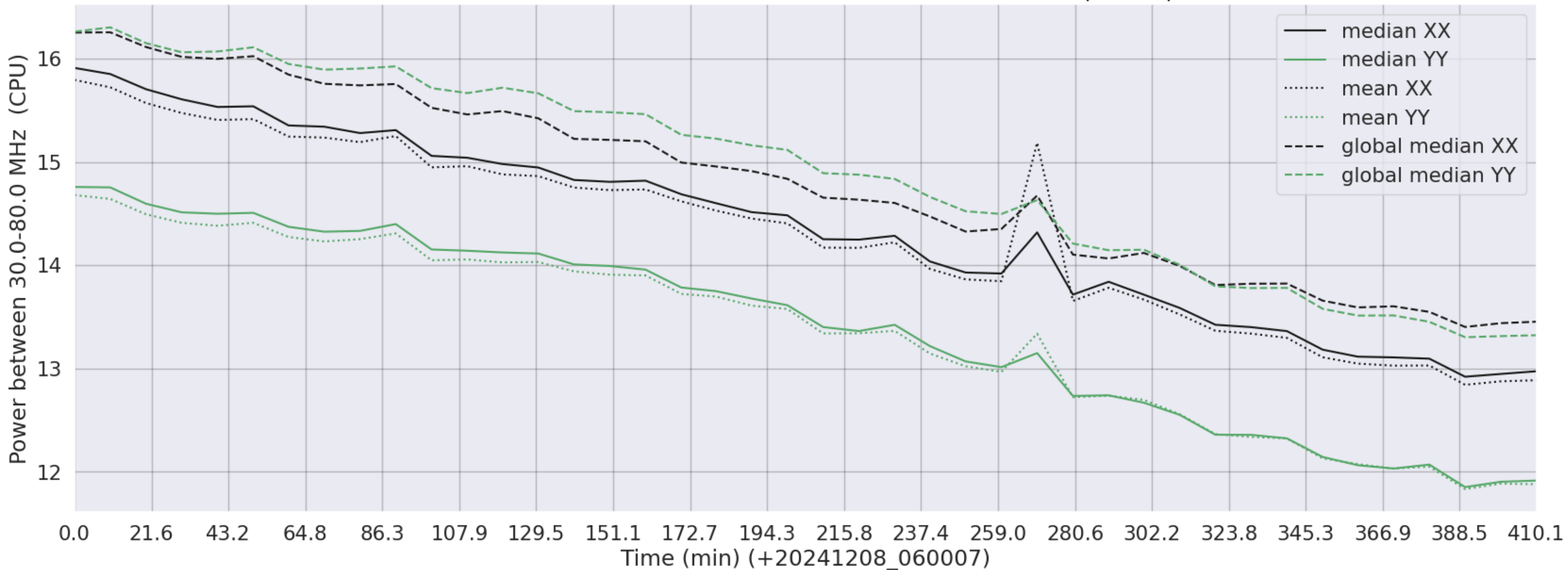
LWA360 - Correlator# 062 - XX FLAGS:Good - YY FLAGS:BadSpecShape
