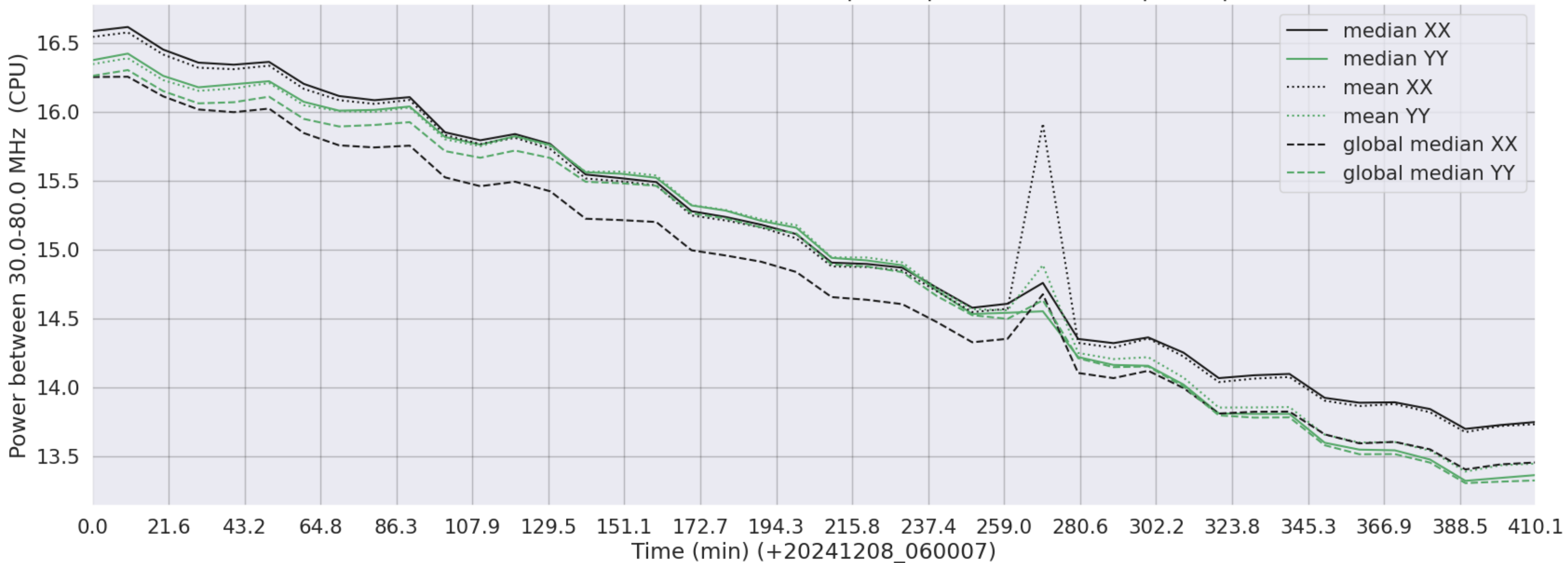
LWA229 - Correlator# 305 - XX FLAGS:BadSpecShape - YY FLAGS:BadSpecShape
