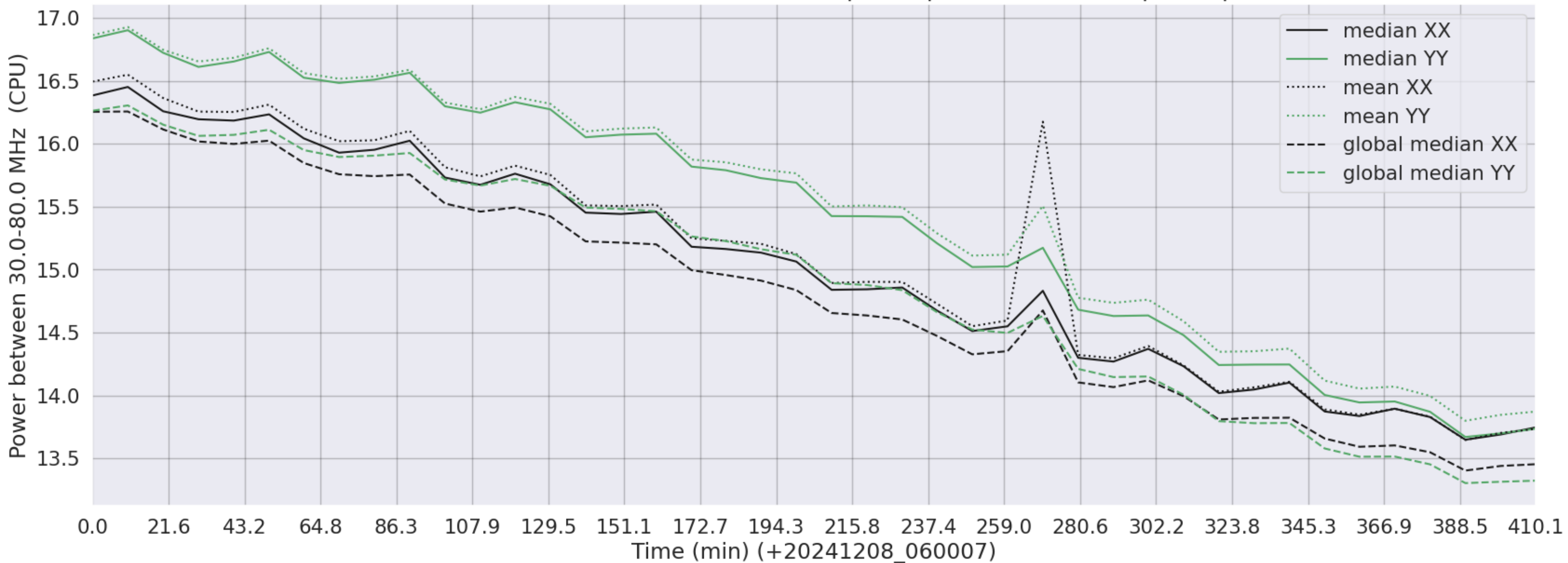
LWA001 - Correlator# 065 - XX FLAGS:BadSpecShape - YY FLAGS:BadSpecShape
