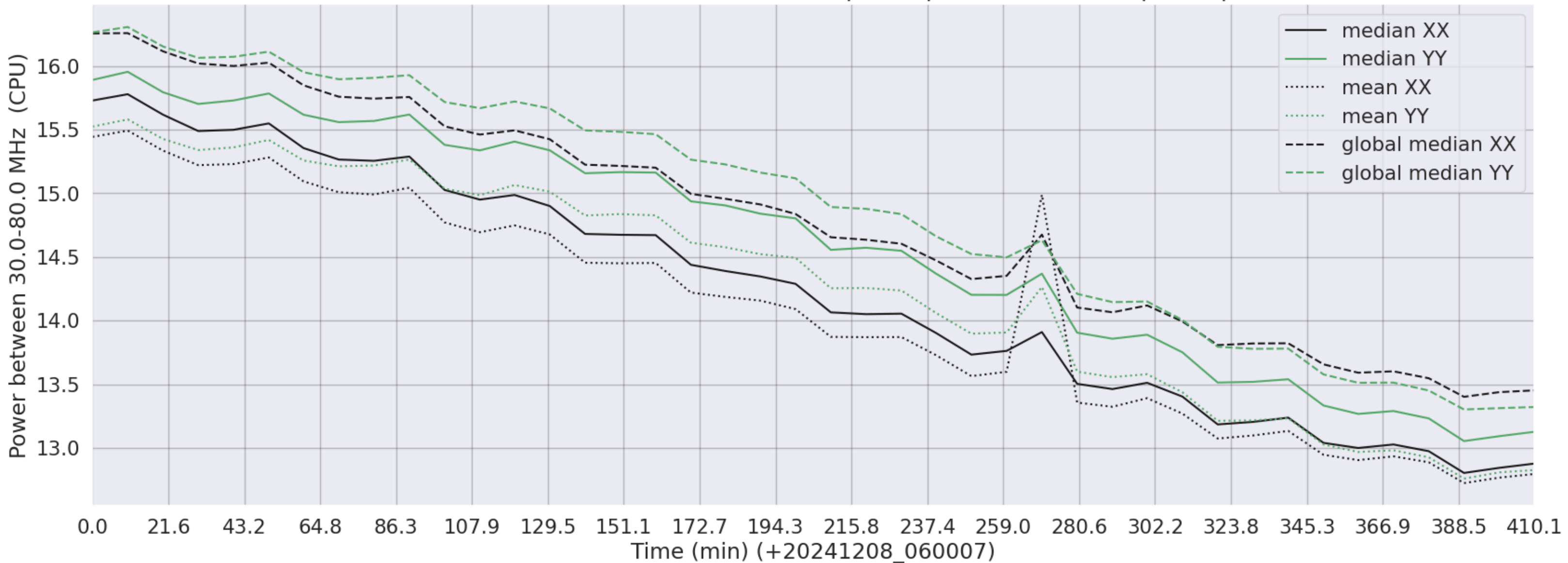
LWA162 - Correlator# 265 - XX FLAGS:BadSpecShape - YY FLAGS:BadSpecShape
