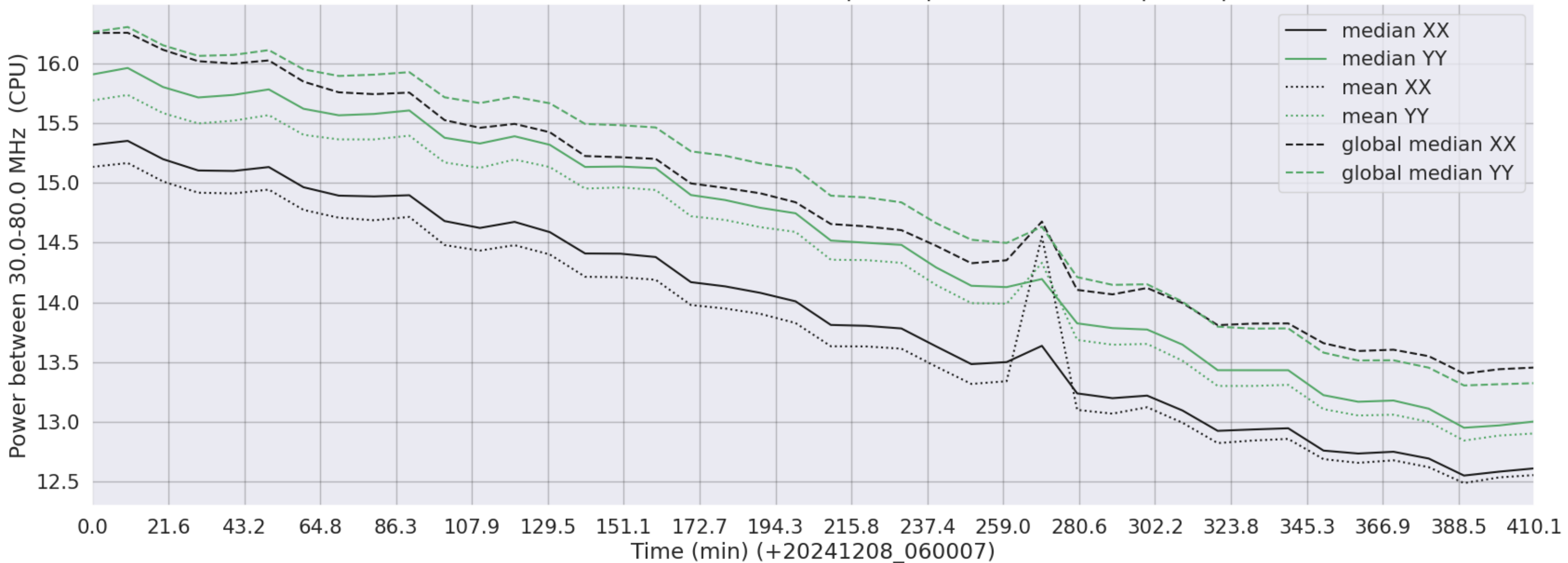
LWA199 - Correlator# 277 - XX FLAGS:BadSpecShape - YY FLAGS:BadSpecShape
