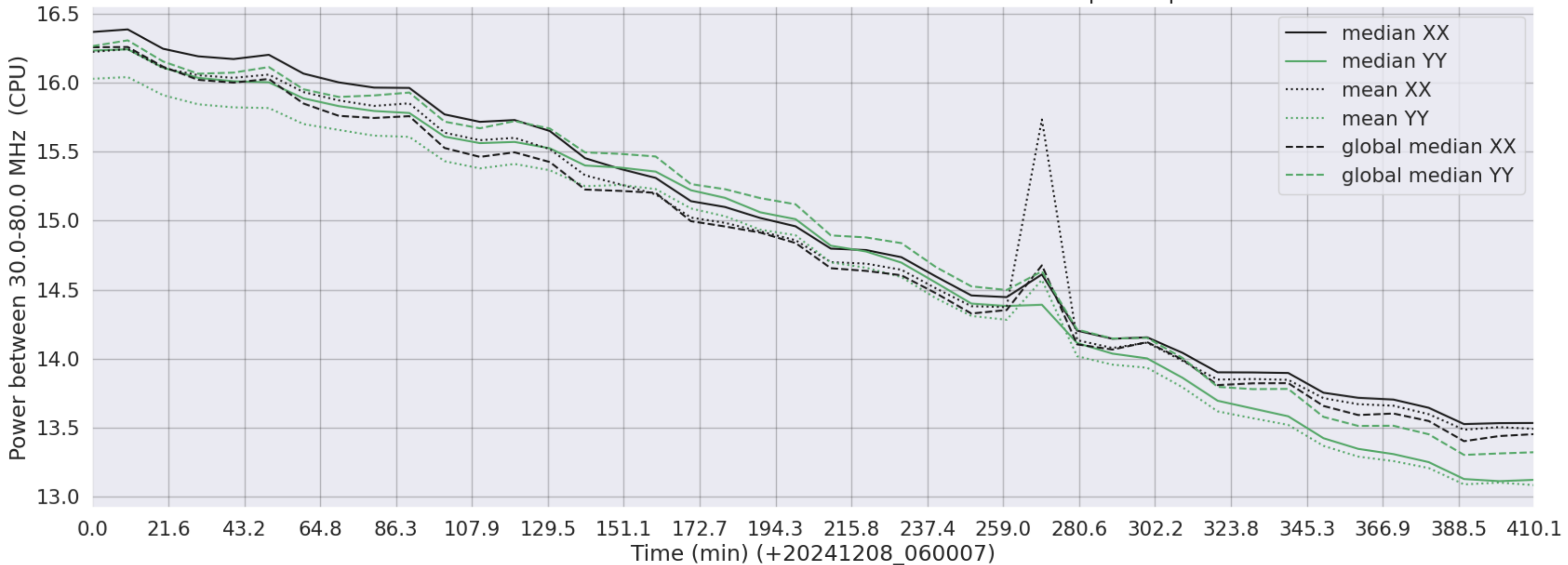
LWA345 - Correlator# 252 - XX FLAGS:Good - YY FLAGS:BadSpecShape
