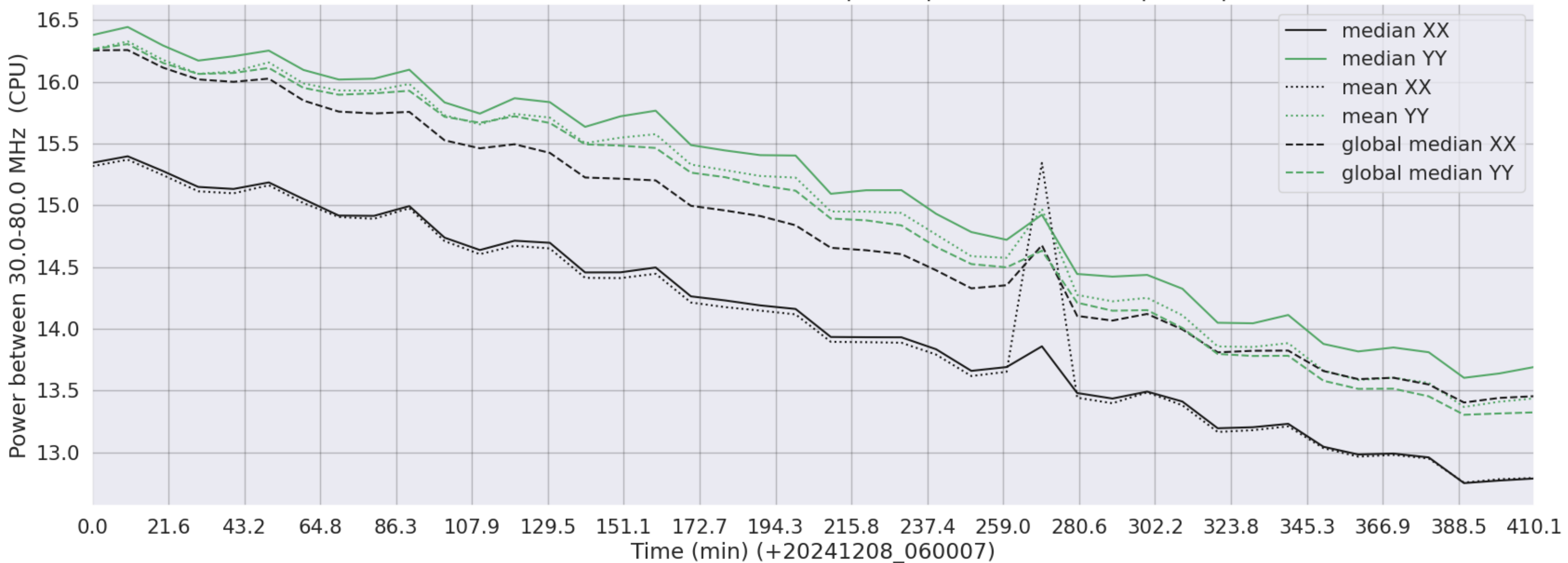
LWA070 - Correlator# 168 - XX FLAGS:BadSpecShape - YY FLAGS:BadSpecShape
