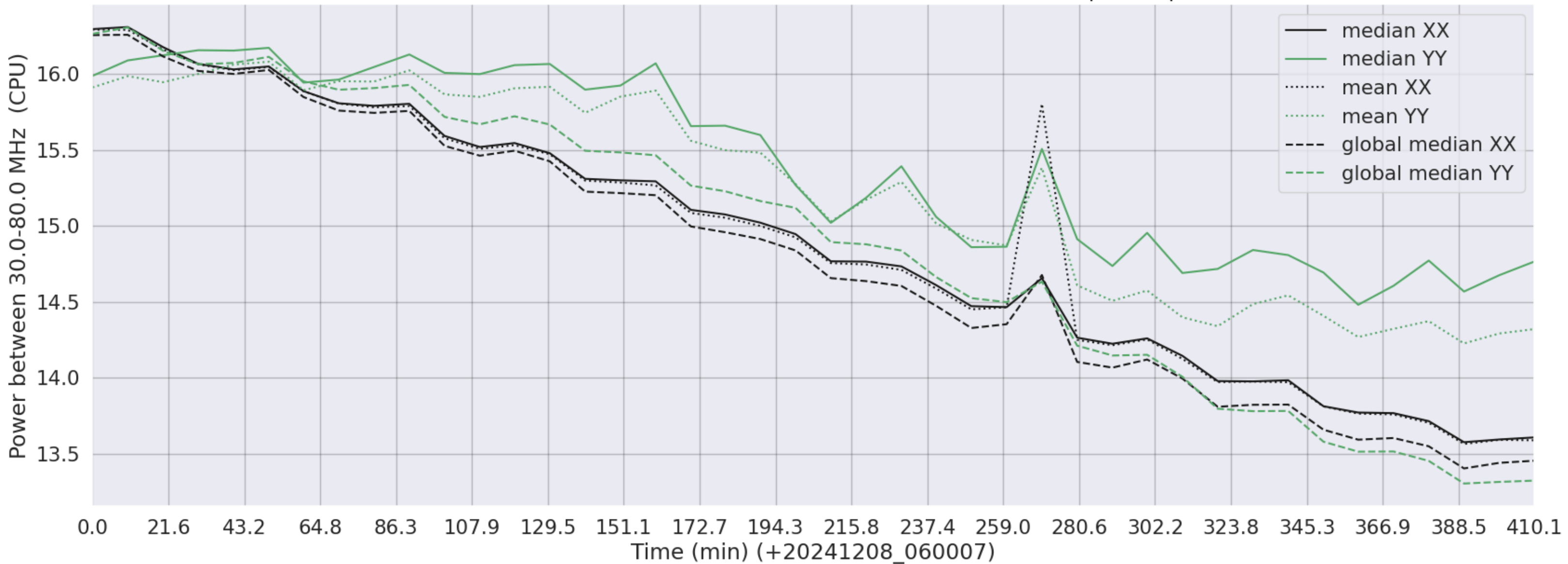
LWA282 - Correlator# 010 - XX FLAGS:Good - YY FLAGS:BadSpecShape
