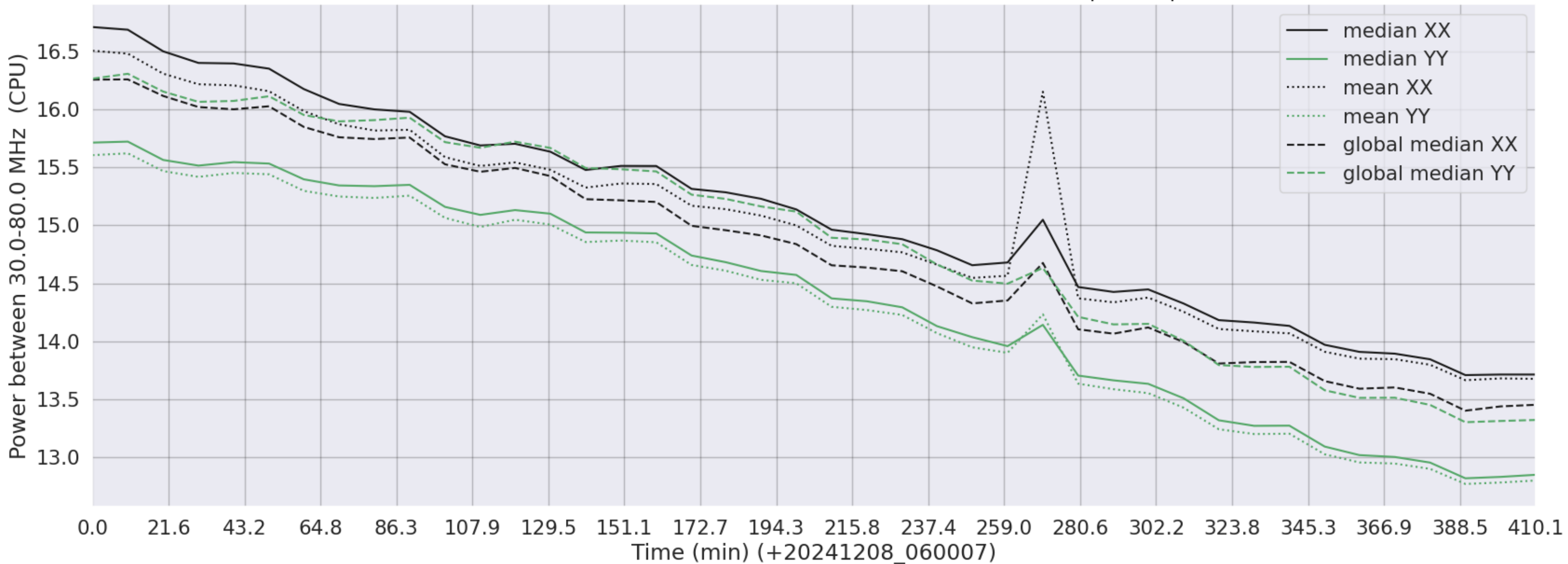
LWA258 - Correlator# 035 - XX FLAGS:Good - YY FLAGS:BadSpecShape
