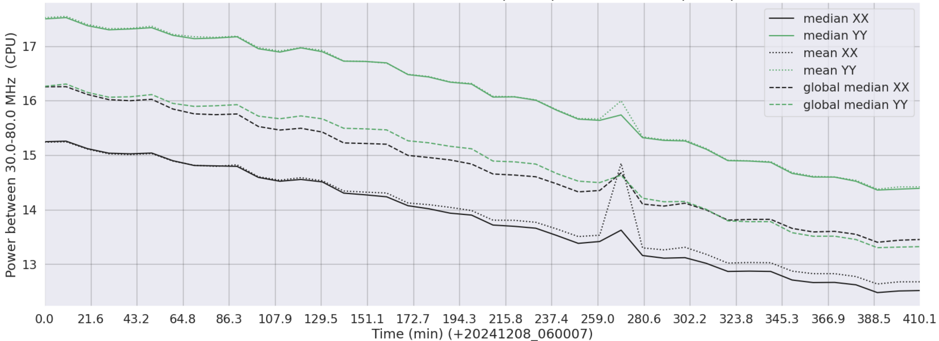
LWA041 - Correlator# 079 - XX FLAGS:BadSpecShape - YY FLAGS:BadSpecShape
