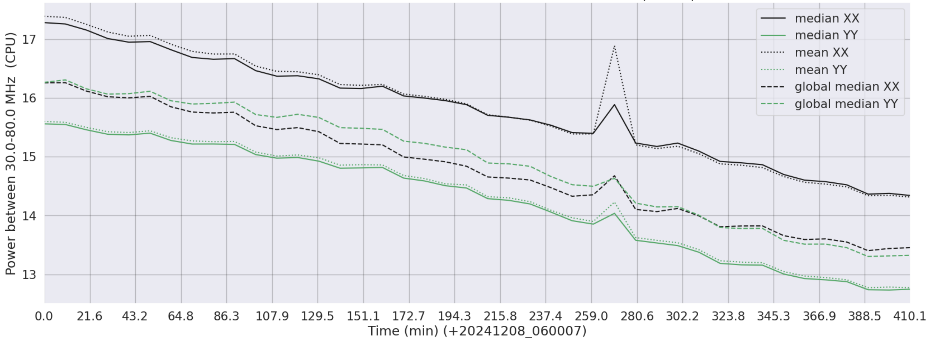
LWA340 - Correlator# 026 - XX FLAGS:Good - YY FLAGS:BadSpecShape
