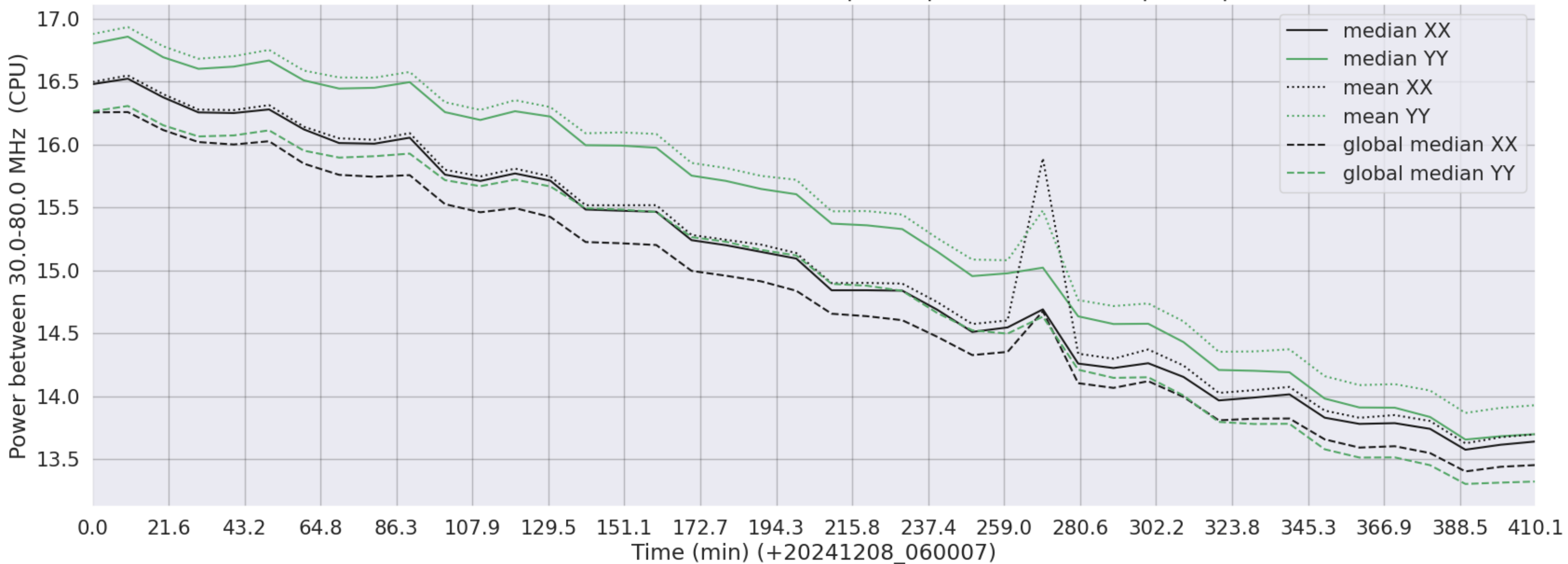
LWA228 - Correlator# 302 - XX FLAGS:BadSpecShape - YY FLAGS:BadSpecShape
