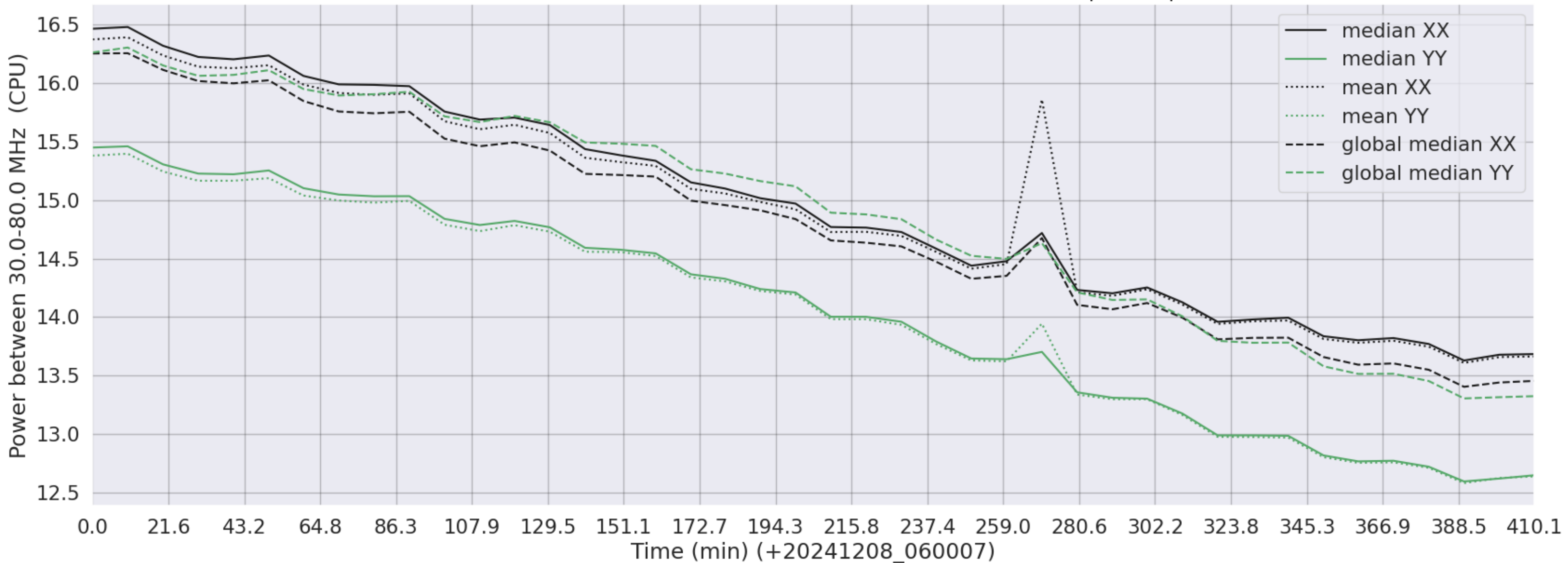
LWA142 - Correlator# 211 - XX FLAGS:Good - YY FLAGS:BadSpecShape
