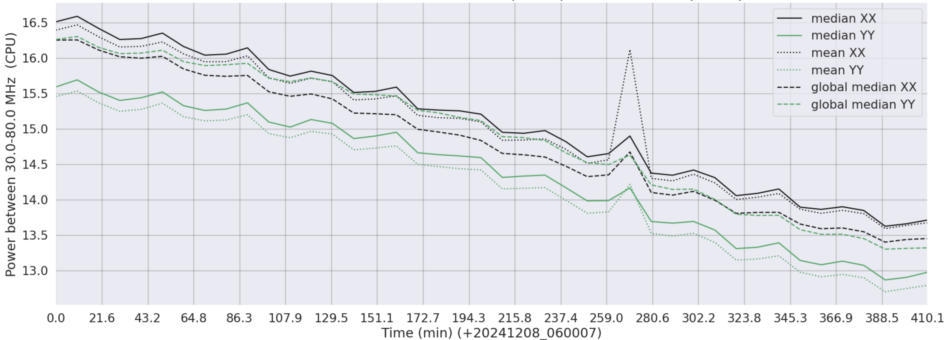
LWA161 - Correlator# 262 - XX FLAGS:BadSpecShape - YY FLAGS:BadSpecShape
