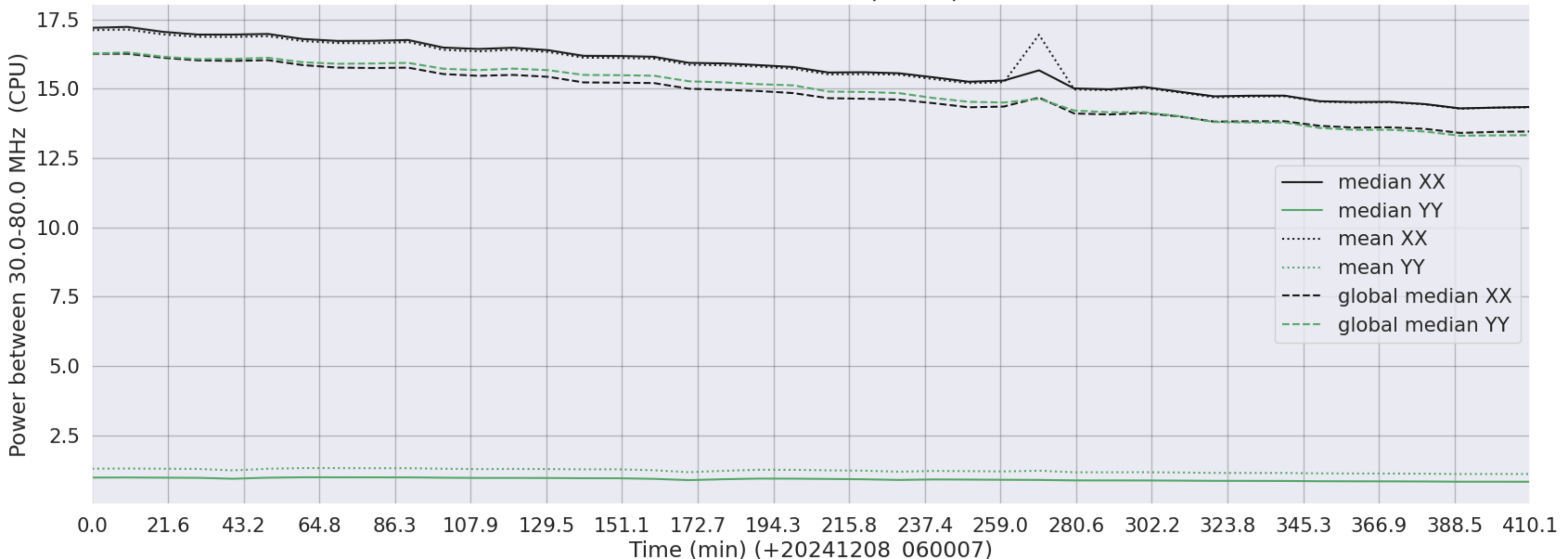
LWA005 - Correlator# 069 - XX FLAGS:BadSpecShape - YY FLAGS:LowPower
