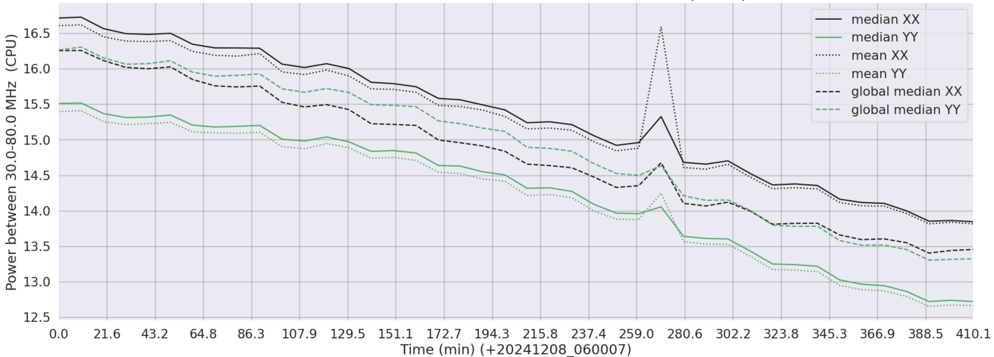
LWA015 - Correlator# 098 - XX FLAGS:Good - YY FLAGS:BadSpecShape
