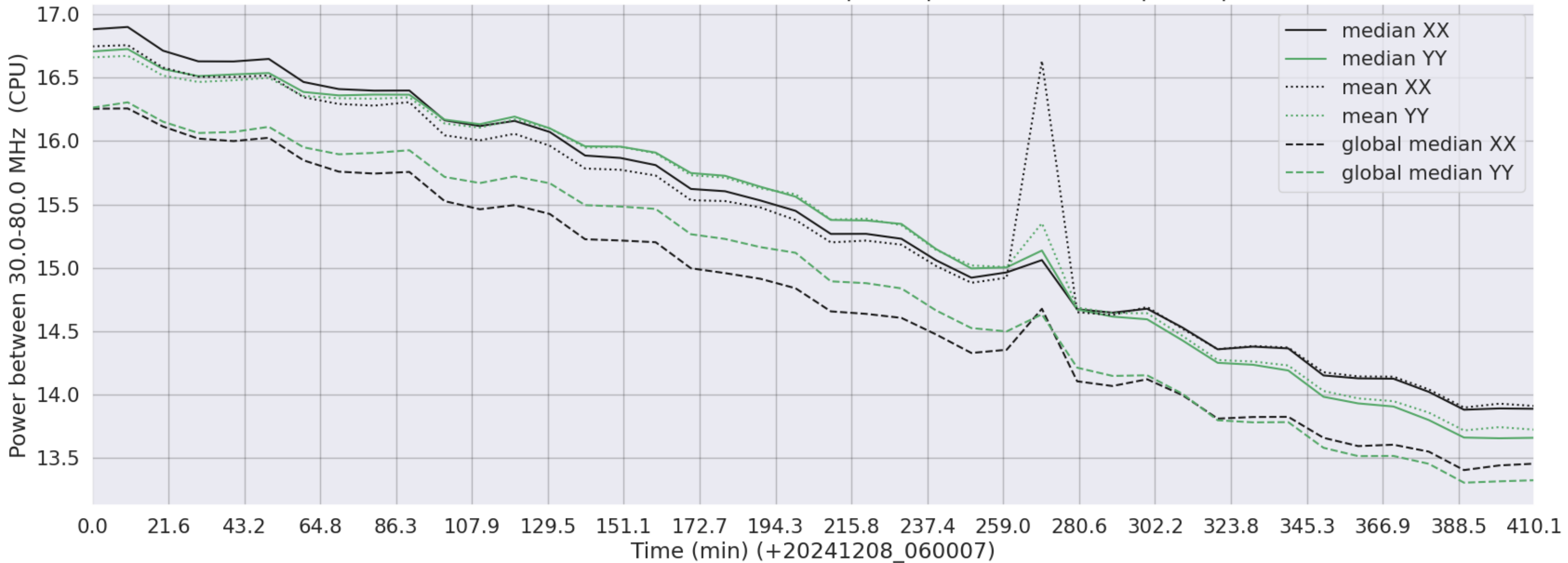
LWA033 - Correlator# 161 - XX FLAGS:BadSpecShape - YY FLAGS:BadSpecShape
