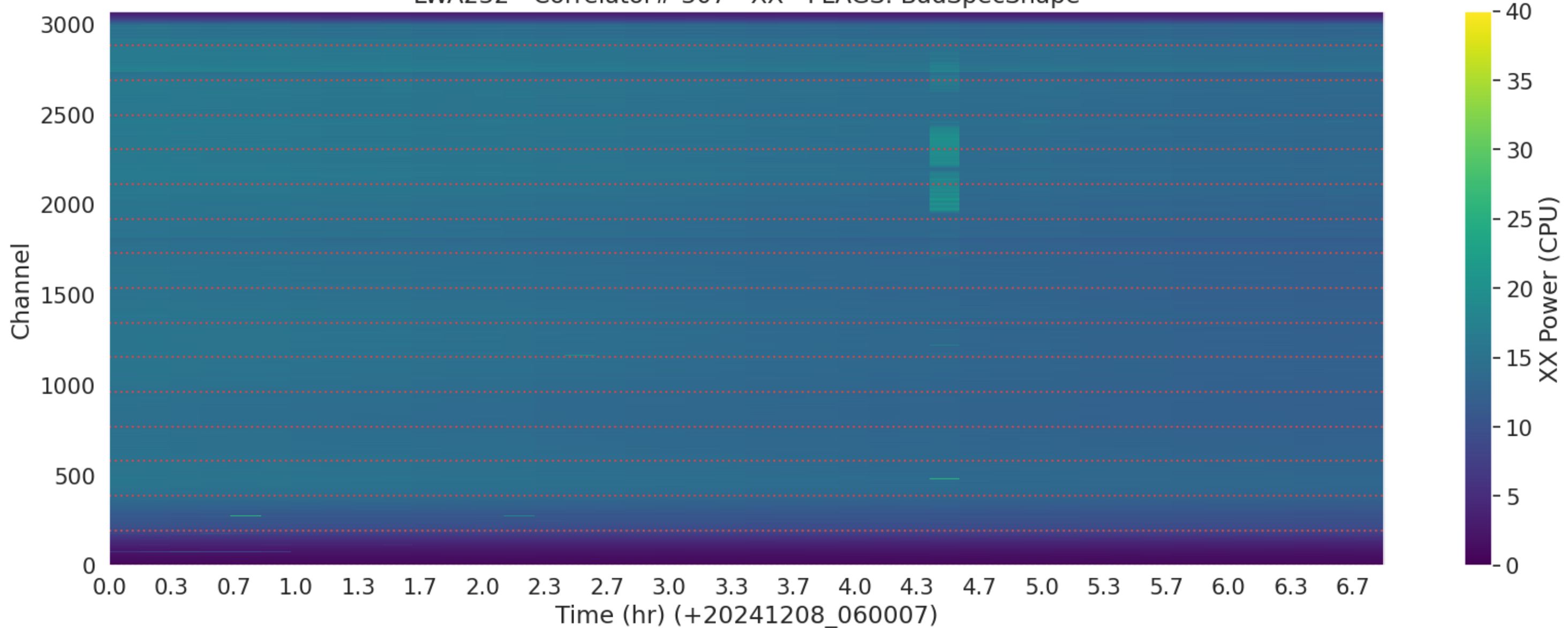
LWA232 - Correlator# 307 - XX - FLAGS: BadSpecShape
