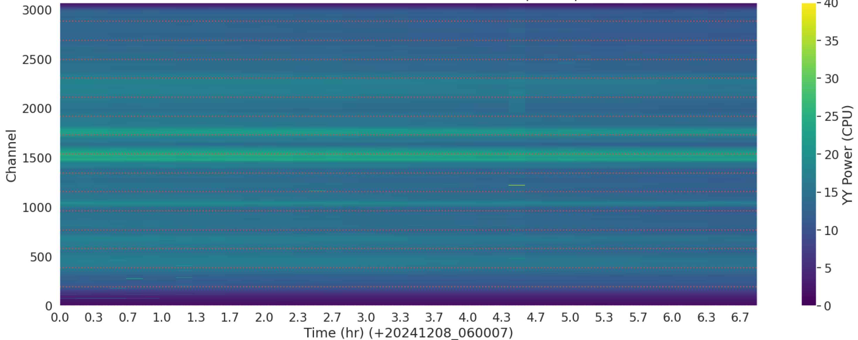
LWA336 - Correlator# 056 - YY - FLAGS: BadSpecShape
