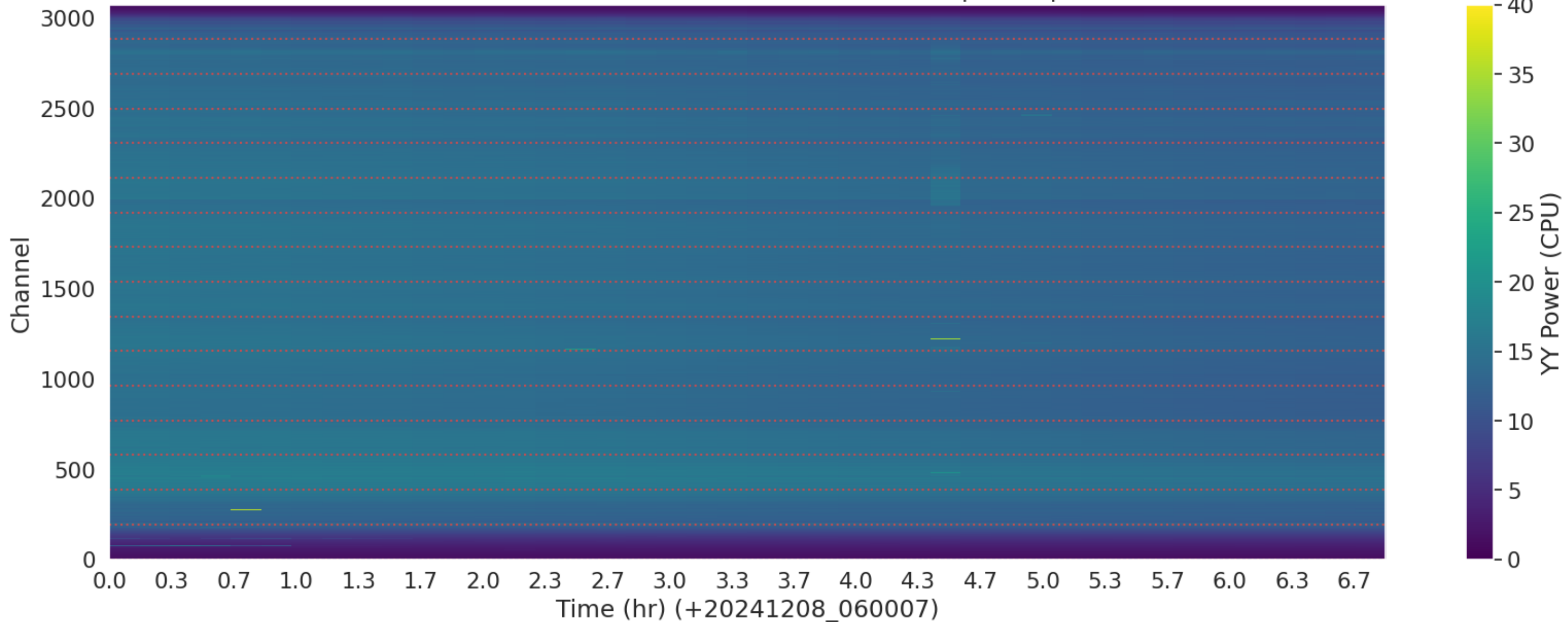
LWA351 - Correlator# 060 - YY - FLAGS: BadSpecShape
