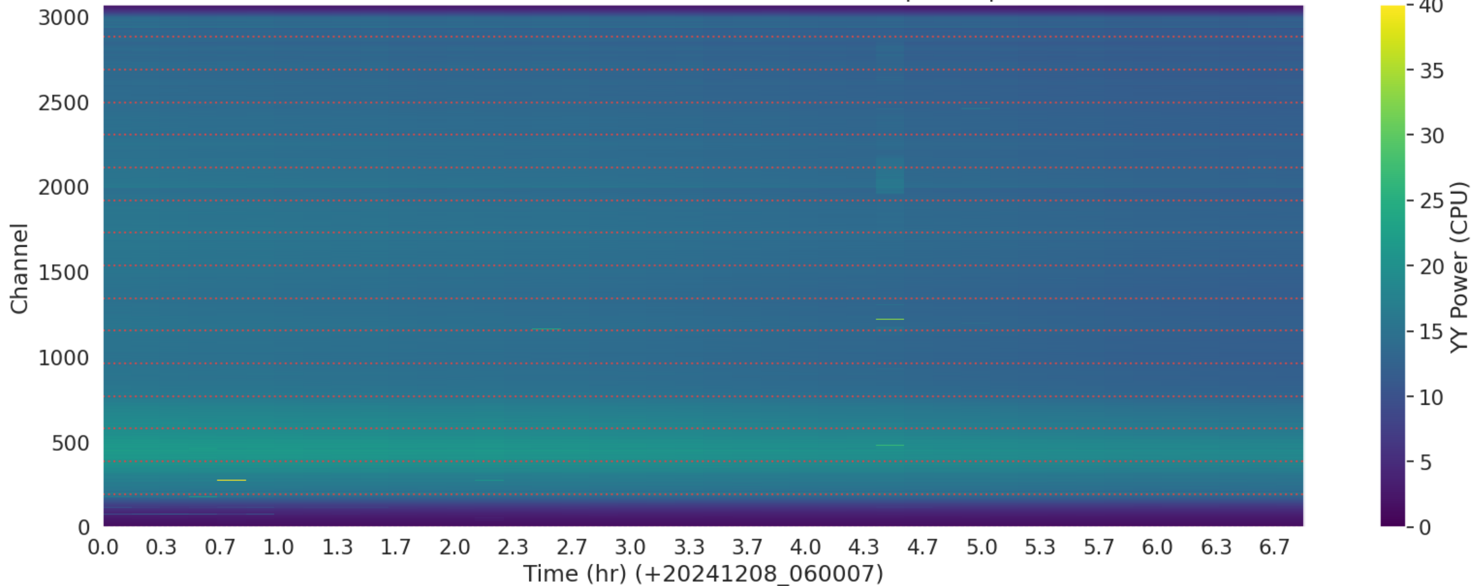
LWA287 - Correlator# 223 - YY - FLAGS: BadSpecShape
