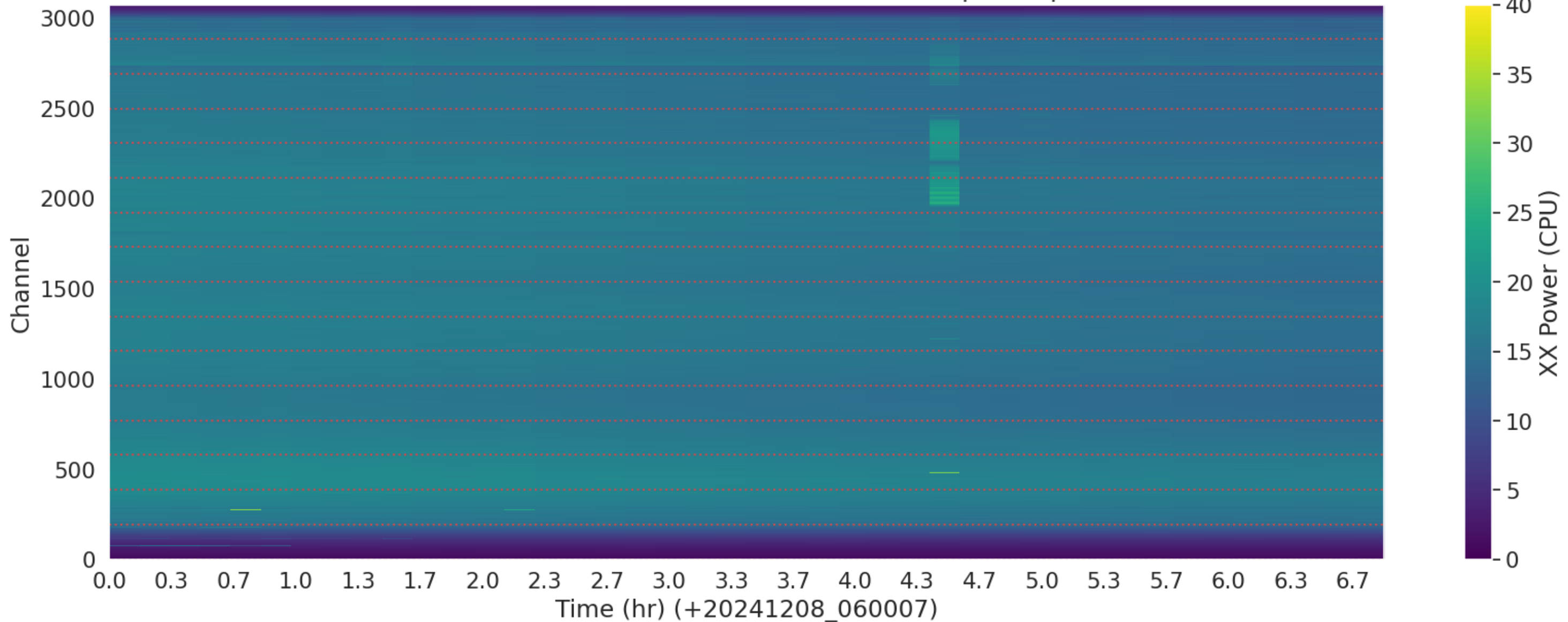
LWA036 - Correlator# 163 - XX - FLAGS: BadSpecShape
