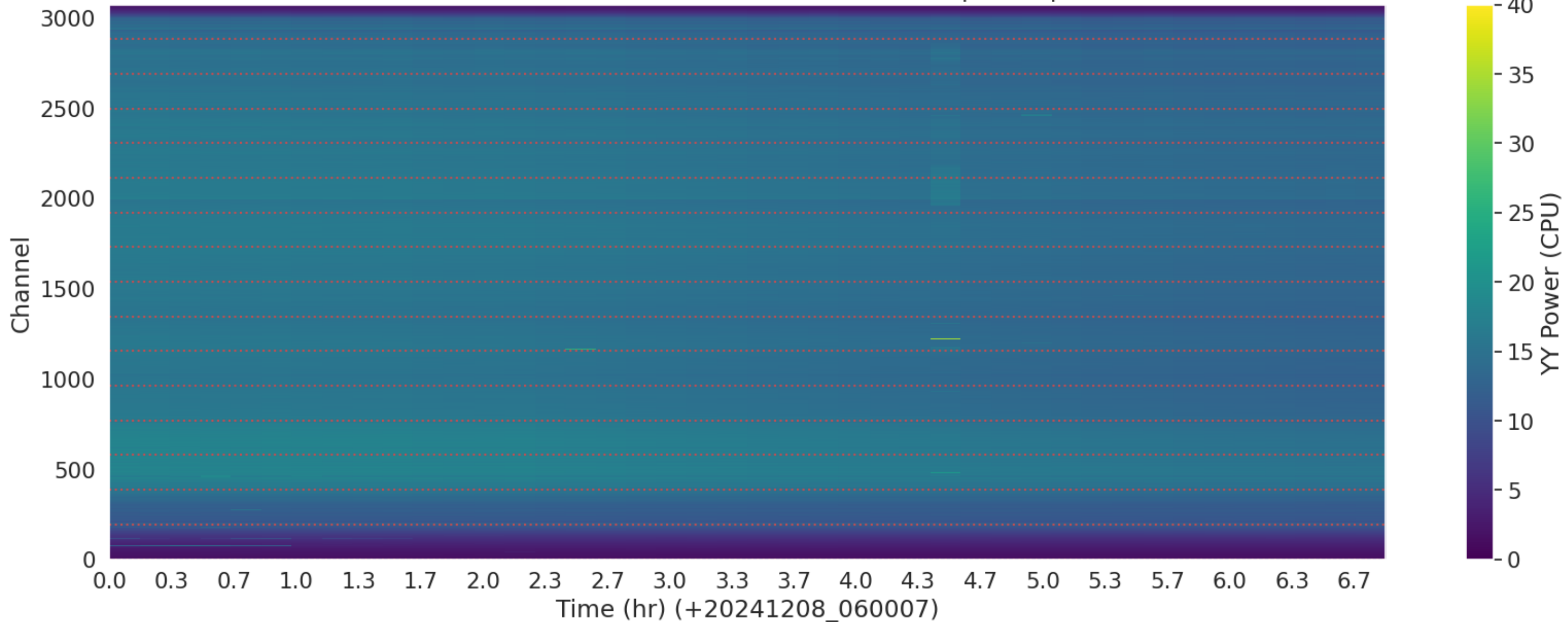
LWA281 - Correlator# 011 - YY - FLAGS: BadSpecShape
