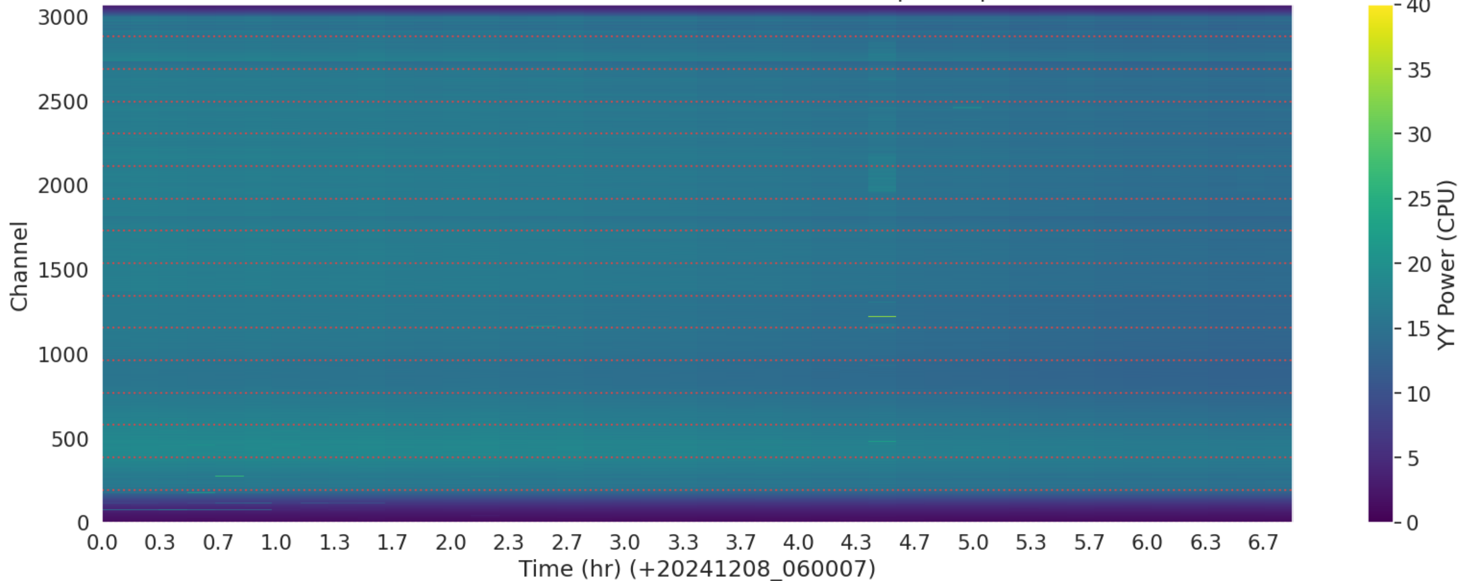
LWA198 - Correlator# 271 - YY - FLAGS: BadSpecShape
