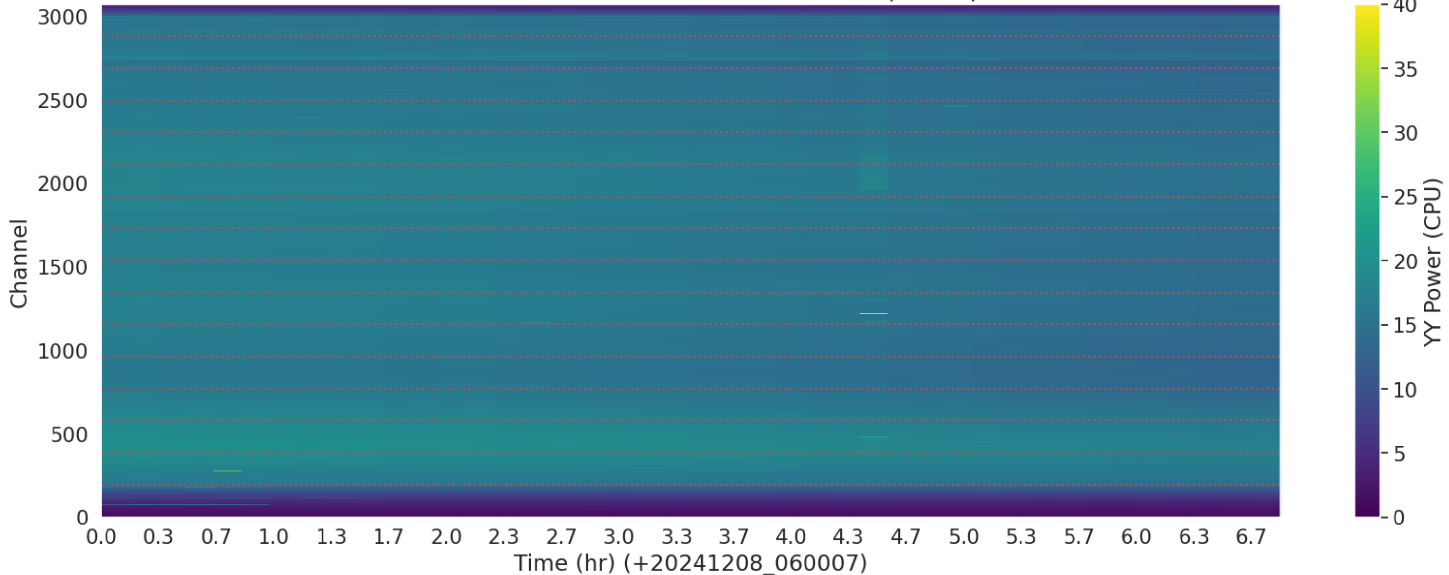
LWA036 - Correlator# 163 - YY - FLAGS: BadSpecShape
