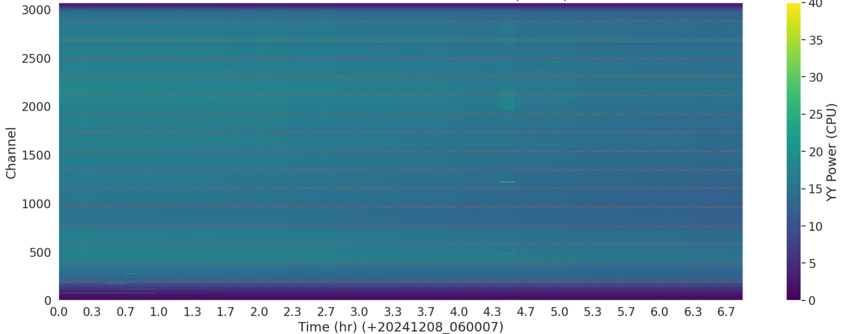
LWA225 - Correlator# 281 - YY - FLAGS: BadSpecShape
