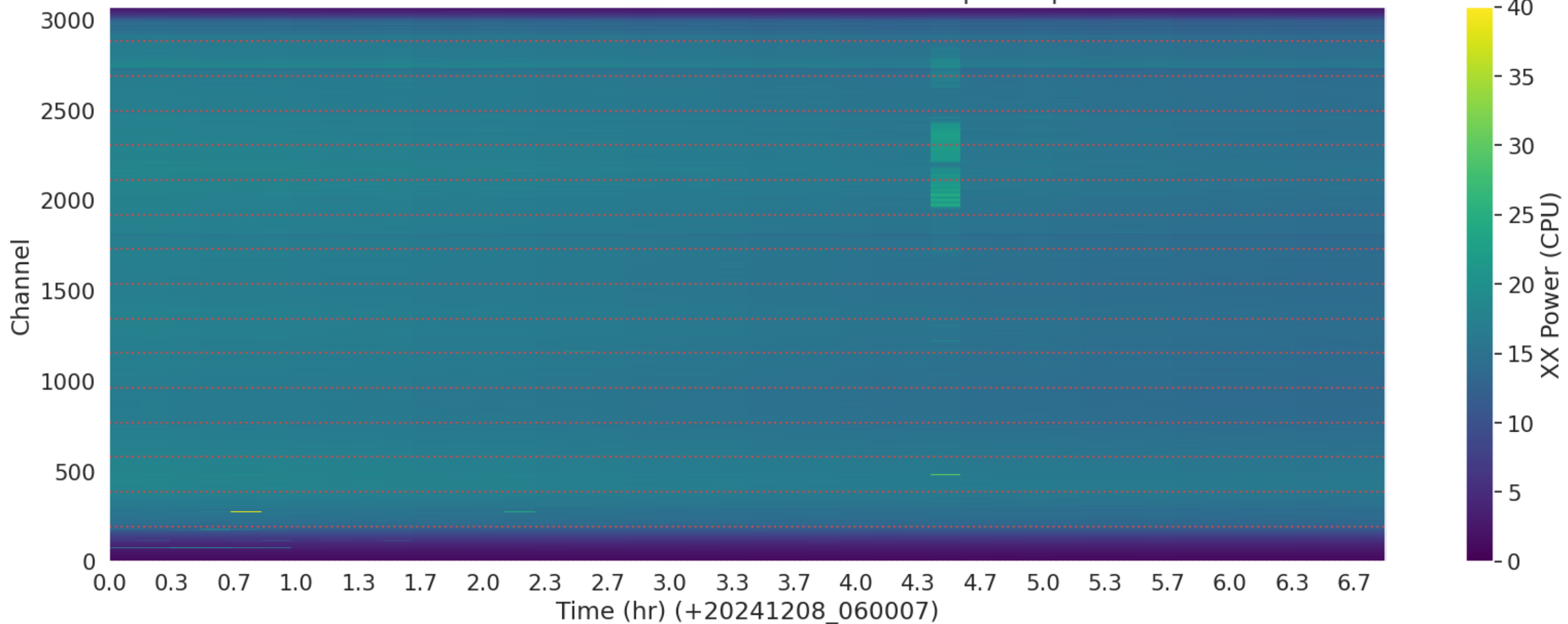
LWA203 - Correlator# 295 - XX - FLAGS: BadSpecShape
