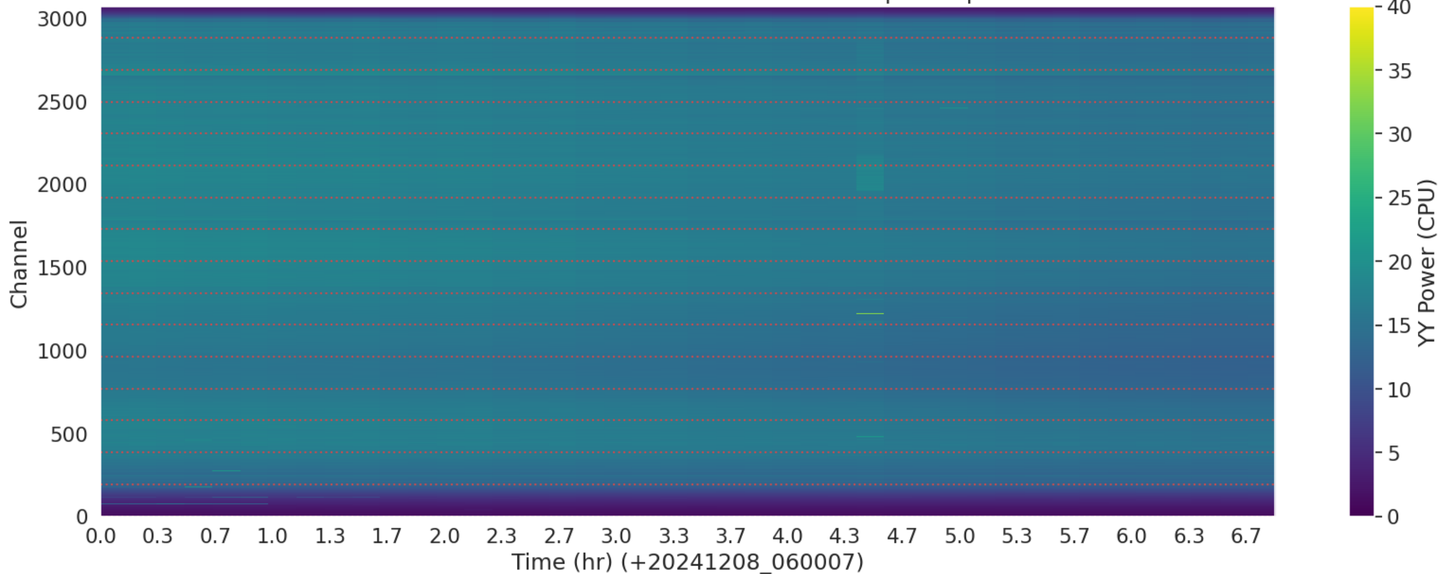
LWA193 - Correlator# 270 - YY - FLAGS: BadSpecShape
