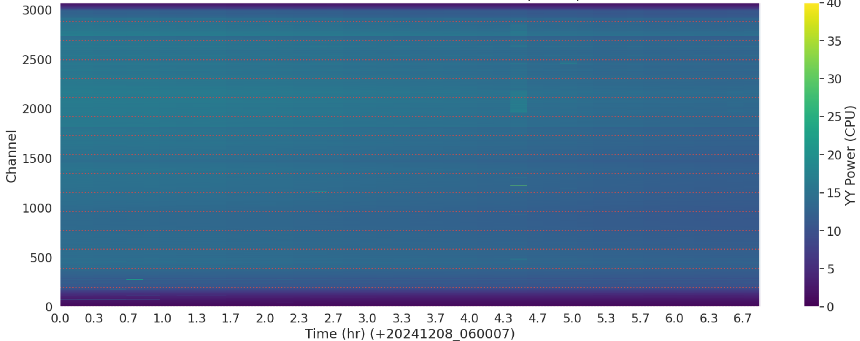
LWA100 - Correlator# 175 - YY - FLAGS: BadSpecShape
