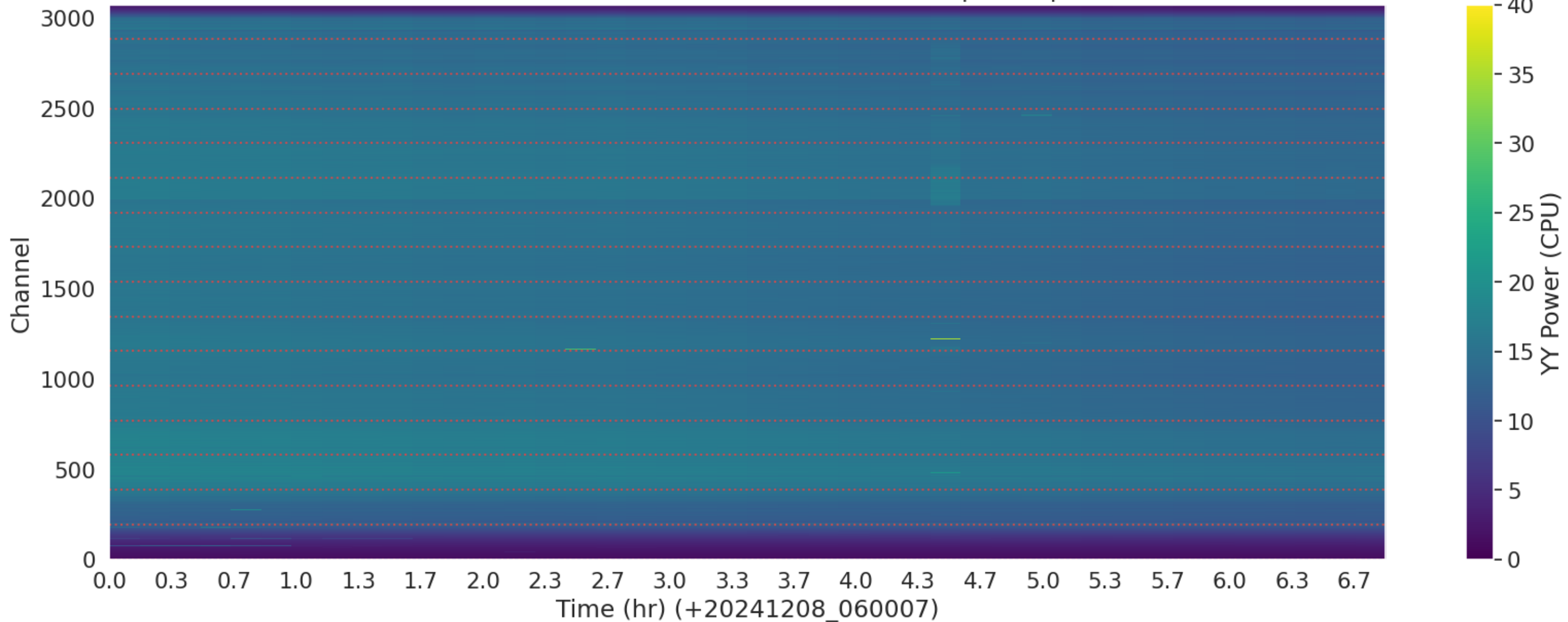
LWA262 - Correlator# 123 - YY - FLAGS: BadSpecShape
