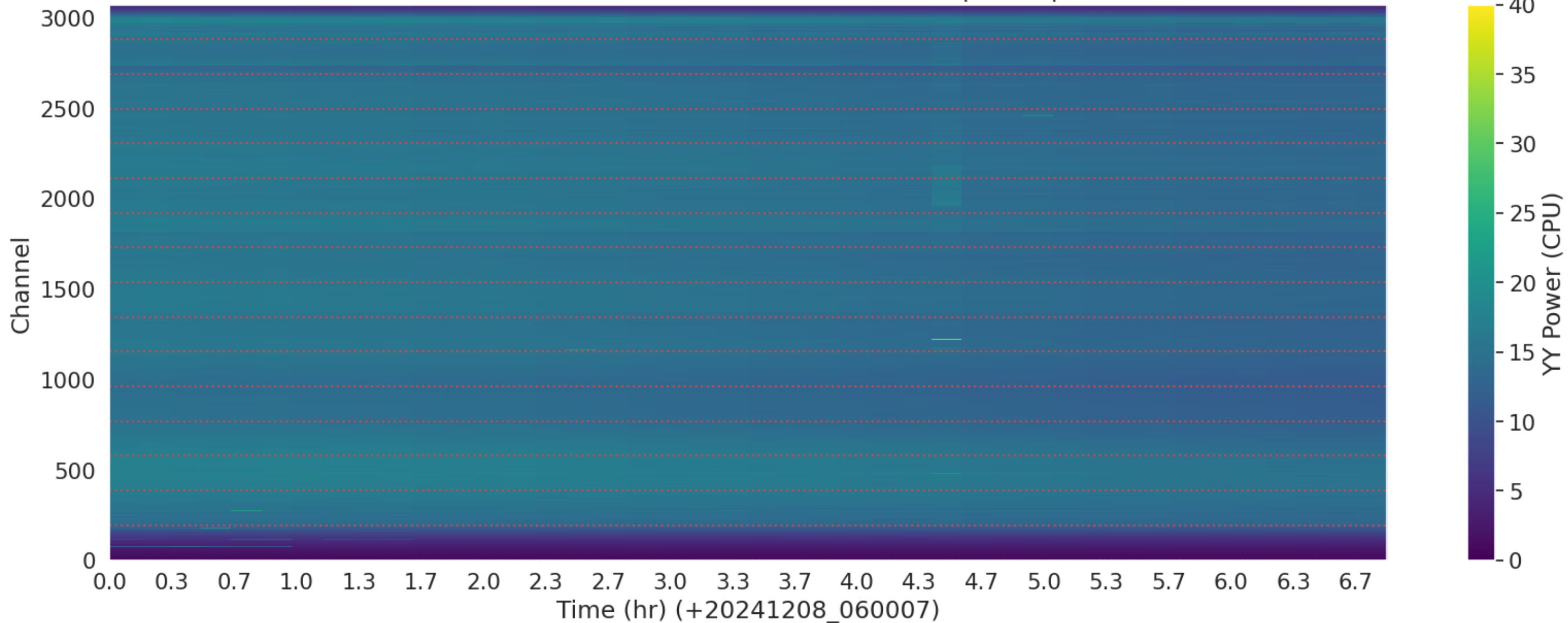
LWA133 - Correlator# 257 - YY - FLAGS: BadSpecShape
