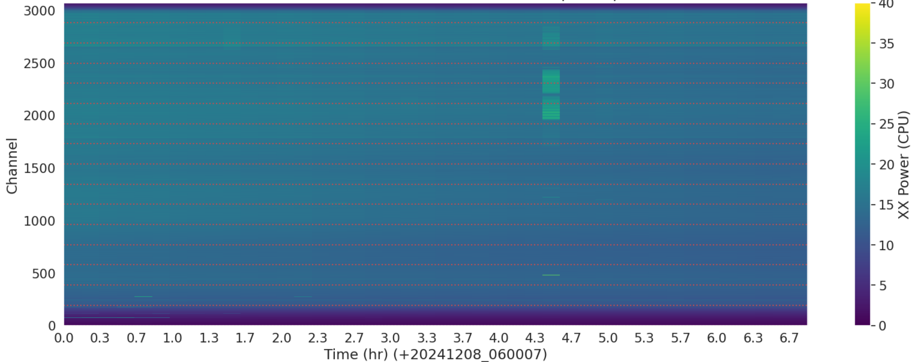
LWA003 - Correlator# 067 - XX - FLAGS: BadSpecShape
