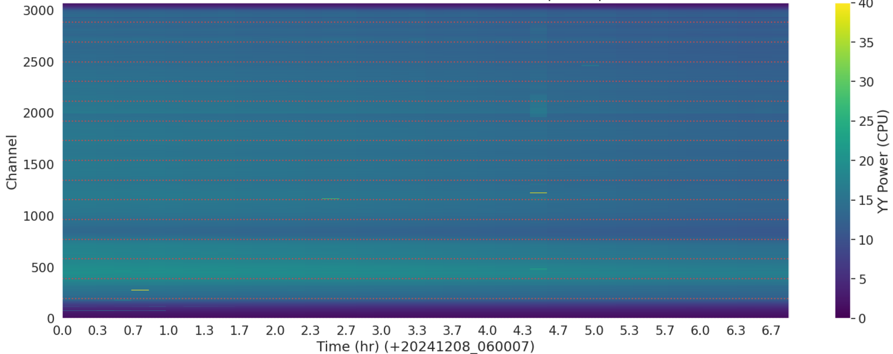
LWA283 - Correlator# 040 - YY - FLAGS: BadSpecShape
