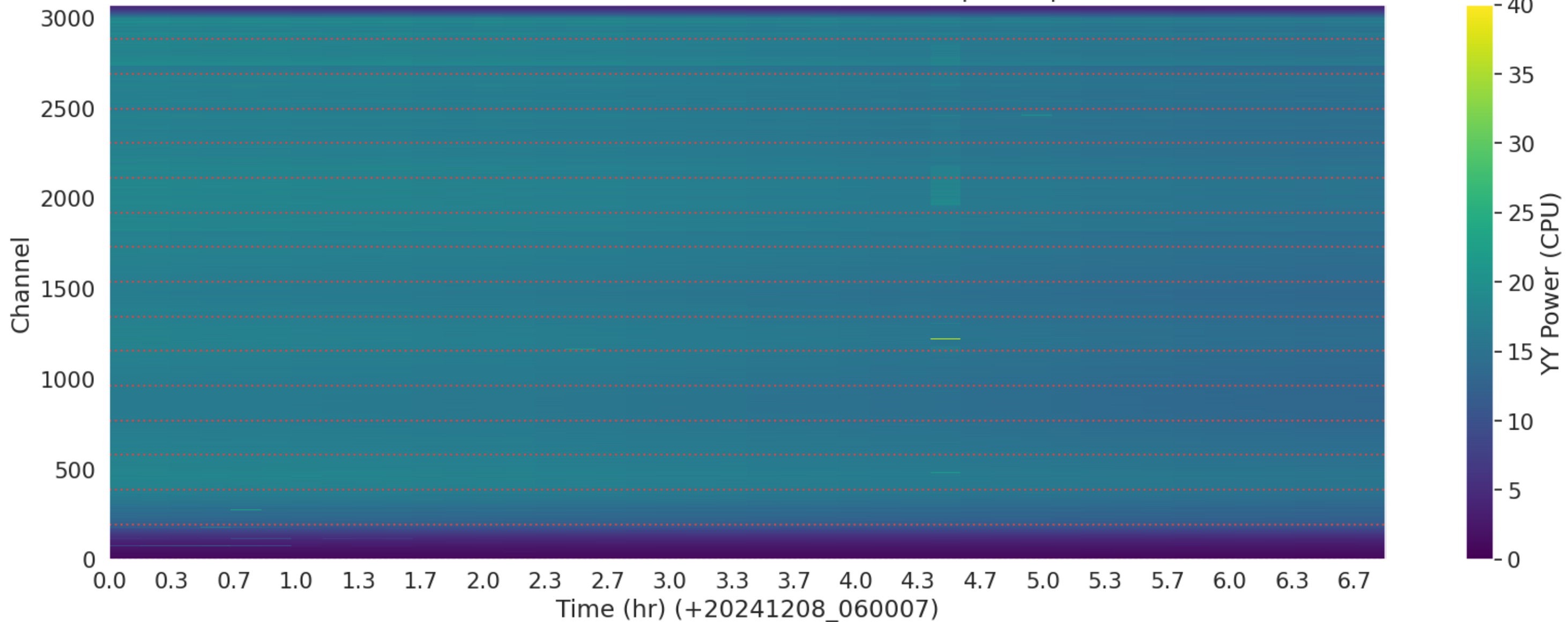
LWA041 - Correlator# 079 - YY - FLAGS: BadSpecShape
