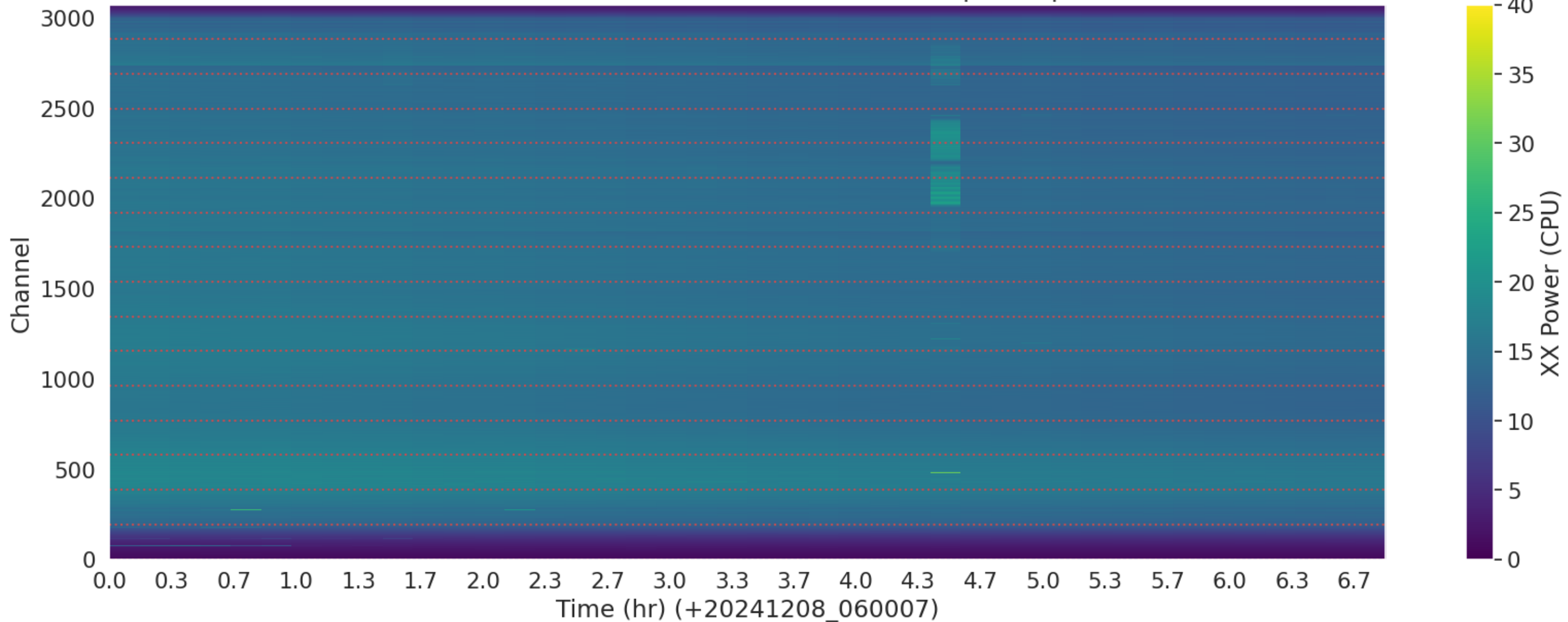
LWA067 - Correlator# 167 - XX - FLAGS: BadSpecShape
