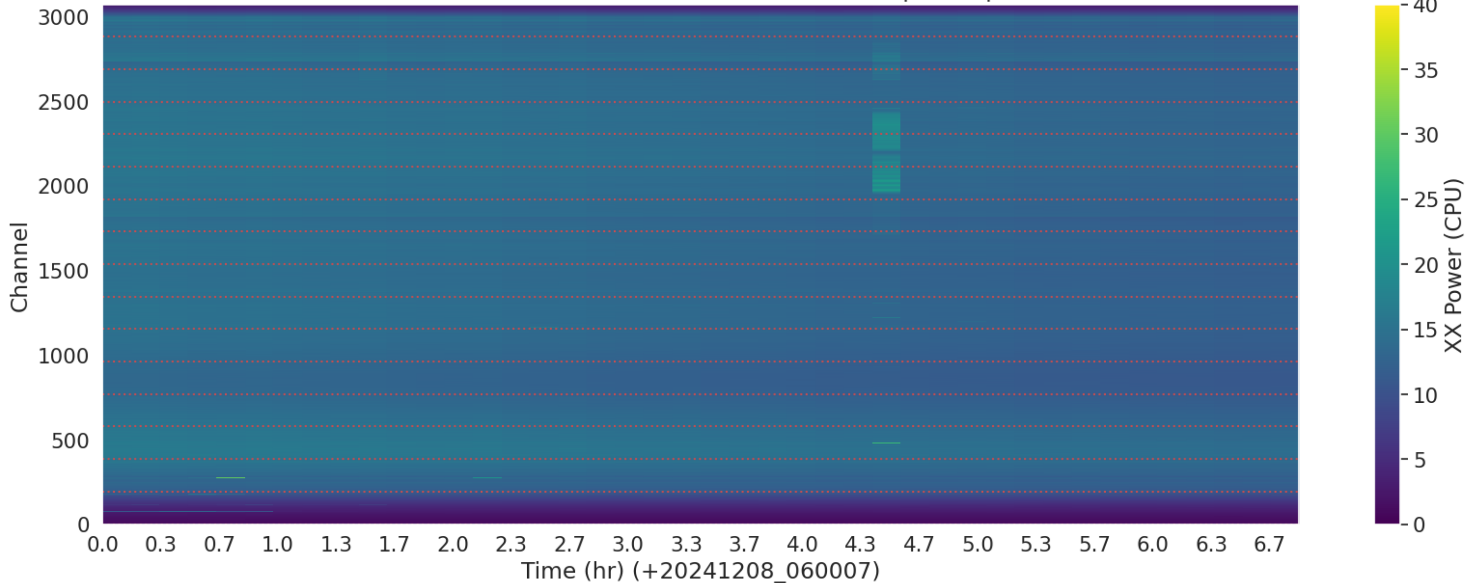
LWA201 - Correlator# 279 - XX - FLAGS: BadSpecShape
