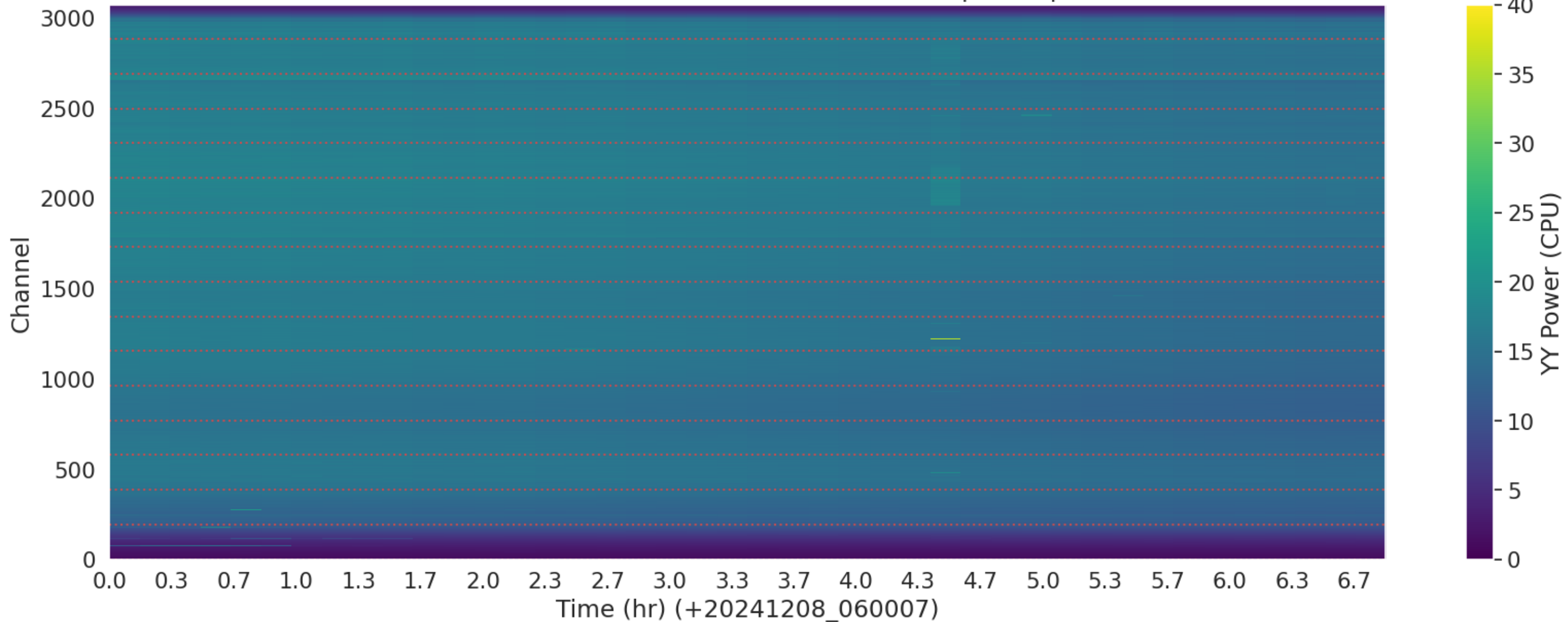
LWA065 - Correlator# 165 - YY - FLAGS: BadSpecShape
