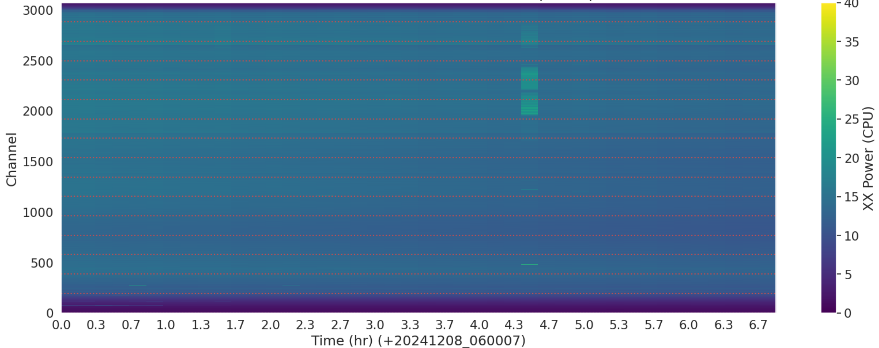
LWA097 - Correlator# 170 - XX - FLAGS: BadSpecShape
