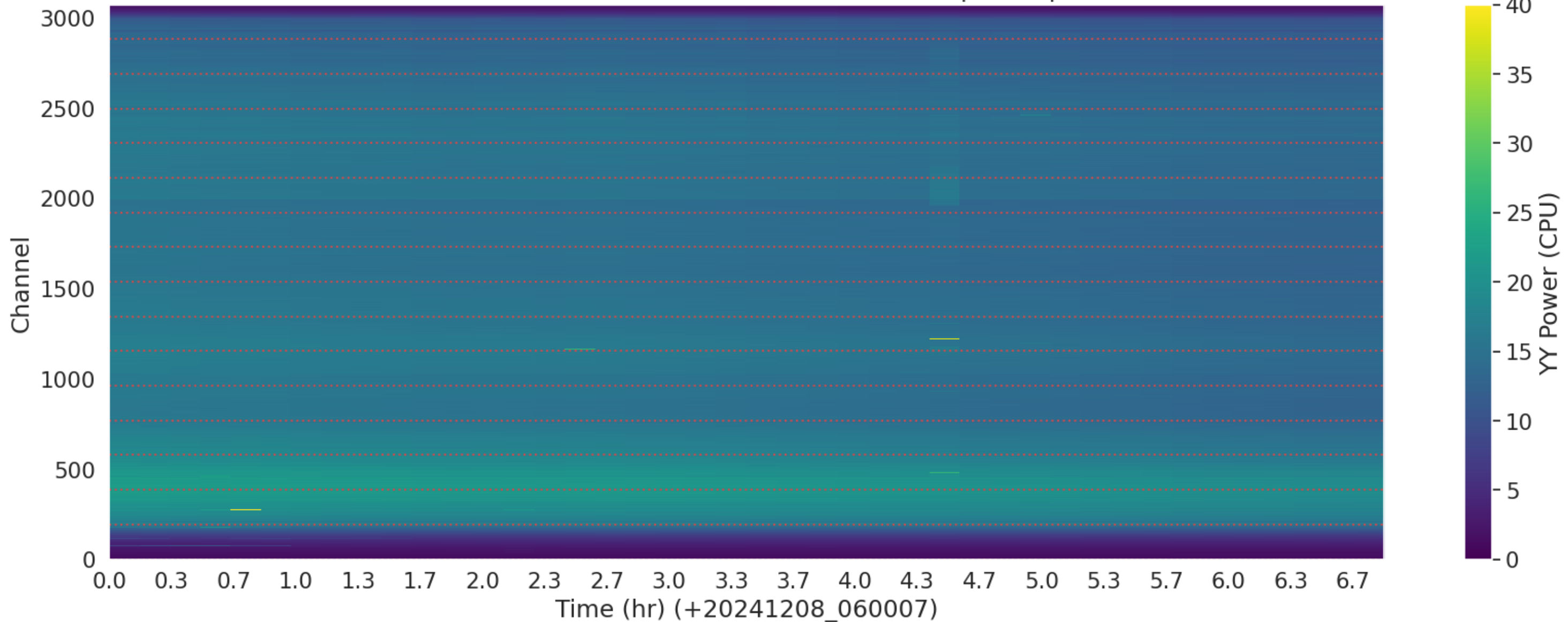
LWA347 - Correlator# 255 - YY - FLAGS: BadSpecShape
