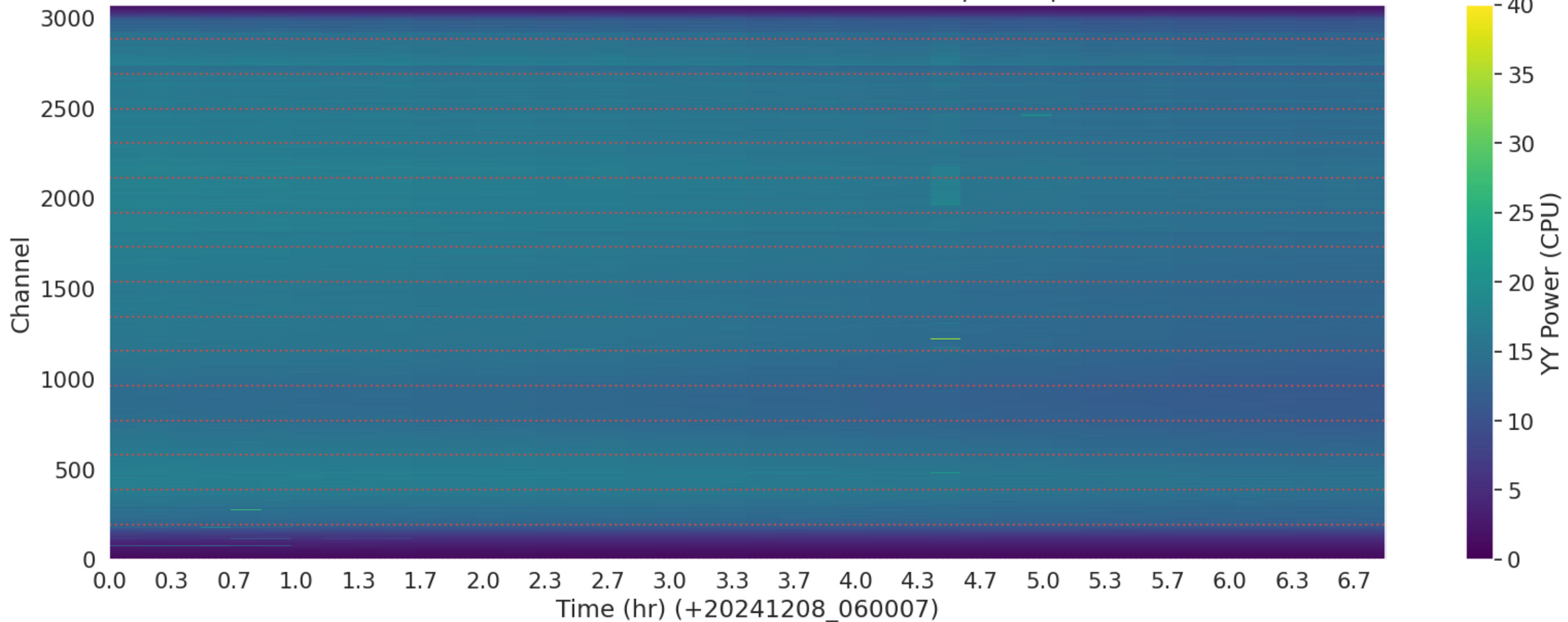
LWA070 - Correlator# 168 - YY - FLAGS: BadSpecShape
