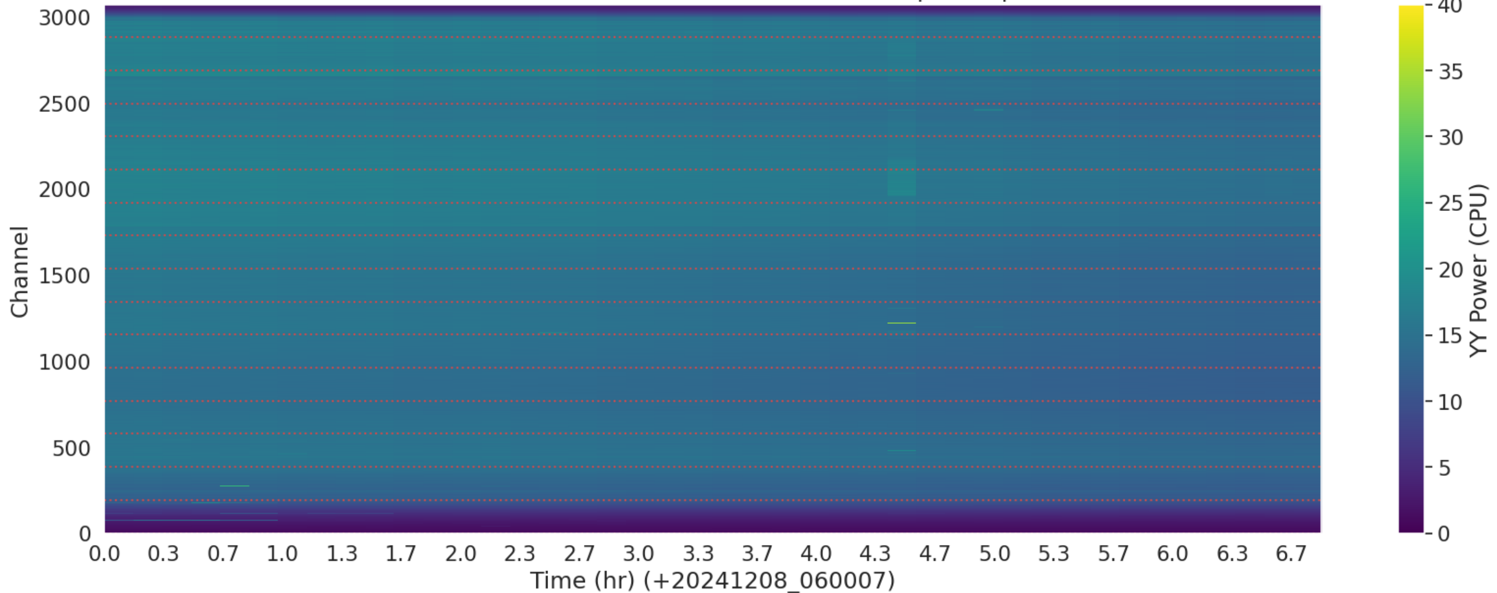
LWA002 - Correlator# 064 - YY - FLAGS: BadSpecShape
