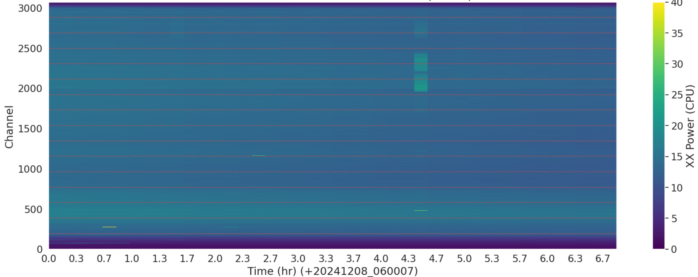
LWA342 - Correlator# 317 - XX - FLAGS: BadSpecShape
