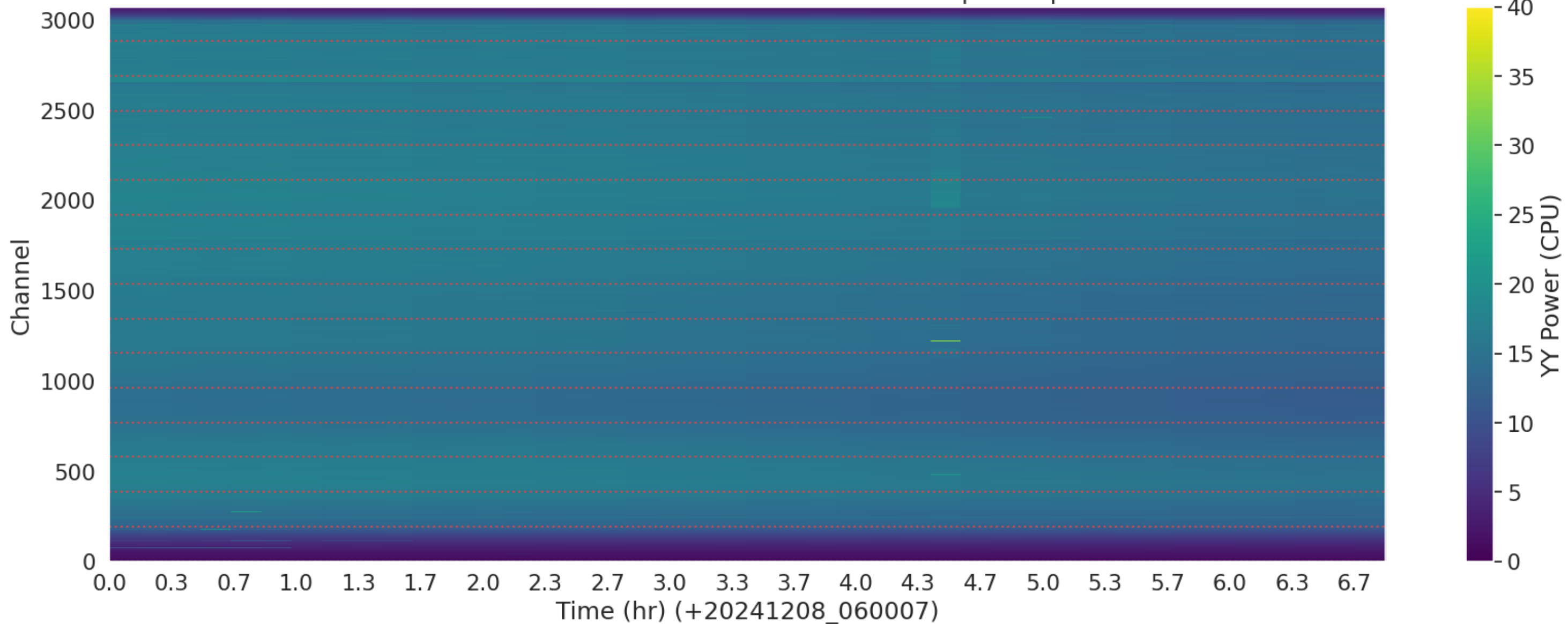
LWA097 - Correlator# 170 - YY - FLAGS: BadSpecShape
