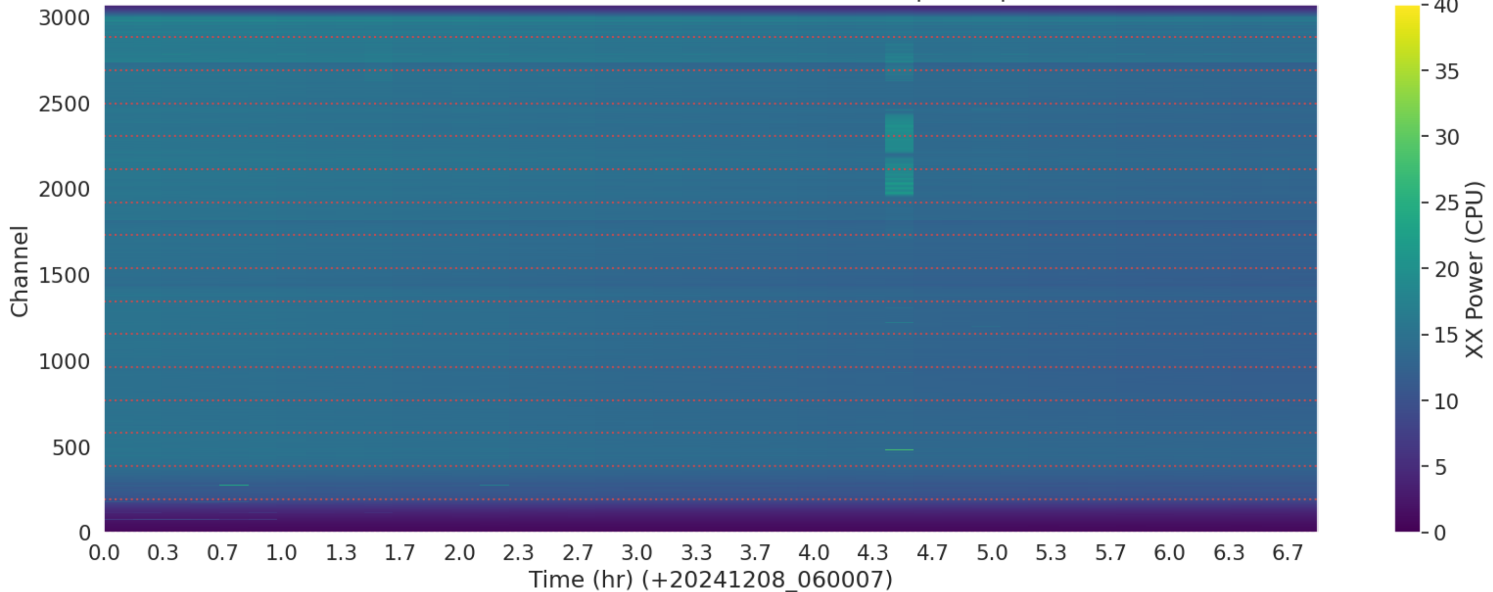
LWA041 - Correlator# 079 - XX - FLAGS: BadSpecShape
