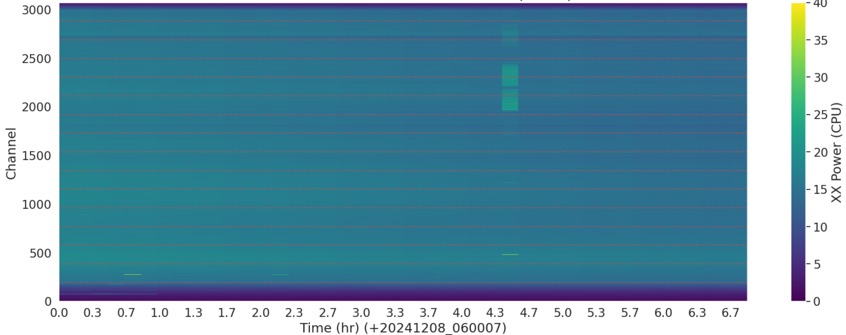
LWA227 - Correlator# 280 - XX - FLAGS: BadSpecShape
