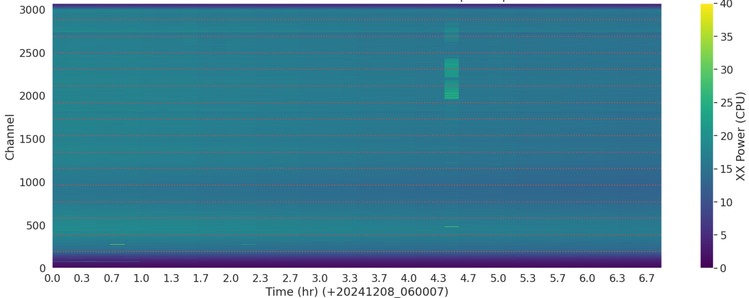
LWA133 - Correlator# 257 - XX - FLAGS: BadSpecShape
