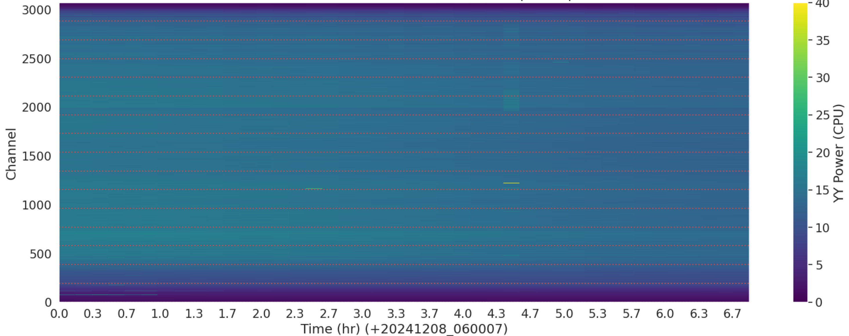
LWA340 - Correlator# 026 - YY - FLAGS: BadSpecShape
