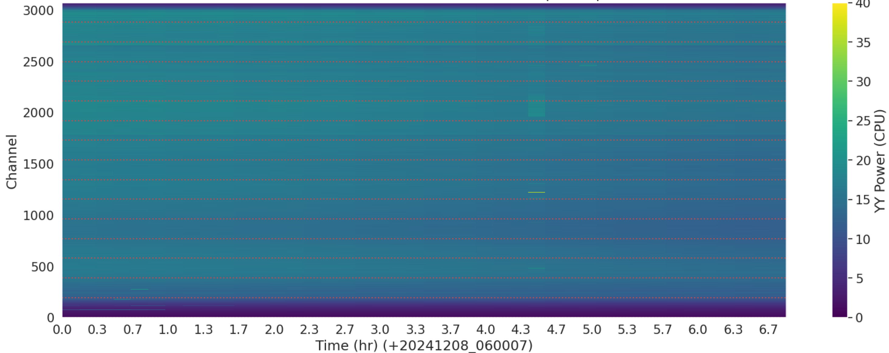
LWA066 - Correlator# 164 - YY - FLAGS: BadSpecShape
