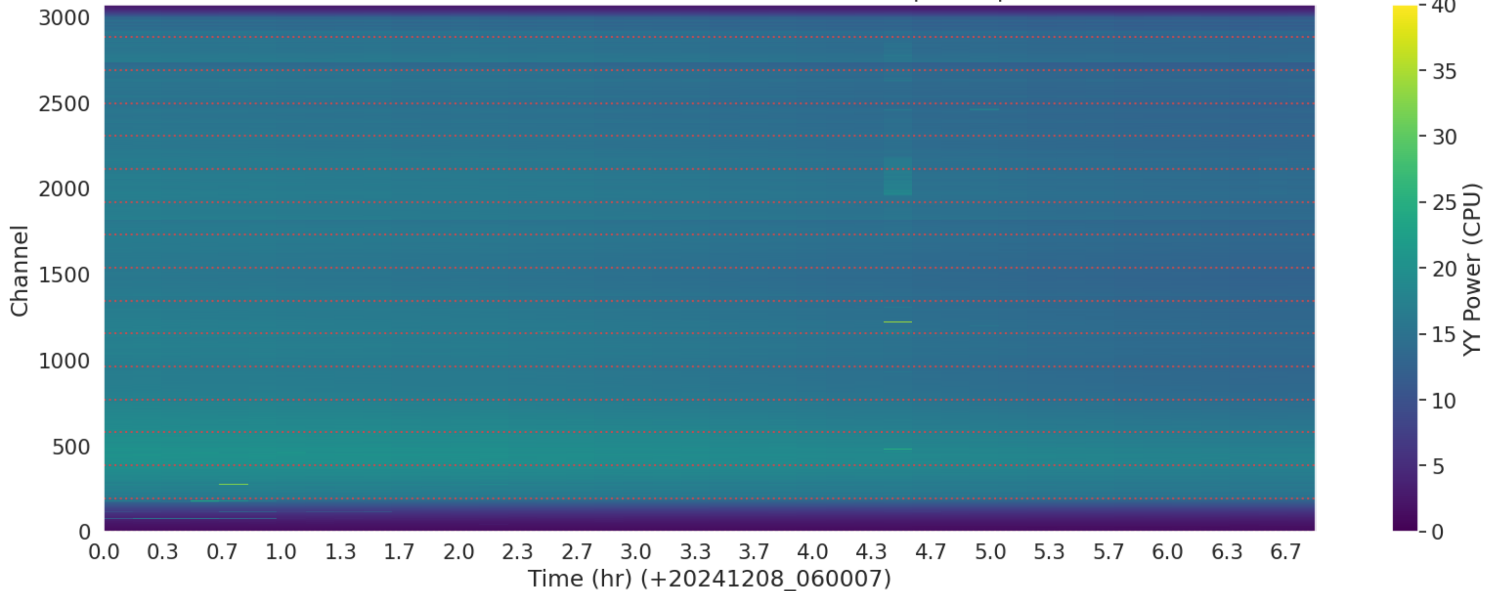
LWA038 - Correlator# 077 - YY - FLAGS: BadSpecShape
