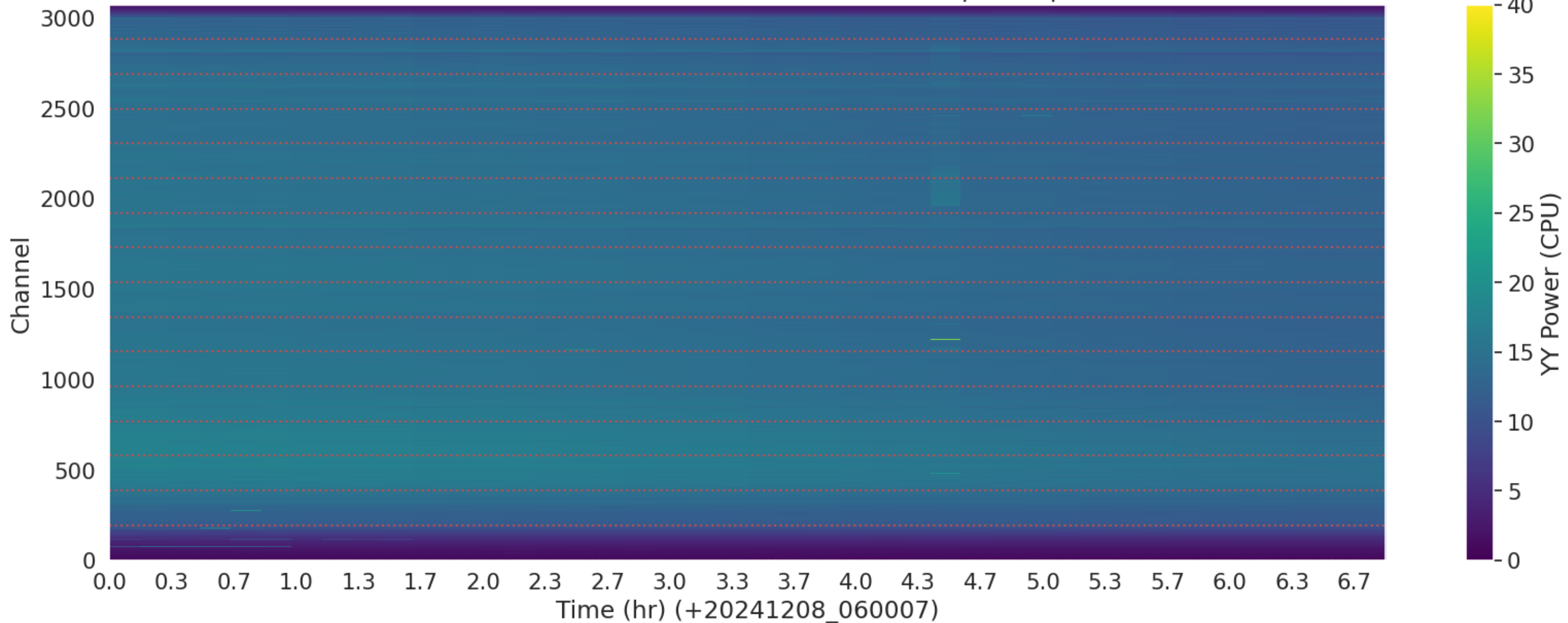
LWA014 - Correlator# 099 - YY - FLAGS: BadSpecShape
