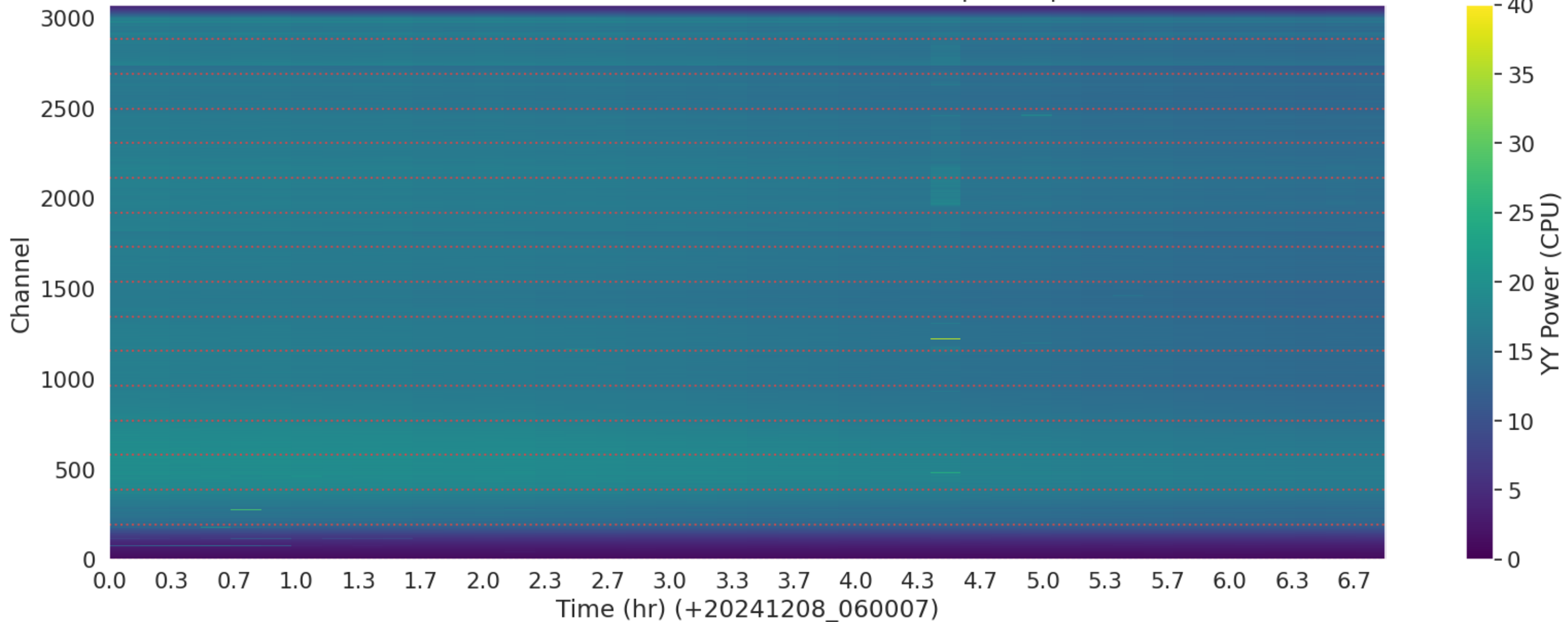
LWA067 - Correlator# 167 - YY - FLAGS: BadSpecShape
