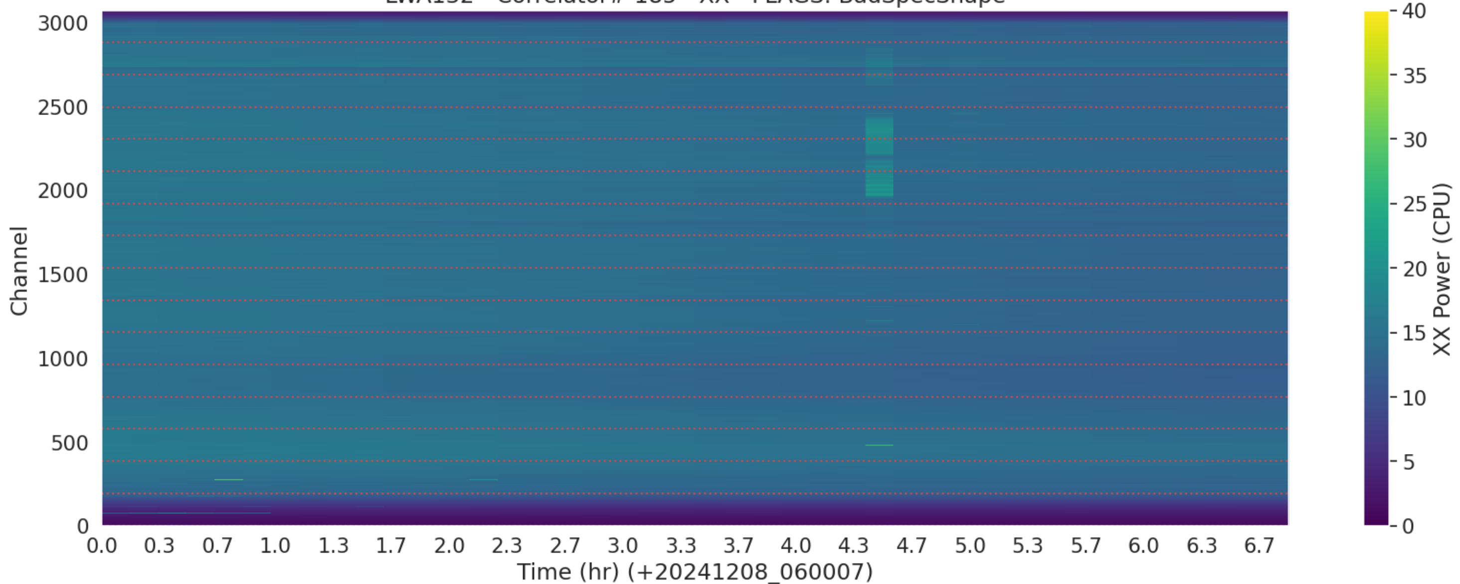
LWA132 - Correlator# 185 - XX - FLAGS: BadSpecShape
