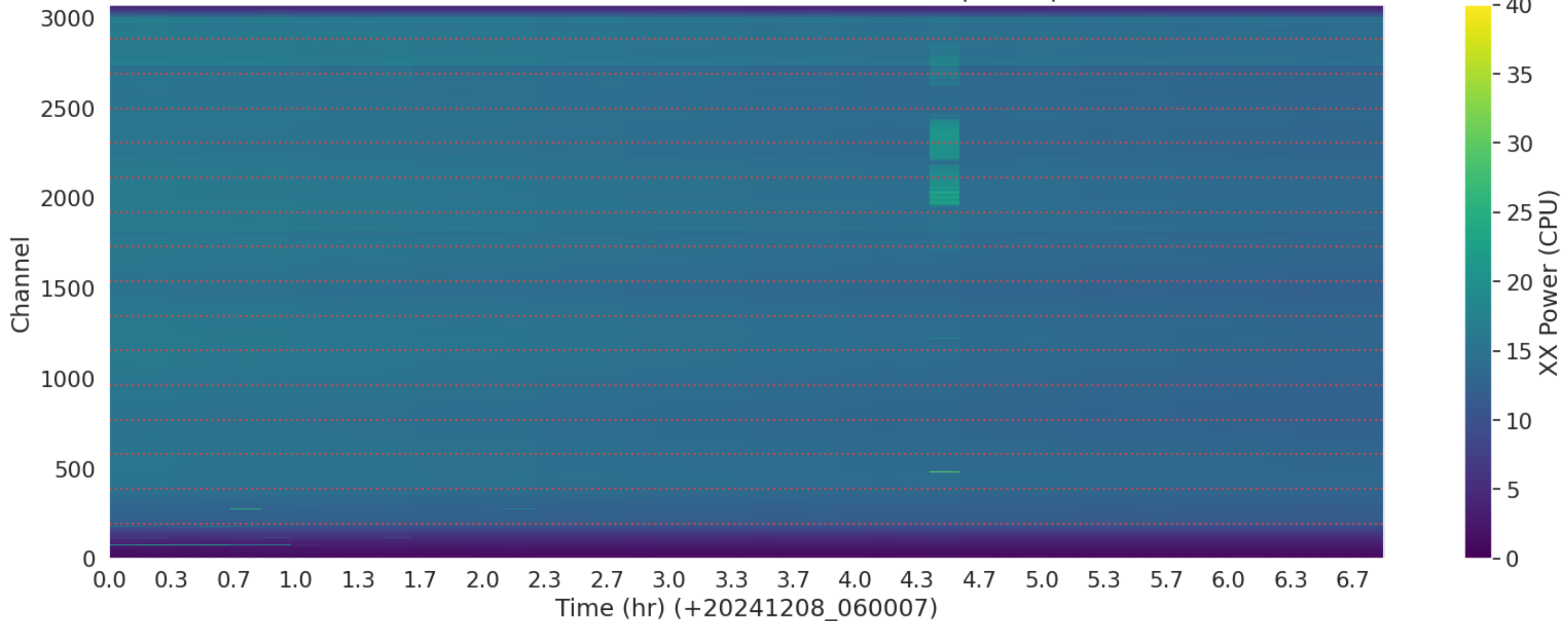
LWA008 - Correlator# 075 - XX - FLAGS: BadSpecShape
