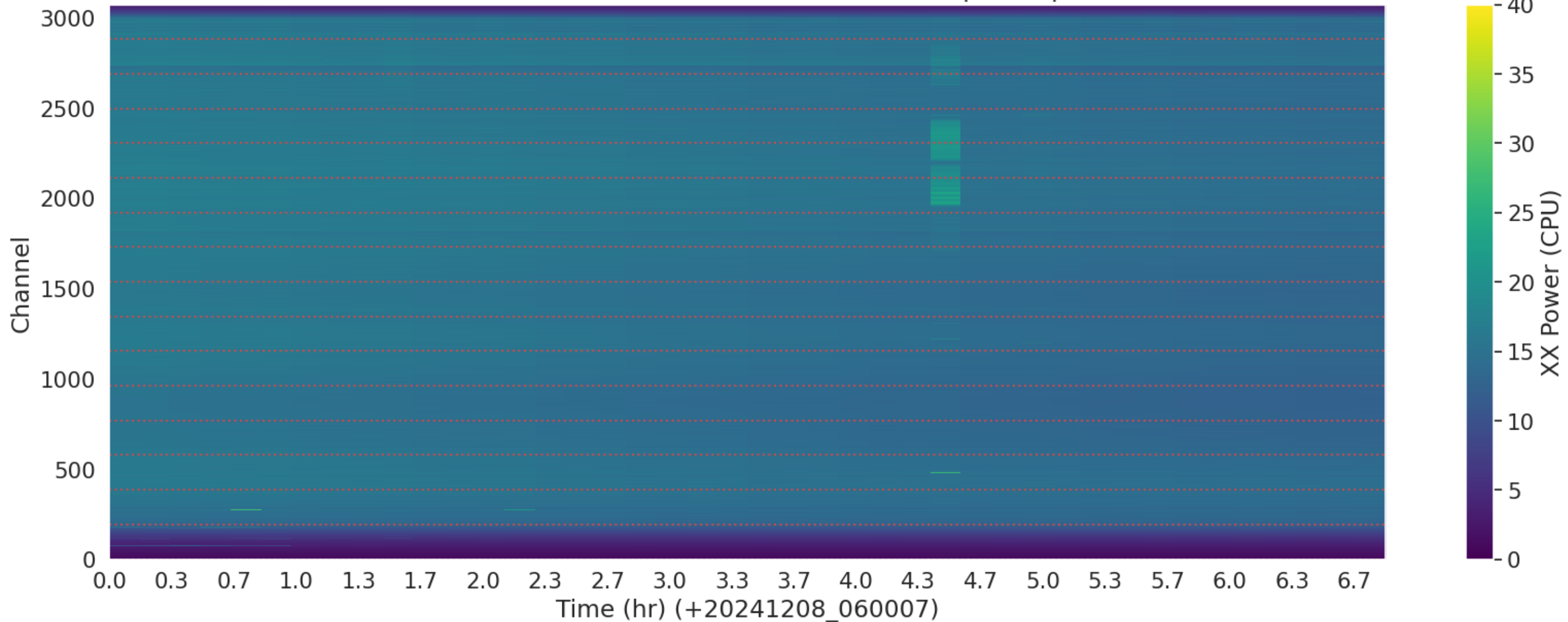
LWA098 - Correlator# 173 - XX - FLAGS: BadSpecShape
