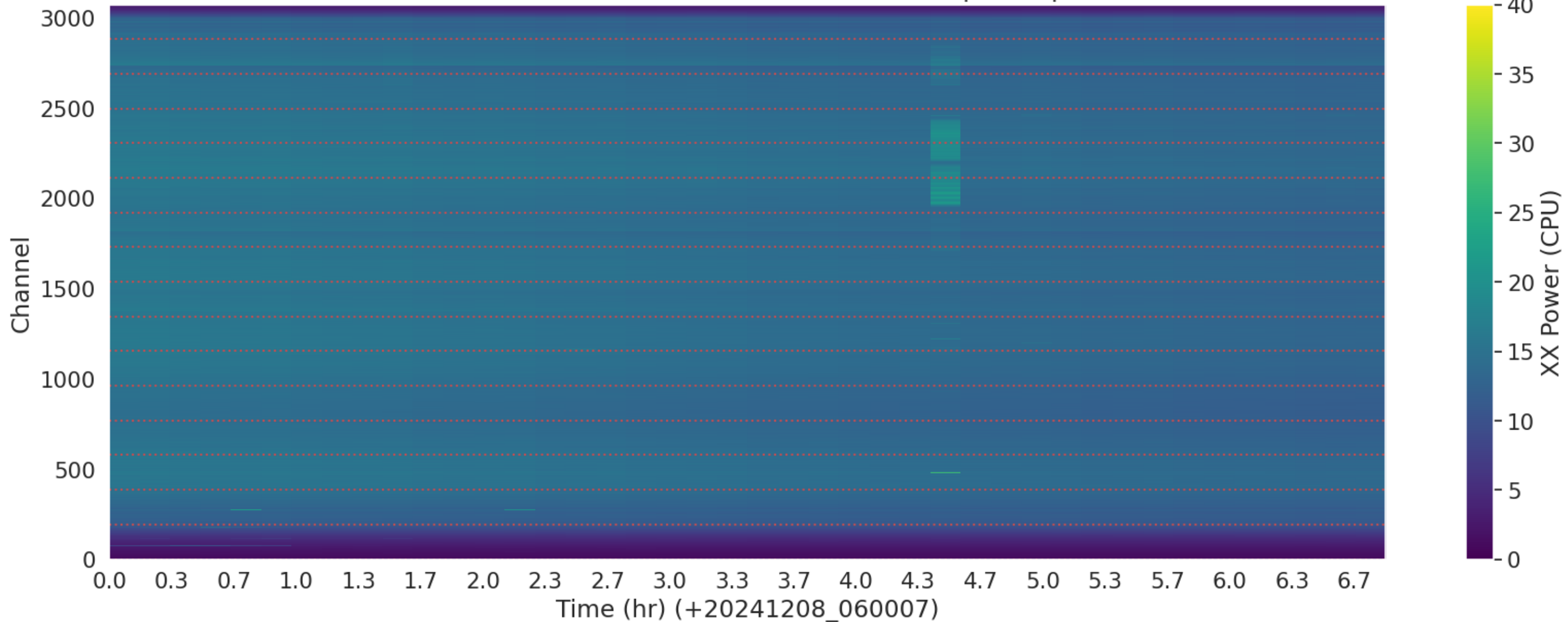
LWA253 - Correlator# 283 - XX - FLAGS: BadSpecShape
