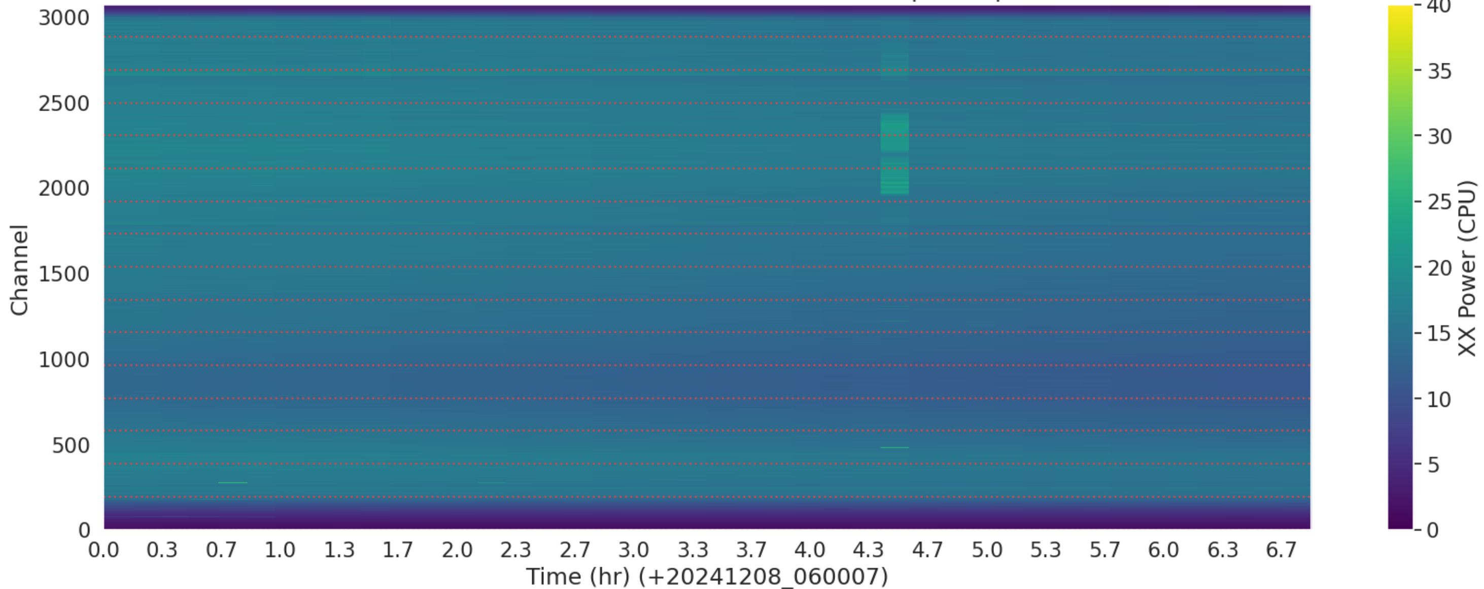
LWA129 - Correlator# 180 - XX - FLAGS: BadSpecShape
