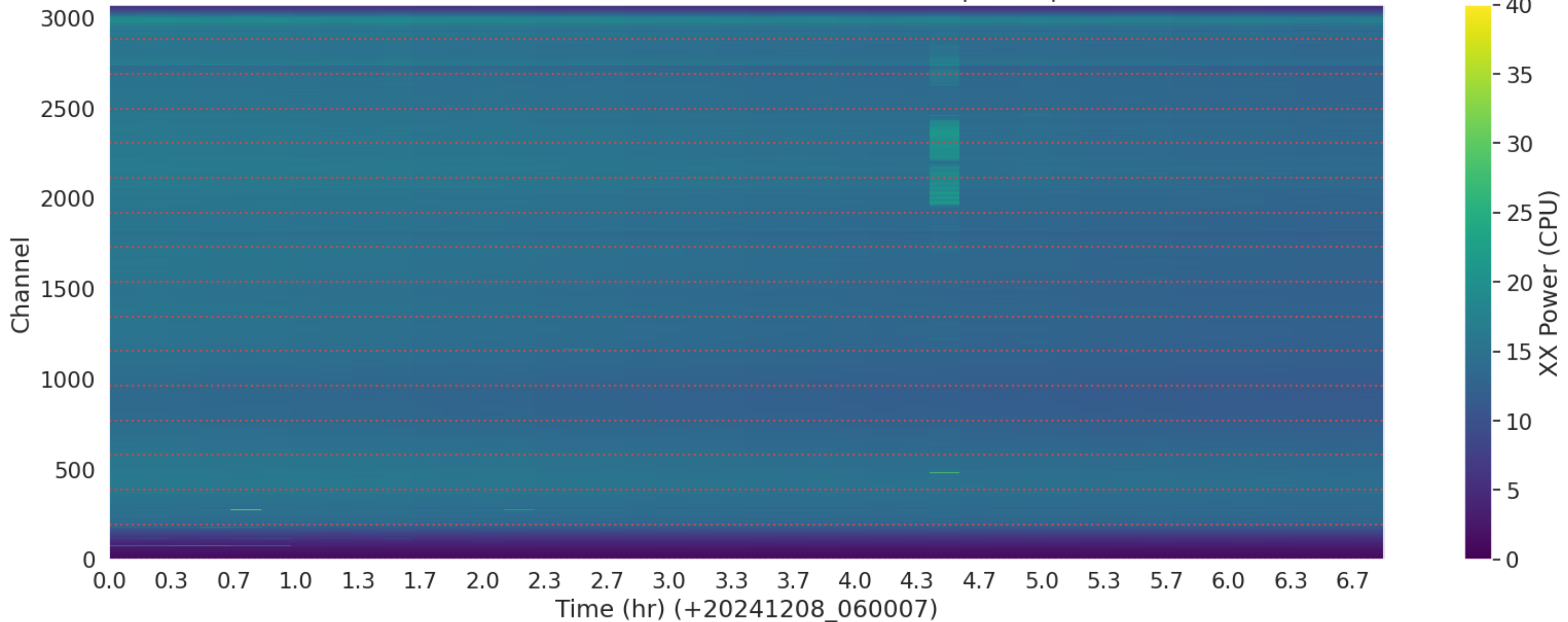
LWA163 - Correlator# 264 - XX - FLAGS: BadSpecShape
