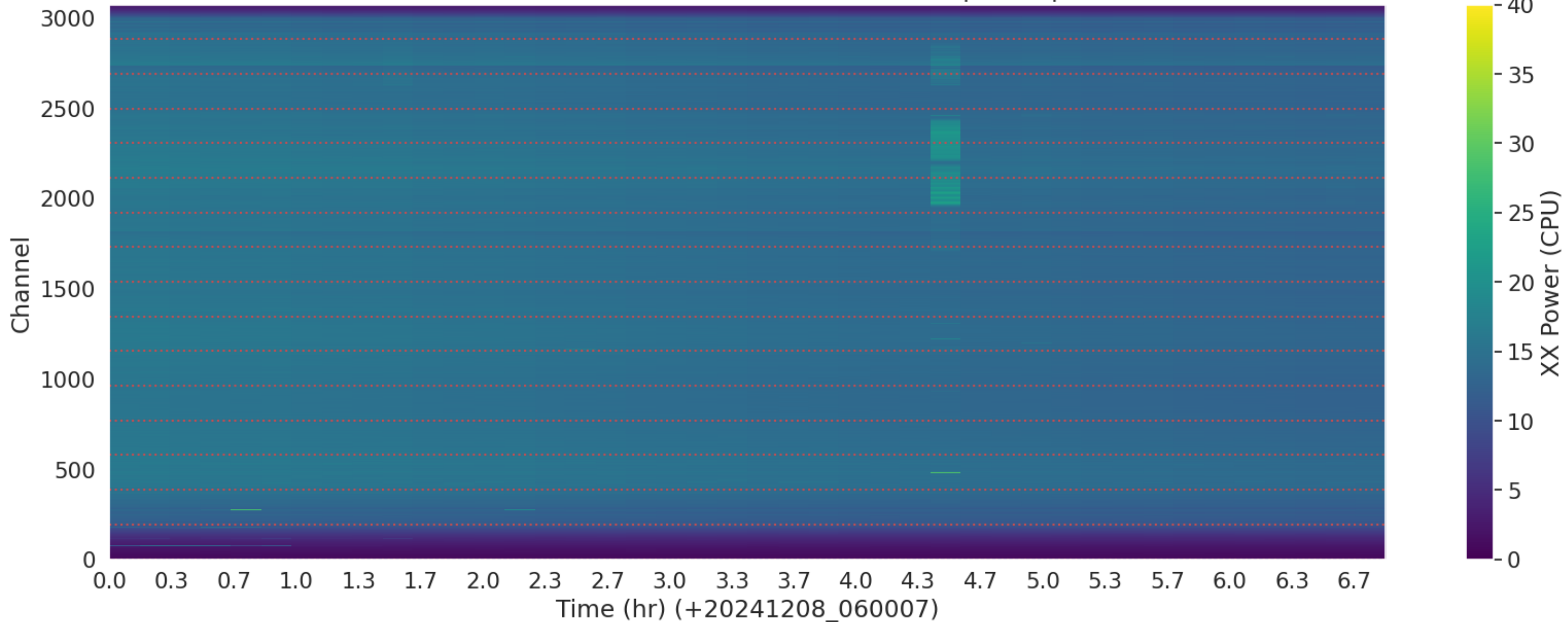
LWA037 - Correlator# 181 - XX - FLAGS: BadSpecShape
