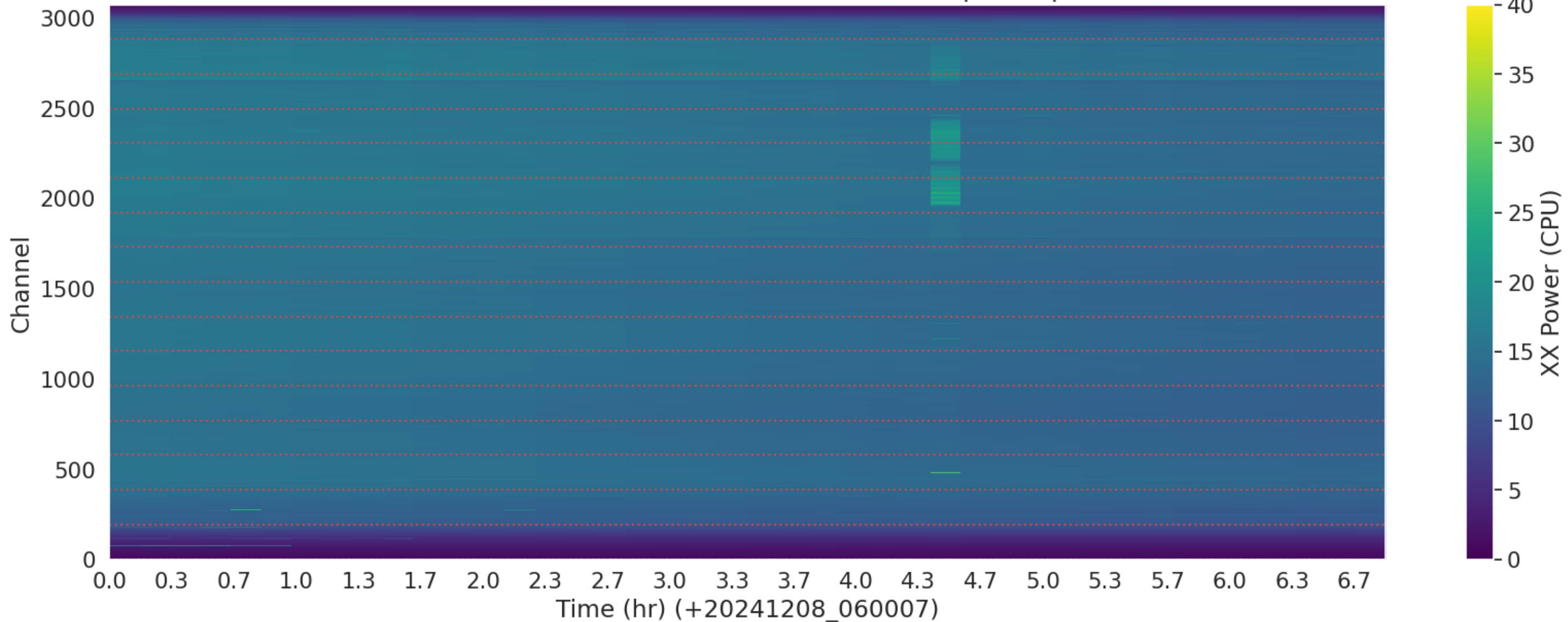
LWA034 - Correlator# 162 - XX - FLAGS: BadSpecShape
