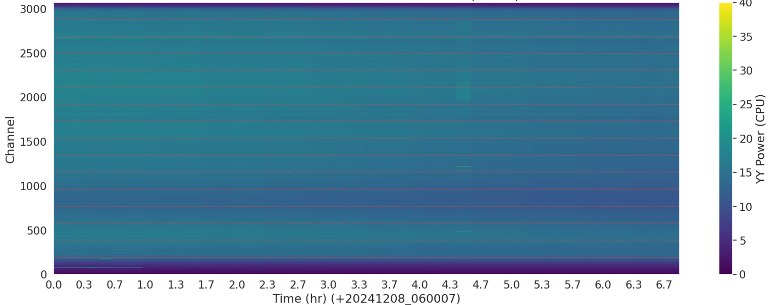
LWA195 - Correlator# 272 - YY - FLAGS: BadSpecShape
