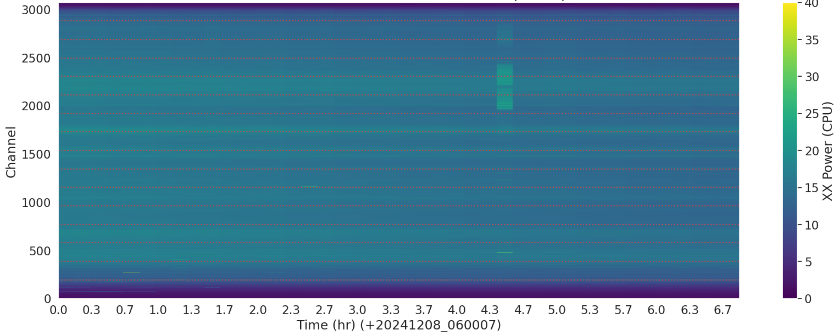
LWA336 - Correlator# 056 - XX - FLAGS: BadSpecShape
