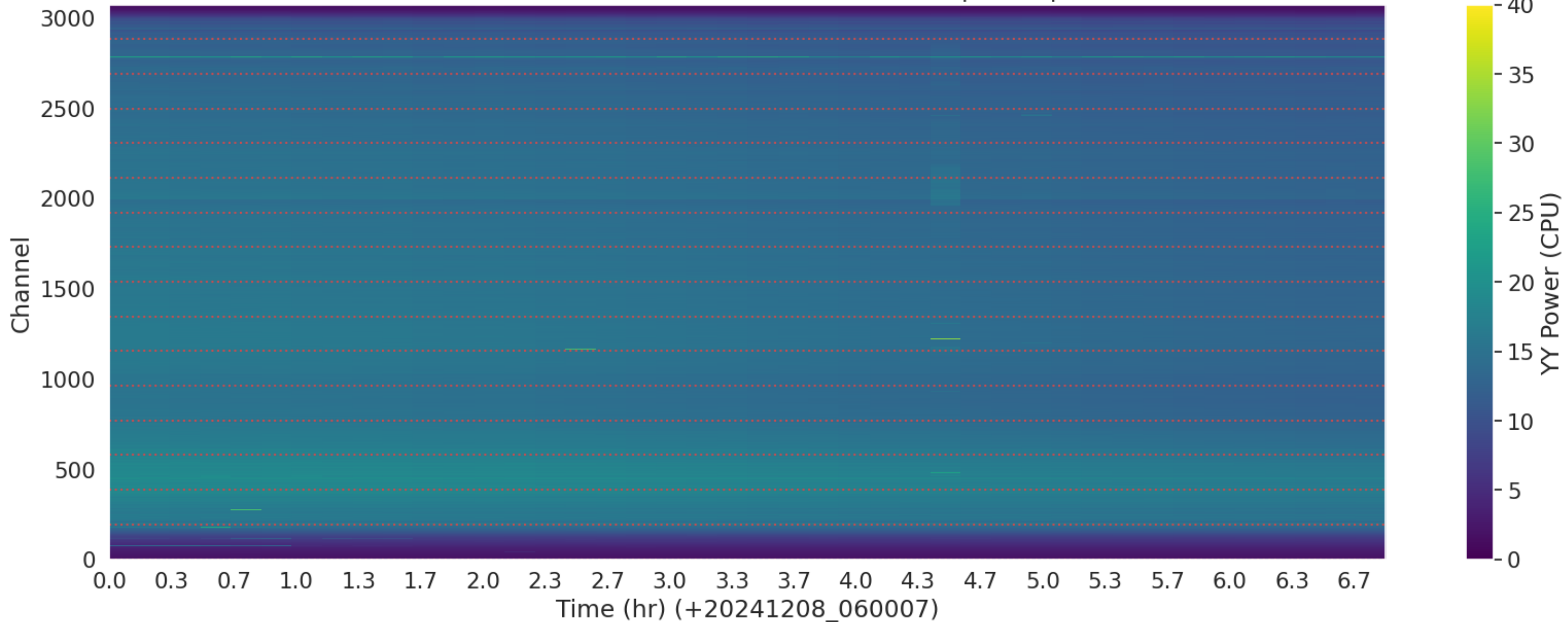
LWA125 - Correlator# 227 - YY - FLAGS: BadSpecShape
