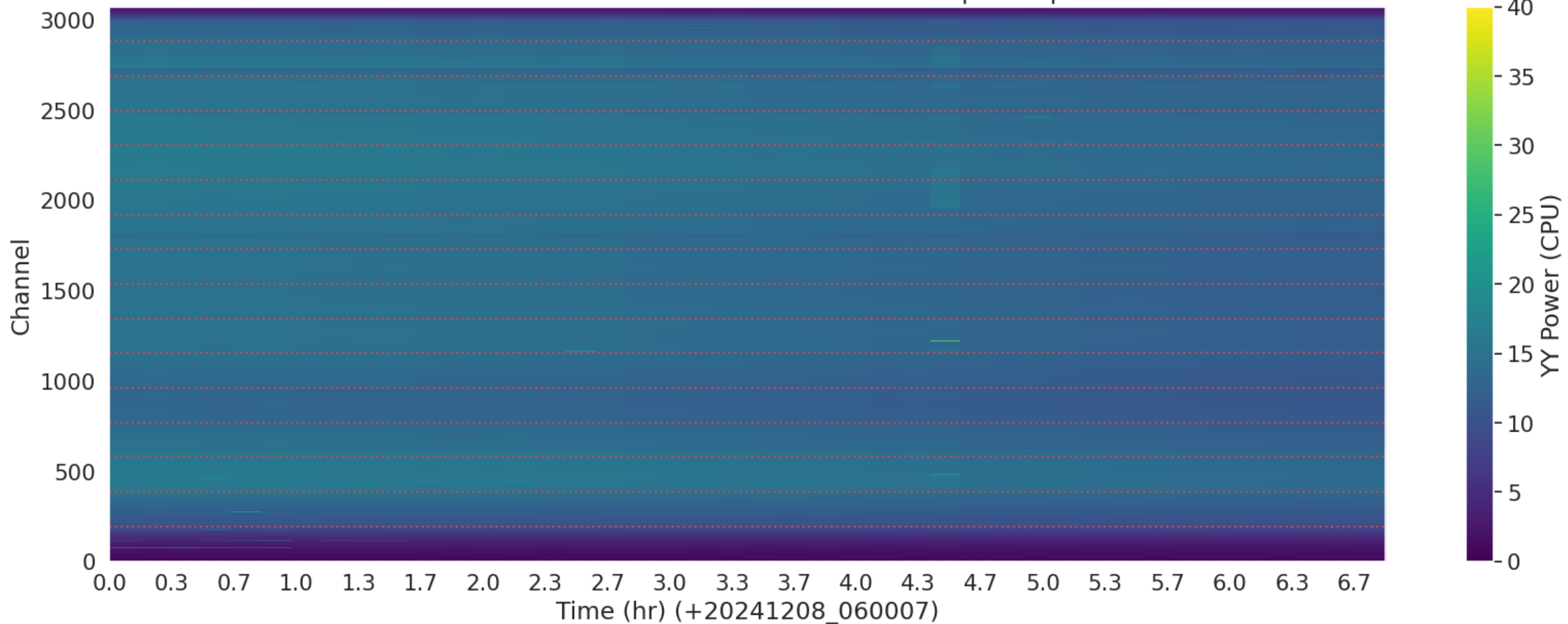
LWA232 - Correlator# 307 - YY - FLAGS: BadSpecShape
