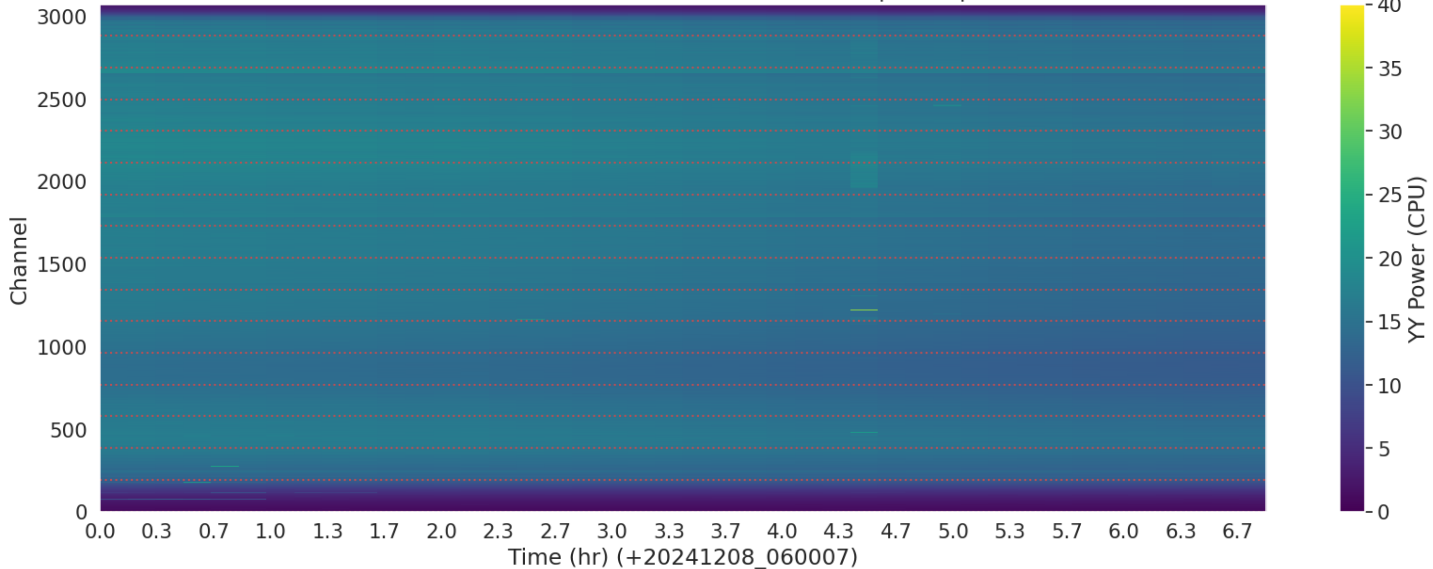
LWA130 - Correlator# 183 - YY - FLAGS: BadSpecShape
