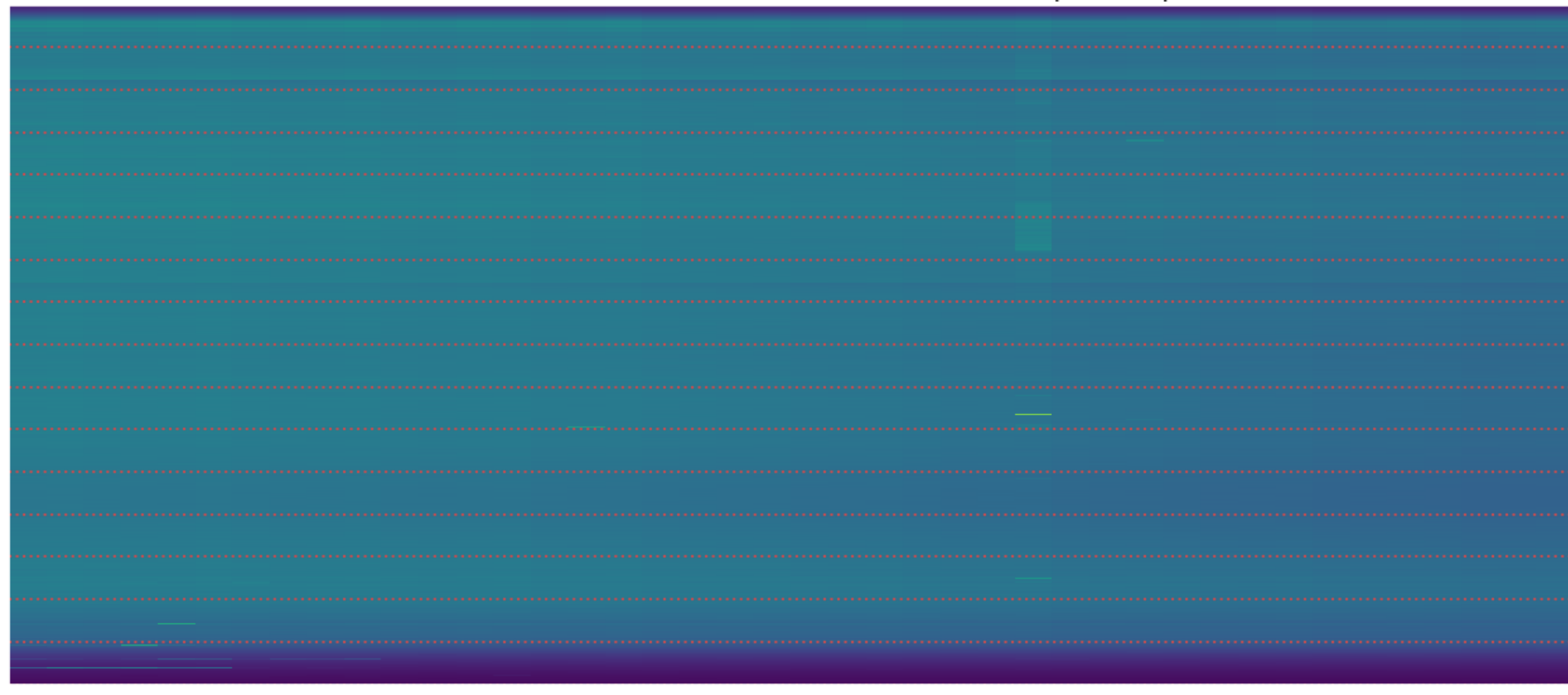
LWA009 - Correlator# 070 - YY - FLAGS: BadSpecShape
