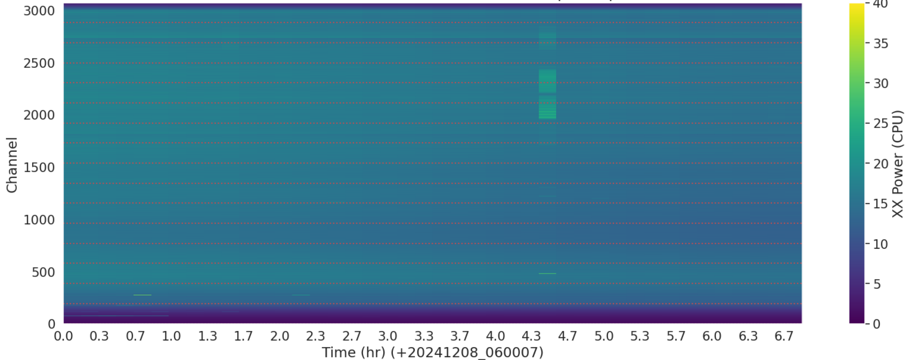
LWA137 - Correlator# 258 - XX - FLAGS: BadSpecShape
