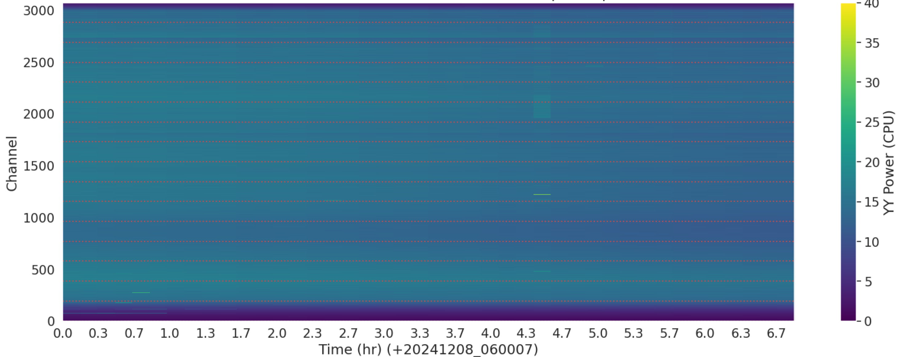
LWA199 - Correlator# 277 - YY - FLAGS: BadSpecShape
