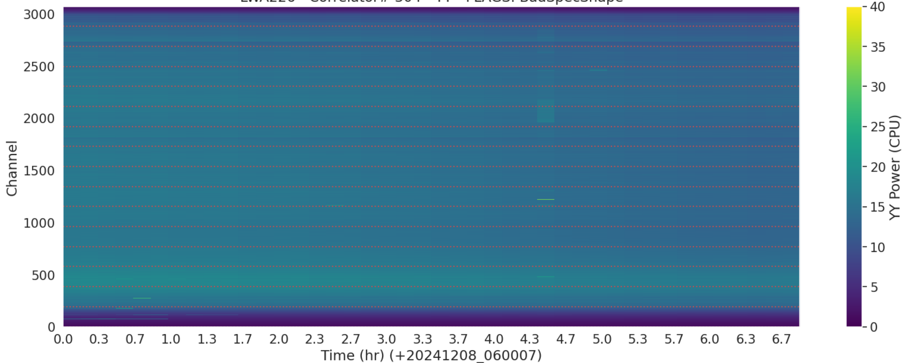
LWA226 - Correlator# 304 - YY - FLAGS: BadSpecShape
