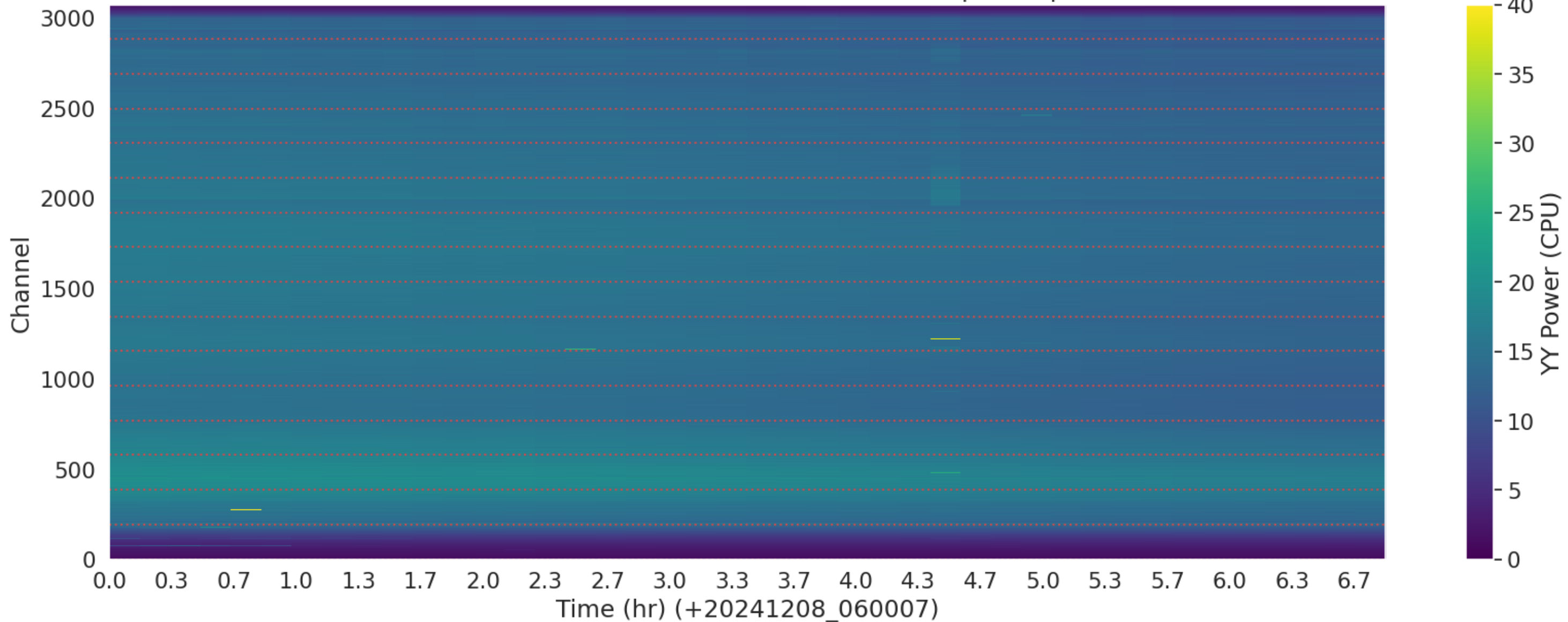
LWA258 - Correlator# 035 - YY - FLAGS: BadSpecShape
