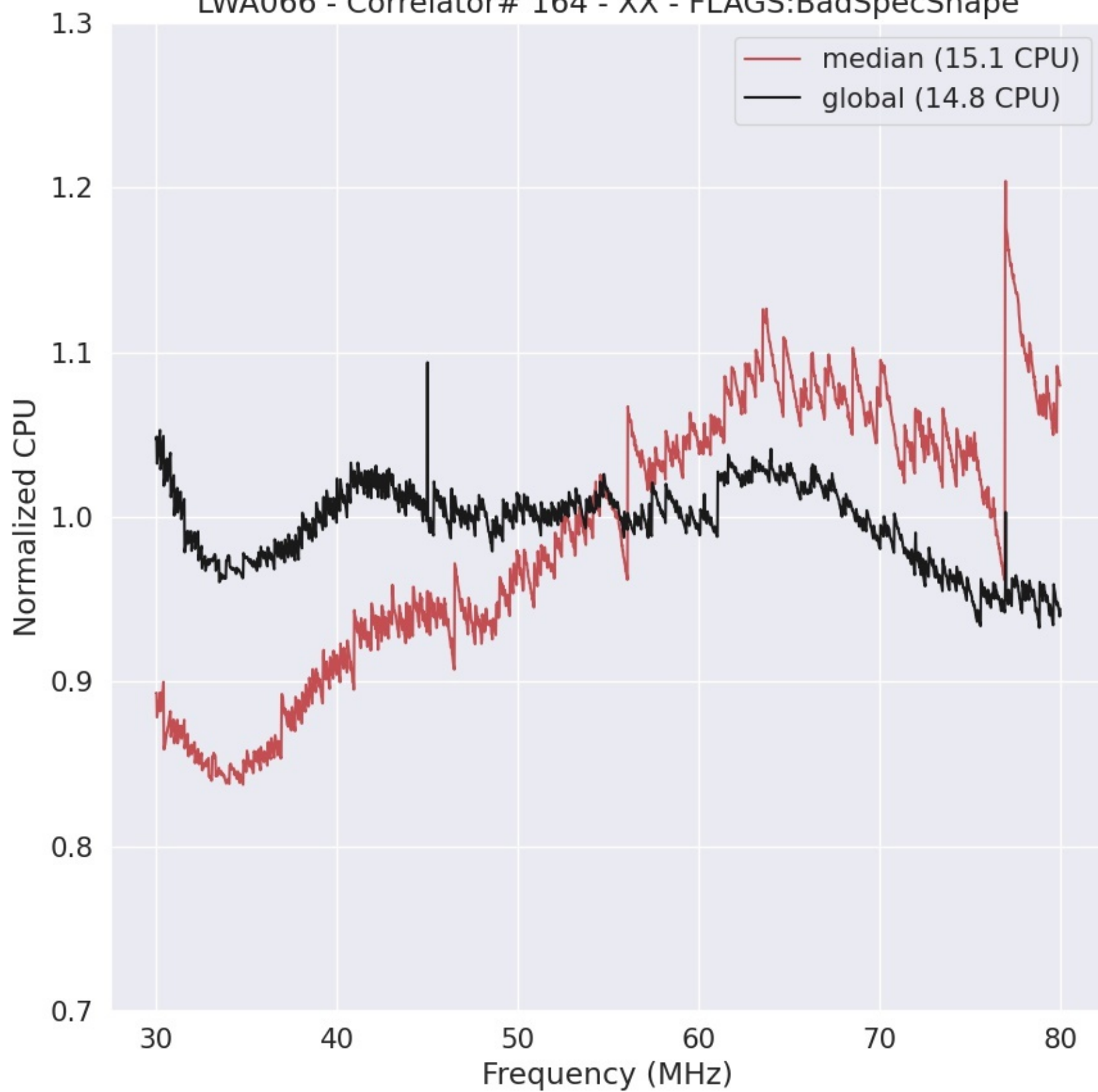
LWA066 - Correlator# 164 - XX - FLAGS:BadSpecShape
