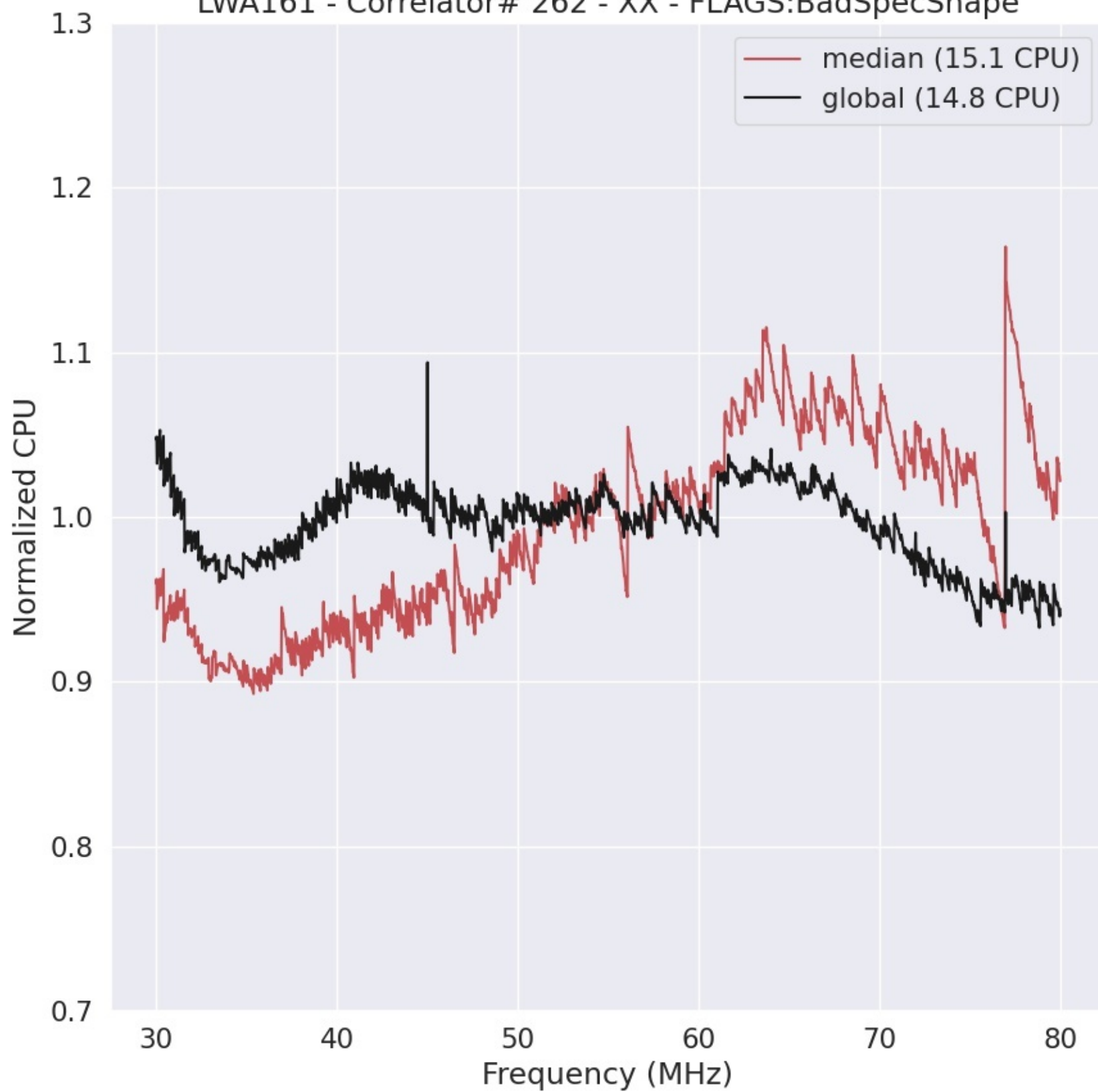
LWA161 - Correlator# 262 - XX - FLAGS:BadSpecShape
