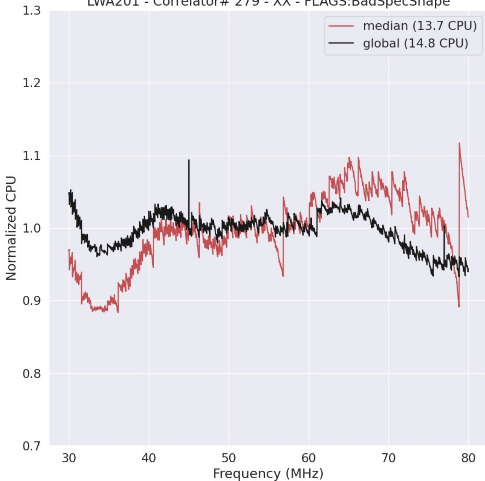
LWA201 - Correlator# 279 - XX - FLAGS:BadSpecShape
