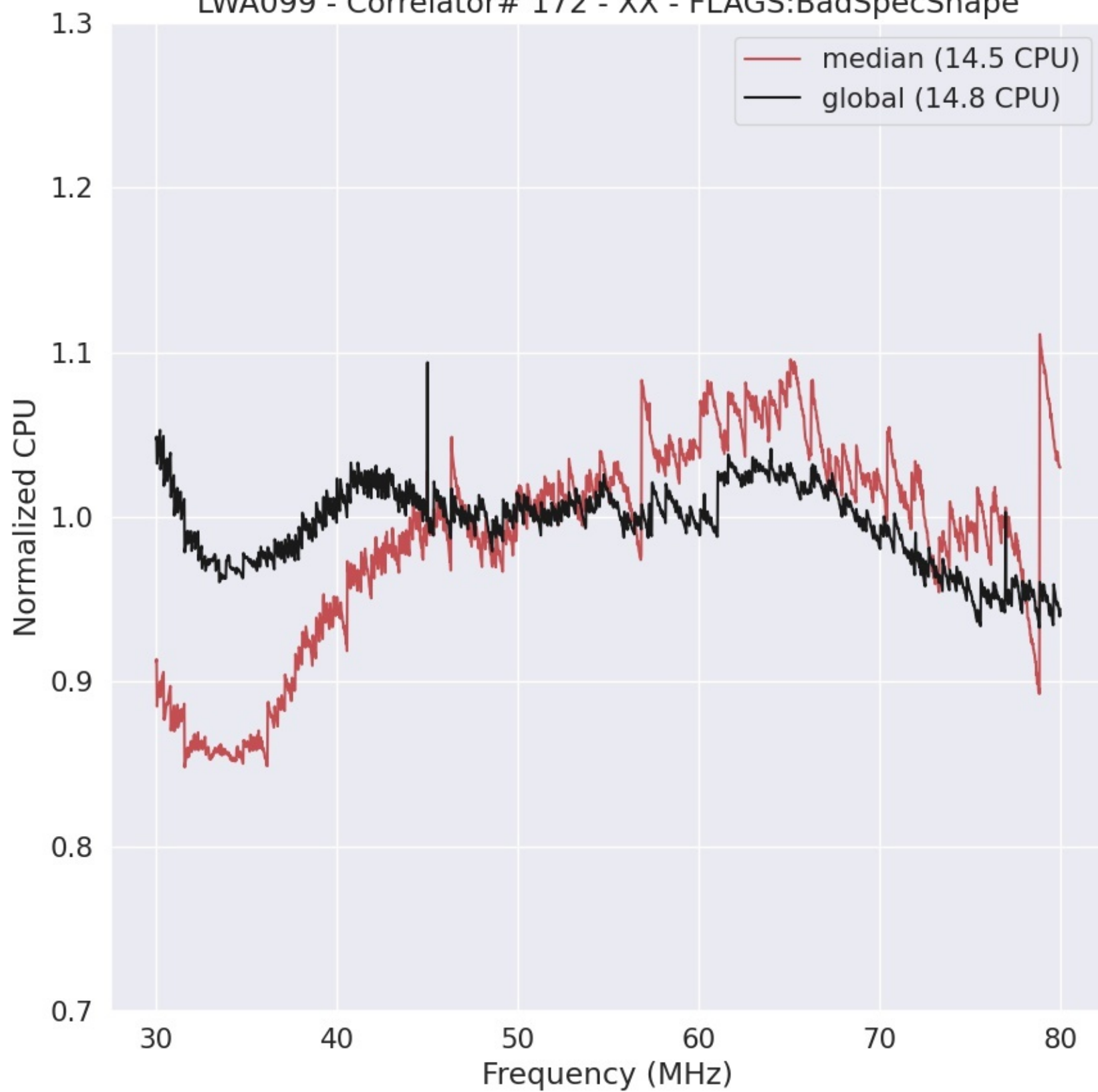
LWA099 - Correlator# 172 - XX - FLAGS:BadSpecShape
