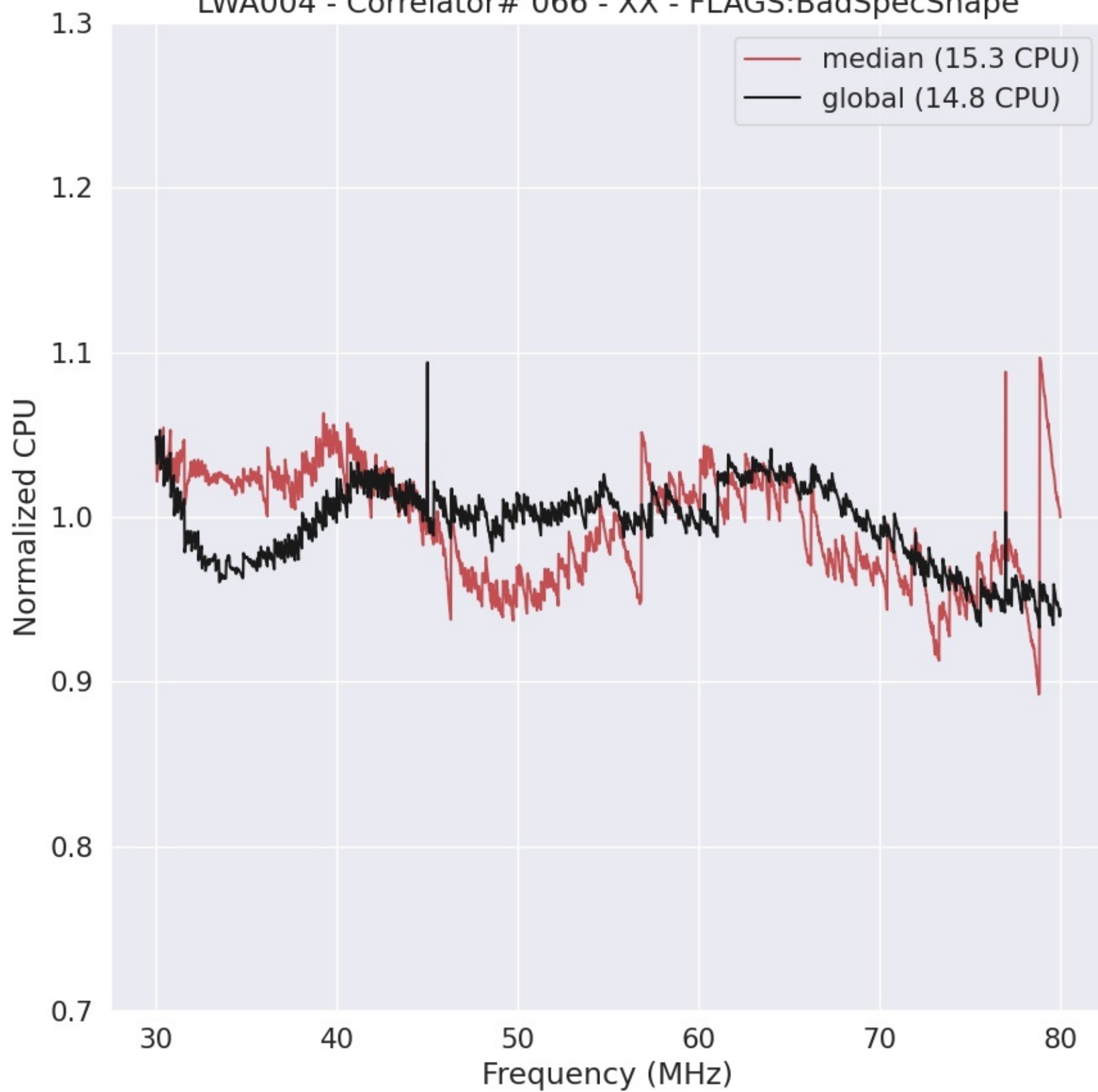
LWA004 - Correlator# 066 - XX - FLAGS:BadSpecShape
