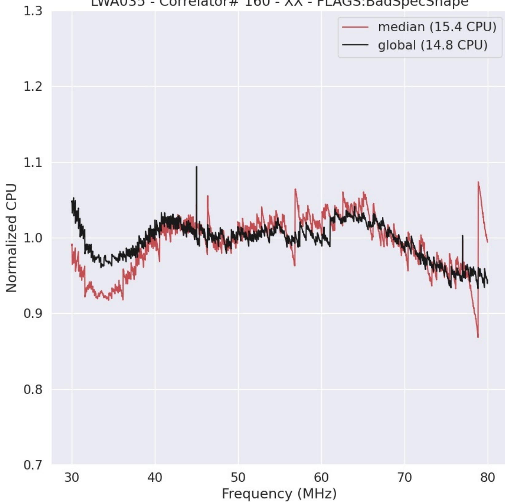
LWA035 - Correlator# 160 - XX - FLAGS:BadSpecShape
