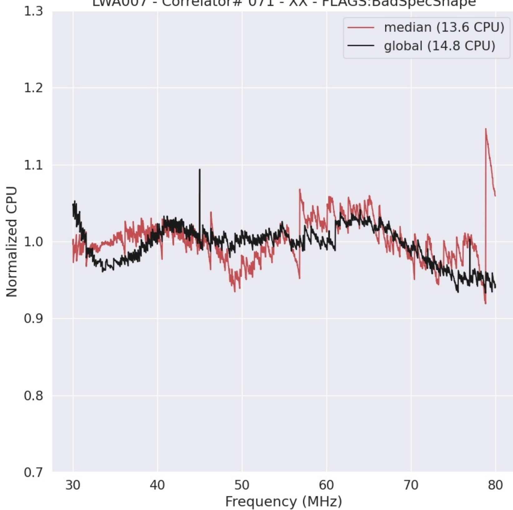
LWA007 - Correlator# 071 - XX - FLAGS:BadSpecShape
