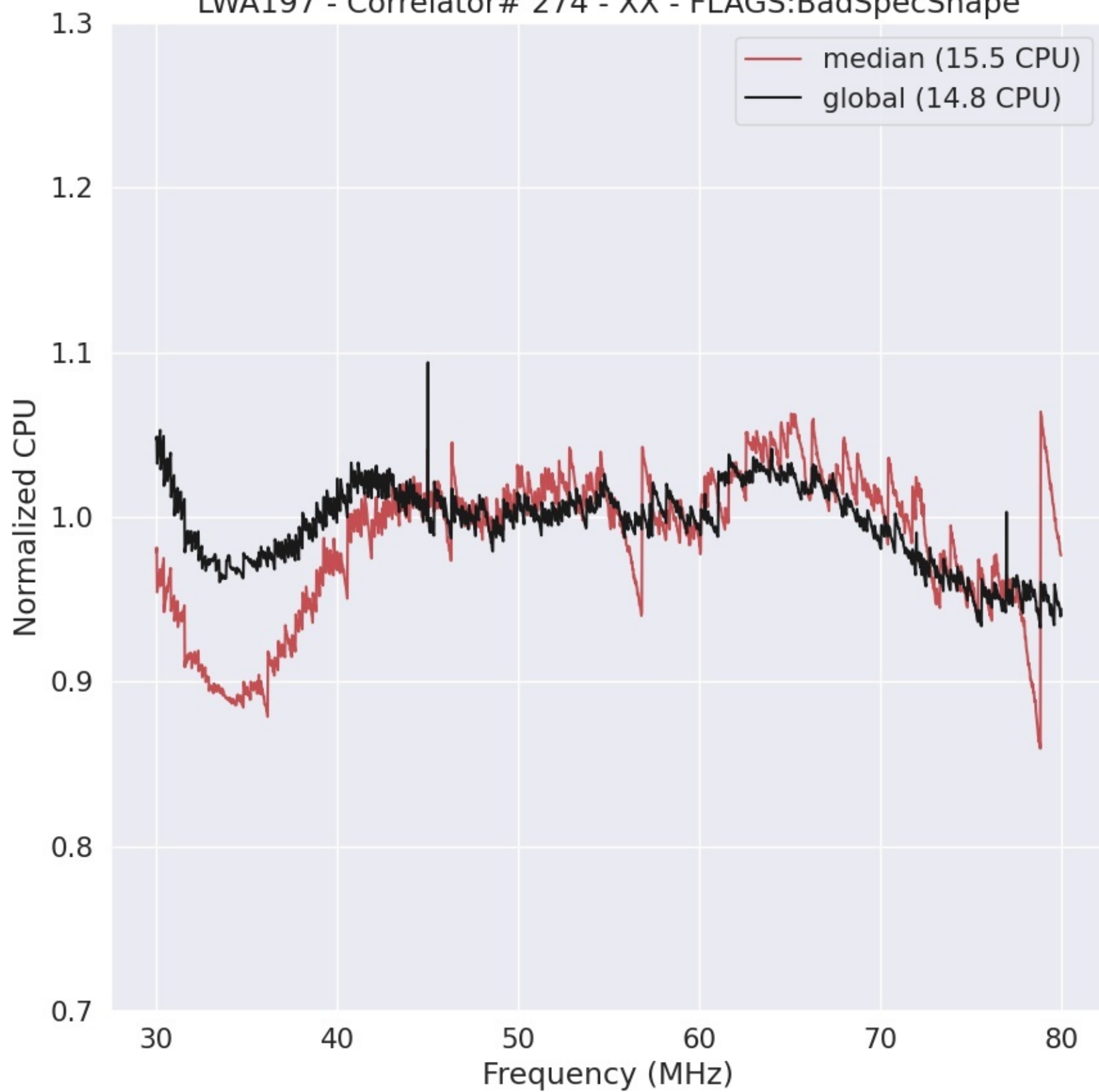
LWA197 - Correlator# 274 - XX - FLAGS:BadSpecShape
