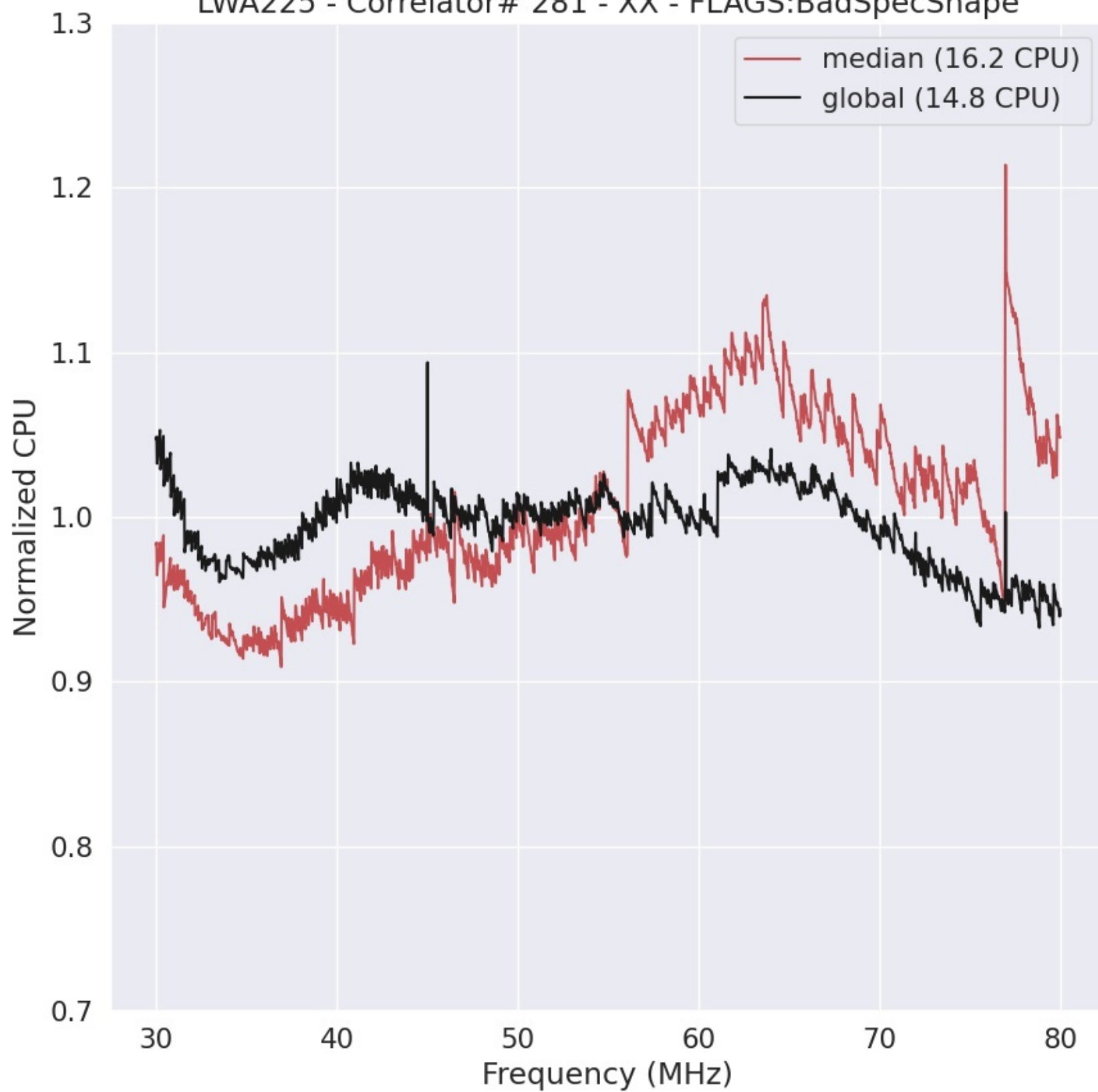
LWA225 - Correlator# 281 - XX - FLAGS:BadSpecShape
