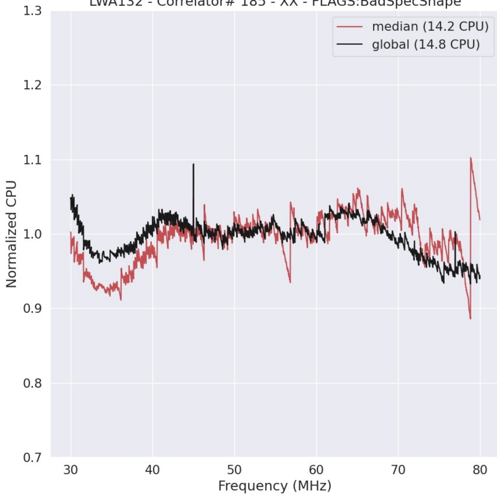
LWA132 - Correlator# 185 - XX - FLAGS:BadSpecShape
