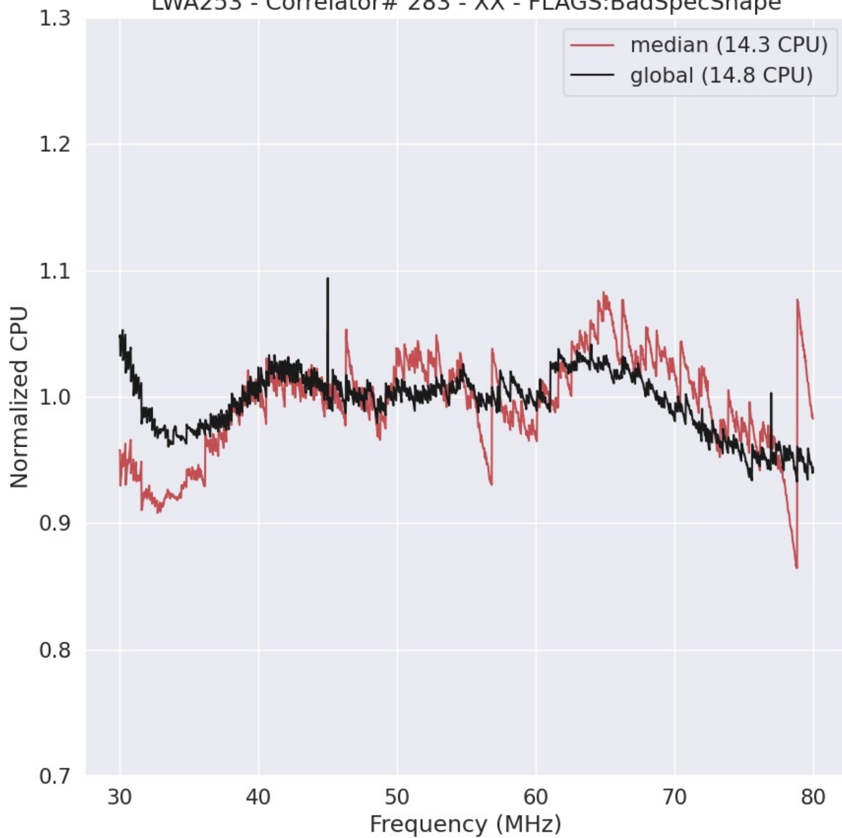
LWA253 - Correlator# 283 - XX - FLAGS:BadSpecShape
