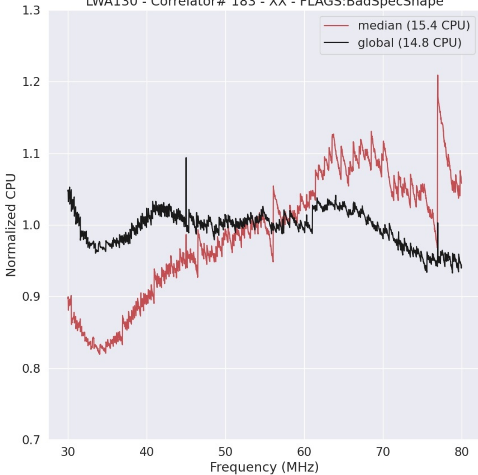
LWA130 - Correlator# 183 - XX - FLAGS:BadSpecShape
