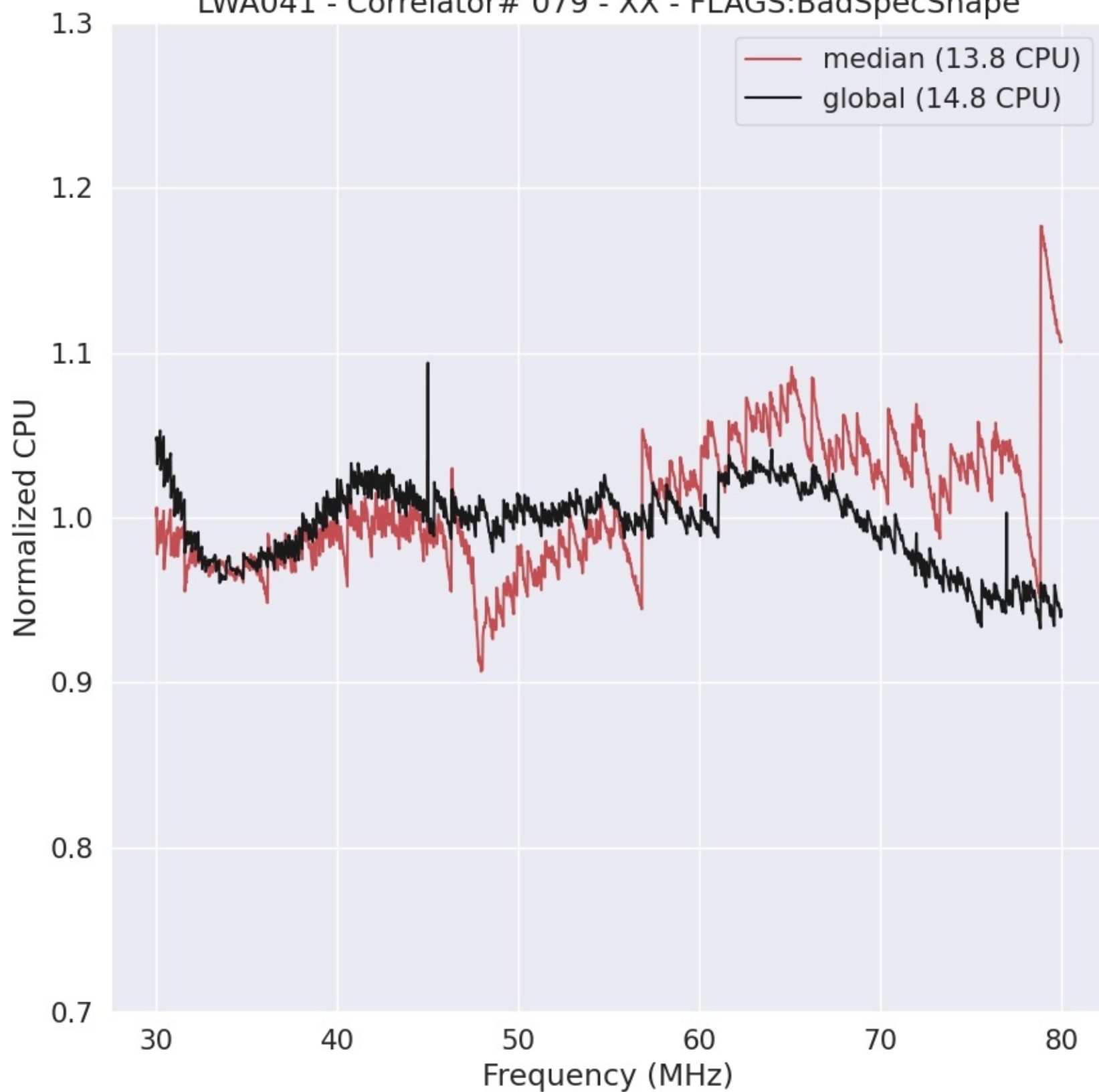
LWA041 - Correlator# 079 - XX - FLAGS:BadSpecShape
