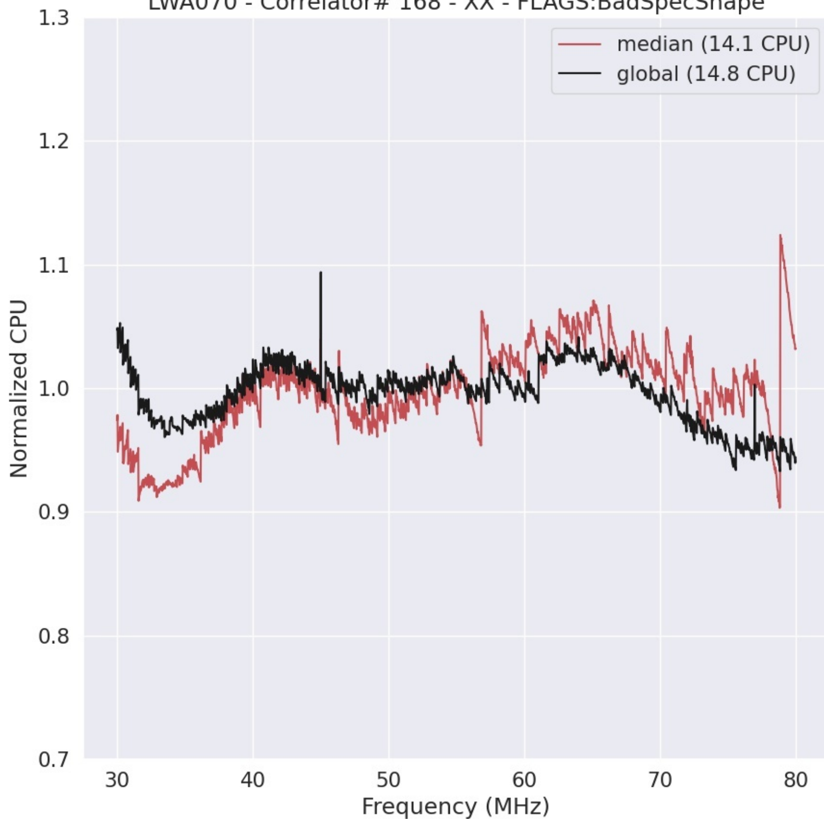
LWA070 - Correlator# 168 - XX - FLAGS:BadSpecShape
