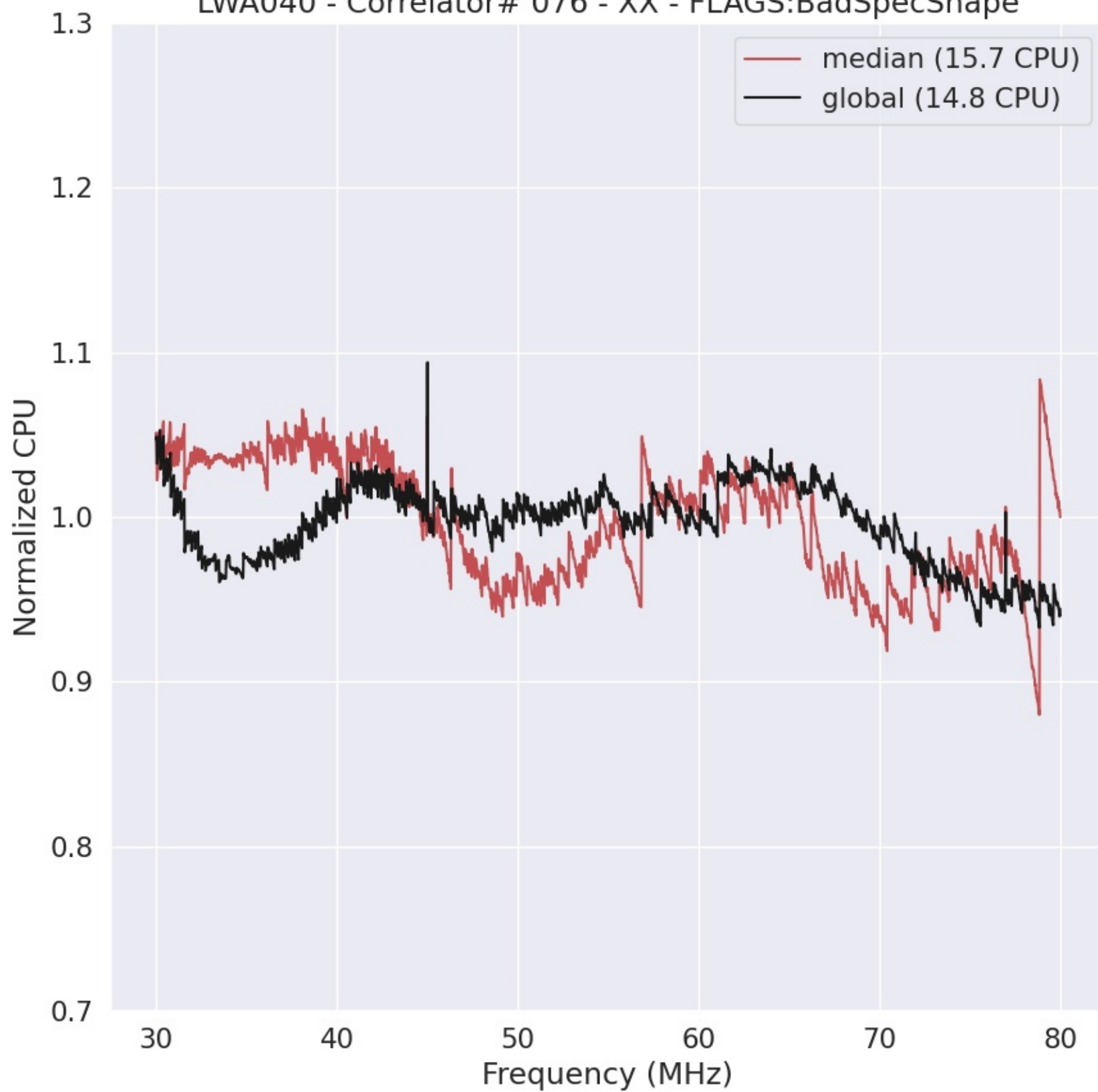
LWA040 - Correlator# 076 - XX - FLAGS:BadSpecShape
