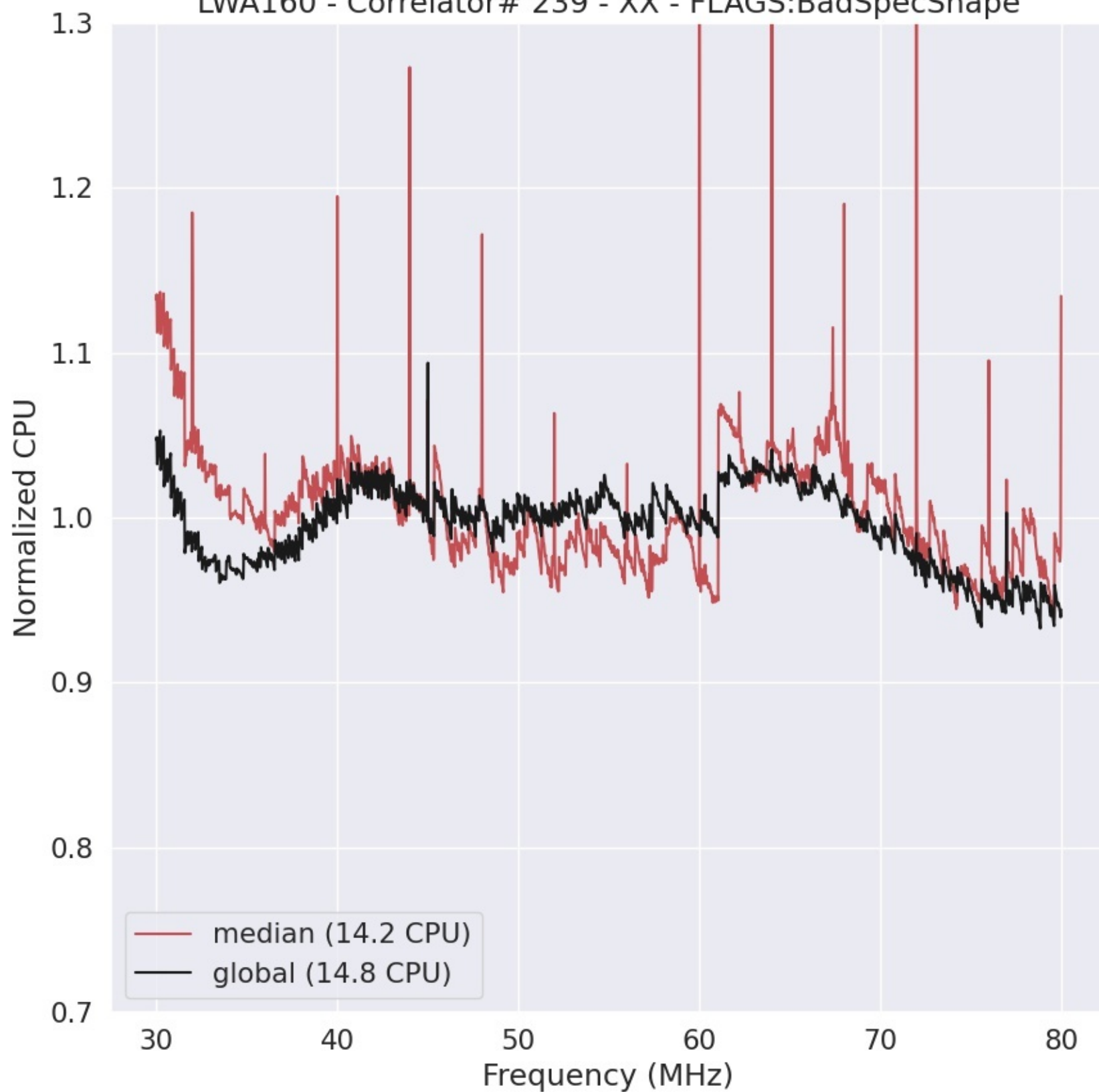
LWA160 - Correlator# 239 - XX - FLAGS:BadSpecShape
