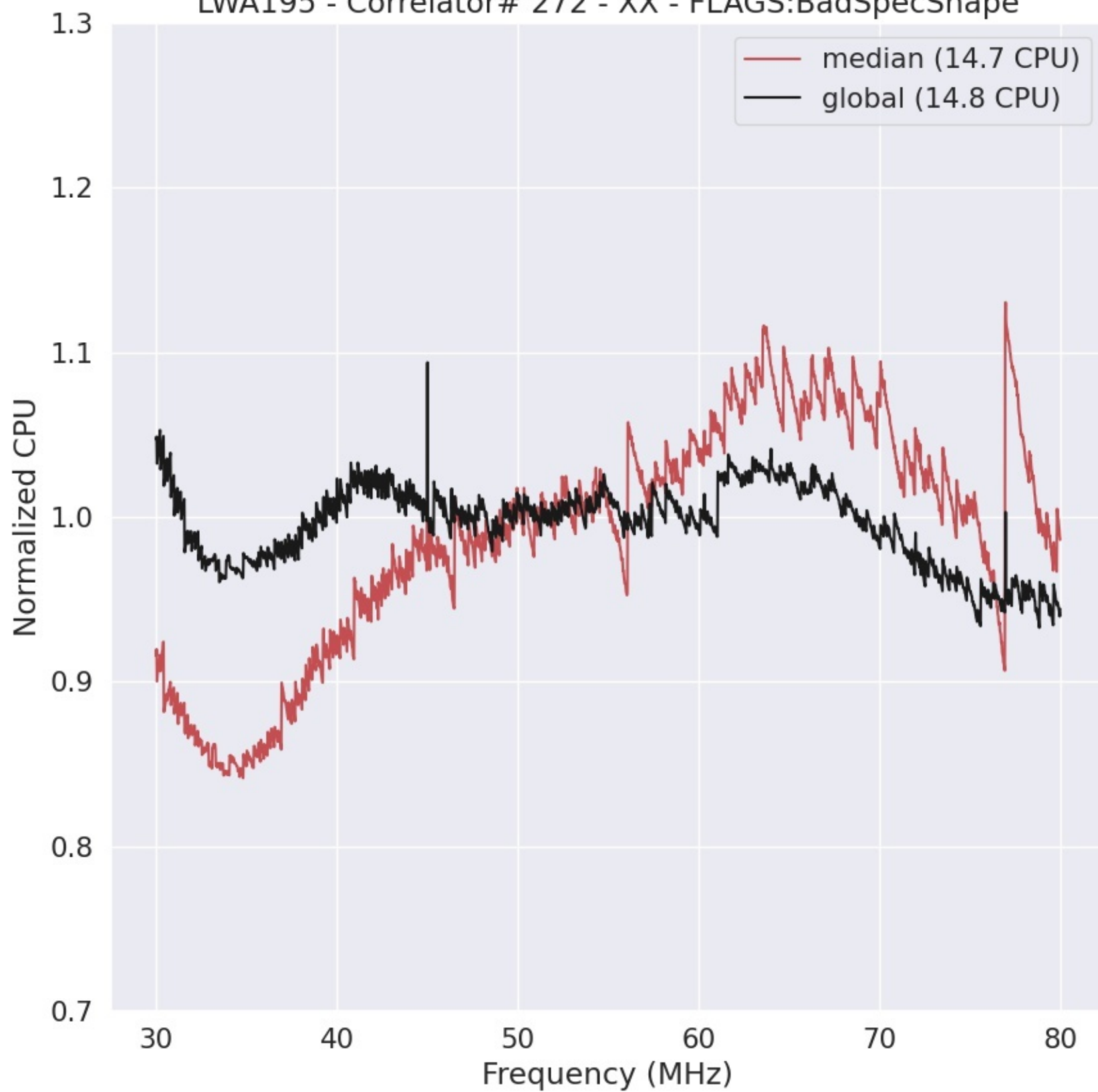
LWA195 - Correlator# 272 - XX - FLAGS:BadSpecShape
