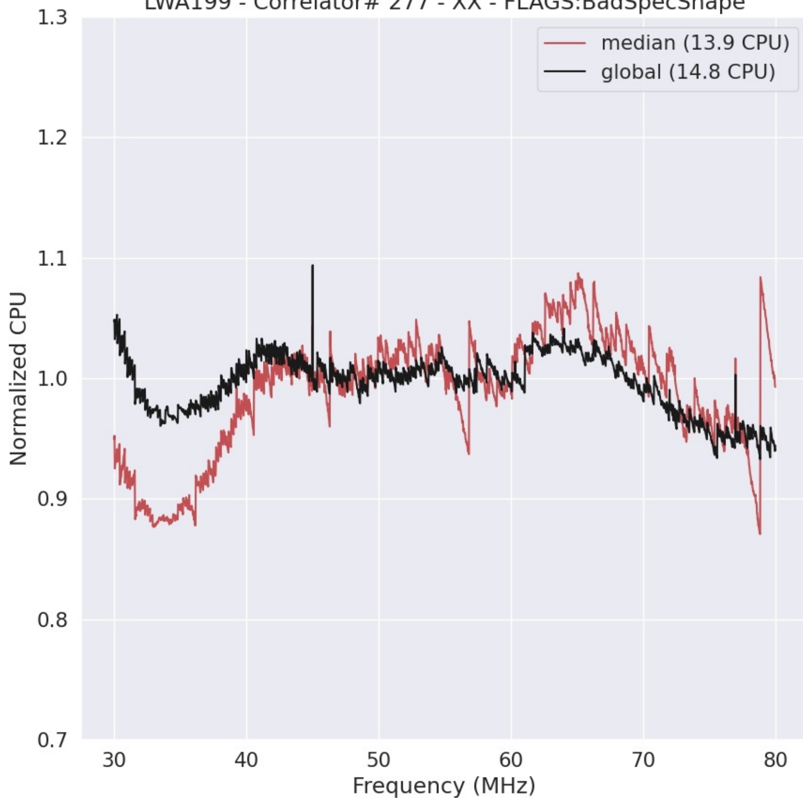
LWA199 - Correlator# 277 - XX - FLAGS:BadSpecShape
