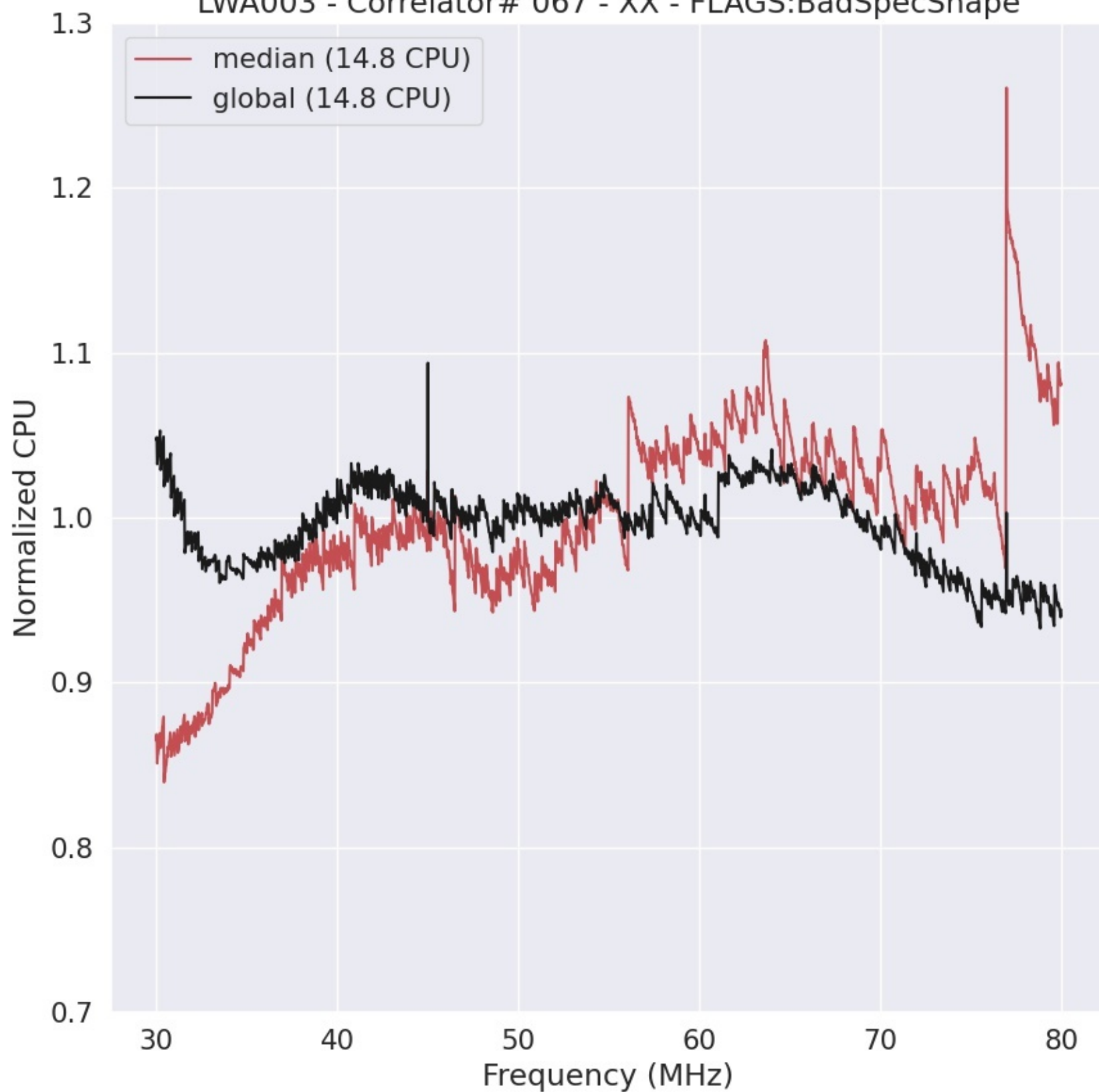
LWA003 - Correlator# 067 - XX - FLAGS:BadSpecShape
