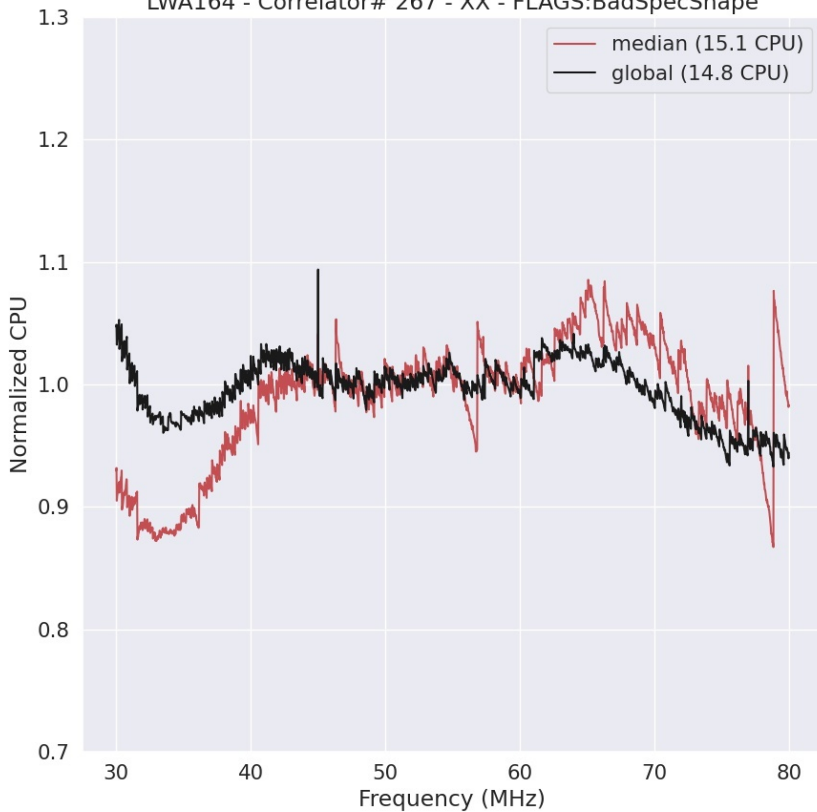
LWA164 - Correlator# 267 - XX - FLAGS:BadSpecShape
