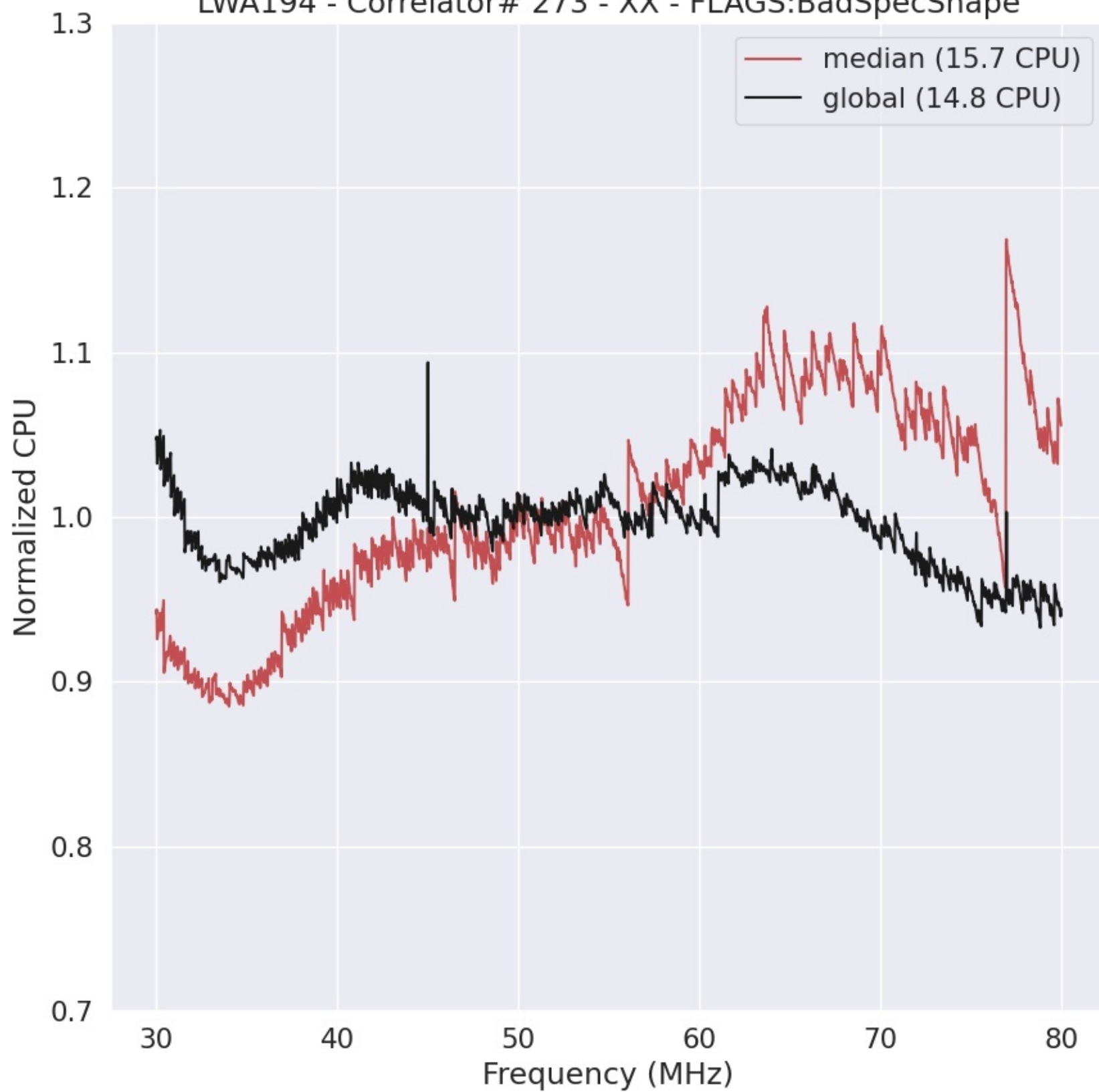
LWA194 - Correlator# 273 - XX - FLAGS:BadSpecShape
