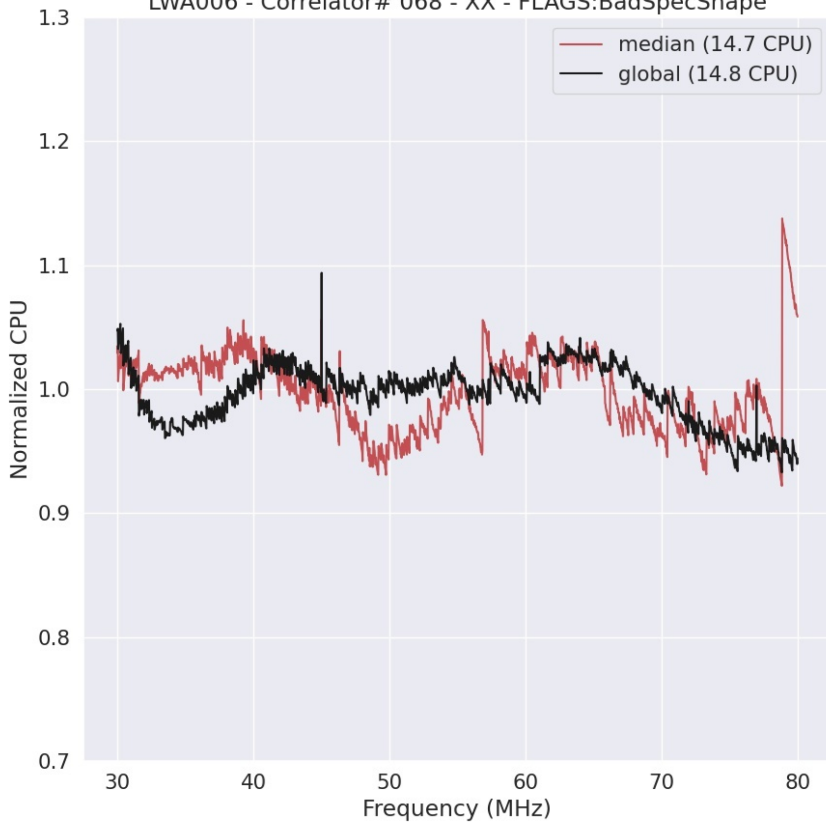
LWA006 - Correlator# 068 - XX - FLAGS:BadSpecShape
