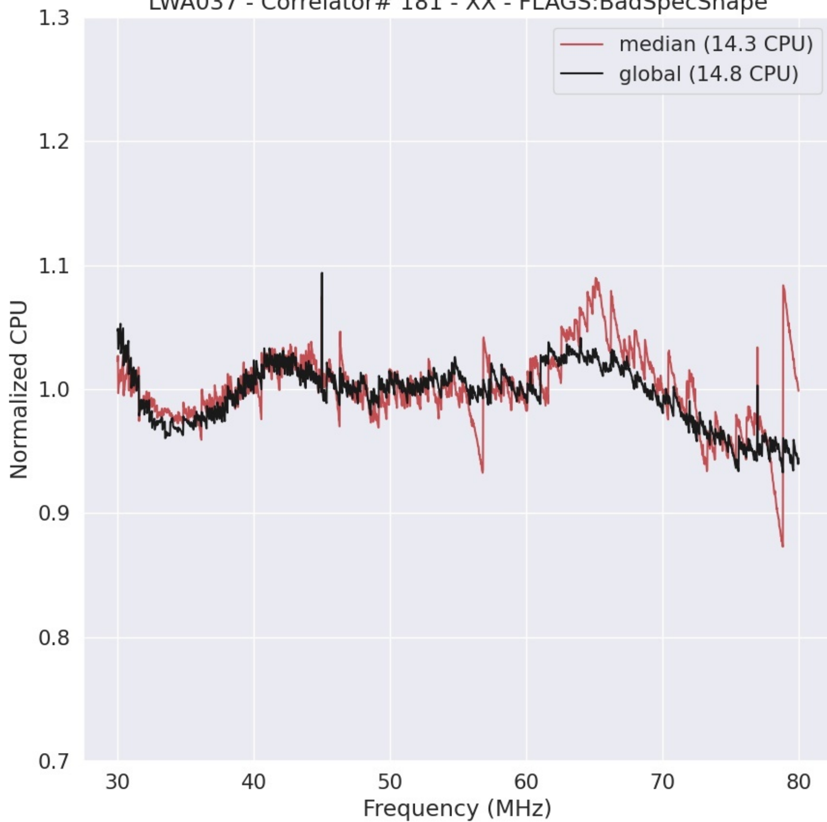
LWA037 - Correlator# 181 - XX - FLAGS:BadSpecShape
