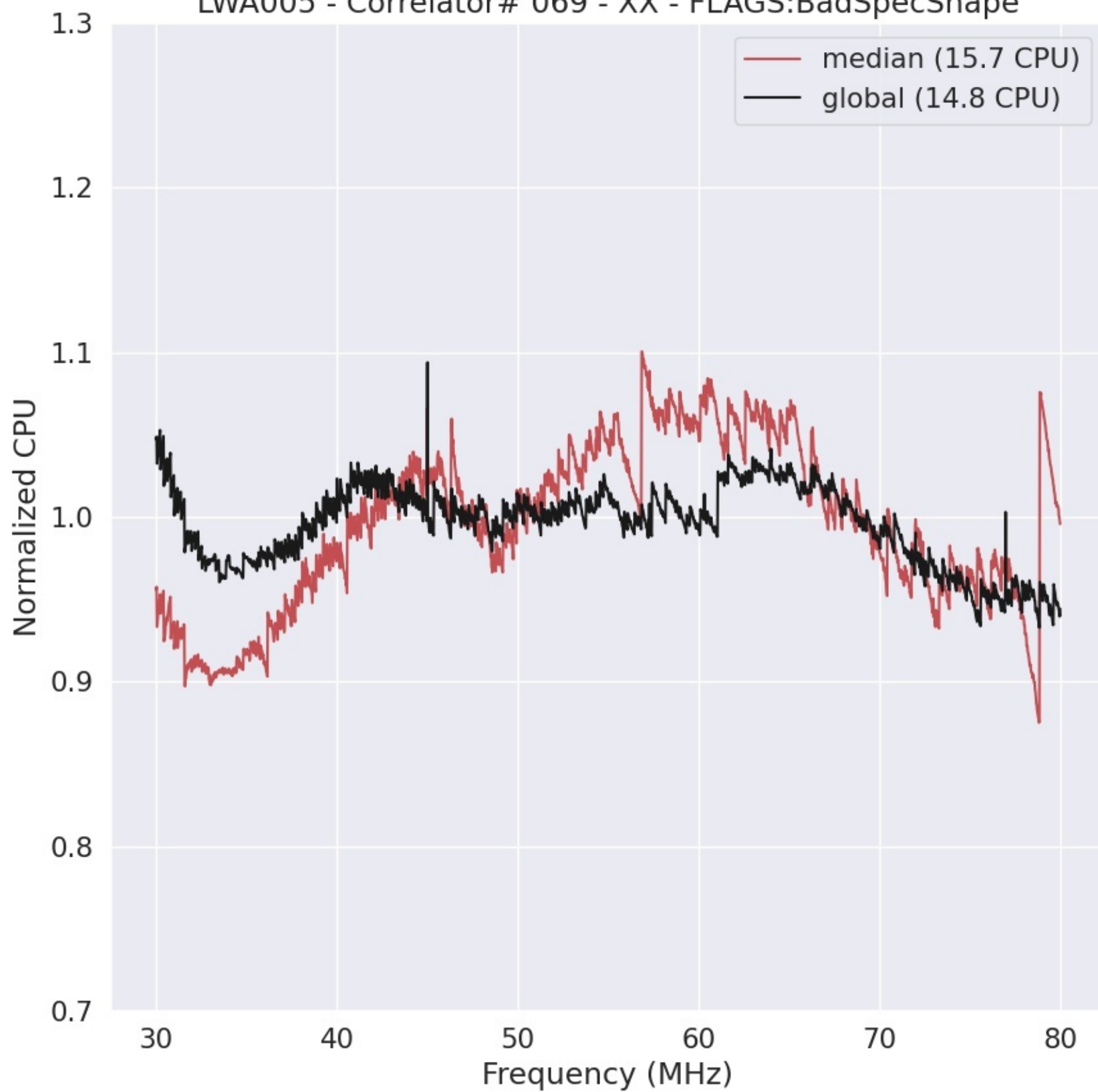
LWA005 - Correlator# 069 - XX - FLAGS:BadSpecShape
