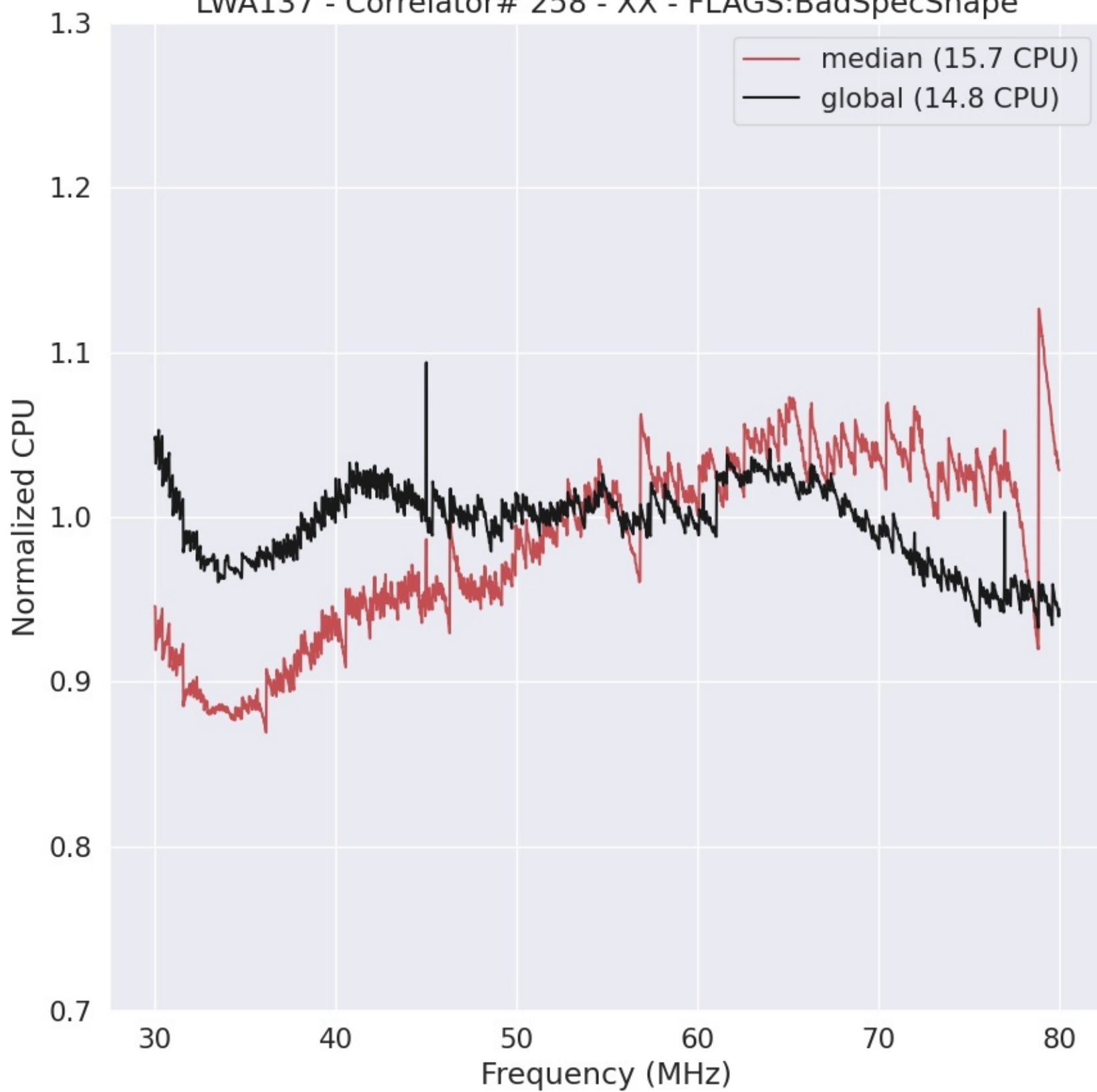
LWA137 - Correlator# 258 - XX - FLAGS:BadSpecShape
