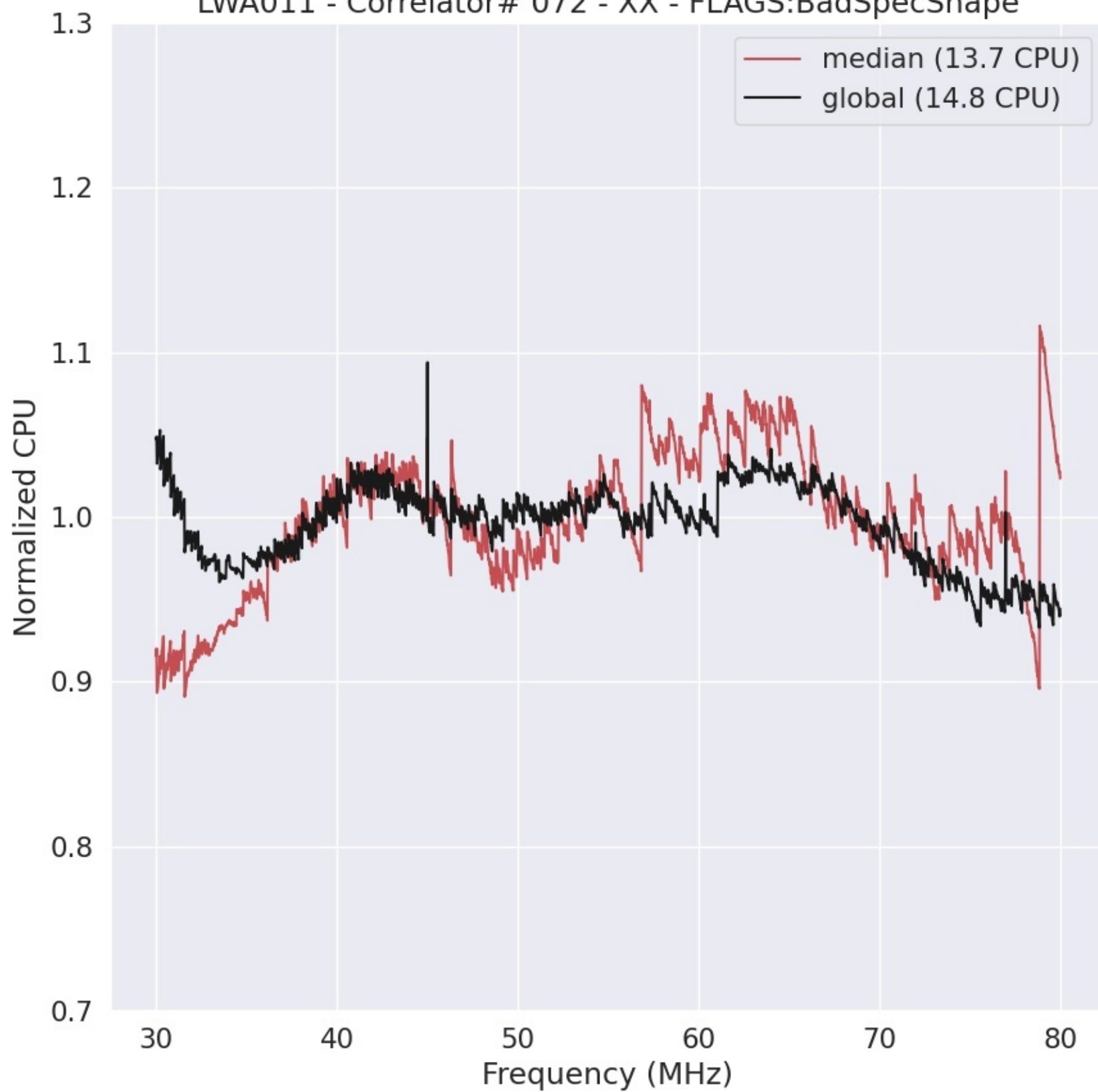
LWA011 - Correlator# 072 - XX - FLAGS:BadSpecShape
