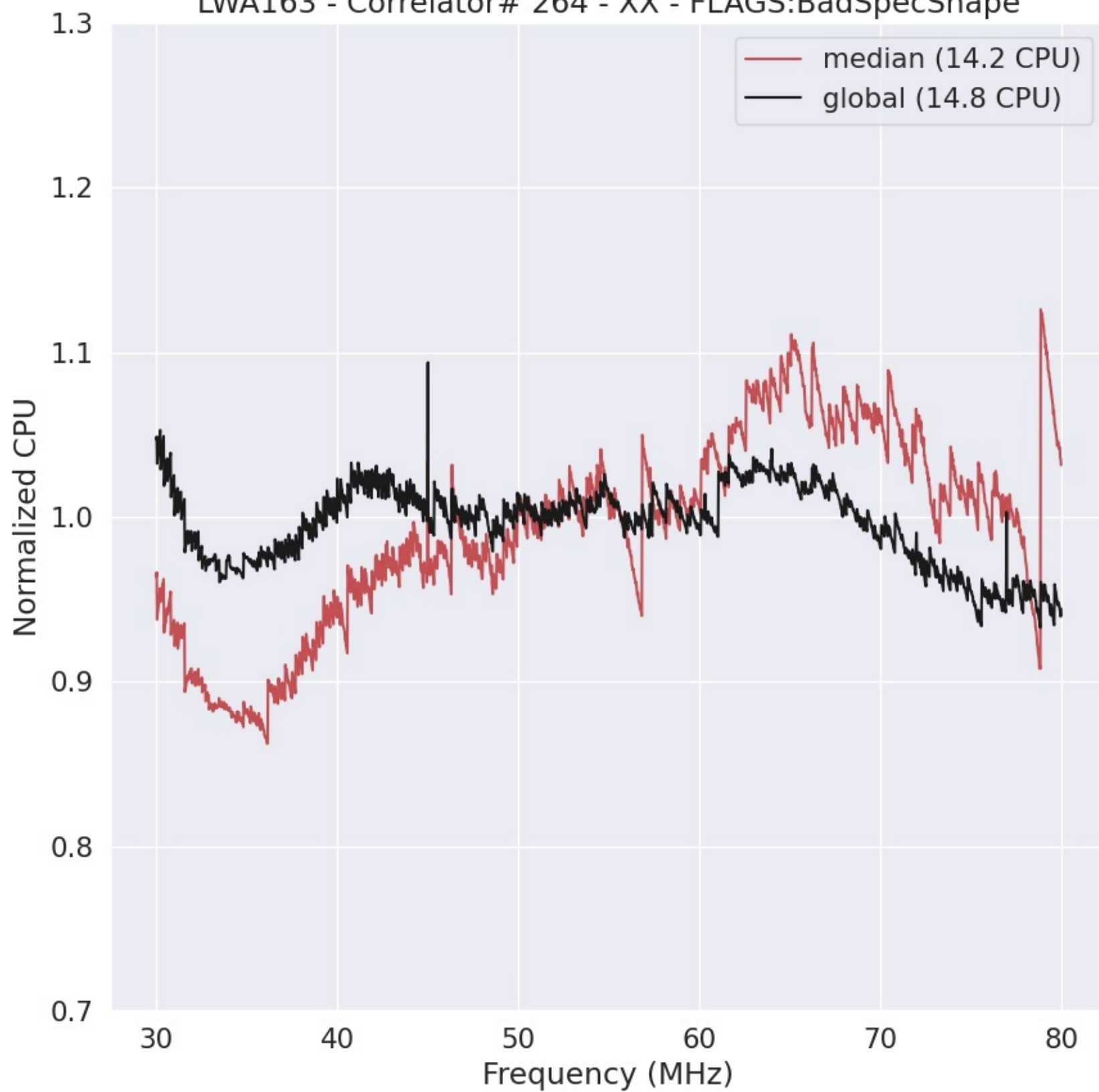
LWA163 - Correlator# 264 - XX - FLAGS:BadSpecShape
