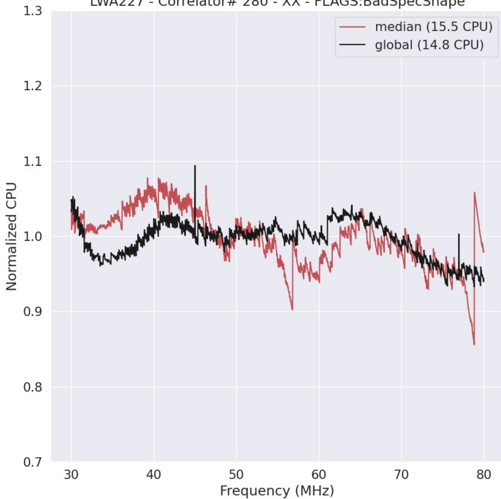
LWA227 - Correlator# 280 - XX - FLAGS:BadSpecShape
