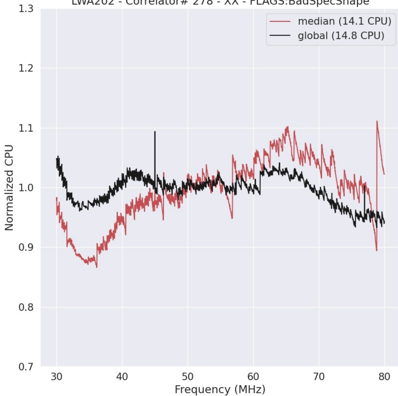
LWA202 - Correlator# 278 - XX - FLAGS:BadSpecShape
