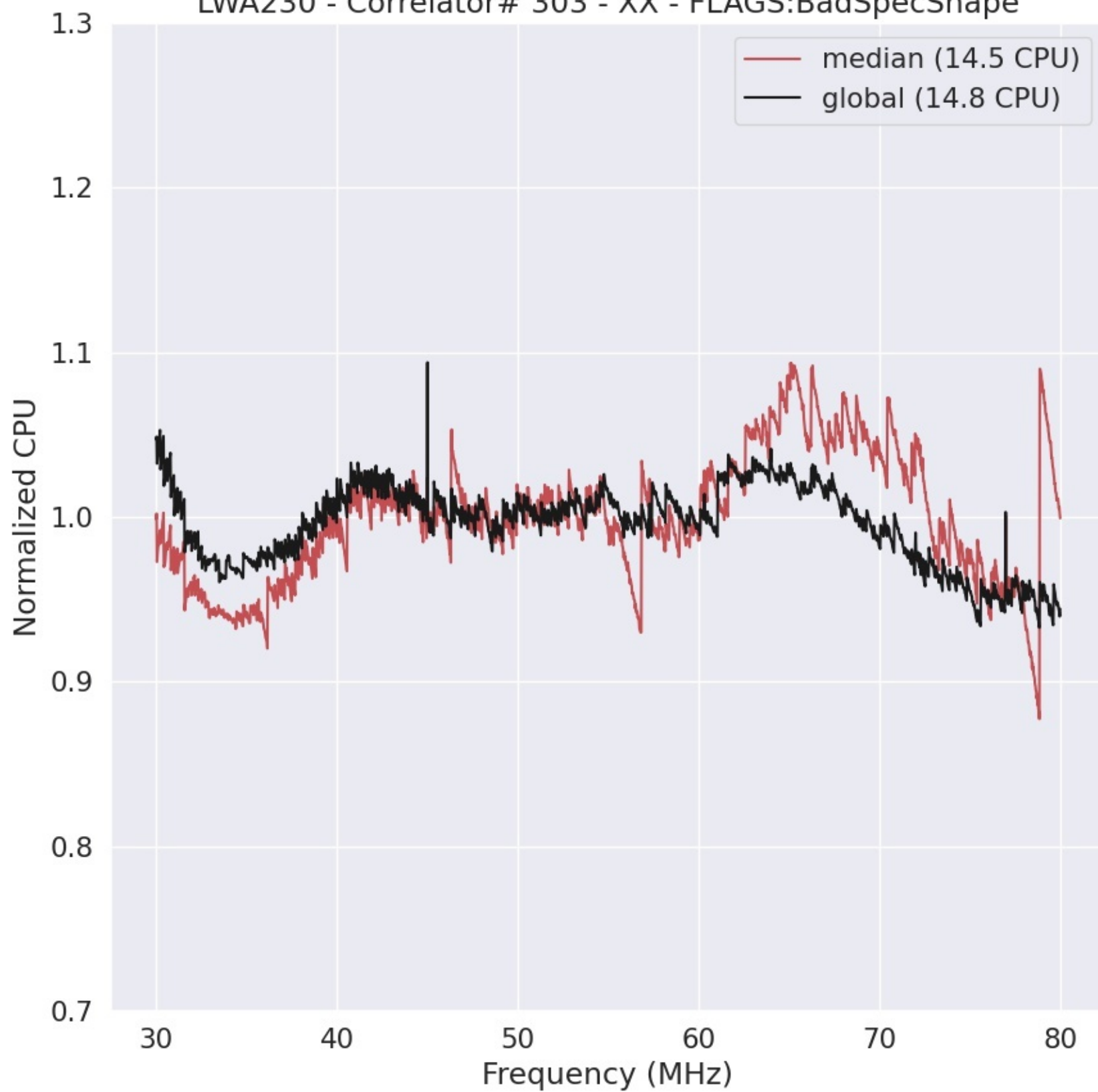
LWA230 - Correlator# 303 - XX - FLAGS:BadSpecShape
