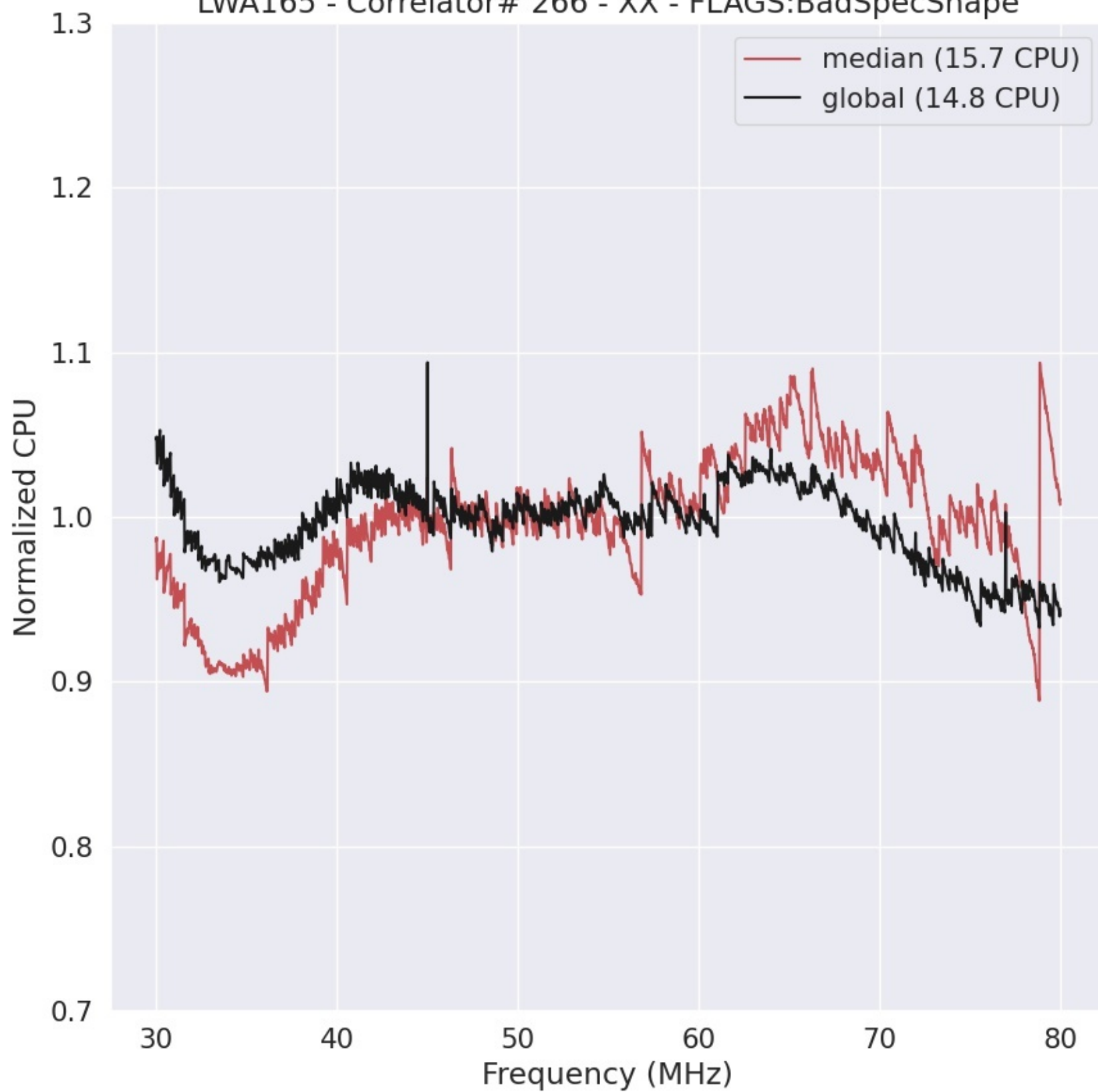
LWA165 - Correlator# 266 - XX - FLAGS:BadSpecShape
