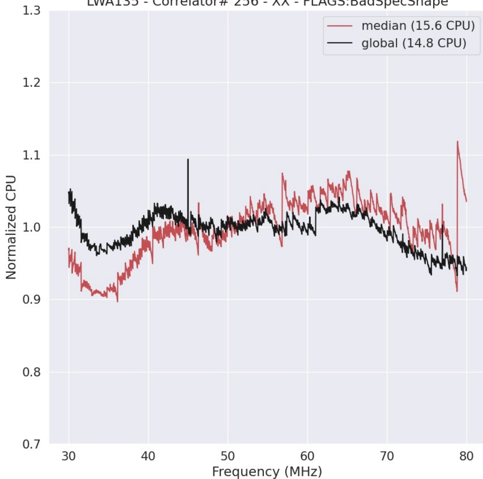
LWA135 - Correlator# 256 - XX - FLAGS:BadSpecShape
