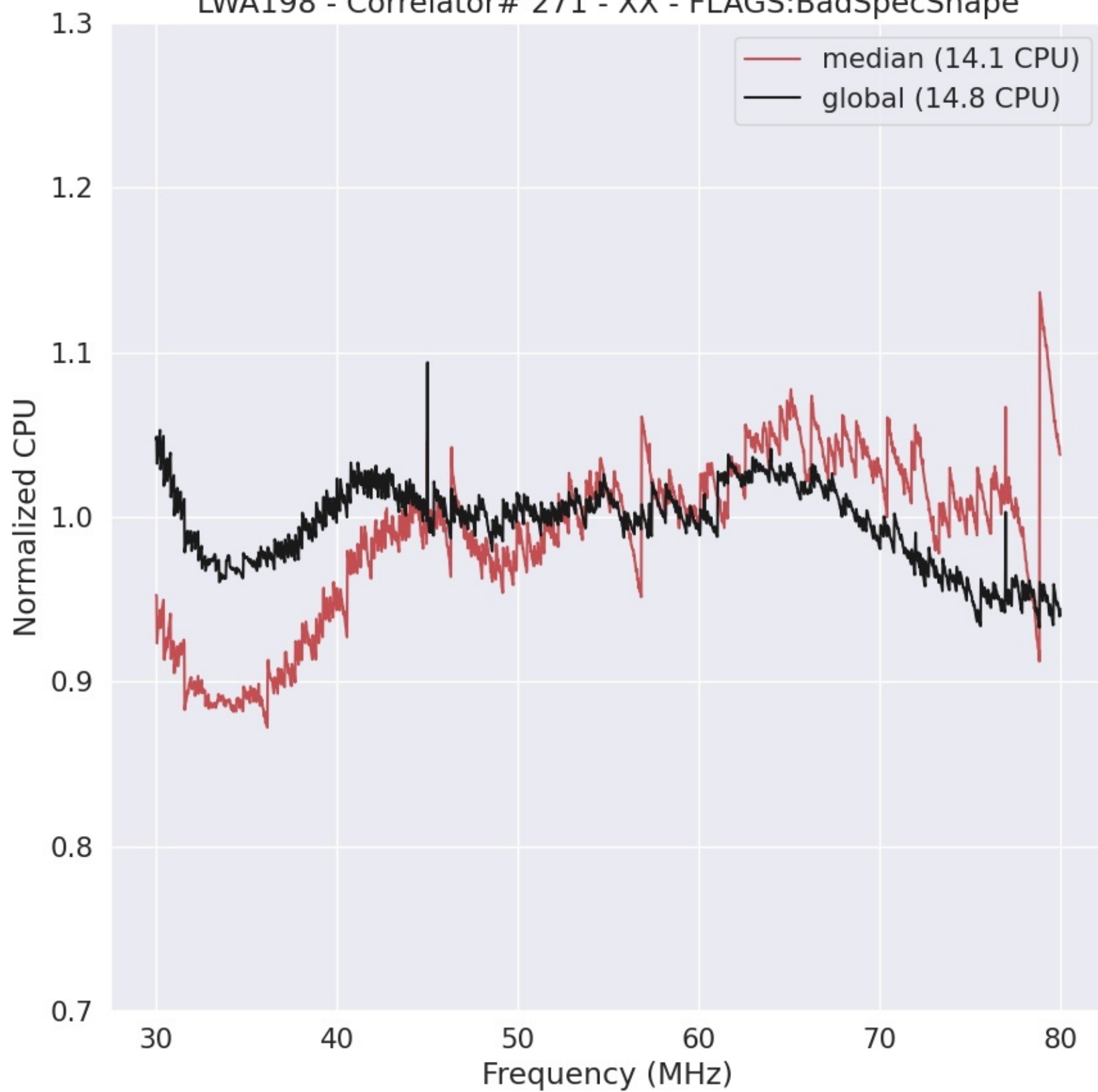
LWA198 - Correlator# 271 - XX - FLAGS:BadSpecShape
