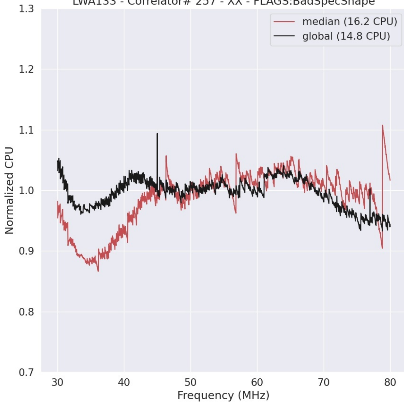
LWA133 - Correlator# 257 - XX - FLAGS:BadSpecShape
