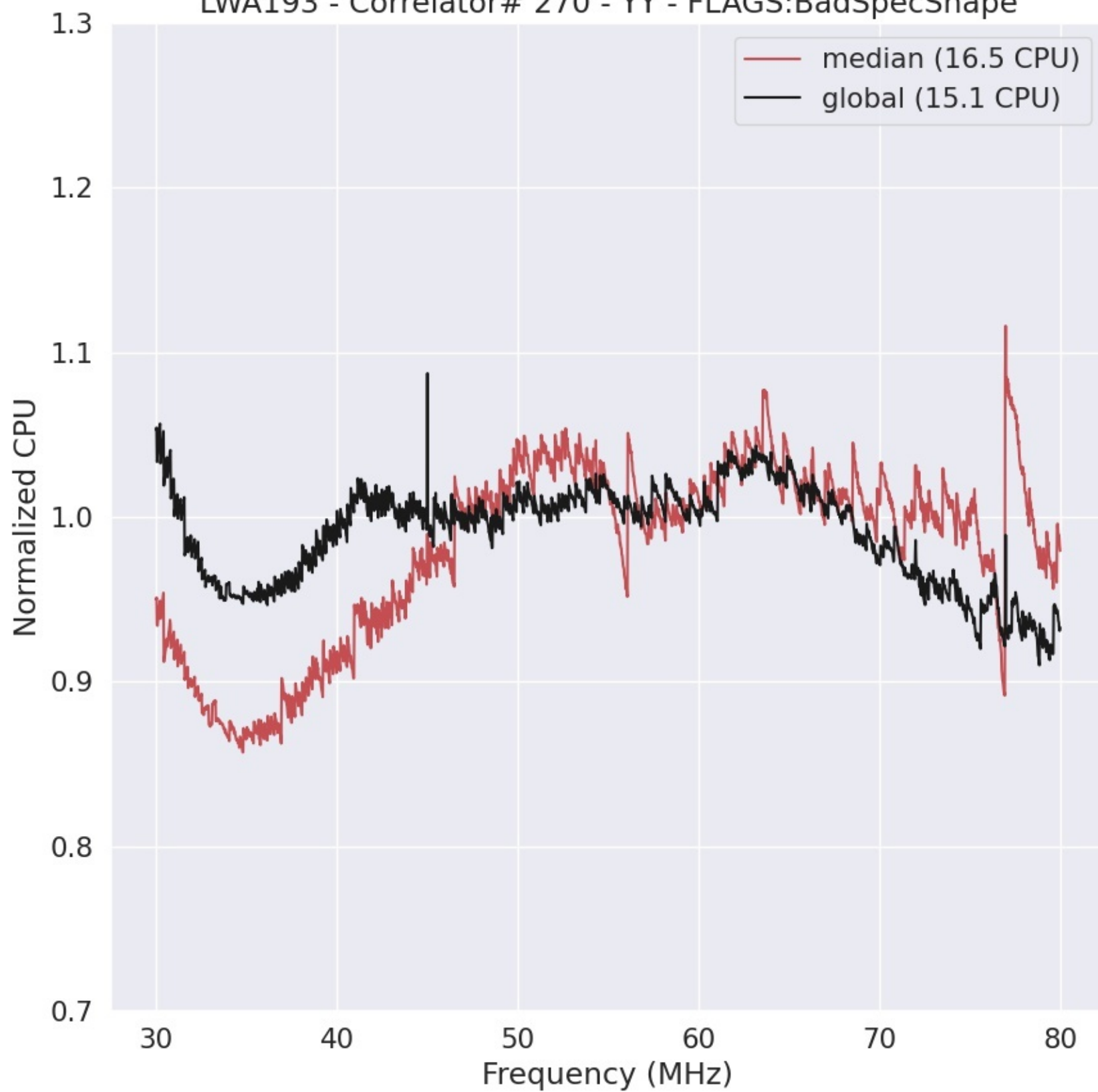
LWA193 - Correlator# 270 - YY - FLAGS:BadSpecShape
