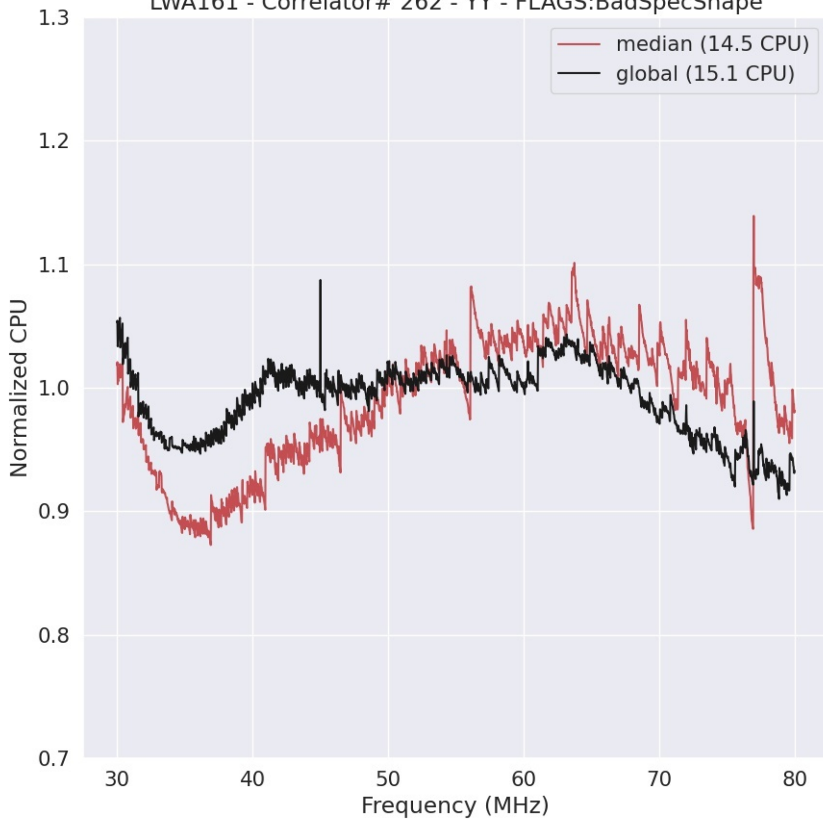
LWA161 - Correlator# 262 - YY - FLAGS:BadSpecShape
