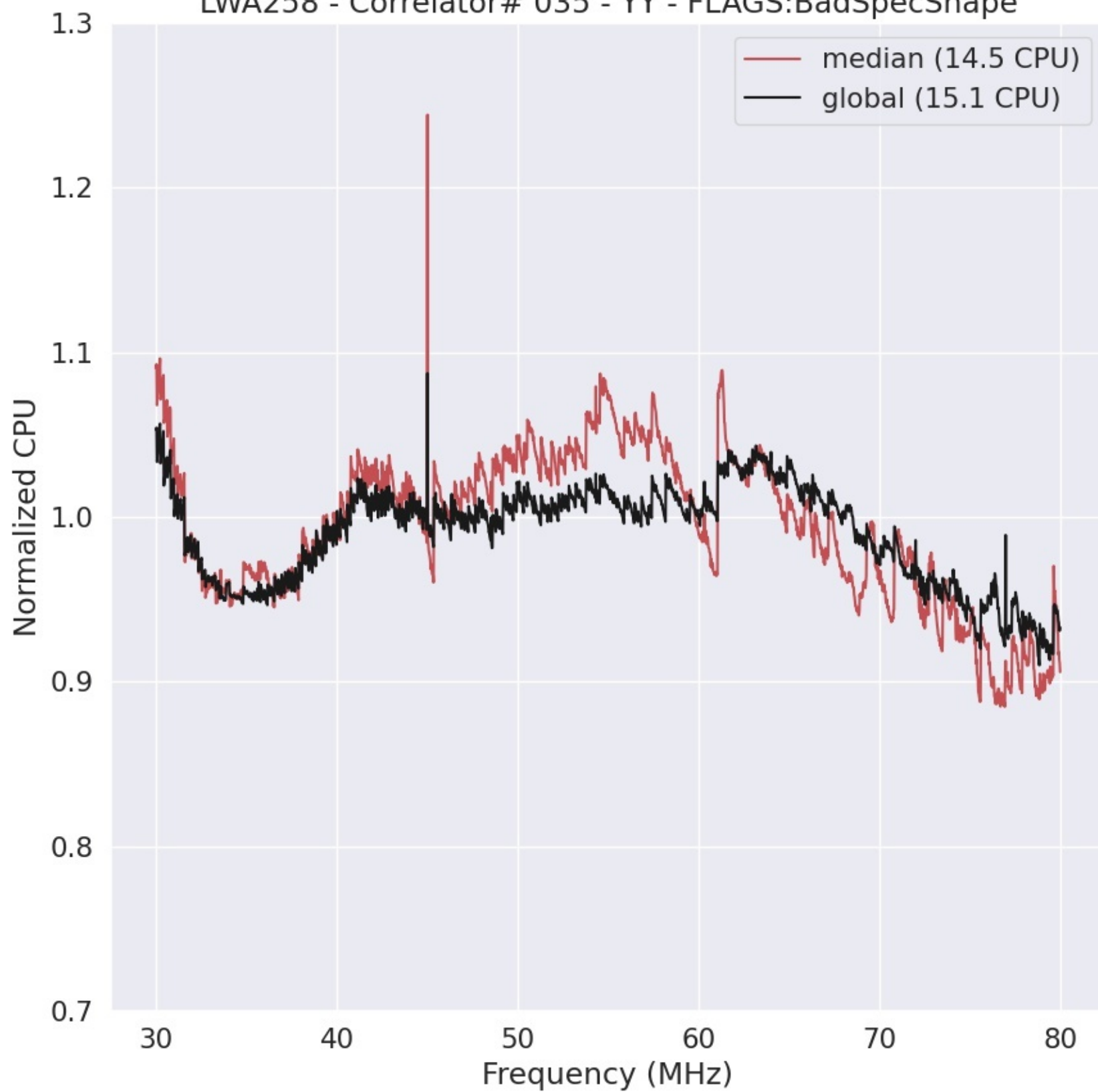
LWA258 - Correlator# 035 - YY - FLAGS:BadSpecShape
