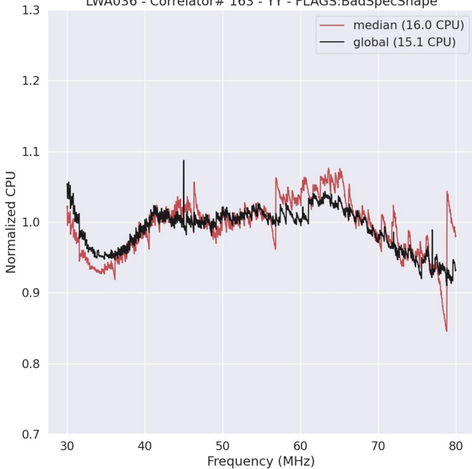
LWA036 - Correlator# 163 - YY - FLAGS:BadSpecShape
