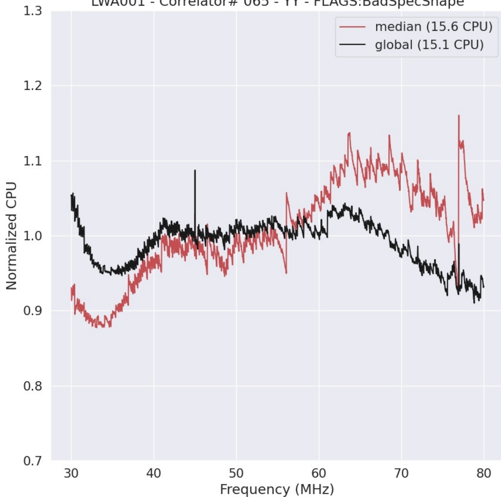
LWA001 - Correlator# 065 - YY - FLAGS:BadSpecShape
