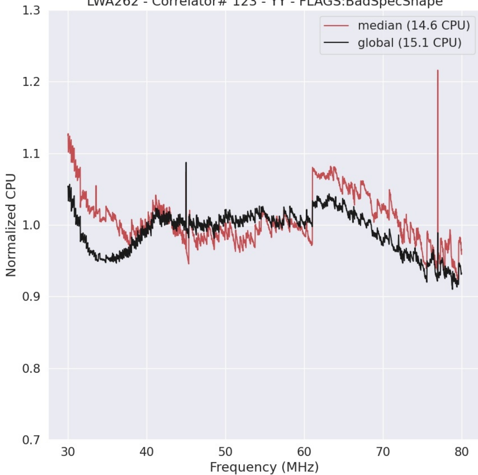
LWA262 - Correlator# 123 - YY - FLAGS:BadSpecShape
