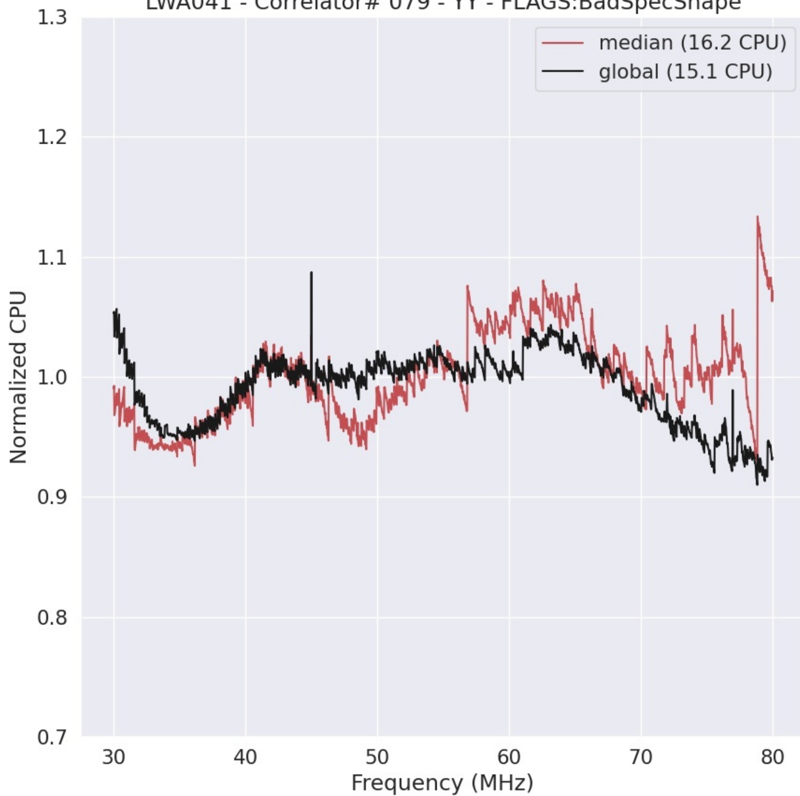
LWA041 - Correlator# 079 - YY - FLAGS:BadSpecShape
