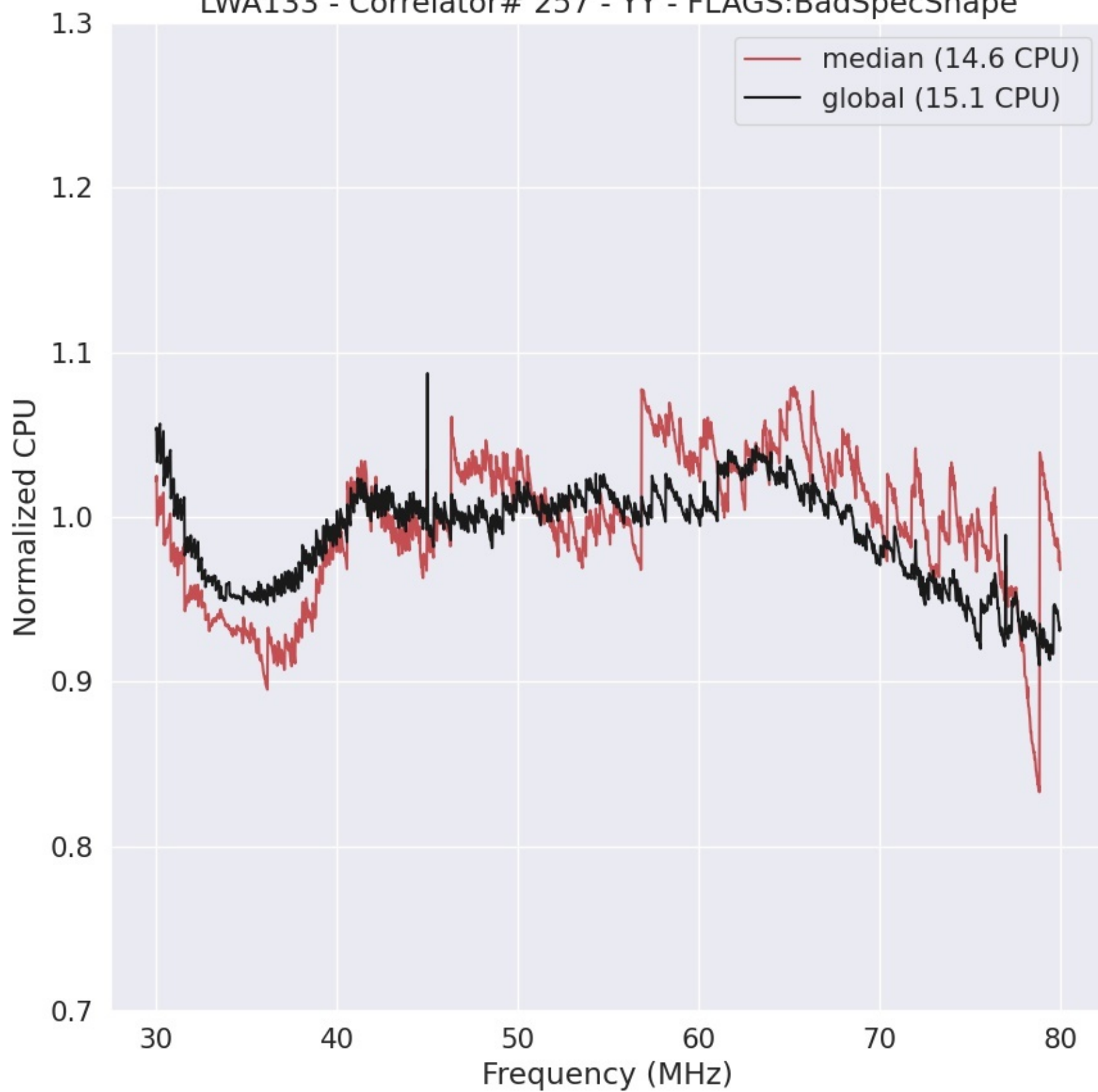
LWA133 - Correlator# 257 - YY - FLAGS:BadSpecShape
