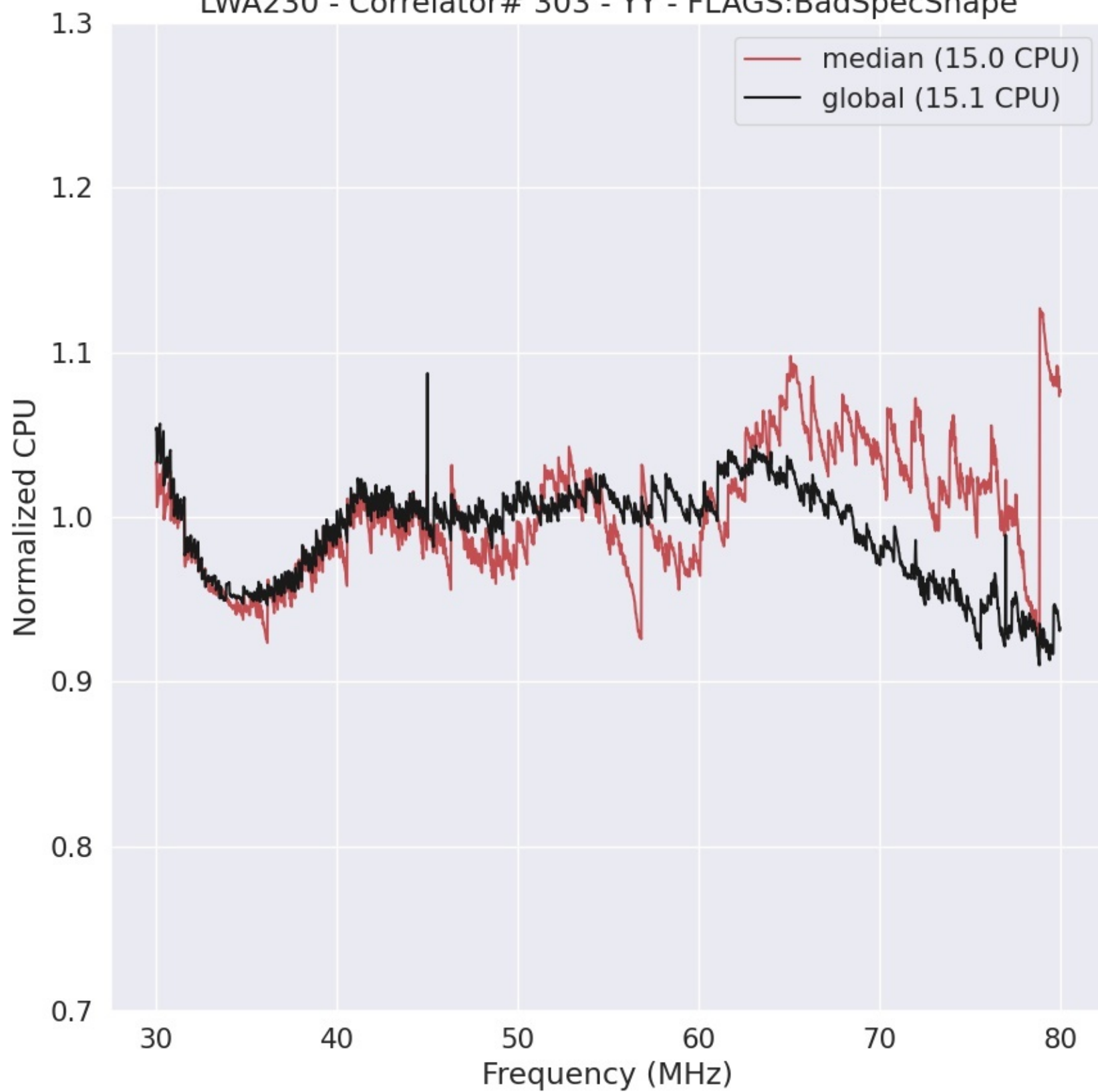
LWA230 - Correlator# 303 - YY - FLAGS:BadSpecShape
