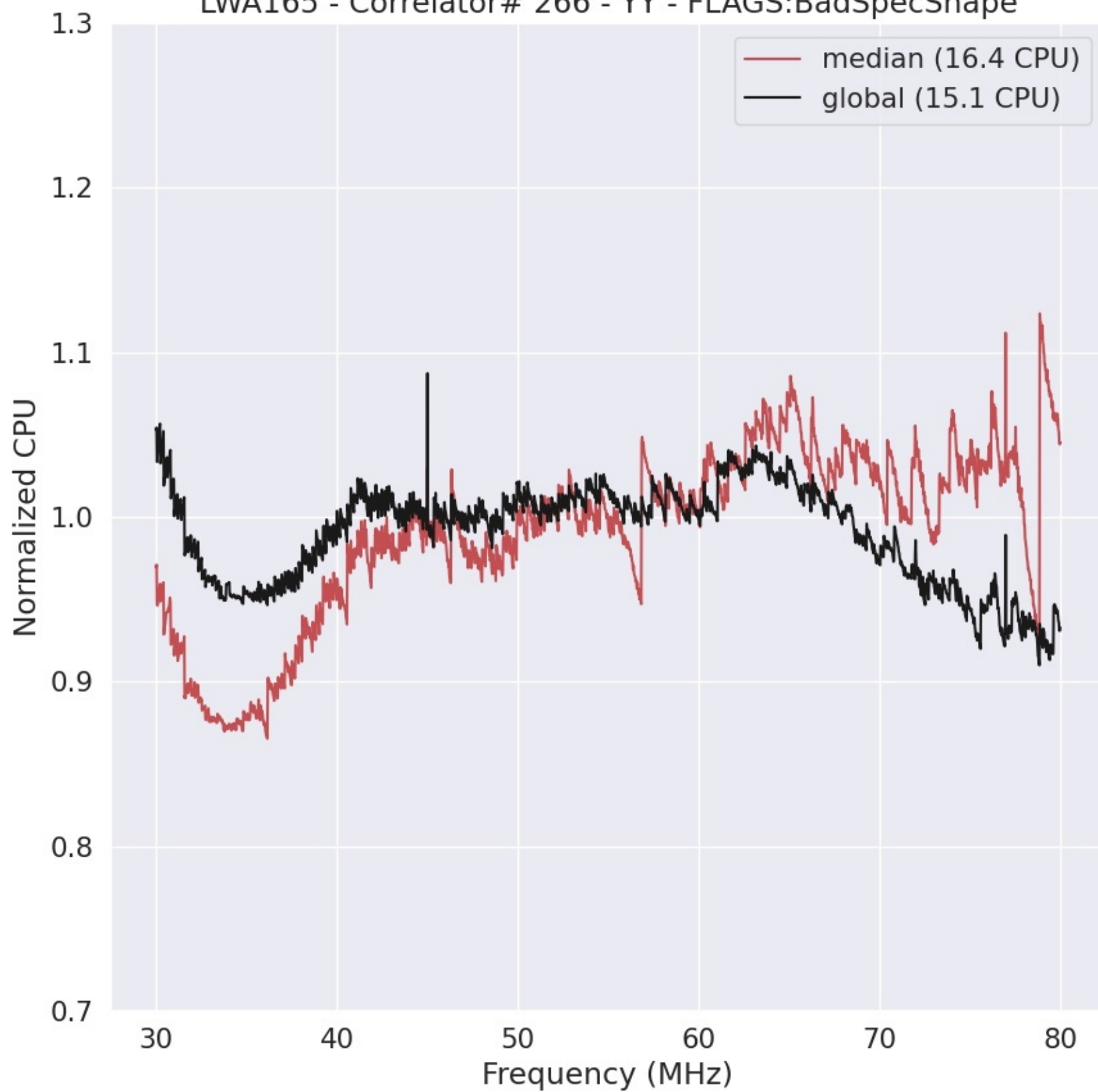
LWA165 - Correlator# 266 - YY - FLAGS:BadSpecShape
