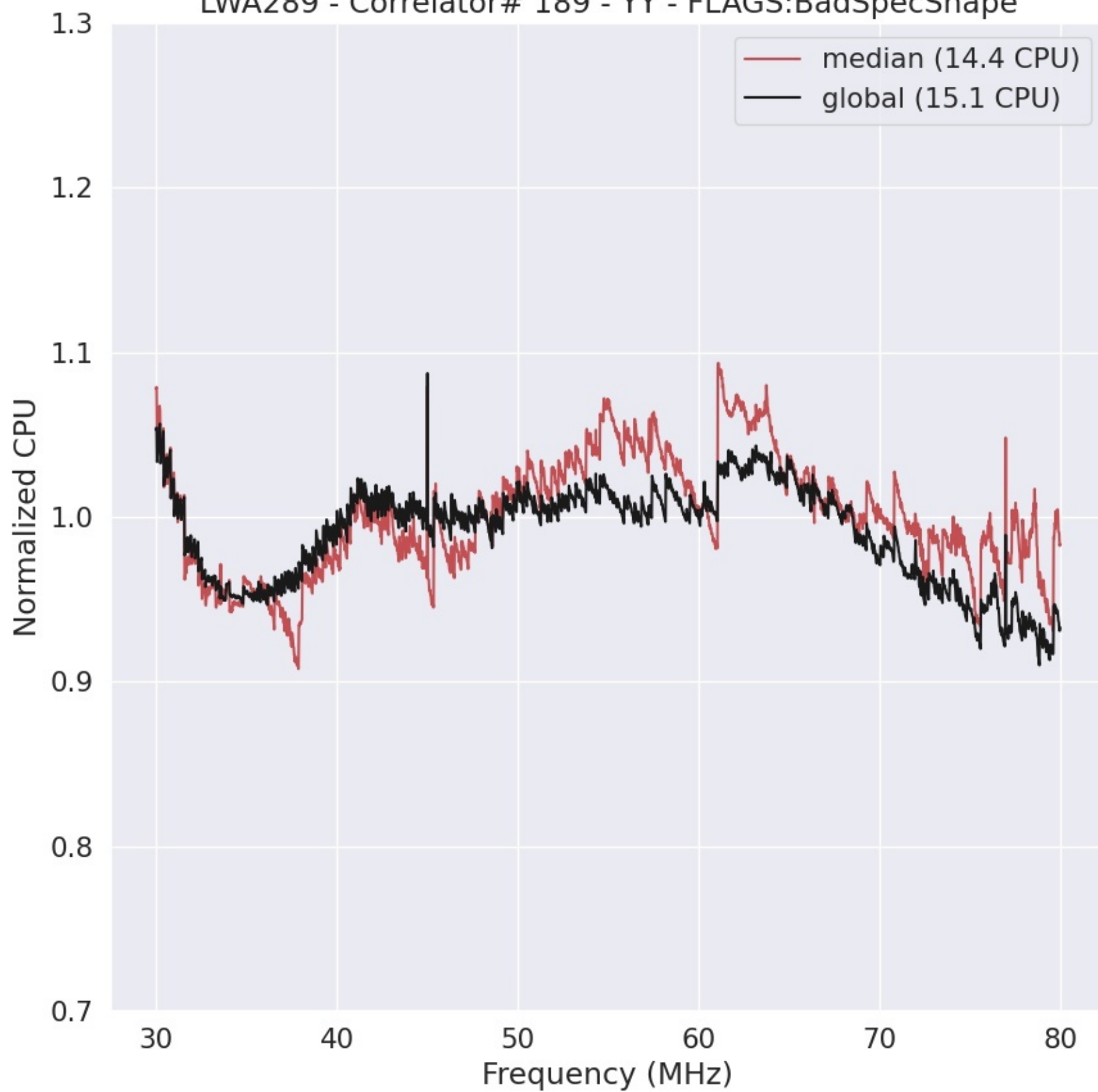
LWA289 - Correlator# 189 - YY - FLAGS:BadSpecShape
