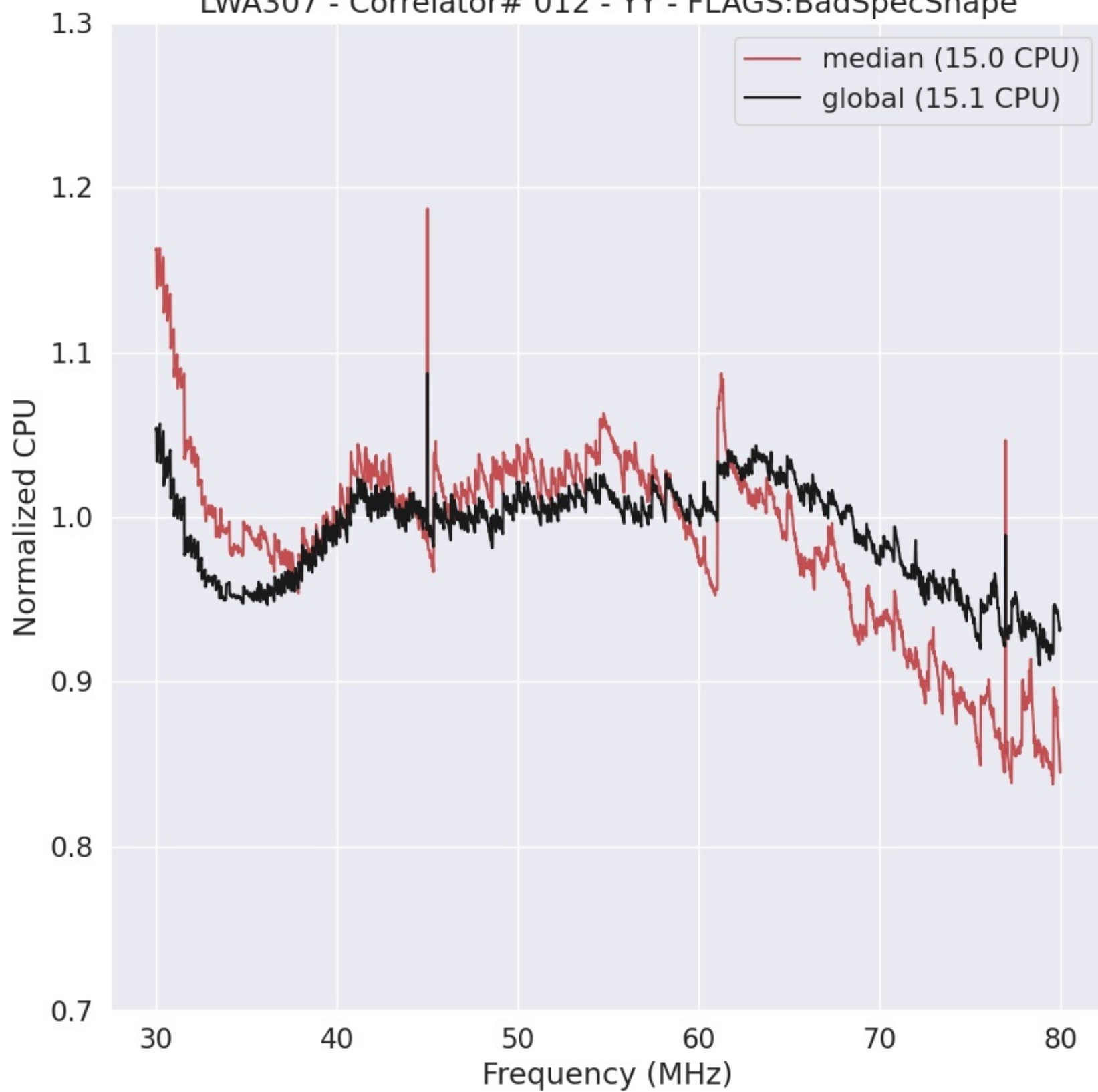
LWA307 - Correlator# 012 - YY - FLAGS:BadSpecShape
