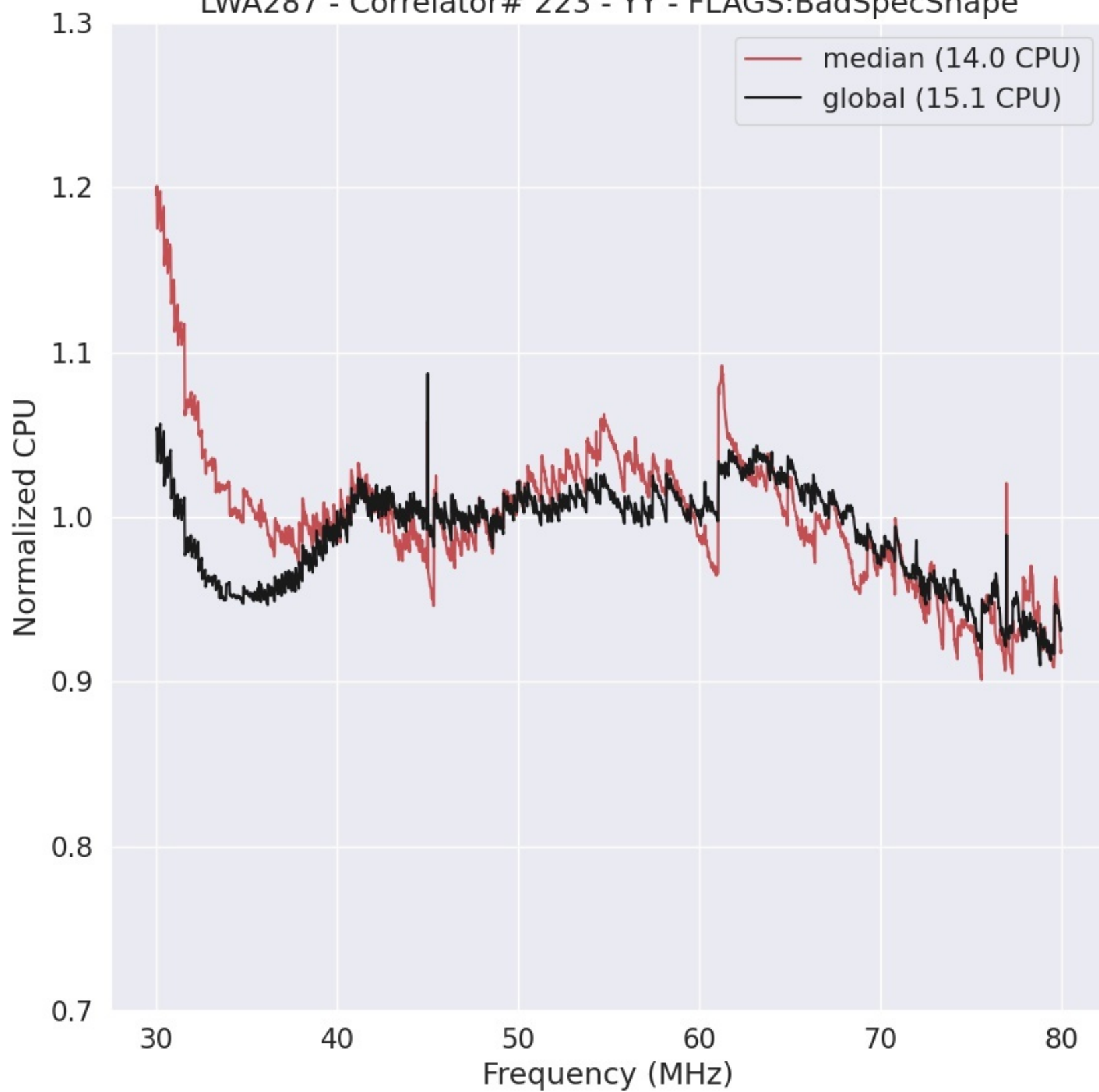
LWA287 - Correlator# 223 - YY - FLAGS:BadSpecShape
