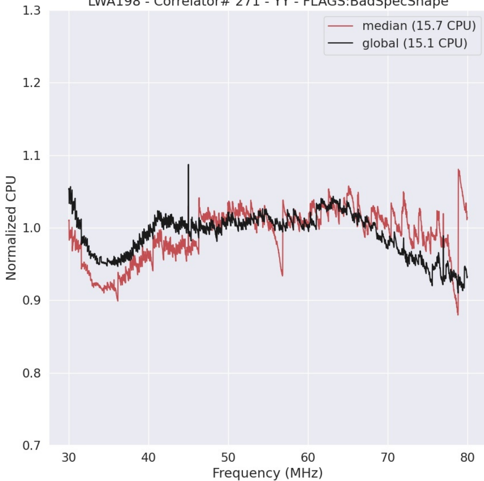
LWA198 - Correlator# 271 - YY - FLAGS:BadSpecShape
