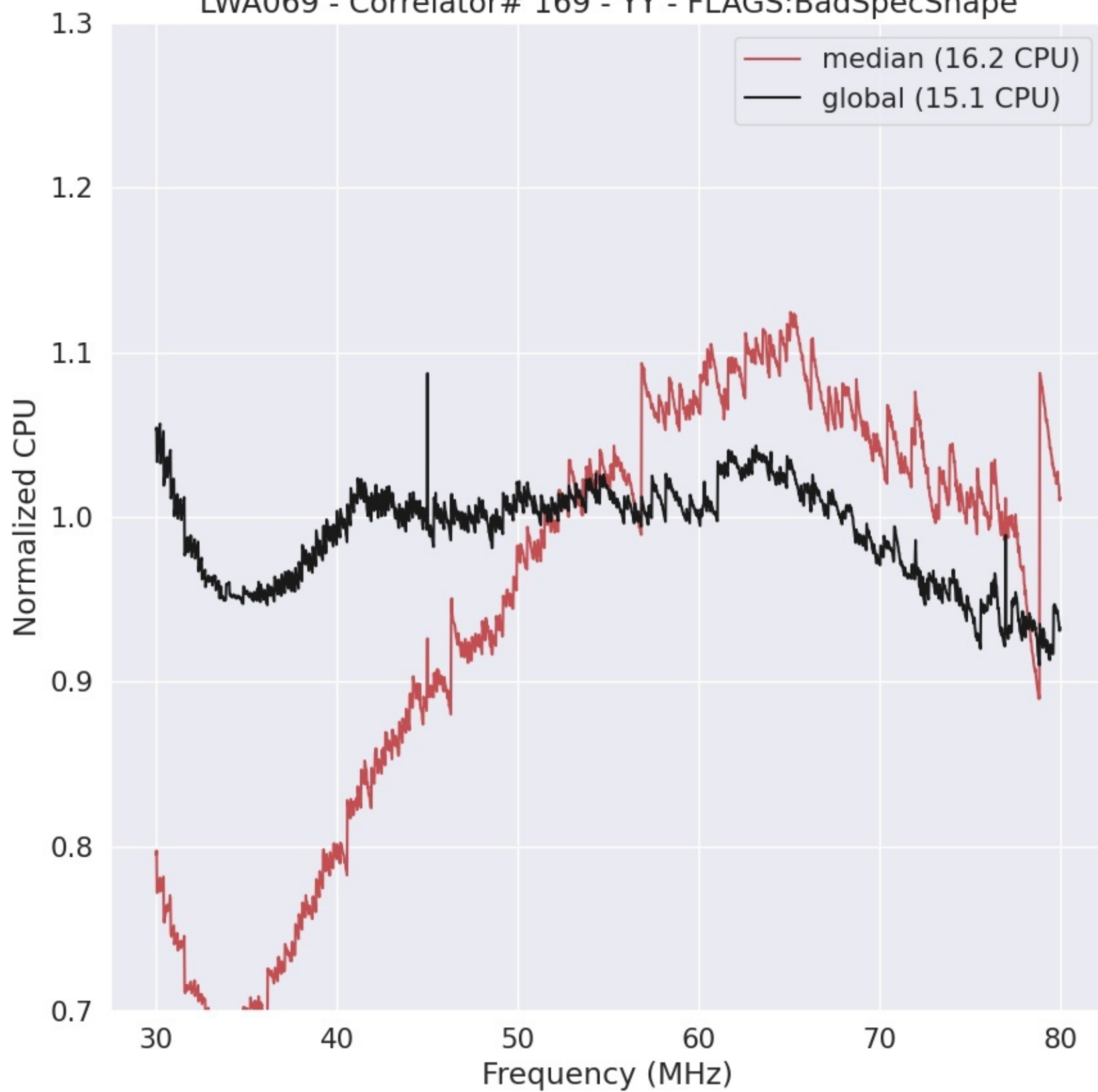
LWA069 - Correlator# 169 - YY - FLAGS:BadSpecShape
