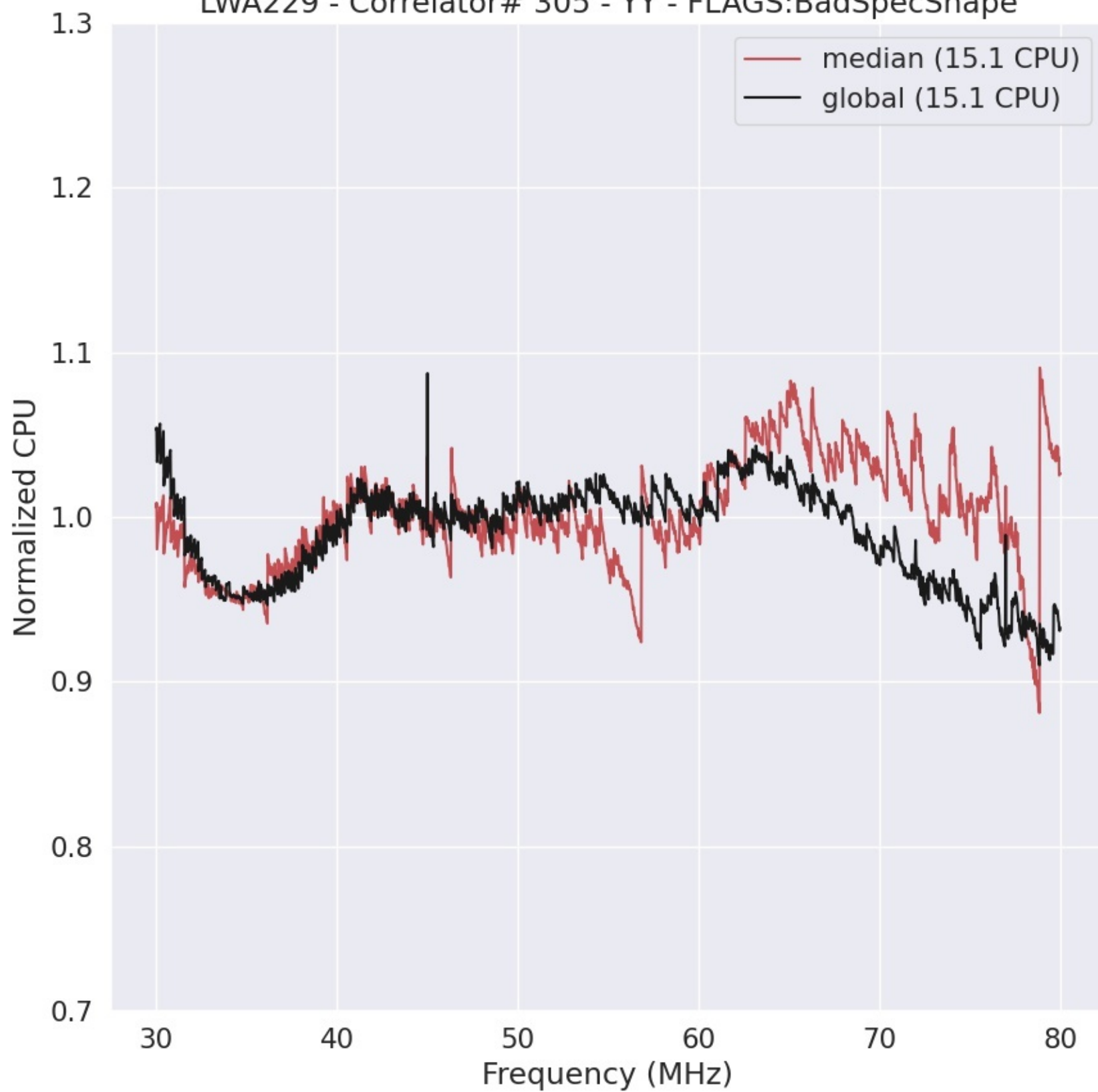
LWA229 - Correlator# 305 - YY - FLAGS:BadSpecShape
