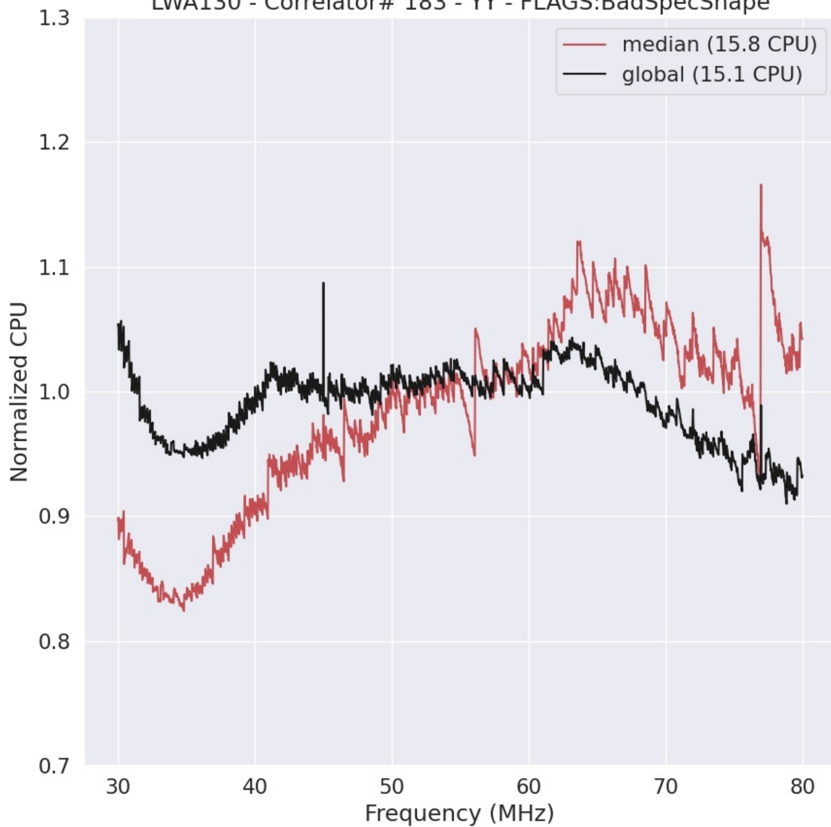
LWA130 - Correlator# 183 - YY - FLAGS:BadSpecShape
