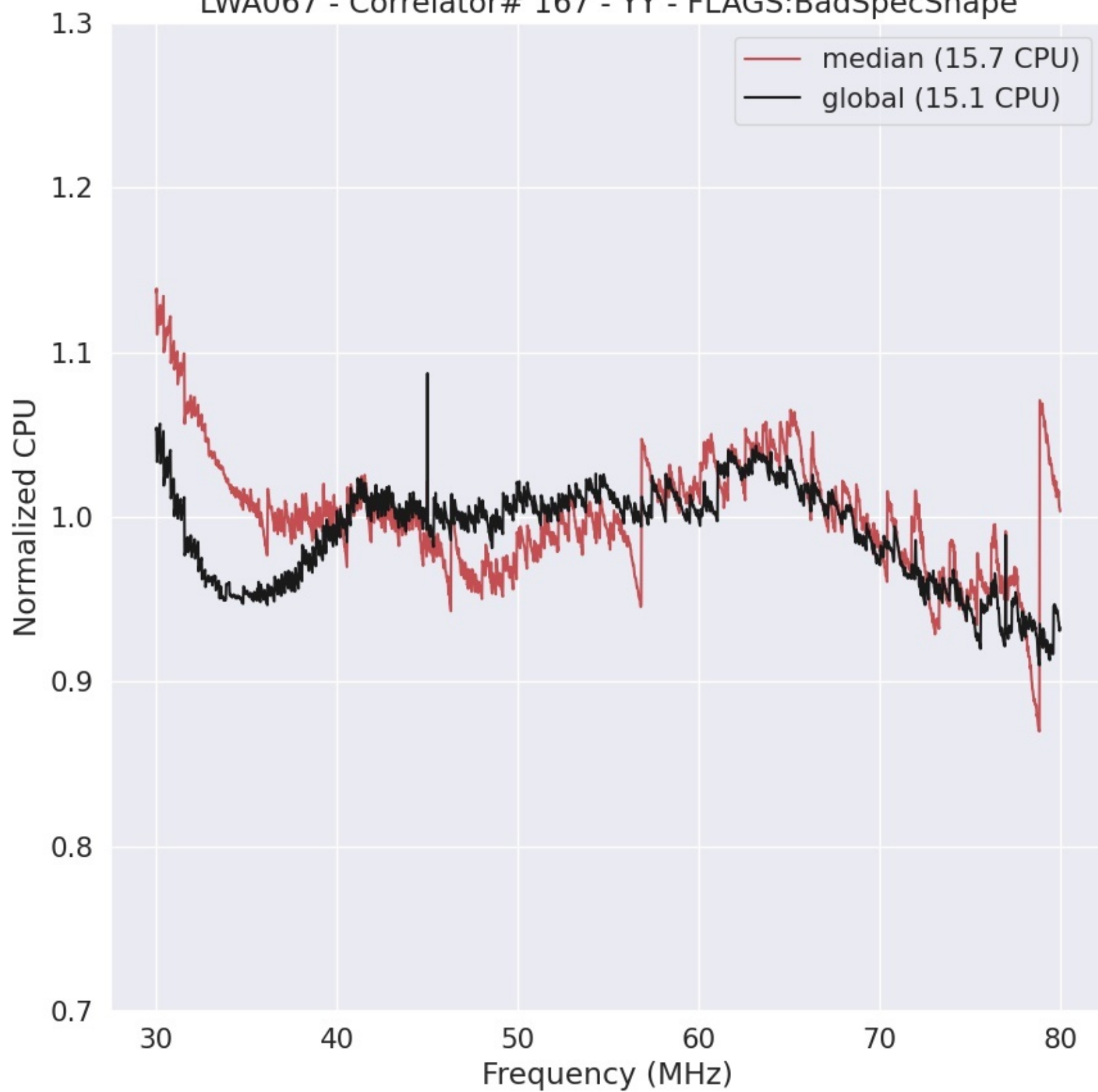
LWA067 - Correlator# 167 - YY - FLAGS:BadSpecShape
