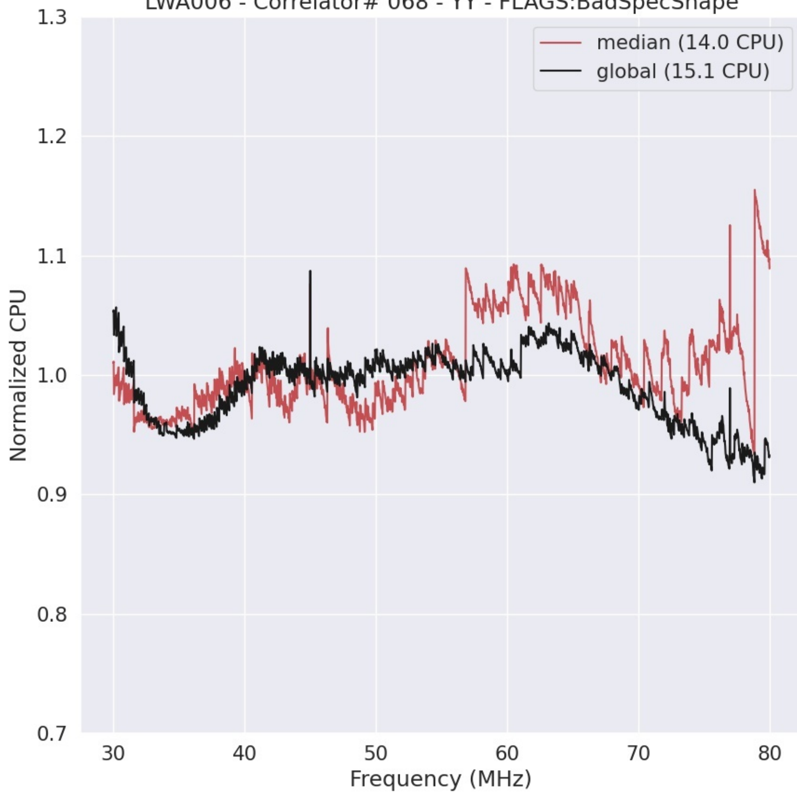
LWA006 - Correlator# 068 - YY - FLAGS:BadSpecShape
