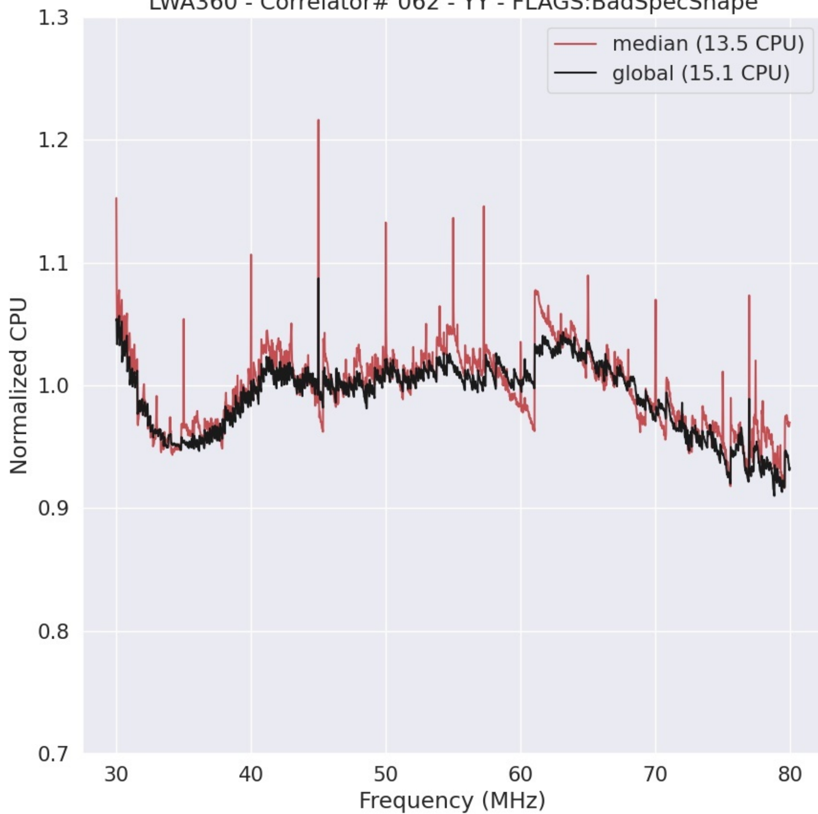
LWA360 - Correlator# 062 - YY - FLAGS:BadSpecShape
