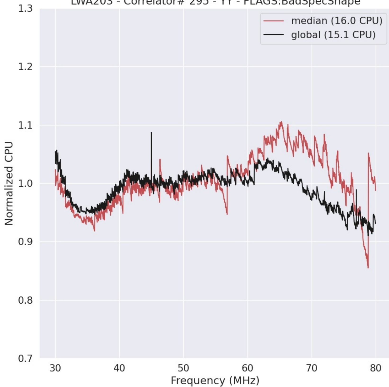
LWA203 - Correlator# 295 - YY - FLAGS:BadSpecShape
