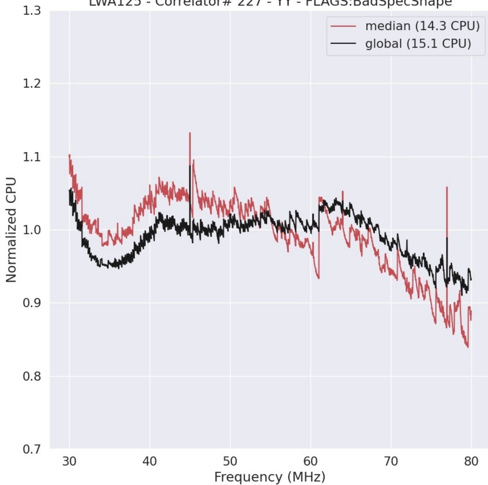
LWA125 - Correlator# 227 - YY - FLAGS:BadSpecShape
