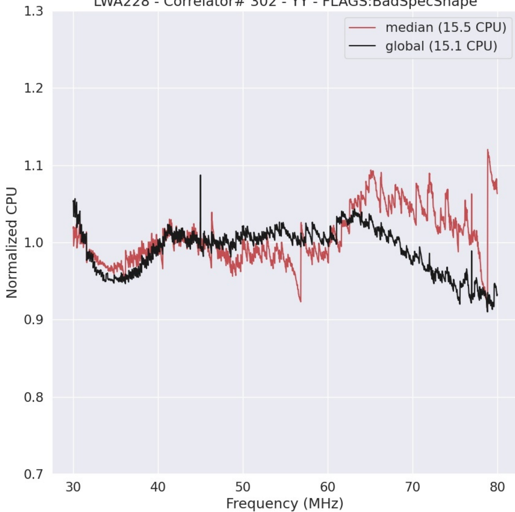
LWA228 - Correlator# 302 - YY - FLAGS:BadSpecShape
