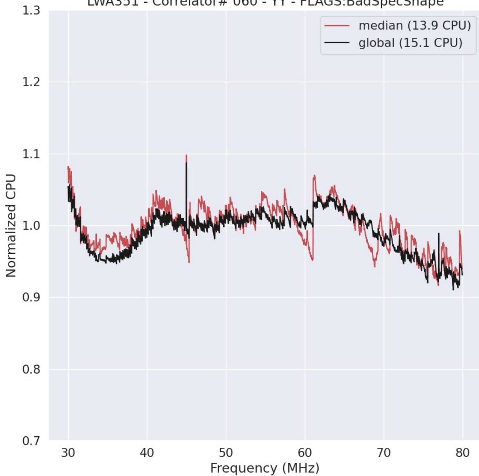
LWA351 - Correlator# 060 - YY - FLAGS:BadSpecShape
