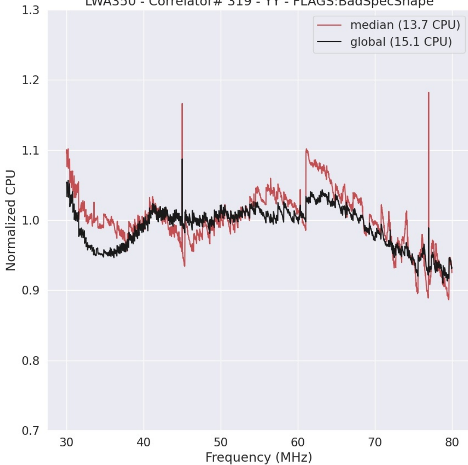
LWA350 - Correlator# 319 - YY - FLAGS:BadSpecShape
