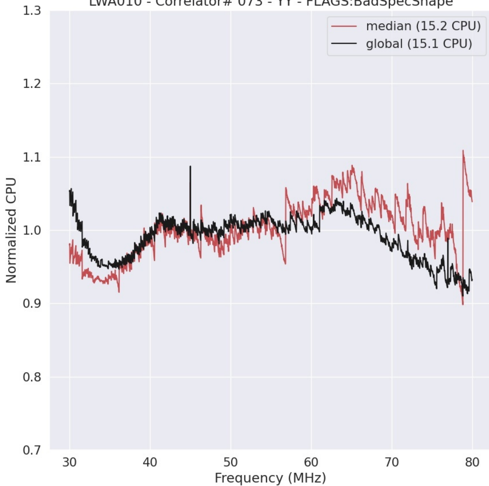
LWA010 - Correlator# 073 - YY - FLAGS:BadSpecShape
