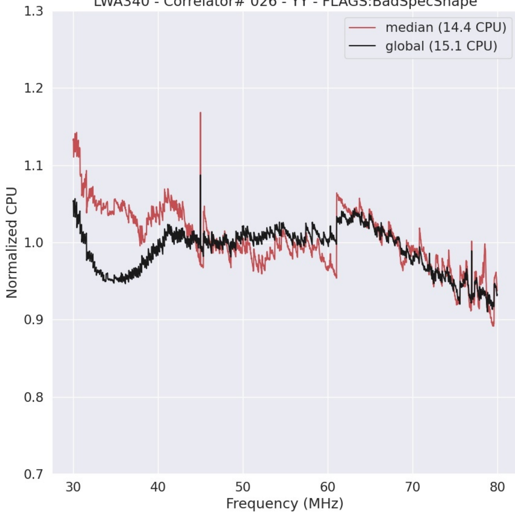
LWA340 - Correlator# 026 - YY - FLAGS:BadSpecShape
