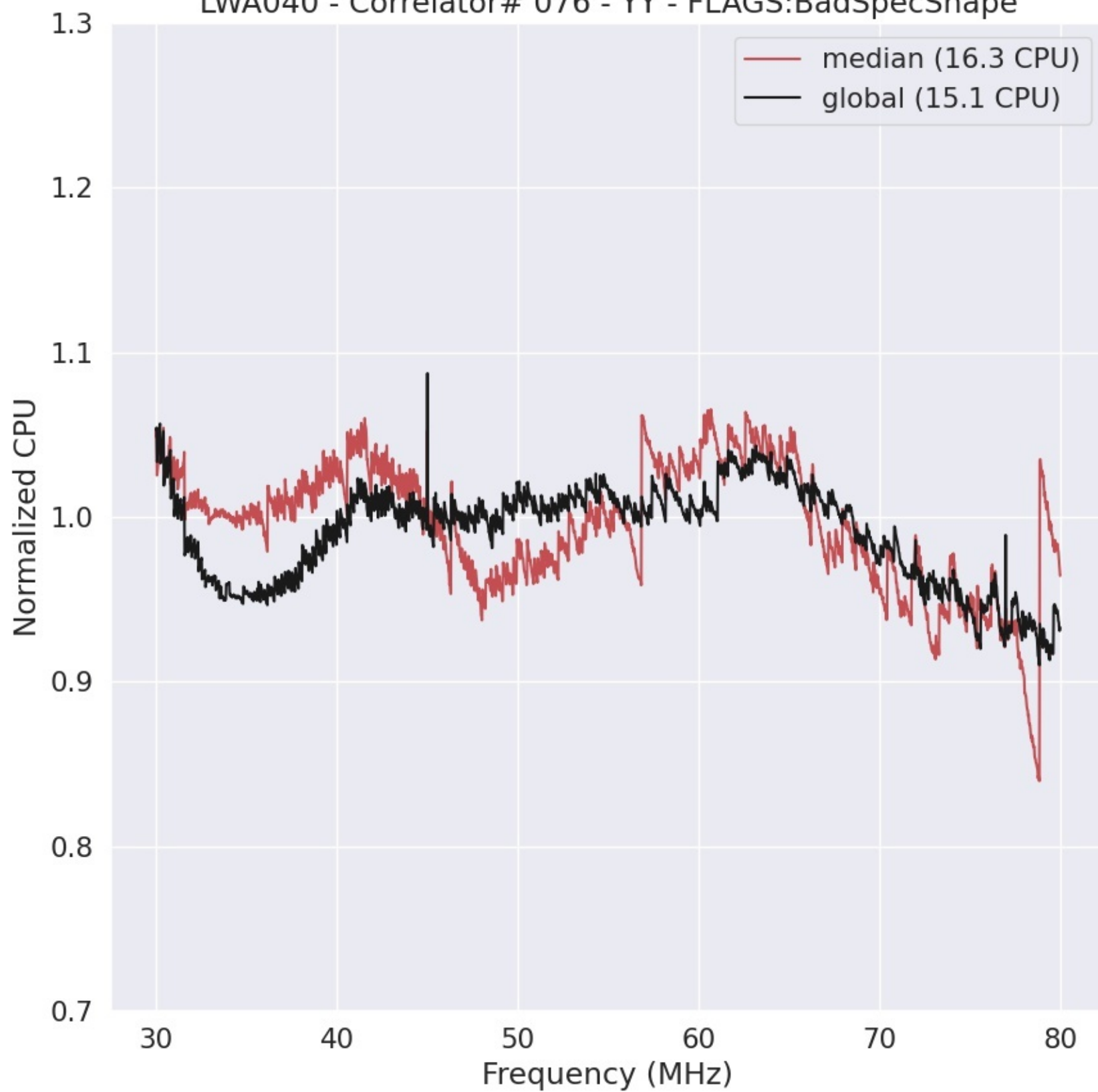
LWA040 - Correlator# 076 - YY - FLAGS:BadSpecShape
