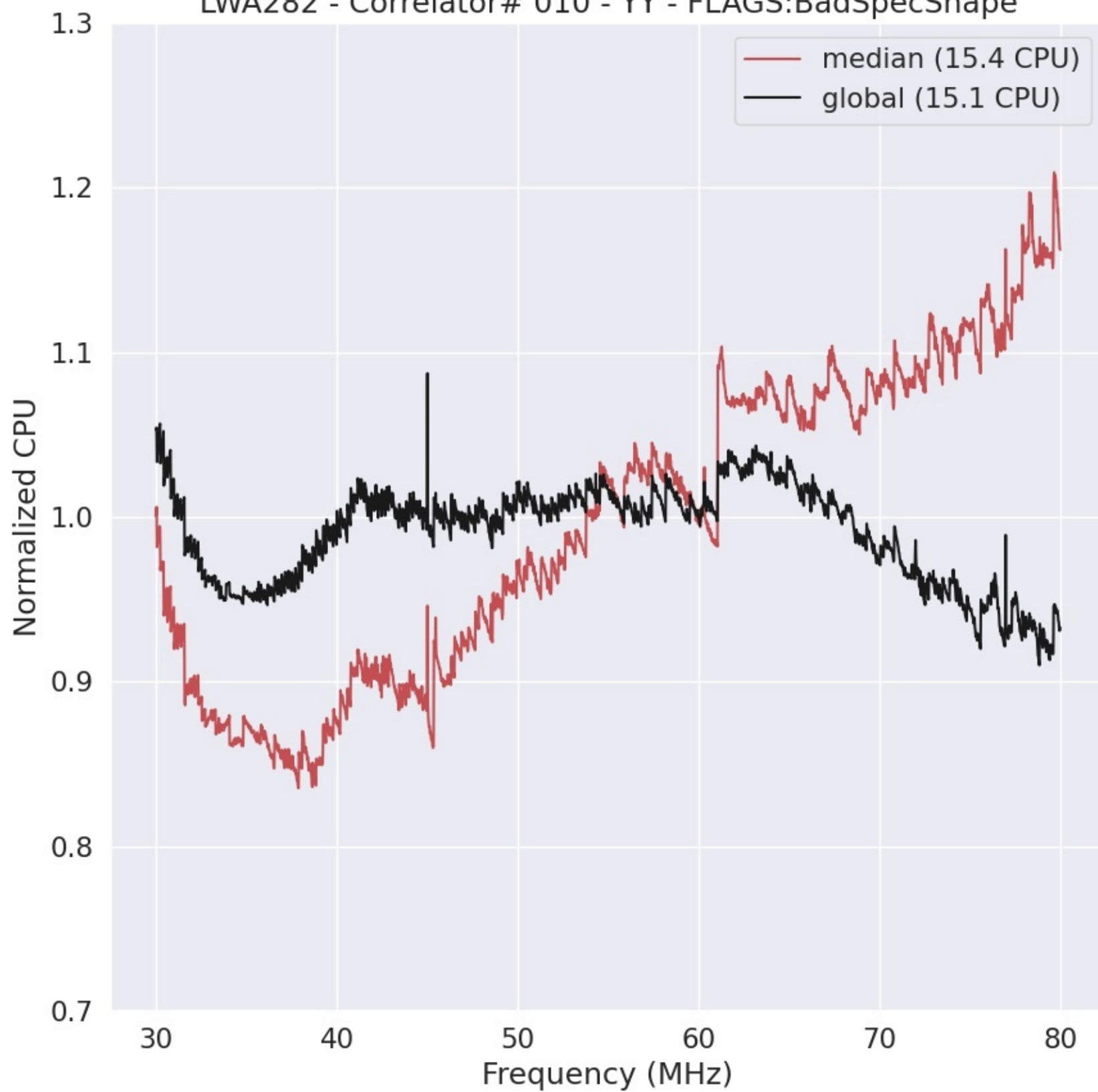
LWA282 - Correlator# 010 - YY - FLAGS:BadSpecShape
