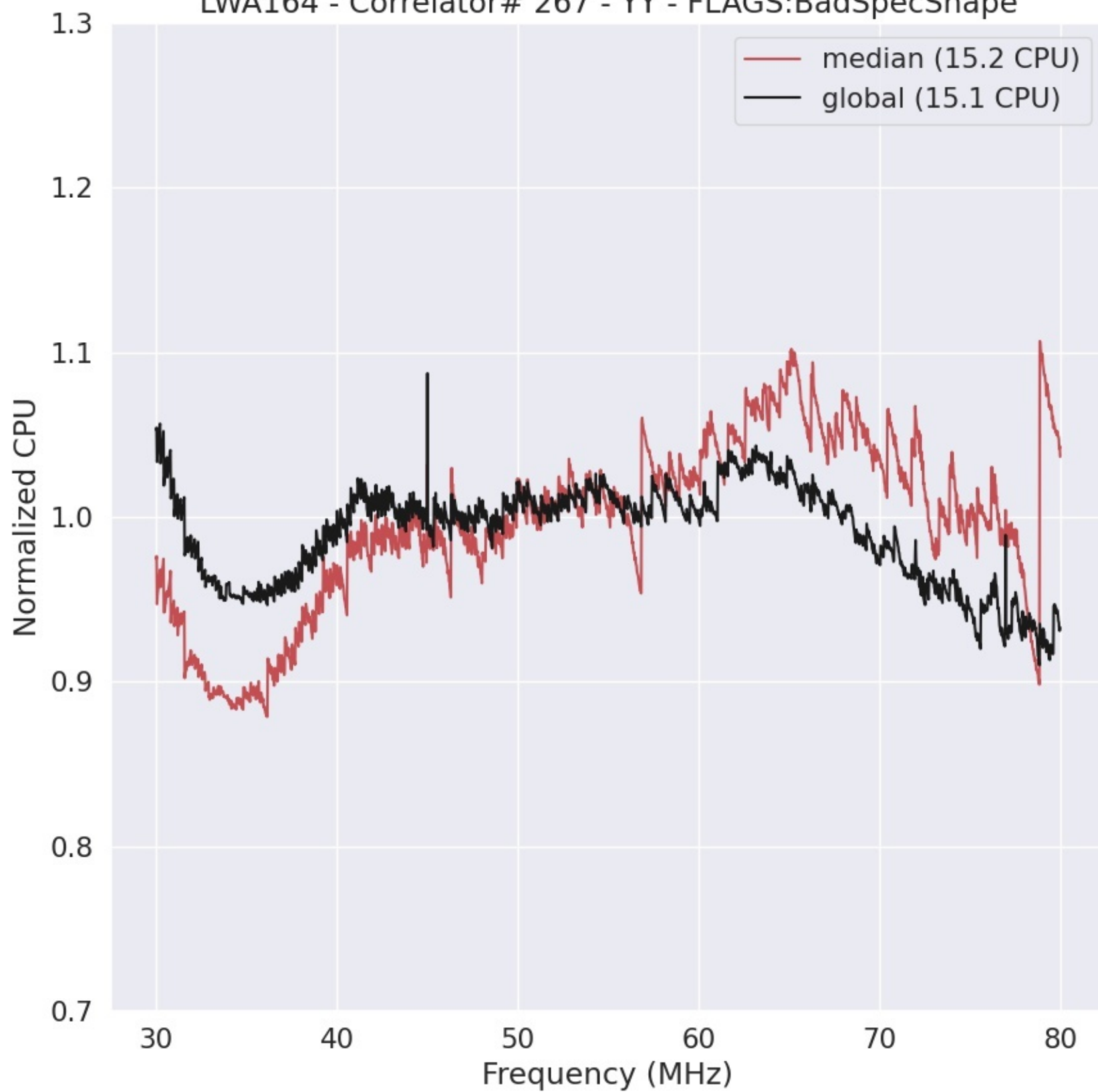
LWA164 - Correlator# 267 - YY - FLAGS:BadSpecShape
