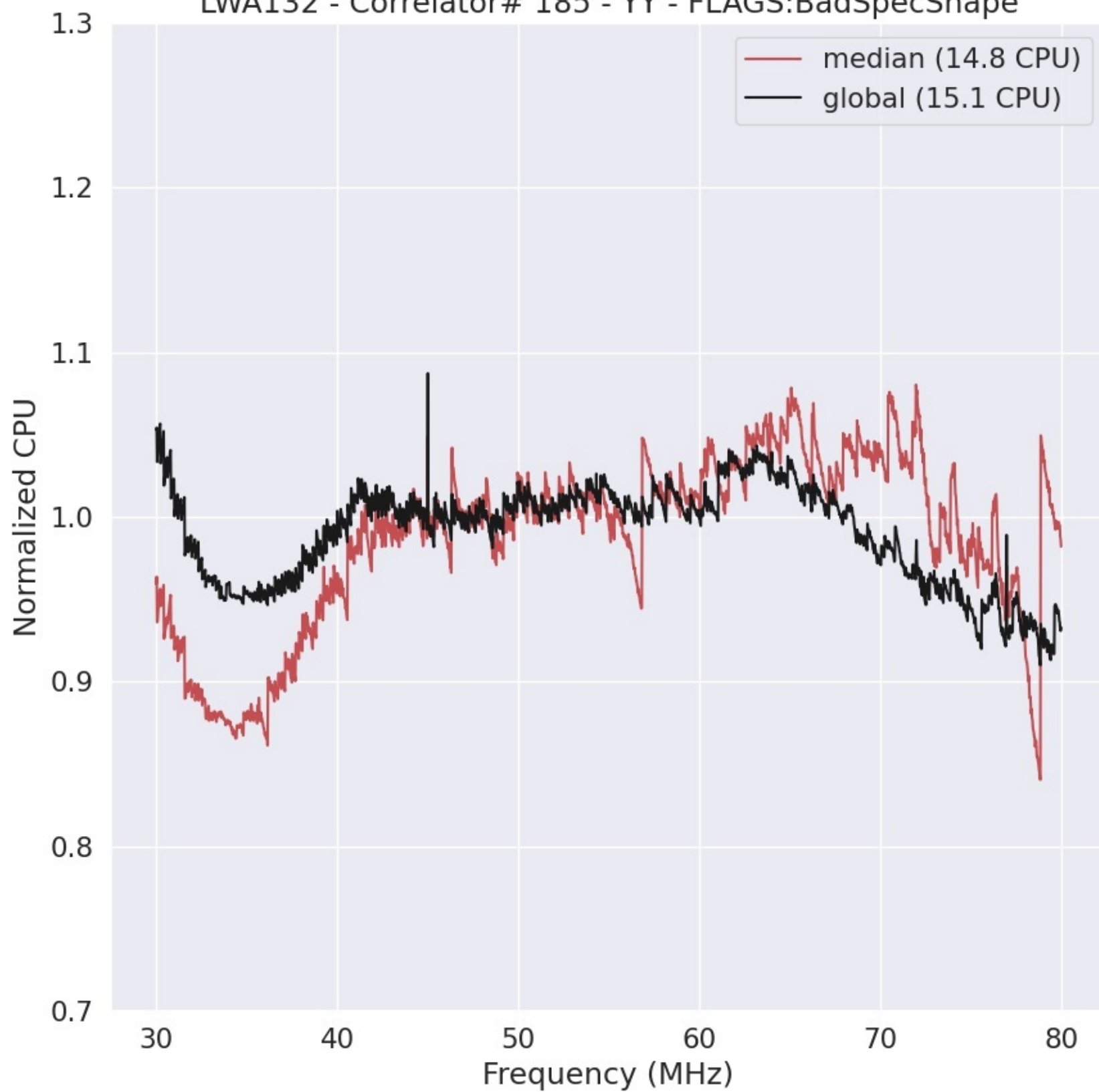
LWA132 - Correlator# 185 - YY - FLAGS:BadSpecShape
