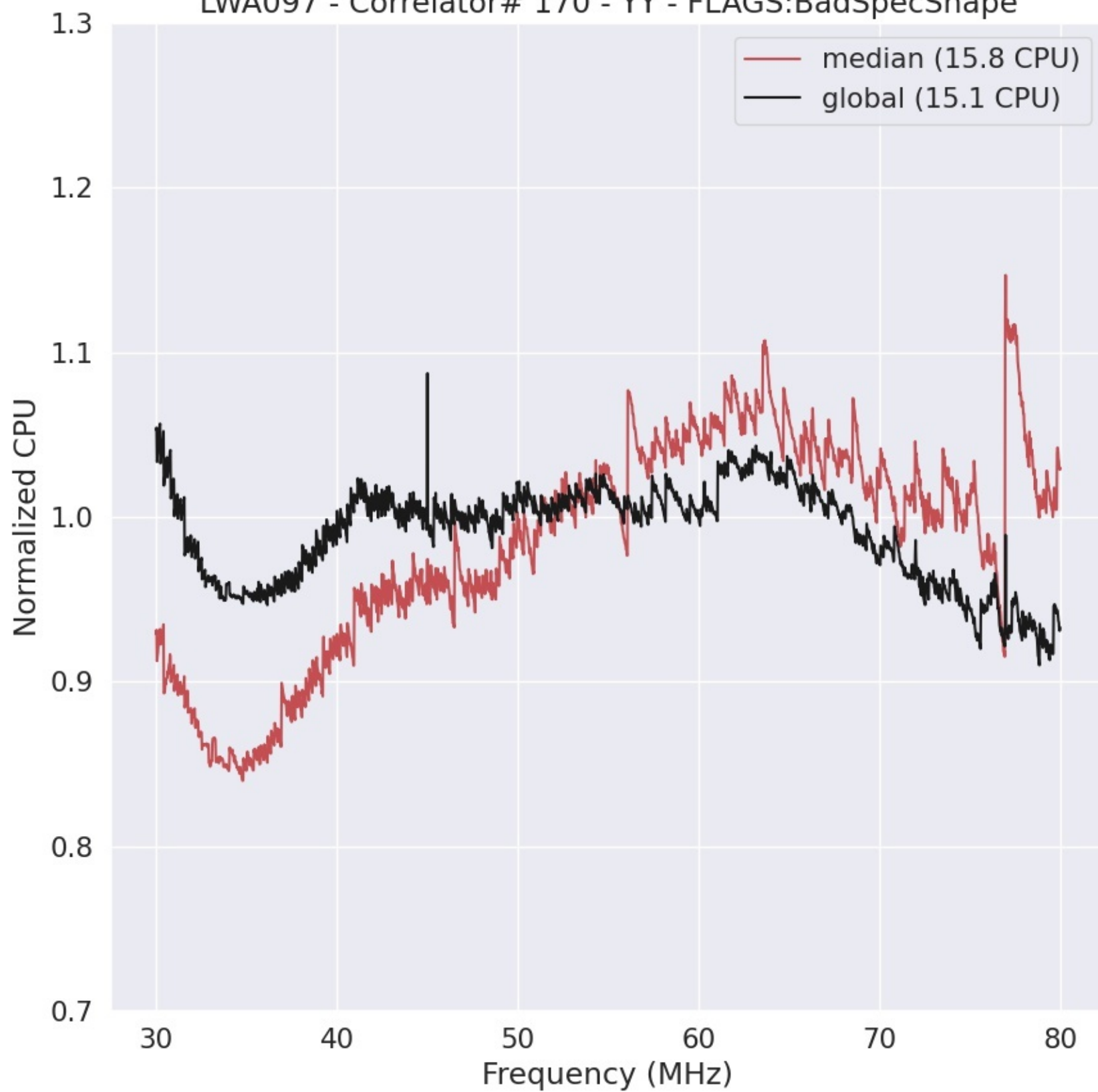
LWA097 - Correlator# 170 - YY - FLAGS:BadSpecShape
