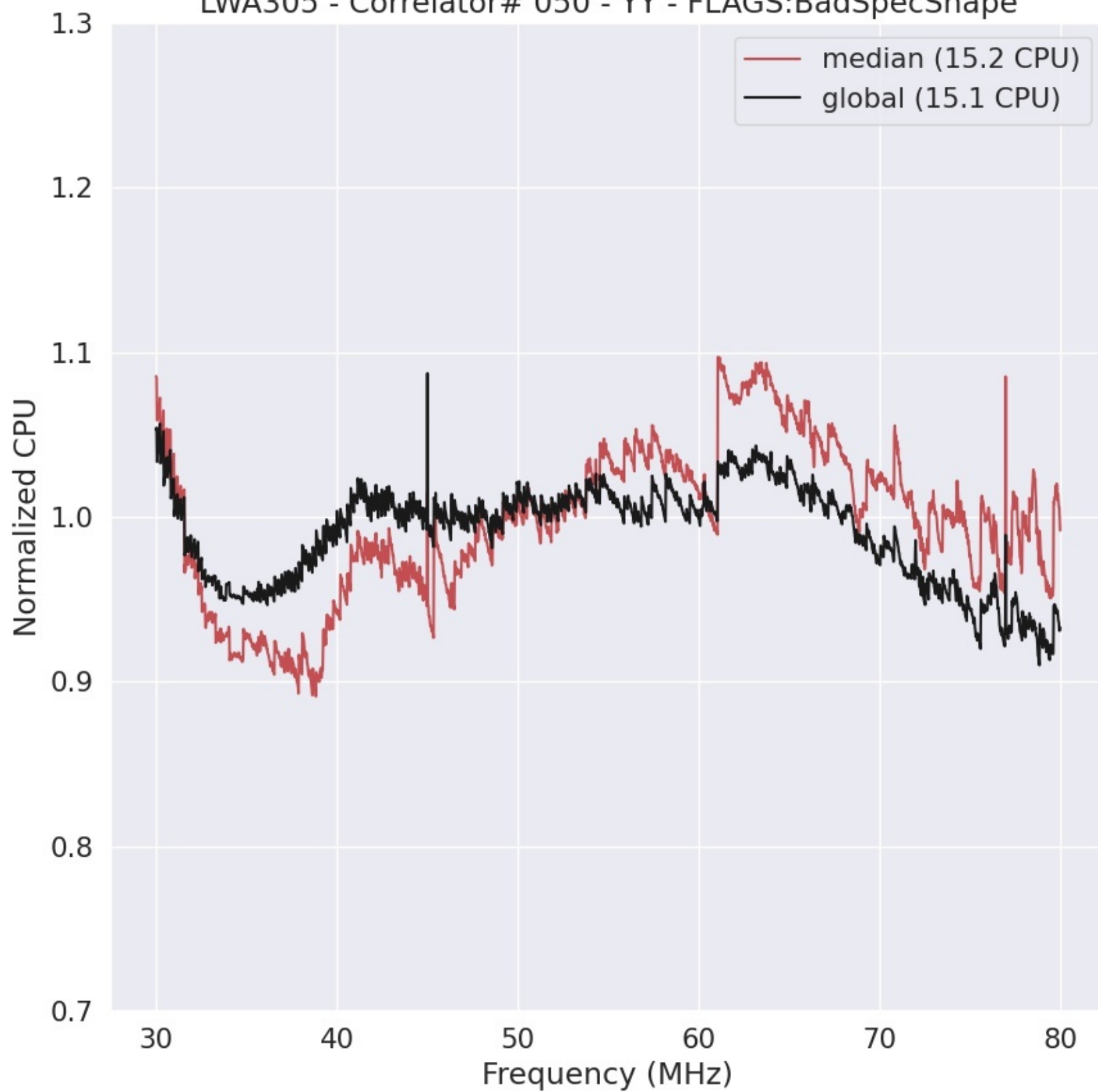
LWA305 - Correlator# 050 - YY - FLAGS:BadSpecShape
