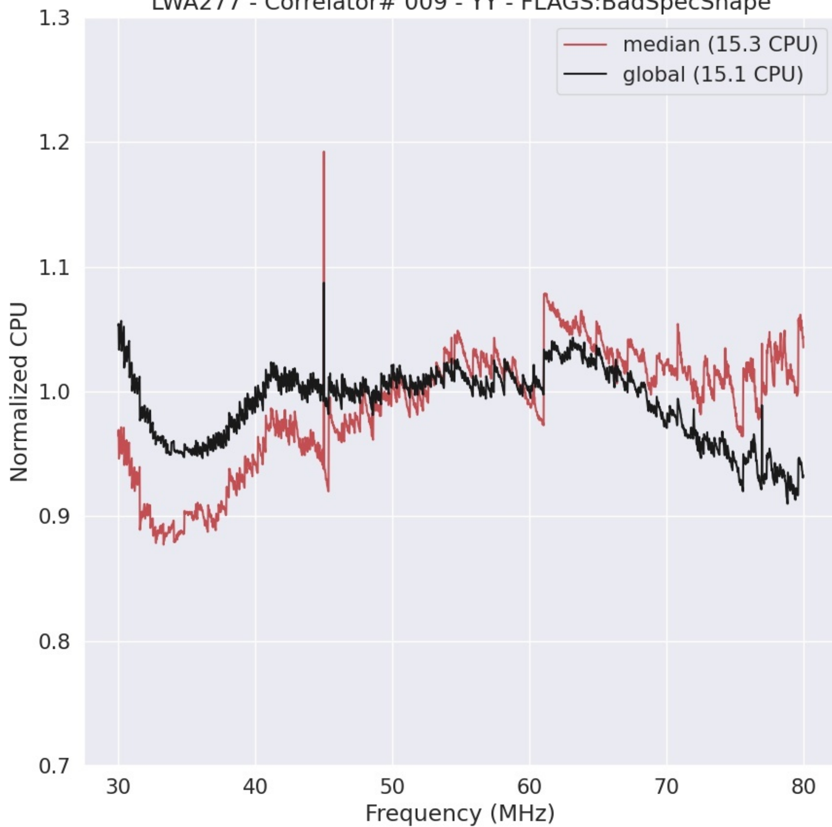
LWA277 - Correlator# 009 - YY - FLAGS:BadSpecShape
