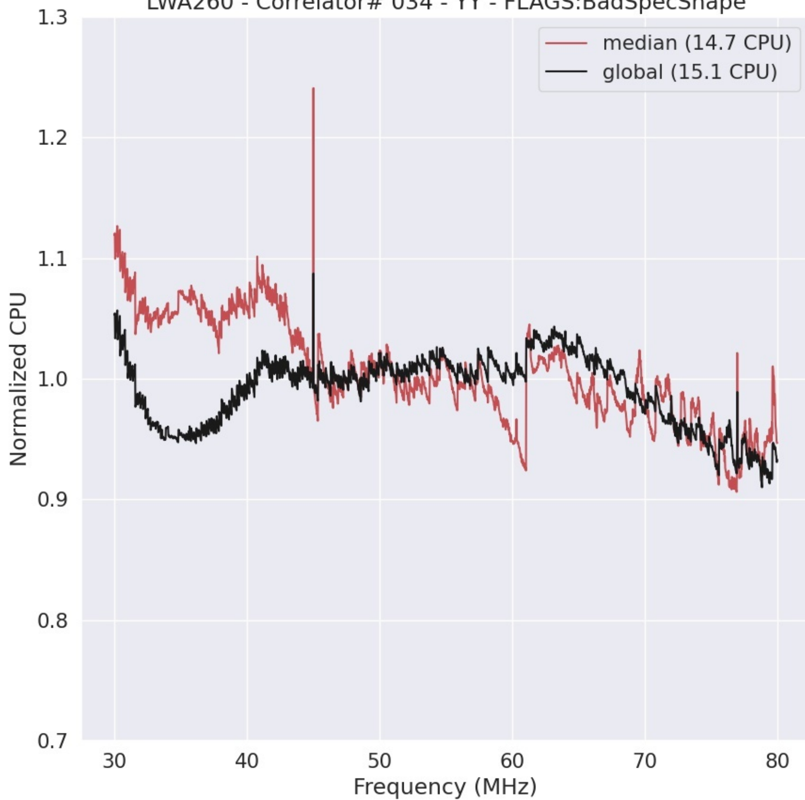
LWA260 - Correlator# 034 - YY - FLAGS:BadSpecShape
