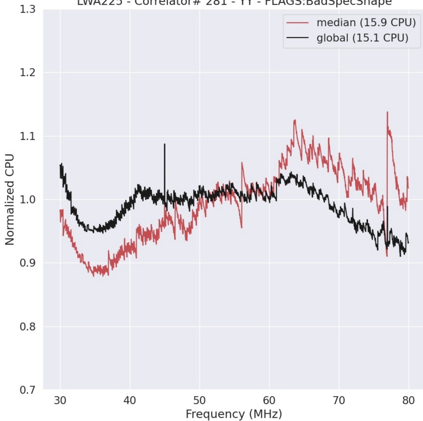
LWA225 - Correlator# 281 - YY - FLAGS:BadSpecShape
