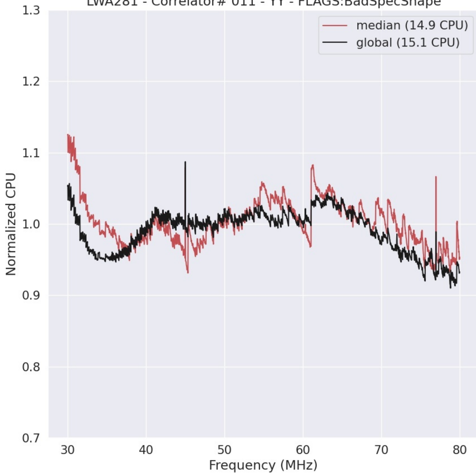
LWA281 - Correlator# 011 - YY - FLAGS:BadSpecShape
