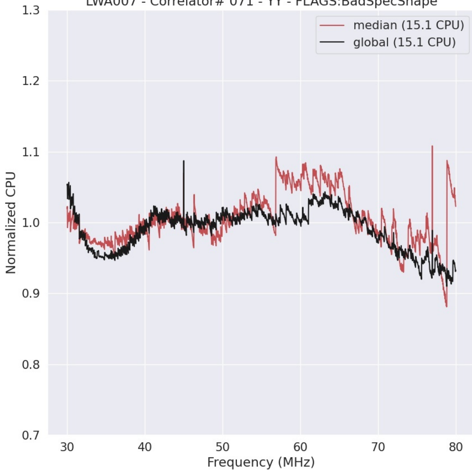
LWA007 - Correlator# 071 - YY - FLAGS:BadSpecShape
