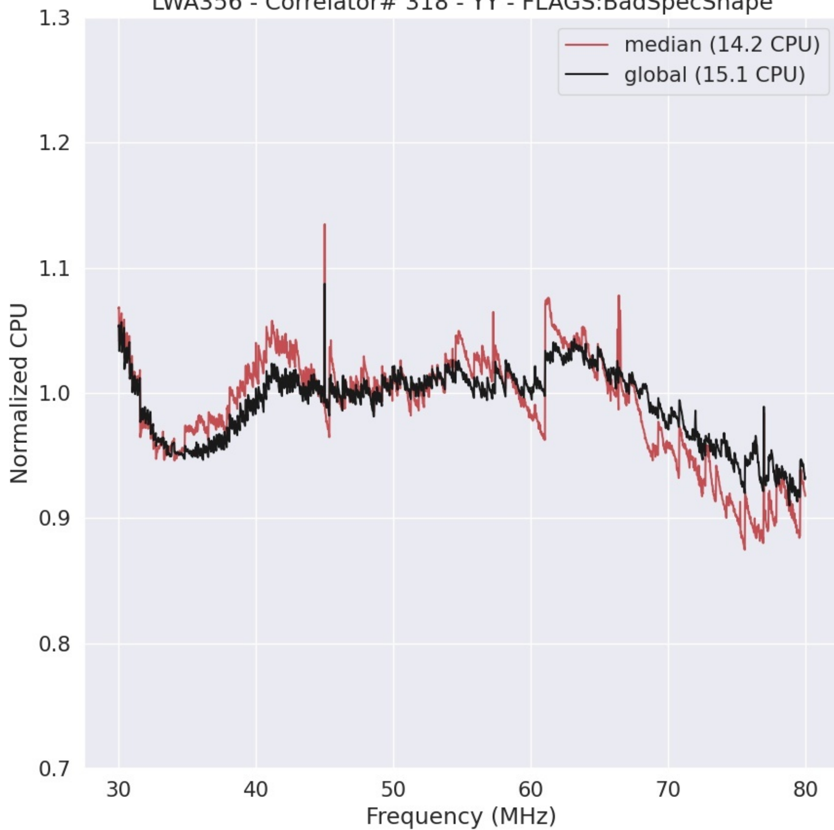
LWA356 - Correlator# 318 - YY - FLAGS:BadSpecShape
