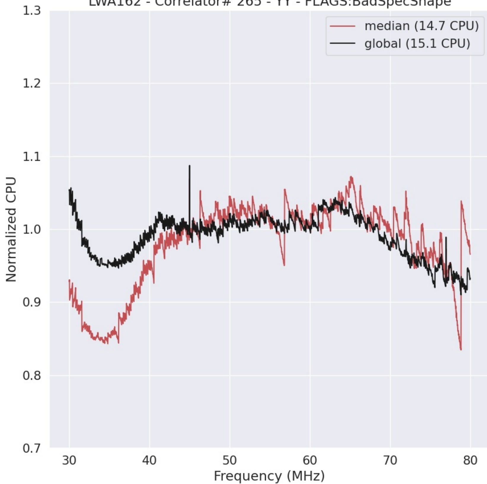
LWA162 - Correlator# 265 - YY - FLAGS:BadSpecShape
