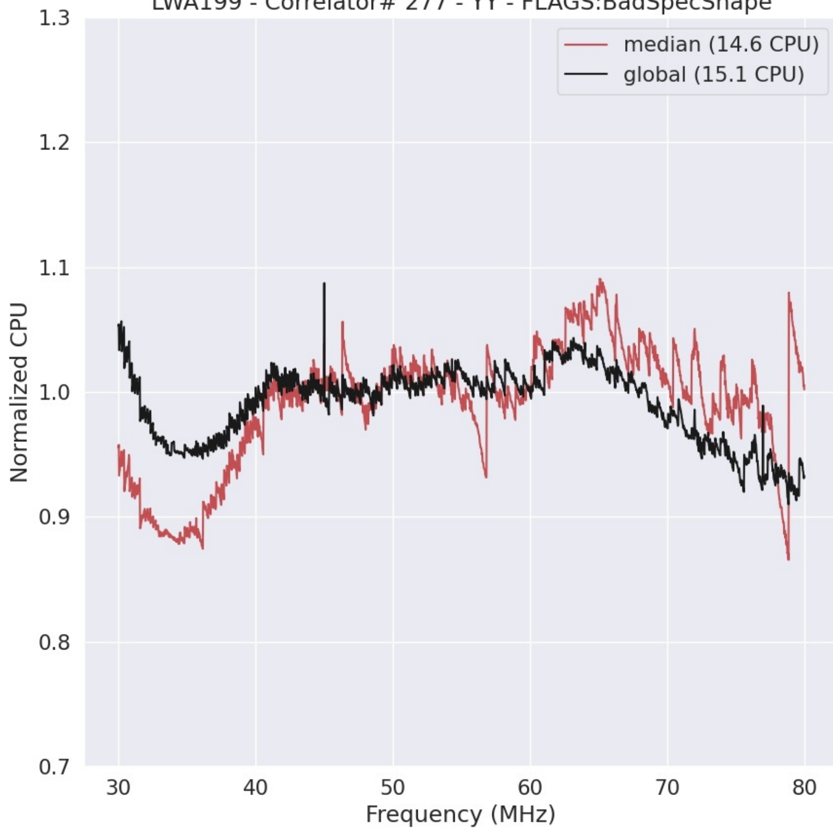
LWA199 - Correlator# 277 - YY - FLAGS:BadSpecShape
