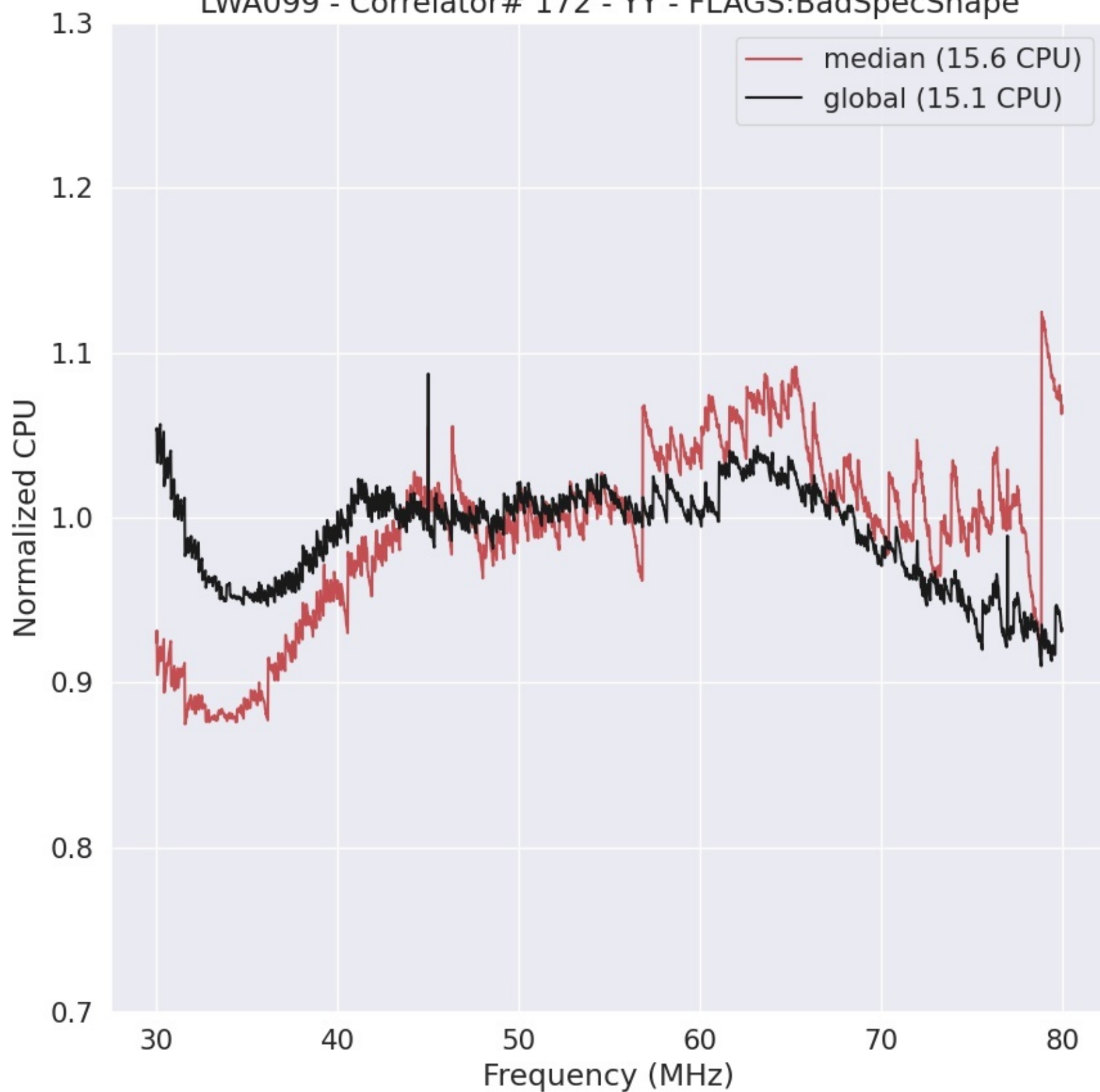
LWA099 - Correlator# 172 - YY - FLAGS:BadSpecShape
