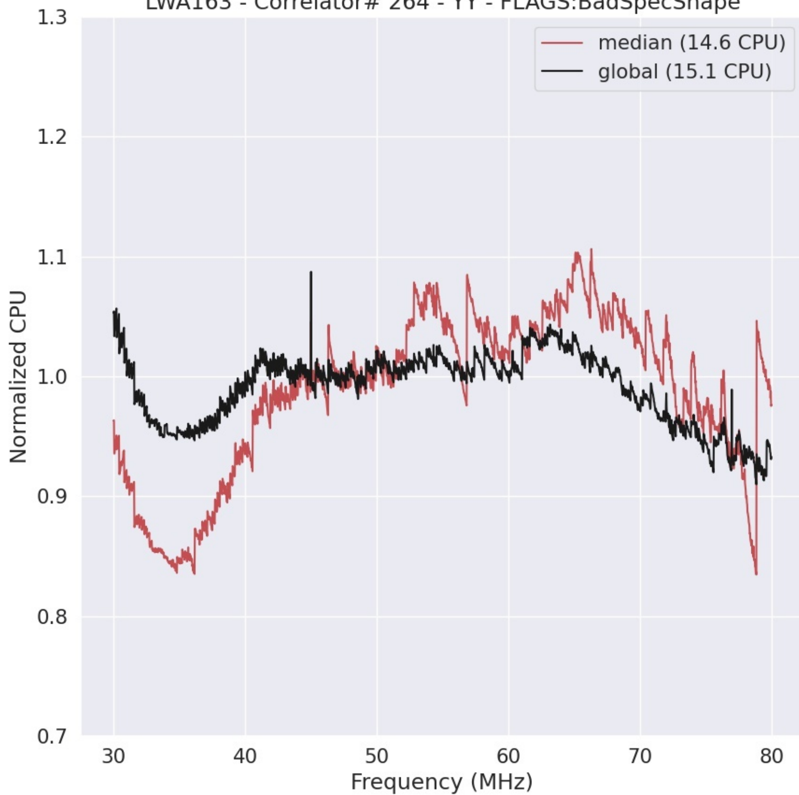
LWA163 - Correlator# 264 - YY - FLAGS:BadSpecShape
