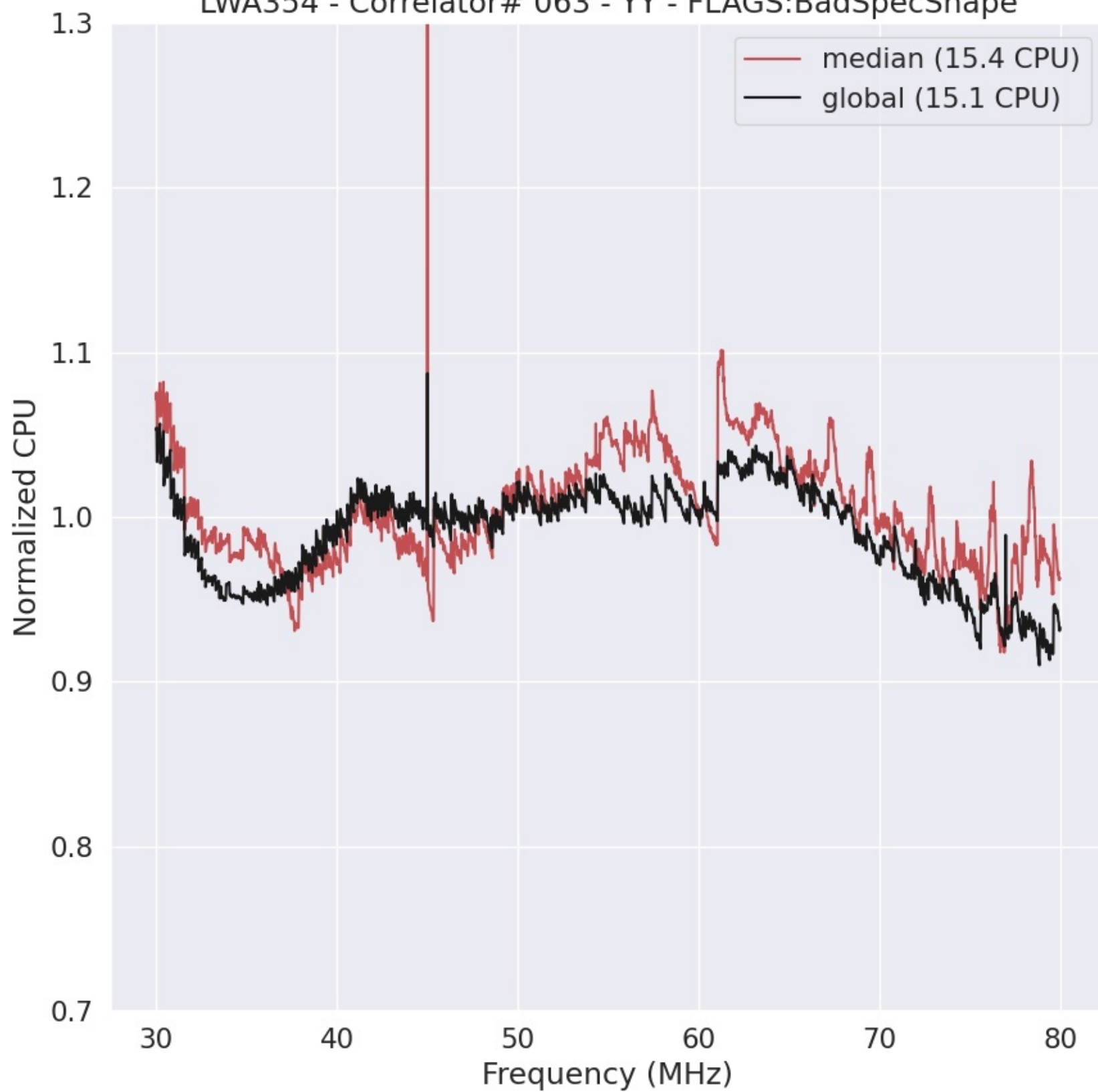
LWA354 - Correlator# 063 - YY - FLAGS:BadSpecShape
