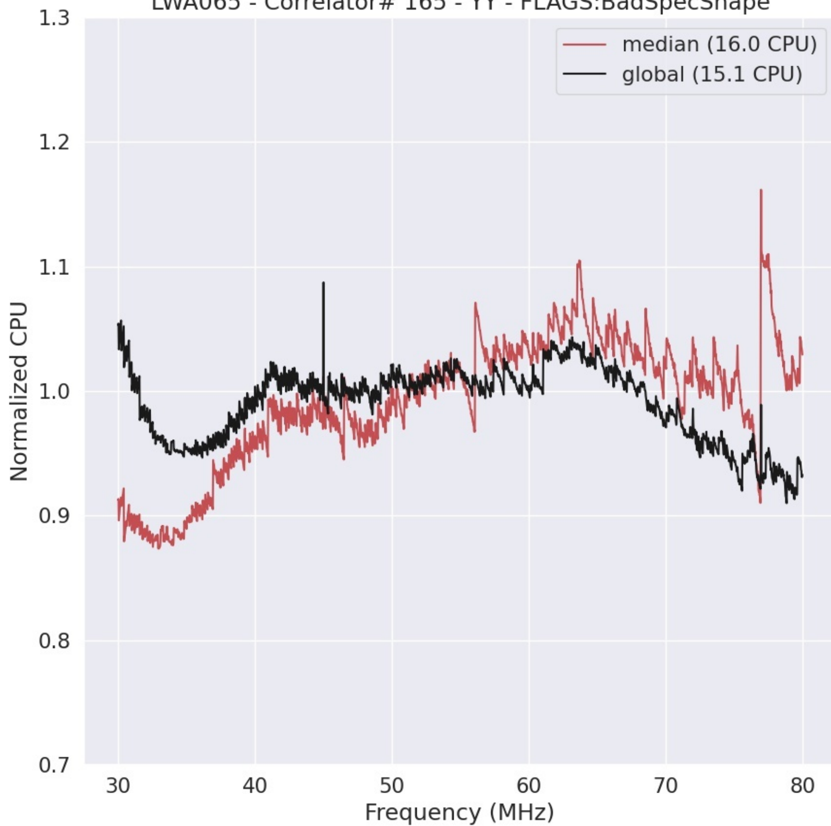
LWA065 - Correlator# 165 - YY - FLAGS:BadSpecShape
