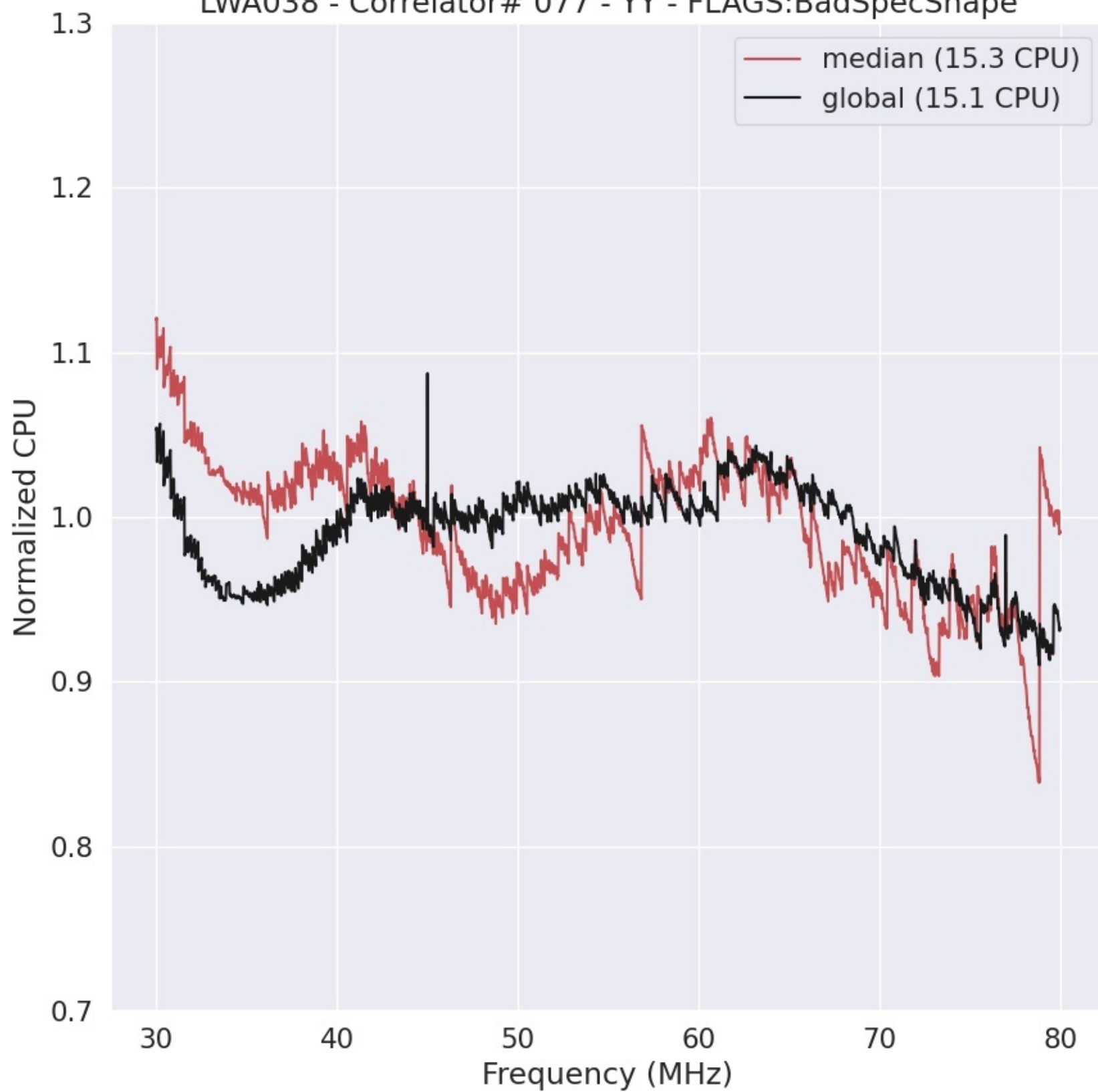
LWA038 - Correlator# 077 - YY - FLAGS:BadSpecShape
