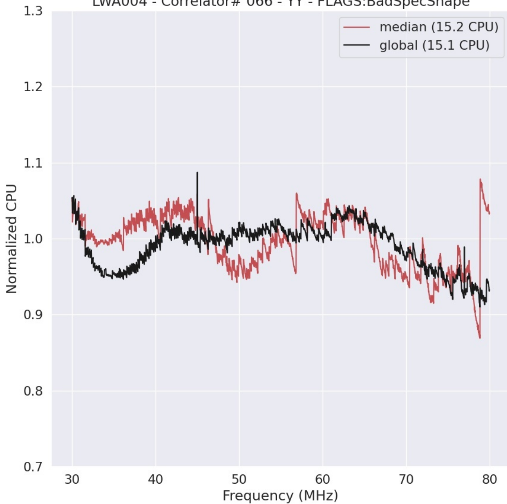
LWA004 - Correlator# 066 - YY - FLAGS:BadSpecShape
