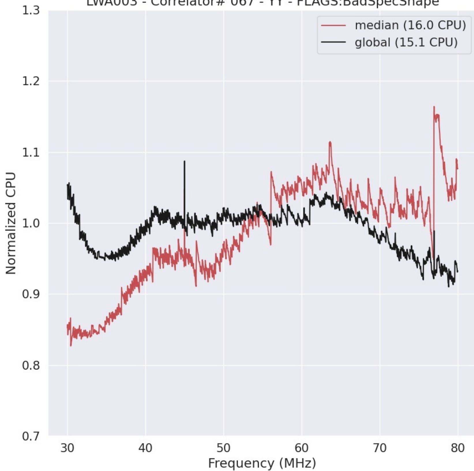
LWA003 - Correlator# 067 - YY - FLAGS:BadSpecShape
