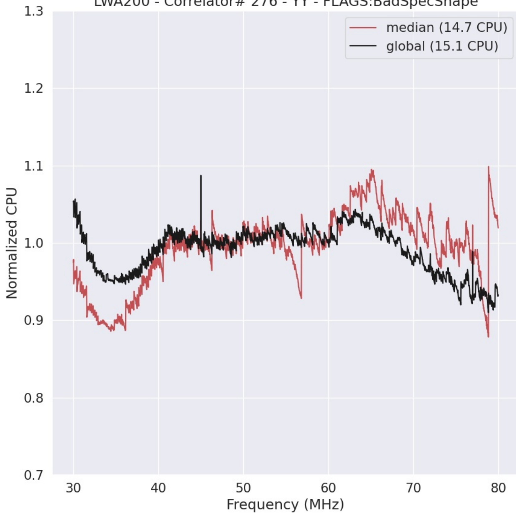
LWA200 - Correlator# 276 - YY - FLAGS:BadSpecShape
