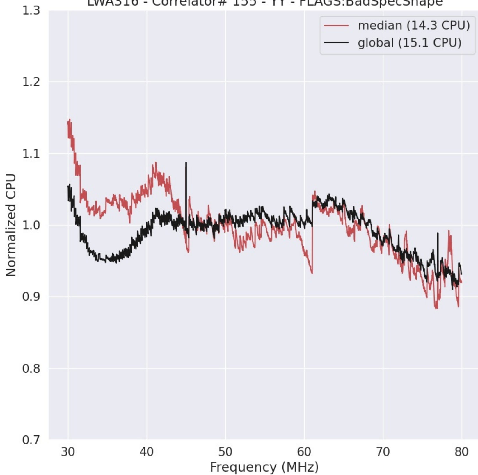
LWA316 - Correlator# 155 - YY - FLAGS:BadSpecShape
