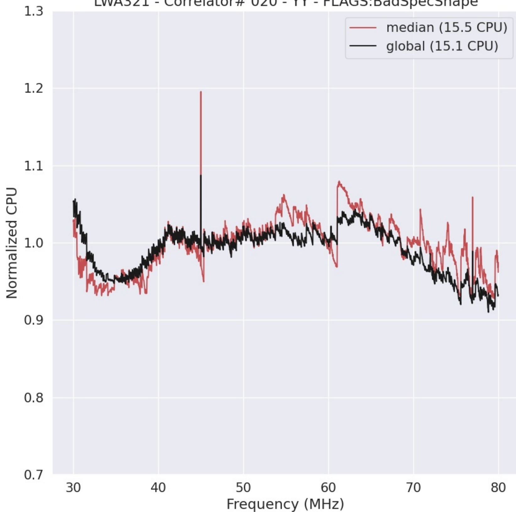
LWA321 - Correlator# 020 - YY - FLAGS:BadSpecShape
