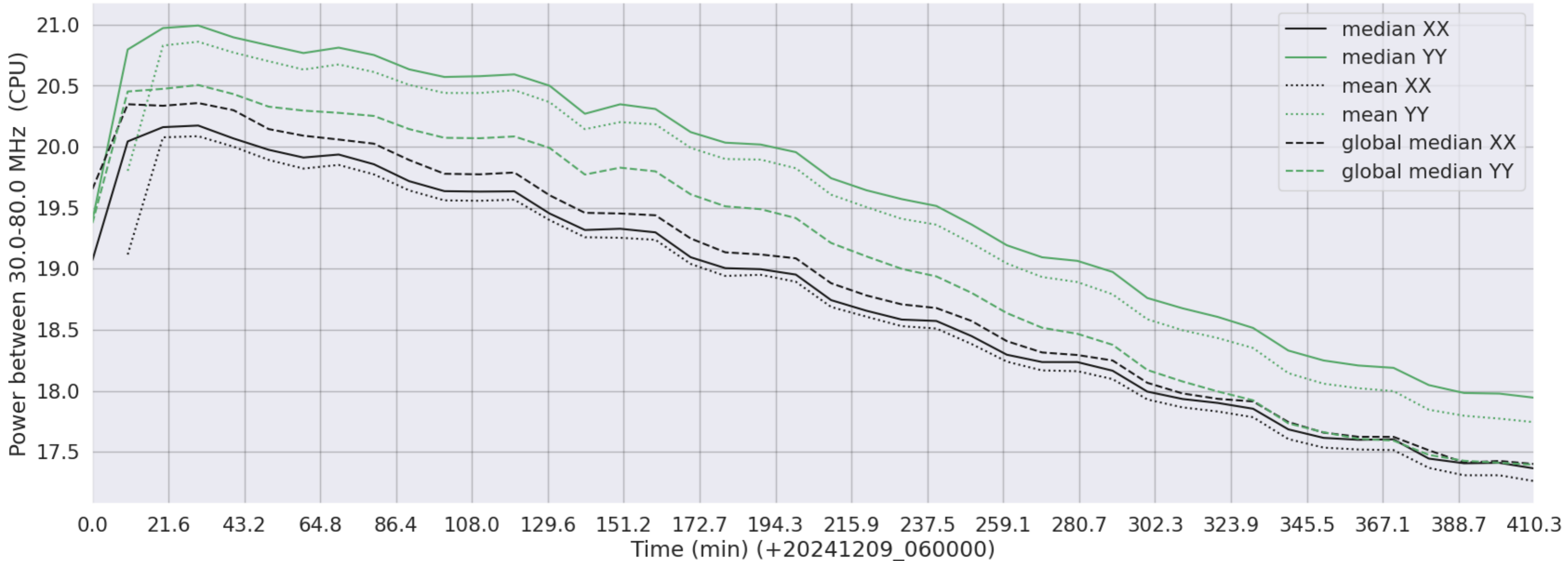
LWA013 - Correlator# 096 - XX FLAGS:Good - YY FLAGS:BadSpecShape
