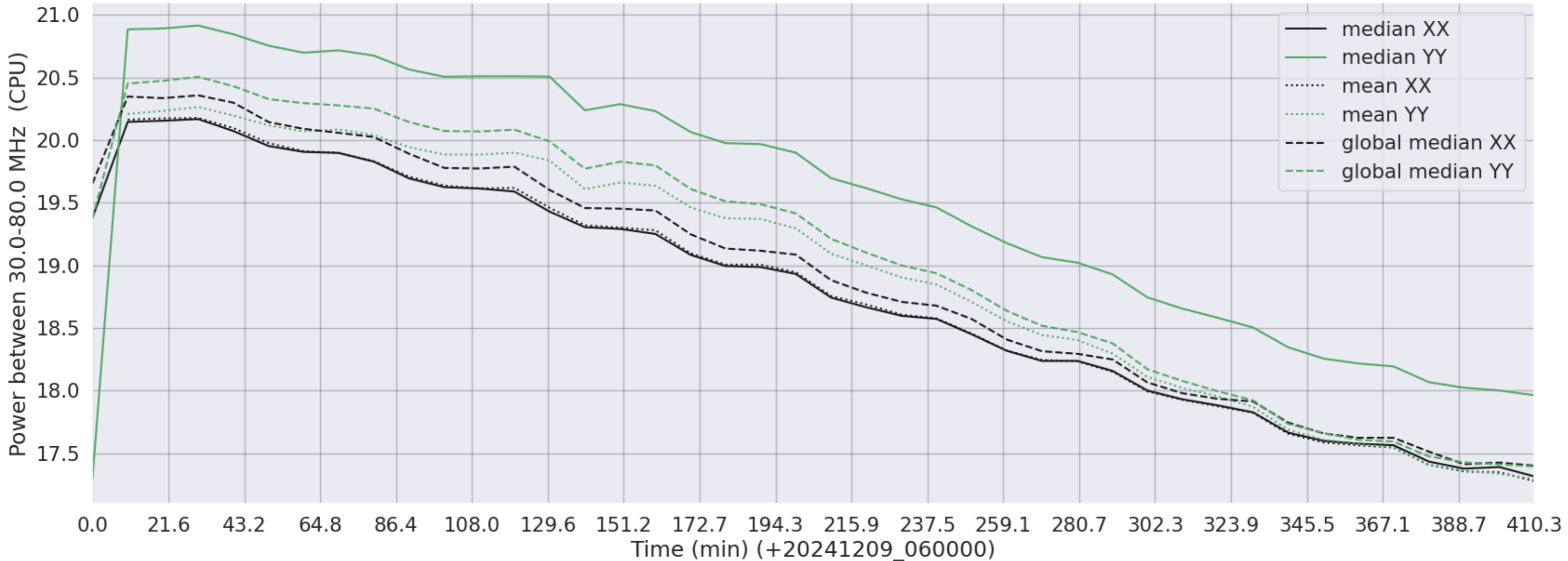
LWA138 - Correlator# 261 - XX FLAGS:Good - YY FLAGS:BadSpecShape
