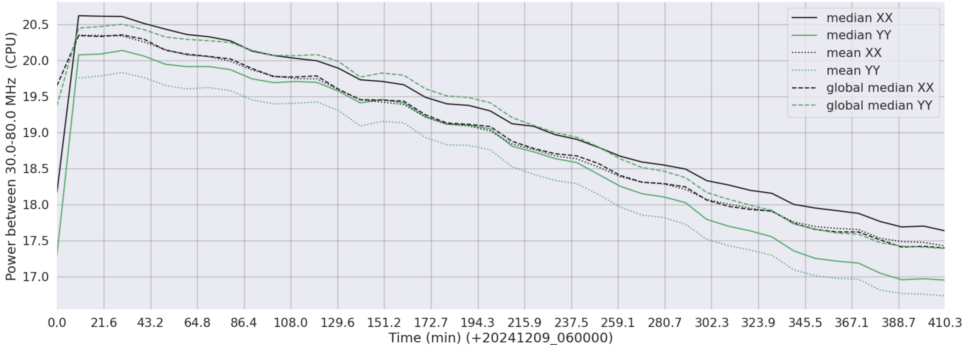
LWA144 - Correlator# 213 - XX FLAGS:Good - YY FLAGS:BadSpecShape
