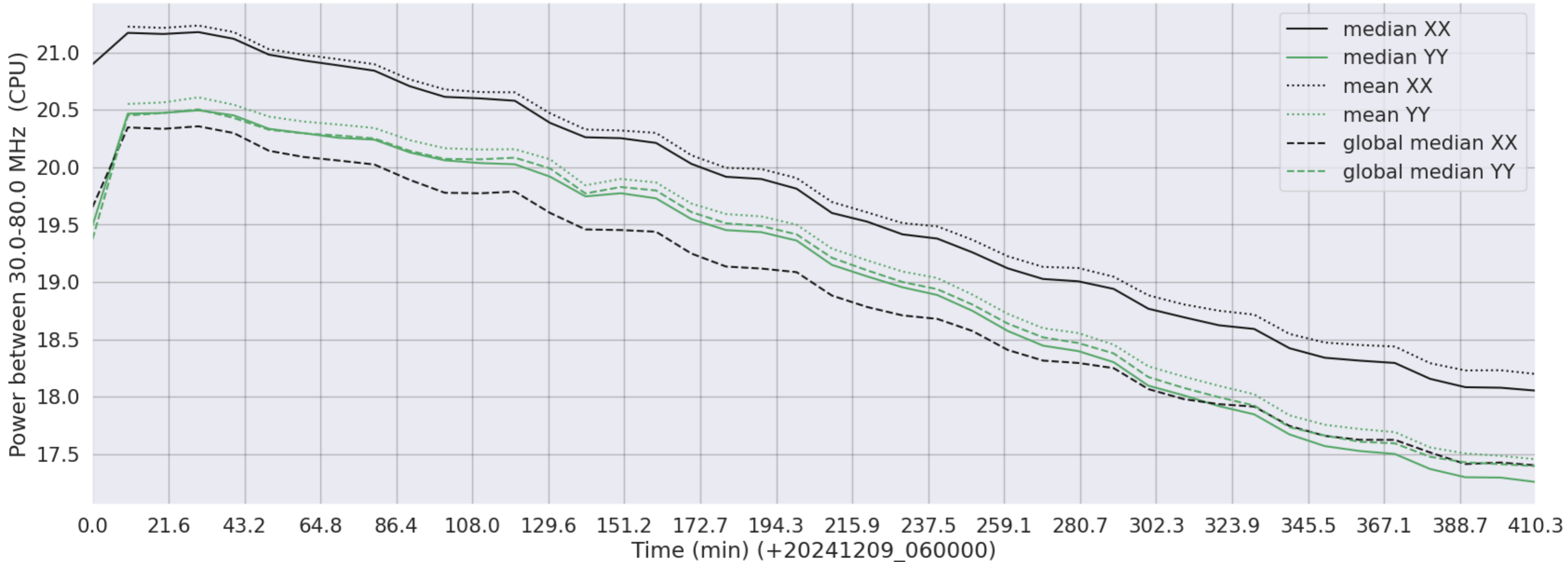
LWA234 - Correlator# 289 - XX FLAGS:Good - YY FLAGS:BadSpecShape
