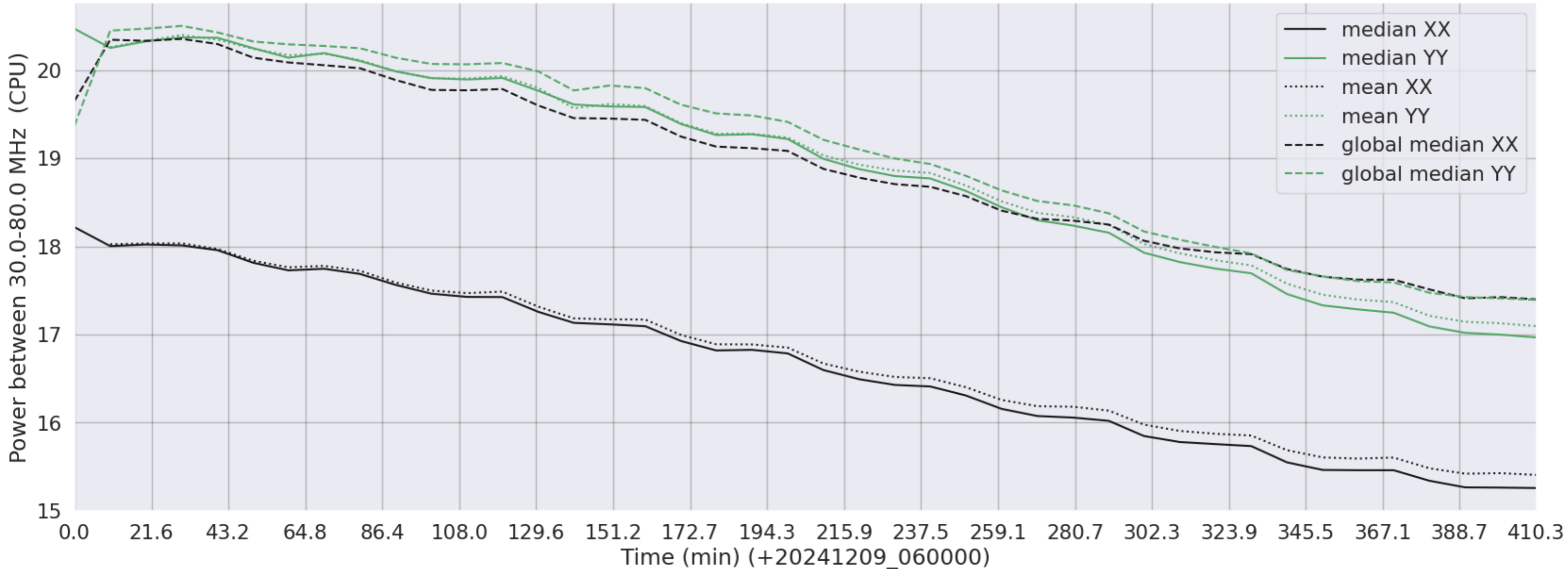
LWA046 - Correlator# 082 - XX FLAGS:BadSpecShape - YY FLAGS:BadSpecShape
