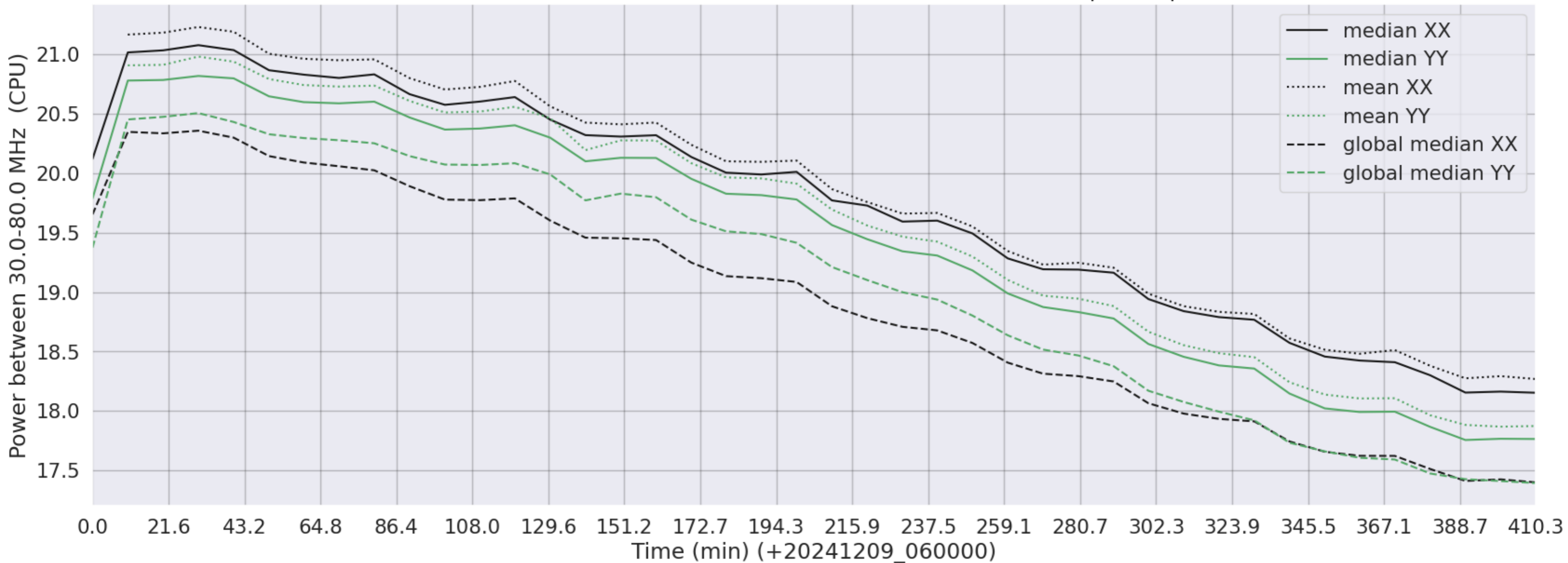
LWA242 - Correlator# 339 - XX FLAGS:Good - YY FLAGS:BadSpecShape
