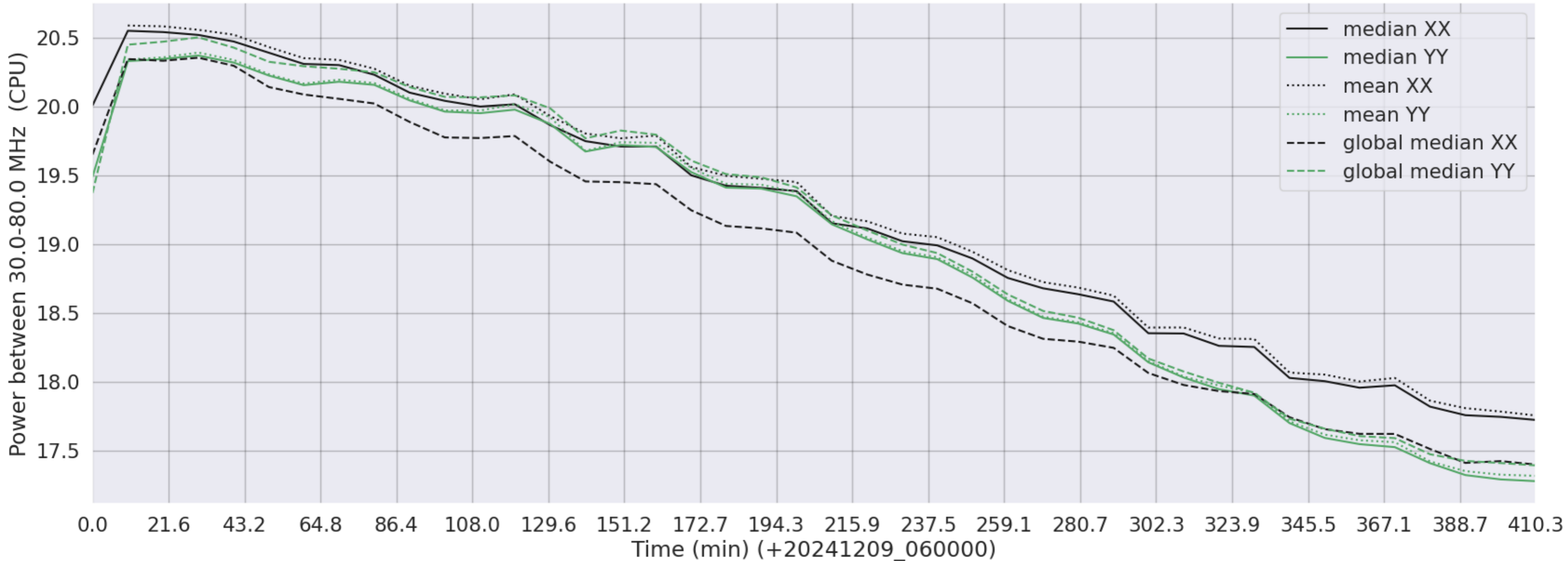
LWA105 - Correlator# 178 - XX FLAGS:Good - YY FLAGS:BadSpecShape
