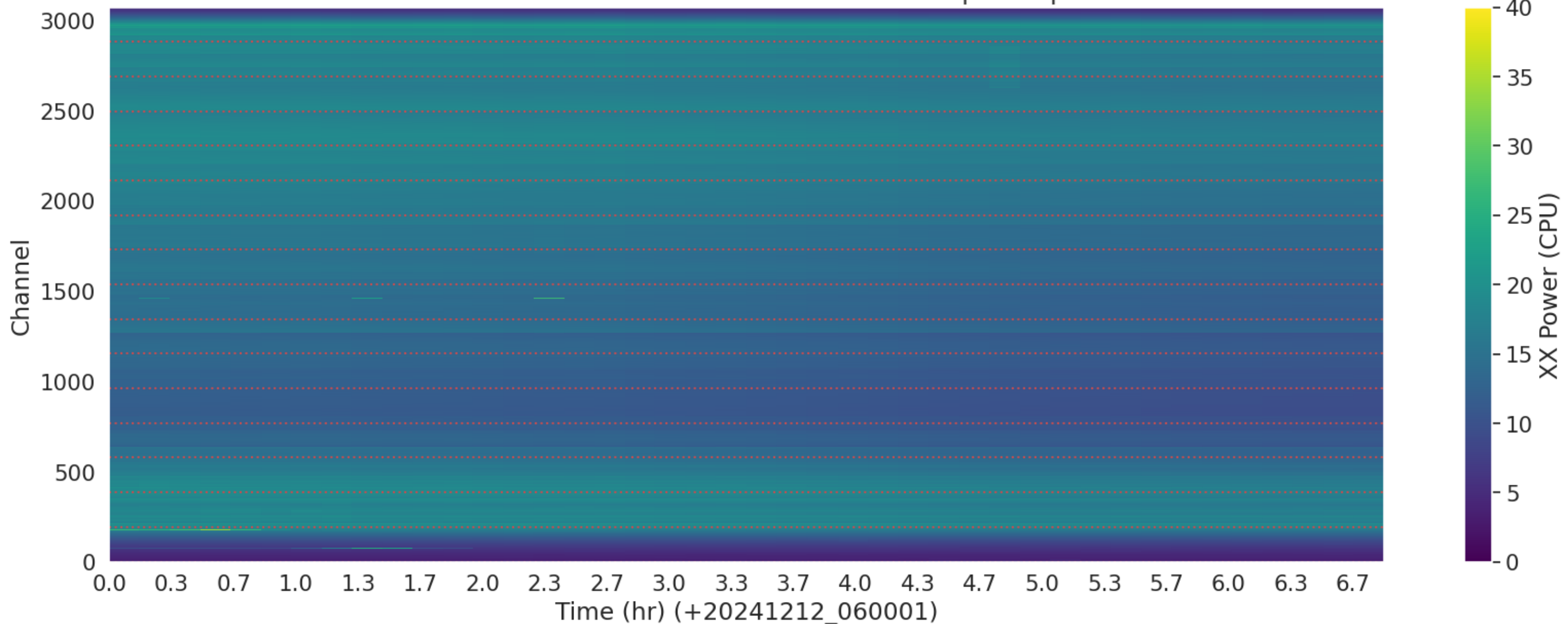
LWA363 - Correlator# 094 - XX - FLAGS: BadSpecShape
