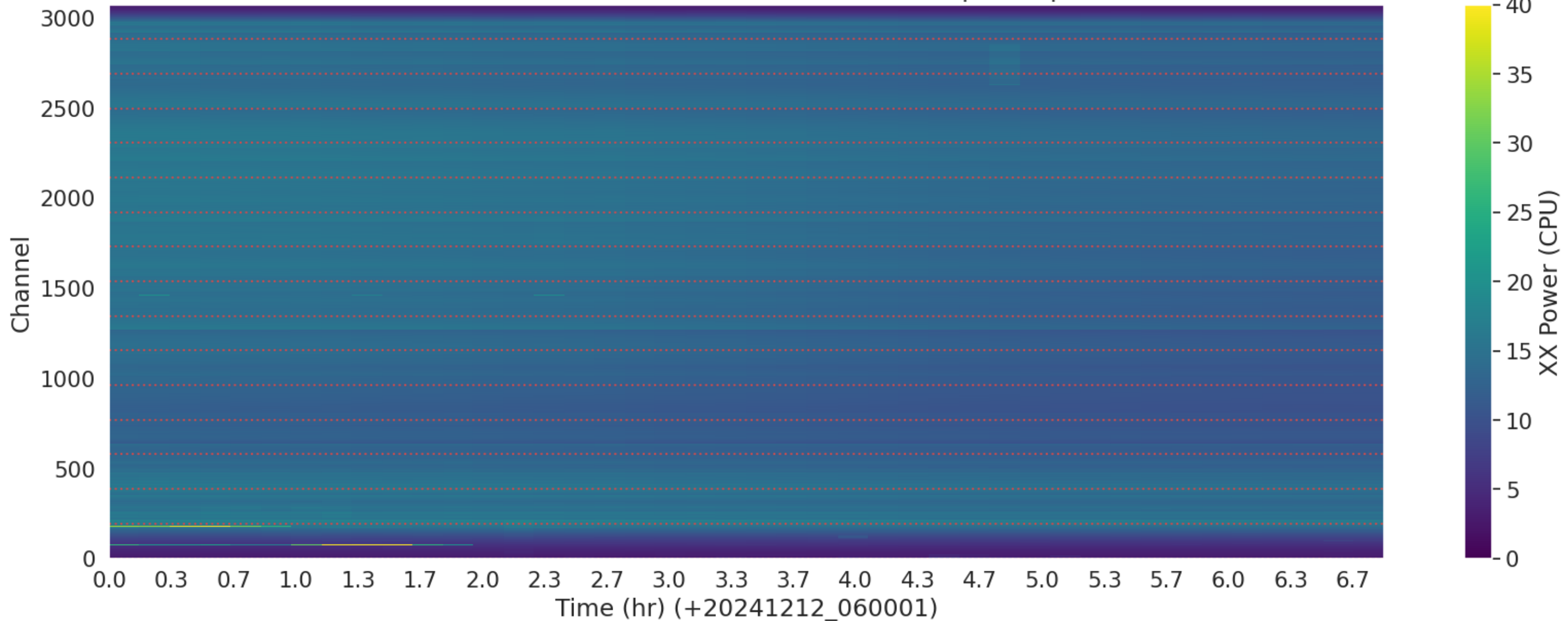
LWA314 - Correlator# 021 - XX - FLAGS: BadSpecShape
