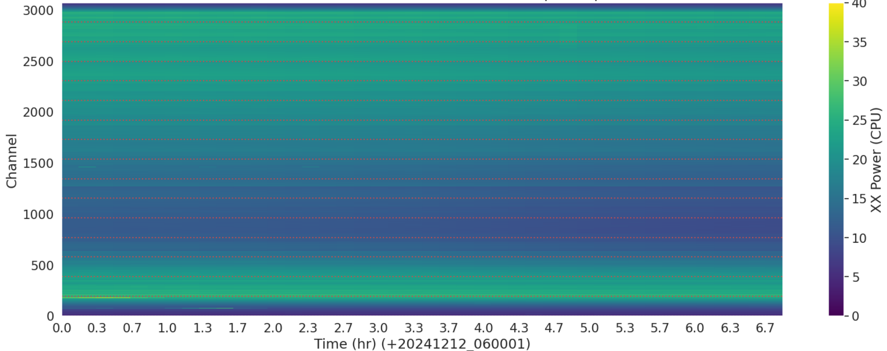
LWA313 - Correlator# 018 - XX - FLAGS: BadSpecShape
