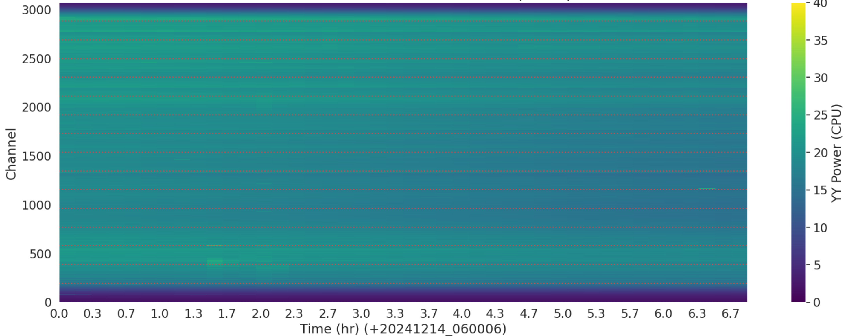
LWA239 - Correlator# 313 - YY - FLAGS: BadSpecShape
