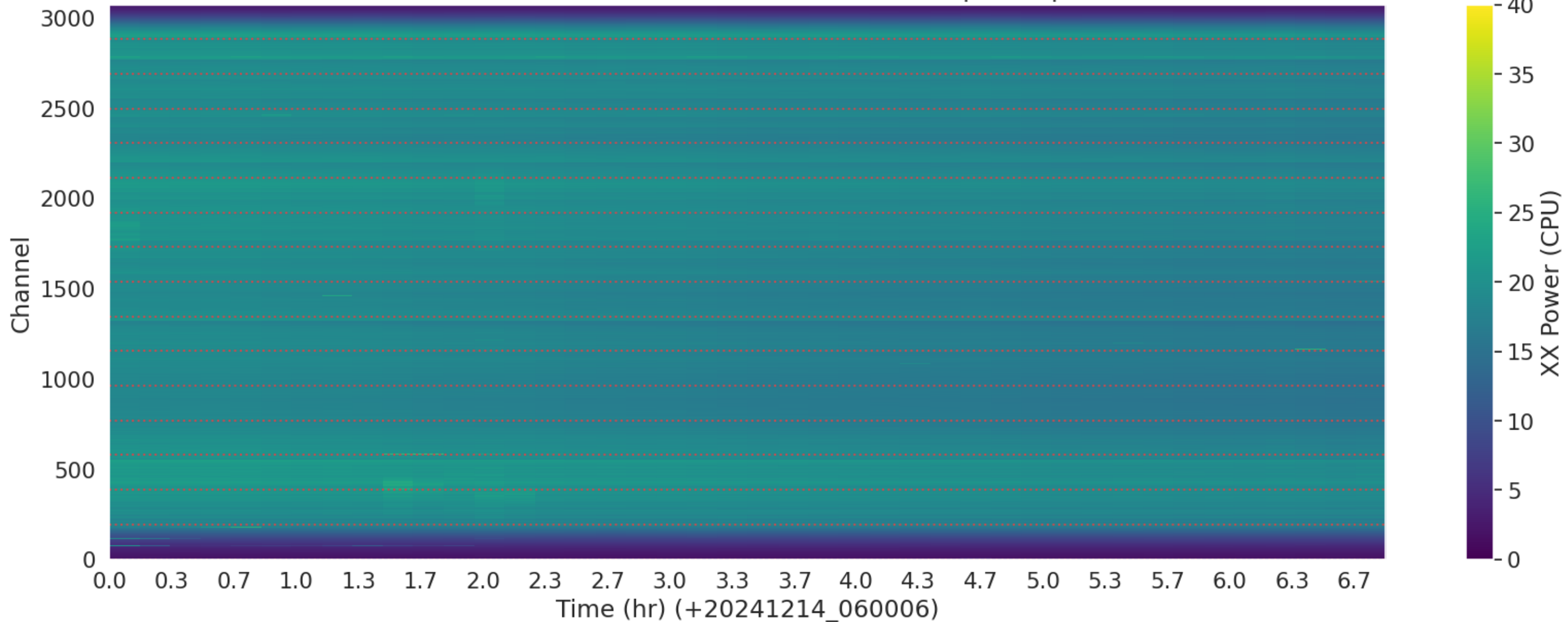
LWA074 - Correlator# 086 - XX - FLAGS: BadSpecShape
