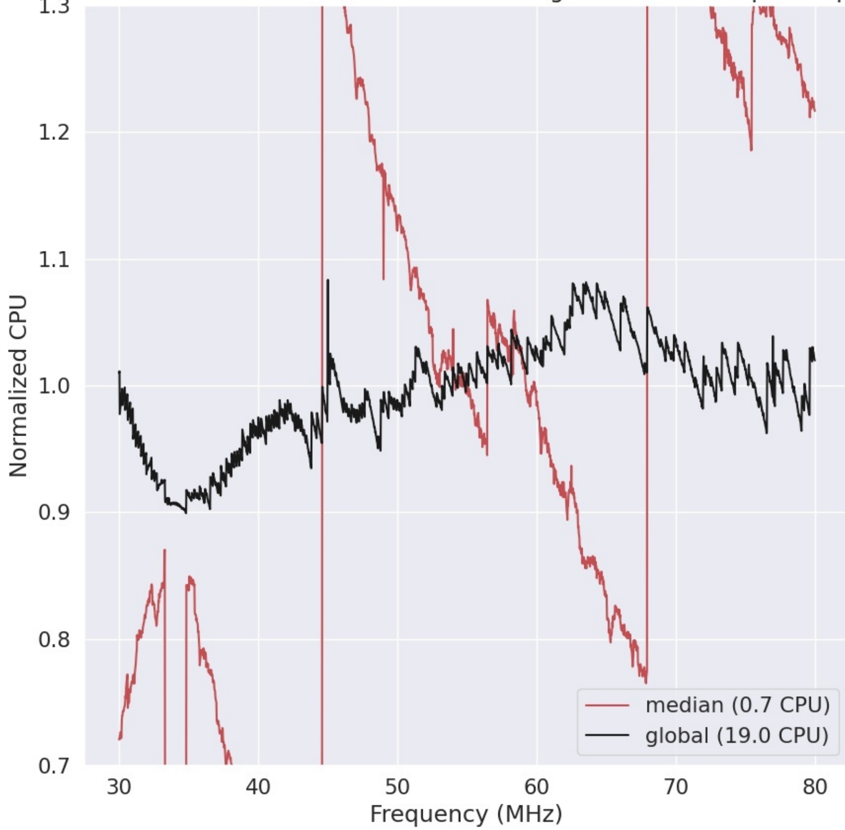
LWA244 - Correlator# 338 - YY - FLAGS:HighTimeVar+BadSpecShape
