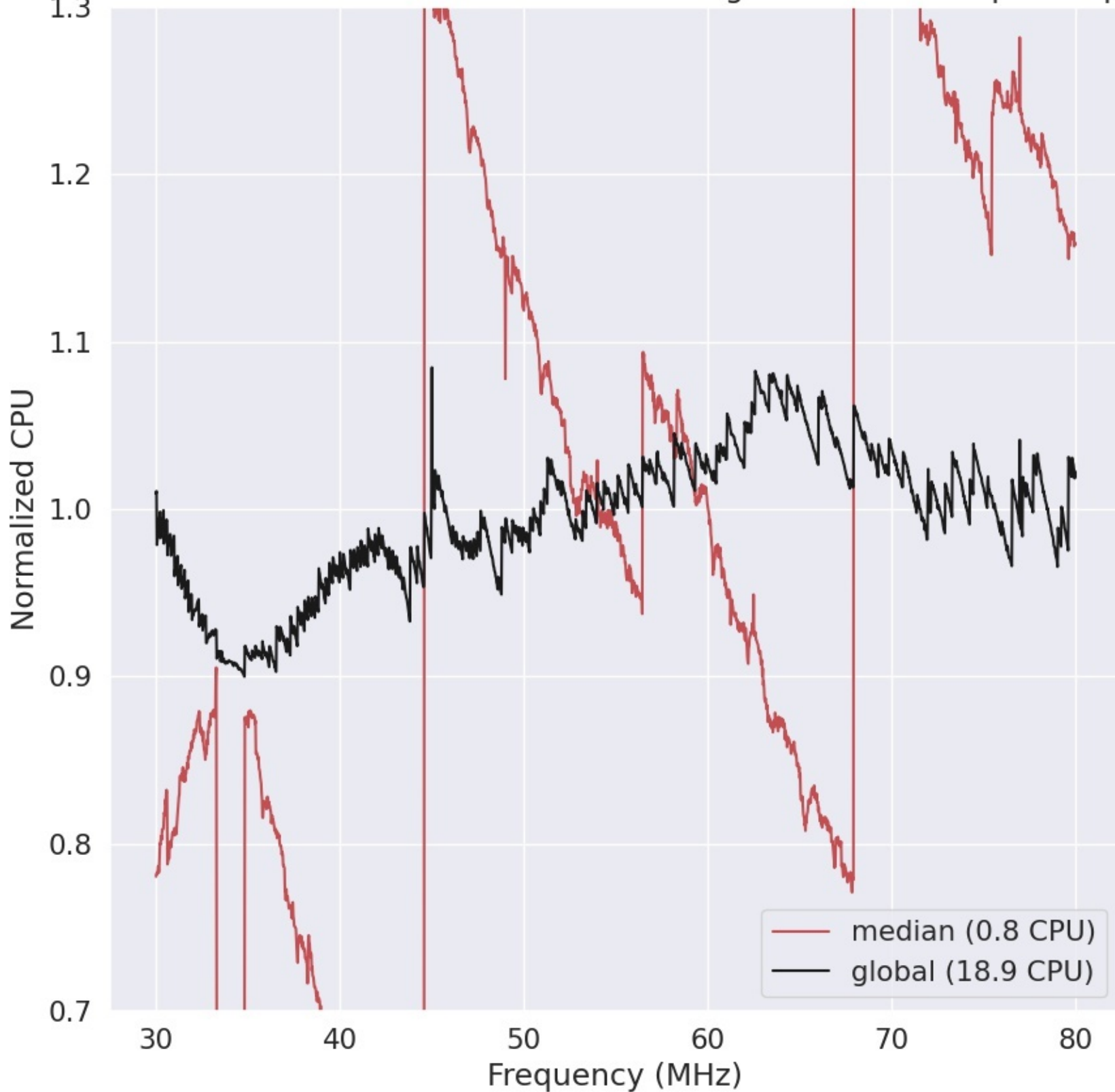
LWA244 - Correlator# 338 - YY - FLAGS:HighTimeVar+BadSpecShape
