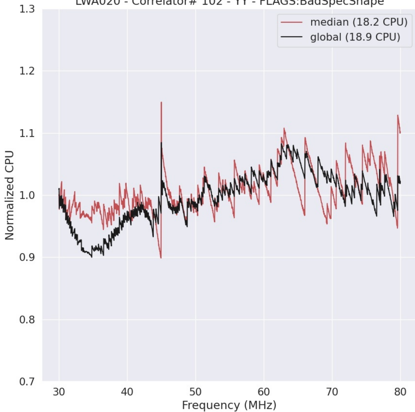
LWA020 - Correlator# 102 - YY - FLAGS:BadSpecShape
