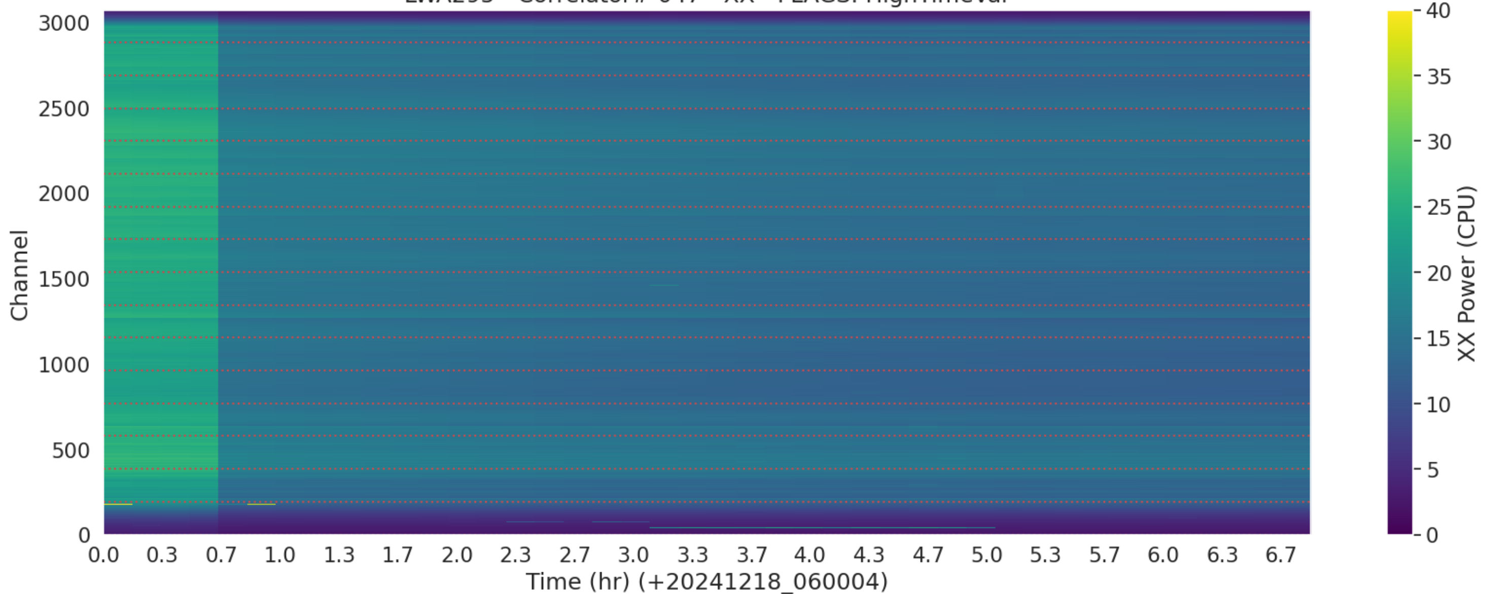
LWA295 - Correlator# 047 - XX - FLAGS: HighTimeVar
