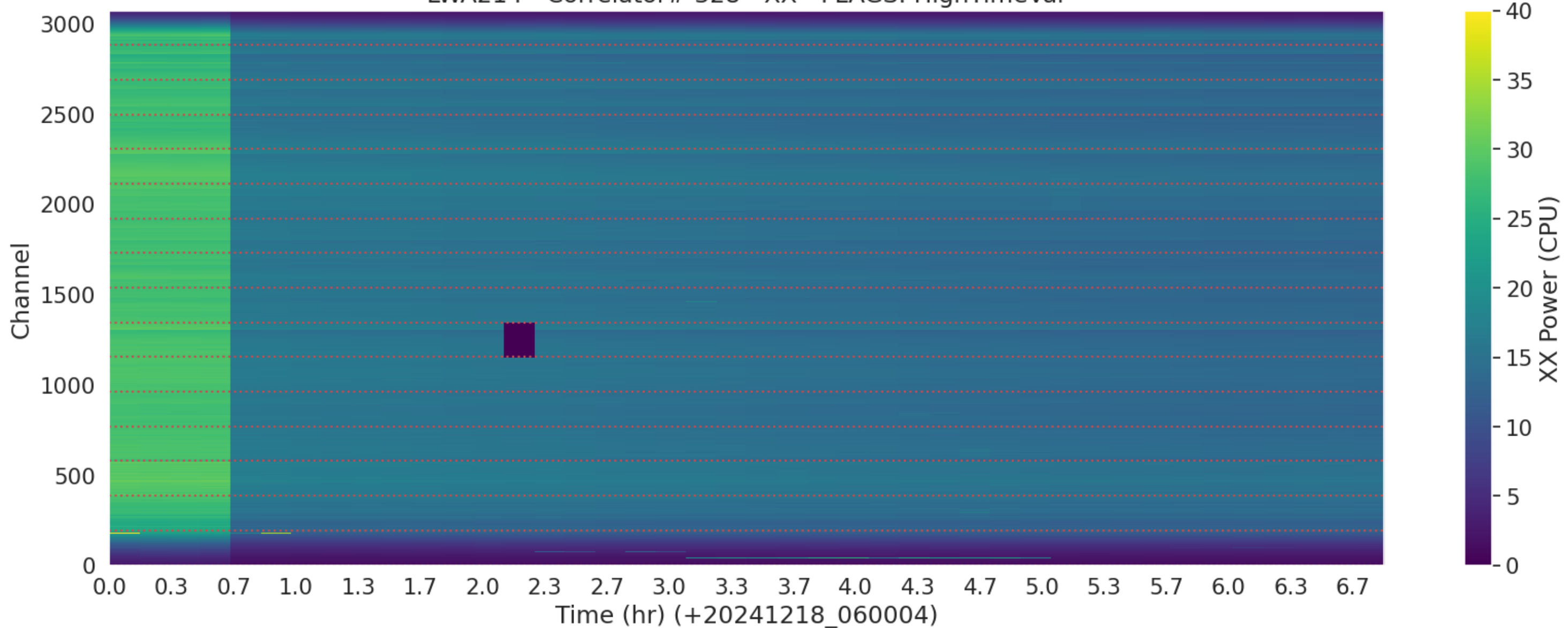
LWA214 - Correlator# 328 - XX - FLAGS: HighTimeVar
