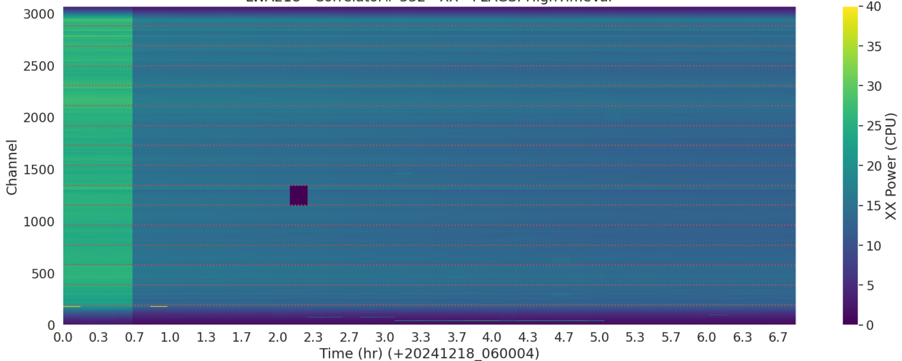
LWA218 - Correlator# 332 - XX - FLAGS: HighTimeVar
