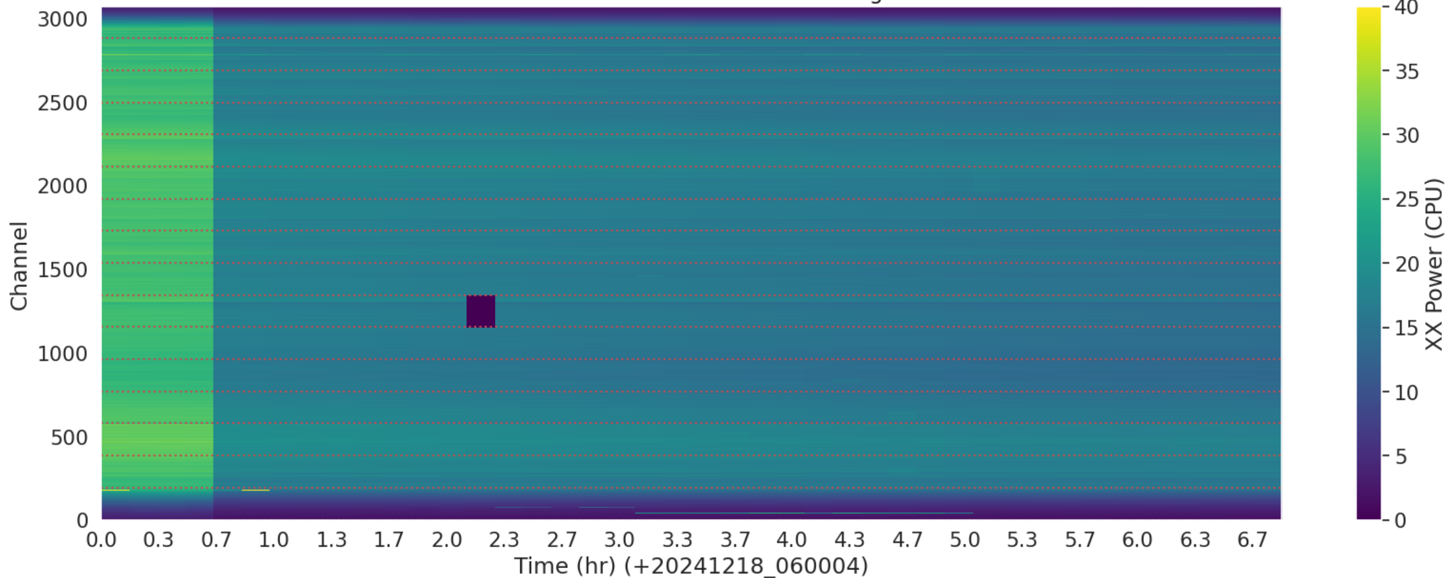
LWA178 - Correlator# 221 - XX - FLAGS: HighTimeVar
