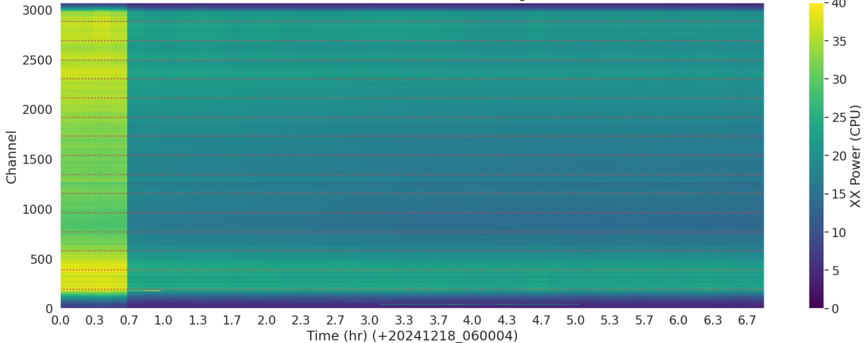
LWA286 - Correlator# 093 - XX - FLAGS: HighTimeVar
