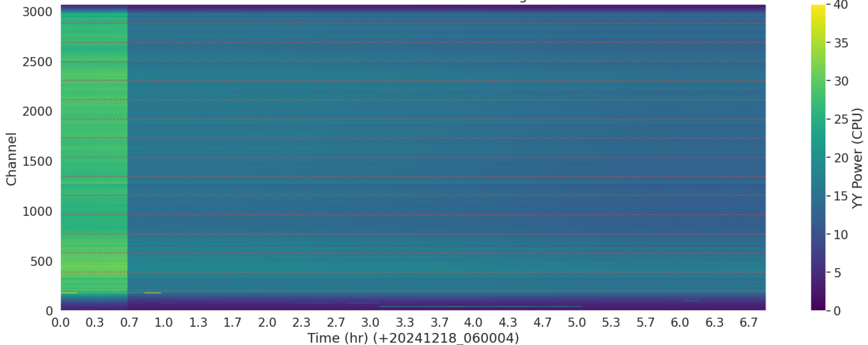
LWA352 - Correlator# 028 - YY - FLAGS: HighTimeVar
