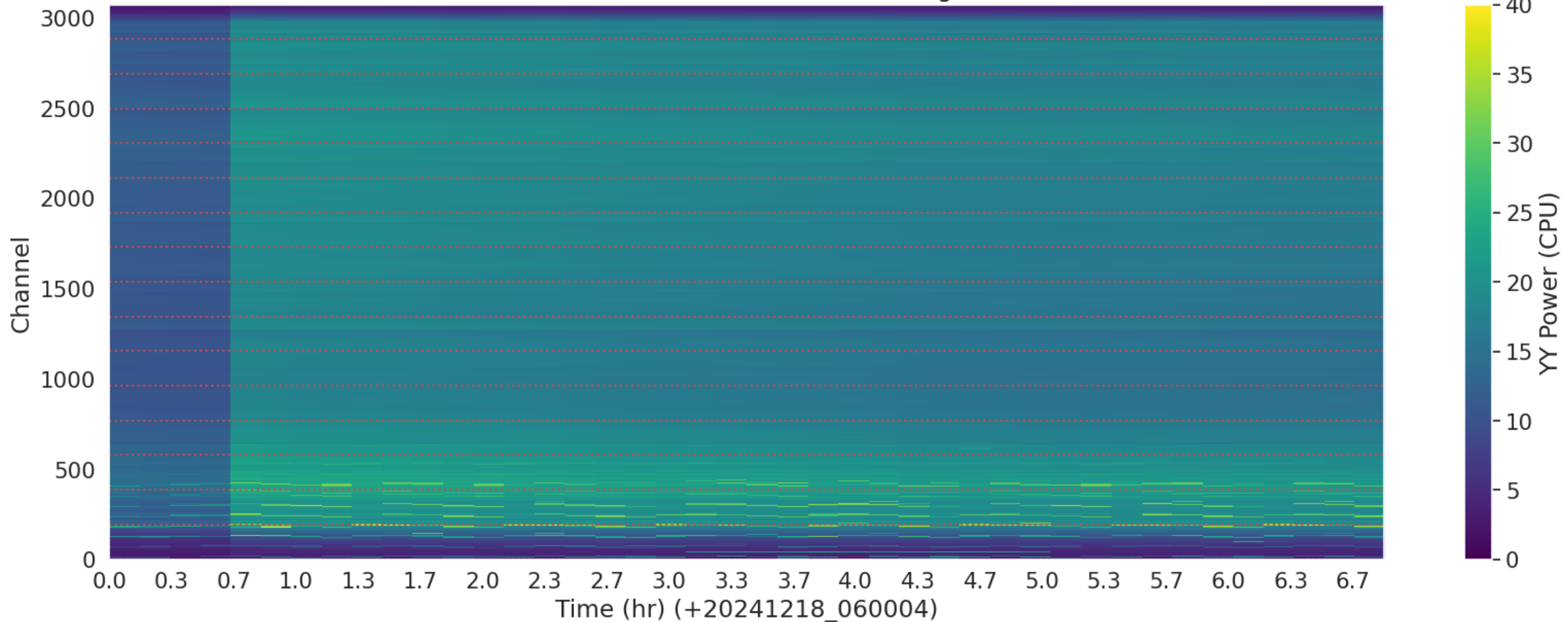
LWA319 - Correlator# 190 - YY - FLAGS: HighTimeVar
