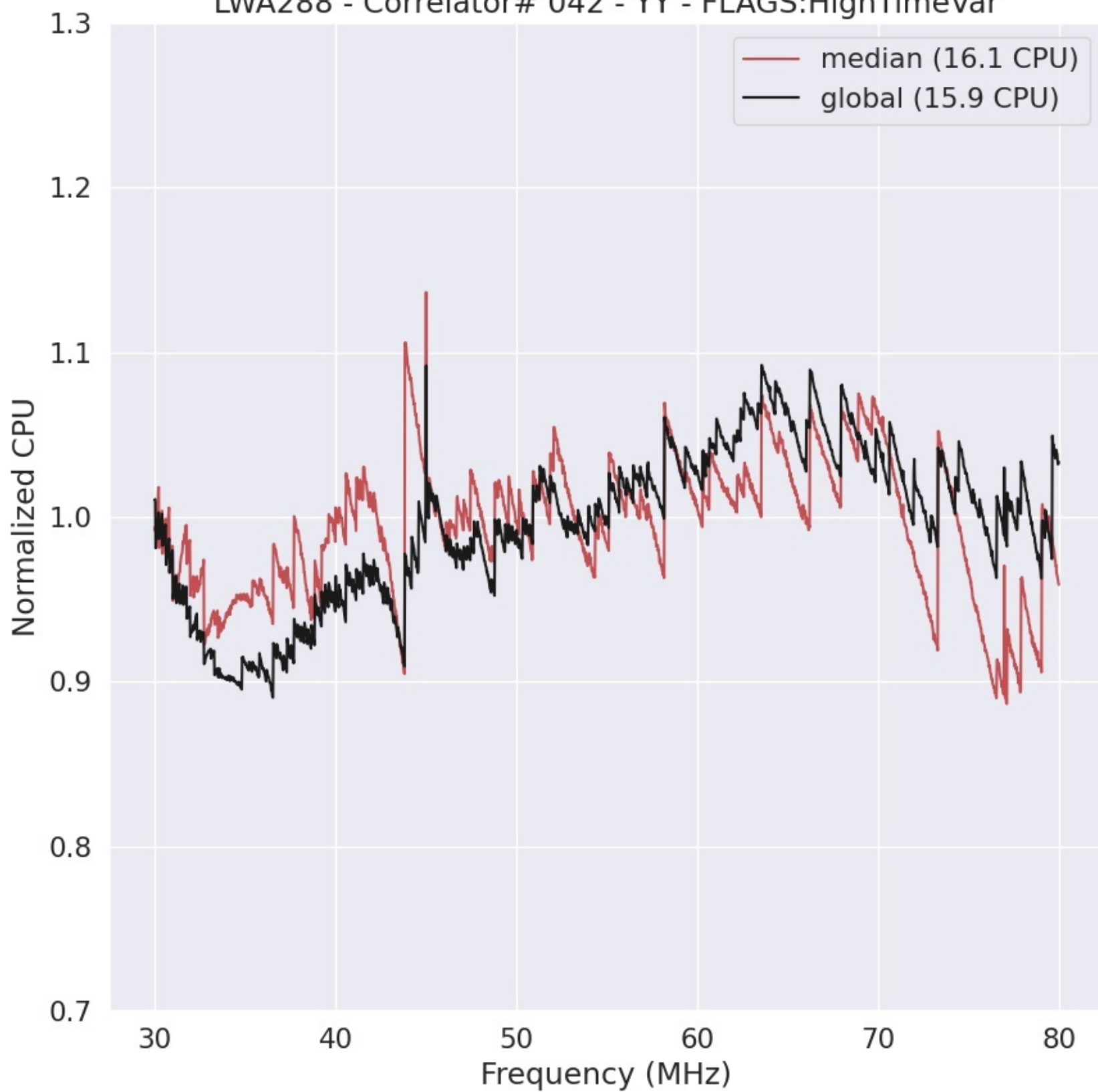
LWA288 - Correlator# 042 - YY - FLAGS:HighTimeVar
