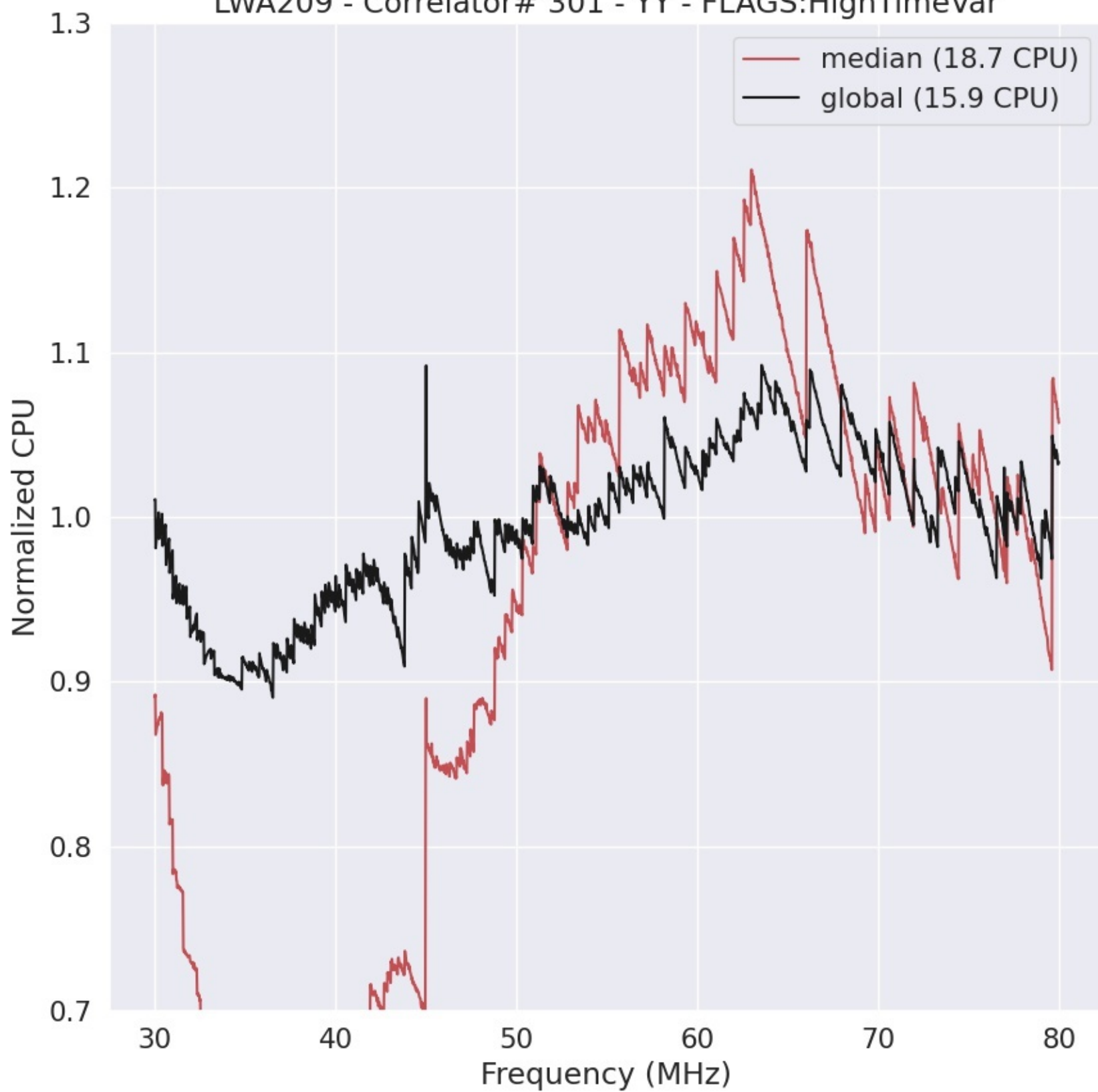
LWA209 - Correlator# 301 - YY - FLAGS:HighTimeVar
