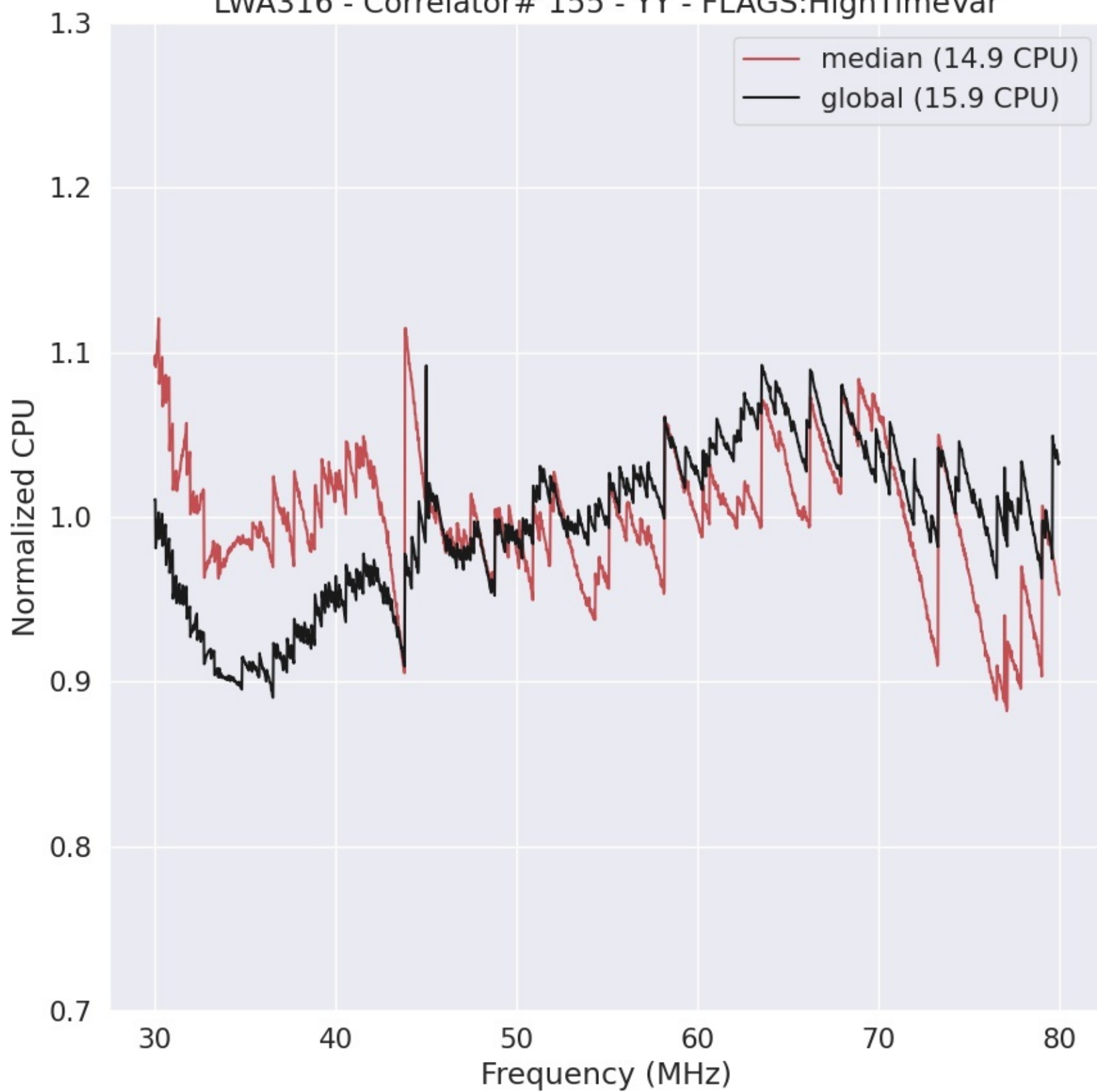
LWA316 - Correlator# 155 - YY - FLAGS:HighTimeVar
