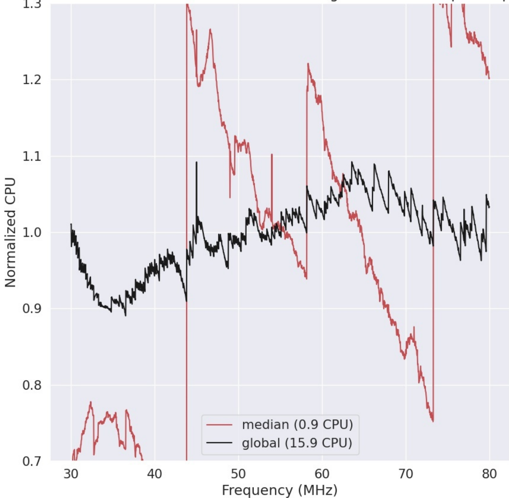
LWA280 - Correlator# 041 - YY - FLAGS:HighTimeVar+BadSpecShape
