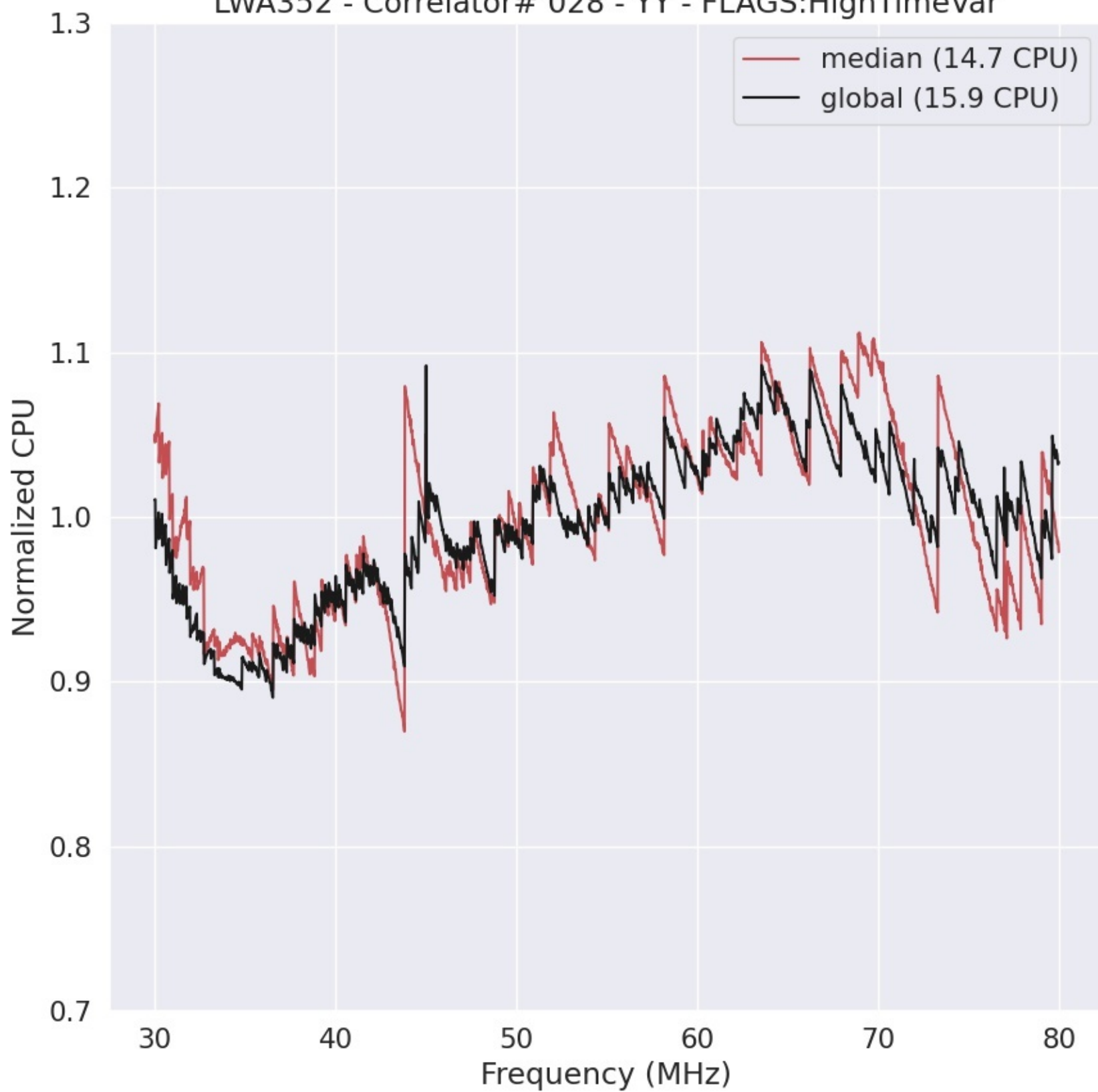
LWA352 - Correlator# 028 - YY - FLAGS:HighTimeVar
